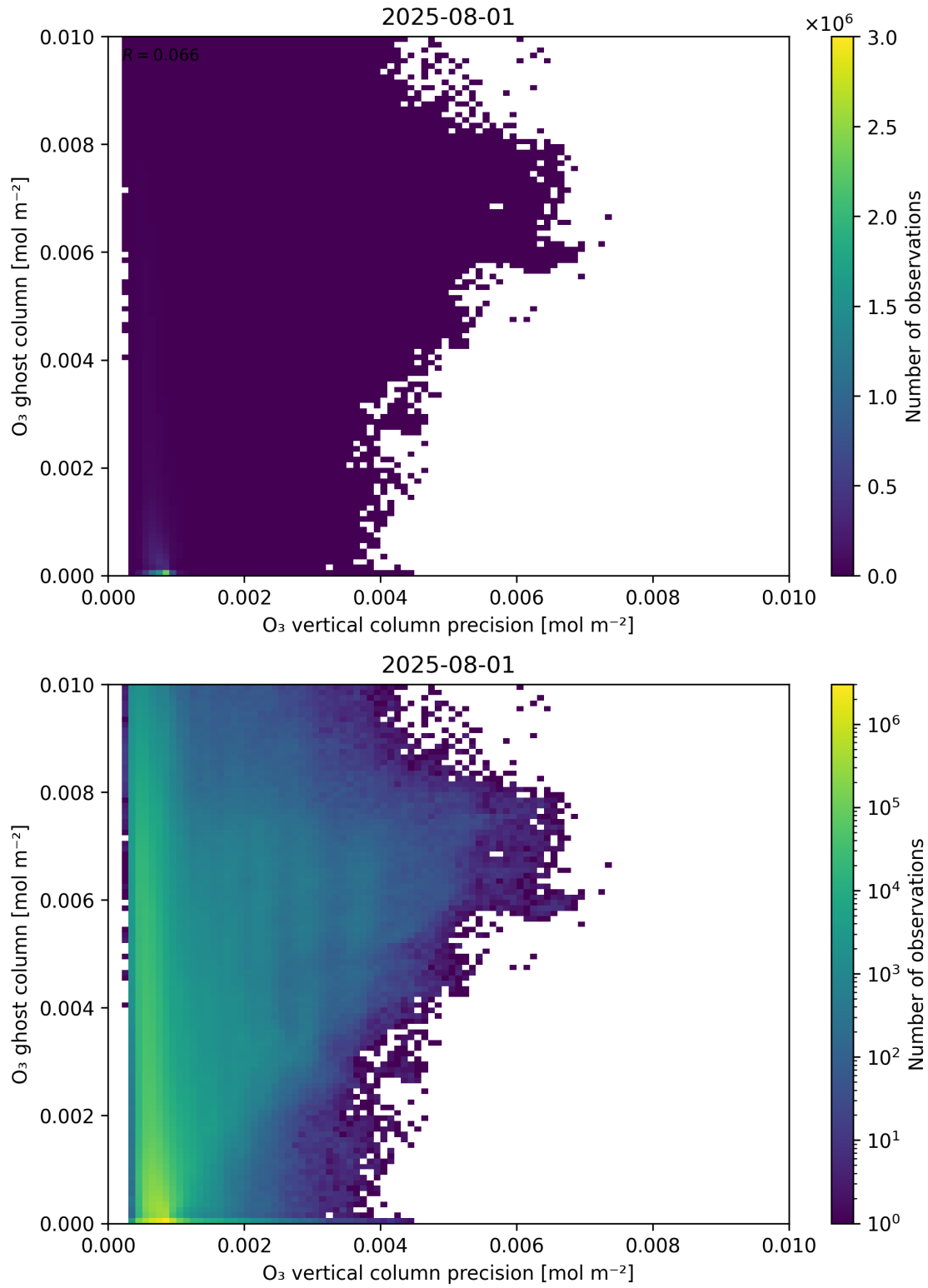
Figure 43: Scatter density plot of “ \text{O}_3 vertical column precision” against “ \text{O}_3 ghost column” for 2025-07-31 to 2025-08-02.
