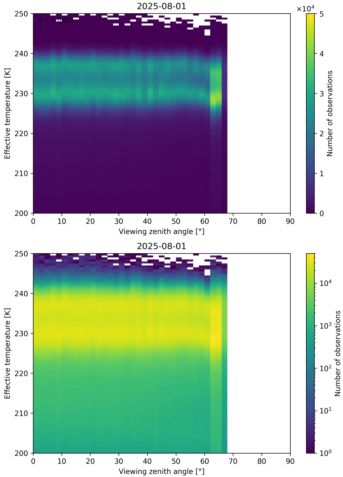
Figure 50: Scatter density plot of “Viewing zenith angle” against “Effective temperature” for 2025-07-31 to 2025-08-02.
