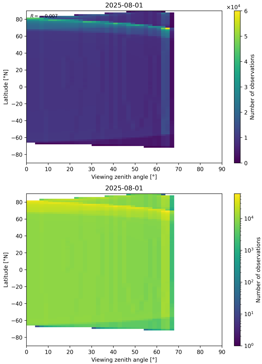
Figure 49: Scatter density plot of “Viewing zenith angle” against “Latitude” for 2025-07-31 to 2025-08-02.
