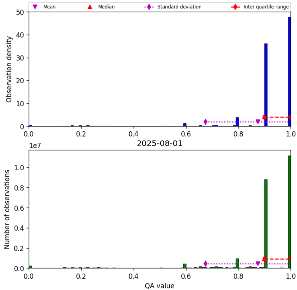
Figure 20: Histogram of “QA value” for 2025-07-31 to 2025-08-02
