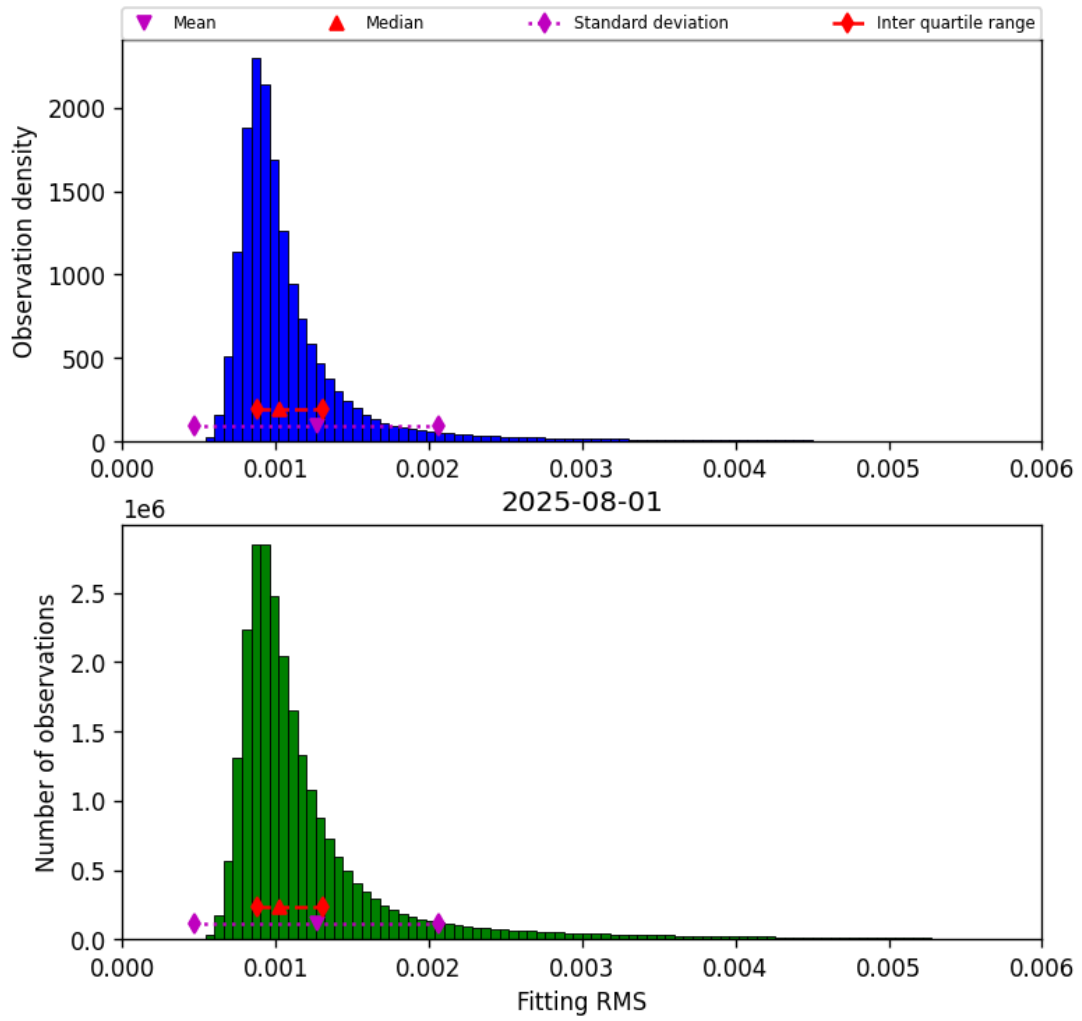
Figure 23: Histogram of “Fitting RMS” for 2025-07-31 to 2025-08-02
