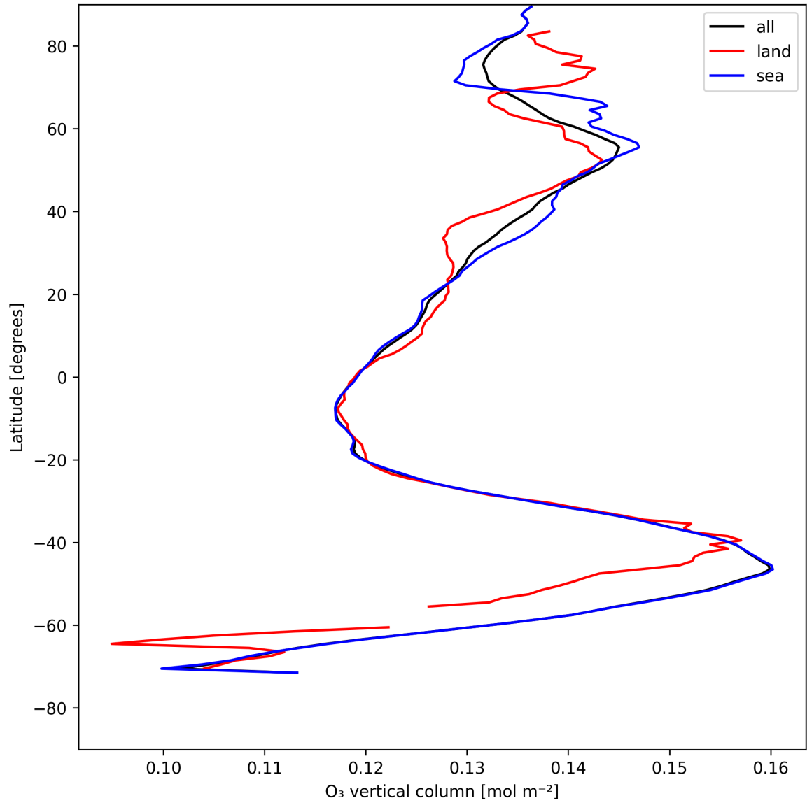
Figure 14: Zonal average of “O 3 vertical column” for 2025-07-31 to 2025-08-02.
