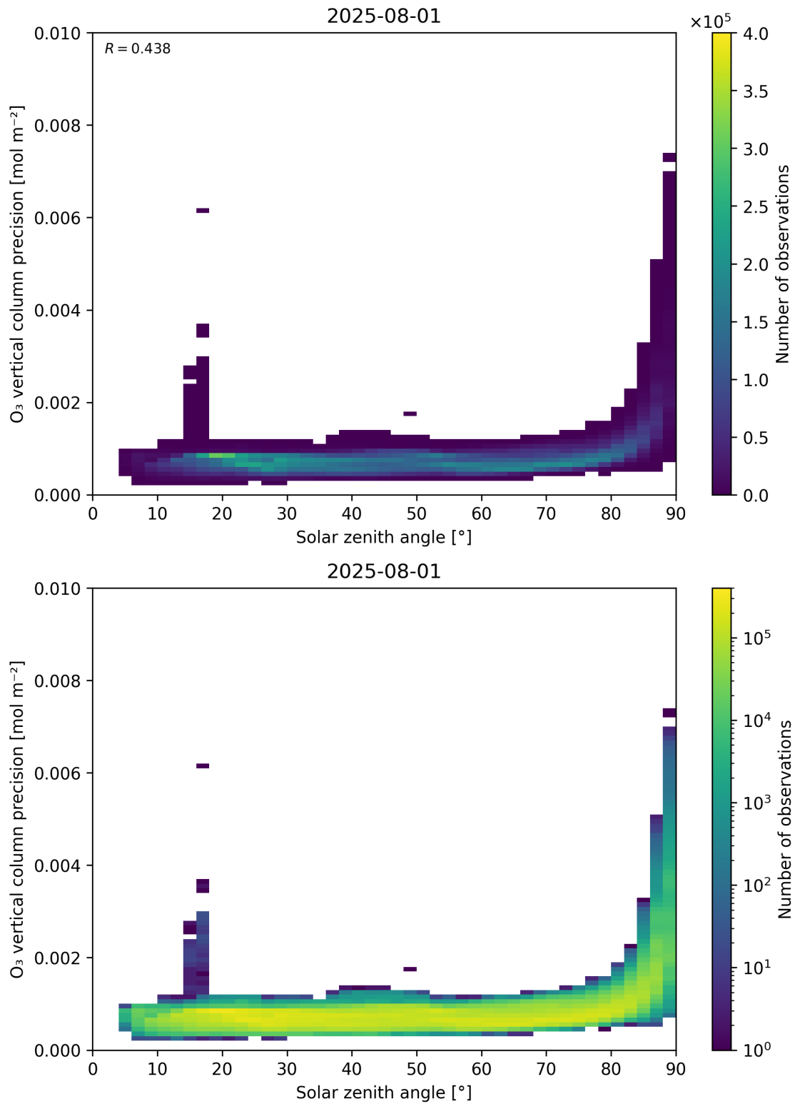
Figure 48: Scatter density plot of “Solar zenith angle” against “O 3 vertical column precision” for 2025-07-31 to 2025-08-02.
