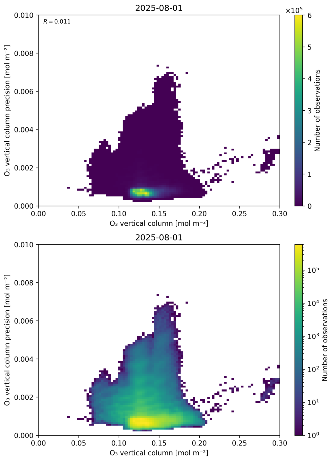
Figure 41: Scatter density plot of “O 3 vertical column” against “O 3 vertical column precision” for 2025-07-31 to 2025-08-02.
