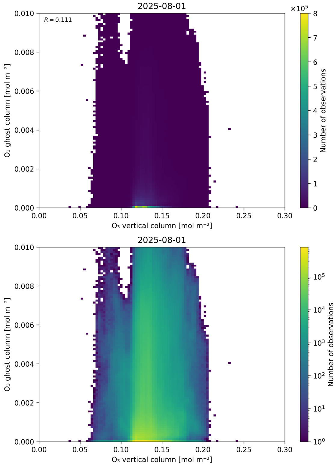
Figure 40: Scatter density plot of “O 3 vertical column” against “O 3 ghost column” for 2025-07-31 to 2025-08-02.
