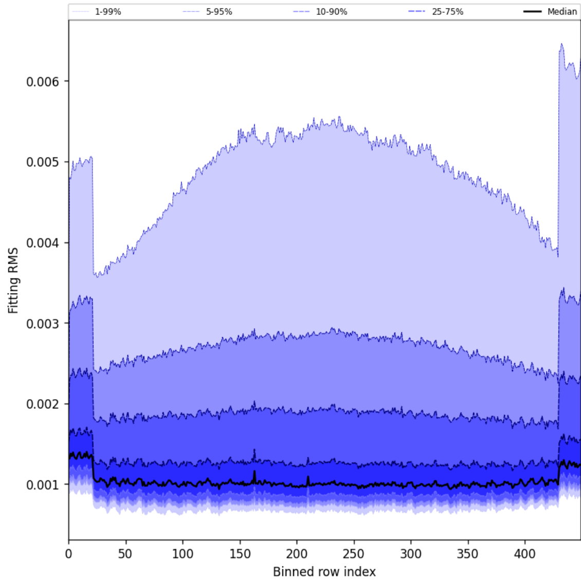
Figure 30: Along track statistics of “Fitting RMS” for 2025-07-31 to 2025-08-02
