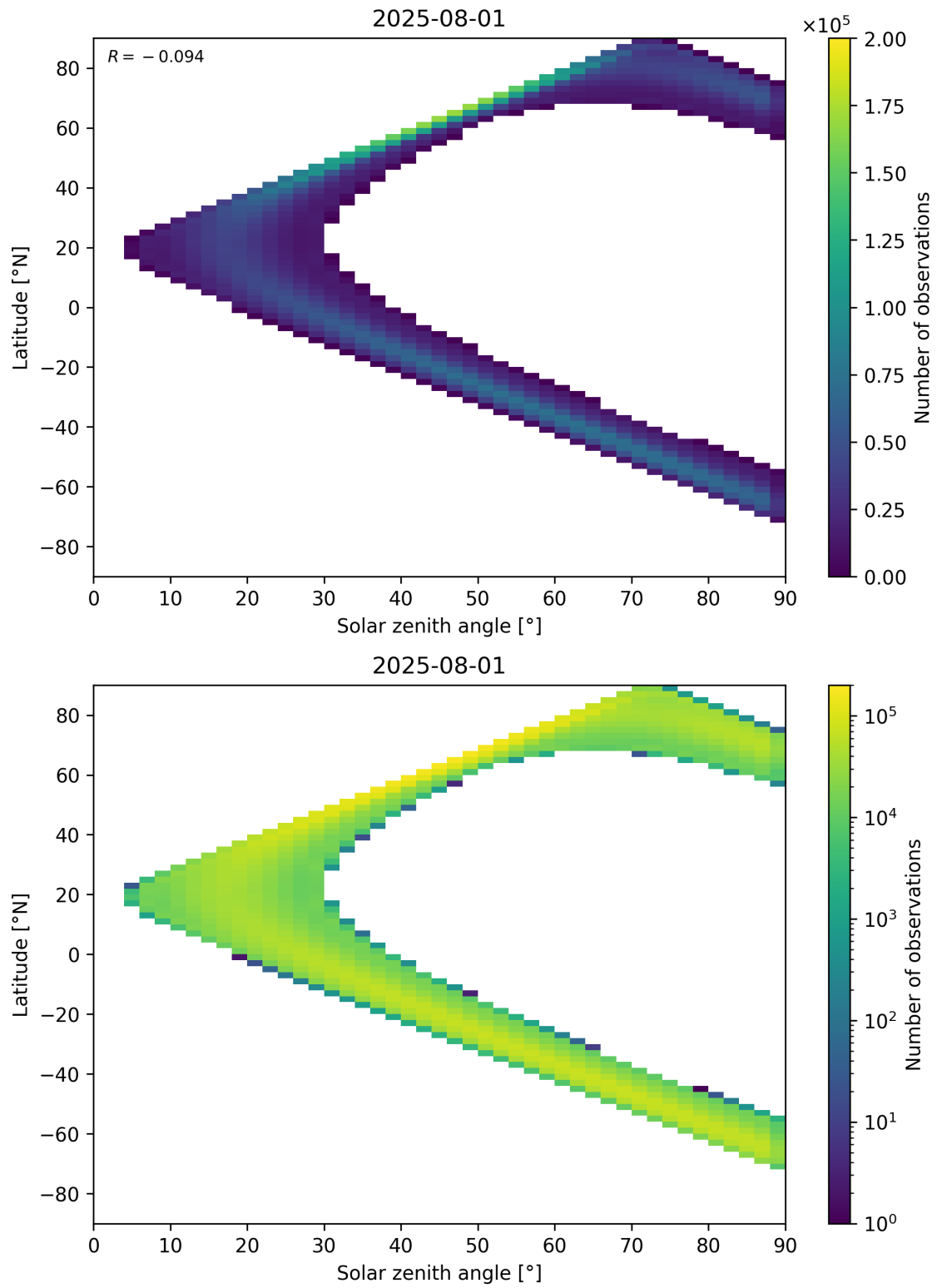
Figure 44: Scatter density plot of “Solar zenith angle” against “Latitude” for 2025-07-31 to 2025-08-02.
