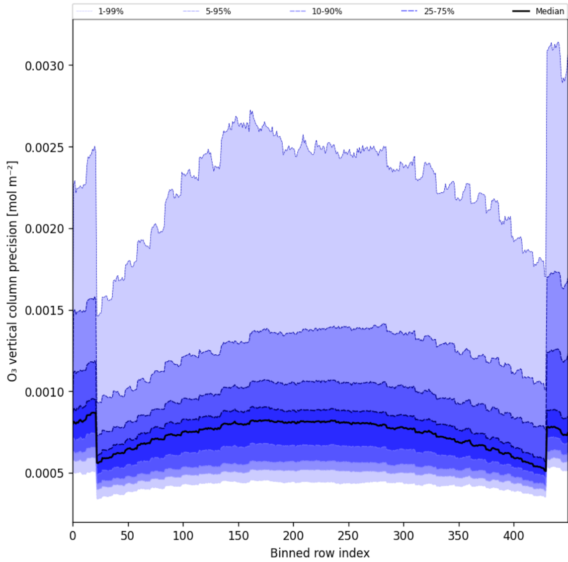
Figure 29: Along track statistics of “O 3 vertical column precision” for 2025-07-31 to 2025-08-02
