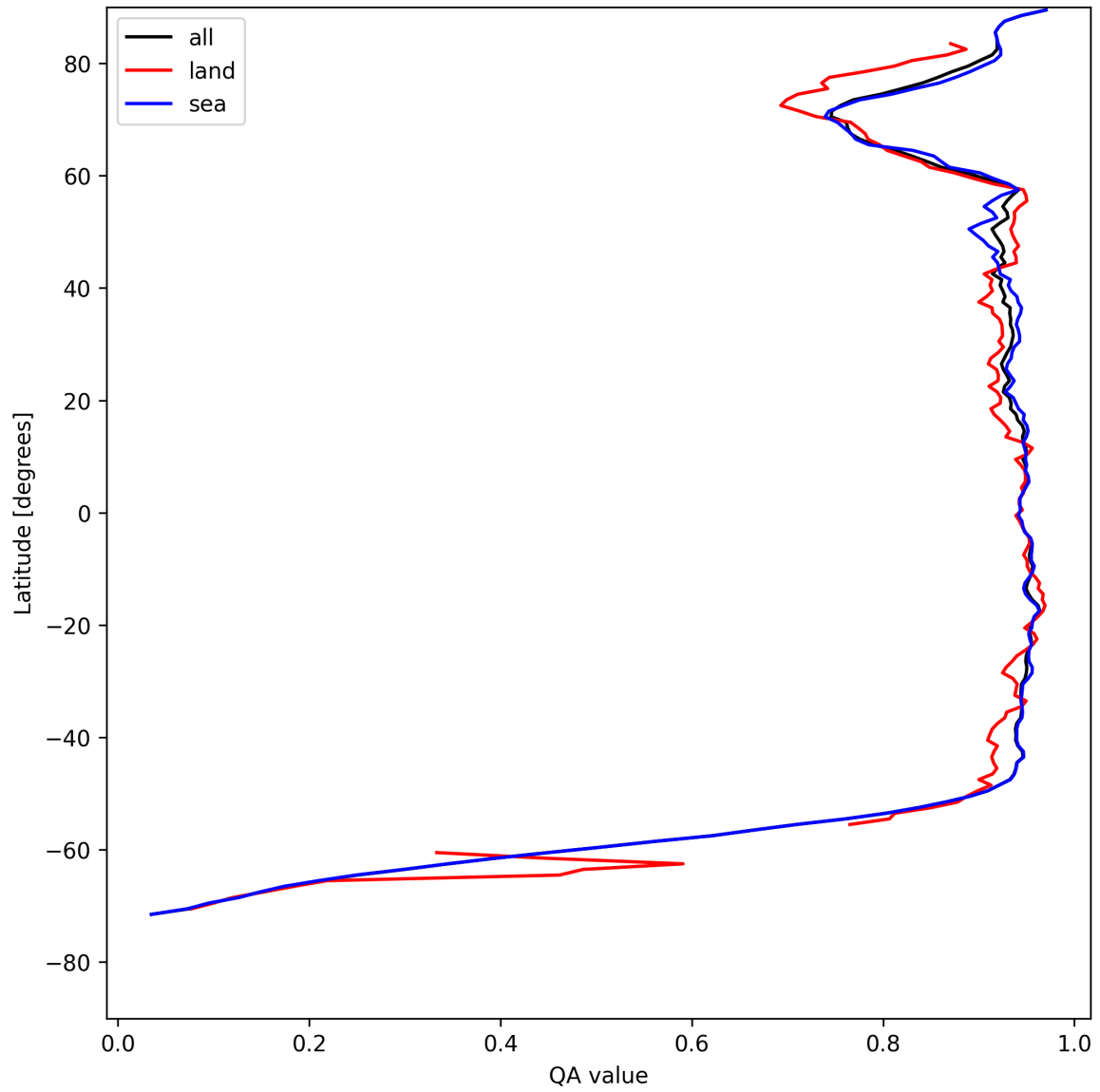
Figure 13: Zonal average of “QA value” for 2025-07-31 to 2025-08-02.
