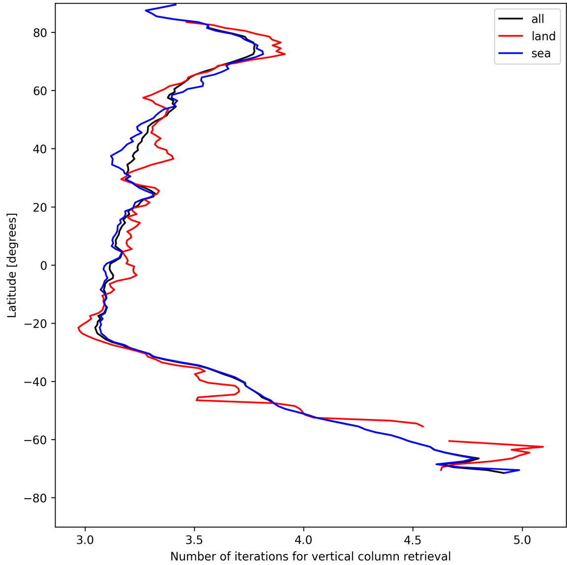
Figure 19: Zonal average of “Number of iterations for vertical column retrieval” for 2025-07-31 to 2025-08-02.
