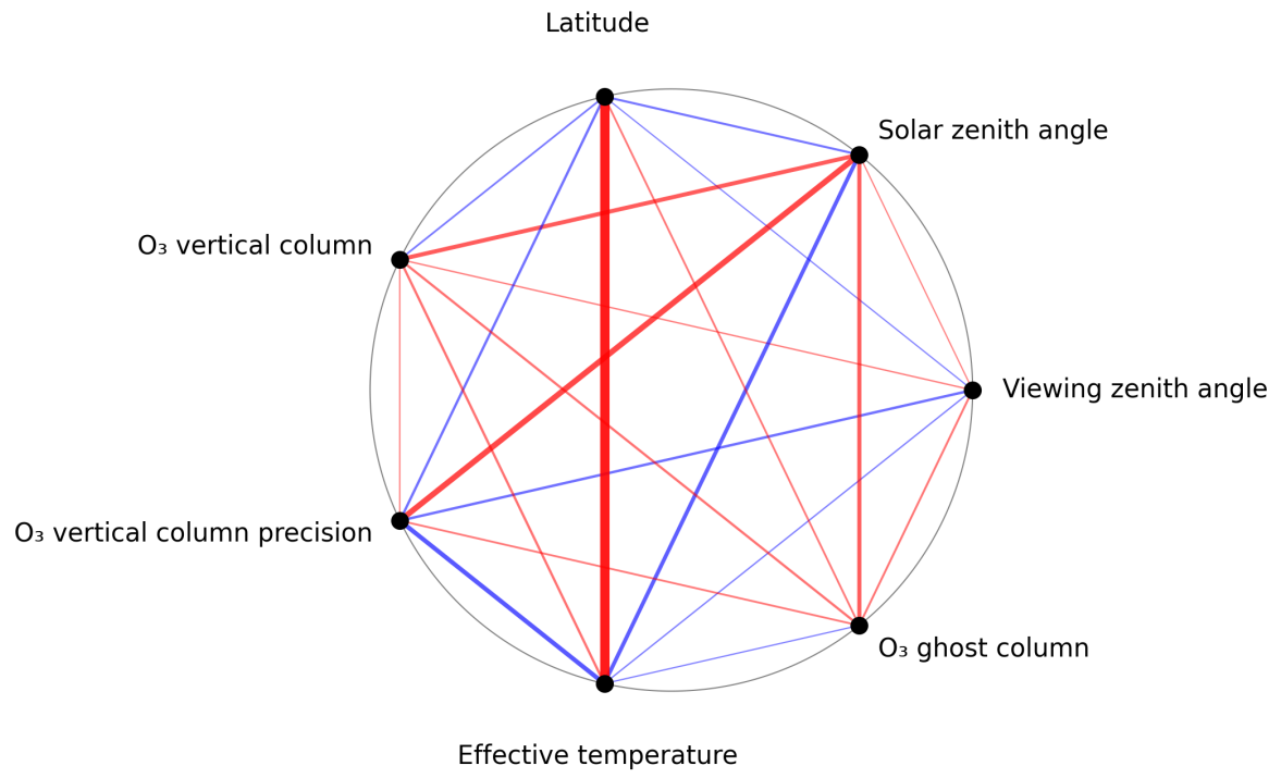
Figure 1: Map of correlation graph for 2025-07-31 to 2025-08-02.
