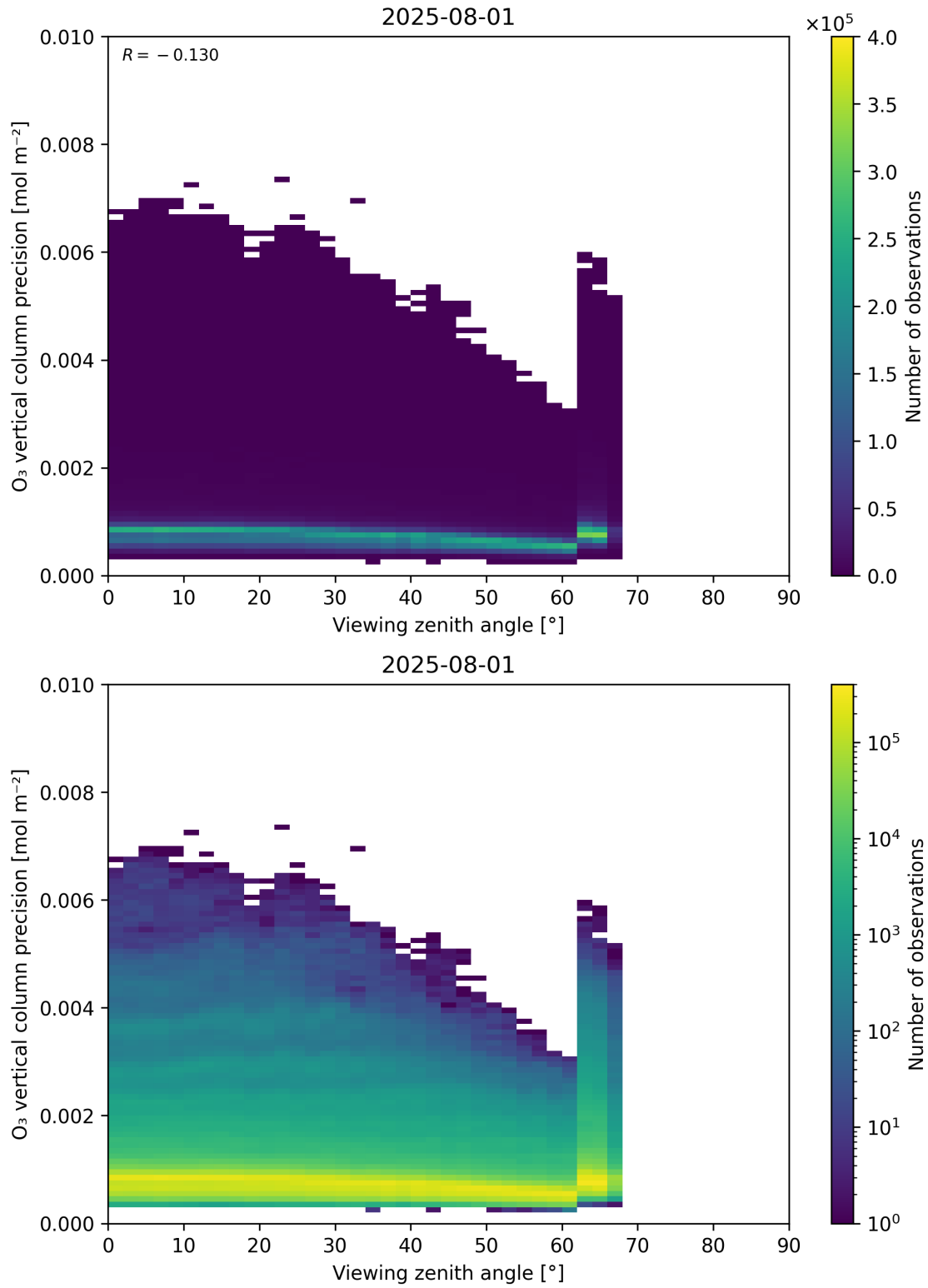
Figure 53: Scatter density plot of “Viewing zenith angle” against “O 3 vertical column precision” for 2025-07-31 to 2025-08-02.
