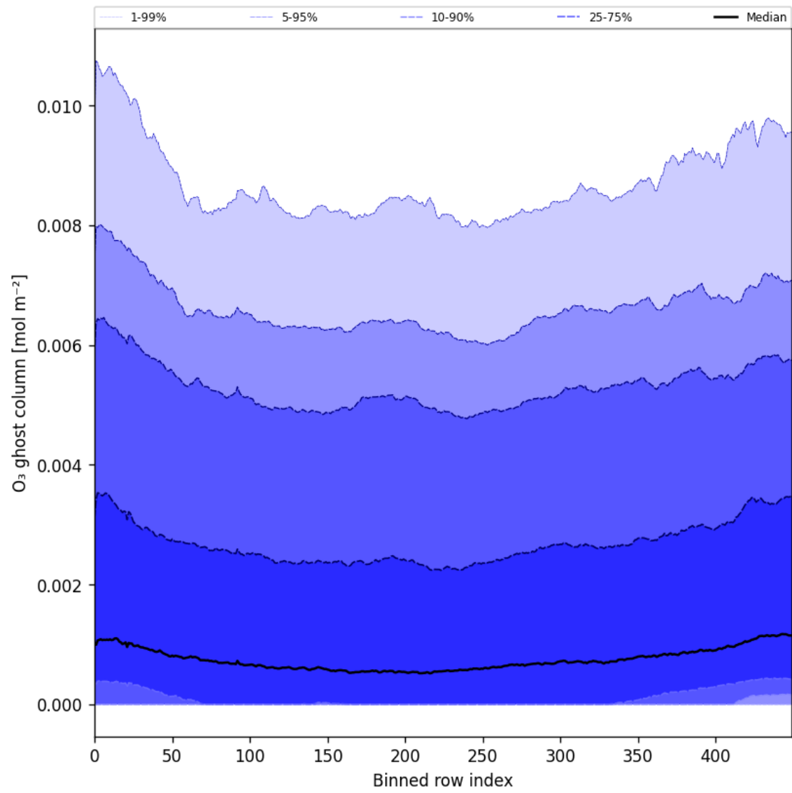
Figure 32: Along track statistics of “O 3 ghost column” for 2025-07-31 to 2025-08-02
