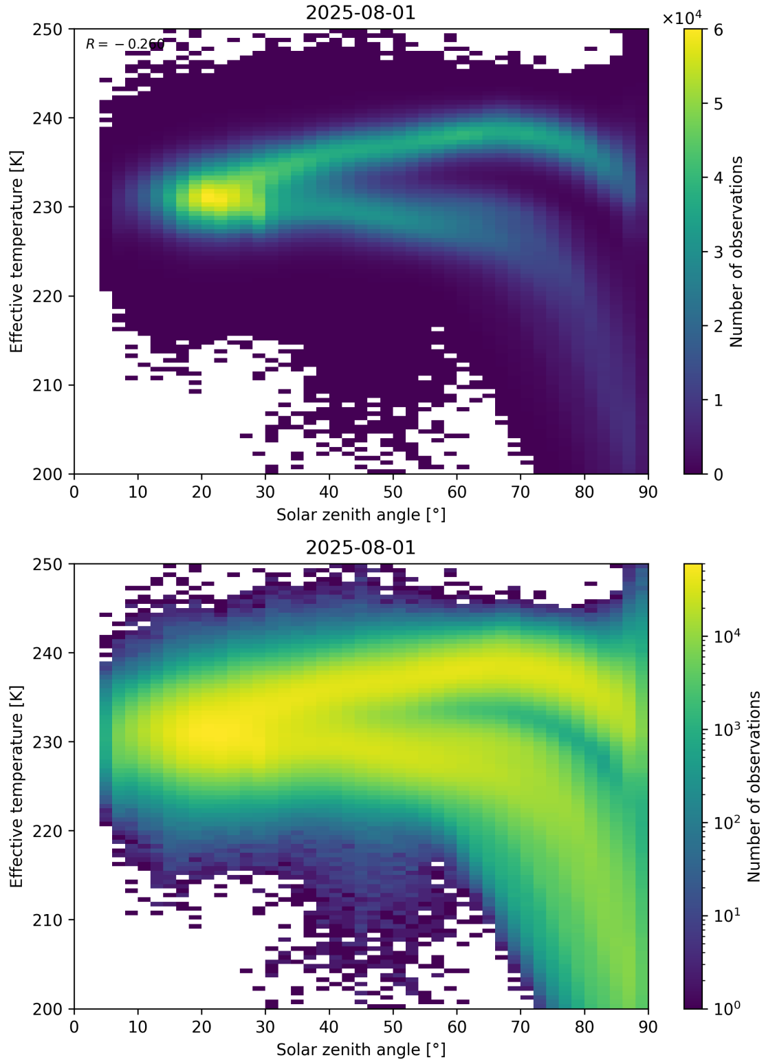
Figure 45: Scatter density plot of “Solar zenith angle” against “Effective temperature” for 2025-07-31 to 2025-08-02.
