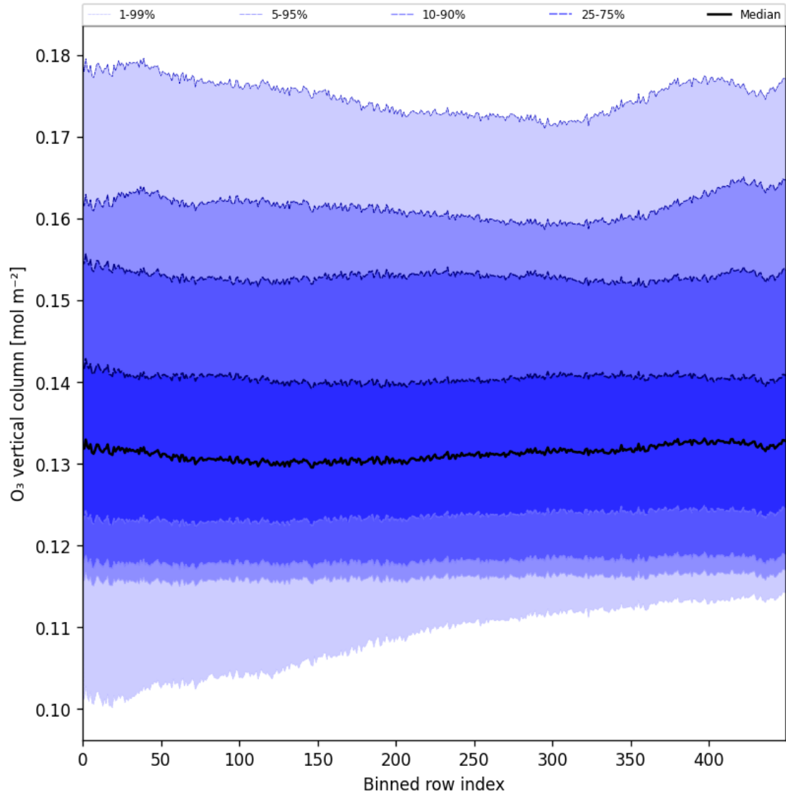
Figure 28: Along track statistics of “O 3 vertical column” for 2025-07-31 to 2025-08-02
