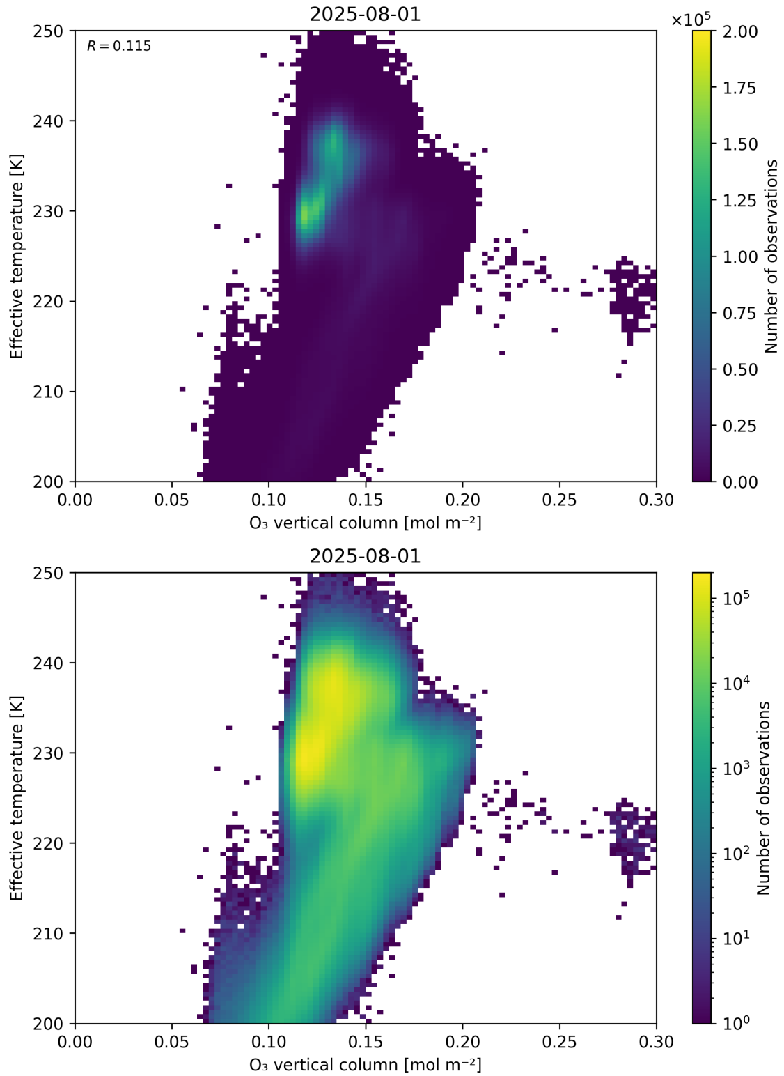
Figure 39: Scatter density plot of “O 3 vertical column” against “Effective temperature” for 2025-07-31 to 2025-08-02.
