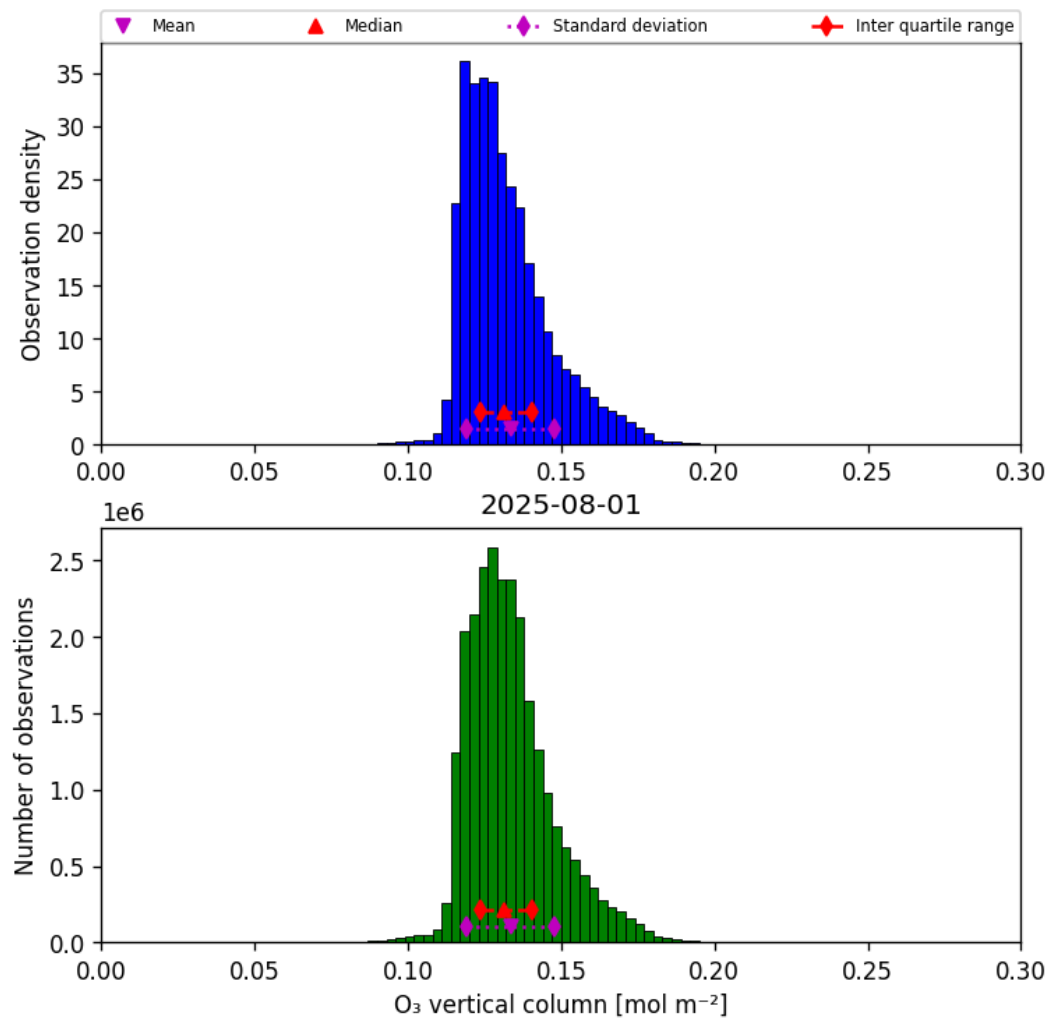
Figure 21: Histogram of “O 3 vertical column” for 2025-07-31 to 2025-08-02
