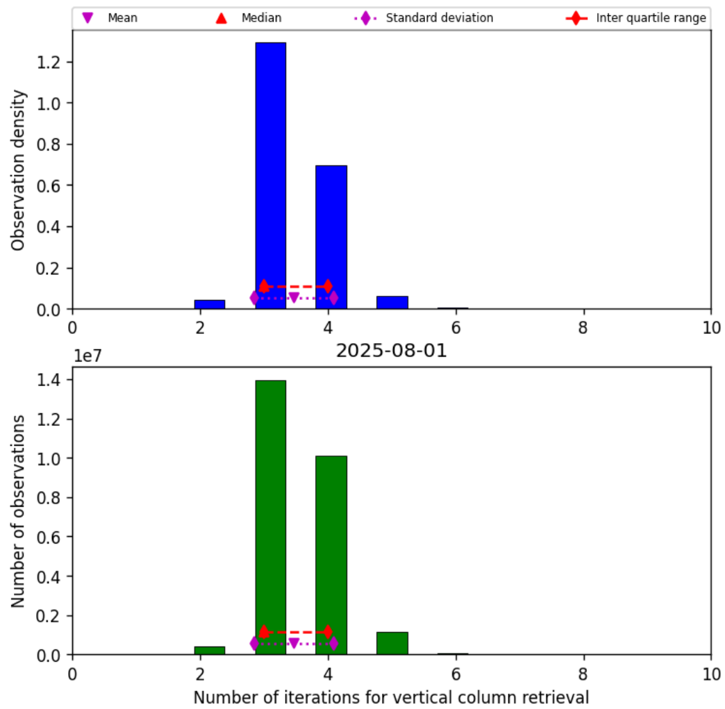
Figure 26: Histogram of “Number of iterations for vertical column retrieval” for 2025-07-31 to 2025-08-02
