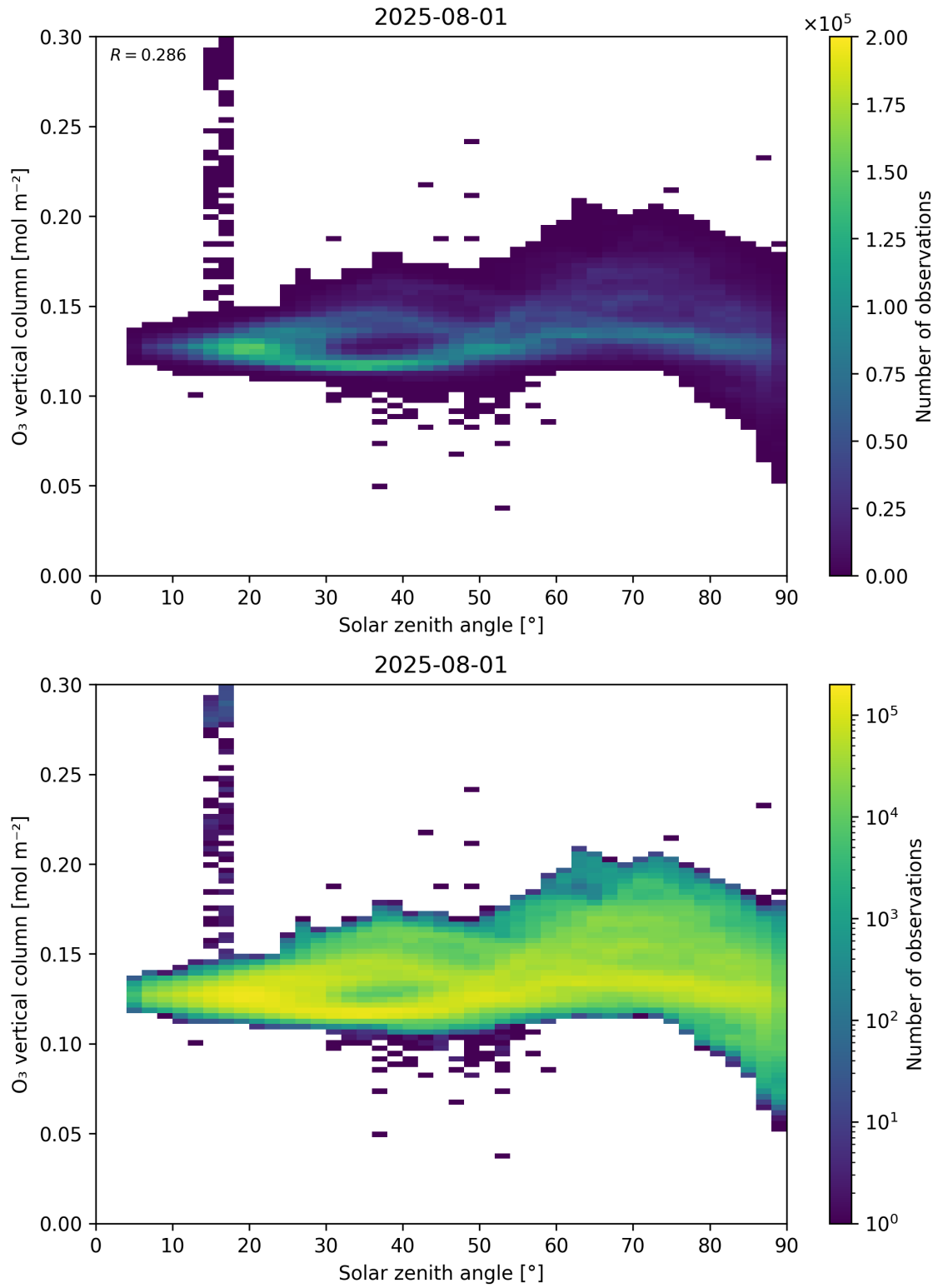
Figure 47: Scatter density plot of “Solar zenith angle” against “O 3 vertical column” for 2025-07-31 to 2025-08-02.
