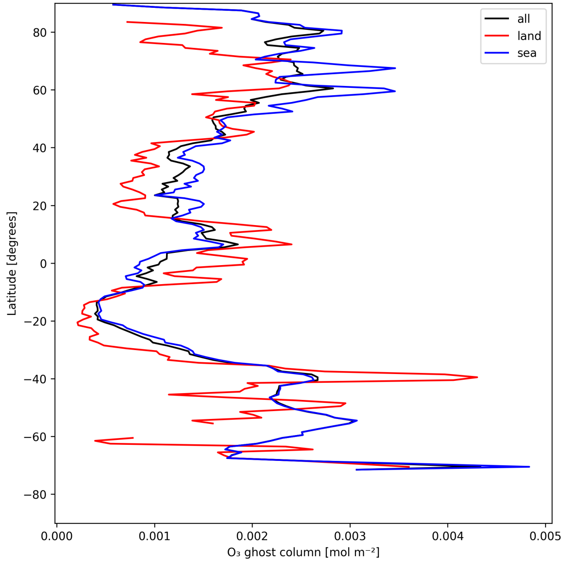
Figure 18: Zonal average of "O 3 ghost column" for 2025-07-31 to 2025-08-02.
