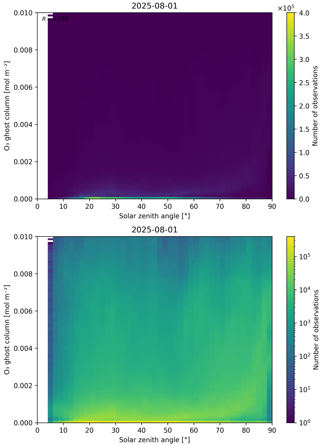
Figure 46: Scatter density plot of “Solar zenith angle” against “O 3 ghost column” for 2025-07-31 to 2025-08-02.
