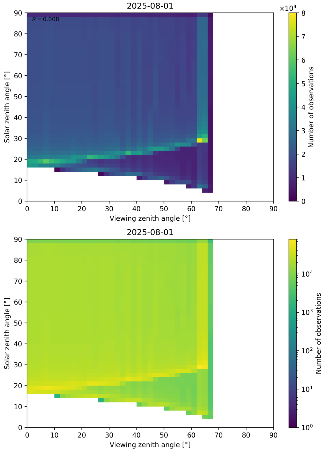
Figure 54: Scatter density plot of “Viewing zenith angle” against “Solar zenith angle” for 2025-07-31 to 2025-08-02.
