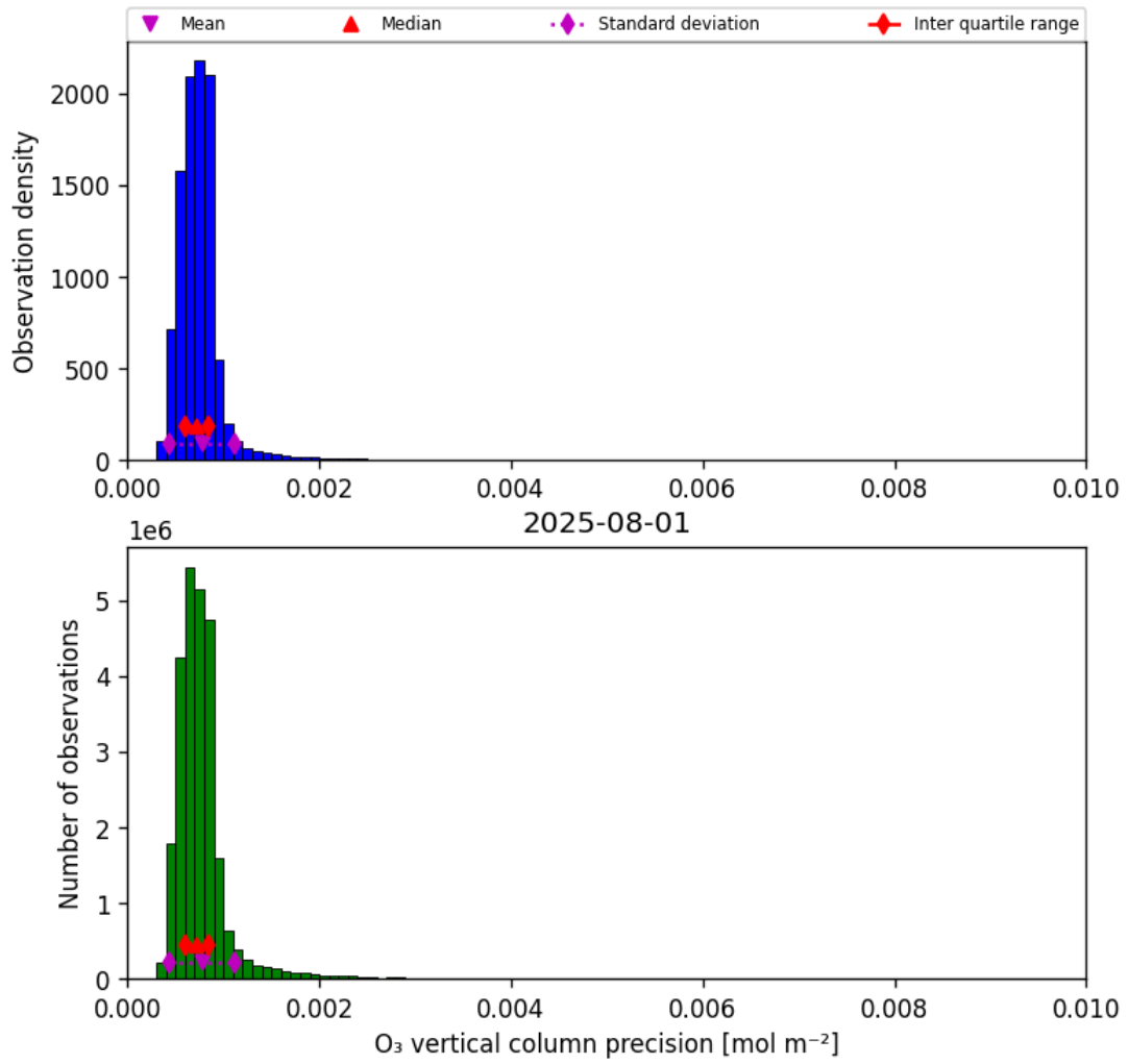
Figure 22: Histogram of “O 3 vertical column precision” for 2025-07-31 to 2025-08-02
