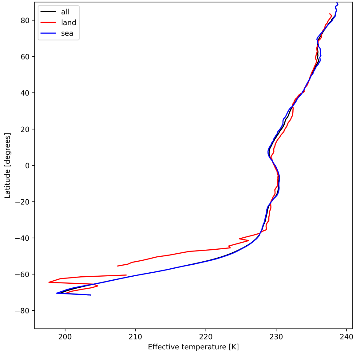
Figure 17: Zonal average of "Effective temperature" for 2025-07-31 to 2025-08-02.
