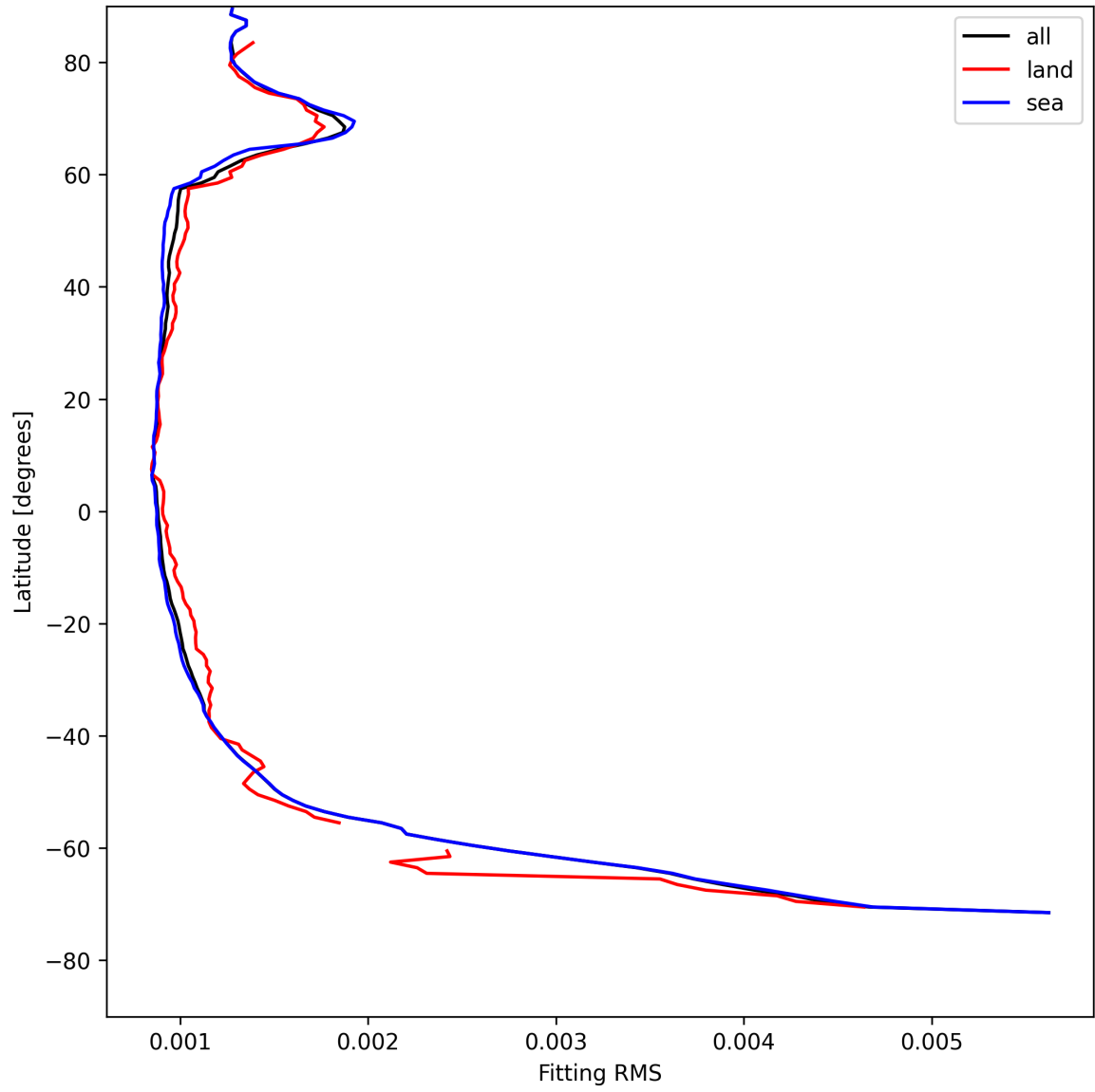
Figure 16: Zonal average of “Fitting RMS” for 2025-07-31 to 2025-08-02.
