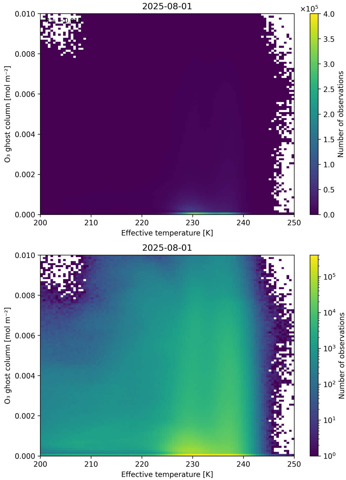
Figure 38: Scatter density plot of “Effective temperature” against “O 3 ghost column” for 2025-07-31 to 2025-08-02.
