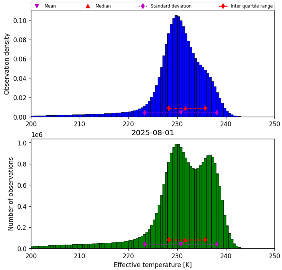
Figure 24: Histogram of “Effective temperature” for 2025-07-31 to 2025-08-02
