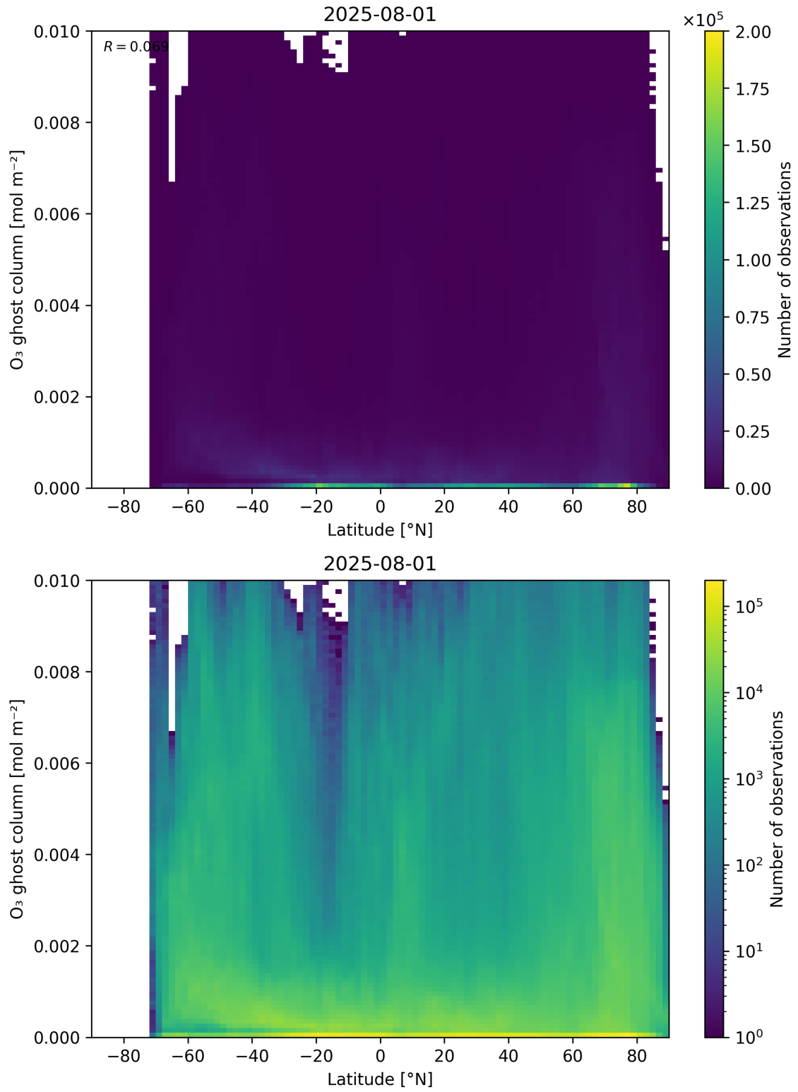
Figure 35: Scatter density plot of “Latitude” against “O 3 ghost column” for 2025-07-31 to 2025-08-02.
