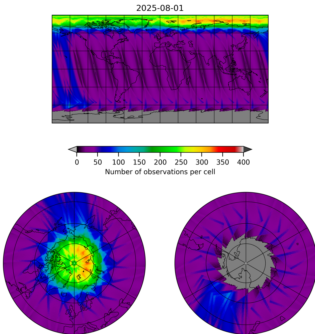
Figure 12: Map of the number of observations for 2025-07-31 to 2025-08-02
