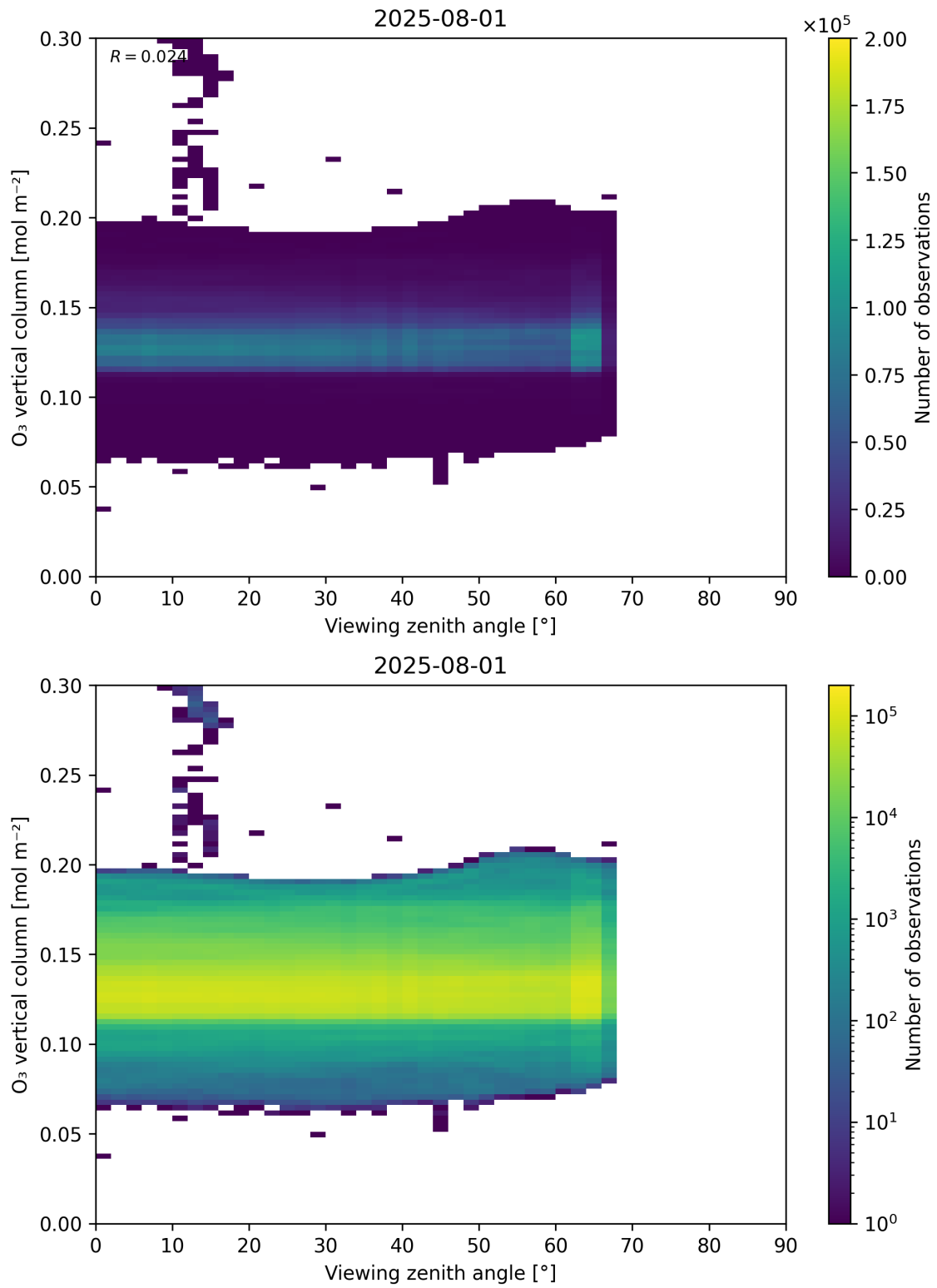
Figure 52: Scatter density plot of “Viewing zenith angle” against “O 3 vertical column” for 2025-07-31 to 2025-08-02.
