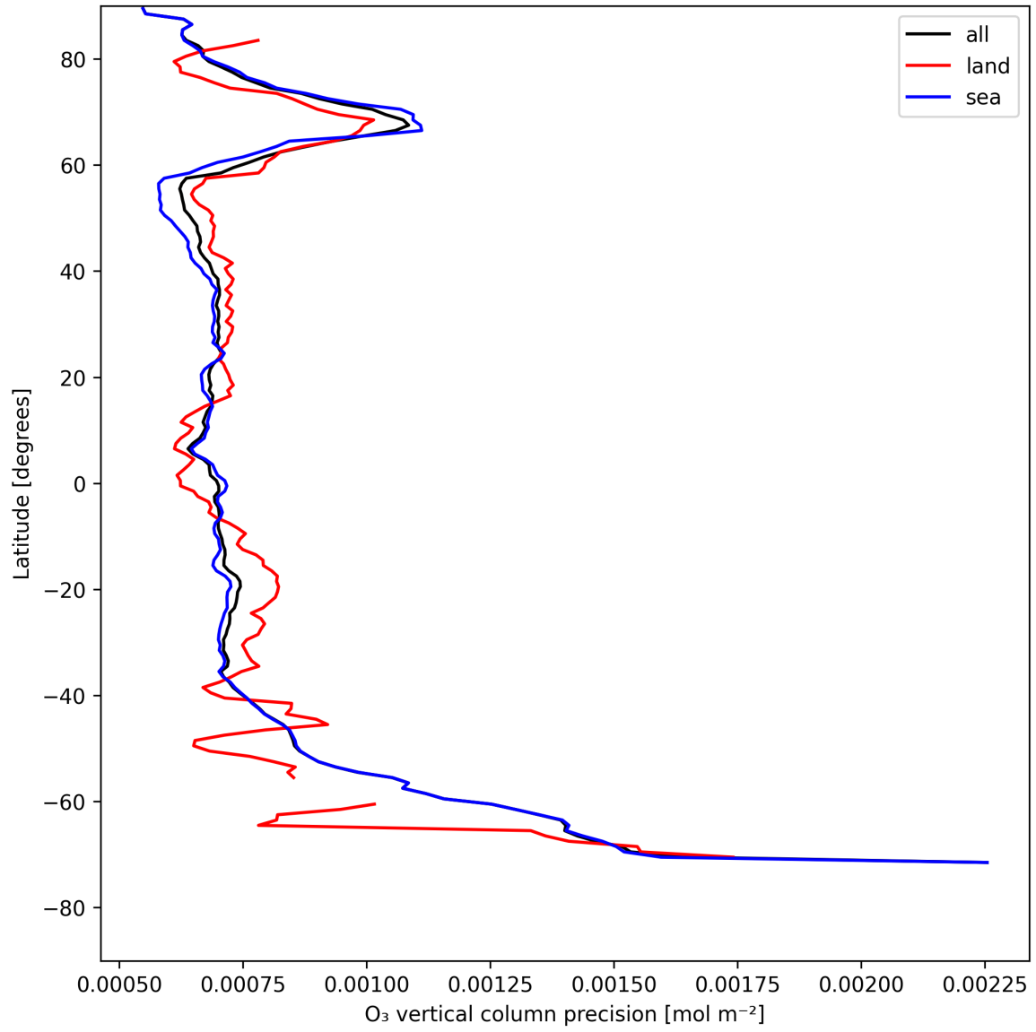
Figure 15: Zonal average of “O 3 vertical column precision” for 2025-07-31 to 2025-08-02.
