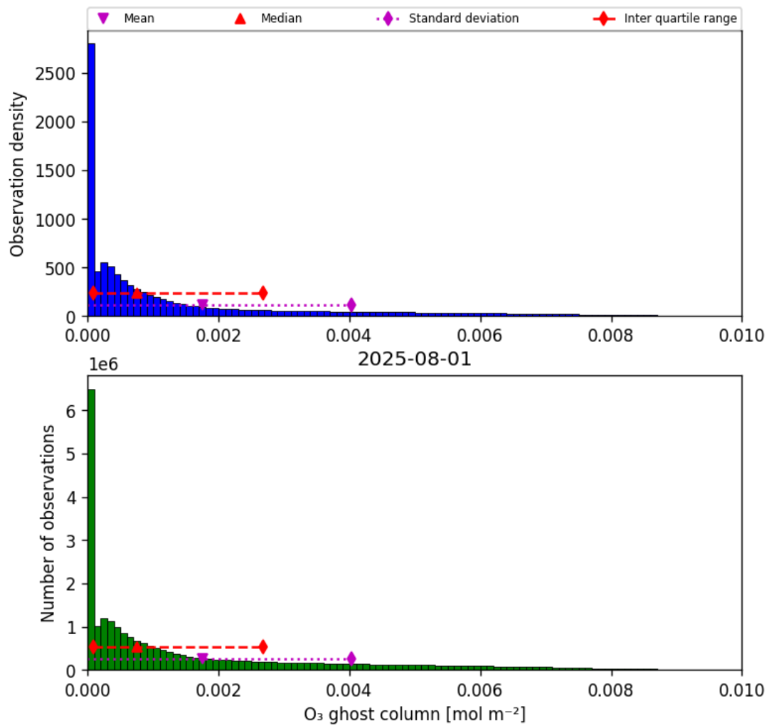
Figure 25: Histogram of “O 3 ghost column” for 2025-07-31 to 2025-08-02
