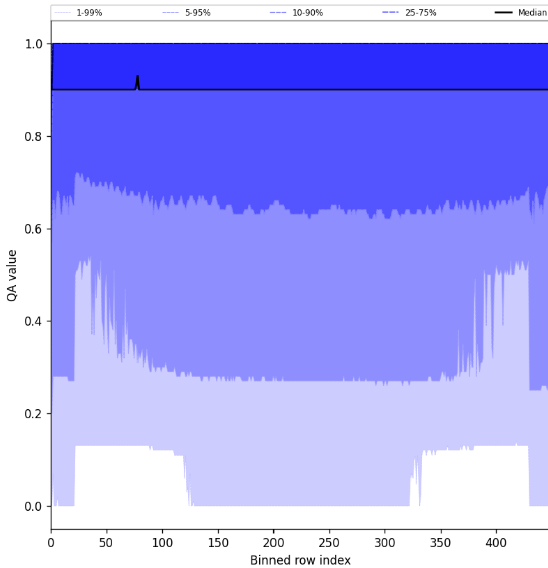
Figure 27: Along track statistics of “QA value” for 2025-07-31 to 2025-08-02
