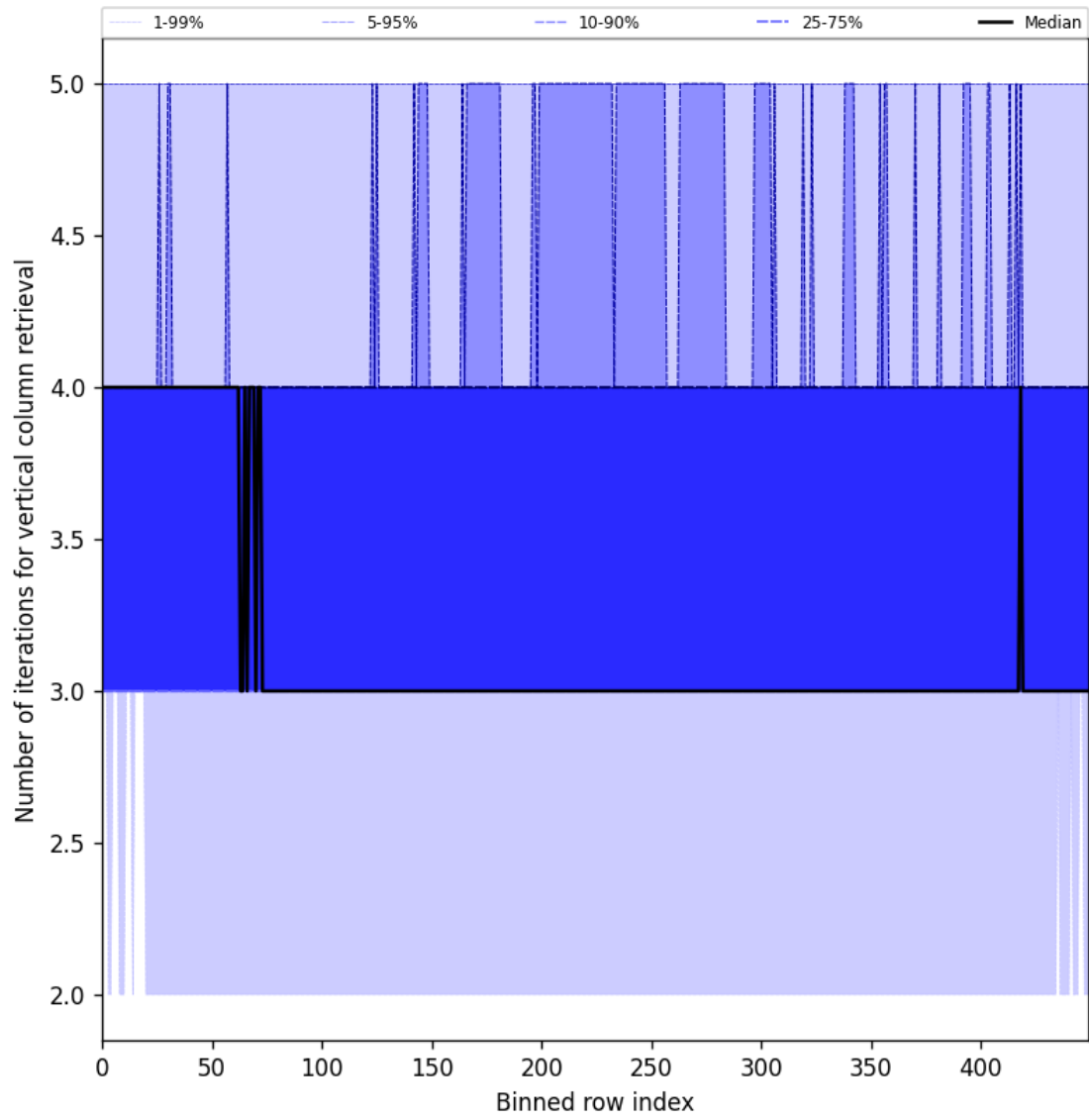
Figure 33: Along track statistics of “Number of iterations for vertical column retrieval” for 2025-07-31 to 2025-08-02
