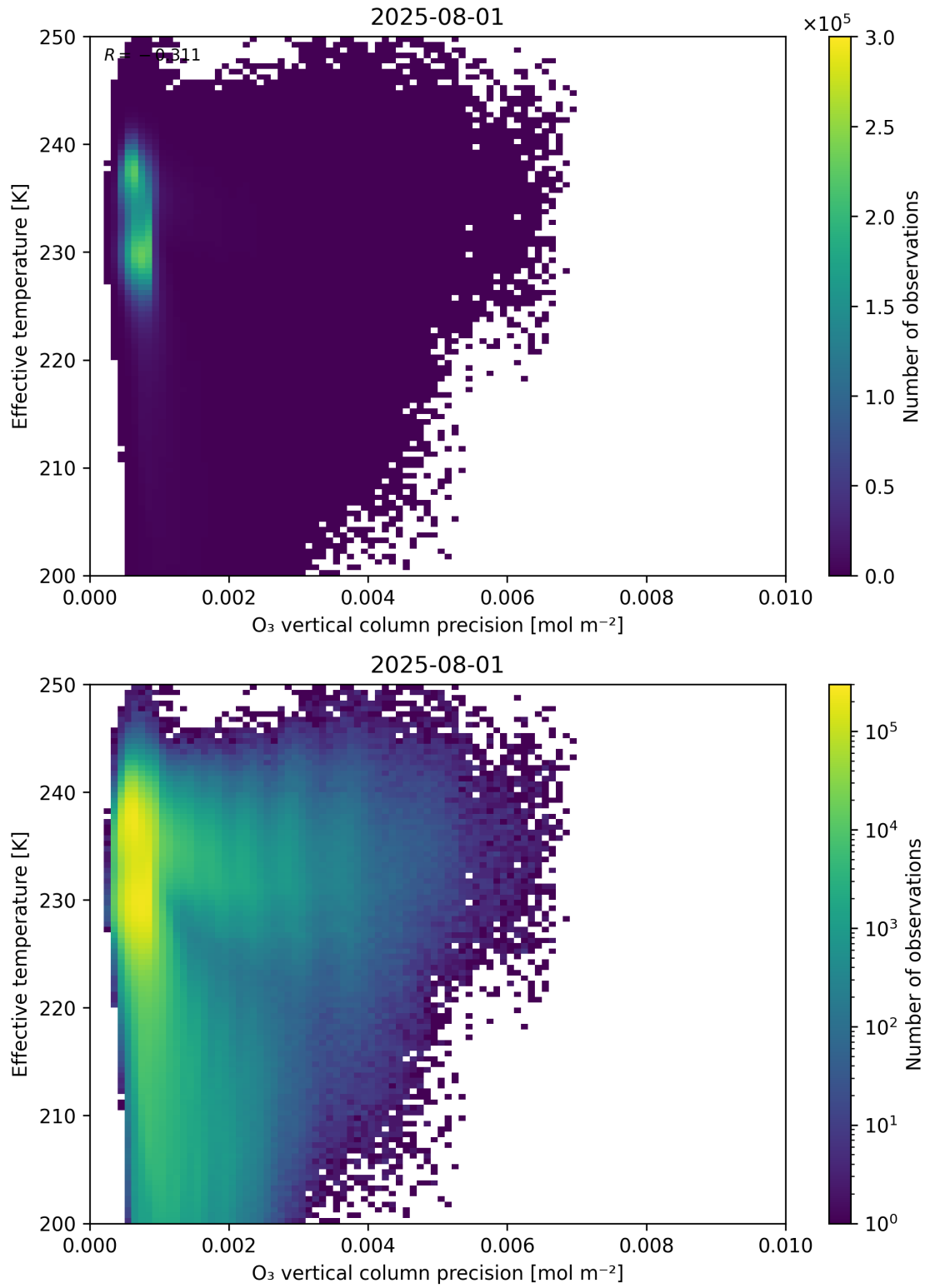
Figure 42: Scatter density plot of “O 3 vertical column precision” against “Effective temperature” for 2025-07-31 to 2025-08-02.
