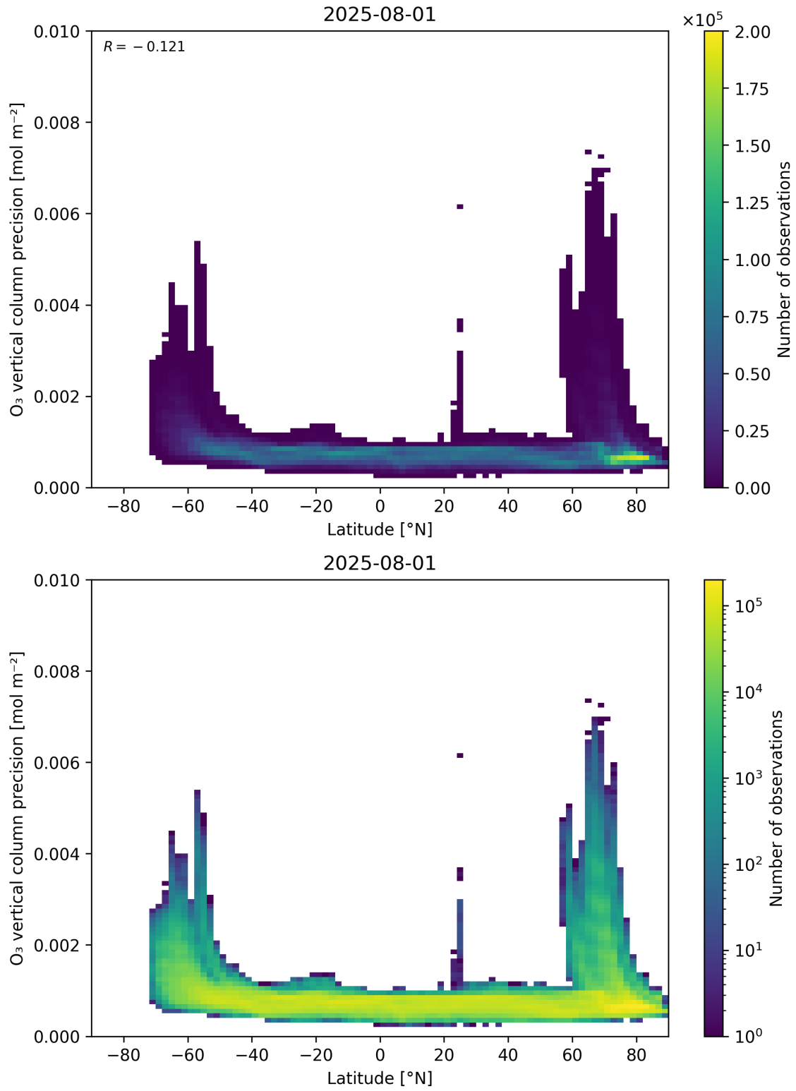
Figure 37: Scatter density plot of “Latitude” against “O 3 vertical column precision” for 2025-07-31 to 2025-08-02.
