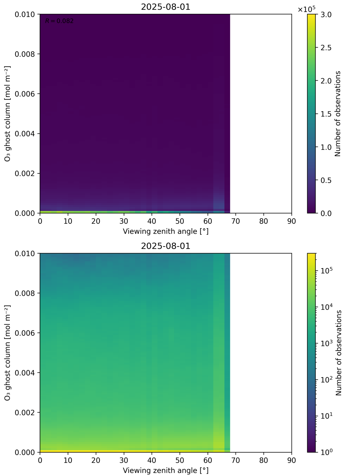
Figure 51: Scatter density plot of “Viewing zenith angle” against “O 3 ghost column” for 2025-07-31 to 2025-08-02.
