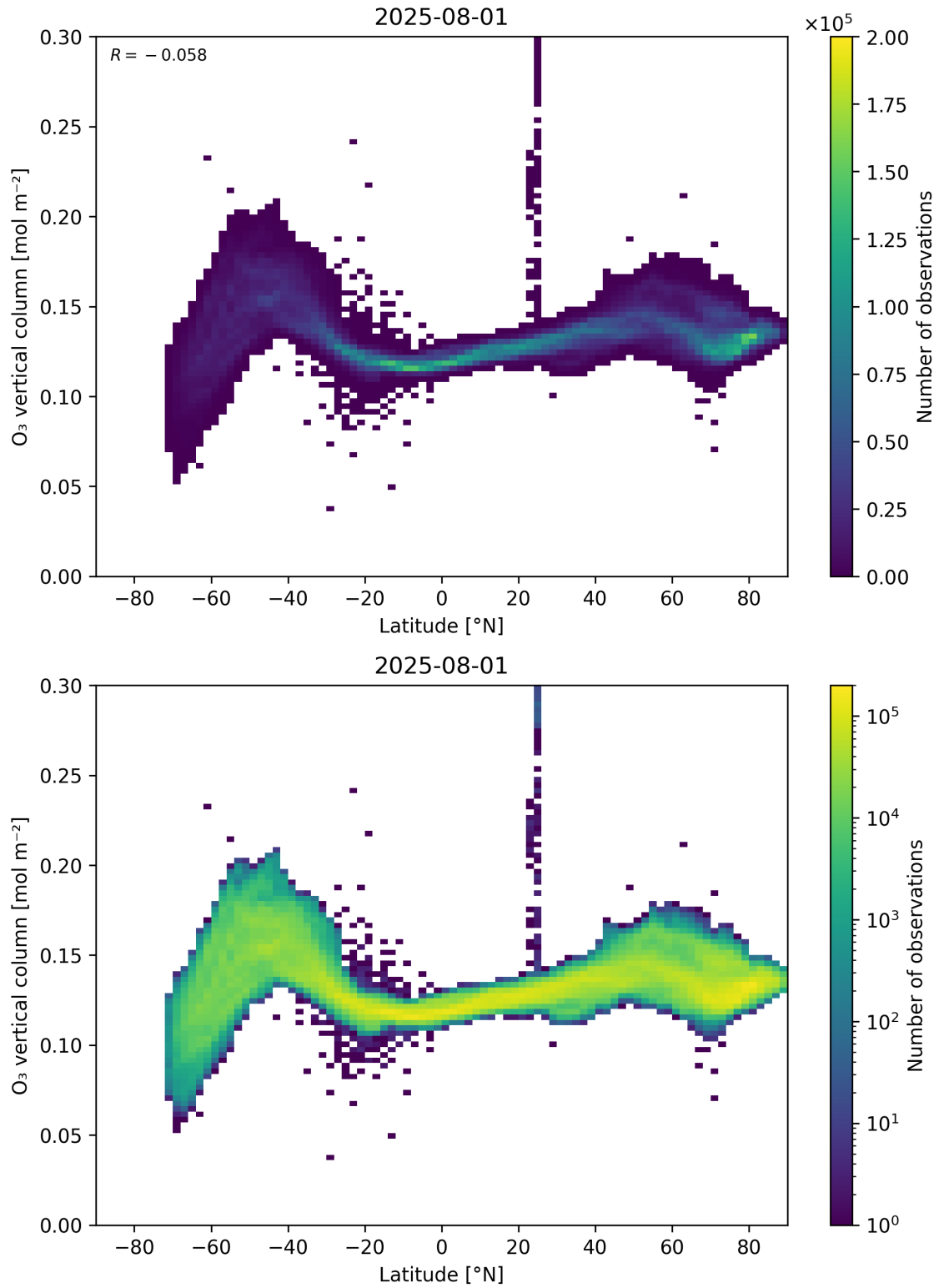
Figure 36: Scatter density plot of “Latitude” against “O 3 vertical column” for 2025-07-31 to 2025-08-02.
