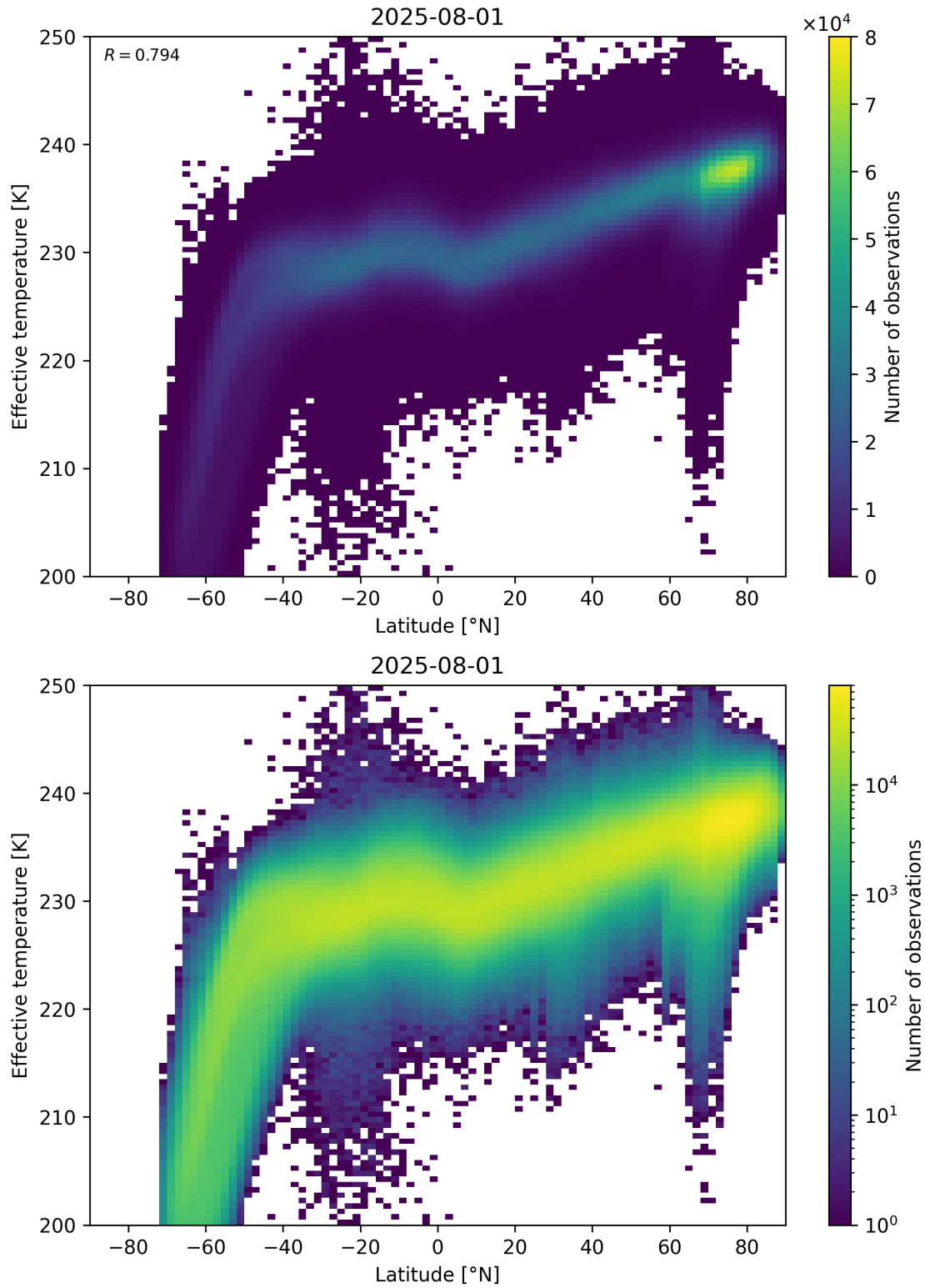
Figure 34: Scatter density plot of “Latitude” against “Effective temperature” for 2025-07-31 to 2025-08-02.
