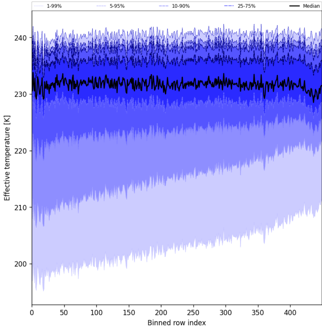
Figure 31: Along track statistics of “Effective temperature” for 2025-07-31 to 2025-08-02
