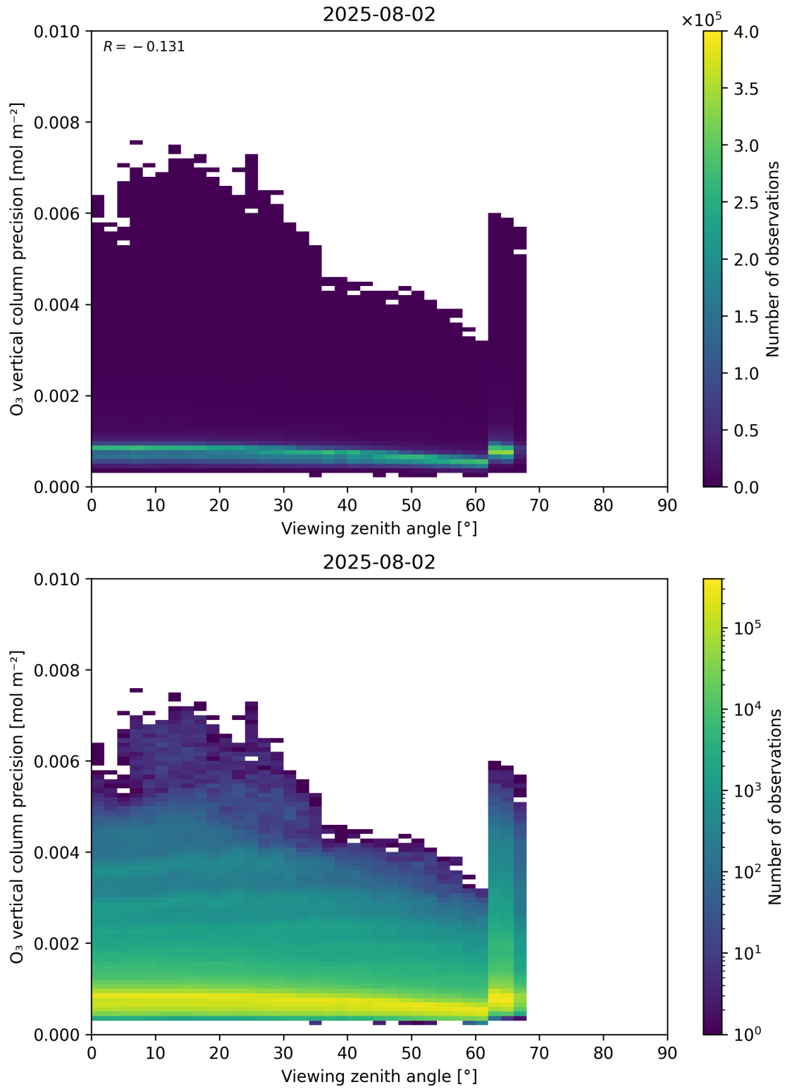
Figure 53: Scatter density plot of “Viewing zenith angle” against “O 3 vertical column precision” for 2025-08-01 to 2025-08-03.
