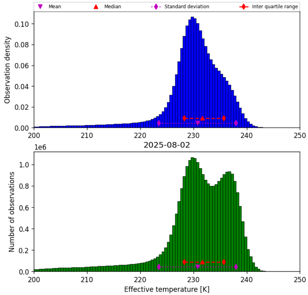
Figure 24: Histogram of “Effective temperature” for 2025-08-01 to 2025-08-03
