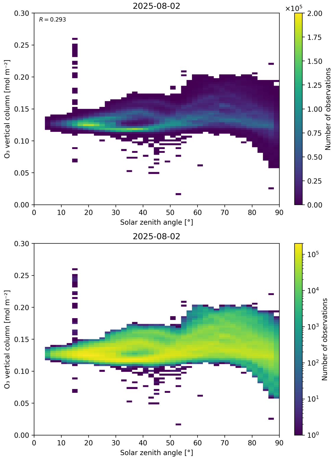
Figure 47: Scatter density plot of “Solar zenith angle” against “O 3 vertical column” for 2025-08-01 to 2025-08-03.
