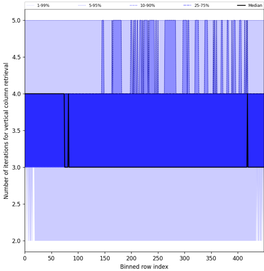
Figure 33: Along track statistics of “Number of iterations for vertical column retrieval” for 2025-08-01 to 2025-08-03
