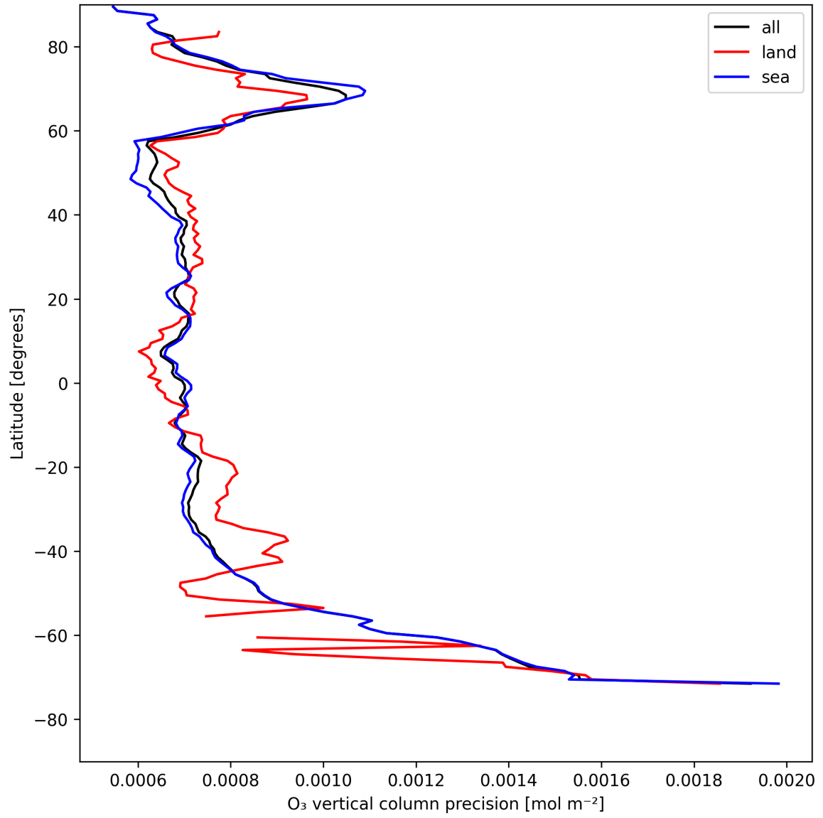
Figure 15: Zonal average of “O 3 vertical column precision” for 2025-08-01 to 2025-08-03.
