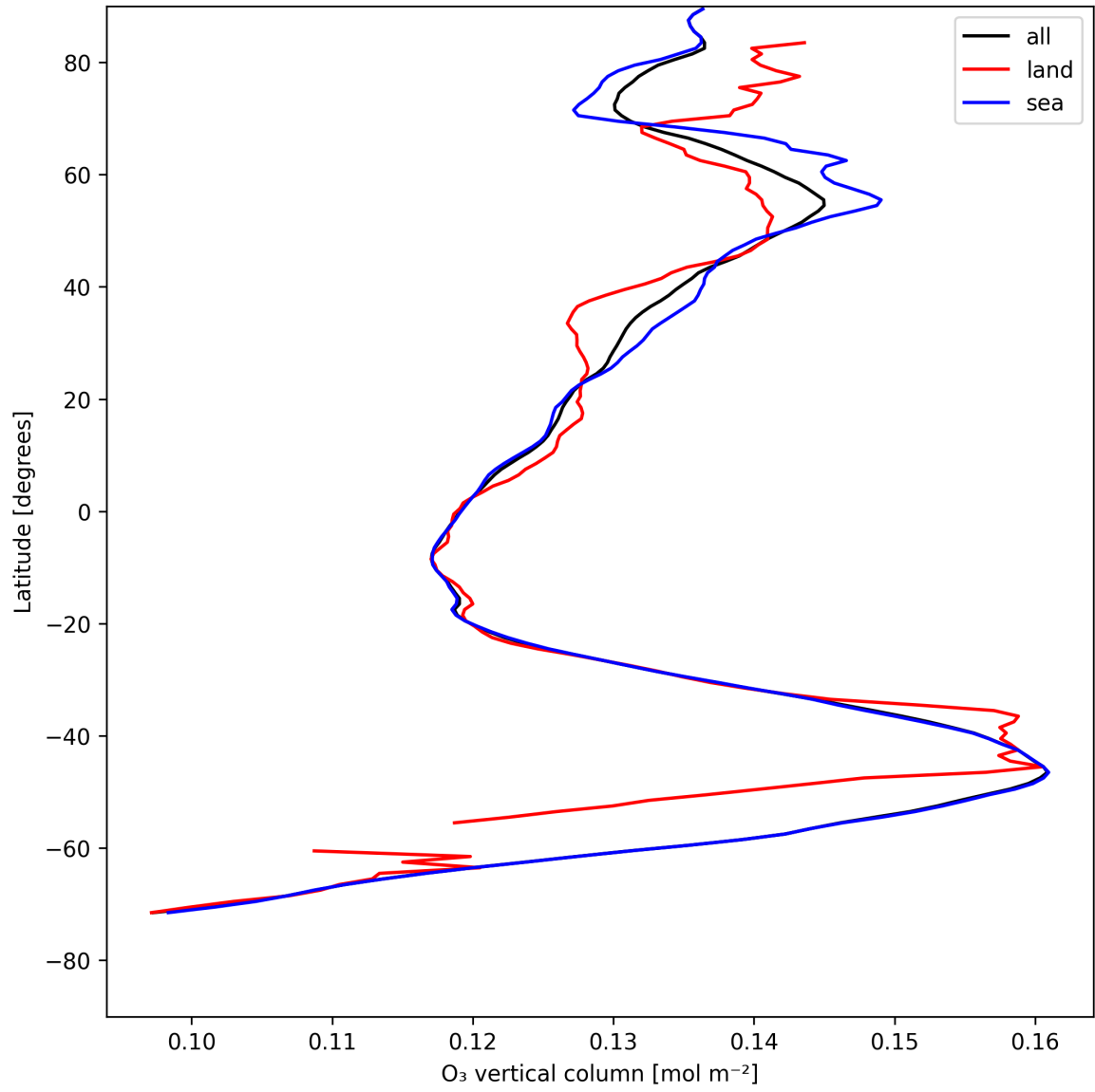
Figure 14: Zonal average of “O 3 vertical column” for 2025-08-01 to 2025-08-03.
