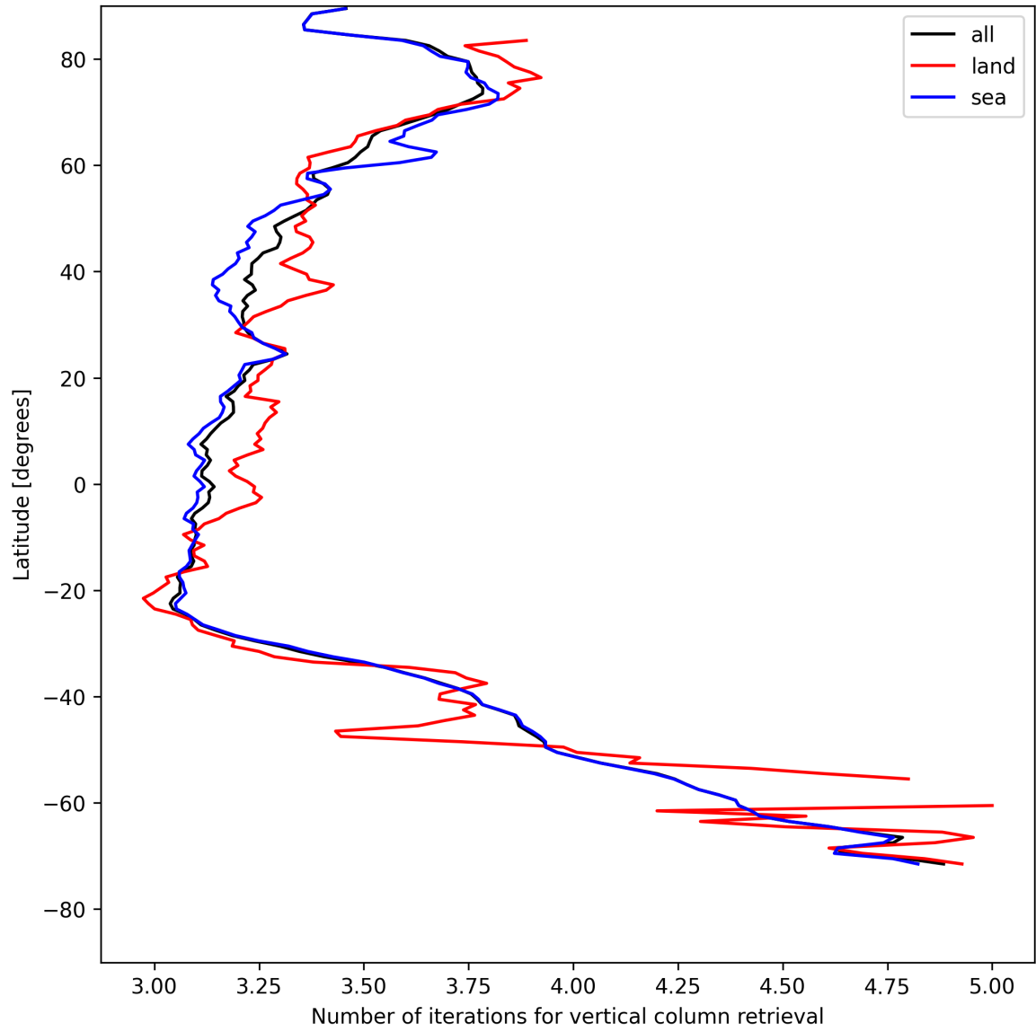
Figure 19: Zonal average of “Number of iterations for vertical column retrieval” for 2025-08-01 to 2025-08-03.
