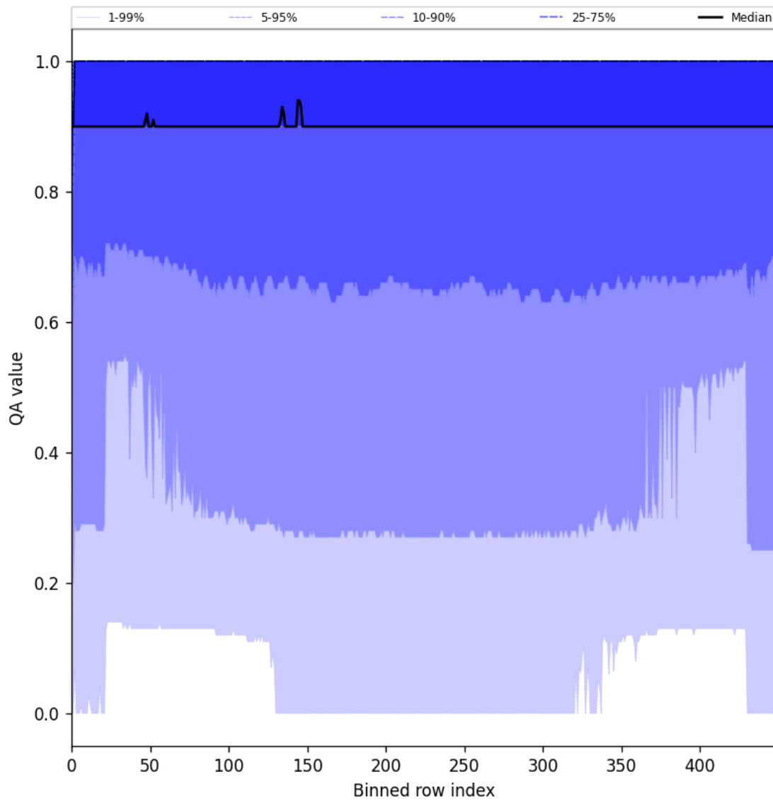
Figure 27: Along track statistics of “QA value” for 2025-08-01 to 2025-08-03
