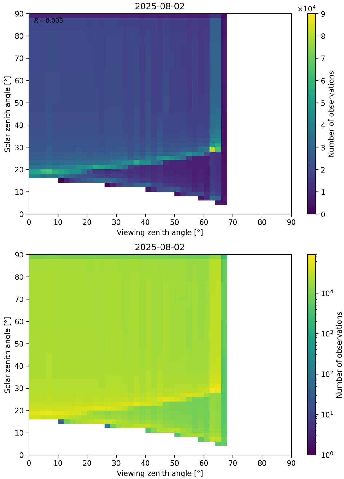
Figure 54: Scatter density plot of “Viewing zenith angle” against “Solar zenith angle” for 2025-08-01 to 2025-08-03.
