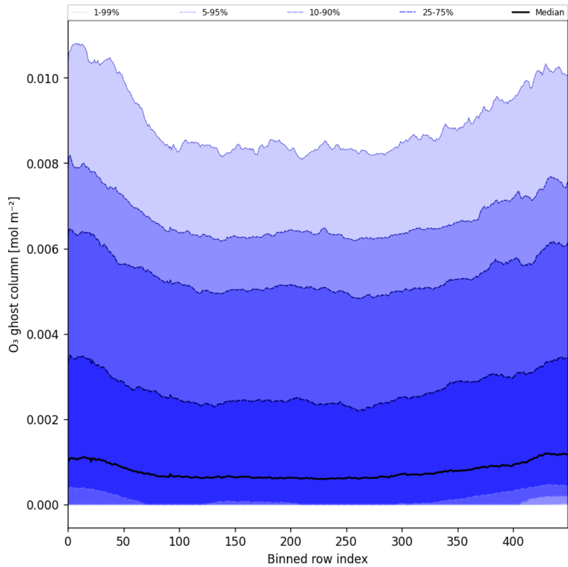
Figure 32: Along track statistics of "O 3 ghost column" for 2025-08-01 to 2025-08-03
