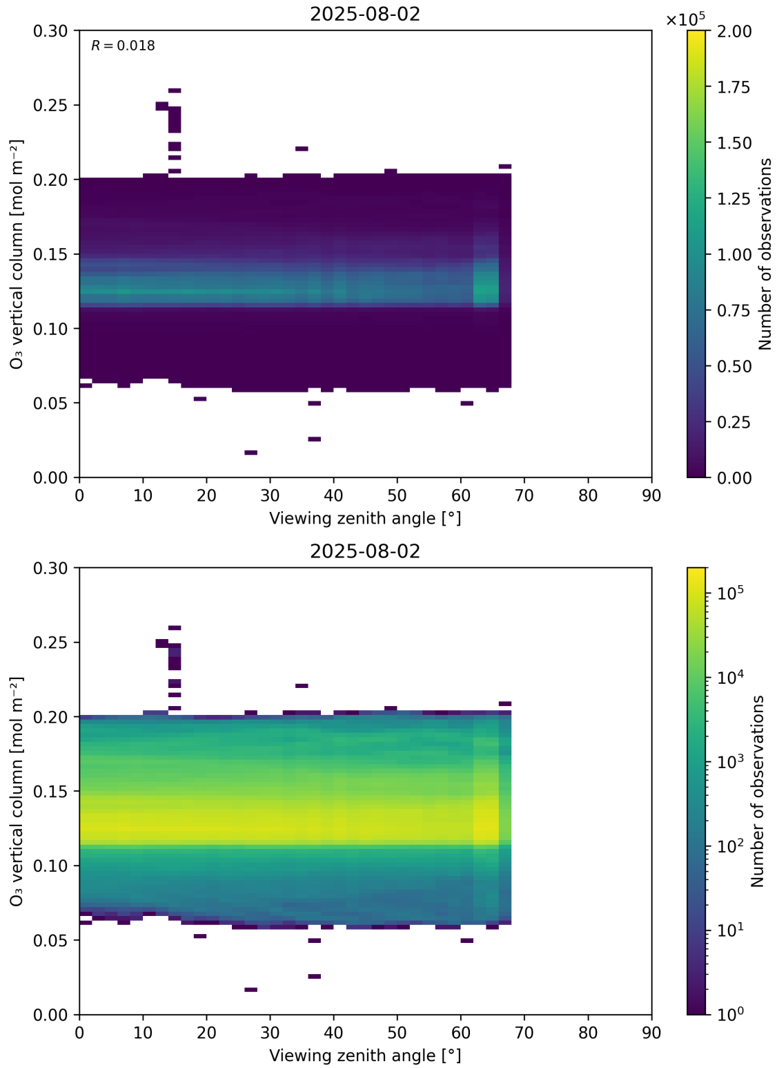
Figure 52: Scatter density plot of “Viewing zenith angle” against “O 3 vertical column” for 2025-08-01 to 2025-08-03.
