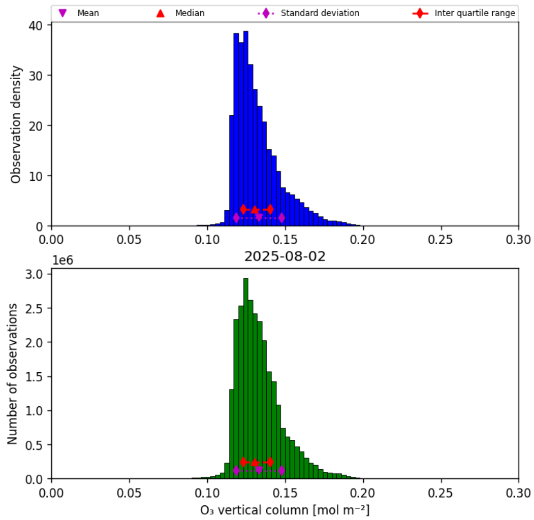
Figure 21: Histogram of “O 3 vertical column” for 2025-08-01 to 2025-08-03
