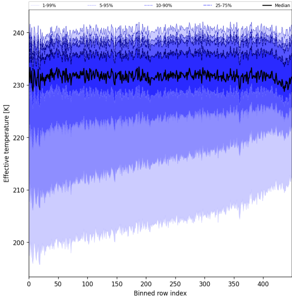
Figure 31: Along track statistics of “Effective temperature” for 2025-08-01 to 2025-08-03
