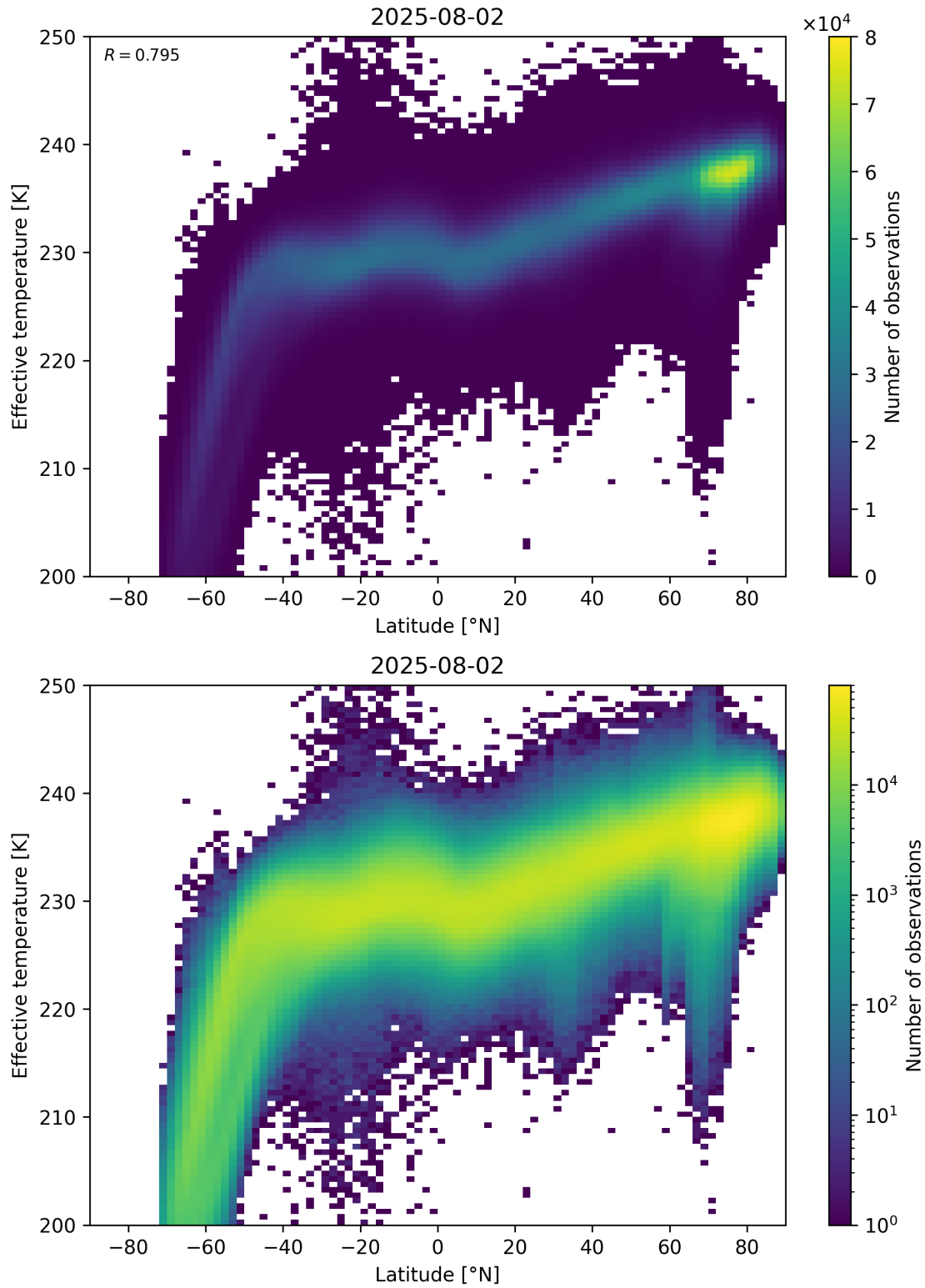
Figure 34: Scatter density plot of “Latitude” against “Effective temperature” for 2025-08-01 to 2025-08-03.
