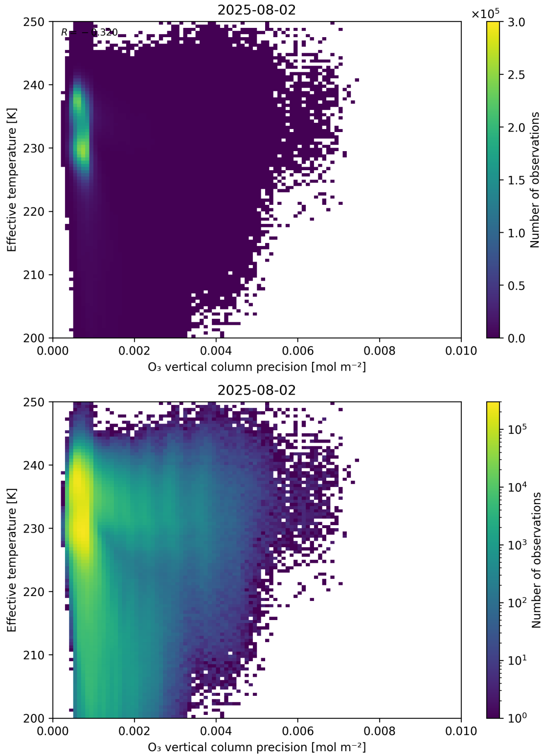
Figure 42: Scatter density plot of “O 3 vertical column precision” against “Effective temperature” for 2025-08-01 to 2025-08-03.
