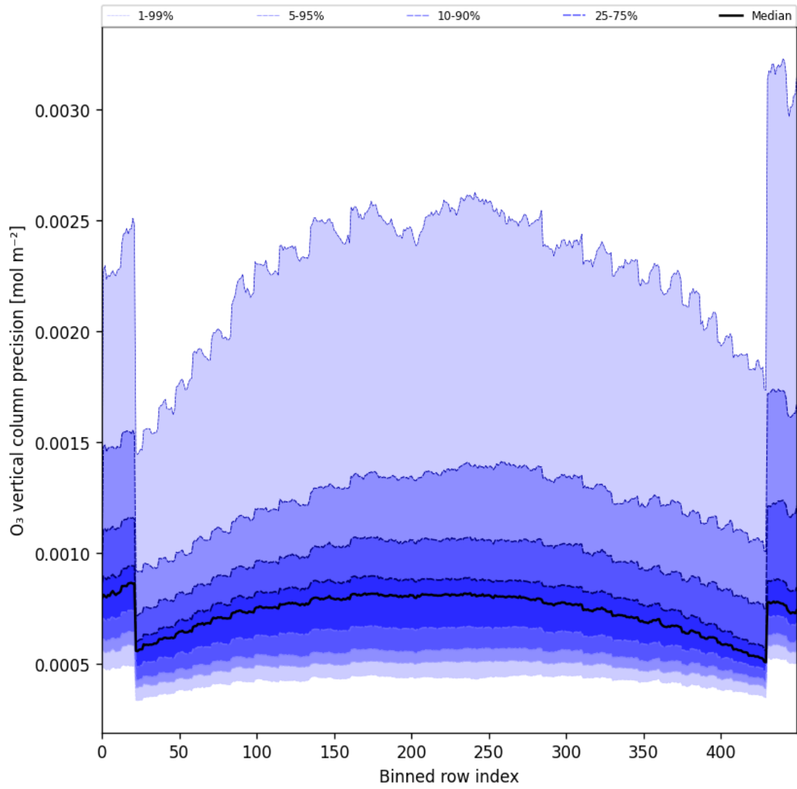
Figure 29: Along track statistics of “O 3 vertical column precision” for 2025-08-01 to 2025-08-03
