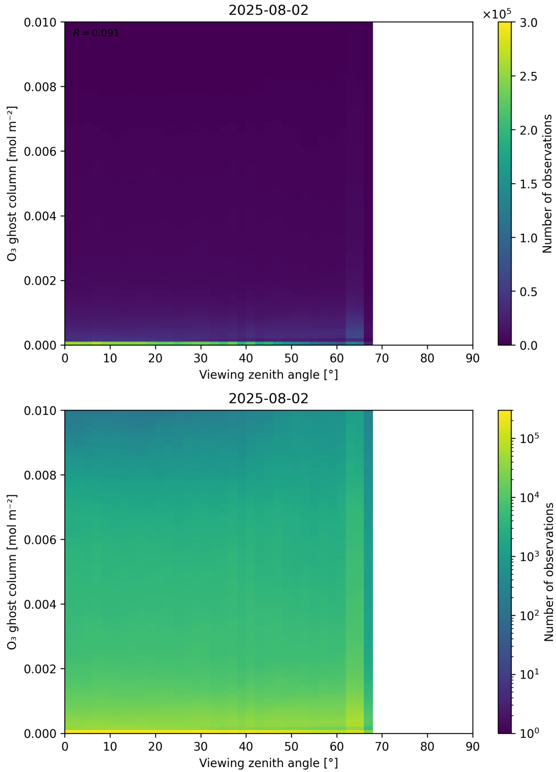
Figure 51: Scatter density plot of “Viewing zenith angle” against “O 3 ghost column” for 2025-08-01 to 2025-08-03.
