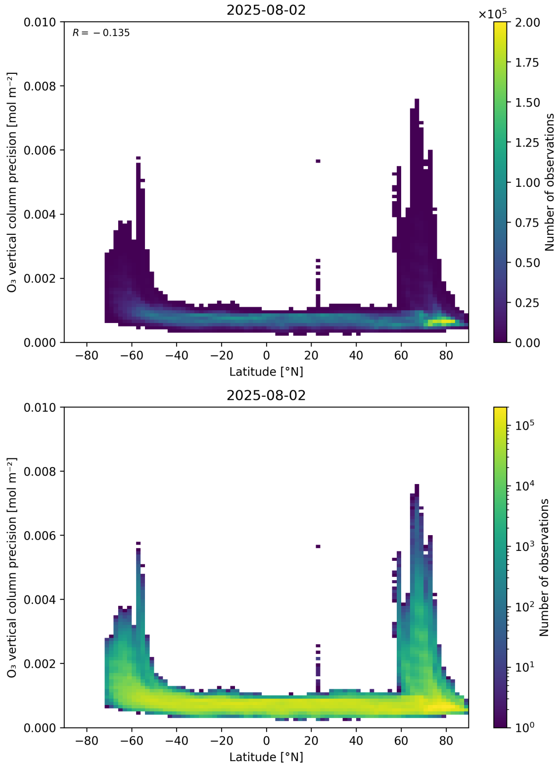
Figure 37: Scatter density plot of “Latitude” against “O 3 vertical column precision” for 2025-08-01 to 2025-08-03.
