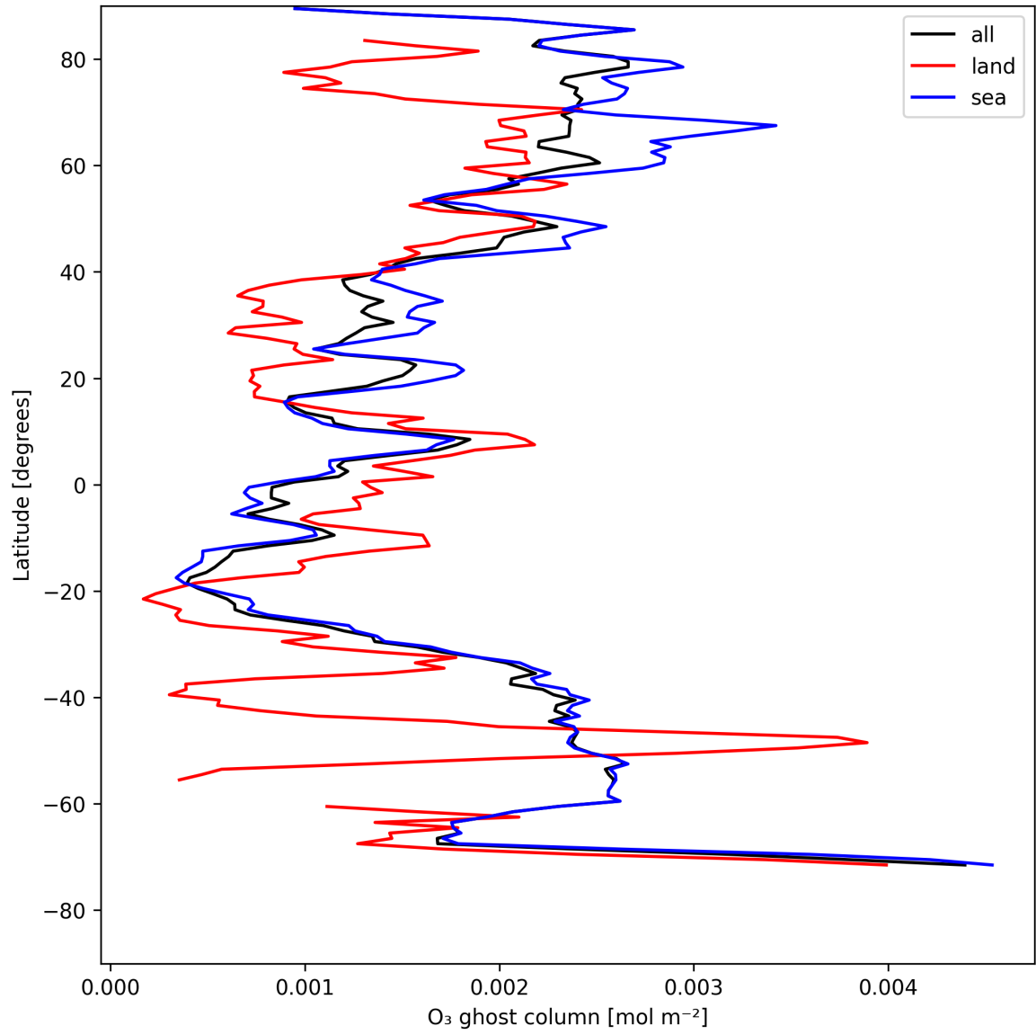
Figure 18: Zonal average of "O 3 ghost column" for 2025-08-01 to 2025-08-03.
