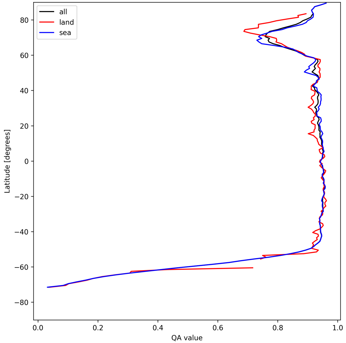
Figure 13: Zonal average of “QA value” for 2025-08-01 to 2025-08-03.
