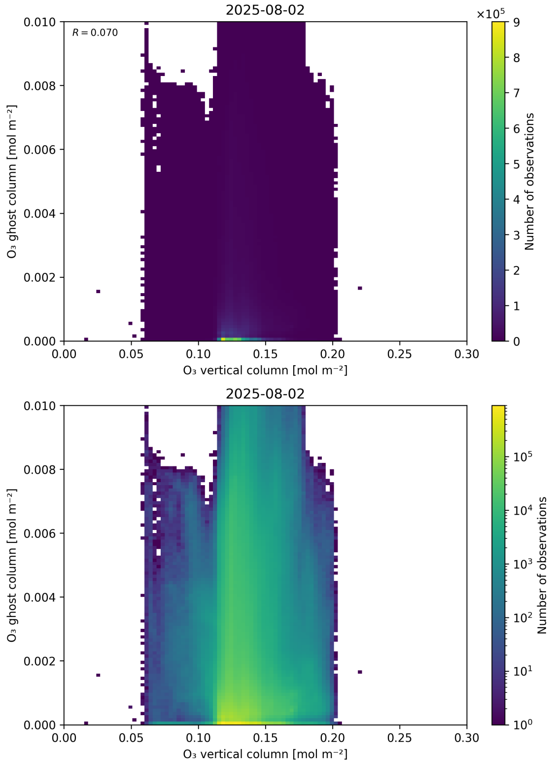
Figure 40: Scatter density plot of “O 3 vertical column” against “O 3 ghost column” for 2025-08-01 to 2025-08-03.
