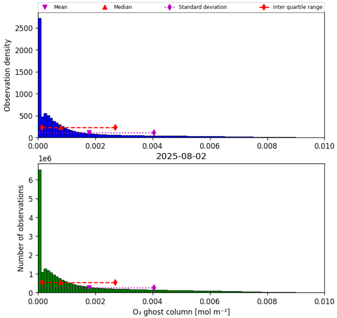
Figure 25: Histogram of “O 3 ghost column” for 2025-08-01 to 2025-08-03
