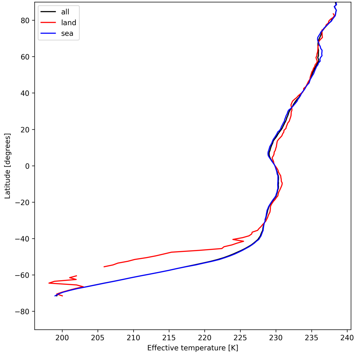
Figure 17: Zonal average of “Effective temperature” for 2025-08-01 to 2025-08-03.
