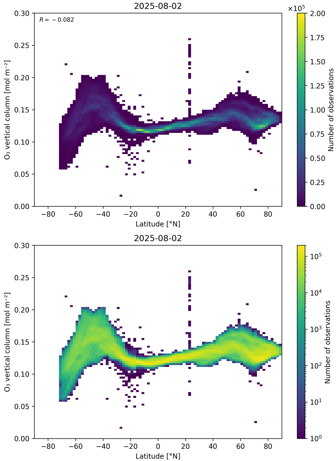
Figure 36: Scatter density plot of “Latitude” against “O 3 vertical column” for 2025-08-01 to 2025-08-03.
