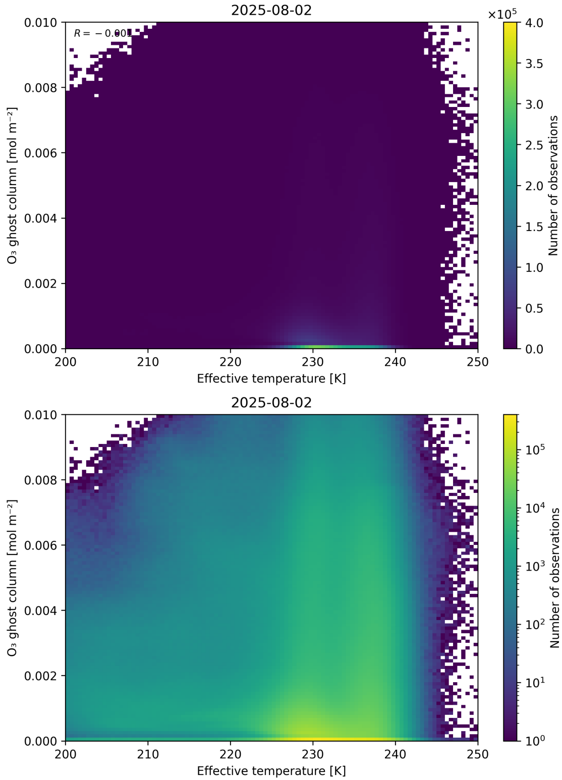
Figure 38: Scatter density plot of “Effective temperature” against “O 3 ghost column” for 2025-08-01 to 2025-08-03.
