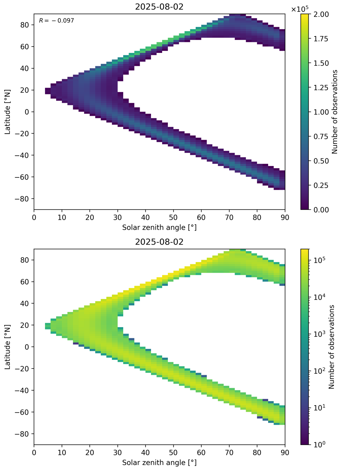
Figure 44: Scatter density plot of “Solar zenith angle” against “Latitude” for 2025-08-01 to 2025-08-03.
