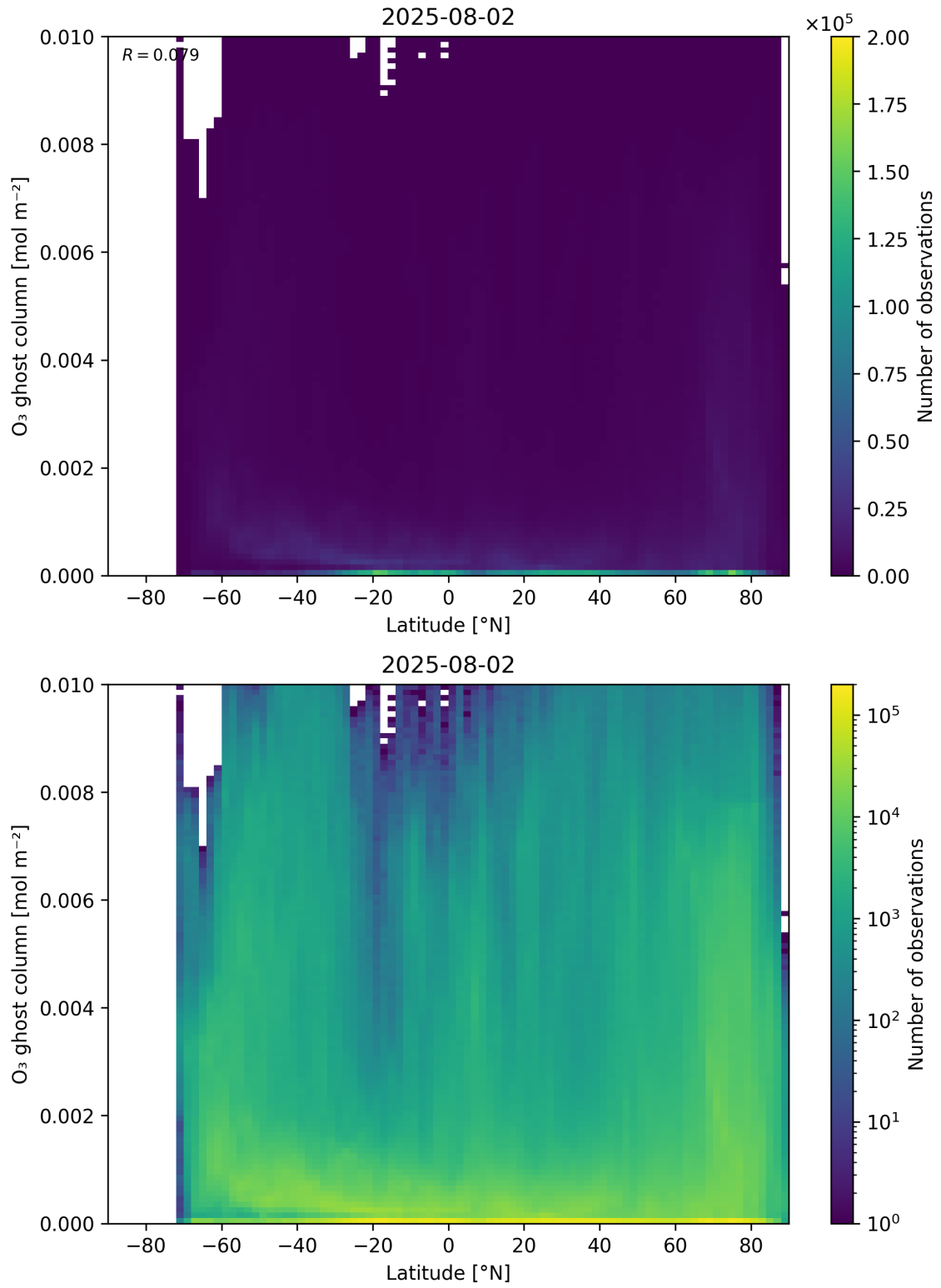
Figure 35: Scatter density plot of “Latitude” against “O 3 ghost column” for 2025-08-01 to 2025-08-03.
