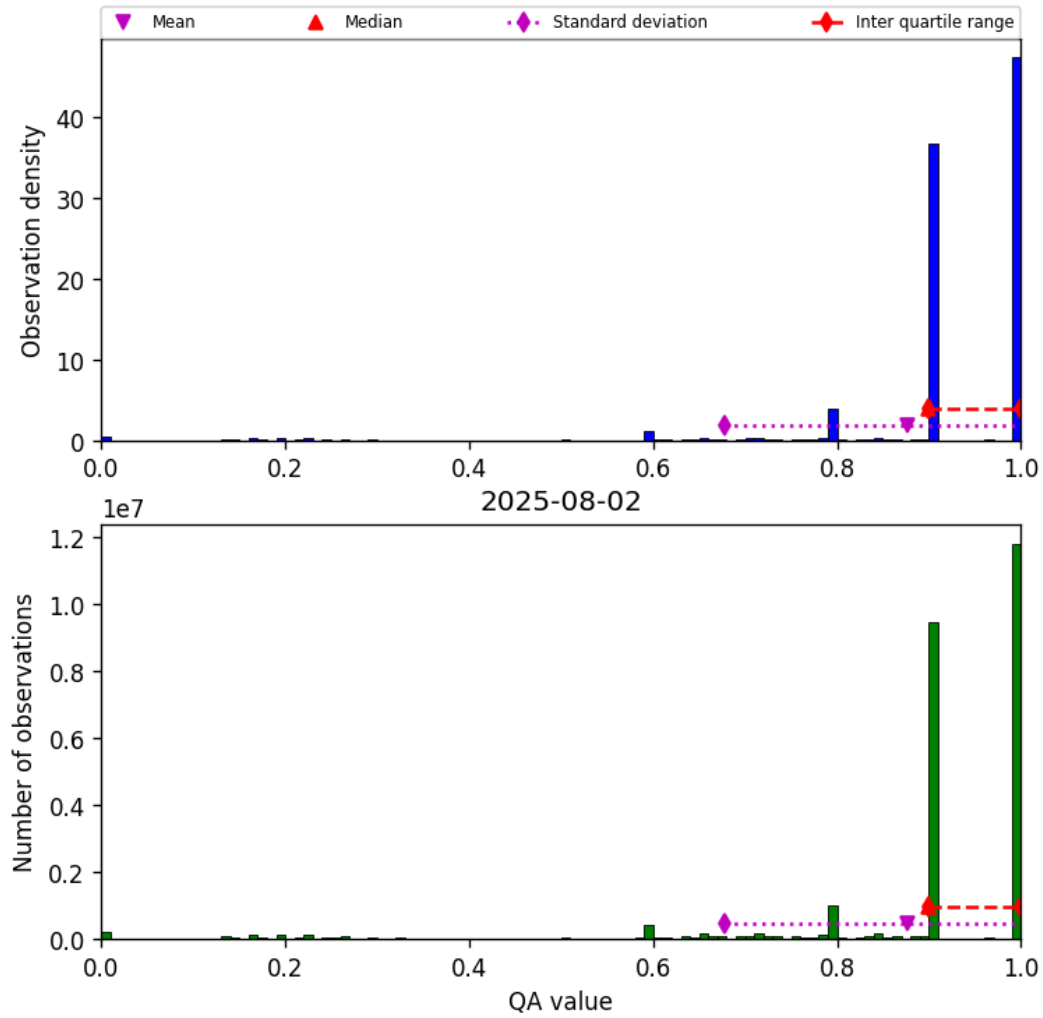
Figure 20: Histogram of “QA value” for 2025-08-01 to 2025-08-03
