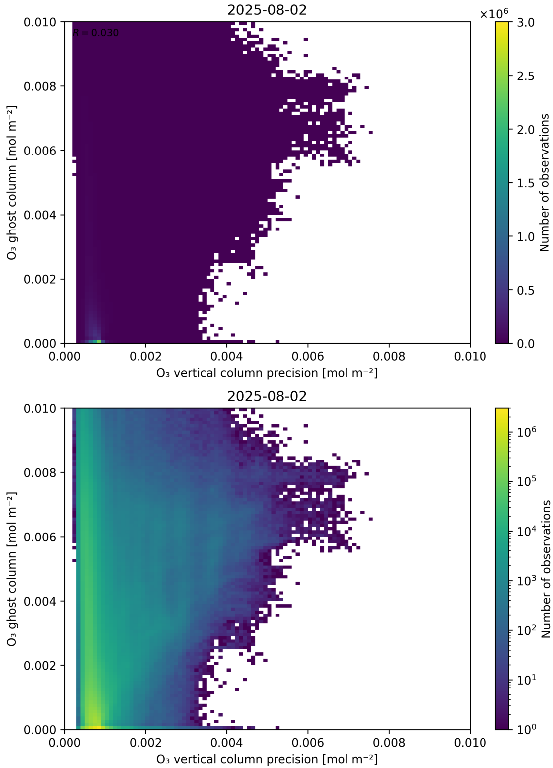
Figure 43: Scatter density plot of “O 3 vertical column precision” against “O 3 ghost column” for 2025-08-01 to 2025-08-03.
