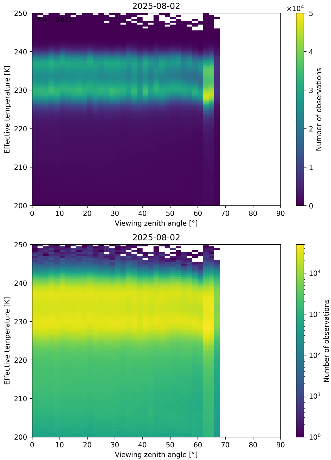
Figure 50: Scatter density plot of “Viewing zenith angle” against “Effective temperature” for 2025-08-01 to 2025-08-03.
