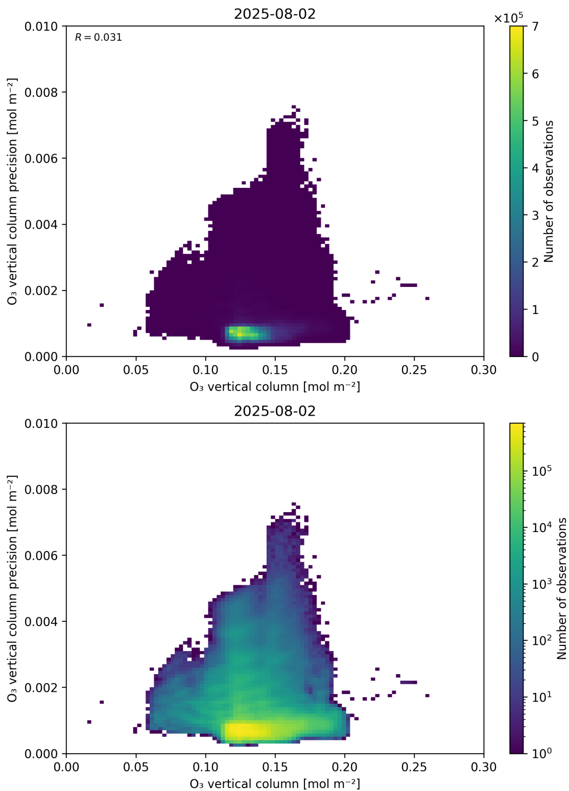
Figure 41: Scatter density plot of “O 3 vertical column” against “O 3 vertical column precision” for 2025-08-01 to 2025-08-03.
