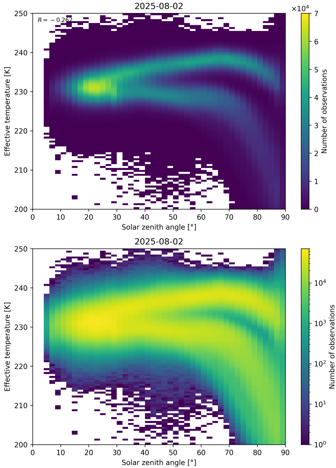
Figure 45: Scatter density plot of “Solar zenith angle” against “Effective temperature” for 2025-08-01 to 2025-08-03.
