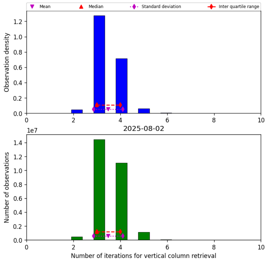
Figure 26: Histogram of “Number of iterations for vertical column retrieval” for 2025-08-01 to 2025-08-03
