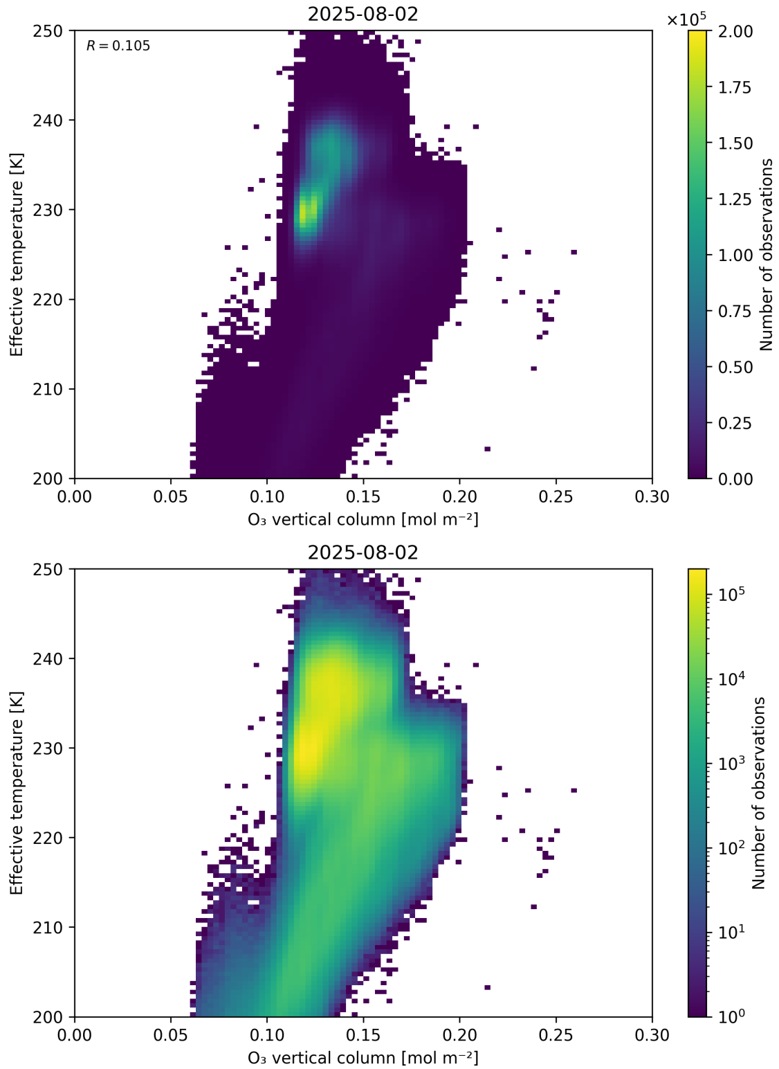
Figure 39: Scatter density plot of “O 3 vertical column” against “Effective temperature” for 2025-08-01 to 2025-08-03.
