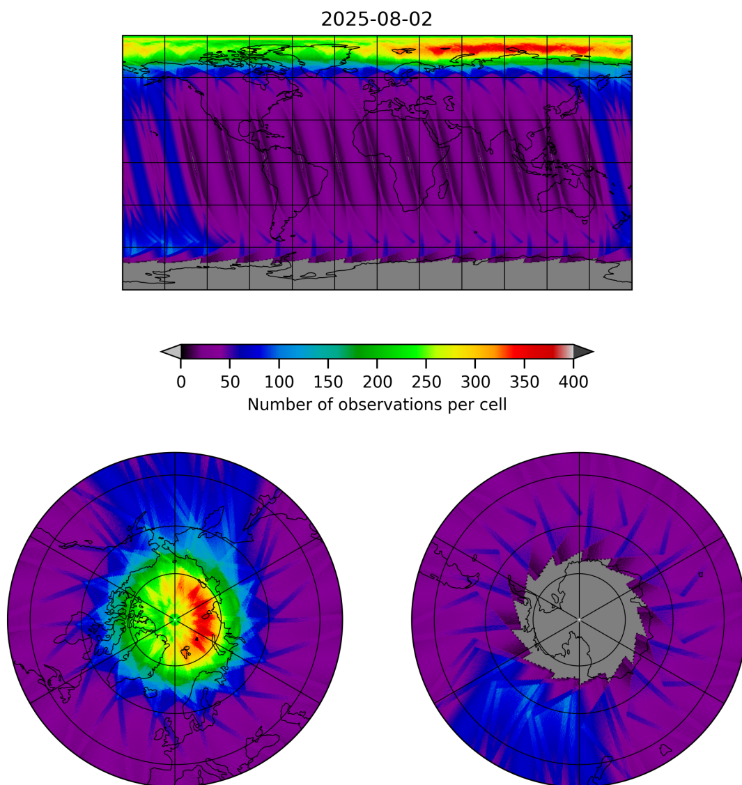
Figure 12: Map of the number of observations for 2025-08-01 to 2025-08-03
