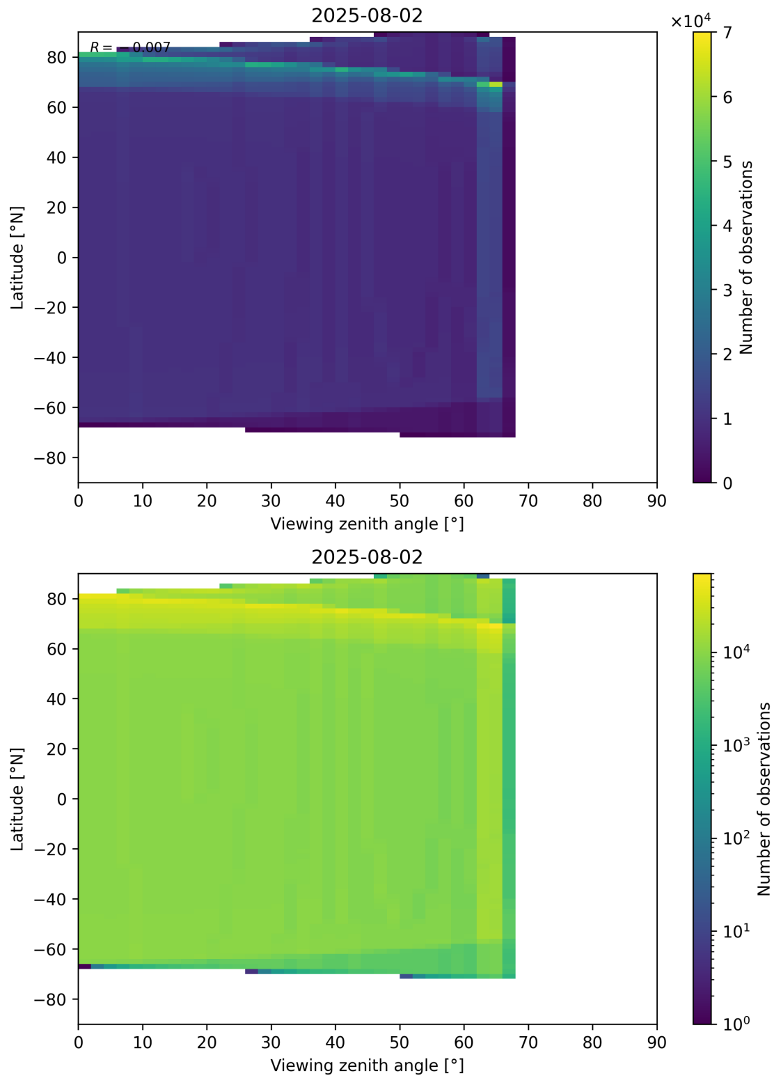
Figure 49: Scatter density plot of “Viewing zenith angle” against “Latitude” for 2025-08-01 to 2025-08-03.
