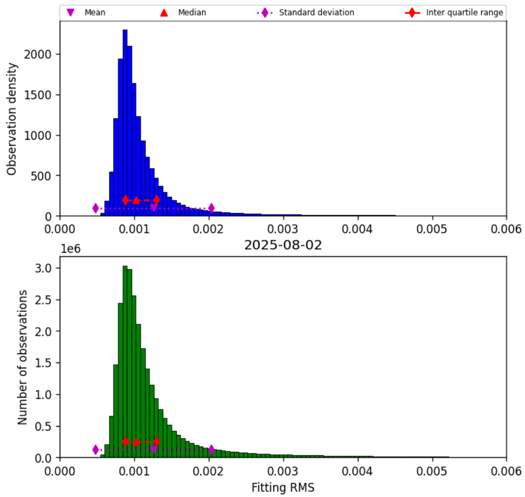
Figure 23: Histogram of “Fitting RMS” for 2025-08-01 to 2025-08-03
