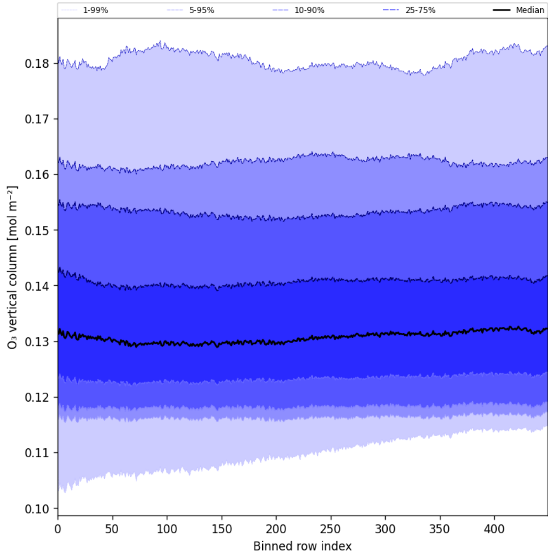
Figure 28: Along track statistics of “O 3 vertical column” for 2025-08-01 to 2025-08-03
