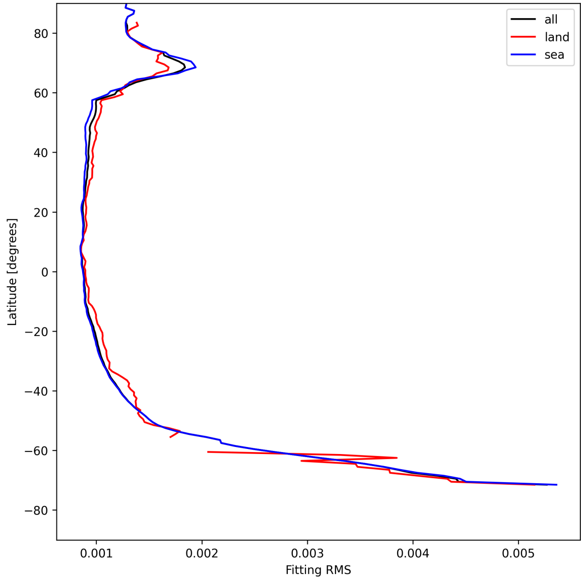
Figure 16: Zonal average of “Fitting RMS” for 2025-08-01 to 2025-08-03.
