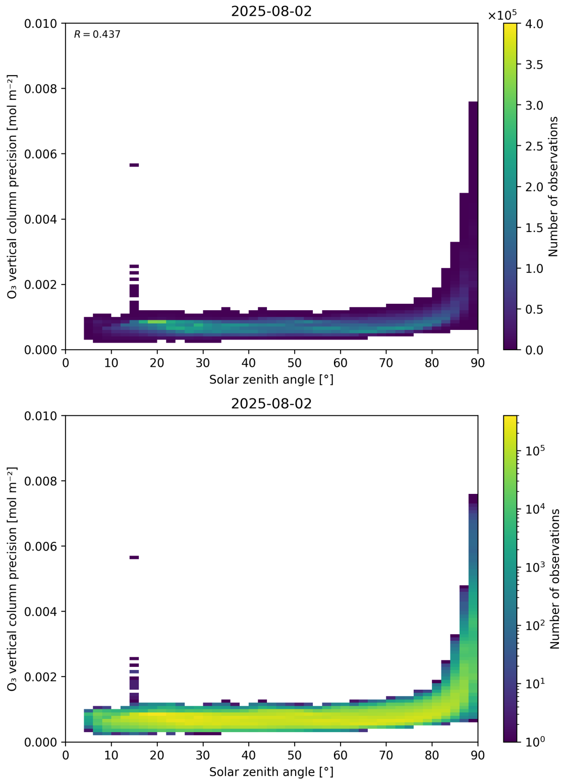
Figure 48: Scatter density plot of “Solar zenith angle” against “O 3 vertical column precision” for 2025-08-01 to 2025-08-03.
