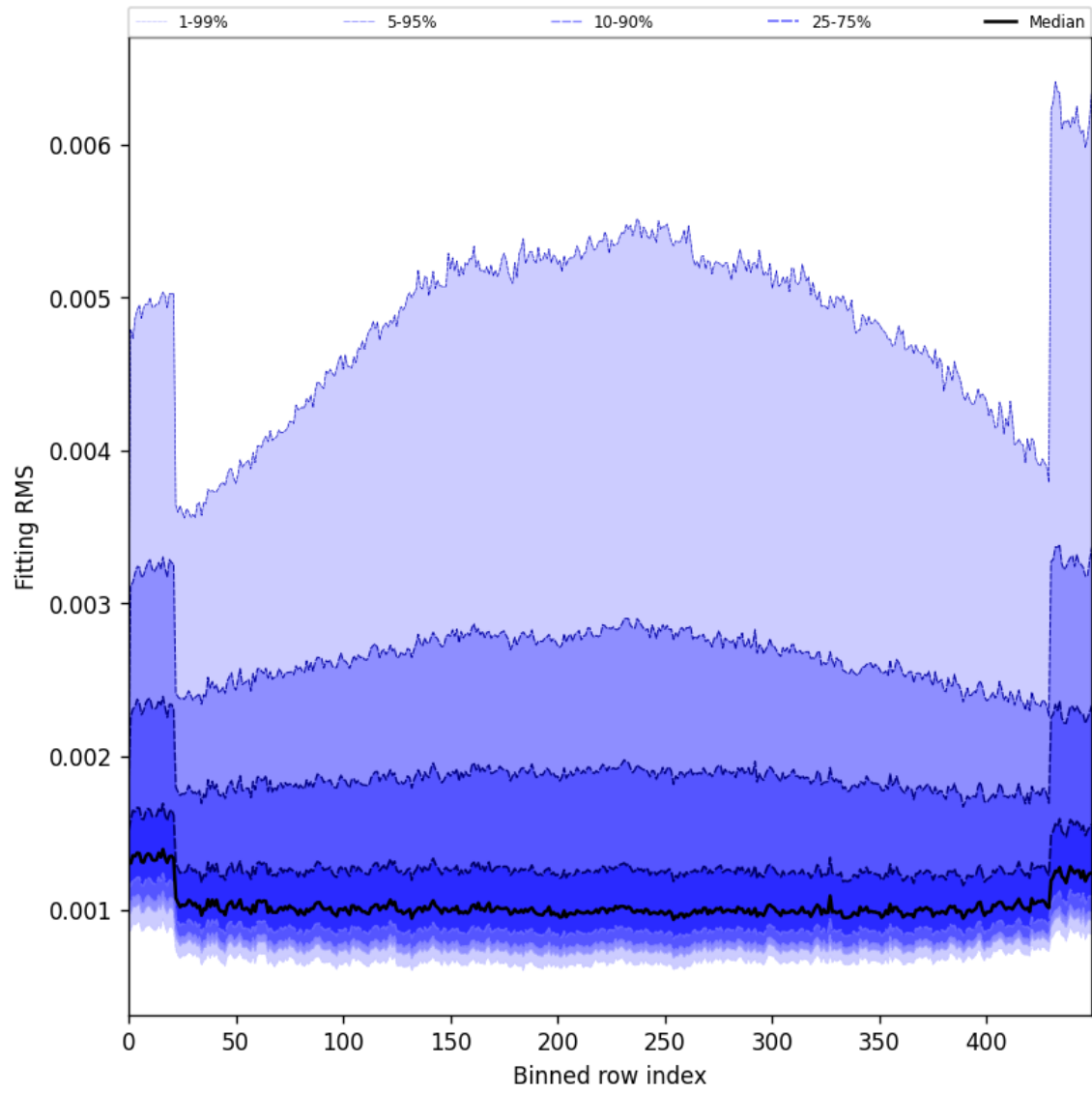
Figure 30: Along track statistics of “Fitting RMS” for 2025-08-01 to 2025-08-03
