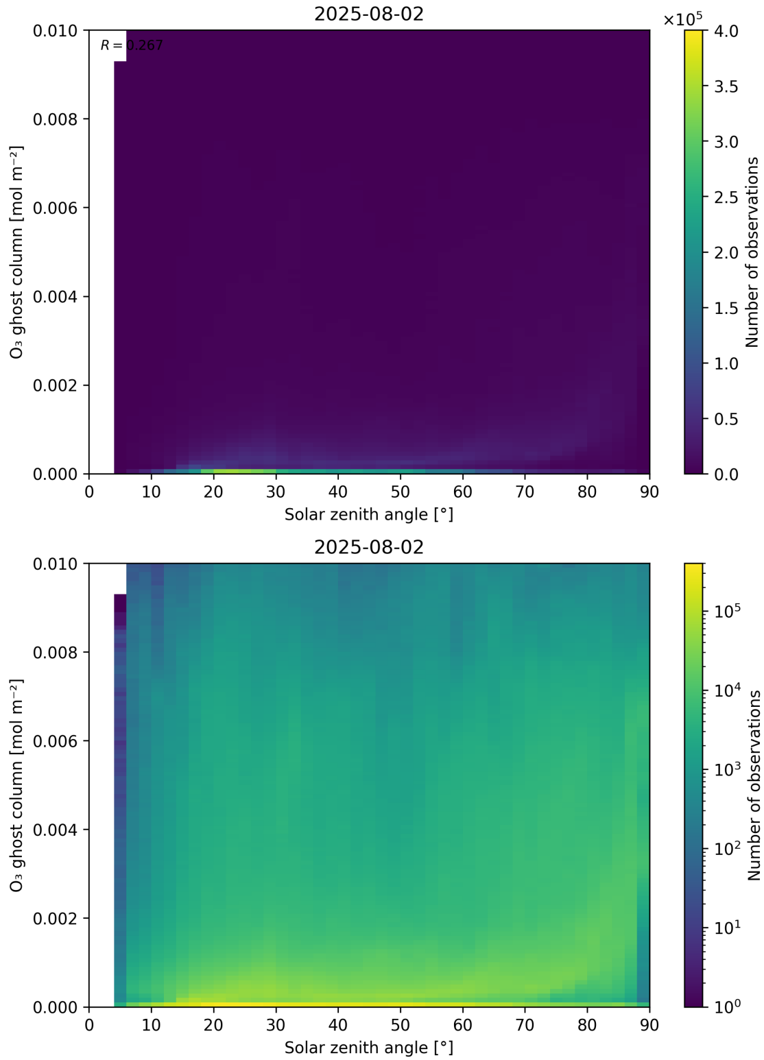
Figure 46: Scatter density plot of “Solar zenith angle” against “O 3 ghost column” for 2025-08-01 to 2025-08-03.
