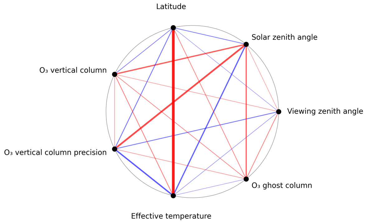
Figure 1: Map of correlation graph for 2025-08-01 to 2025-08-03.
