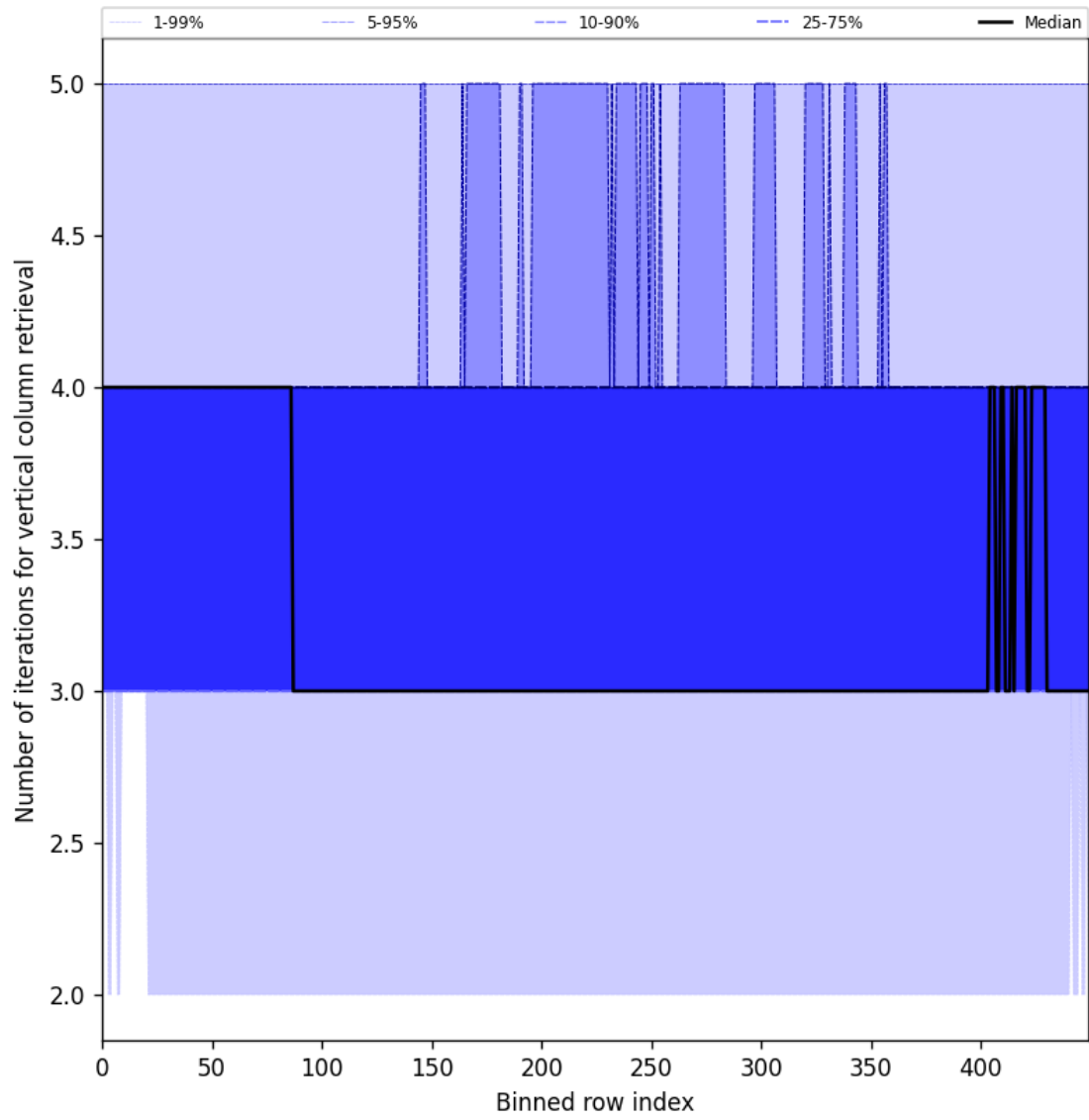
Figure 33: Along track statistics of “Number of iterations for vertical column retrieval” for 2025-08-03 to 2025-08-04
