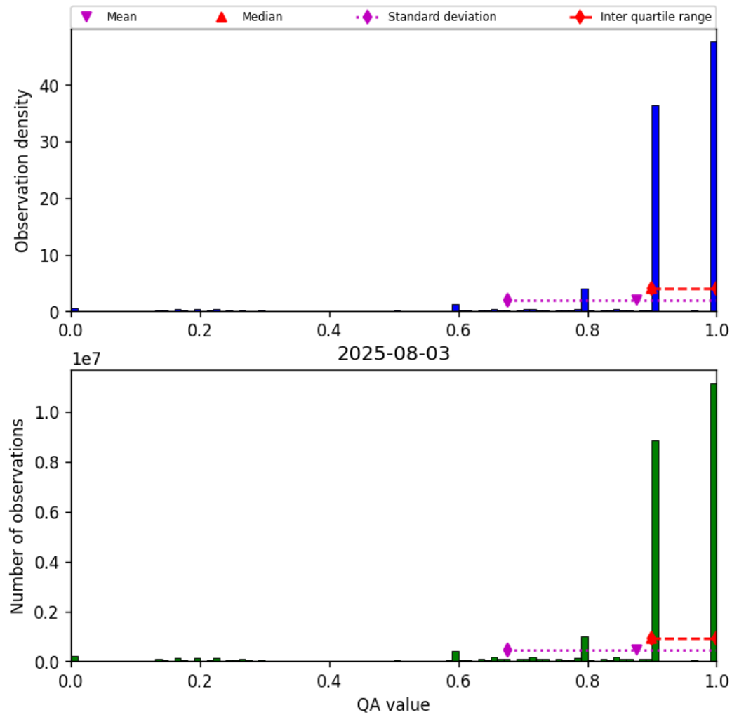
Figure 20: Histogram of “QA value” for 2025-08-03 to 2025-08-04
