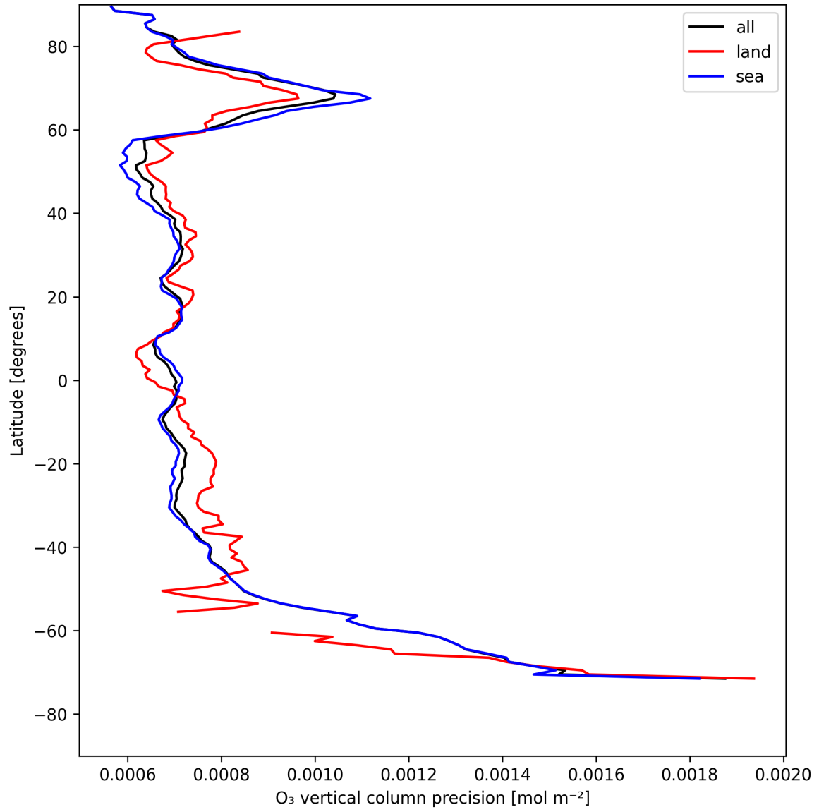
Figure 15: Zonal average of “O 3 vertical column precision” for 2025-08-03 to 2025-08-04.
