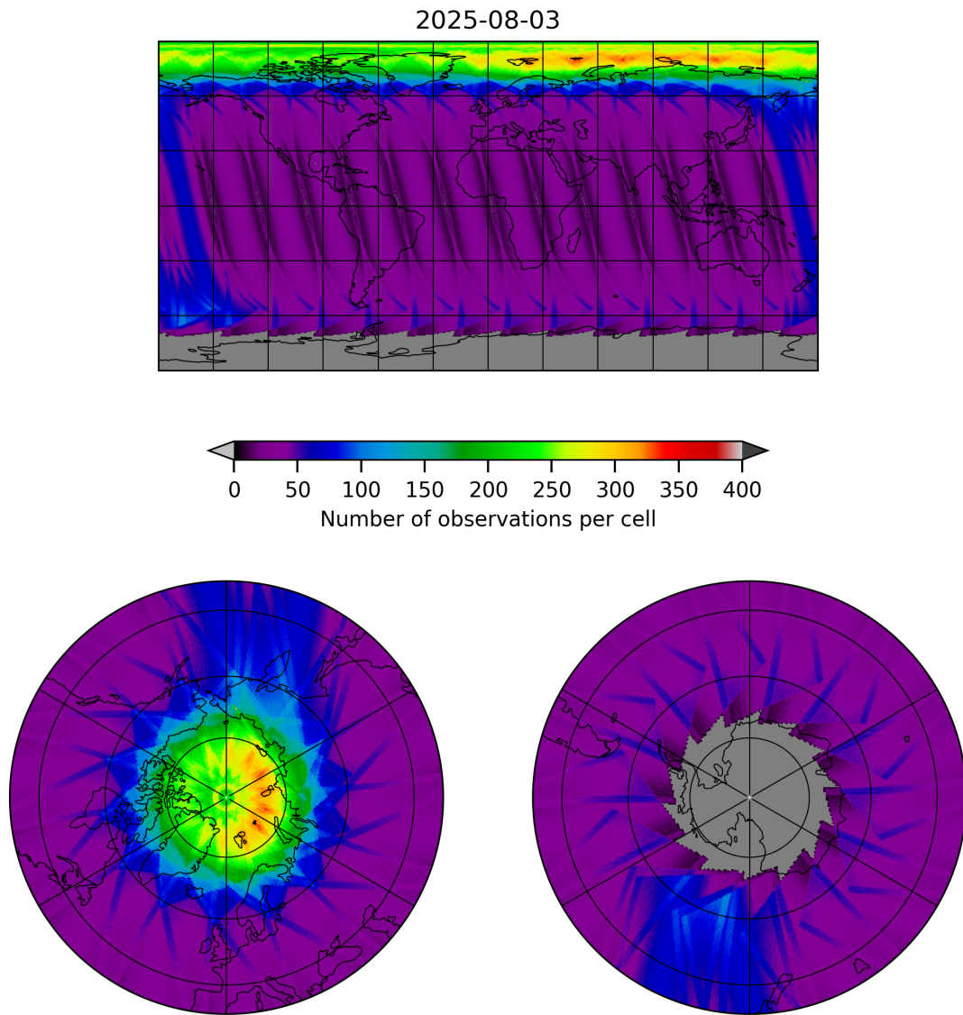
Figure 12: Map of the number of observations for 2025-08-03 to 2025-08-04
