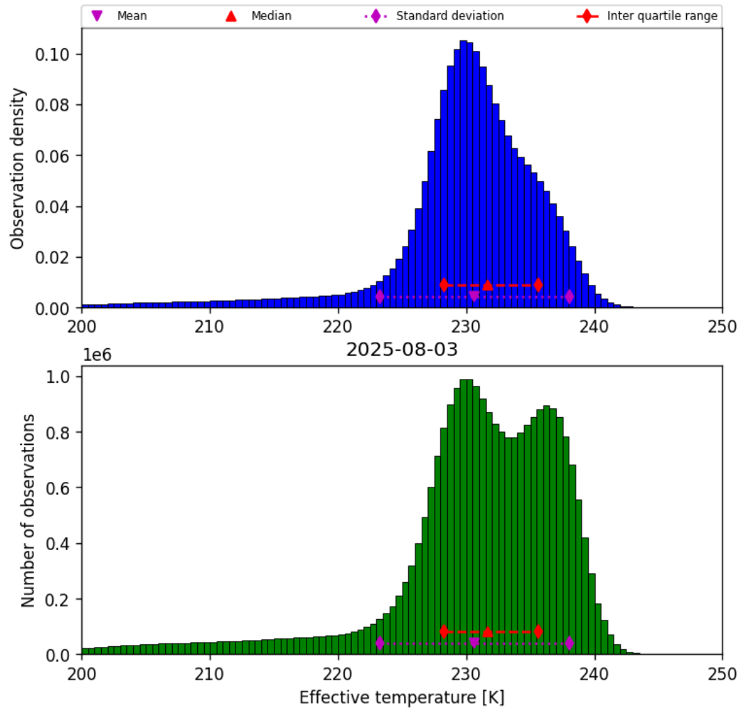
Figure 24: Histogram of “Effective temperature” for 2025-08-03 to 2025-08-04
