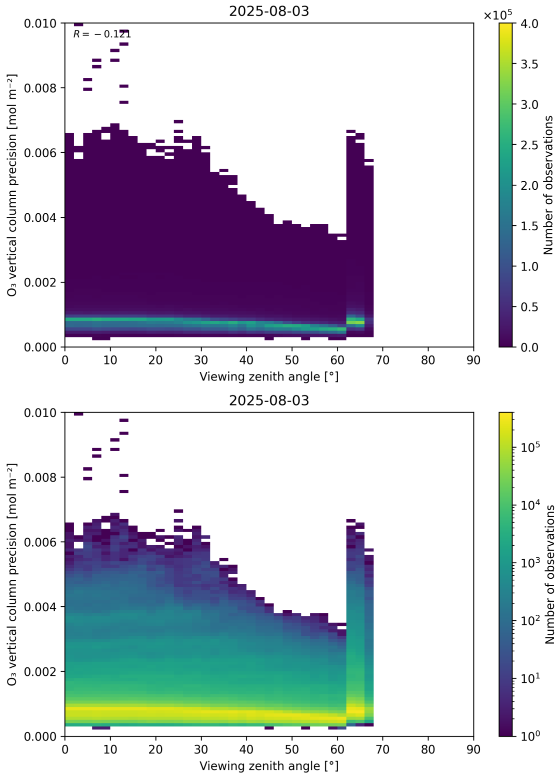
Figure 53: Scatter density plot of “Viewing zenith angle” against “O 3 vertical column precision” for 2025-08-03 to 2025-08-04.
