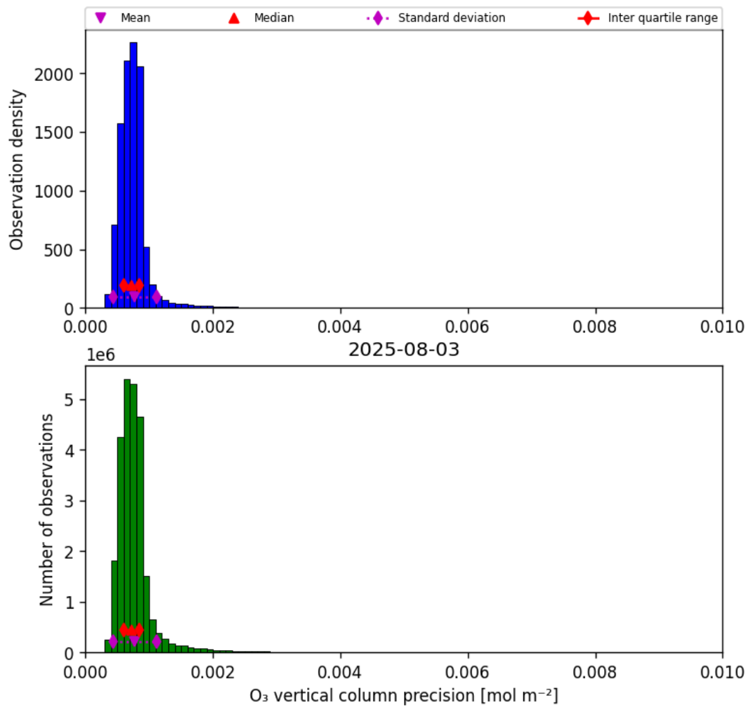
Figure 22: Histogram of “O 3 vertical column precision” for 2025-08-03 to 2025-08-04
