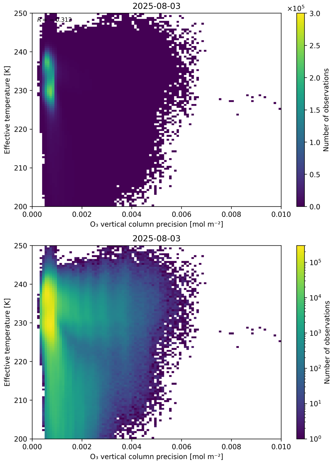
Figure 42: Scatter density plot of “O 3 vertical column precision” against “Effective temperature” for 2025-08-03 to 2025-08-04.
