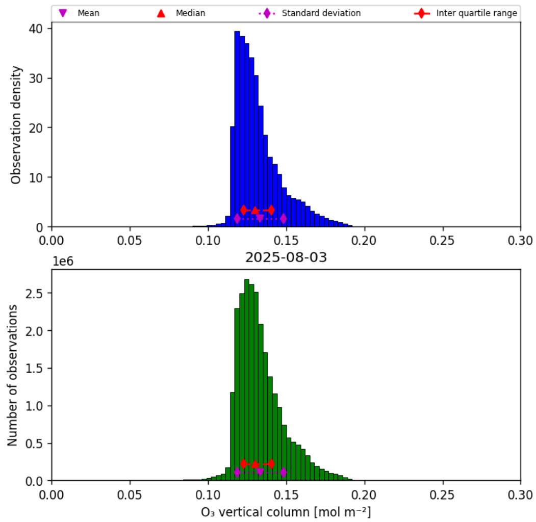
Figure 21: Histogram of “O 3 vertical column” for 2025-08-03 to 2025-08-04
