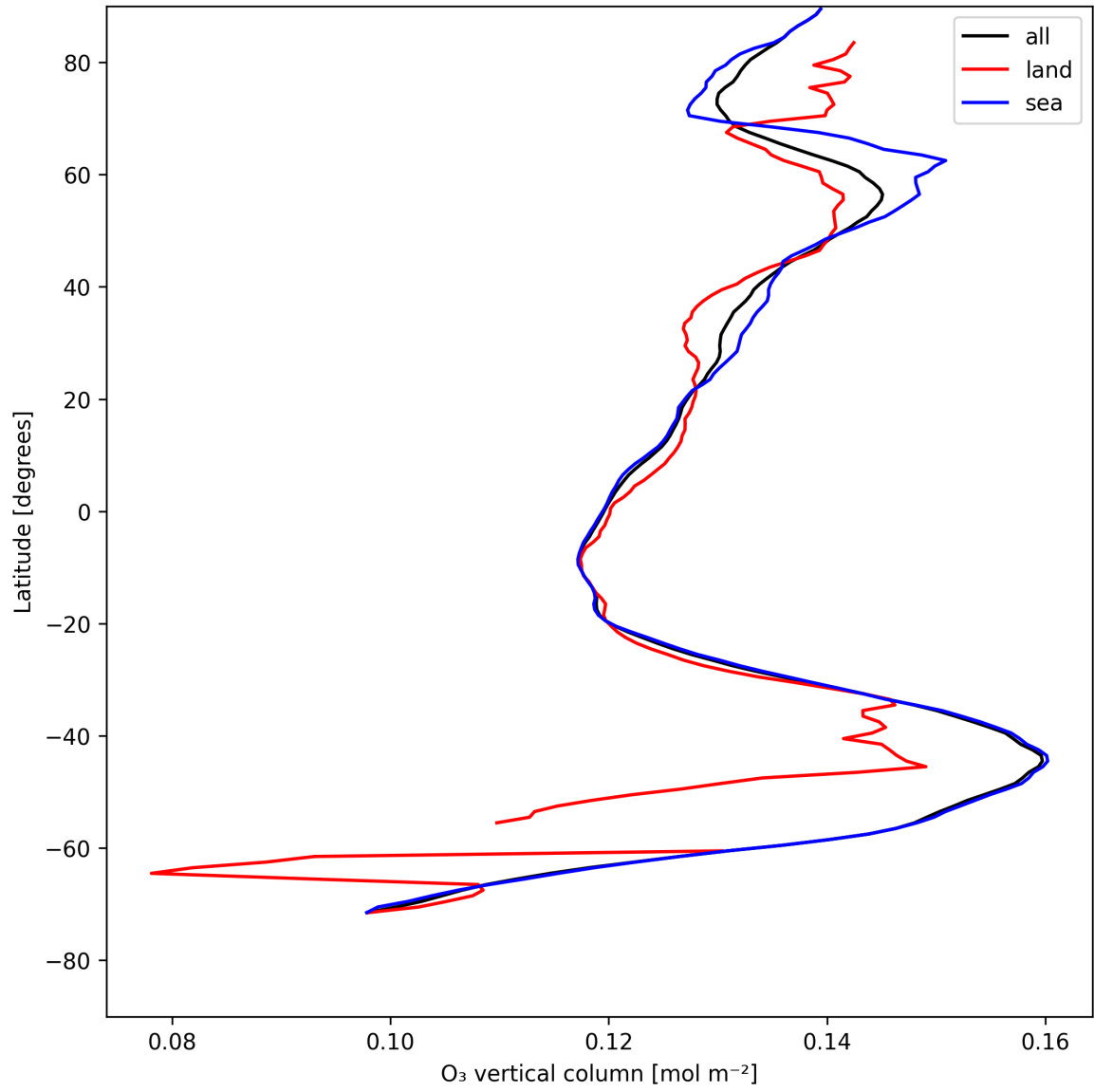
Figure 14: Zonal average of “O 3 vertical column” for 2025-08-03 to 2025-08-04.
