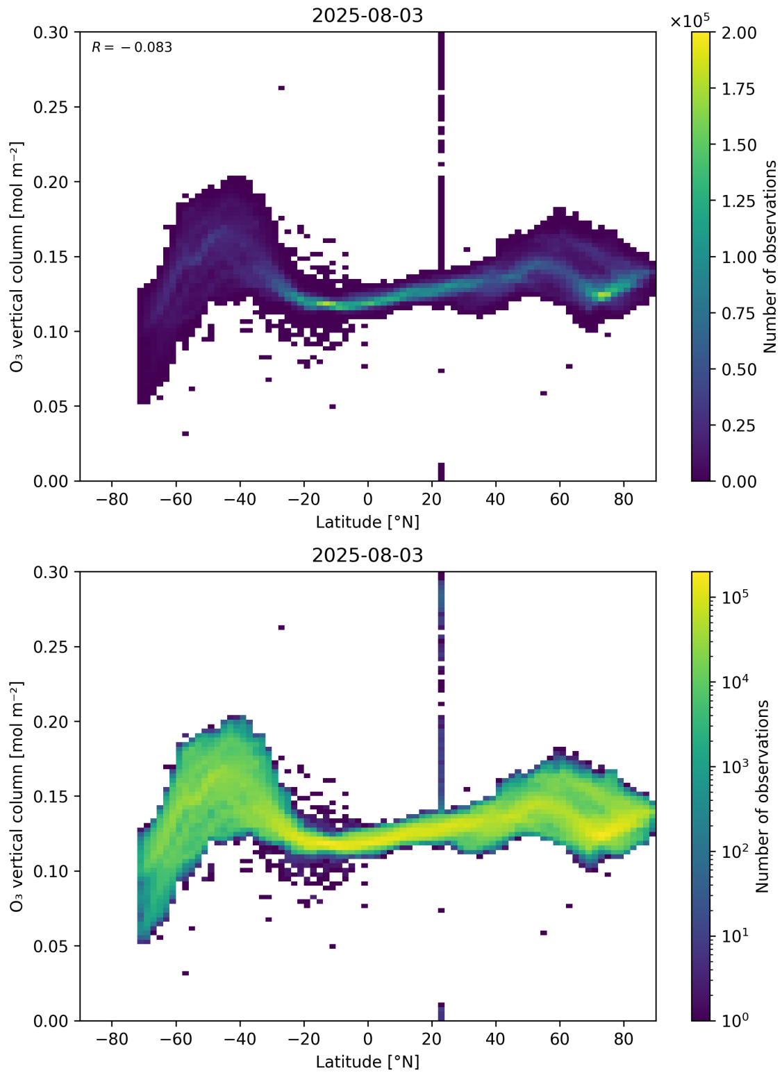
Figure 36: Scatter density plot of “Latitude” against “O 3 vertical column” for 2025-08-03 to 2025-08-04.
