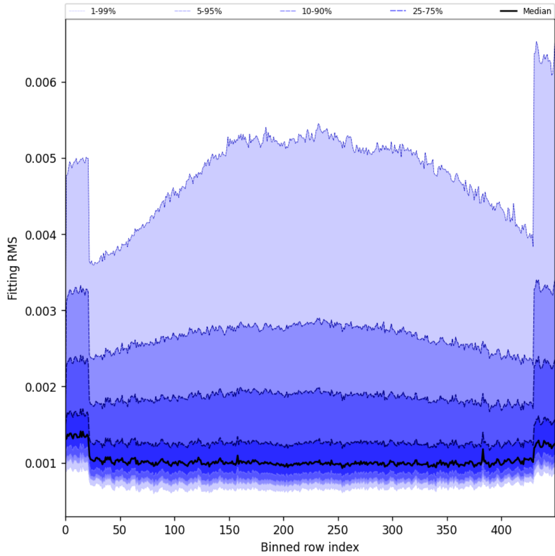
Figure 30: Along track statistics of “Fitting RMS” for 2025-08-03 to 2025-08-04
