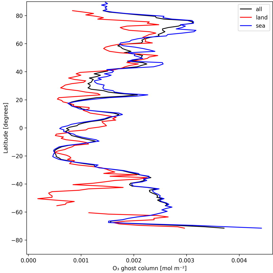
Figure 18: Zonal average of “O 3 ghost column” for 2025-08-03 to 2025-08-04.
