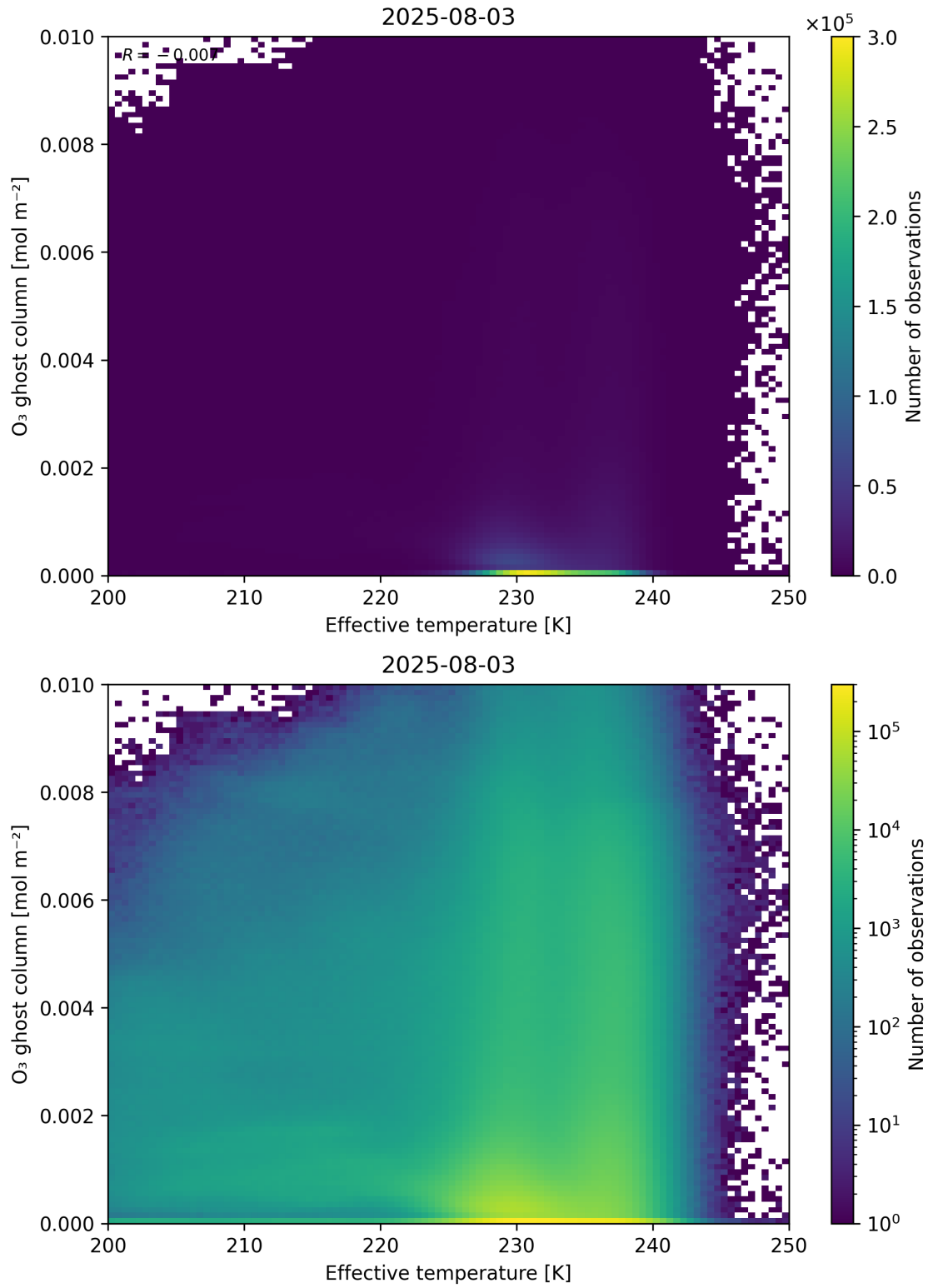
Figure 38: Scatter density plot of “Effective temperature” against “O 3 ghost column” for 2025-08-03 to 2025-08-04.
