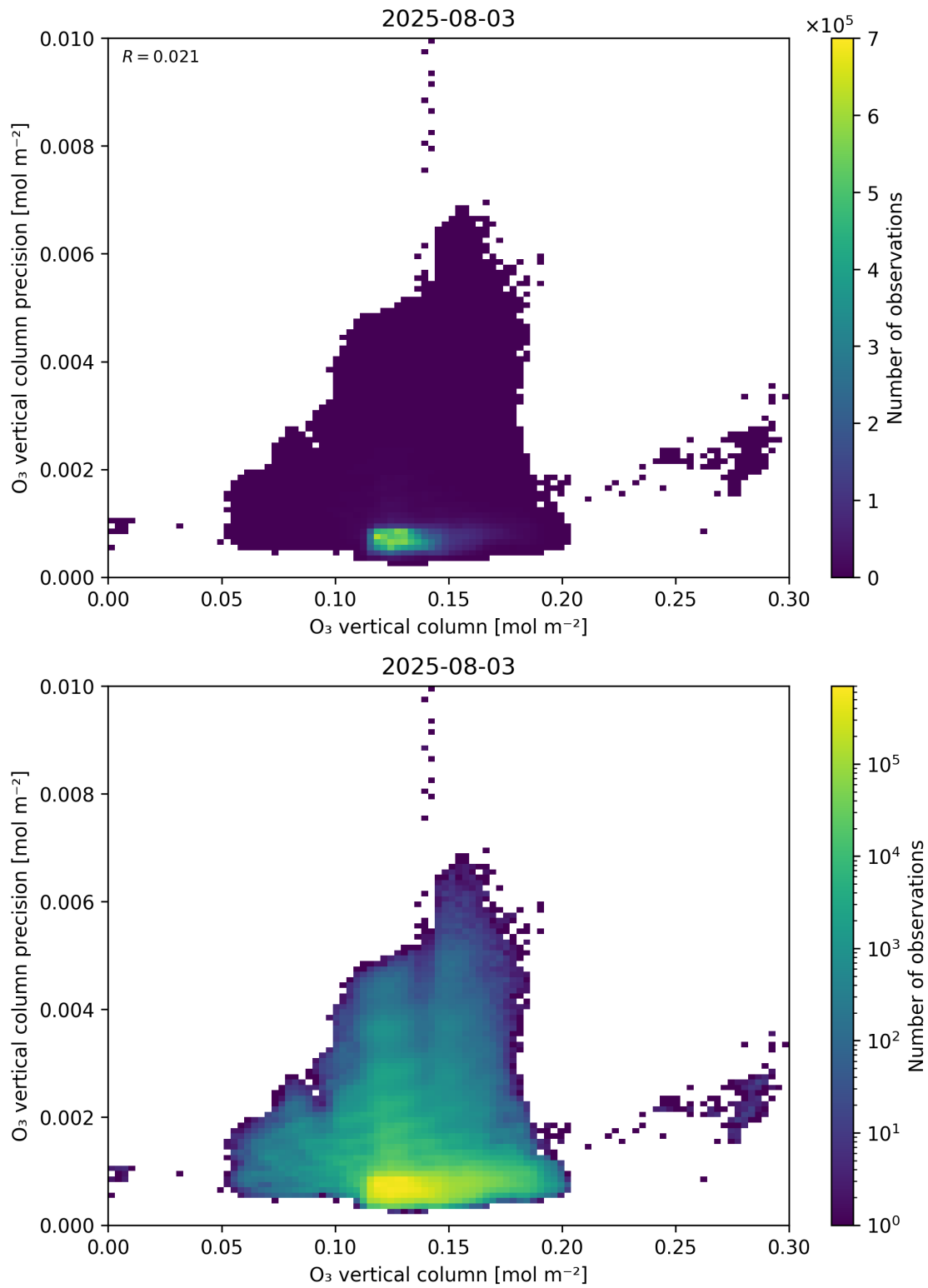
Figure 41: Scatter density plot of “O 3 vertical column” against “O 3 vertical column precision” for 2025-08-03 to 2025-08-04.
