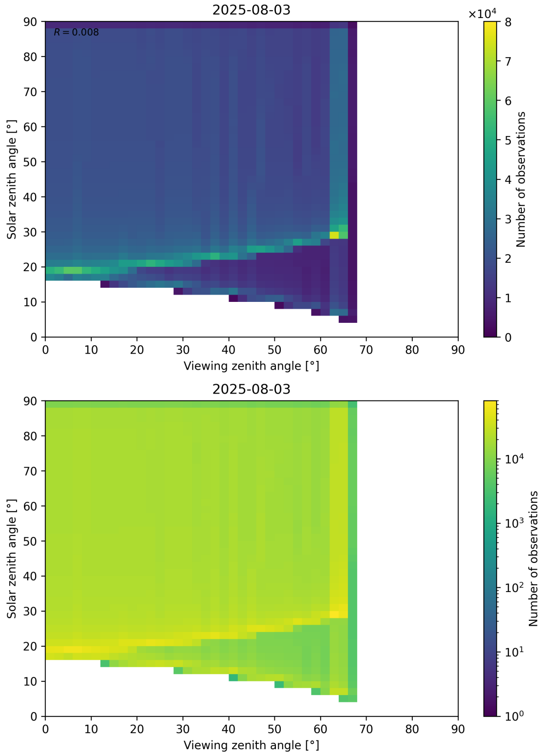
Figure 54: Scatter density plot of “Viewing zenith angle” against “Solar zenith angle” for 2025-08-03 to 2025-08-04.
