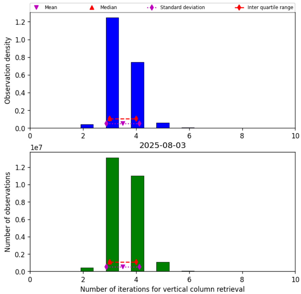
Figure 26: Histogram of “Number of iterations for vertical column retrieval” for 2025-08-03 to 2025-08-04
