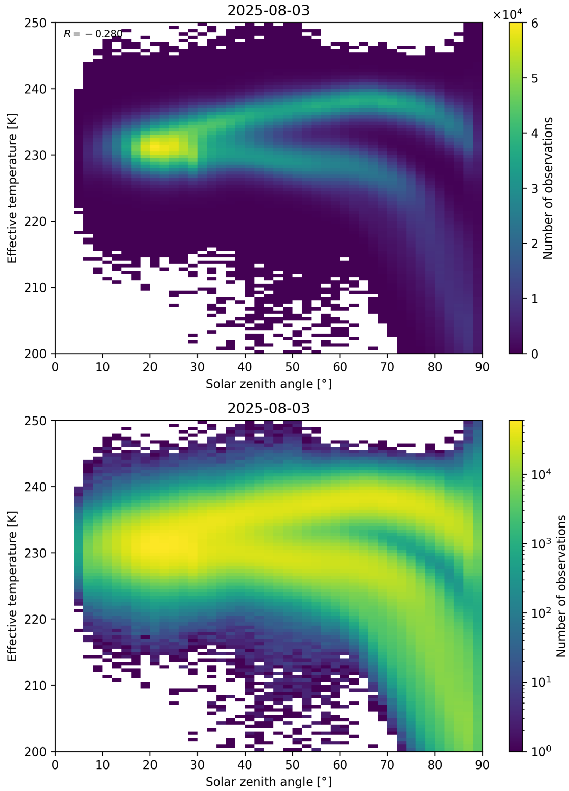
Figure 45: Scatter density plot of “Solar zenith angle” against “Effective temperature” for 2025-08-03 to 2025-08-04.
