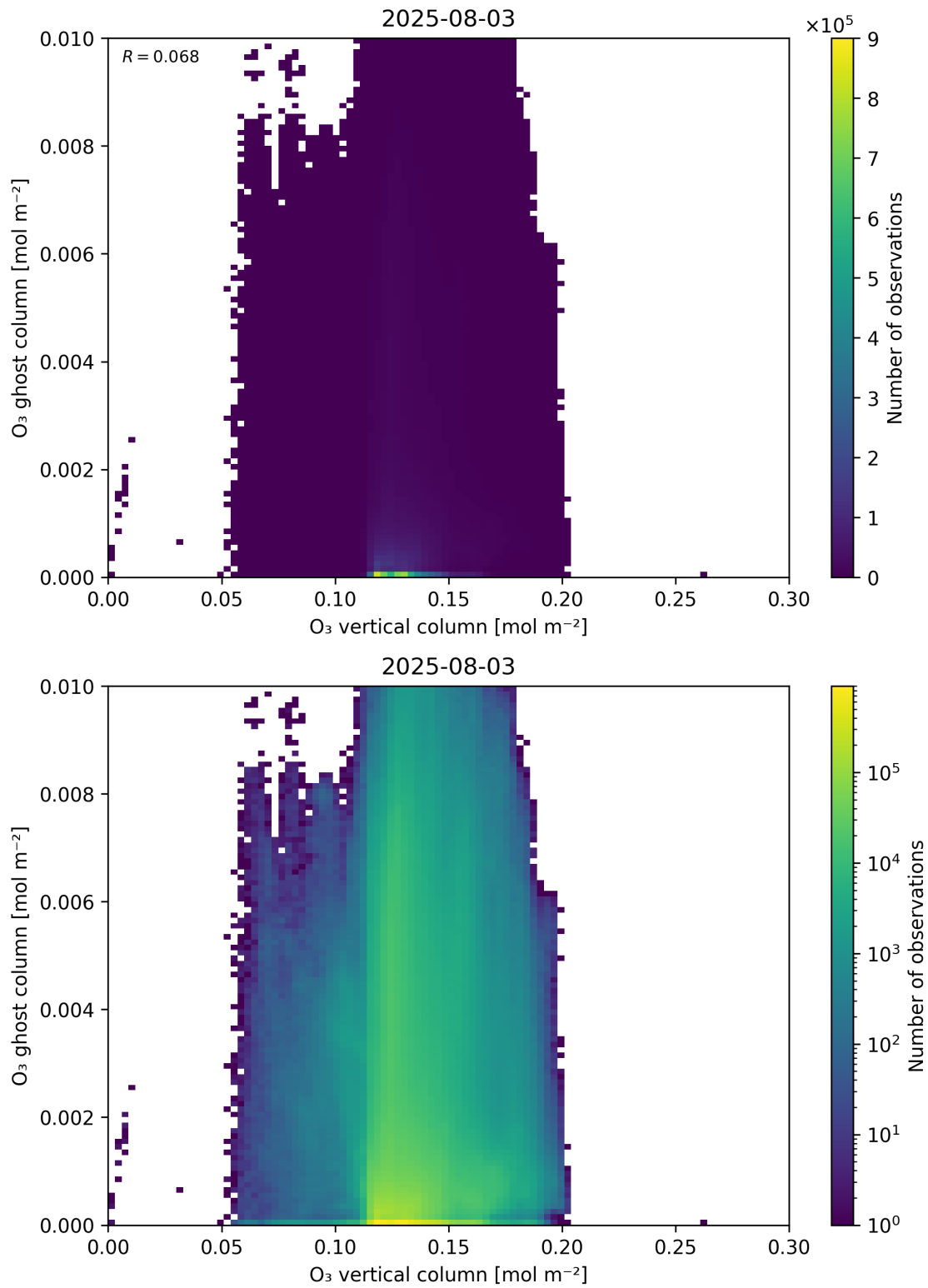
Figure 40: Scatter density plot of “O 3 vertical column” against “O 3 ghost column” for 2025-08-03 to 2025-08-04.
