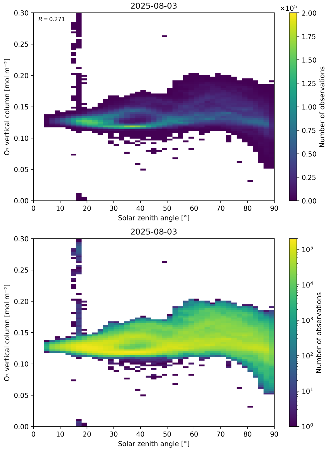
Figure 47: Scatter density plot of “Solar zenith angle” against “O 3 vertical column” for 2025-08-03 to 2025-08-04.
