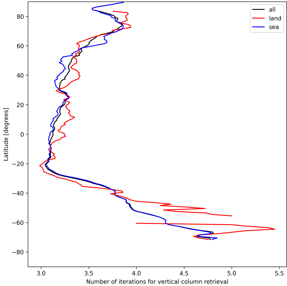
Figure 19: Zonal average of “Number of iterations for vertical column retrieval” for 2025-08-03 to 2025-08-04.
