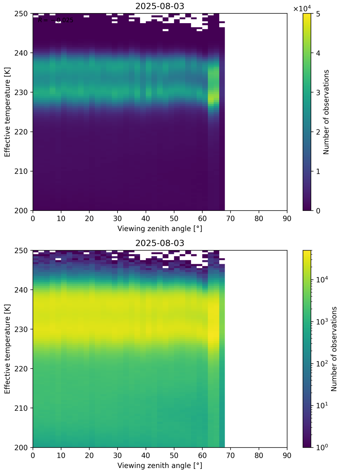
Figure 50: Scatter density plot of “Viewing zenith angle” against “Effective temperature” for 2025-08-03 to 2025-08-04.
