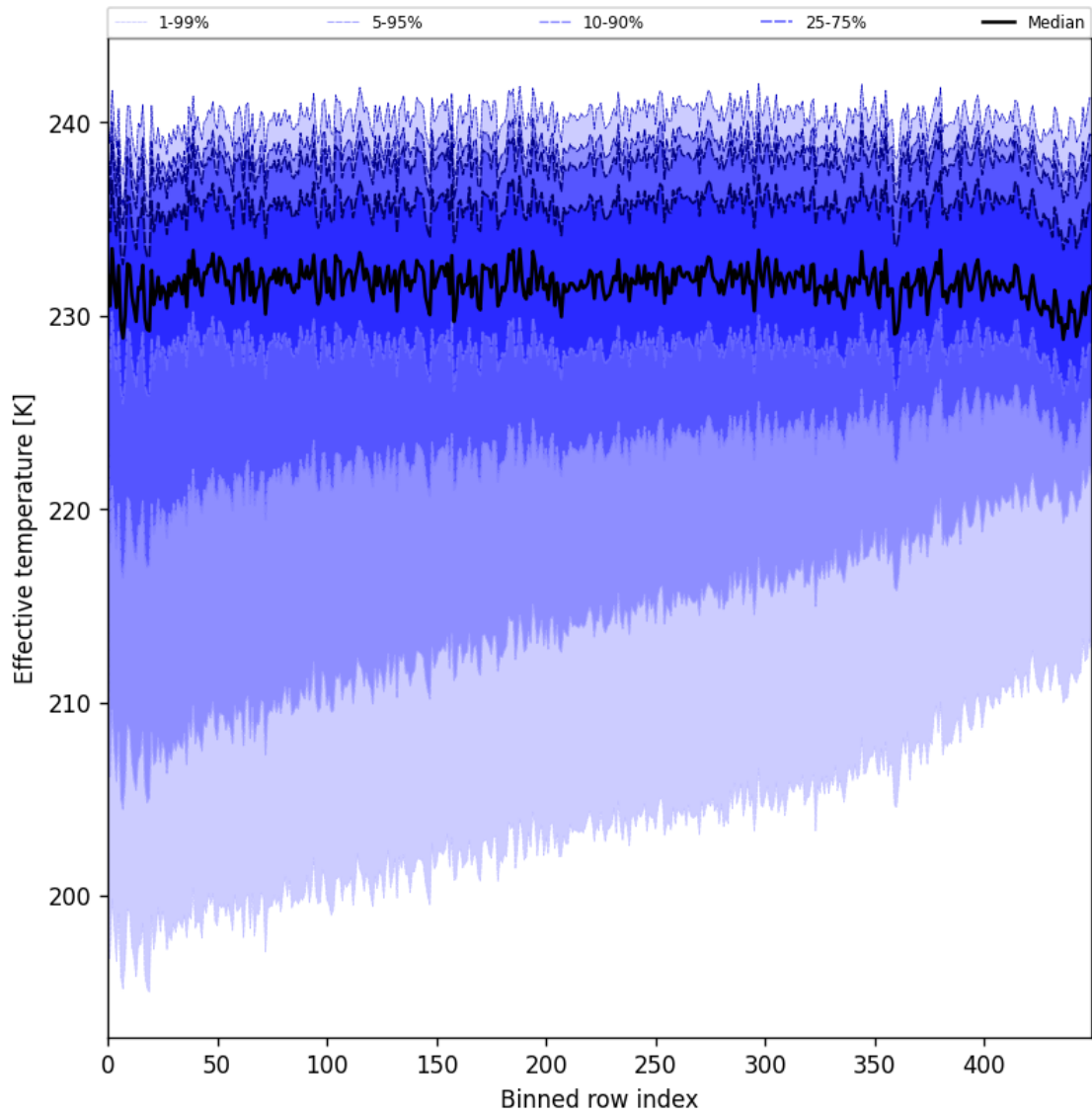
Figure 31: Along track statistics of “Effective temperature” for 2025-08-03 to 2025-08-04
