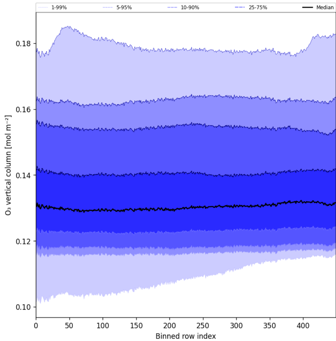
Figure 28: Along track statistics of “O 3 vertical column” for 2025-08-03 to 2025-08-04
