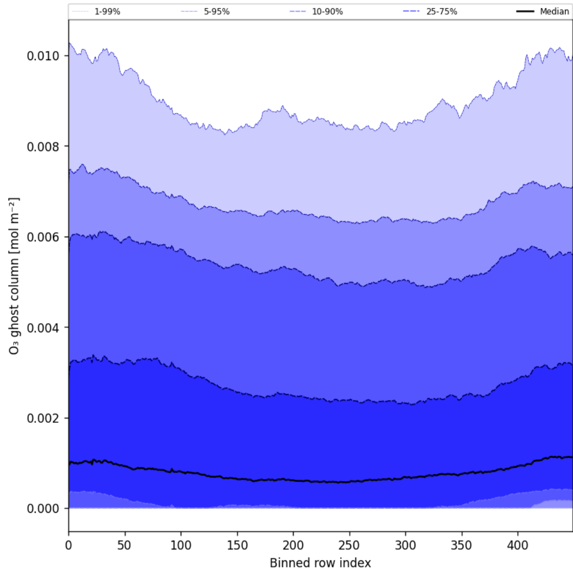
Figure 32: Along track statistics of “O 3 ghost column” for 2025-08-03 to 2025-08-04
