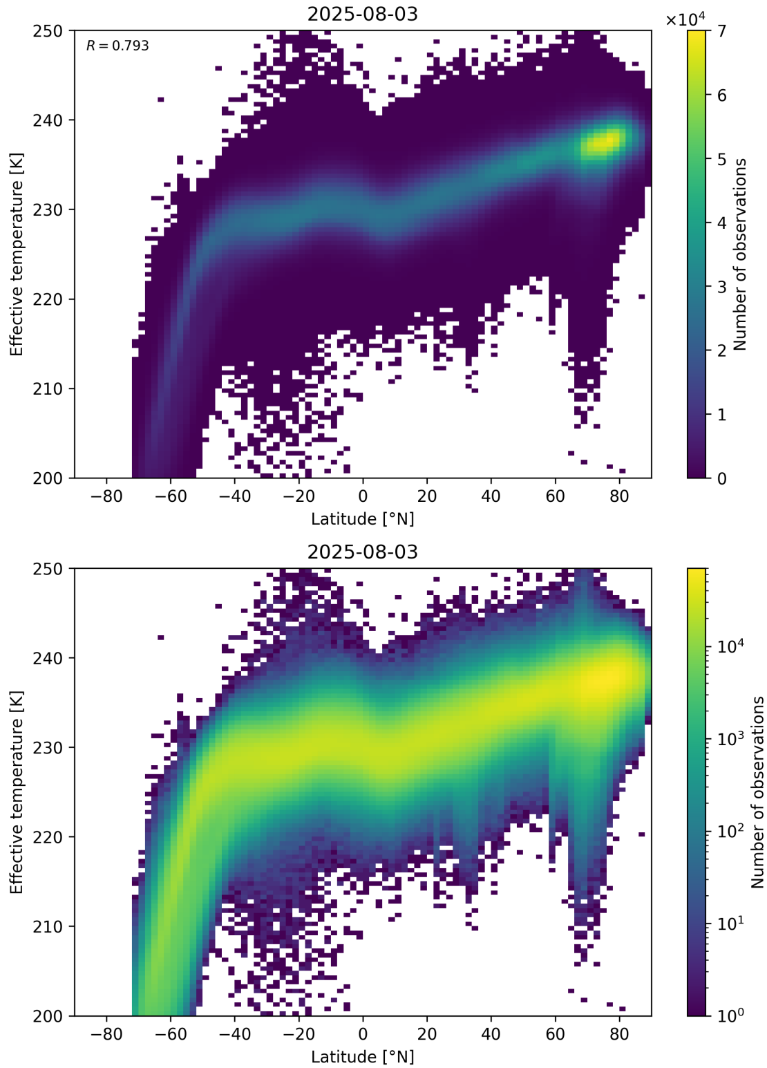
Figure 34: Scatter density plot of “Latitude” against “Effective temperature” for 2025-08-03 to 2025-08-04.
