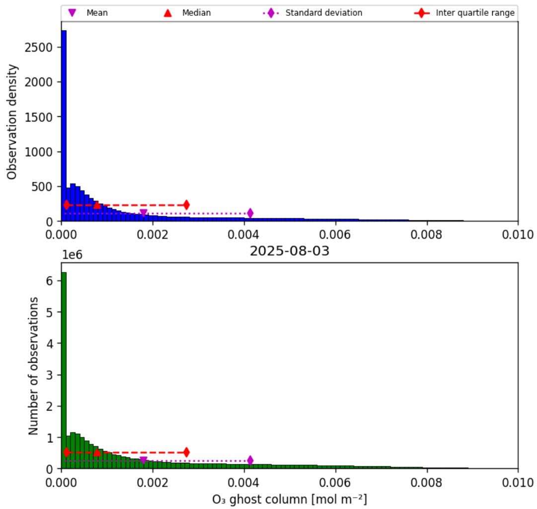
Figure 25: Histogram of “O 3 ghost column” for 2025-08-03 to 2025-08-04
