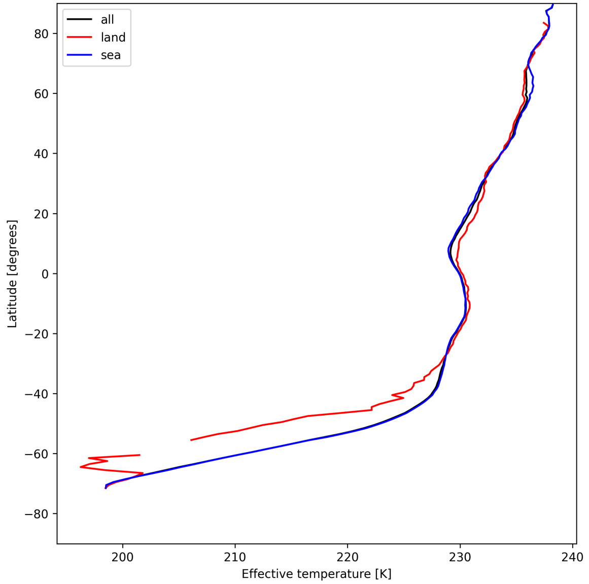
Figure 17: Zonal average of "Effective temperature" for 2025-08-03 to 2025-08-04.
