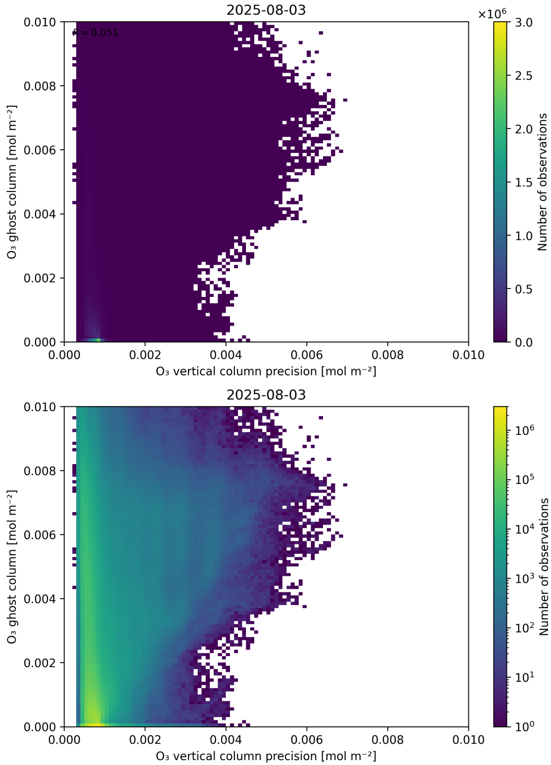
Figure 43: Scatter density plot of “O 3 vertical column precision” against “O 3 ghost column” for 2025-08-03 to 2025-08-04.
