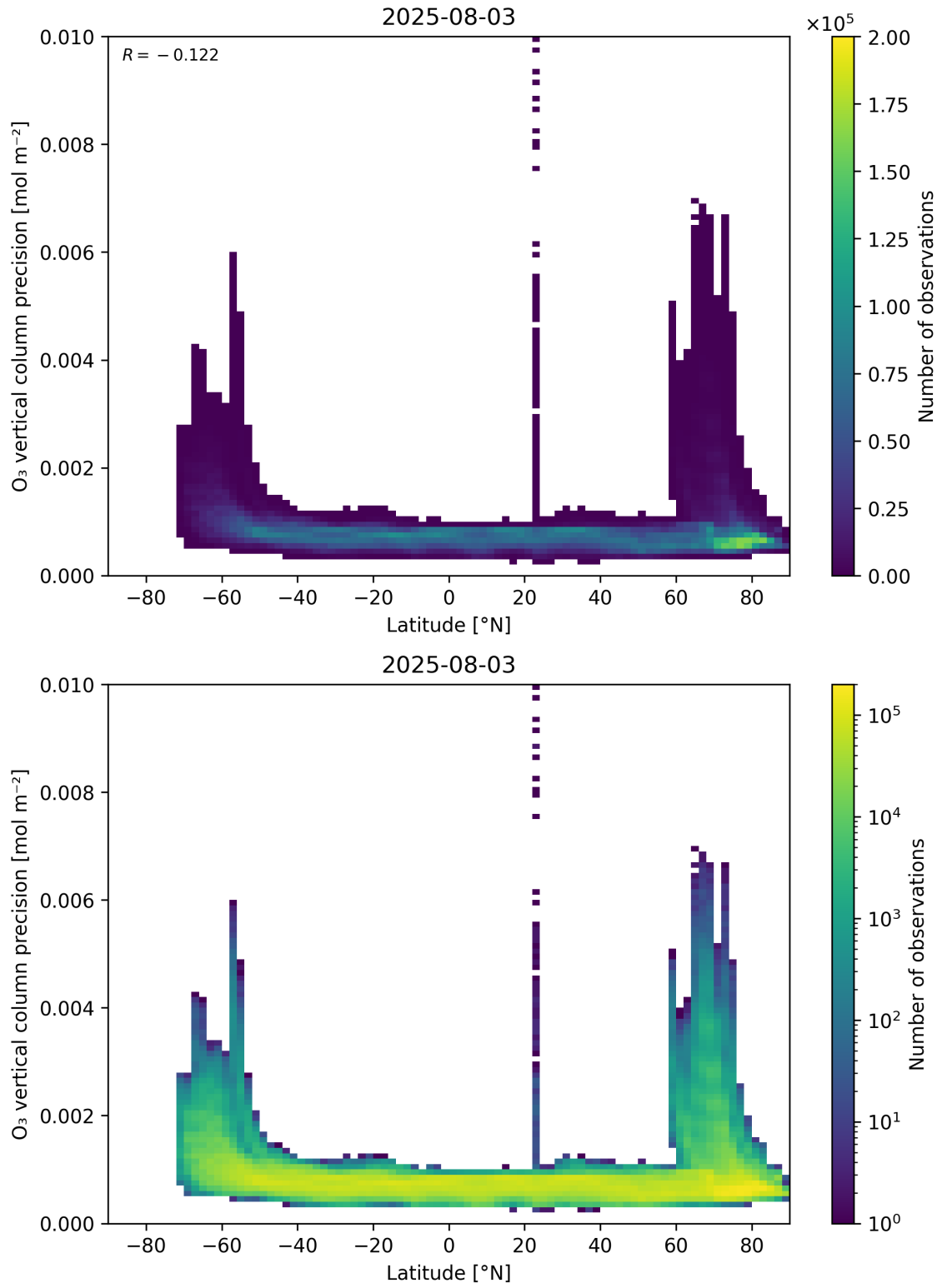
Figure 37: Scatter density plot of “Latitude” against “O 3 vertical column precision” for 2025-08-03 to 2025-08-04.
