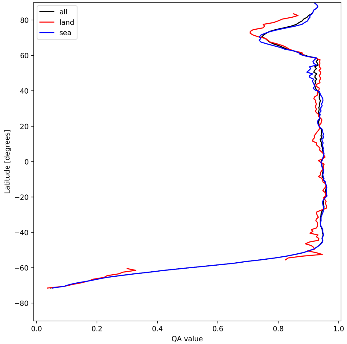
Figure 13: Zonal average of “QA value” for 2025-08-03 to 2025-08-04.
