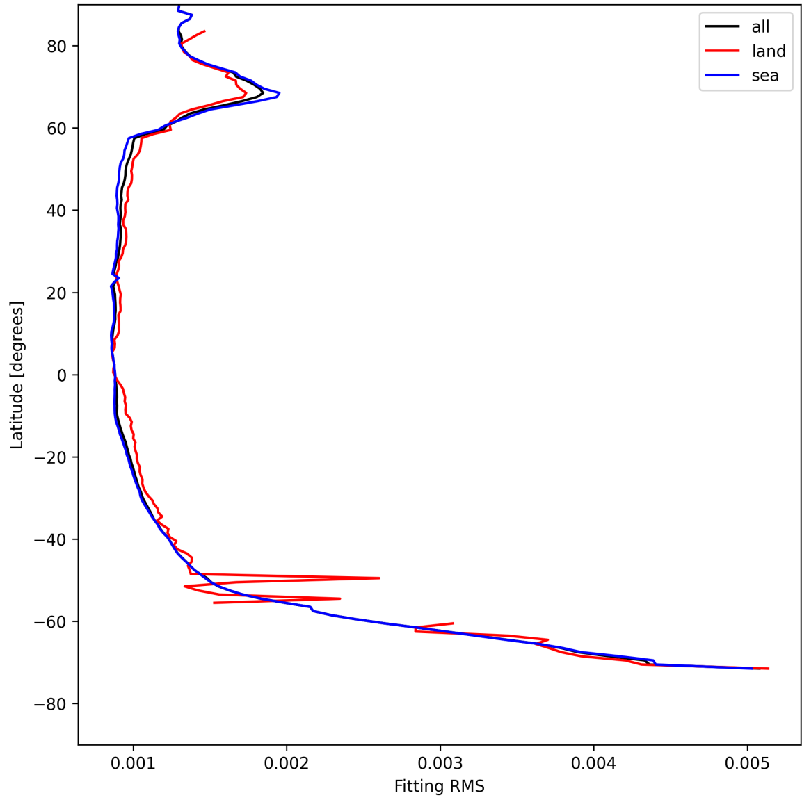
Figure 16: Zonal average of “Fitting RMS” for 2025-08-03 to 2025-08-04.
