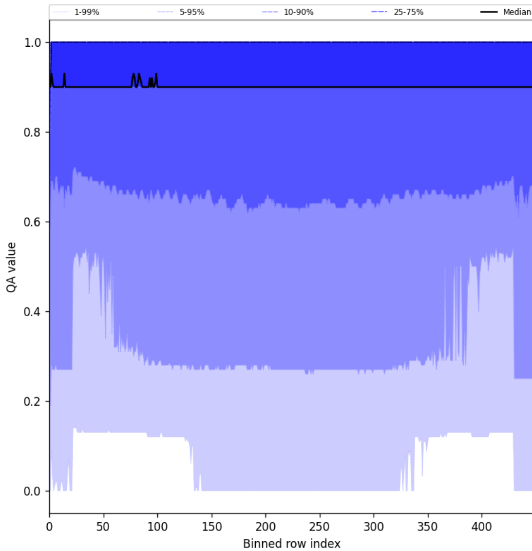
Figure 27: Along track statistics of “QA value” for 2025-08-03 to 2025-08-04
