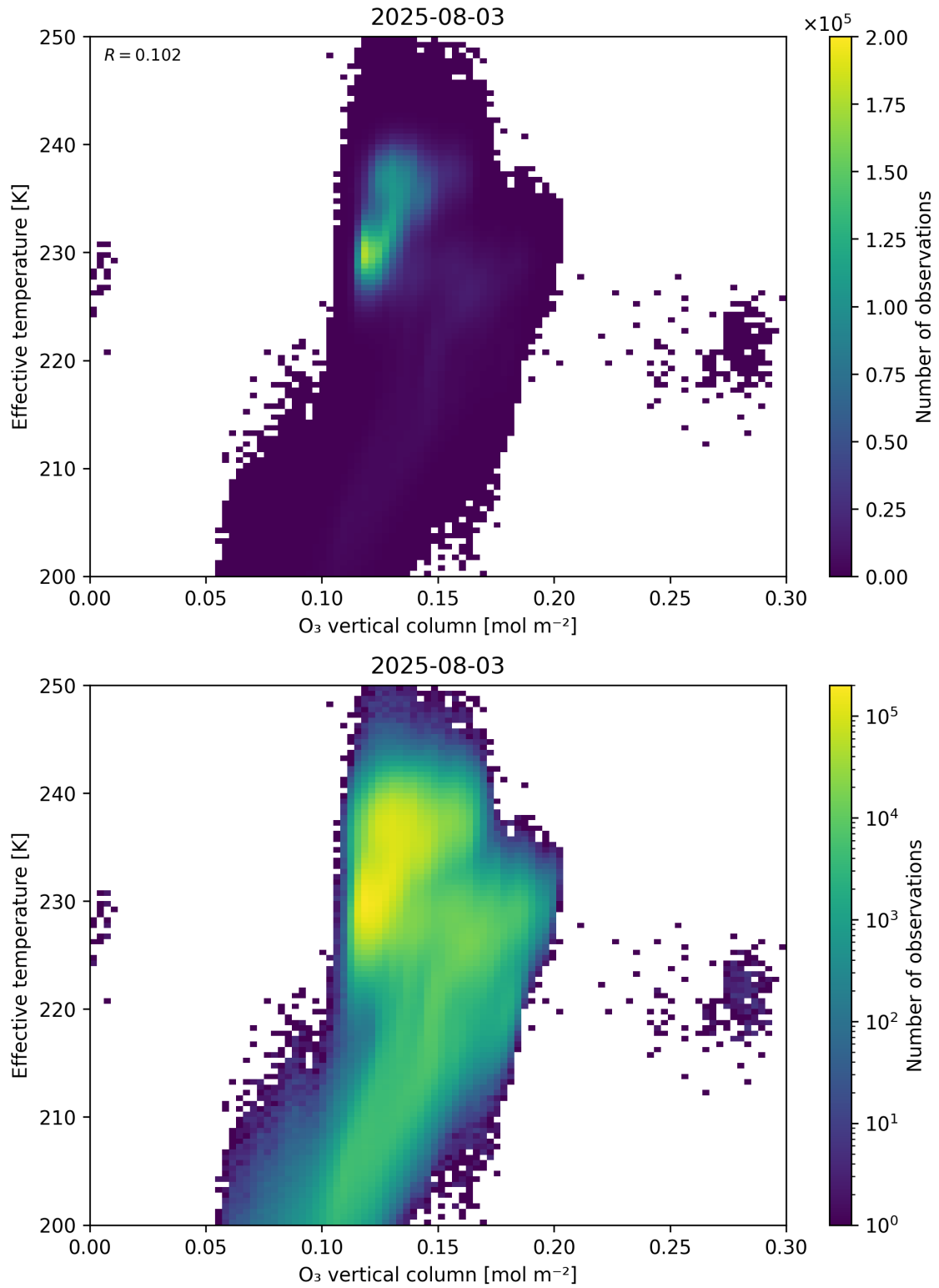
Figure 39: Scatter density plot of “O 3 vertical column” against “Effective temperature” for 2025-08-03 to 2025-08-04.
