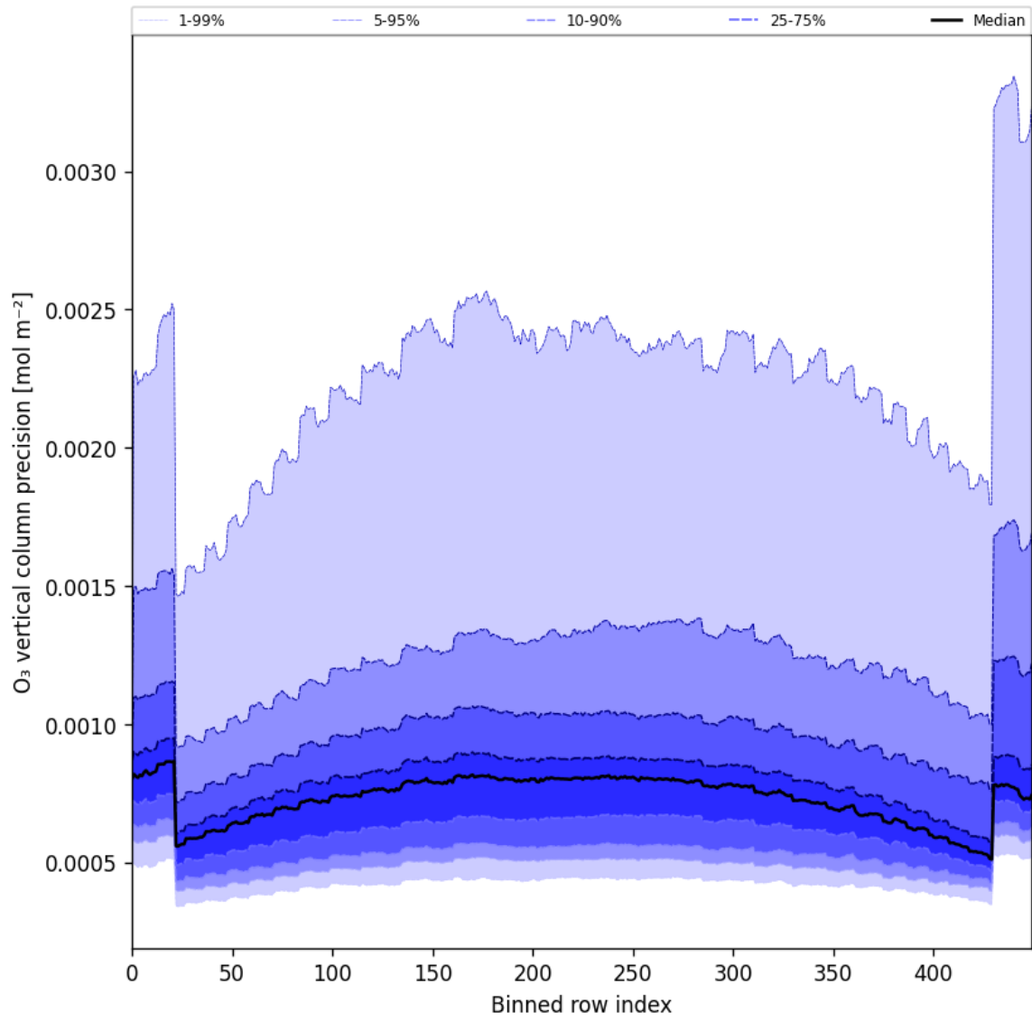
Figure 29: Along track statistics of “O 3 vertical column precision” for 2025-08-03 to 2025-08-04
