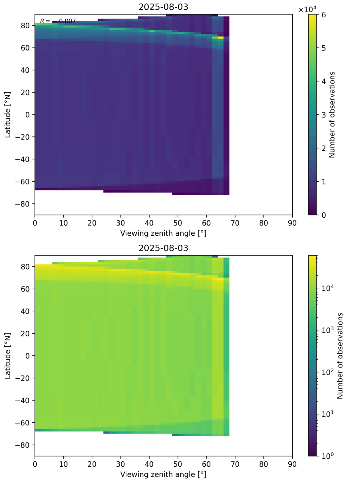
Figure 49: Scatter density plot of “Viewing zenith angle” against “Latitude” for 2025-08-03 to 2025-08-04.
