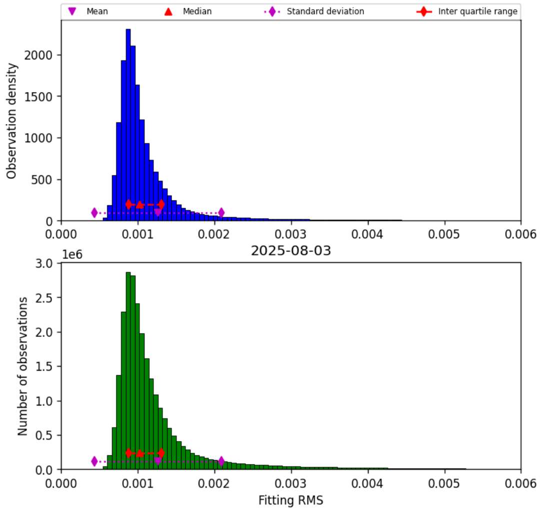
Figure 23: Histogram of “Fitting RMS” for 2025-08-03 to 2025-08-04
