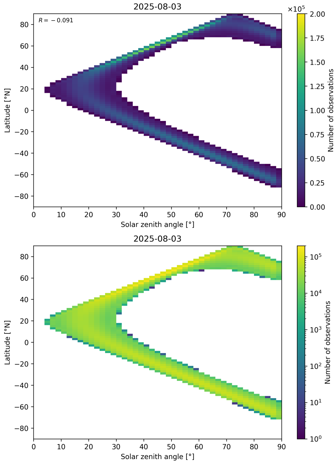
Figure 44: Scatter density plot of “Solar zenith angle” against “Latitude” for 2025-08-03 to 2025-08-04.
