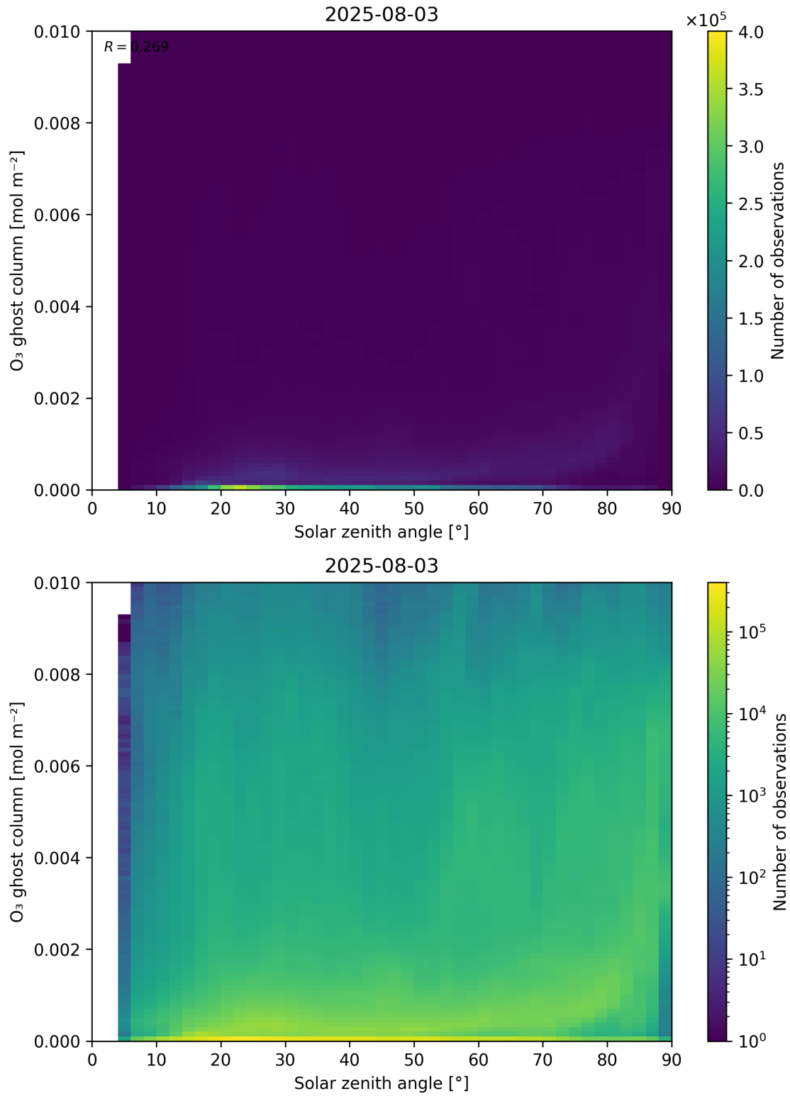
Figure 46: Scatter density plot of “Solar zenith angle” against “O 3 ghost column” for 2025-08-03 to 2025-08-04.
