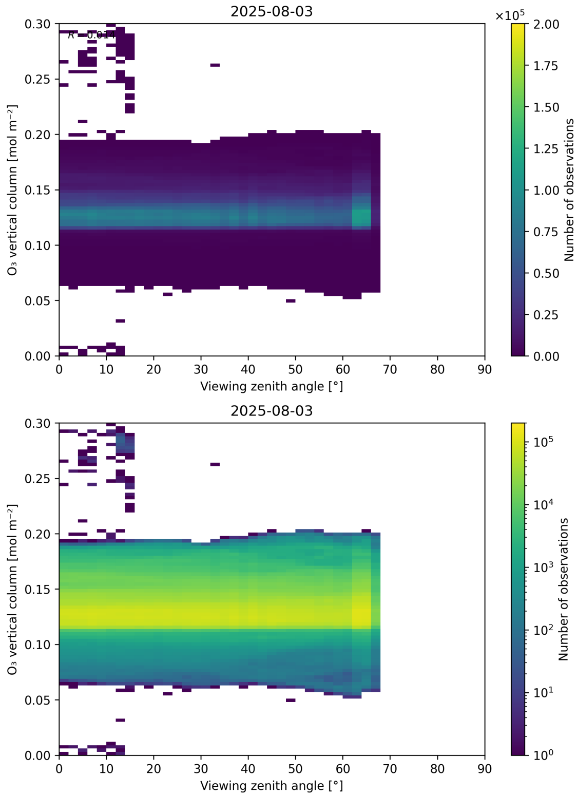
Figure 52: Scatter density plot of “Viewing zenith angle” against “O 3 vertical column” for 2025-08-03 to 2025-08-04.
