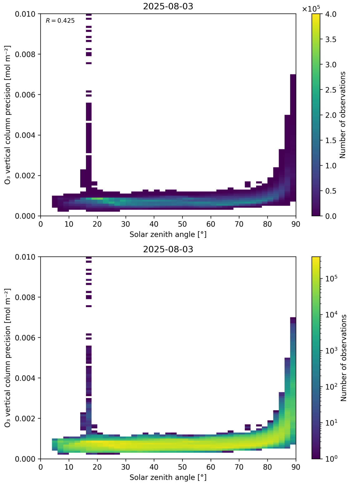
Figure 48: Scatter density plot of “Solar zenith angle” against “O 3 vertical column precision” for 2025-08-03 to 2025-08-04.
