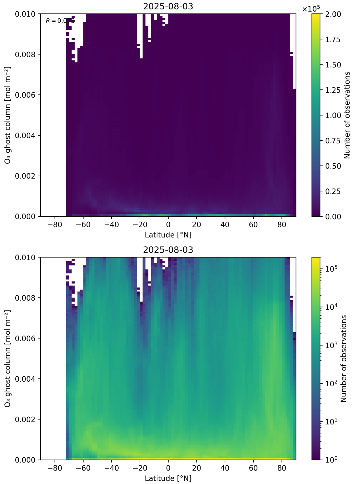
Figure 35: Scatter density plot of “Latitude” against “O 3 ghost column” for 2025-08-03 to 2025-08-04.
