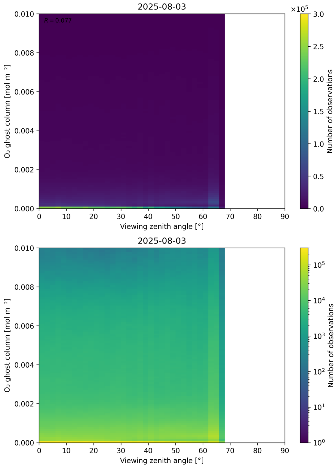
Figure 51: Scatter density plot of “Viewing zenith angle” against “O 3 ghost column” for 2025-08-03 to 2025-08-04.
