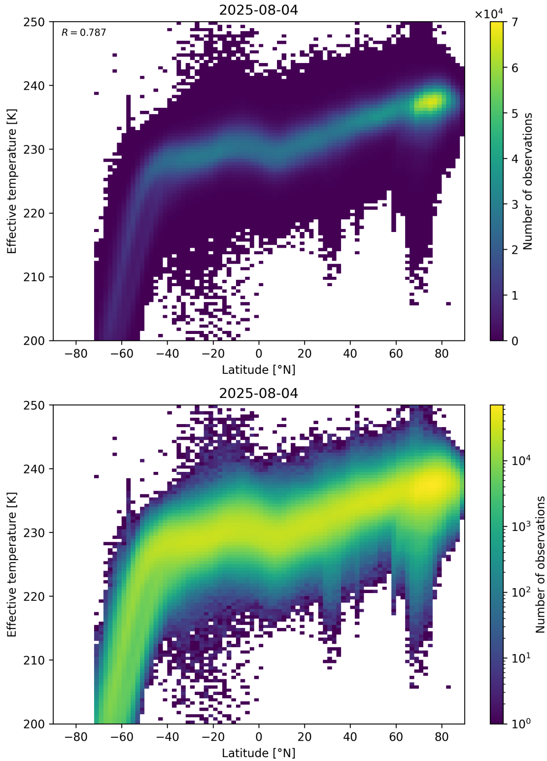
Figure 34: Scatter density plot of “Latitude” against “Effective temperature” for 2025-08-04 to 2025-08-05.
