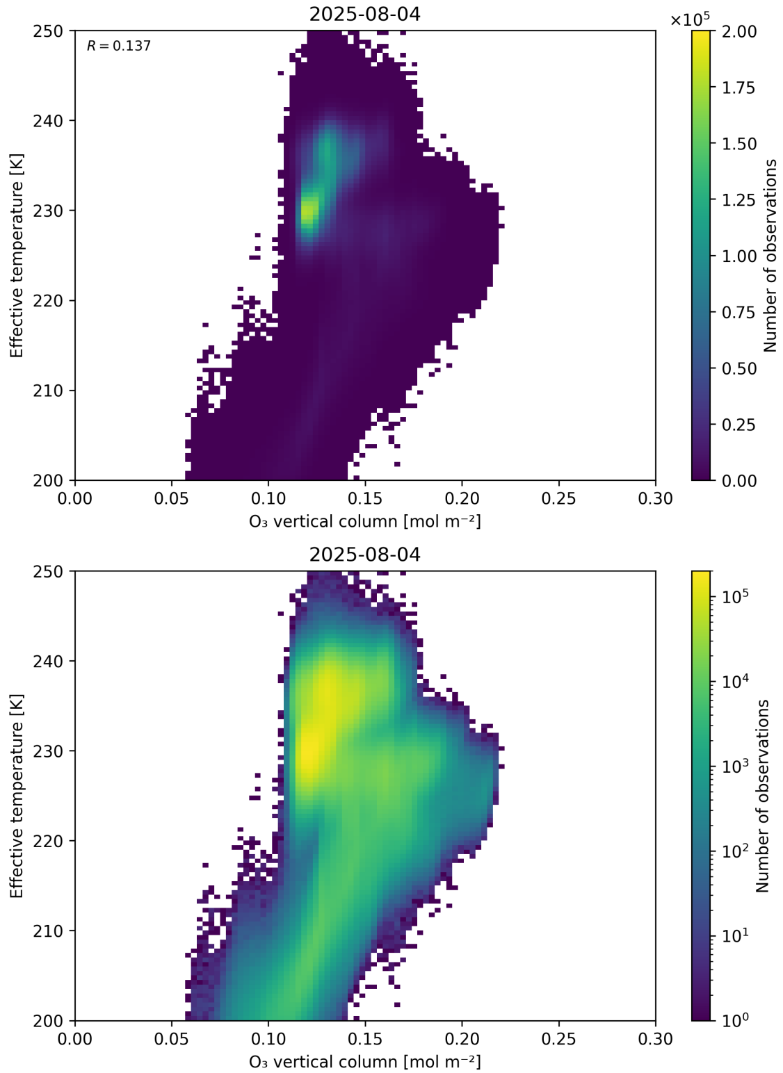
Figure 39: Scatter density plot of “O 3 vertical column” against “Effective temperature” for 2025-08-04 to 2025-08-05.
