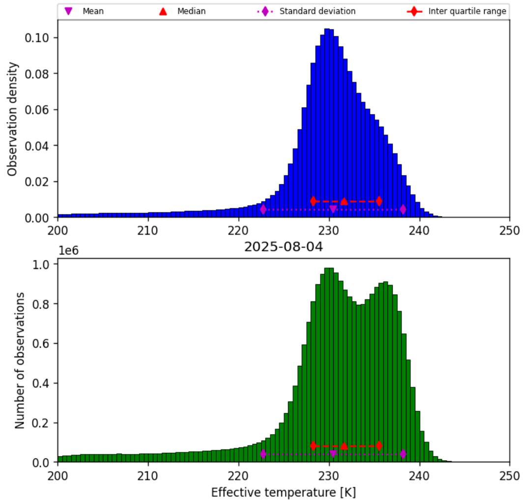
Figure 24: Histogram of “Effective temperature” for 2025-08-04 to 2025-08-05
