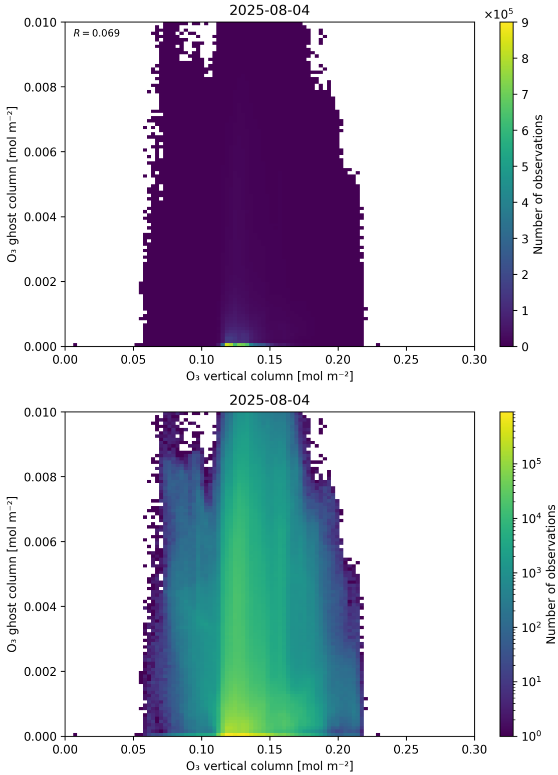
Figure 40: Scatter density plot of “O 3 vertical column” against “O 3 ghost column” for 2025-08-04 to 2025-08-05.
