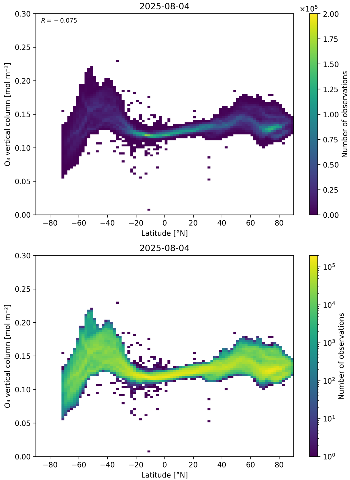
Figure 36: Scatter density plot of “Latitude” against “O 3 vertical column” for 2025-08-04 to 2025-08-05.
