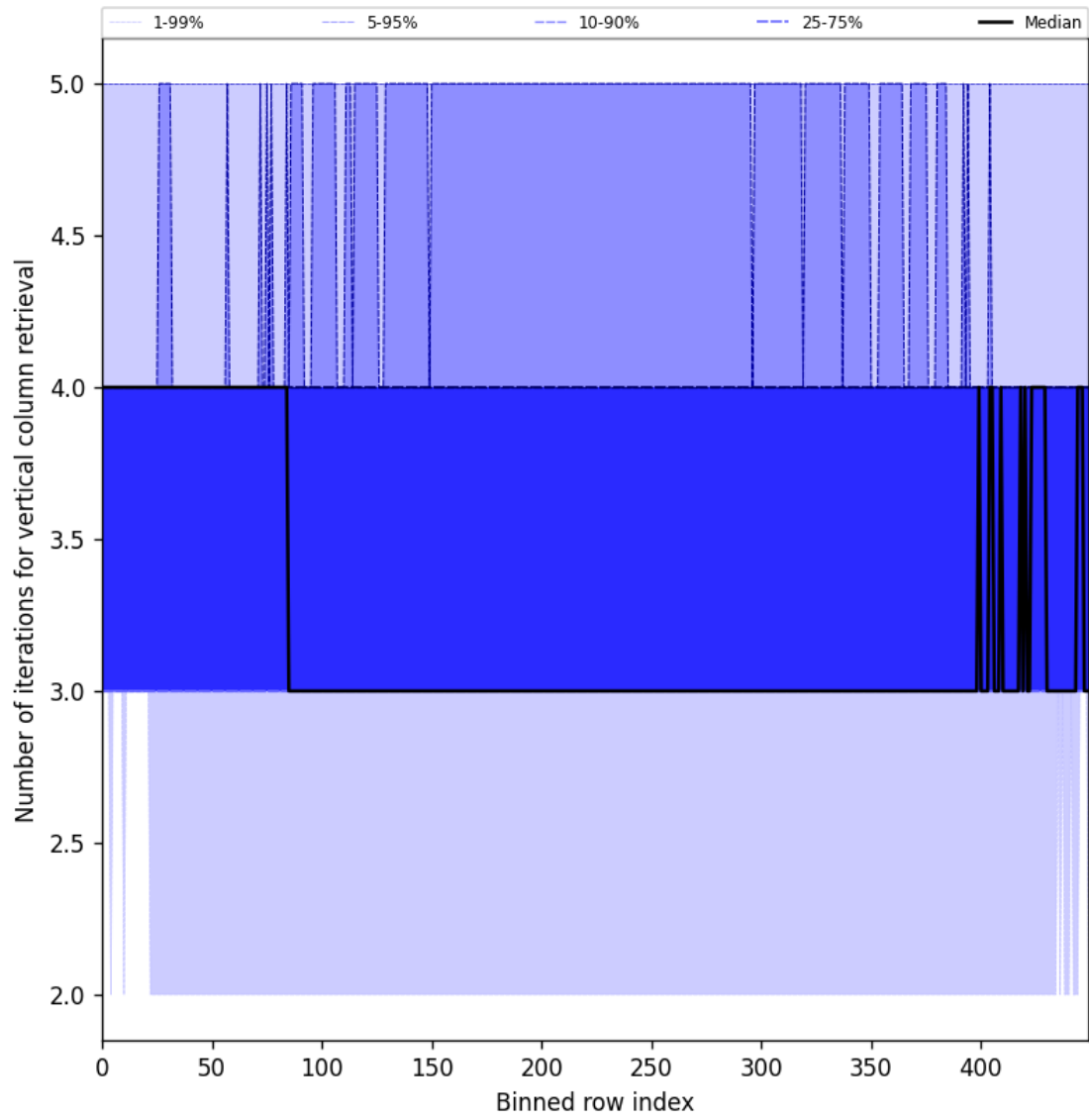
Figure 33: Along track statistics of “Number of iterations for vertical column retrieval” for 2025-08-04 to 2025-08-05
