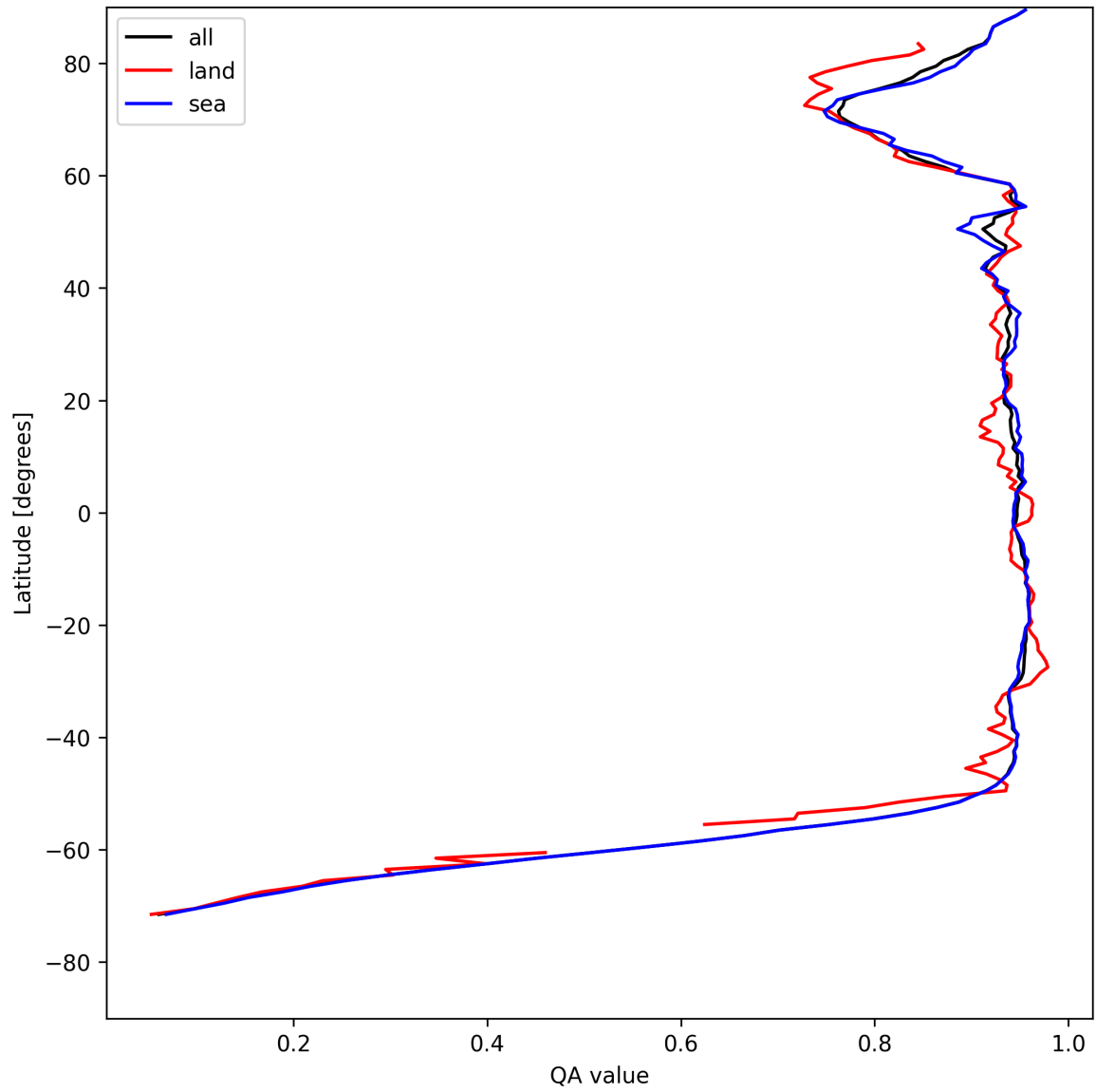
Figure 13: Zonal average of “QA value” for 2025-08-04 to 2025-08-05.
