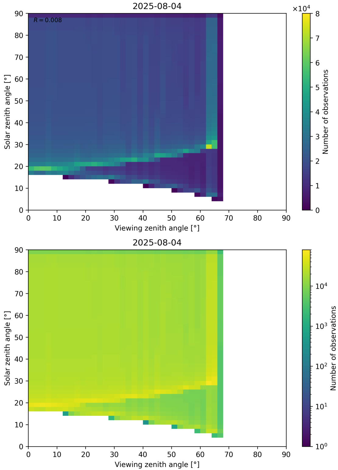
Figure 54: Scatter density plot of “Viewing zenith angle” against “Solar zenith angle” for 2025-08-04 to 2025-08-05.
