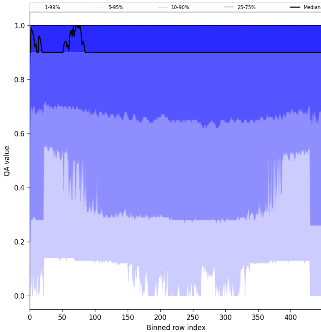
Figure 27: Along track statistics of “QA value” for 2025-08-04 to 2025-08-05
