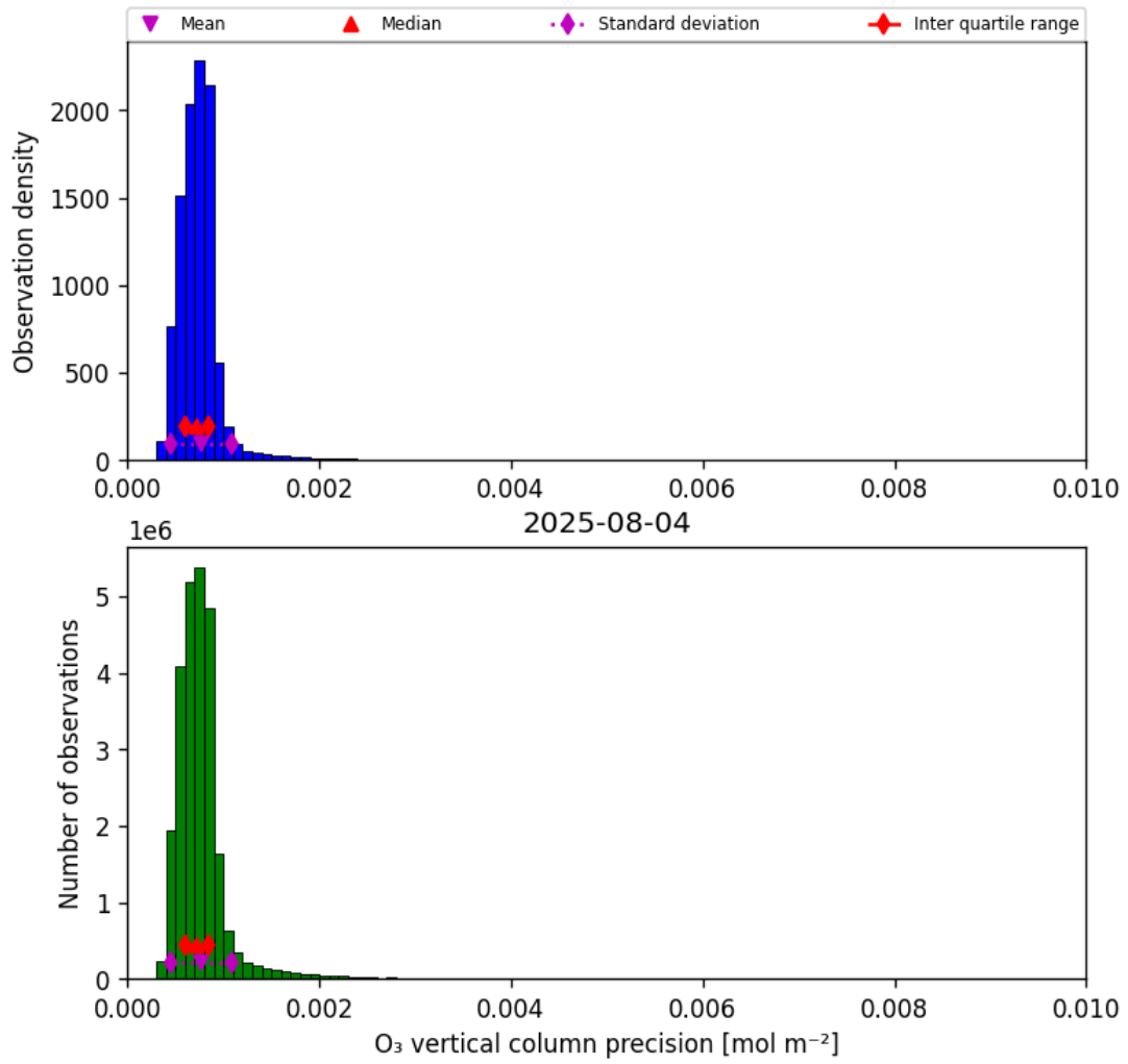
Figure 22: Histogram of “O 3 vertical column precision” for 2025-08-04 to 2025-08-05
