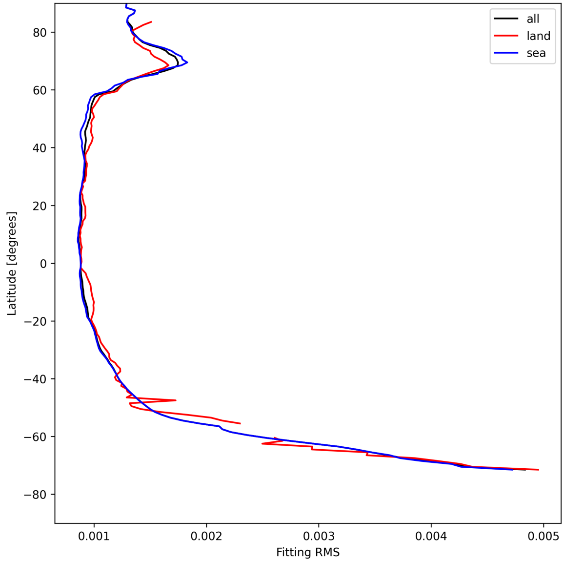
Figure 16: Zonal average of “Fitting RMS” for 2025-08-04 to 2025-08-05.
