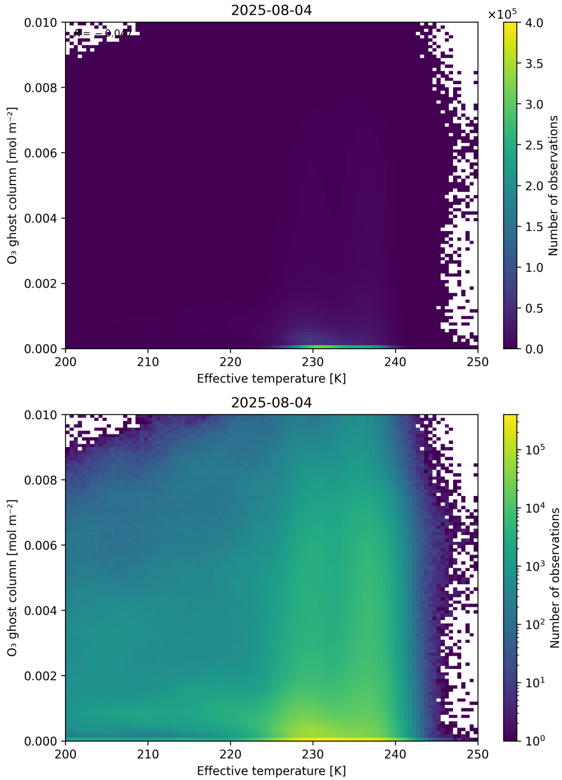
Figure 38: Scatter density plot of “Effective temperature” against “O 3 ghost column” for 2025-08-04 to 2025-08-05.
