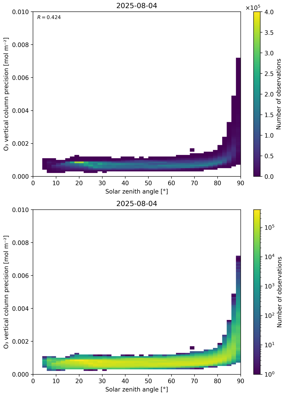
Figure 48: Scatter density plot of “Solar zenith angle” against “O 3 vertical column precision” for 2025-08-04 to 2025-08-05.
