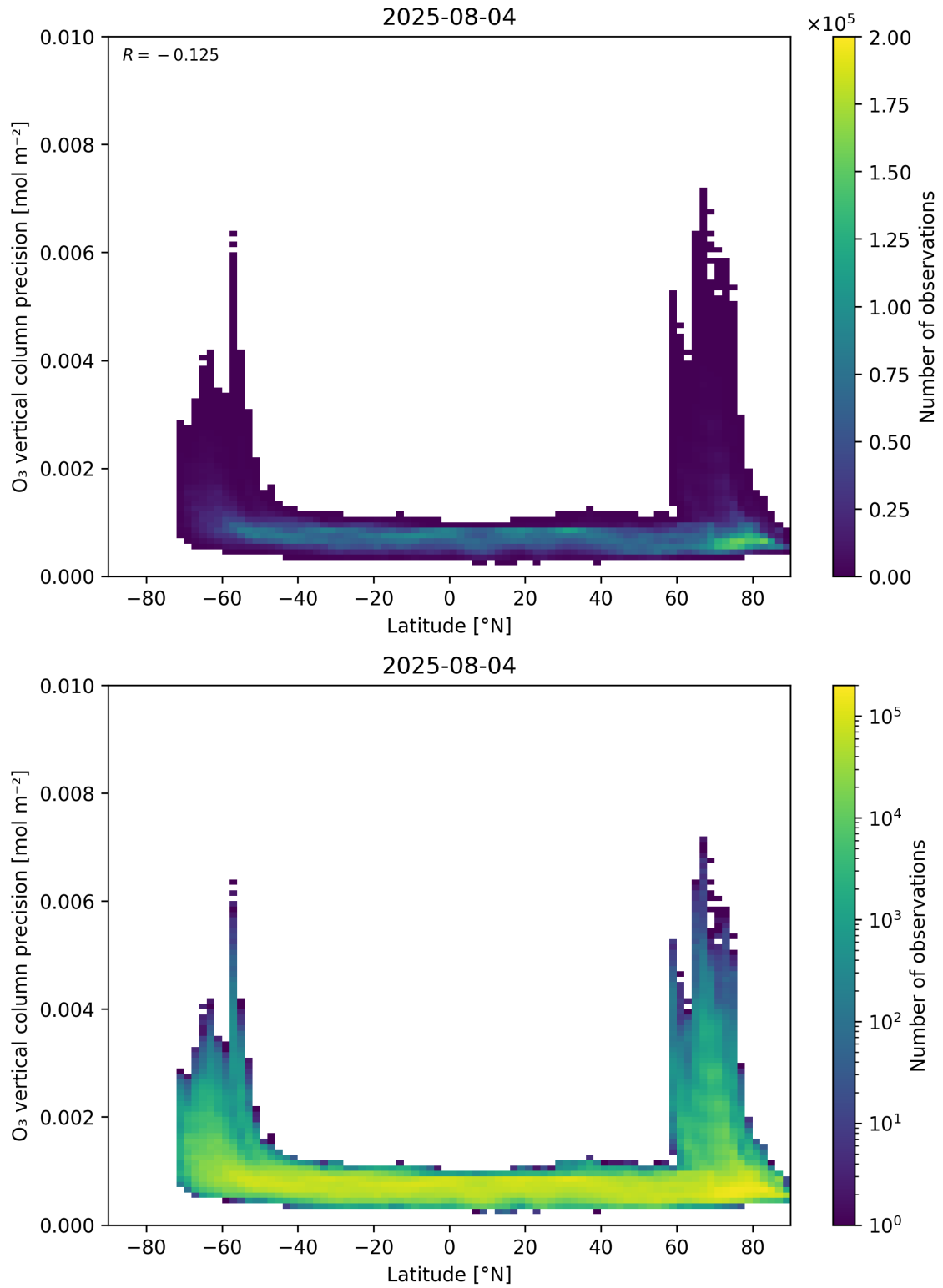
Figure 37: Scatter density plot of “Latitude” against “O 3 vertical column precision” for 2025-08-04 to 2025-08-05.
