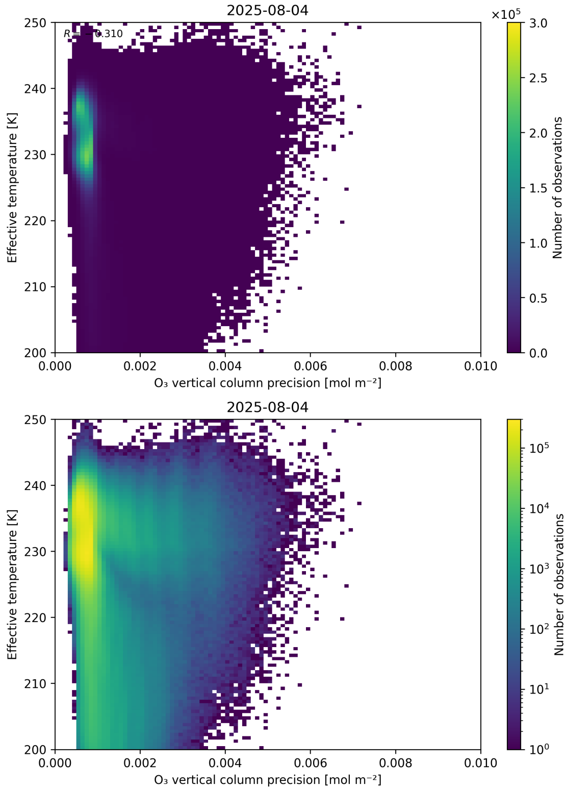
Figure 42: Scatter density plot of “O 3 vertical column precision” against “Effective temperature” for 2025-08-04 to 2025-08-05.
