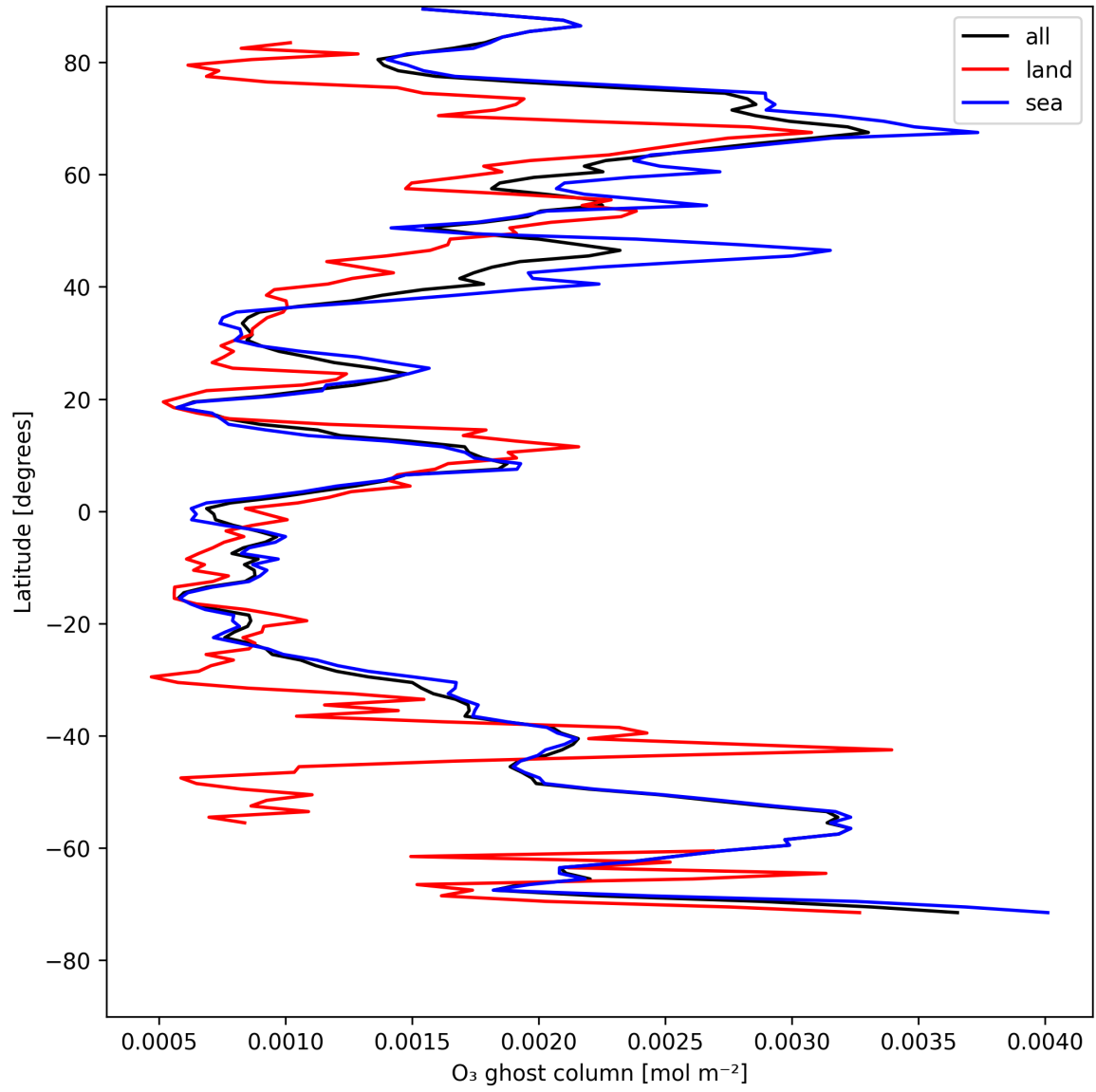
Figure 18: Zonal average of "O 3 ghost column" for 2025-08-04 to 2025-08-05.
