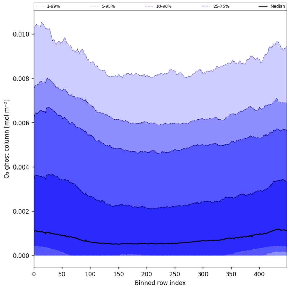
Figure 32: Along track statistics of “O 3 ghost column” for 2025-08-04 to 2025-08-05
