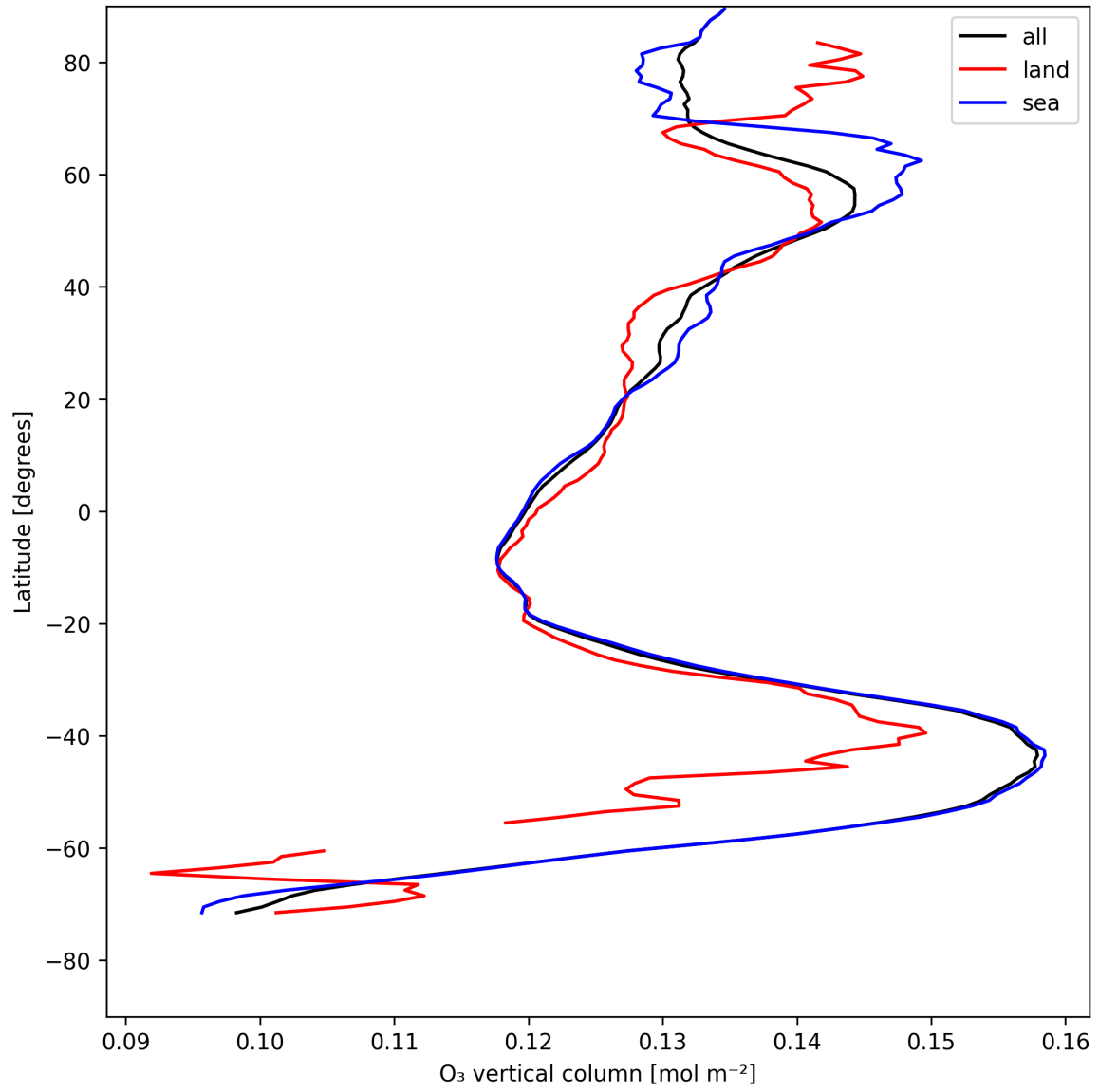
Figure 14: Zonal average of “O 3 vertical column” for 2025-08-04 to 2025-08-05.
