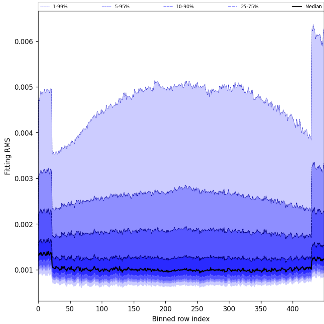
Figure 30: Along track statistics of “Fitting RMS” for 2025-08-04 to 2025-08-05
