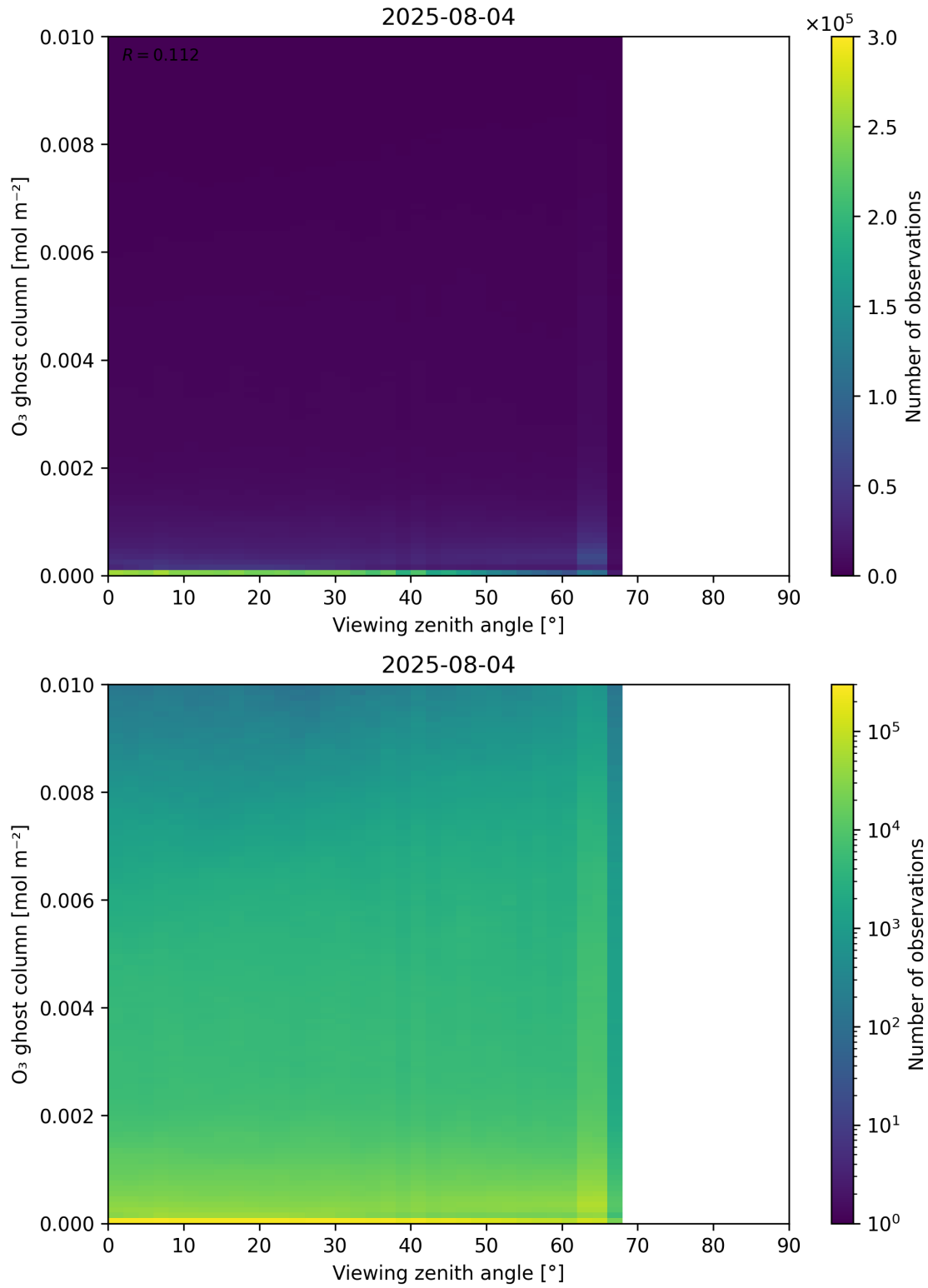
Figure 51: Scatter density plot of “Viewing zenith angle” against “O 3 ghost column” for 2025-08-04 to 2025-08-05.
