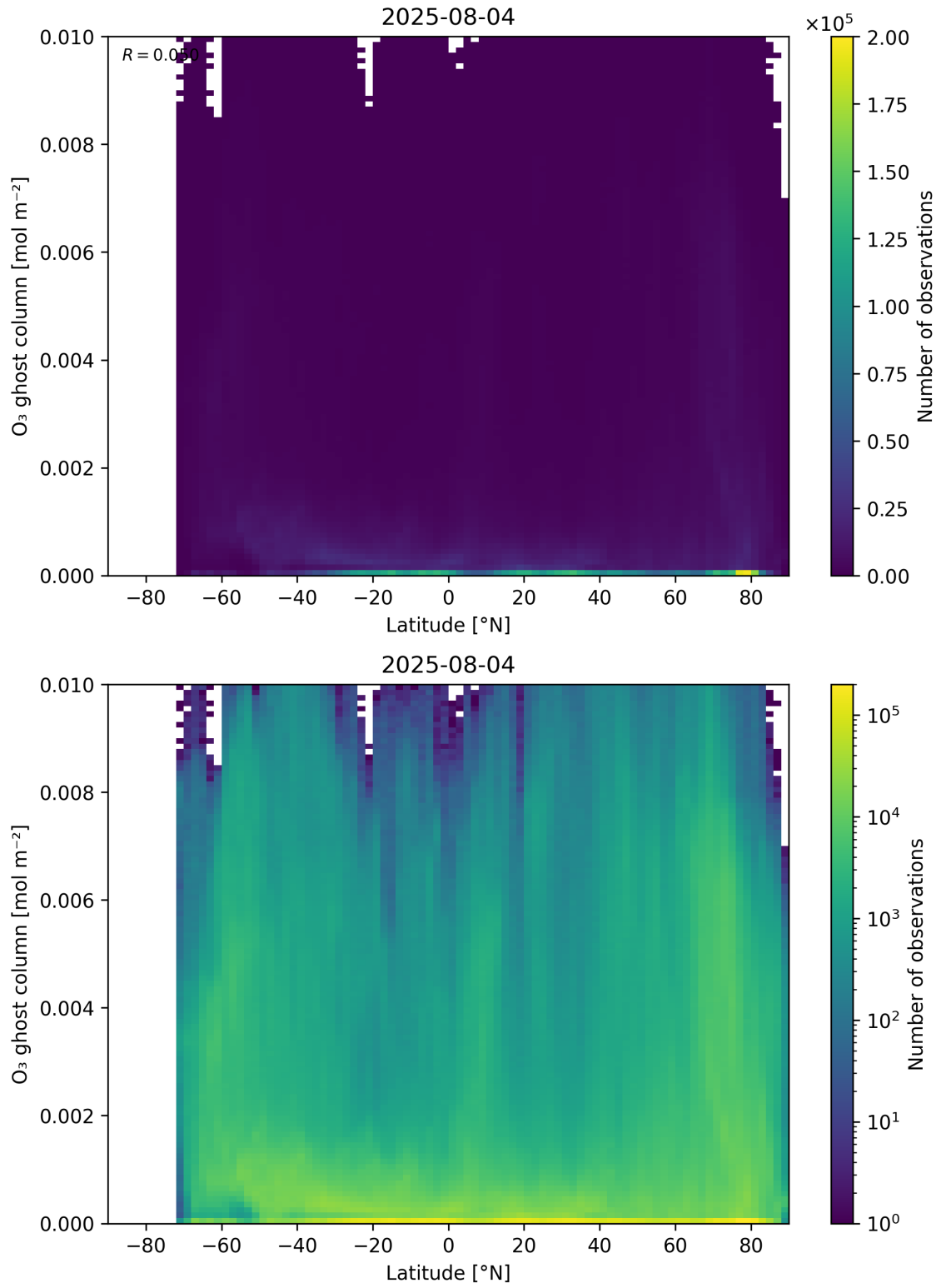
Figure 35: Scatter density plot of “Latitude” against “O 3 ghost column” for 2025-08-04 to 2025-08-05.
