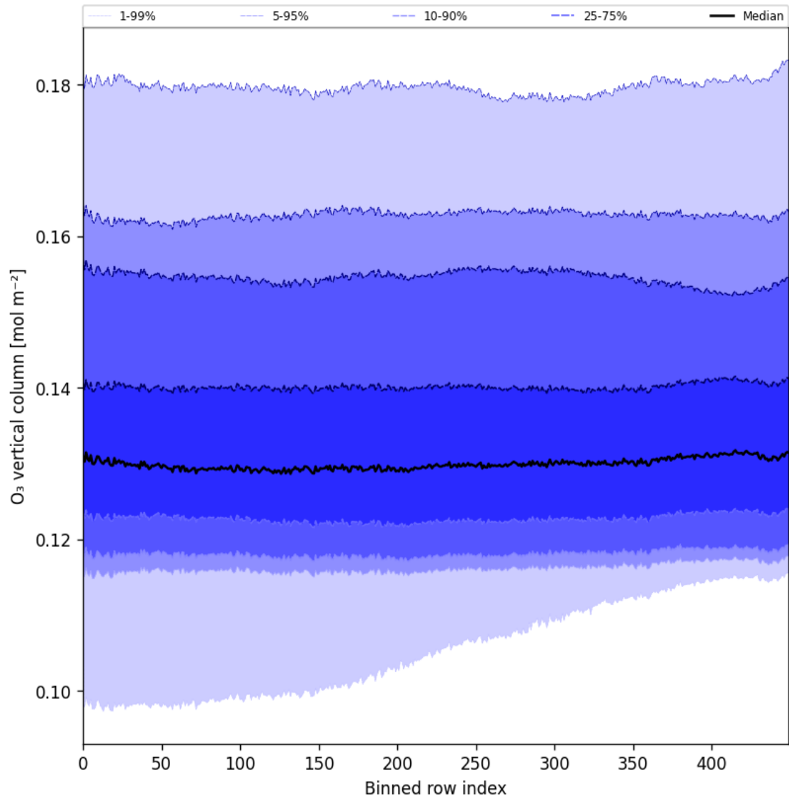
Figure 28: Along track statistics of “O 3 vertical column” for 2025-08-04 to 2025-08-05
