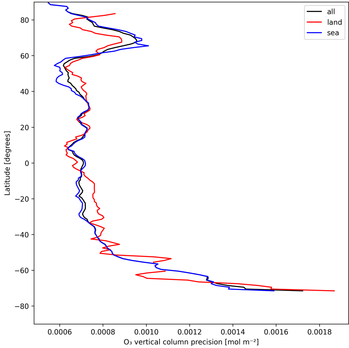
Figure 15: Zonal average of "O 3 vertical column precision" for 2025-08-04 to 2025-08-05.
