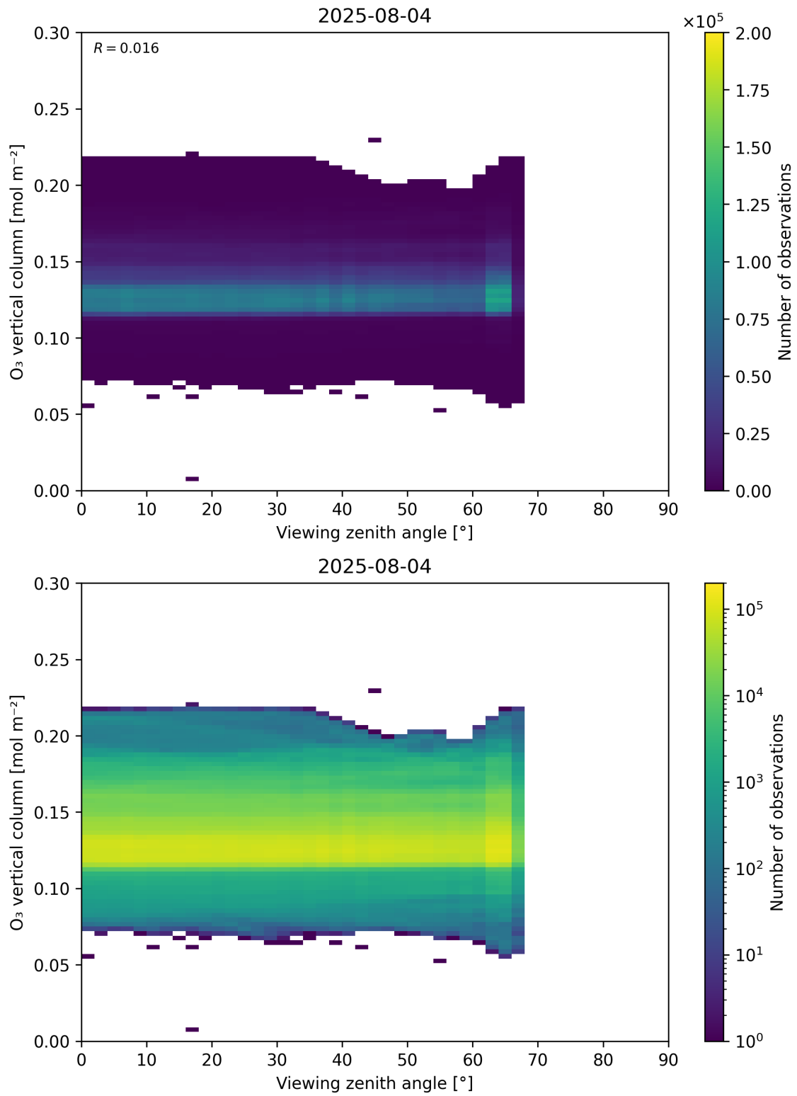
Figure 52: Scatter density plot of “Viewing zenith angle” against “O 3 vertical column” for 2025-08-04 to 2025-08-05.
