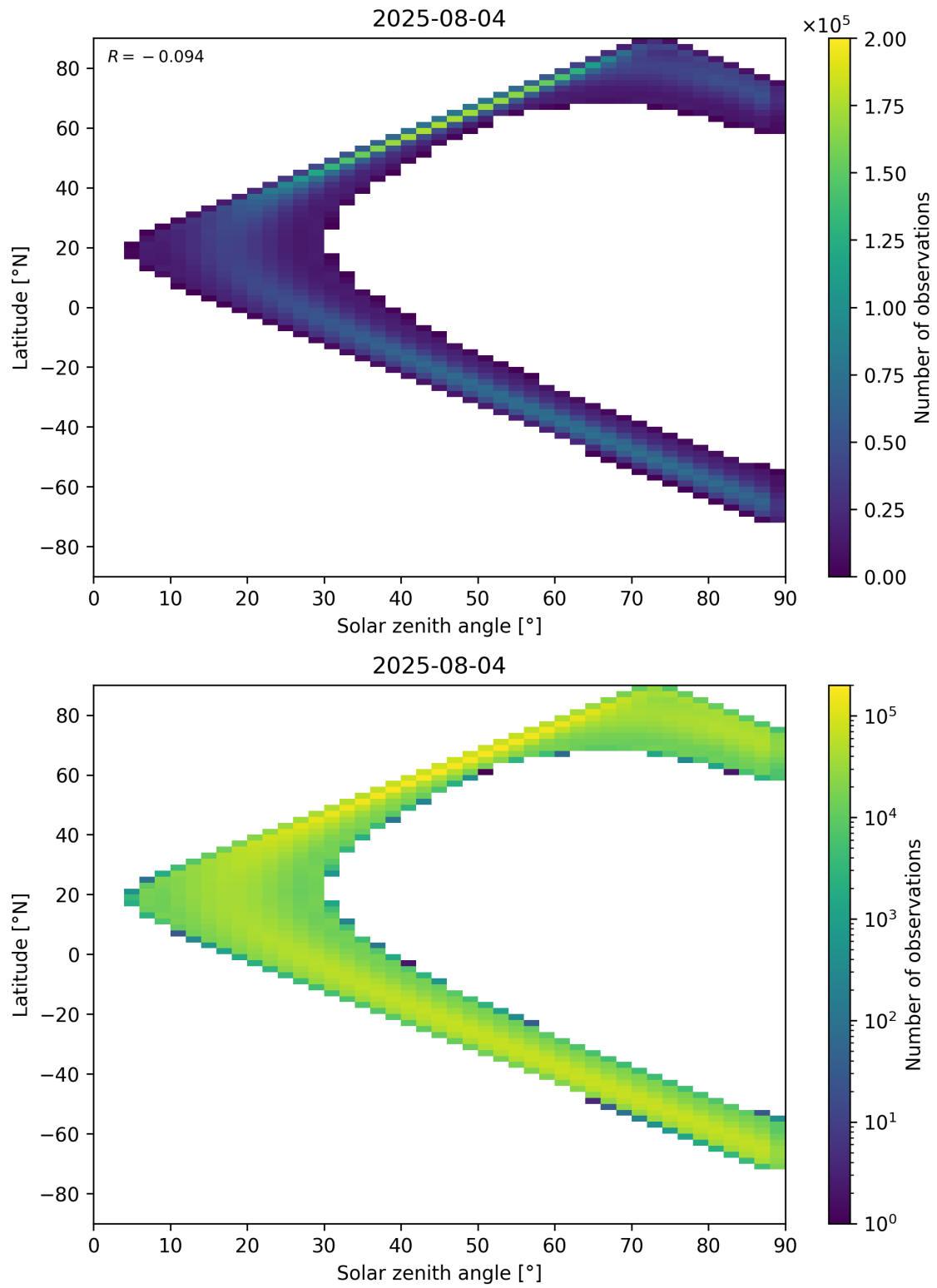
Figure 44: Scatter density plot of “Solar zenith angle” against “Latitude” for 2025-08-04 to 2025-08-05.
