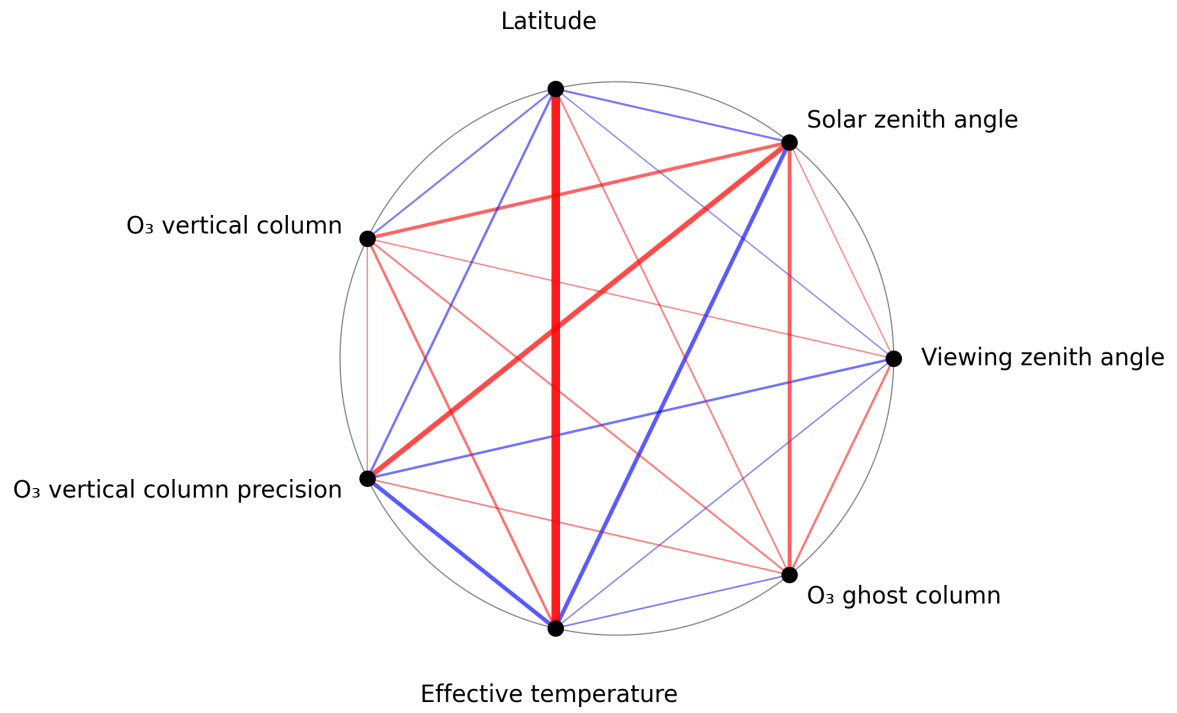
Figure 1: Map of correlation graph for 2025-08-04 to 2025-08-05.
