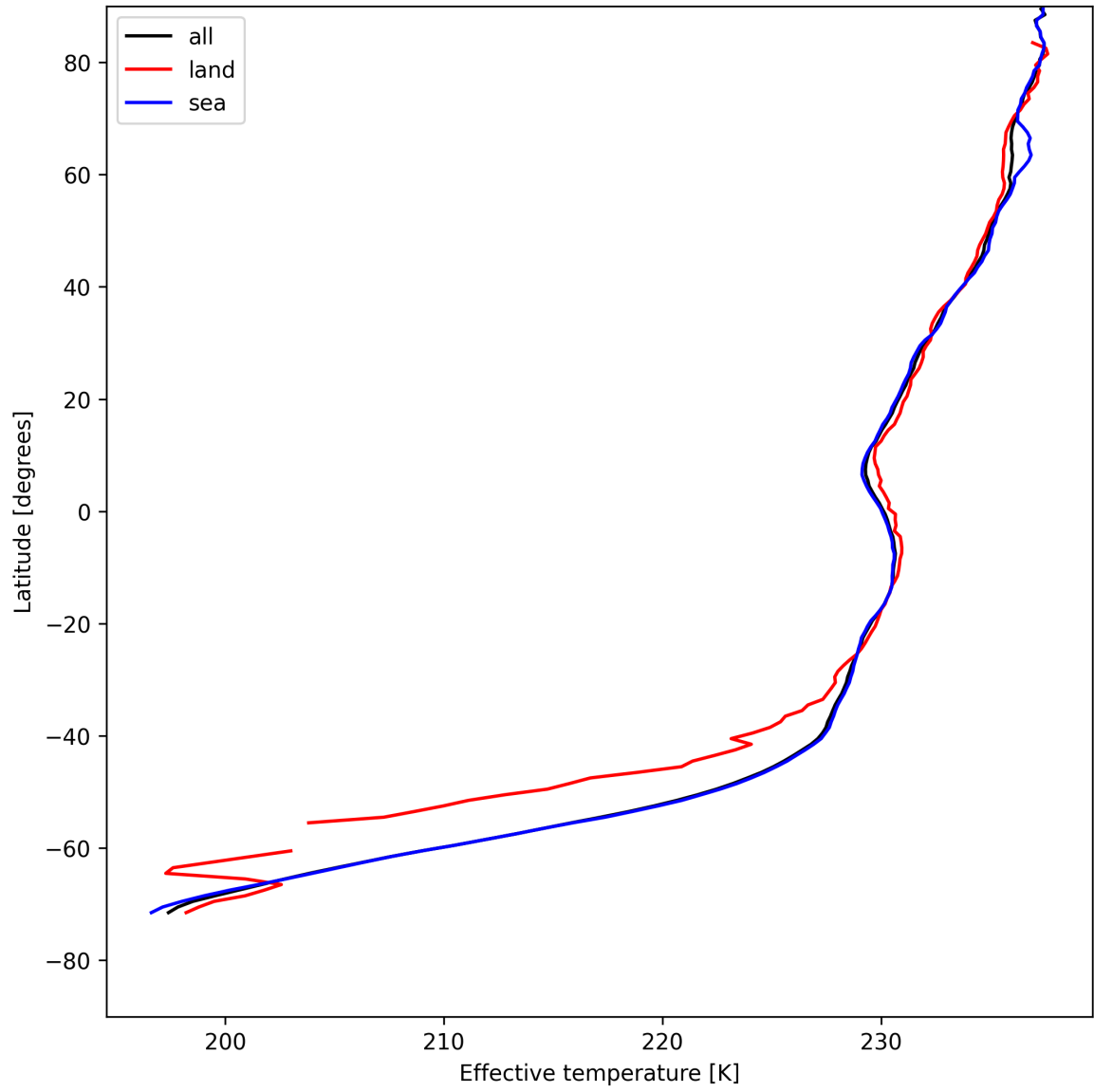
Figure 17: Zonal average of "Effective temperature" for 2025-08-04 to 2025-08-05.
