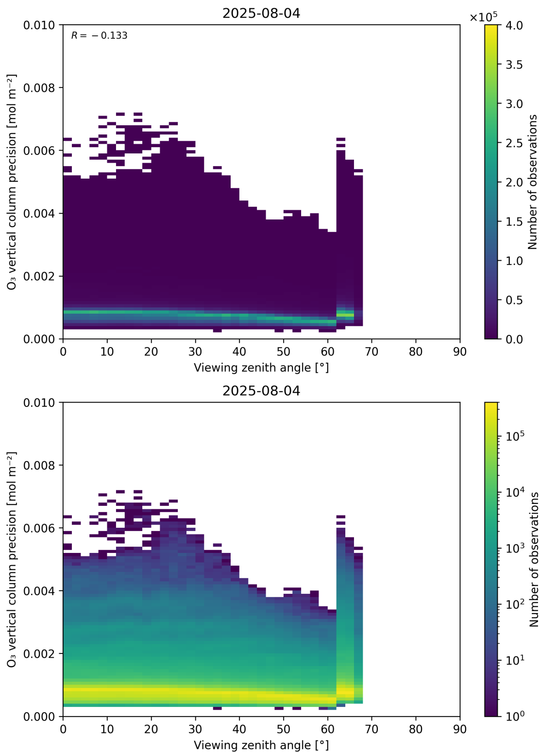
Figure 53: Scatter density plot of “Viewing zenith angle” against “O 3 vertical column precision” for 2025-08-04 to 2025-08-05.
