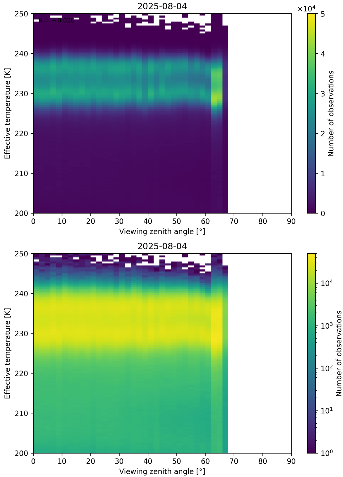
Figure 50: Scatter density plot of “Viewing zenith angle” against “Effective temperature” for 2025-08-04 to 2025-08-05.
