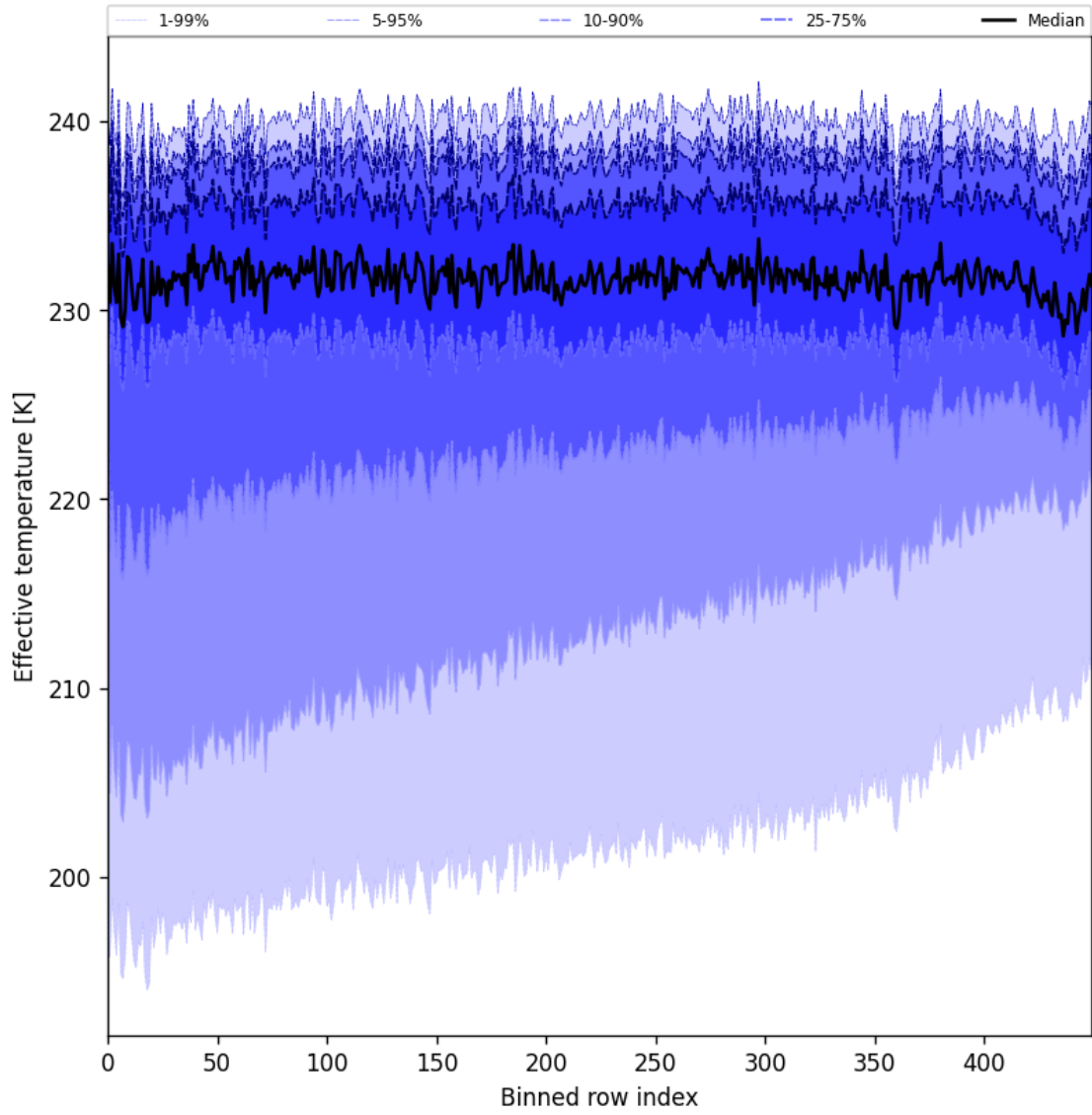
Figure 31: Along track statistics of “Effective temperature” for 2025-08-04 to 2025-08-05
