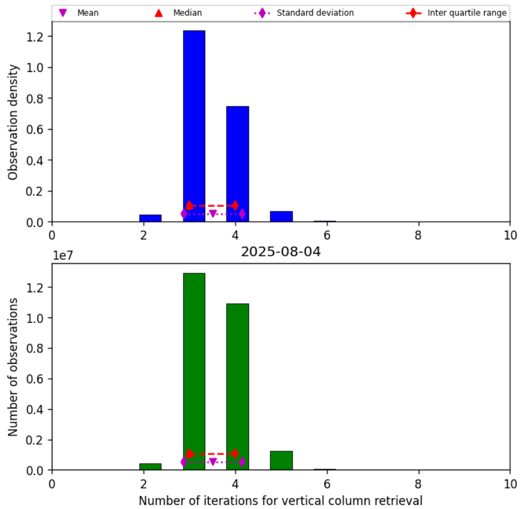
Figure 26: Histogram of “Number of iterations for vertical column retrieval” for 2025-08-04 to 2025-08-05
