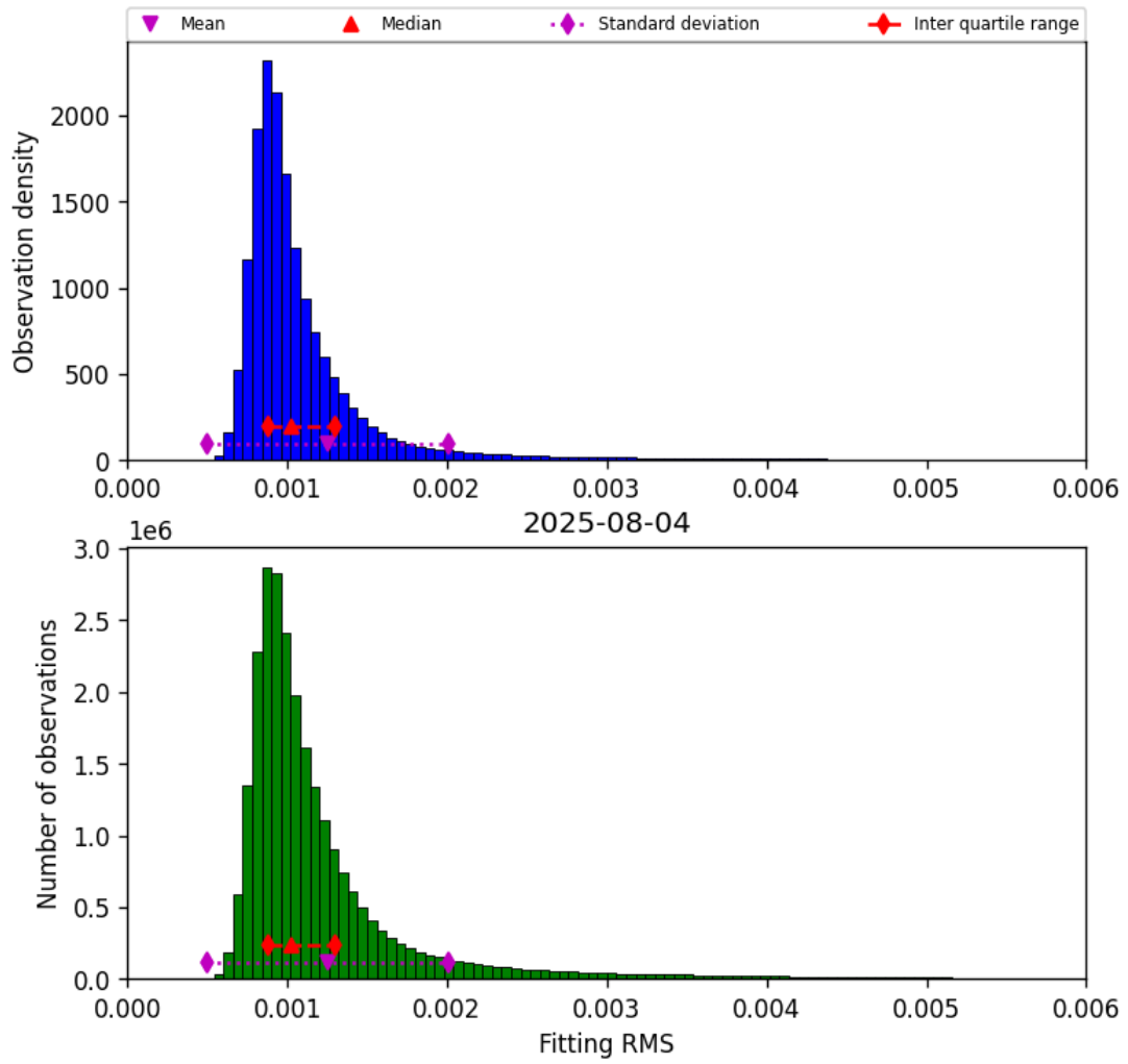
Figure 23: Histogram of “Fitting RMS” for 2025-08-04 to 2025-08-05
