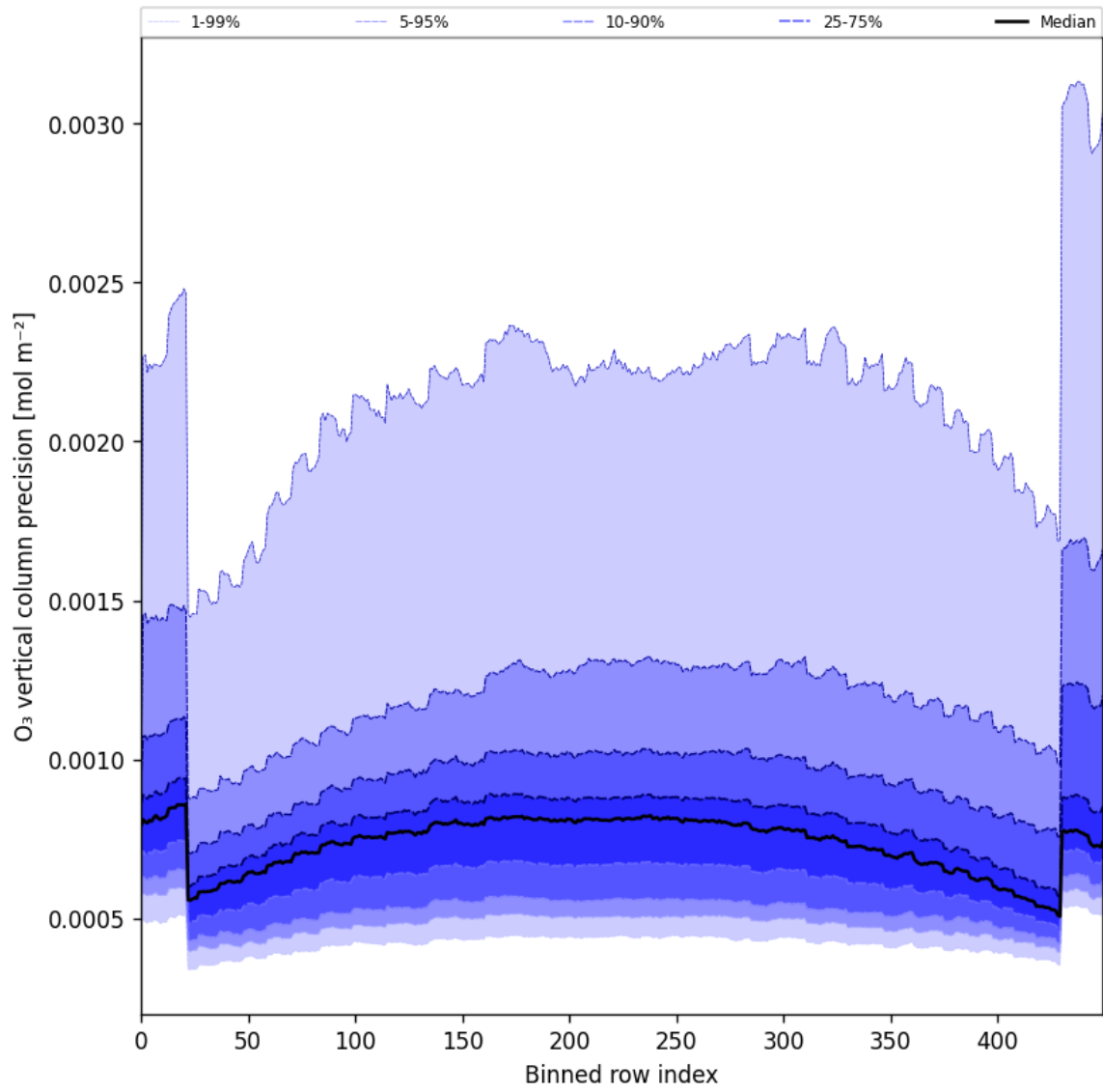
Figure 29: Along track statistics of “O 3 vertical column precision” for 2025-08-04 to 2025-08-05
