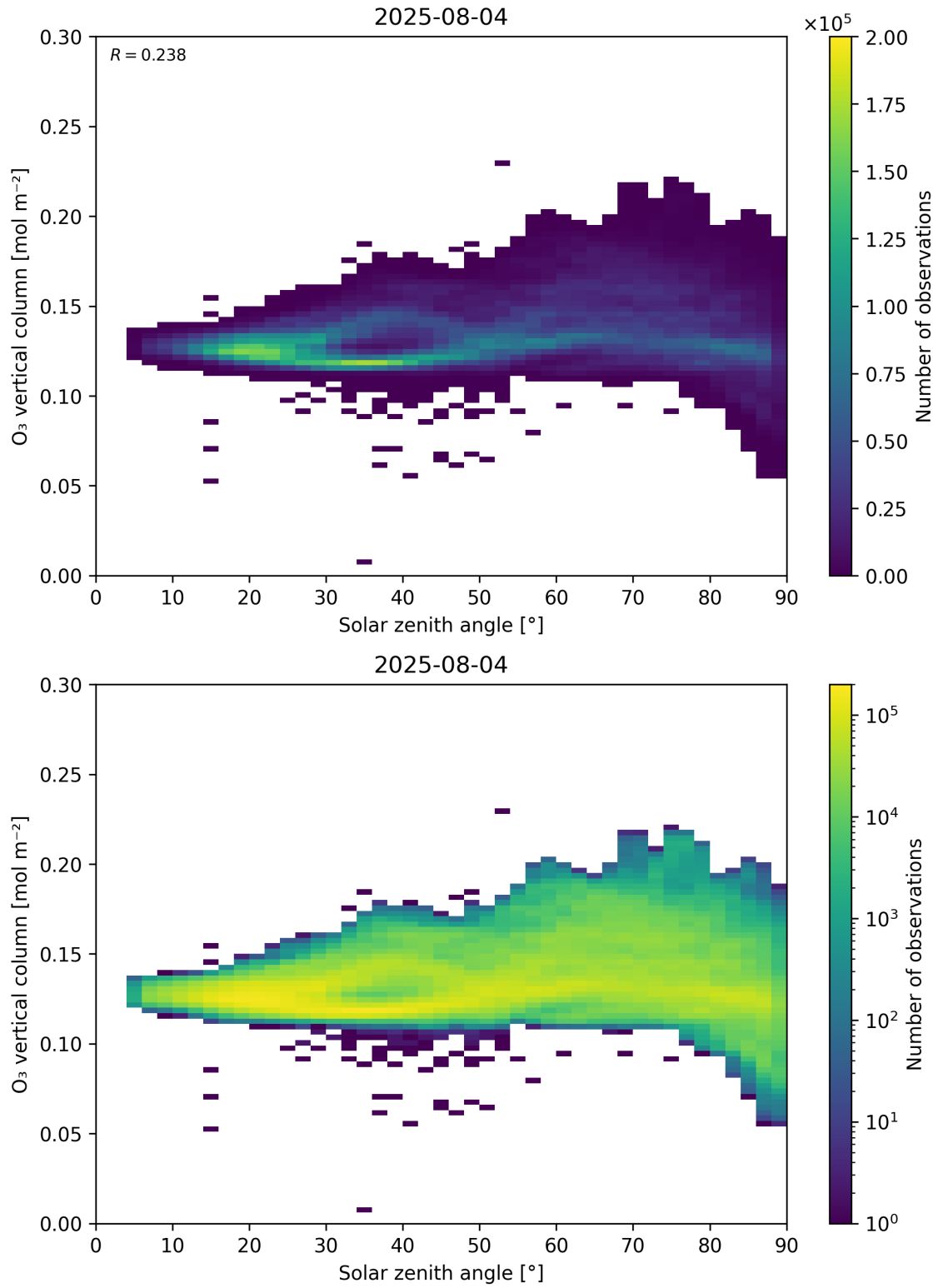
Figure 47: Scatter density plot of “Solar zenith angle” against “O 3 vertical column” for 2025-08-04 to 2025-08-05.
