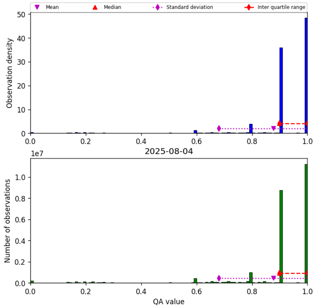
Figure 20: Histogram of “QA value” for 2025-08-04 to 2025-08-05
