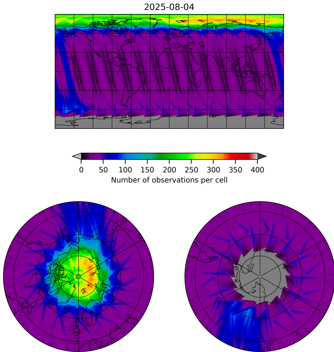
Figure 12: Map of the number of observations for 2025-08-04 to 2025-08-05
