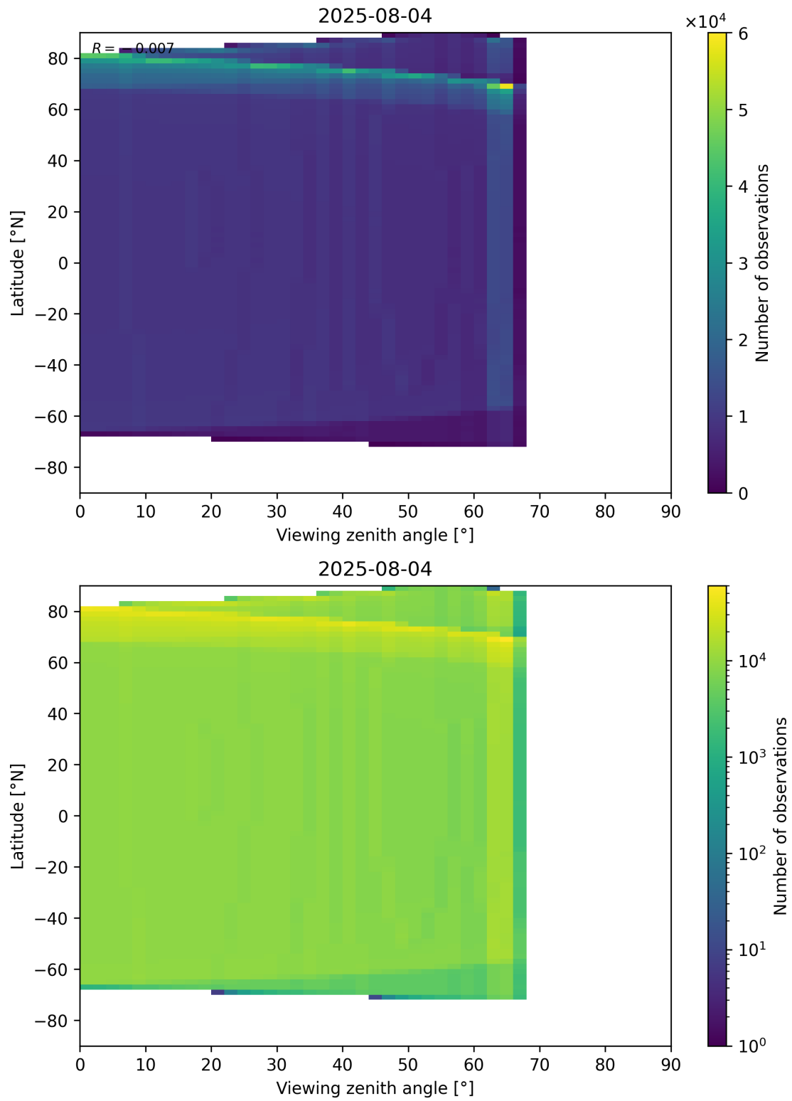
Figure 49: Scatter density plot of “Viewing zenith angle” against “Latitude” for 2025-08-04 to 2025-08-05.
