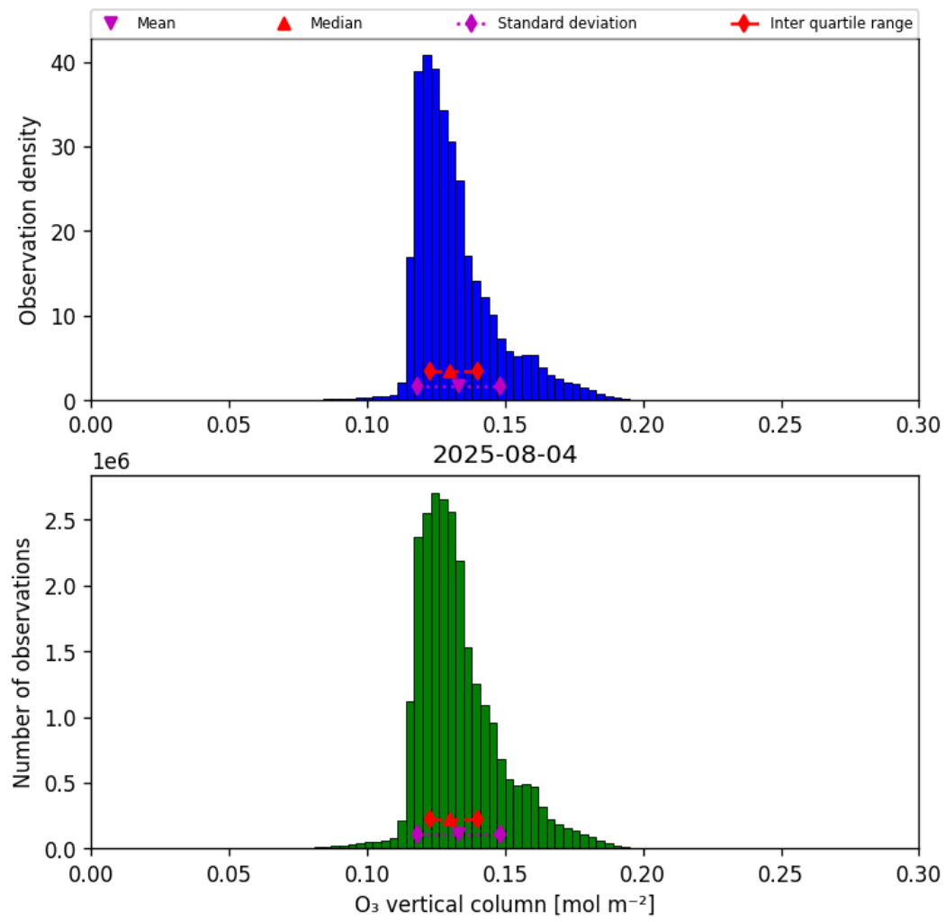
Figure 21: Histogram of “O 3 vertical column” for 2025-08-04 to 2025-08-05
