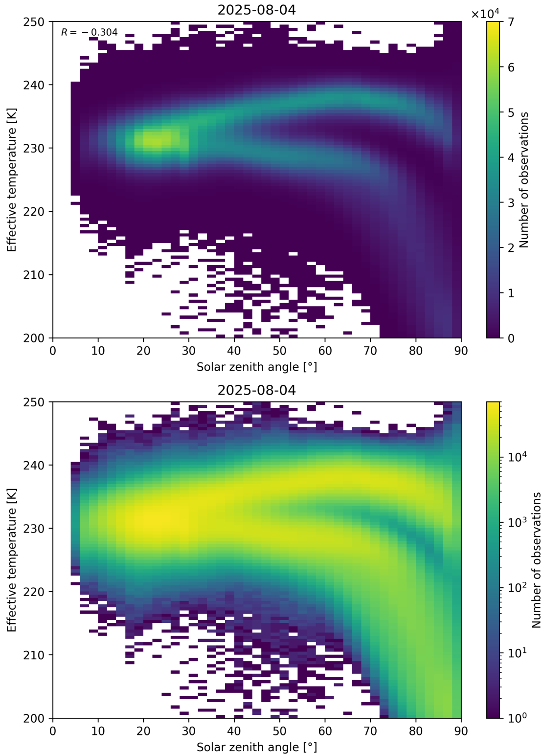
Figure 45: Scatter density plot of “Solar zenith angle” against “Effective temperature” for 2025-08-04 to 2025-08-05.
