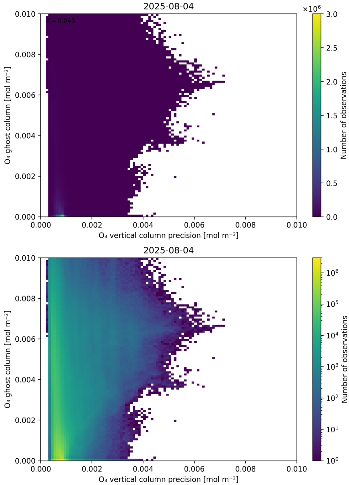
Figure 43: Scatter density plot of “O 3 vertical column precision” against “O 3 ghost column” for 2025-08-04 to 2025-08-05.
