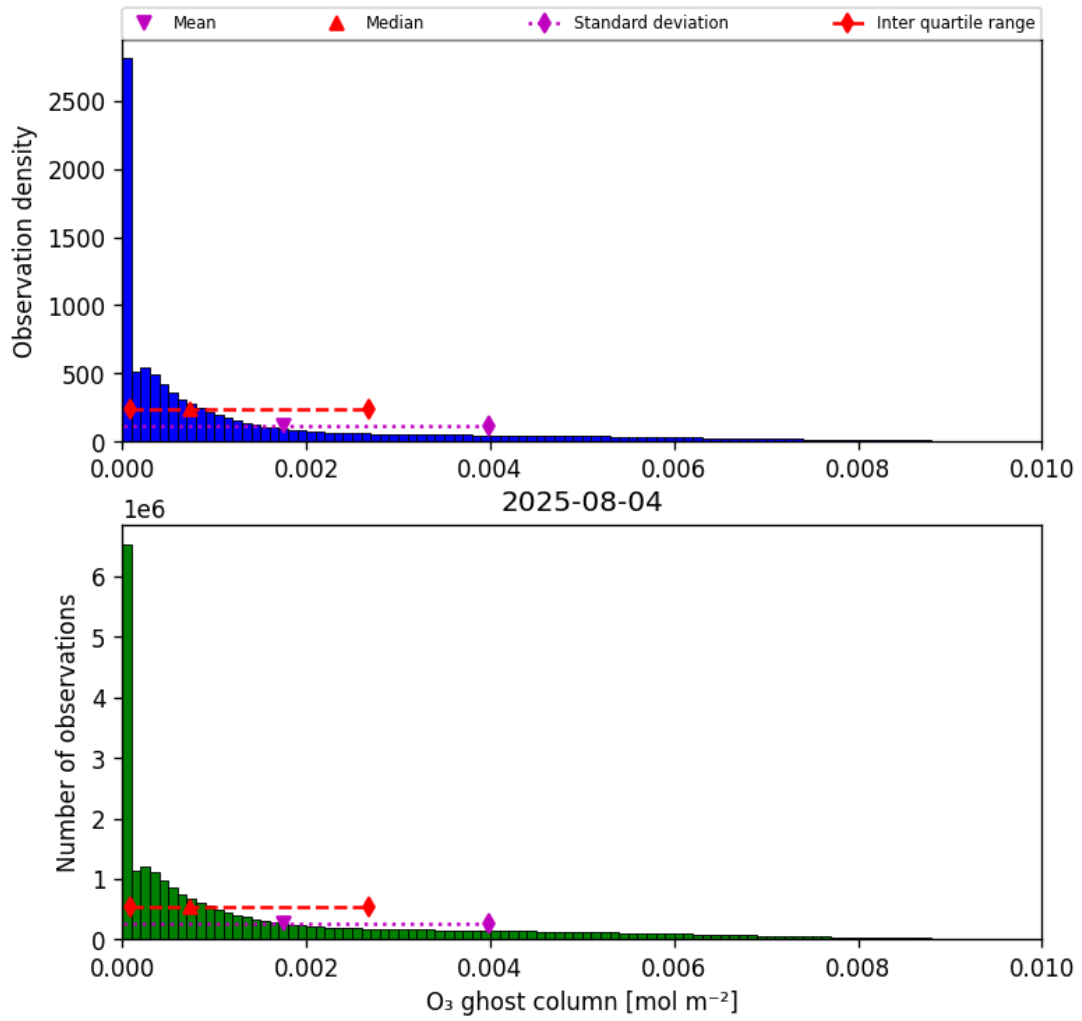
Figure 25: Histogram of “O 3 ghost column” for 2025-08-04 to 2025-08-05
