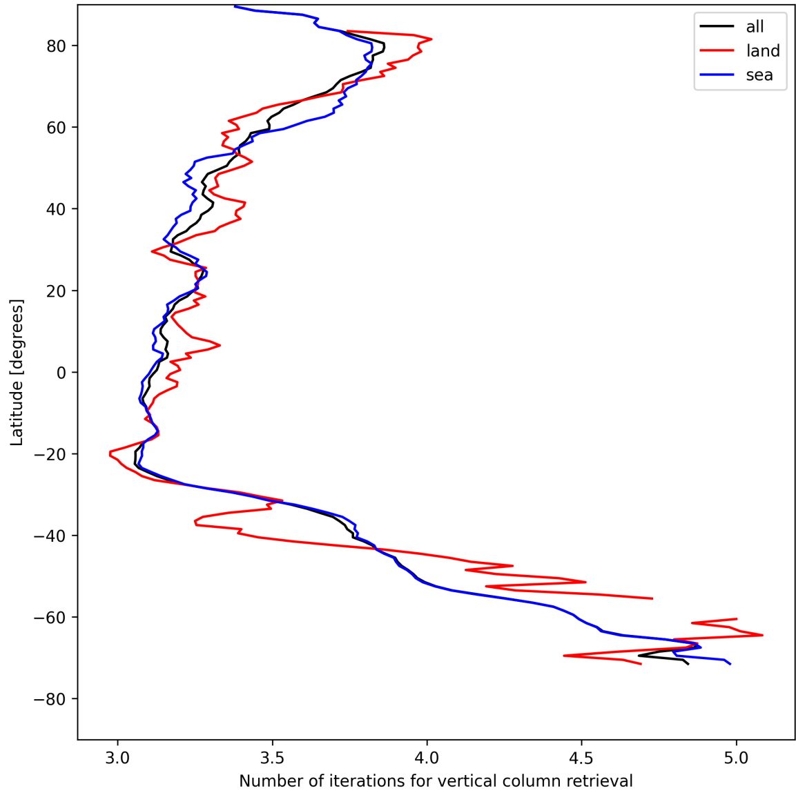
Figure 19: Zonal average of “Number of iterations for vertical column retrieval” for 2025-08-04 to 2025-08-05.
