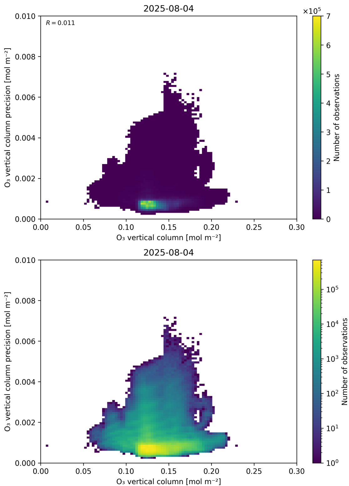
Figure 41: Scatter density plot of “O 3 vertical column” against “O 3 vertical column precision” for 2025-08-04 to 2025-08-05.
