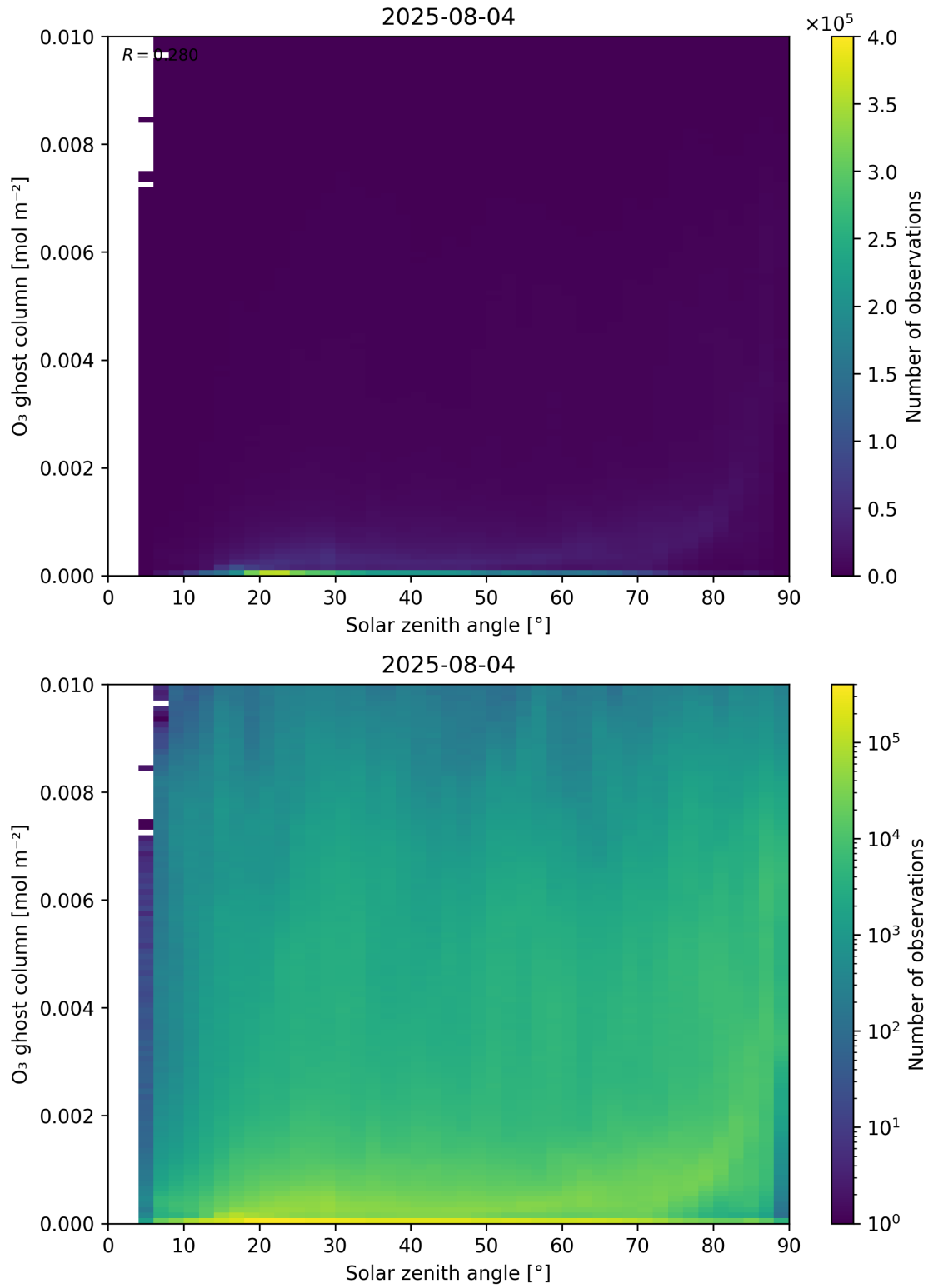
Figure 46: Scatter density plot of “Solar zenith angle” against “O 3 ghost column” for 2025-08-04 to 2025-08-05.
