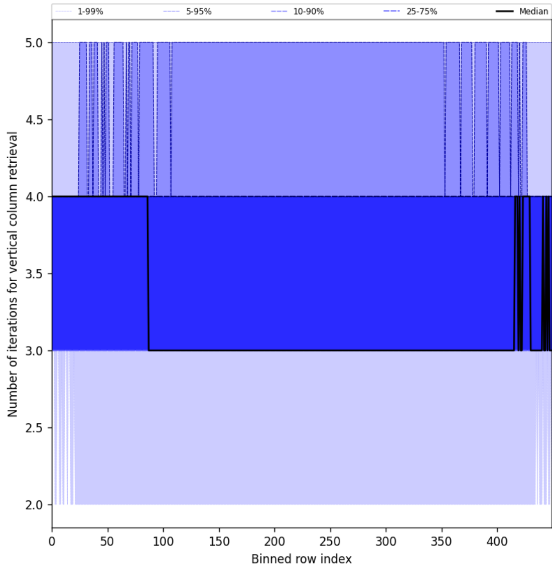
Figure 33: Along track statistics of “Number of iterations for vertical column retrieval” for 2025-08-04 to 2025-08-06
