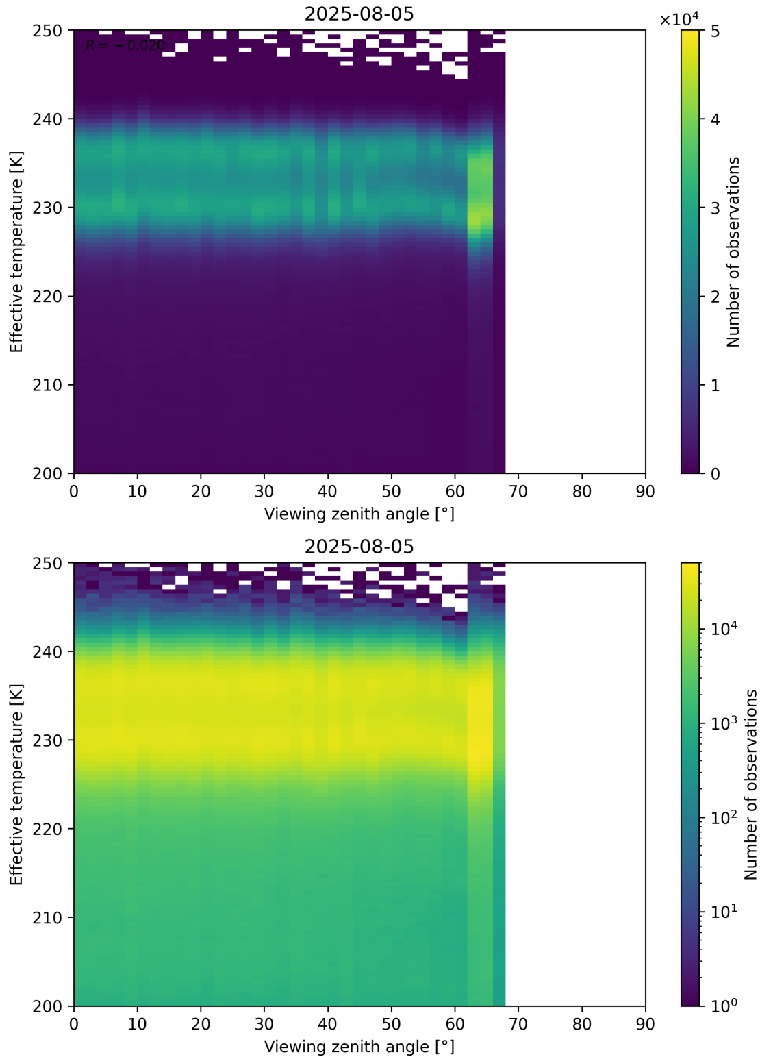
Figure 50: Scatter density plot of “Viewing zenith angle” against “Effective temperature” for 2025-08-04 to 2025-08-06.
