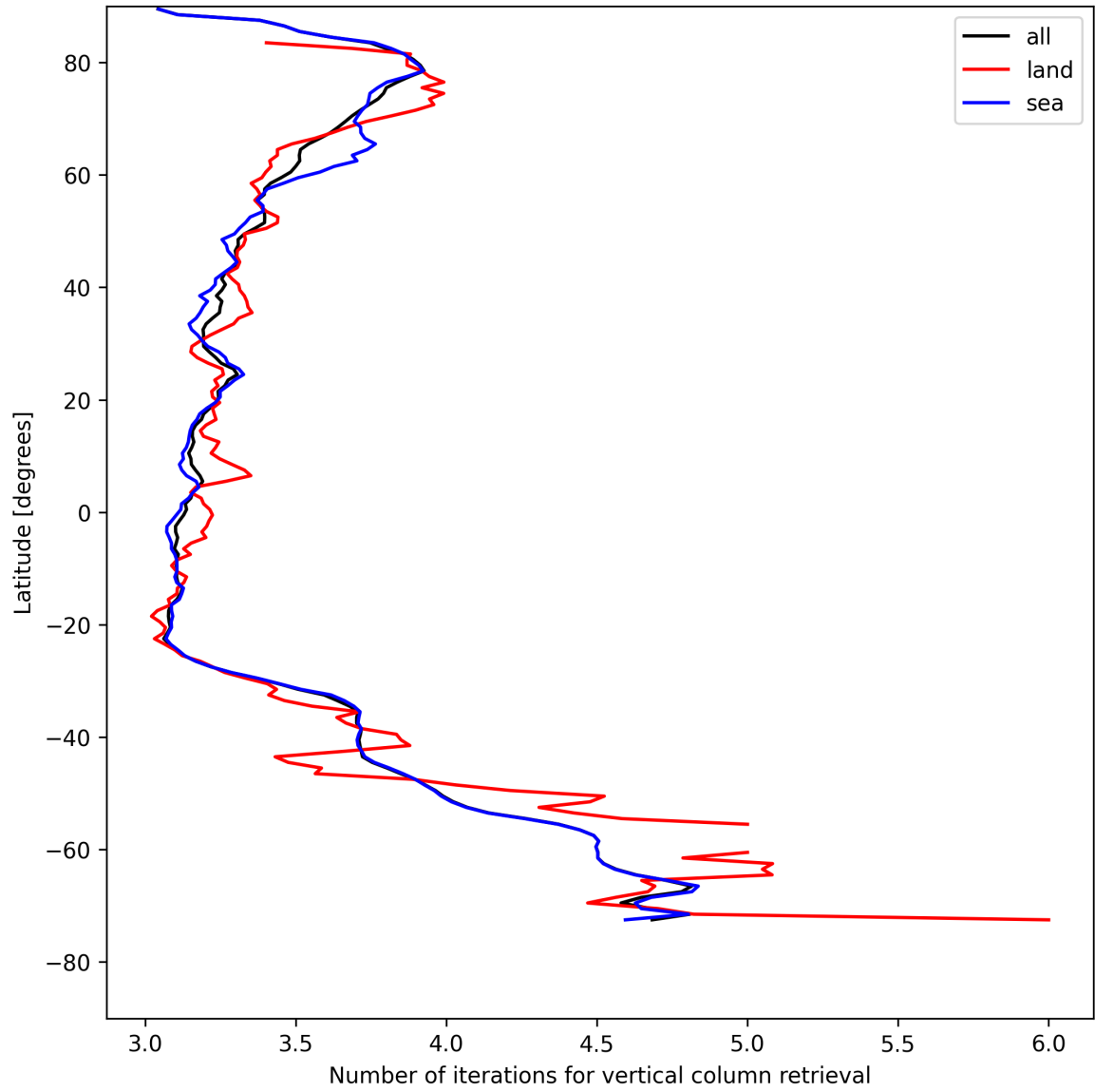
Figure 19: Zonal average of “Number of iterations for vertical column retrieval” for 2025-08-04 to 2025-08-06.
