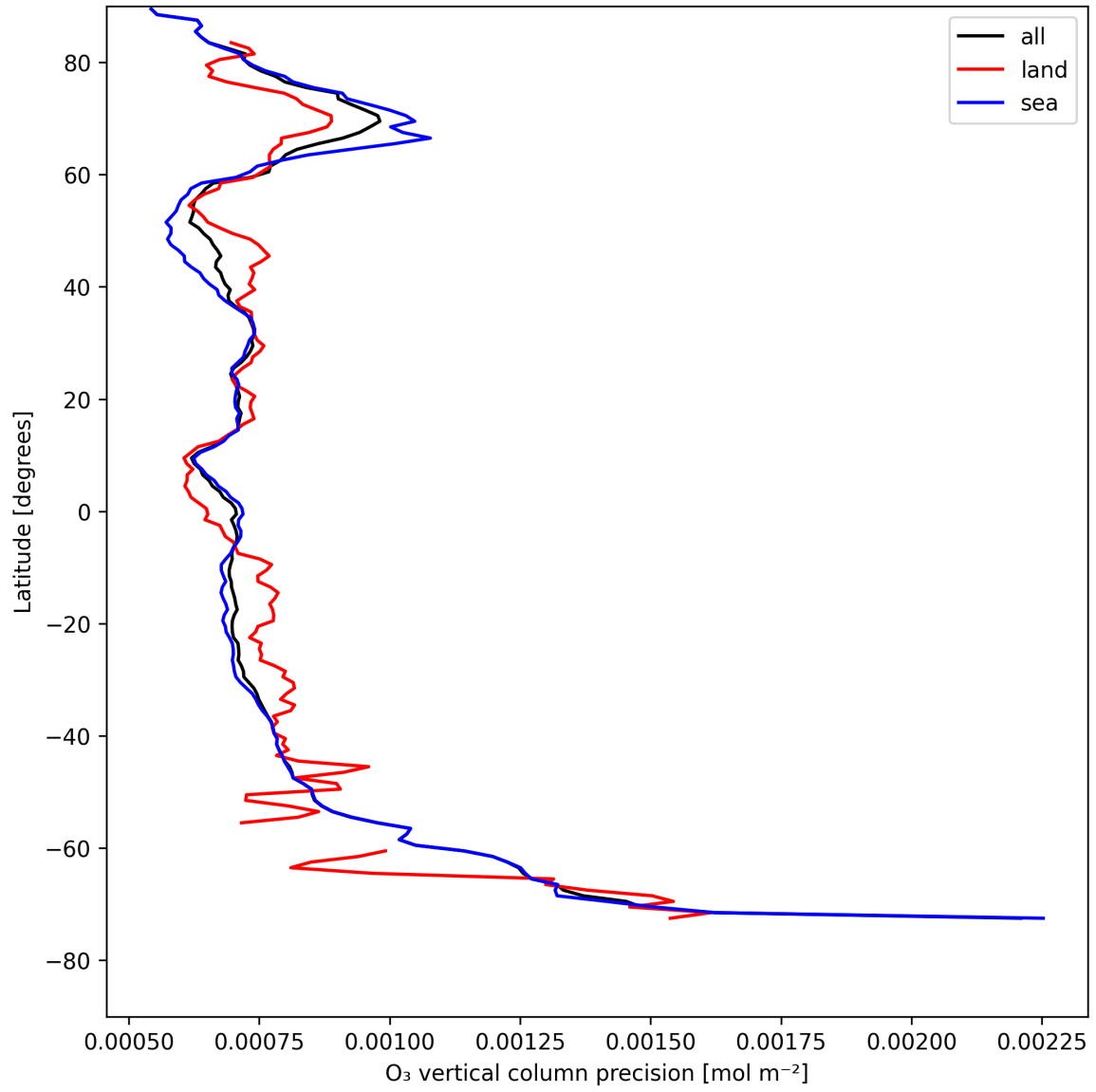
Figure 15: Zonal average of "O 3 vertical column precision" for 2025-08-04 to 2025-08-06.
