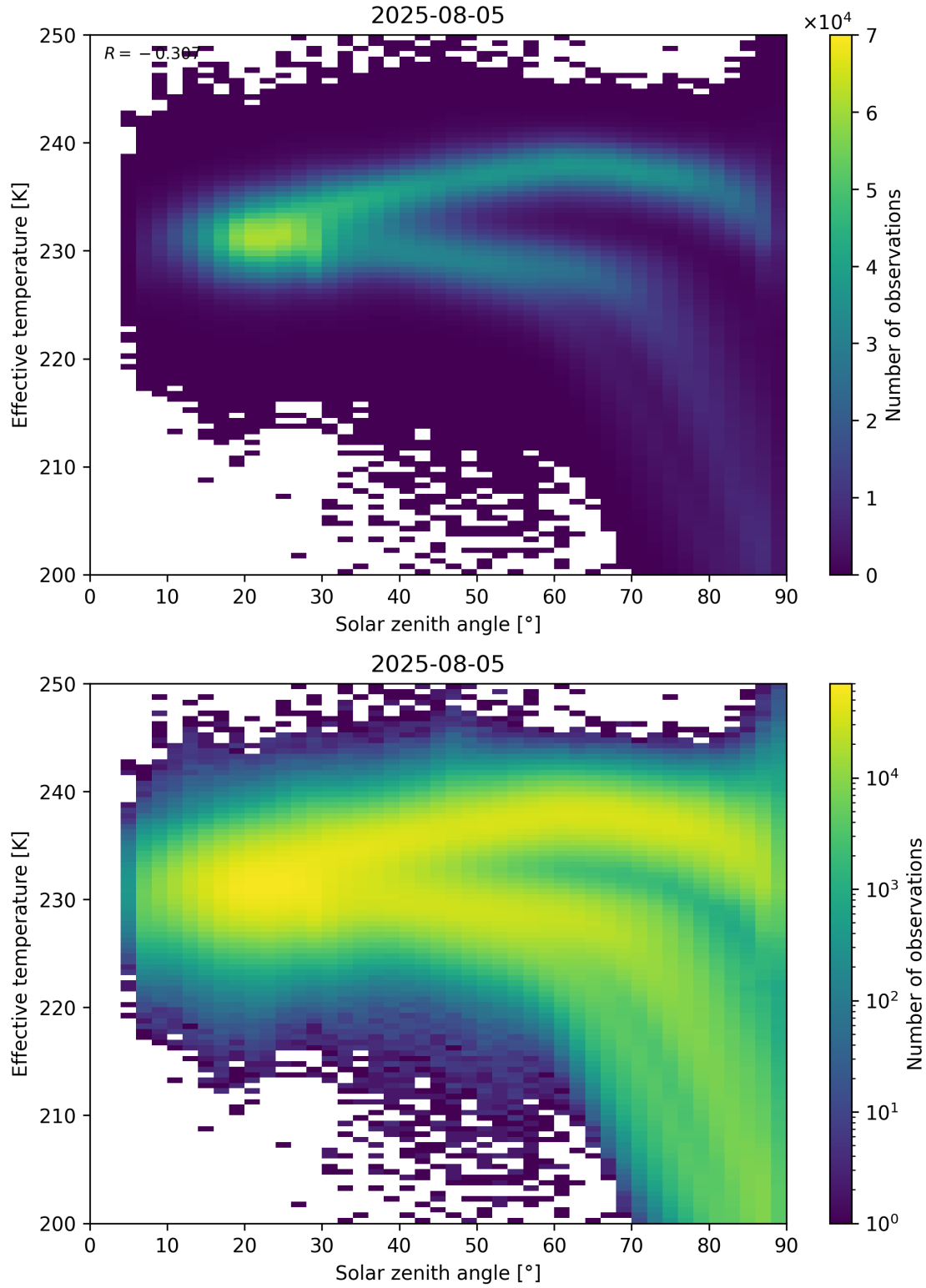
Figure 45: Scatter density plot of “Solar zenith angle” against “Effective temperature” for 2025-08-04 to 2025-08-06.
