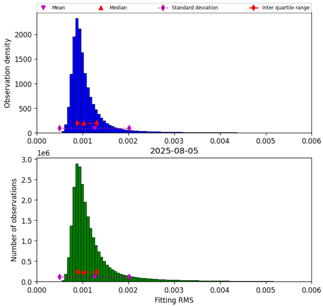
Figure 23: Histogram of “Fitting RMS” for 2025-08-04 to 2025-08-06
