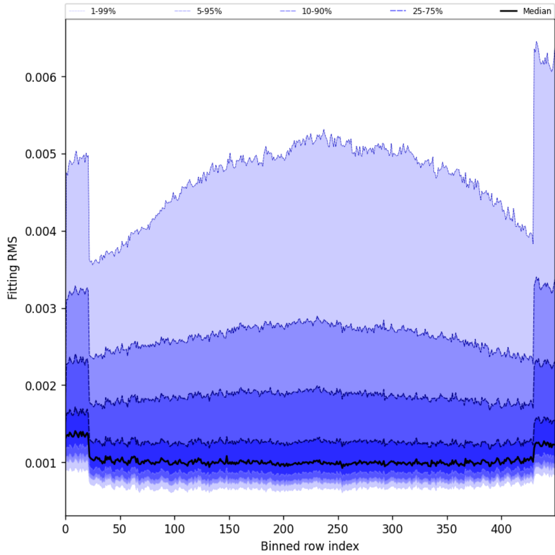
Figure 30: Along track statistics of “Fitting RMS” for 2025-08-04 to 2025-08-06
