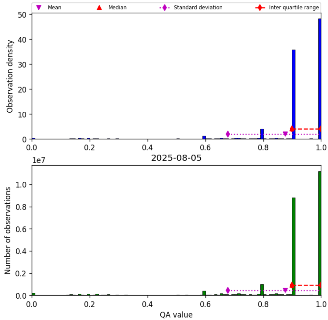
Figure 20: Histogram of “QA value” for 2025-08-04 to 2025-08-06
