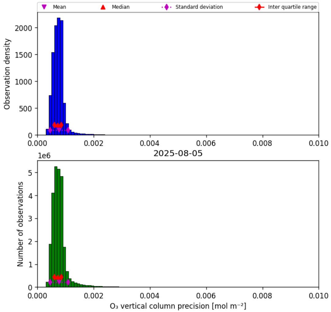
Figure 22: Histogram of “O 3 vertical column precision” for 2025-08-04 to 2025-08-06
