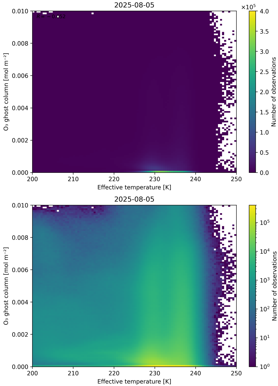
Figure 38: Scatter density plot of “Effective temperature” against “O 3 ghost column” for 2025-08-04 to 2025-08-06.
