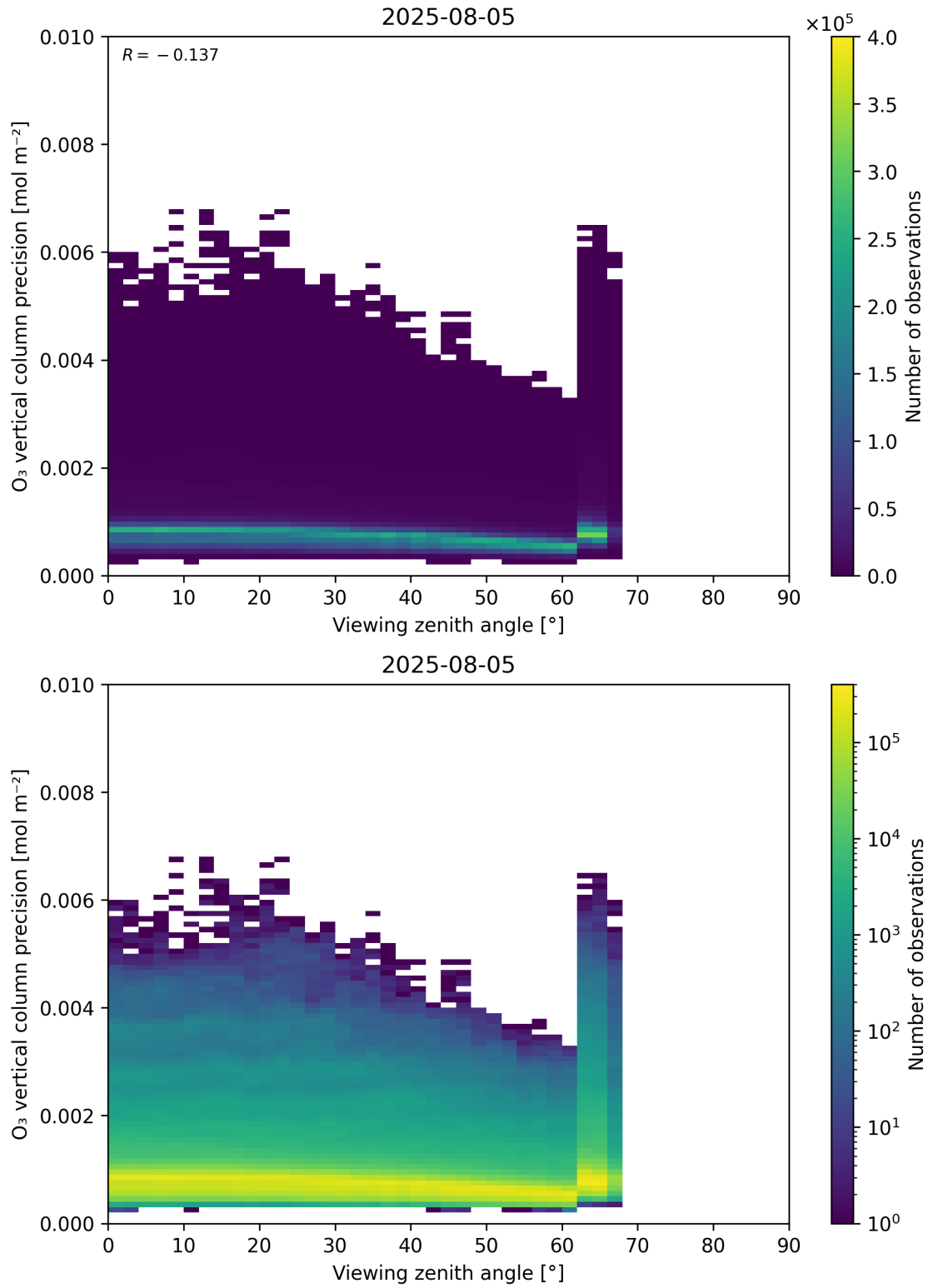
Figure 53: Scatter density plot of “Viewing zenith angle” against “O 3 vertical column precision” for 2025-08-04 to 2025-08-06.
