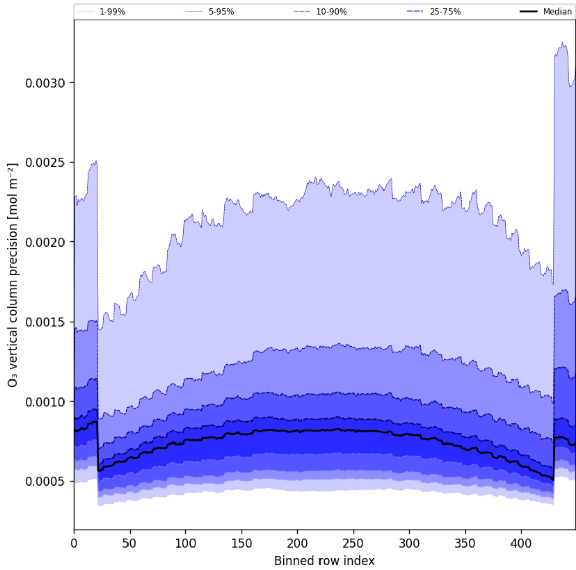
Figure 29: Along track statistics of “O 3 vertical column precision” for 2025-08-04 to 2025-08-06
