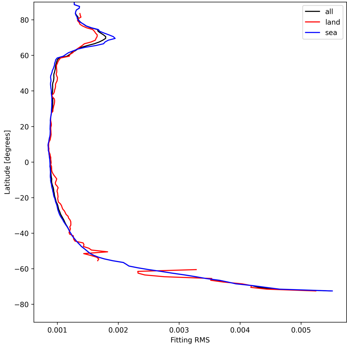
Figure 16: Zonal average of “Fitting RMS” for 2025-08-04 to 2025-08-06.
