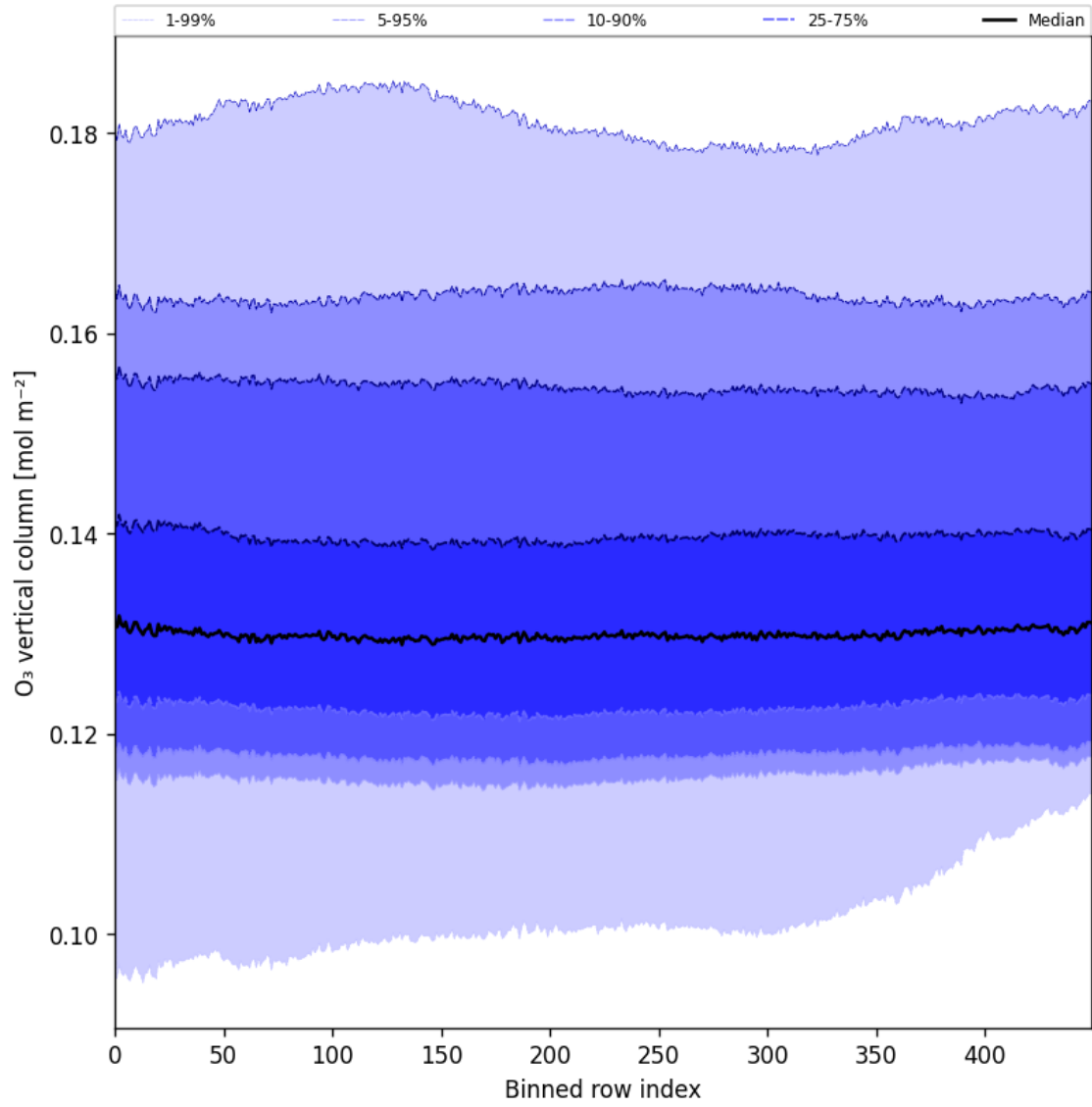
Figure 28: Along track statistics of “O 3 vertical column” for 2025-08-04 to 2025-08-06
