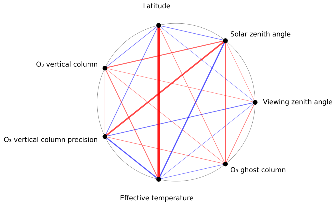
Figure 1: Map of correlation graph for 2025-08-04 to 2025-08-06.
