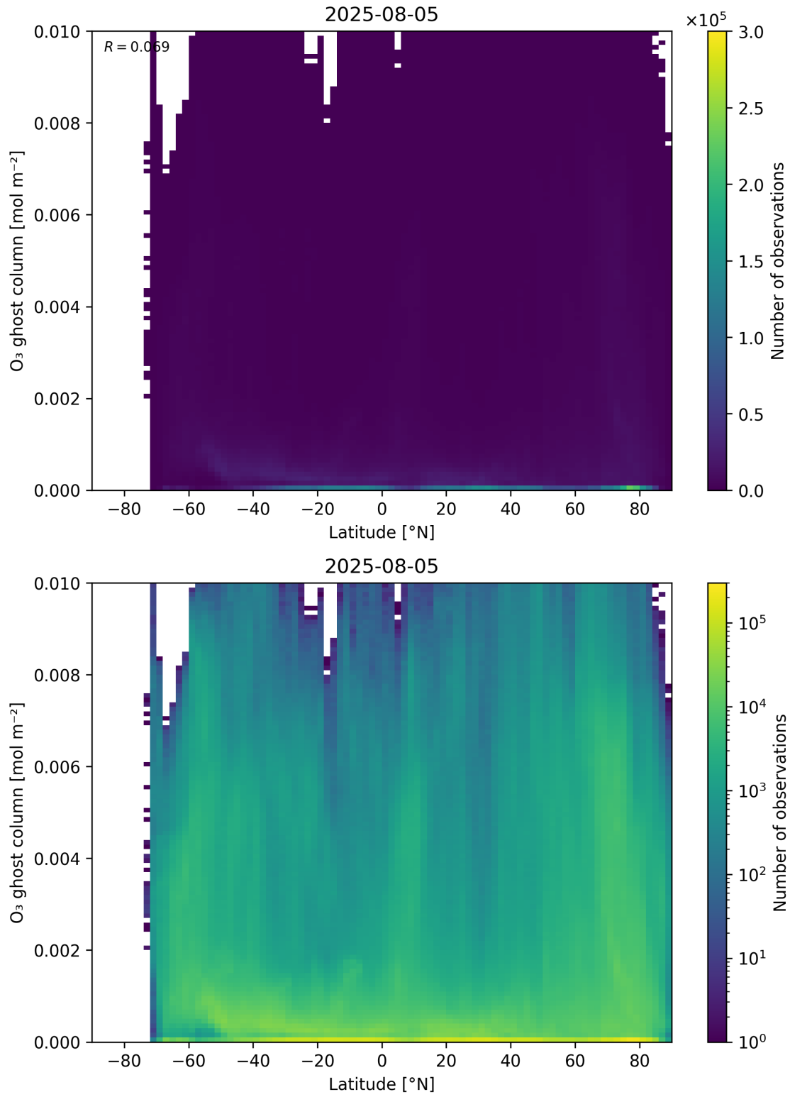
Figure 35: Scatter density plot of “Latitude” against “O 3 ghost column” for 2025-08-04 to 2025-08-06.
