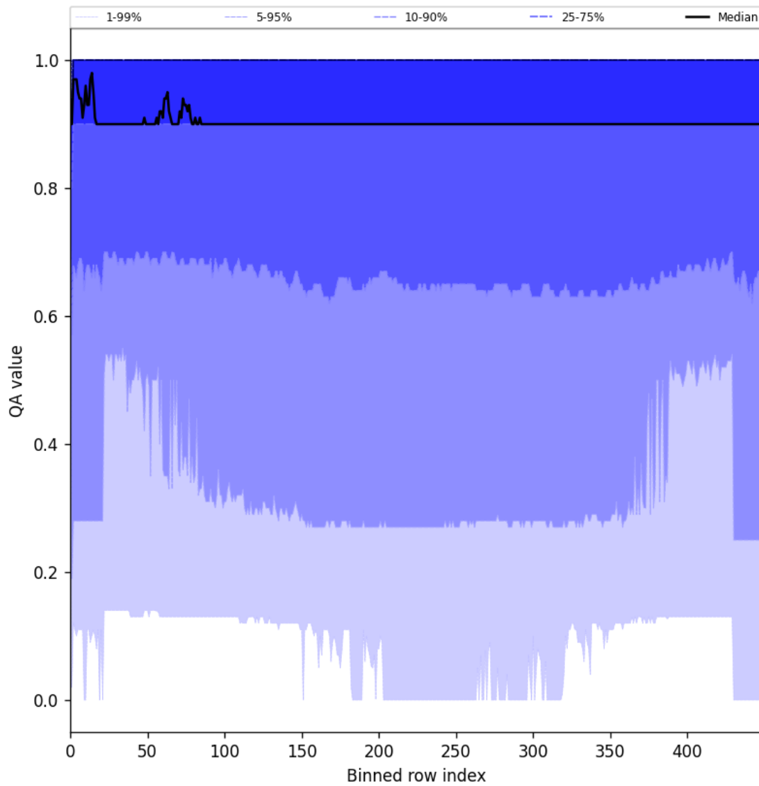
Figure 27: Along track statistics of “QA value” for 2025-08-04 to 2025-08-06
