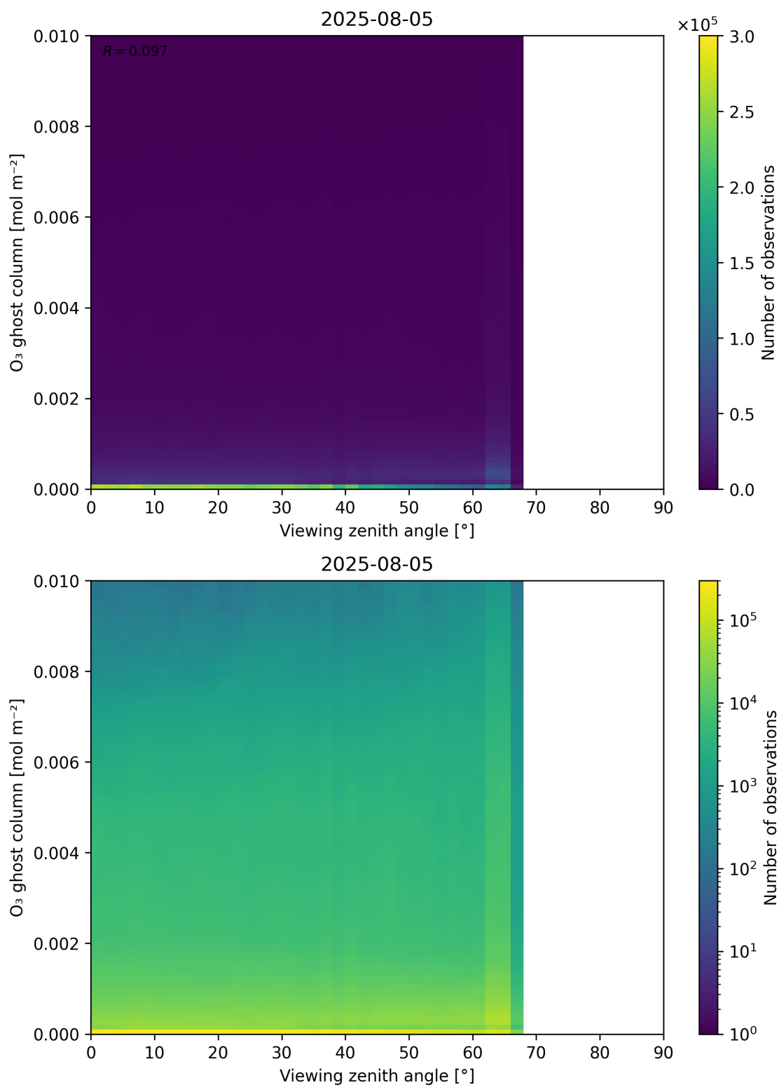
Figure 51: Scatter density plot of “Viewing zenith angle” against “O 3 ghost column” for 2025-08-04 to 2025-08-06.
