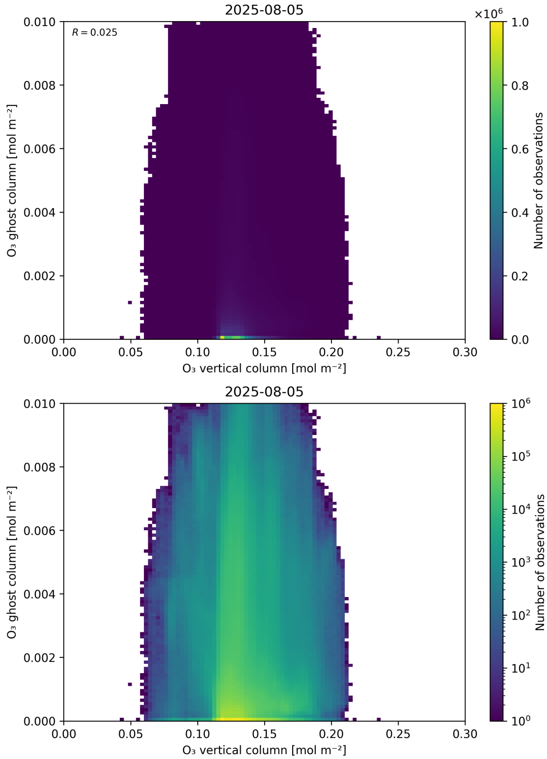
Figure 40: Scatter density plot of “O 3 vertical column” against “O 3 ghost column” for 2025-08-04 to 2025-08-06.
