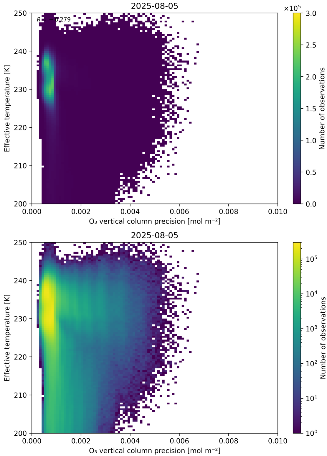
Figure 42: Scatter density plot of “O 3 vertical column precision” against “Effective temperature” for 2025-08-04 to 2025-08-06.
