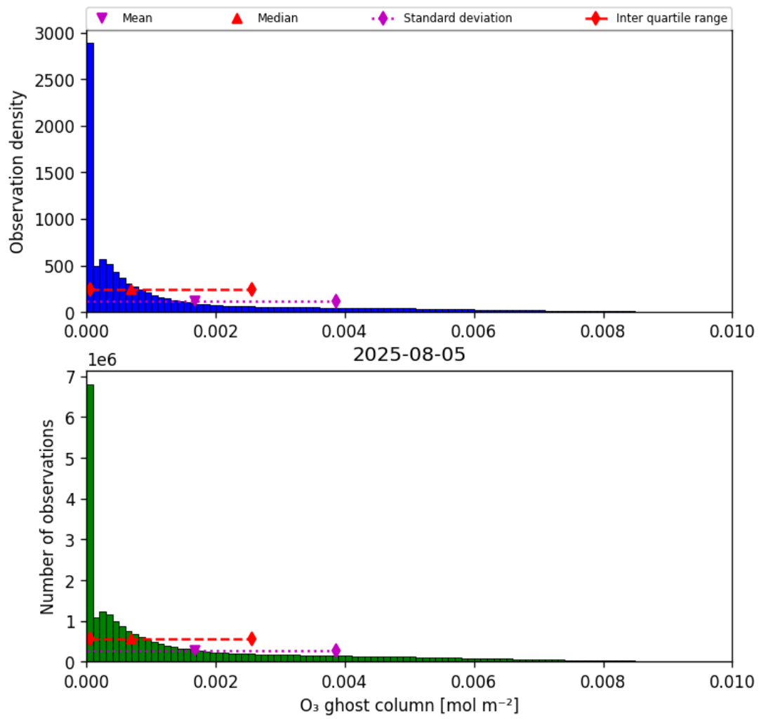
Figure 25: Histogram of “O 3 ghost column” for 2025-08-04 to 2025-08-06
