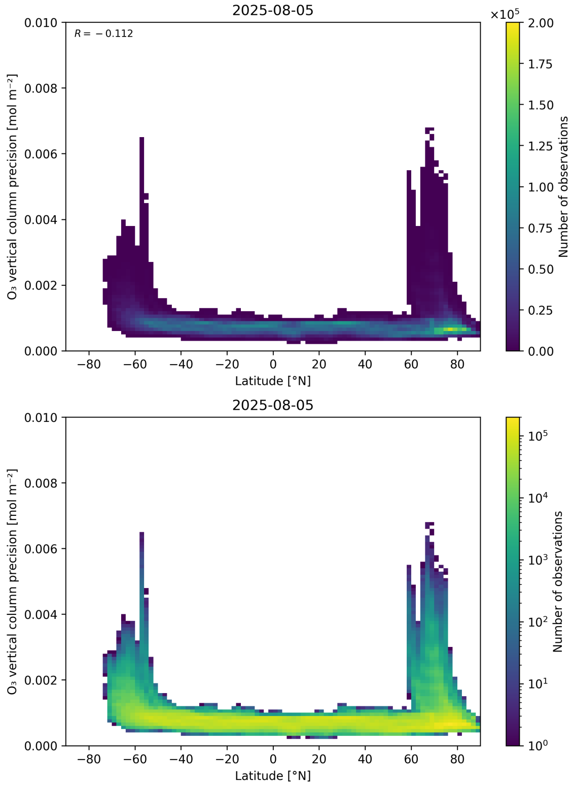
Figure 37: Scatter density plot of “Latitude” against “O 3 vertical column precision” for 2025-08-04 to 2025-08-06.
