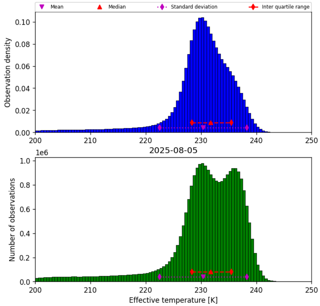
Figure 24: Histogram of “Effective temperature” for 2025-08-04 to 2025-08-06
