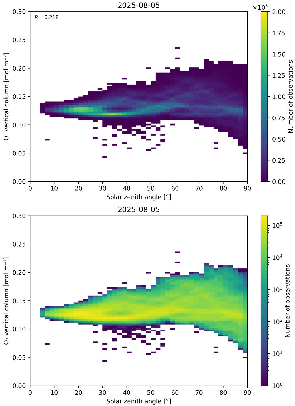
Figure 47: Scatter density plot of “Solar zenith angle” against “O 3 vertical column” for 2025-08-04 to 2025-08-06.
