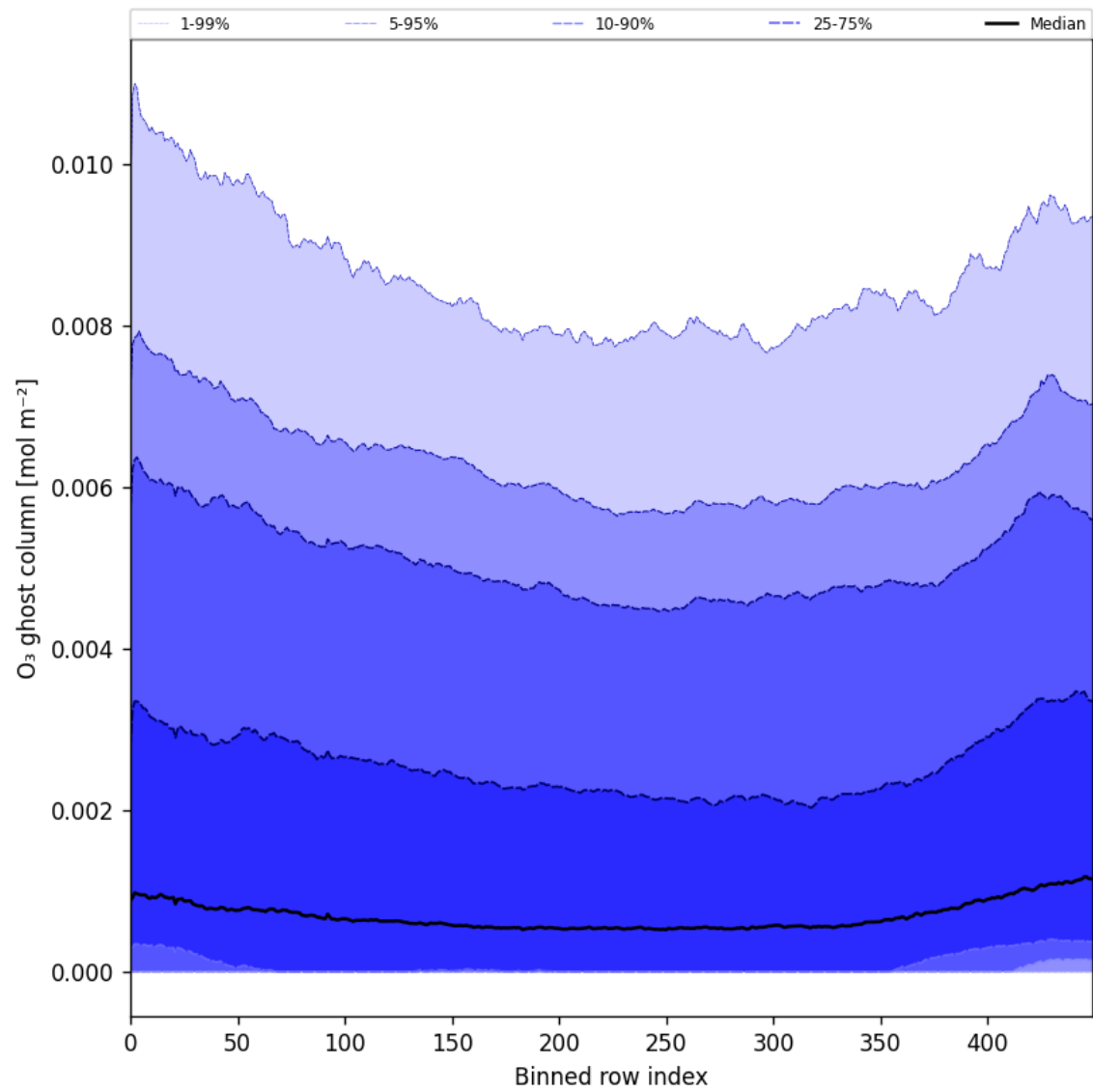
Figure 32: Along track statistics of “O 3 ghost column” for 2025-08-04 to 2025-08-06
