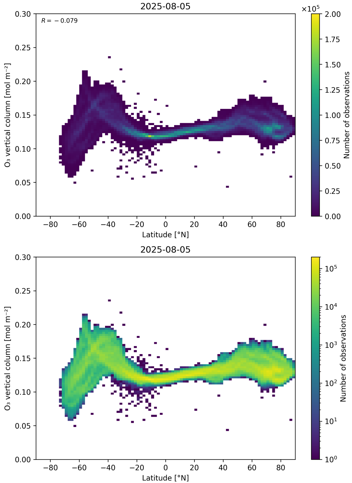
Figure 36: Scatter density plot of “Latitude” against “O 3 vertical column” for 2025-08-04 to 2025-08-06.
