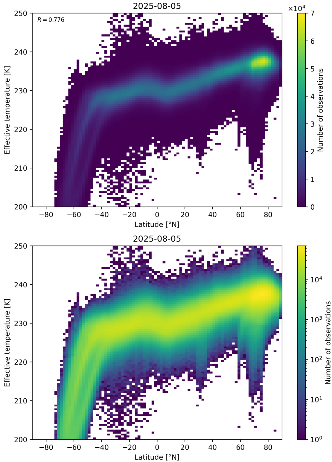
Figure 34: Scatter density plot of “Latitude” against “Effective temperature” for 2025-08-04 to 2025-08-06.
