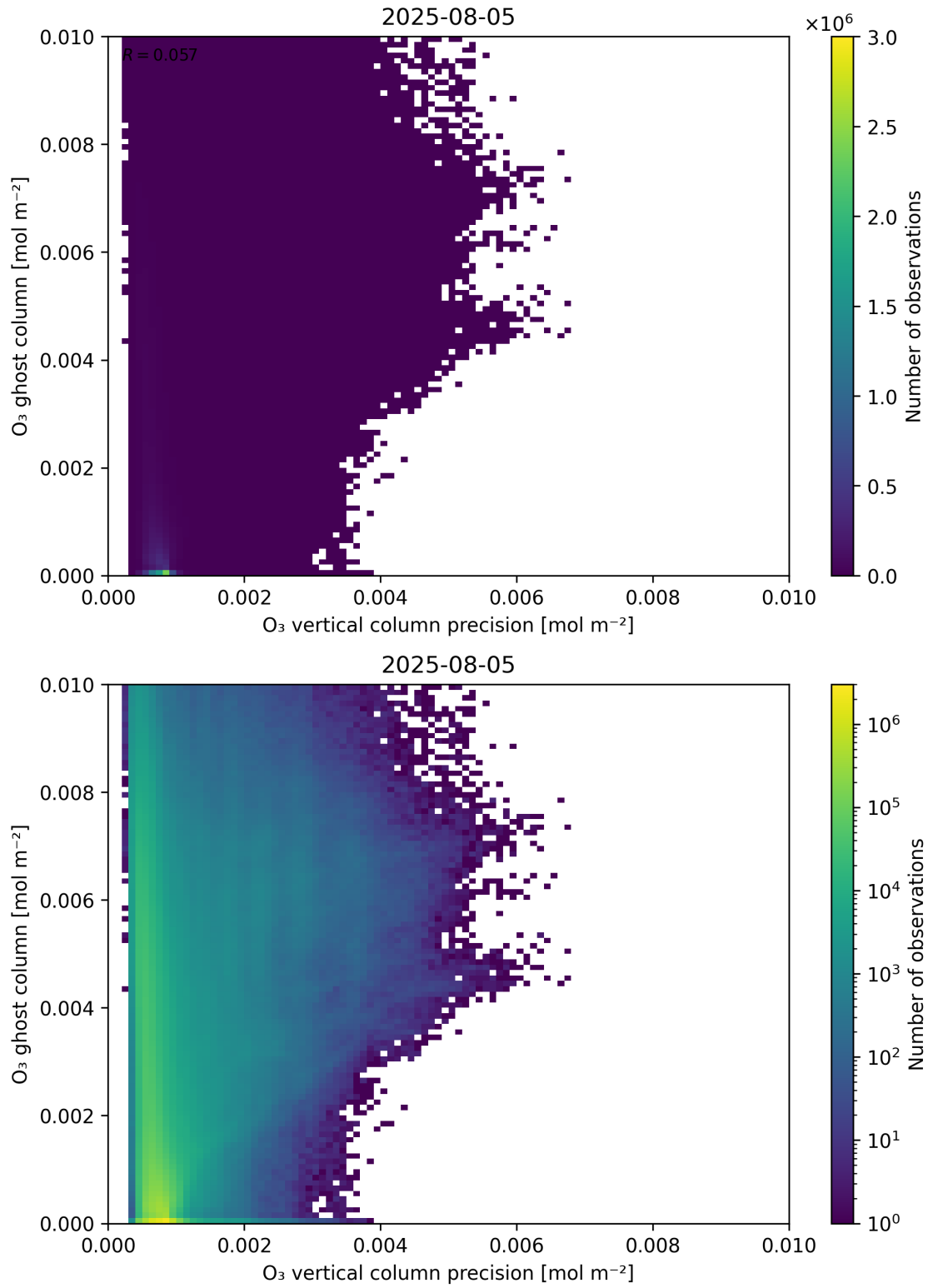
Figure 43: Scatter density plot of “O 3 vertical column precision” against “O 3 ghost column” for 2025-08-04 to 2025-08-06.
