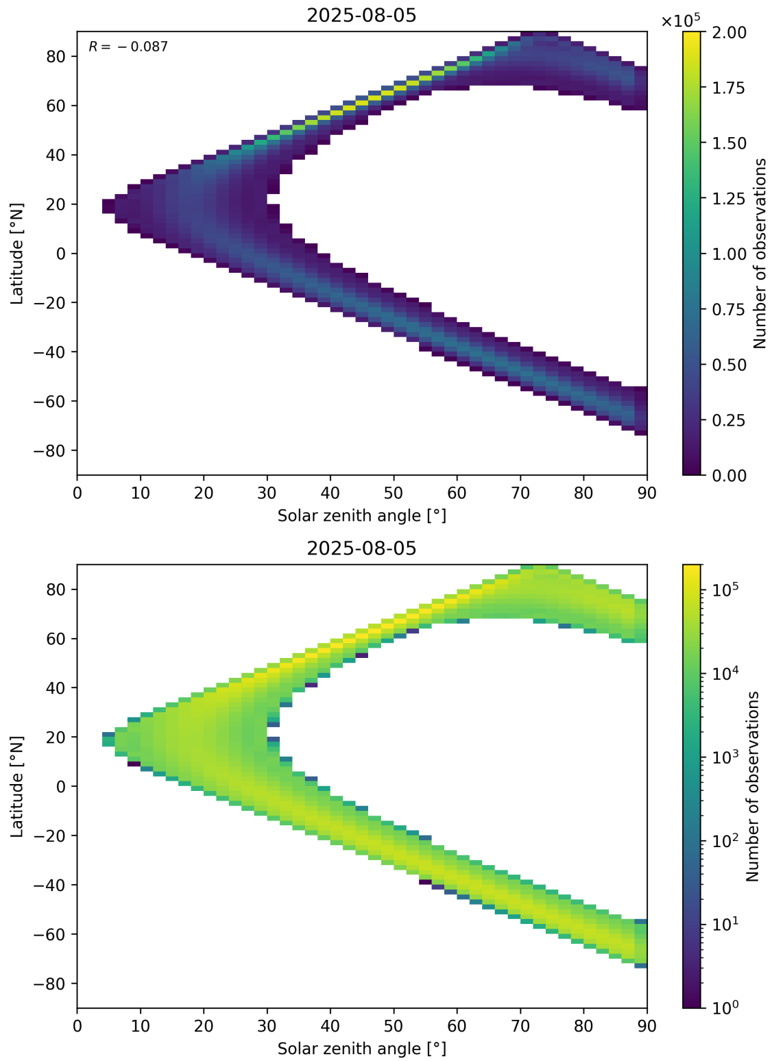
Figure 44: Scatter density plot of “Solar zenith angle” against “Latitude” for 2025-08-04 to 2025-08-06.
