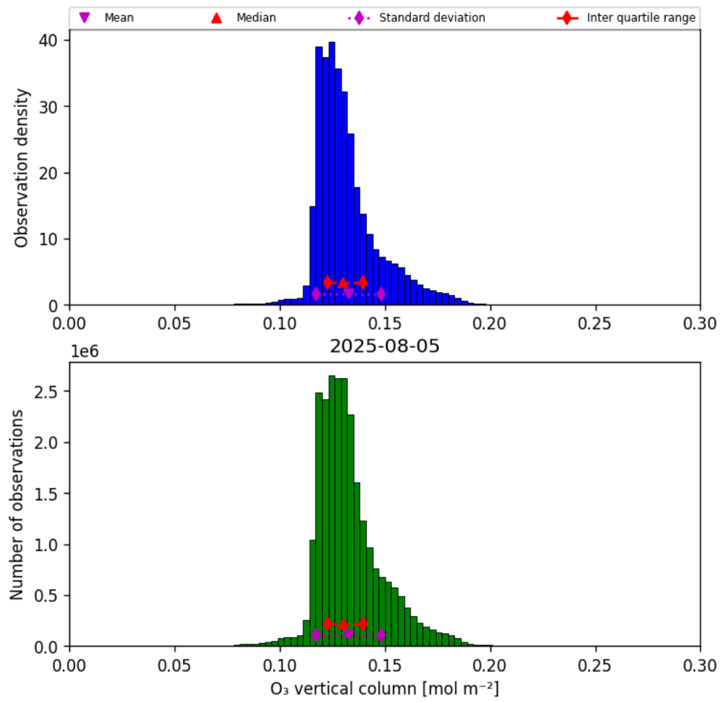
Figure 21: Histogram of “O 3 vertical column” for 2025-08-04 to 2025-08-06
