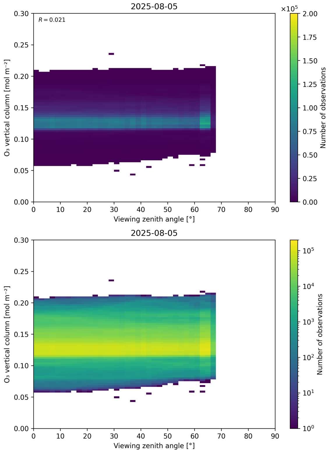
Figure 52: Scatter density plot of “Viewing zenith angle” against “O 3 vertical column” for 2025-08-04 to 2025-08-06.
