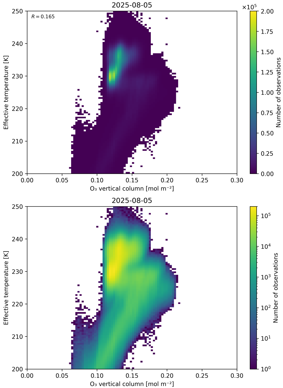
Figure 39: Scatter density plot of “O 3 vertical column” against “Effective temperature” for 2025-08-04 to 2025-08-06.
