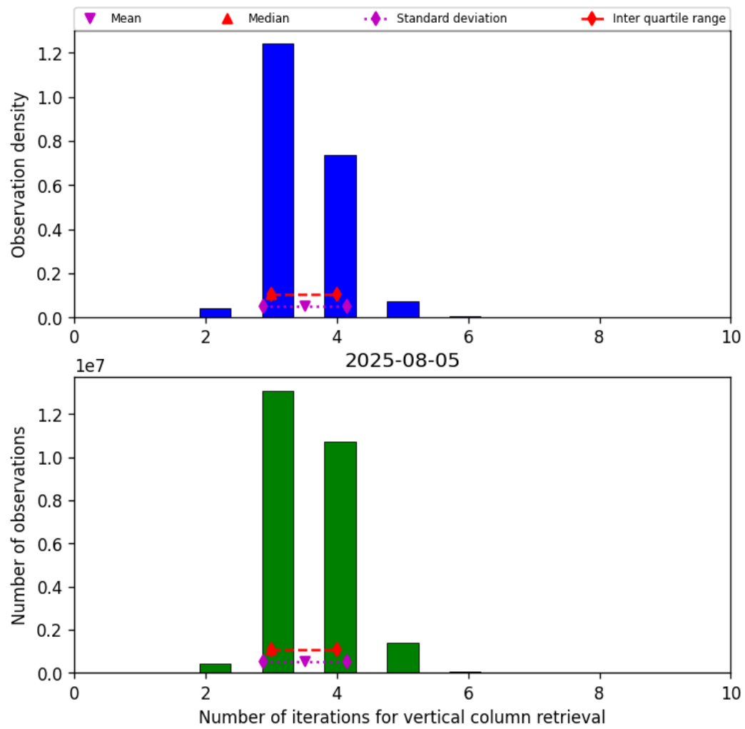
Figure 26: Histogram of “Number of iterations for vertical column retrieval” for 2025-08-04 to 2025-08-06
