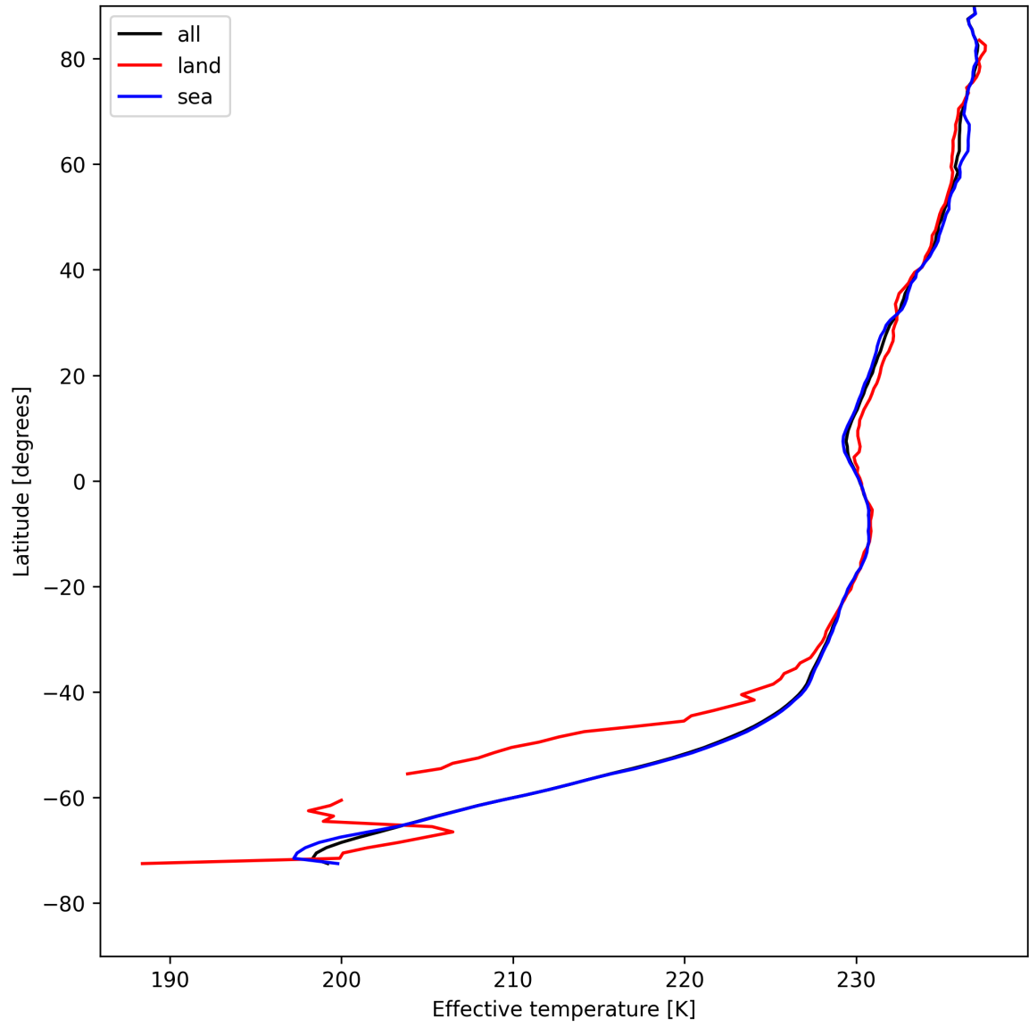
Figure 17: Zonal average of "Effective temperature" for 2025-08-04 to 2025-08-06.
