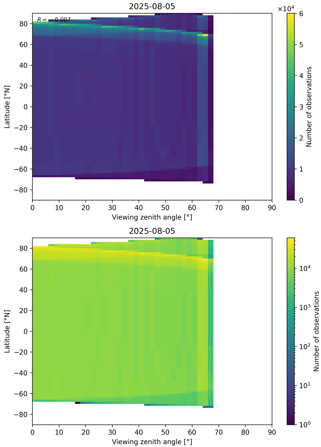
Figure 49: Scatter density plot of “Viewing zenith angle” against “Latitude” for 2025-08-04 to 2025-08-06.
