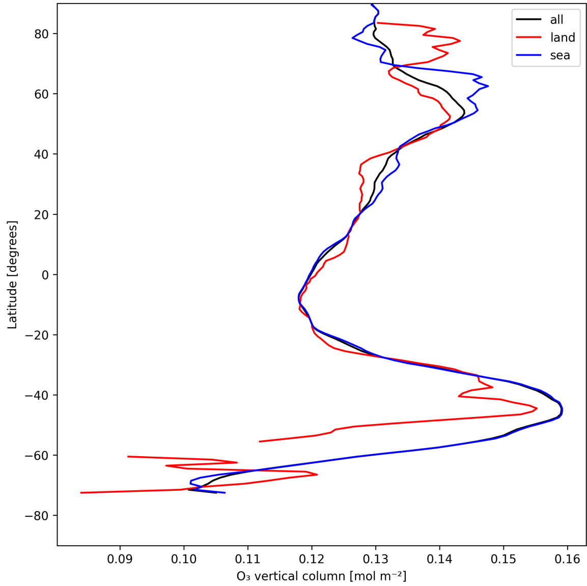
Figure 14: Zonal average of “O 3 vertical column” for 2025-08-04 to 2025-08-06.
