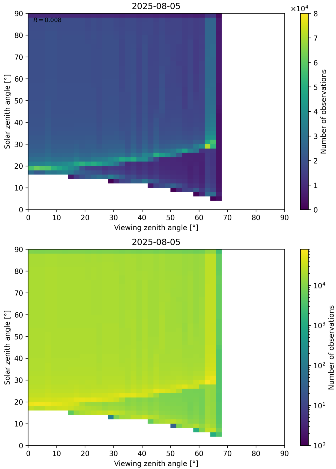
Figure 54: Scatter density plot of “Viewing zenith angle” against “Solar zenith angle” for 2025-08-04 to 2025-08-06.
