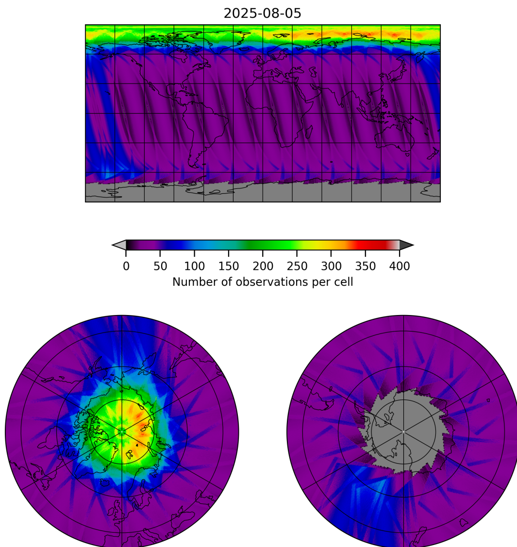
Figure 12: Map of the number of observations for 2025-08-04 to 2025-08-06
