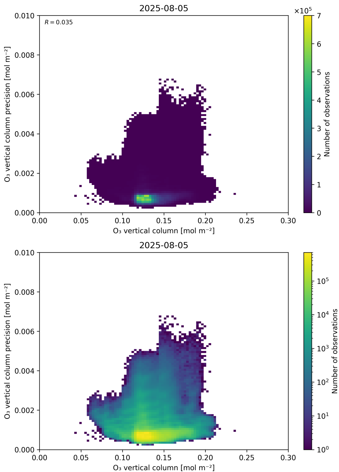
Figure 41: Scatter density plot of “O 3 vertical column” against “O 3 vertical column precision” for 2025-08-04 to 2025-08-06.
