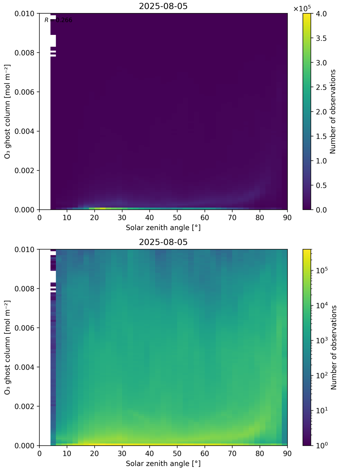
Figure 46: Scatter density plot of “Solar zenith angle” against “O 3 ghost column” for 2025-08-04 to 2025-08-06.
