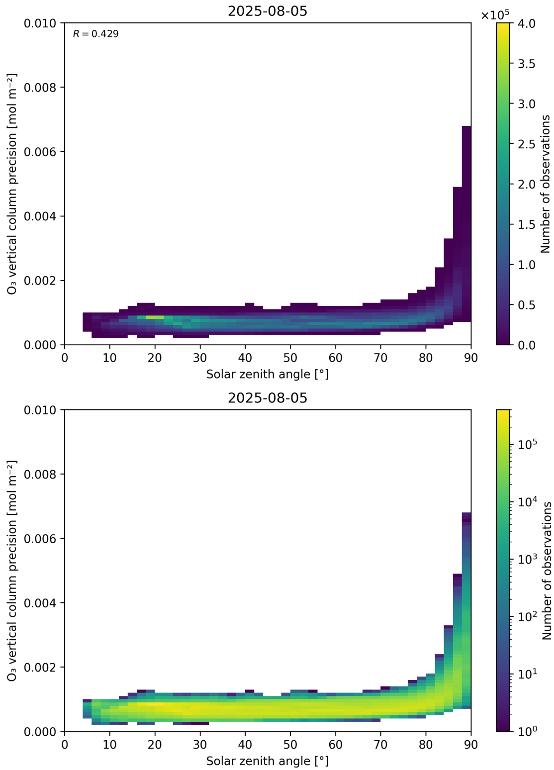
Figure 48: Scatter density plot of “Solar zenith angle” against “O 3 vertical column precision” for 2025-08-04 to 2025-08-06.
