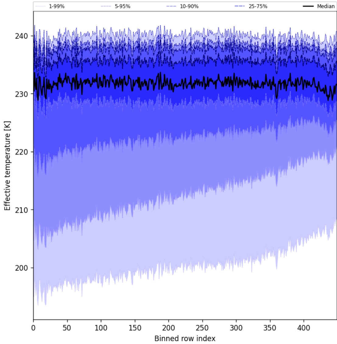
Figure 31: Along track statistics of “Effective temperature” for 2025-08-04 to 2025-08-06
