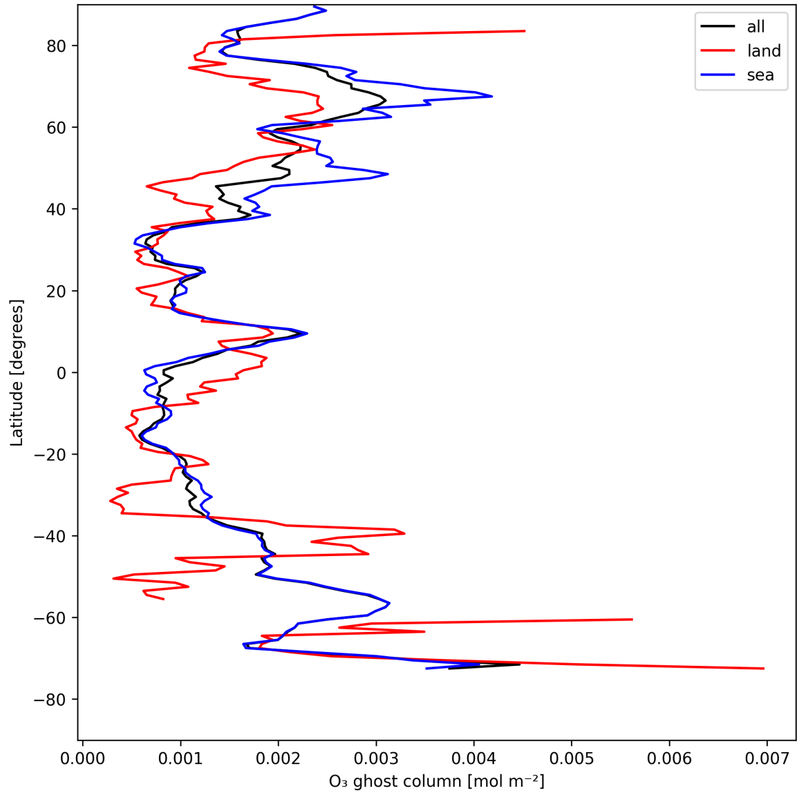
Figure 18: Zonal average of "O 3 ghost column" for 2025-08-04 to 2025-08-06.
