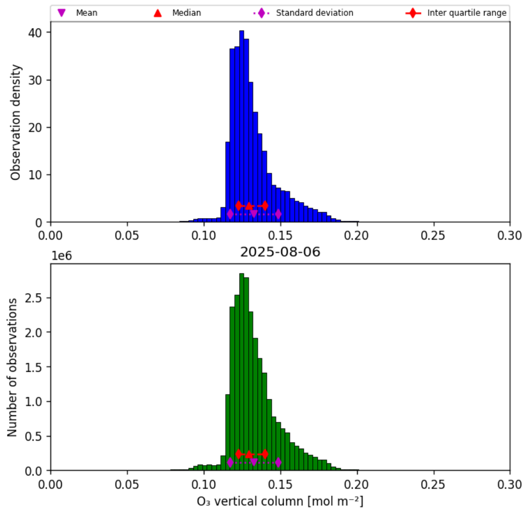
Figure 21: Histogram of “O 3 vertical column” for 2025-08-05 to 2025-08-07
