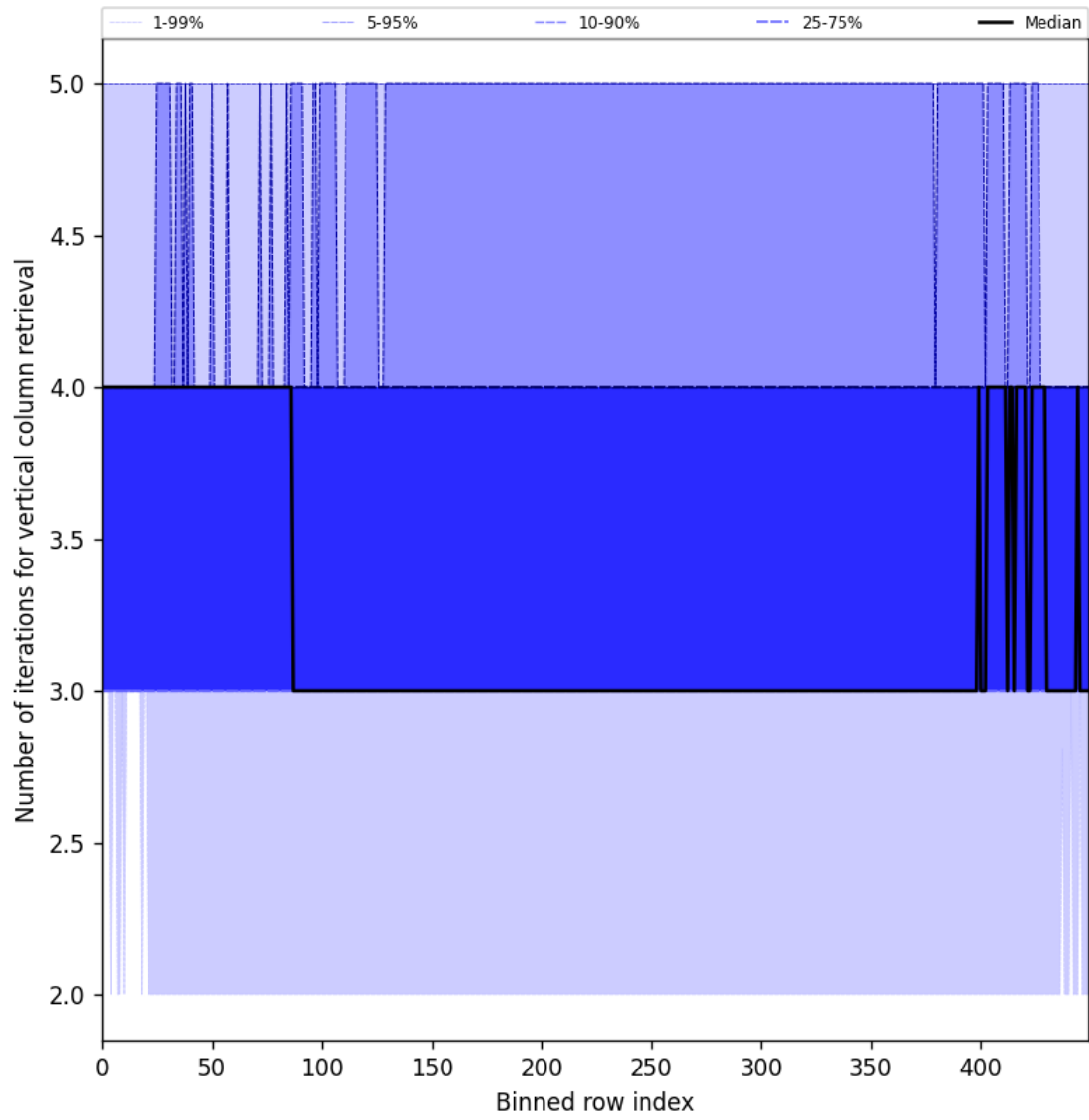
Figure 33: Along track statistics of “Number of iterations for vertical column retrieval” for 2025-08-05 to 2025-08-07
