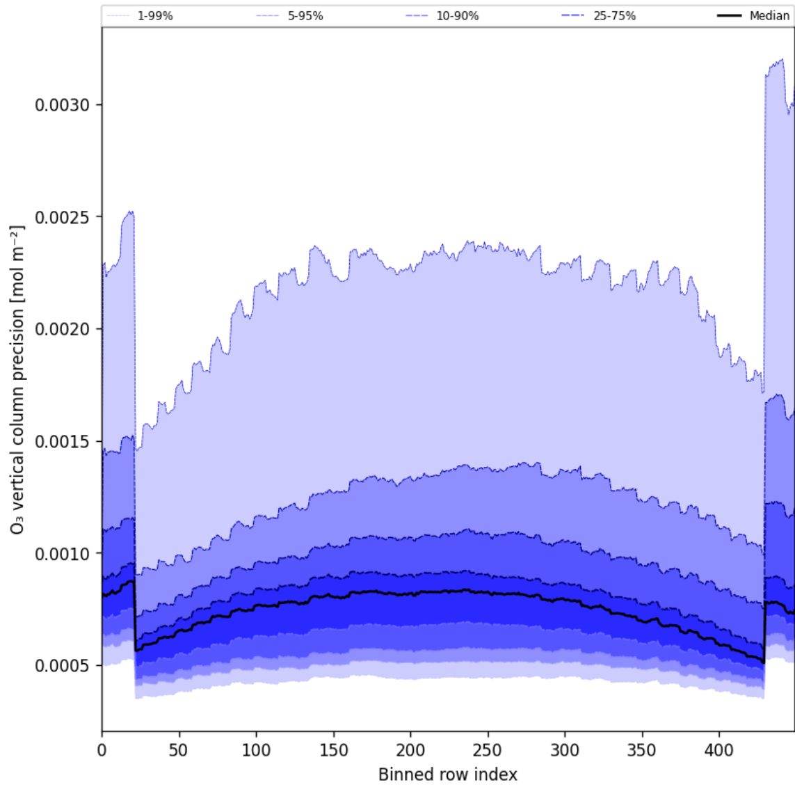
Figure 29: Along track statistics of “O 3 vertical column precision” for 2025-08-05 to 2025-08-07
