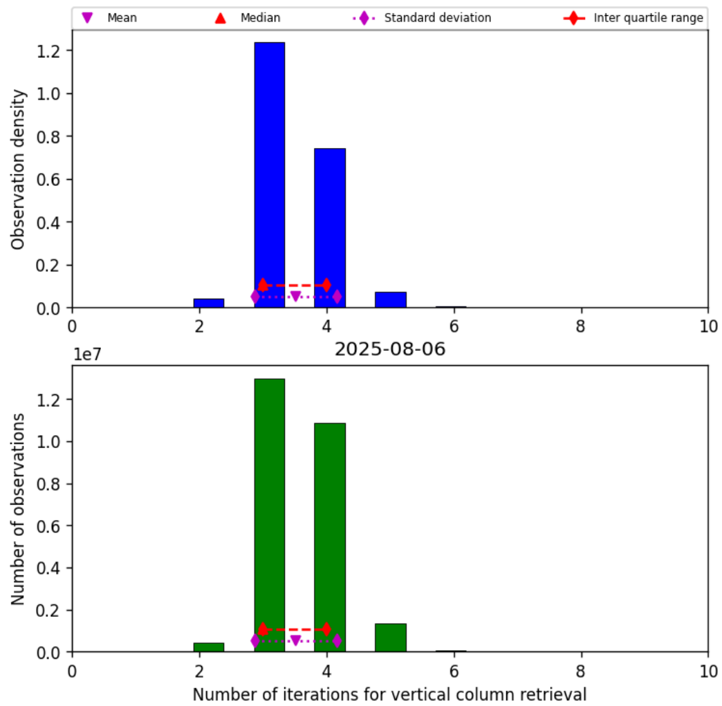
Figure 26: Histogram of “Number of iterations for vertical column retrieval” for 2025-08-05 to 2025-08-07
