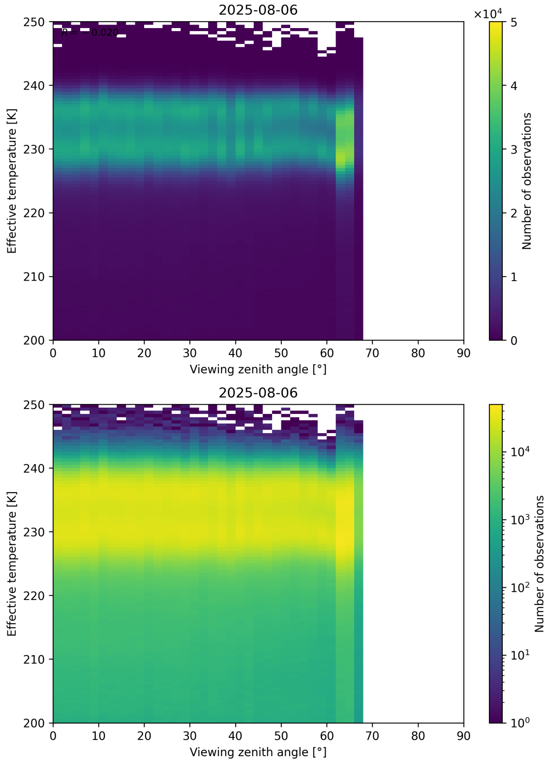
Figure 50: Scatter density plot of “Viewing zenith angle” against “Effective temperature” for 2025-08-05 to 2025-08-07.
