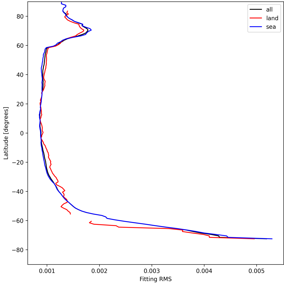
Figure 16: Zonal average of “Fitting RMS” for 2025-08-05 to 2025-08-07.
