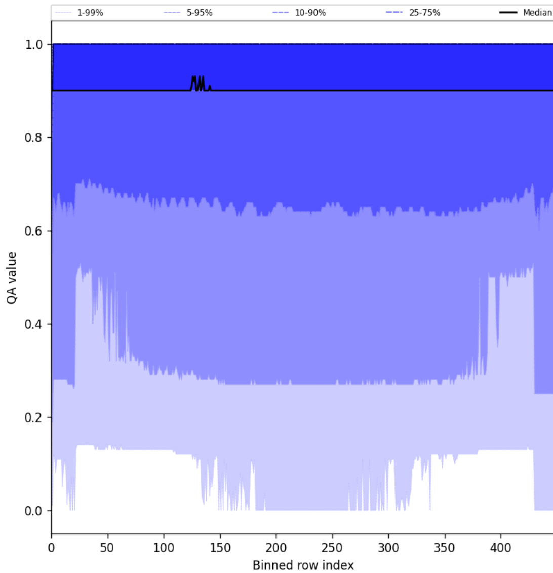
Figure 27: Along track statistics of “QA value” for 2025-08-05 to 2025-08-07
