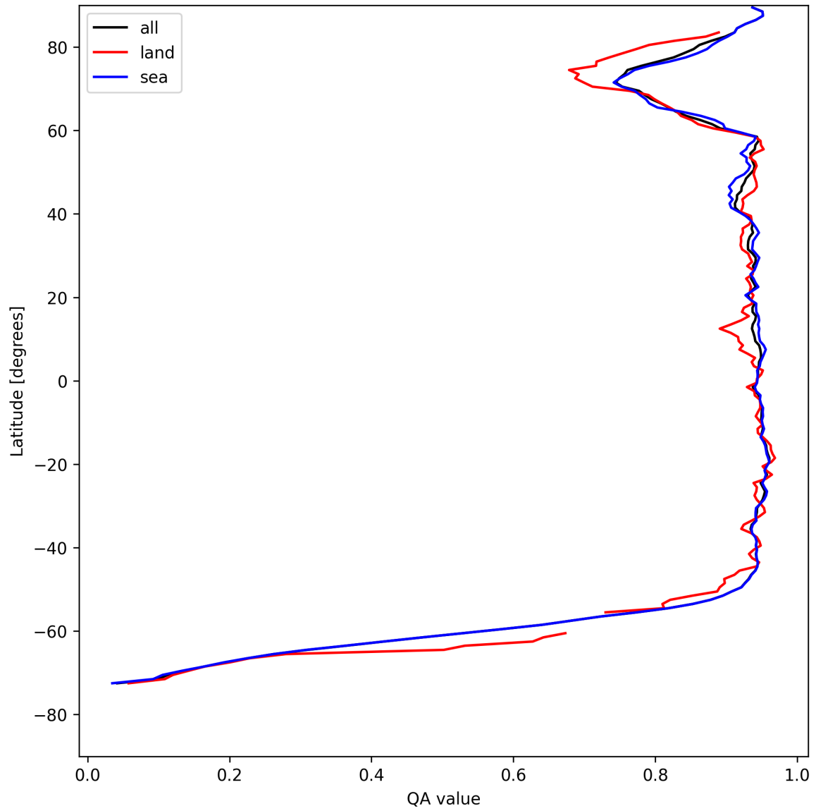
Figure 13: Zonal average of “QA value” for 2025-08-05 to 2025-08-07.
