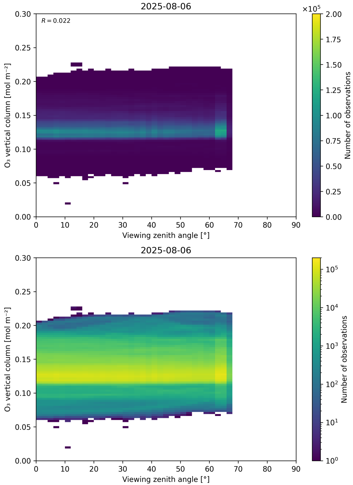
Figure 52: Scatter density plot of “Viewing zenith angle” against “O 3 vertical column” for 2025-08-05 to 2025-08-07.
