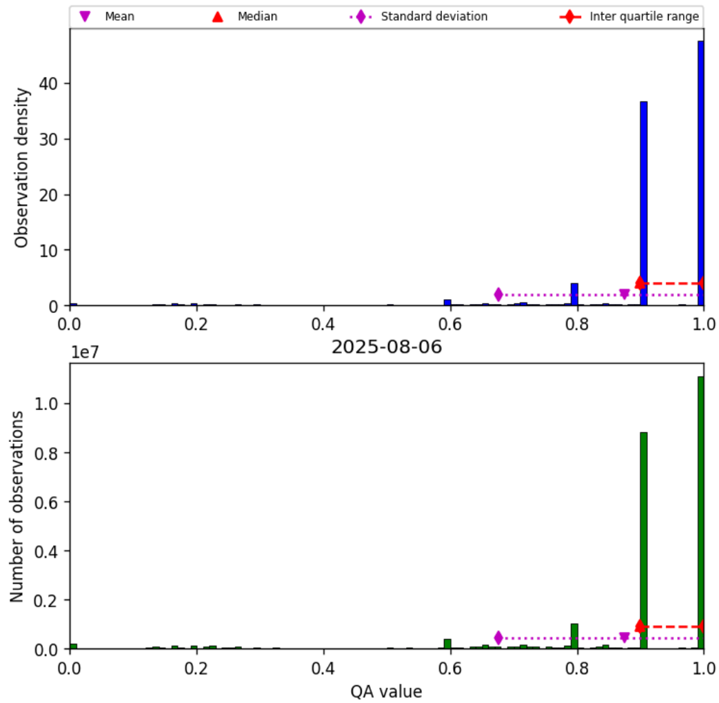
Figure 20: Histogram of “QA value” for 2025-08-05 to 2025-08-07
