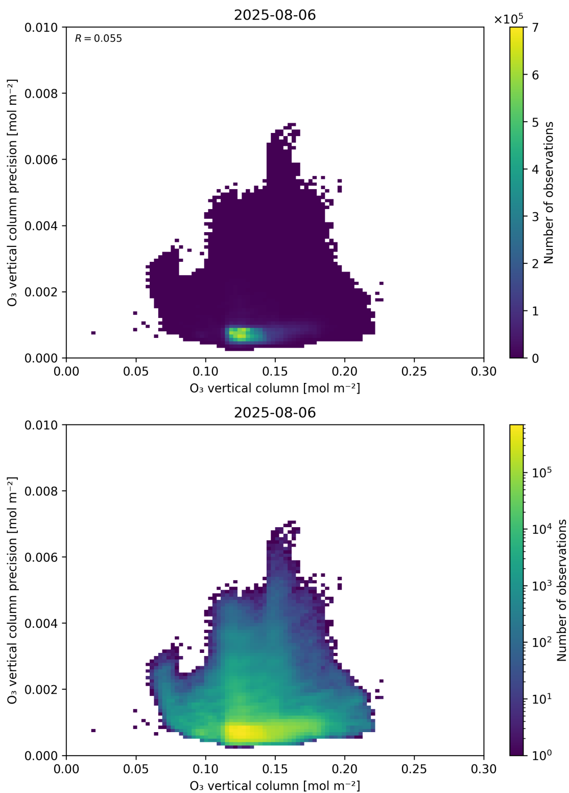
Figure 41: Scatter density plot of “O 3 vertical column” against “O 3 vertical column precision” for 2025-08-05 to 2025-08-07.
