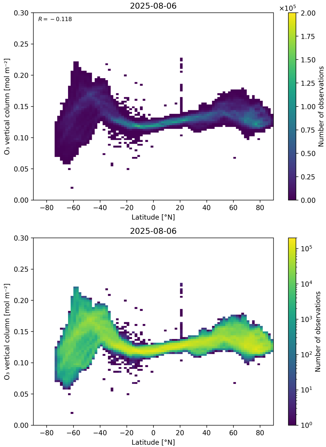
Figure 36: Scatter density plot of “Latitude” against “O 3 vertical column” for 2025-08-05 to 2025-08-07.
