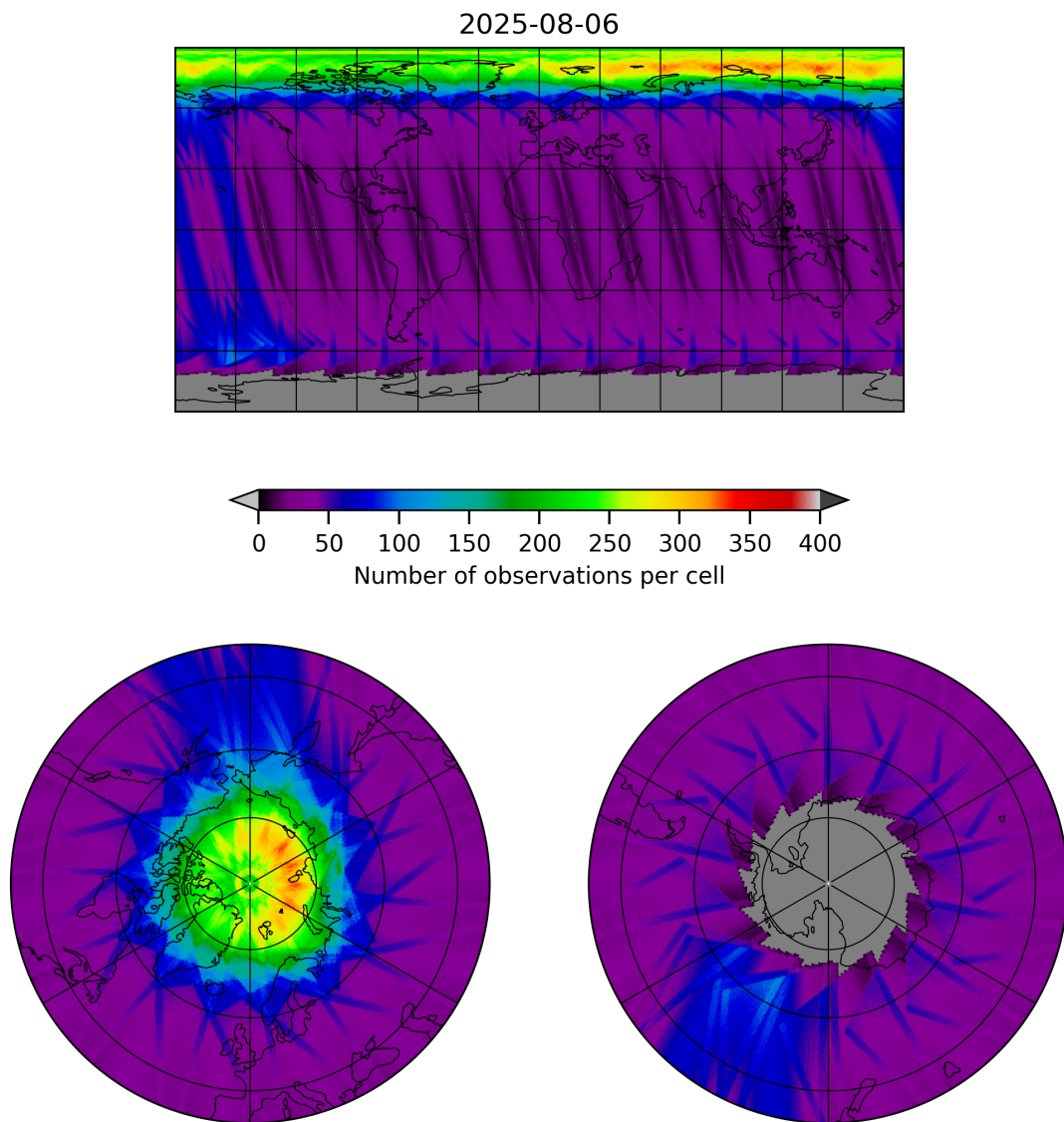
Figure 12: Map of the number of observations for 2025-08-05 to 2025-08-07
