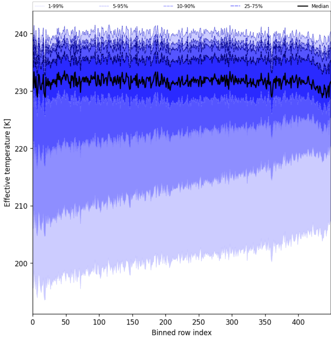
Figure 31: Along track statistics of “Effective temperature” for 2025-08-05 to 2025-08-07
