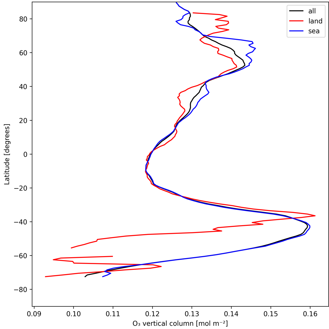
Figure 14: Zonal average of “O 3 vertical column” for 2025-08-05 to 2025-08-07.
