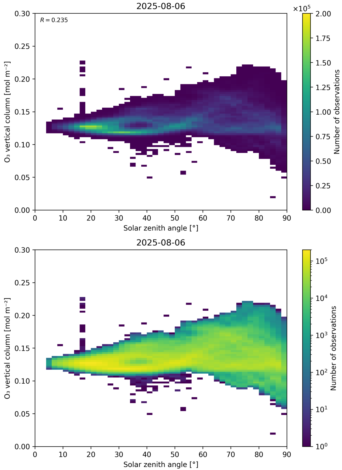
Figure 47: Scatter density plot of “Solar zenith angle” against “O 3 vertical column” for 2025-08-05 to 2025-08-07.
