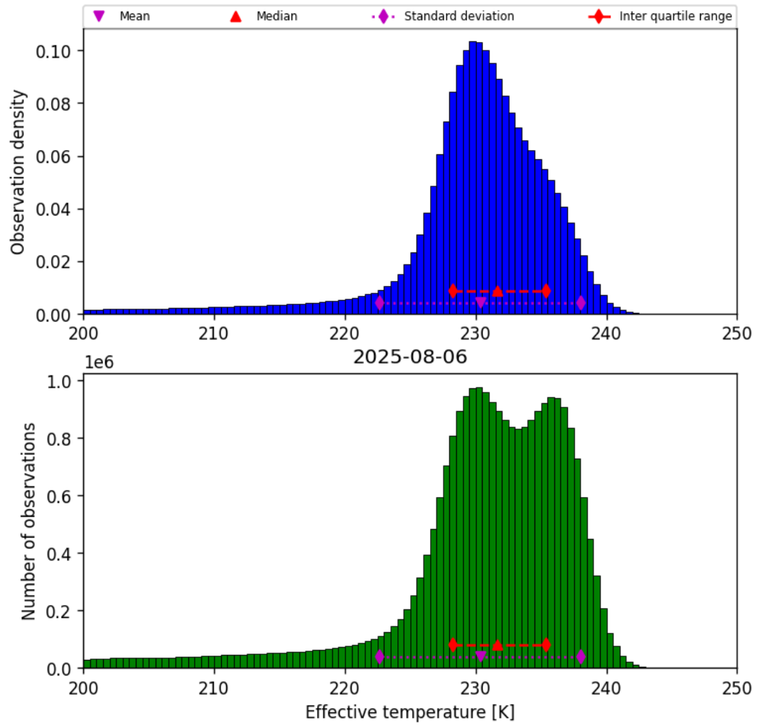
Figure 24: Histogram of “Effective temperature” for 2025-08-05 to 2025-08-07
