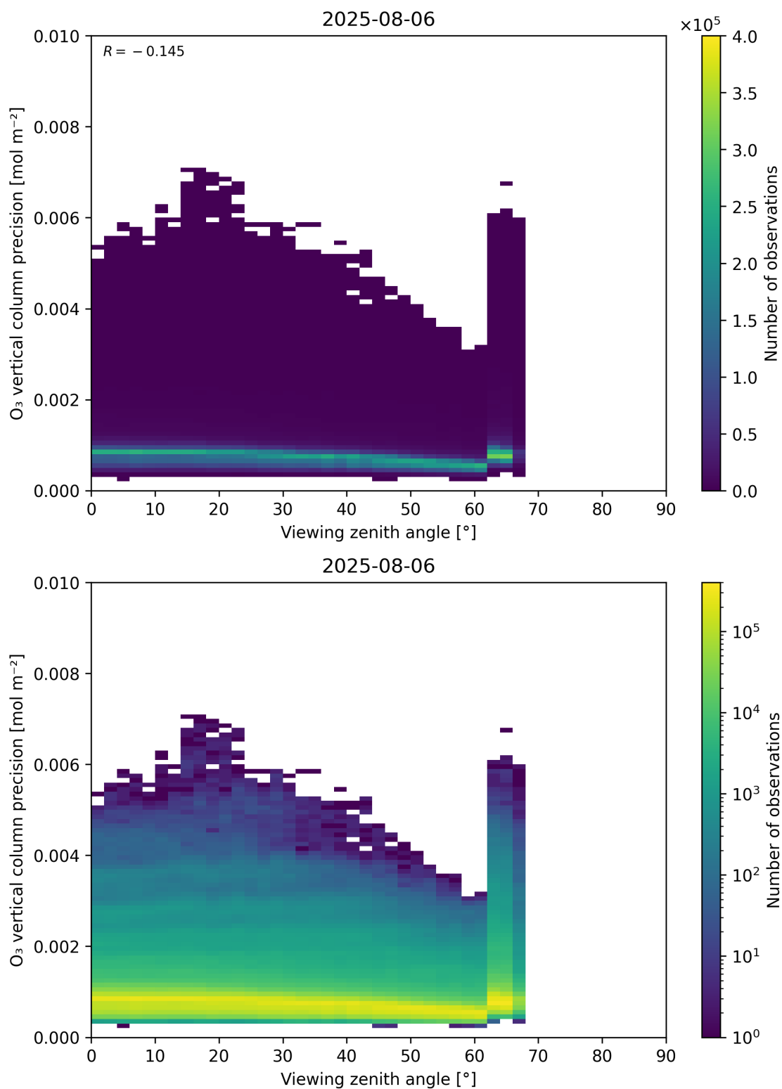
Figure 53: Scatter density plot of “Viewing zenith angle” against “O 3 vertical column precision” for 2025-08-05 to 2025-08-07.
