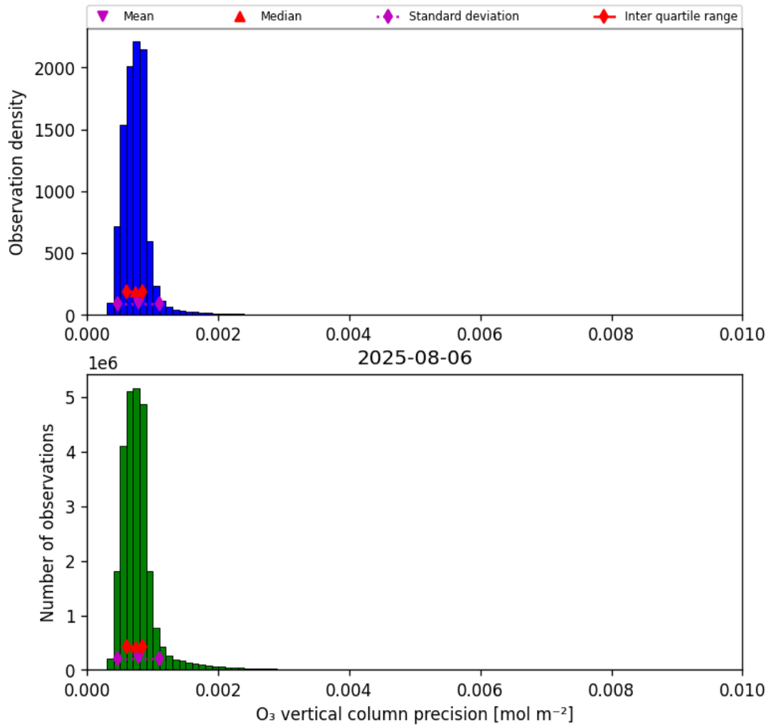
Figure 22: Histogram of “O 3 vertical column precision” for 2025-08-05 to 2025-08-07
