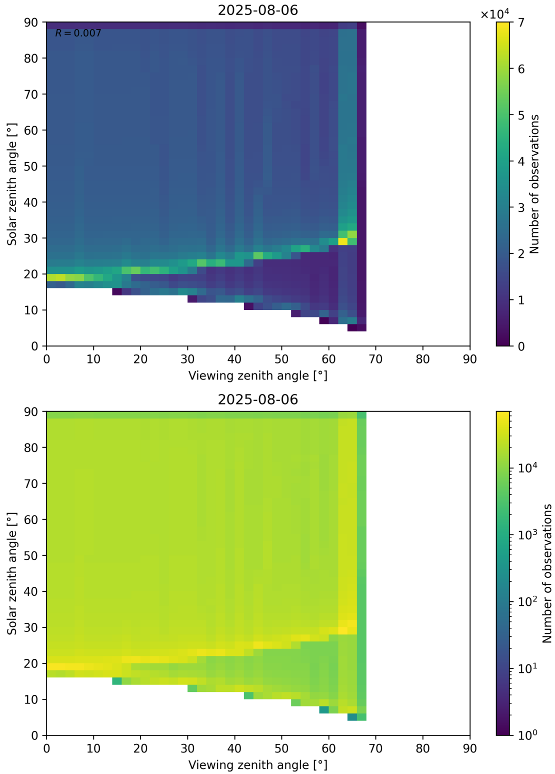
Figure 54: Scatter density plot of “Viewing zenith angle” against “Solar zenith angle” for 2025-08-05 to 2025-08-07.
