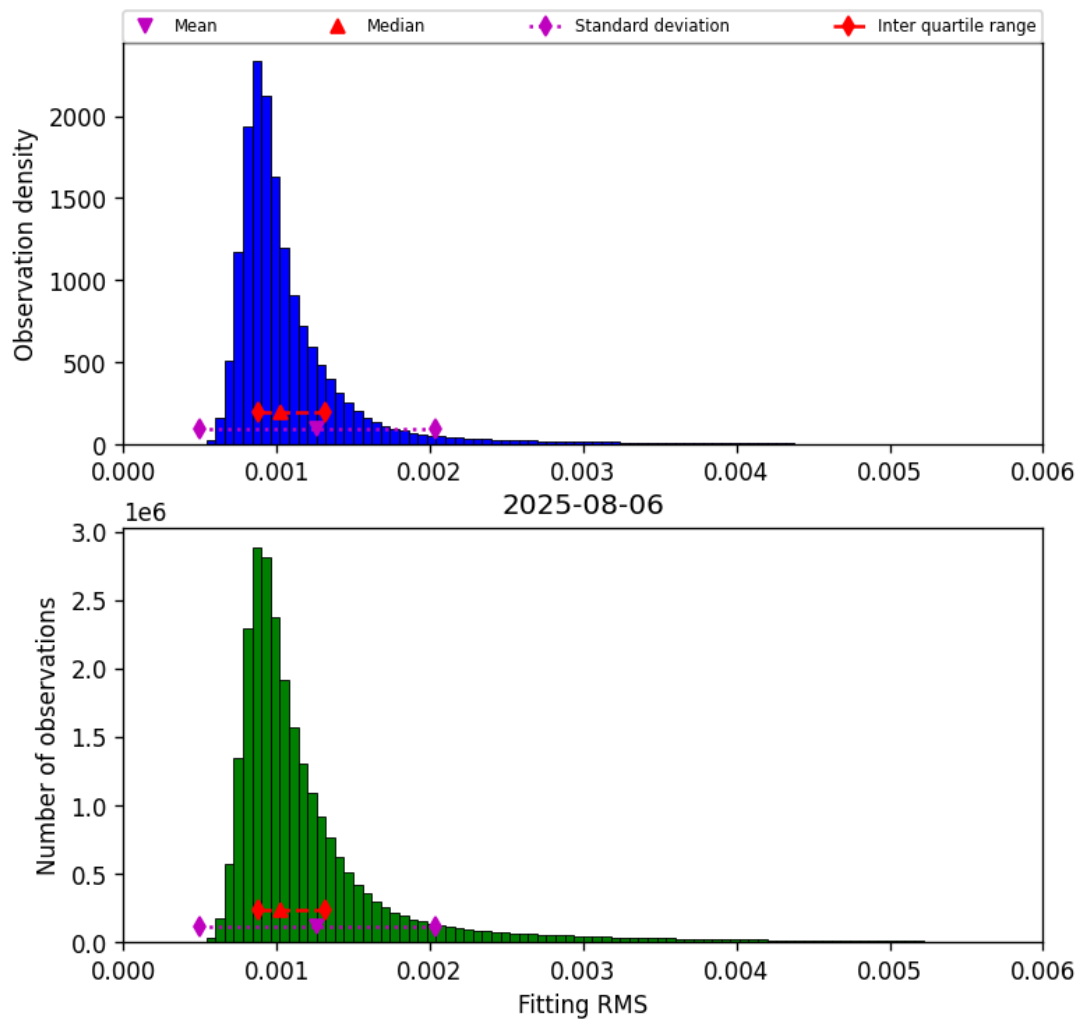
Figure 23: Histogram of “Fitting RMS” for 2025-08-05 to 2025-08-07
