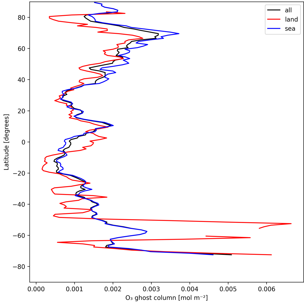
Figure 18: Zonal average of "O 3 ghost column" for 2025-08-05 to 2025-08-07.
