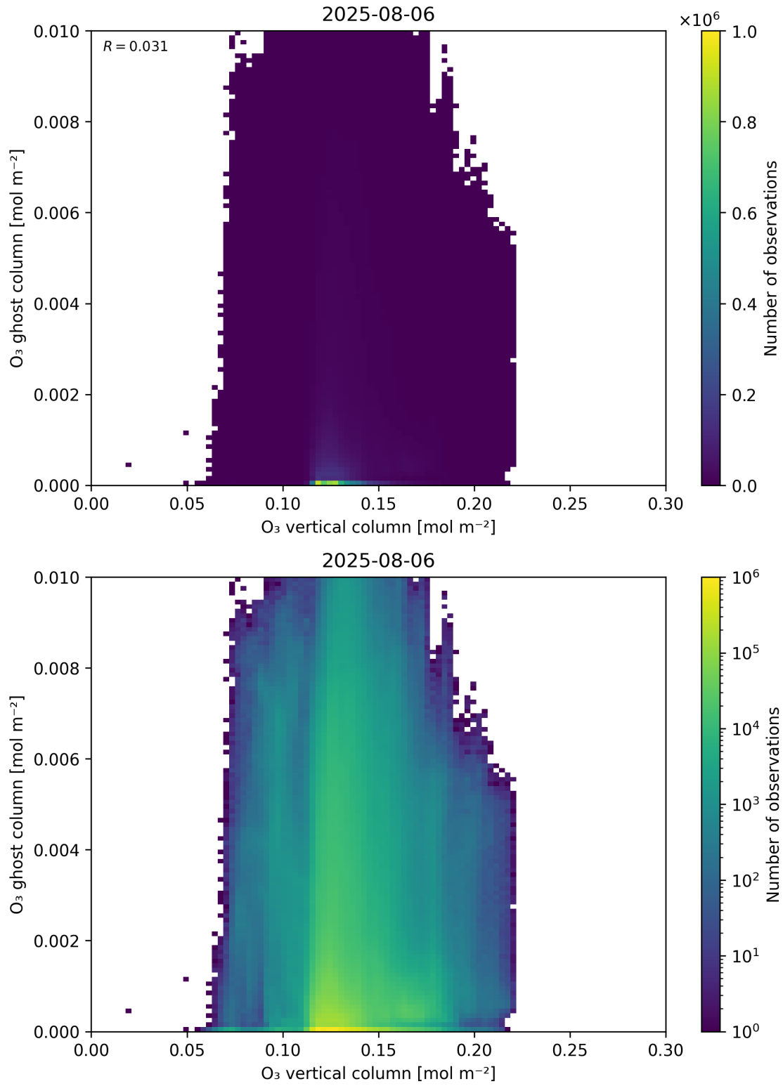
Figure 40: Scatter density plot of “O 3 vertical column” against “O 3 ghost column” for 2025-08-05 to 2025-08-07.
