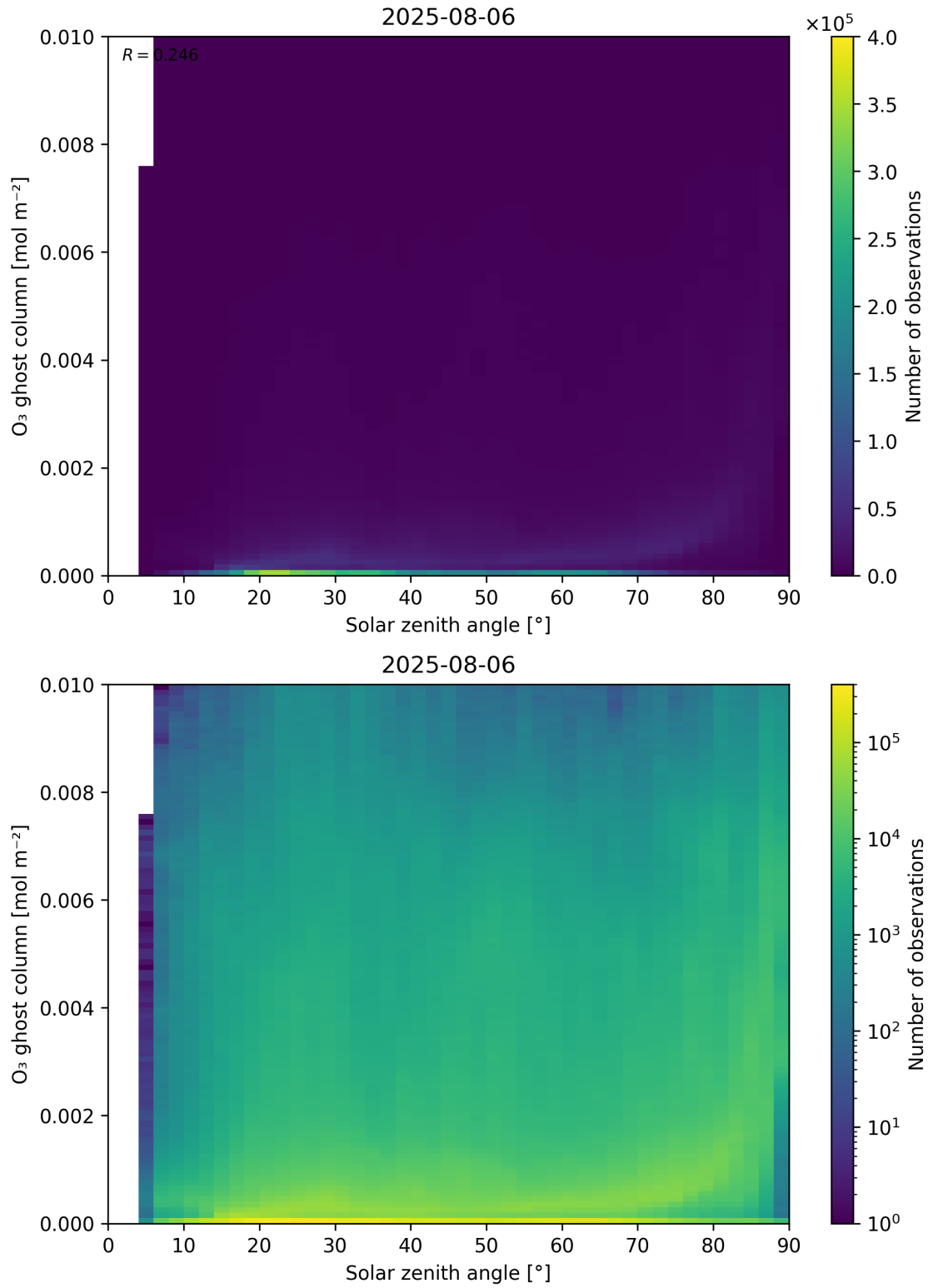
Figure 46: Scatter density plot of “Solar zenith angle” against “O 3 ghost column” for 2025-08-05 to 2025-08-07.
