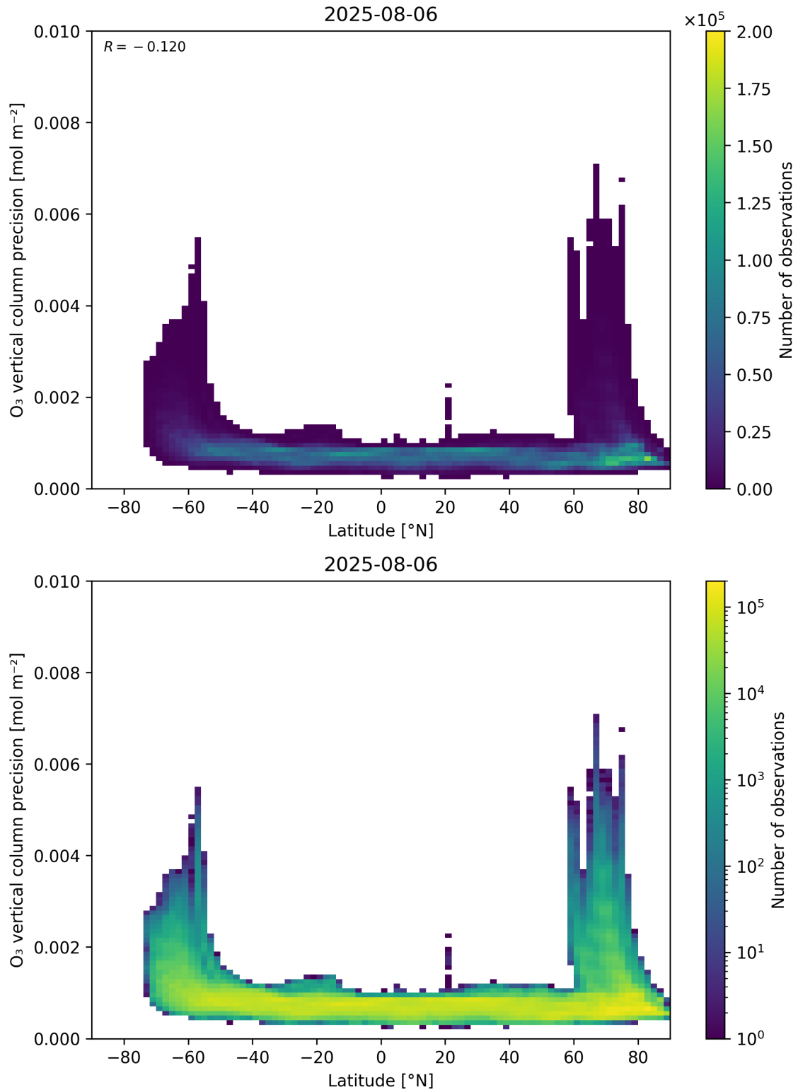
Figure 37: Scatter density plot of “Latitude” against “O 3 vertical column precision” for 2025-08-05 to 2025-08-07.
