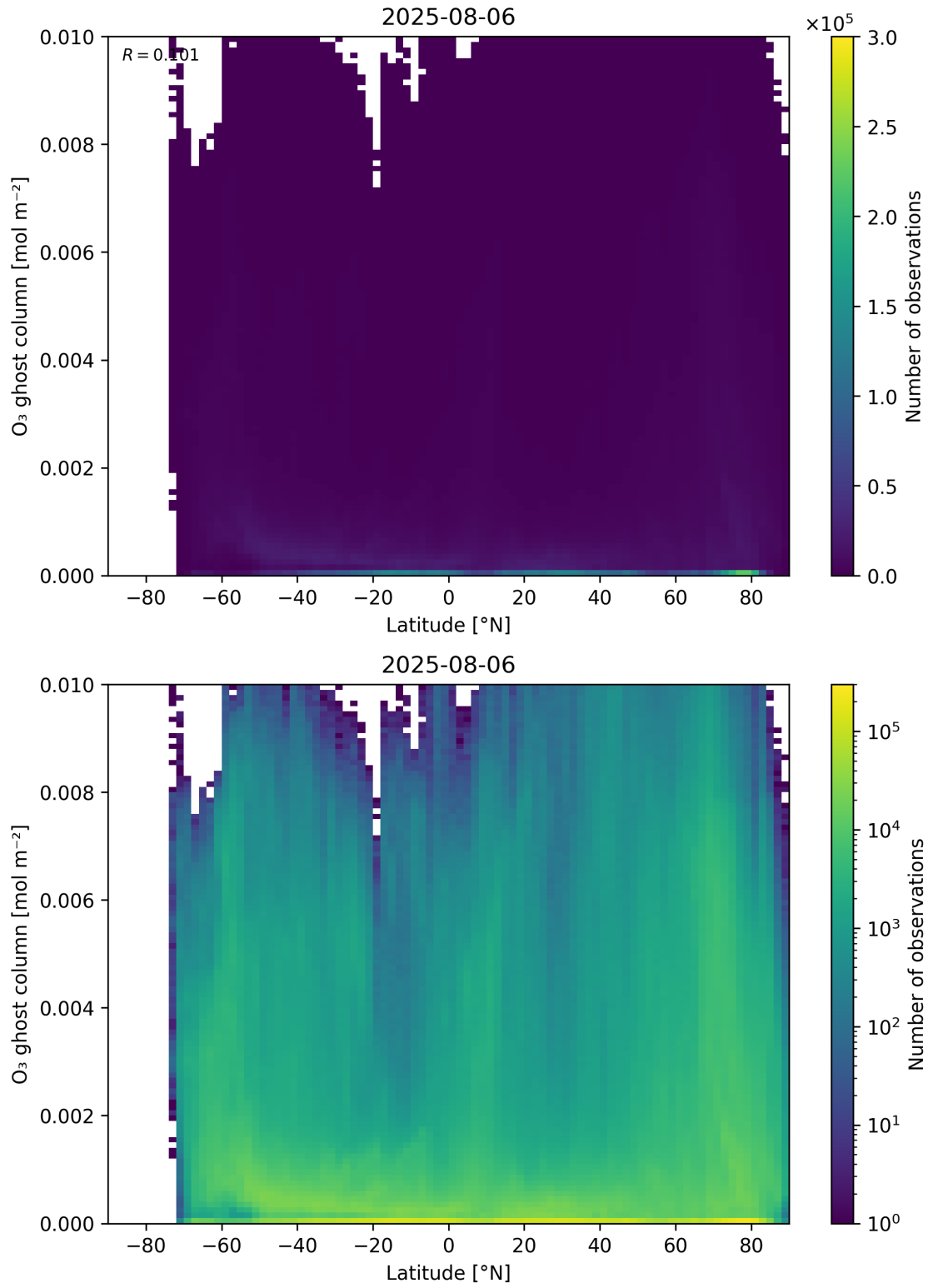
Figure 35: Scatter density plot of “Latitude” against “O 3 ghost column” for 2025-08-05 to 2025-08-07.
