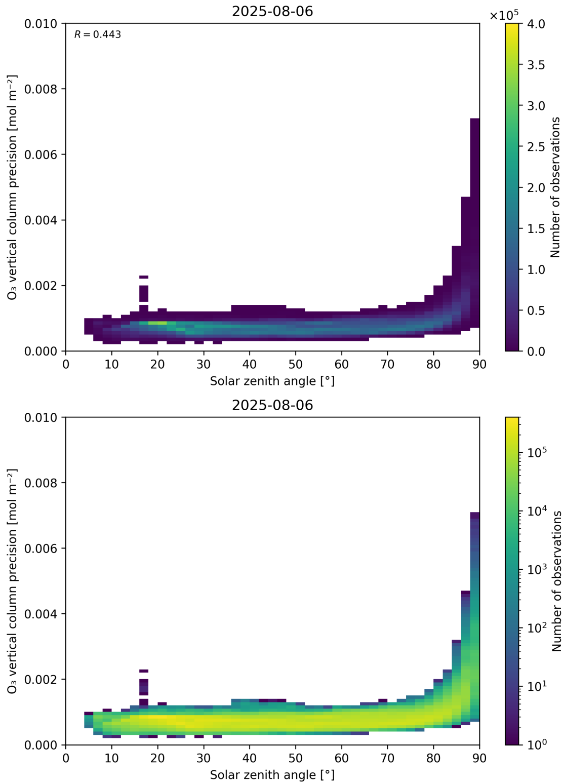
Figure 48: Scatter density plot of “Solar zenith angle” against “O 3 vertical column precision” for 2025-08-05 to 2025-08-07.
