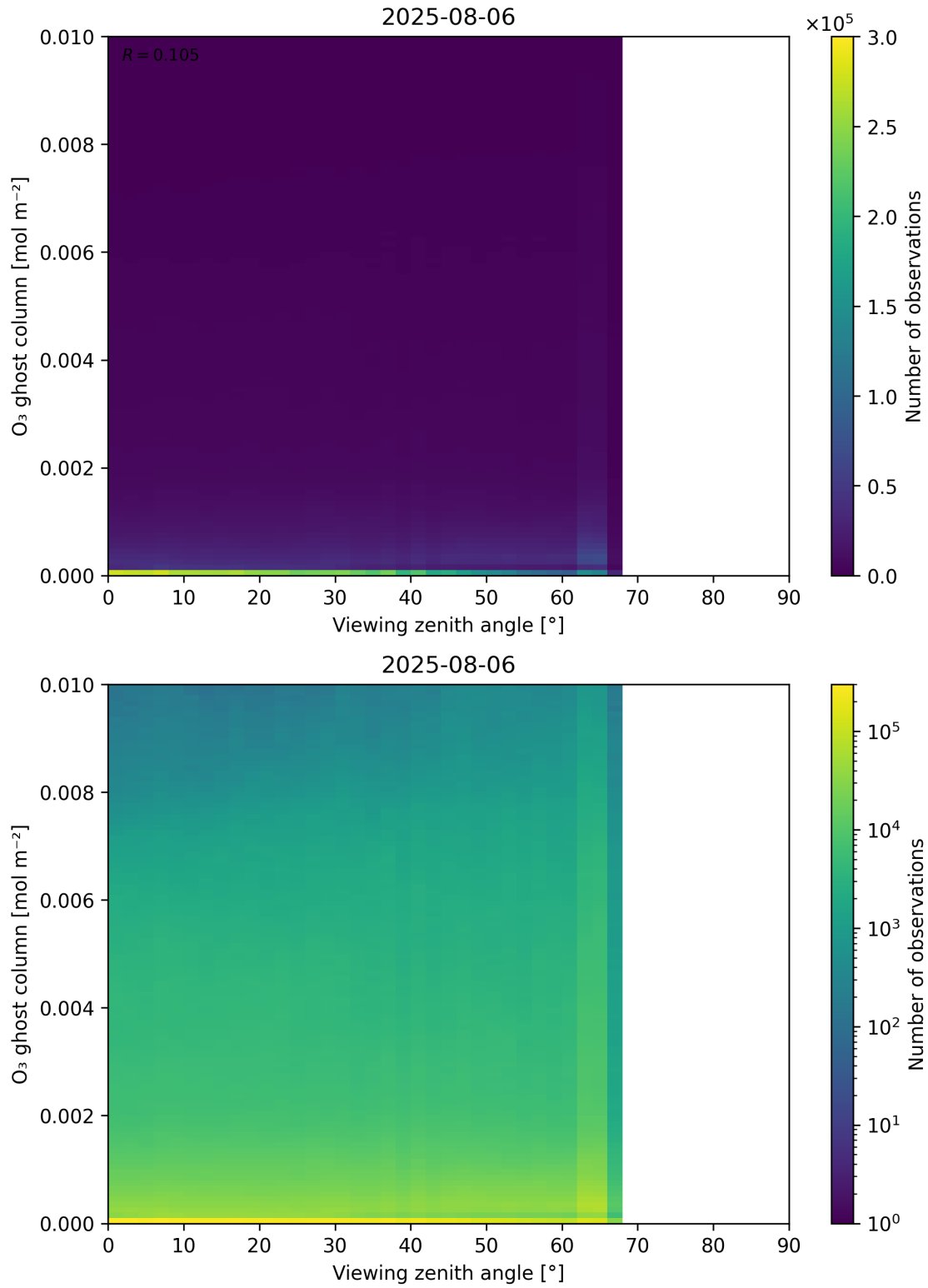
Figure 51: Scatter density plot of “Viewing zenith angle” against “O 3 ghost column” for 2025-08-05 to 2025-08-07.
