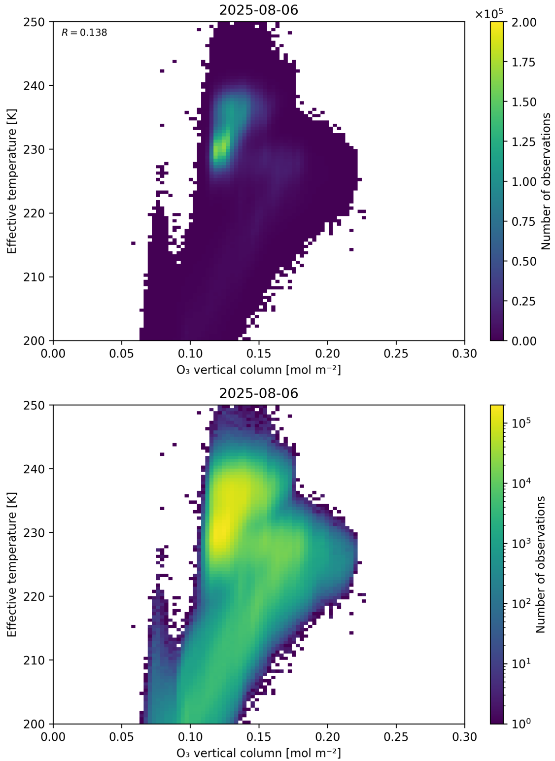
Figure 39: Scatter density plot of “O 3 vertical column” against “Effective temperature” for 2025-08-05 to 2025-08-07.
