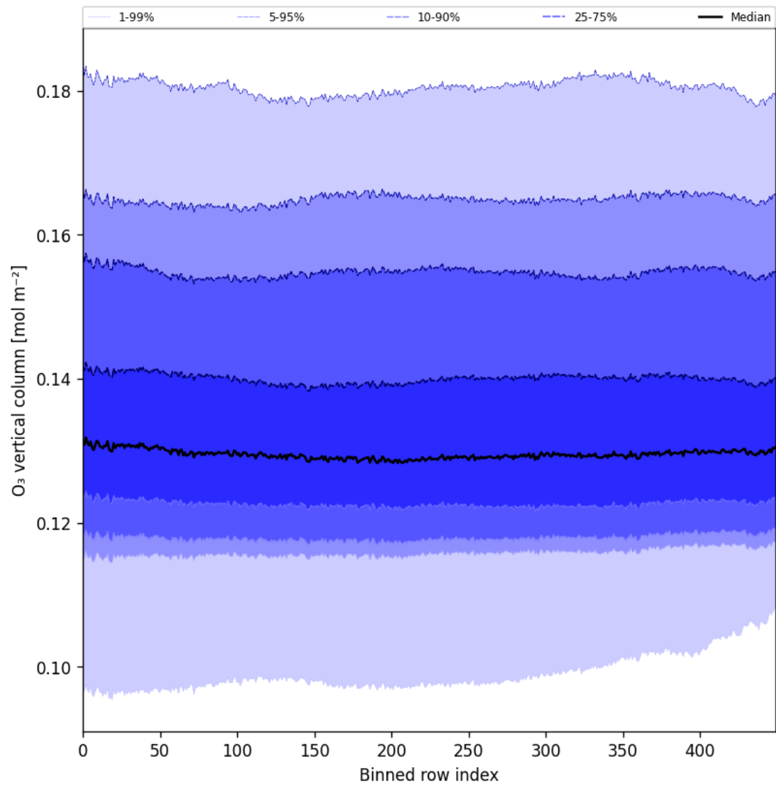
Figure 28: Along track statistics of “O 3 vertical column” for 2025-08-05 to 2025-08-07
