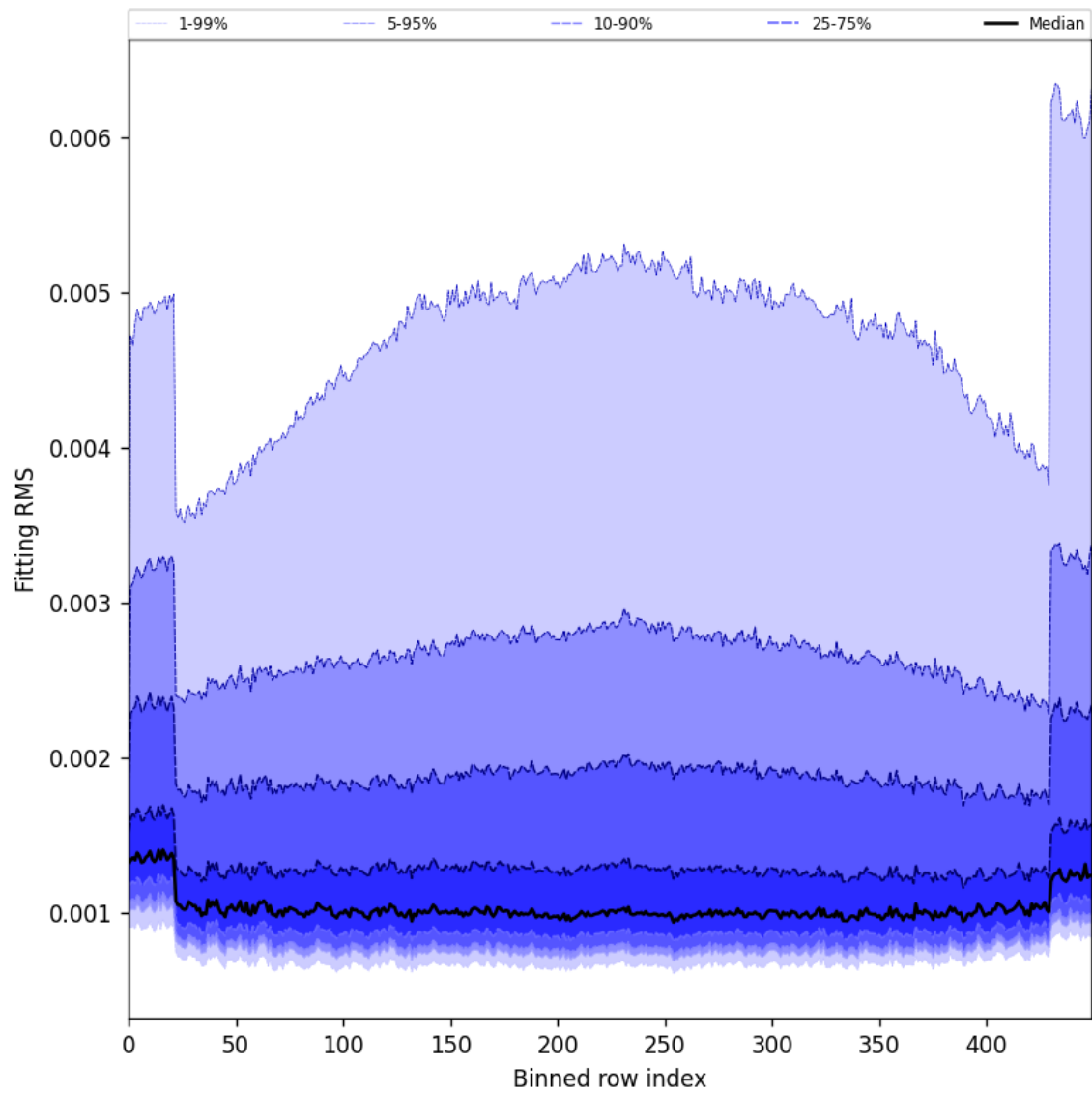
Figure 30: Along track statistics of “Fitting RMS” for 2025-08-05 to 2025-08-07
