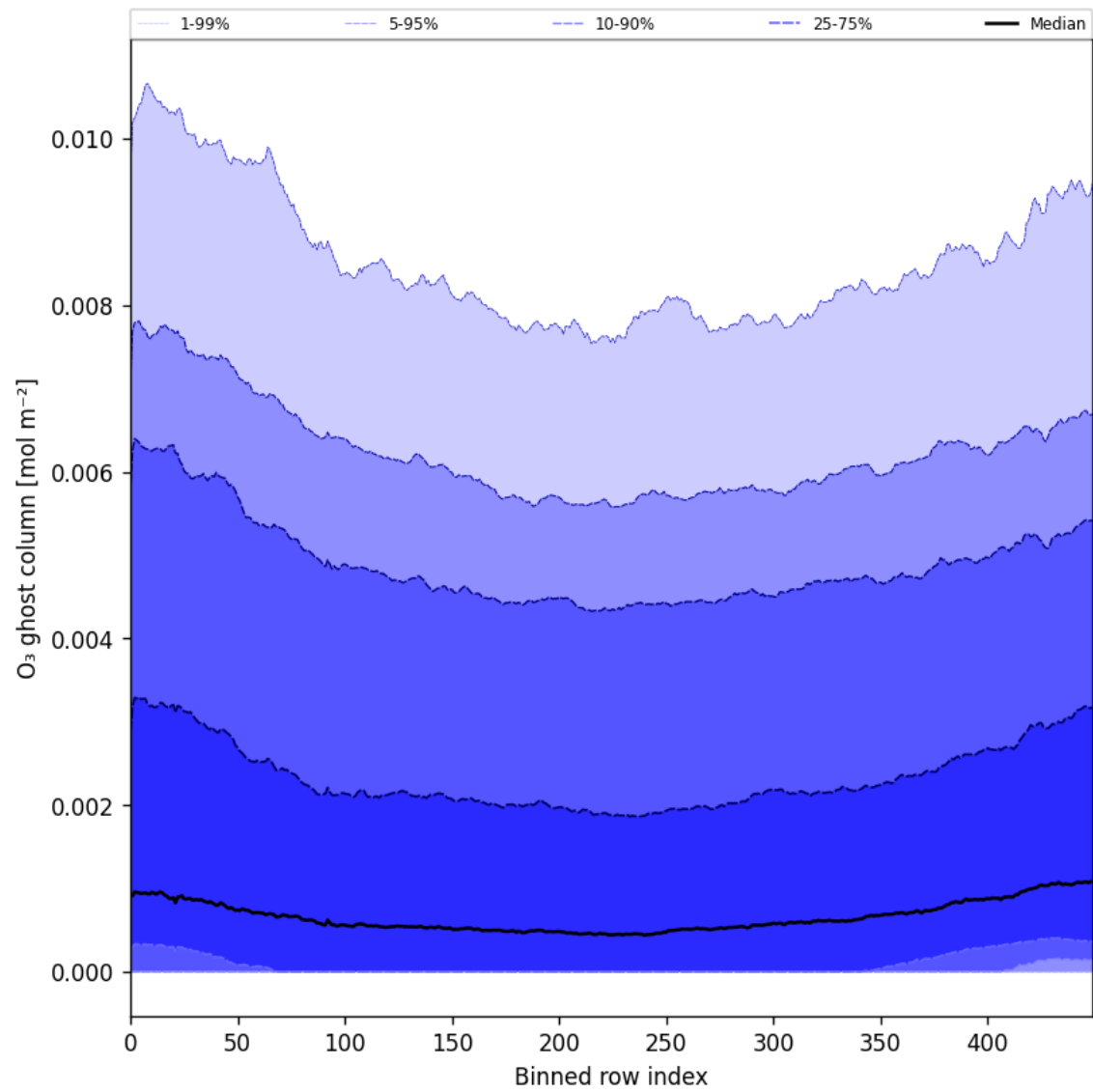
Figure 32: Along track statistics of “O 3 ghost column” for 2025-08-05 to 2025-08-07
