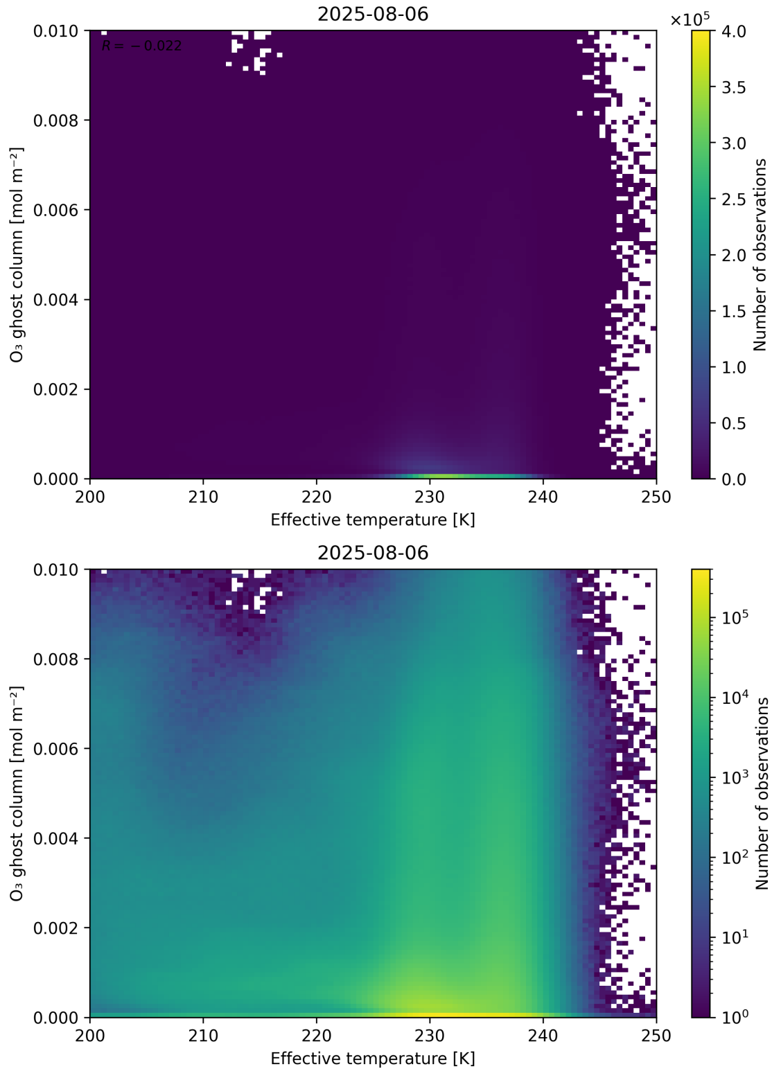
Figure 38: Scatter density plot of “Effective temperature” against “O 3 ghost column” for 2025-08-05 to 2025-08-07.
