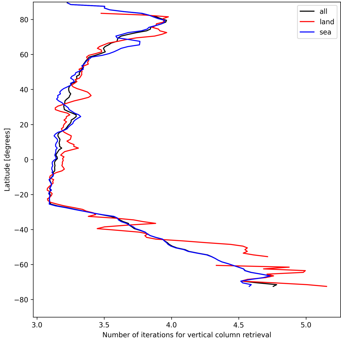
Figure 19: Zonal average of “Number of iterations for vertical column retrieval” for 2025-08-05 to 2025-08-07.
