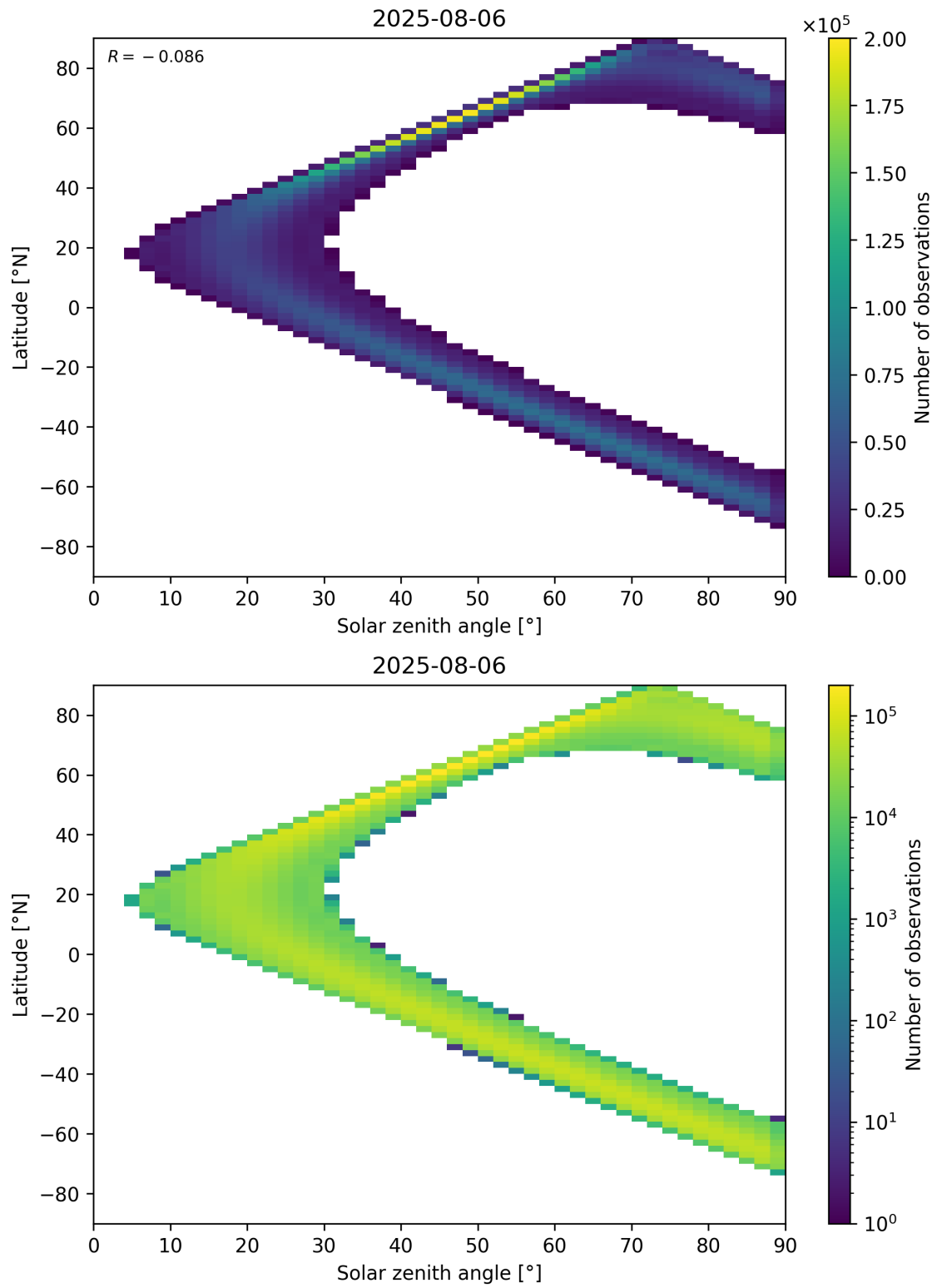
Figure 44: Scatter density plot of “Solar zenith angle” against “Latitude” for 2025-08-05 to 2025-08-07.
