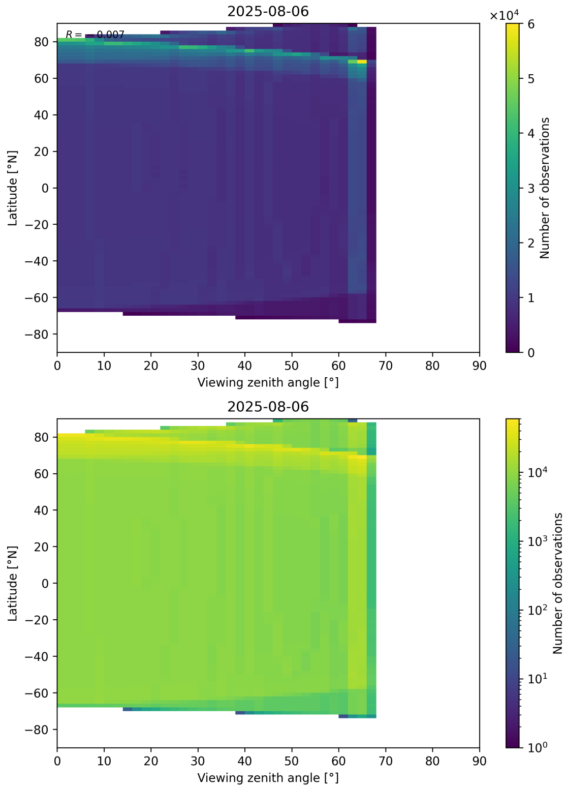
Figure 49: Scatter density plot of “Viewing zenith angle” against “Latitude” for 2025-08-05 to 2025-08-07.
