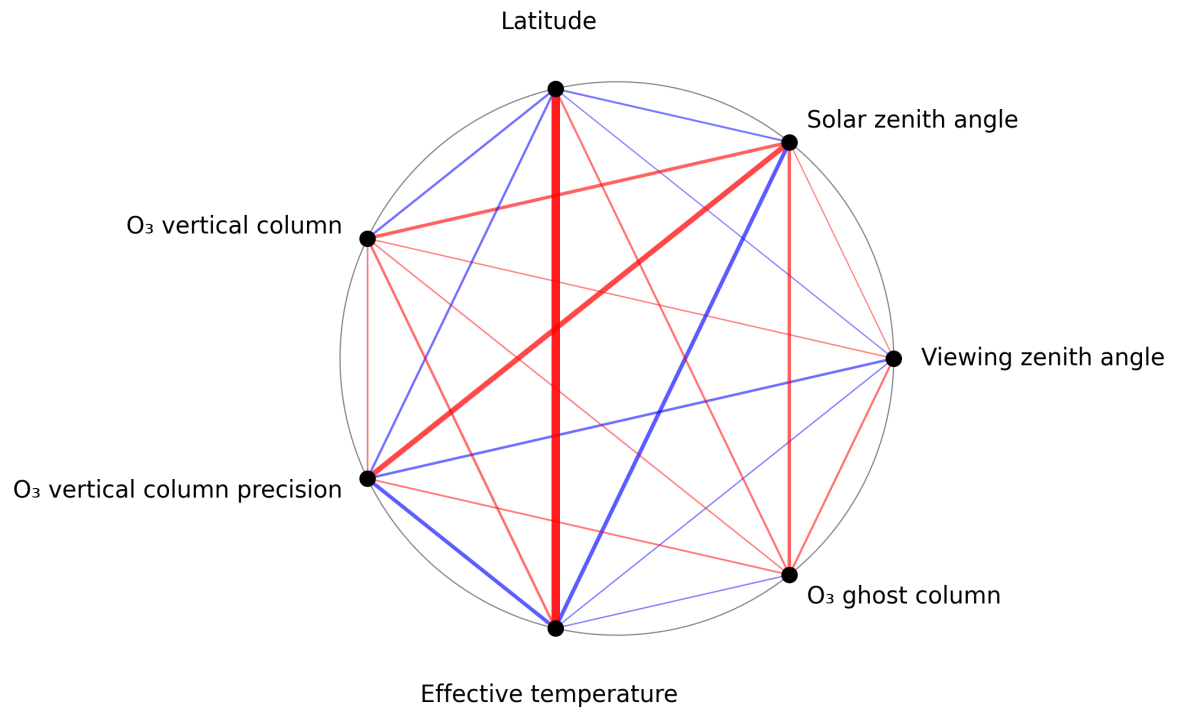
Figure 1: Map of correlation graph for 2025-08-05 to 2025-08-07.
