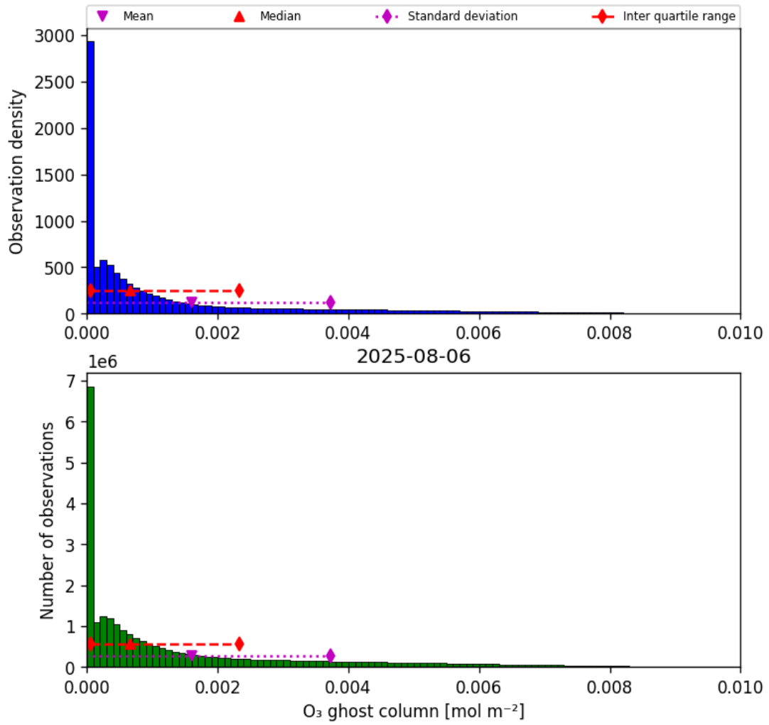
Figure 25: Histogram of “O 3 ghost column” for 2025-08-05 to 2025-08-07
