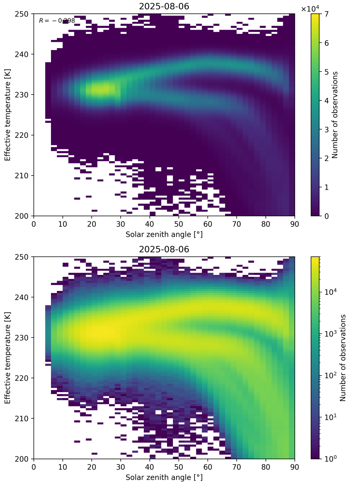
Figure 45: Scatter density plot of “Solar zenith angle” against “Effective temperature” for 2025-08-05 to 2025-08-07.
