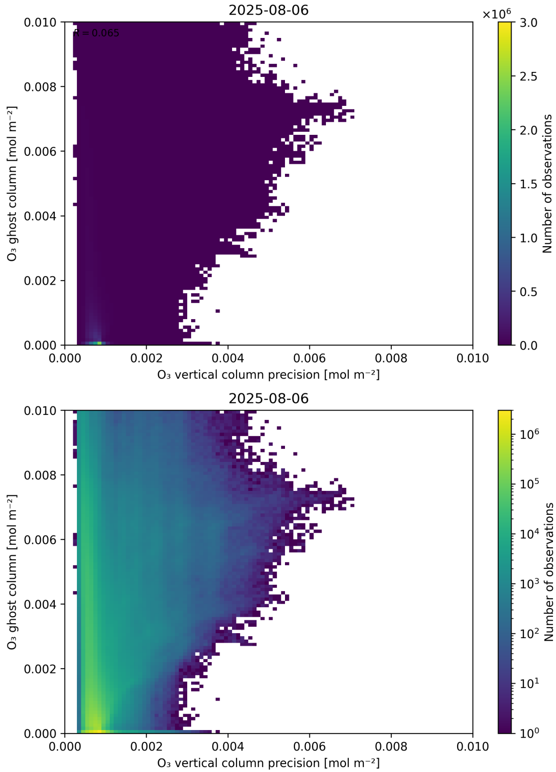
Figure 43: Scatter density plot of “ \text{O}_3 vertical column precision” against “ \text{O}_3 ghost column” for 2025-08-05 to 2025-08-07.
