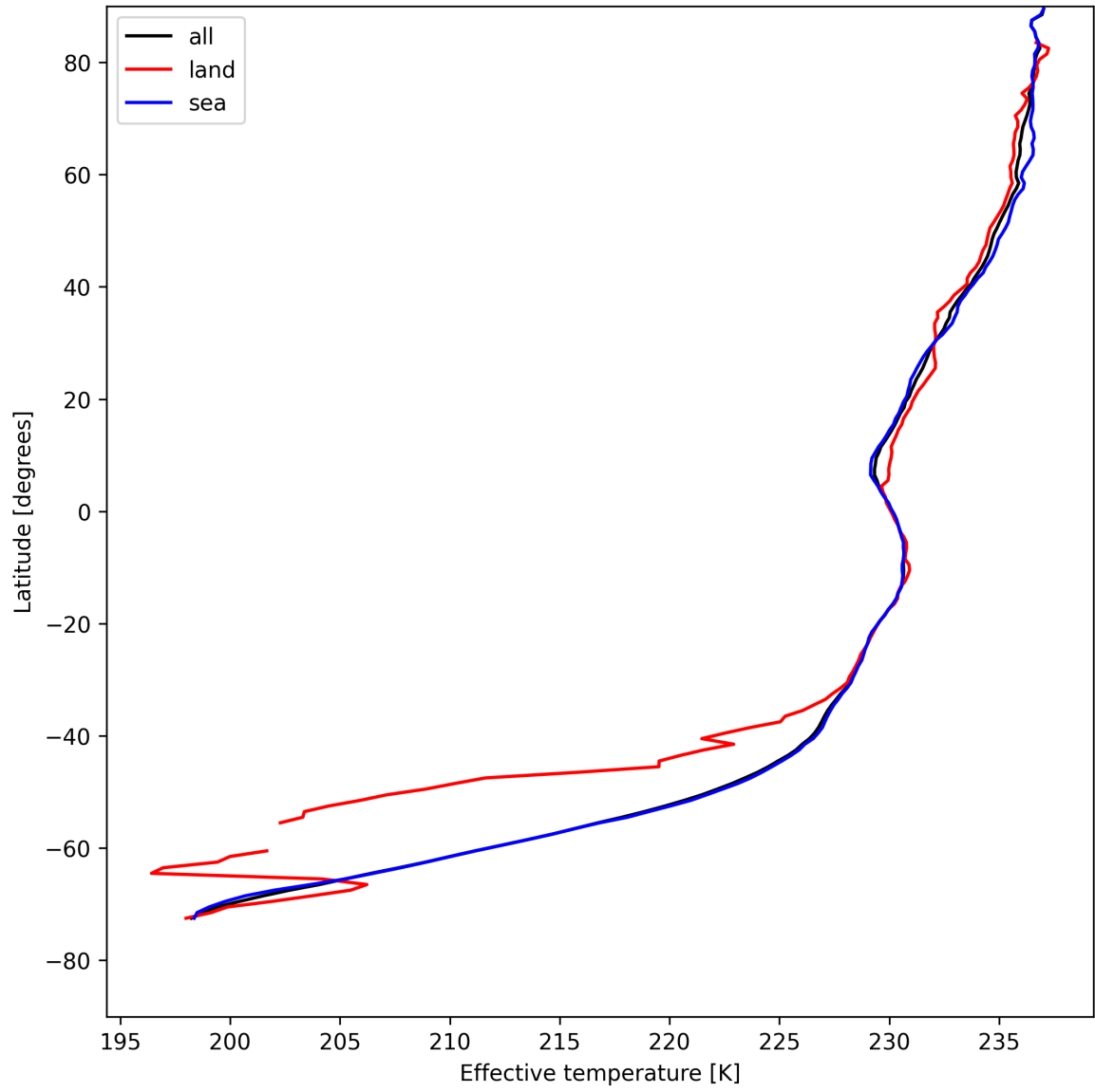
Figure 17: Zonal average of "Effective temperature" for 2025-08-05 to 2025-08-07.
