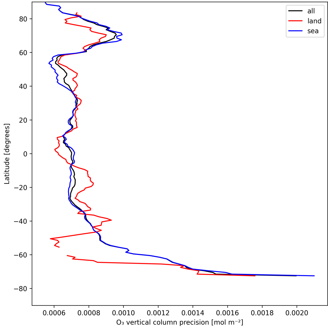
Figure 15: Zonal average of “O 3 vertical column precision” for 2025-08-05 to 2025-08-07.
