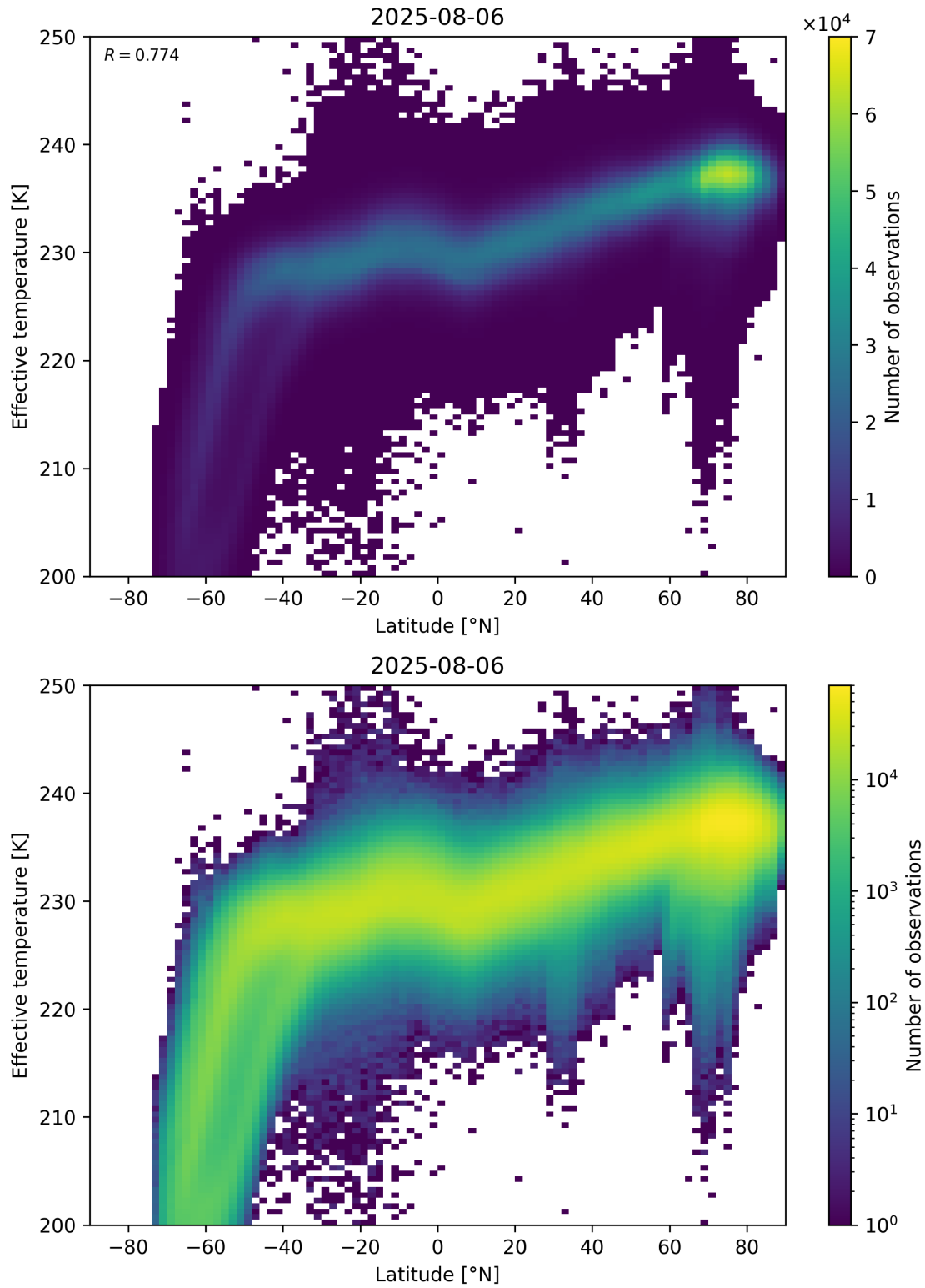
Figure 34: Scatter density plot of “Latitude” against “Effective temperature” for 2025-08-05 to 2025-08-07.
