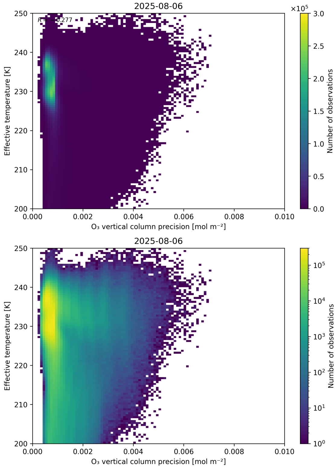
Figure 42: Scatter density plot of “O 3 vertical column precision” against “Effective temperature” for 2025-08-05 to 2025-08-07.
