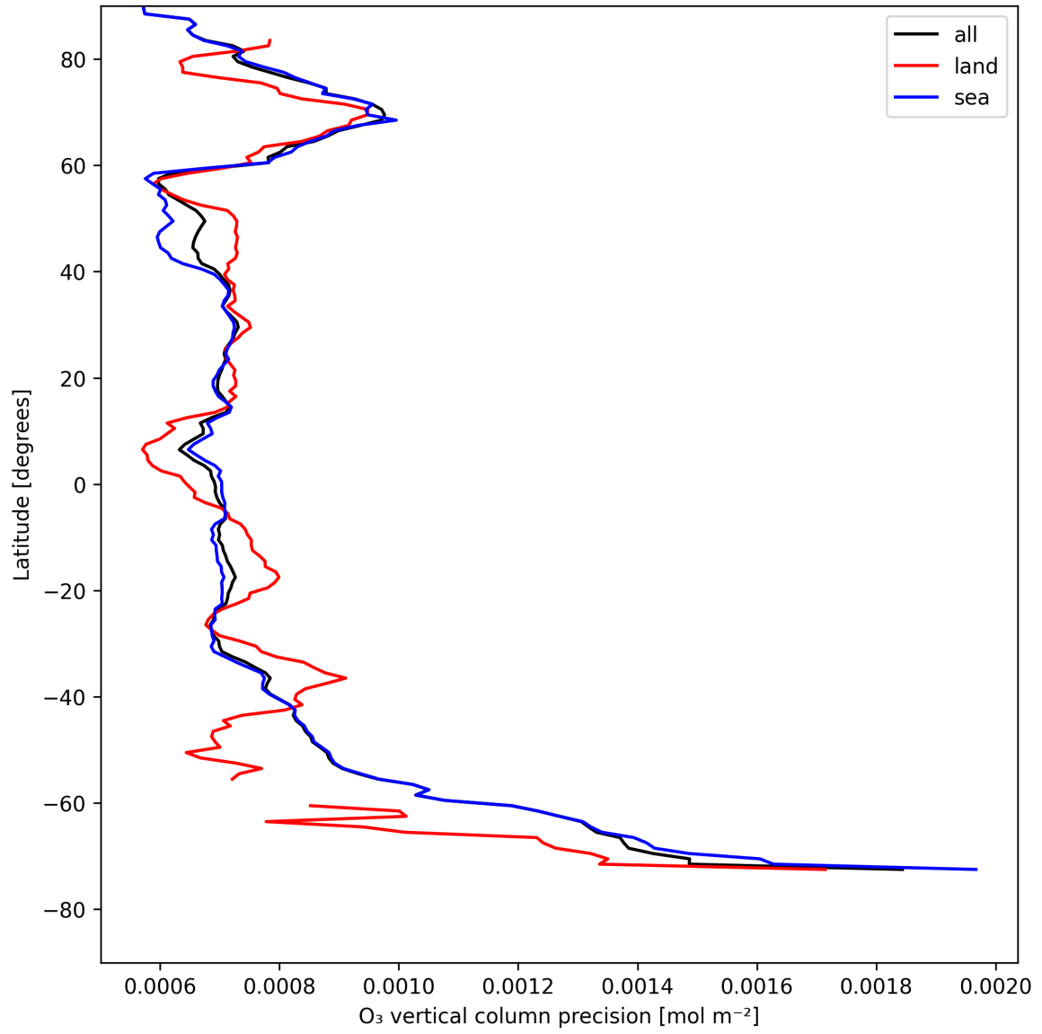
Figure 15: Zonal average of "O 3 vertical column precision" for 2025-08-06 to 2025-08-08.
