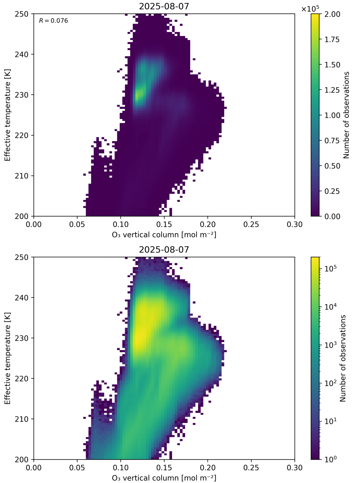
Figure 39: Scatter density plot of “O 3 vertical column” against “Effective temperature” for 2025-08-06 to 2025-08-08.
