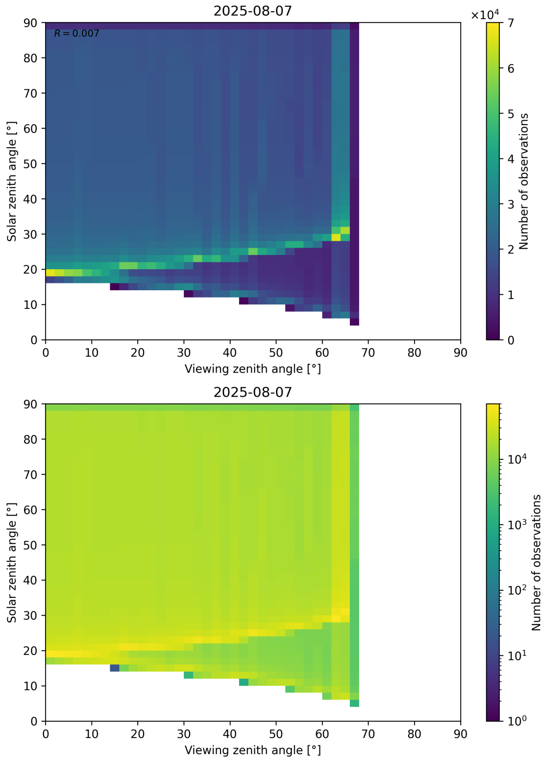
Figure 54: Scatter density plot of “Viewing zenith angle” against “Solar zenith angle” for 2025-08-06 to 2025-08-08.
