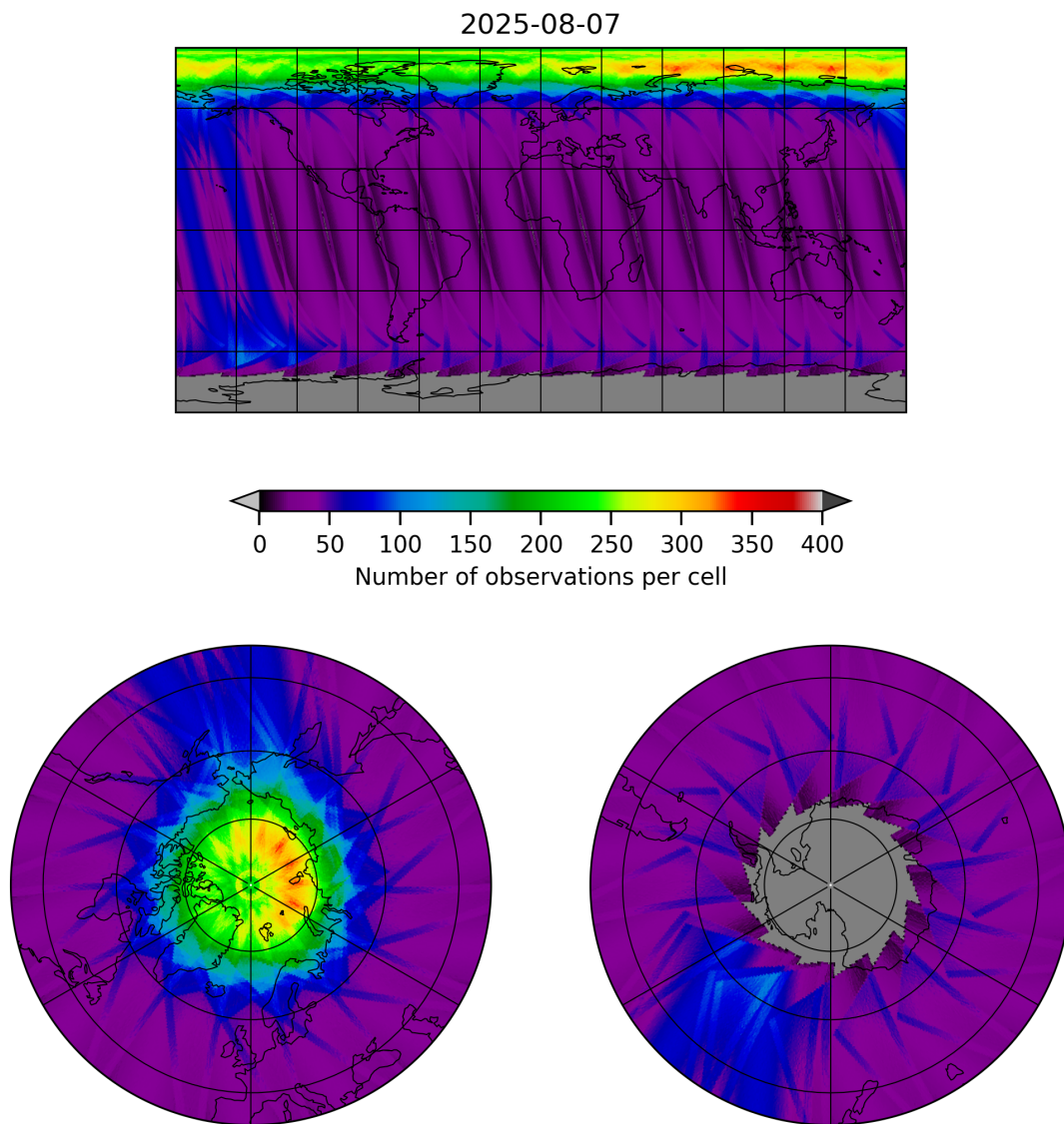
Figure 12: Map of the number of observations for 2025-08-06 to 2025-08-08
