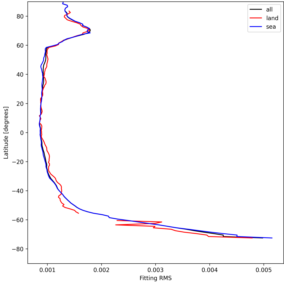
Figure 16: Zonal average of “Fitting RMS” for 2025-08-06 to 2025-08-08.
