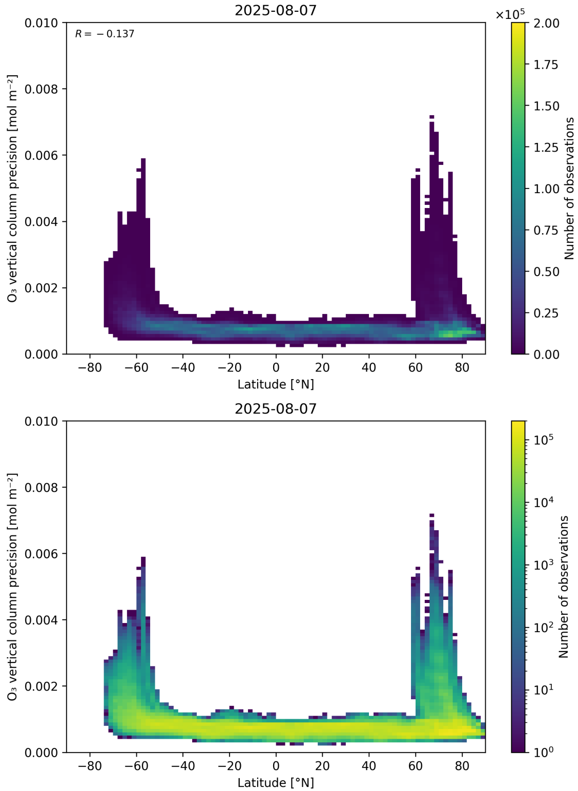
Figure 37: Scatter density plot of “Latitude” against “O 3 vertical column precision” for 2025-08-06 to 2025-08-08.
