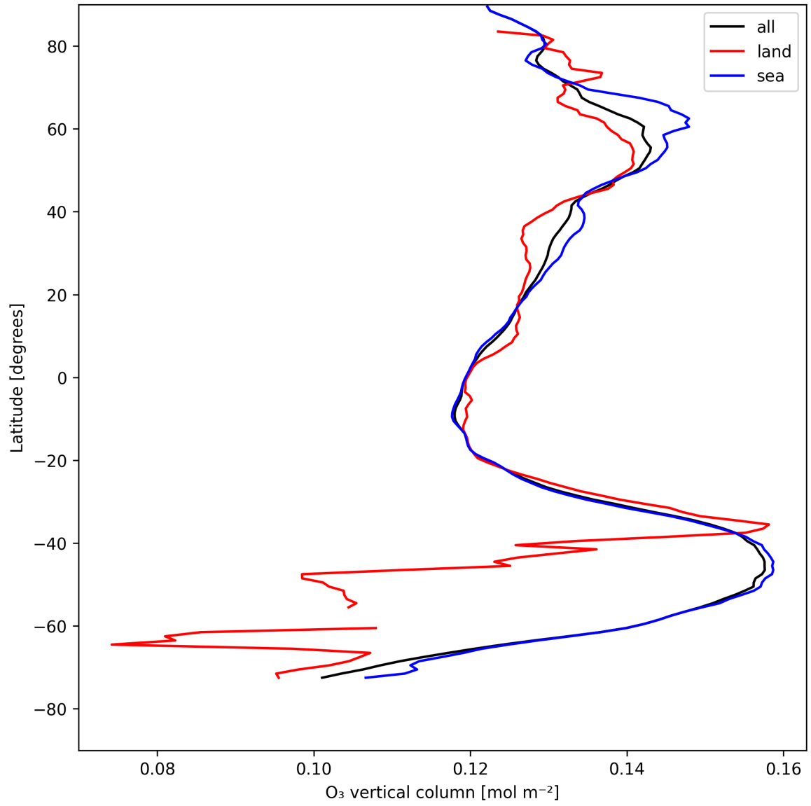
Figure 14: Zonal average of “O 3 vertical column” for 2025-08-06 to 2025-08-08.
