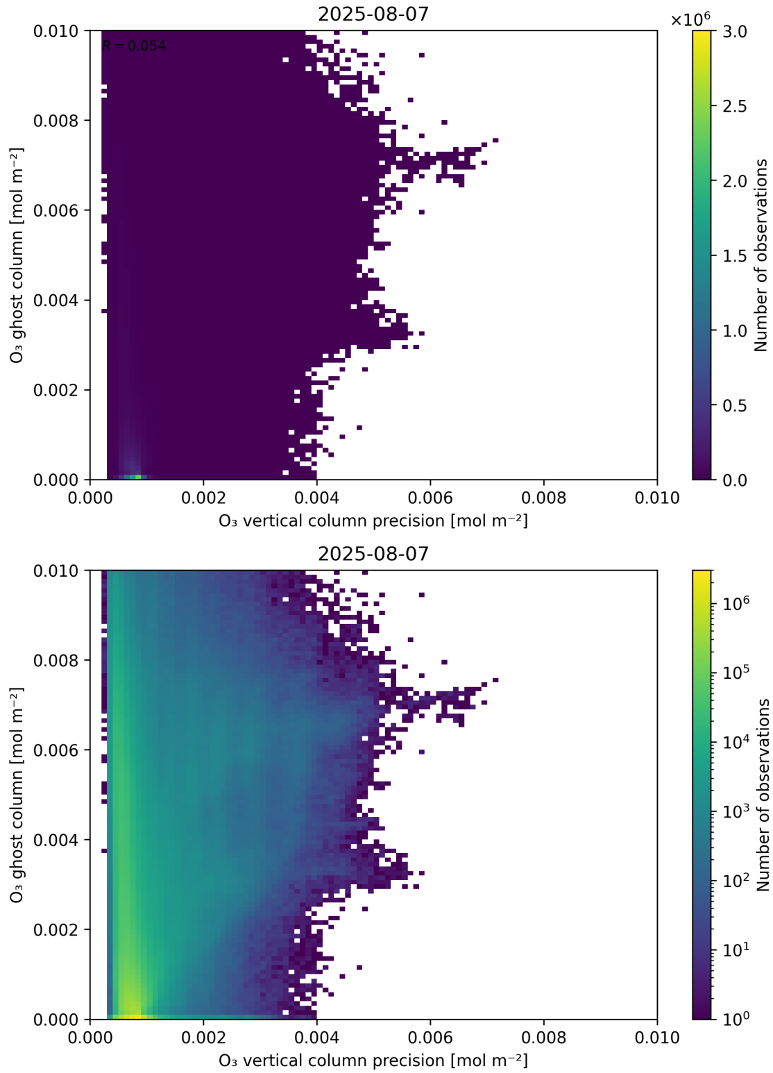
Figure 43: Scatter density plot of “ O_3 vertical column precision” against “ O_3 ghost column” for 2025-08-06 to 2025-08-08.
