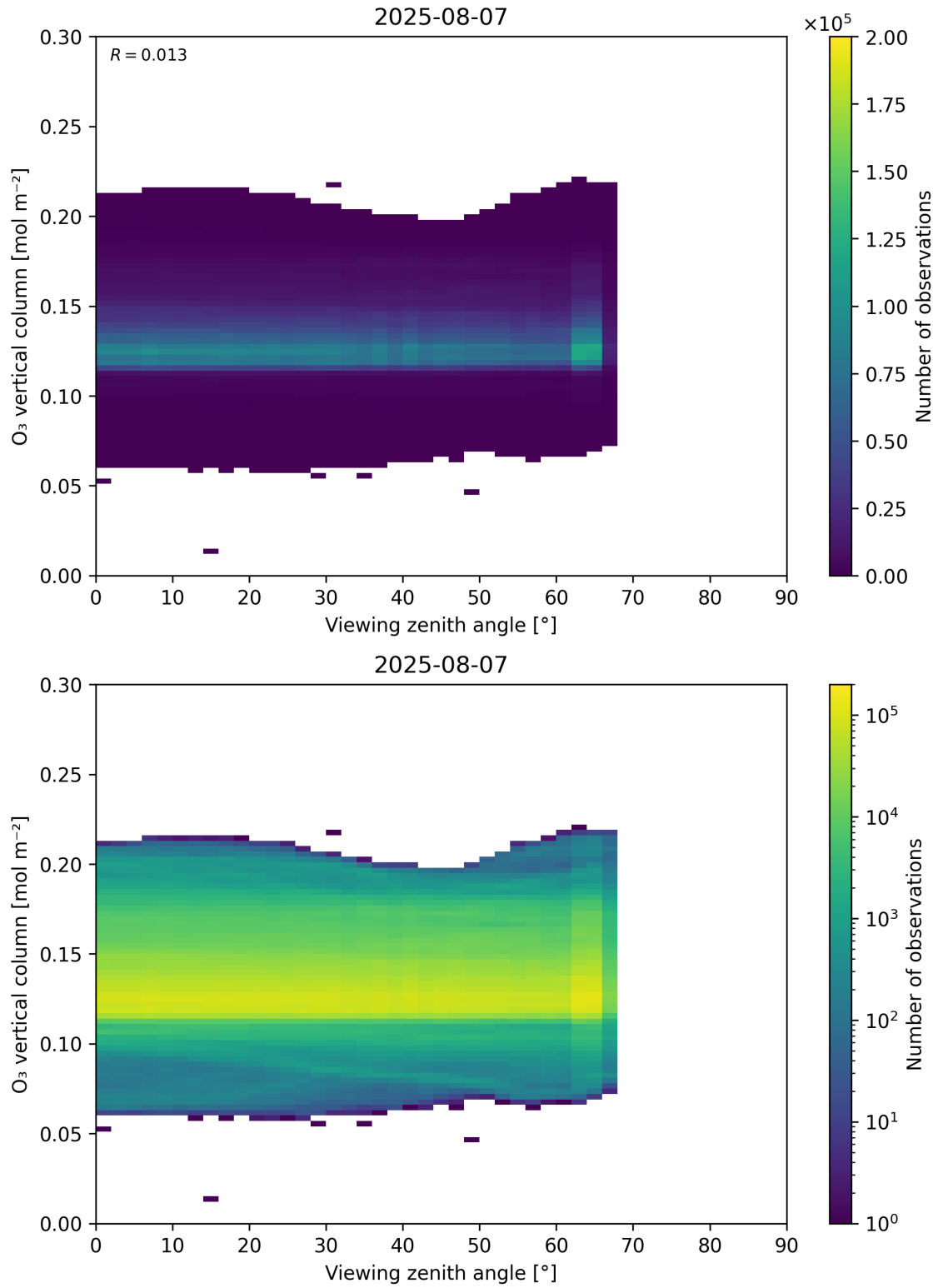
Figure 52: Scatter density plot of “Viewing zenith angle” against “O 3 vertical column” for 2025-08-06 to 2025-08-08.
