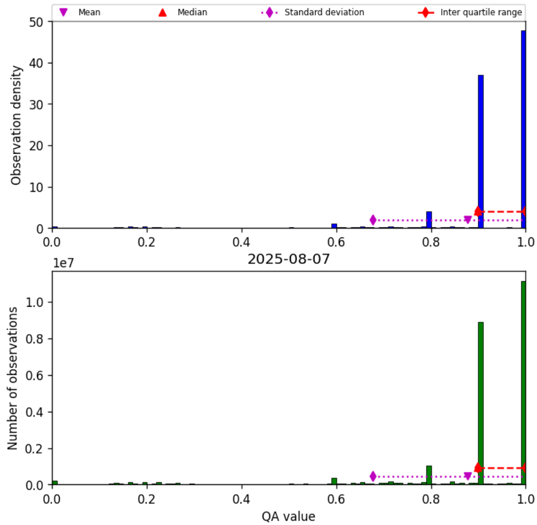
Figure 20: Histogram of “QA value” for 2025-08-06 to 2025-08-08
