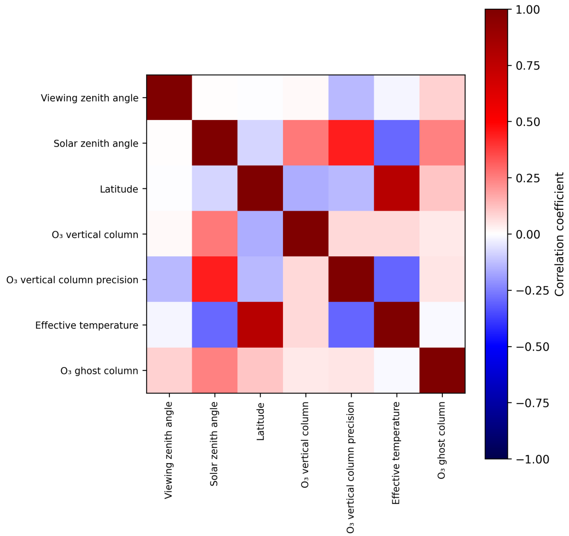
Figure 2: Map of correlation matrix for 2025-08-06 to 2025-08-08.
