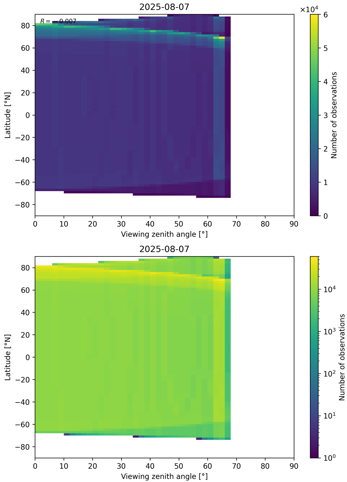
Figure 49: Scatter density plot of “Viewing zenith angle” against “Latitude” for 2025-08-06 to 2025-08-08.
