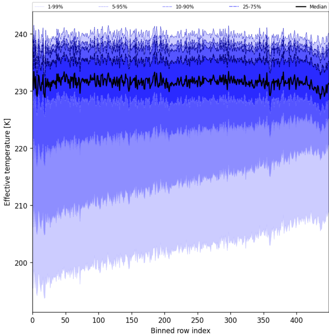
Figure 31: Along track statistics of “Effective temperature” for 2025-08-06 to 2025-08-08
