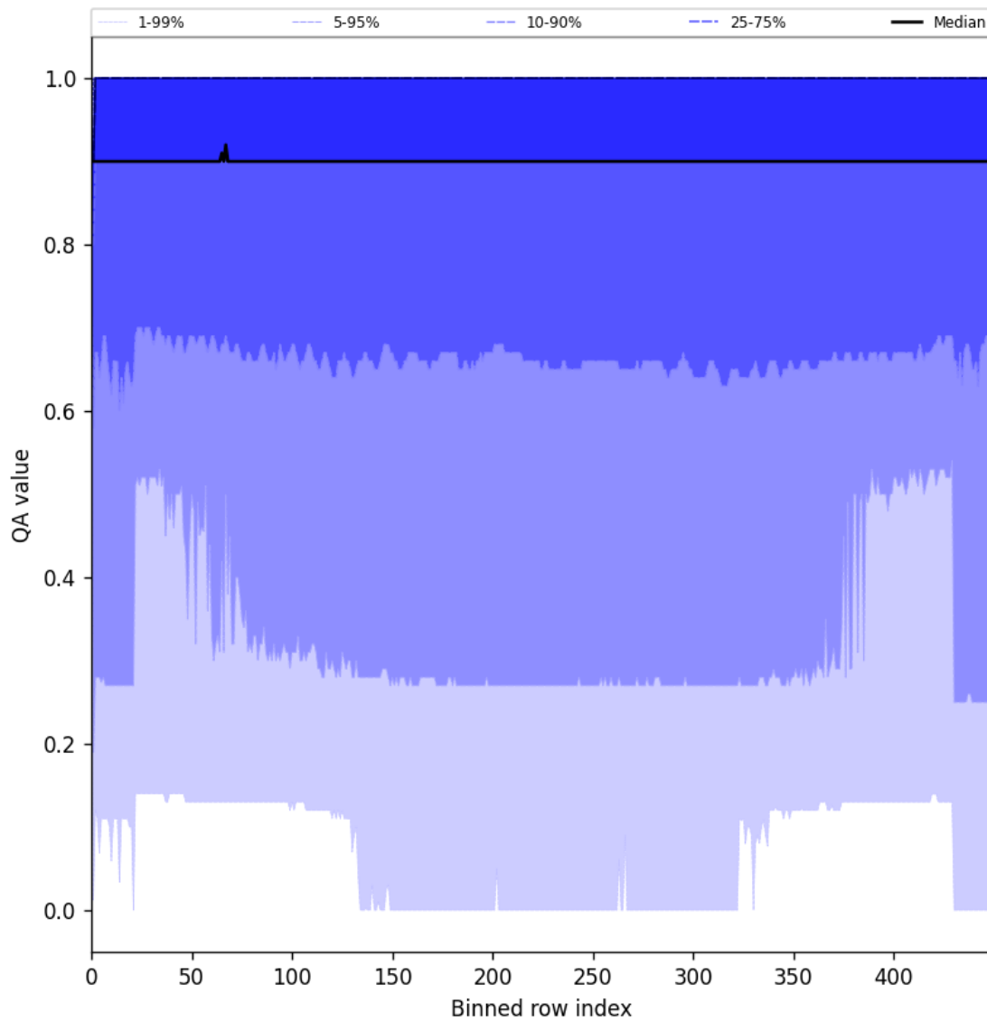
Figure 27: Along track statistics of “QA value” for 2025-08-06 to 2025-08-08
