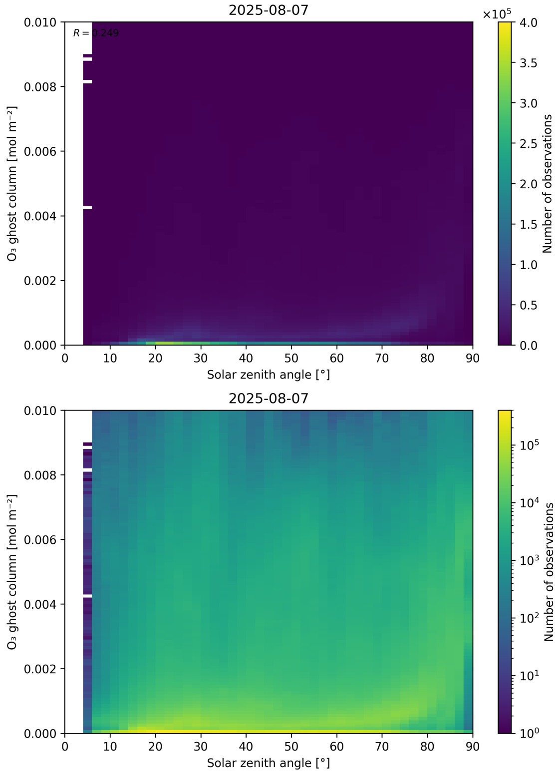
Figure 46: Scatter density plot of “Solar zenith angle” against “O 3 ghost column” for 2025-08-06 to 2025-08-08.
