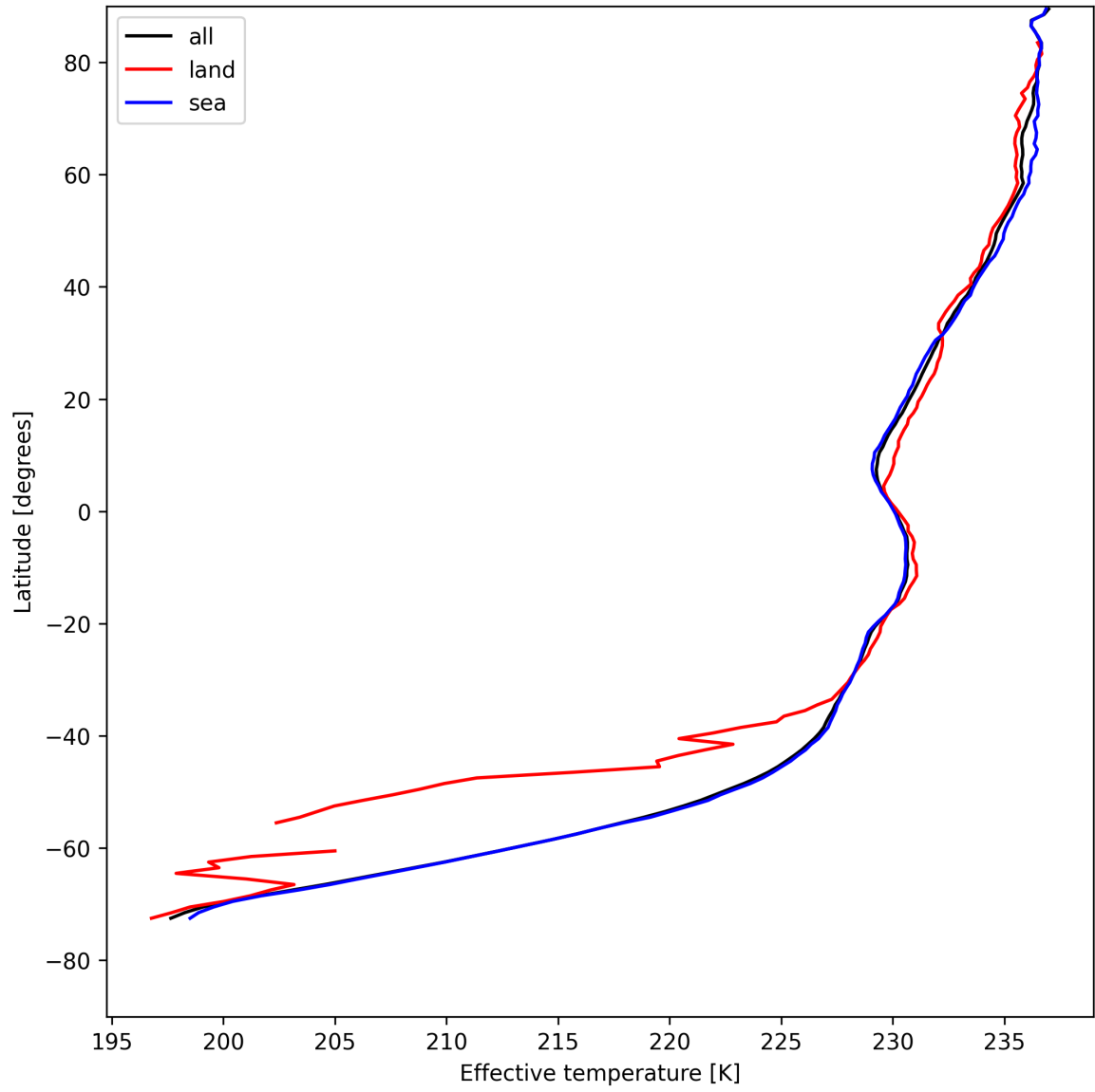
Figure 17: Zonal average of "Effective temperature" for 2025-08-06 to 2025-08-08.
