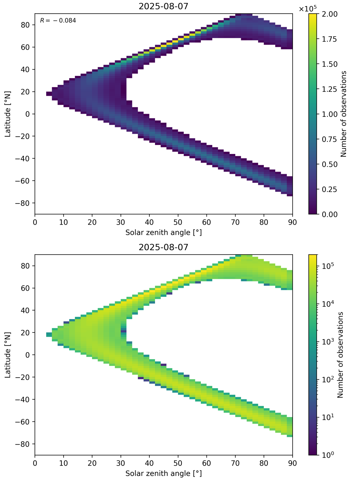
Figure 44: Scatter density plot of “Solar zenith angle” against “Latitude” for 2025-08-06 to 2025-08-08.
