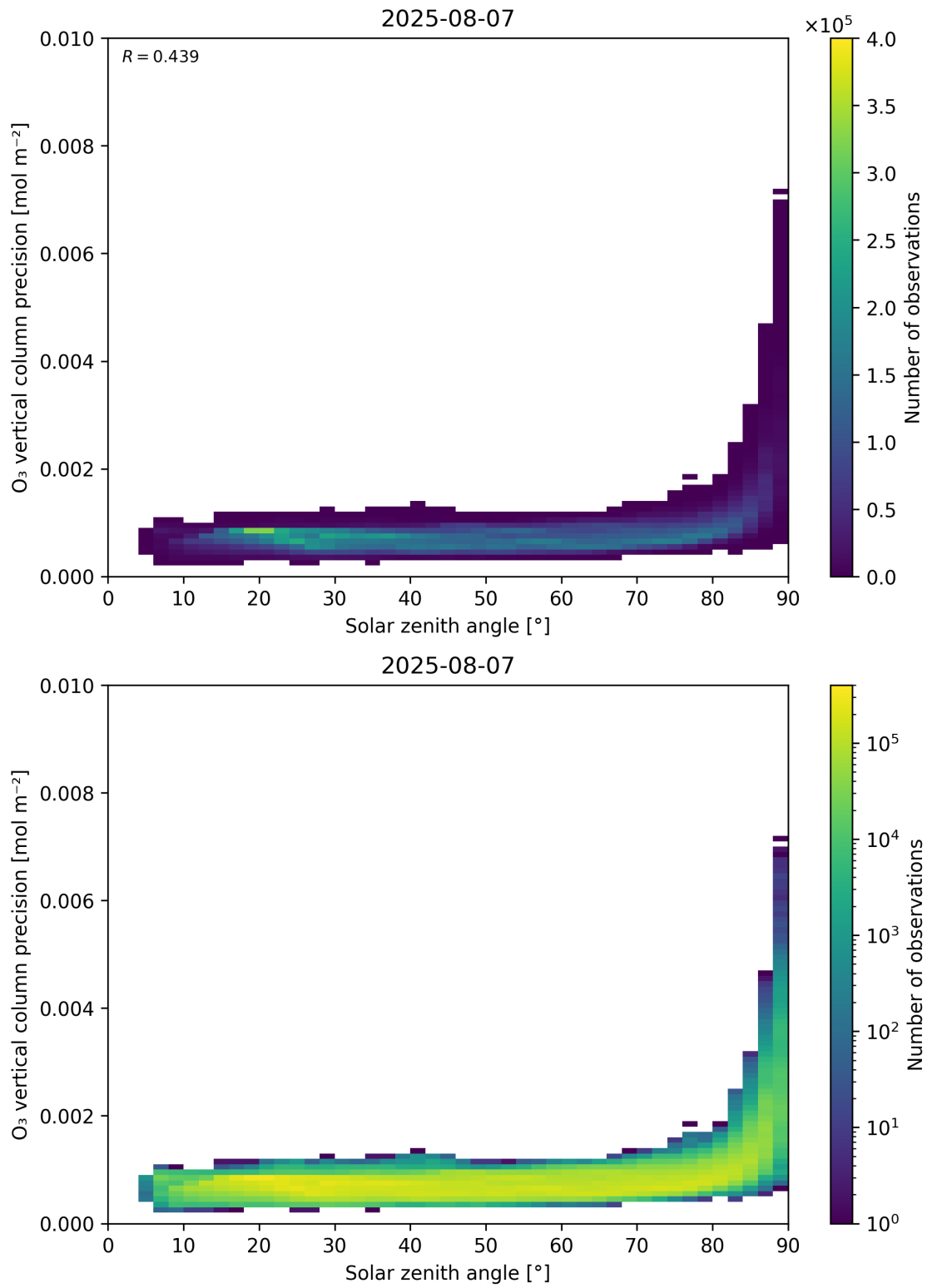
Figure 48: Scatter density plot of “Solar zenith angle” against “O 3 vertical column precision” for 2025-08-06 to 2025-08-08.
