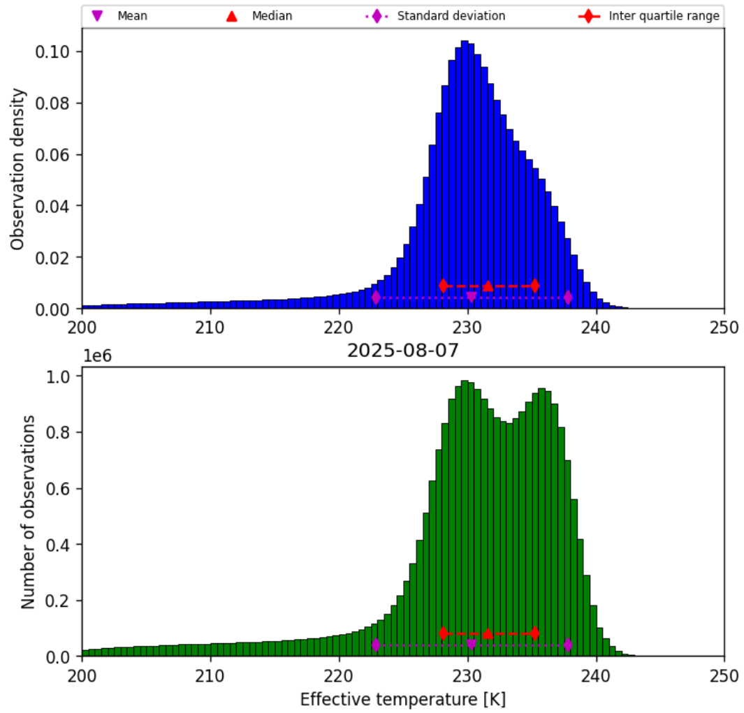
Figure 24: Histogram of “Effective temperature” for 2025-08-06 to 2025-08-08
