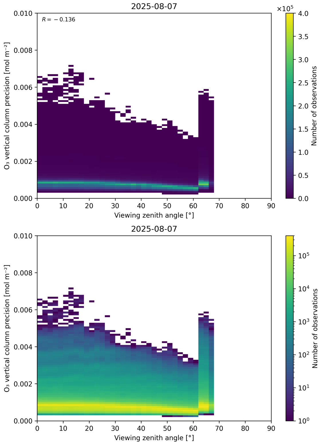
Figure 53: Scatter density plot of “Viewing zenith angle” against “O 3 vertical column precision” for 2025-08-06 to 2025-08-08.
