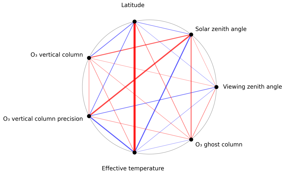
Figure 1: Map of correlation graph for 2025-08-06 to 2025-08-08.
