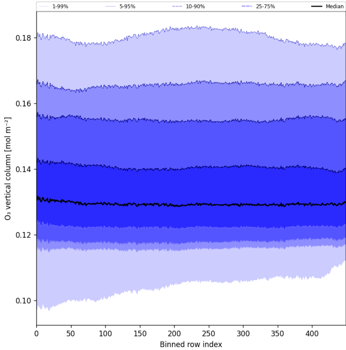
Figure 28: Along track statistics of “O 3 vertical column” for 2025-08-06 to 2025-08-08
