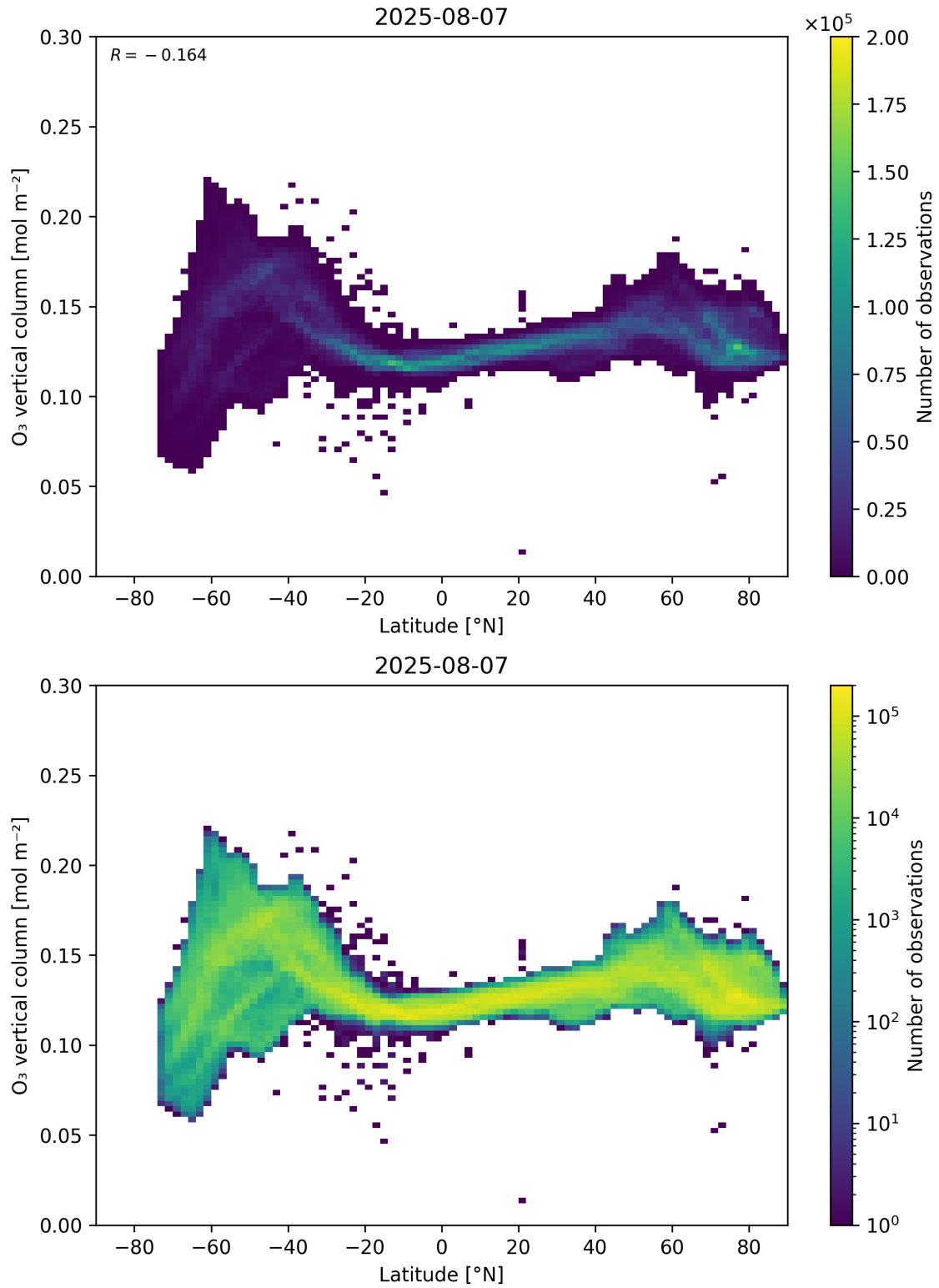
Figure 36: Scatter density plot of “Latitude” against “O 3 vertical column” for 2025-08-06 to 2025-08-08.
