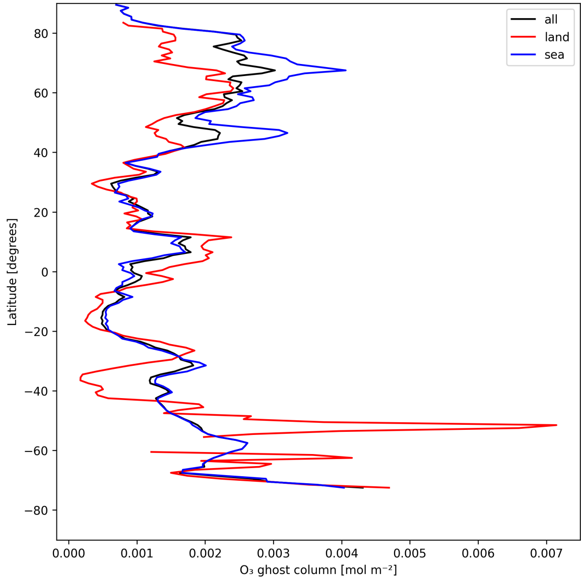
Figure 18: Zonal average of “O 3 ghost column” for 2025-08-06 to 2025-08-08.
