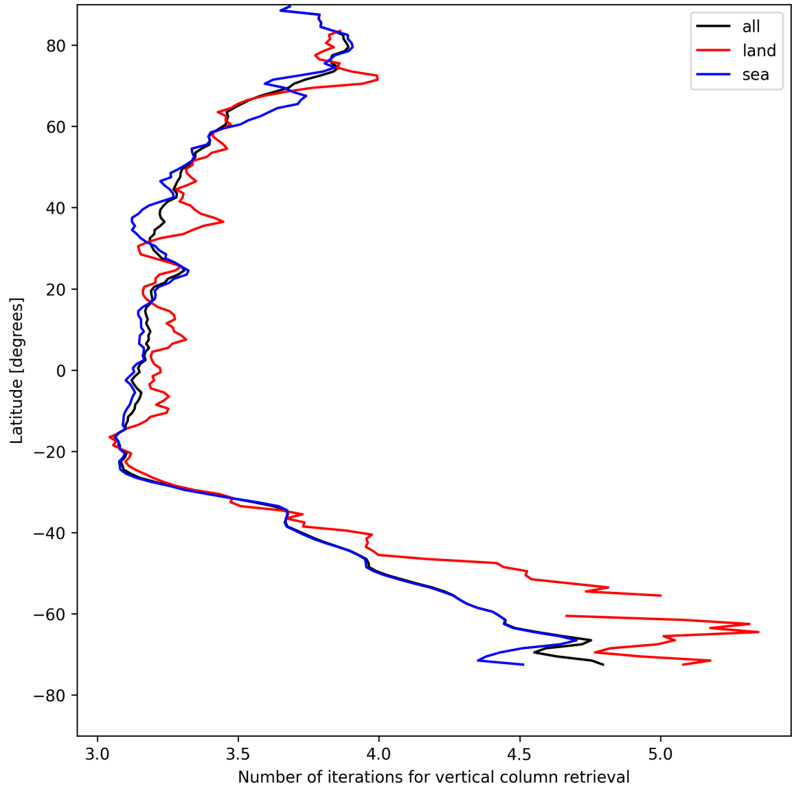
Figure 19: Zonal average of “Number of iterations for vertical column retrieval” for 2025-08-06 to 2025-08-08.
