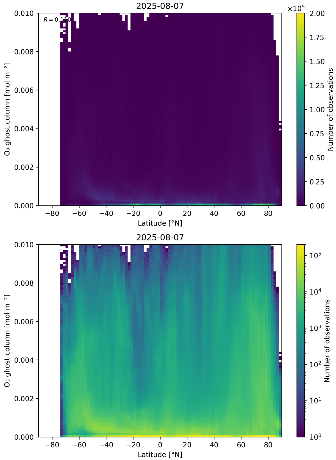
Figure 35: Scatter density plot of “Latitude” against “O 3 ghost column” for 2025-08-06 to 2025-08-08.
