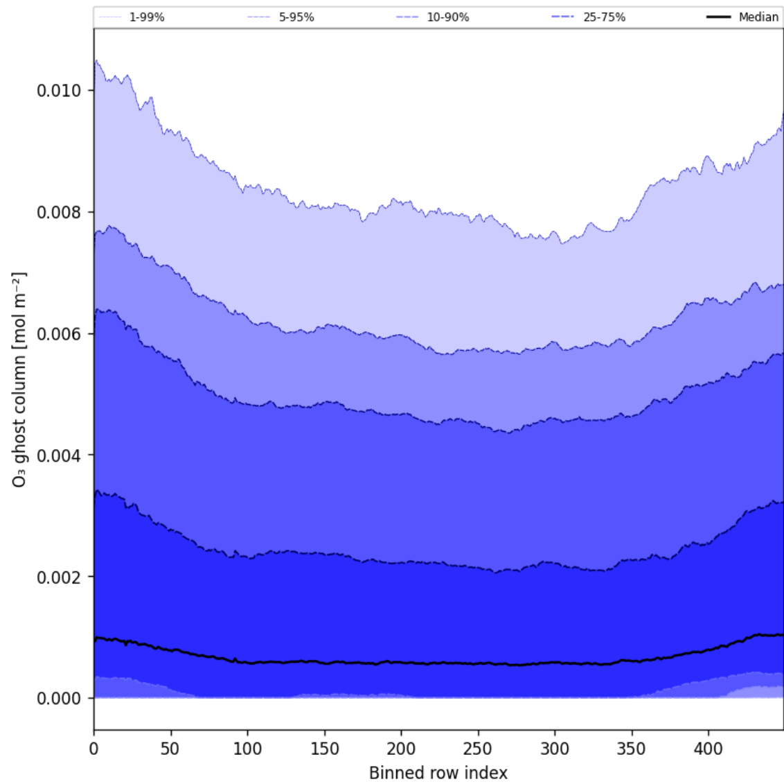
Figure 32: Along track statistics of “O 3 ghost column” for 2025-08-06 to 2025-08-08
