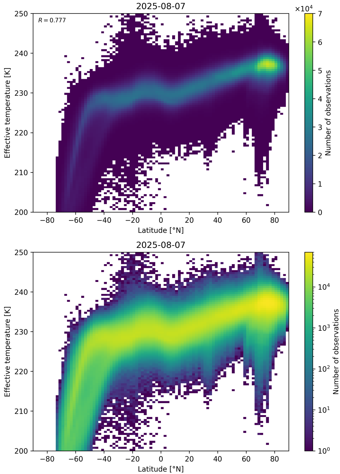
Figure 34: Scatter density plot of “Latitude” against “Effective temperature” for 2025-08-06 to 2025-08-08.
