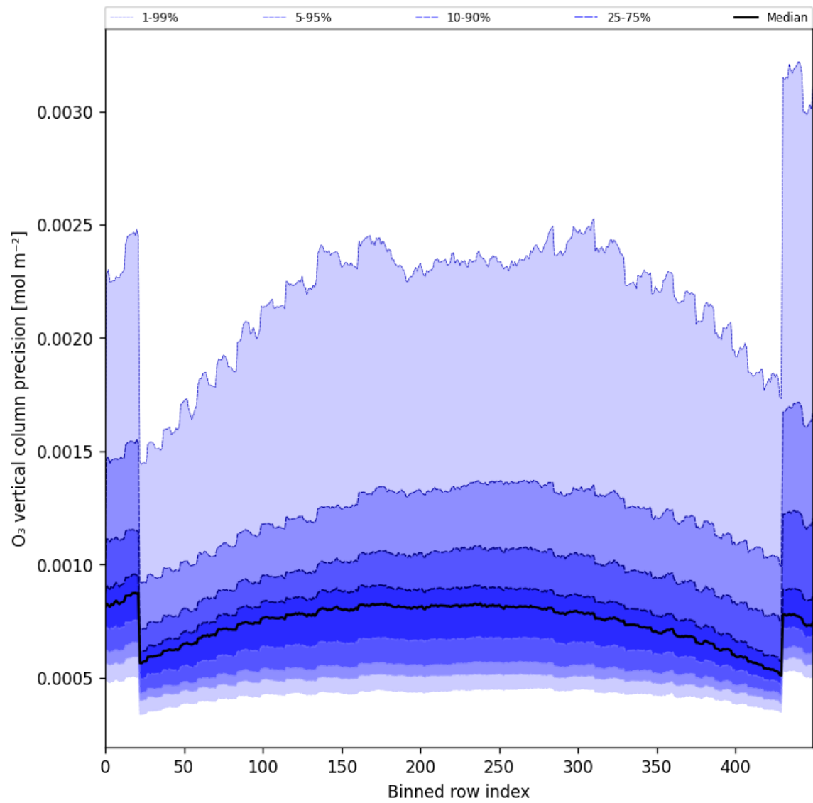
Figure 29: Along track statistics of “O 3 vertical column precision” for 2025-08-06 to 2025-08-08
