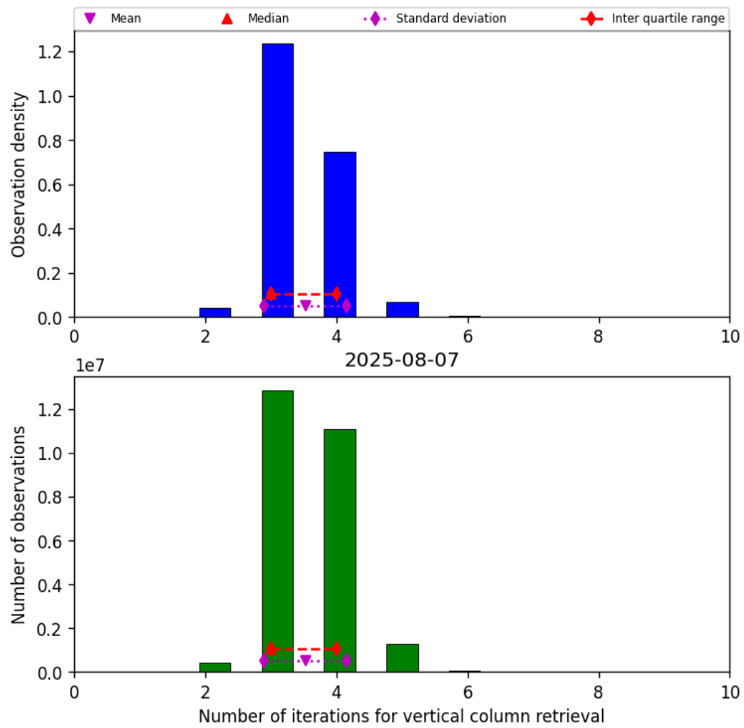
Figure 26: Histogram of “Number of iterations for vertical column retrieval” for 2025-08-06 to 2025-08-08
