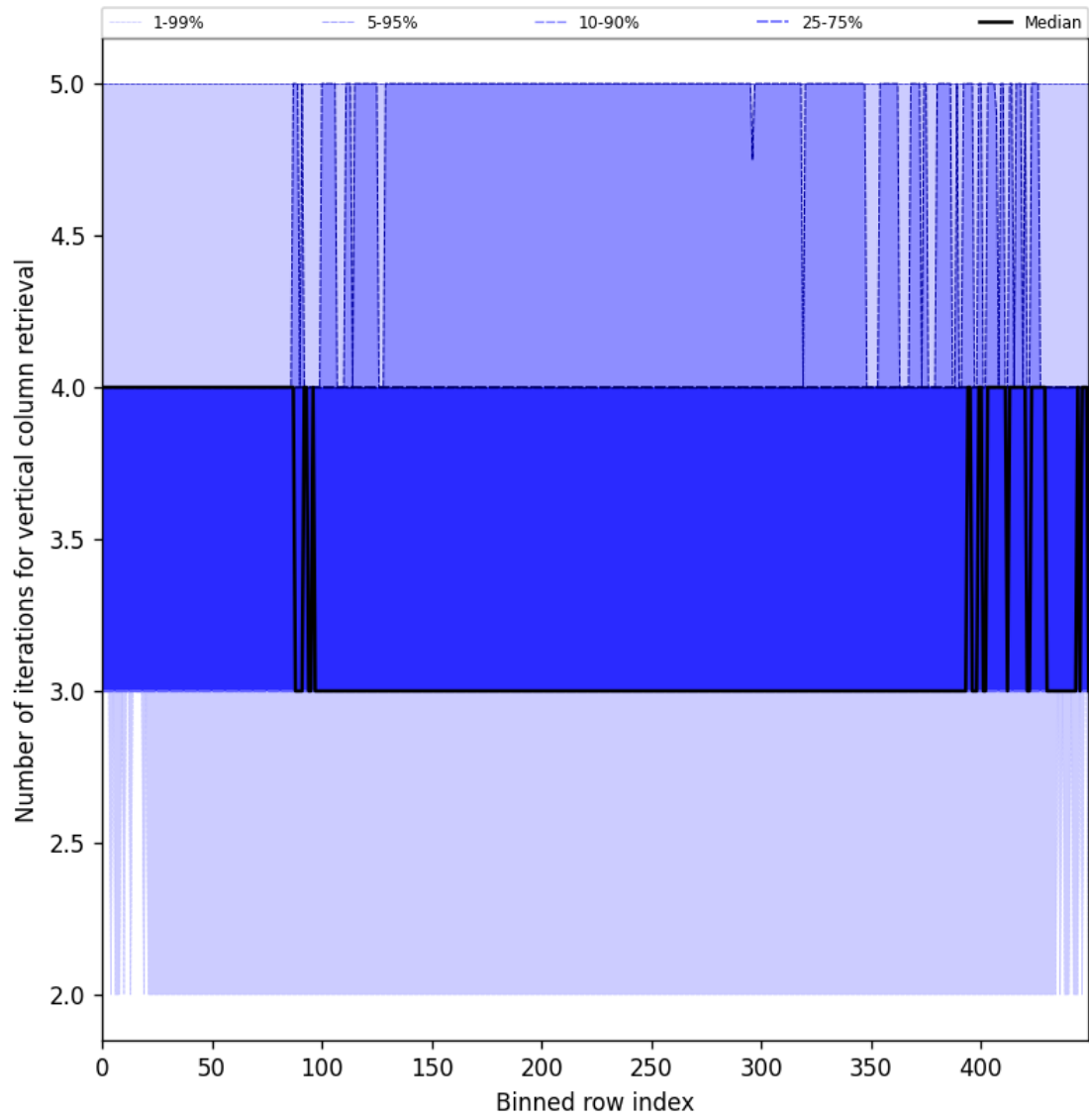
Figure 33: Along track statistics of “Number of iterations for vertical column retrieval” for 2025-08-06 to 2025-08-08
