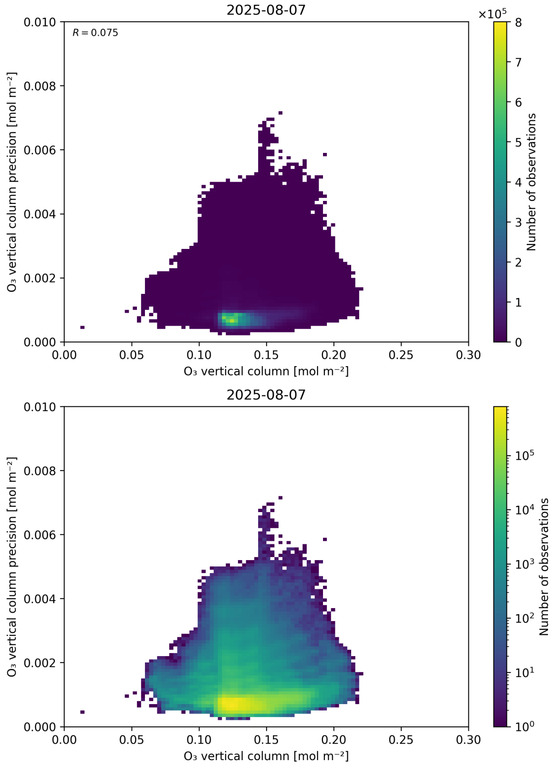
Figure 41: Scatter density plot of “O 3 vertical column” against “O 3 vertical column precision” for 2025-08-06 to 2025-08-08.
