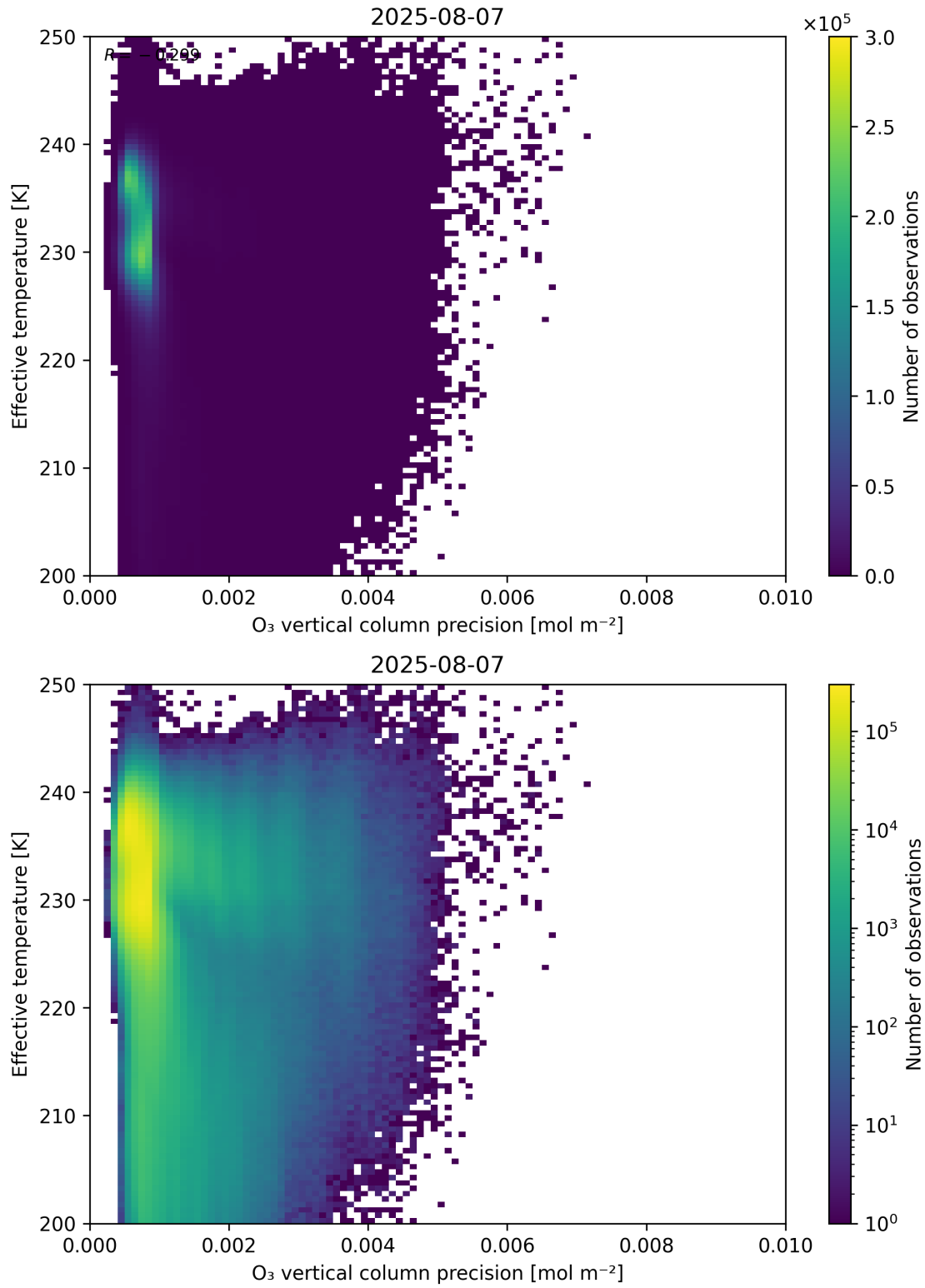
Figure 42: Scatter density plot of “O 3 vertical column precision” against “Effective temperature” for 2025-08-06 to 2025-08-08.
