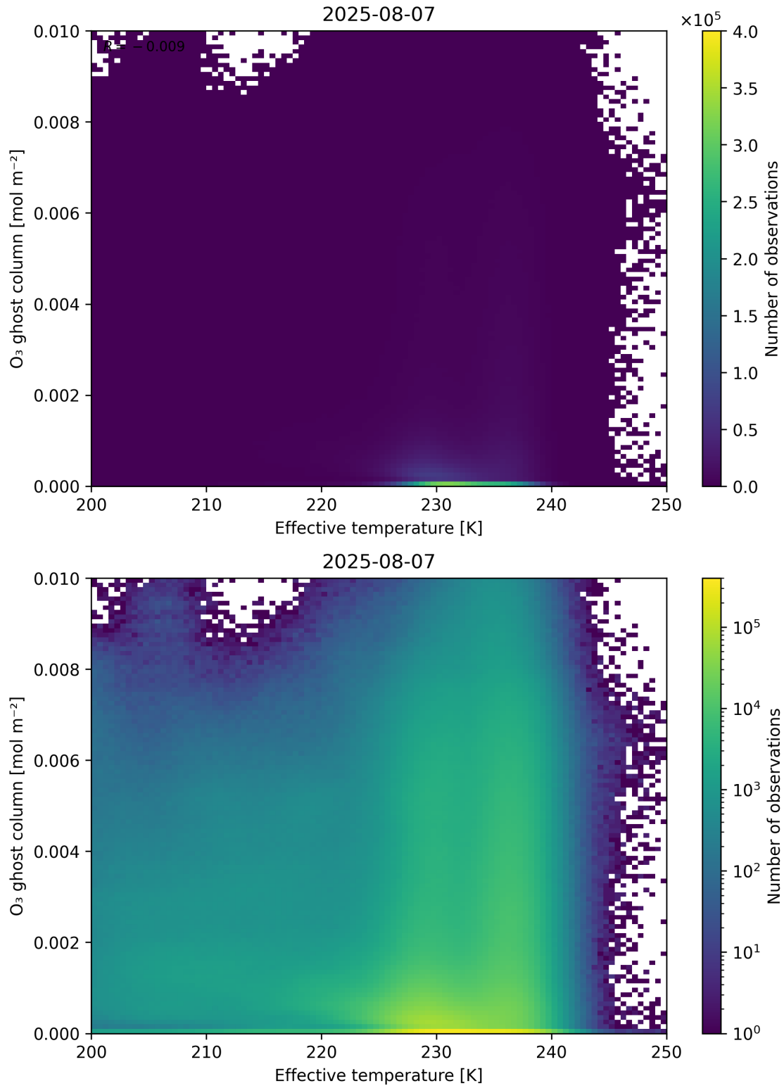
Figure 38: Scatter density plot of “Effective temperature” against “O 3 ghost column” for 2025-08-06 to 2025-08-08.
