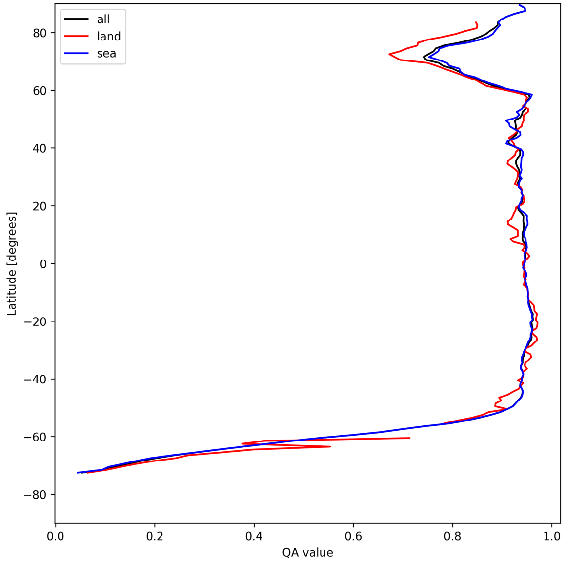
Figure 13: Zonal average of “QA value” for 2025-08-06 to 2025-08-08.
