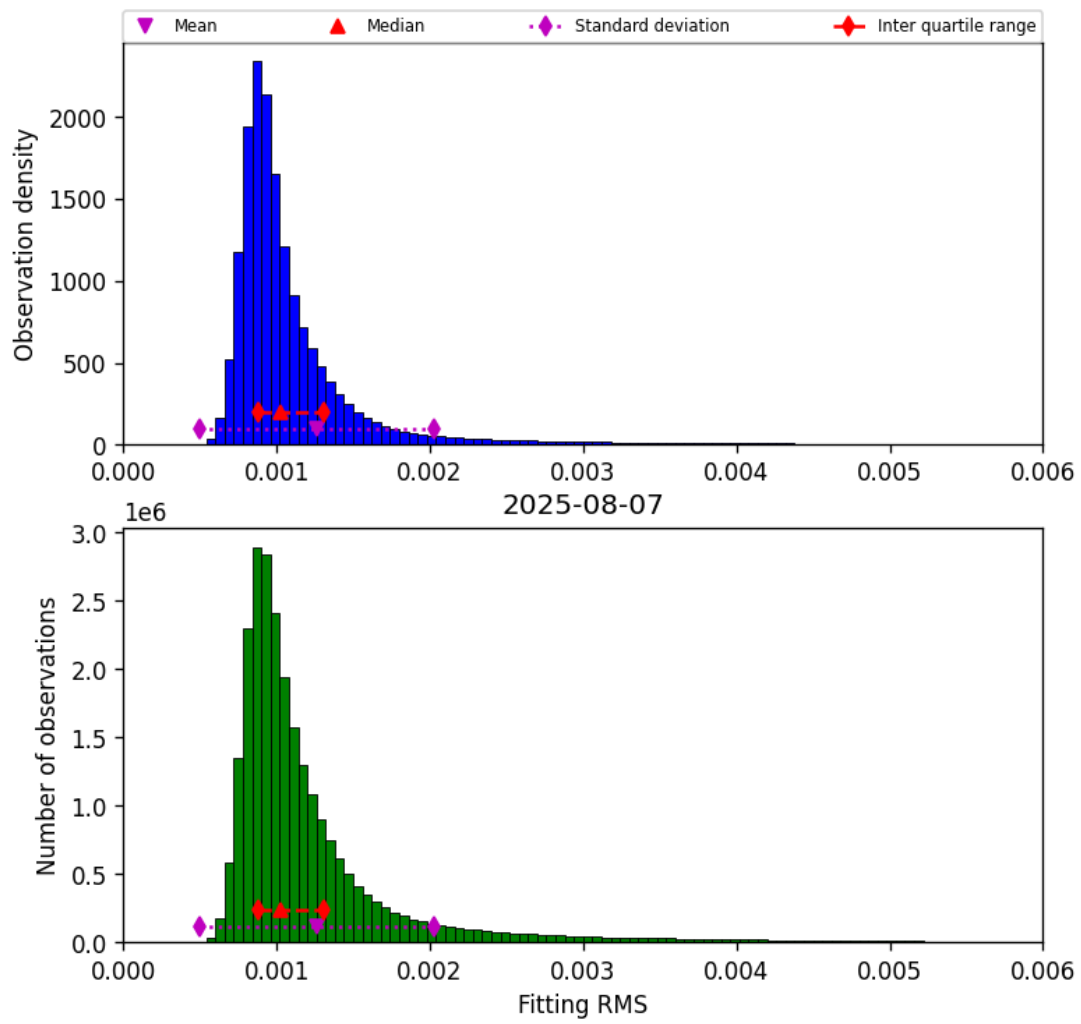
Figure 23: Histogram of “Fitting RMS” for 2025-08-06 to 2025-08-08
