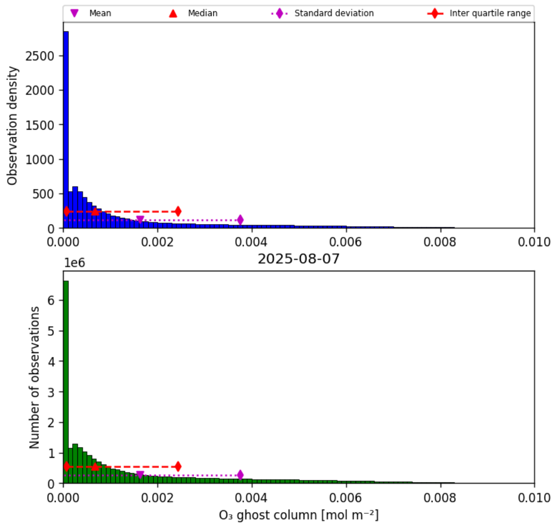
Figure 25: Histogram of “O 3 ghost column” for 2025-08-06 to 2025-08-08
