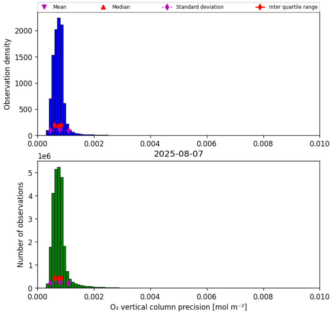
Figure 22: Histogram of “O 3 vertical column precision” for 2025-08-06 to 2025-08-08
