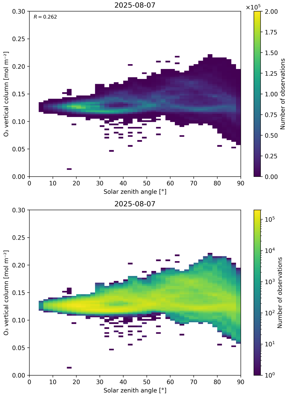
Figure 47: Scatter density plot of “Solar zenith angle” against “O 3 vertical column” for 2025-08-06 to 2025-08-08.
