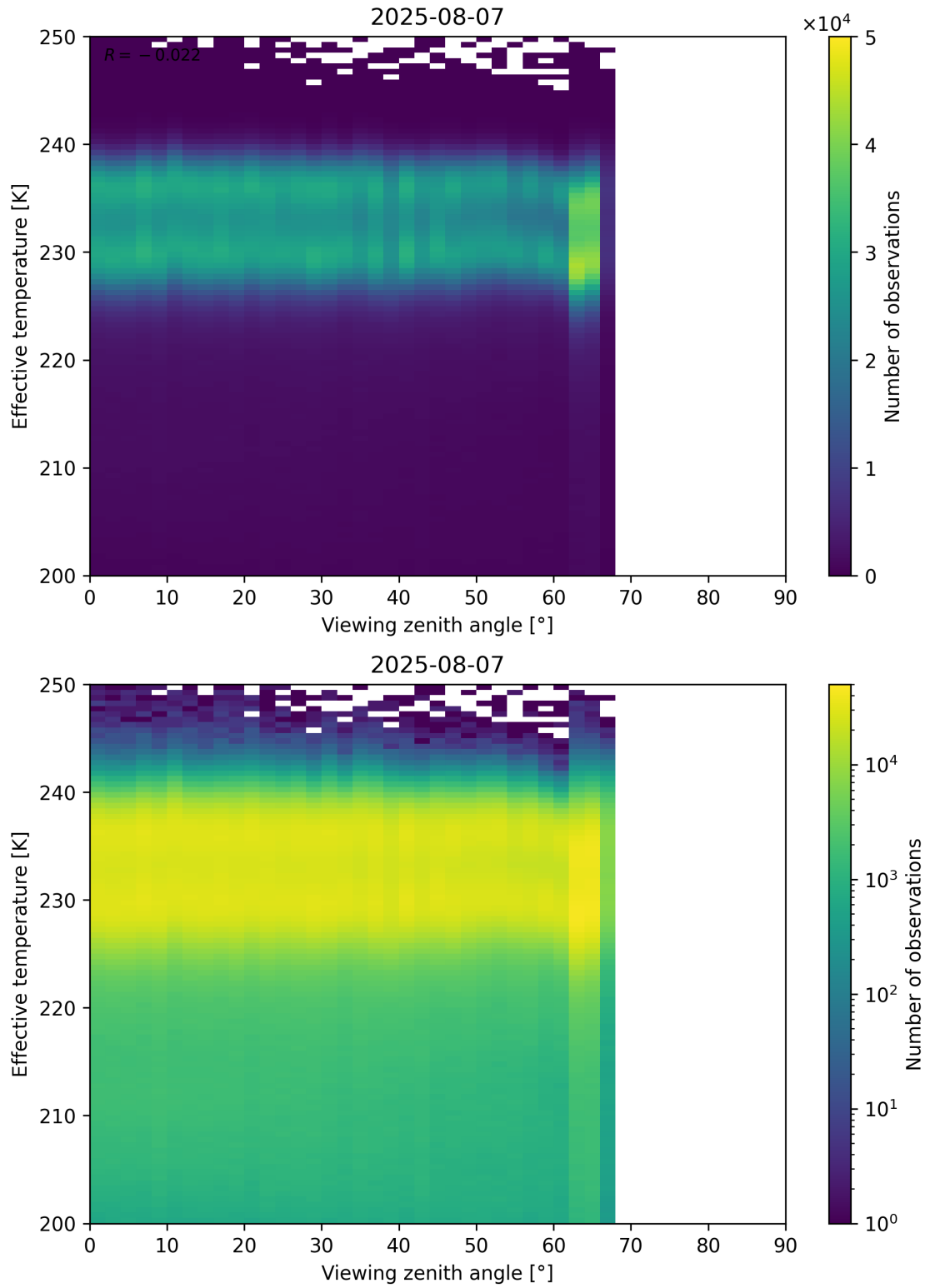
Figure 50: Scatter density plot of “Viewing zenith angle” against “Effective temperature” for 2025-08-06 to 2025-08-08.
