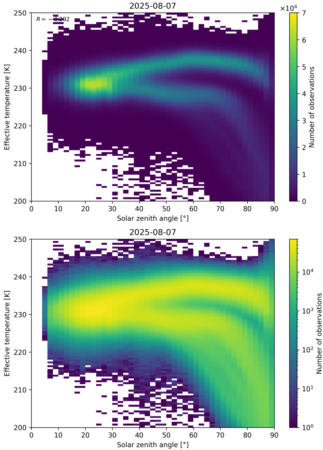
Figure 45: Scatter density plot of “Solar zenith angle” against “Effective temperature” for 2025-08-06 to 2025-08-08.
