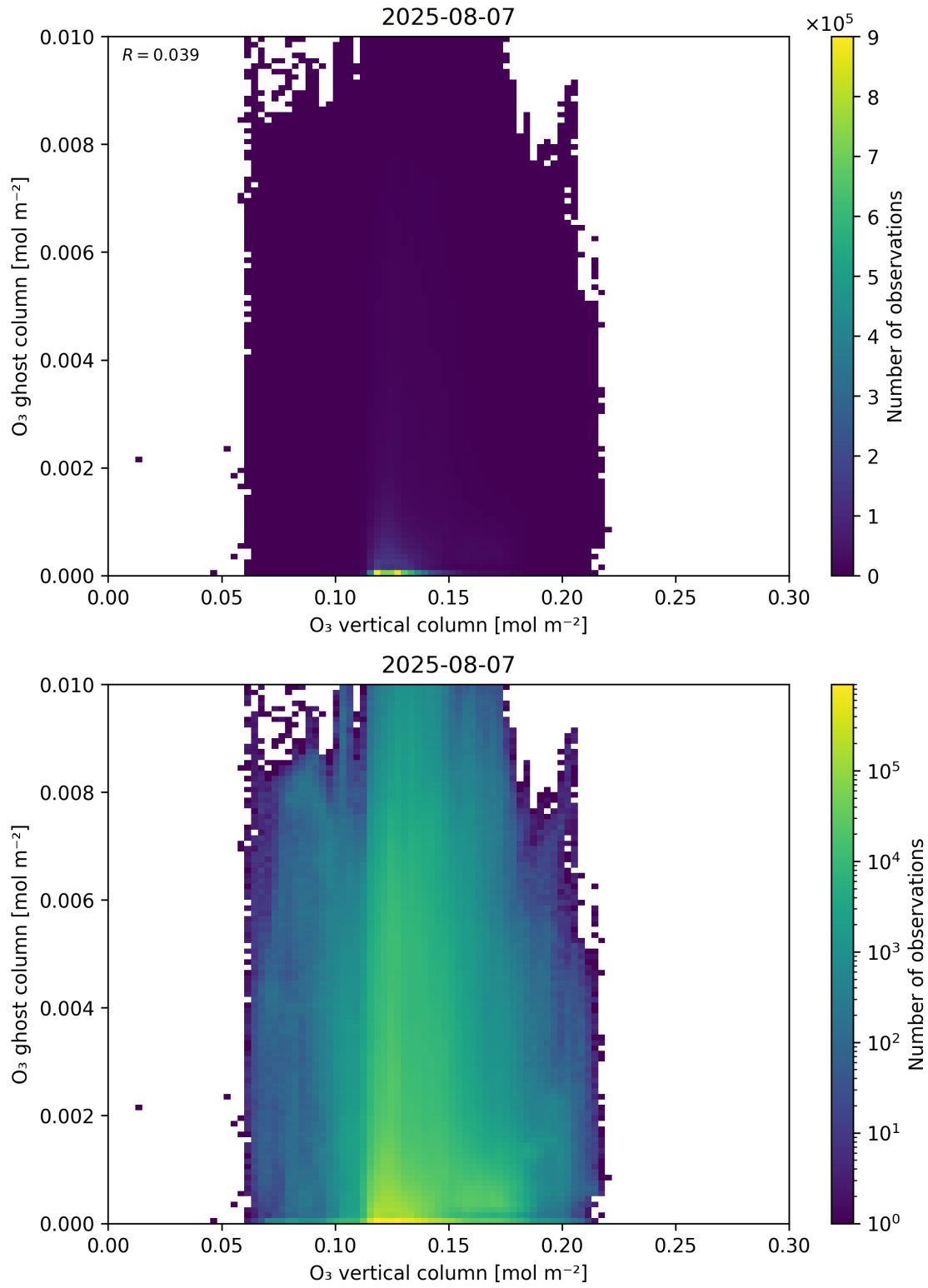
Figure 40: Scatter density plot of “O 3 vertical column” against “O 3 ghost column” for 2025-08-06 to 2025-08-08.
