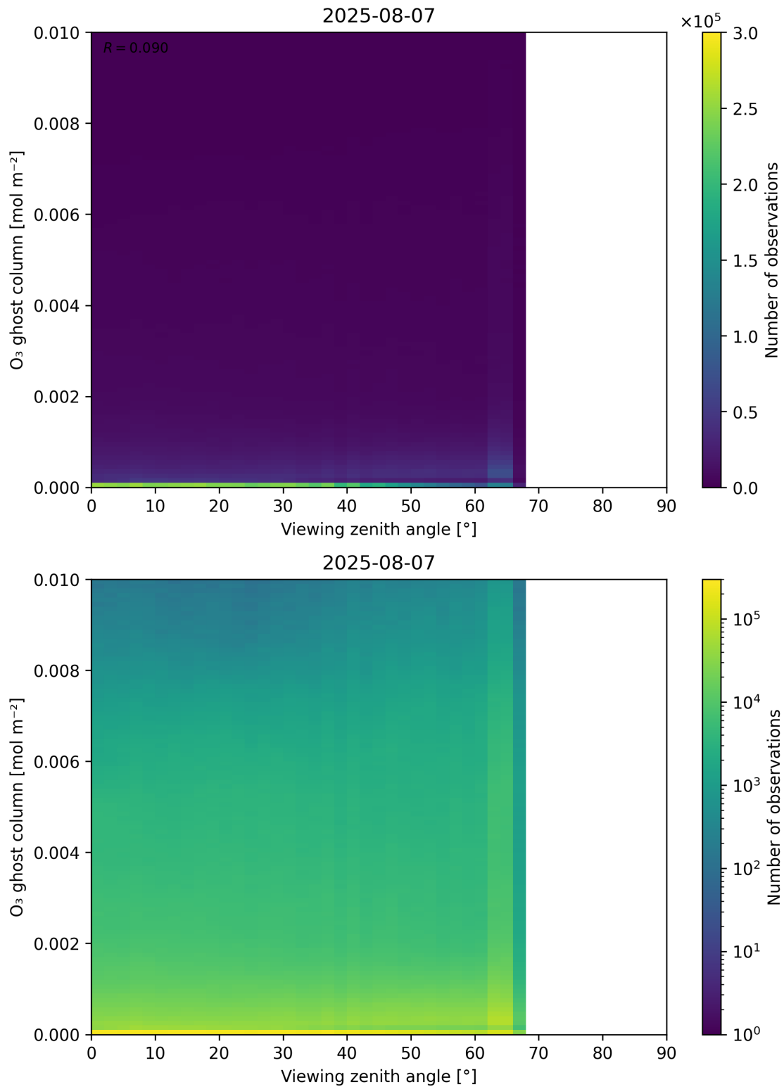
Figure 51: Scatter density plot of “Viewing zenith angle” against “O 3 ghost column” for 2025-08-06 to 2025-08-08.
