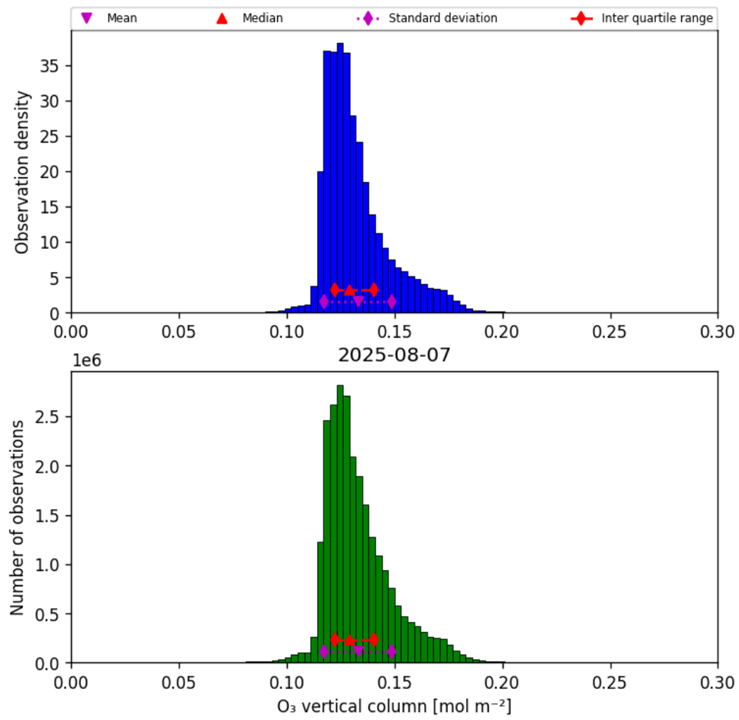
Figure 21: Histogram of “O 3 vertical column” for 2025-08-06 to 2025-08-08
