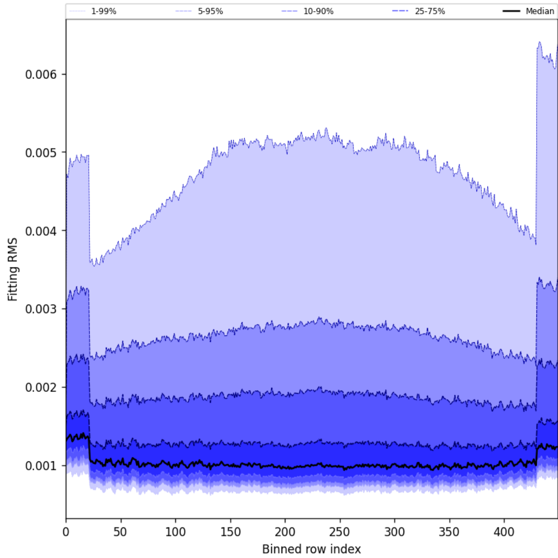
Figure 30: Along track statistics of “Fitting RMS” for 2025-08-06 to 2025-08-08
