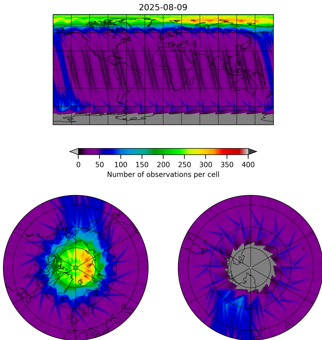
Figure 12: Map of the number of observations for 2025-08-09 to 2025-08-10
