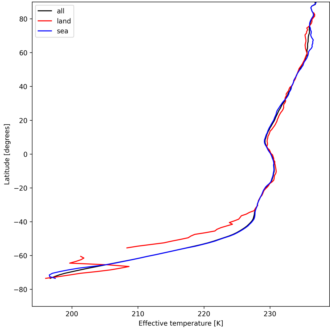
Figure 17: Zonal average of "Effective temperature" for 2025-08-09 to 2025-08-10.
