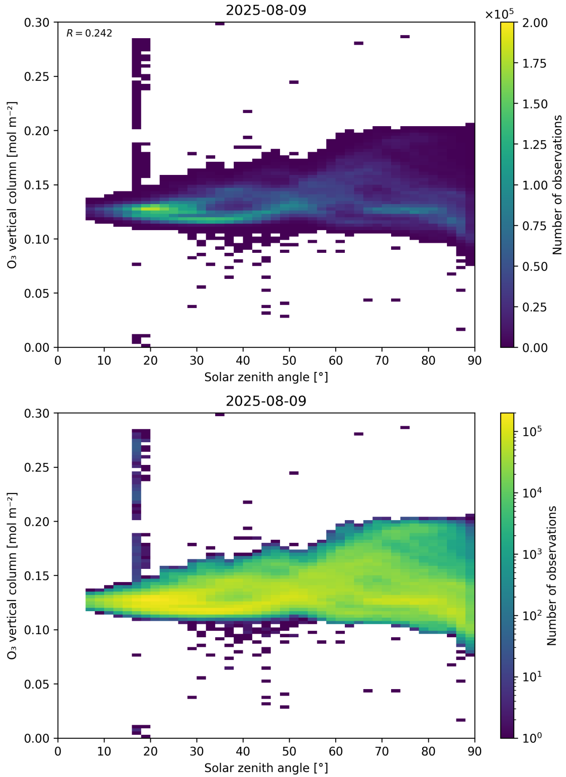
Figure 47: Scatter density plot of “Solar zenith angle” against “O 3 vertical column” for 2025-08-09 to 2025-08-10.
