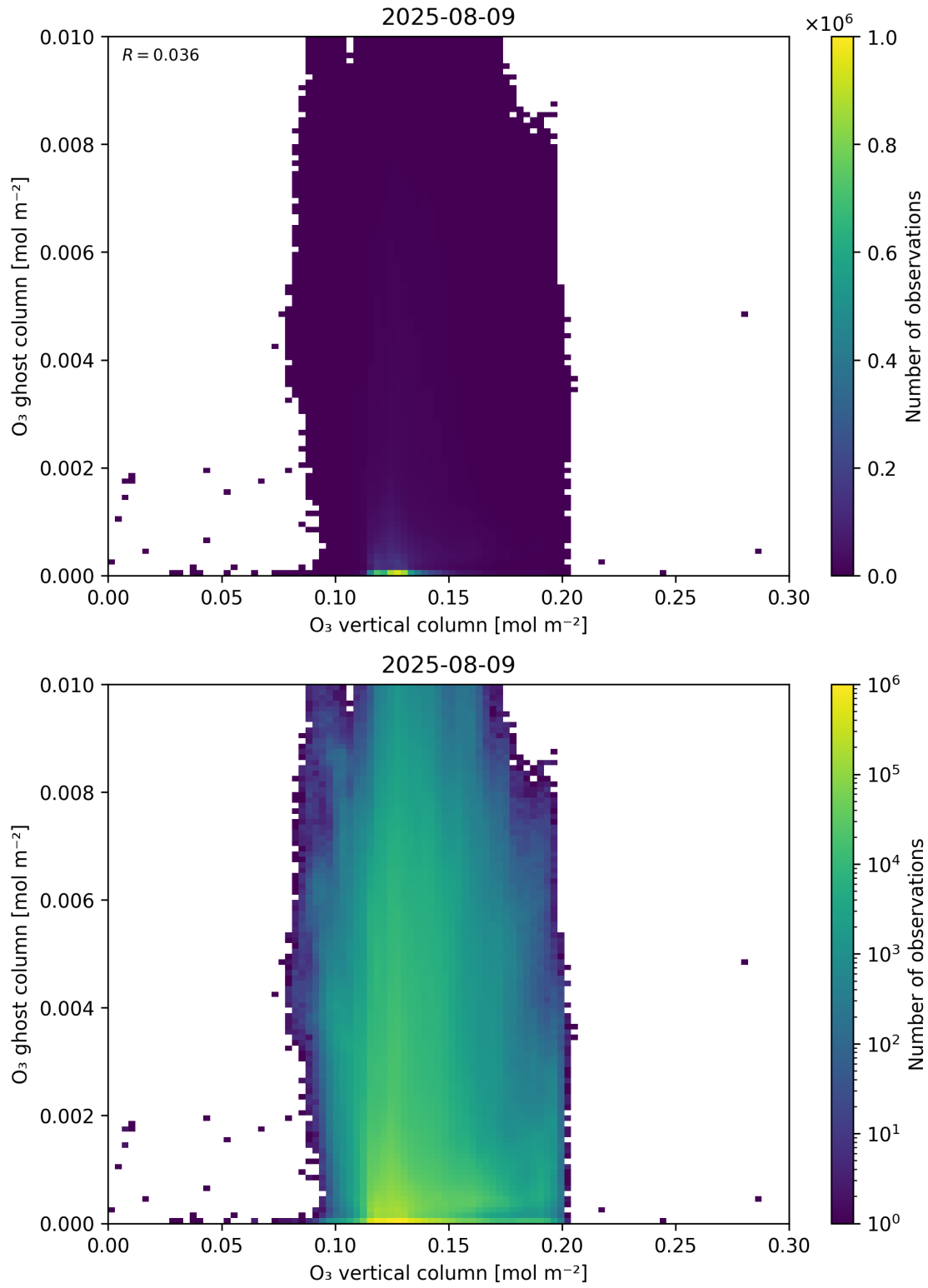
Figure 40: Scatter density plot of “O 3 vertical column” against “O 3 ghost column” for 2025-08-09 to 2025-08-10.
