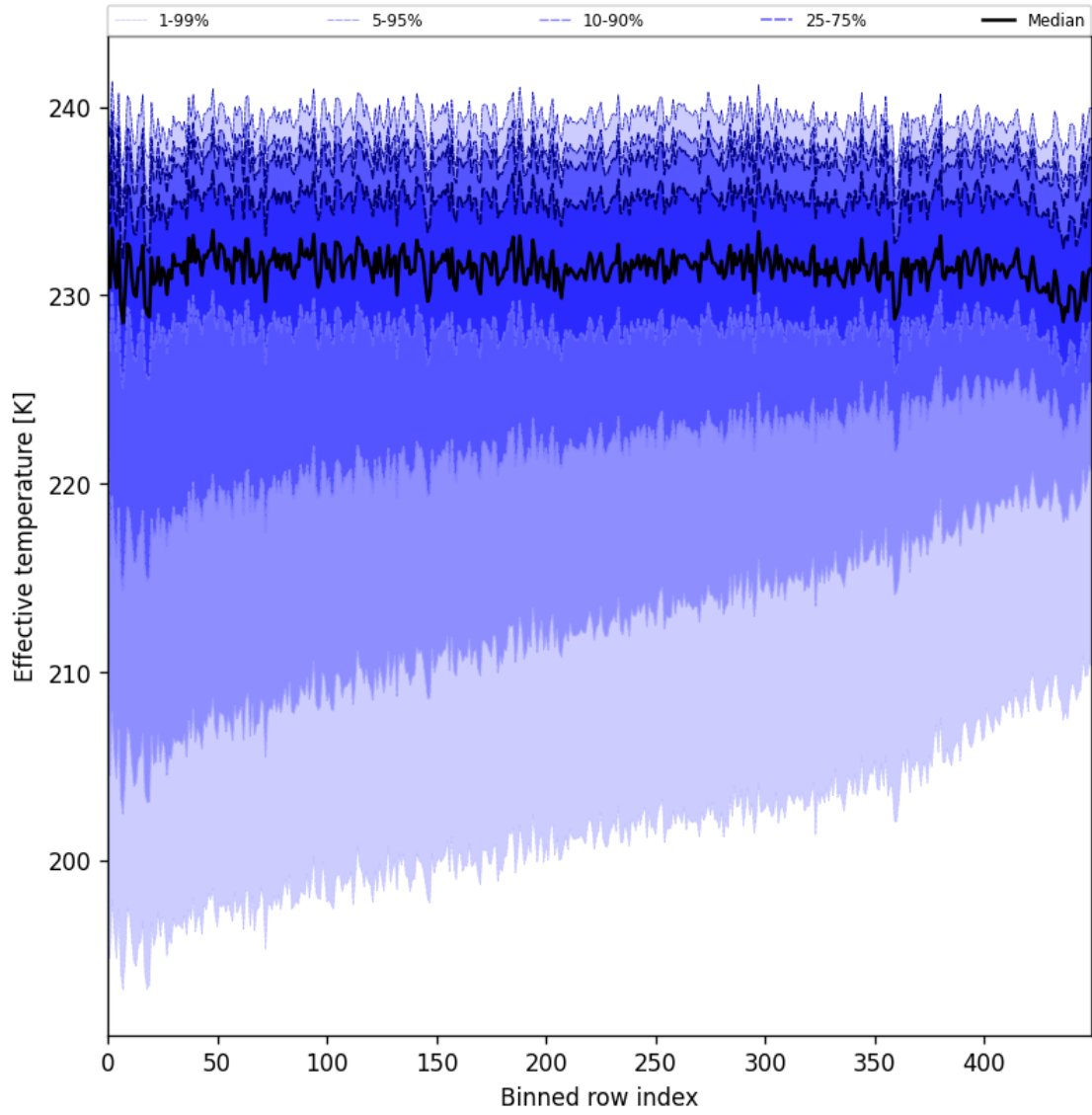
Figure 31: Along track statistics of “Effective temperature” for 2025-08-09 to 2025-08-10
