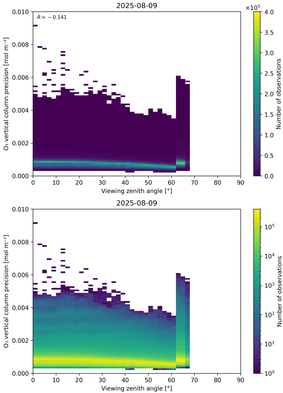
Figure 53: Scatter density plot of “Viewing zenith angle” against “O 3 vertical column precision” for 2025-08-09 to 2025-08-10.
