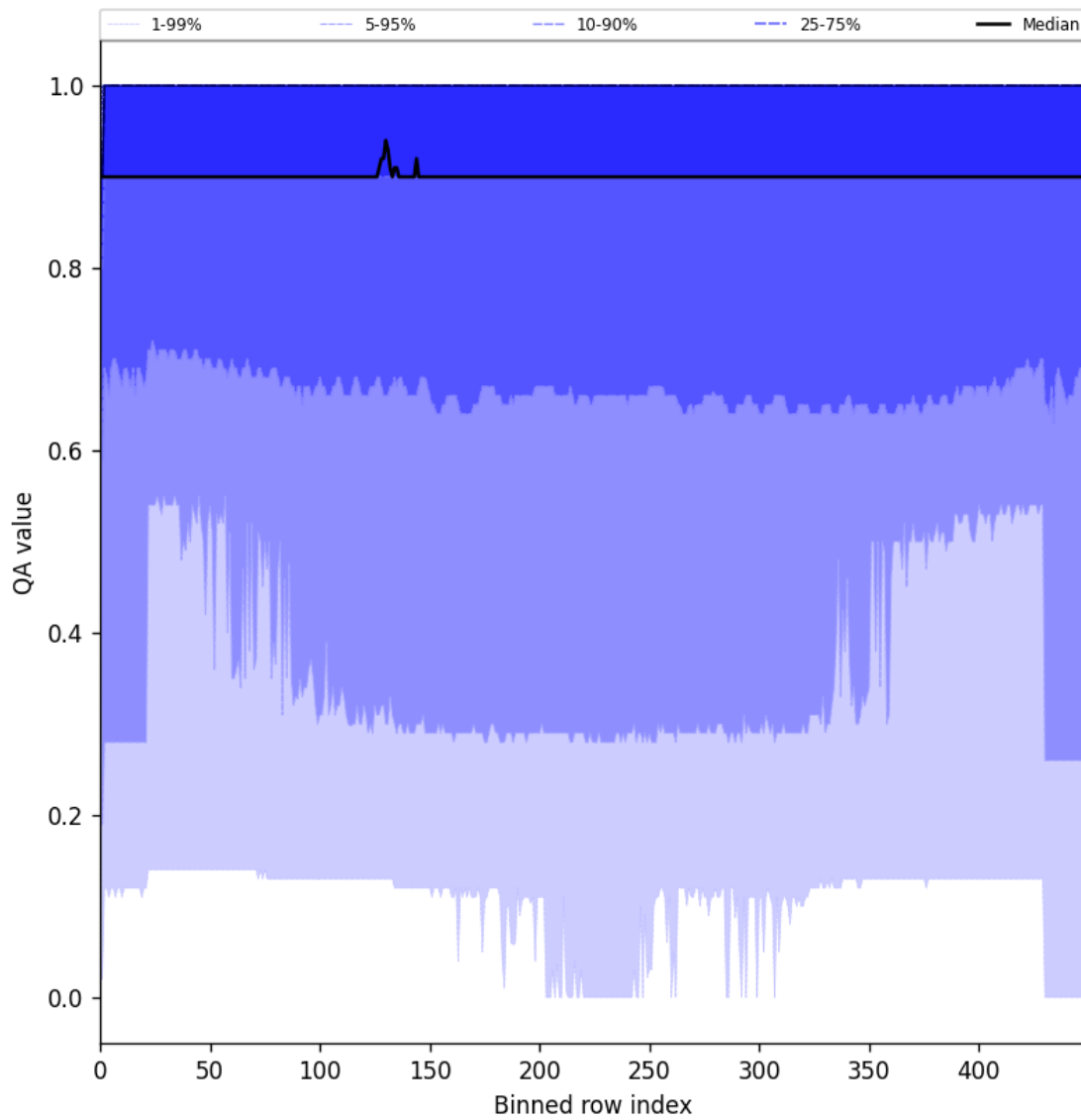
Figure 27: Along track statistics of “QA value” for 2025-08-09 to 2025-08-10
