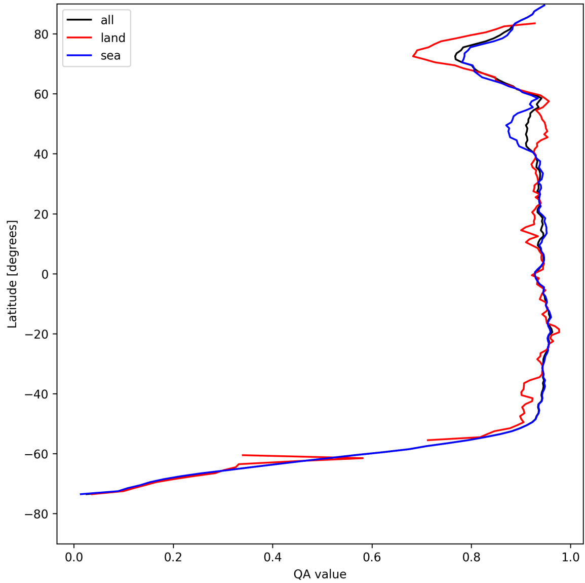
Figure 13: Zonal average of “QA value” for 2025-08-09 to 2025-08-10.
