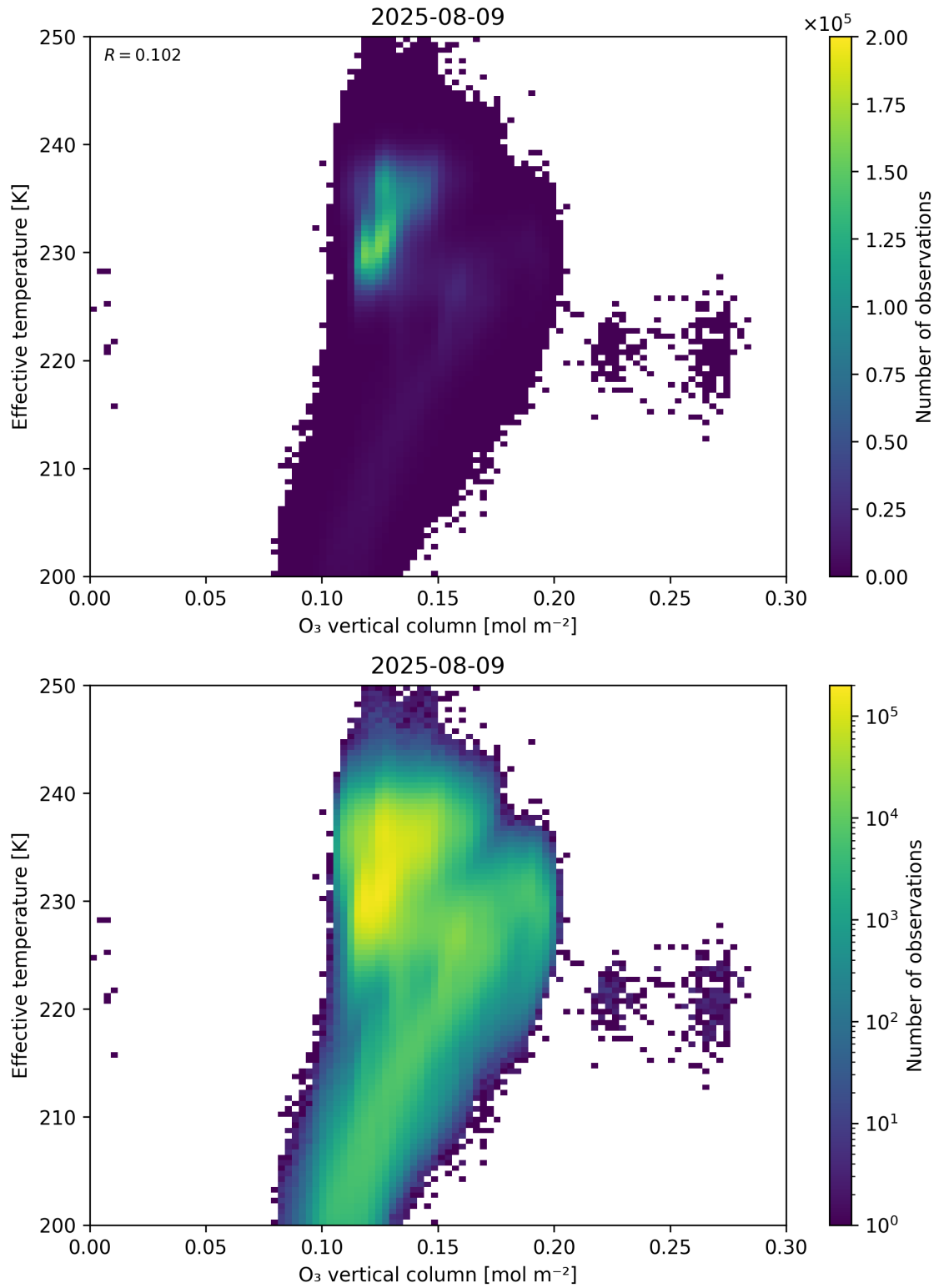
Figure 39: Scatter density plot of “O 3 vertical column” against “Effective temperature” for 2025-08-09 to 2025-08-10.
