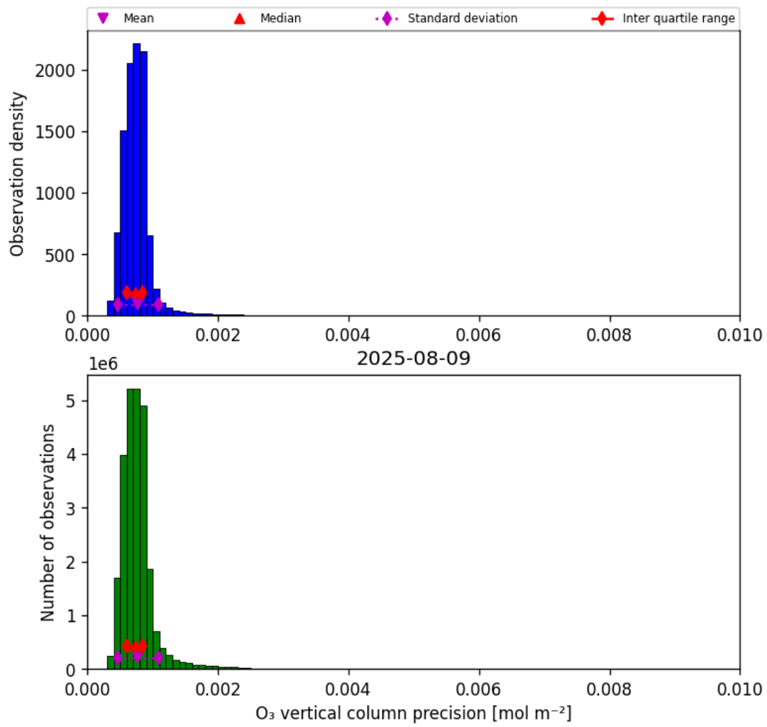
Figure 22: Histogram of “O 3 vertical column precision” for 2025-08-09 to 2025-08-10
