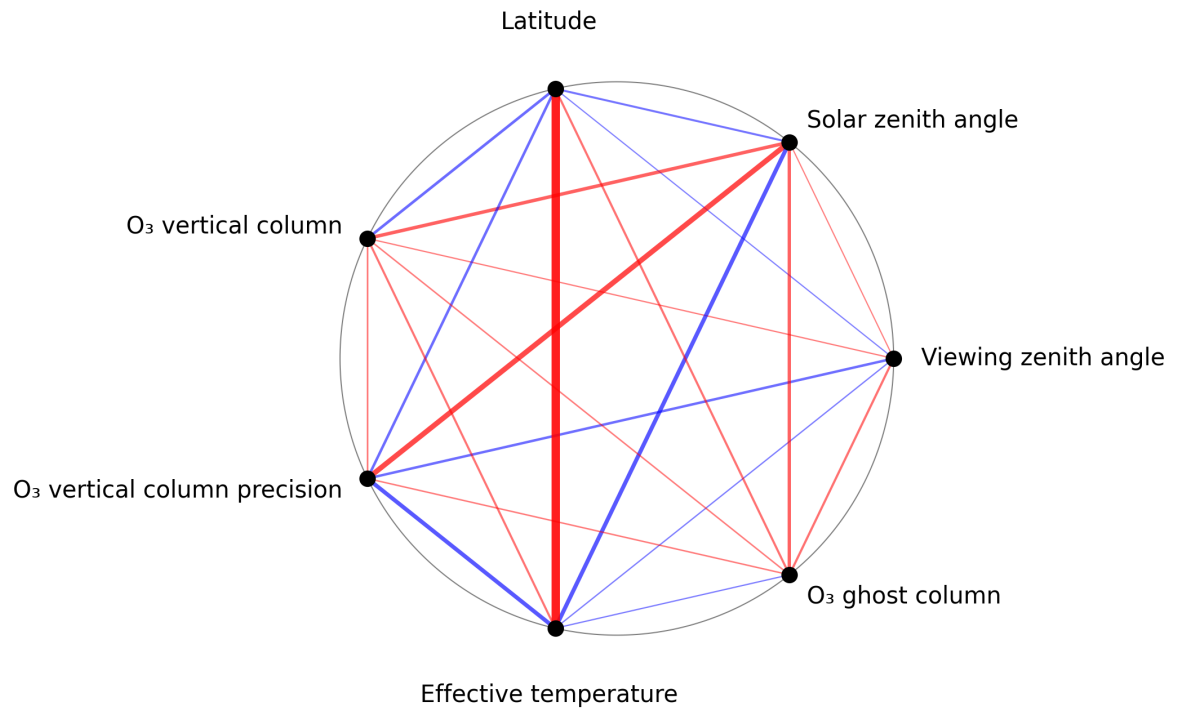
Figure 1: Map of correlation graph for 2025-08-09 to 2025-08-10.
