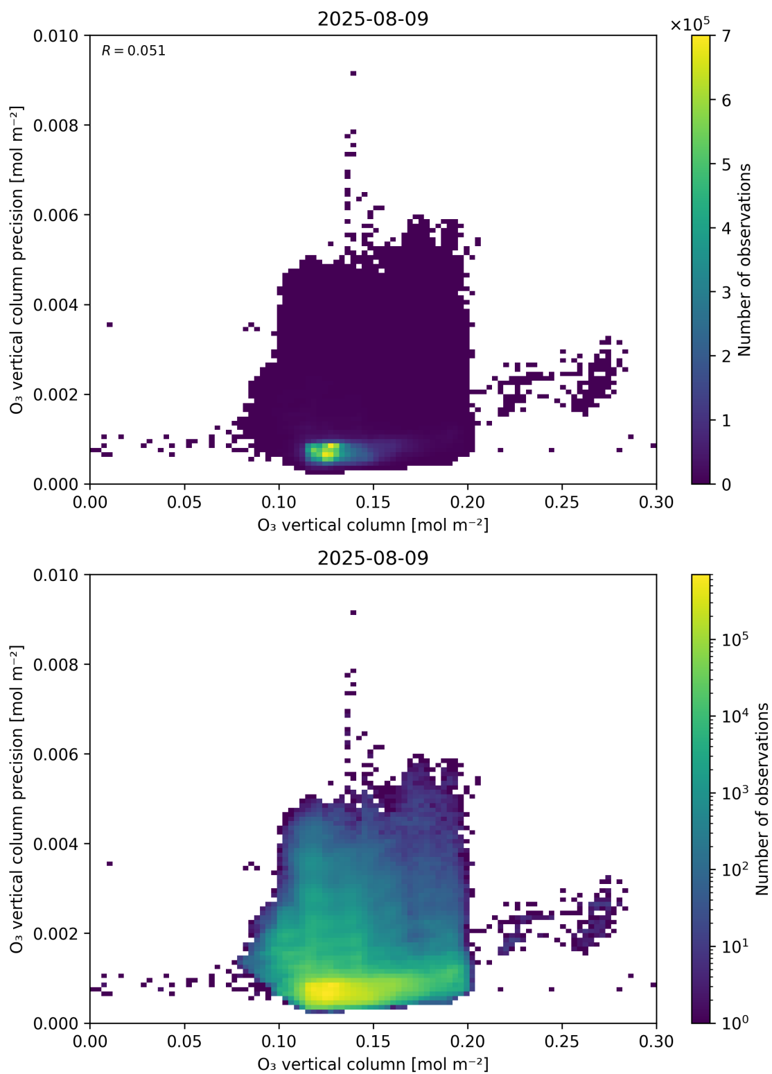
Figure 41: Scatter density plot of “O 3 vertical column” against “O 3 vertical column precision” for 2025-08-09 to 2025-08-10.
