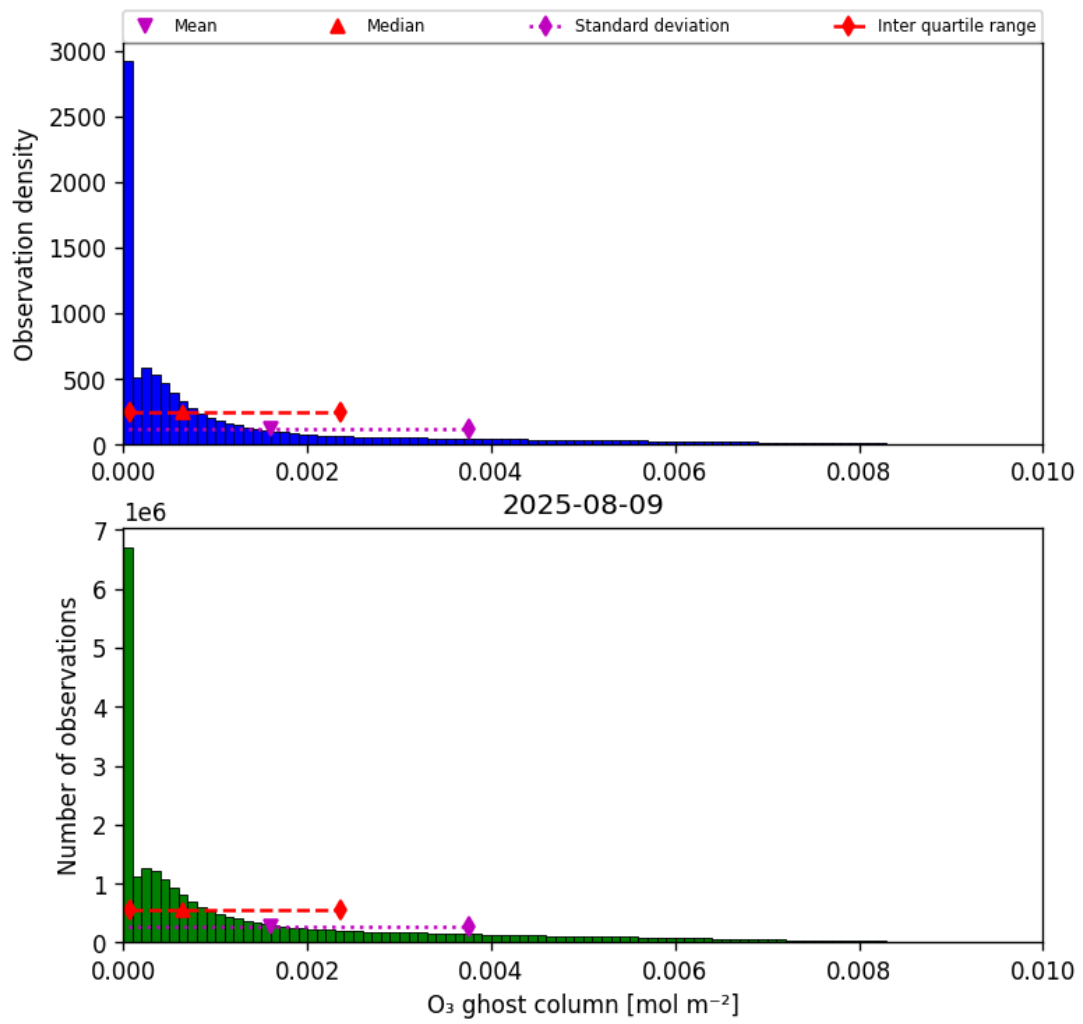
Figure 25: Histogram of “O 3 ghost column” for 2025-08-09 to 2025-08-10
