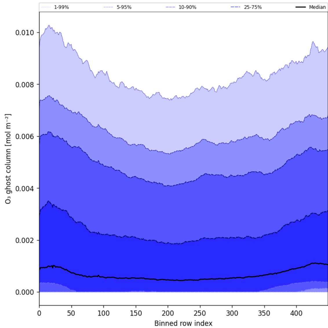
Figure 32: Along track statistics of “O 3 ghost column” for 2025-08-09 to 2025-08-10
