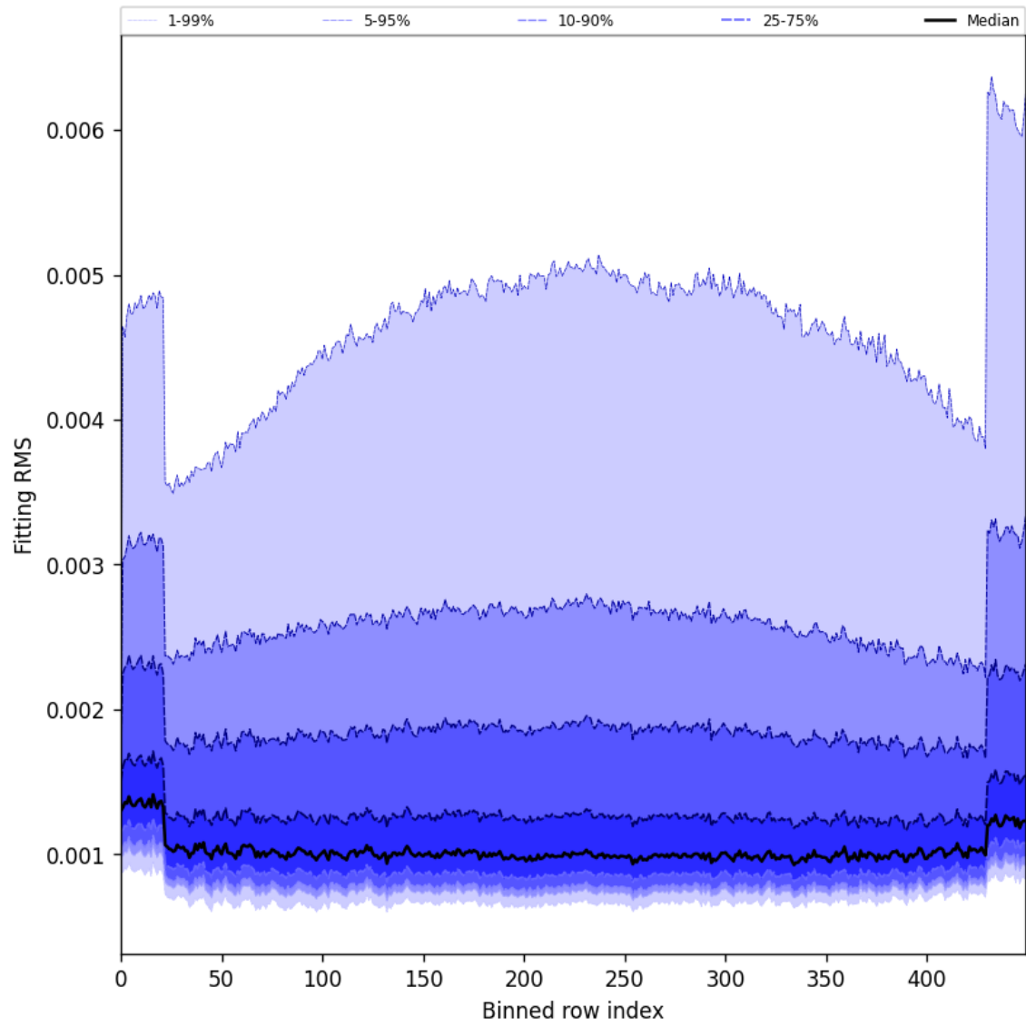
Figure 30: Along track statistics of “Fitting RMS” for 2025-08-09 to 2025-08-10
