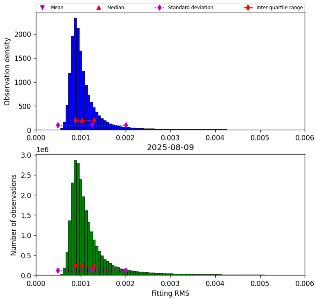
Figure 23: Histogram of “Fitting RMS” for 2025-08-09 to 2025-08-10
