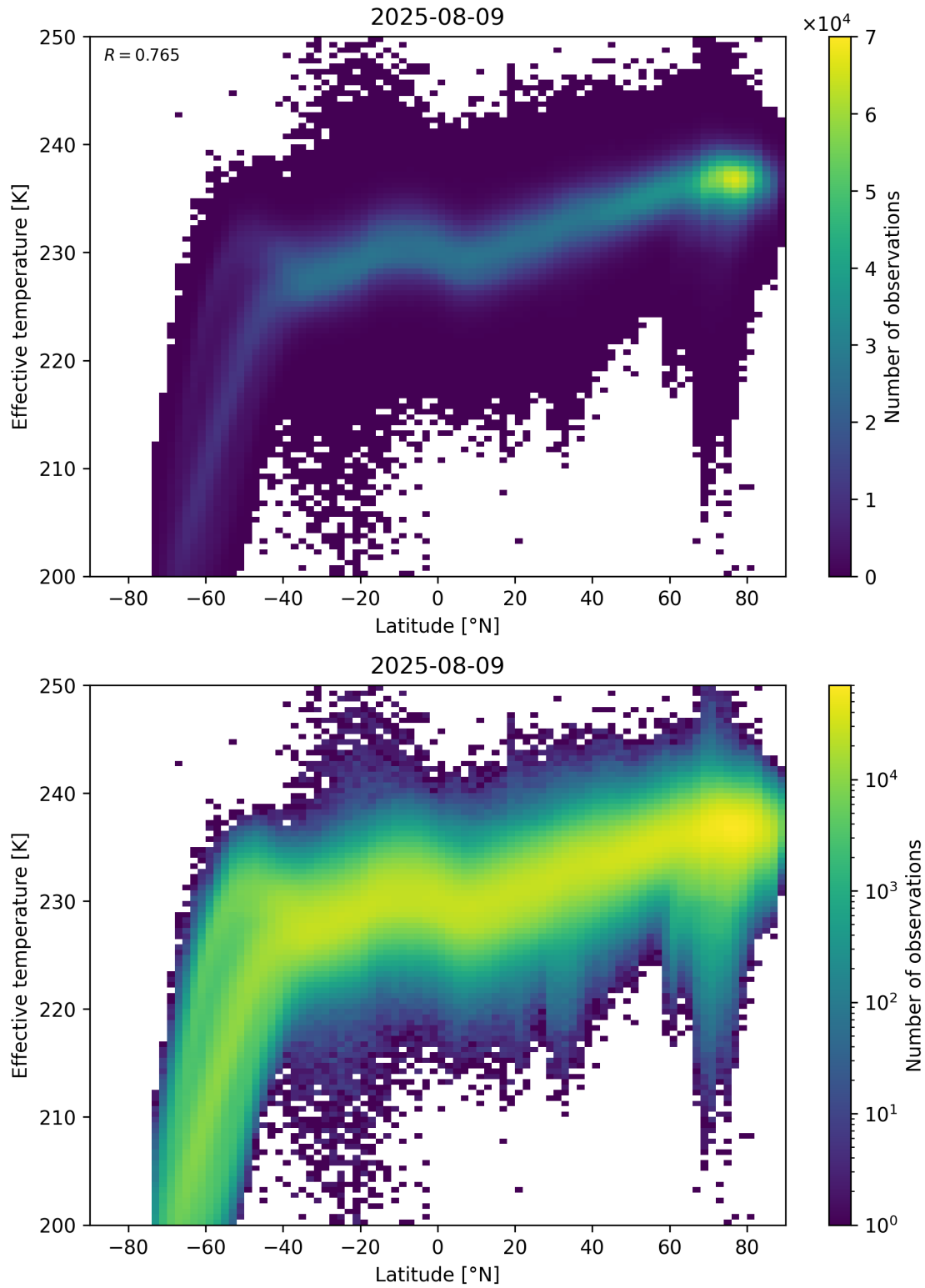
Figure 34: Scatter density plot of “Latitude” against “Effective temperature” for 2025-08-09 to 2025-08-10.
