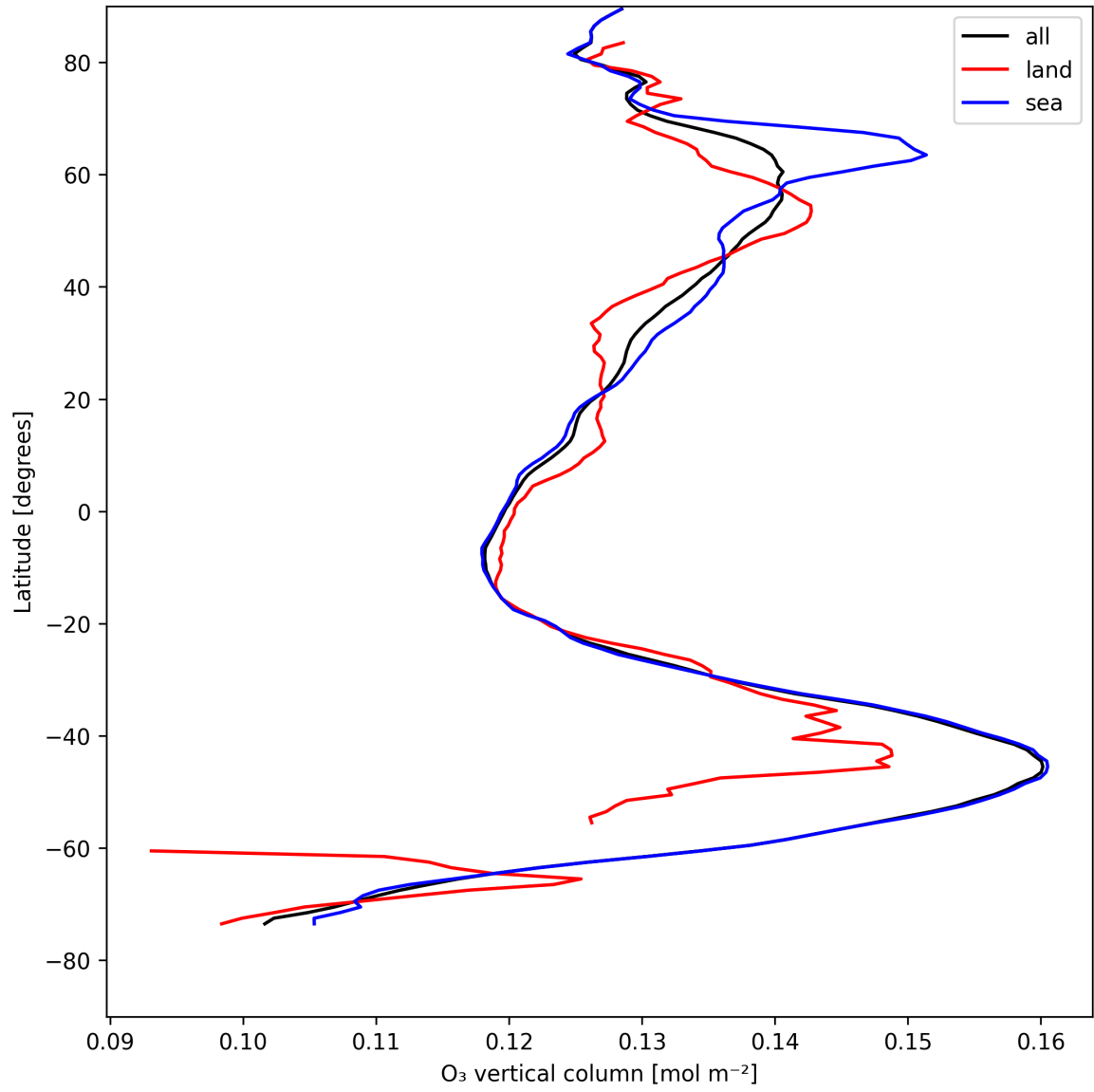
Figure 14: Zonal average of “O 3 vertical column” for 2025-08-09 to 2025-08-10.
