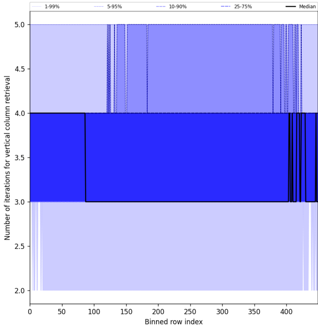
Figure 33: Along track statistics of “Number of iterations for vertical column retrieval” for 2025-08-09 to 2025-08-10
