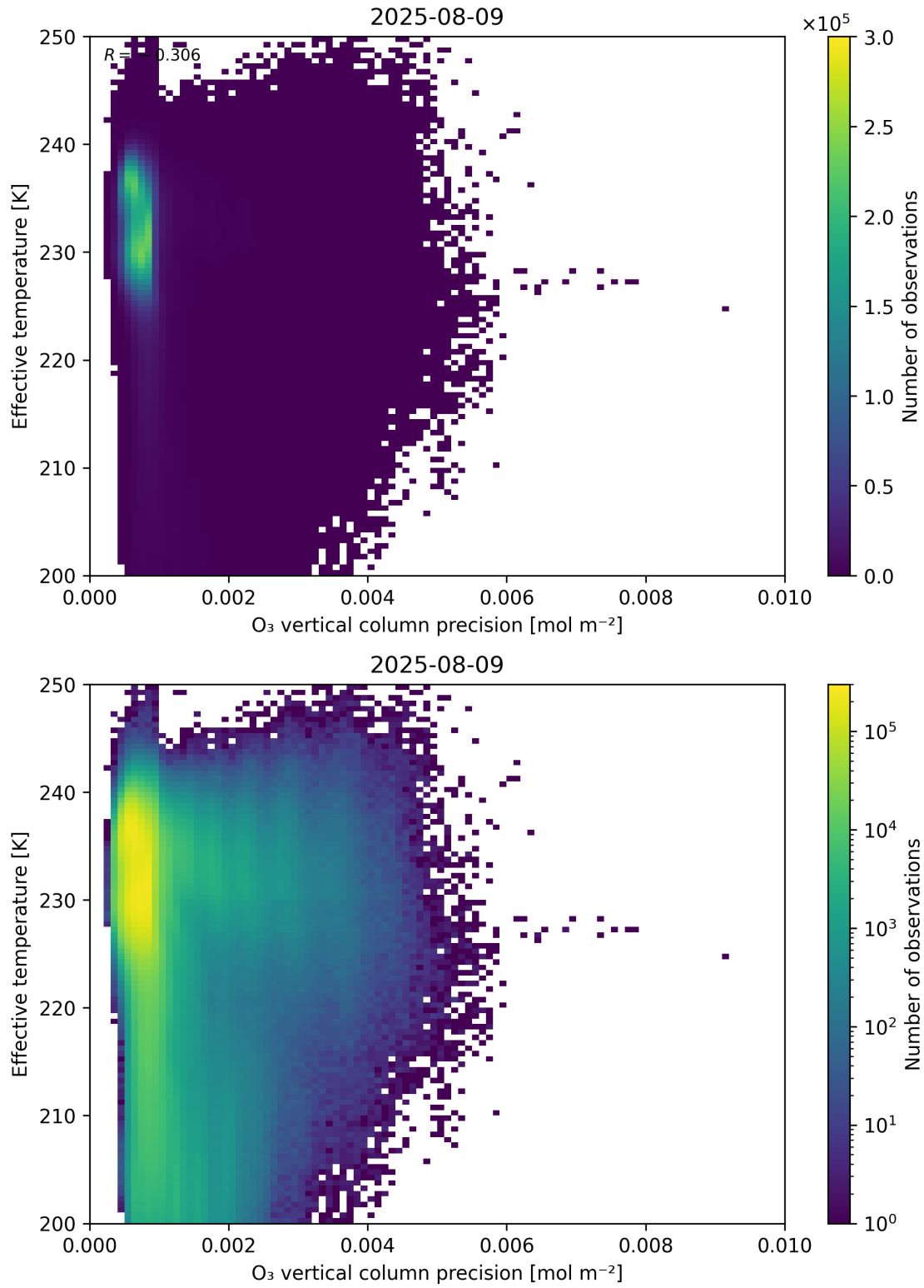
Figure 42: Scatter density plot of “O 3 vertical column precision” against “Effective temperature” for 2025-08-09 to 2025-08-10.
