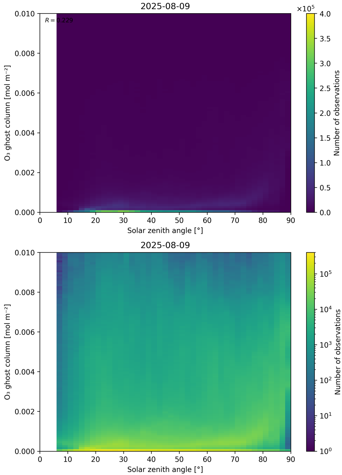
Figure 46: Scatter density plot of “Solar zenith angle” against “O 3 ghost column” for 2025-08-09 to 2025-08-10.
