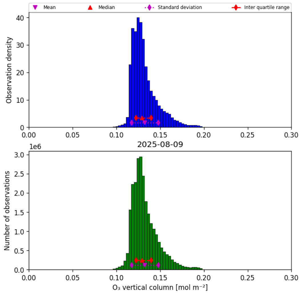
Figure 21: Histogram of “O 3 vertical column” for 2025-08-09 to 2025-08-10
