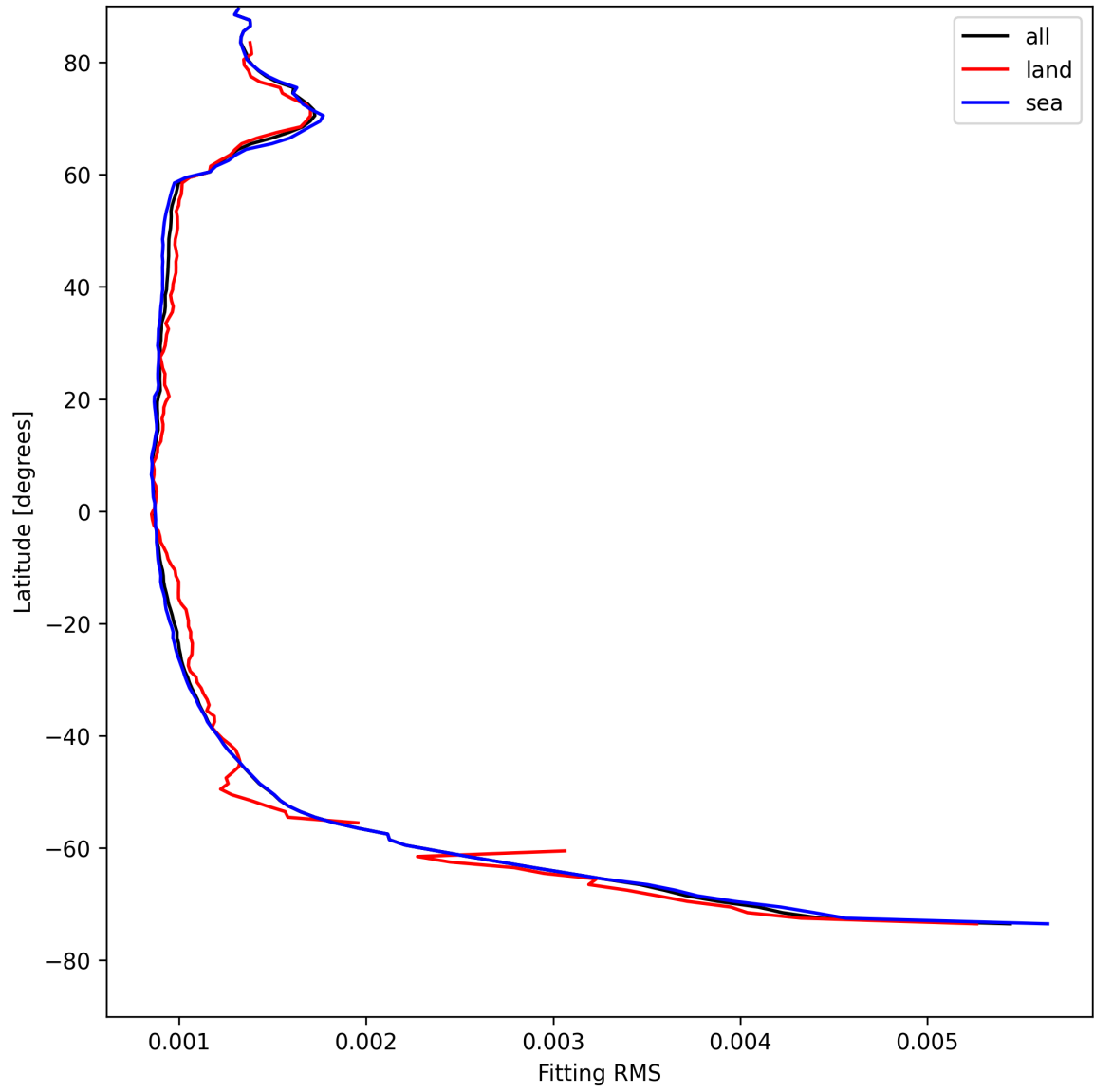
Figure 16: Zonal average of “Fitting RMS” for 2025-08-09 to 2025-08-10.
