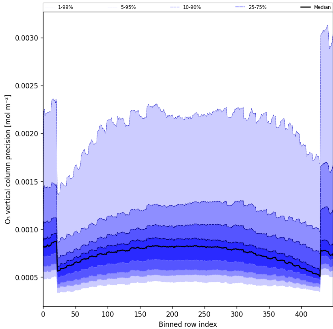
Figure 29: Along track statistics of “O 3 vertical column precision” for 2025-08-09 to 2025-08-10
