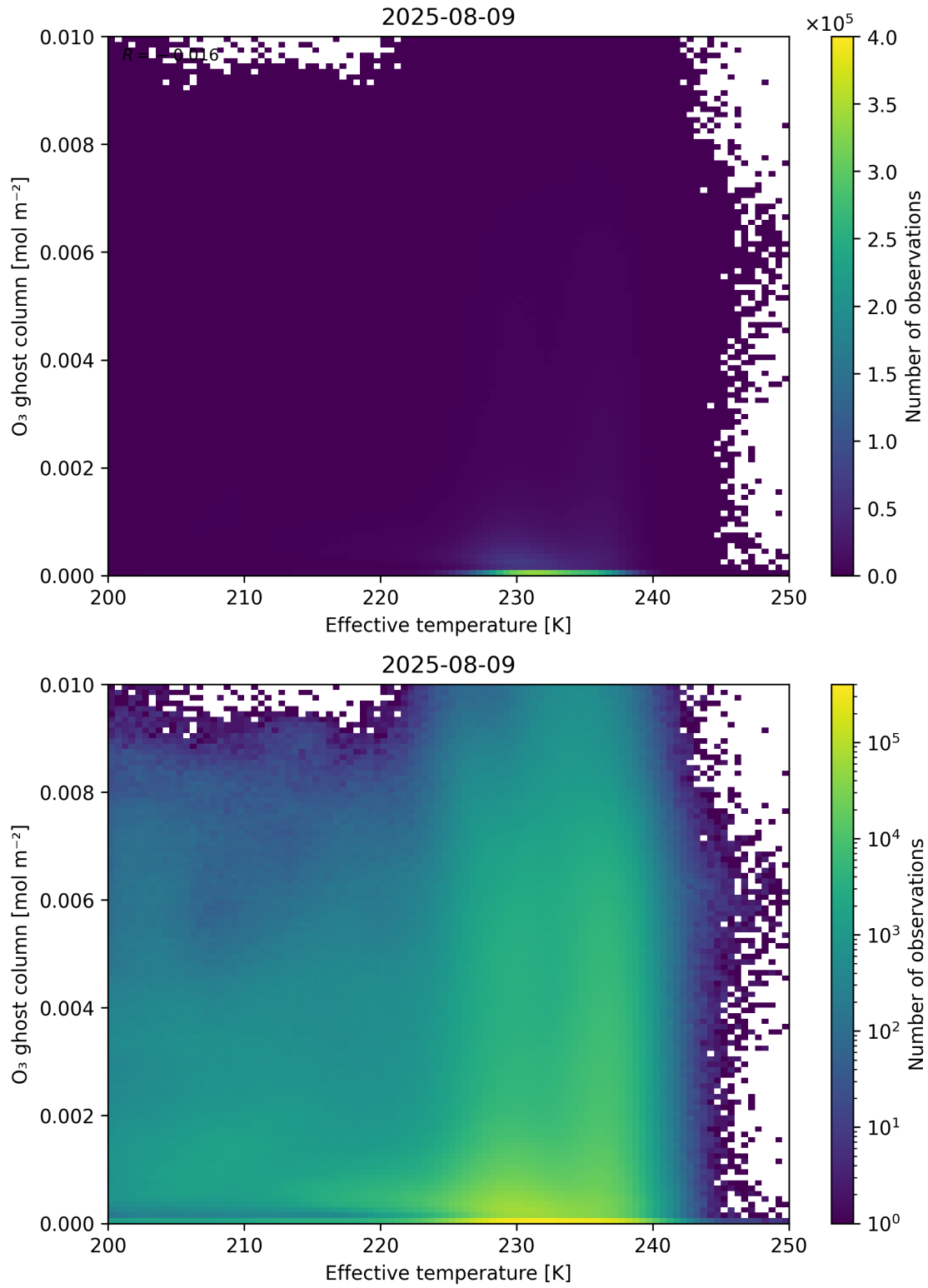
Figure 38: Scatter density plot of “Effective temperature” against “O 3 ghost column” for 2025-08-09 to 2025-08-10.
