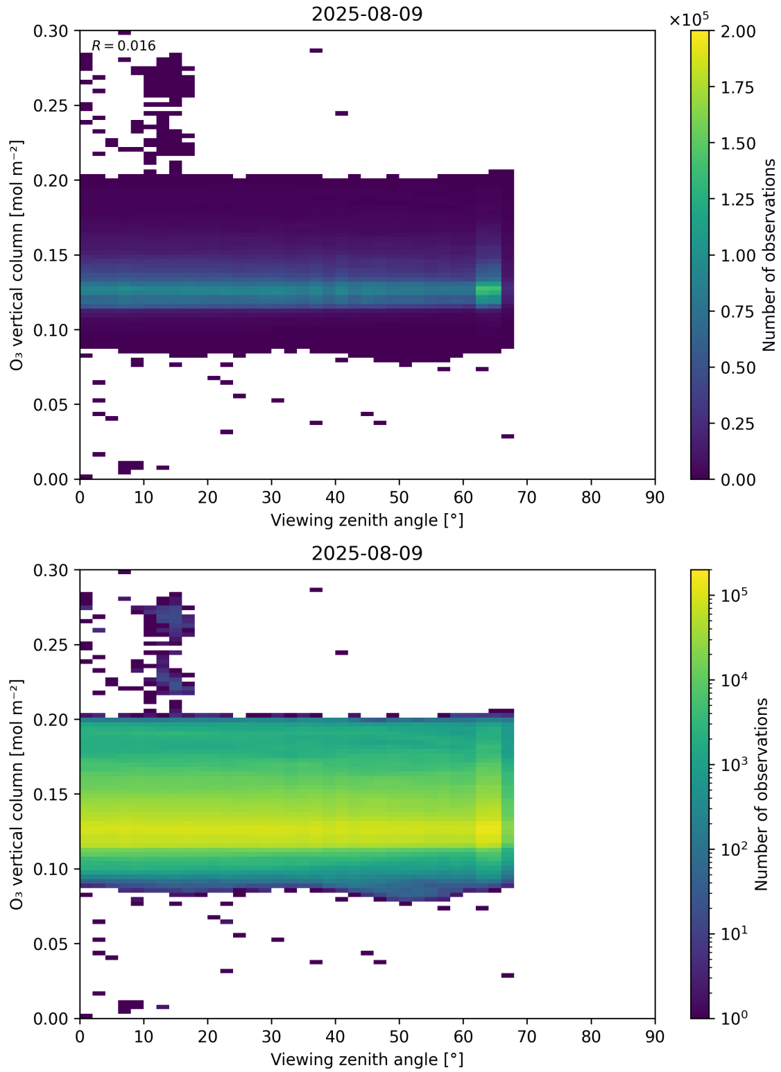
Figure 52: Scatter density plot of “Viewing zenith angle” against “O 3 vertical column” for 2025-08-09 to 2025-08-10.
