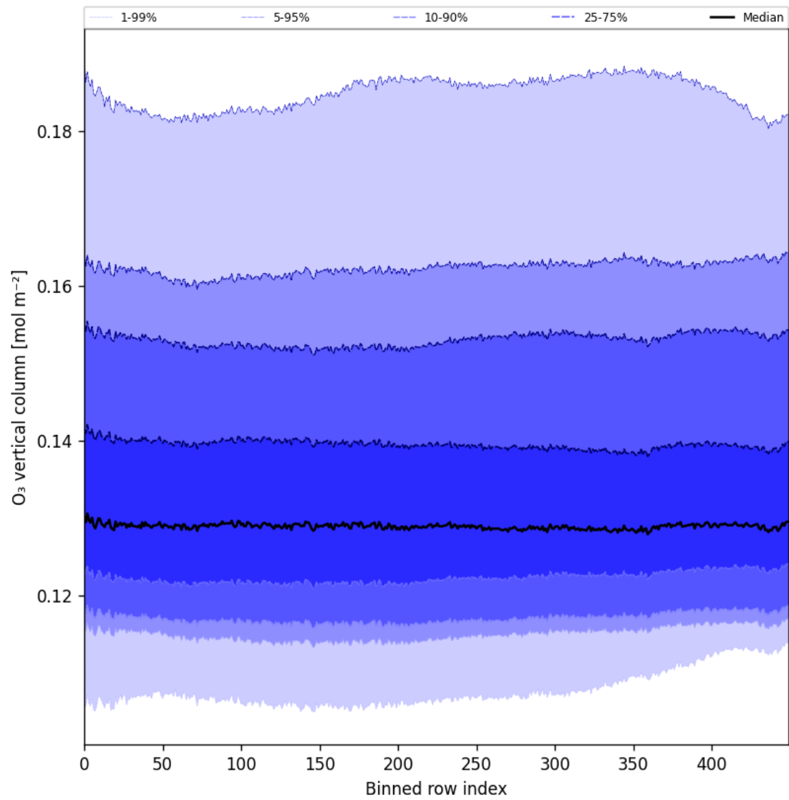
Figure 28: Along track statistics of “O 3 vertical column” for 2025-08-09 to 2025-08-10
