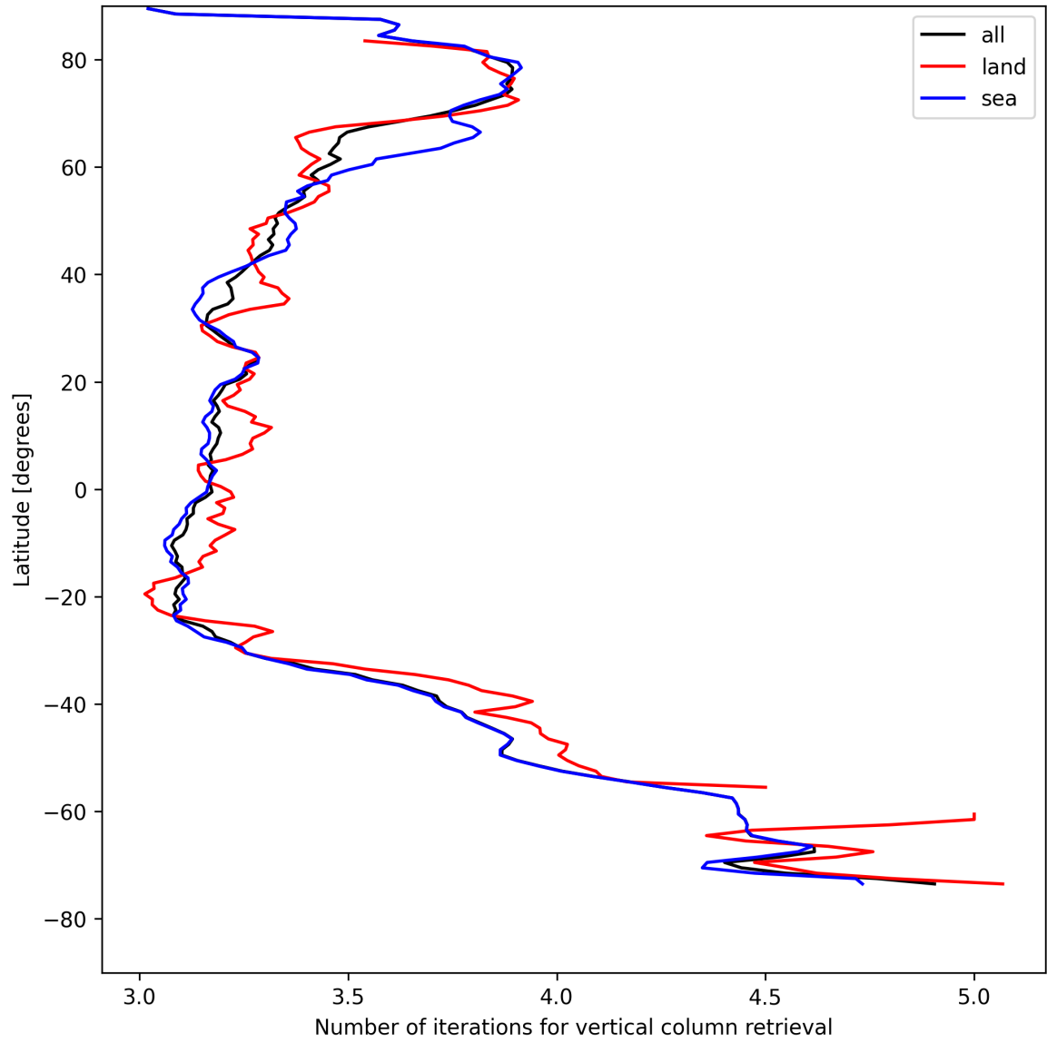
Figure 19: Zonal average of “Number of iterations for vertical column retrieval” for 2025-08-09 to 2025-08-10.
