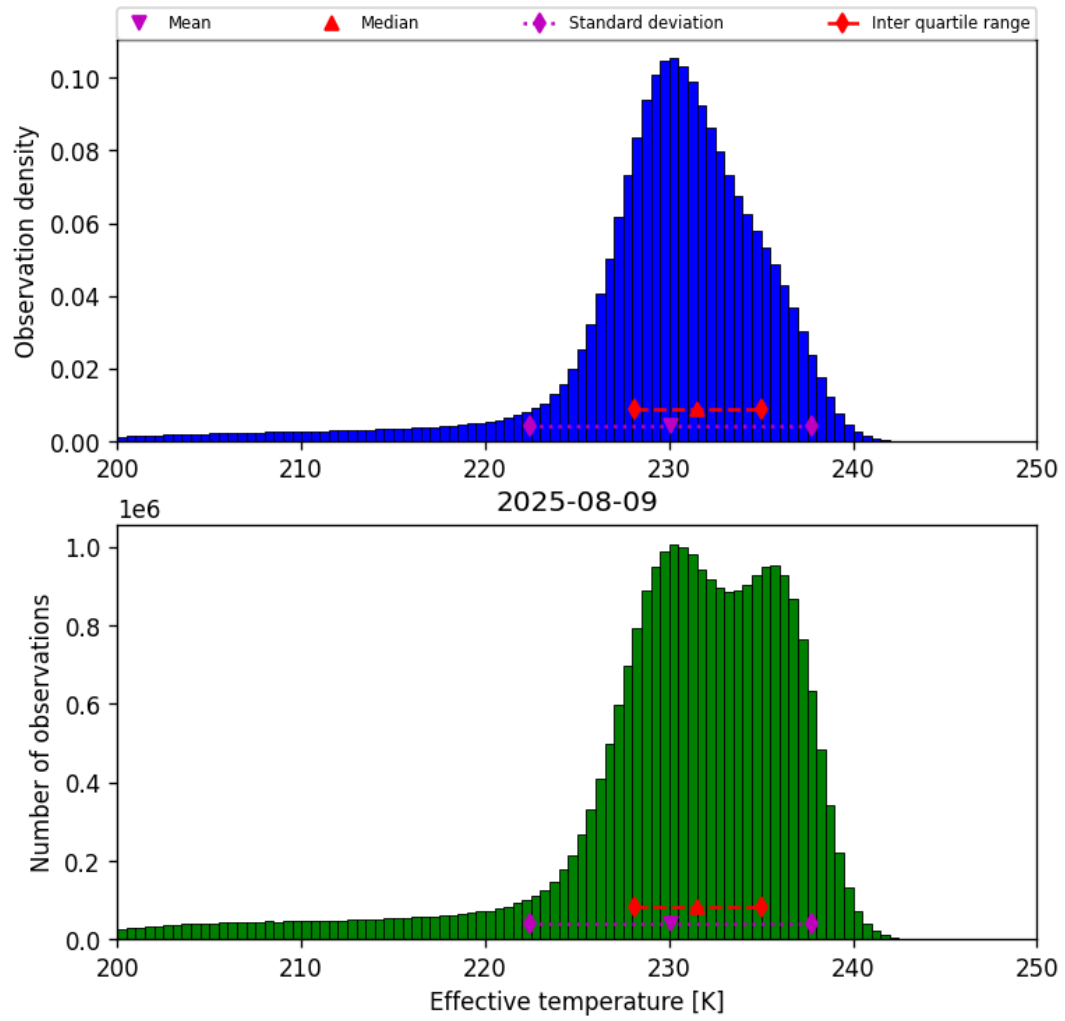
Figure 24: Histogram of “Effective temperature” for 2025-08-09 to 2025-08-10
