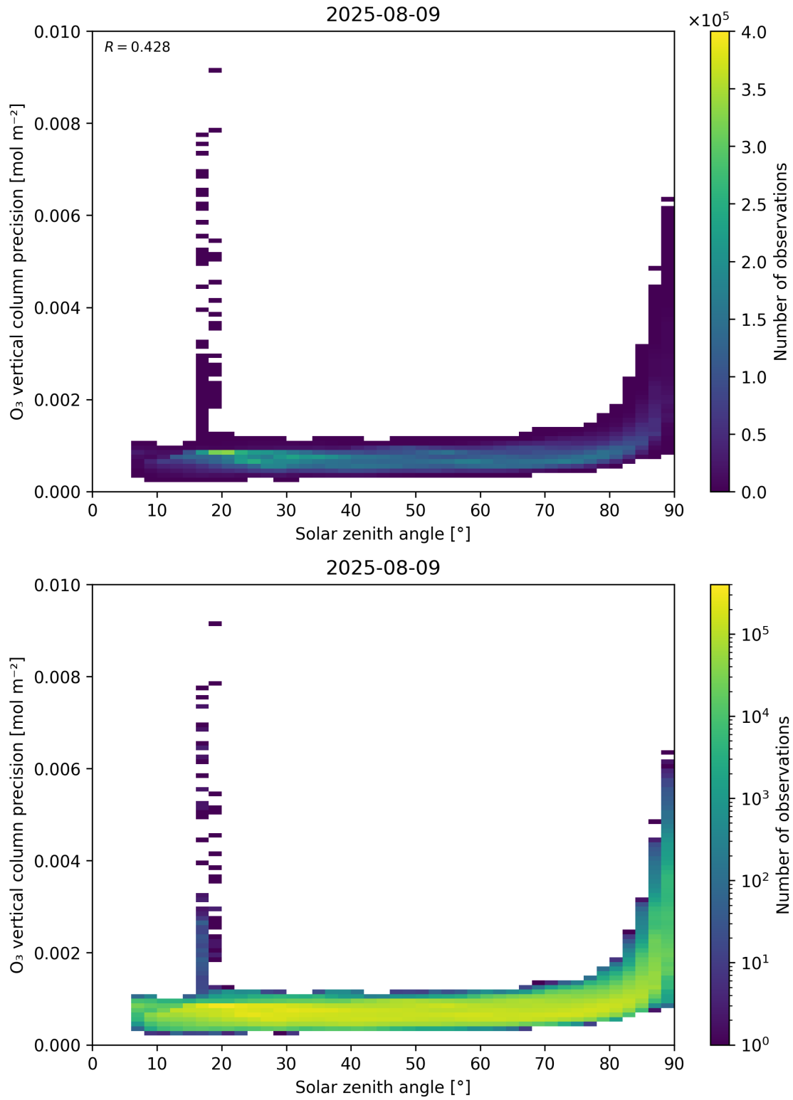
Figure 48: Scatter density plot of “Solar zenith angle” against “O 3 vertical column precision” for 2025-08-09 to 2025-08-10.
