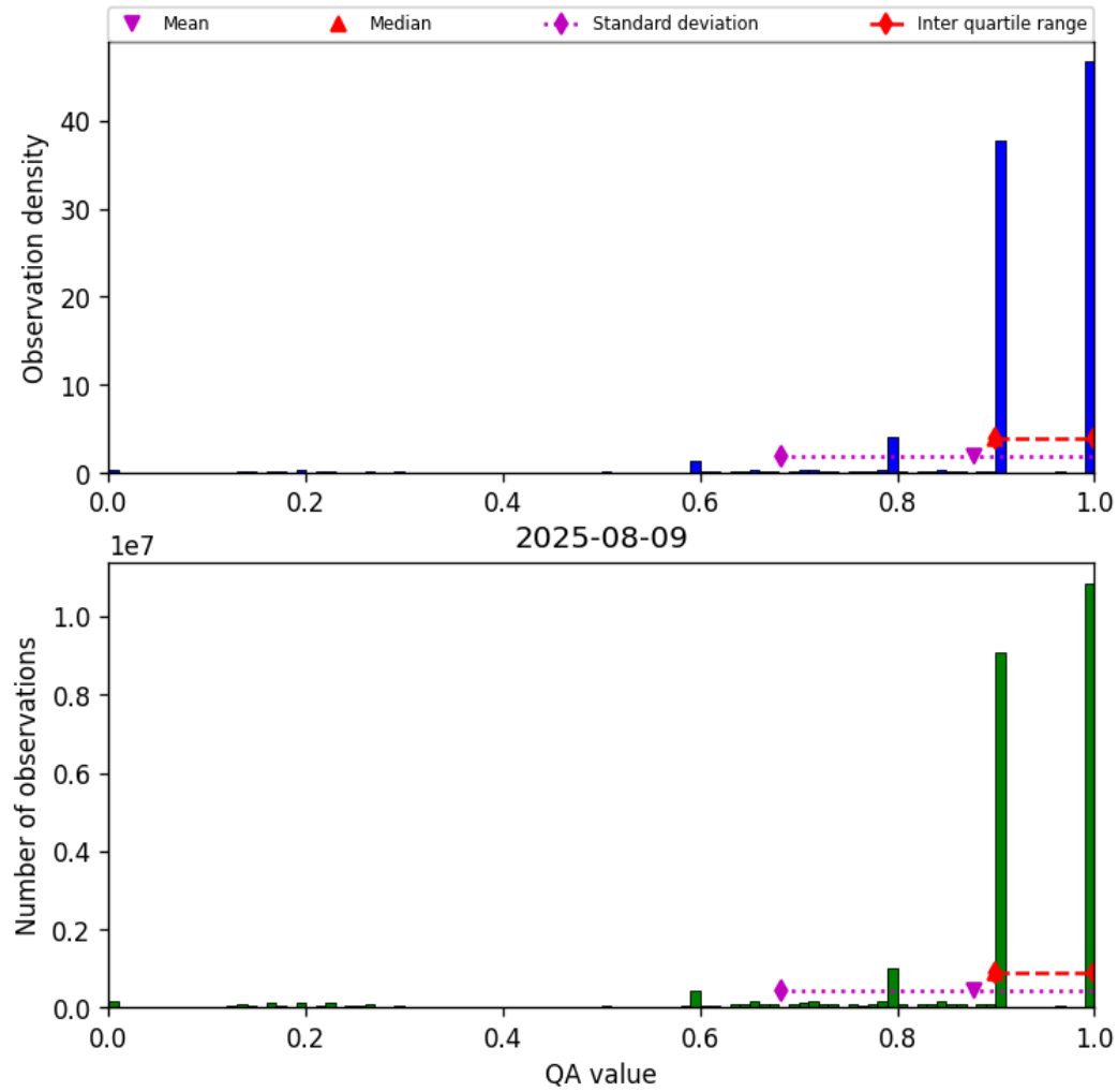
Figure 20: Histogram of “QA value” for 2025-08-09 to 2025-08-10
