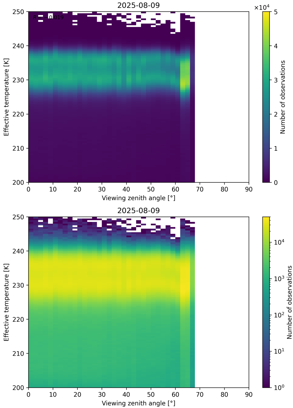
Figure 50: Scatter density plot of “Viewing zenith angle” against “Effective temperature” for 2025-08-09 to 2025-08-10.
