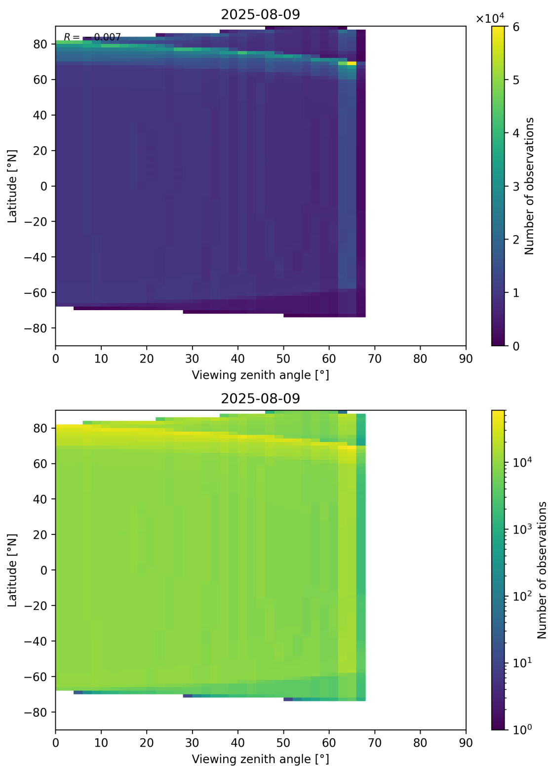
Figure 49: Scatter density plot of “Viewing zenith angle” against “Latitude” for 2025-08-09 to 2025-08-10.
