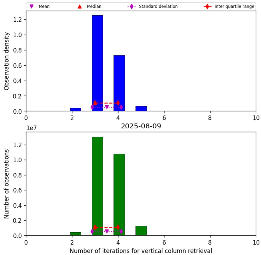
Figure 26: Histogram of “Number of iterations for vertical column retrieval” for 2025-08-09 to 2025-08-10
