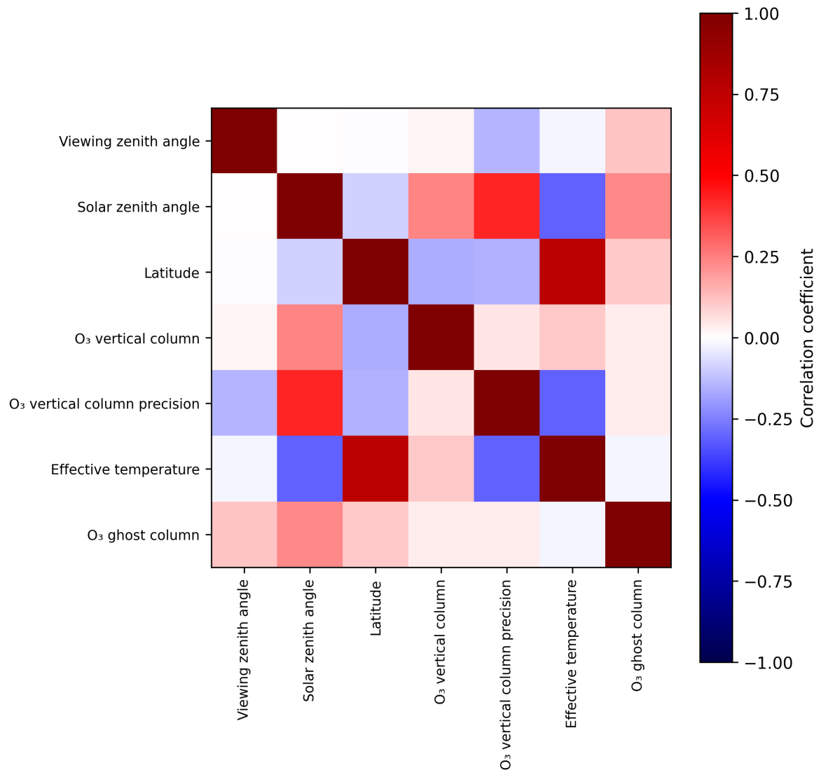
Figure 2: Map of correlation matrix for 2025-08-09 to 2025-08-10.
