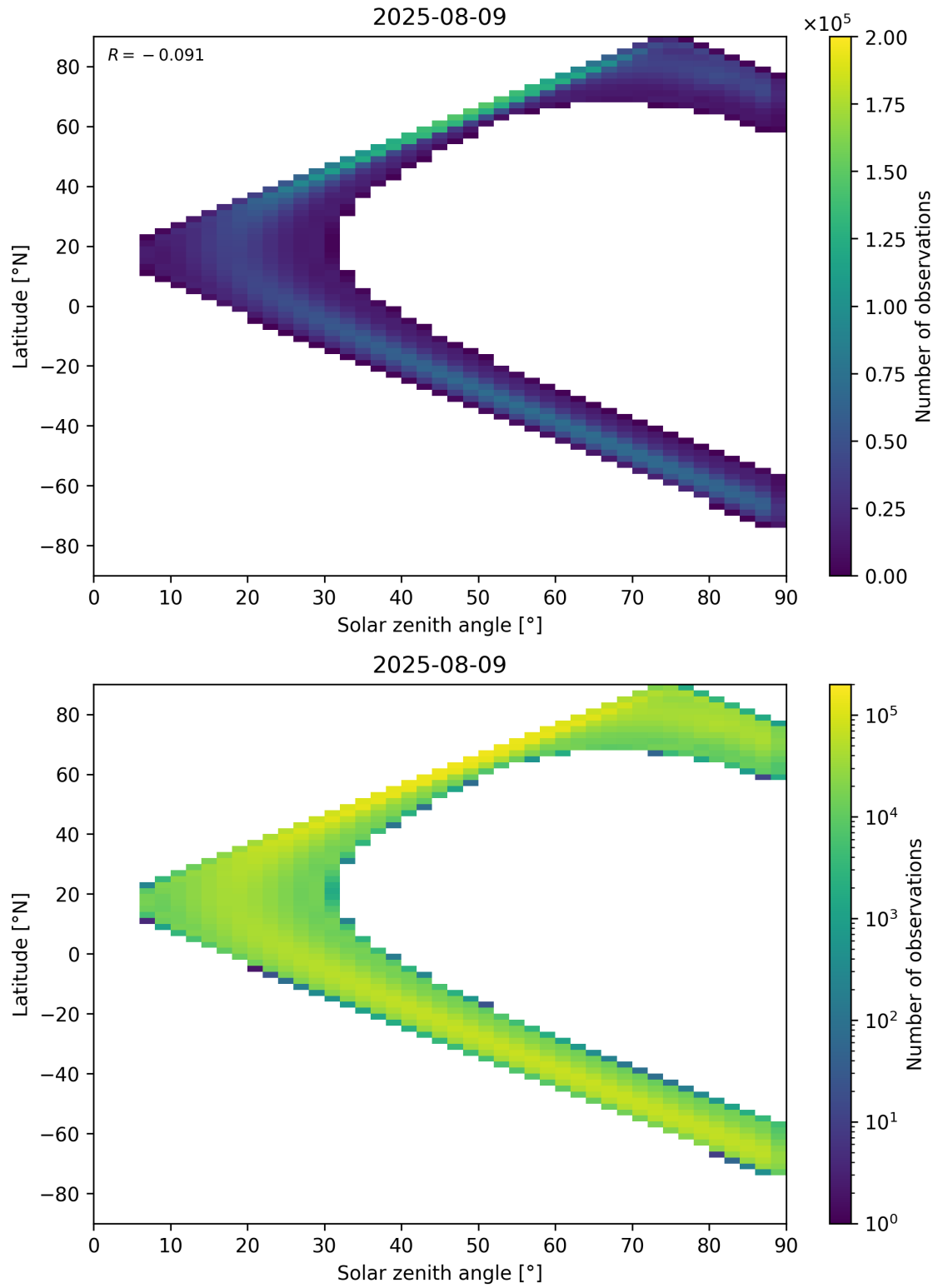
Figure 44: Scatter density plot of “Solar zenith angle” against “Latitude” for 2025-08-09 to 2025-08-10.
