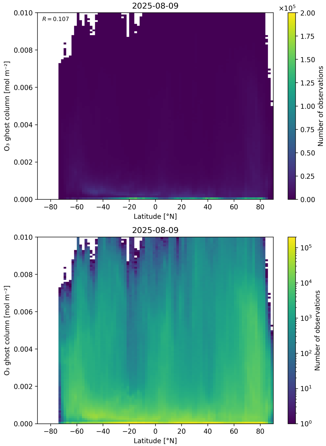
Figure 35: Scatter density plot of “Latitude” against “O 3 ghost column” for 2025-08-09 to 2025-08-10.
