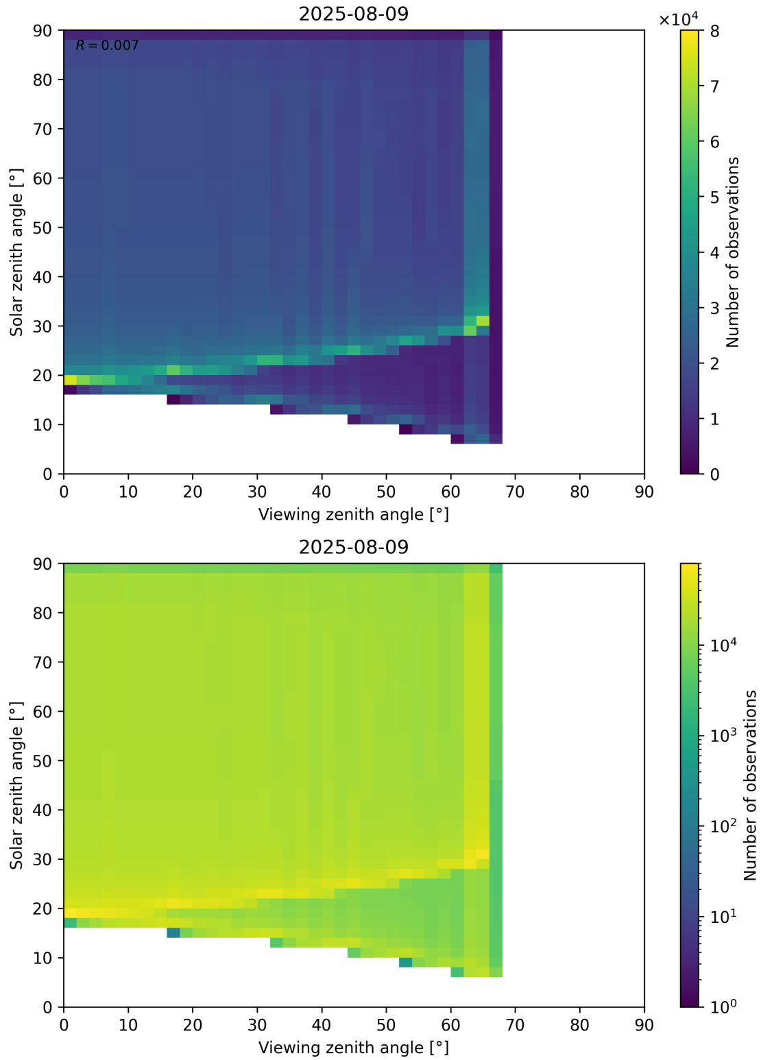
Figure 54: Scatter density plot of “Viewing zenith angle” against “Solar zenith angle” for 2025-08-09 to 2025-08-10.
