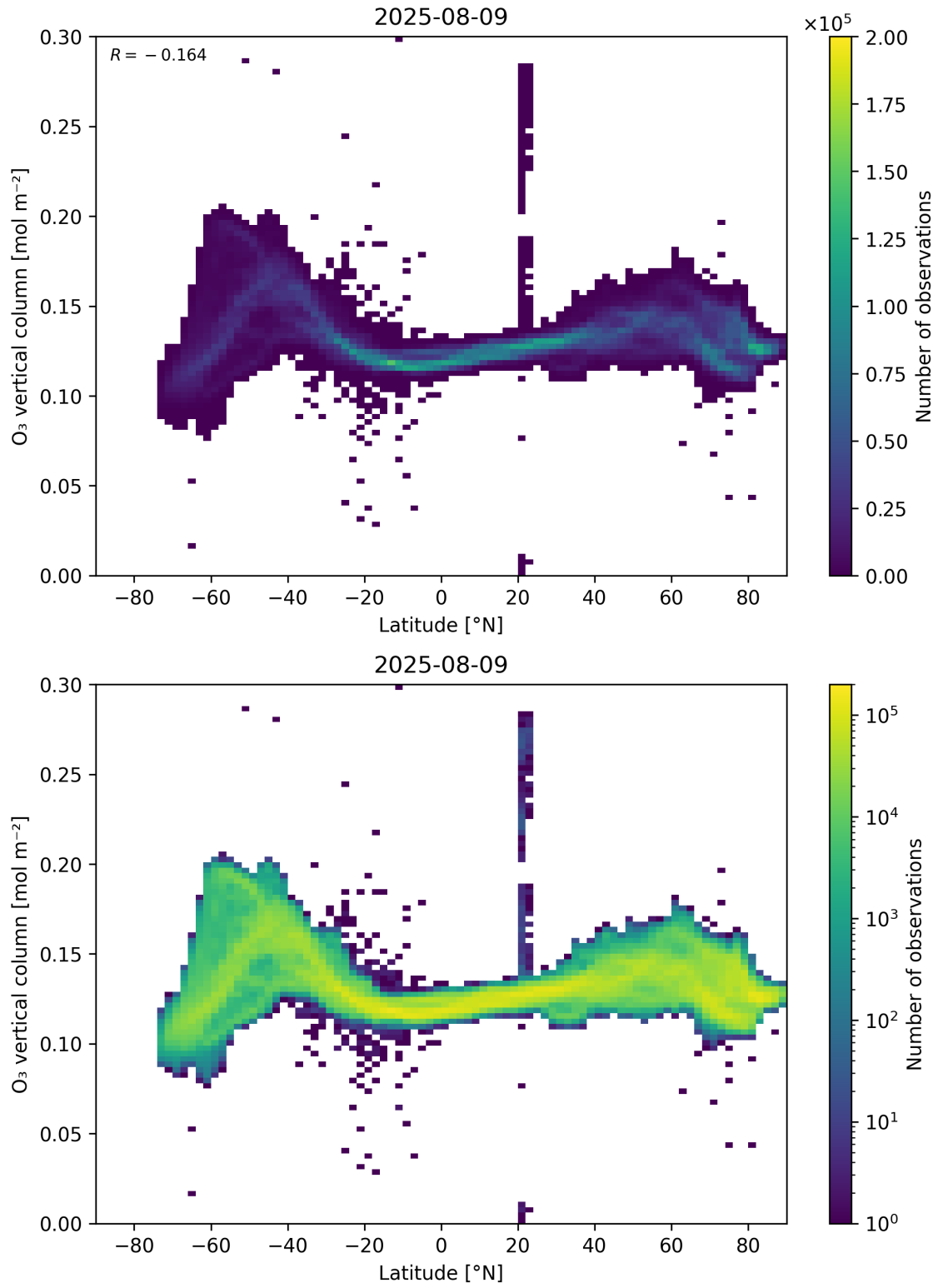
Figure 36: Scatter density plot of “Latitude” against “O 3 vertical column” for 2025-08-09 to 2025-08-10.
