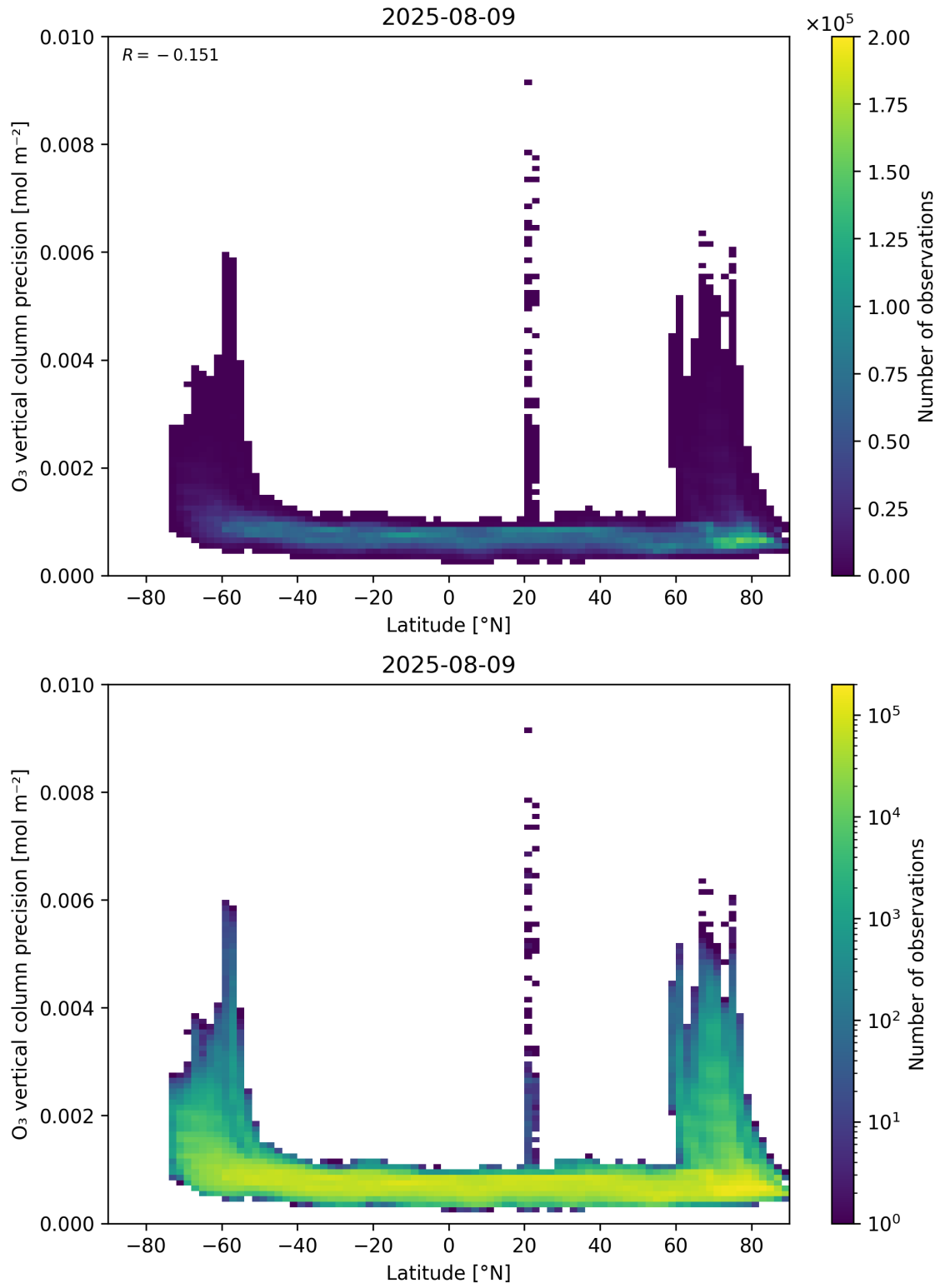
Figure 37: Scatter density plot of “Latitude” against “O 3 vertical column precision” for 2025-08-09 to 2025-08-10.
