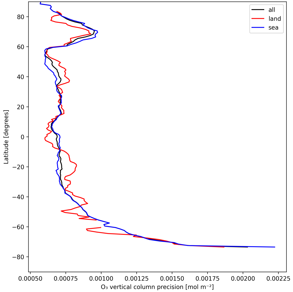
Figure 15: Zonal average of "O 3 vertical column precision" for 2025-08-09 to 2025-08-10.
