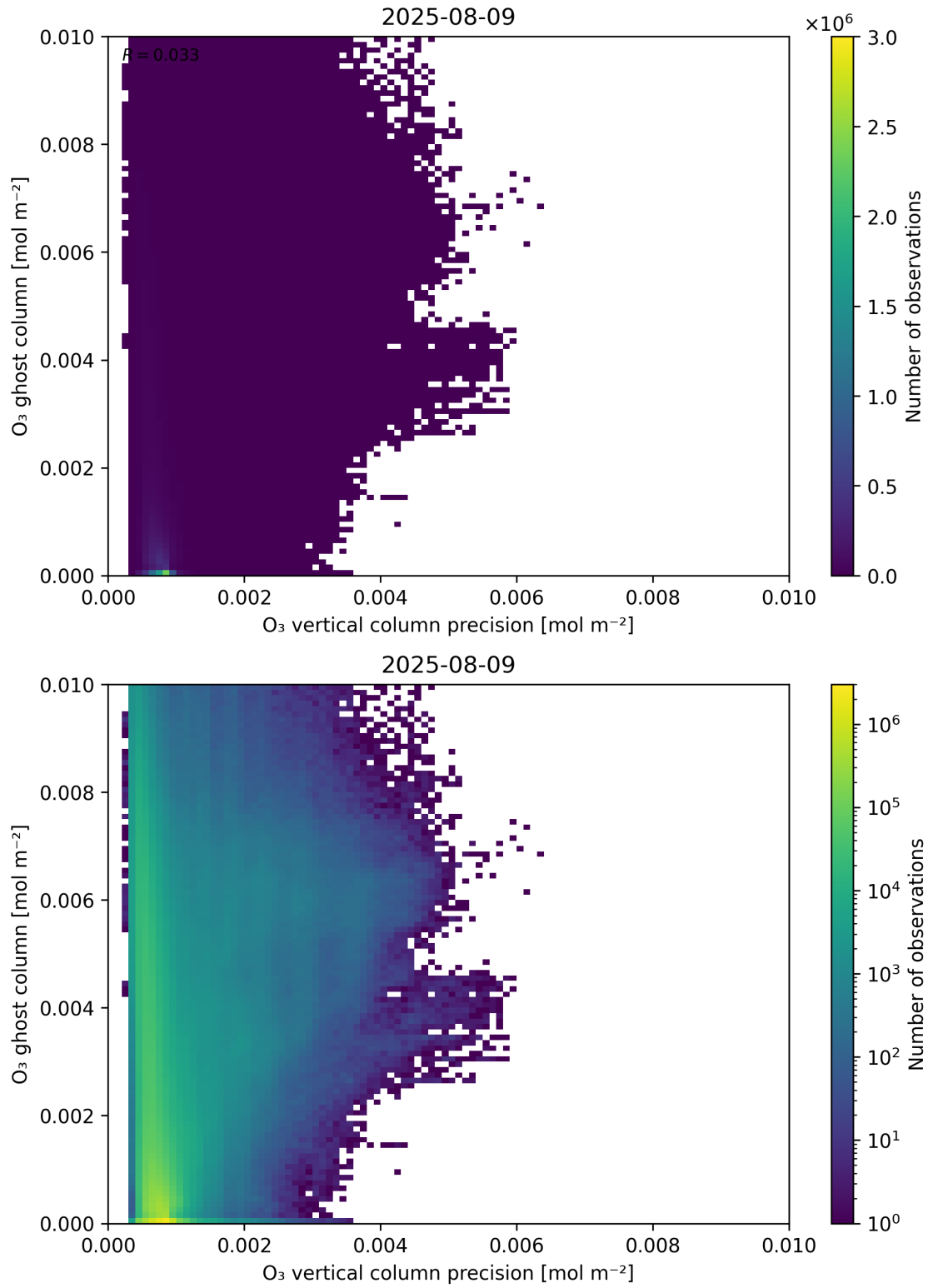
Figure 43: Scatter density plot of “O 3 vertical column precision” against “O 3 ghost column” for 2025-08-09 to 2025-08-10.
