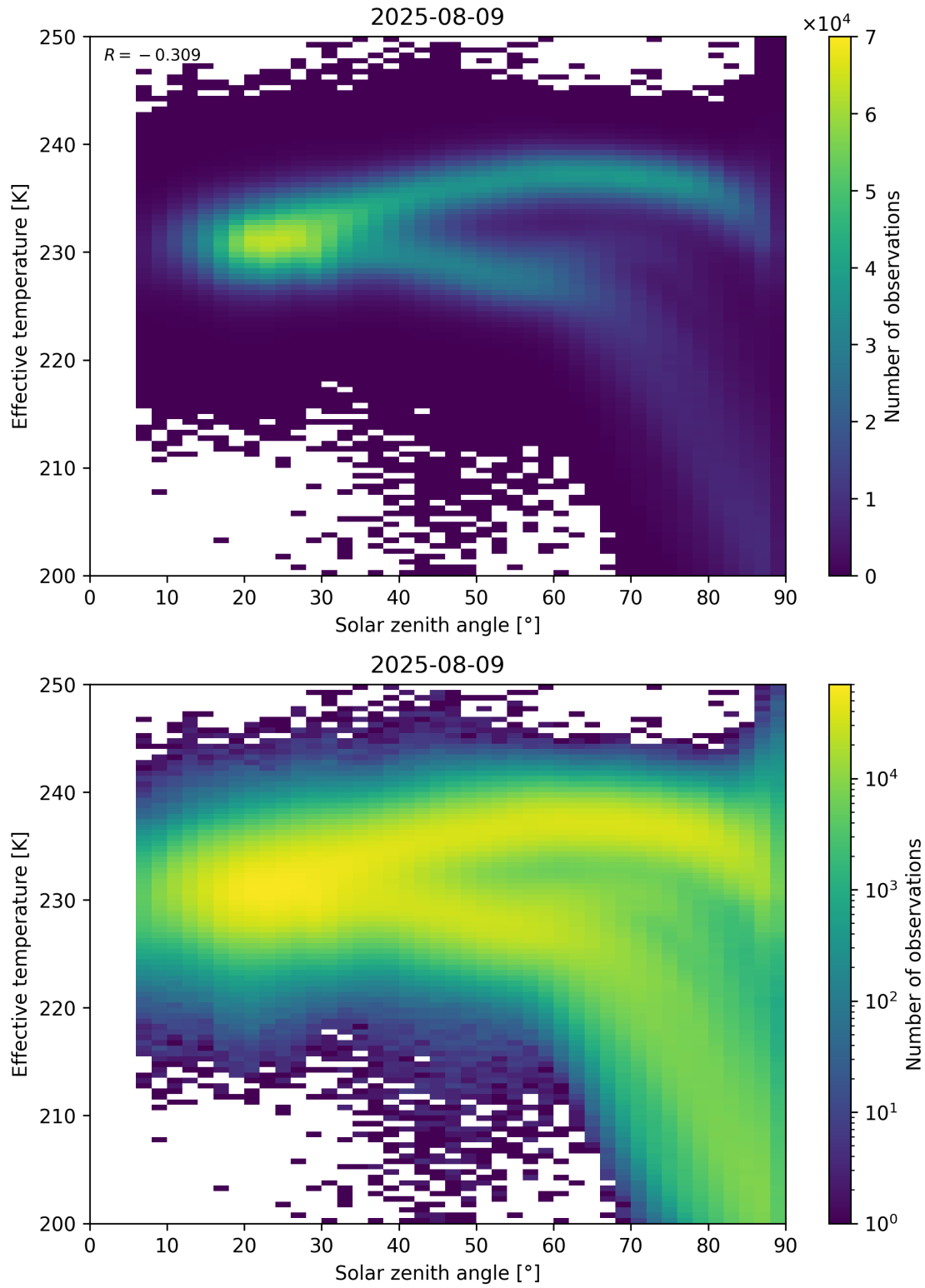
Figure 45: Scatter density plot of “Solar zenith angle” against “Effective temperature” for 2025-08-09 to 2025-08-10.
