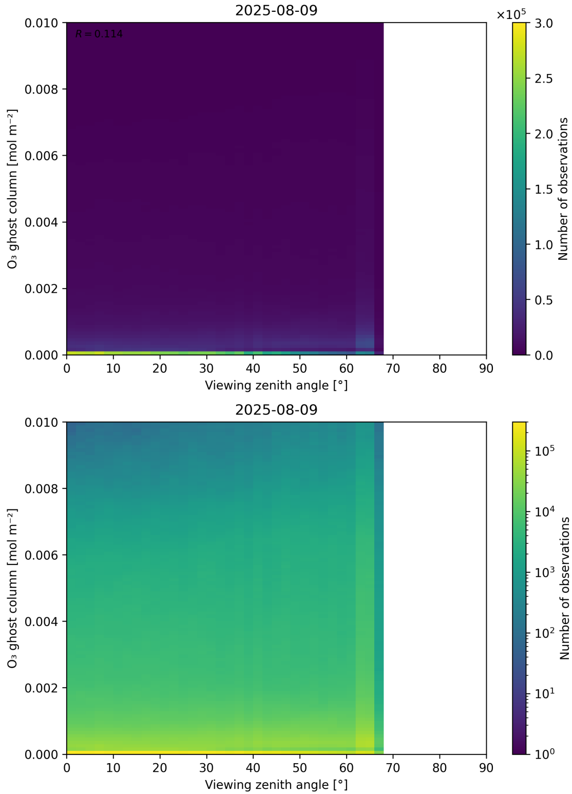
Figure 51: Scatter density plot of “Viewing zenith angle” against “O 3 ghost column” for 2025-08-09 to 2025-08-10.
