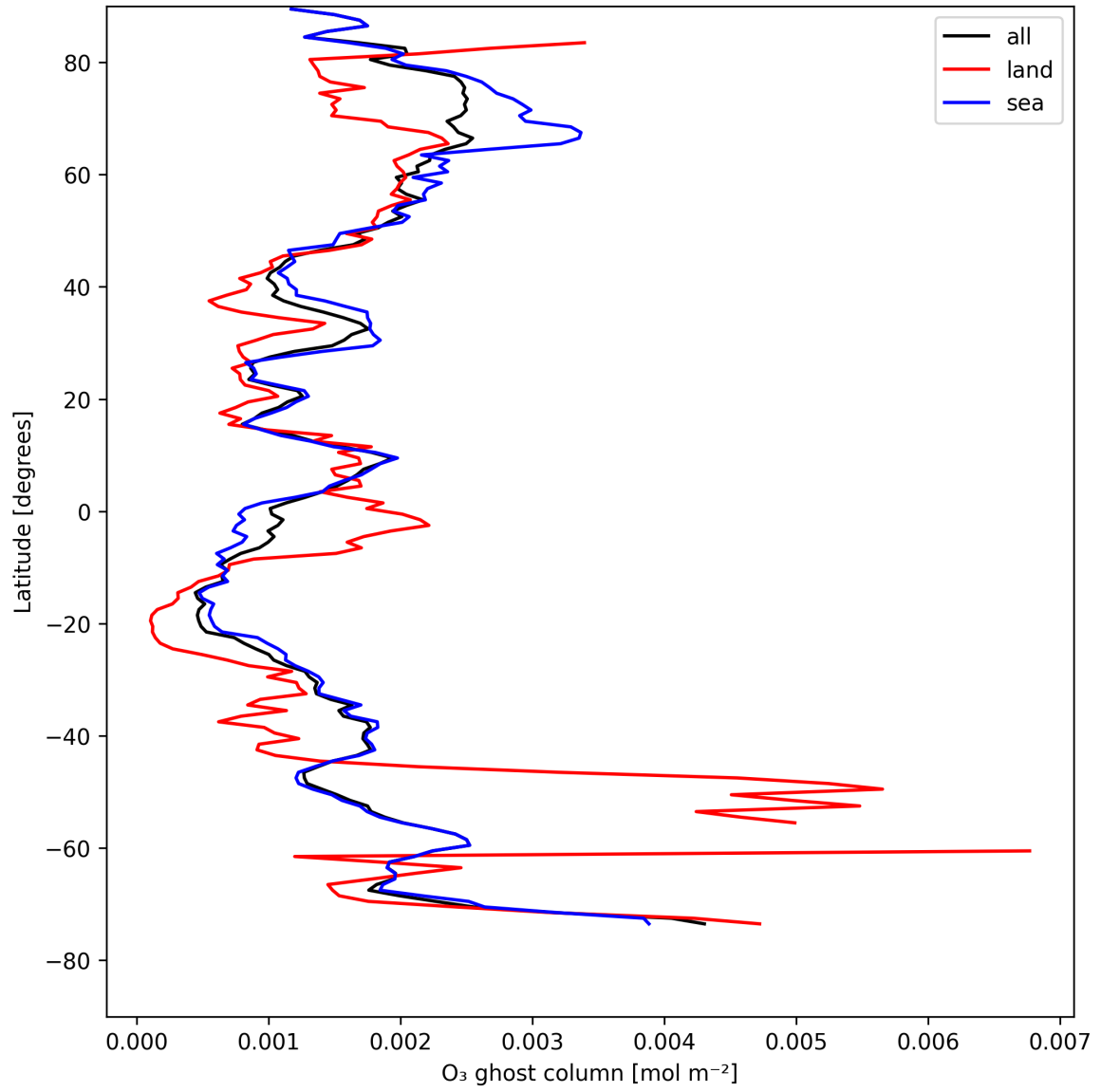
Figure 18: Zonal average of “O 3 ghost column” for 2025-08-09 to 2025-08-10.
