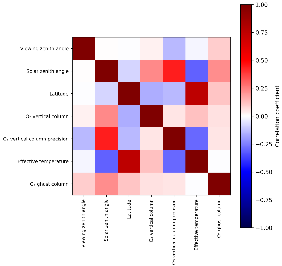
Figure 2: Map of correlation matrix for 2025-08-09 to 2025-08-11.
