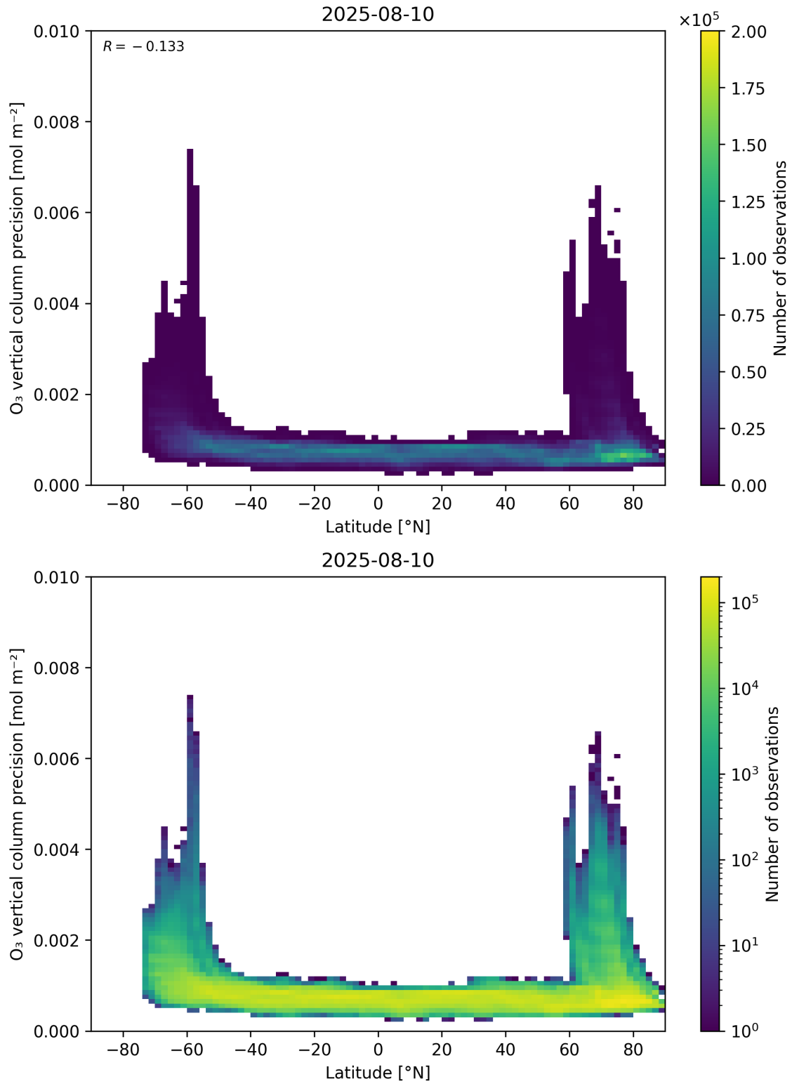
Figure 37: Scatter density plot of “Latitude” against “O 3 vertical column precision” for 2025-08-09 to 2025-08-11.
