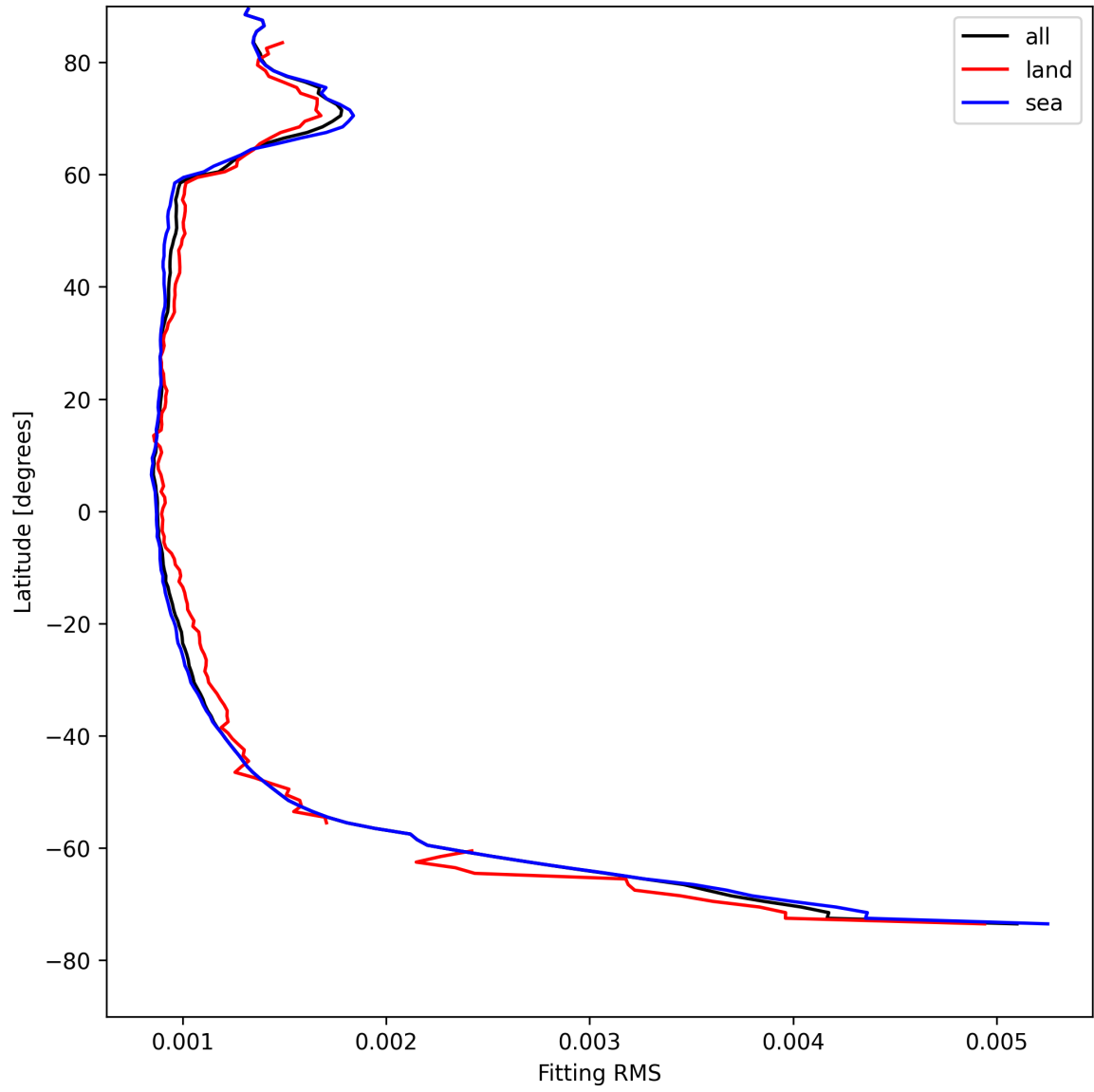
Figure 16: Zonal average of “Fitting RMS” for 2025-08-09 to 2025-08-11.
