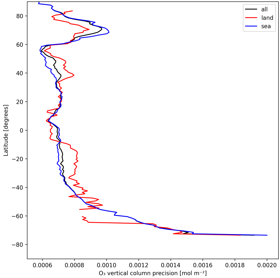
Figure 15: Zonal average of "O 3 vertical column precision" for 2025-08-09 to 2025-08-11.
