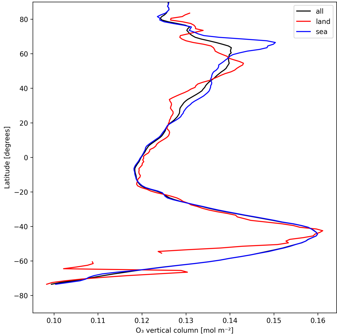
Figure 14: Zonal average of “O 3 vertical column” for 2025-08-09 to 2025-08-11.
