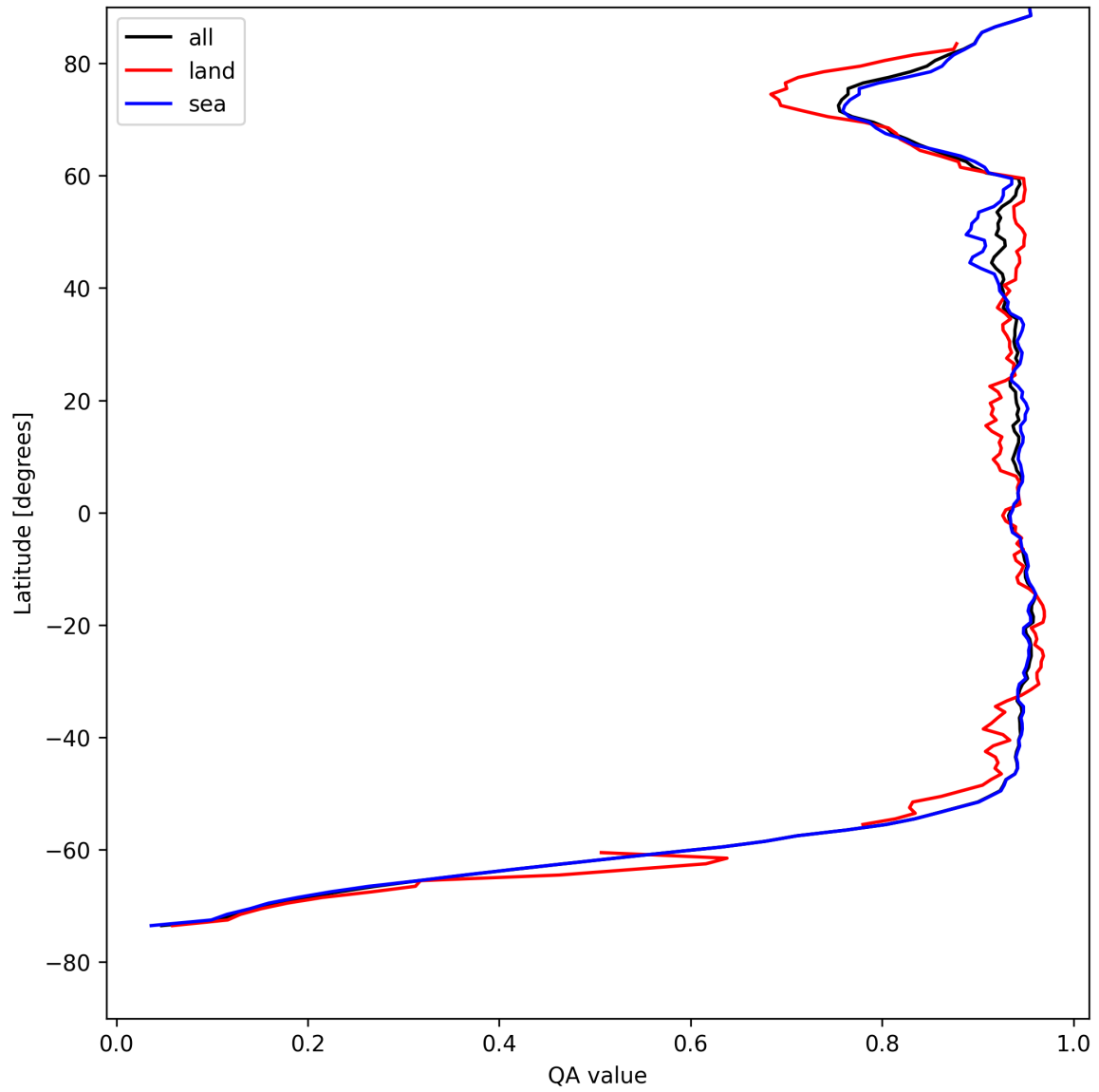
Figure 13: Zonal average of “QA value” for 2025-08-09 to 2025-08-11.
