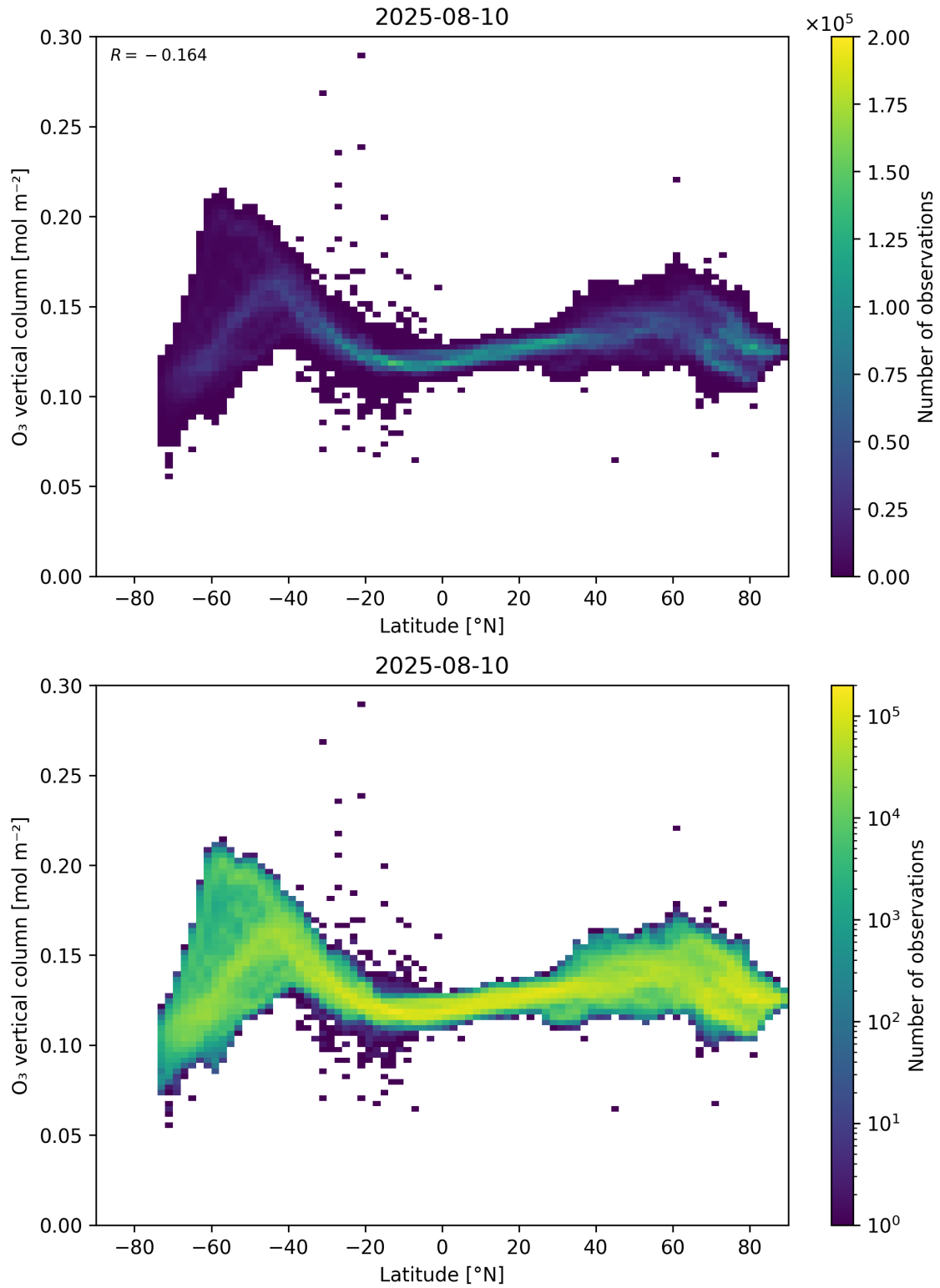
Figure 36: Scatter density plot of “Latitude” against “O 3 vertical column” for 2025-08-09 to 2025-08-11.
