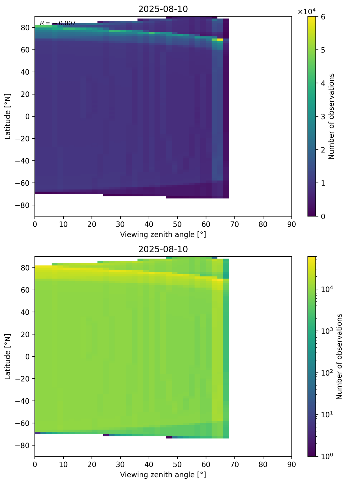
Figure 49: Scatter density plot of “Viewing zenith angle” against “Latitude” for 2025-08-09 to 2025-08-11.
