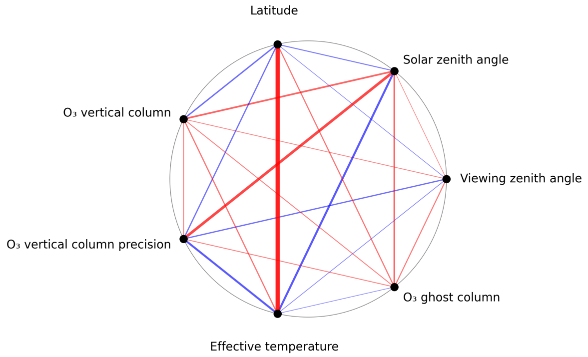
Figure 1: Map of correlation graph for 2025-08-09 to 2025-08-11.
