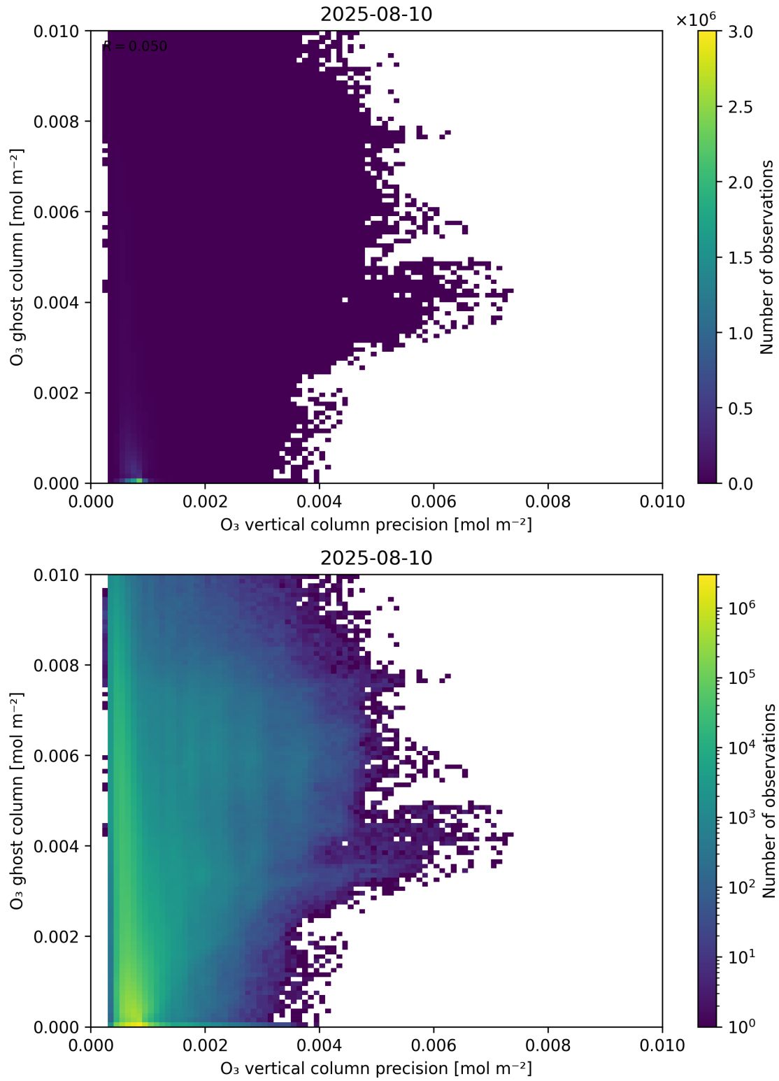
Figure 43: Scatter density plot of “O 3 vertical column precision” against “O 3 ghost column” for 2025-08-09 to 2025-08-11.
