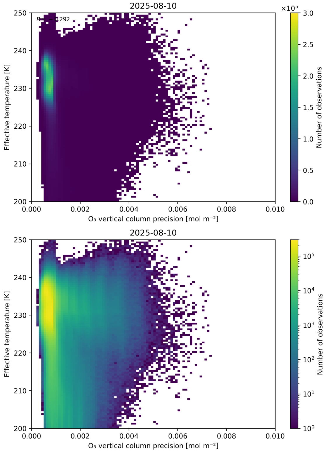
Figure 42: Scatter density plot of “O 3 vertical column precision” against “Effective temperature” for 2025-08-09 to 2025-08-11.
