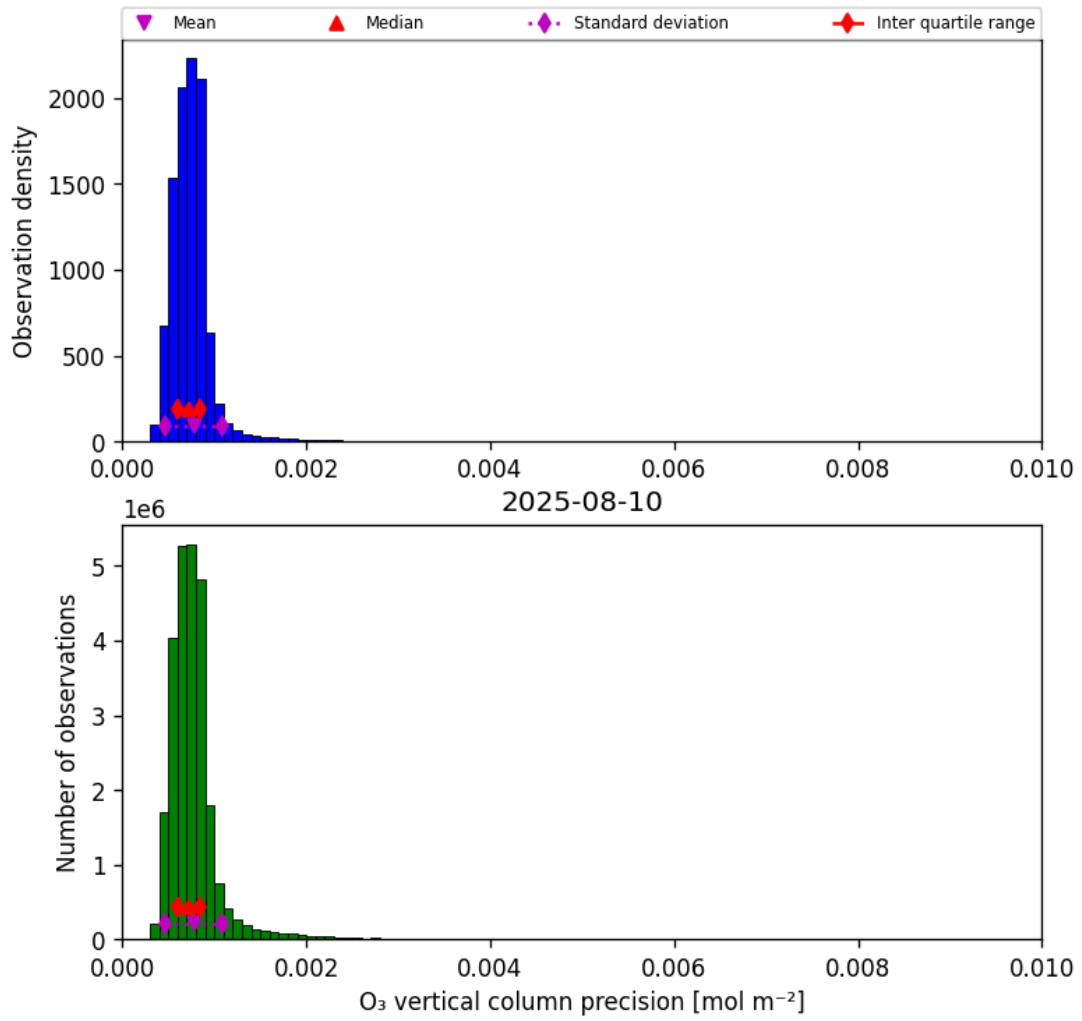
Figure 22: Histogram of “O 3 vertical column precision” for 2025-08-09 to 2025-08-11
