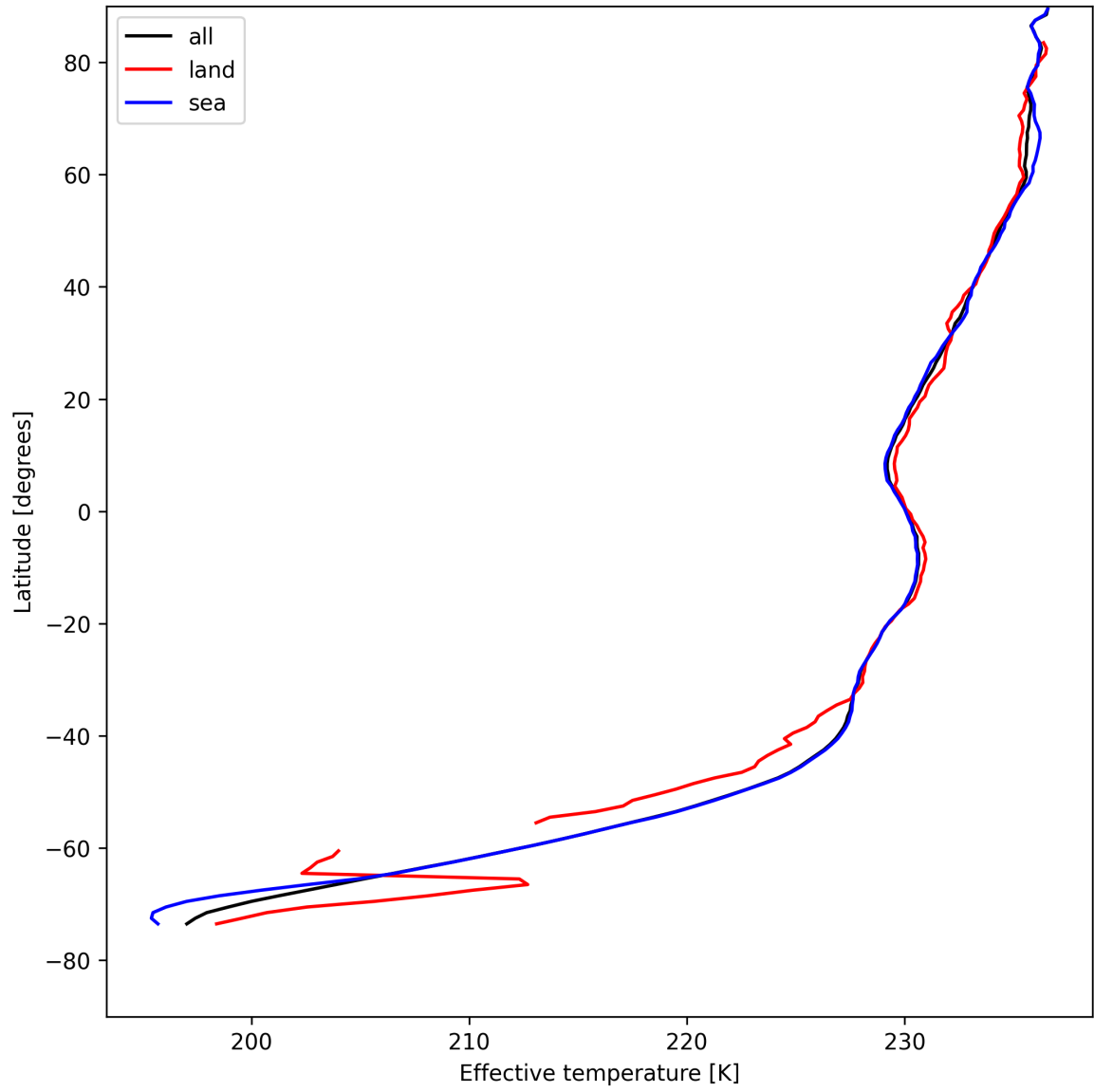
Figure 17: Zonal average of "Effective temperature" for 2025-08-09 to 2025-08-11.
