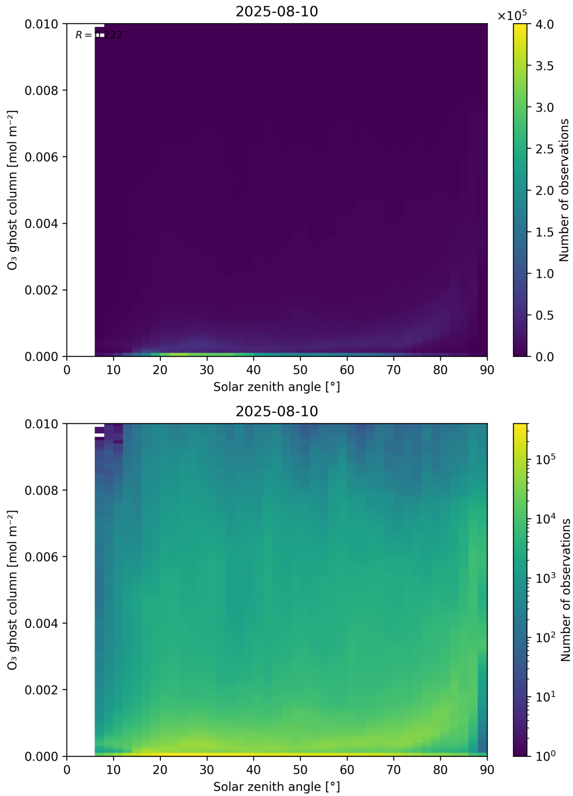
Figure 46: Scatter density plot of “Solar zenith angle” against “O 3 ghost column” for 2025-08-09 to 2025-08-11.
