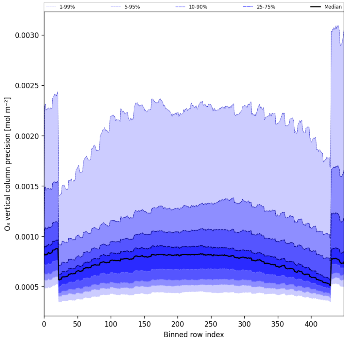
Figure 29: Along track statistics of “O 3 vertical column precision” for 2025-08-09 to 2025-08-11
