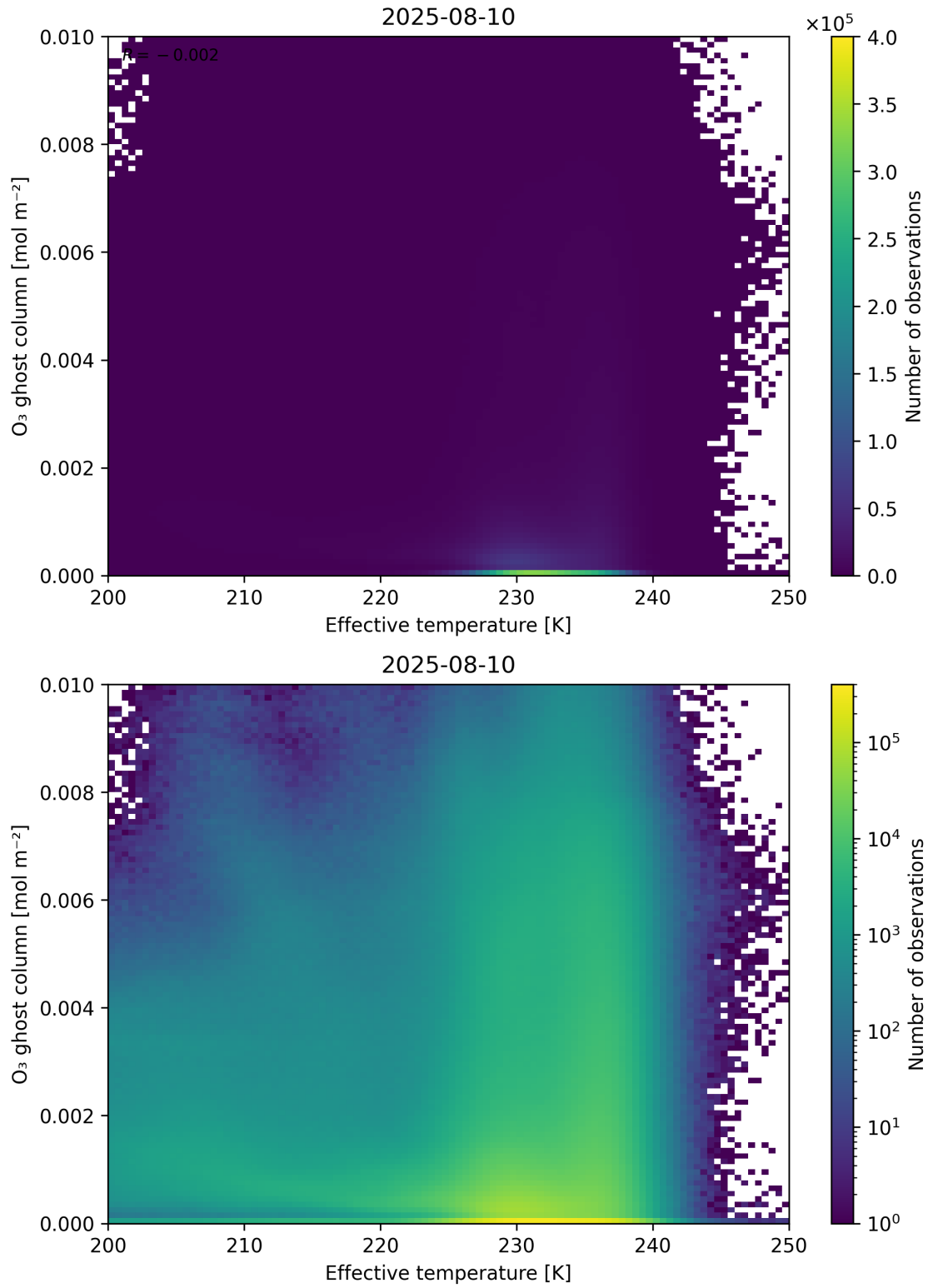
Figure 38: Scatter density plot of “Effective temperature” against “O 3 ghost column” for 2025-08-09 to 2025-08-11.
