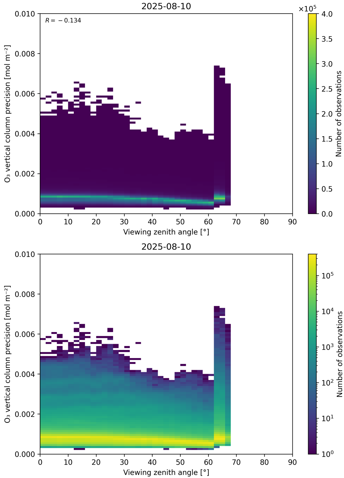
Figure 53: Scatter density plot of “Viewing zenith angle” against “O 3 vertical column precision” for 2025-08-09 to 2025-08-11.
