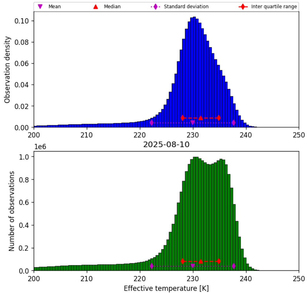
Figure 24: Histogram of “Effective temperature” for 2025-08-09 to 2025-08-11
