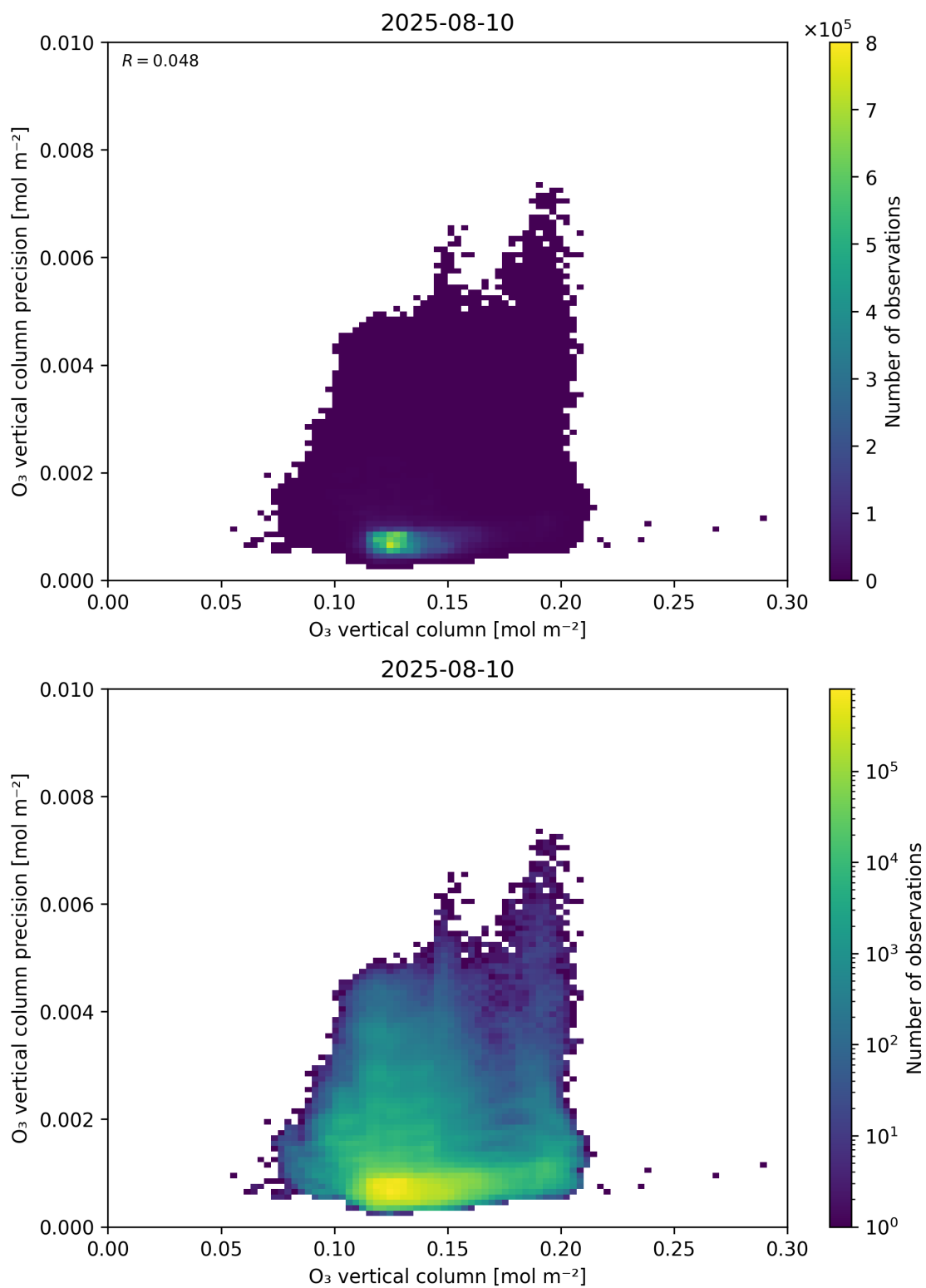
Figure 41: Scatter density plot of “O 3 vertical column” against “O 3 vertical column precision” for 2025-08-09 to 2025-08-11.
