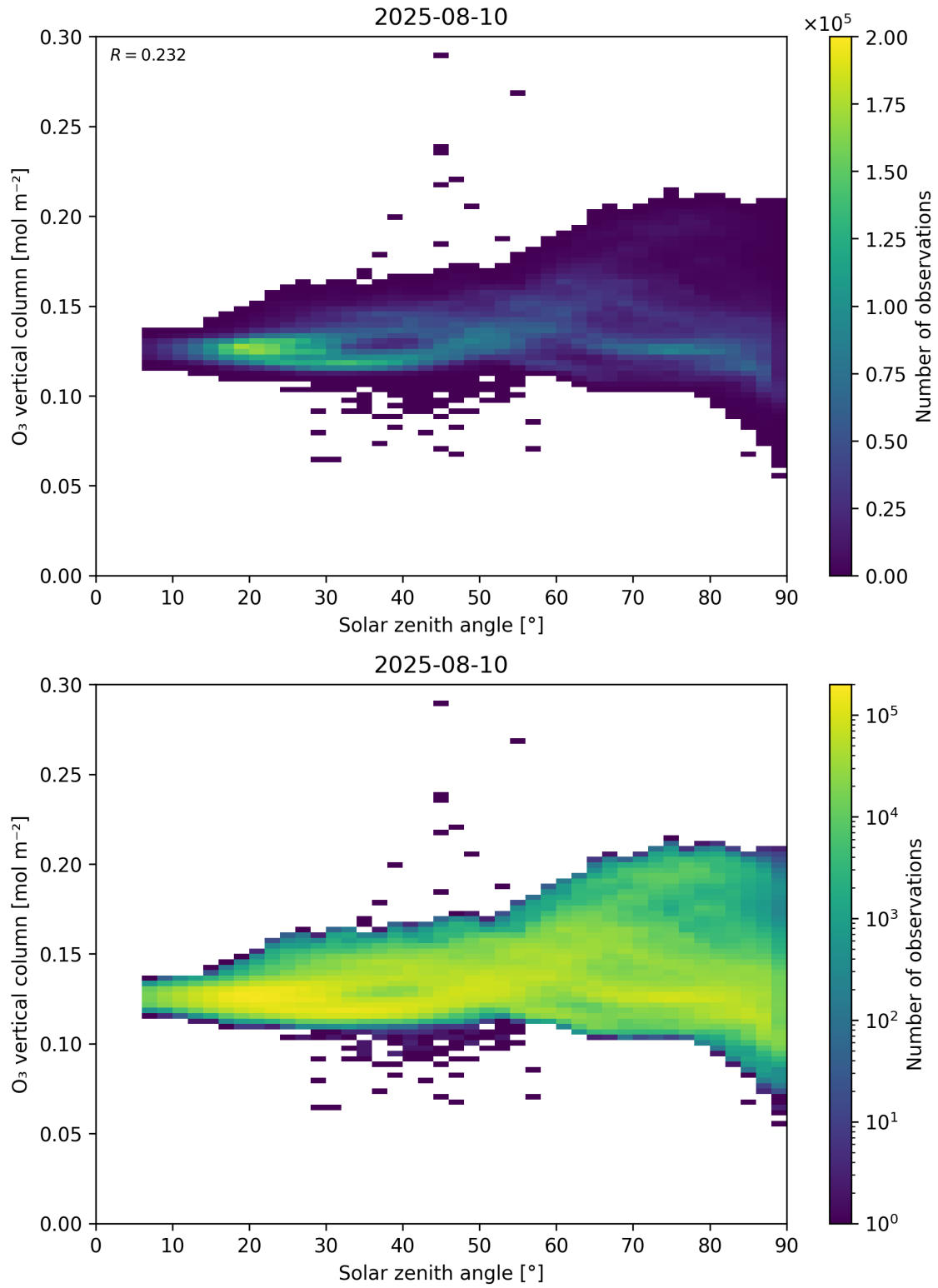
Figure 47: Scatter density plot of “Solar zenith angle” against “O 3 vertical column” for 2025-08-09 to 2025-08-11.
