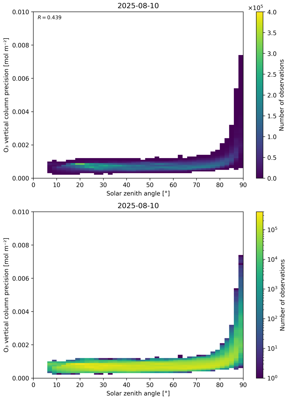
Figure 48: Scatter density plot of “Solar zenith angle” against “O 3 vertical column precision” for 2025-08-09 to 2025-08-11.
