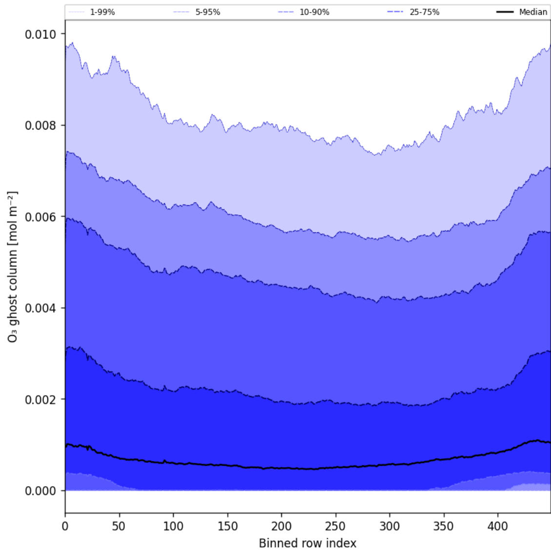
Figure 32: Along track statistics of “O 3 ghost column” for 2025-08-09 to 2025-08-11
