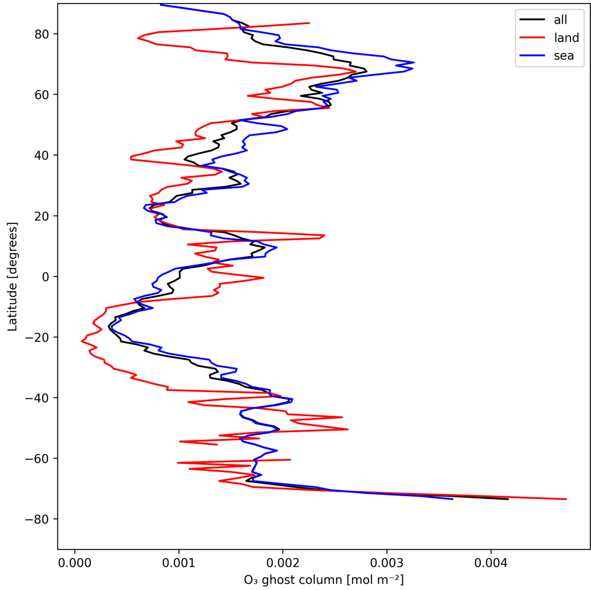
Figure 18: Zonal average of “O 3 ghost column” for 2025-08-09 to 2025-08-11.
