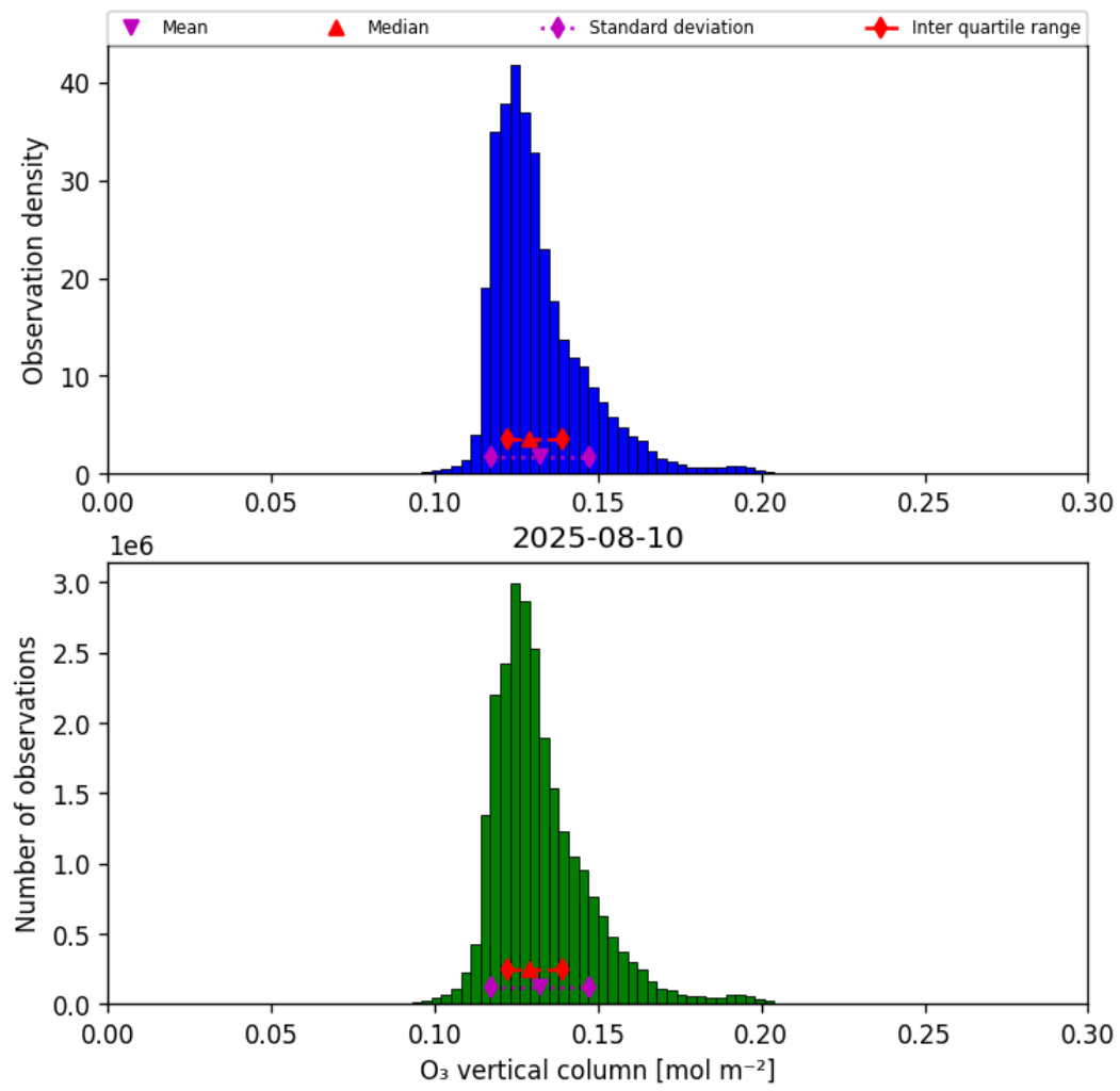
Figure 21: Histogram of “O 3 vertical column” for 2025-08-09 to 2025-08-11
