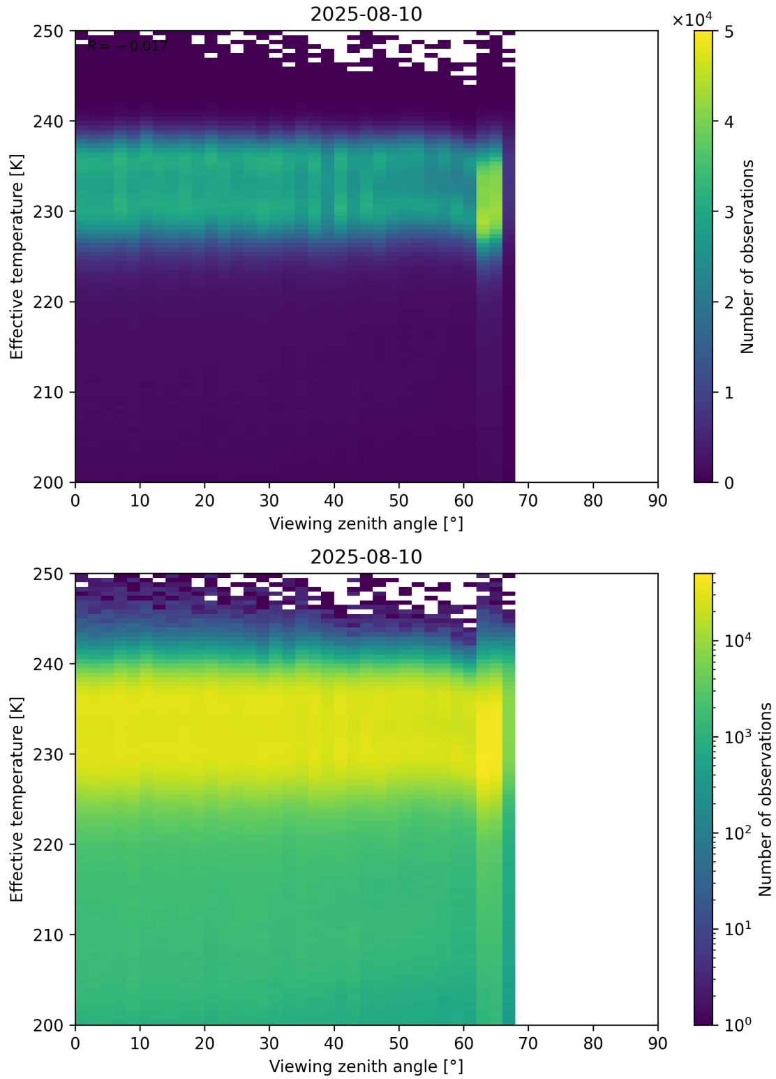
Figure 50: Scatter density plot of “Viewing zenith angle” against “Effective temperature” for 2025-08-09 to 2025-08-11.
