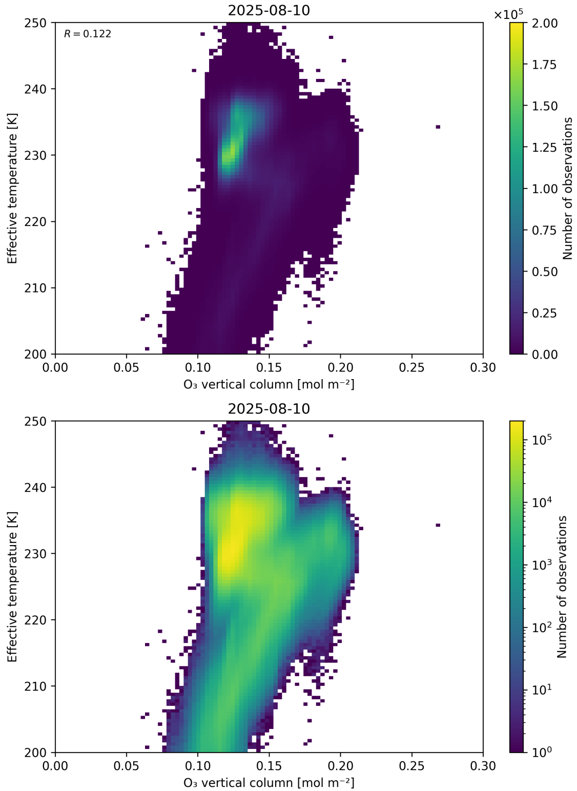
Figure 39: Scatter density plot of “O 3 vertical column” against “Effective temperature” for 2025-08-09 to 2025-08-11.
