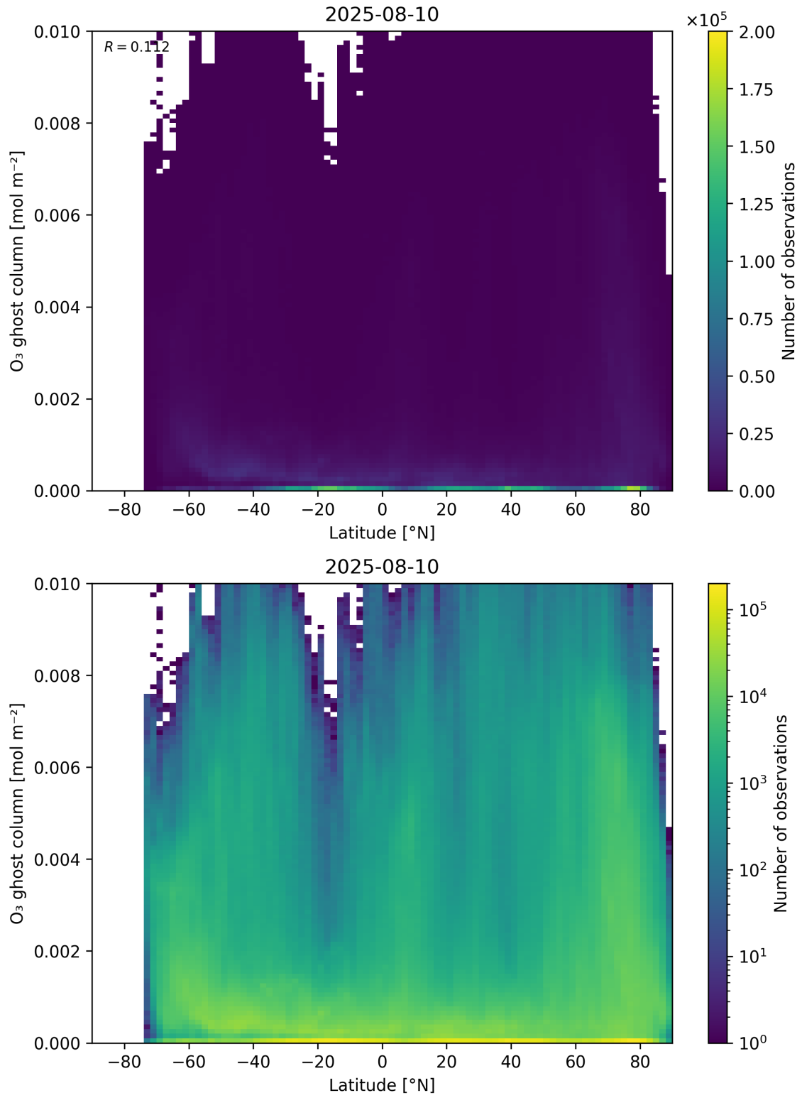
Figure 35: Scatter density plot of “Latitude” against “O 3 ghost column” for 2025-08-09 to 2025-08-11.
