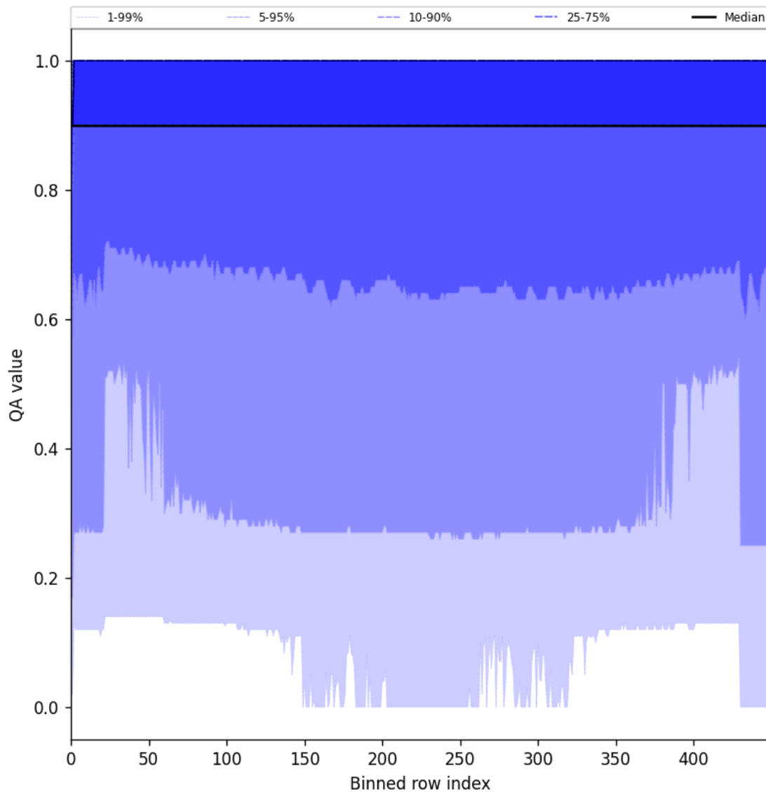
Figure 27: Along track statistics of “QA value” for 2025-08-09 to 2025-08-11
