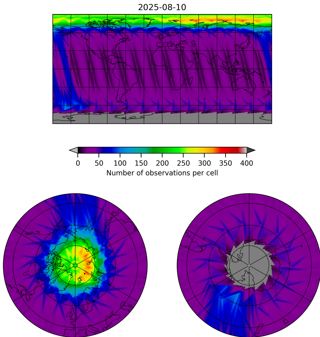
Figure 12: Map of the number of observations for 2025-08-09 to 2025-08-11
