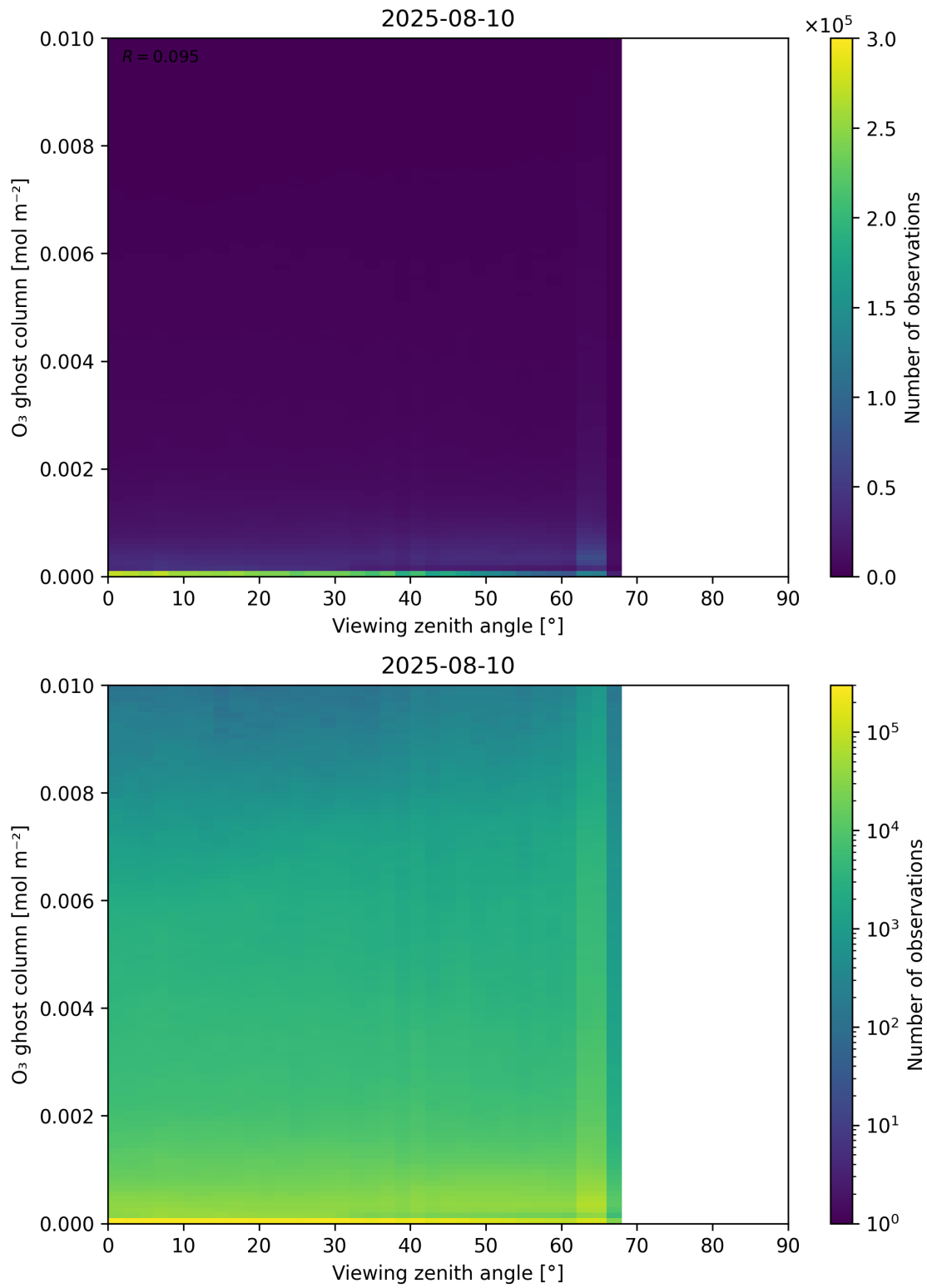
Figure 51: Scatter density plot of “Viewing zenith angle” against “O 3 ghost column” for 2025-08-09 to 2025-08-11.
