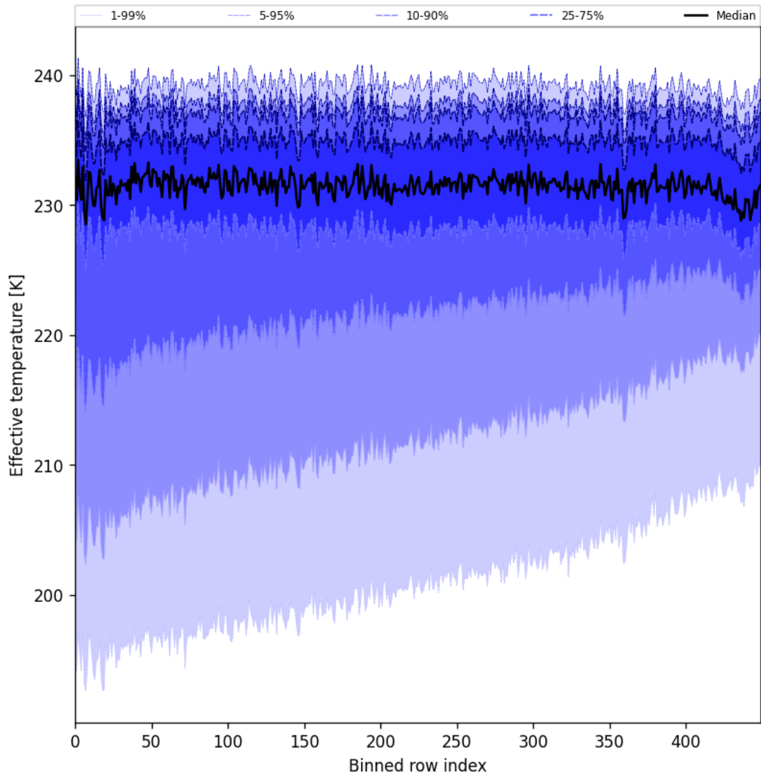
Figure 31: Along track statistics of “Effective temperature” for 2025-08-09 to 2025-08-11
