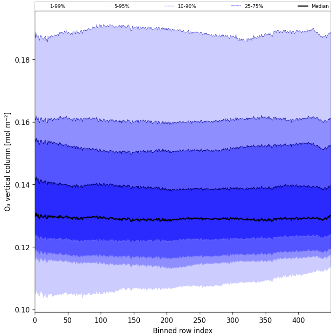
Figure 28: Along track statistics of “O 3 vertical column” for 2025-08-09 to 2025-08-11
