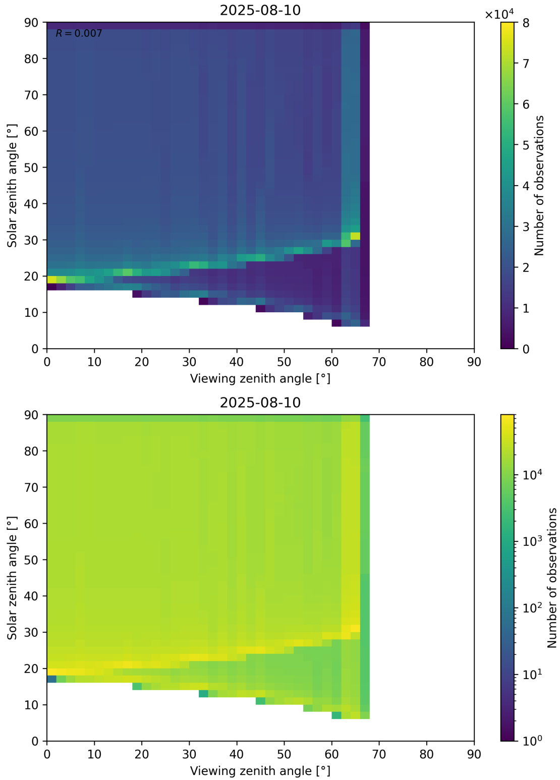
Figure 54: Scatter density plot of “Viewing zenith angle” against “Solar zenith angle” for 2025-08-09 to 2025-08-11.
