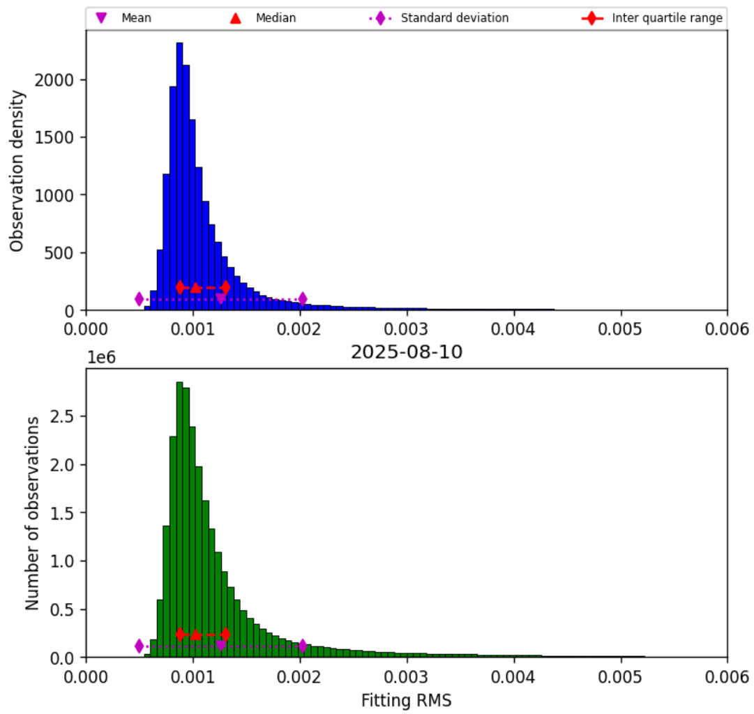
Figure 23: Histogram of “Fitting RMS” for 2025-08-09 to 2025-08-11
