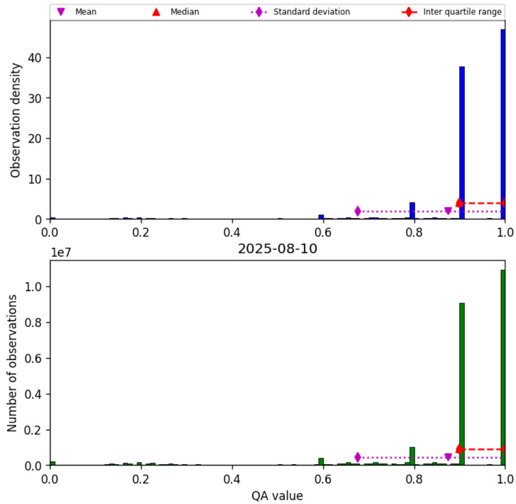
Figure 20: Histogram of “QA value” for 2025-08-09 to 2025-08-11
