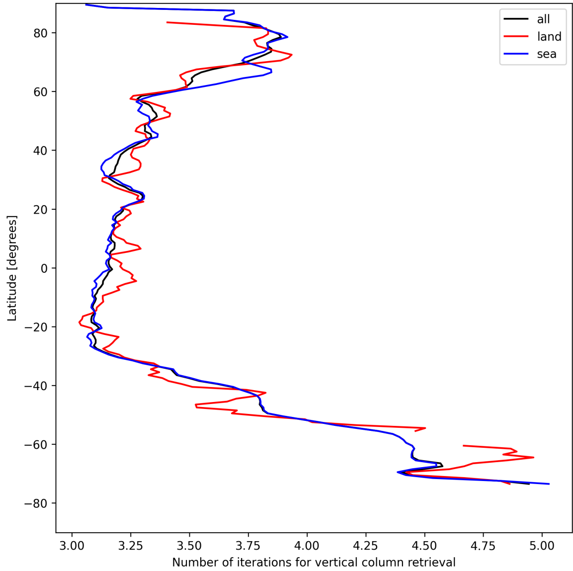
Figure 19: Zonal average of “Number of iterations for vertical column retrieval” for 2025-08-09 to 2025-08-11.
