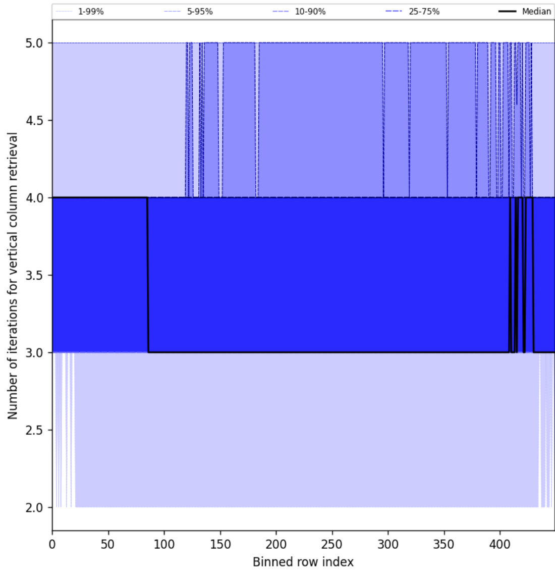
Figure 33: Along track statistics of “Number of iterations for vertical column retrieval” for 2025-08-09 to 2025-08-11
