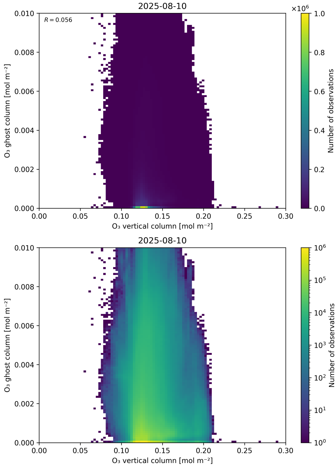
Figure 40: Scatter density plot of “O 3 vertical column” against “O 3 ghost column” for 2025-08-09 to 2025-08-11.
