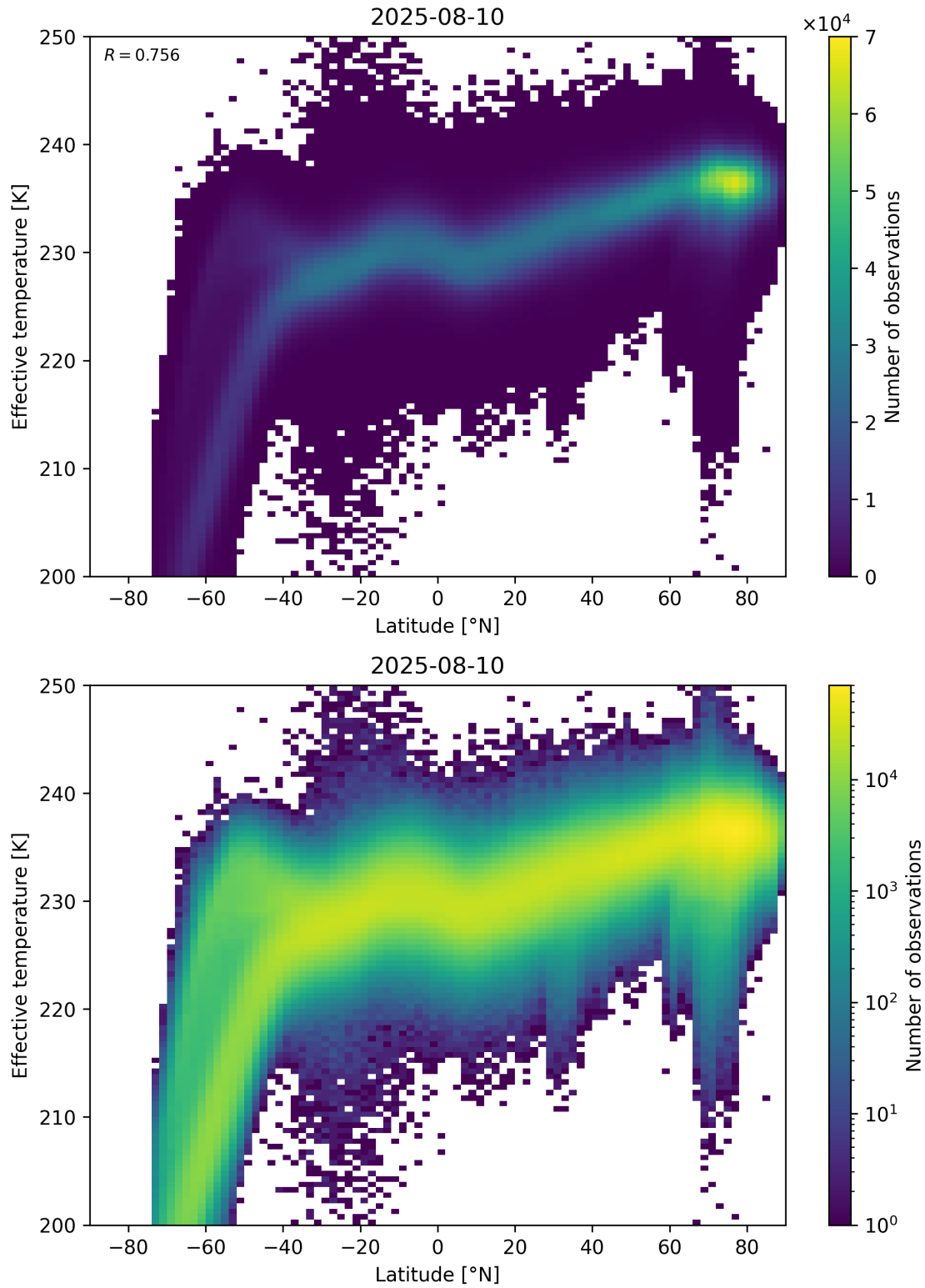
Figure 34: Scatter density plot of “Latitude” against “Effective temperature” for 2025-08-09 to 2025-08-11.
