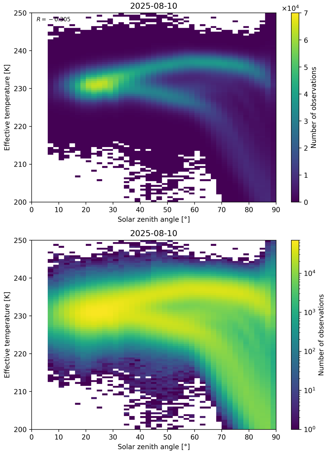
Figure 45: Scatter density plot of “Solar zenith angle” against “Effective temperature” for 2025-08-09 to 2025-08-11.
