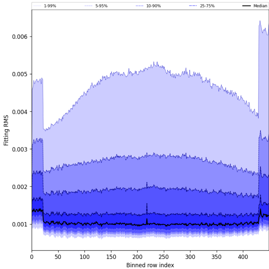
Figure 30: Along track statistics of “Fitting RMS” for 2025-08-09 to 2025-08-11
