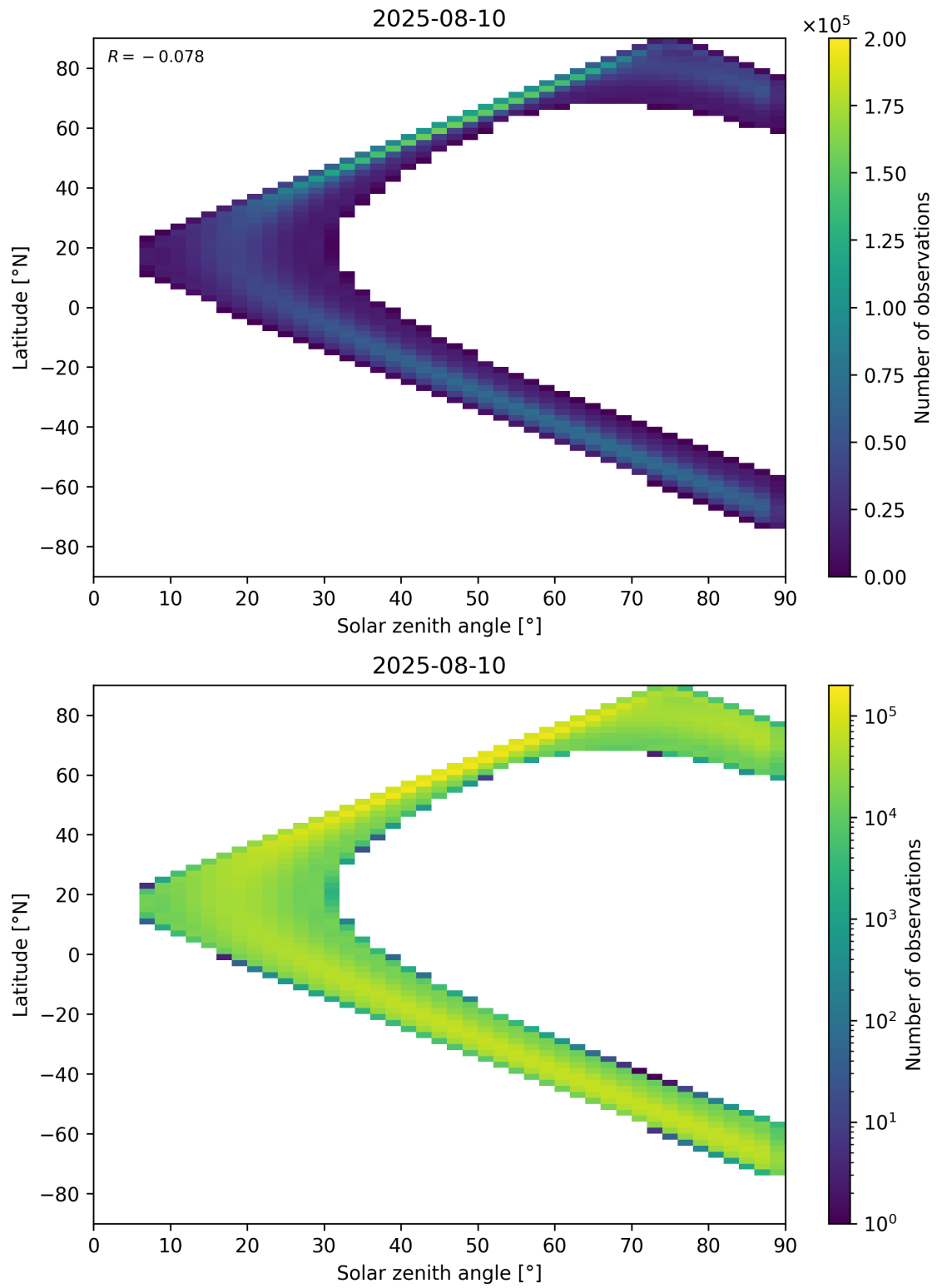
Figure 44: Scatter density plot of “Solar zenith angle” against “Latitude” for 2025-08-09 to 2025-08-11.
