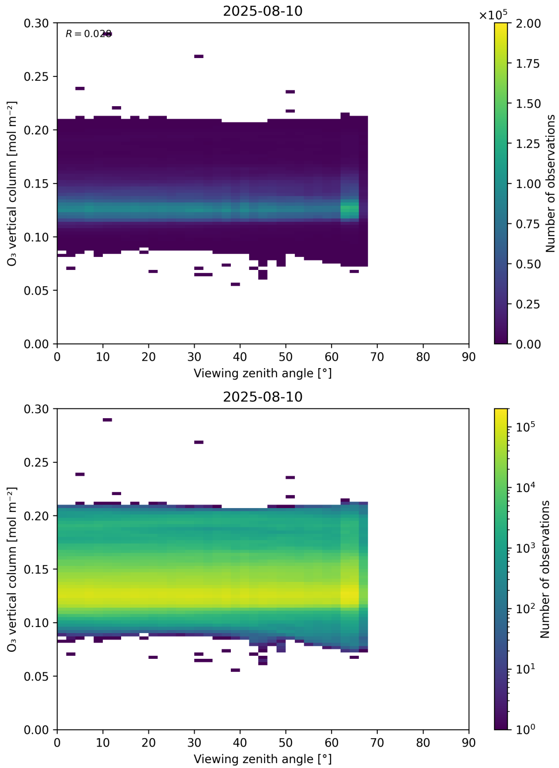
Figure 52: Scatter density plot of “Viewing zenith angle” against “O 3 vertical column” for 2025-08-09 to 2025-08-11.
