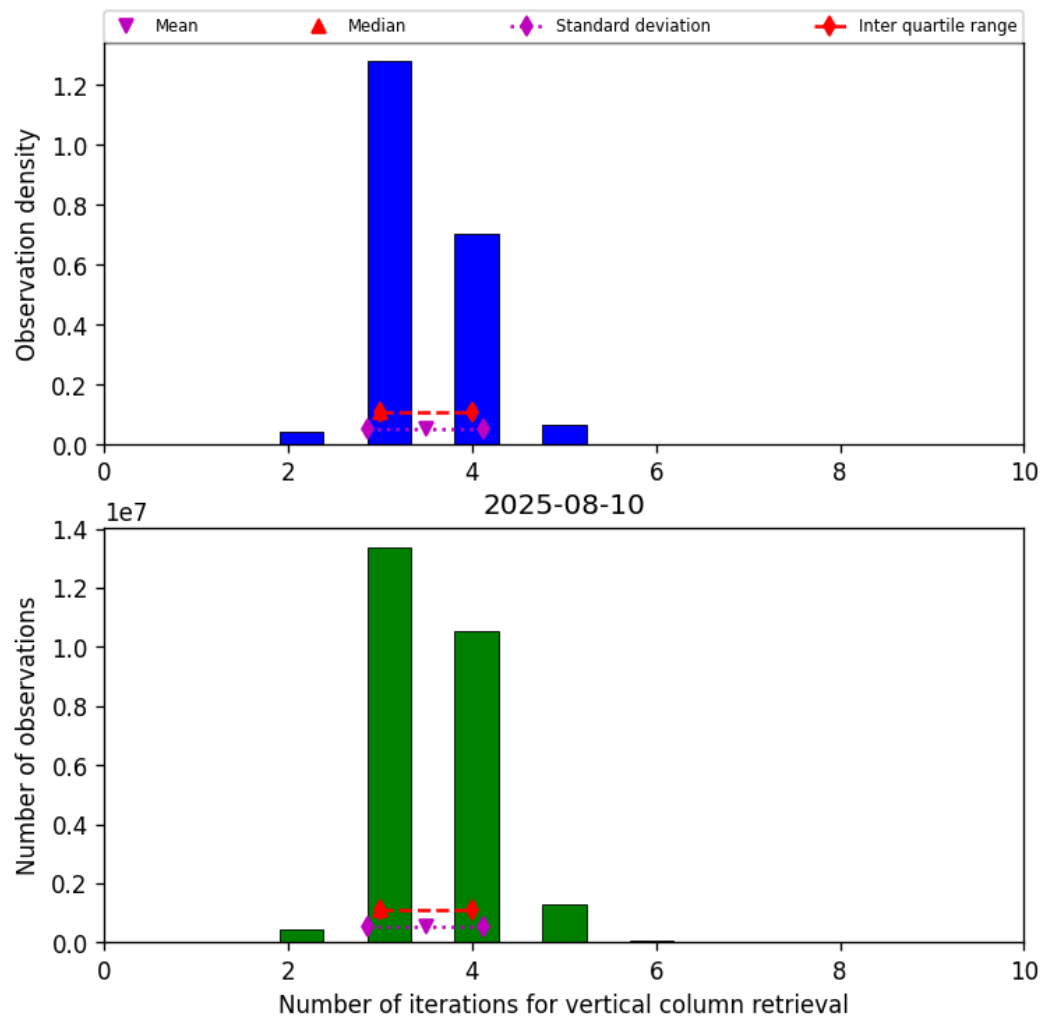
Figure 26: Histogram of “Number of iterations for vertical column retrieval” for 2025-08-09 to 2025-08-11
