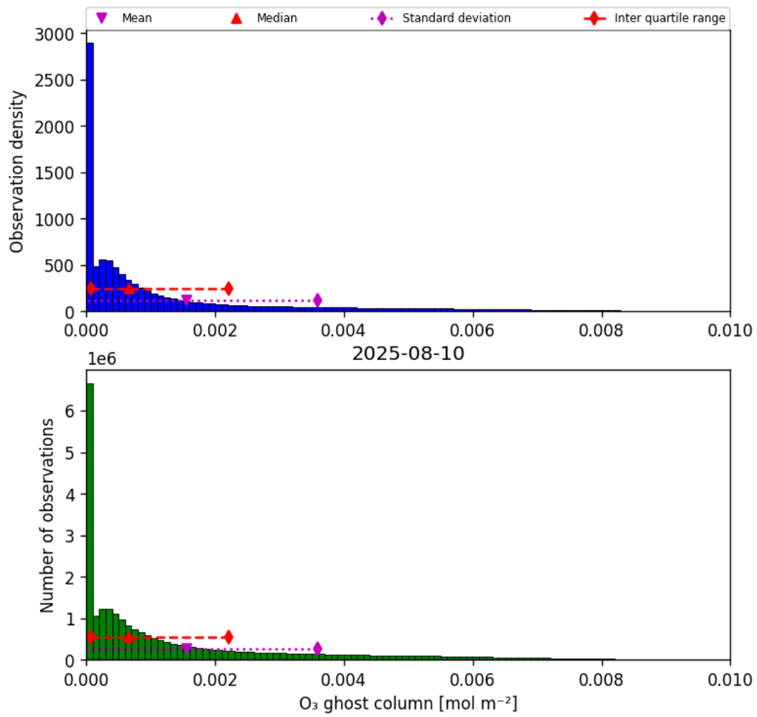
Figure 25: Histogram of “O 3 ghost column” for 2025-08-09 to 2025-08-11
