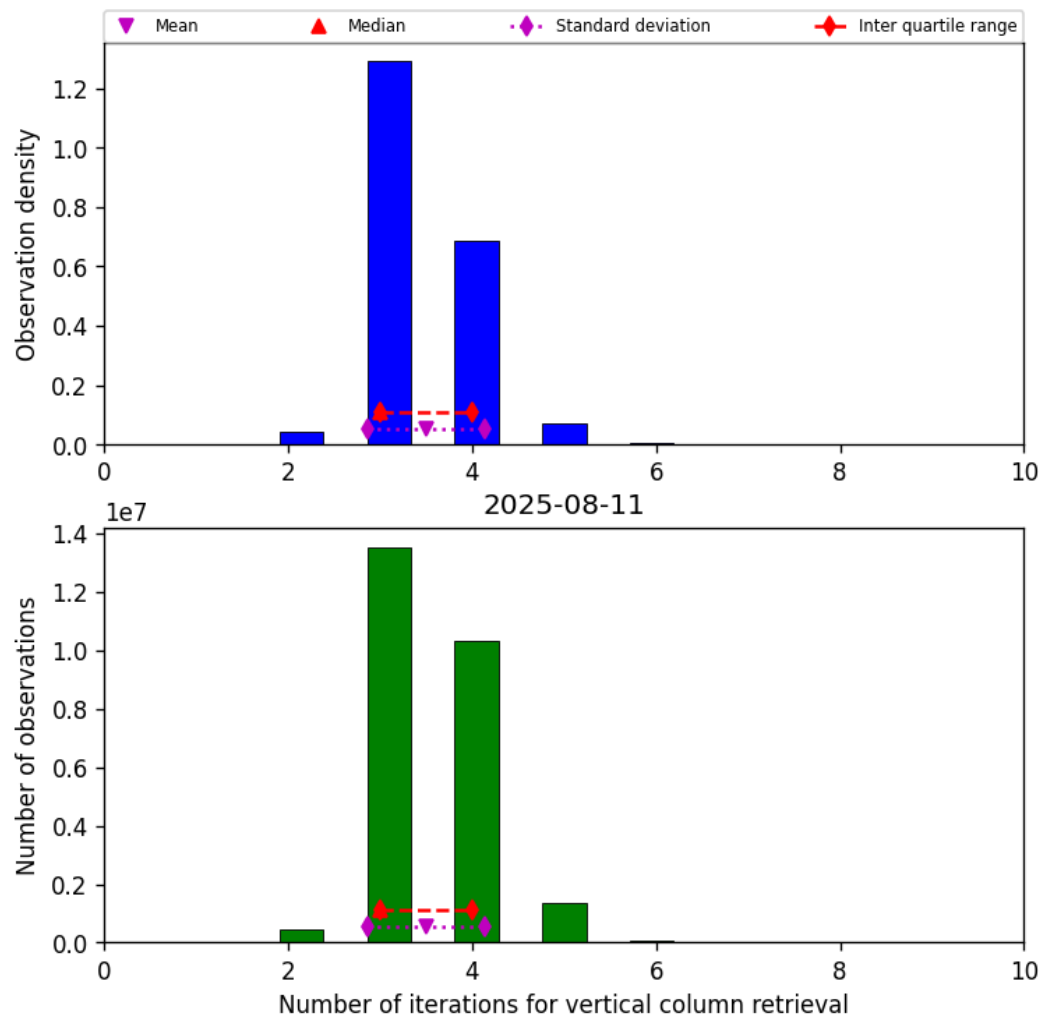
Figure 26: Histogram of “Number of iterations for vertical column retrieval” for 2025-08-10 to 2025-08-12
