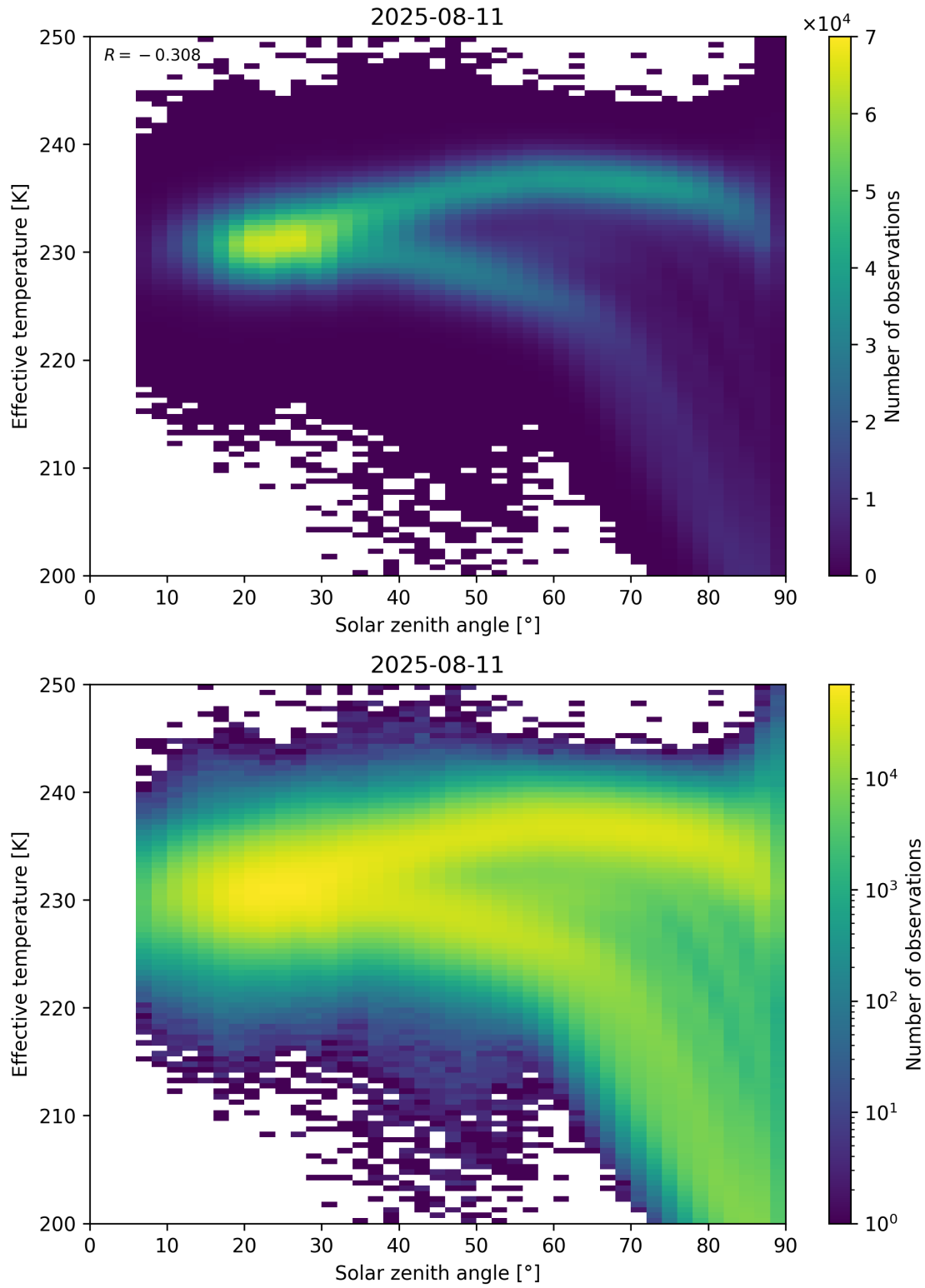
Figure 45: Scatter density plot of “Solar zenith angle” against “Effective temperature” for 2025-08-10 to 2025-08-12.
