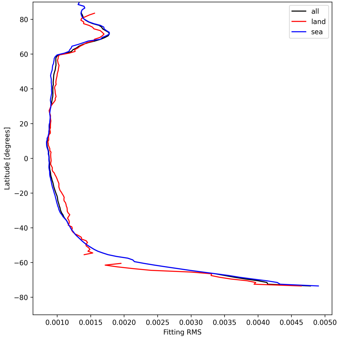
Figure 16: Zonal average of “Fitting RMS” for 2025-08-10 to 2025-08-12.
