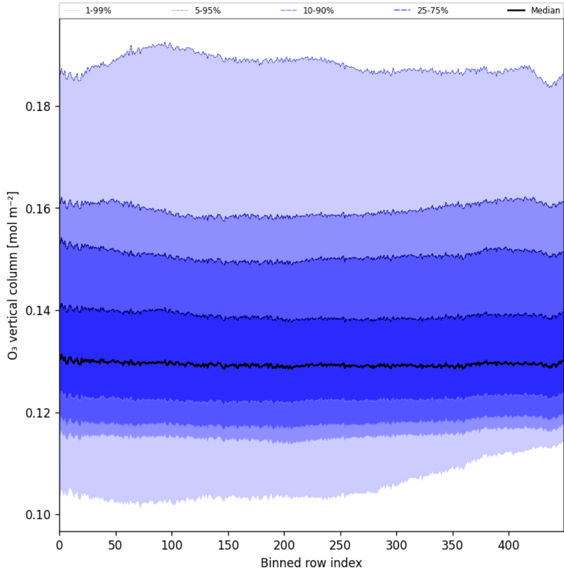
Figure 28: Along track statistics of “O 3 vertical column” for 2025-08-10 to 2025-08-12
