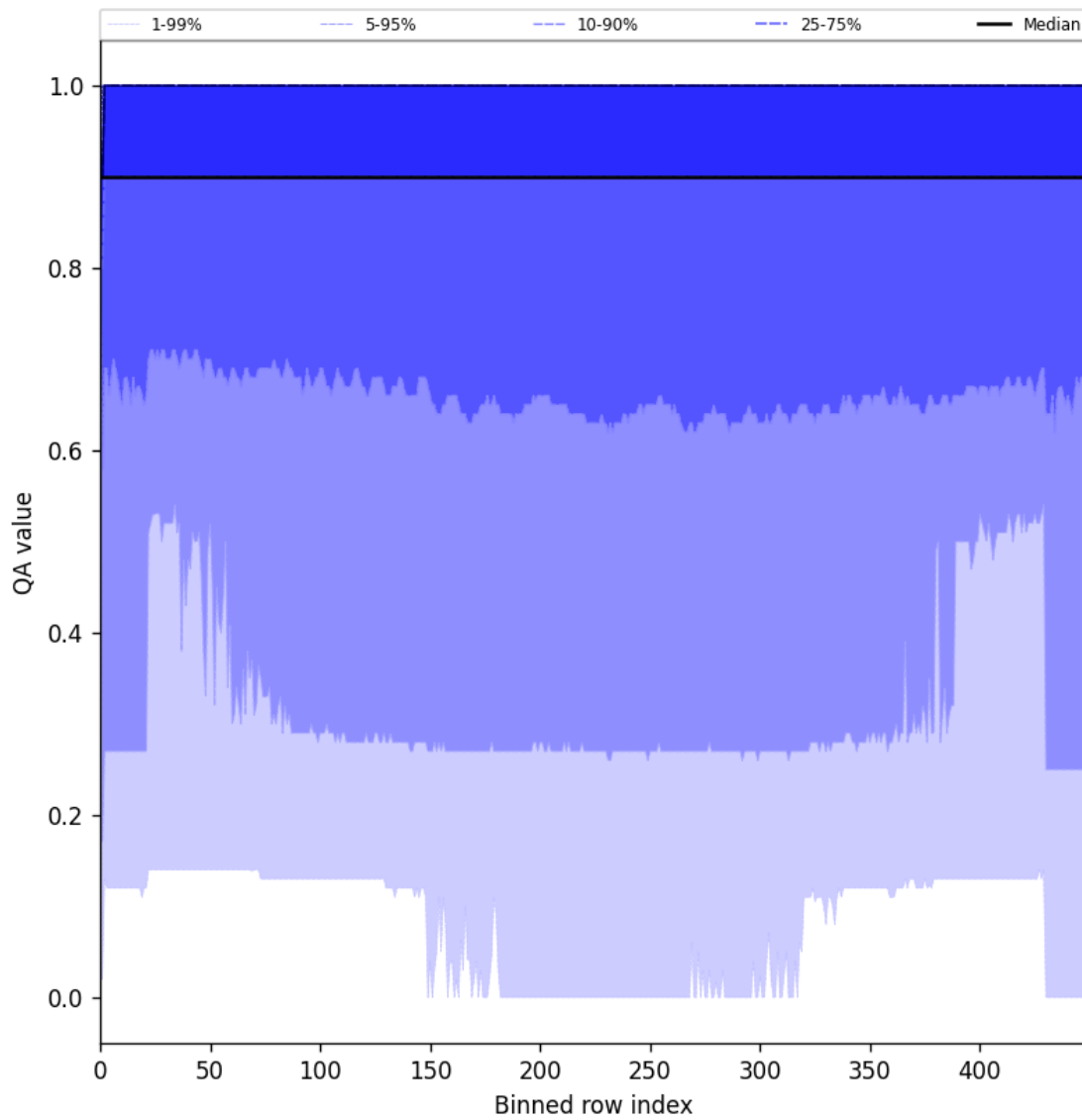
Figure 27: Along track statistics of “QA value” for 2025-08-10 to 2025-08-12
