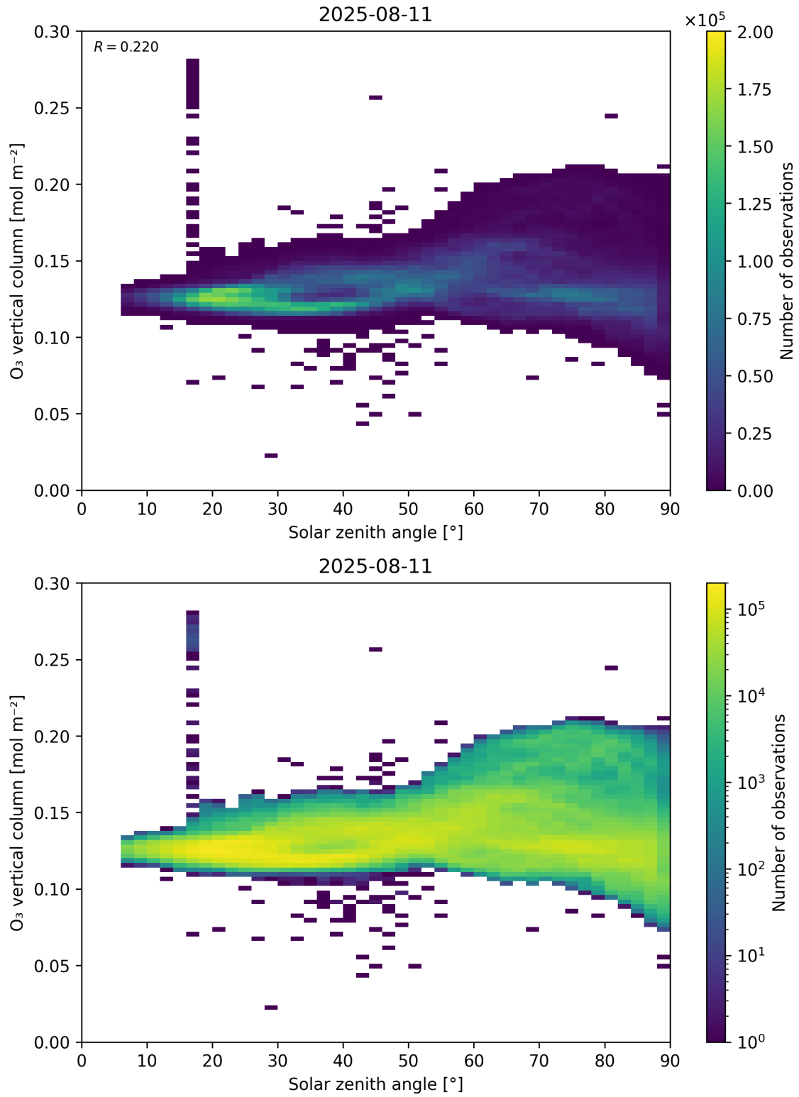
Figure 47: Scatter density plot of “Solar zenith angle” against “O 3 vertical column” for 2025-08-10 to 2025-08-12.
