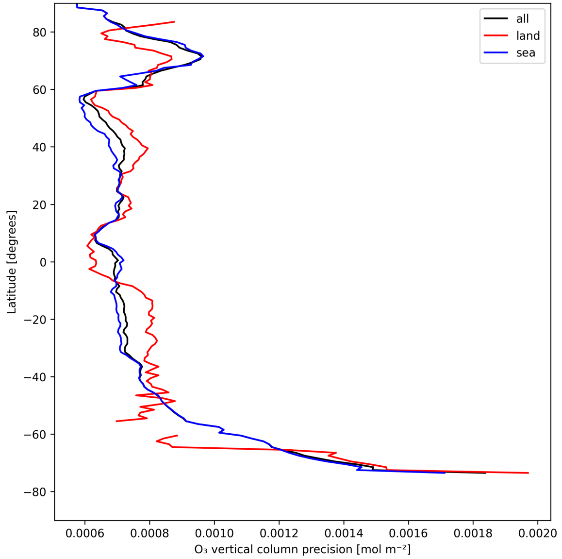
Figure 15: Zonal average of "O 3 vertical column precision" for 2025-08-10 to 2025-08-12.
