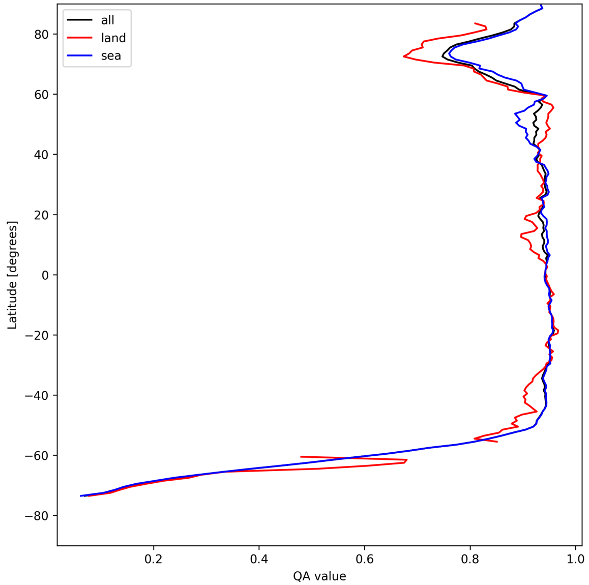
Figure 13: Zonal average of “QA value” for 2025-08-10 to 2025-08-12.
