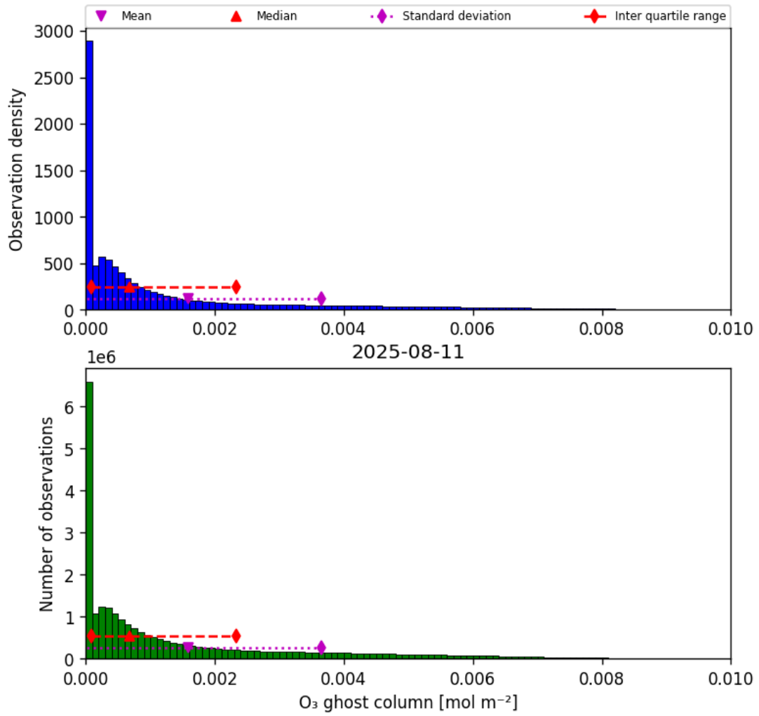
Figure 25: Histogram of “O 3 ghost column” for 2025-08-10 to 2025-08-12
