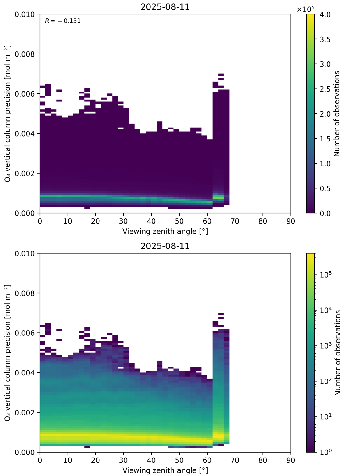
Figure 53: Scatter density plot of “Viewing zenith angle” against “O 3 vertical column precision” for 2025-08-10 to 2025-08-12.
