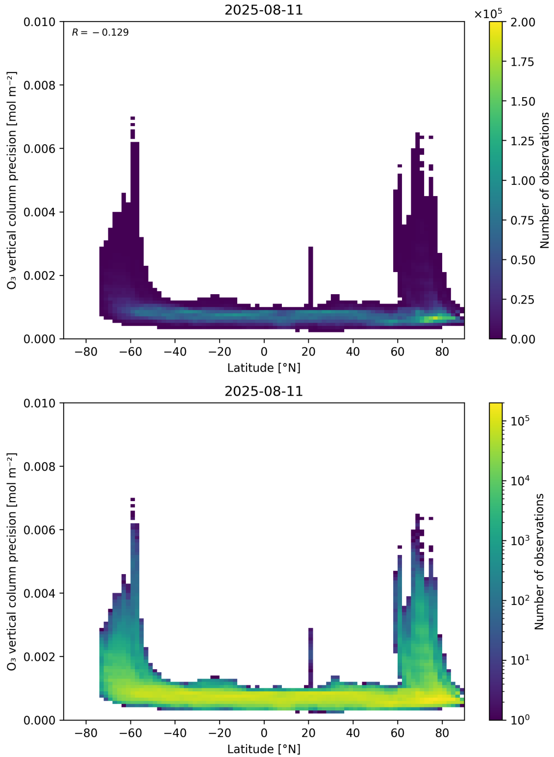
Figure 37: Scatter density plot of “Latitude” against “O 3 vertical column precision” for 2025-08-10 to 2025-08-12.
