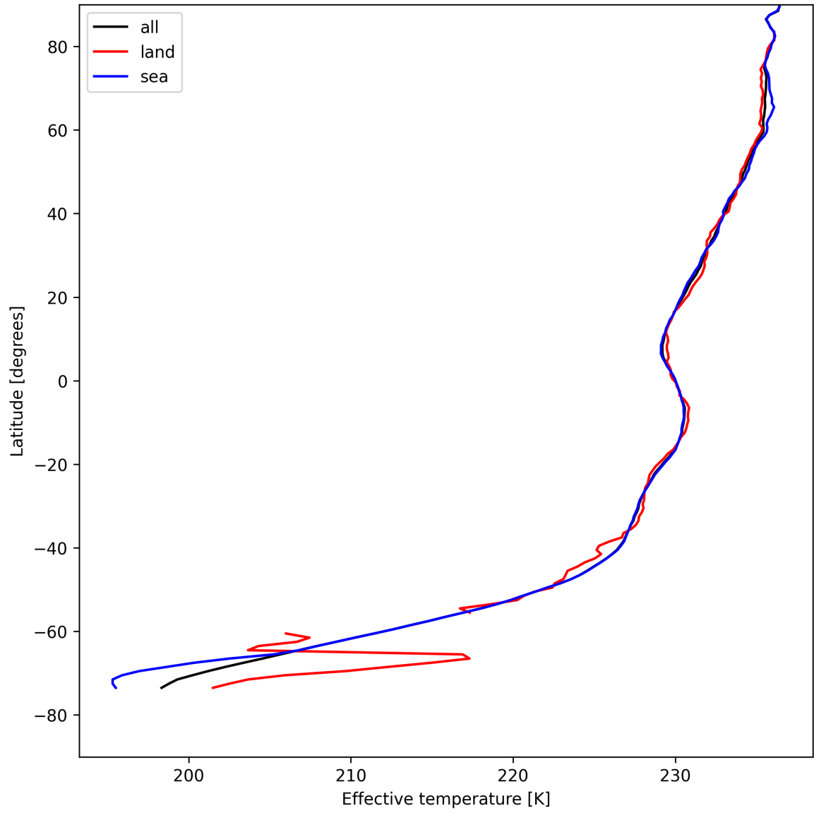
Figure 17: Zonal average of "Effective temperature" for 2025-08-10 to 2025-08-12.
