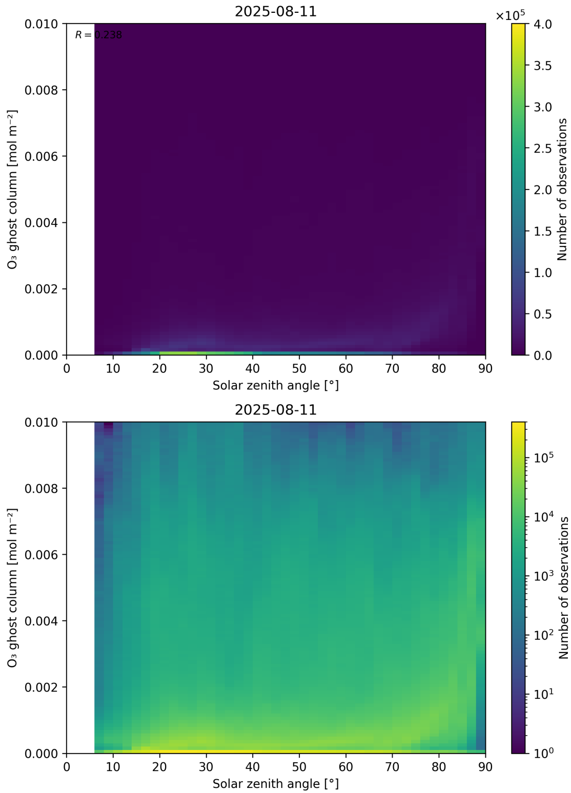
Figure 46: Scatter density plot of “Solar zenith angle” against “O 3 ghost column” for 2025-08-10 to 2025-08-12.
