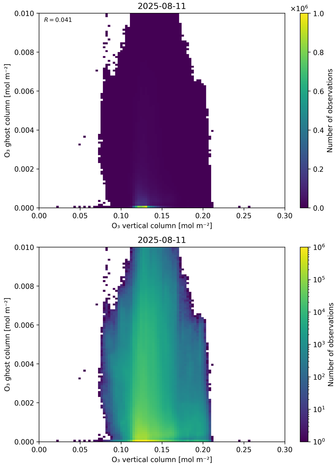
Figure 40: Scatter density plot of “O 3 vertical column” against “O 3 ghost column” for 2025-08-10 to 2025-08-12.
