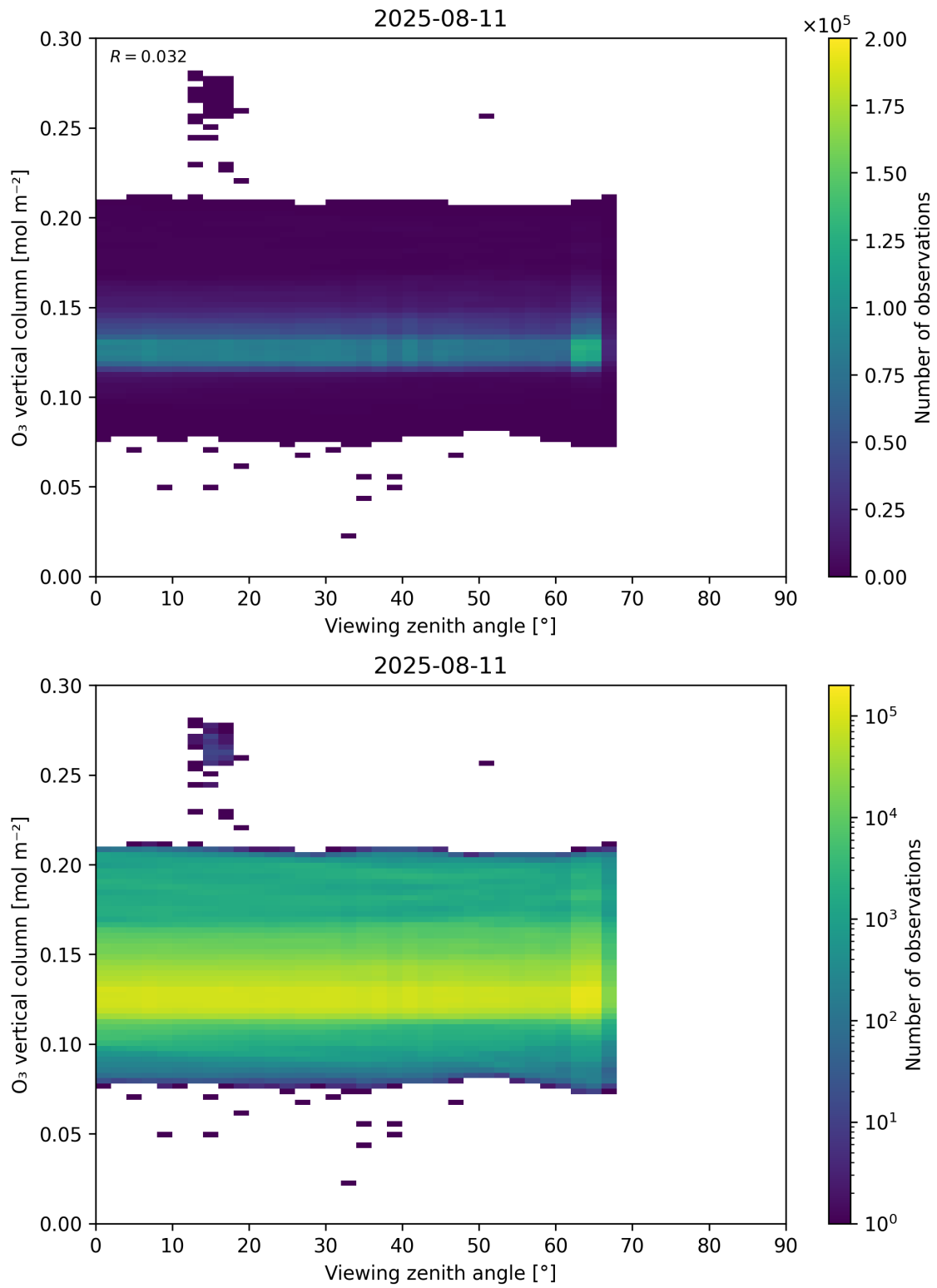
Figure 52: Scatter density plot of “Viewing zenith angle” against “O 3 vertical column” for 2025-08-10 to 2025-08-12.
