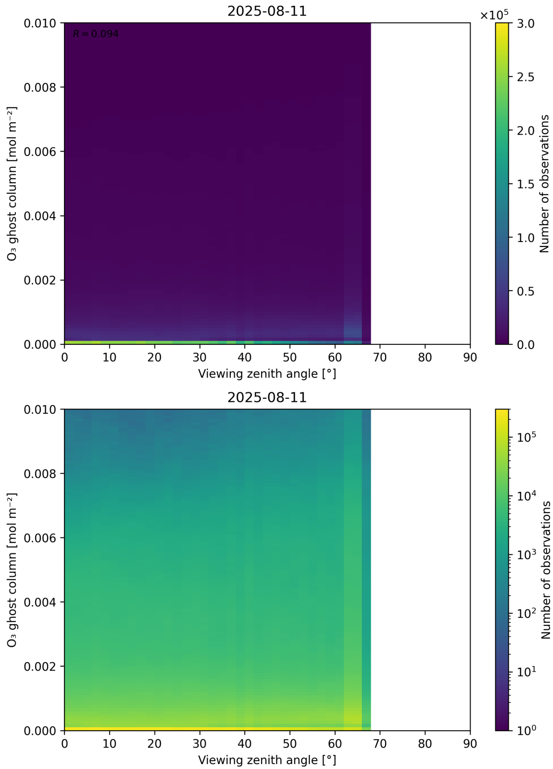
Figure 51: Scatter density plot of “Viewing zenith angle” against “O 3 ghost column” for 2025-08-10 to 2025-08-12.
