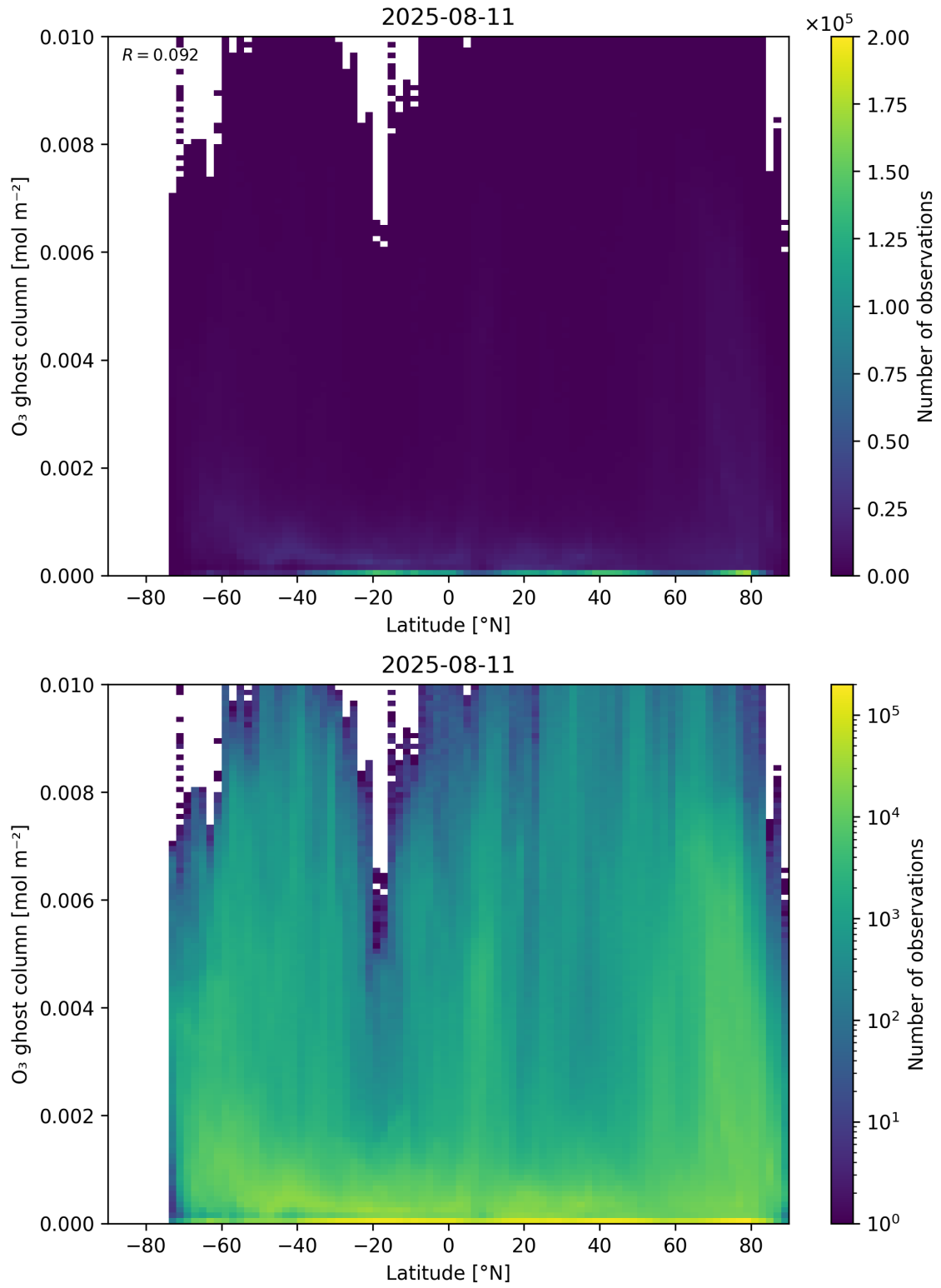
Figure 35: Scatter density plot of “Latitude” against “O 3 ghost column” for 2025-08-10 to 2025-08-12.
