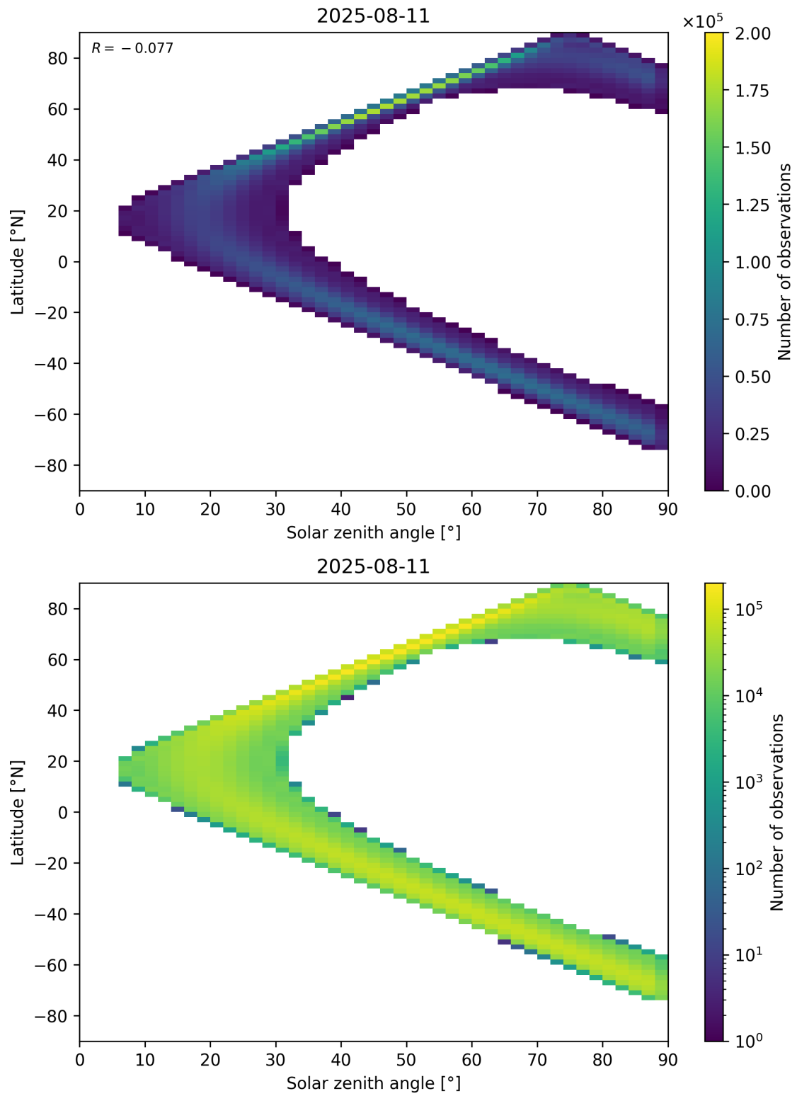
Figure 44: Scatter density plot of “Solar zenith angle” against “Latitude” for 2025-08-10 to 2025-08-12.
