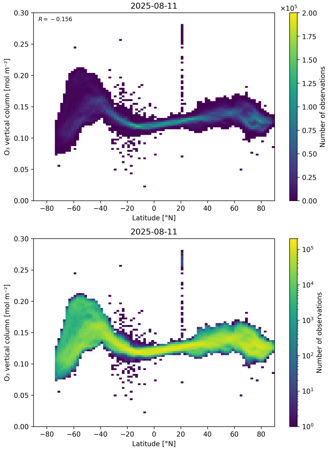
Figure 36: Scatter density plot of “Latitude” against “O 3 vertical column” for 2025-08-10 to 2025-08-12.
