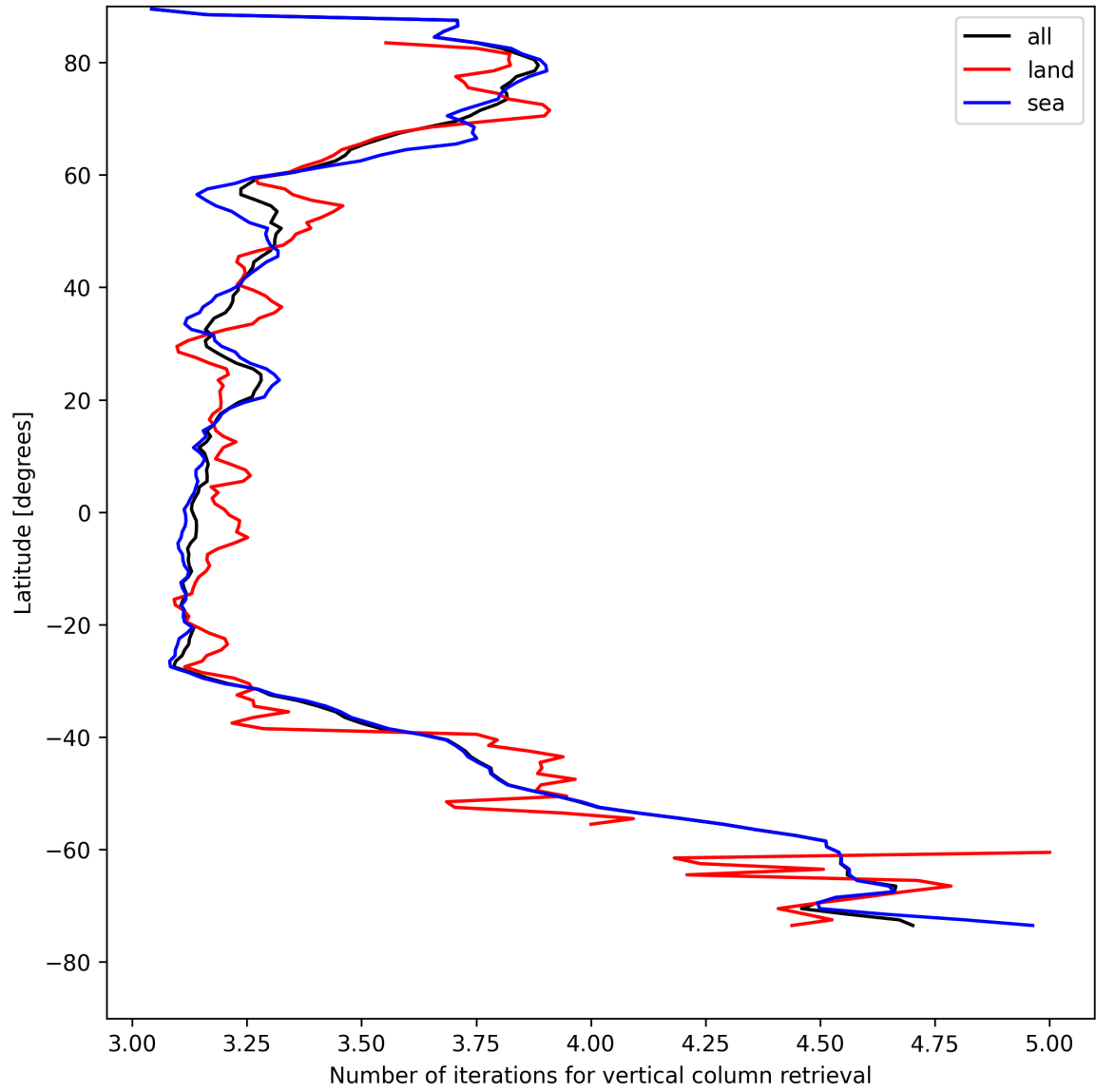
Figure 19: Zonal average of “Number of iterations for vertical column retrieval” for 2025-08-10 to 2025-08-12.
