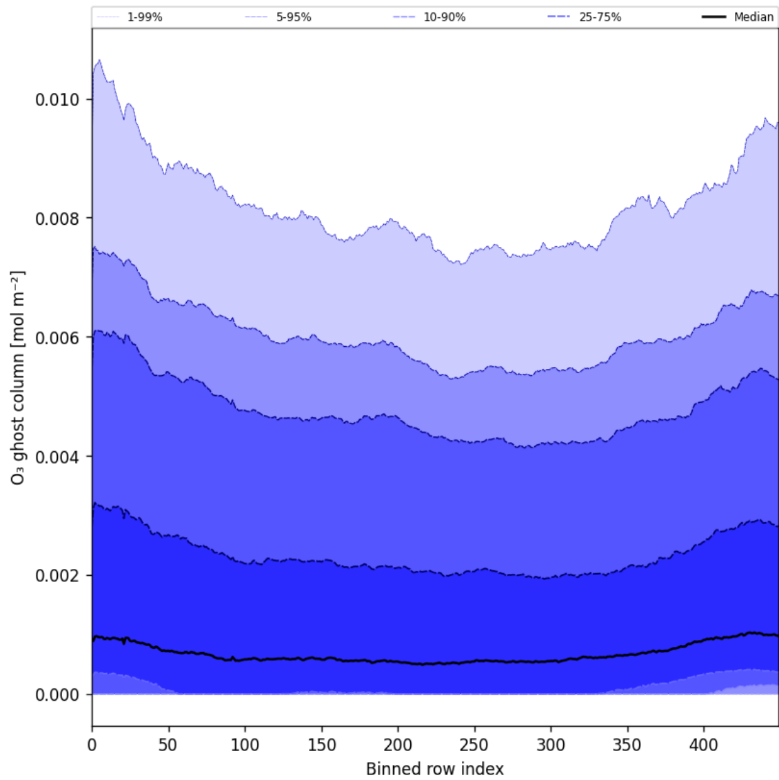
Figure 32: Along track statistics of “O 3 ghost column” for 2025-08-10 to 2025-08-12
