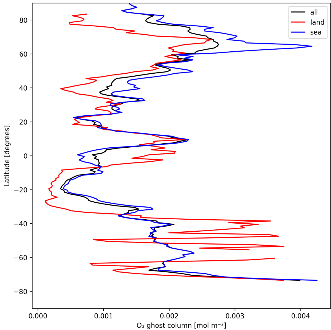
Figure 18: Zonal average of “O 3 ghost column” for 2025-08-10 to 2025-08-12.
