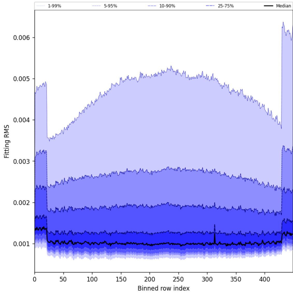
Figure 30: Along track statistics of “Fitting RMS” for 2025-08-10 to 2025-08-12
