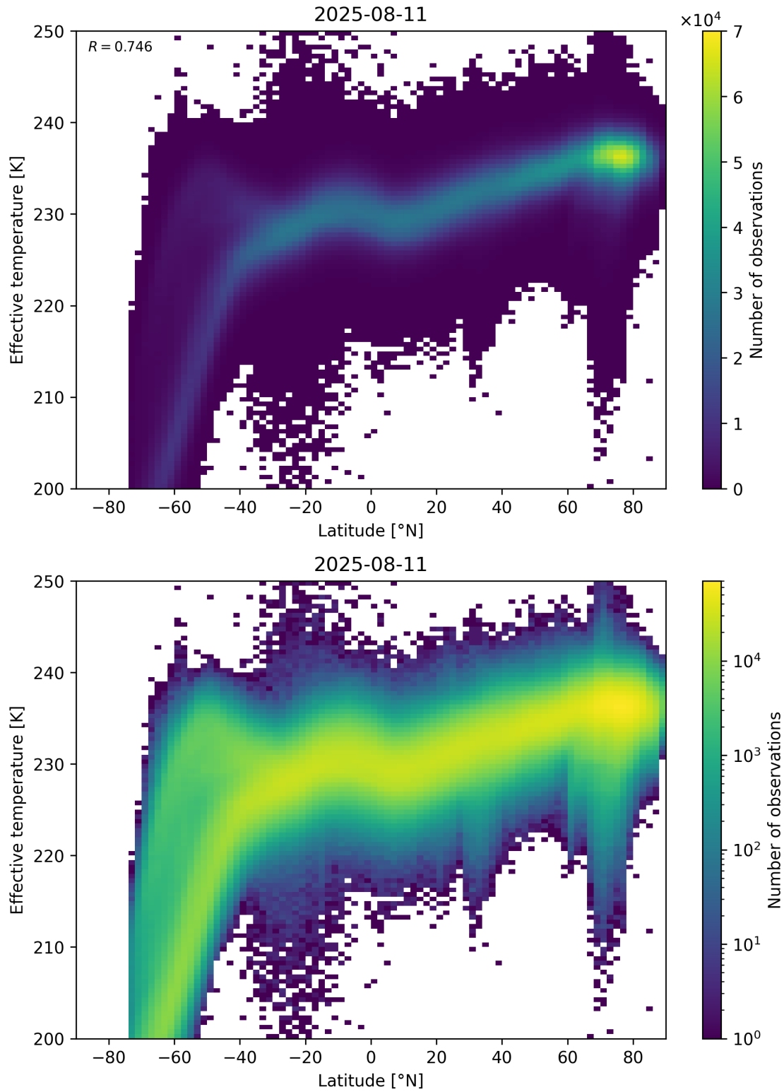
Figure 34: Scatter density plot of “Latitude” against “Effective temperature” for 2025-08-10 to 2025-08-12.
