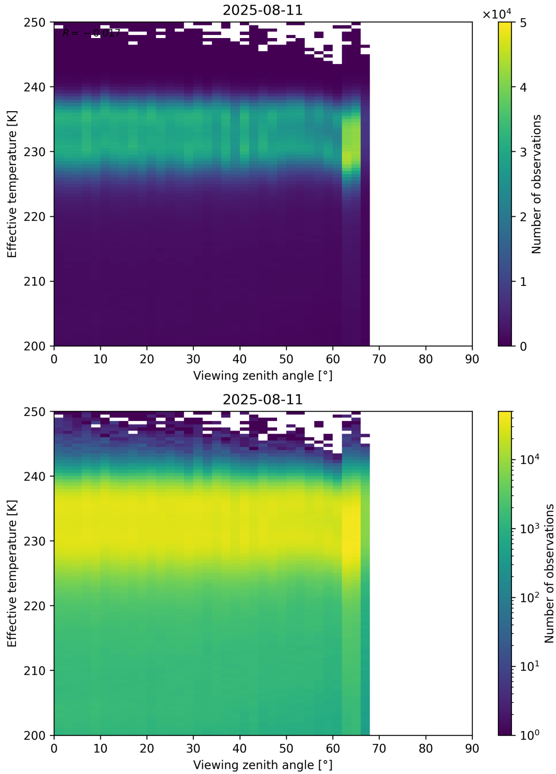
Figure 50: Scatter density plot of “Viewing zenith angle” against “Effective temperature” for 2025-08-10 to 2025-08-12.
