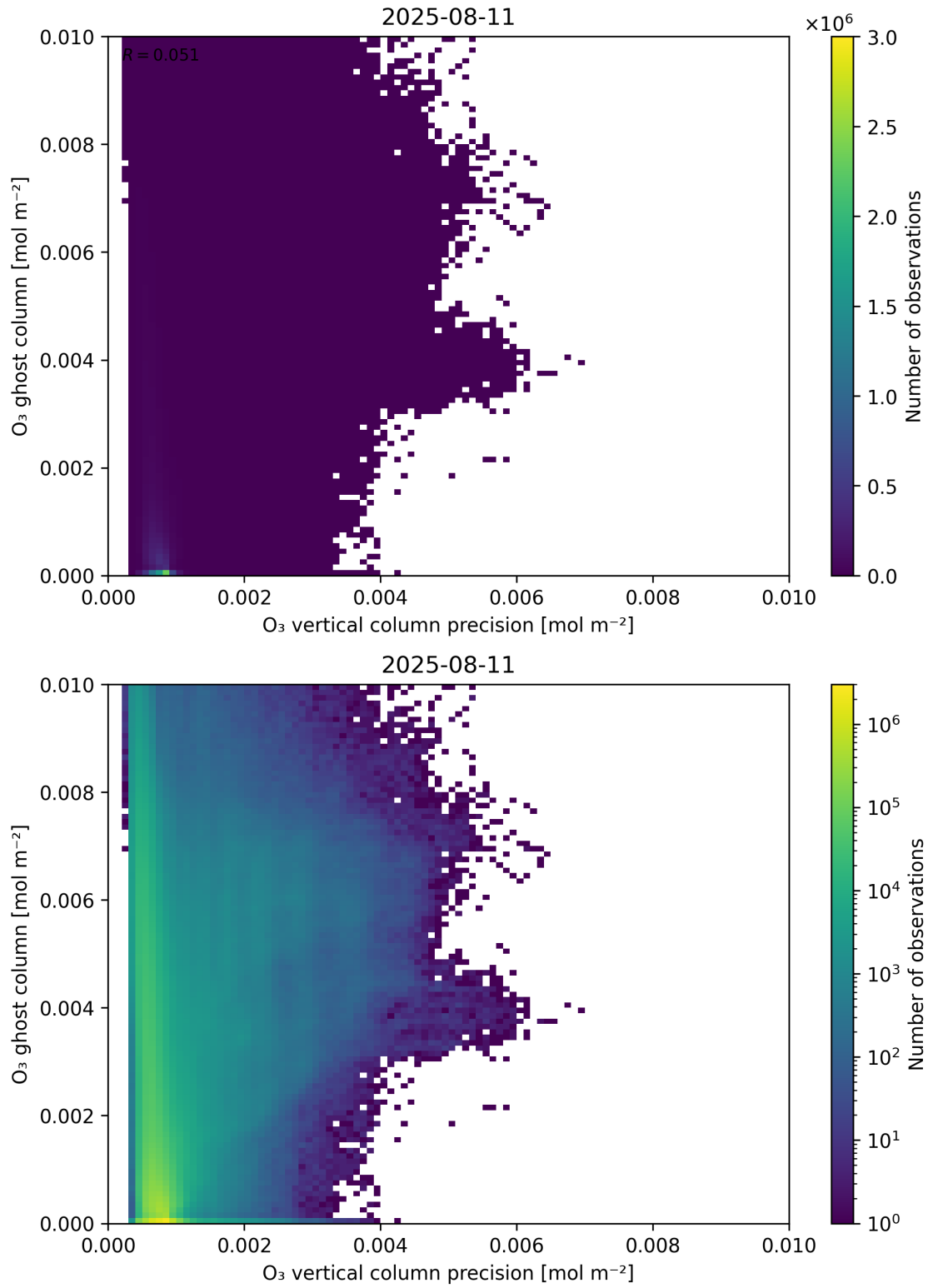
Figure 43: Scatter density plot of “ \text{O}_3 vertical column precision” against “ \text{O}_3 ghost column” for 2025-08-10 to 2025-08-12.
