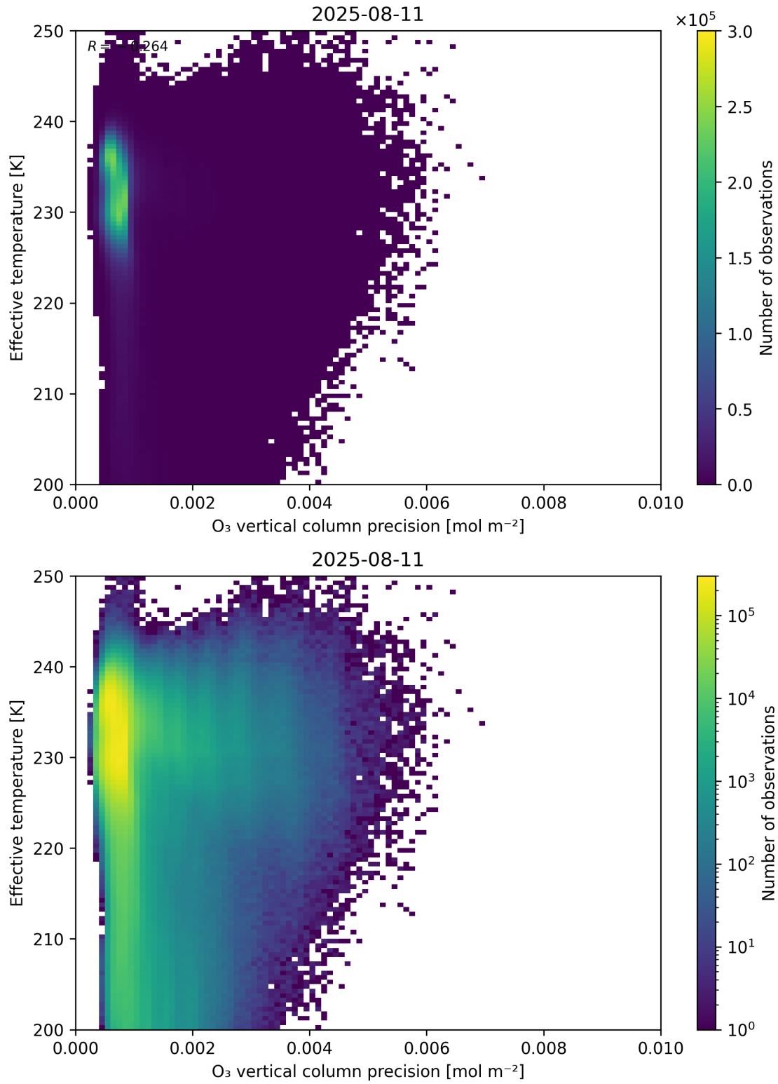
Figure 42: Scatter density plot of “O 3 vertical column precision” against “Effective temperature” for 2025-08-10 to 2025-08-12.
