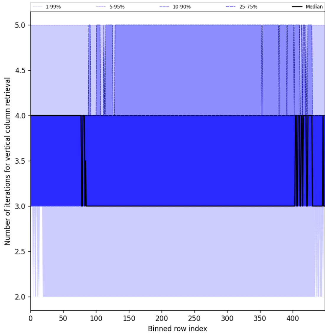
Figure 33: Along track statistics of “Number of iterations for vertical column retrieval” for 2025-08-10 to 2025-08-12
