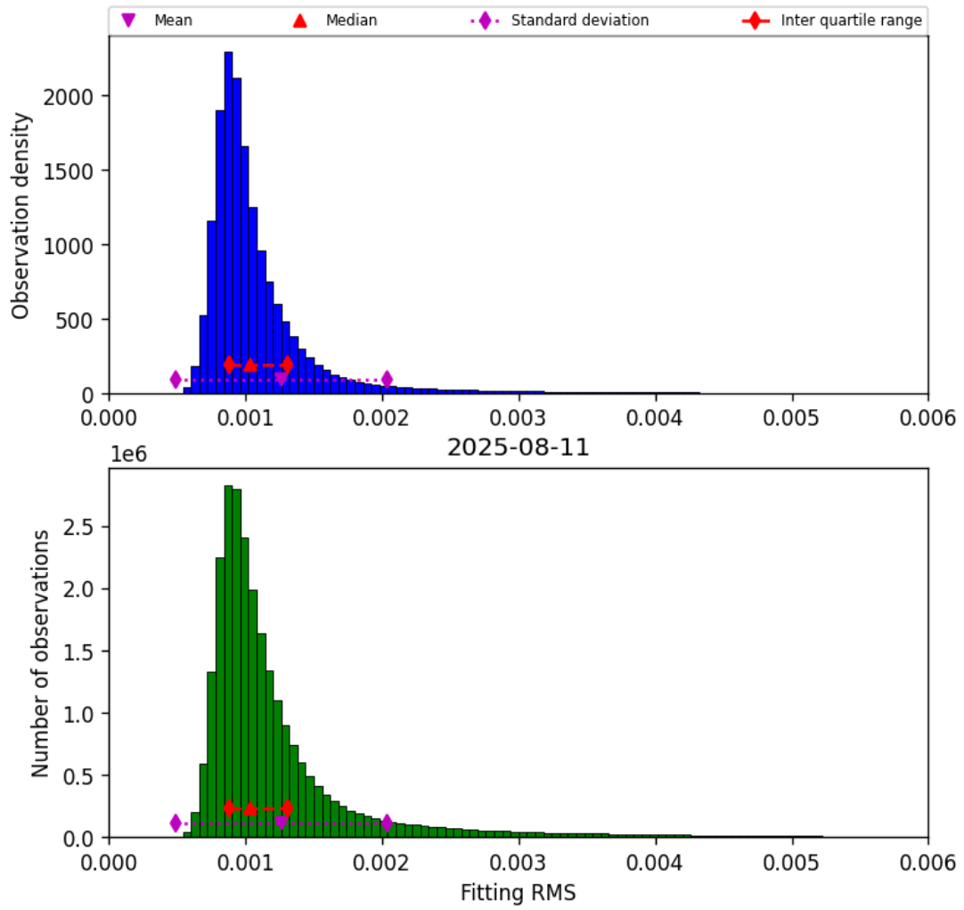
Figure 23: Histogram of “Fitting RMS” for 2025-08-10 to 2025-08-12
