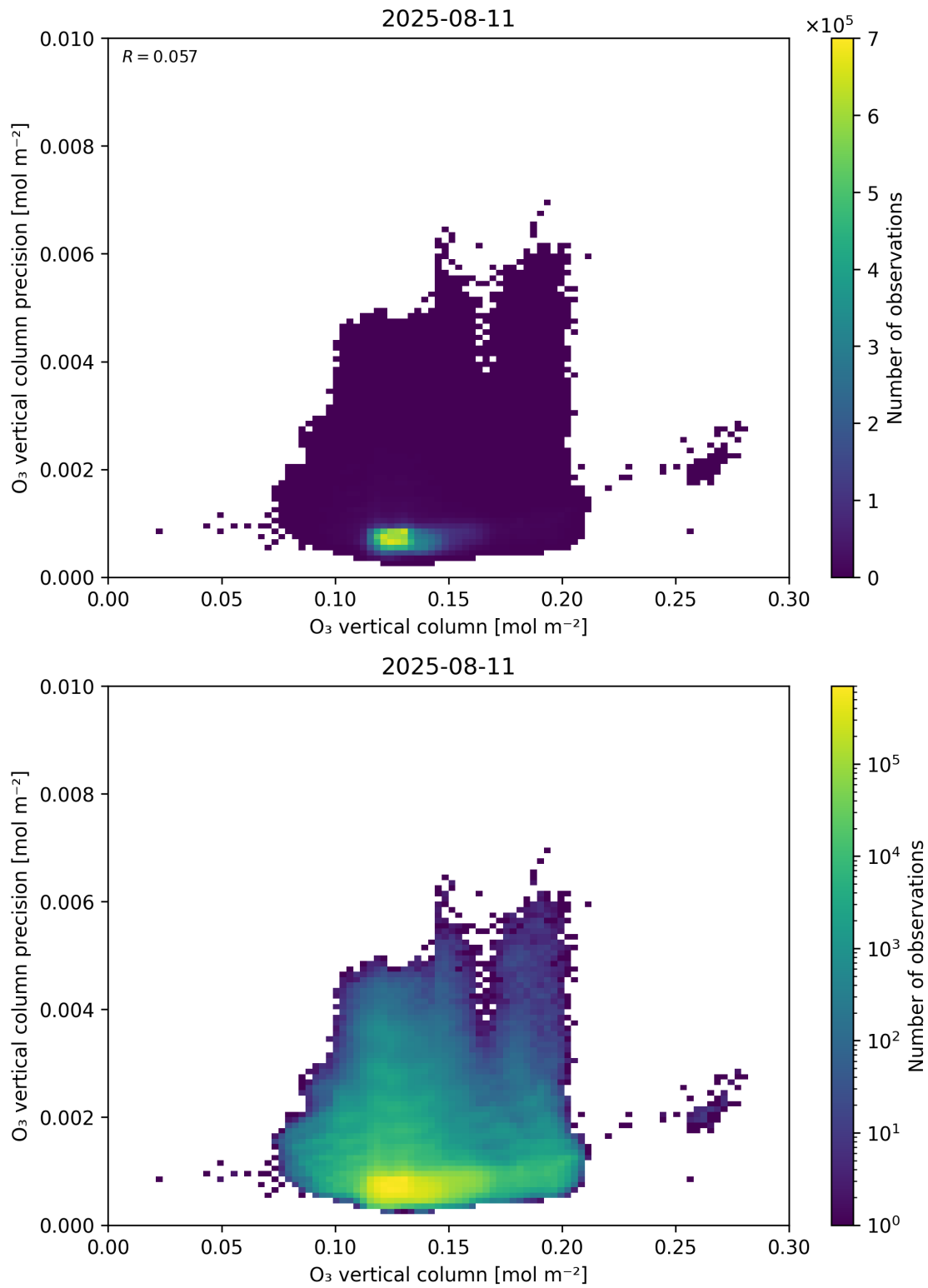
Figure 41: Scatter density plot of “O 3 vertical column” against “O 3 vertical column precision” for 2025-08-10 to 2025-08-12.
