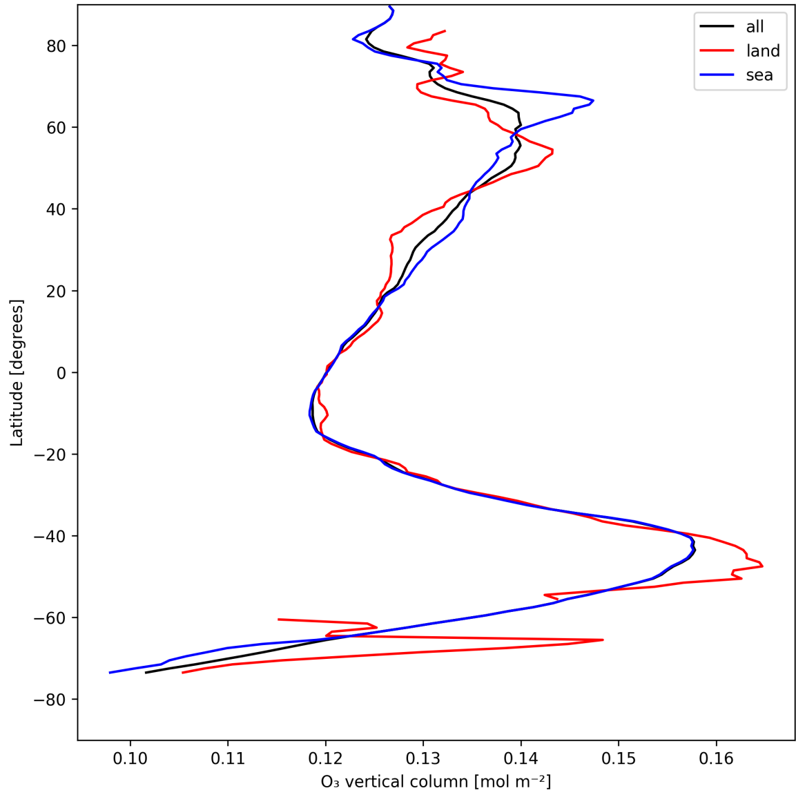
Figure 14: Zonal average of “O 3 vertical column” for 2025-08-10 to 2025-08-12.
