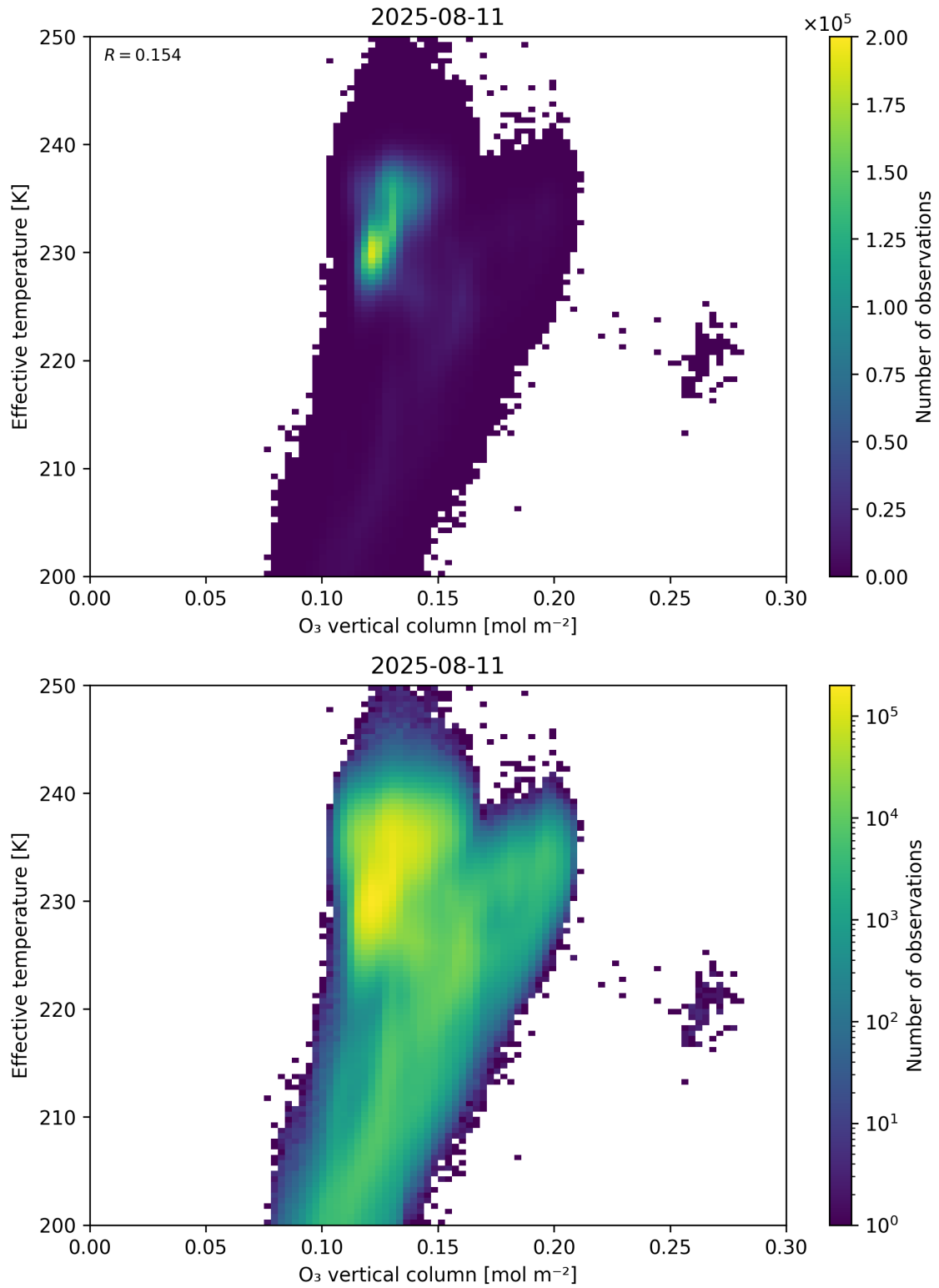
Figure 39: Scatter density plot of “O 3 vertical column” against “Effective temperature” for 2025-08-10 to 2025-08-12.
