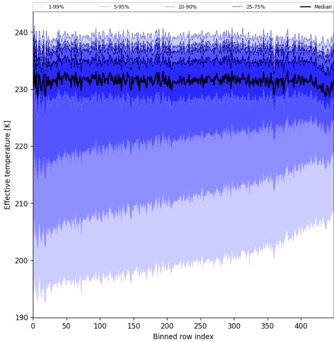
Figure 31: Along track statistics of “Effective temperature” for 2025-08-10 to 2025-08-12
