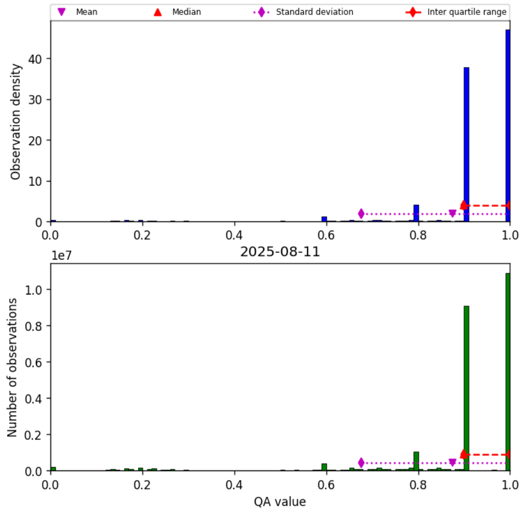
Figure 20: Histogram of “QA value” for 2025-08-10 to 2025-08-12
