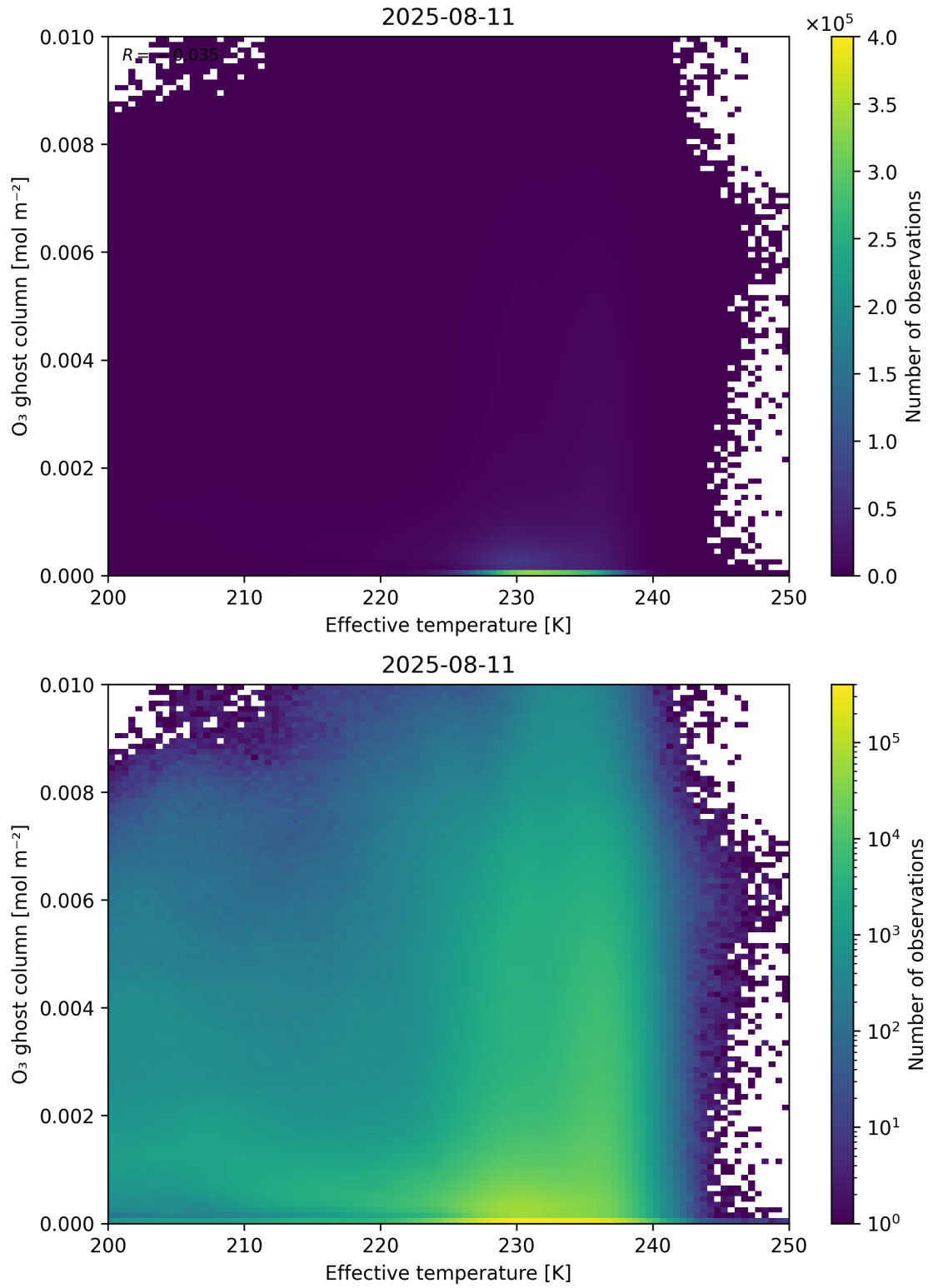
Figure 38: Scatter density plot of “Effective temperature” against “O 3 ghost column” for 2025-08-10 to 2025-08-12.
