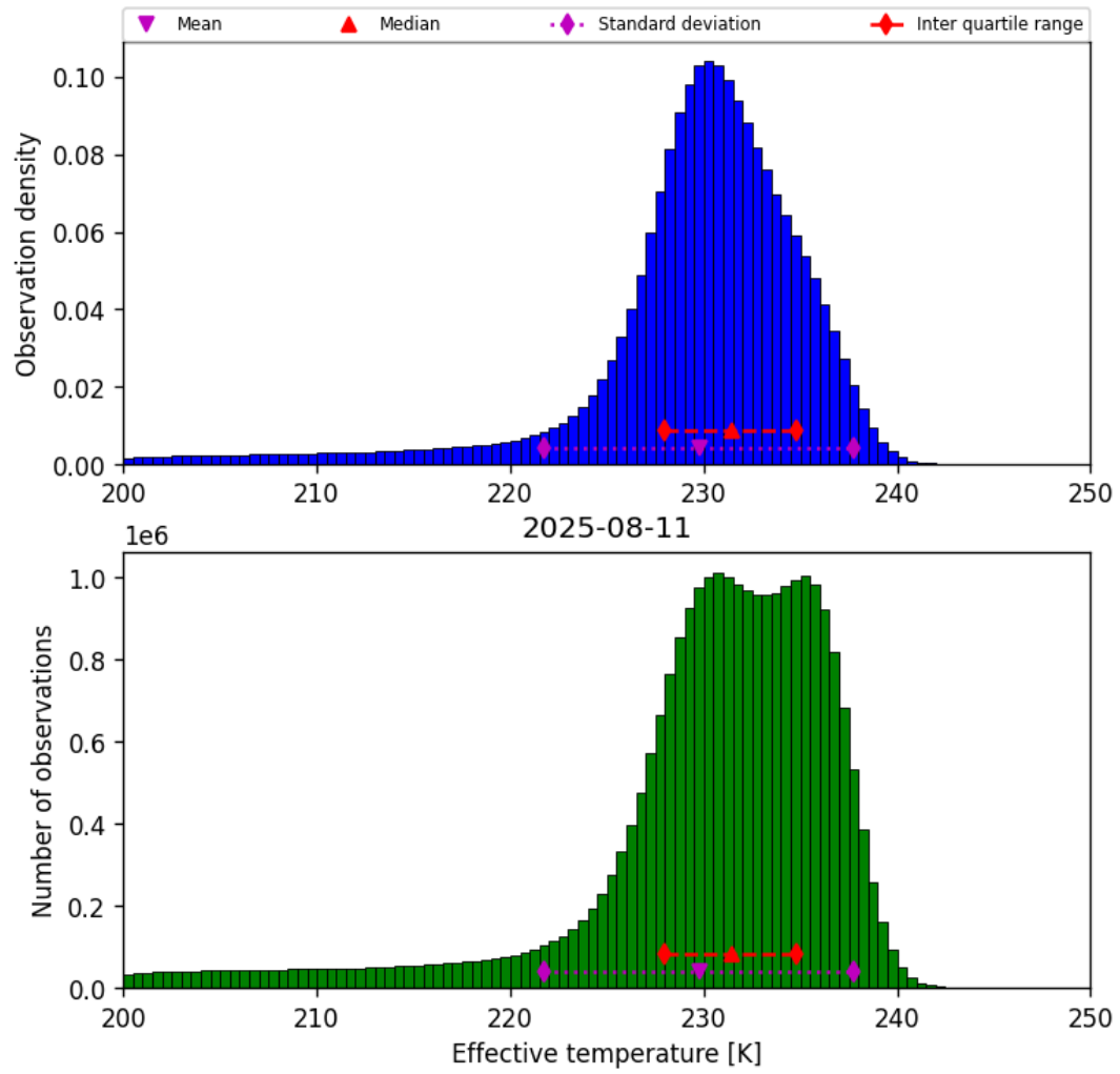
Figure 24: Histogram of “Effective temperature” for 2025-08-10 to 2025-08-12
