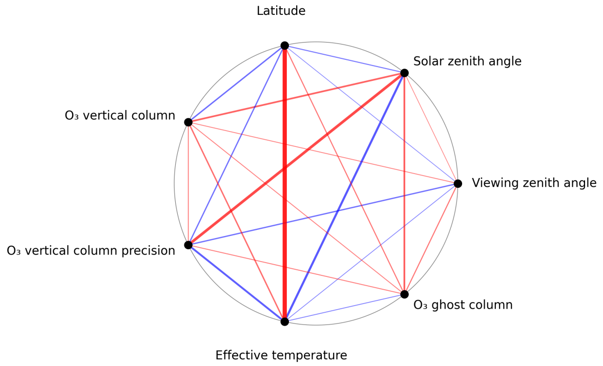
Figure 1: Map of correlation graph for 2025-08-10 to 2025-08-12.
