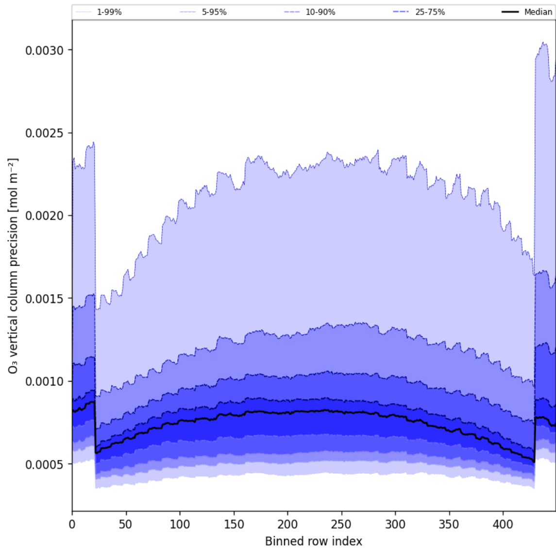
Figure 29: Along track statistics of “O 3 vertical column precision” for 2025-08-10 to 2025-08-12
