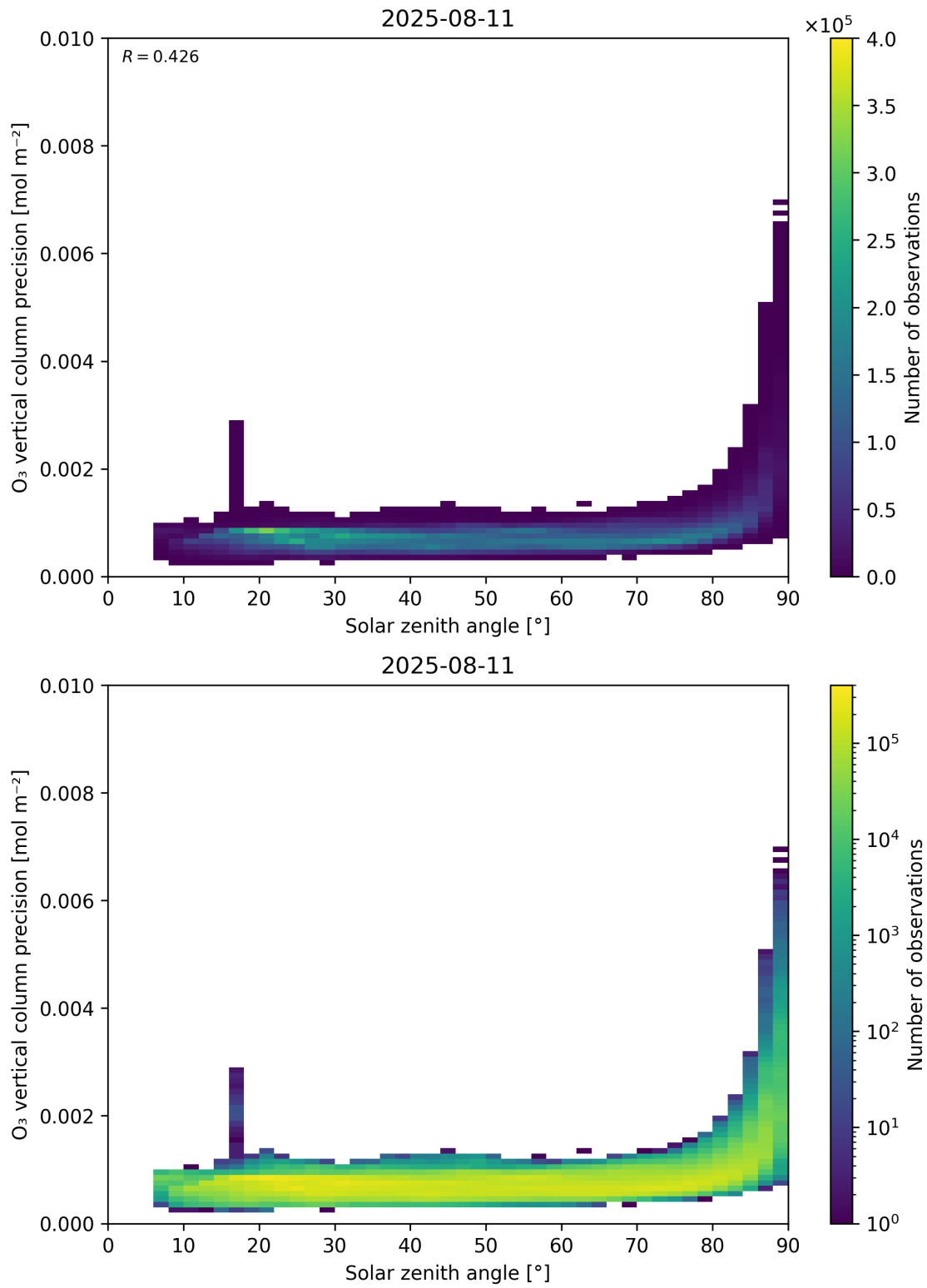
Figure 48: Scatter density plot of “Solar zenith angle” against “O 3 vertical column precision” for 2025-08-10 to 2025-08-12.
