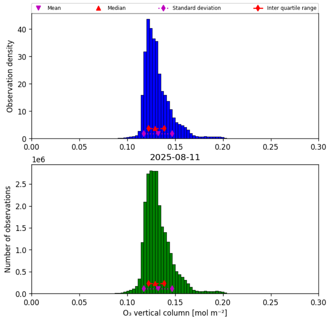
Figure 21: Histogram of “O 3 vertical column” for 2025-08-10 to 2025-08-12
