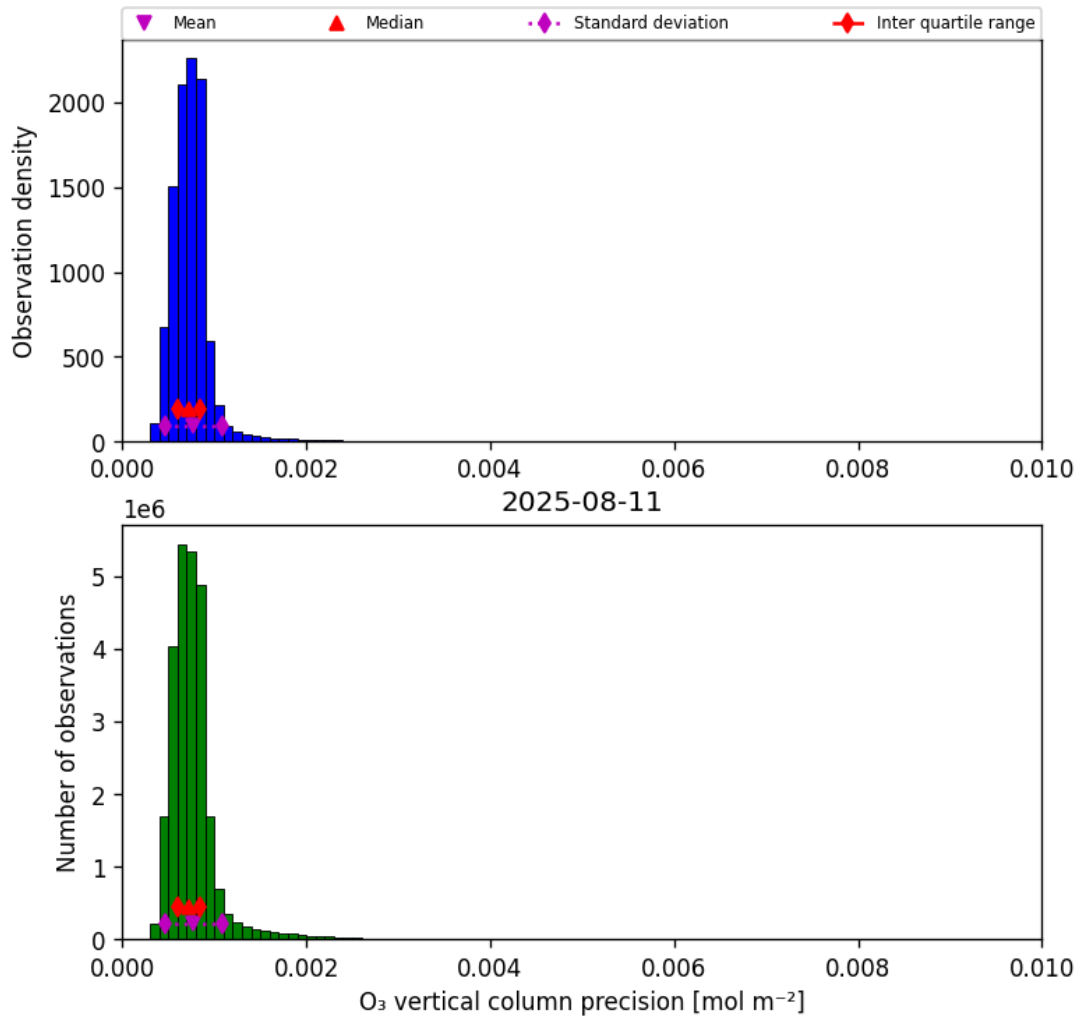
Figure 22: Histogram of “O 3 vertical column precision” for 2025-08-10 to 2025-08-12
