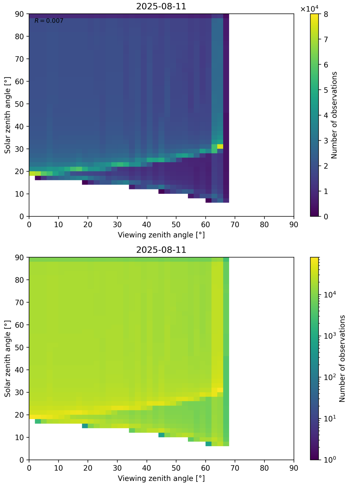
Figure 54: Scatter density plot of “Viewing zenith angle” against “Solar zenith angle” for 2025-08-10 to 2025-08-12.
