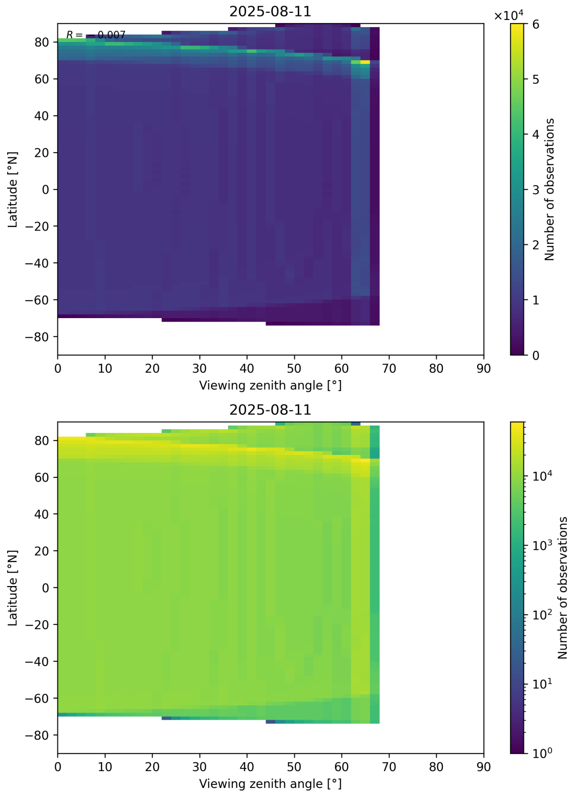
Figure 49: Scatter density plot of “Viewing zenith angle” against “Latitude” for 2025-08-10 to 2025-08-12.
