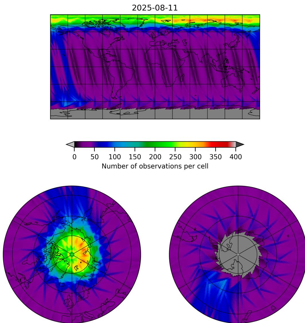
Figure 12: Map of the number of observations for 2025-08-10 to 2025-08-12
