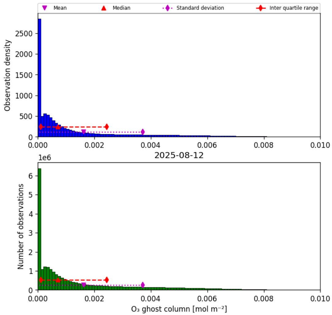
Figure 25: Histogram of “O 3 ghost column” for 2025-08-11 to 2025-08-13
