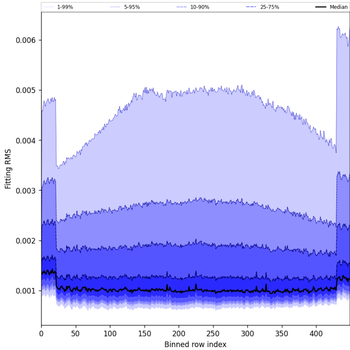
Figure 30: Along track statistics of “Fitting RMS” for 2025-08-11 to 2025-08-13
