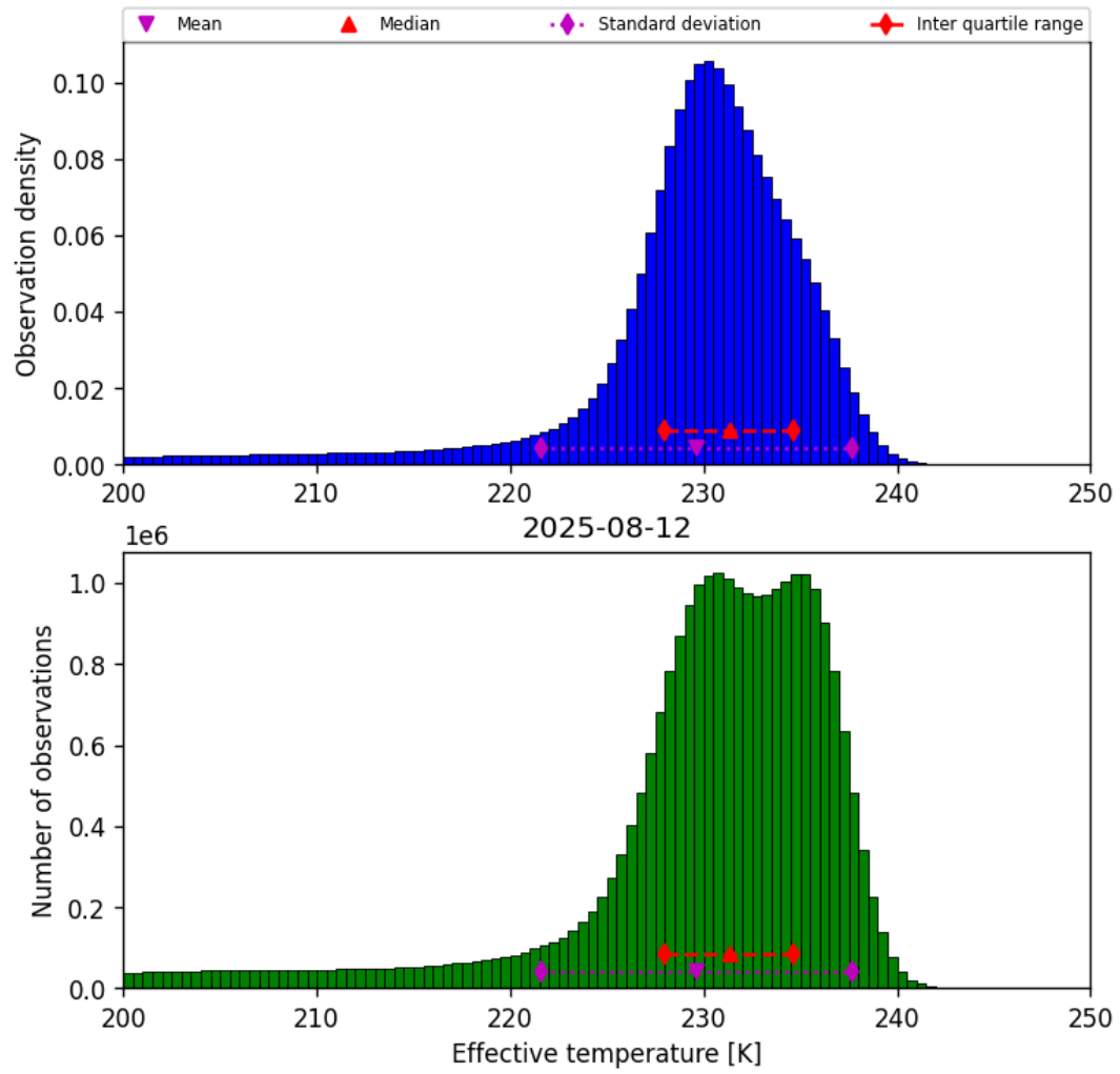
Figure 24: Histogram of “Effective temperature” for 2025-08-11 to 2025-08-13
