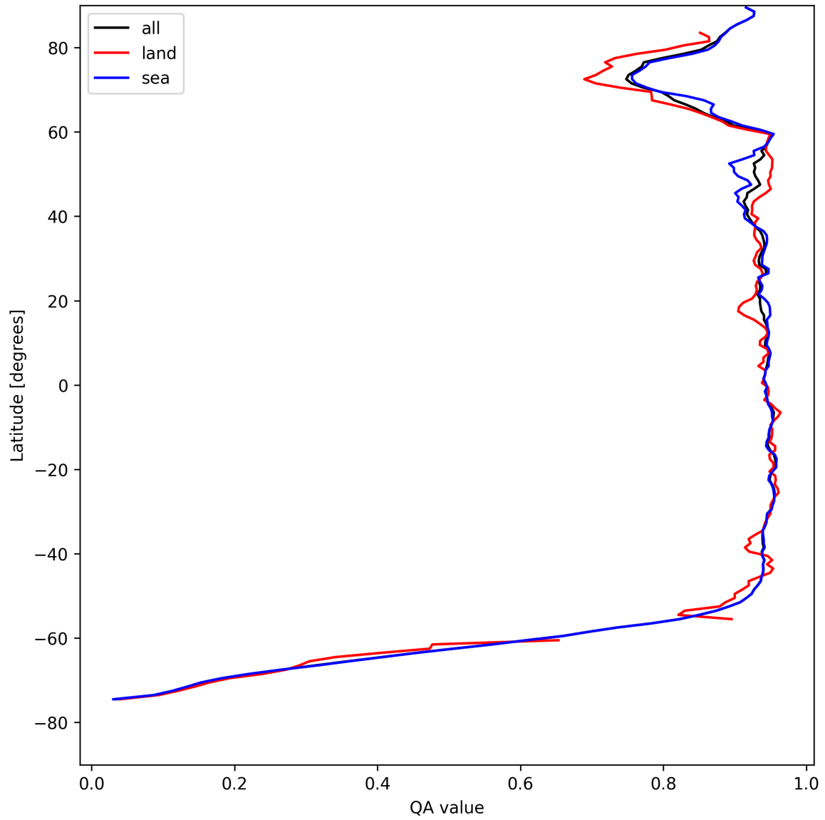
Figure 13: Zonal average of “QA value” for 2025-08-11 to 2025-08-13.
