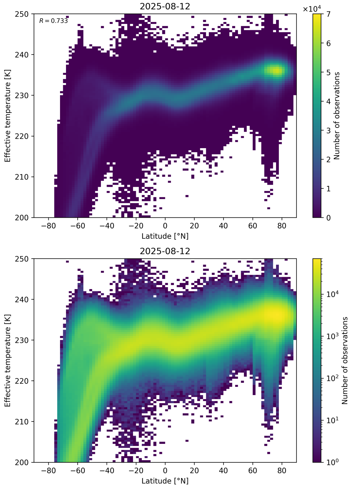
Figure 34: Scatter density plot of “Latitude” against “Effective temperature” for 2025-08-11 to 2025-08-13.
