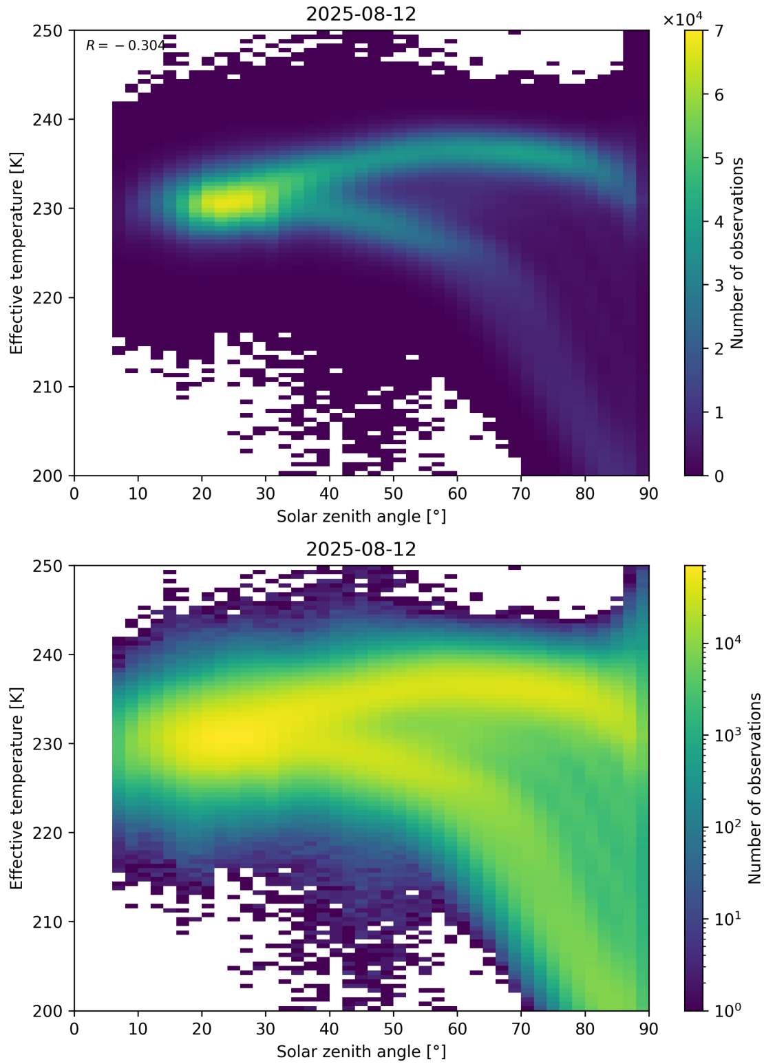
Figure 45: Scatter density plot of “Solar zenith angle” against “Effective temperature” for 2025-08-11 to 2025-08-13.
