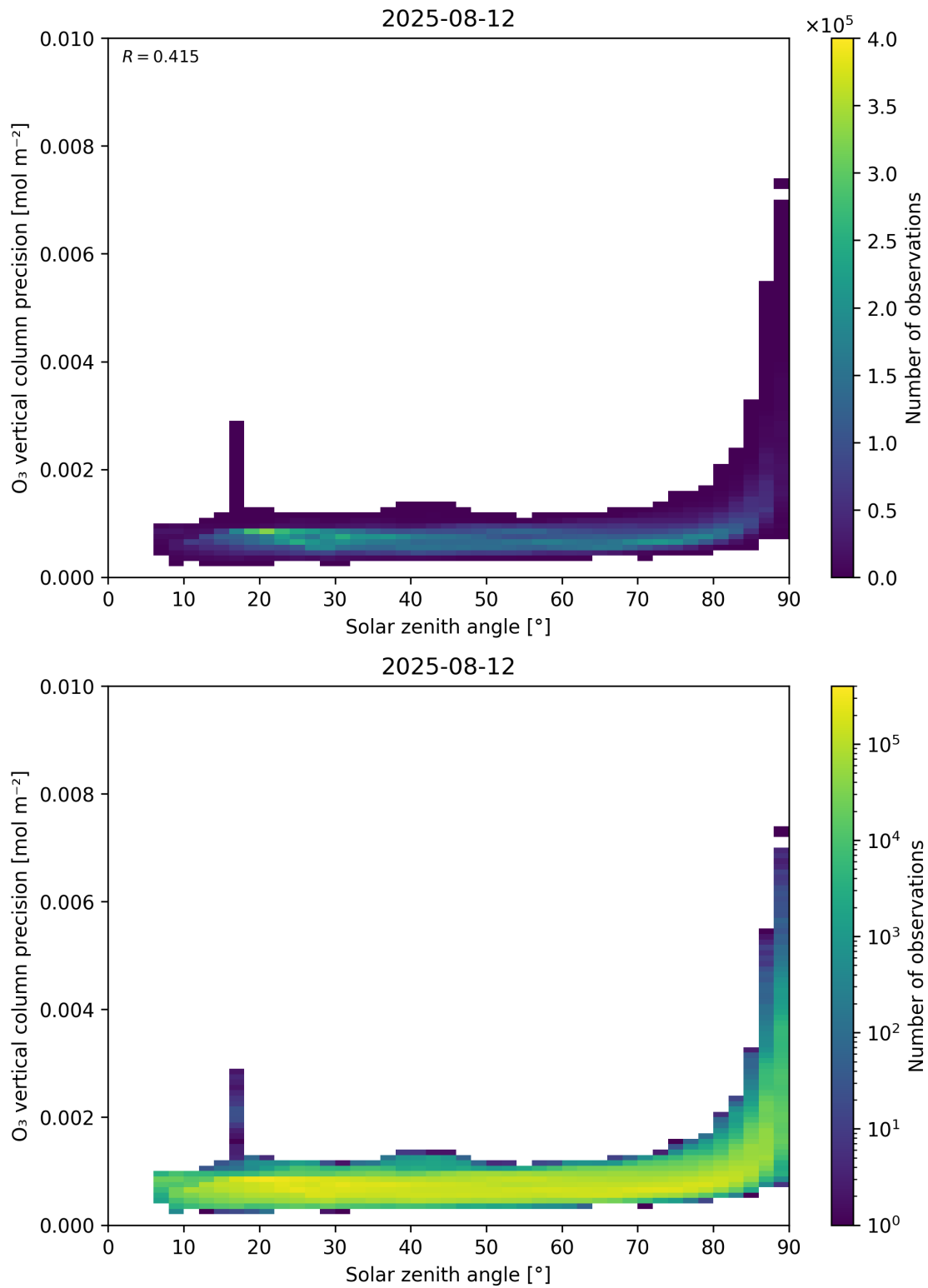
Figure 48: Scatter density plot of “Solar zenith angle” against “O 3 vertical column precision” for 2025-08-11 to 2025-08-13.
