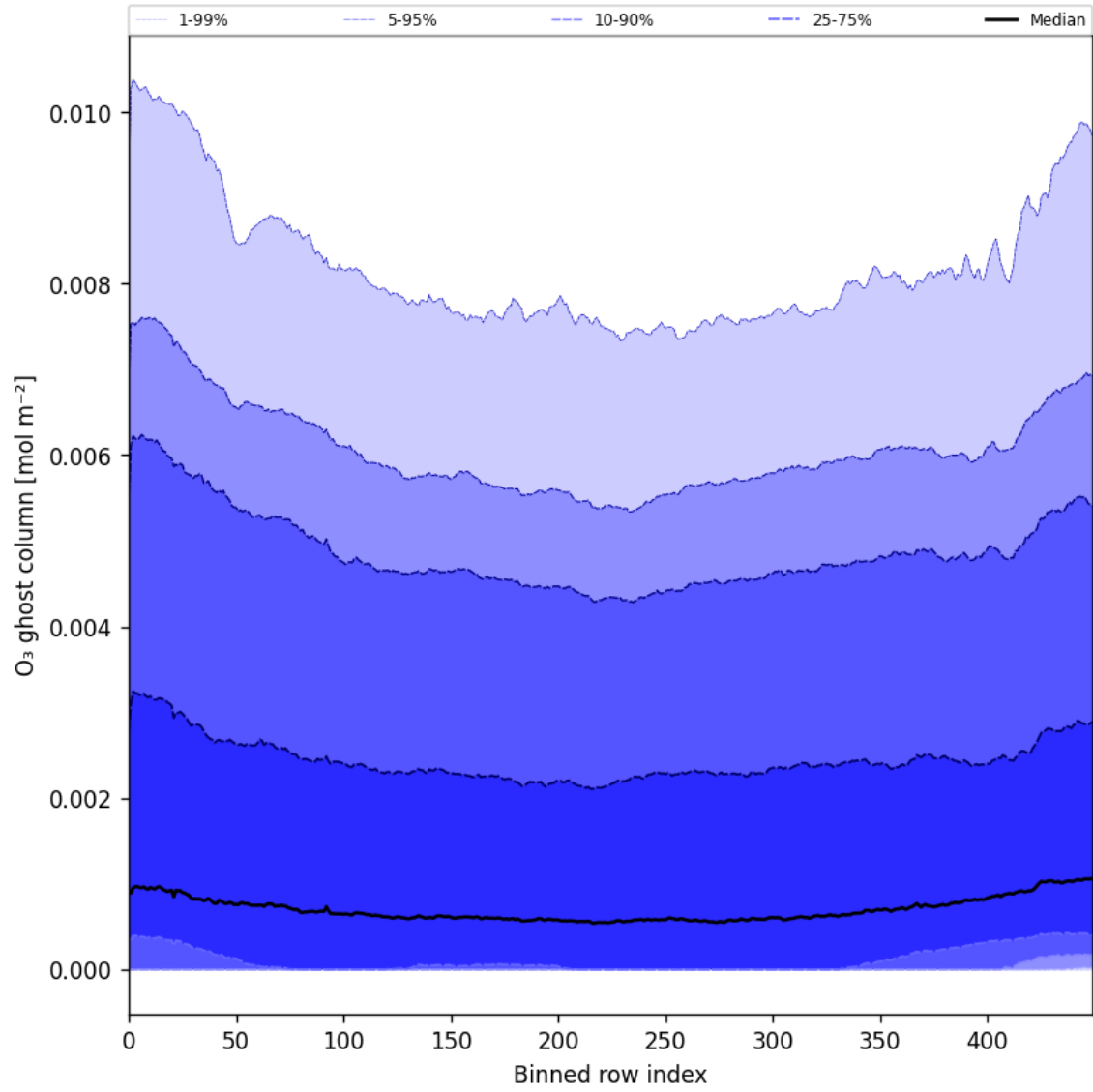
Figure 32: Along track statistics of “O 3 ghost column” for 2025-08-11 to 2025-08-13
