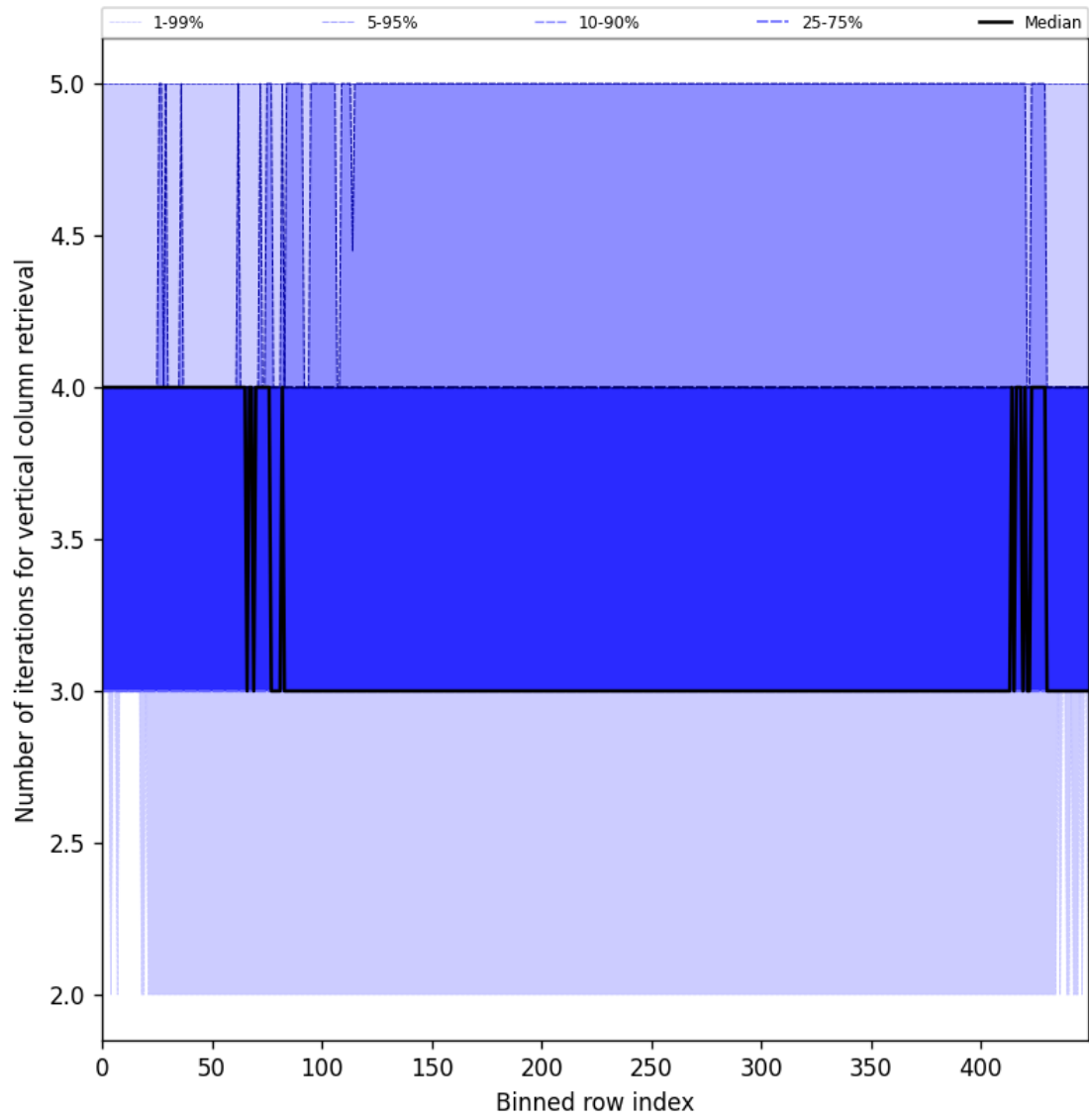
Figure 33: Along track statistics of “Number of iterations for vertical column retrieval” for 2025-08-11 to 2025-08-13
