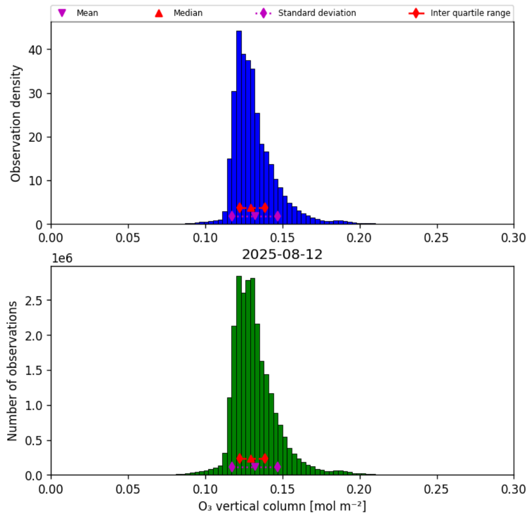
Figure 21: Histogram of “O 3 vertical column” for 2025-08-11 to 2025-08-13
