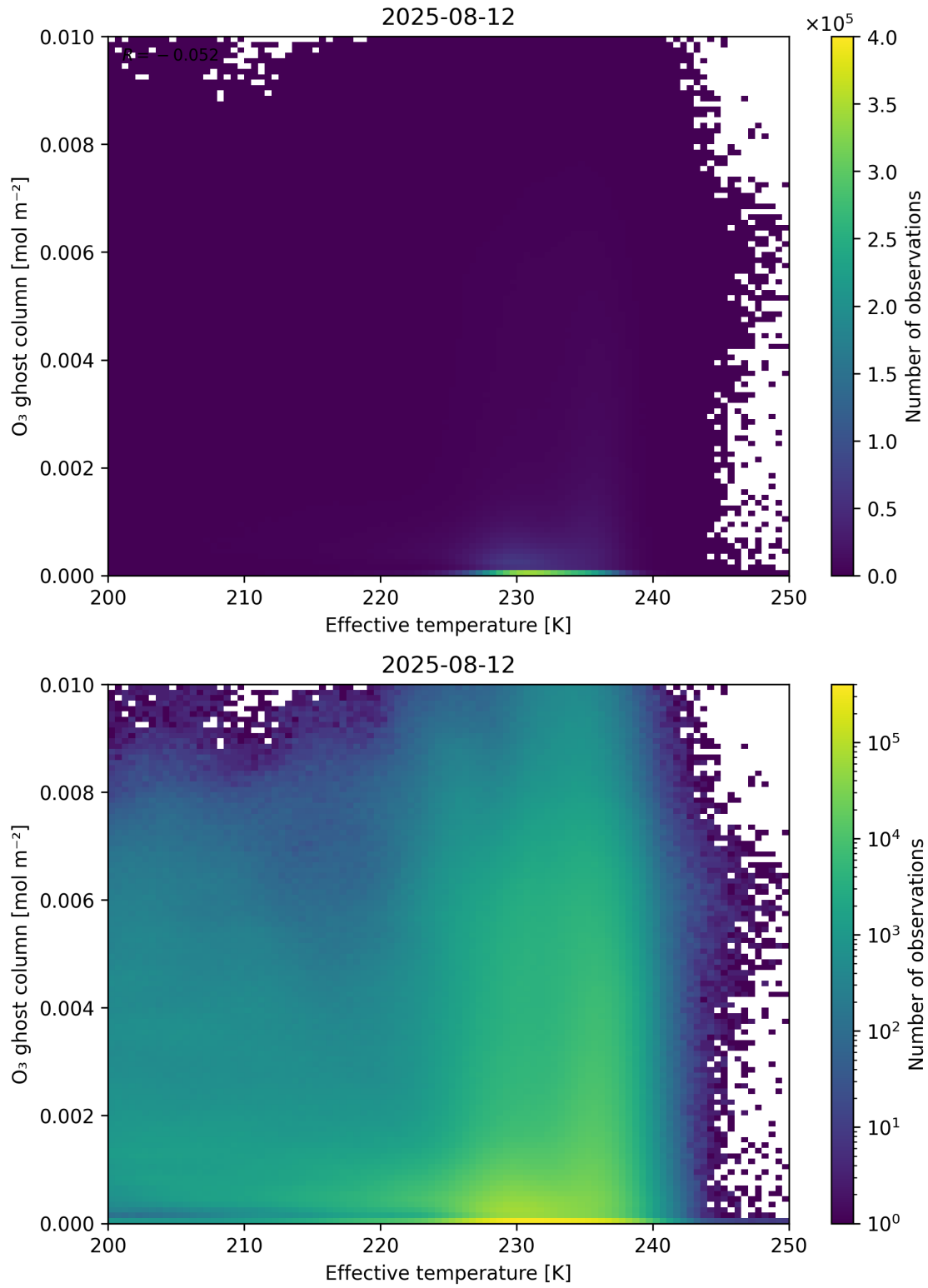
Figure 38: Scatter density plot of “Effective temperature” against “O 3 ghost column” for 2025-08-11 to 2025-08-13.
