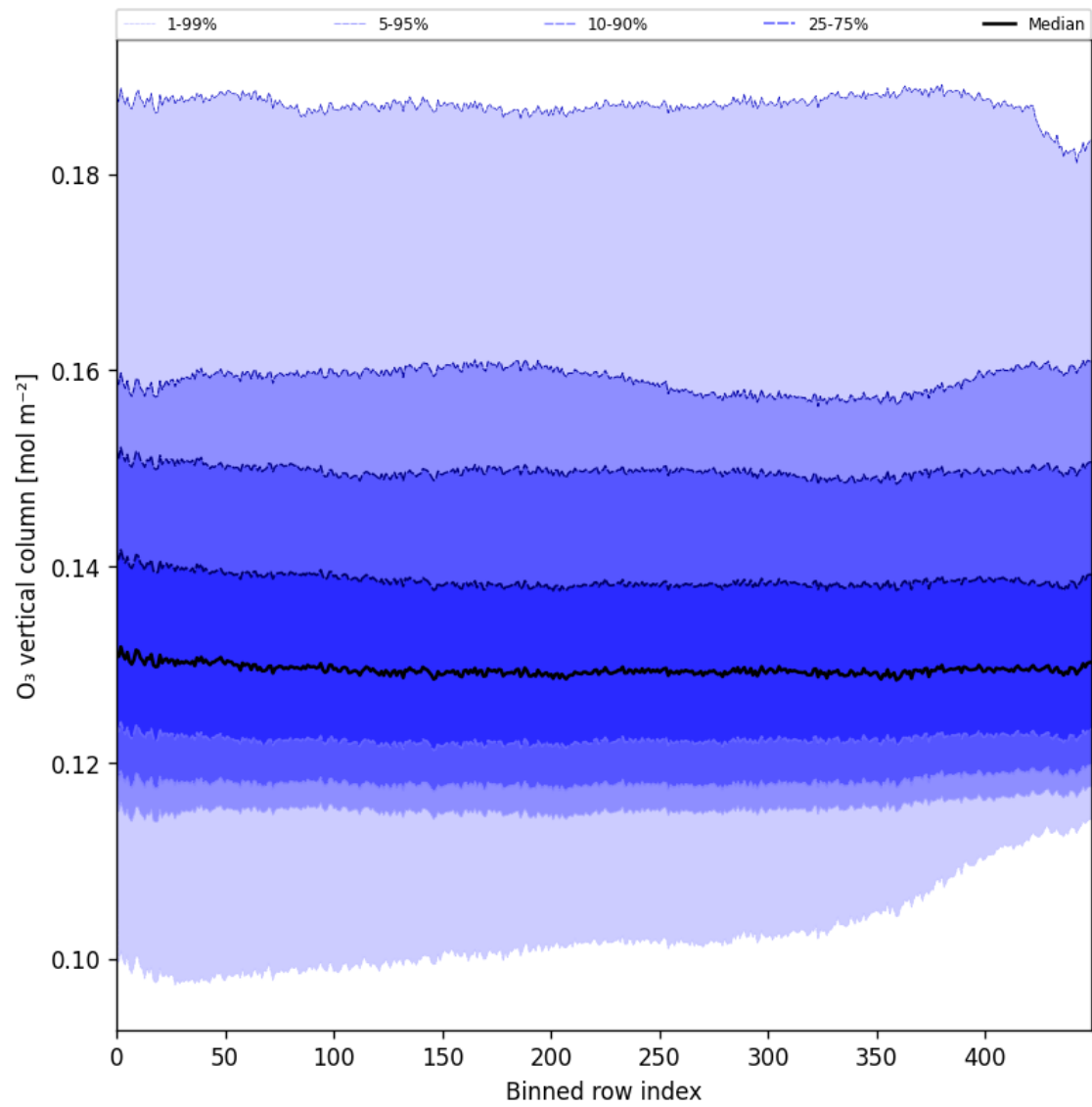
Figure 28: Along track statistics of “O 3 vertical column” for 2025-08-11 to 2025-08-13
