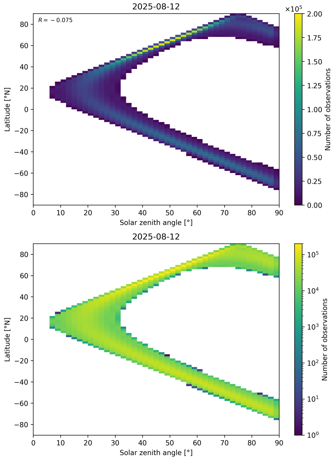
Figure 44: Scatter density plot of “Solar zenith angle” against “Latitude” for 2025-08-11 to 2025-08-13.
