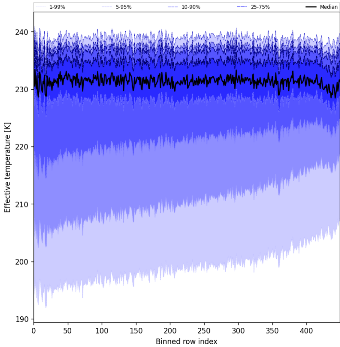
Figure 31: Along track statistics of “Effective temperature” for 2025-08-11 to 2025-08-13
