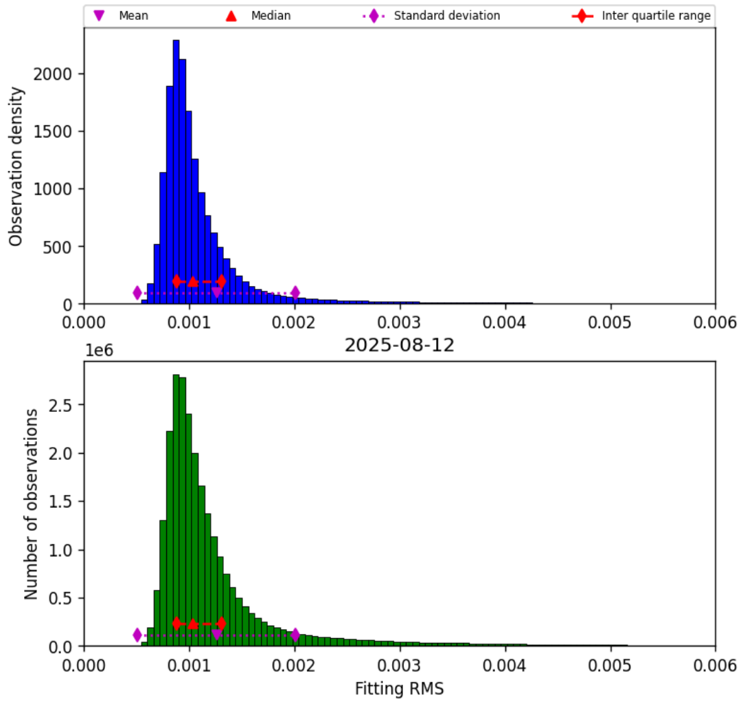
Figure 23: Histogram of “Fitting RMS” for 2025-08-11 to 2025-08-13
