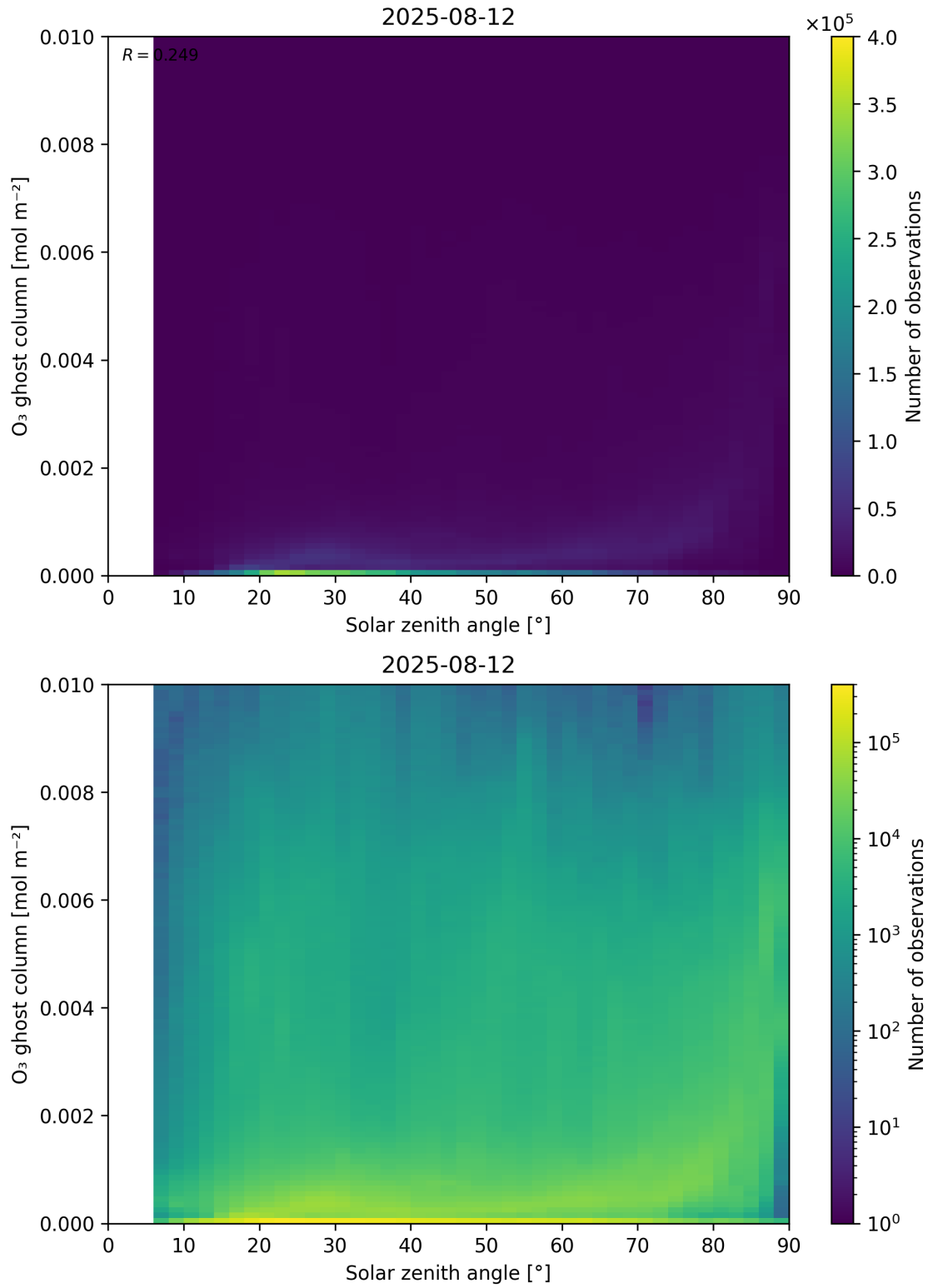
Figure 46: Scatter density plot of “Solar zenith angle” against “O 3 ghost column” for 2025-08-11 to 2025-08-13.
