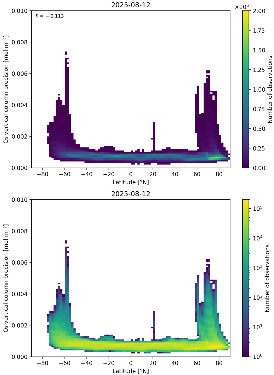
Figure 37: Scatter density plot of “Latitude” against “O 3 vertical column precision” for 2025-08-11 to 2025-08-13.
