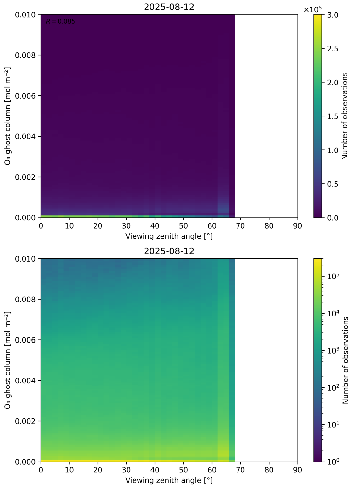
Figure 51: Scatter density plot of “Viewing zenith angle” against “O 3 ghost column” for 2025-08-11 to 2025-08-13.
