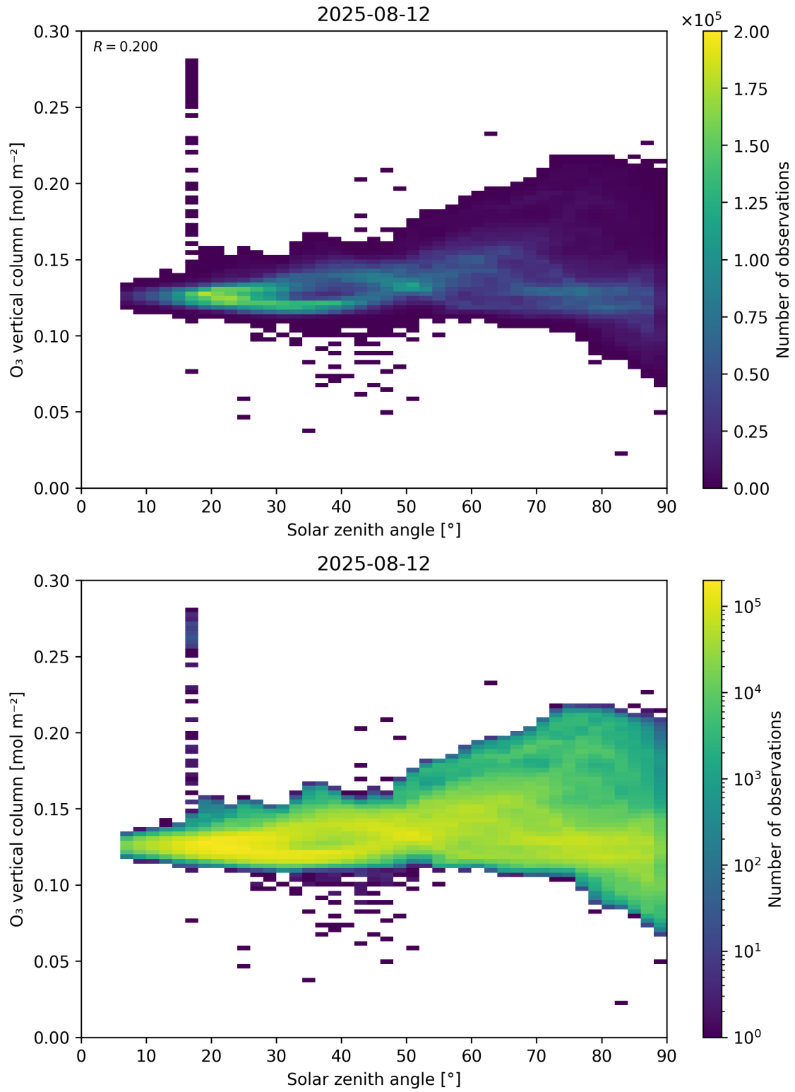
Figure 47: Scatter density plot of “Solar zenith angle” against “O 3 vertical column” for 2025-08-11 to 2025-08-13.
