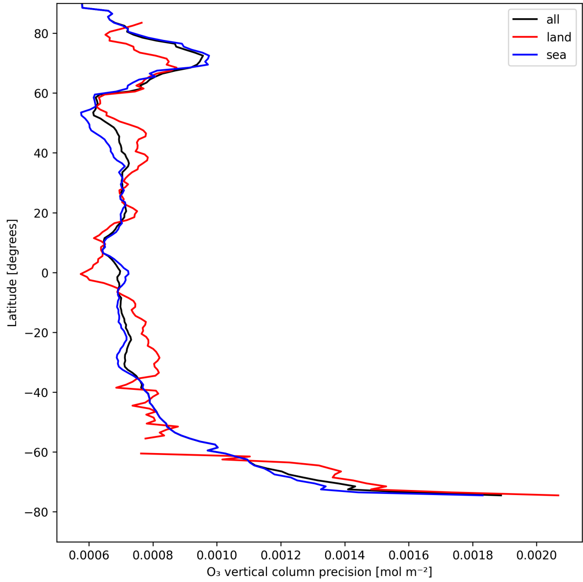
Figure 15: Zonal average of "O 3 vertical column precision" for 2025-08-11 to 2025-08-13.
