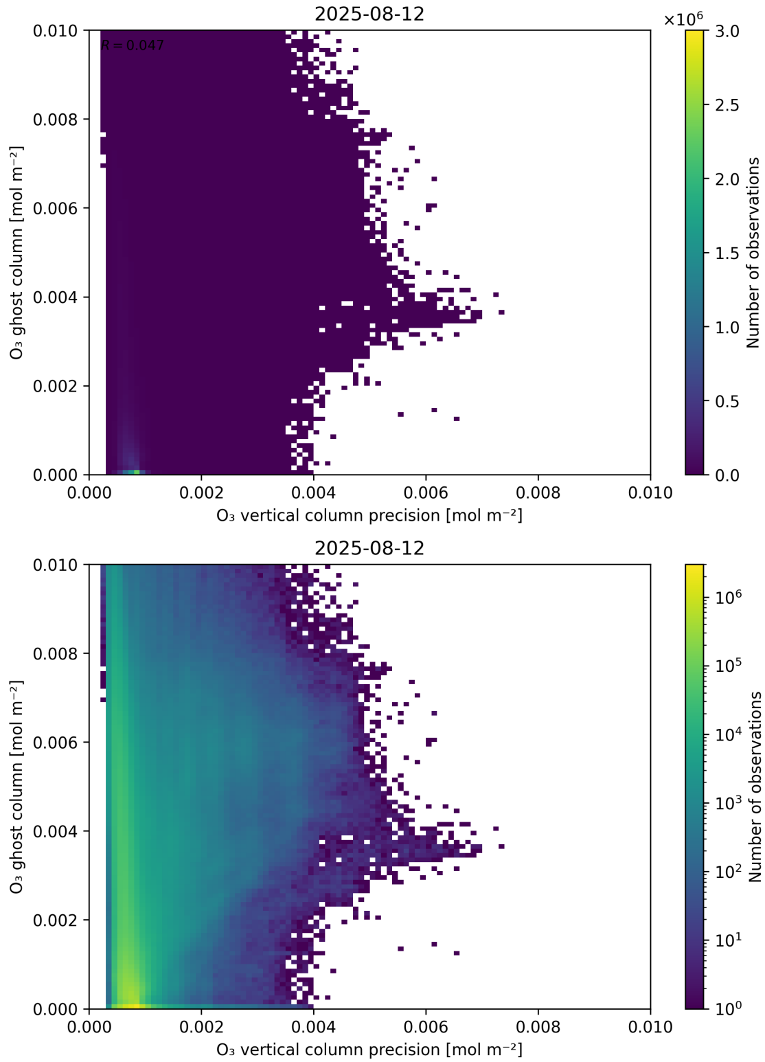
Figure 43: Scatter density plot of “ O_3 vertical column precision” against “ O_3 ghost column” for 2025-08-11 to 2025-08-13.
