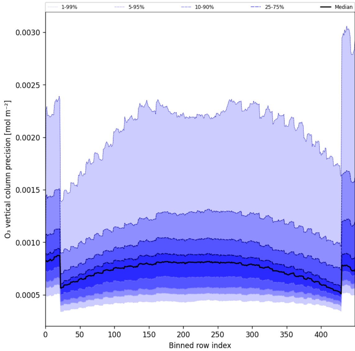
Figure 29: Along track statistics of “O 3 vertical column precision” for 2025-08-11 to 2025-08-13
