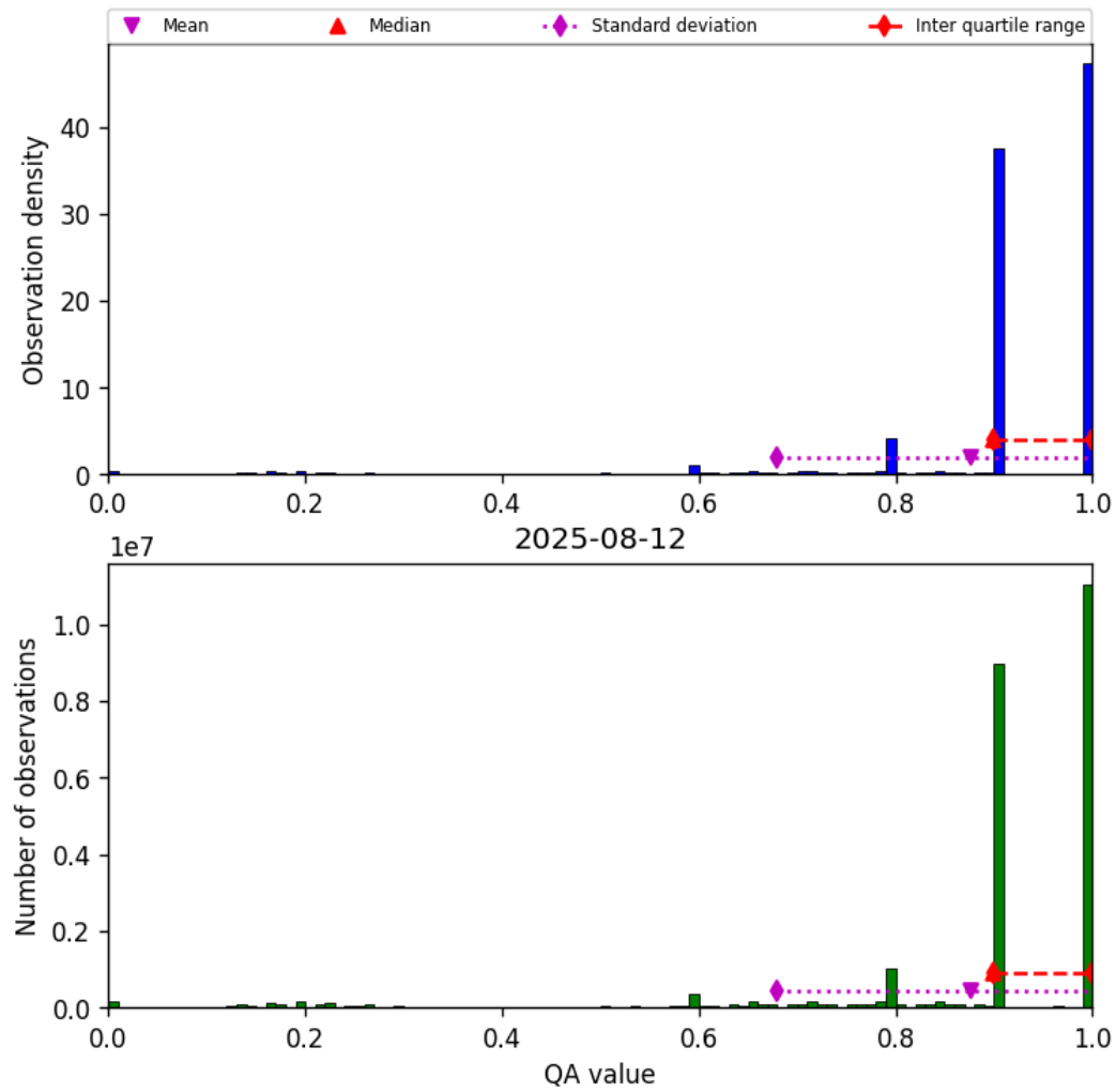
Figure 20: Histogram of “QA value” for 2025-08-11 to 2025-08-13
