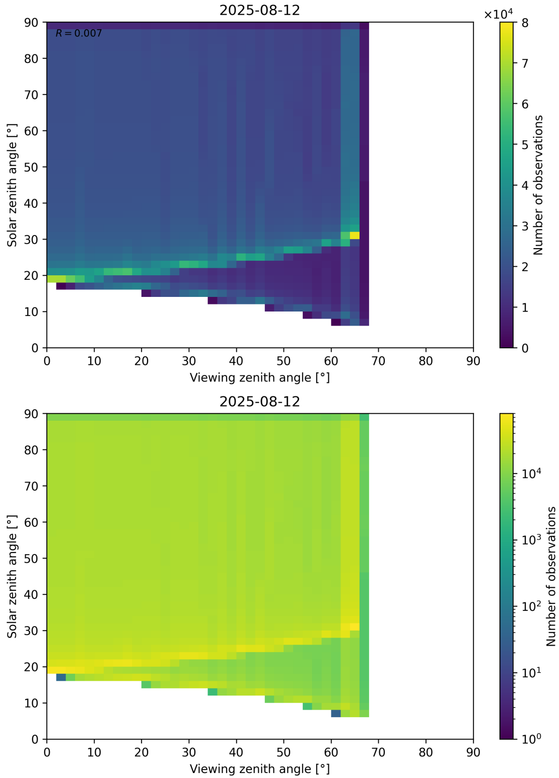
Figure 54: Scatter density plot of “Viewing zenith angle” against “Solar zenith angle” for 2025-08-11 to 2025-08-13.
