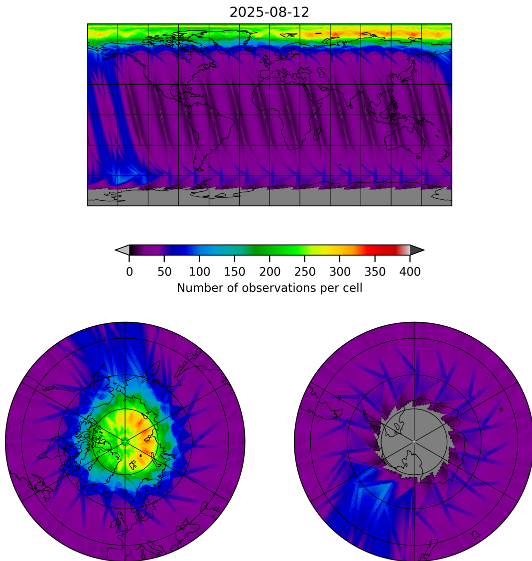
Figure 12: Map of the number of observations for 2025-08-11 to 2025-08-13
