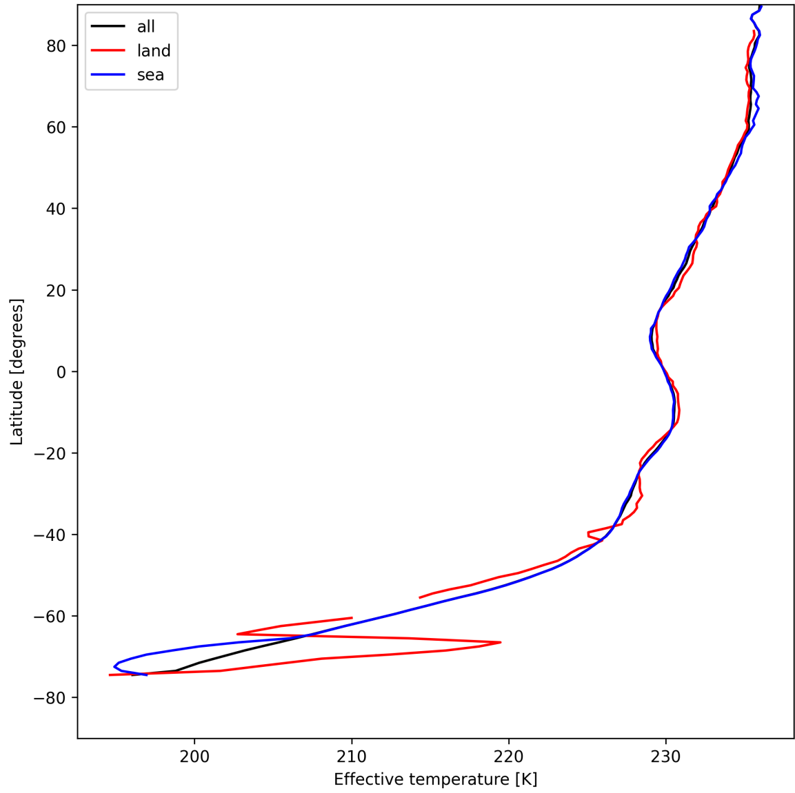
Figure 17: Zonal average of "Effective temperature" for 2025-08-11 to 2025-08-13.
