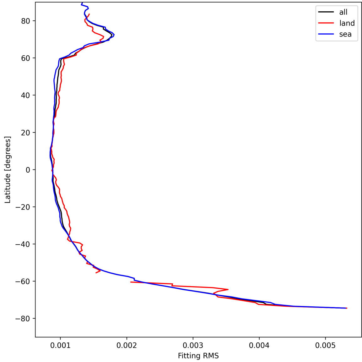
Figure 16: Zonal average of “Fitting RMS” for 2025-08-11 to 2025-08-13.
