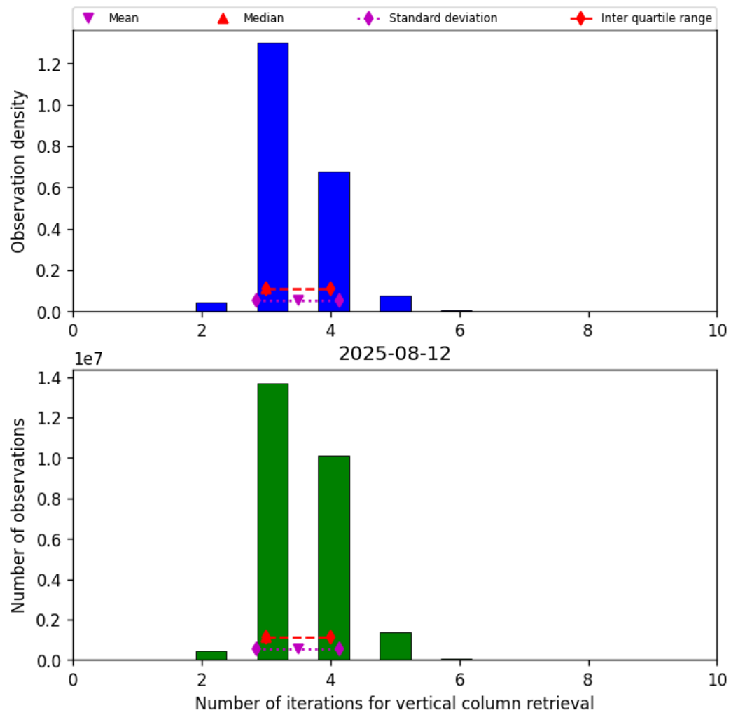
Figure 26: Histogram of “Number of iterations for vertical column retrieval” for 2025-08-11 to 2025-08-13
