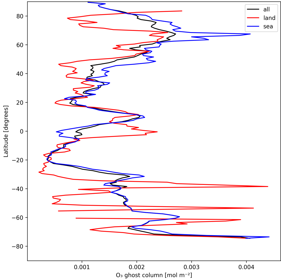
Figure 18: Zonal average of "O 3 ghost column" for 2025-08-11 to 2025-08-13.
