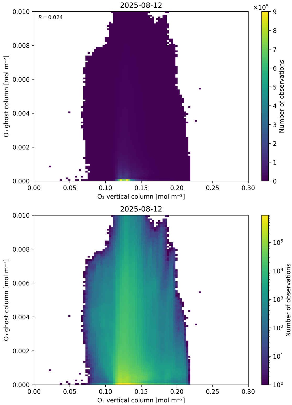
Figure 40: Scatter density plot of “O 3 vertical column” against “O 3 ghost column” for 2025-08-11 to 2025-08-13.
