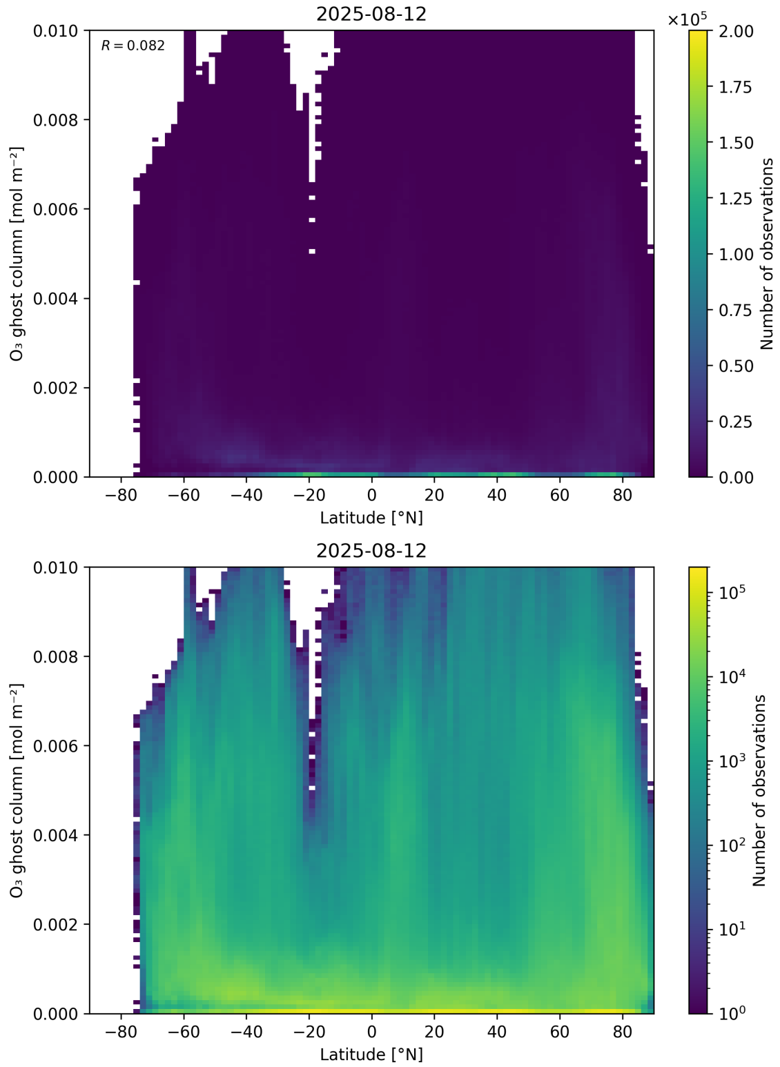
Figure 35: Scatter density plot of “Latitude” against “O 3 ghost column” for 2025-08-11 to 2025-08-13.
