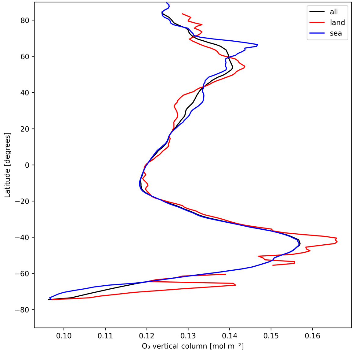
Figure 14: Zonal average of “O 3 vertical column” for 2025-08-11 to 2025-08-13.
