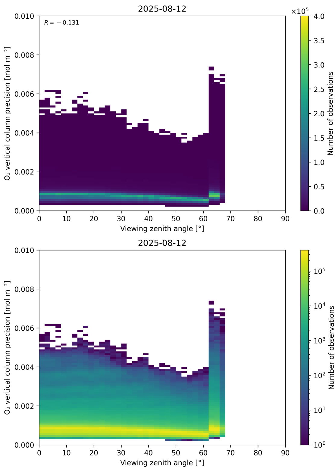
Figure 53: Scatter density plot of “Viewing zenith angle” against “O 3 vertical column precision” for 2025-08-11 to 2025-08-13.
