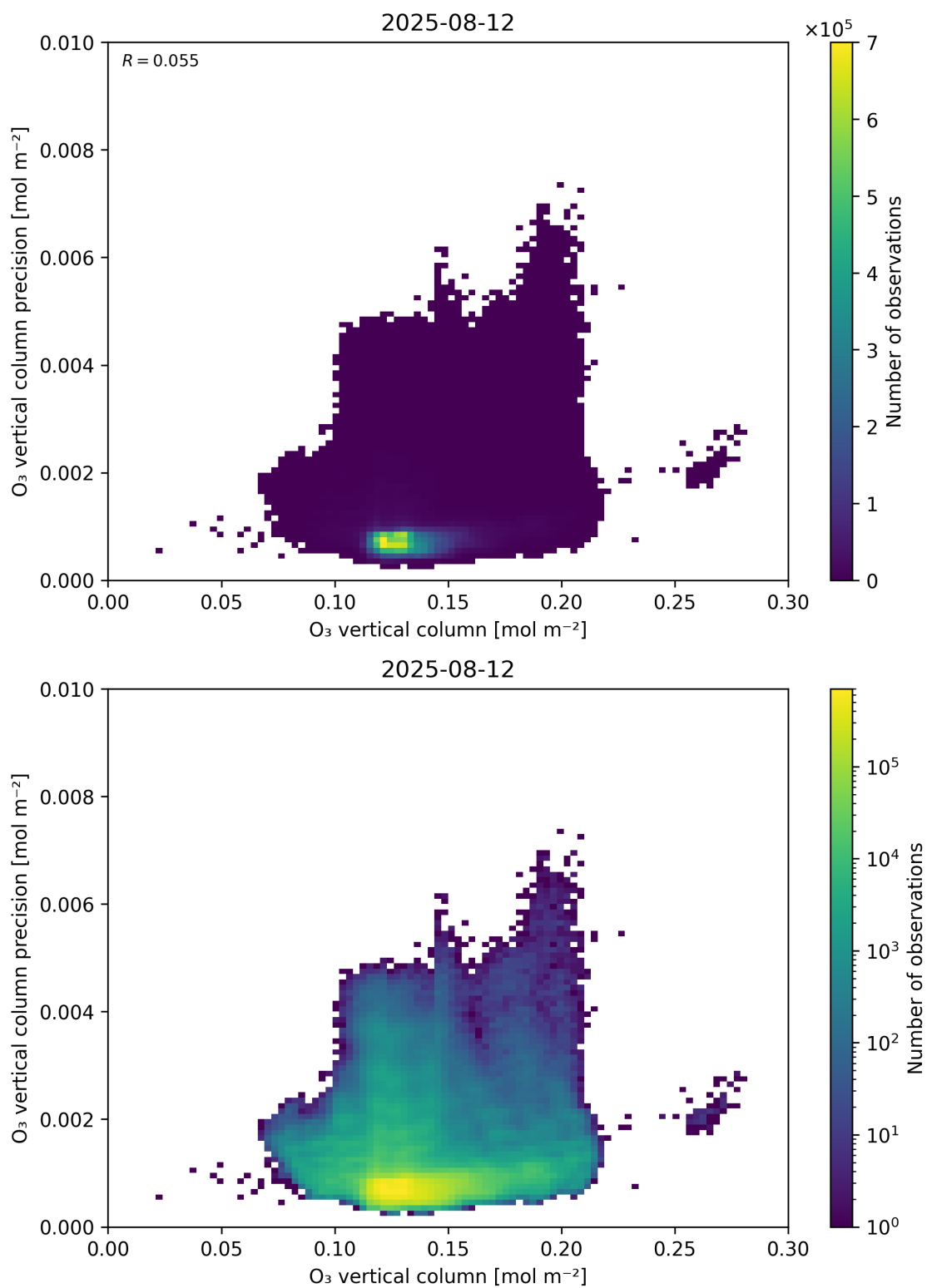
Figure 41: Scatter density plot of “O 3 vertical column” against “O 3 vertical column precision” for 2025-08-11 to 2025-08-13.
