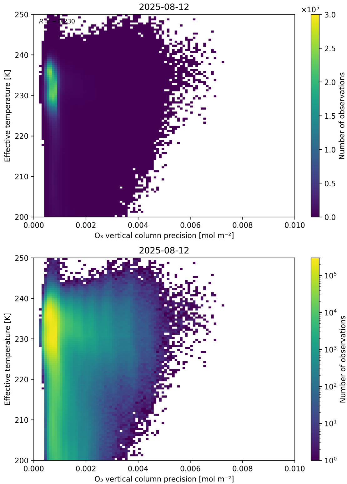
Figure 42: Scatter density plot of “O 3 vertical column precision” against “Effective temperature” for 2025-08-11 to 2025-08-13.
