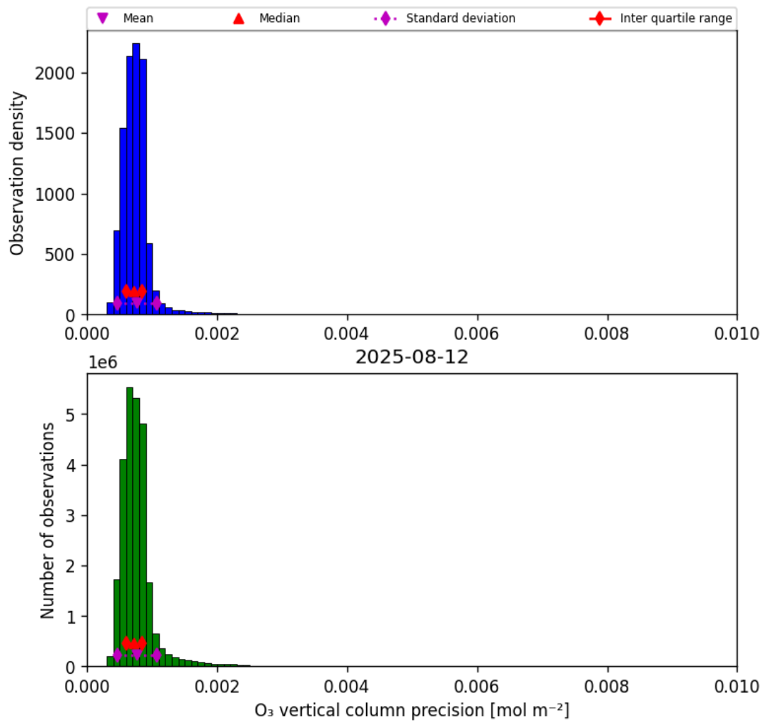
Figure 22: Histogram of “O 3 vertical column precision” for 2025-08-11 to 2025-08-13
