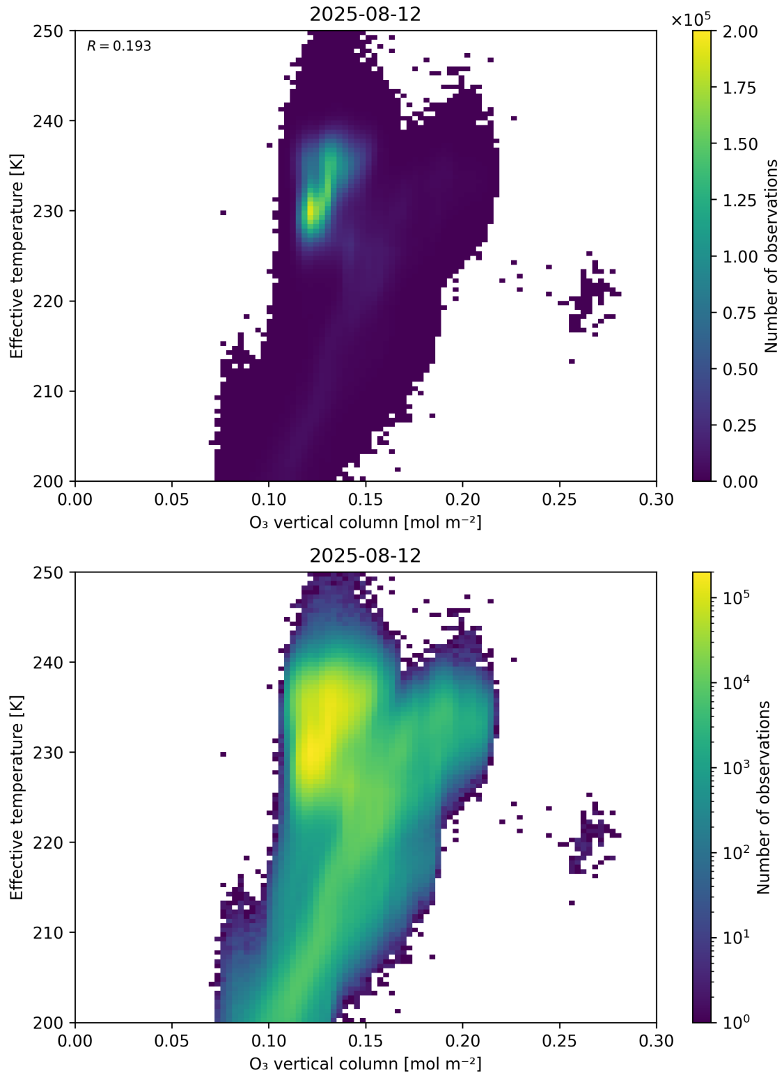
Figure 39: Scatter density plot of “O 3 vertical column” against “Effective temperature” for 2025-08-11 to 2025-08-13.
