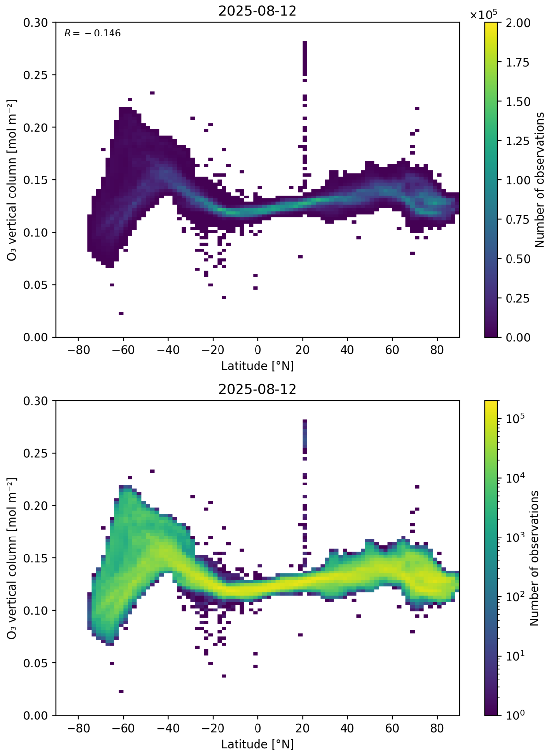
Figure 36: Scatter density plot of “Latitude” against “O 3 vertical column” for 2025-08-11 to 2025-08-13.
