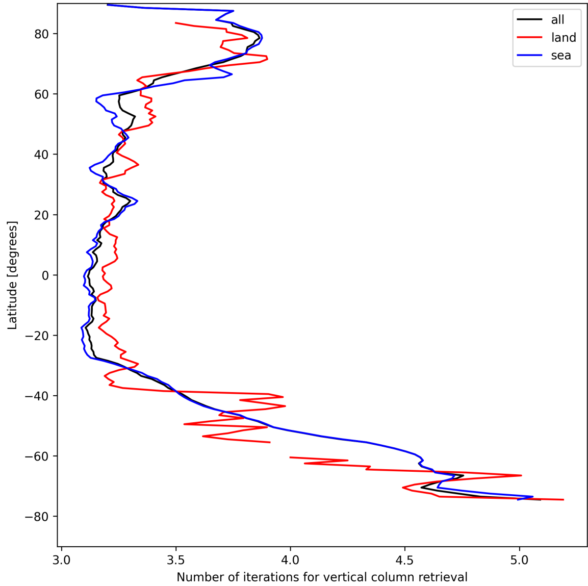
Figure 19: Zonal average of “Number of iterations for vertical column retrieval” for 2025-08-11 to 2025-08-13.
