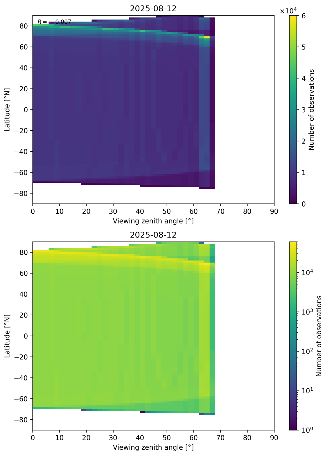
Figure 49: Scatter density plot of “Viewing zenith angle” against “Latitude” for 2025-08-11 to 2025-08-13.
