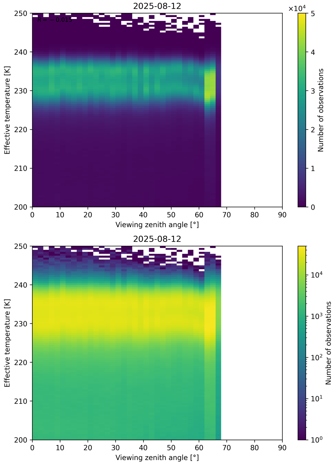
Figure 50: Scatter density plot of “Viewing zenith angle” against “Effective temperature” for 2025-08-11 to 2025-08-13.
