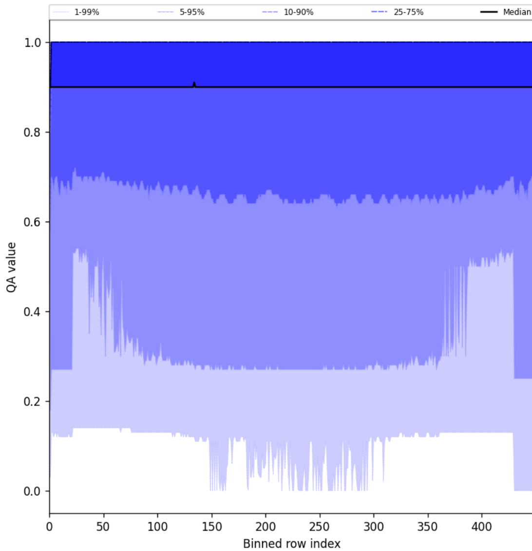
Figure 27: Along track statistics of “QA value” for 2025-08-11 to 2025-08-13
