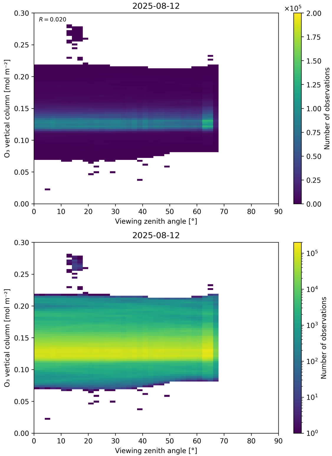
Figure 52: Scatter density plot of “Viewing zenith angle” against “O 3 vertical column” for 2025-08-11 to 2025-08-13.
