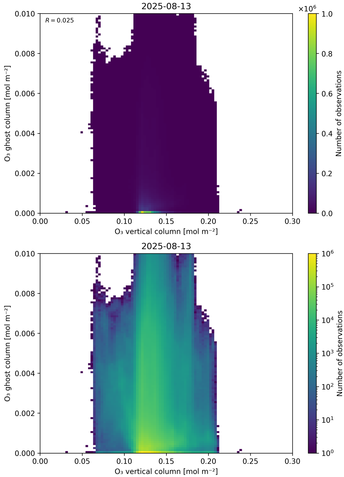
Figure 40: Scatter density plot of “O 3 vertical column” against “O 3 ghost column” for 2025-08-12 to 2025-08-14.
