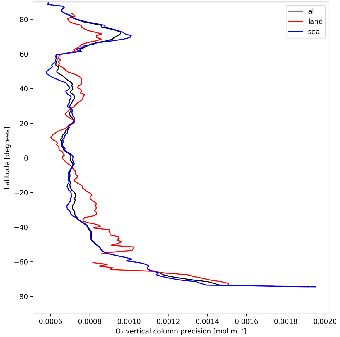
Figure 15: Zonal average of “O 3 vertical column precision” for 2025-08-12 to 2025-08-14.
