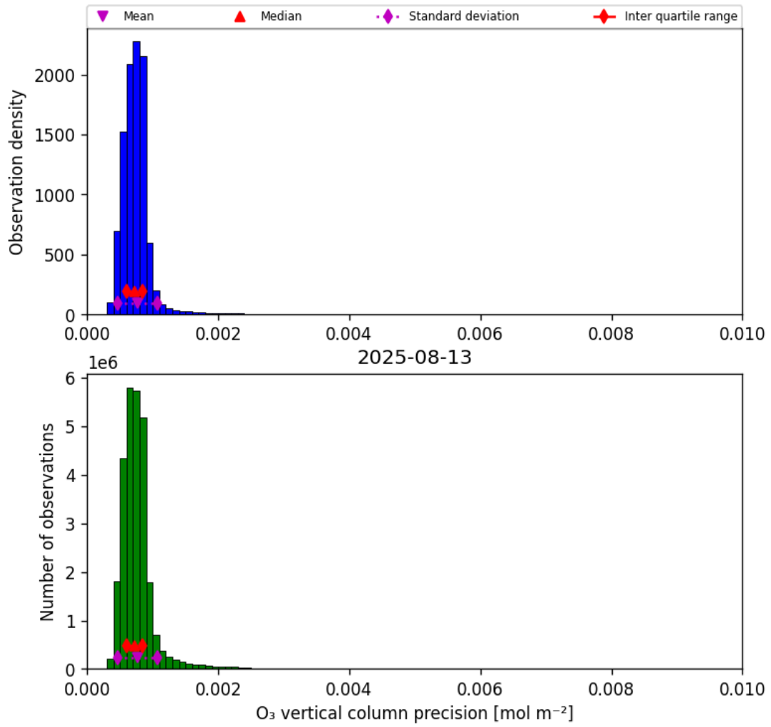
Figure 22: Histogram of “O 3 vertical column precision” for 2025-08-12 to 2025-08-14
