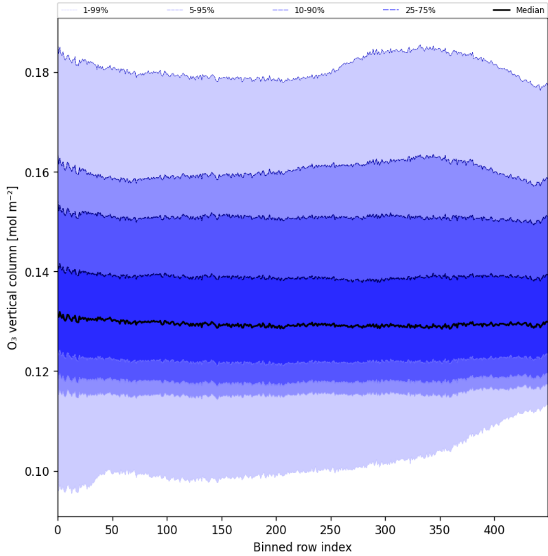
Figure 28: Along track statistics of “O 3 vertical column” for 2025-08-12 to 2025-08-14
