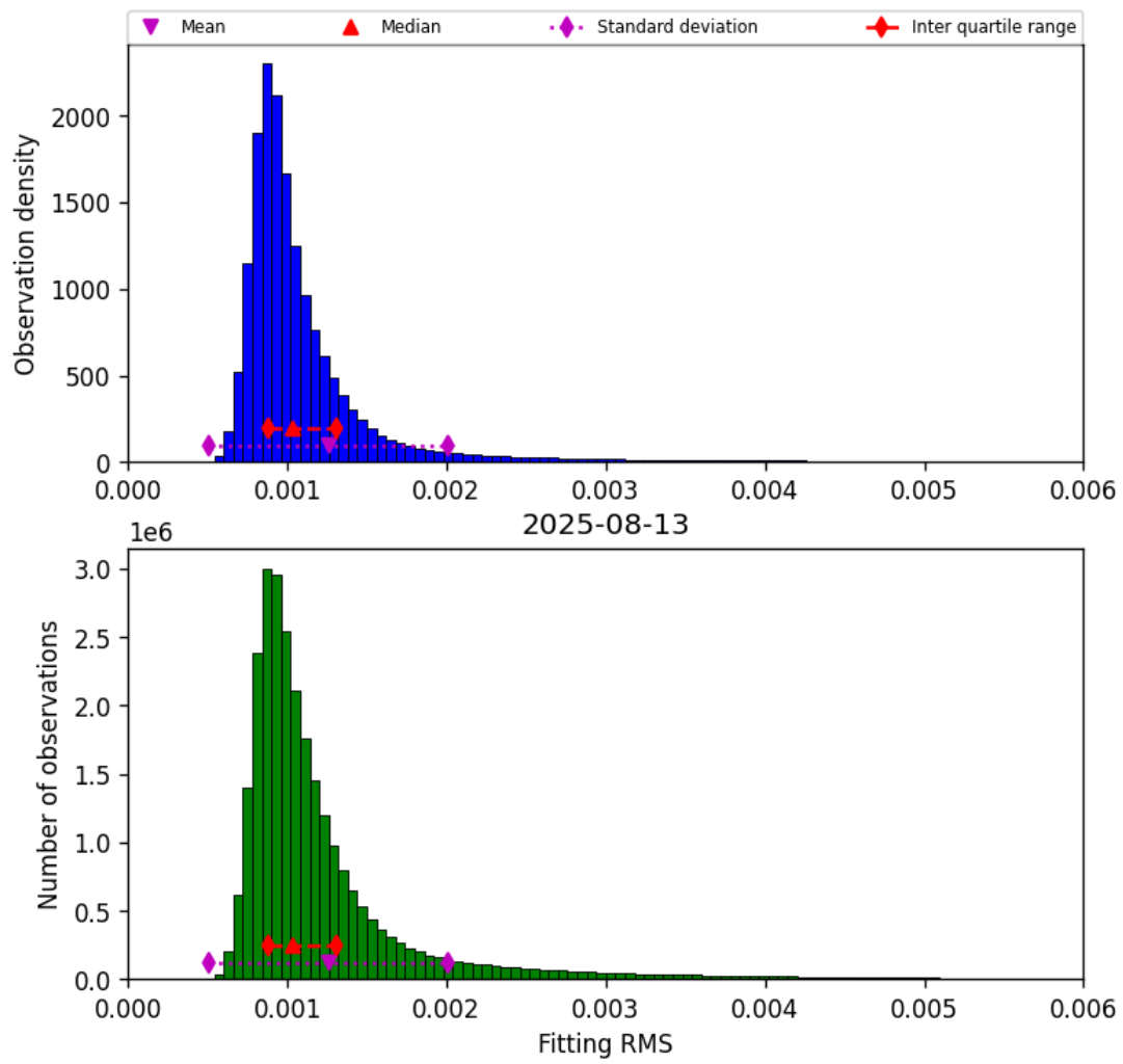
Figure 23: Histogram of “Fitting RMS” for 2025-08-12 to 2025-08-14
