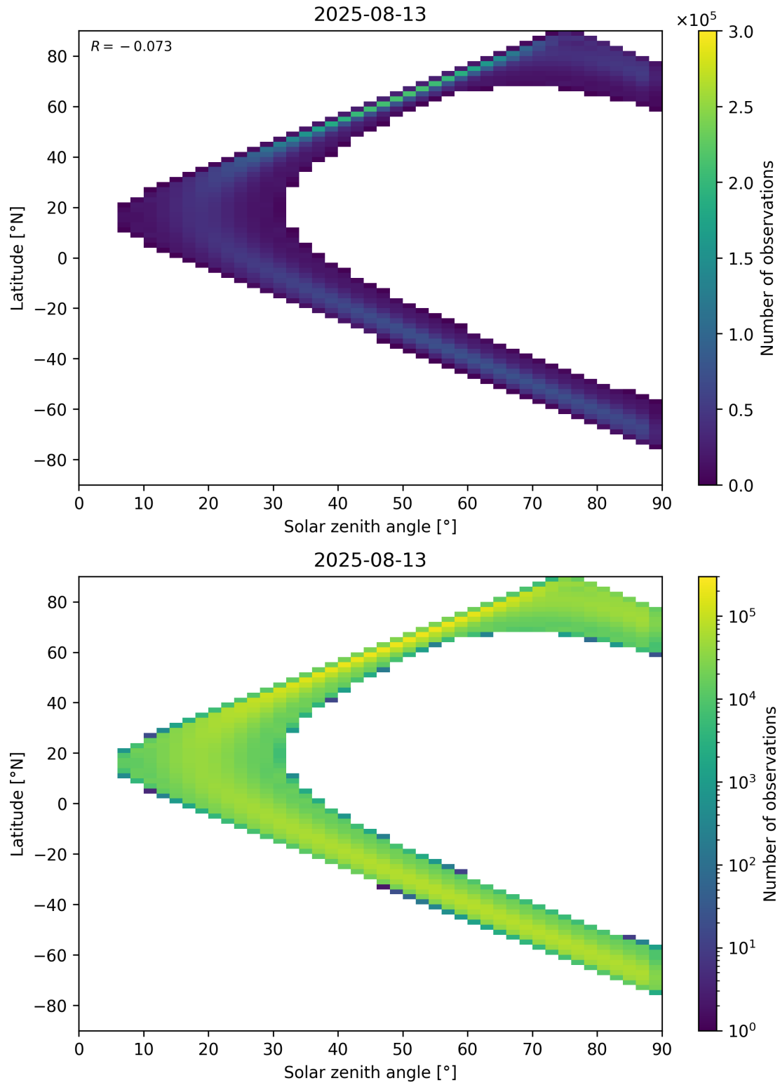
Figure 44: Scatter density plot of “Solar zenith angle” against “Latitude” for 2025-08-12 to 2025-08-14.
