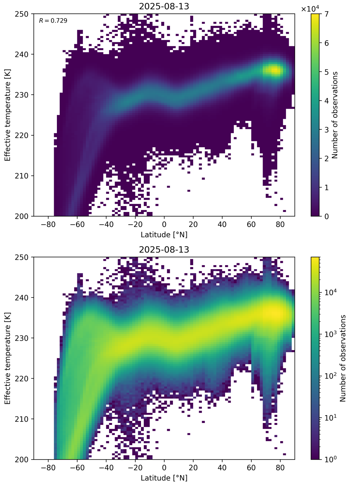
Figure 34: Scatter density plot of “Latitude” against “Effective temperature” for 2025-08-12 to 2025-08-14.
