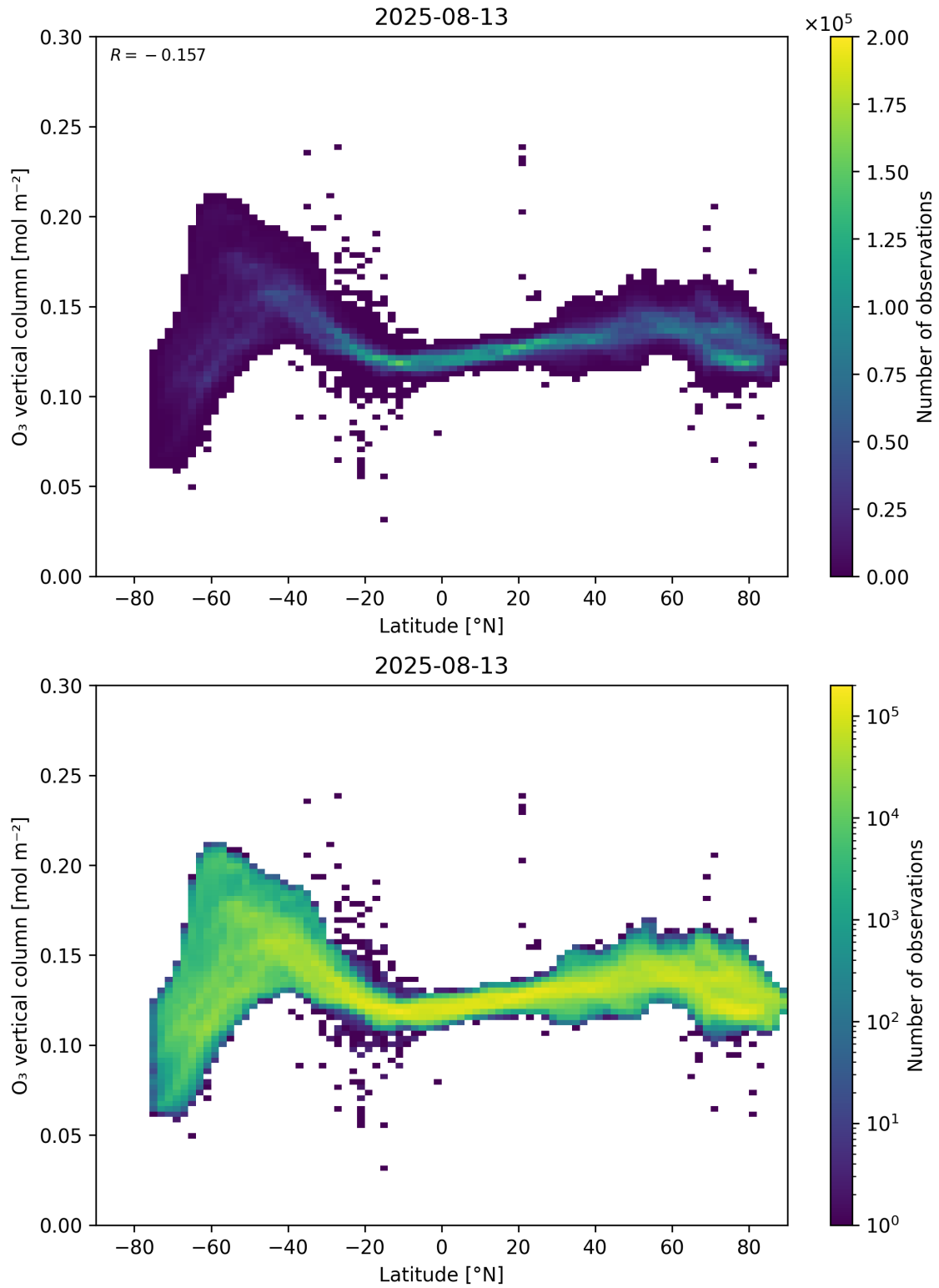
Figure 36: Scatter density plot of “Latitude” against “O 3 vertical column” for 2025-08-12 to 2025-08-14.
