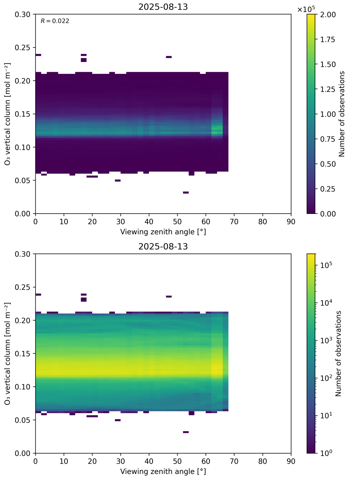
Figure 52: Scatter density plot of “Viewing zenith angle” against “O 3 vertical column” for 2025-08-12 to 2025-08-14.
