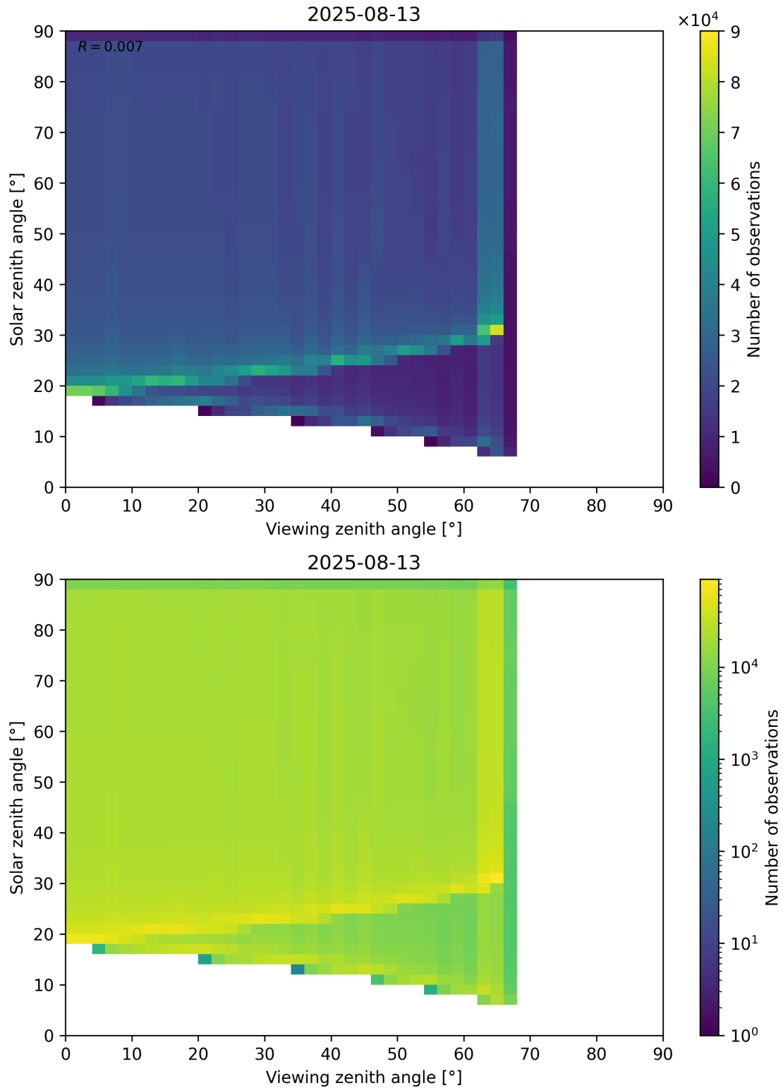
Figure 54: Scatter density plot of “Viewing zenith angle” against “Solar zenith angle” for 2025-08-12 to 2025-08-14.
