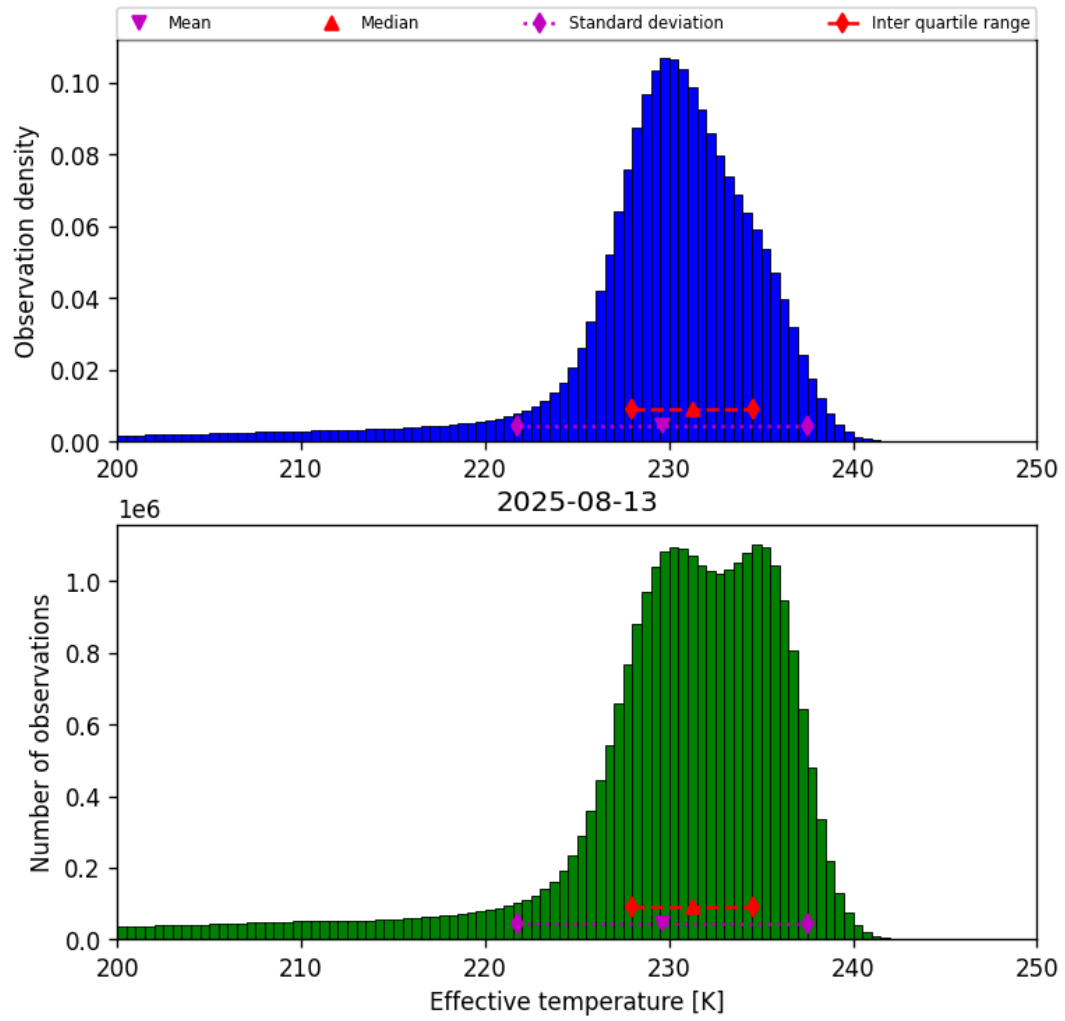
Figure 24: Histogram of “Effective temperature” for 2025-08-12 to 2025-08-14
