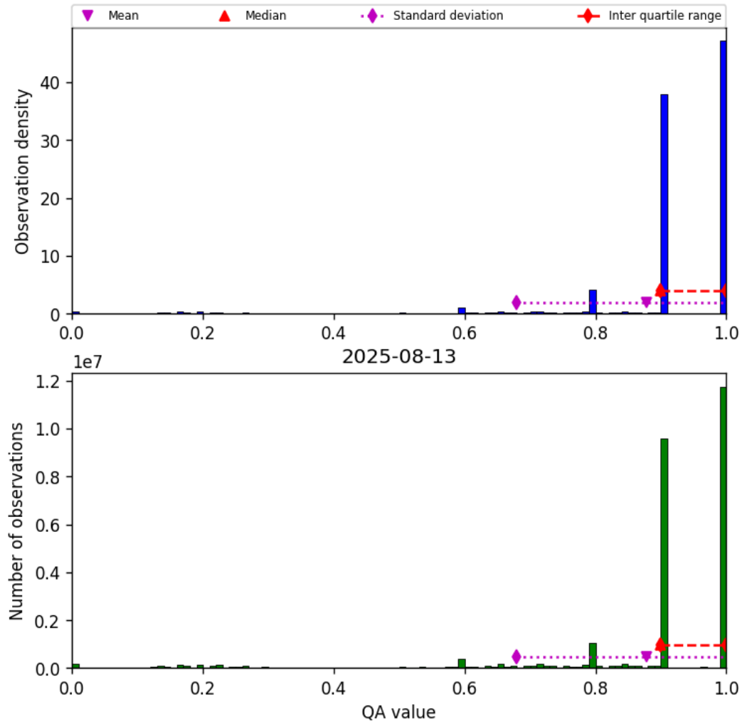
Figure 20: Histogram of “QA value” for 2025-08-12 to 2025-08-14
