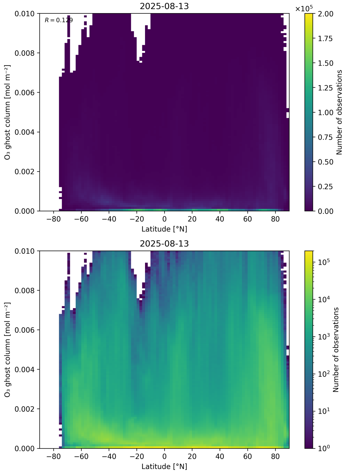
Figure 35: Scatter density plot of “Latitude” against “O 3 ghost column” for 2025-08-12 to 2025-08-14.
