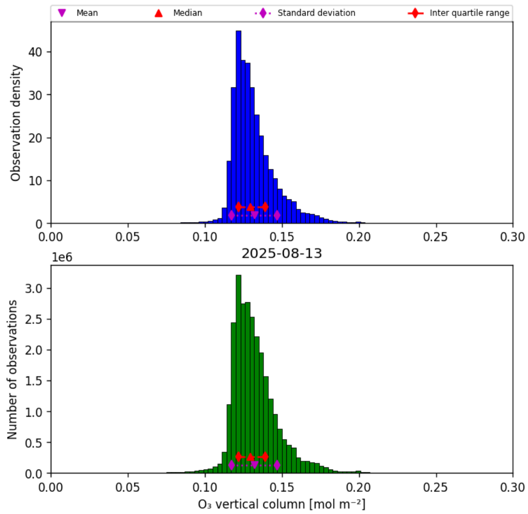
Figure 21: Histogram of “O 3 vertical column” for 2025-08-12 to 2025-08-14
