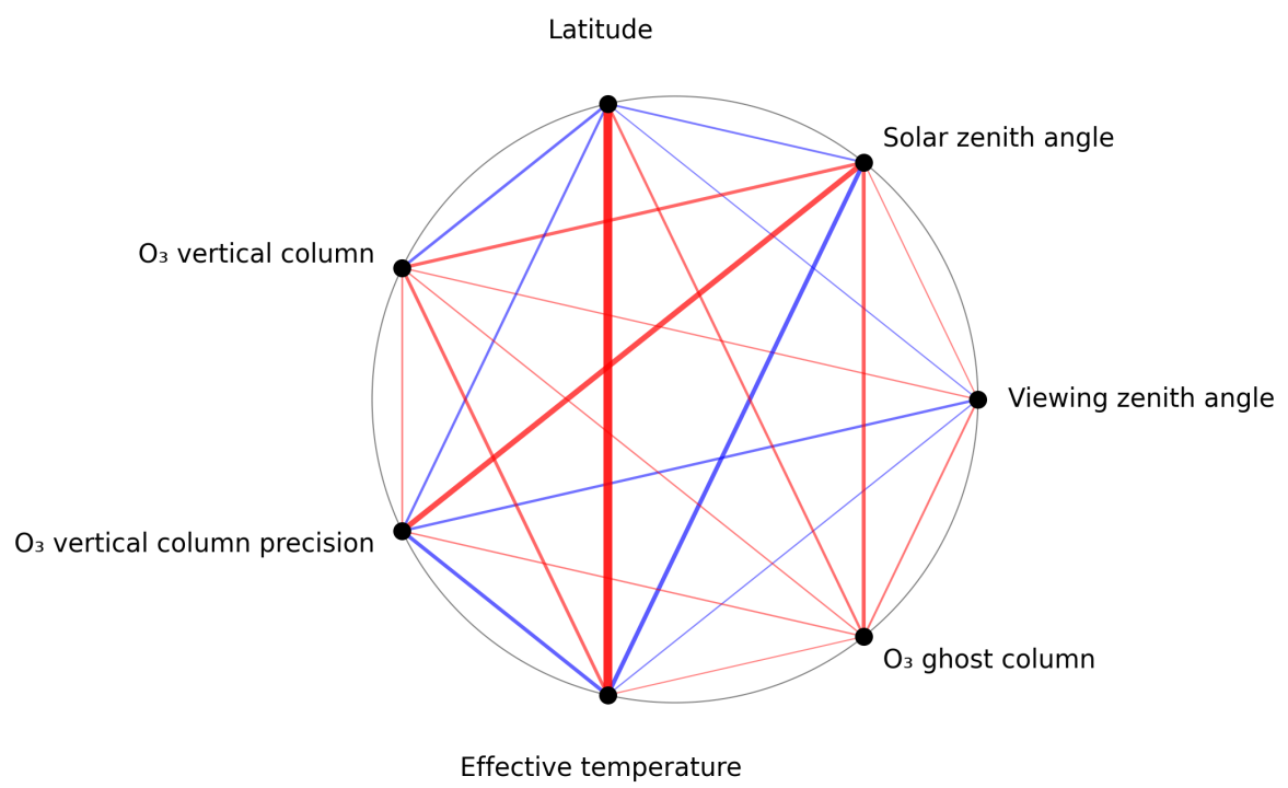
Figure 1: Map of correlation graph for 2025-08-12 to 2025-08-14.
