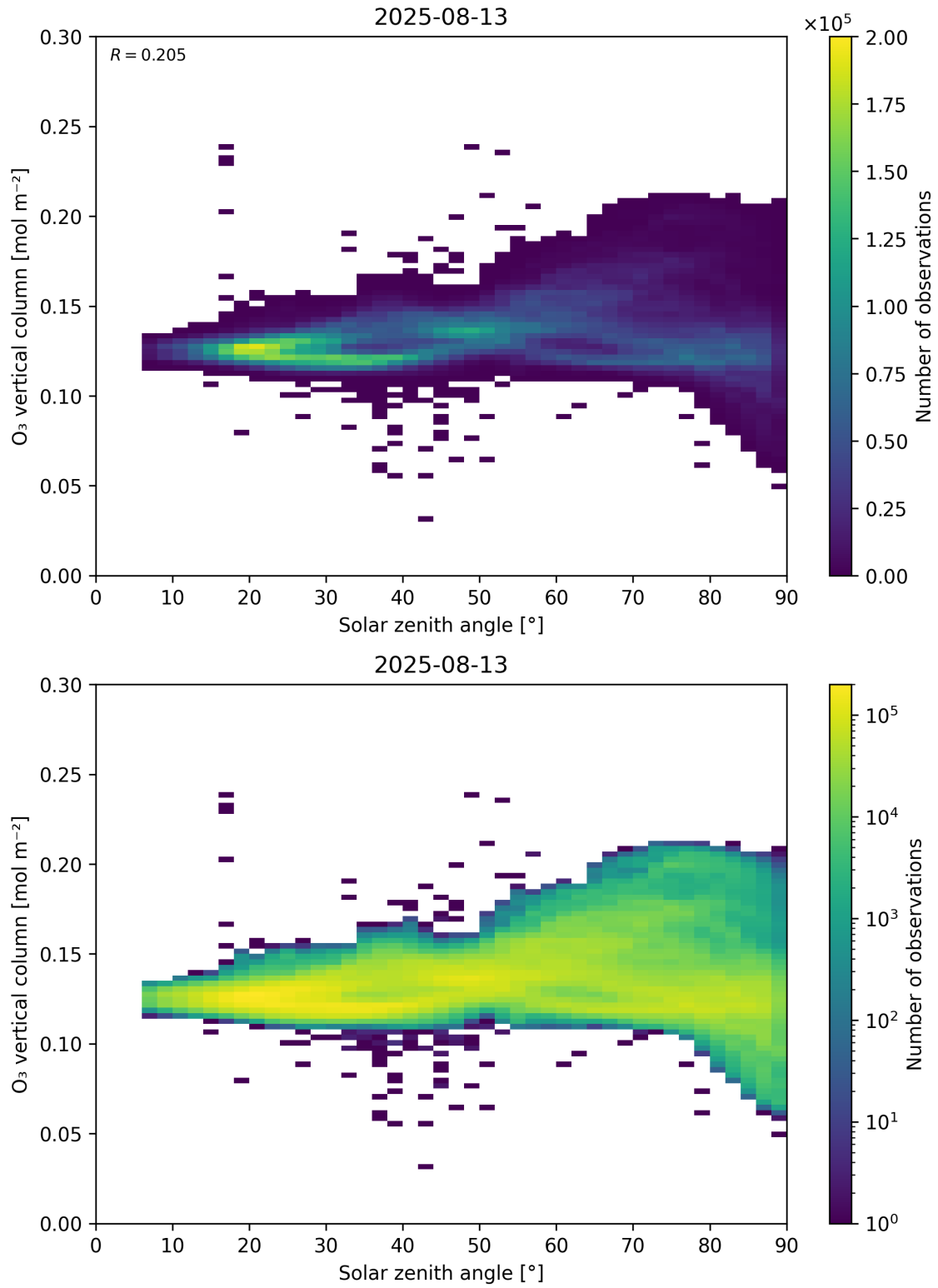
Figure 47: Scatter density plot of “Solar zenith angle” against “O 3 vertical column” for 2025-08-12 to 2025-08-14.
