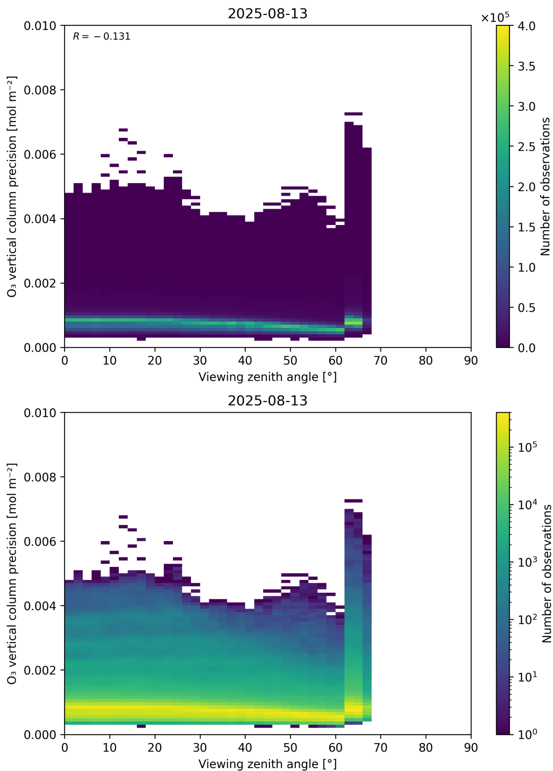
Figure 53: Scatter density plot of “Viewing zenith angle” against “O 3 vertical column precision” for 2025-08-12 to 2025-08-14.
