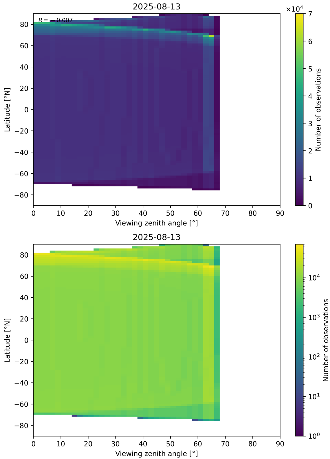
Figure 49: Scatter density plot of “Viewing zenith angle” against “Latitude” for 2025-08-12 to 2025-08-14.
