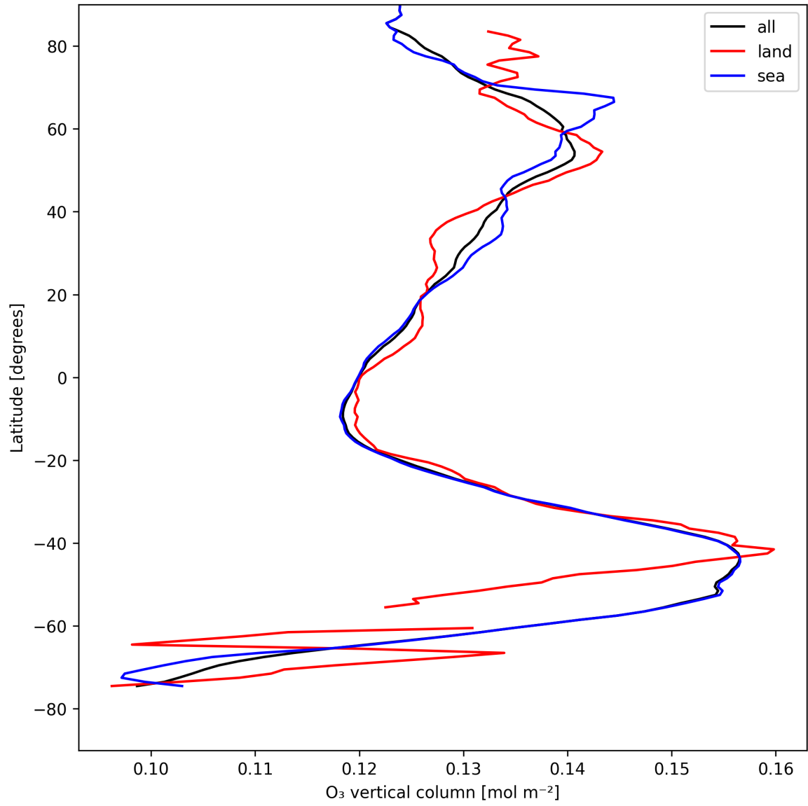
Figure 14: Zonal average of “O 3 vertical column” for 2025-08-12 to 2025-08-14.
