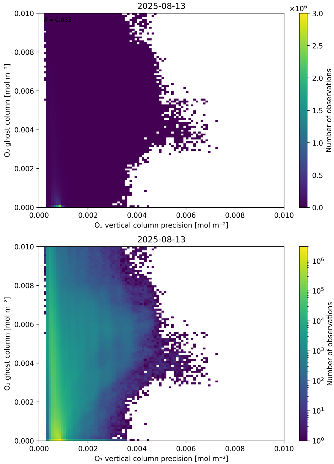
Figure 43: Scatter density plot of “ \text{O}_3 vertical column precision” against “ \text{O}_3 ghost column” for 2025-08-12 to 2025-08-14.
