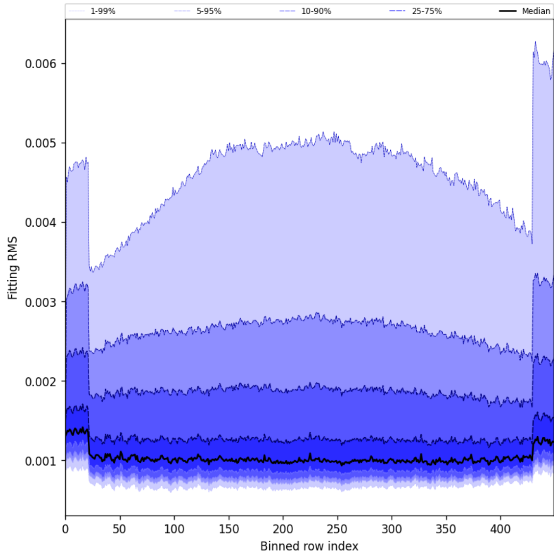
Figure 30: Along track statistics of “Fitting RMS” for 2025-08-12 to 2025-08-14
