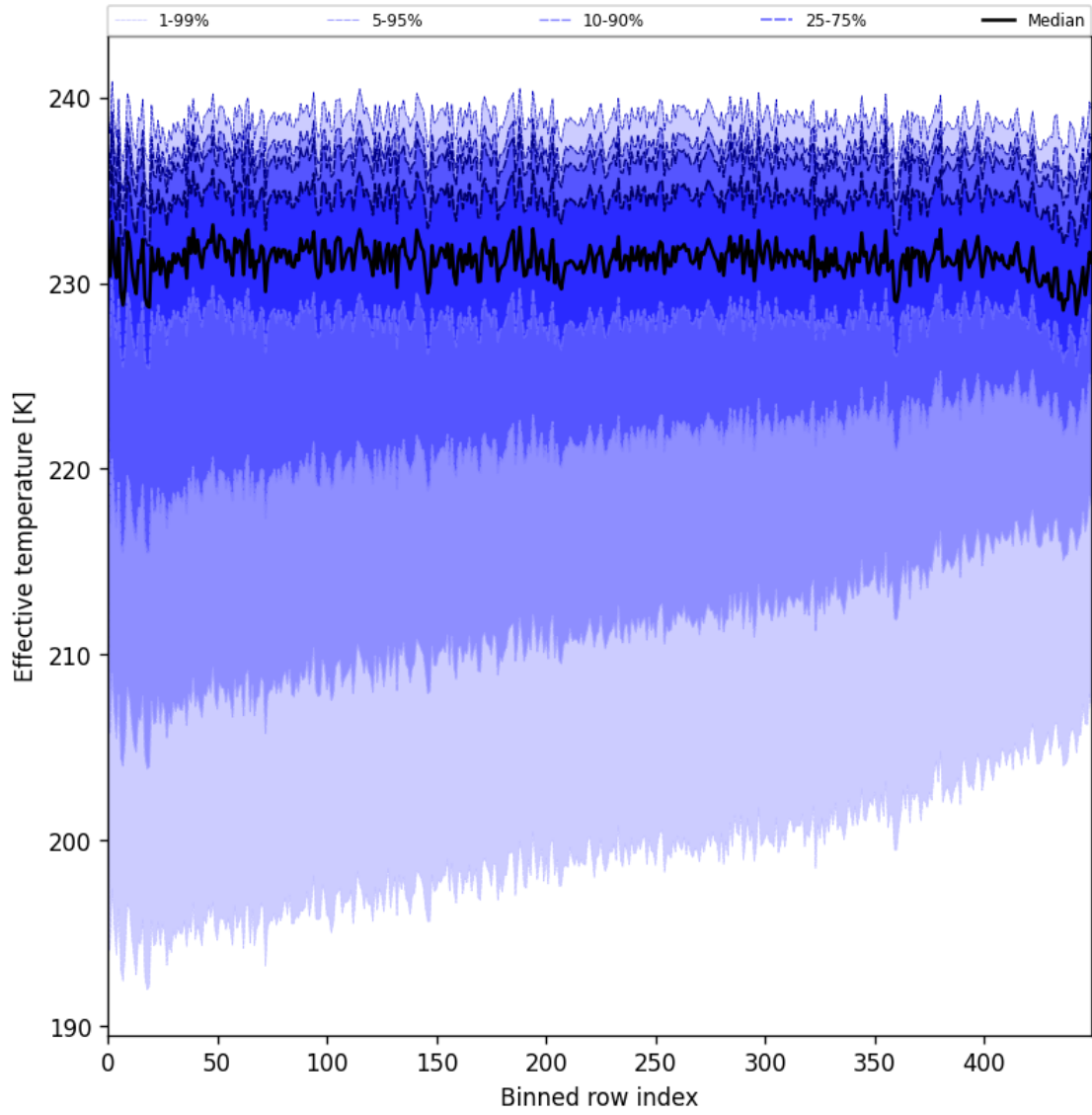
Figure 31: Along track statistics of “Effective temperature” for 2025-08-12 to 2025-08-14
