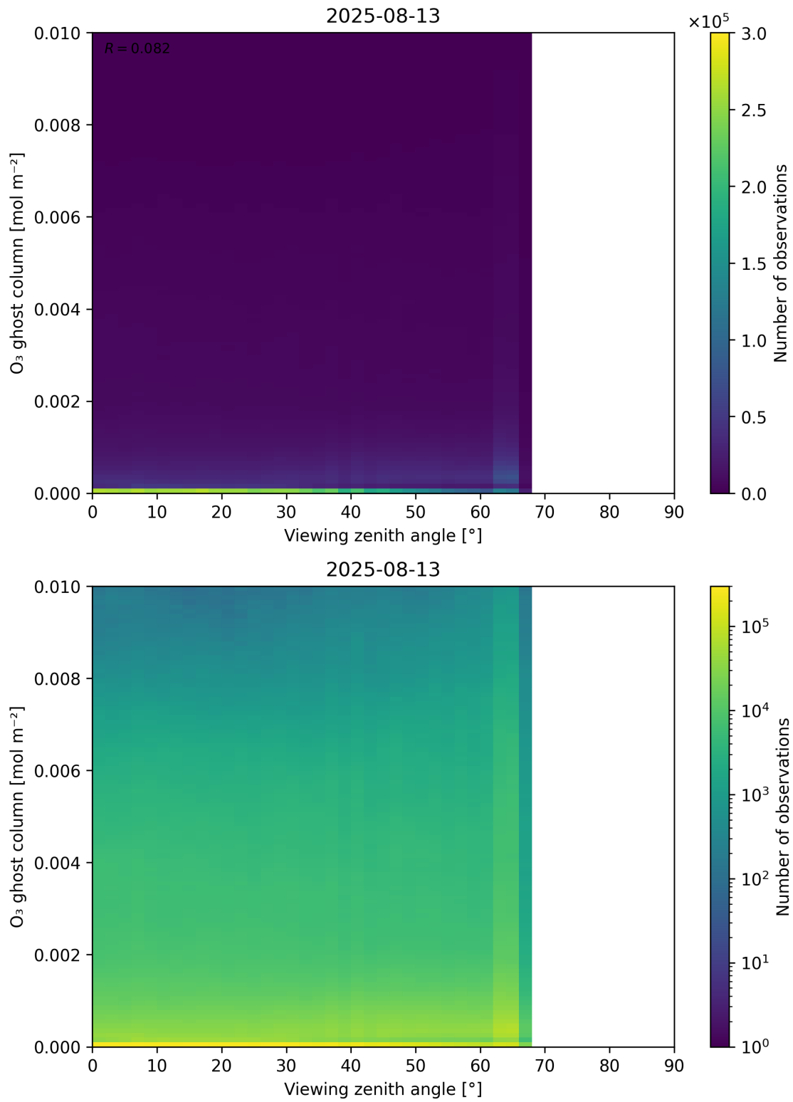
Figure 51: Scatter density plot of “Viewing zenith angle” against “O 3 ghost column” for 2025-08-12 to 2025-08-14.
