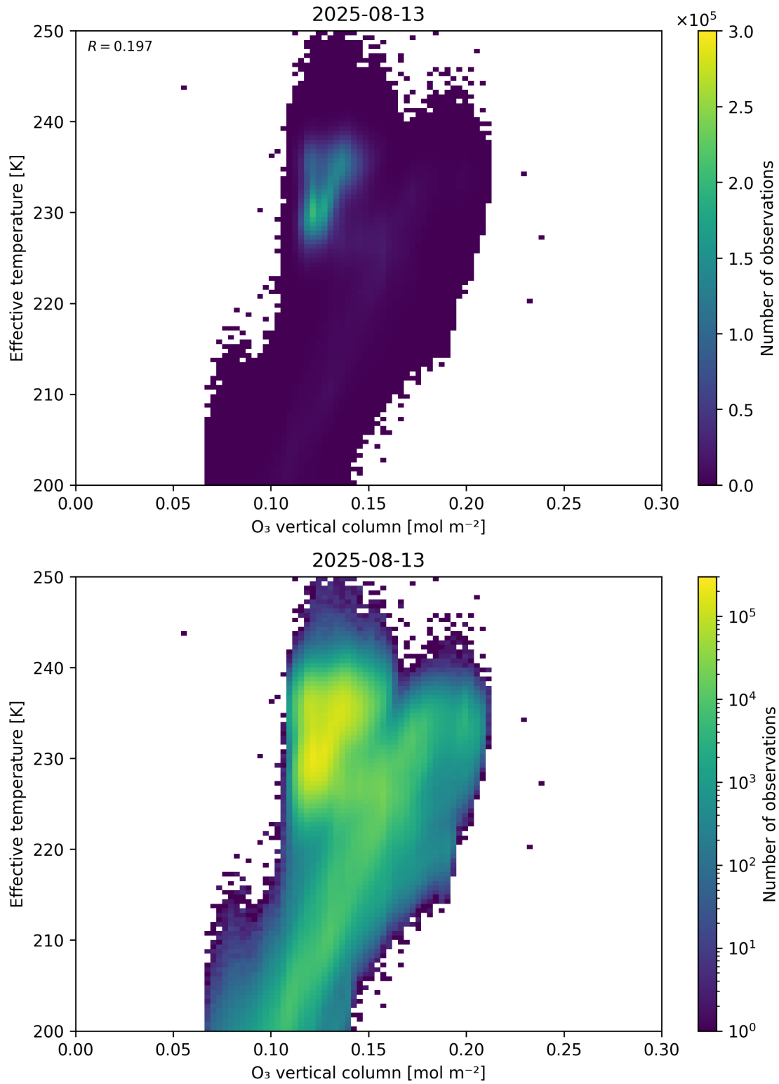
Figure 39: Scatter density plot of “O 3 vertical column” against “Effective temperature” for 2025-08-12 to 2025-08-14.
