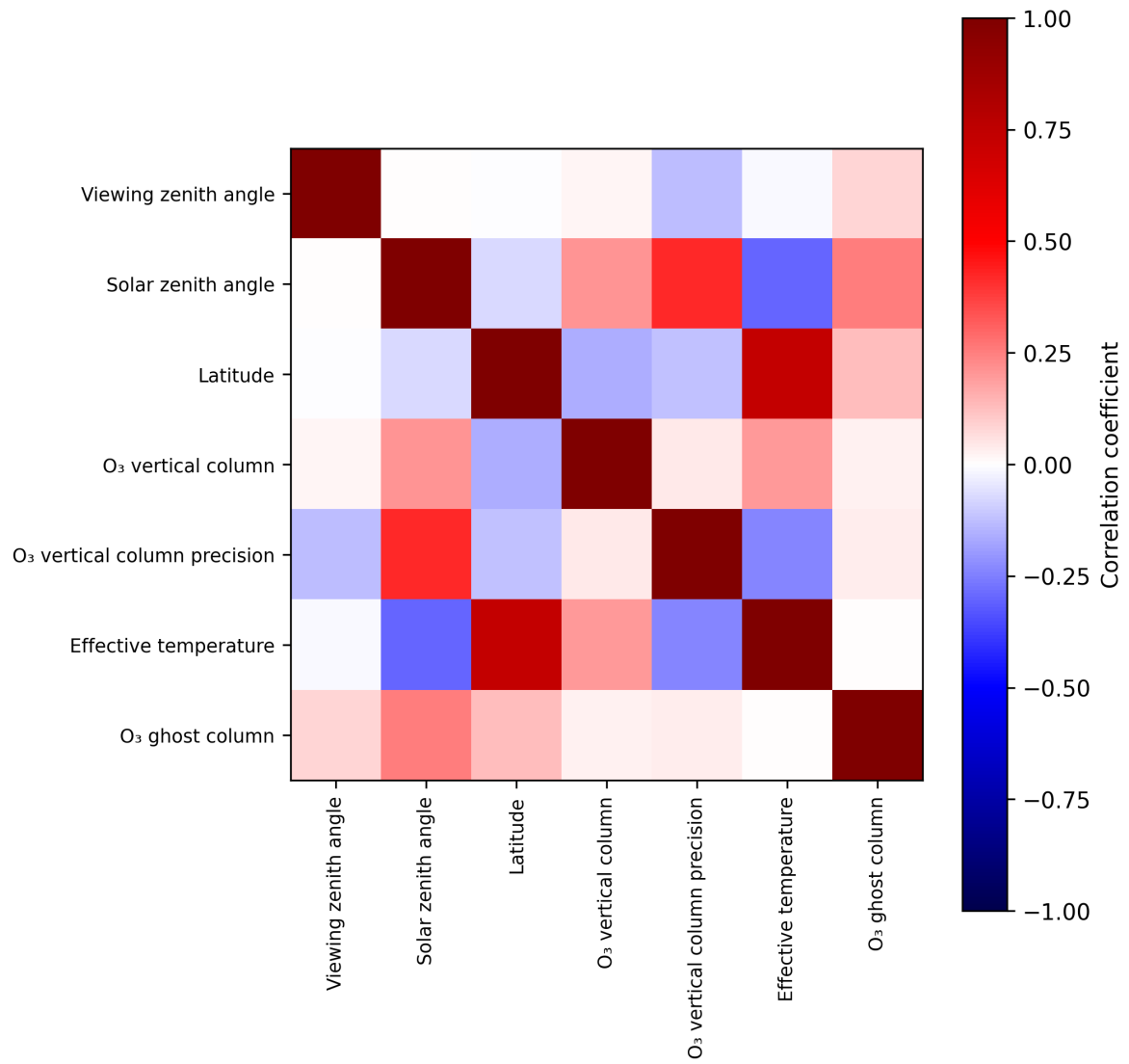
Figure 2: Map of correlation matrix for 2025-08-12 to 2025-08-14.
