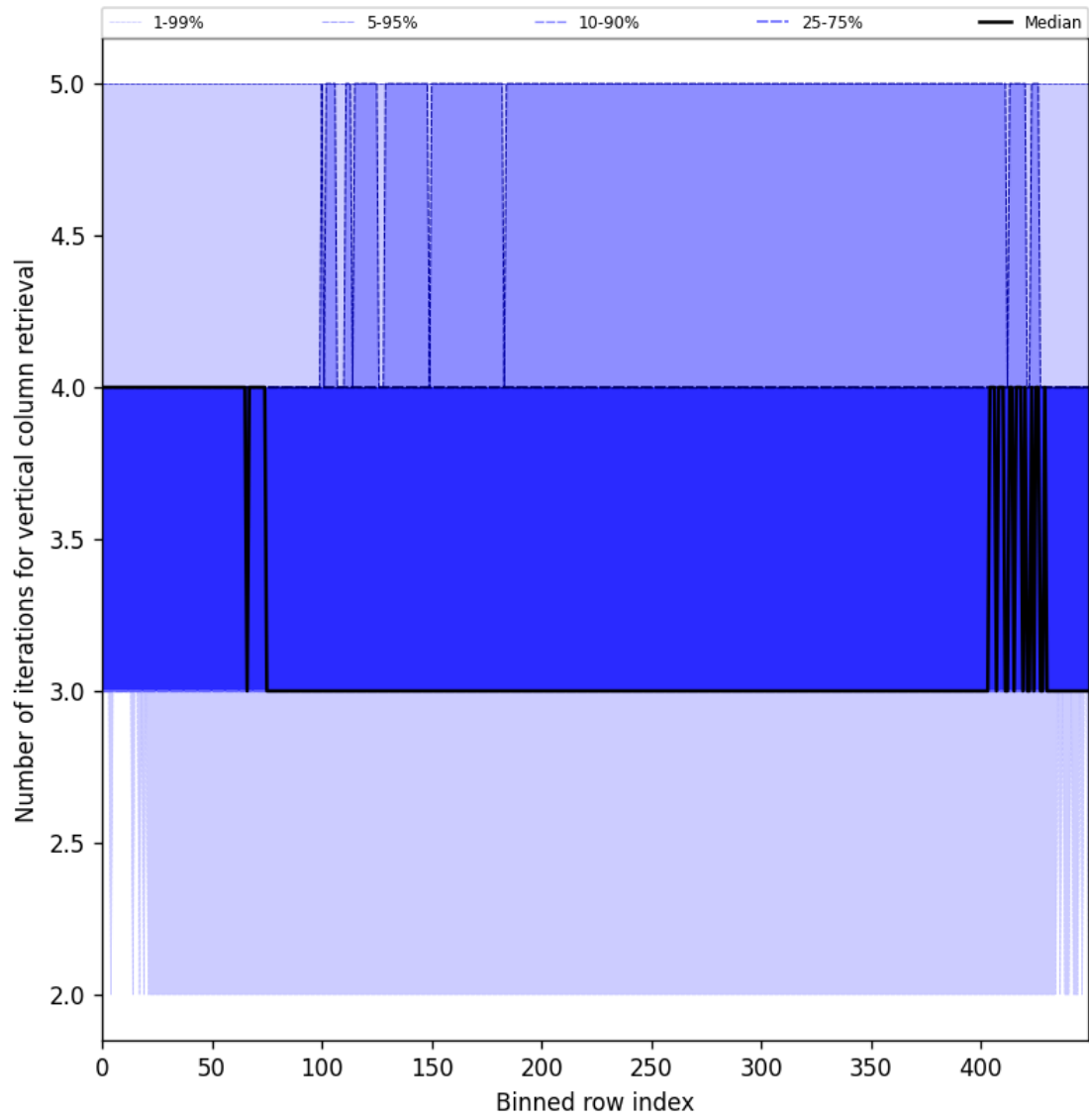
Figure 33: Along track statistics of “Number of iterations for vertical column retrieval” for 2025-08-12 to 2025-08-14
