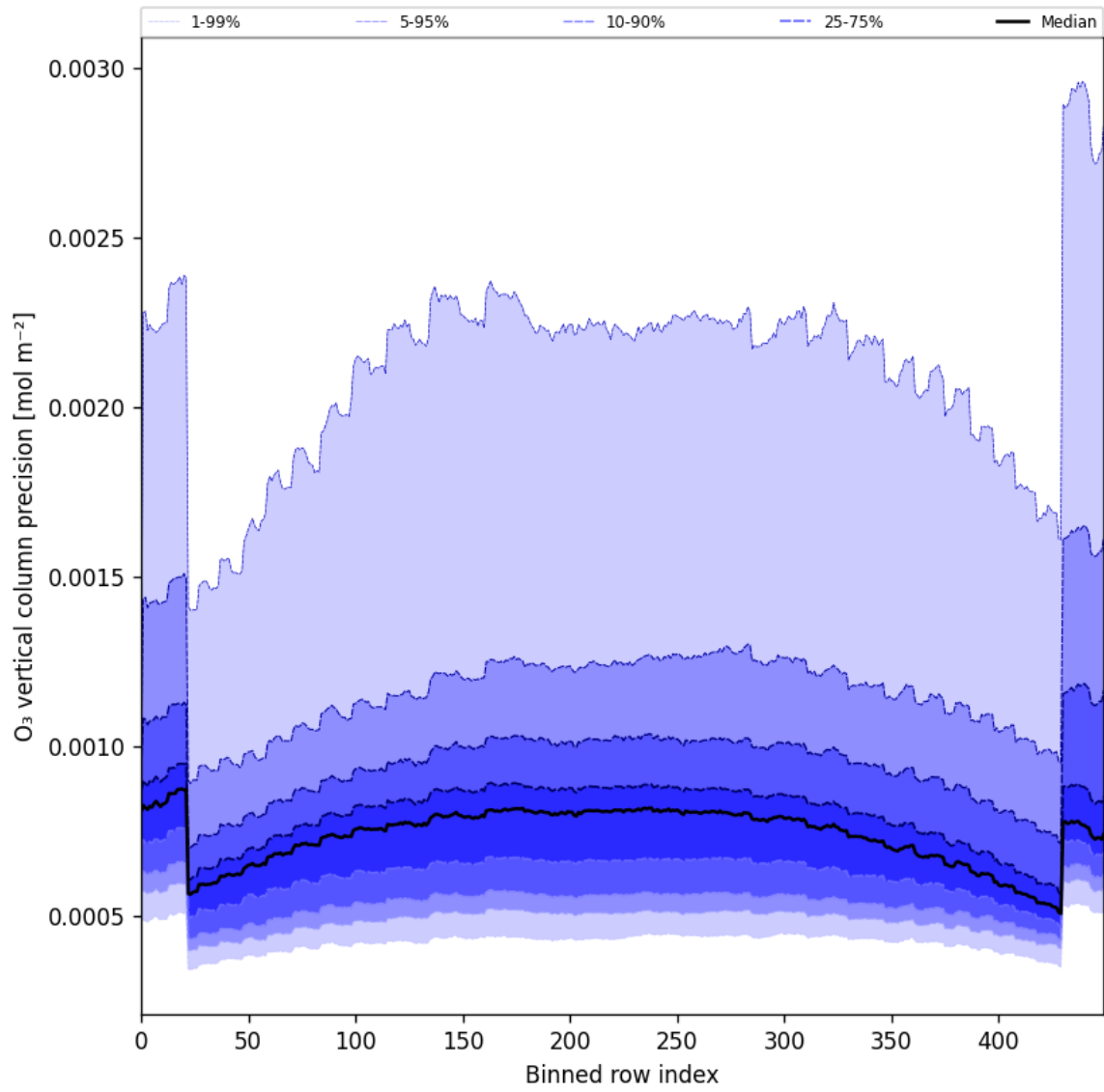
Figure 29: Along track statistics of “O 3 vertical column precision” for 2025-08-12 to 2025-08-14
