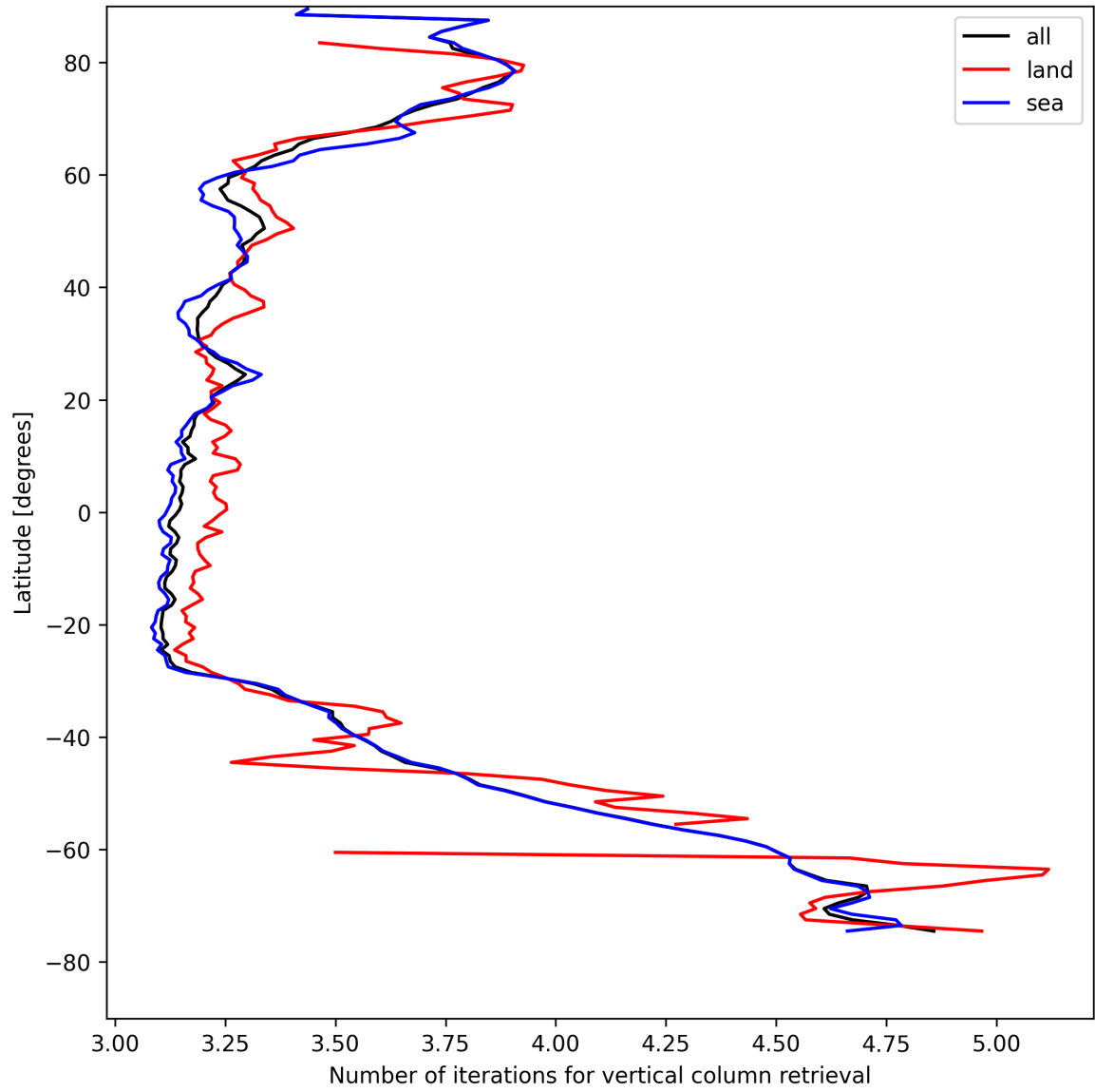
Figure 19: Zonal average of “Number of iterations for vertical column retrieval” for 2025-08-12 to 2025-08-14.
