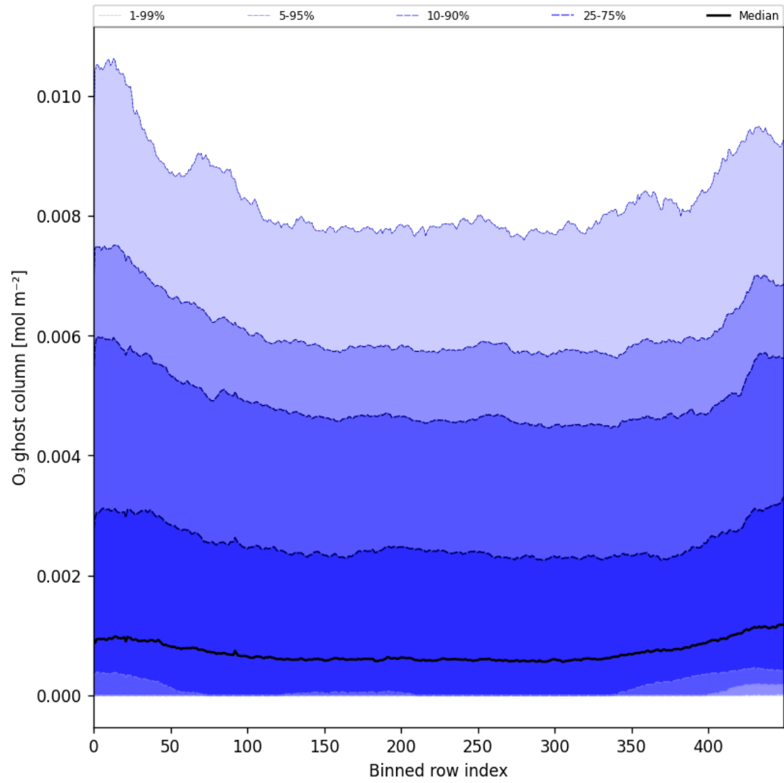
Figure 32: Along track statistics of “O 3 ghost column” for 2025-08-12 to 2025-08-14
