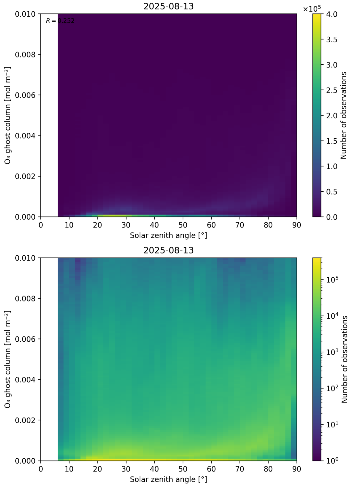
Figure 46: Scatter density plot of “Solar zenith angle” against “O 3 ghost column” for 2025-08-12 to 2025-08-14.
