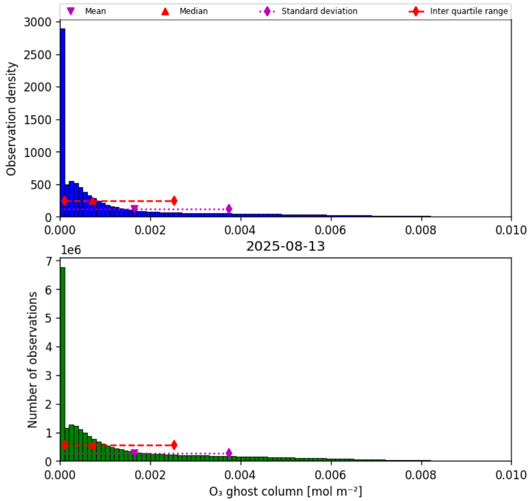
Figure 25: Histogram of "O 3 ghost column" for 2025-08-12 to 2025-08-14
