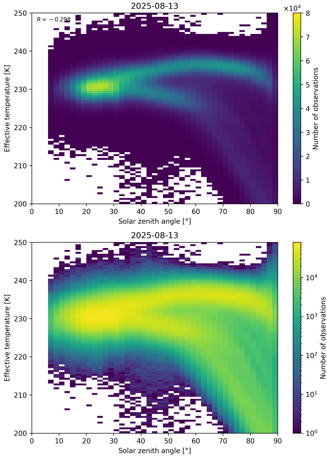
Figure 45: Scatter density plot of “Solar zenith angle” against “Effective temperature” for 2025-08-12 to 2025-08-14.
