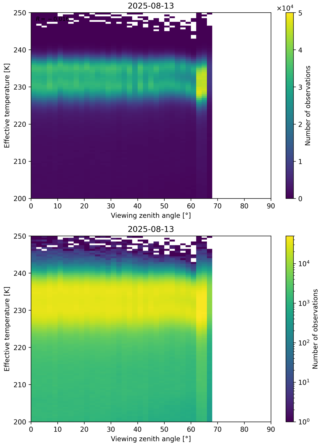
Figure 50: Scatter density plot of “Viewing zenith angle” against “Effective temperature” for 2025-08-12 to 2025-08-14.
