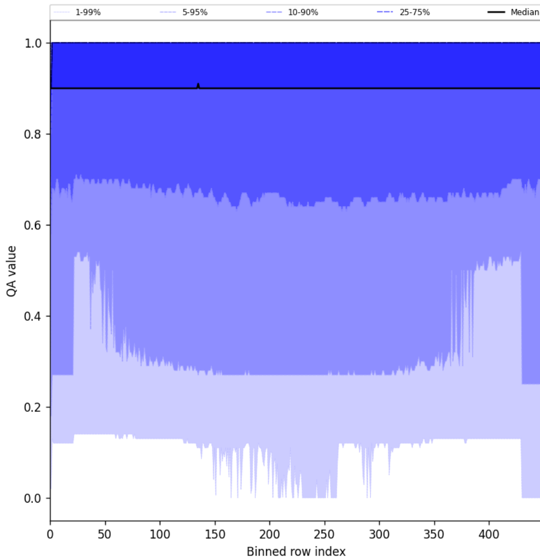
Figure 27: Along track statistics of “QA value” for 2025-08-12 to 2025-08-14
