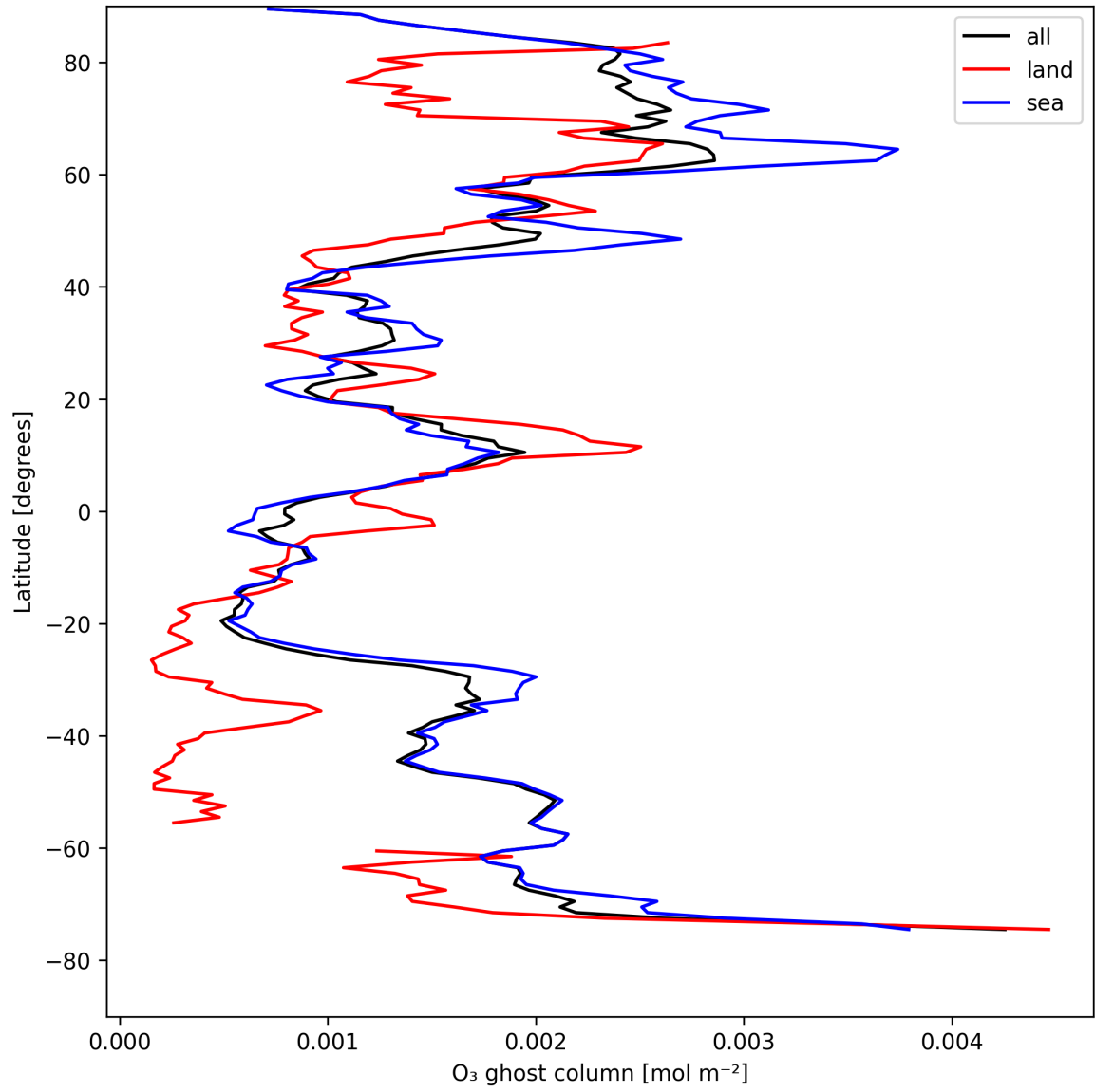
Figure 18: Zonal average of “O 3 ghost column” for 2025-08-12 to 2025-08-14.
