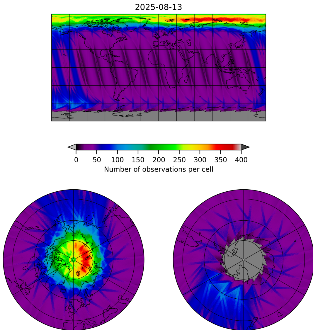
Figure 12: Map of the number of observations for 2025-08-12 to 2025-08-14
