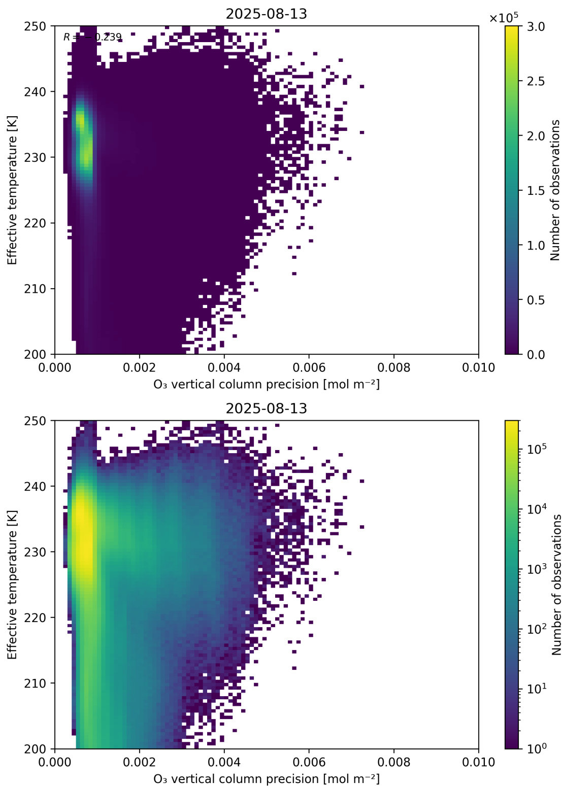
Figure 42: Scatter density plot of “O 3 vertical column precision” against “Effective temperature” for 2025-08-12 to 2025-08-14.
