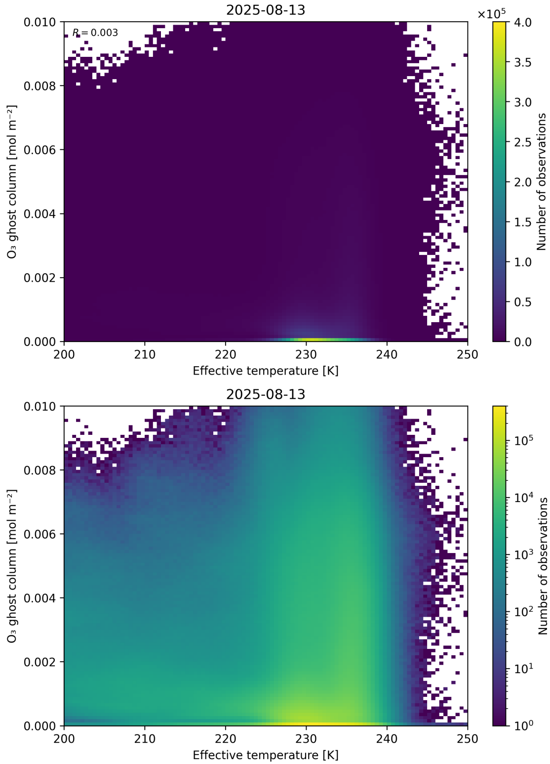
Figure 38: Scatter density plot of “Effective temperature” against “O 3 ghost column” for 2025-08-12 to 2025-08-14.
