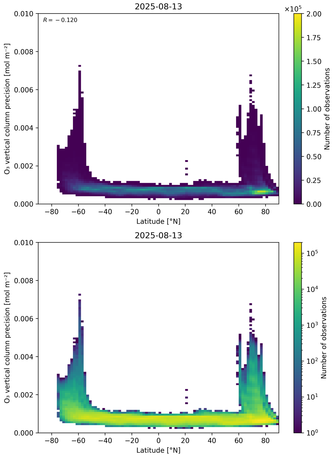
Figure 37: Scatter density plot of “Latitude” against “O 3 vertical column precision” for 2025-08-12 to 2025-08-14.
