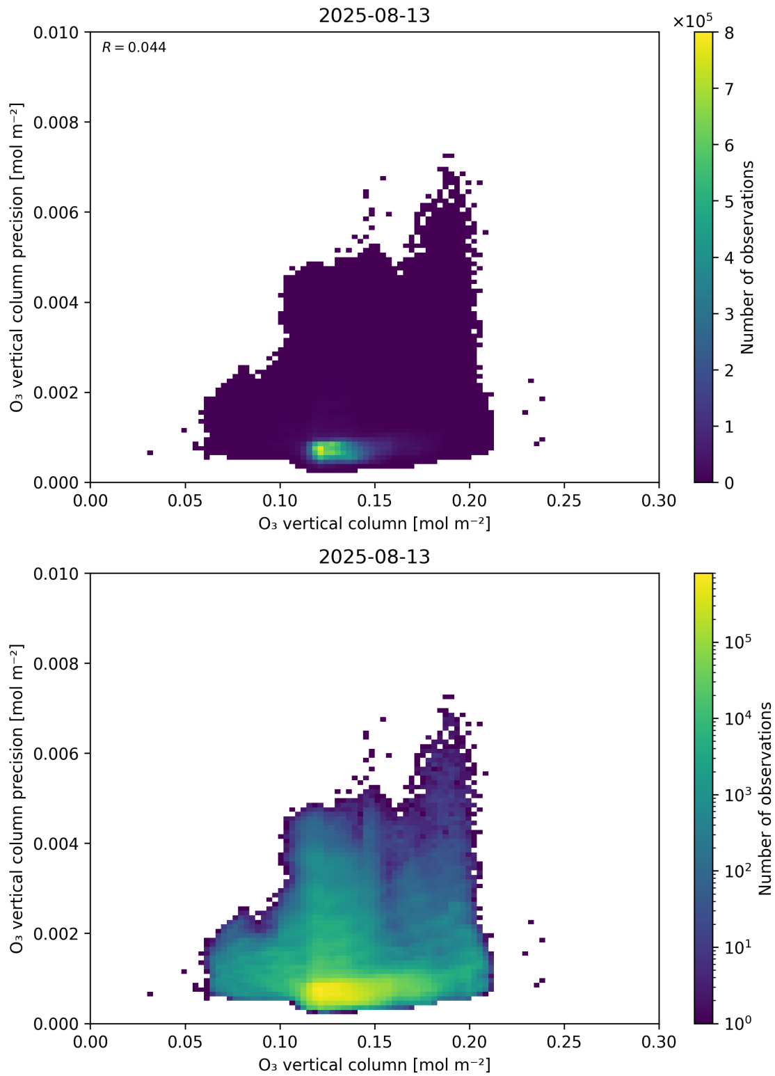
Figure 41: Scatter density plot of “O 3 vertical column” against “O 3 vertical column precision” for 2025-08-12 to 2025-08-14.
