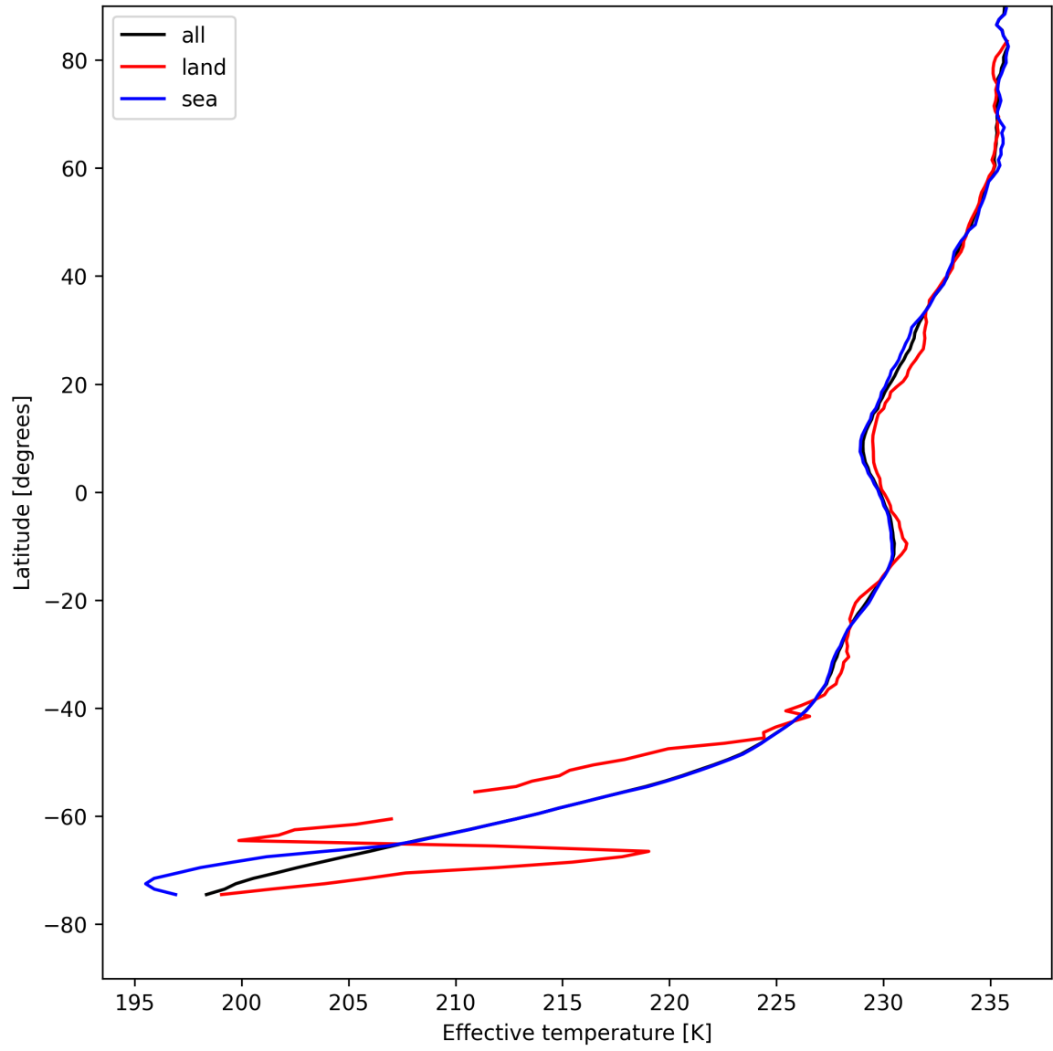
Figure 17: Zonal average of “Effective temperature” for 2025-08-12 to 2025-08-14.
