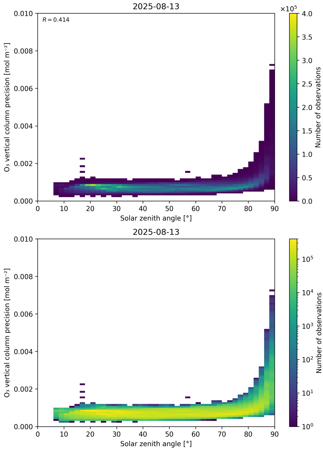
Figure 48: Scatter density plot of “Solar zenith angle” against “O 3 vertical column precision” for 2025-08-12 to 2025-08-14.
