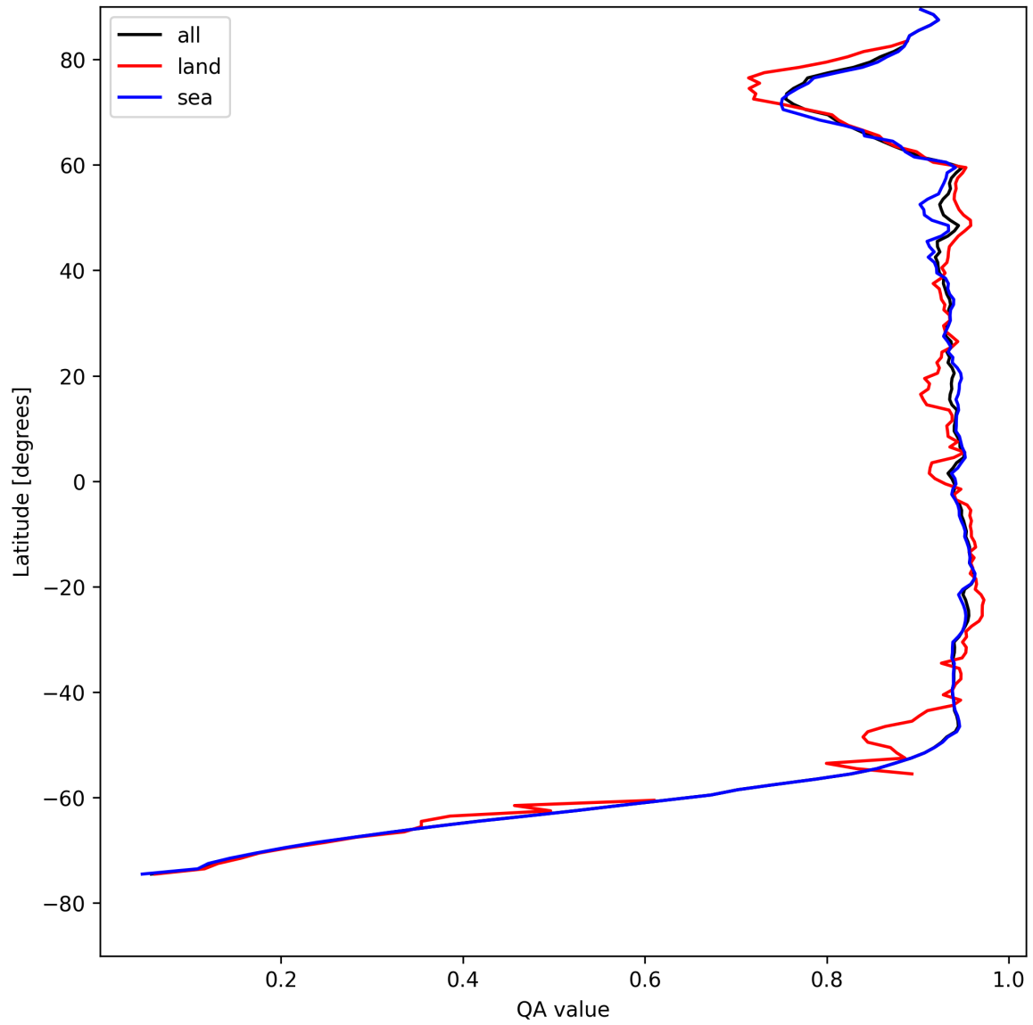
Figure 13: Zonal average of “QA value” for 2025-08-12 to 2025-08-14.
