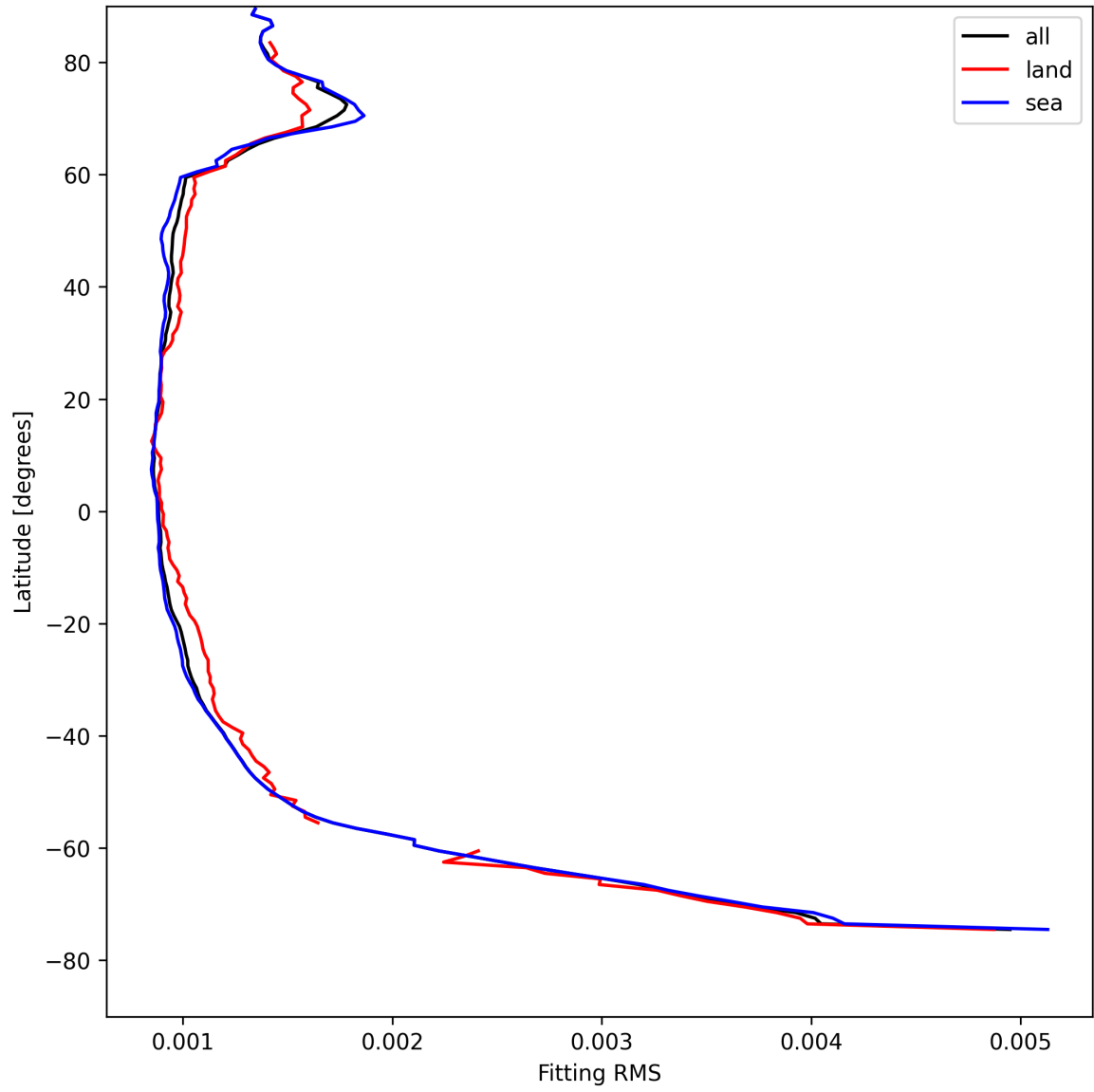
Figure 16: Zonal average of “Fitting RMS” for 2025-08-12 to 2025-08-14.
