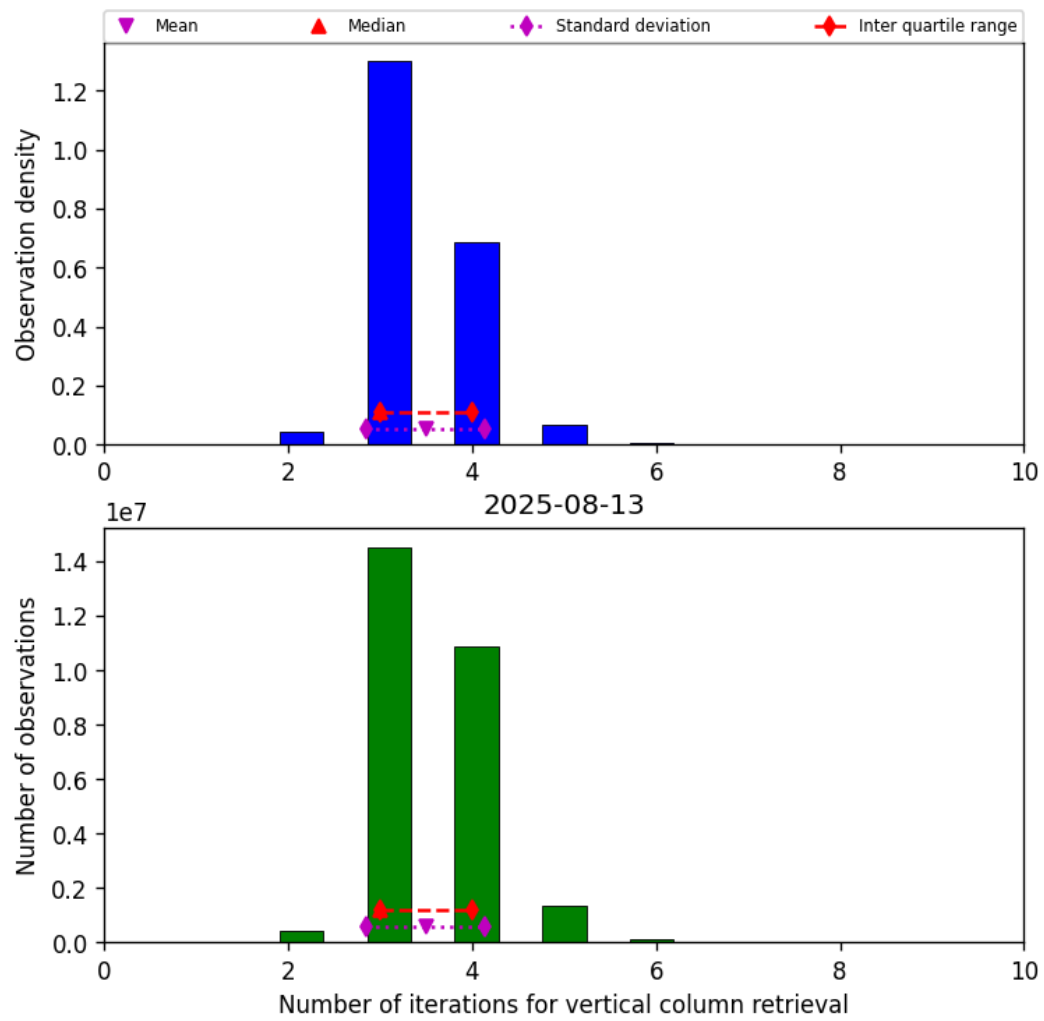
Figure 26: Histogram of “Number of iterations for vertical column retrieval” for 2025-08-12 to 2025-08-14
