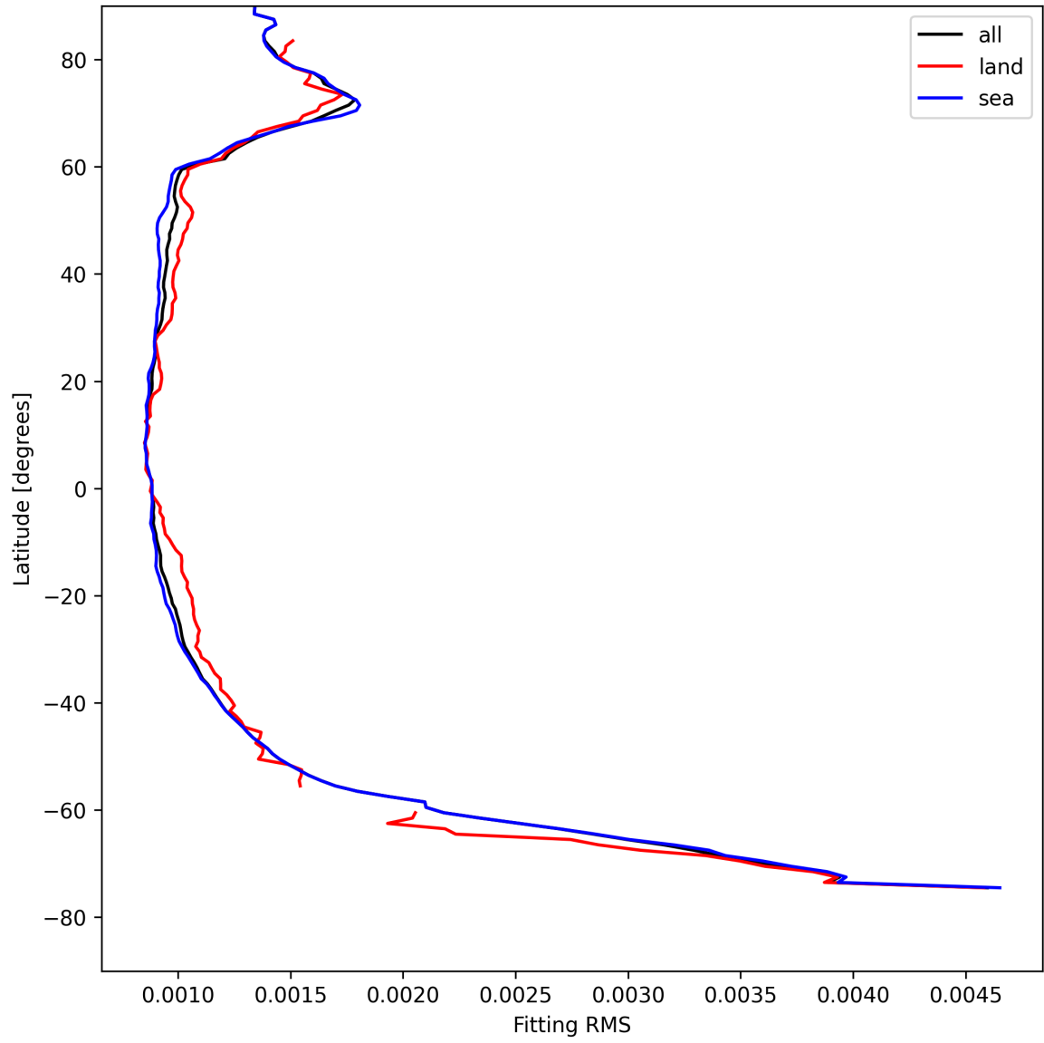
Figure 16: Zonal average of “Fitting RMS” for 2025-08-14 to 2025-08-15.
