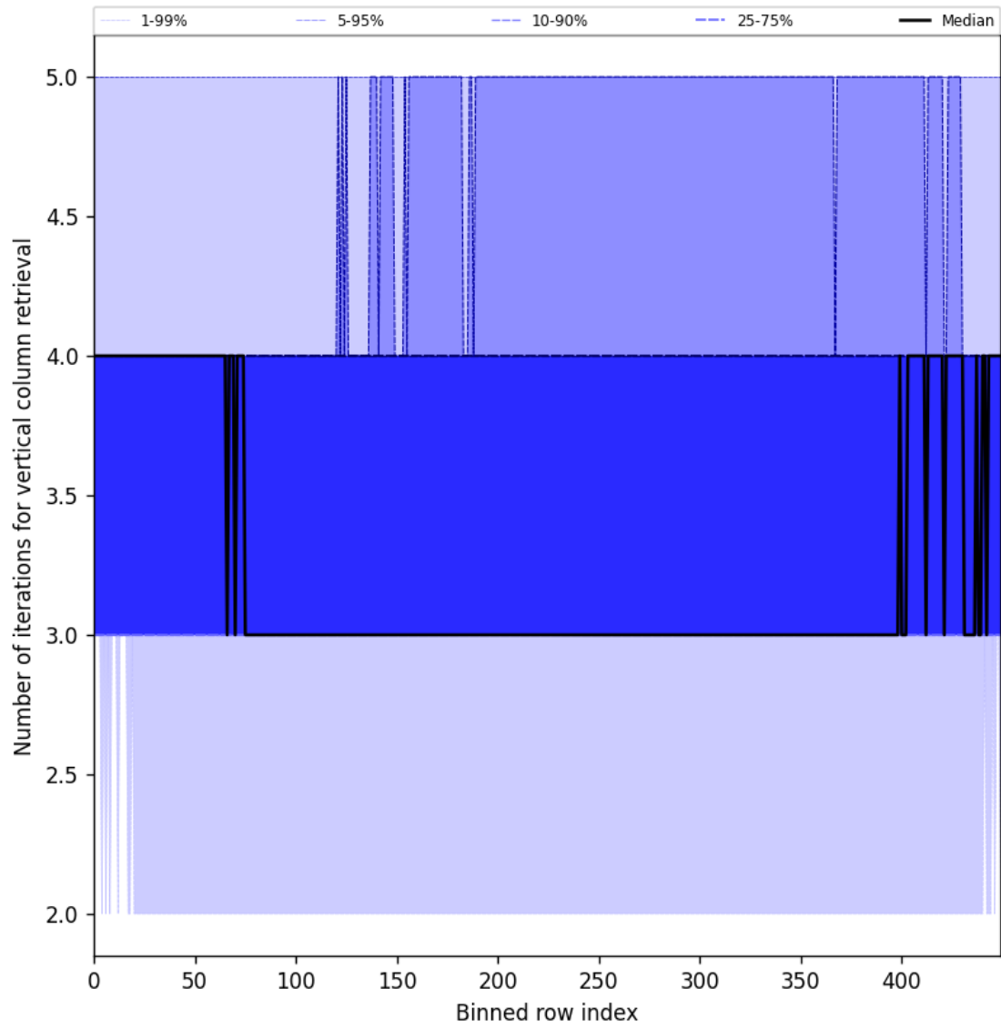
Figure 33: Along track statistics of “Number of iterations for vertical column retrieval” for 2025-08-14 to 2025-08-15
