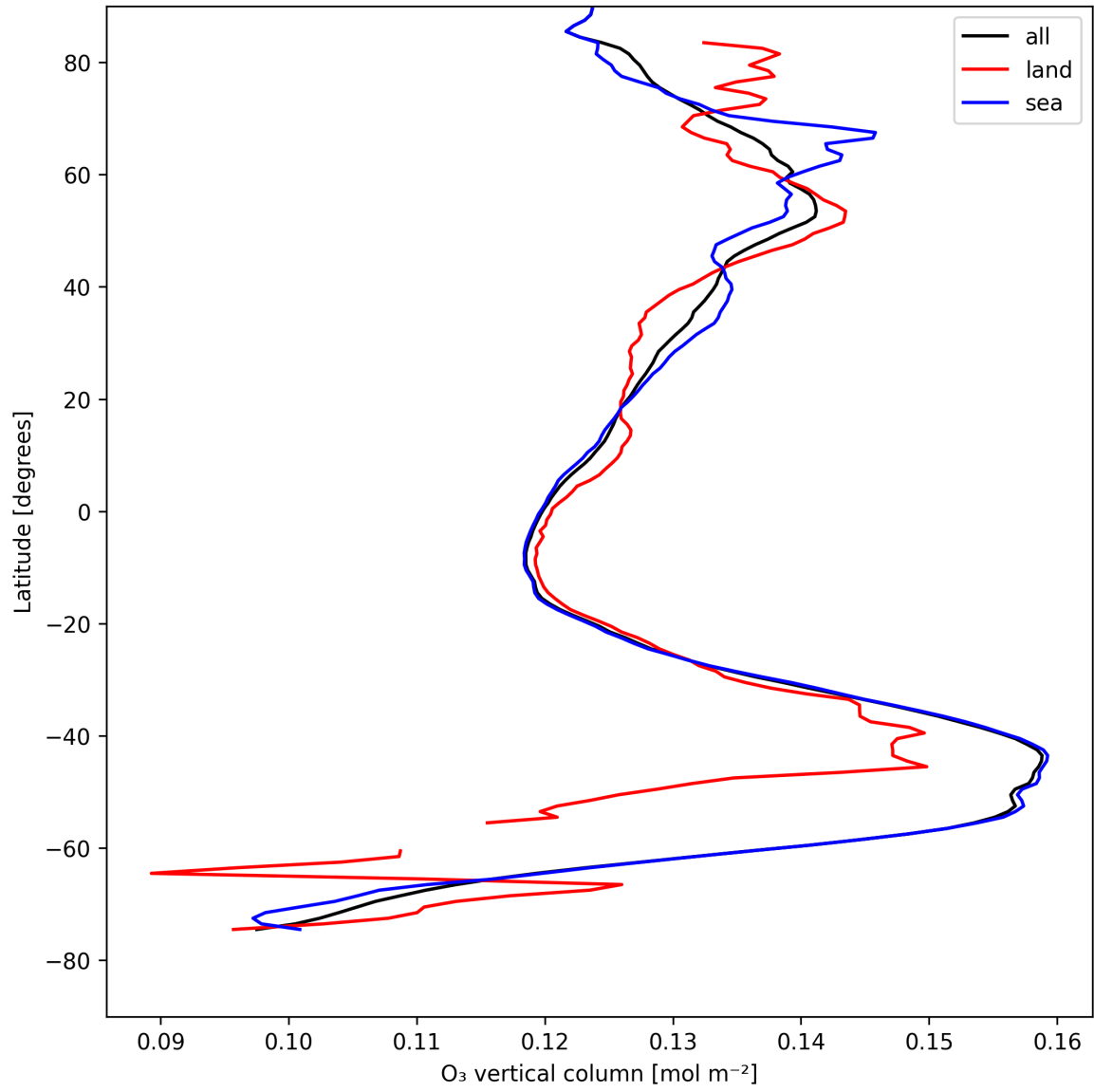
Figure 14: Zonal average of “O 3 vertical column” for 2025-08-14 to 2025-08-15.
