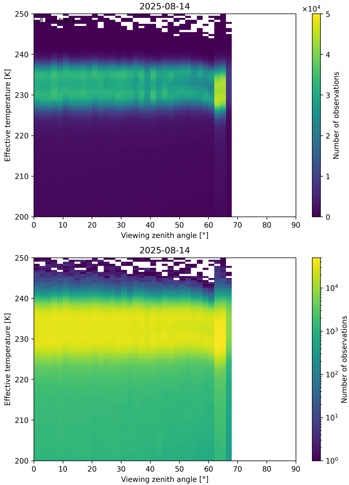
Figure 50: Scatter density plot of “Viewing zenith angle” against “Effective temperature” for 2025-08-14 to 2025-08-15.
