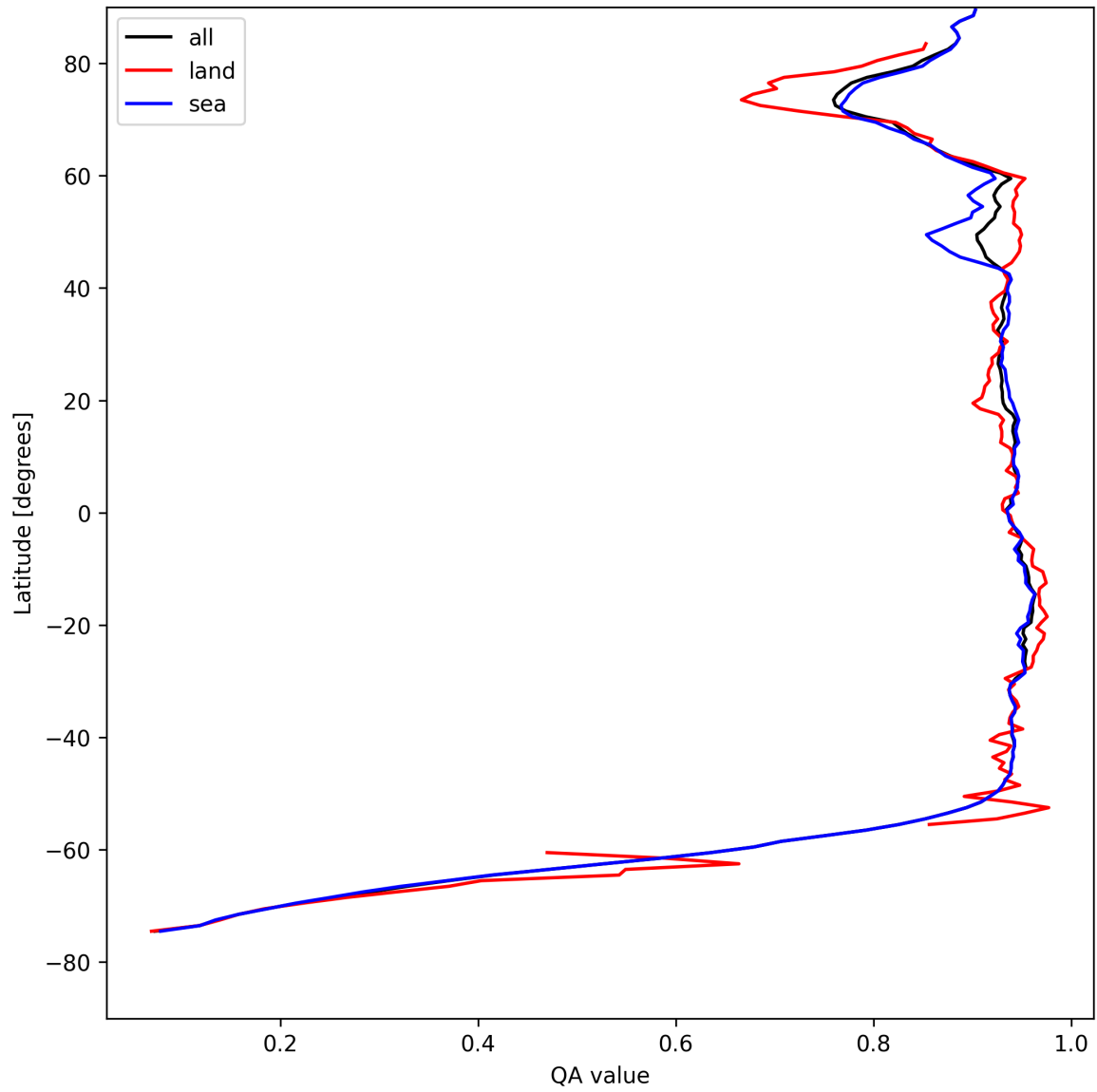
Figure 13: Zonal average of “QA value” for 2025-08-14 to 2025-08-15.
