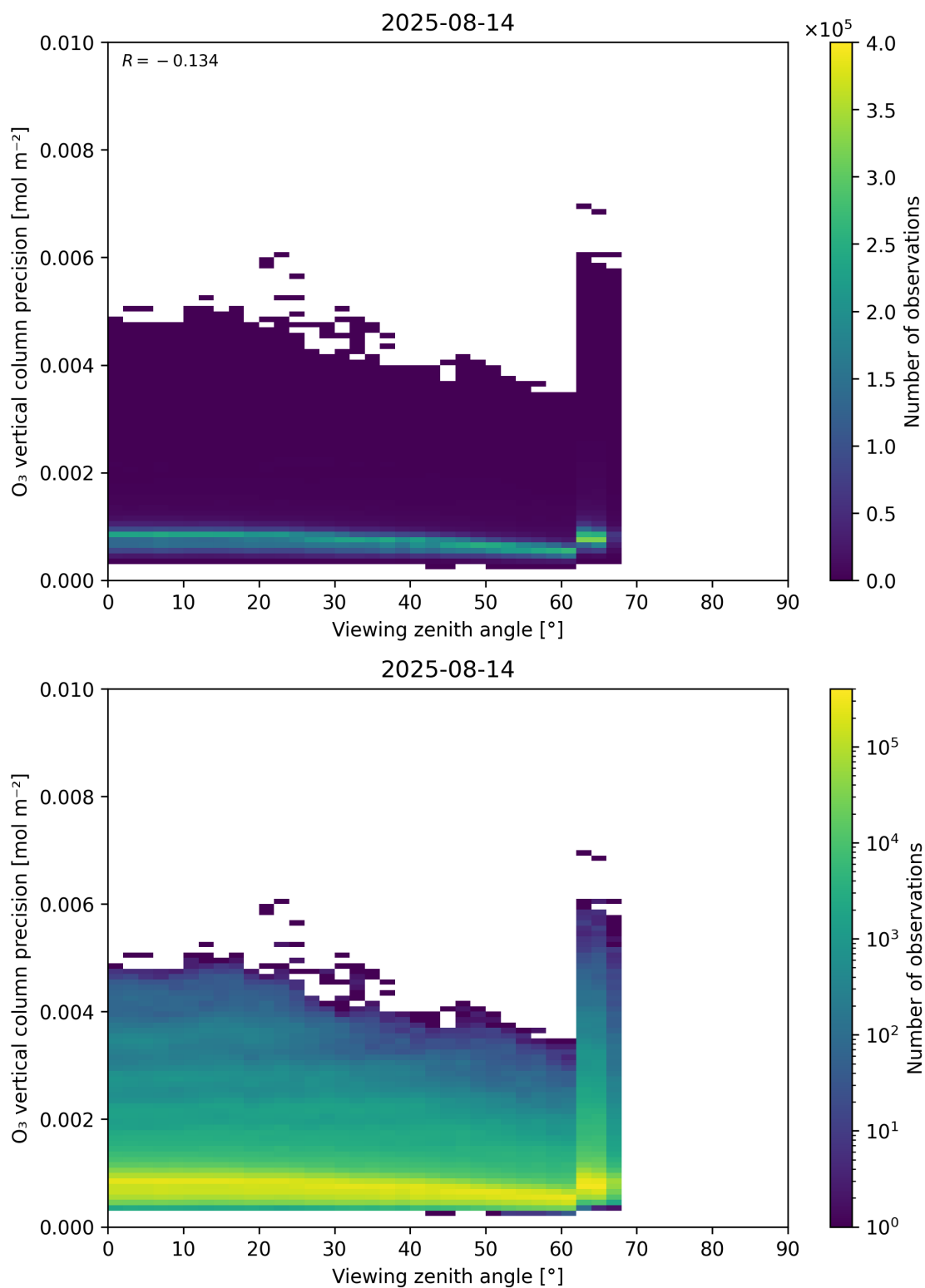
Figure 53: Scatter density plot of “Viewing zenith angle” against “O 3 vertical column precision” for 2025-08-14 to 2025-08-15.
