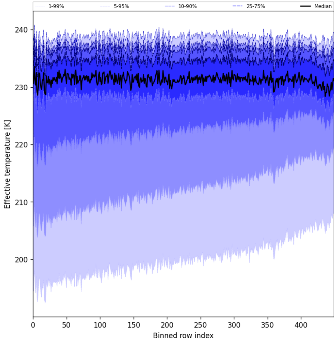
Figure 31: Along track statistics of “Effective temperature” for 2025-08-14 to 2025-08-15
