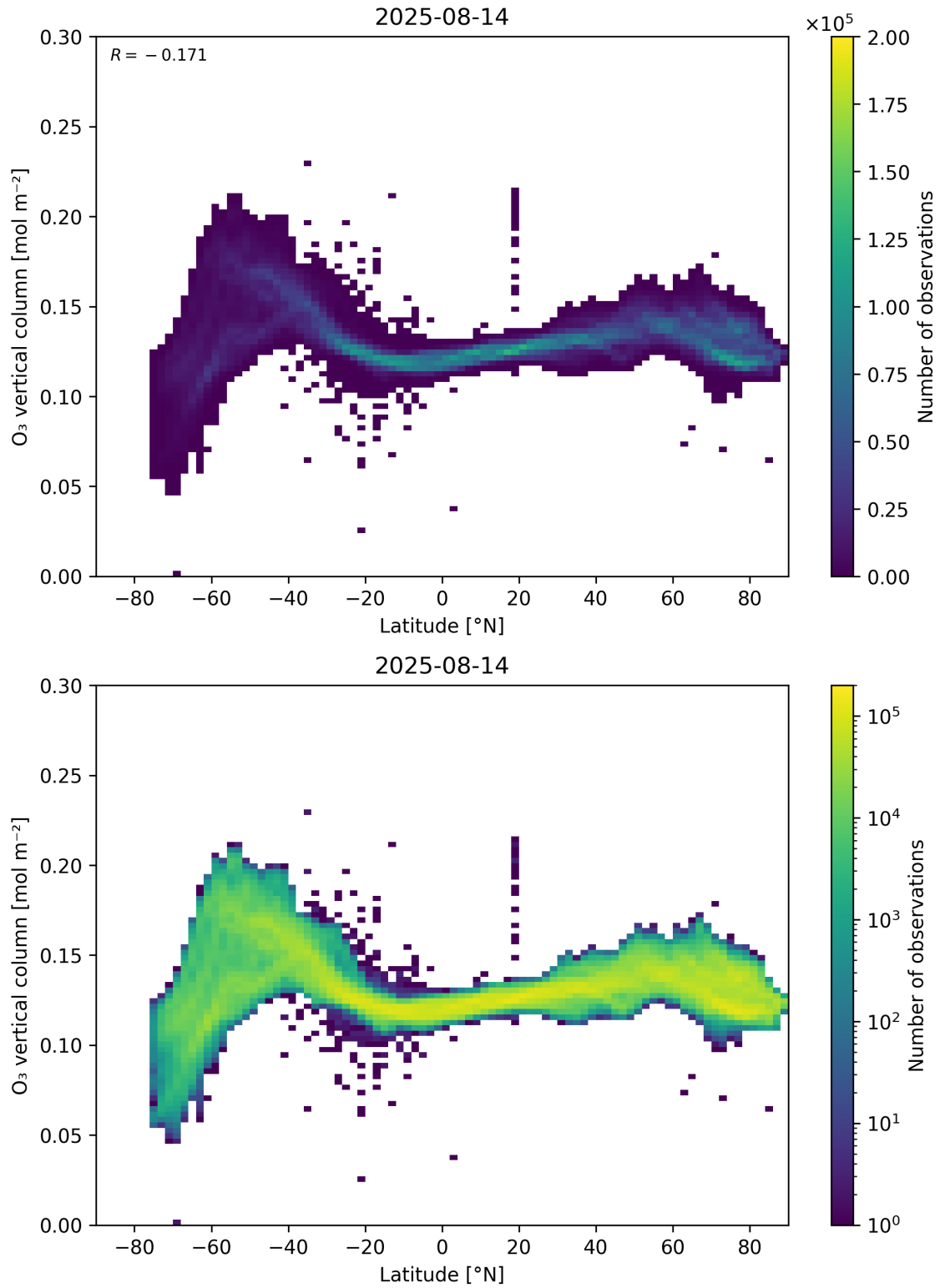
Figure 36: Scatter density plot of “Latitude” against “O 3 vertical column” for 2025-08-14 to 2025-08-15.
