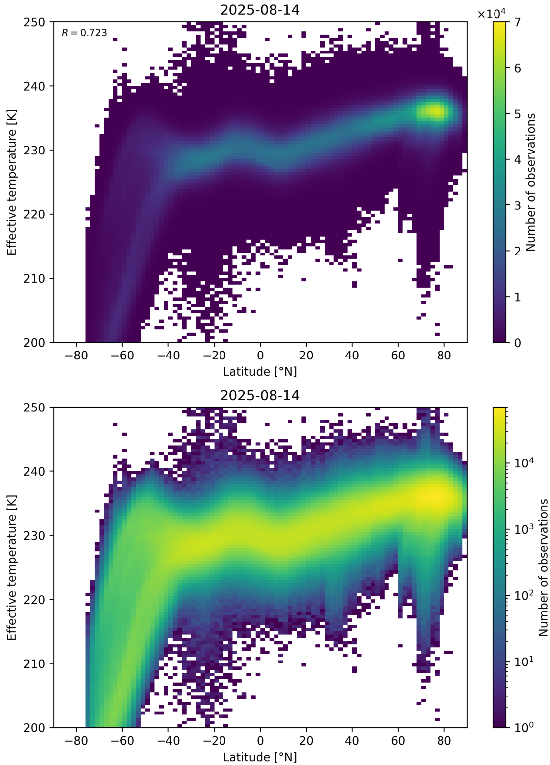
Figure 34: Scatter density plot of “Latitude” against “Effective temperature” for 2025-08-14 to 2025-08-15.
