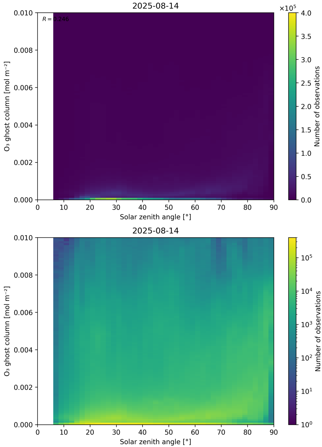
Figure 46: Scatter density plot of “Solar zenith angle” against “O 3 ghost column” for 2025-08-14 to 2025-08-15.
