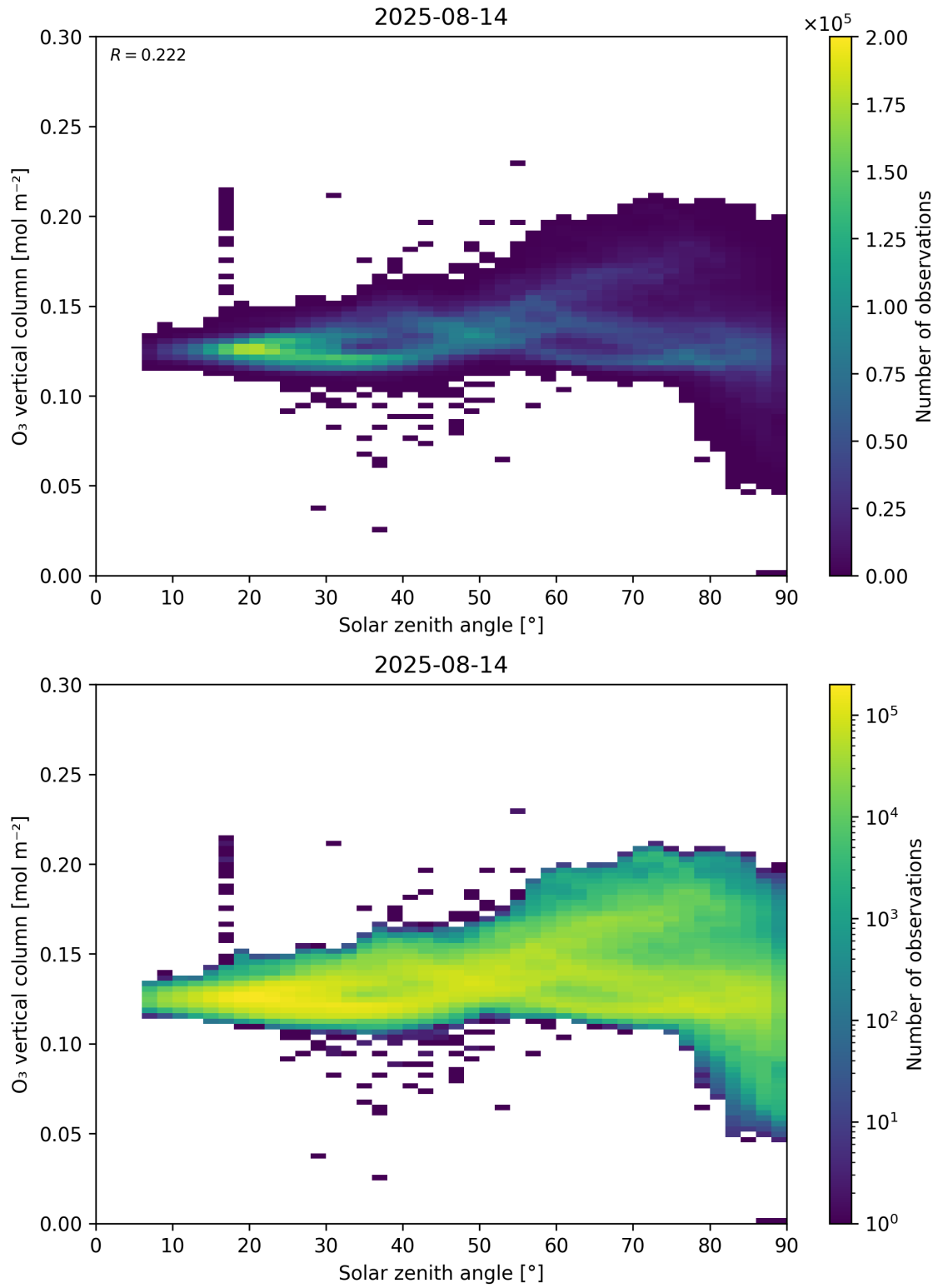
Figure 47: Scatter density plot of “Solar zenith angle” against “O 3 vertical column” for 2025-08-14 to 2025-08-15.
