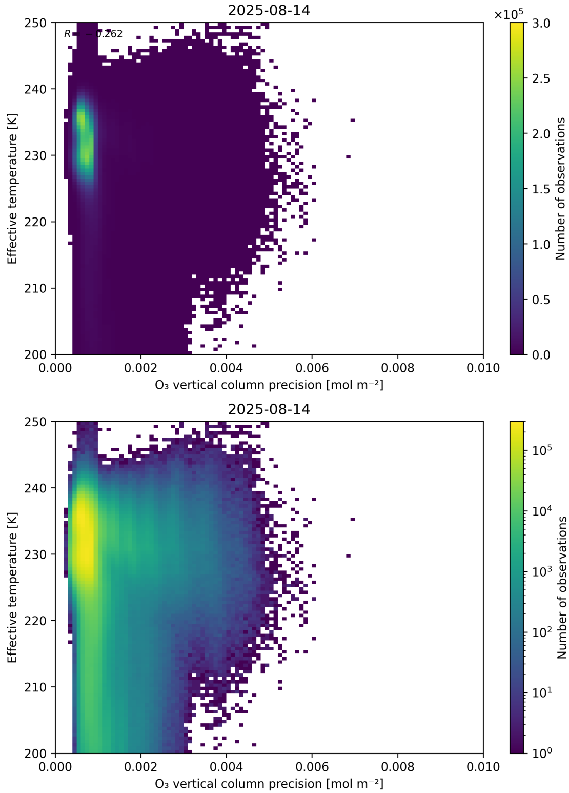
Figure 42: Scatter density plot of “O 3 vertical column precision” against “Effective temperature” for 2025-08-14 to 2025-08-15.
