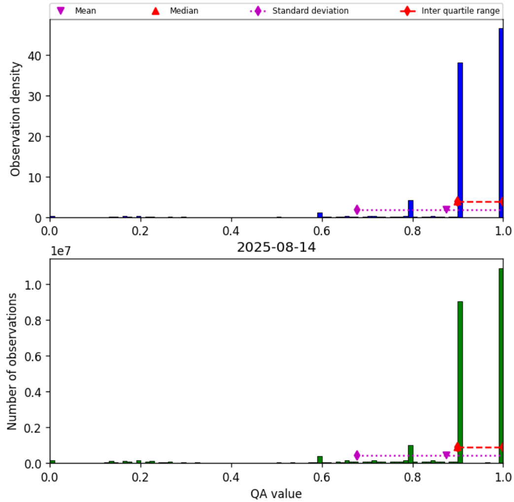
Figure 20: Histogram of “QA value” for 2025-08-14 to 2025-08-15
