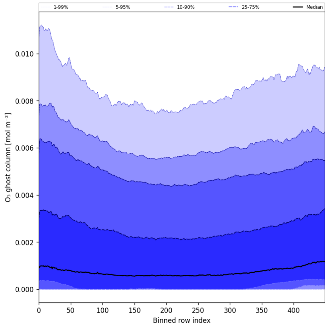
Figure 32: Along track statistics of “O 3 ghost column” for 2025-08-14 to 2025-08-15
