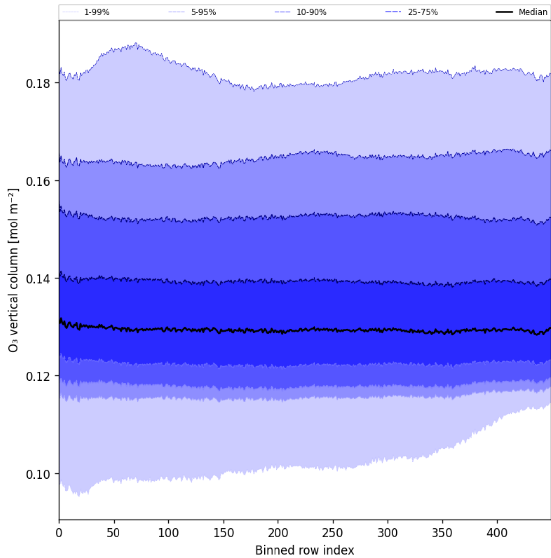
Figure 28: Along track statistics of “O 3 vertical column” for 2025-08-14 to 2025-08-15
