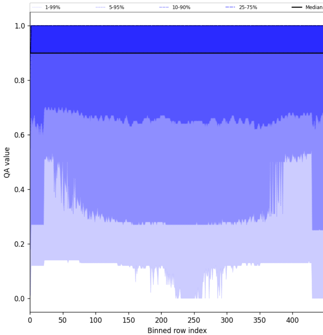
Figure 27: Along track statistics of “QA value” for 2025-08-14 to 2025-08-15
