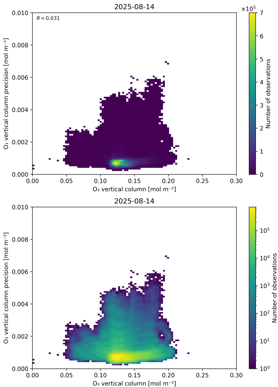
Figure 41: Scatter density plot of “O 3 vertical column” against “O 3 vertical column precision” for 2025-08-14 to 2025-08-15.
