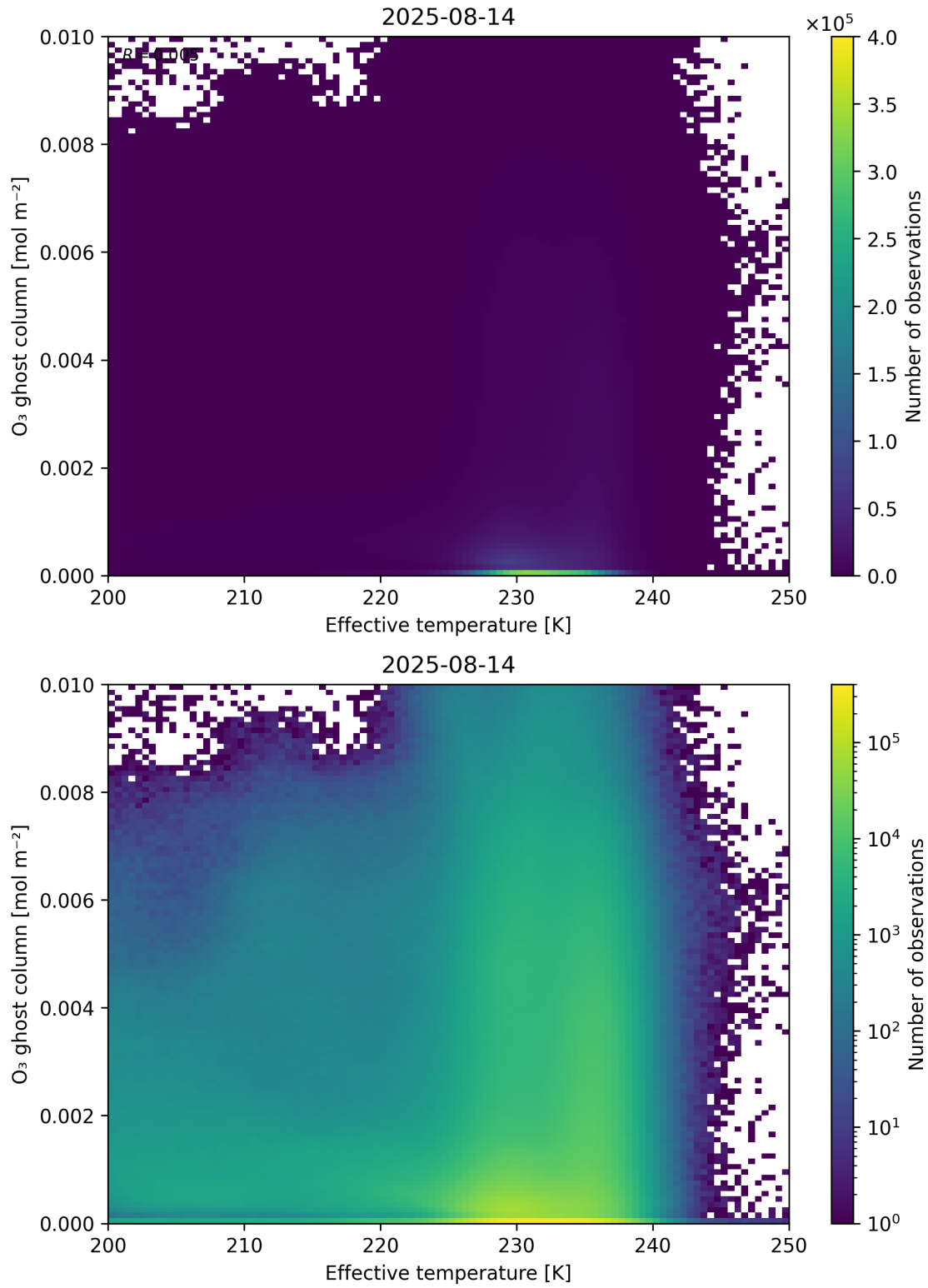
Figure 38: Scatter density plot of “Effective temperature” against “O 3 ghost column” for 2025-08-14 to 2025-08-15.
