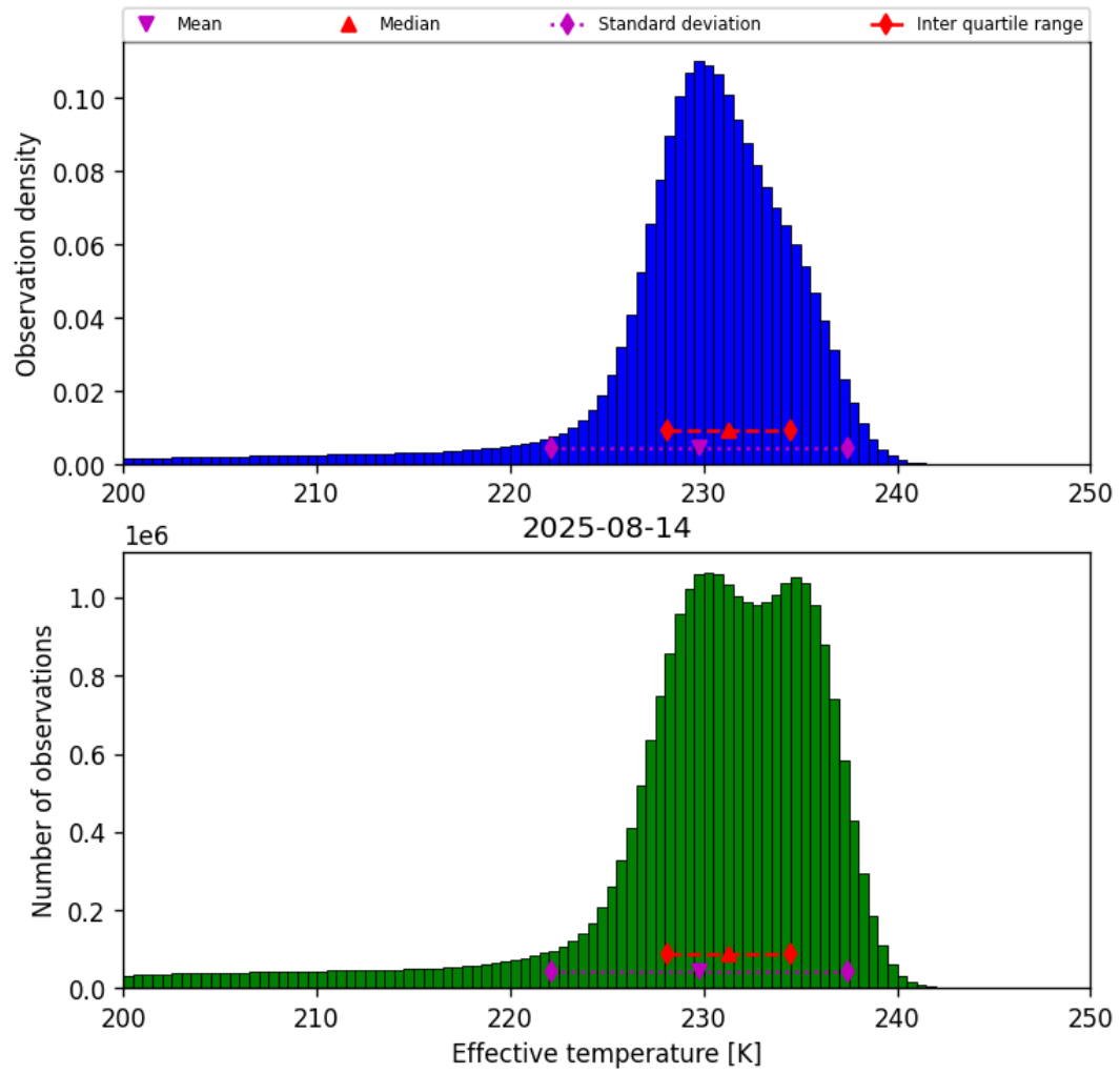
Figure 24: Histogram of “Effective temperature” for 2025-08-14 to 2025-08-15
