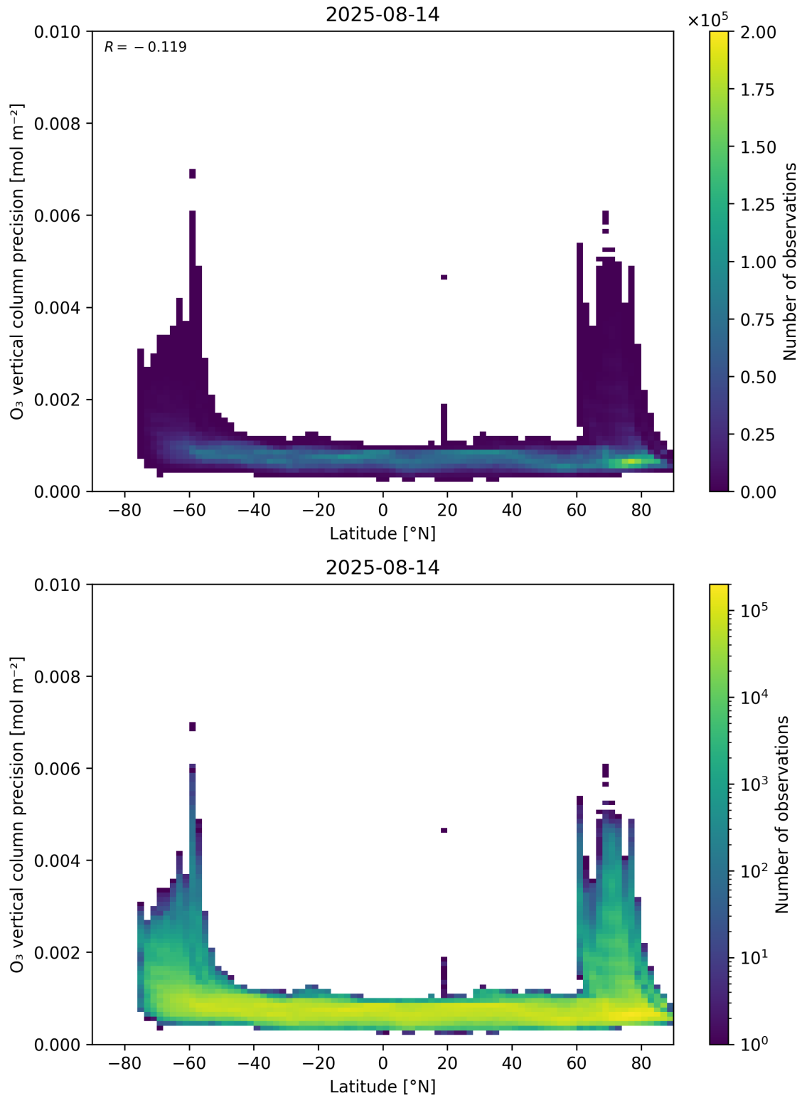
Figure 37: Scatter density plot of “Latitude” against “O 3 vertical column precision” for 2025-08-14 to 2025-08-15.
