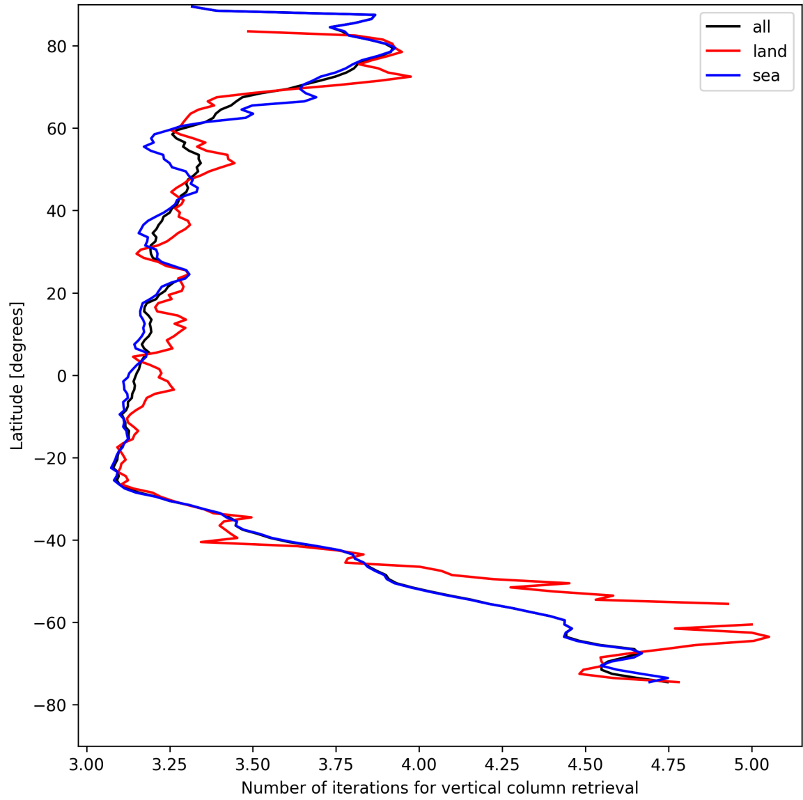
Figure 19: Zonal average of “Number of iterations for vertical column retrieval” for 2025-08-14 to 2025-08-15.
