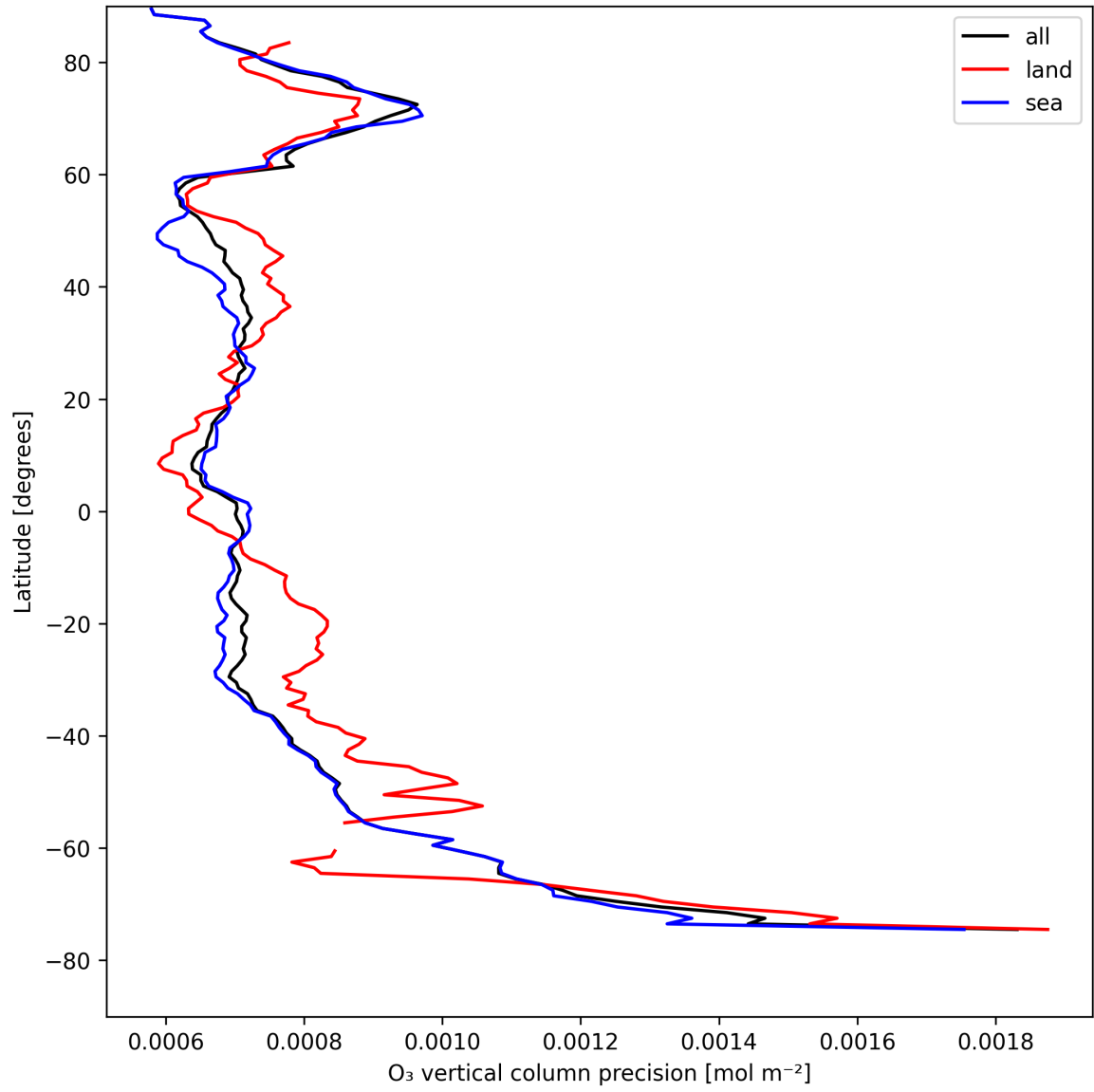
Figure 15: Zonal average of "O 3 vertical column precision" for 2025-08-14 to 2025-08-15.
