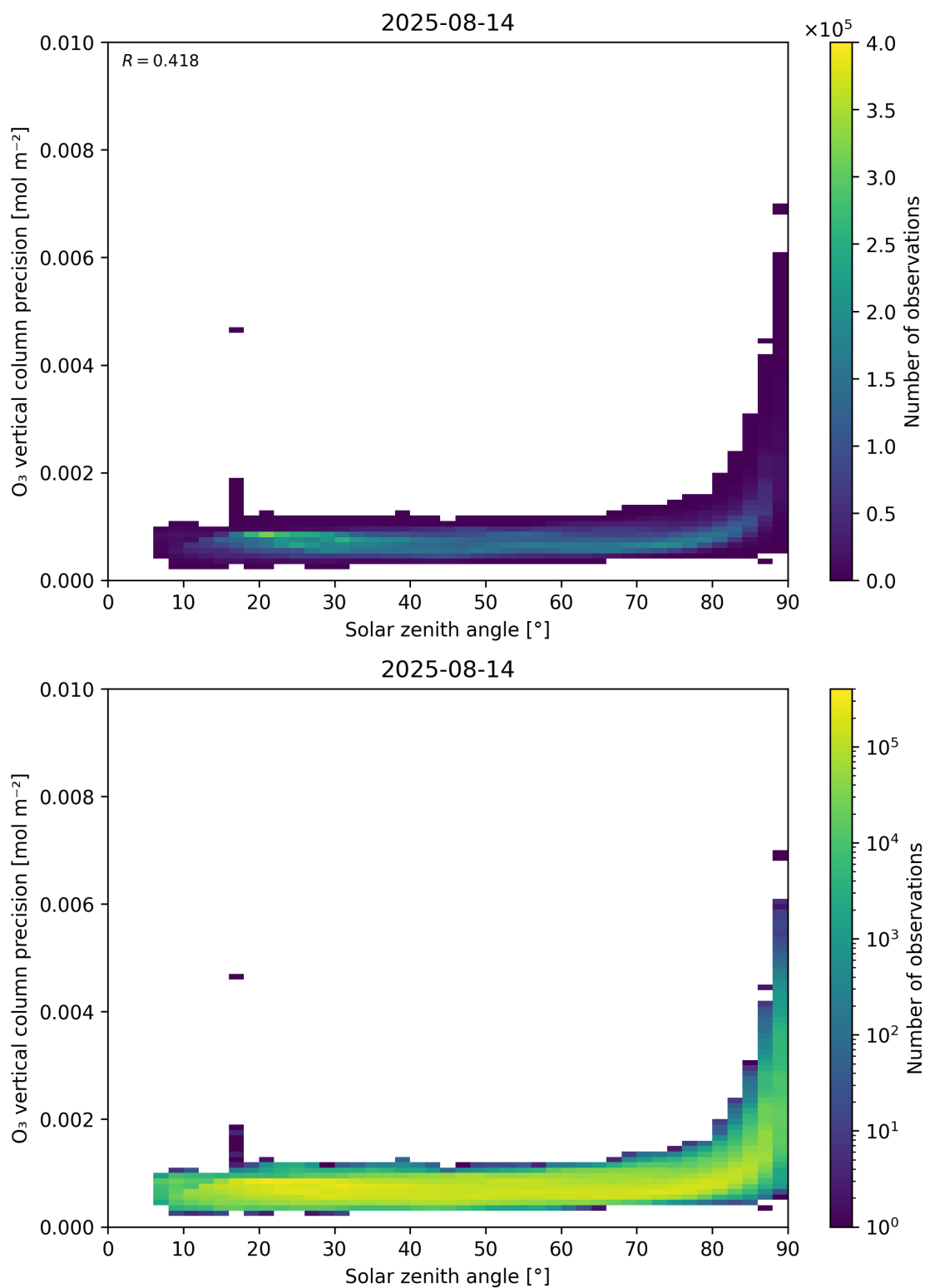
Figure 48: Scatter density plot of “Solar zenith angle” against “O 3 vertical column precision” for 2025-08-14 to 2025-08-15.
