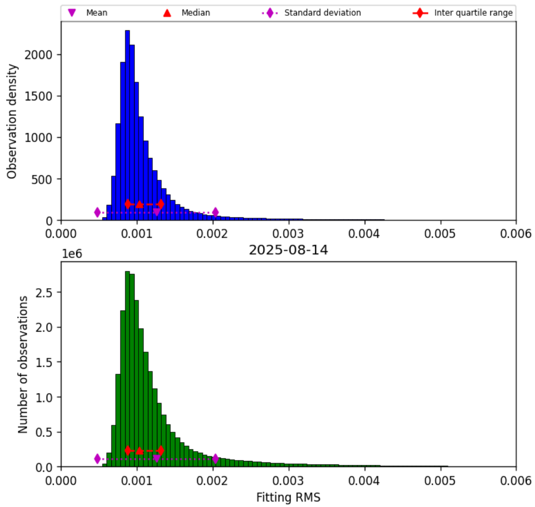
Figure 23: Histogram of “Fitting RMS” for 2025-08-14 to 2025-08-15
