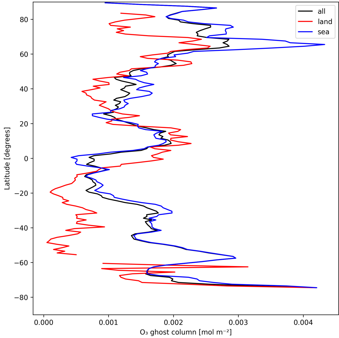
Figure 18: Zonal average of “O 3 ghost column” for 2025-08-14 to 2025-08-15.
