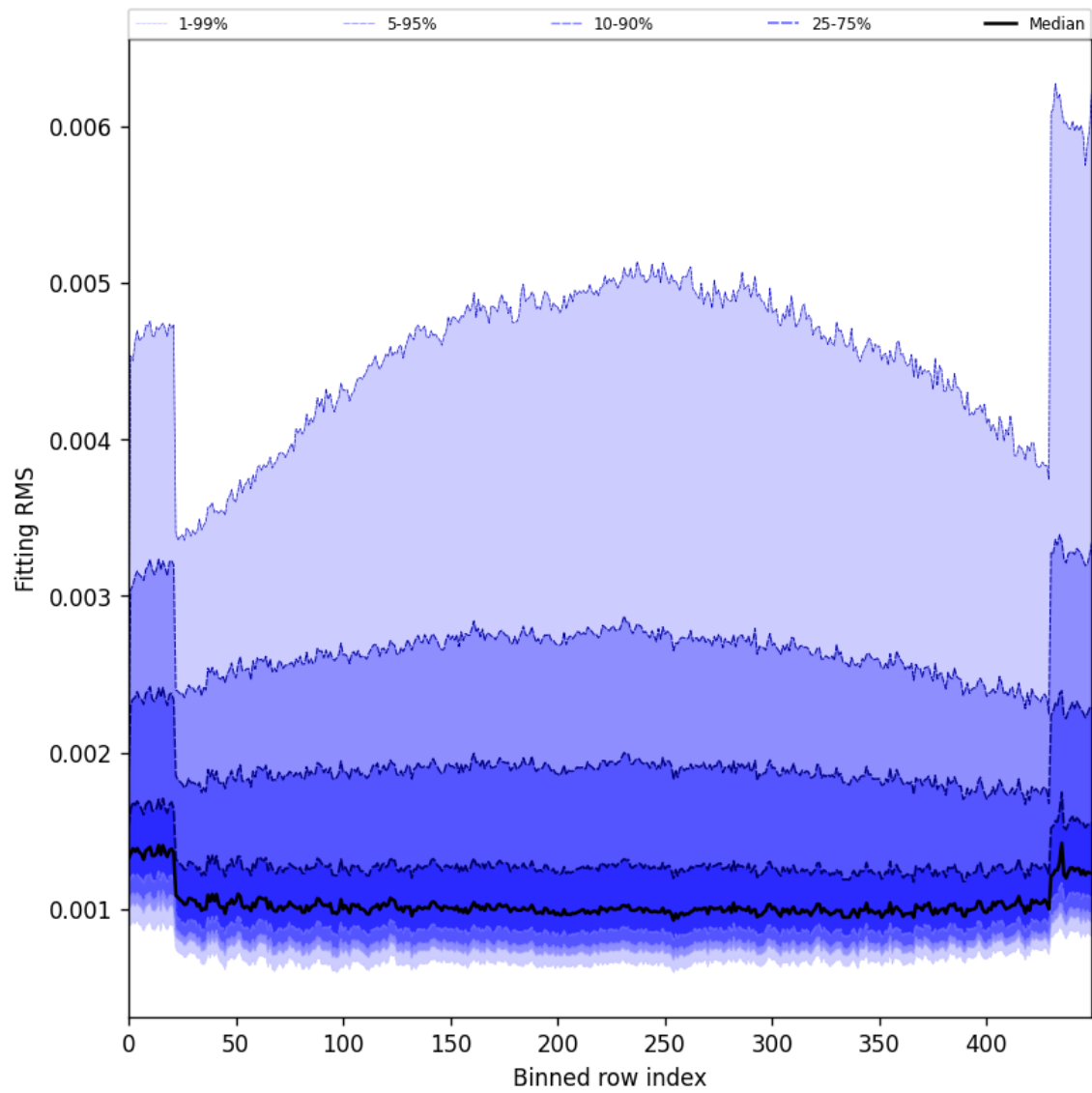
Figure 30: Along track statistics of “Fitting RMS” for 2025-08-14 to 2025-08-15
