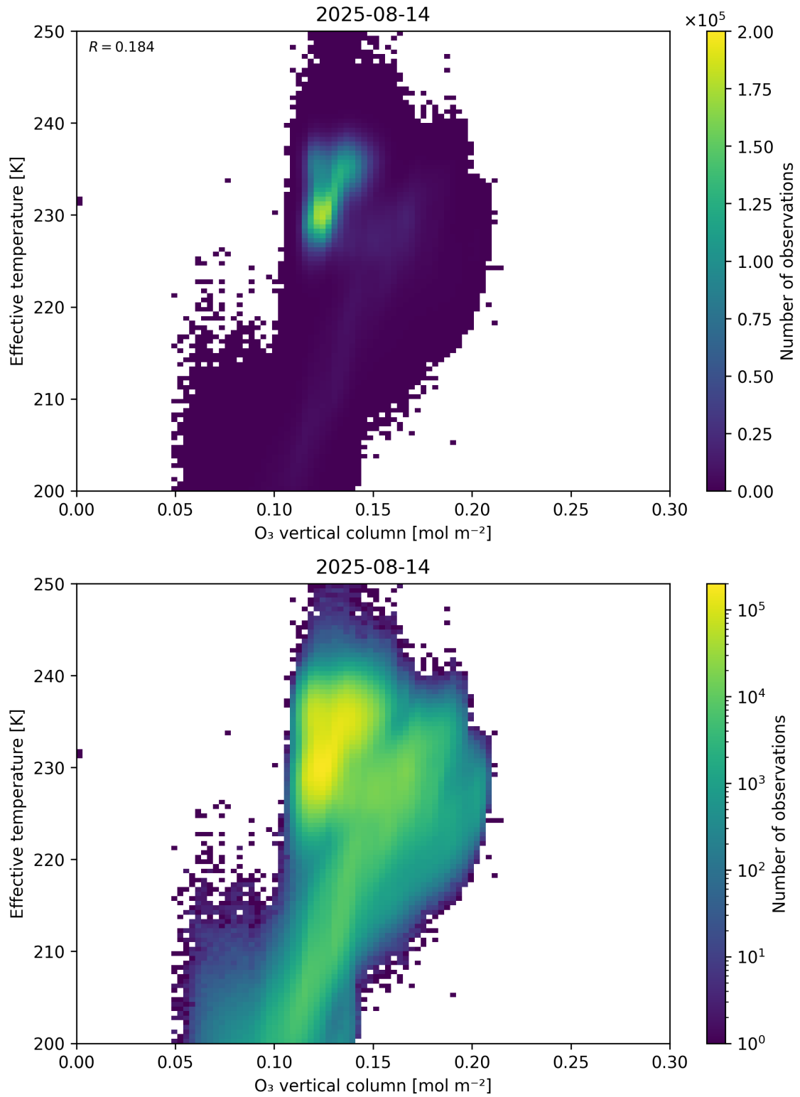
Figure 39: Scatter density plot of “O 3 vertical column” against “Effective temperature” for 2025-08-14 to 2025-08-15.
