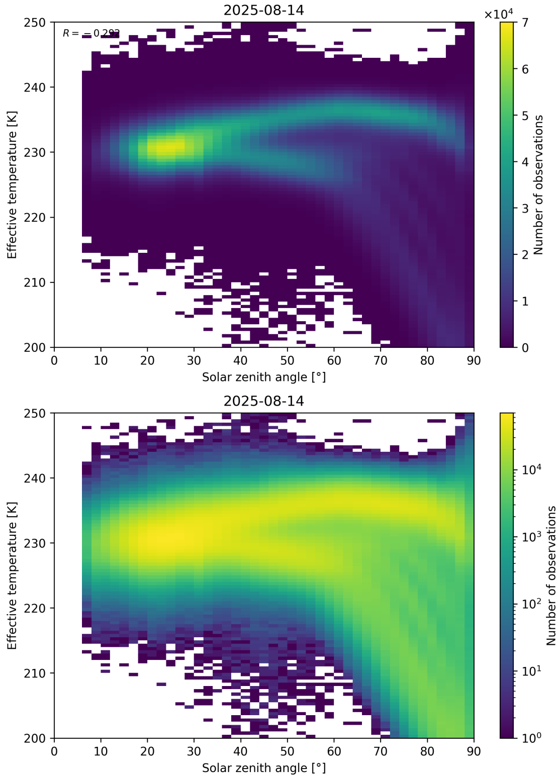
Figure 45: Scatter density plot of “Solar zenith angle” against “Effective temperature” for 2025-08-14 to 2025-08-15.
