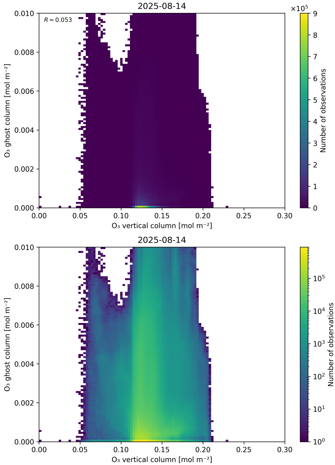
Figure 40: Scatter density plot of “O 3 vertical column” against “O 3 ghost column” for 2025-08-14 to 2025-08-15.
