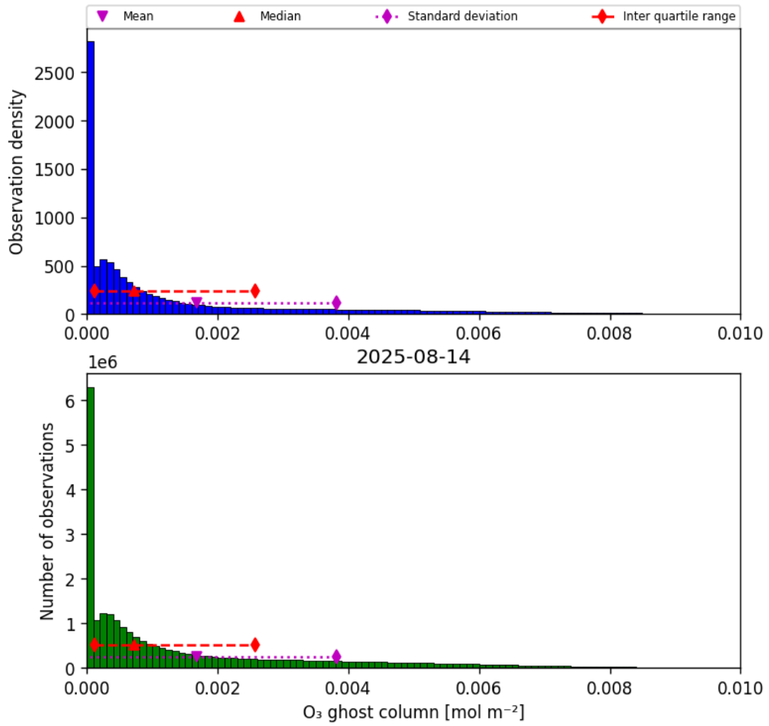
Figure 25: Histogram of “O 3 ghost column” for 2025-08-14 to 2025-08-15
