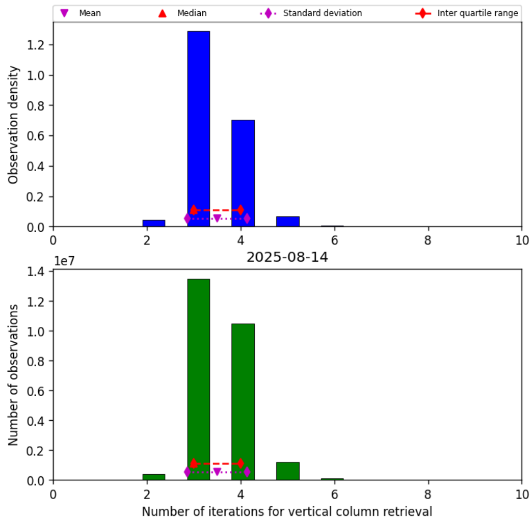
Figure 26: Histogram of “Number of iterations for vertical column retrieval” for 2025-08-14 to 2025-08-15
