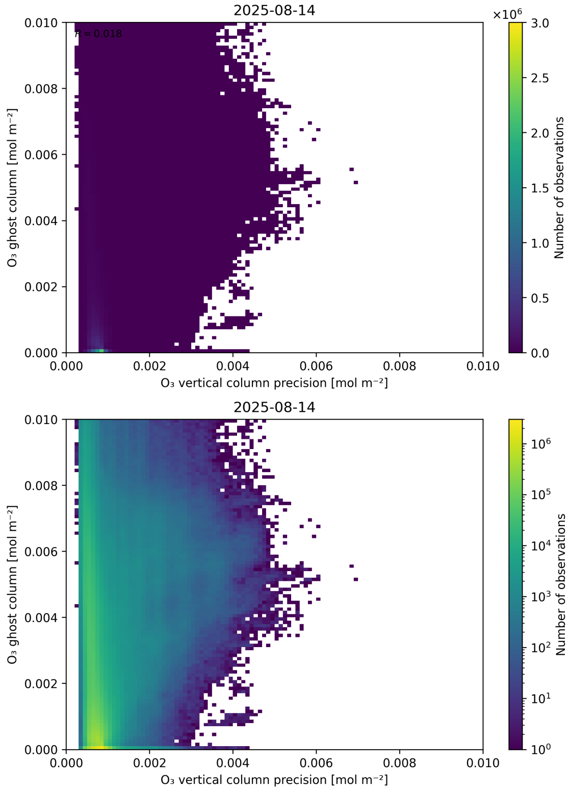
Figure 43: Scatter density plot of “O 3 vertical column precision” against “O 3 ghost column” for 2025-08-14 to 2025-08-15.
