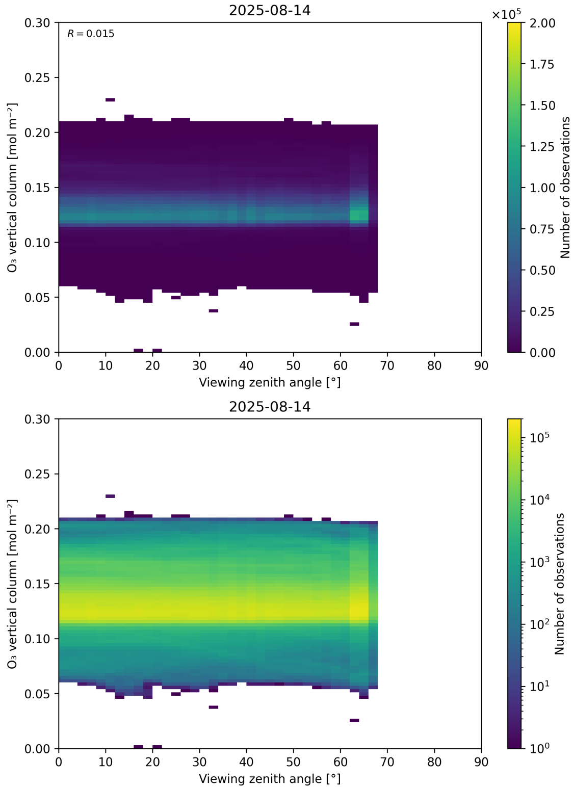
Figure 52: Scatter density plot of “Viewing zenith angle” against “O 3 vertical column” for 2025-08-14 to 2025-08-15.
