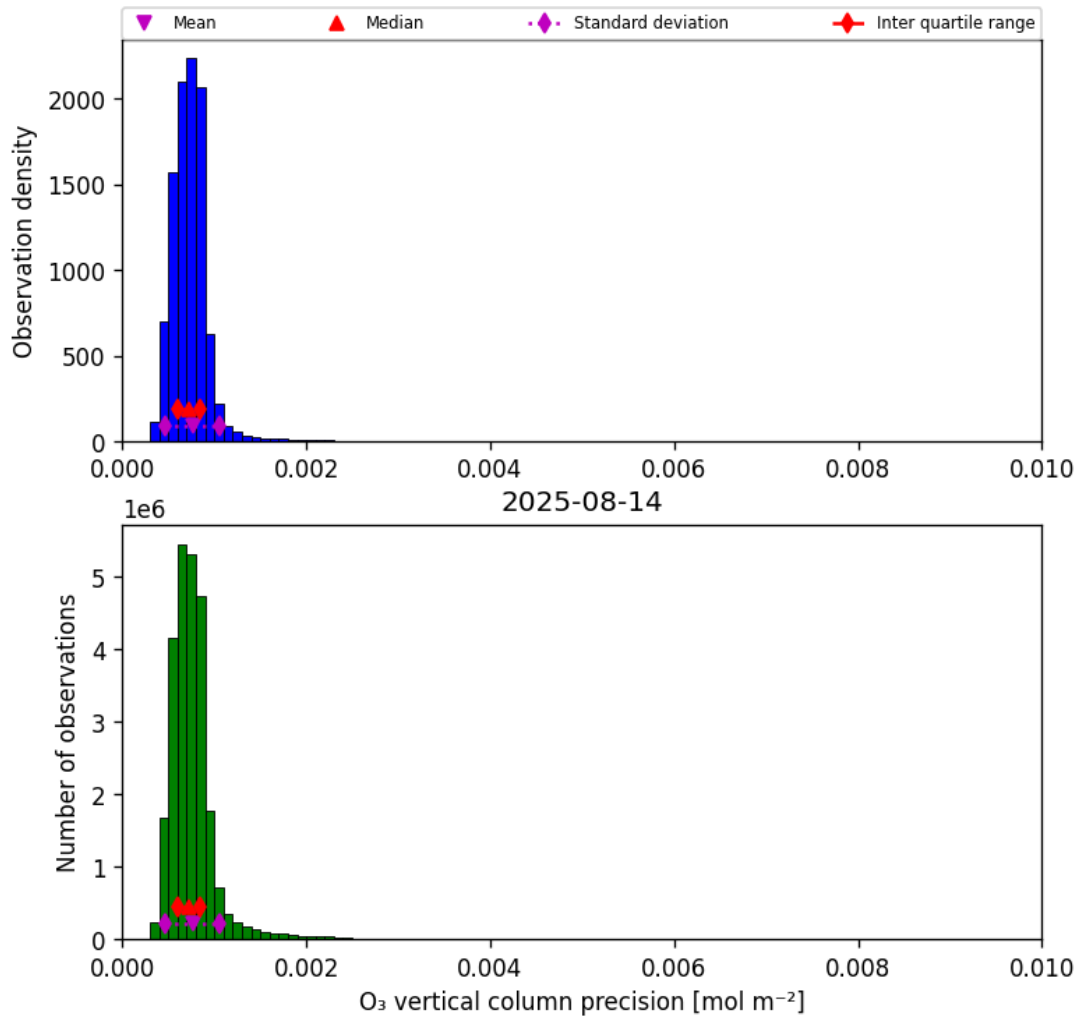
Figure 22: Histogram of “O 3 vertical column precision” for 2025-08-14 to 2025-08-15
