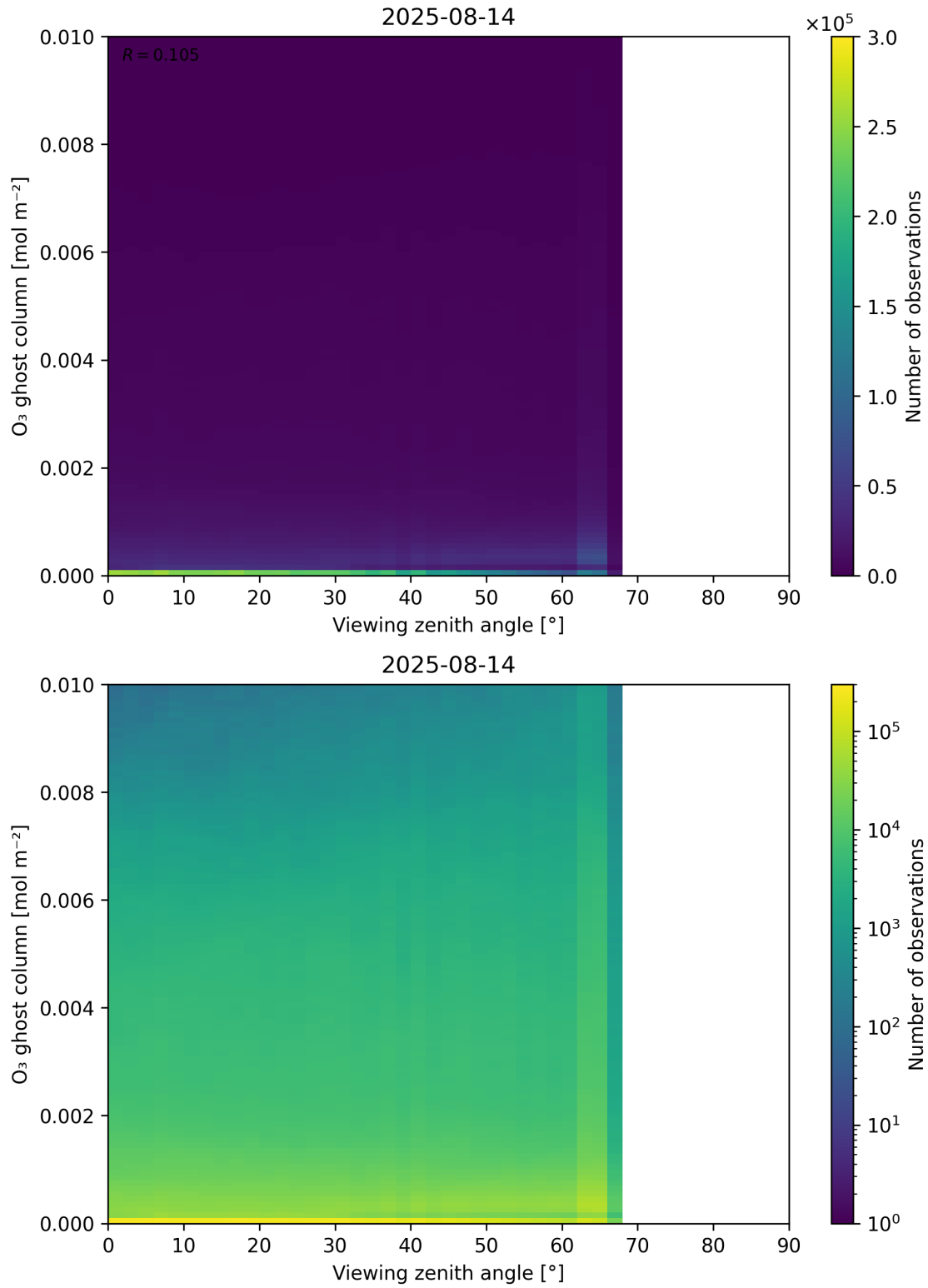
Figure 51: Scatter density plot of “Viewing zenith angle” against “O 3 ghost column” for 2025-08-14 to 2025-08-15.
