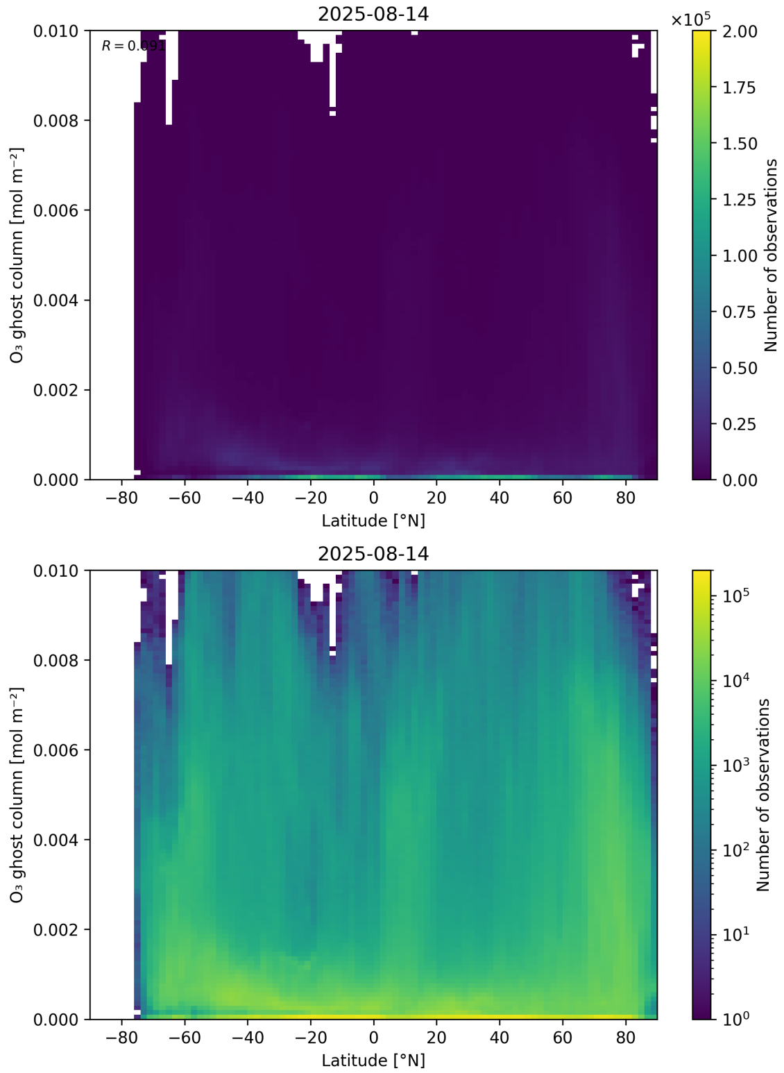
Figure 35: Scatter density plot of “Latitude” against “O 3 ghost column” for 2025-08-14 to 2025-08-15.
