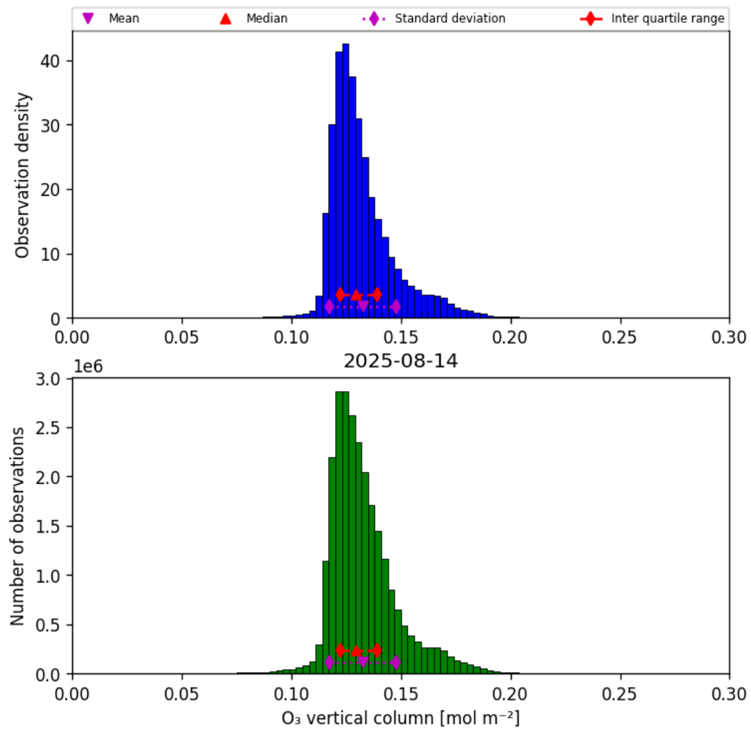
Figure 21: Histogram of “O 3 vertical column” for 2025-08-14 to 2025-08-15
