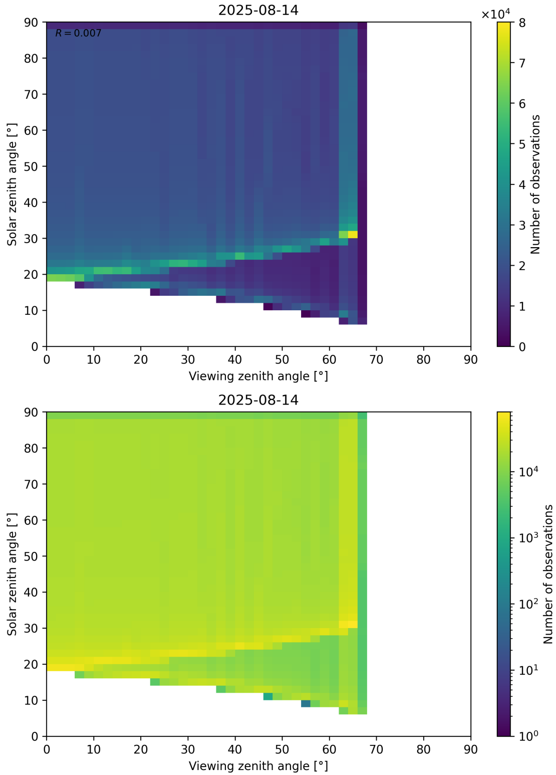
Figure 54: Scatter density plot of “Viewing zenith angle” against “Solar zenith angle” for 2025-08-14 to 2025-08-15.
