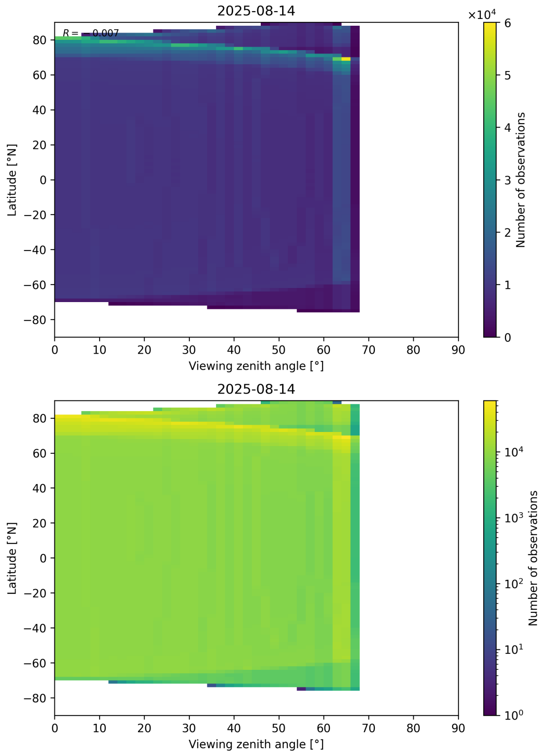
Figure 49: Scatter density plot of “Viewing zenith angle” against “Latitude” for 2025-08-14 to 2025-08-15.
