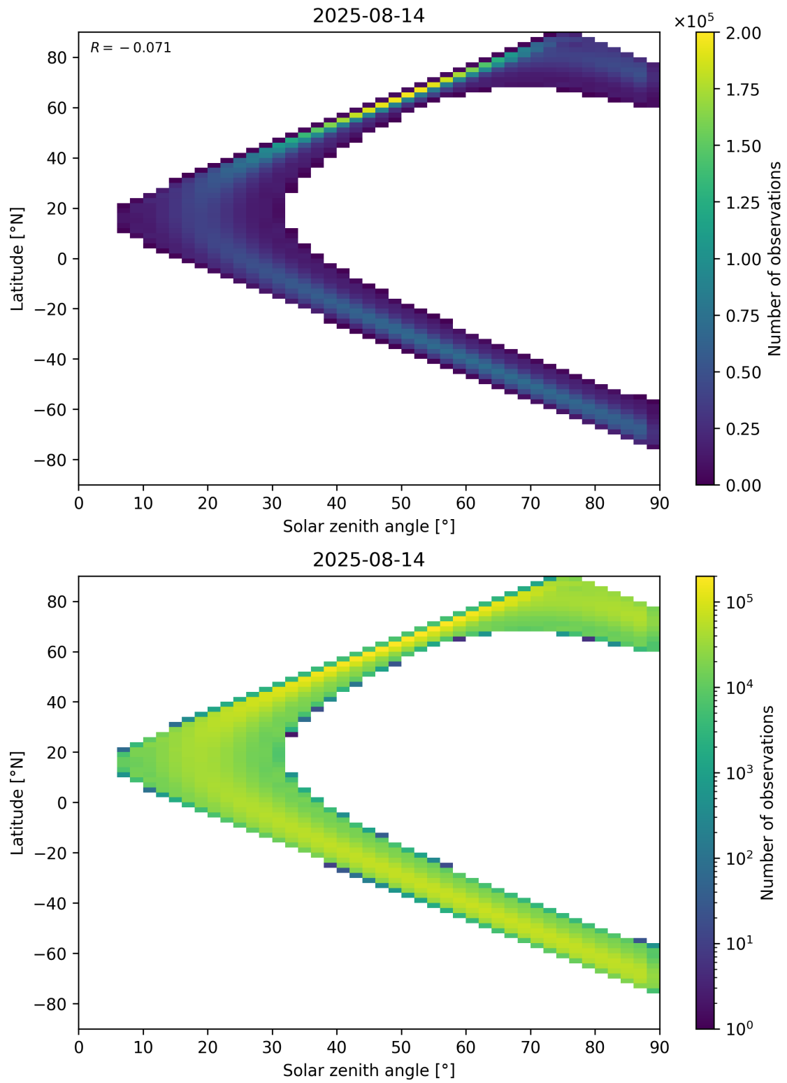
Figure 44: Scatter density plot of “Solar zenith angle” against “Latitude” for 2025-08-14 to 2025-08-15.
