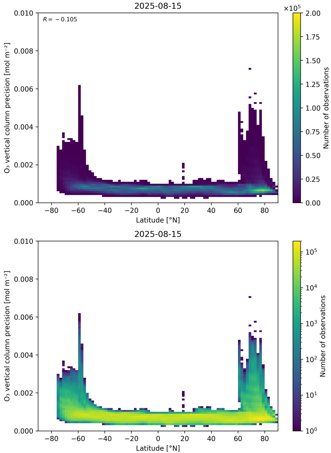
Figure 37: Scatter density plot of “Latitude” against “O 3 vertical column precision” for 2025-08-14 to 2025-08-16.
