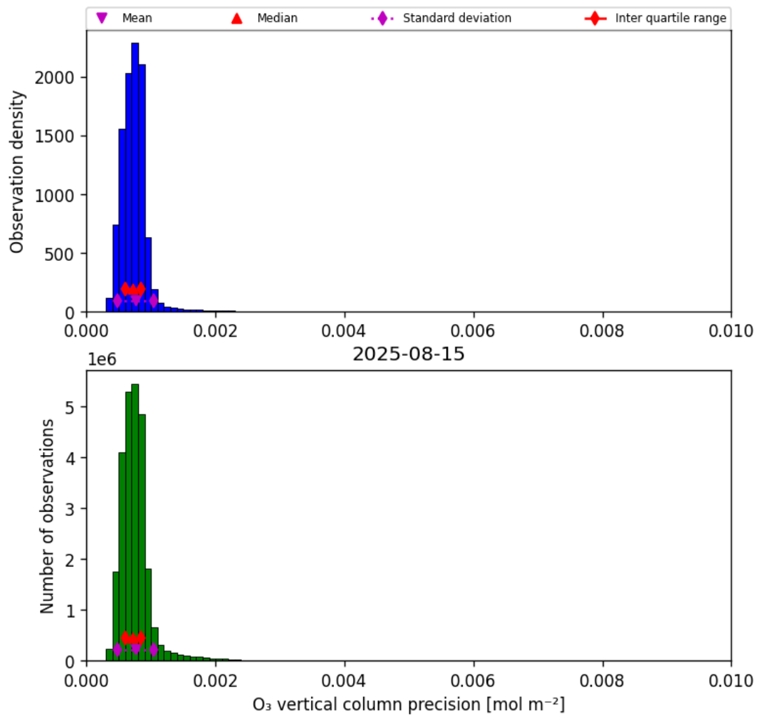
Figure 22: Histogram of “O 3 vertical column precision” for 2025-08-14 to 2025-08-16
