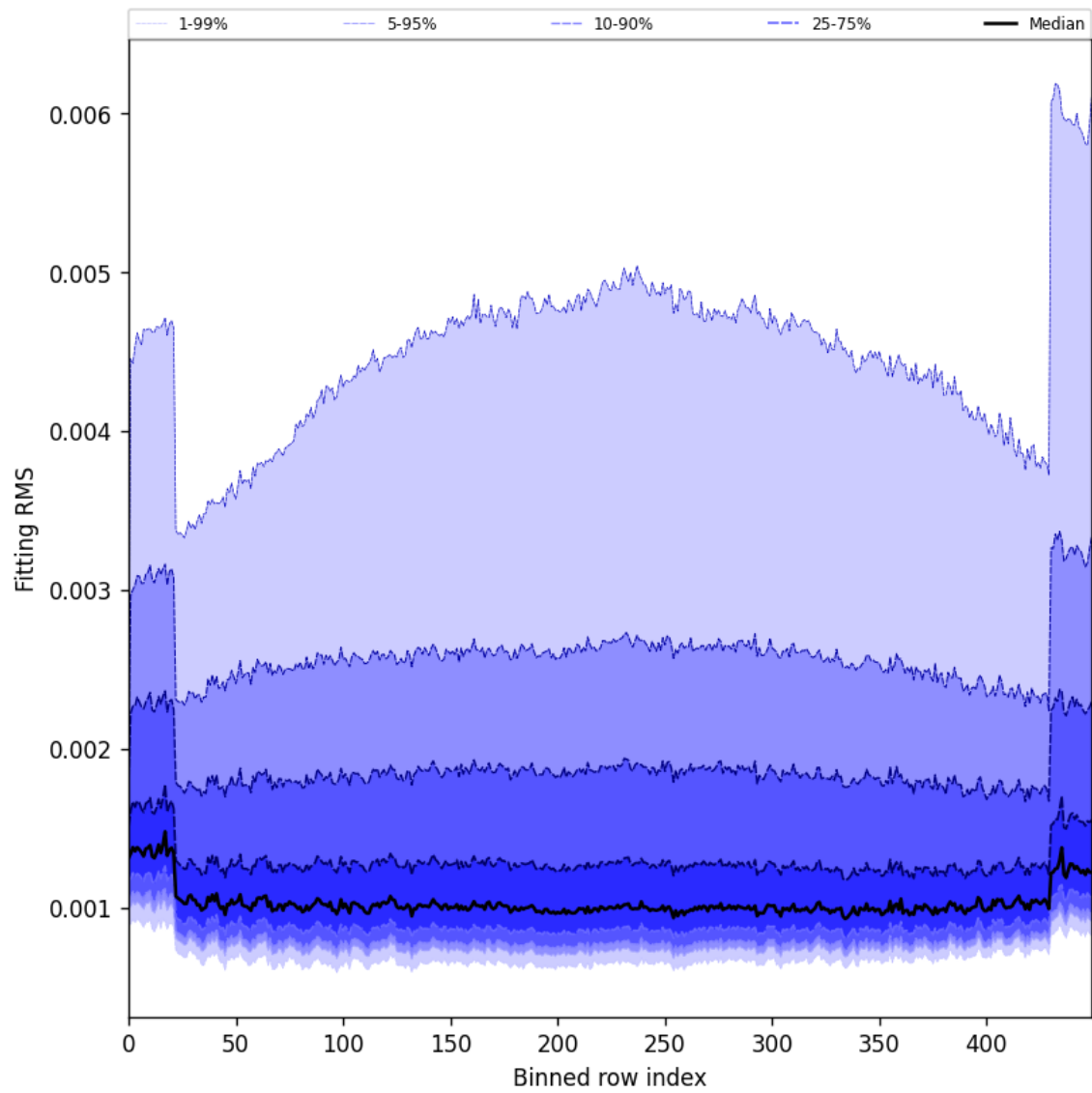
Figure 30: Along track statistics of “Fitting RMS” for 2025-08-14 to 2025-08-16
