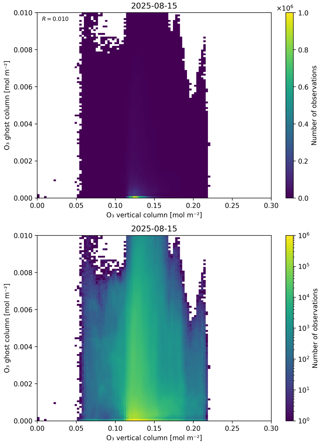
Figure 40: Scatter density plot of “O 3 vertical column” against “O 3 ghost column” for 2025-08-14 to 2025-08-16.
