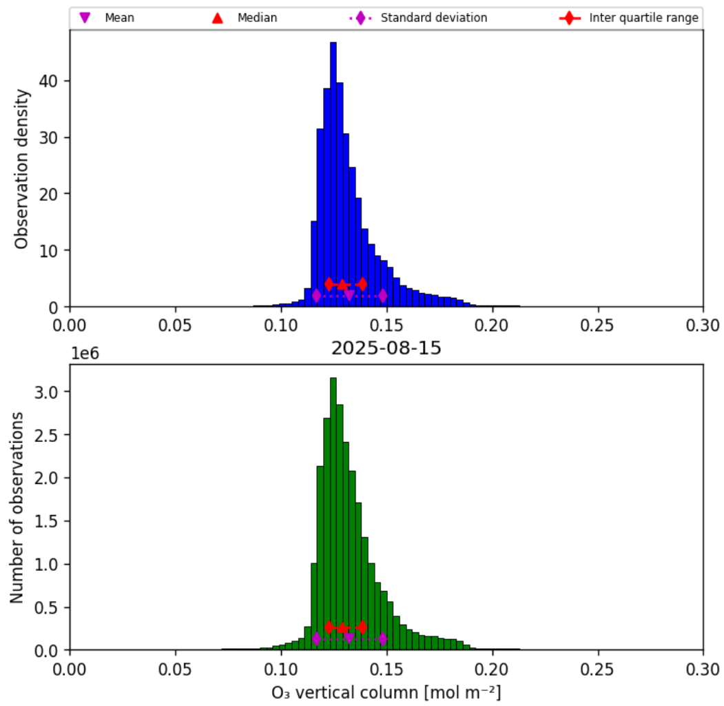
Figure 21: Histogram of “O 3 vertical column” for 2025-08-14 to 2025-08-16
