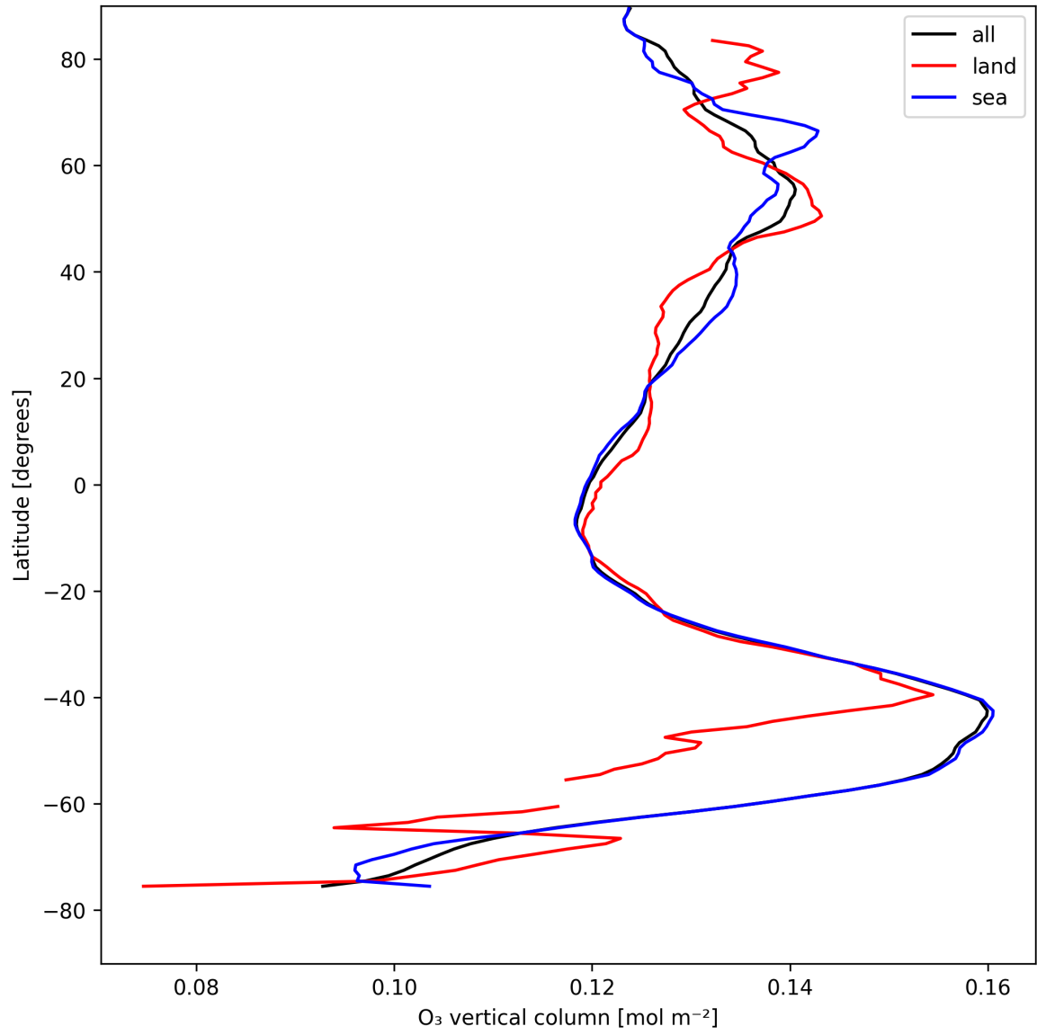
Figure 14: Zonal average of “O 3 vertical column” for 2025-08-14 to 2025-08-16.
