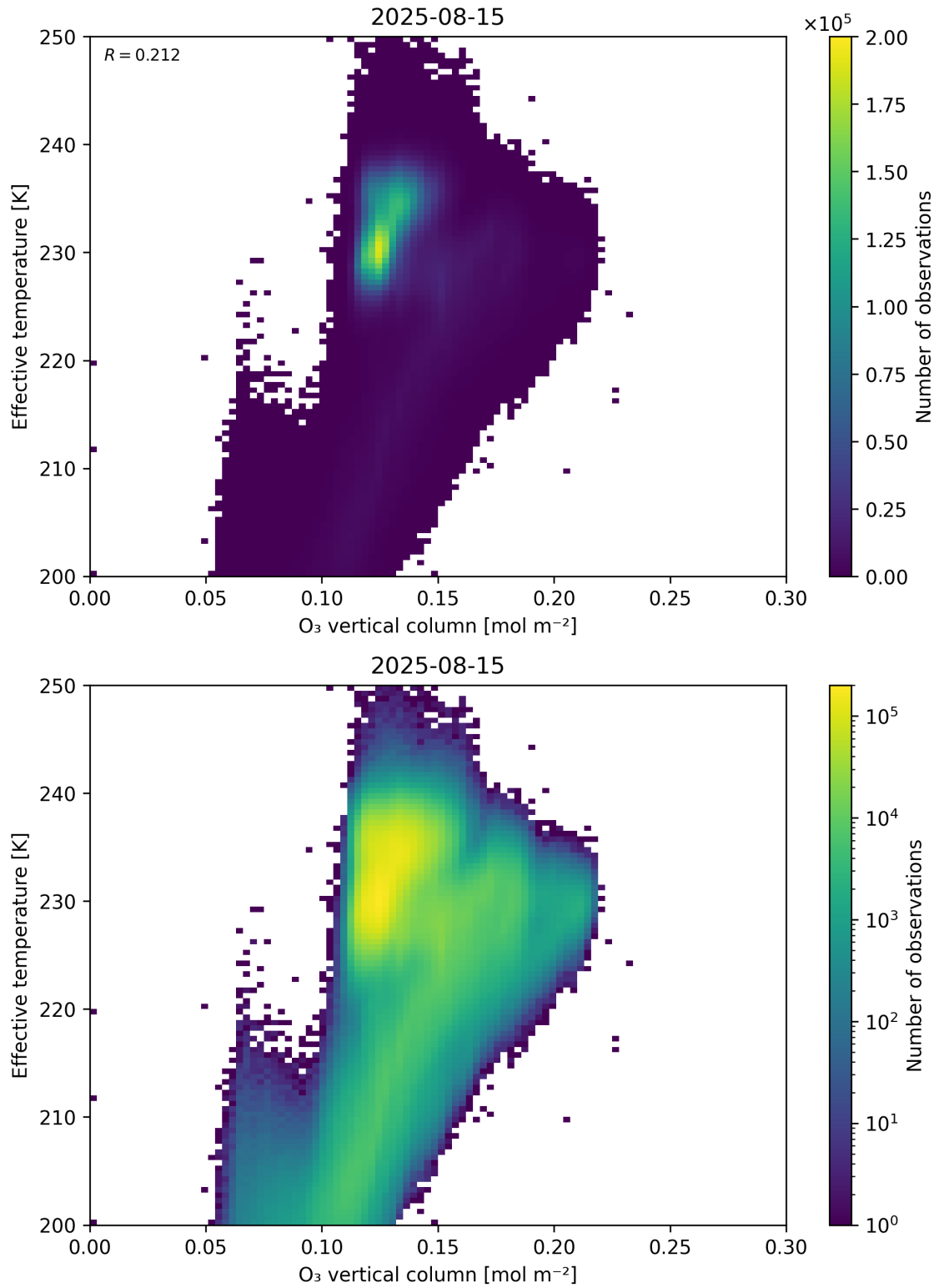
Figure 39: Scatter density plot of “O 3 vertical column” against “Effective temperature” for 2025-08-14 to 2025-08-16.
