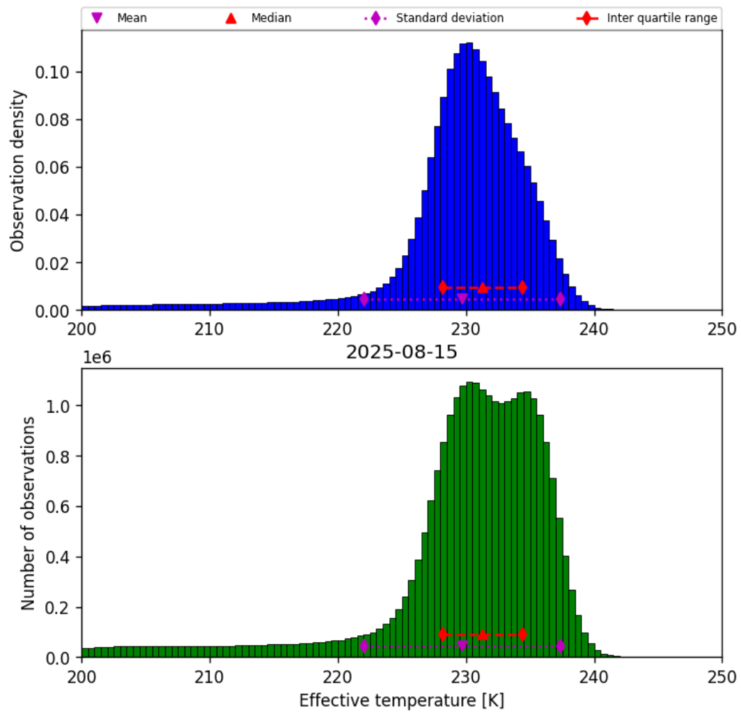
Figure 24: Histogram of “Effective temperature” for 2025-08-14 to 2025-08-16
