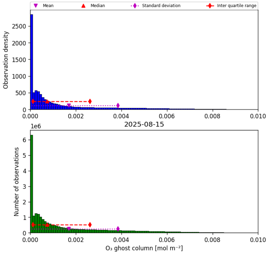
Figure 25: Histogram of “O 3 ghost column” for 2025-08-14 to 2025-08-16
