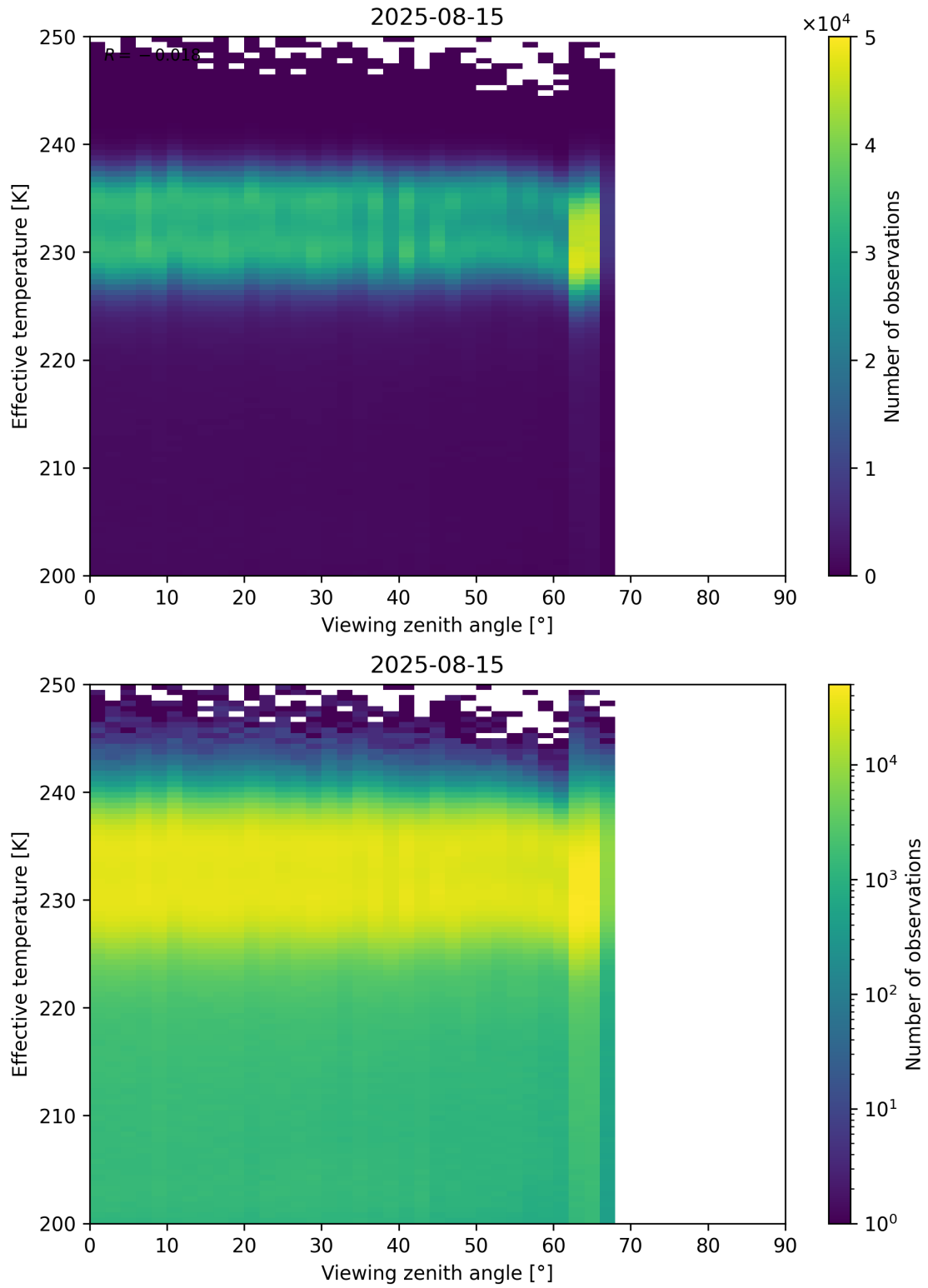
Figure 50: Scatter density plot of “Viewing zenith angle” against “Effective temperature” for 2025-08-14 to 2025-08-16.
