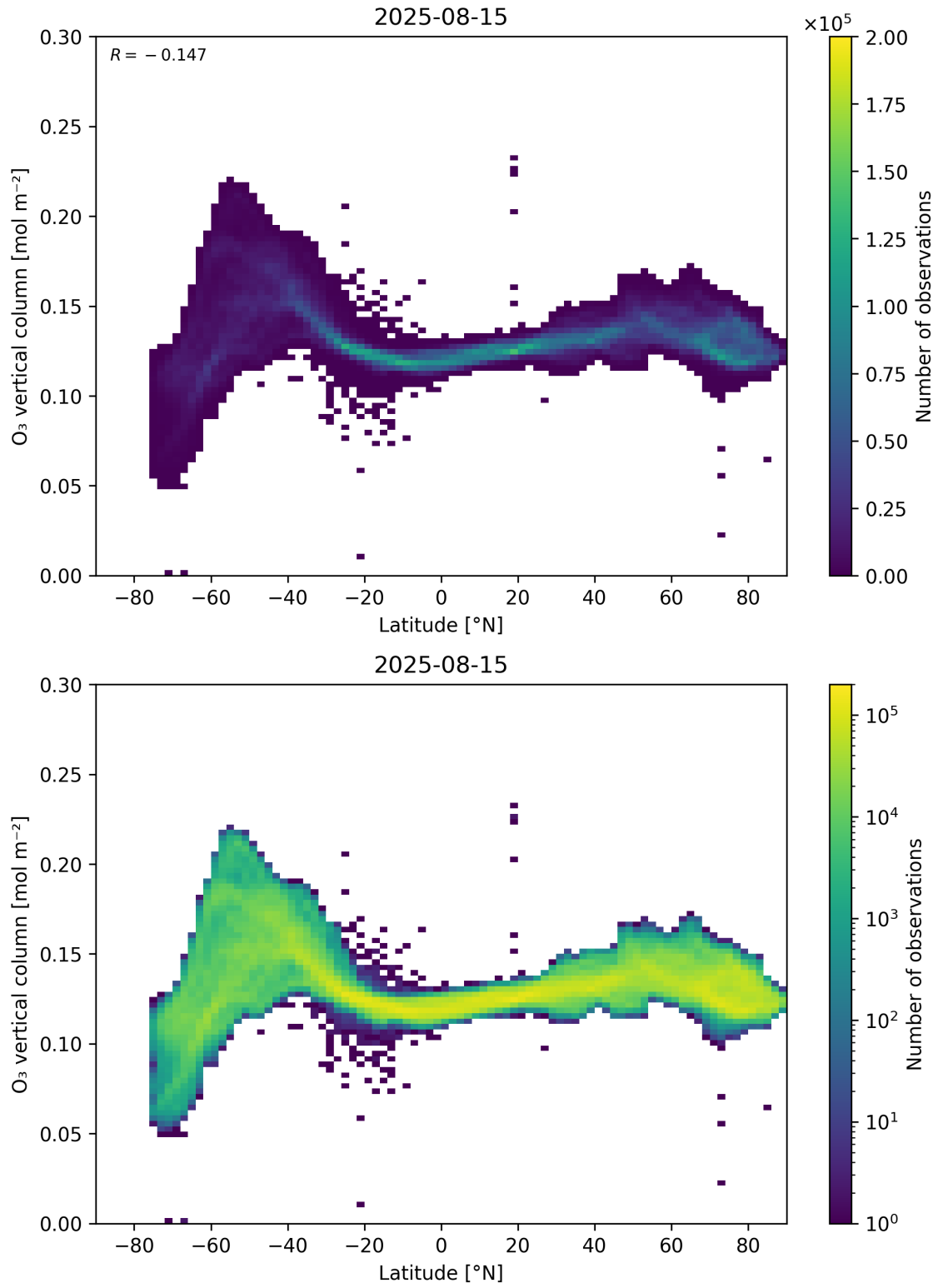
Figure 36: Scatter density plot of “Latitude” against “O 3 vertical column” for 2025-08-14 to 2025-08-16.
