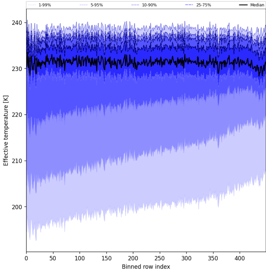
Figure 31: Along track statistics of “Effective temperature” for 2025-08-14 to 2025-08-16
