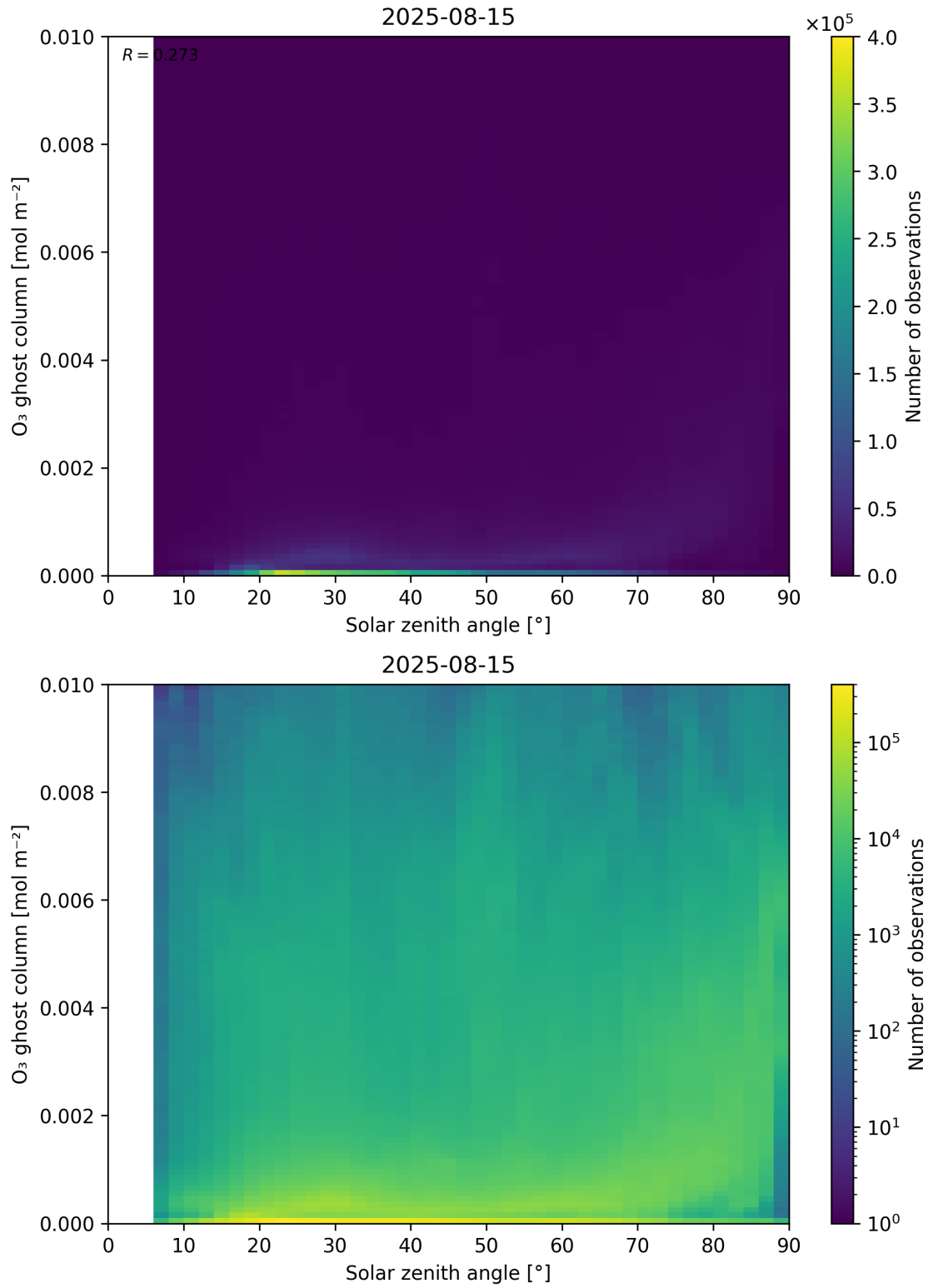
Figure 46: Scatter density plot of “Solar zenith angle” against “O 3 ghost column” for 2025-08-14 to 2025-08-16.
