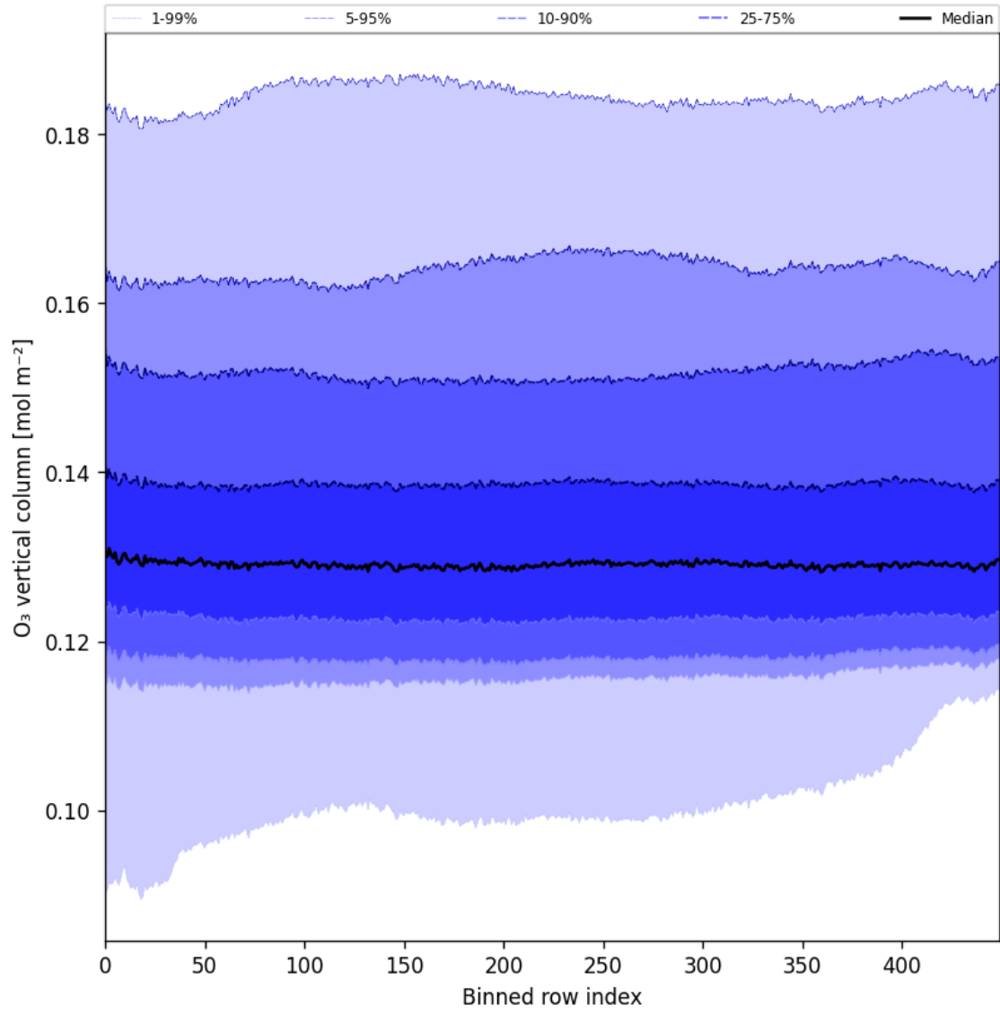
Figure 28: Along track statistics of “O 3 vertical column” for 2025-08-14 to 2025-08-16
