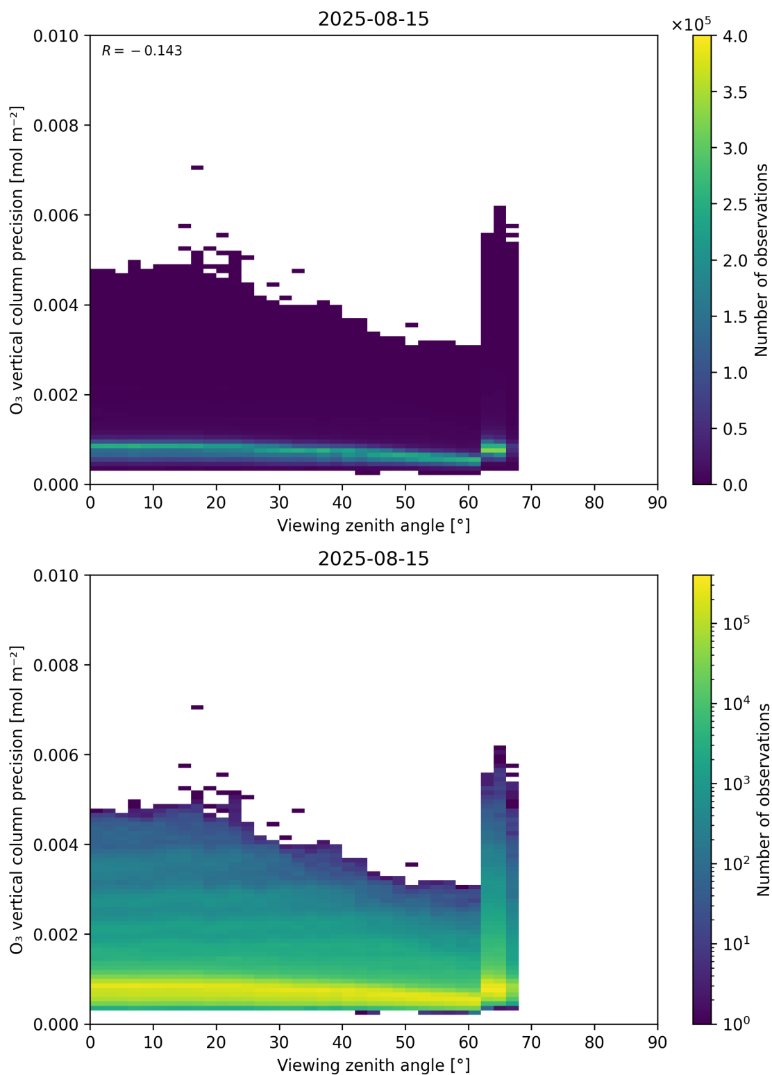
Figure 53: Scatter density plot of “Viewing zenith angle” against “O 3 vertical column precision” for 2025-08-14 to 2025-08-16.
