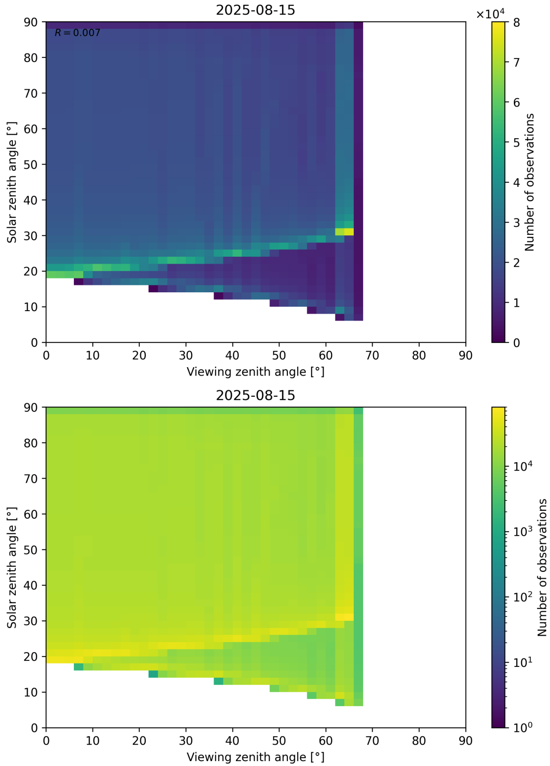
Figure 54: Scatter density plot of “Viewing zenith angle” against “Solar zenith angle” for 2025-08-14 to 2025-08-16.
