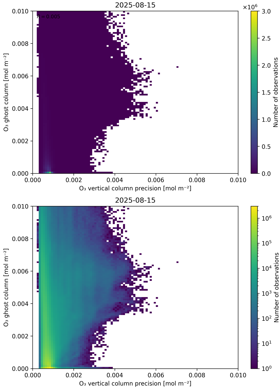
Figure 43: Scatter density plot of “O 3 vertical column precision” against “O 3 ghost column” for 2025-08-14 to 2025-08-16.
