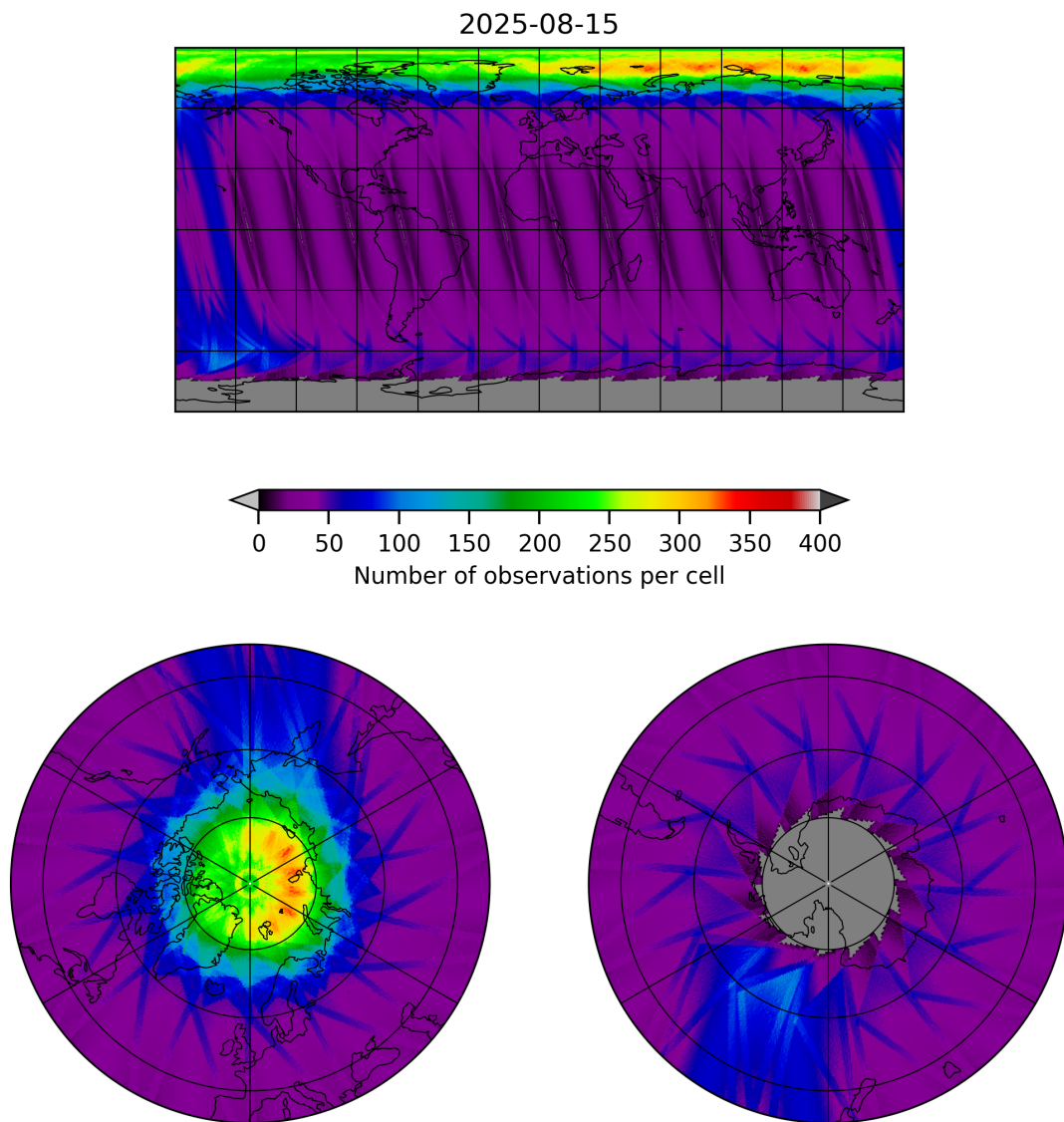
Figure 12: Map of the number of observations for 2025-08-14 to 2025-08-16
