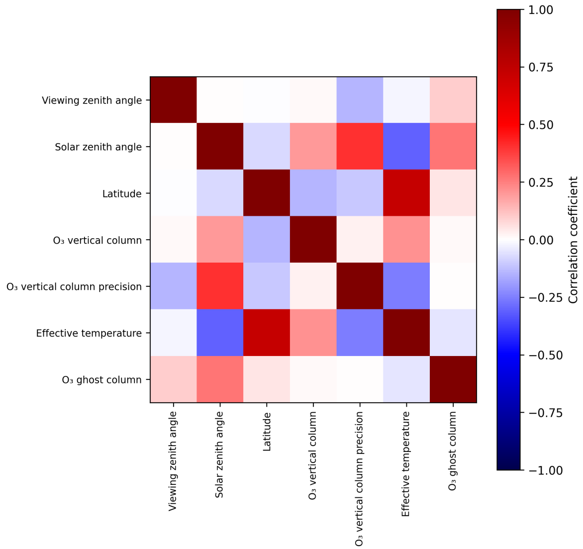
Figure 2: Map of correlation matrix for 2025-08-14 to 2025-08-16.
