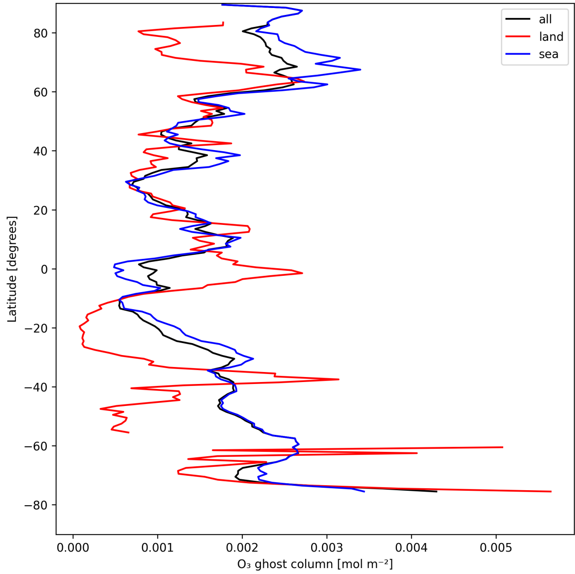
Figure 18: Zonal average of “O 3 ghost column” for 2025-08-14 to 2025-08-16.
