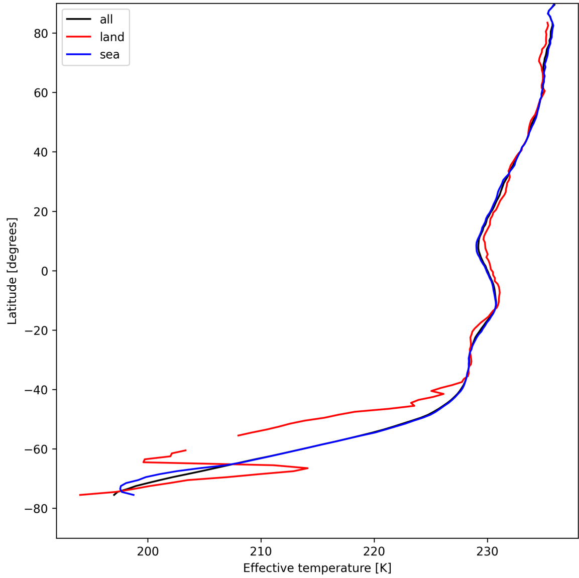
Figure 17: Zonal average of "Effective temperature" for 2025-08-14 to 2025-08-16.
