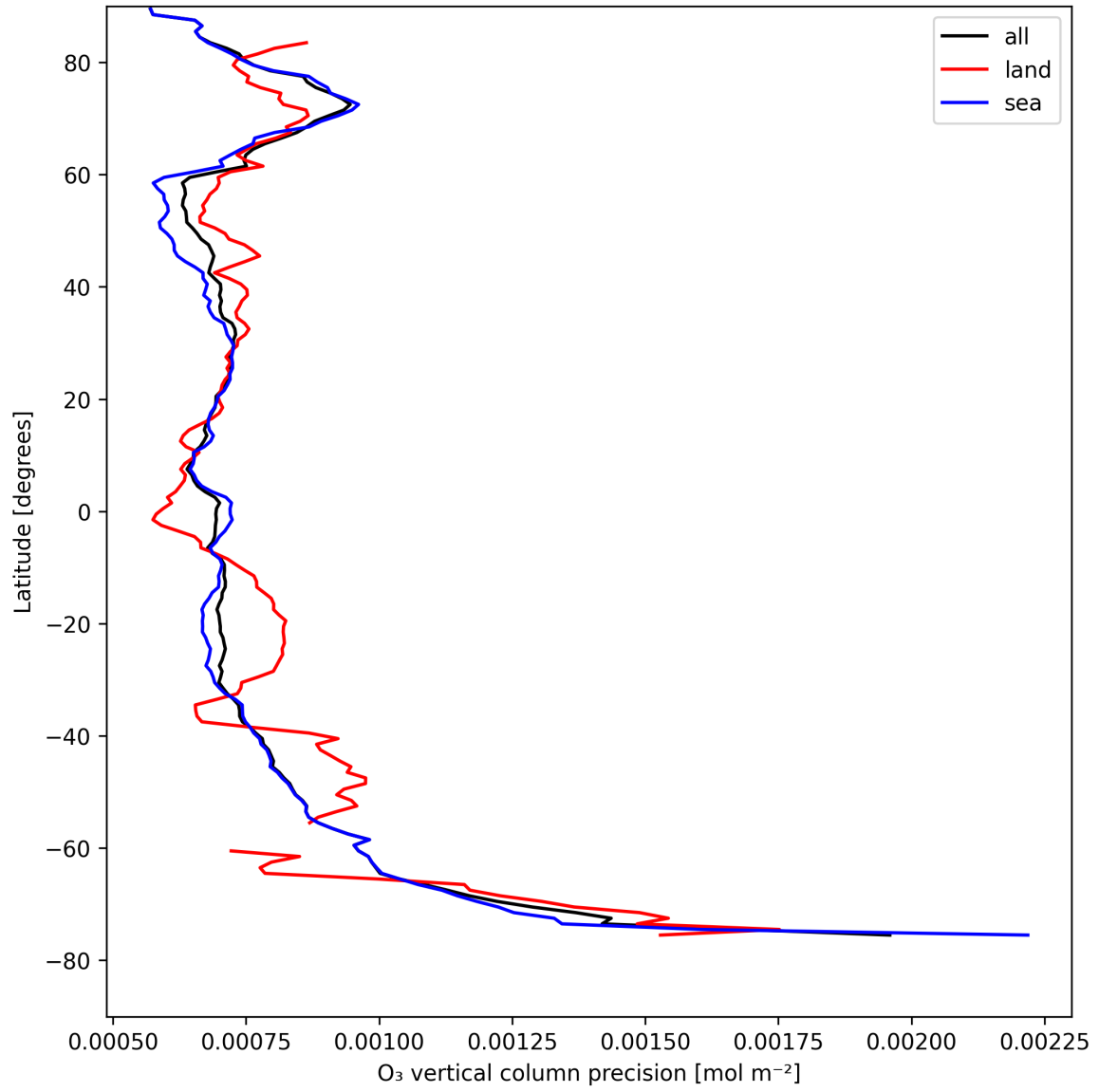
Figure 15: Zonal average of "O 3 vertical column precision" for 2025-08-14 to 2025-08-16.
