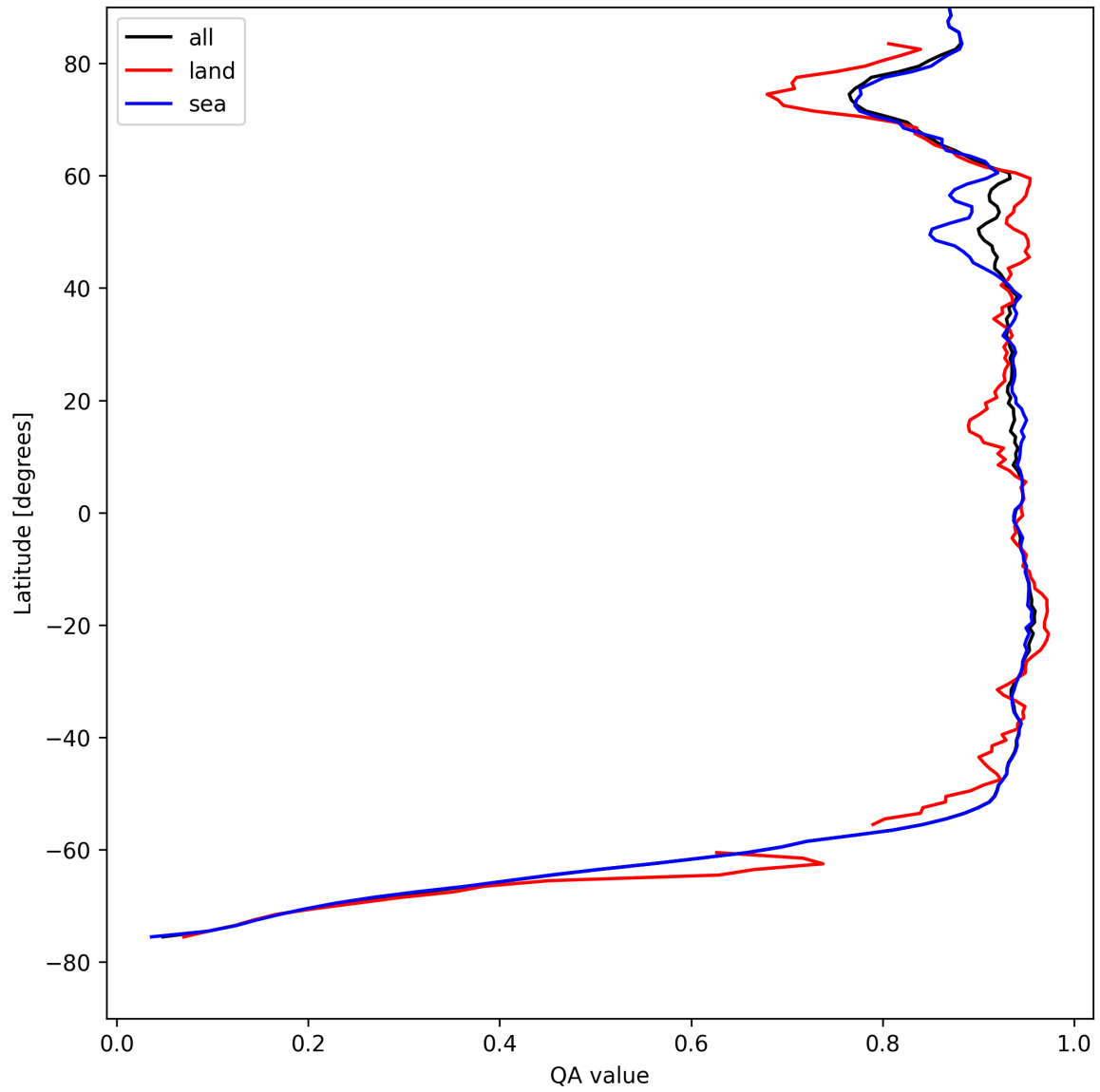
Figure 13: Zonal average of “QA value” for 2025-08-14 to 2025-08-16.
