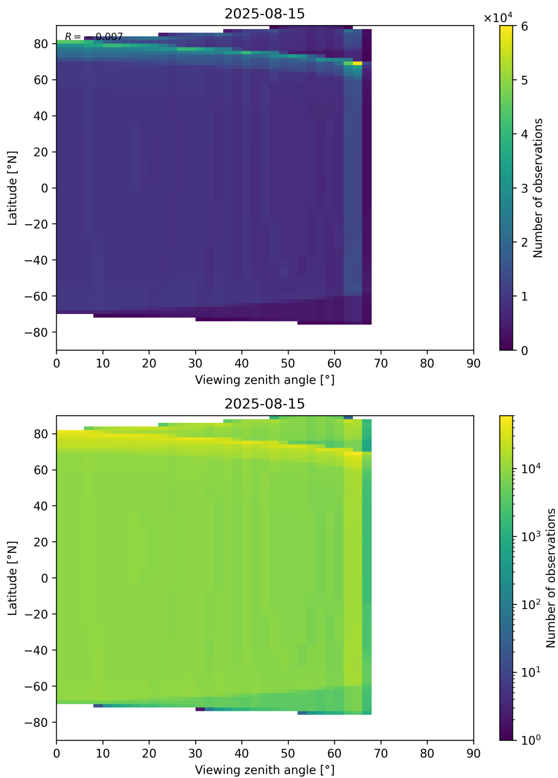
Figure 49: Scatter density plot of “Viewing zenith angle” against “Latitude” for 2025-08-14 to 2025-08-16.
