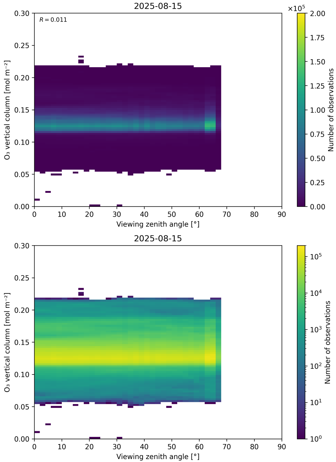
Figure 52: Scatter density plot of “Viewing zenith angle” against “O 3 vertical column” for 2025-08-14 to 2025-08-16.
