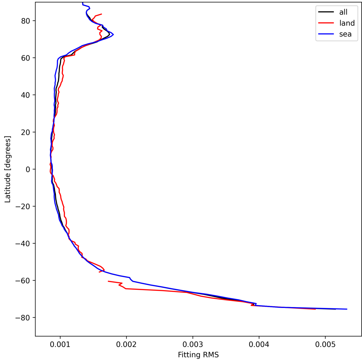
Figure 16: Zonal average of “Fitting RMS” for 2025-08-14 to 2025-08-16.
