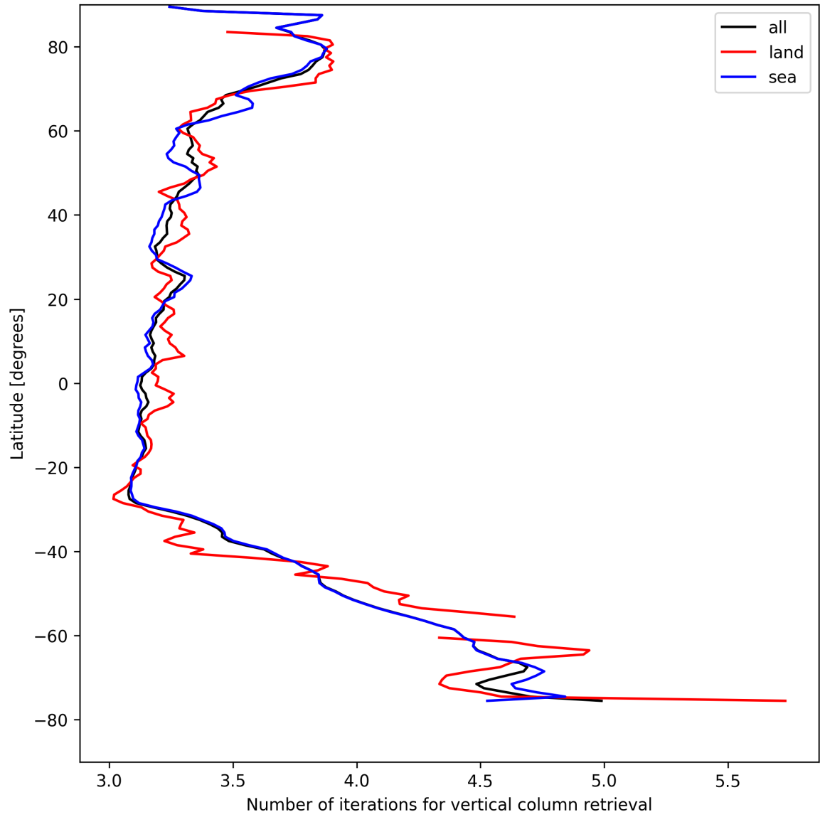
Figure 19: Zonal average of “Number of iterations for vertical column retrieval” for 2025-08-14 to 2025-08-16.
