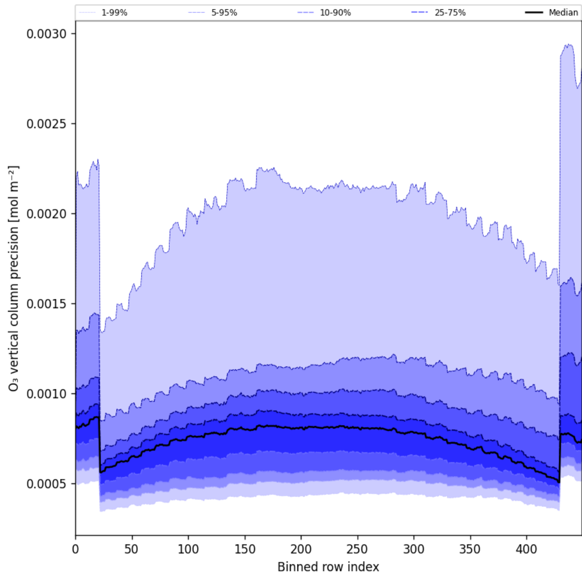
Figure 29: Along track statistics of “O 3 vertical column precision” for 2025-08-14 to 2025-08-16
