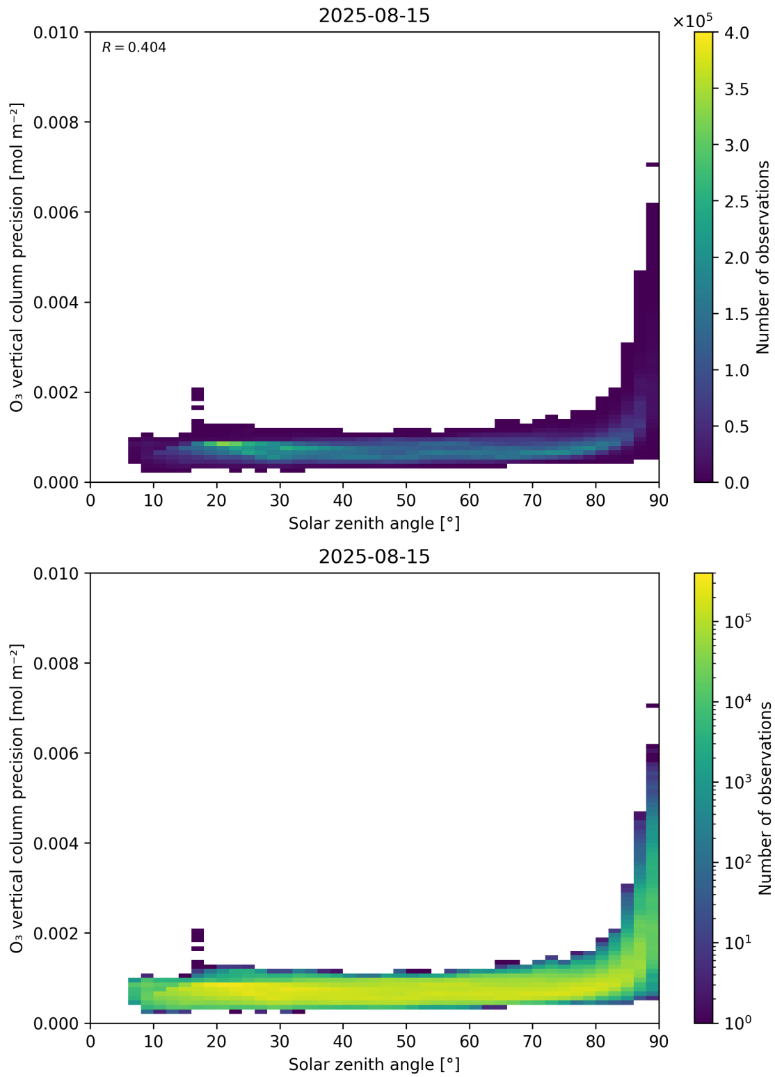
Figure 48: Scatter density plot of “Solar zenith angle” against “O 3 vertical column precision” for 2025-08-14 to 2025-08-16.
