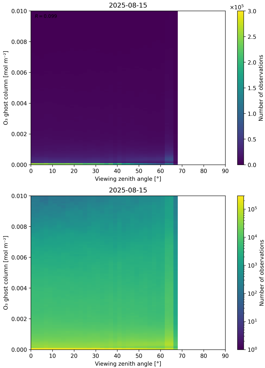
Figure 51: Scatter density plot of “Viewing zenith angle” against “O 3 ghost column” for 2025-08-14 to 2025-08-16.
