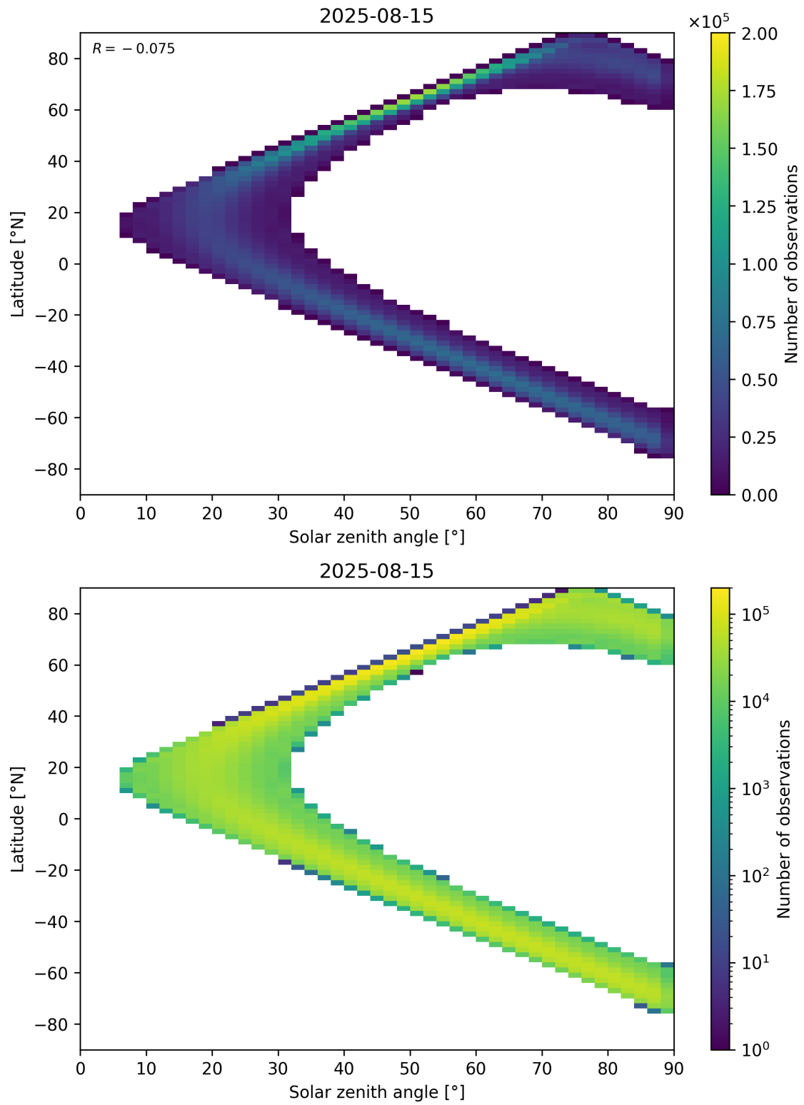
Figure 44: Scatter density plot of “Solar zenith angle” against “Latitude” for 2025-08-14 to 2025-08-16.
