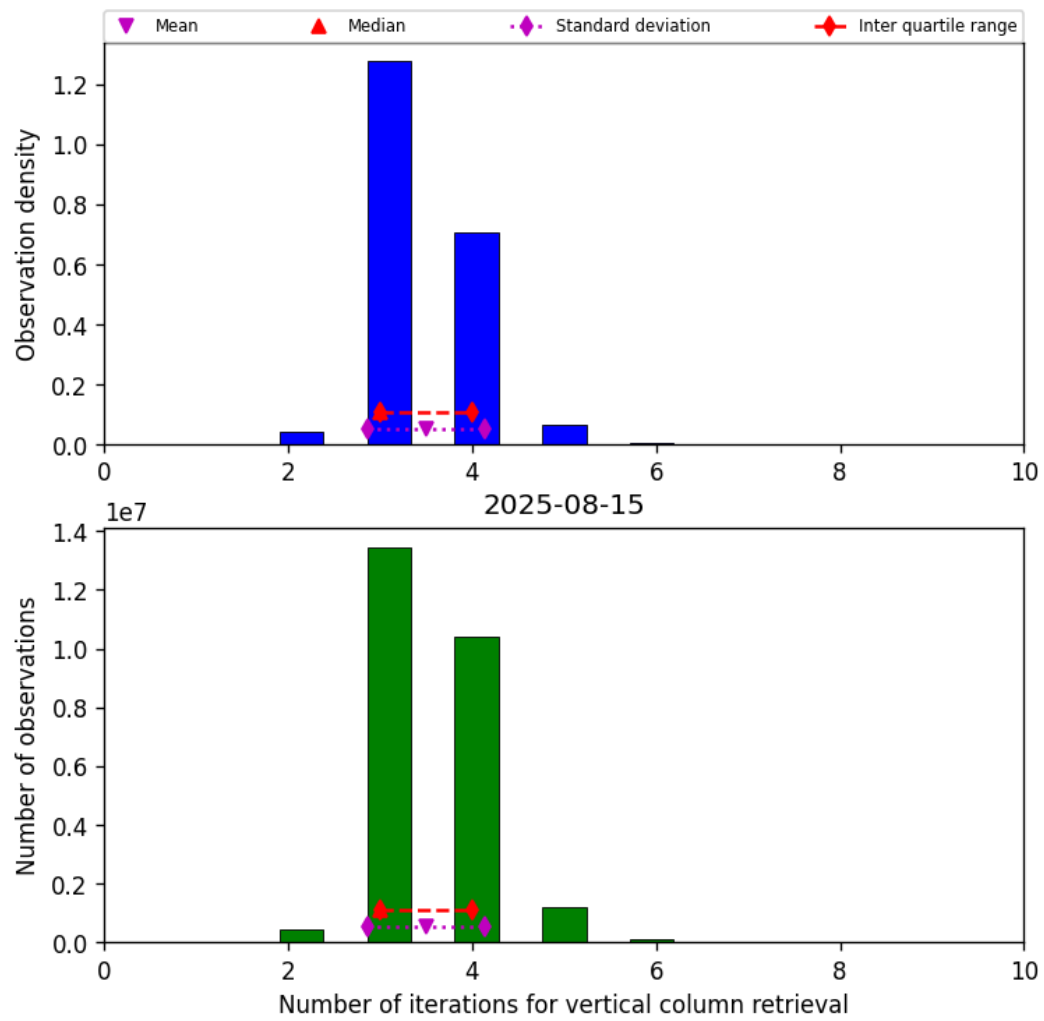
Figure 26: Histogram of “Number of iterations for vertical column retrieval” for 2025-08-14 to 2025-08-16
