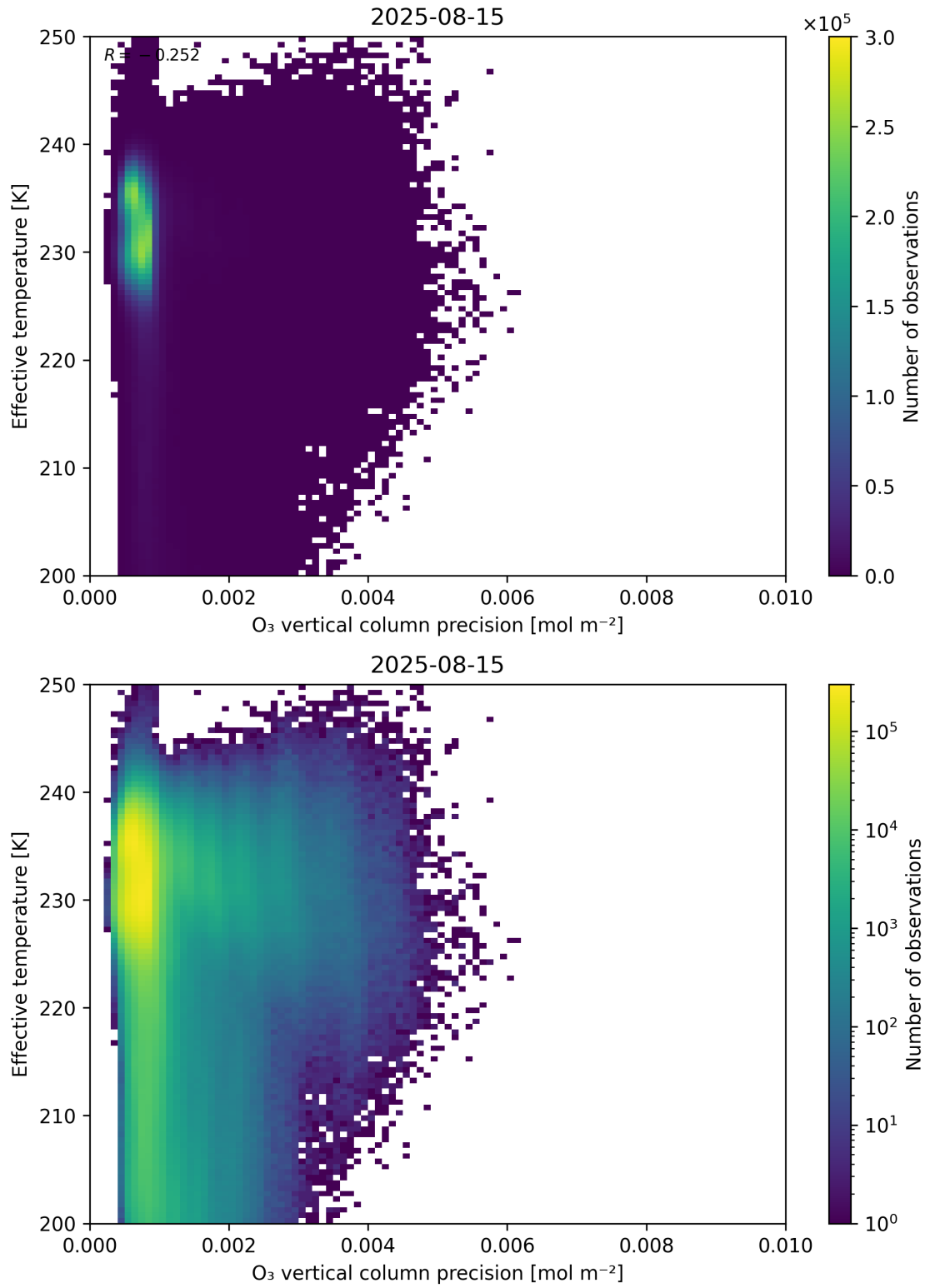
Figure 42: Scatter density plot of “O 3 vertical column precision” against “Effective temperature” for 2025-08-14 to 2025-08-16.
