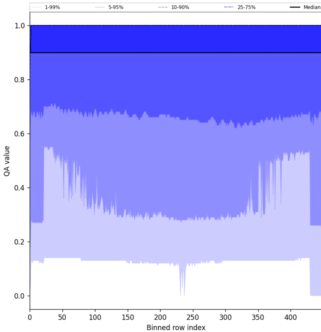
Figure 27: Along track statistics of “QA value” for 2025-08-14 to 2025-08-16
