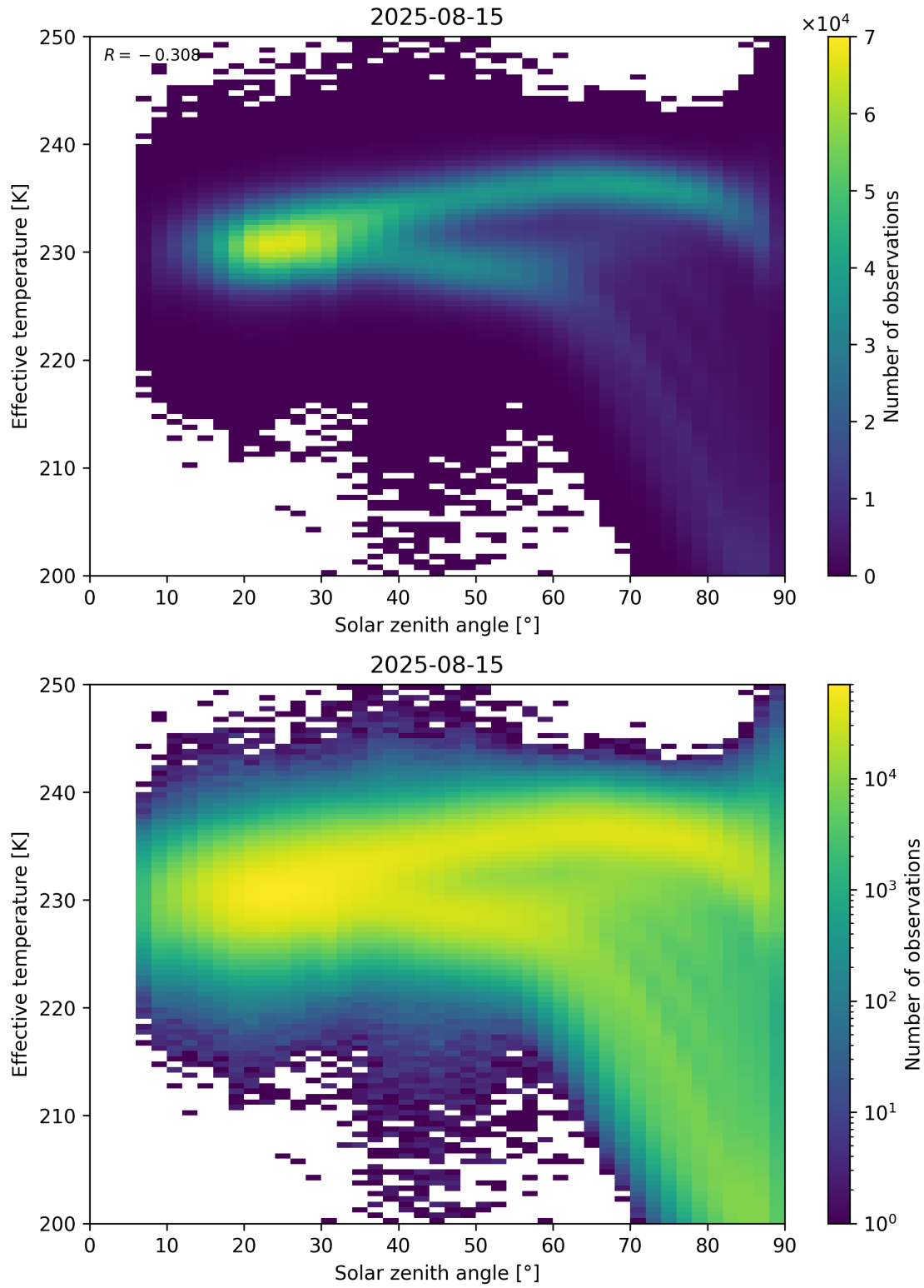
Figure 45: Scatter density plot of “Solar zenith angle” against “Effective temperature” for 2025-08-14 to 2025-08-16.
