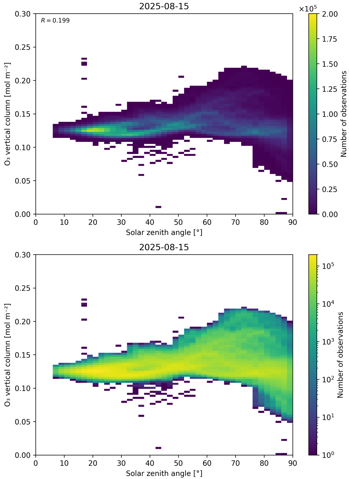
Figure 47: Scatter density plot of “Solar zenith angle” against “O 3 vertical column” for 2025-08-14 to 2025-08-16.
