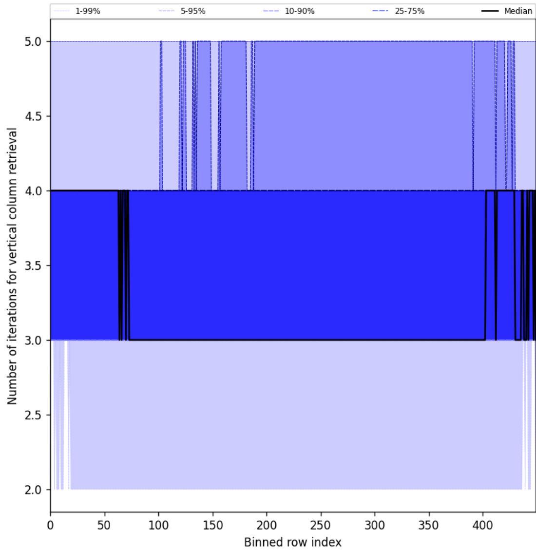
Figure 33: Along track statistics of “Number of iterations for vertical column retrieval” for 2025-08-14 to 2025-08-16
