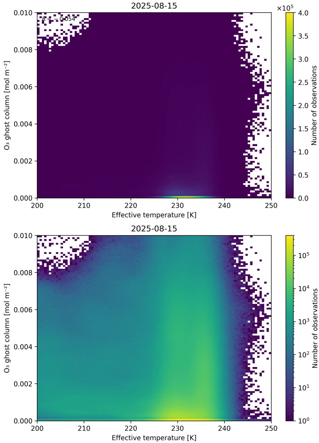
Figure 38: Scatter density plot of “Effective temperature” against “O 3 ghost column” for 2025-08-14 to 2025-08-16.
