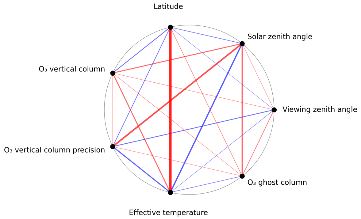
Figure 1: Map of correlation graph for 2025-08-14 to 2025-08-16.
