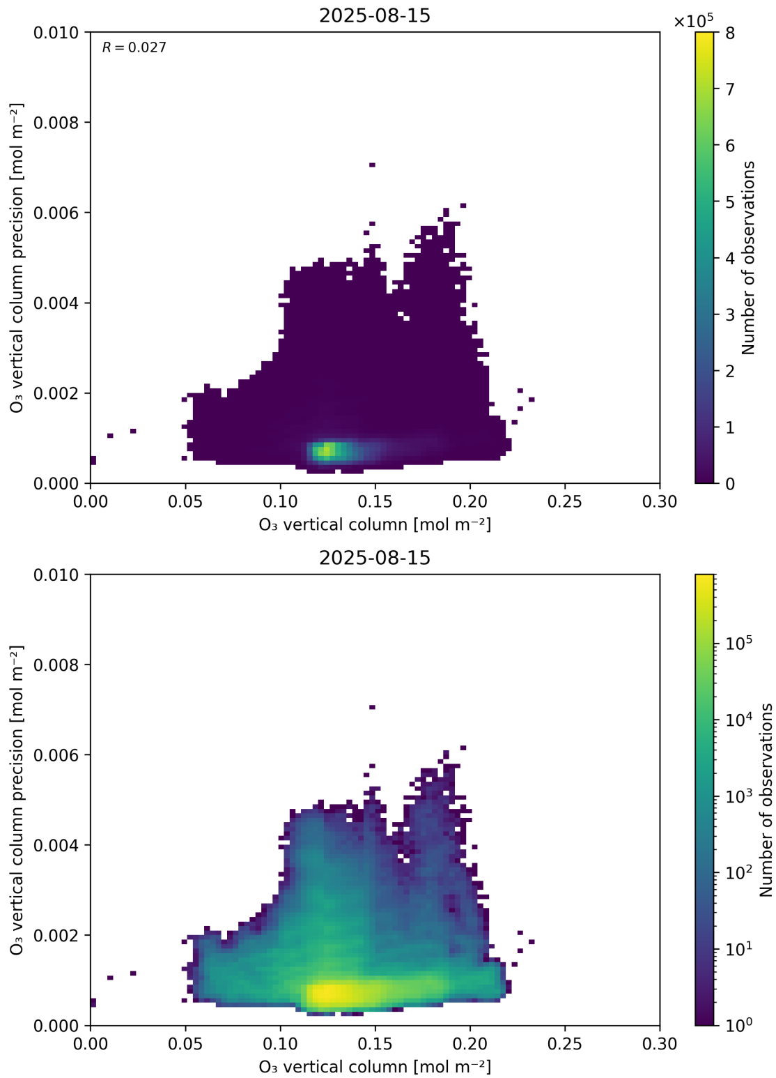
Figure 41: Scatter density plot of “O 3 vertical column” against “O 3 vertical column precision” for 2025-08-14 to 2025-08-16.
