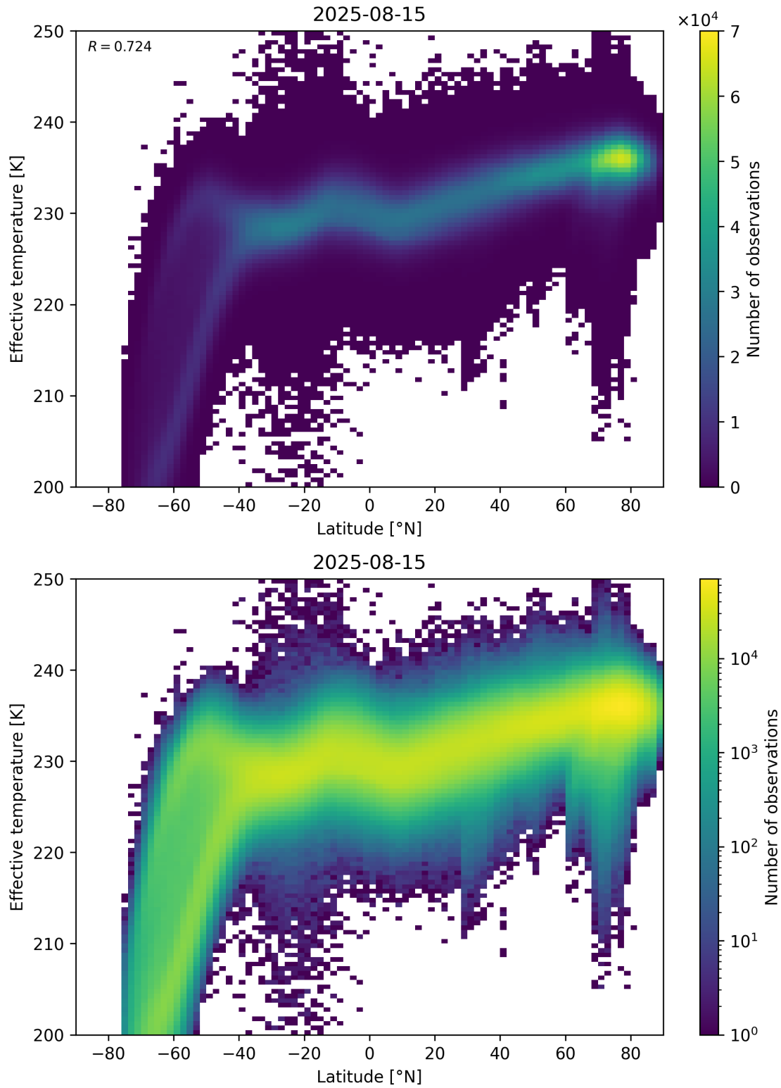
Figure 34: Scatter density plot of “Latitude” against “Effective temperature” for 2025-08-14 to 2025-08-16.
