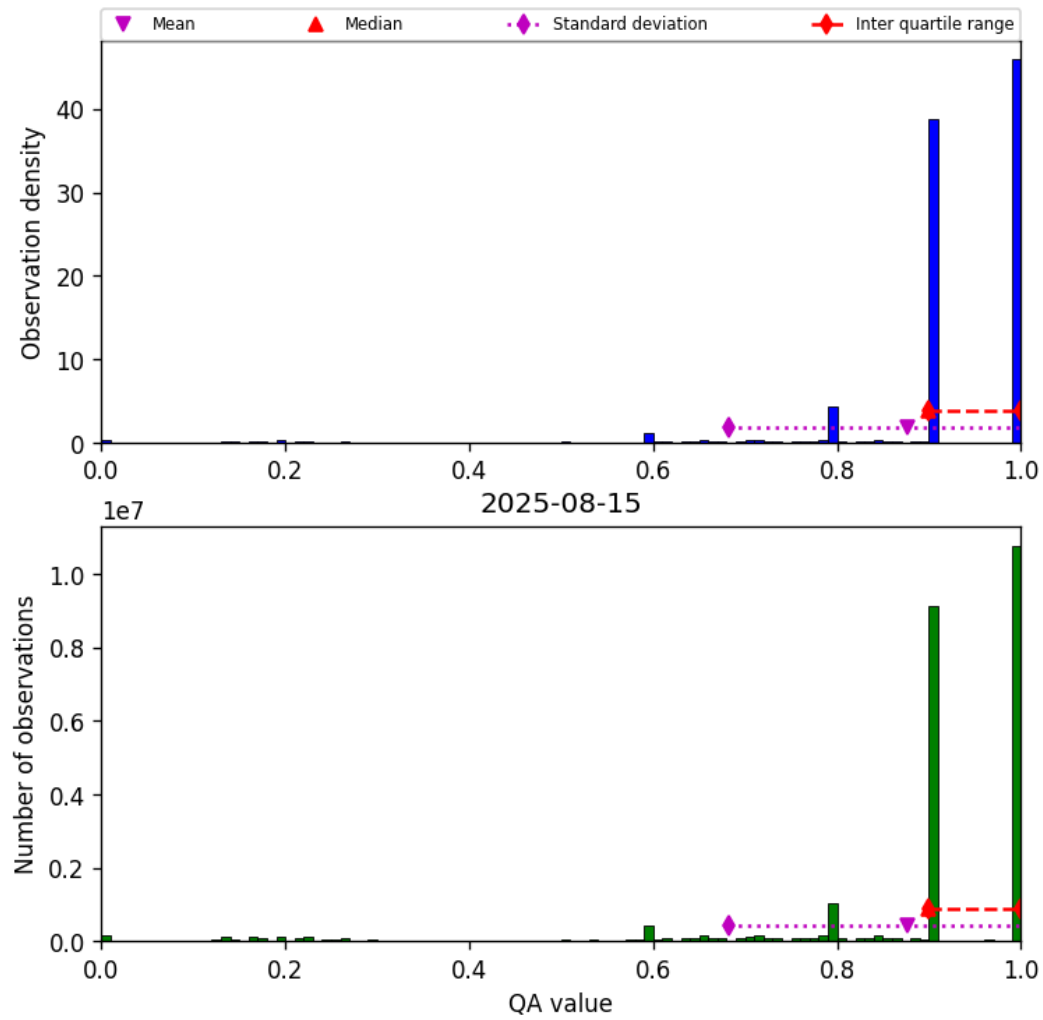
Figure 20: Histogram of “QA value” for 2025-08-14 to 2025-08-16
