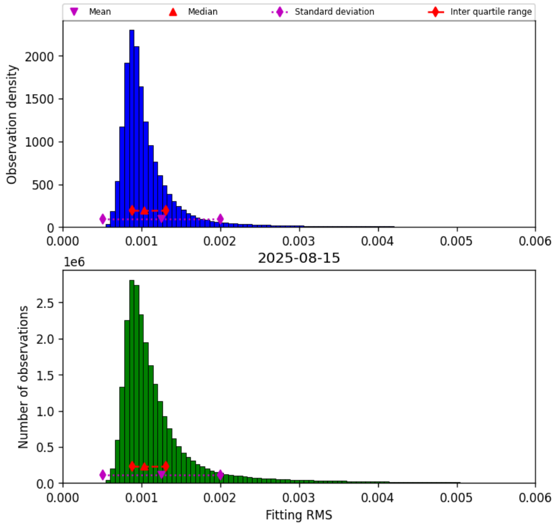
Figure 23: Histogram of “Fitting RMS” for 2025-08-14 to 2025-08-16
