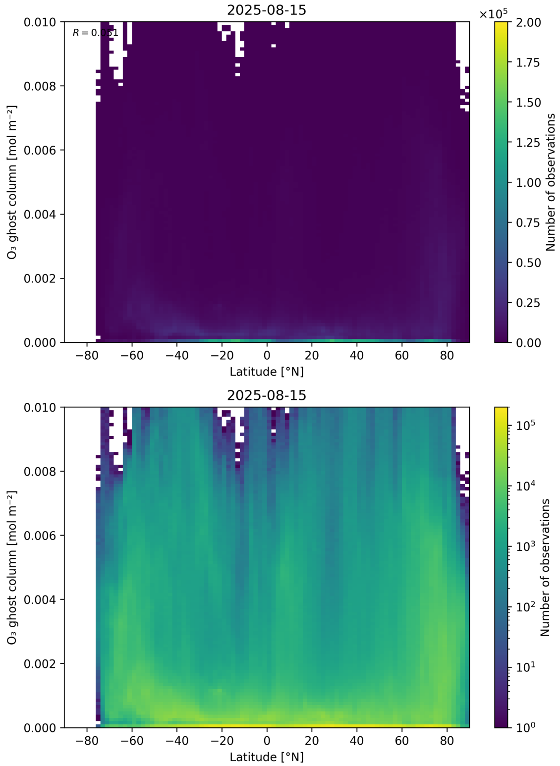
Figure 35: Scatter density plot of “Latitude” against “O 3 ghost column” for 2025-08-14 to 2025-08-16.
