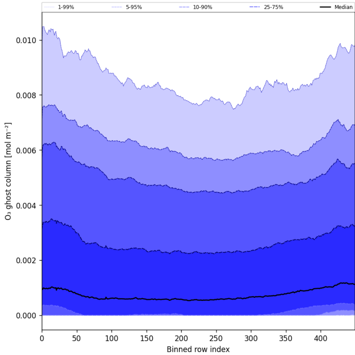
Figure 32: Along track statistics of “O 3 ghost column” for 2025-08-14 to 2025-08-16
