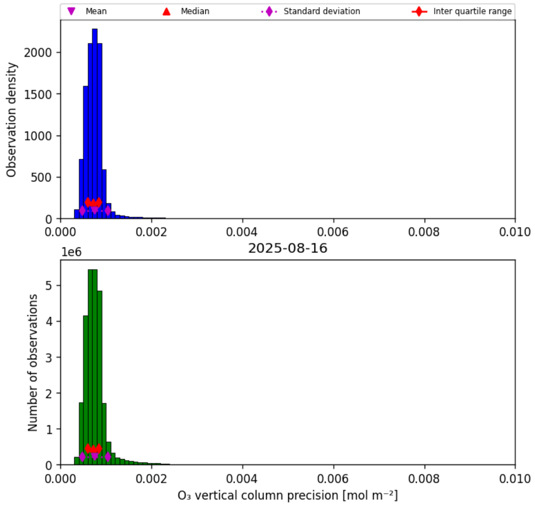
Figure 22: Histogram of “O 3 vertical column precision” for 2025-08-15 to 2025-08-17
