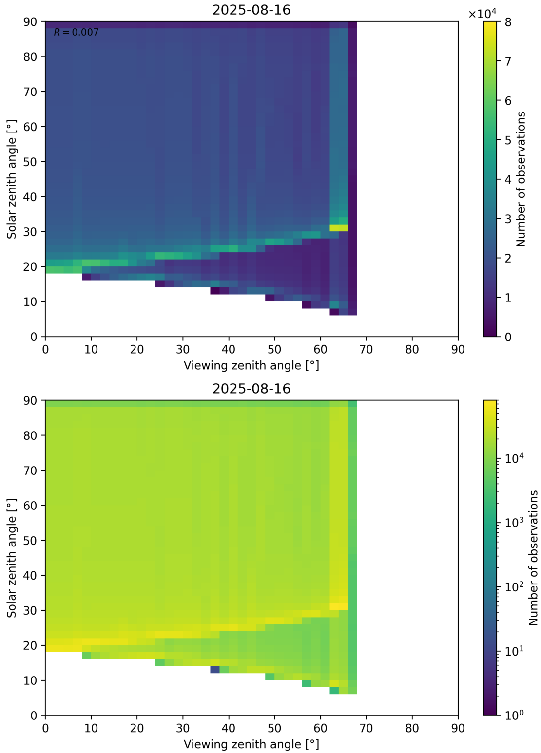
Figure 54: Scatter density plot of “Viewing zenith angle” against “Solar zenith angle” for 2025-08-15 to 2025-08-17.
