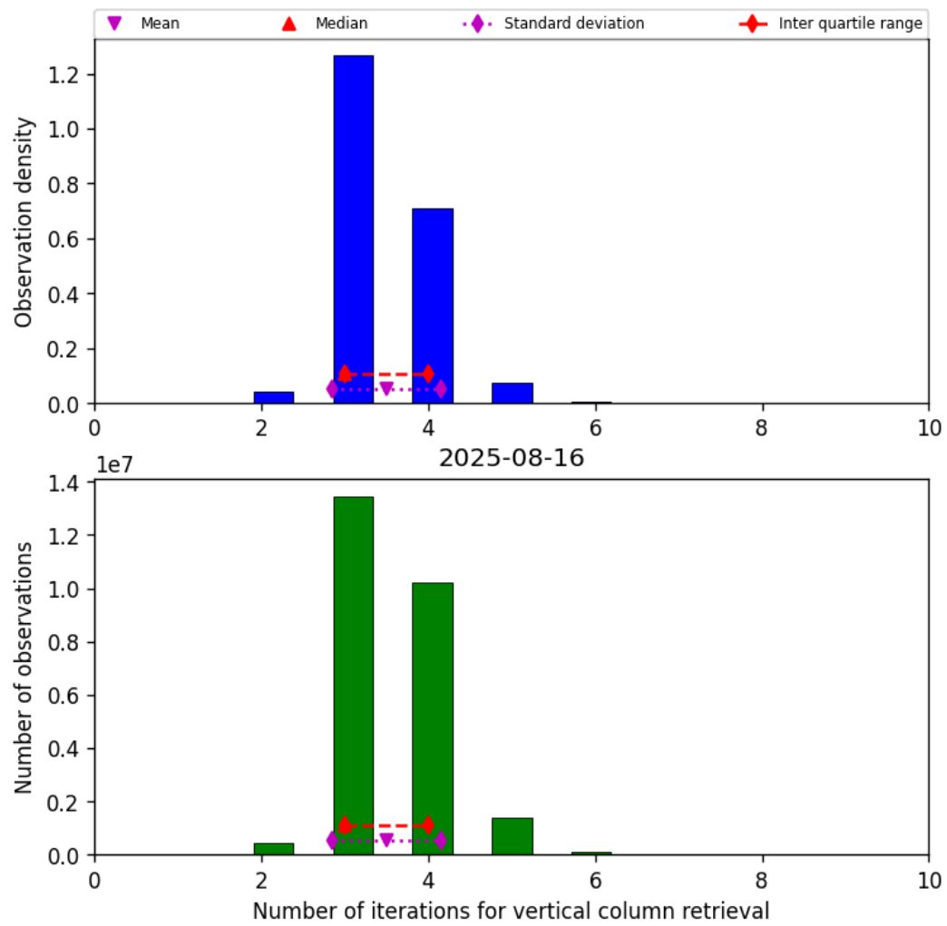
Figure 26: Histogram of “Number of iterations for vertical column retrieval” for 2025-08-15 to 2025-08-17
