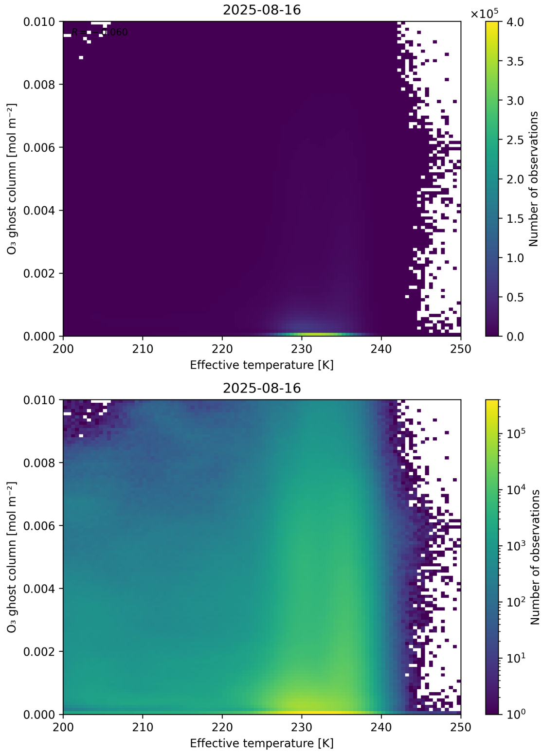
Figure 38: Scatter density plot of “Effective temperature” against “O 3 ghost column” for 2025-08-15 to 2025-08-17.
