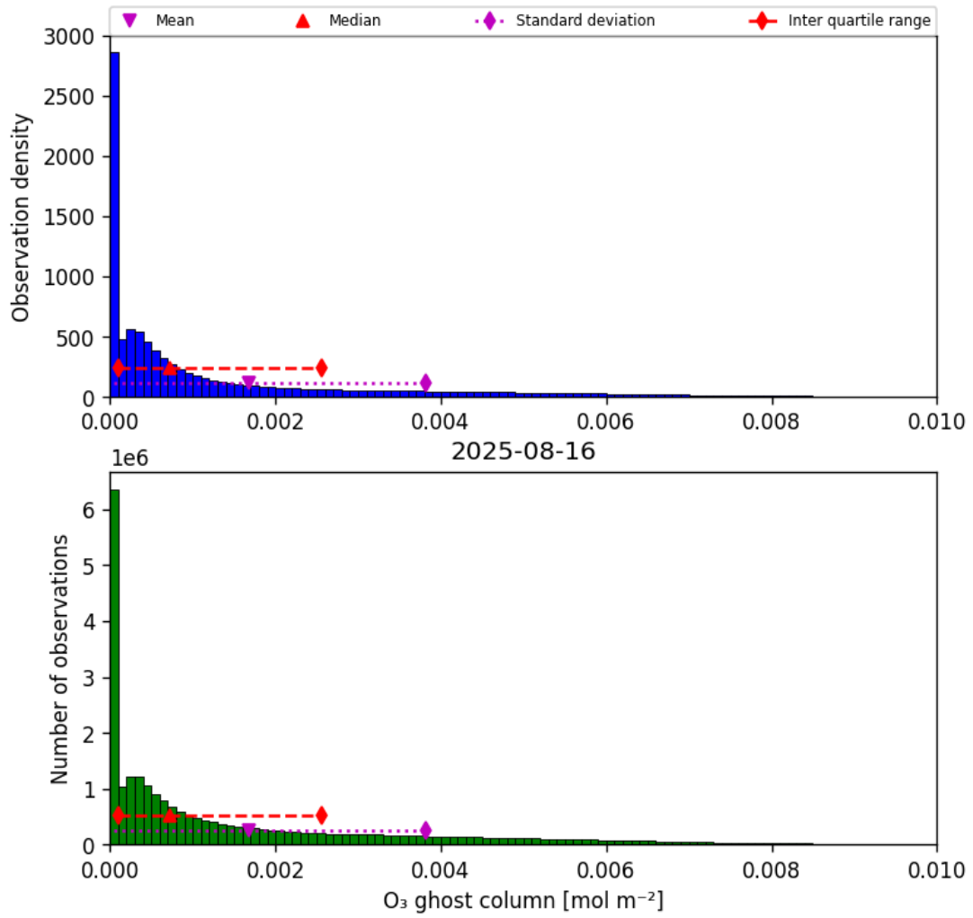
Figure 25: Histogram of “O 3 ghost column” for 2025-08-15 to 2025-08-17
