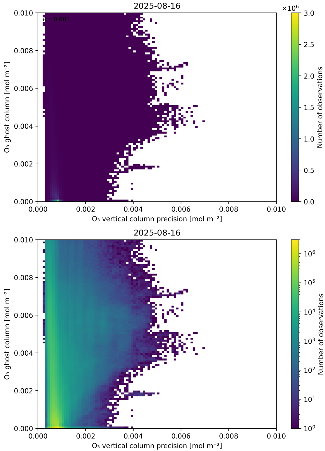
Figure 43: Scatter density plot of “O 3 vertical column precision” against “O 3 ghost column” for 2025-08-15 to 2025-08-17.
