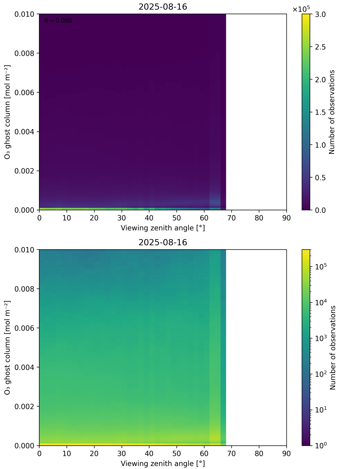
Figure 51: Scatter density plot of “Viewing zenith angle” against “O 3 ghost column” for 2025-08-15 to 2025-08-17.
