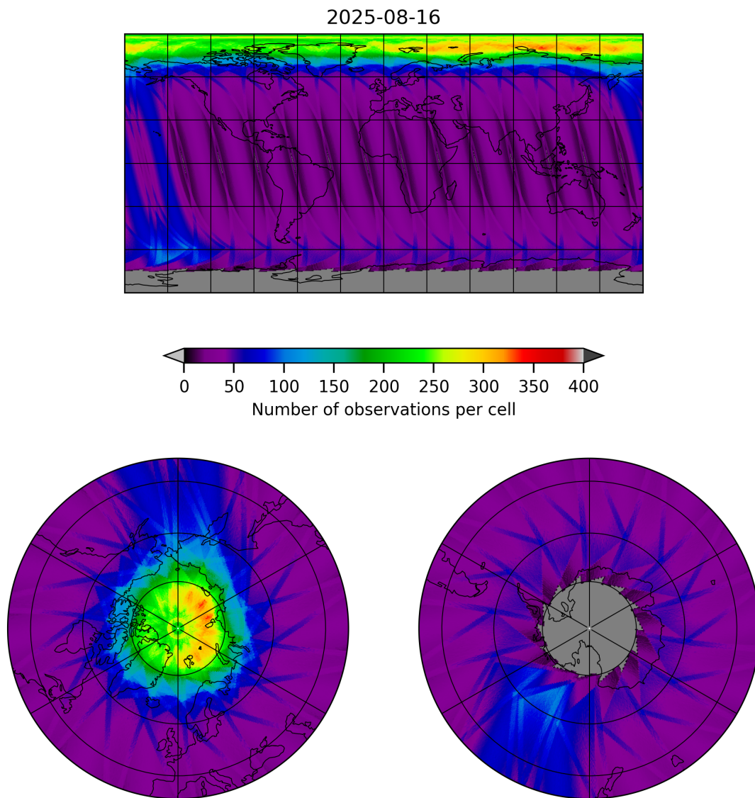
Figure 12: Map of the number of observations for 2025-08-15 to 2025-08-17
