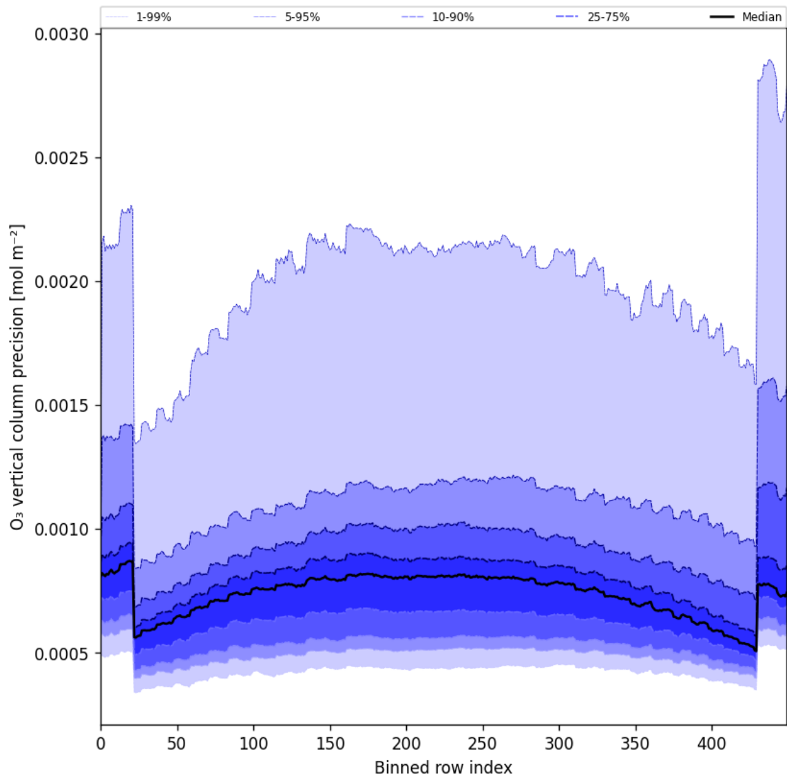
Figure 29: Along track statistics of “O 3 vertical column precision” for 2025-08-15 to 2025-08-17
