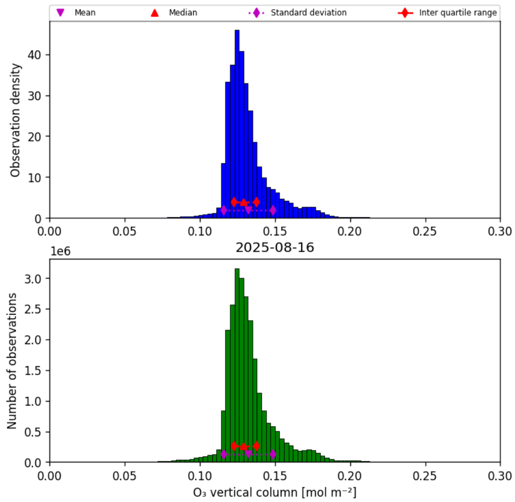
Figure 21: Histogram of “O 3 vertical column” for 2025-08-15 to 2025-08-17
