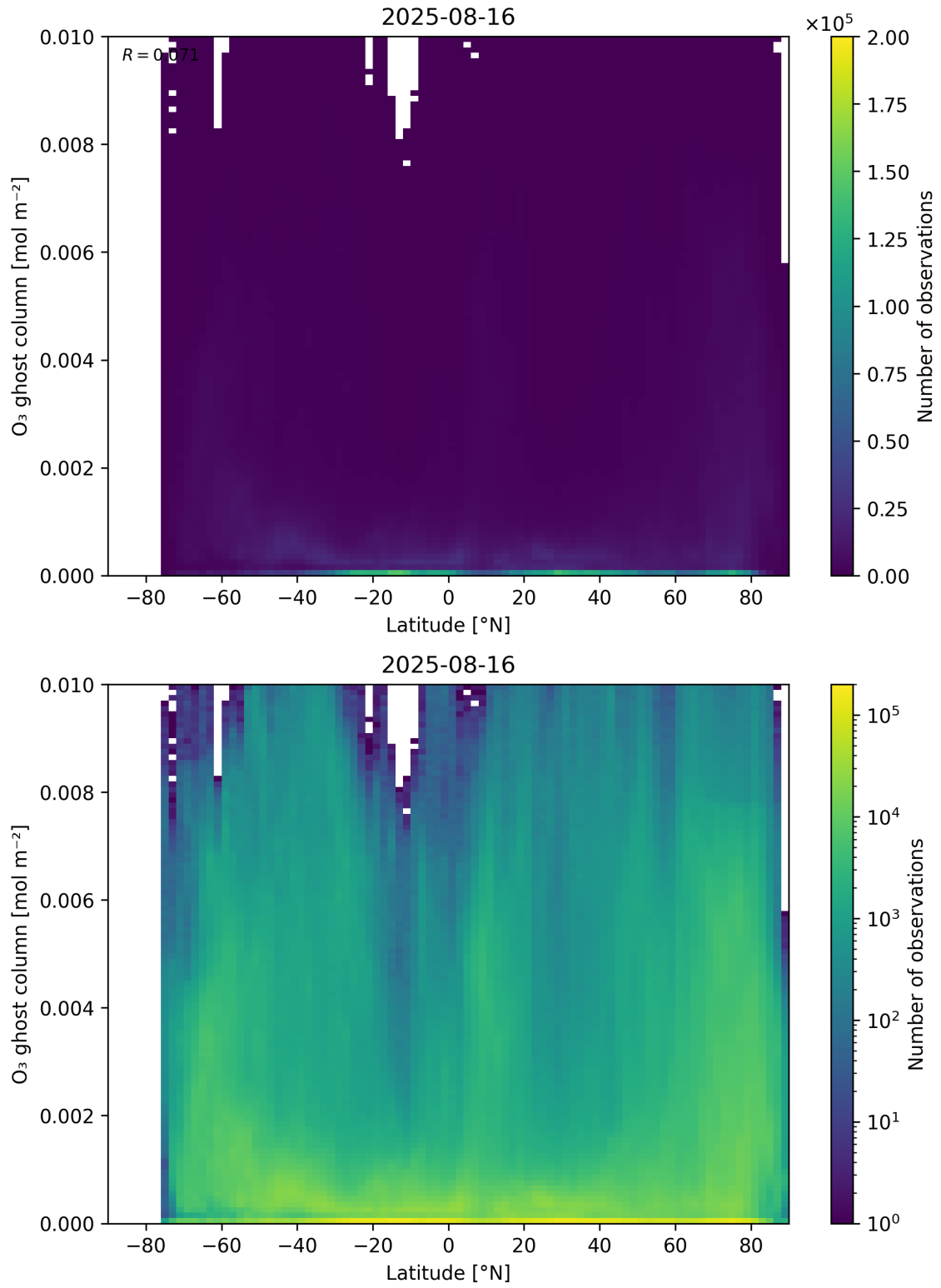
Figure 35: Scatter density plot of “Latitude” against “O 3 ghost column” for 2025-08-15 to 2025-08-17.
