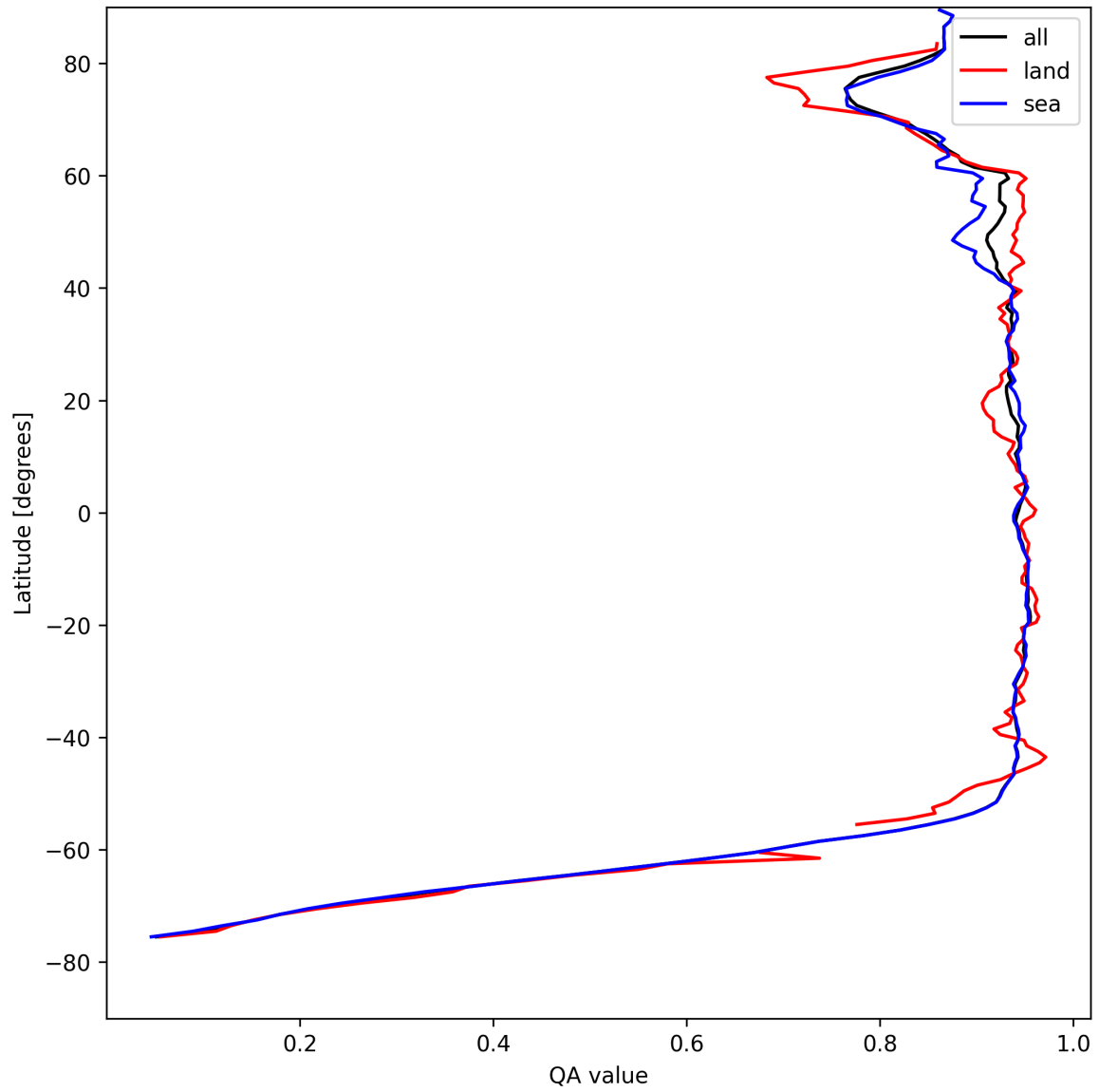
Figure 13: Zonal average of “QA value” for 2025-08-15 to 2025-08-17.
