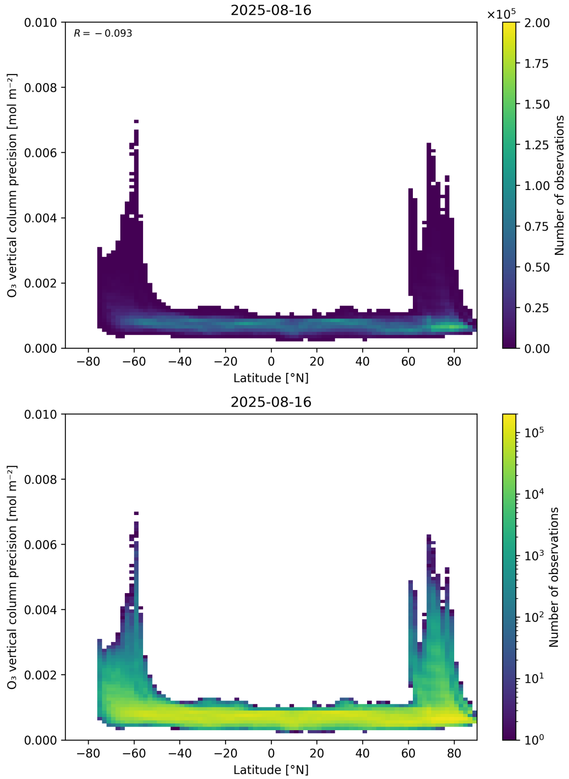
Figure 37: Scatter density plot of “Latitude” against “O 3 vertical column precision” for 2025-08-15 to 2025-08-17.
