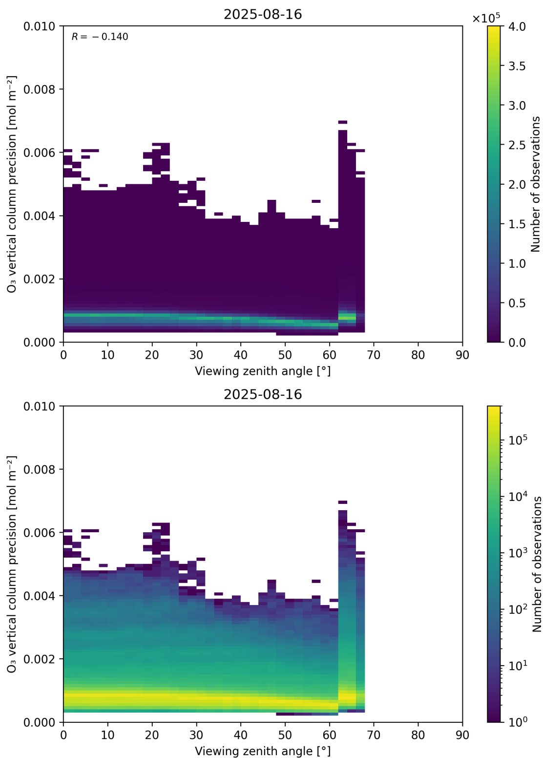
Figure 53: Scatter density plot of “Viewing zenith angle” against “O 3 vertical column precision” for 2025-08-15 to 2025-08-17.
