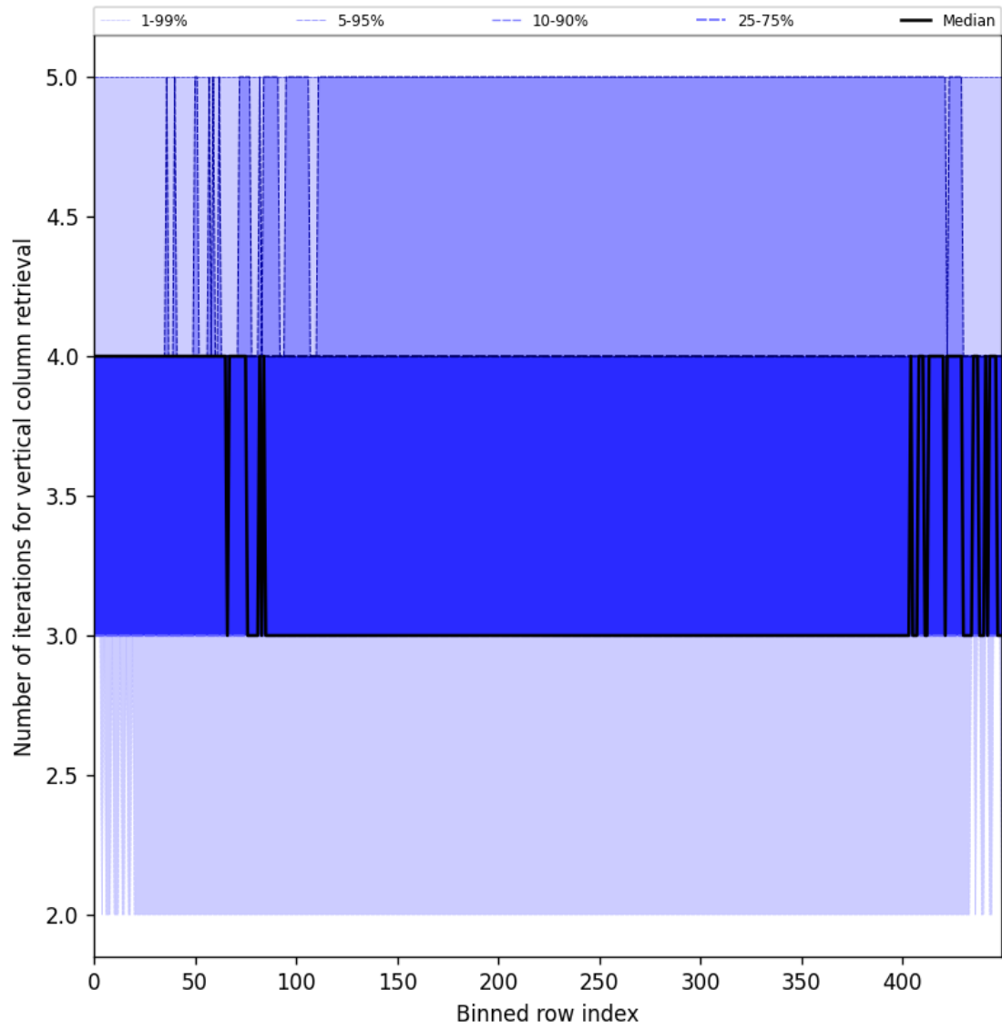
Figure 33: Along track statistics of “Number of iterations for vertical column retrieval” for 2025-08-15 to 2025-08-17
