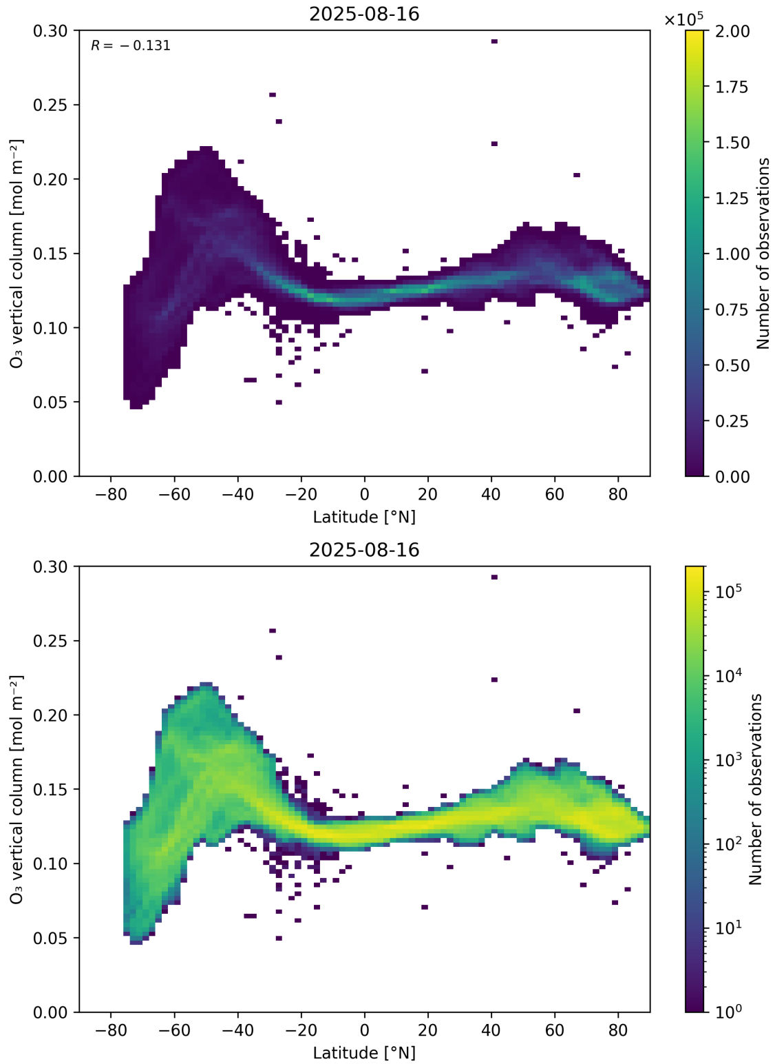
Figure 36: Scatter density plot of “Latitude” against “O 3 vertical column” for 2025-08-15 to 2025-08-17.
