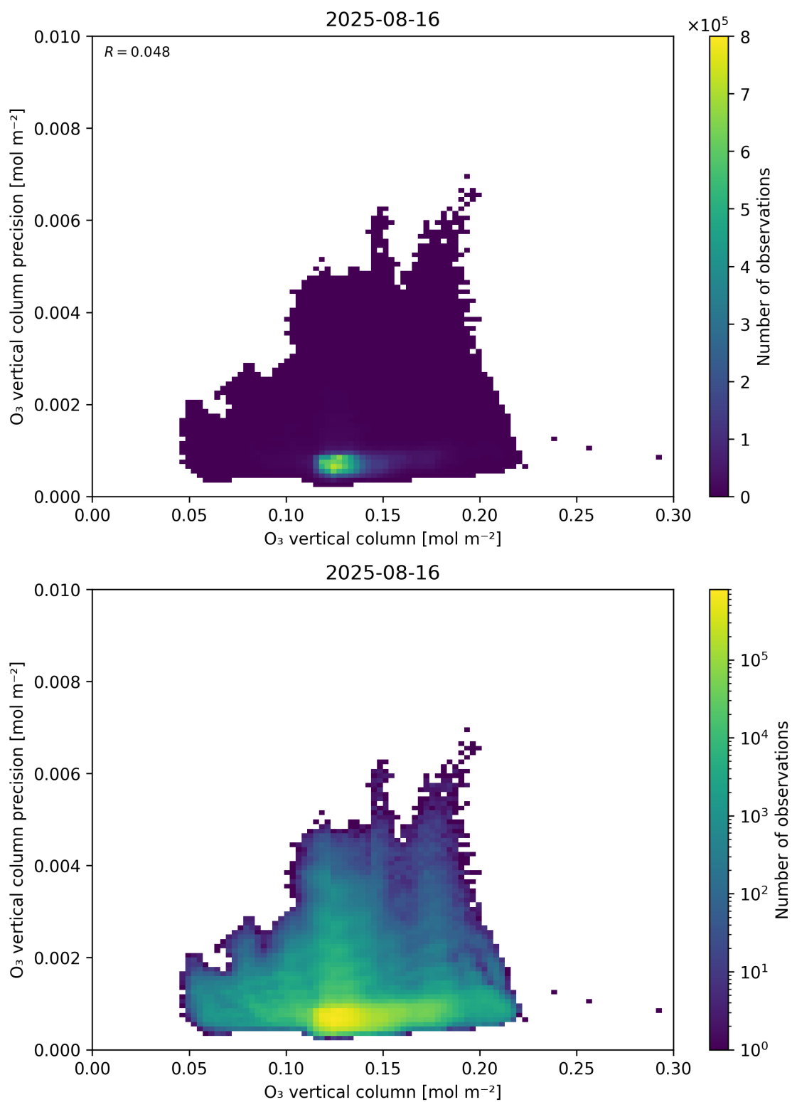
Figure 41: Scatter density plot of “O 3 vertical column” against “O 3 vertical column precision” for 2025-08-15 to 2025-08-17.
