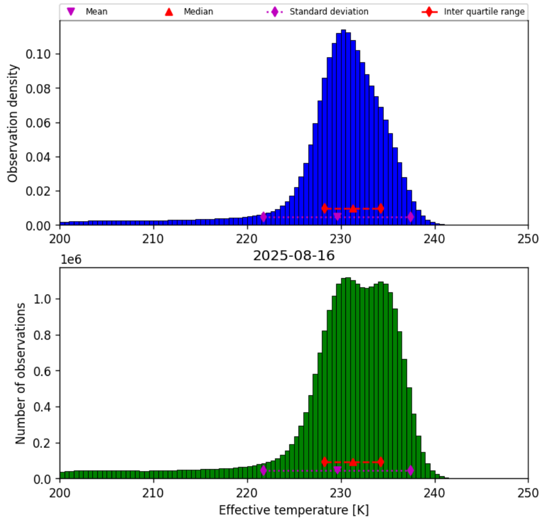
Figure 24: Histogram of “Effective temperature” for 2025-08-15 to 2025-08-17
