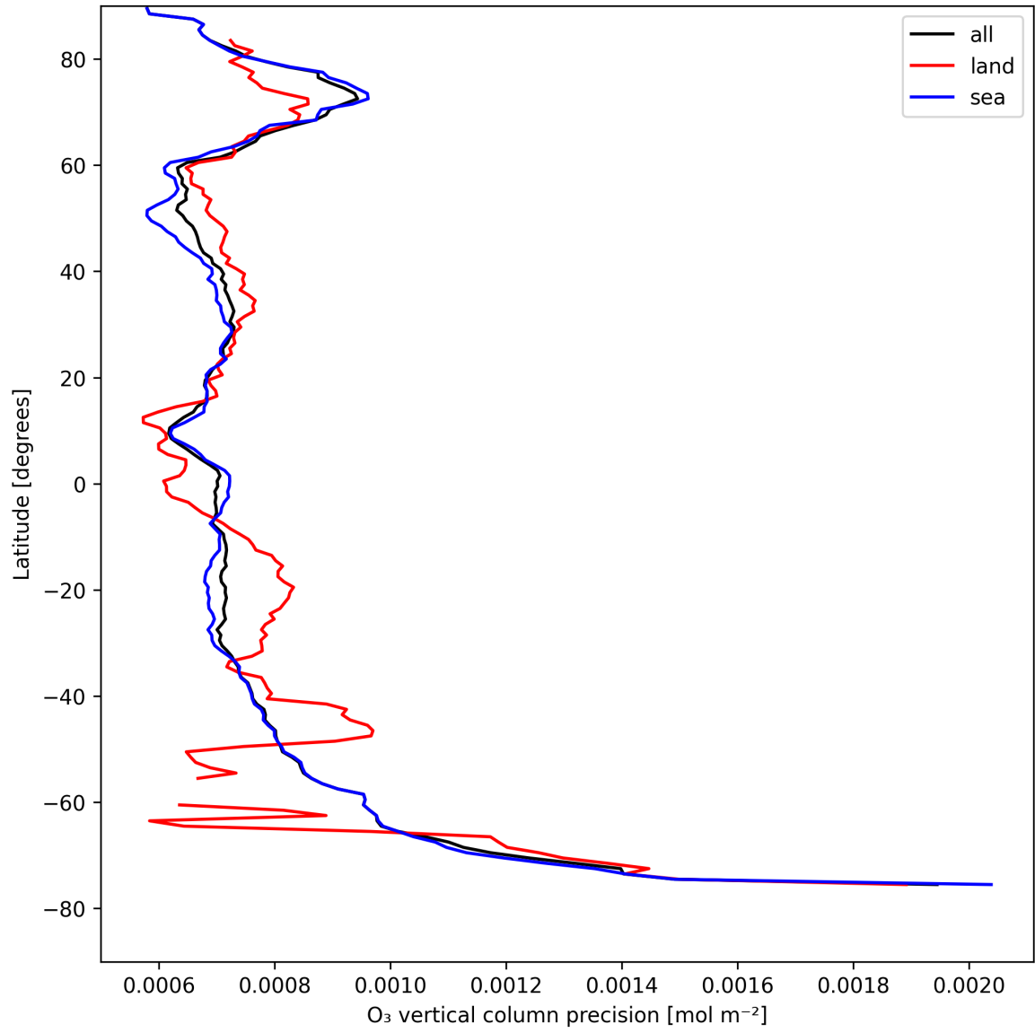
Figure 15: Zonal average of “O 3 vertical column precision” for 2025-08-15 to 2025-08-17.
