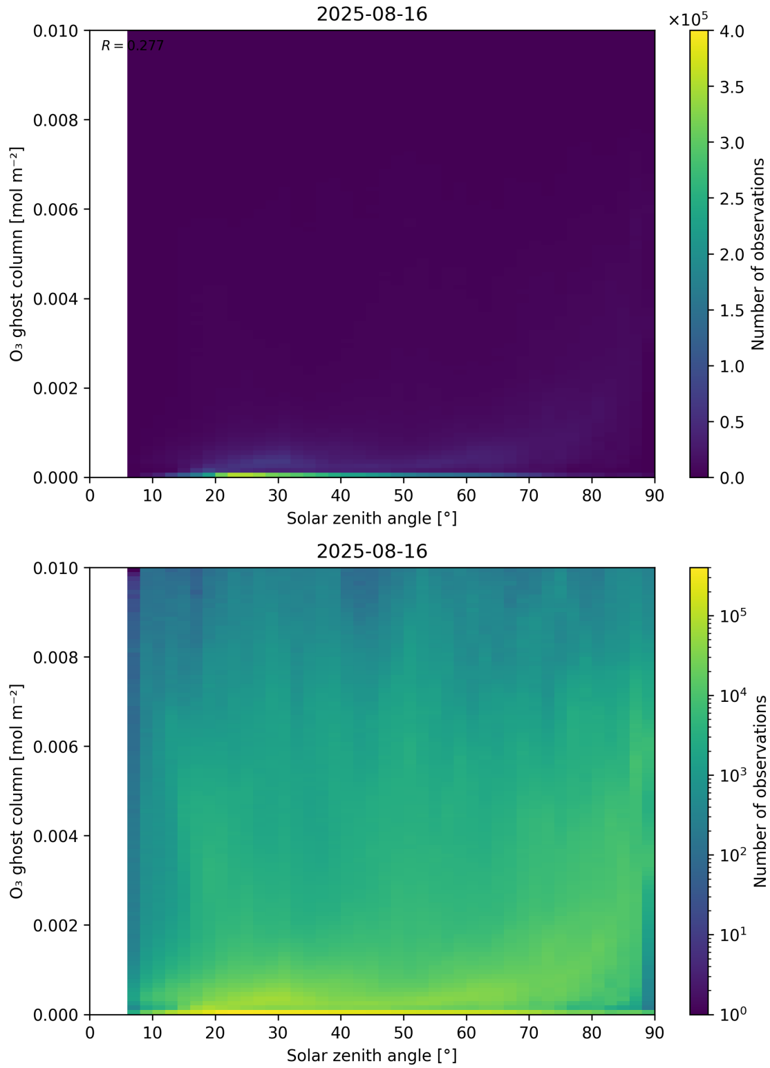
Figure 46: Scatter density plot of “Solar zenith angle” against “O 3 ghost column” for 2025-08-15 to 2025-08-17.
