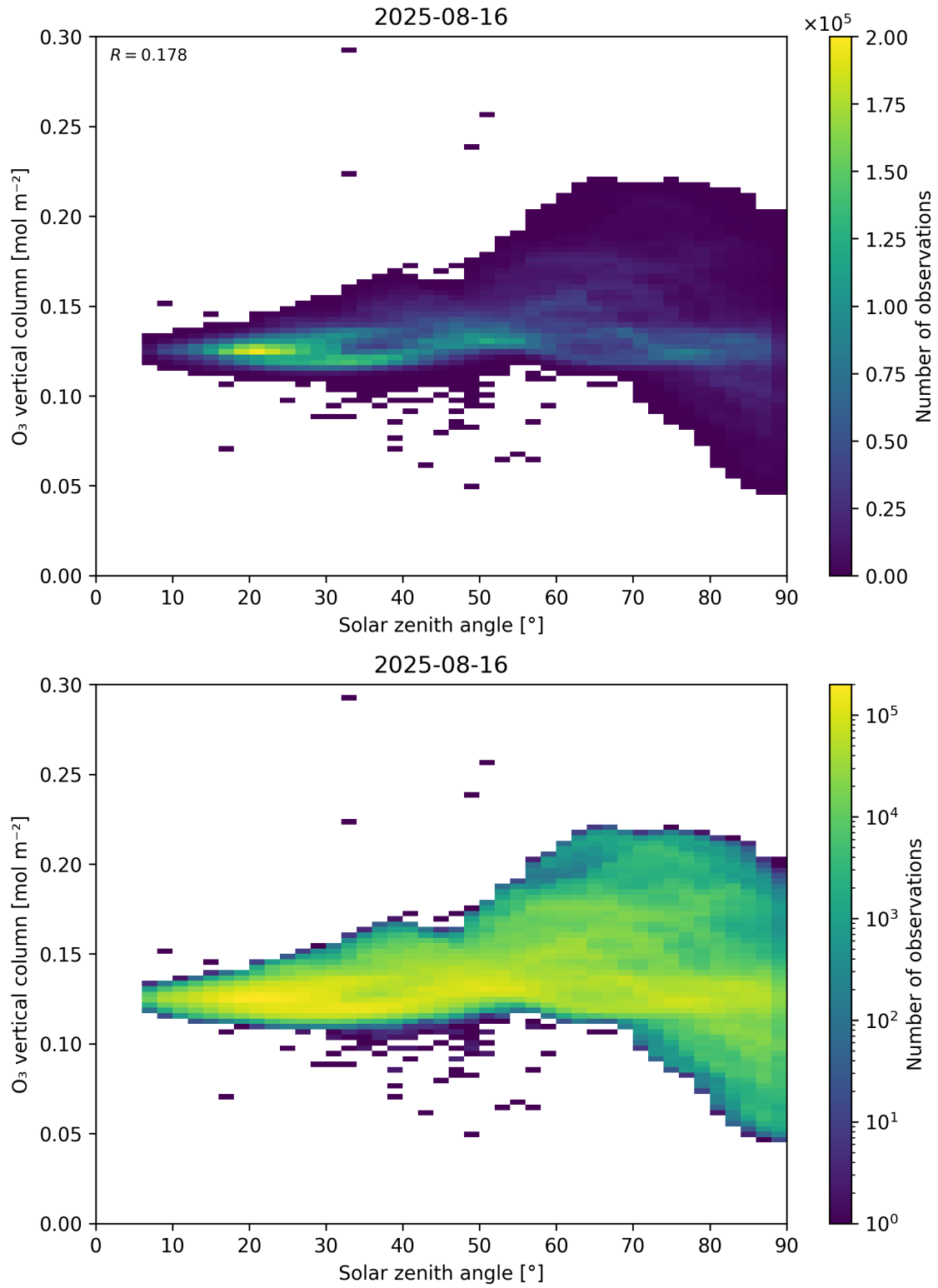
Figure 47: Scatter density plot of “Solar zenith angle” against “O 3 vertical column” for 2025-08-15 to 2025-08-17.
