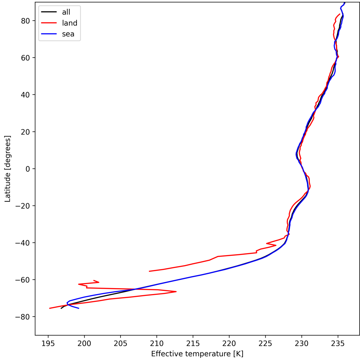
Figure 17: Zonal average of "Effective temperature" for 2025-08-15 to 2025-08-17.
