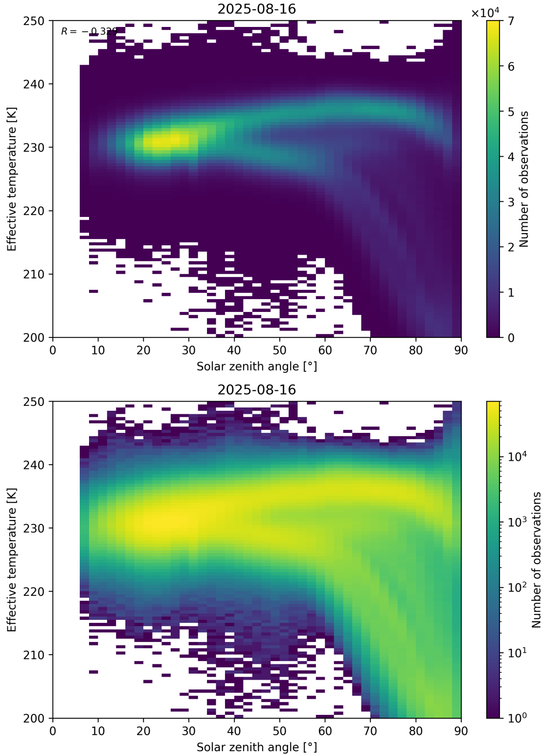
Figure 45: Scatter density plot of “Solar zenith angle” against “Effective temperature” for 2025-08-15 to 2025-08-17.
