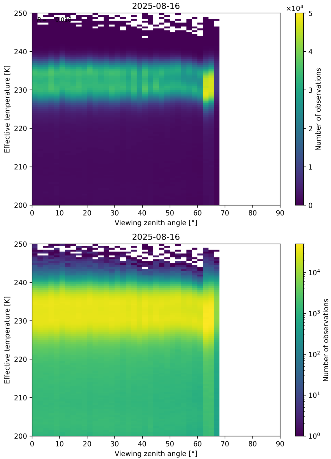
Figure 50: Scatter density plot of “Viewing zenith angle” against “Effective temperature” for 2025-08-15 to 2025-08-17.
