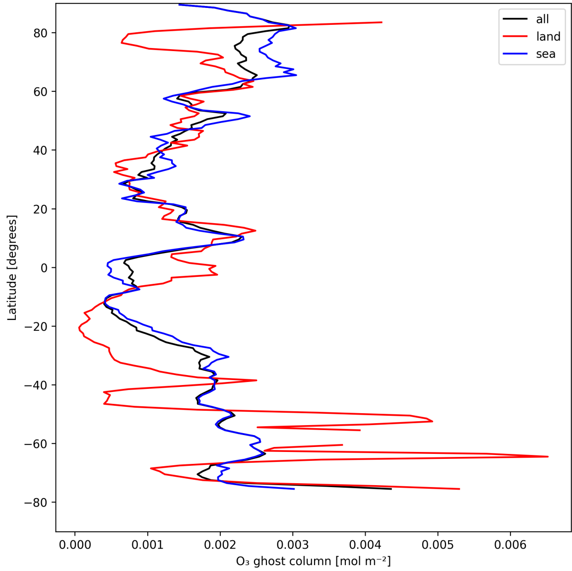
Figure 18: Zonal average of "O 3 ghost column" for 2025-08-15 to 2025-08-17.
