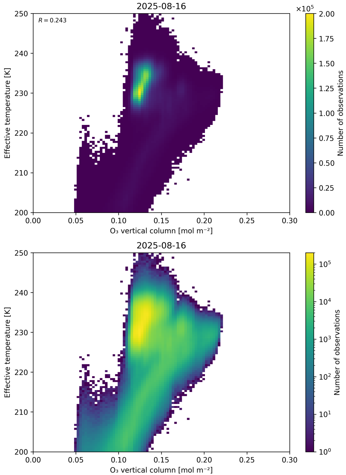
Figure 39: Scatter density plot of “O 3 vertical column” against “Effective temperature” for 2025-08-15 to 2025-08-17.
