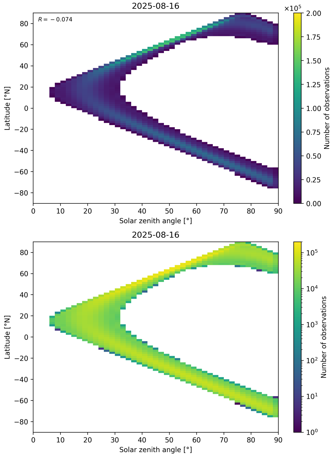
Figure 44: Scatter density plot of “Solar zenith angle” against “Latitude” for 2025-08-15 to 2025-08-17.
