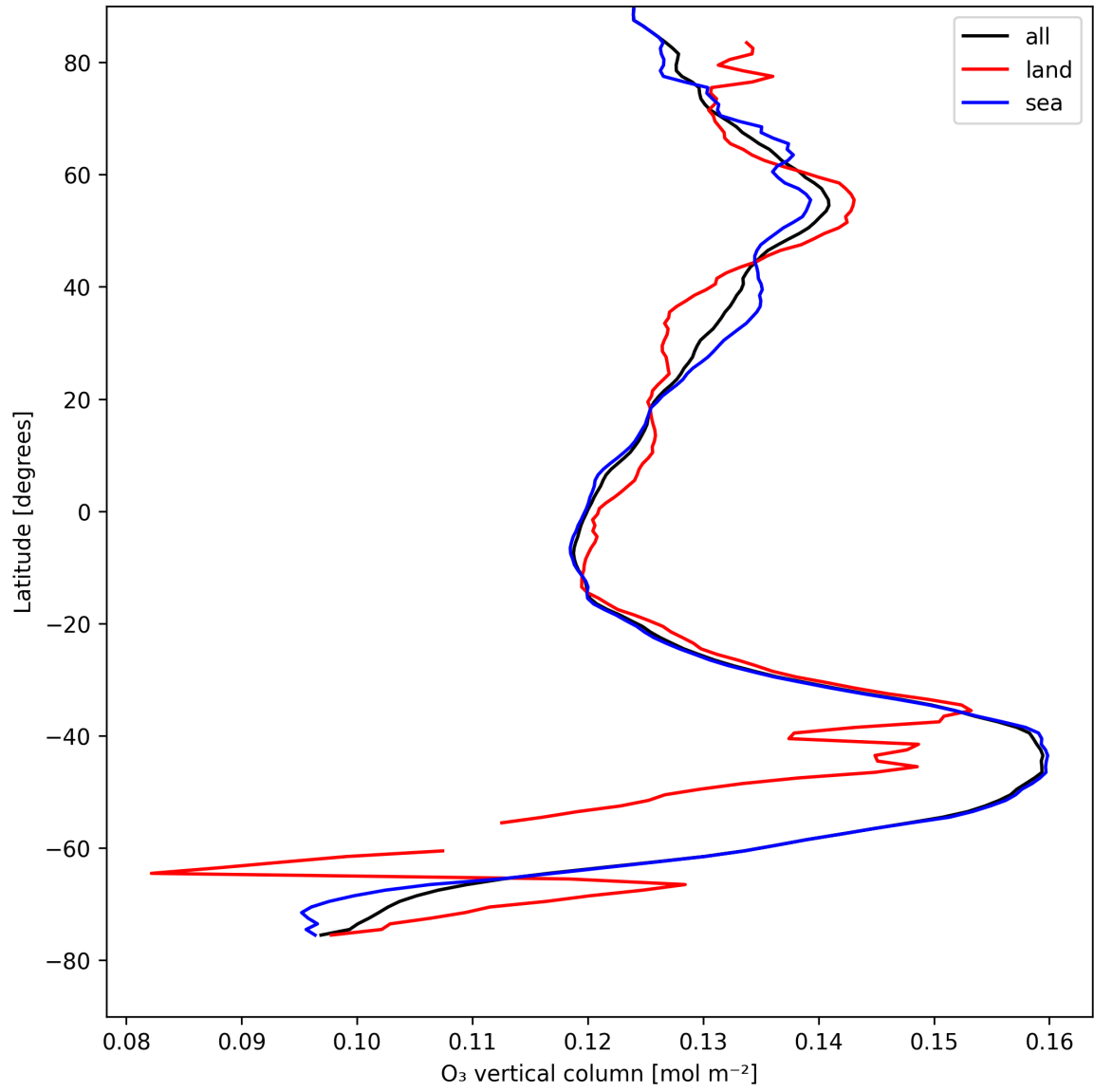
Figure 14: Zonal average of “O 3 vertical column” for 2025-08-15 to 2025-08-17.
