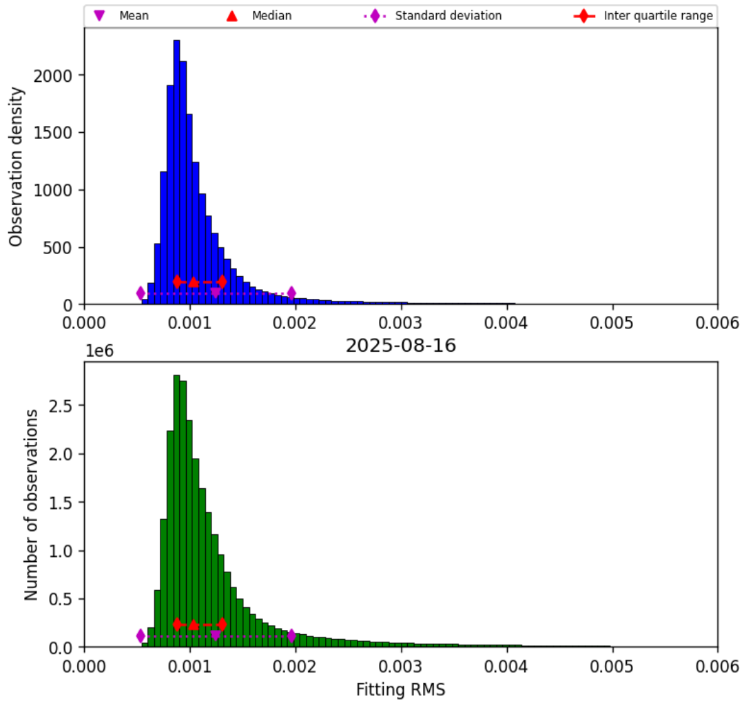
Figure 23: Histogram of “Fitting RMS” for 2025-08-15 to 2025-08-17
