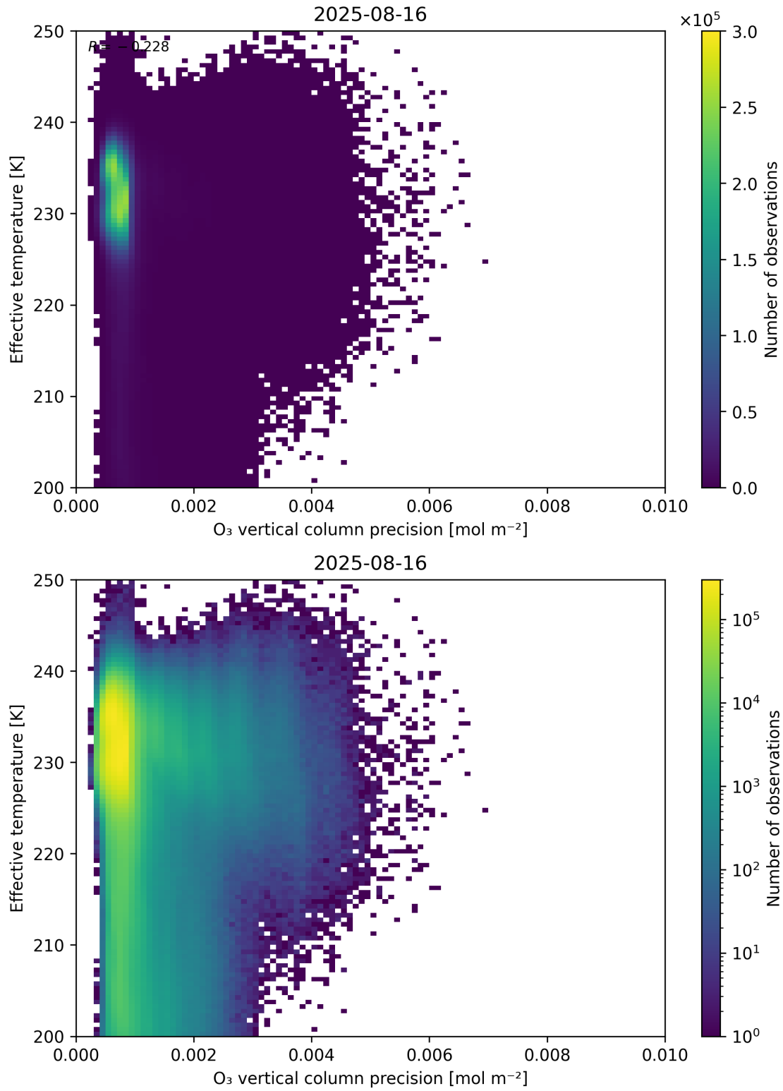
Figure 42: Scatter density plot of “O 3 vertical column precision” against “Effective temperature” for 2025-08-15 to 2025-08-17.
