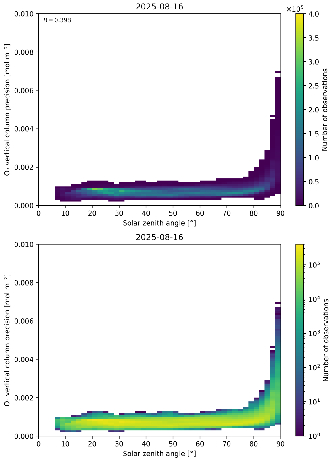
Figure 48: Scatter density plot of “Solar zenith angle” against “O 3 vertical column precision” for 2025-08-15 to 2025-08-17.
