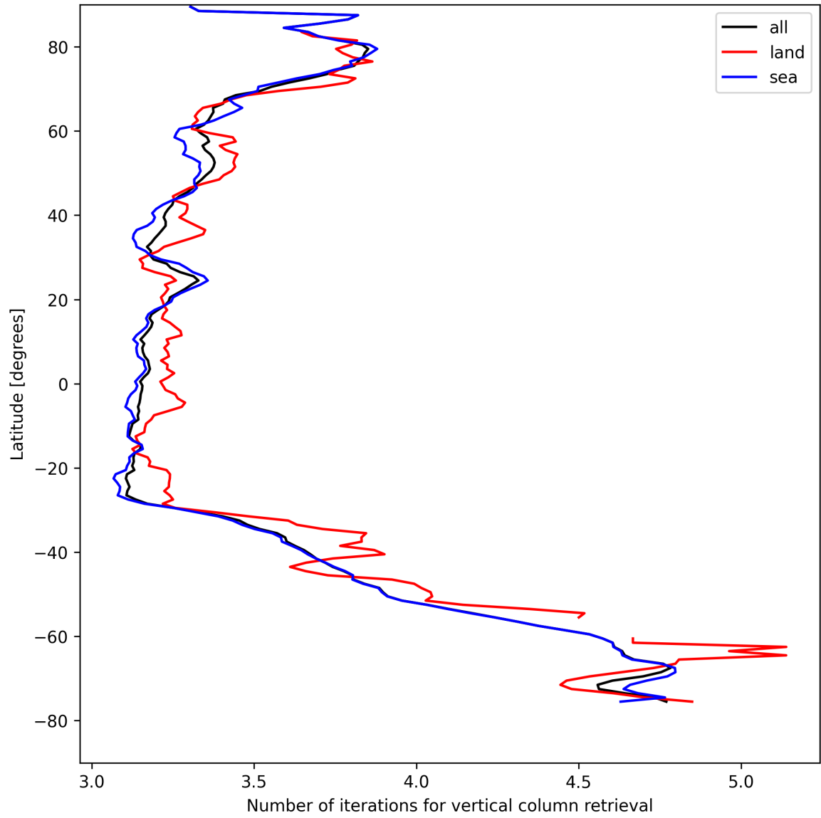
Figure 19: Zonal average of “Number of iterations for vertical column retrieval” for 2025-08-15 to 2025-08-17.
