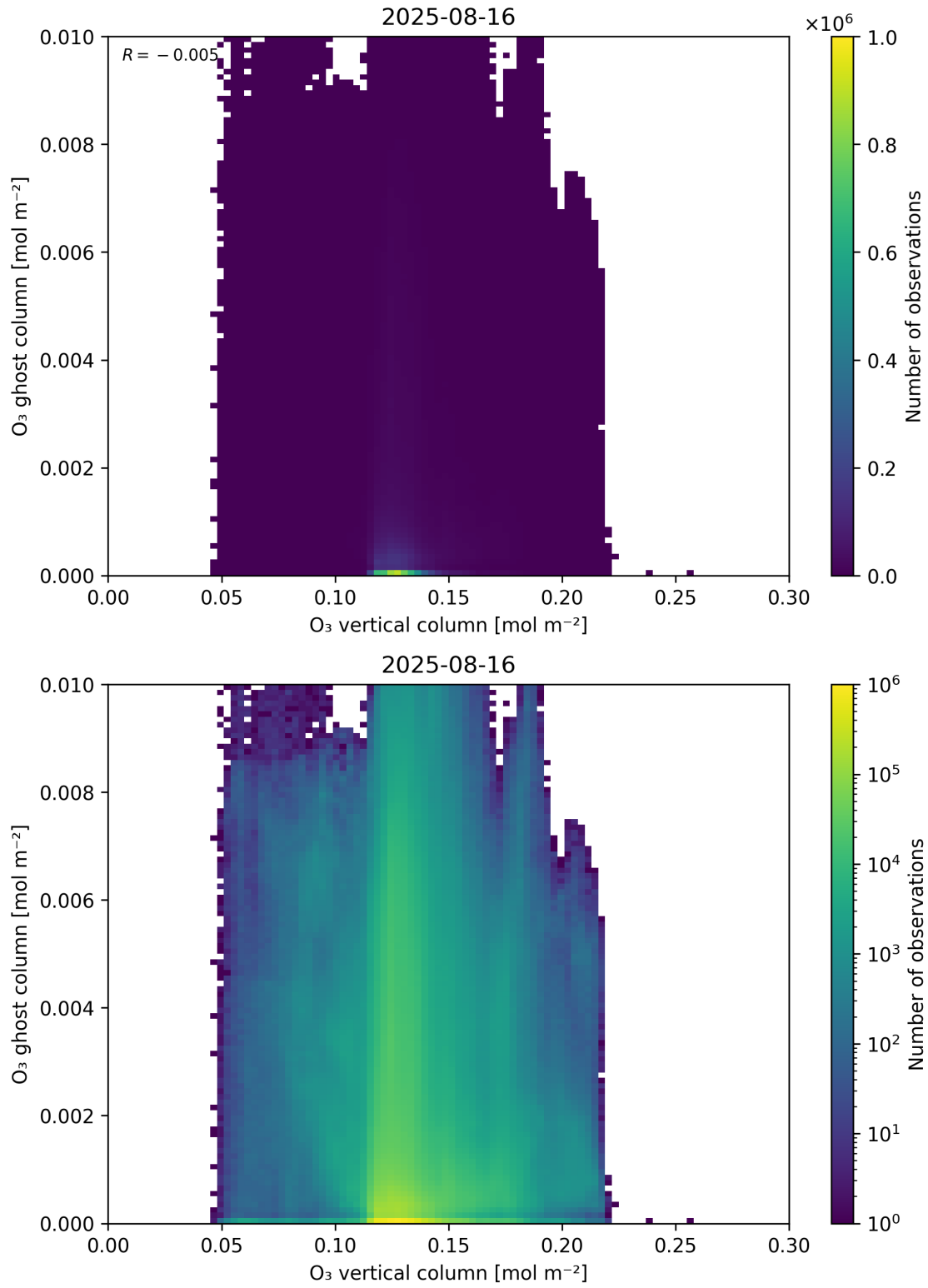
Figure 40: Scatter density plot of “O 3 vertical column” against “O 3 ghost column” for 2025-08-15 to 2025-08-17.
