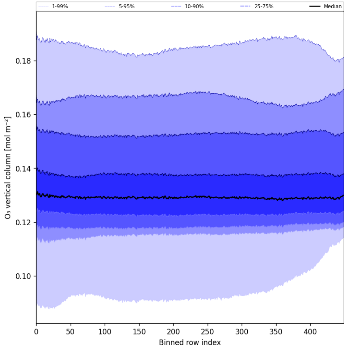
Figure 28: Along track statistics of “O 3 vertical column” for 2025-08-15 to 2025-08-17
