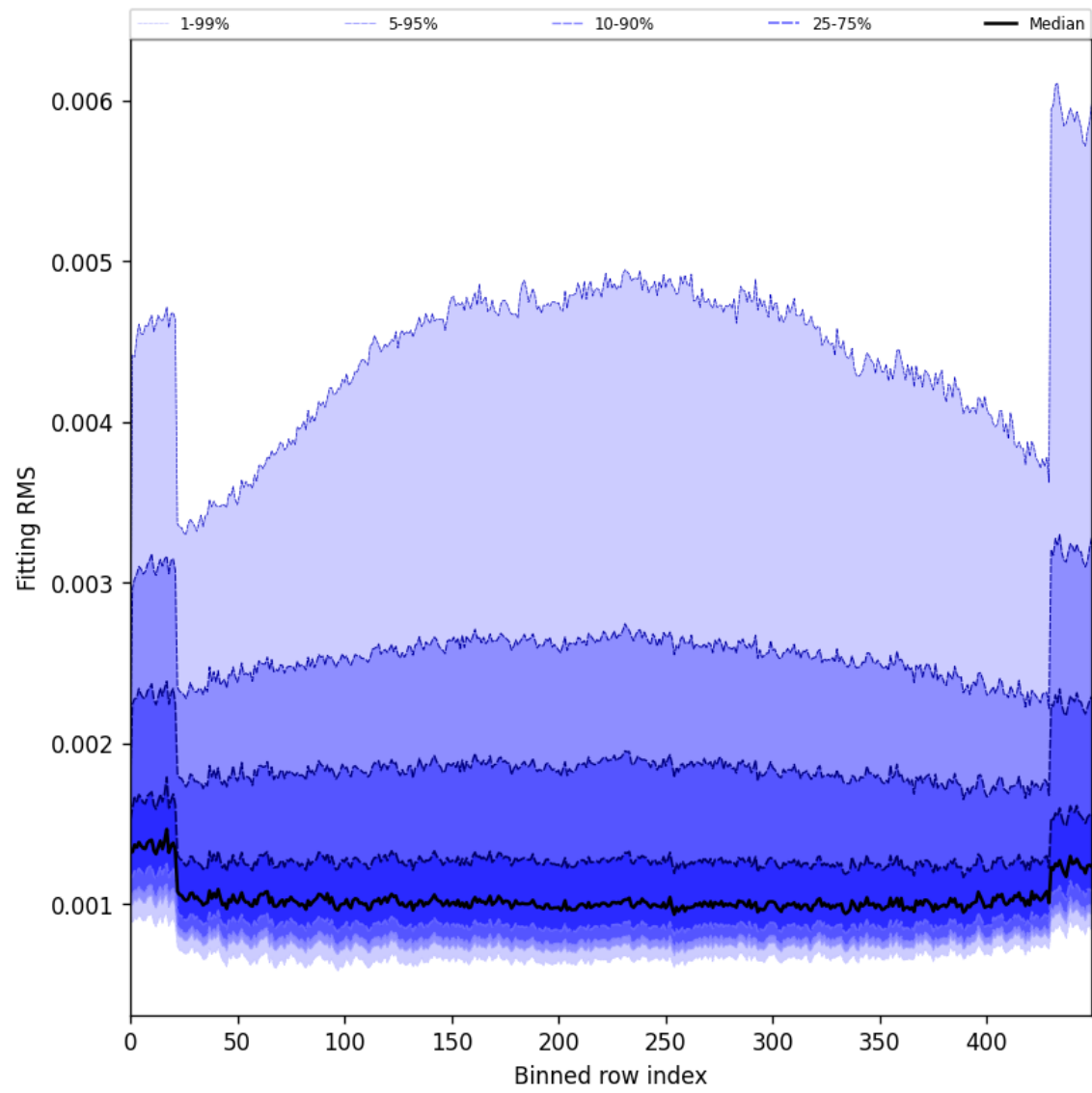
Figure 30: Along track statistics of “Fitting RMS” for 2025-08-15 to 2025-08-17
