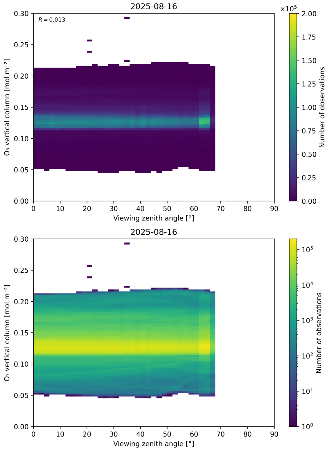
Figure 52: Scatter density plot of “Viewing zenith angle” against “O 3 vertical column” for 2025-08-15 to 2025-08-17.
