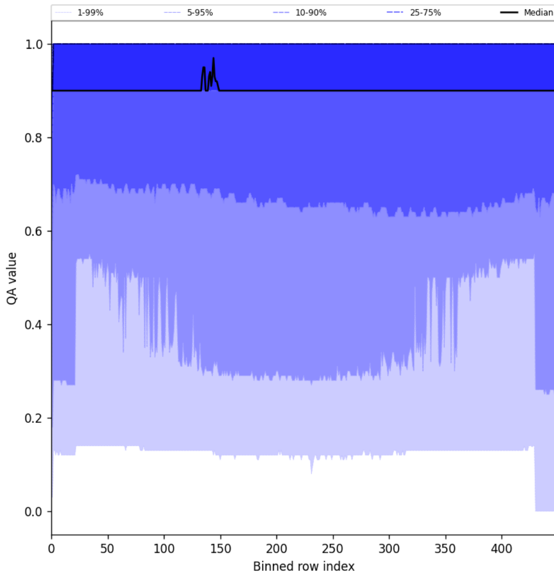
Figure 27: Along track statistics of “QA value” for 2025-08-15 to 2025-08-17
