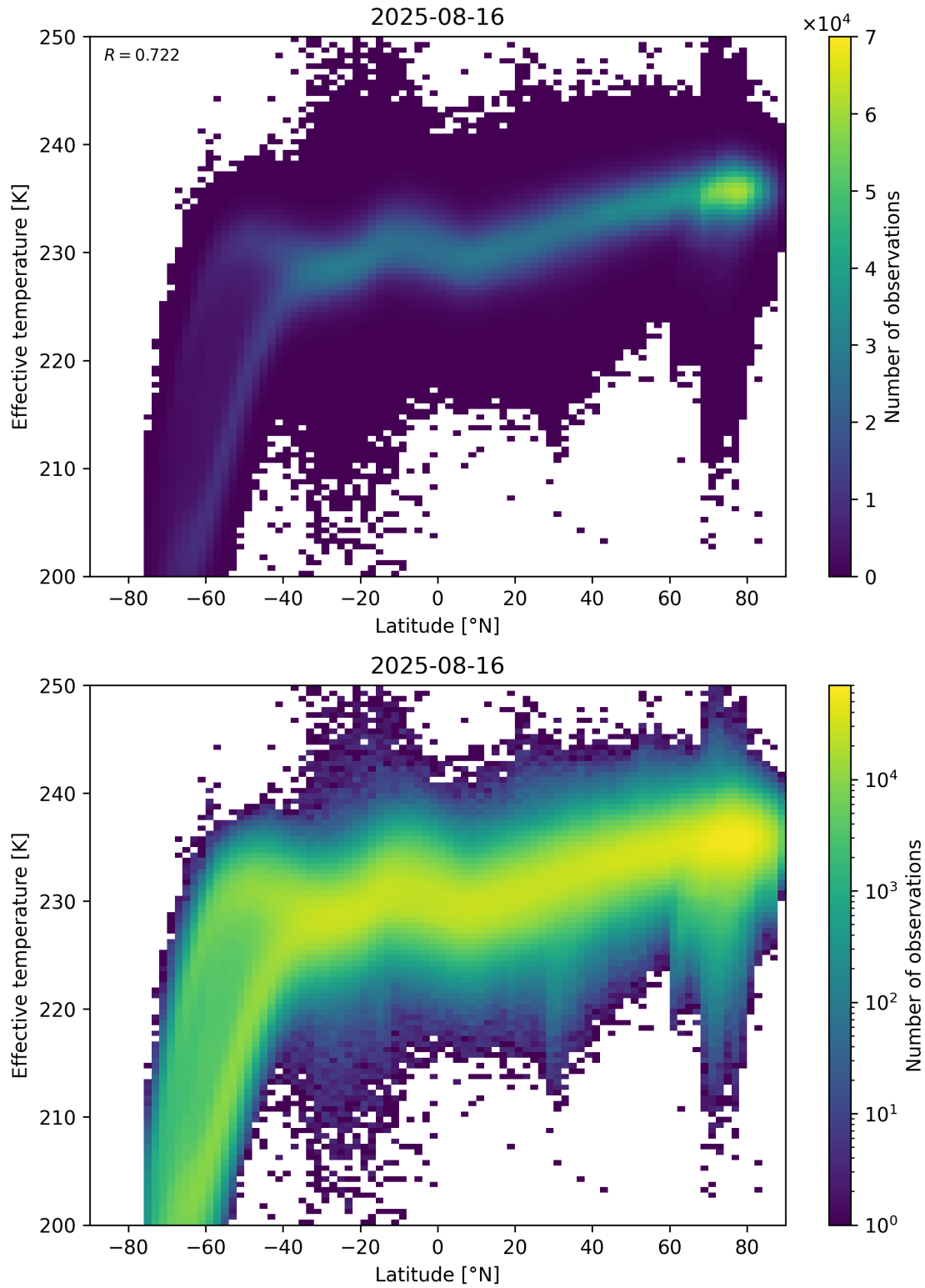
Figure 34: Scatter density plot of “Latitude” against “Effective temperature” for 2025-08-15 to 2025-08-17.
