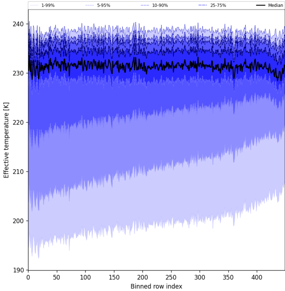
Figure 31: Along track statistics of “Effective temperature” for 2025-08-15 to 2025-08-17
