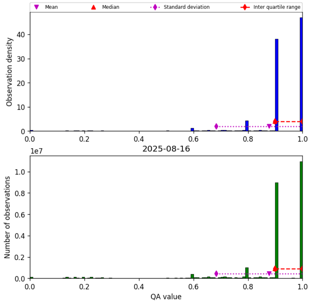
Figure 20: Histogram of “QA value” for 2025-08-15 to 2025-08-17
