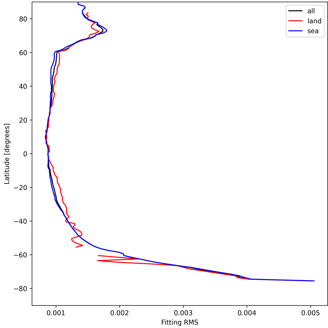
Figure 16: Zonal average of “Fitting RMS” for 2025-08-15 to 2025-08-17.
