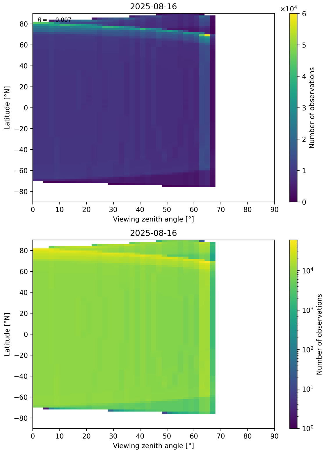
Figure 49: Scatter density plot of “Viewing zenith angle” against “Latitude” for 2025-08-15 to 2025-08-17.
