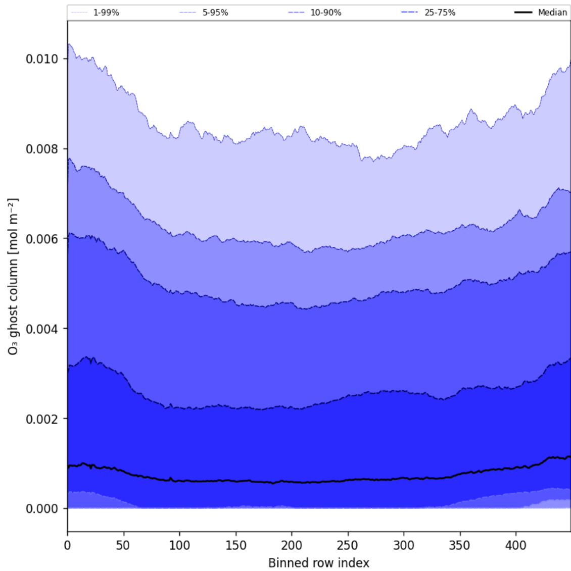
Figure 32: Along track statistics of “O 3 ghost column” for 2025-08-15 to 2025-08-17
