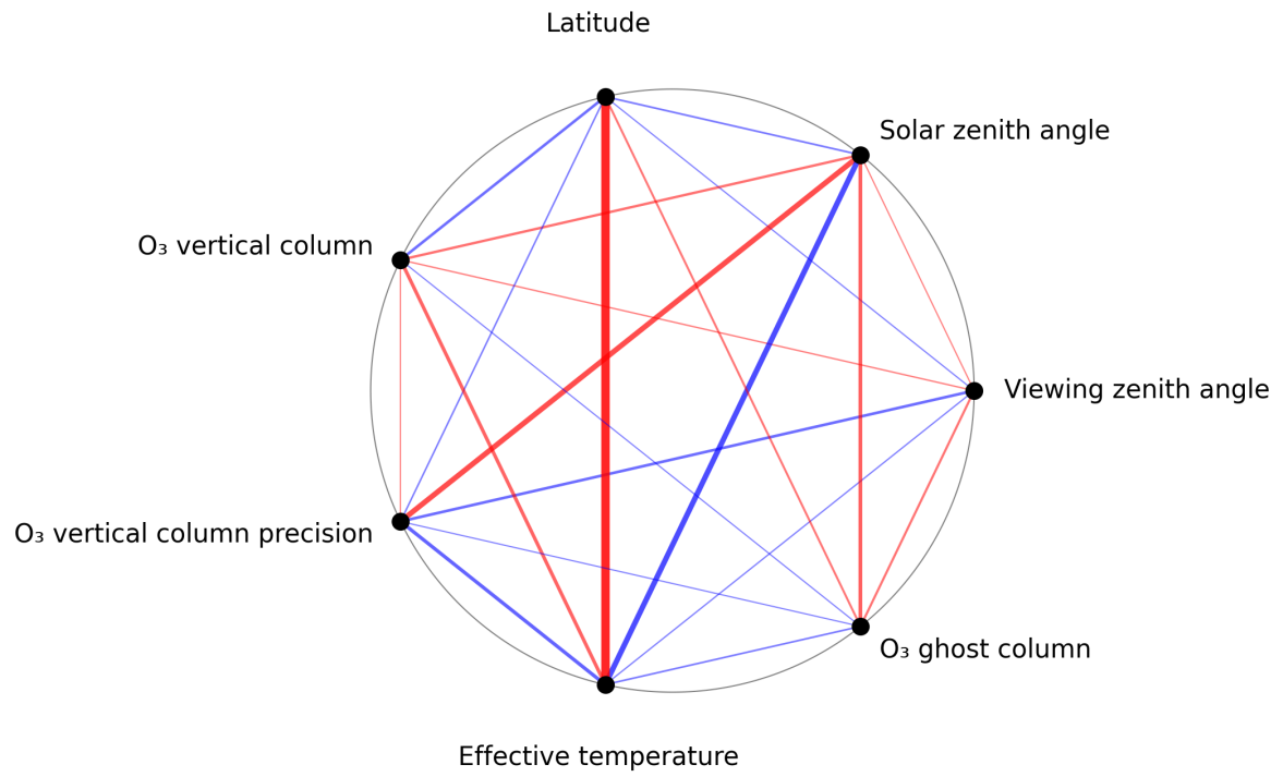
Figure 1: Map of correlation graph for 2025-08-21 to 2025-08-23.
