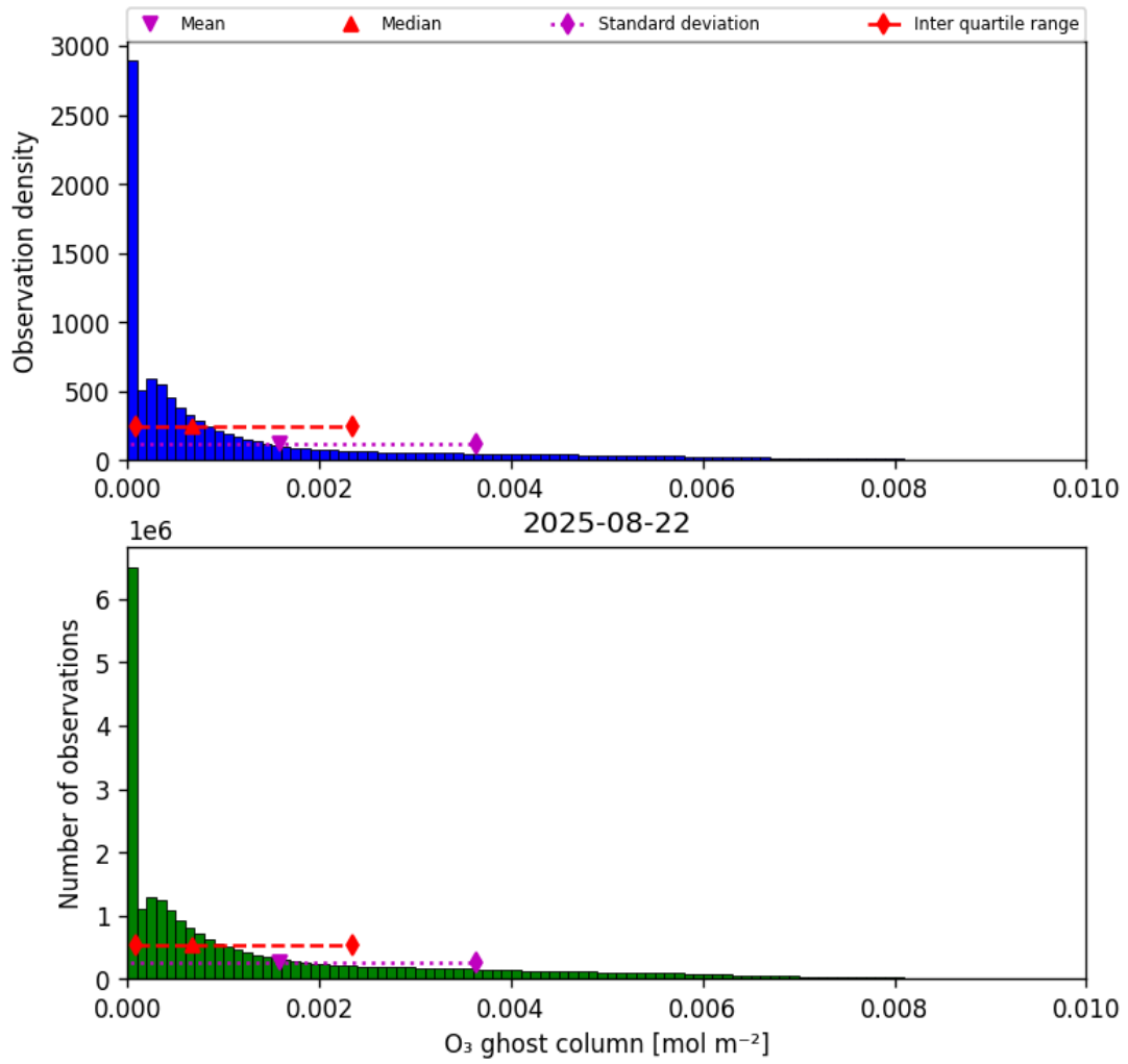
Figure 25: Histogram of “O 3 ghost column” for 2025-08-21 to 2025-08-23
