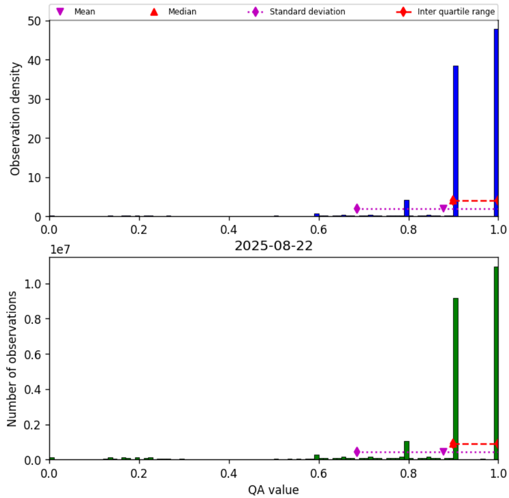
Figure 20: Histogram of “QA value” for 2025-08-21 to 2025-08-23
