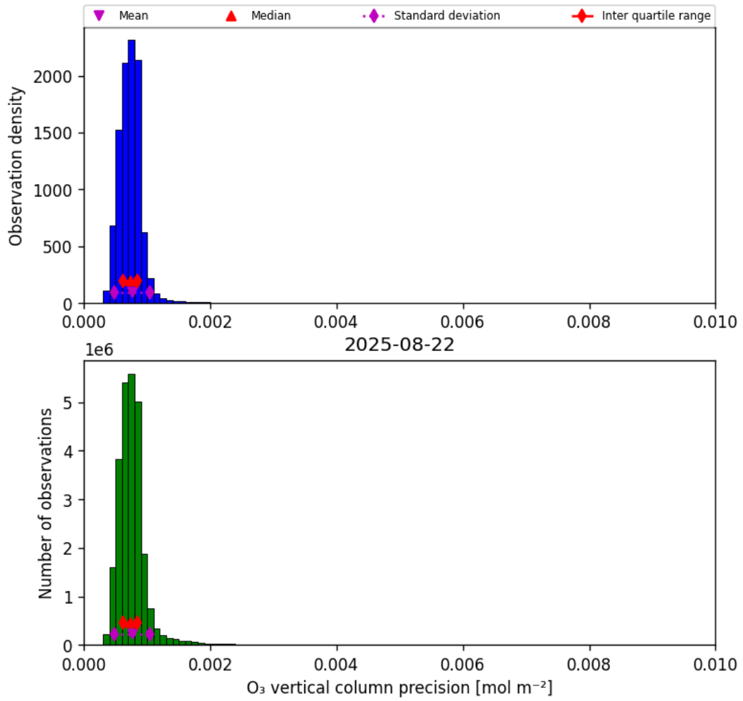
Figure 22: Histogram of “O 3 vertical column precision” for 2025-08-21 to 2025-08-23
