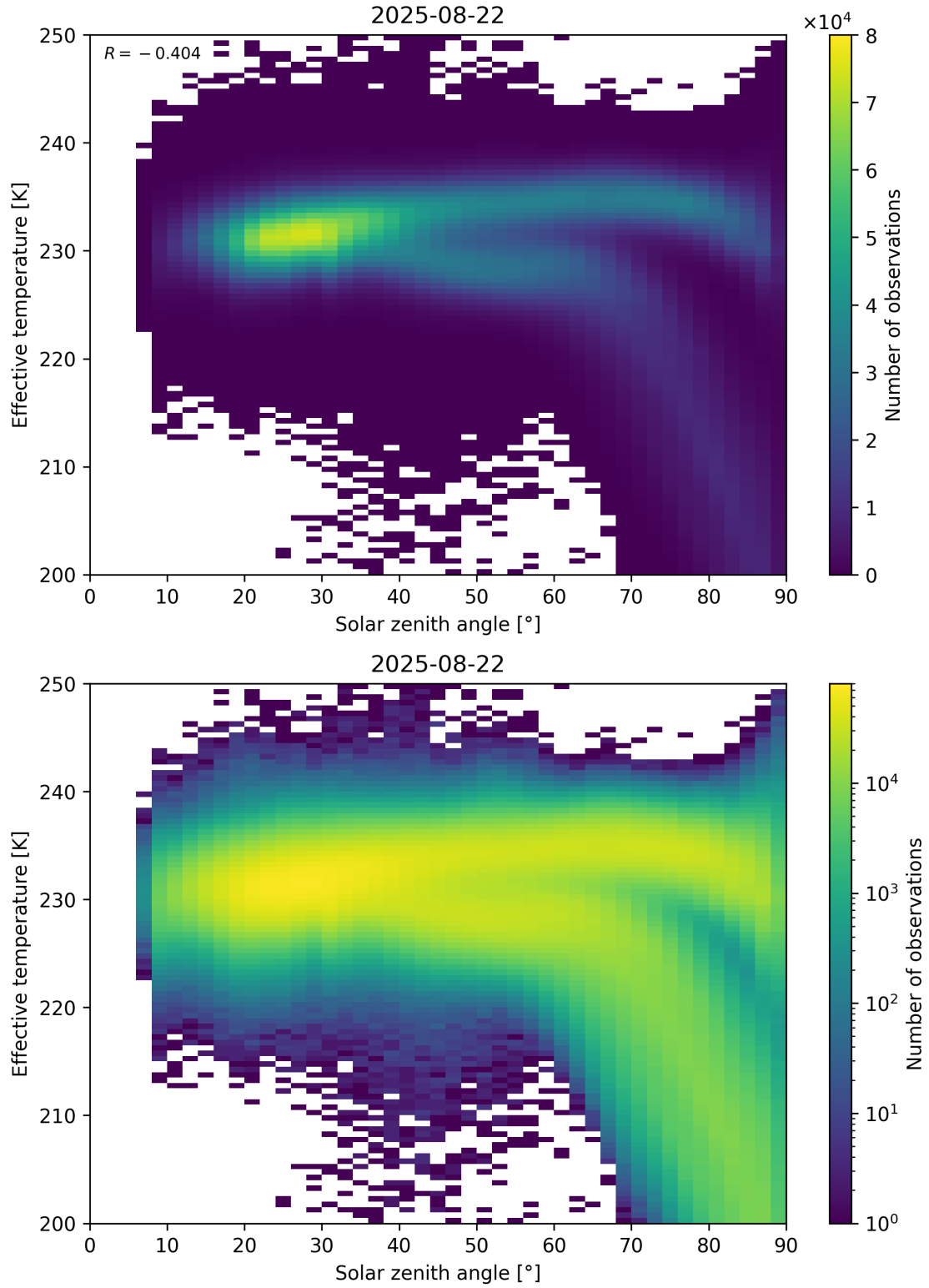
Figure 45: Scatter density plot of “Solar zenith angle” against “Effective temperature” for 2025-08-21 to 2025-08-23.
