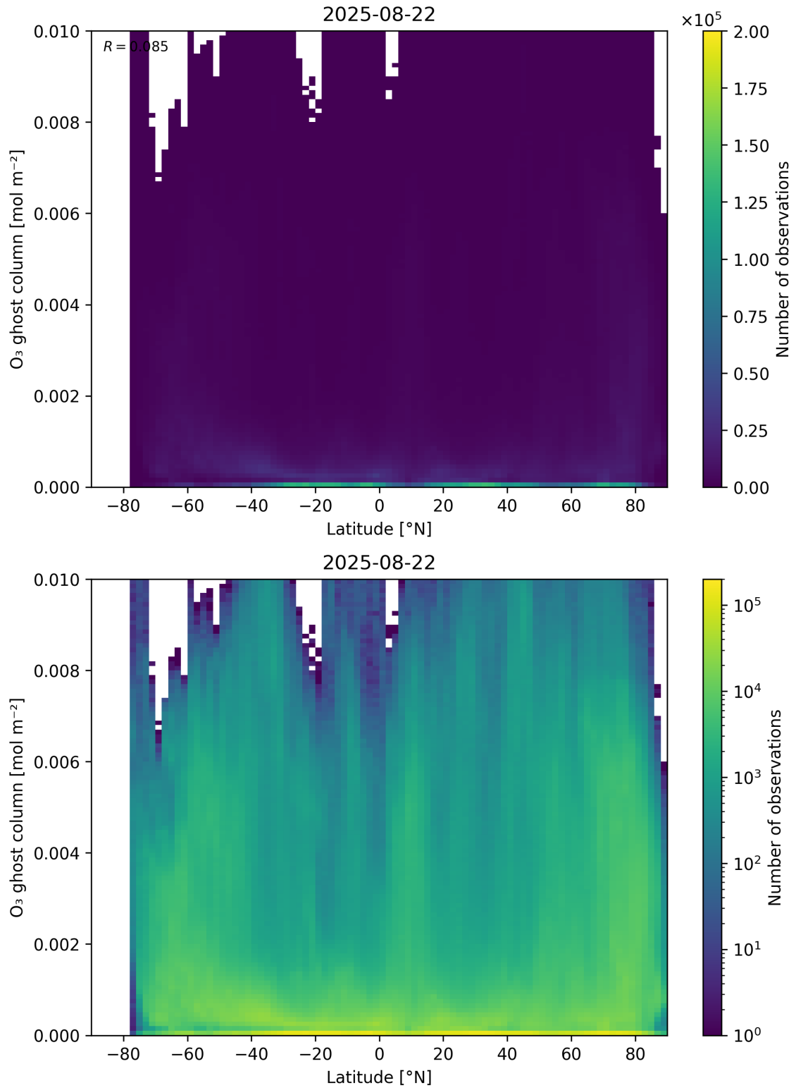
Figure 35: Scatter density plot of “Latitude” against “O 3 ghost column” for 2025-08-21 to 2025-08-23.
