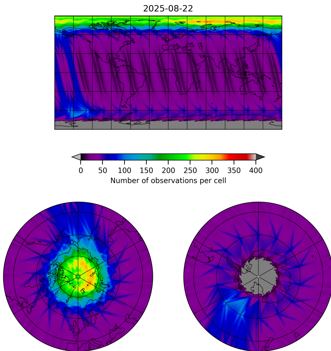
Figure 12: Map of the number of observations for 2025-08-21 to 2025-08-23
