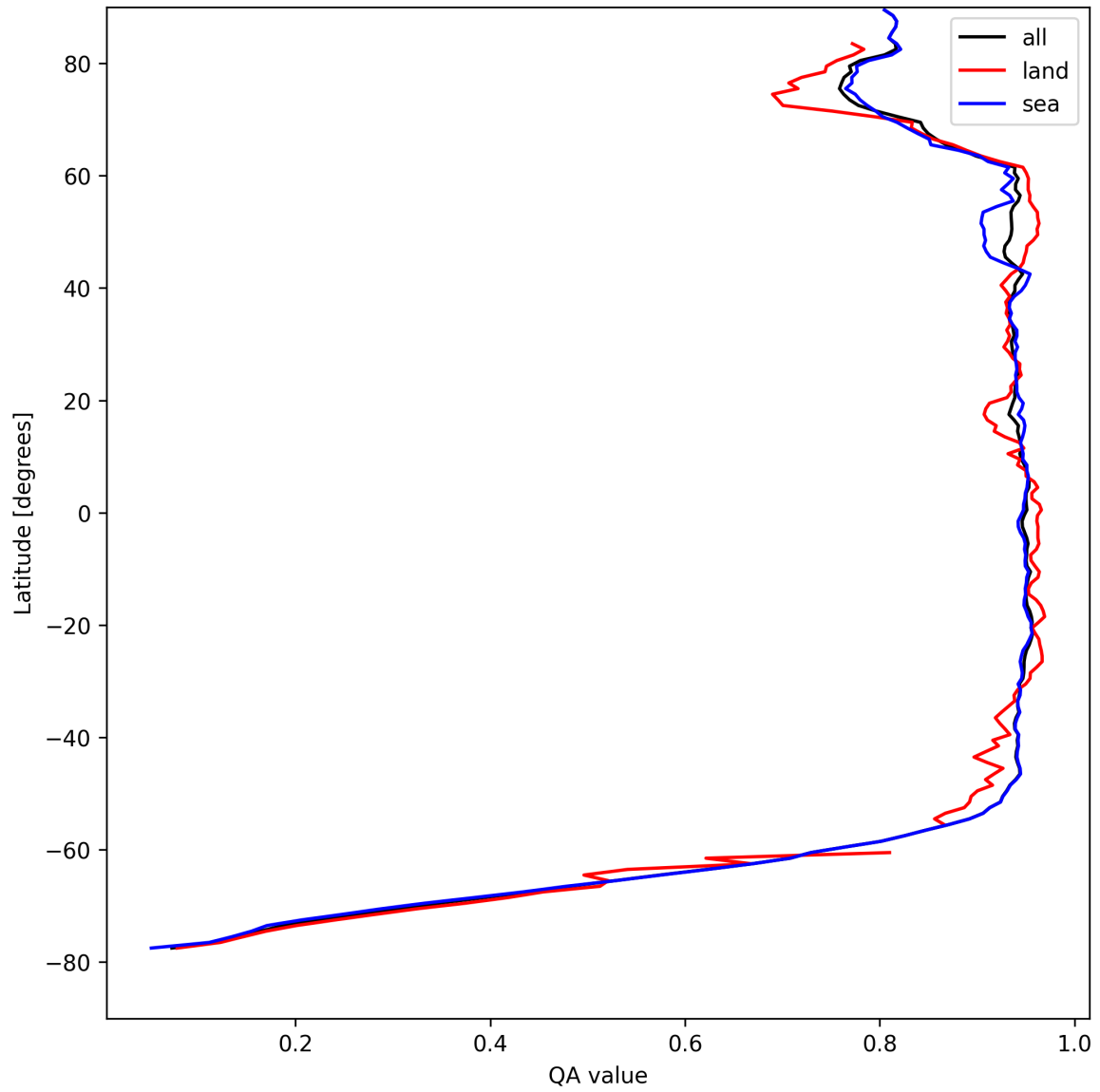
Figure 13: Zonal average of “QA value” for 2025-08-21 to 2025-08-23.
