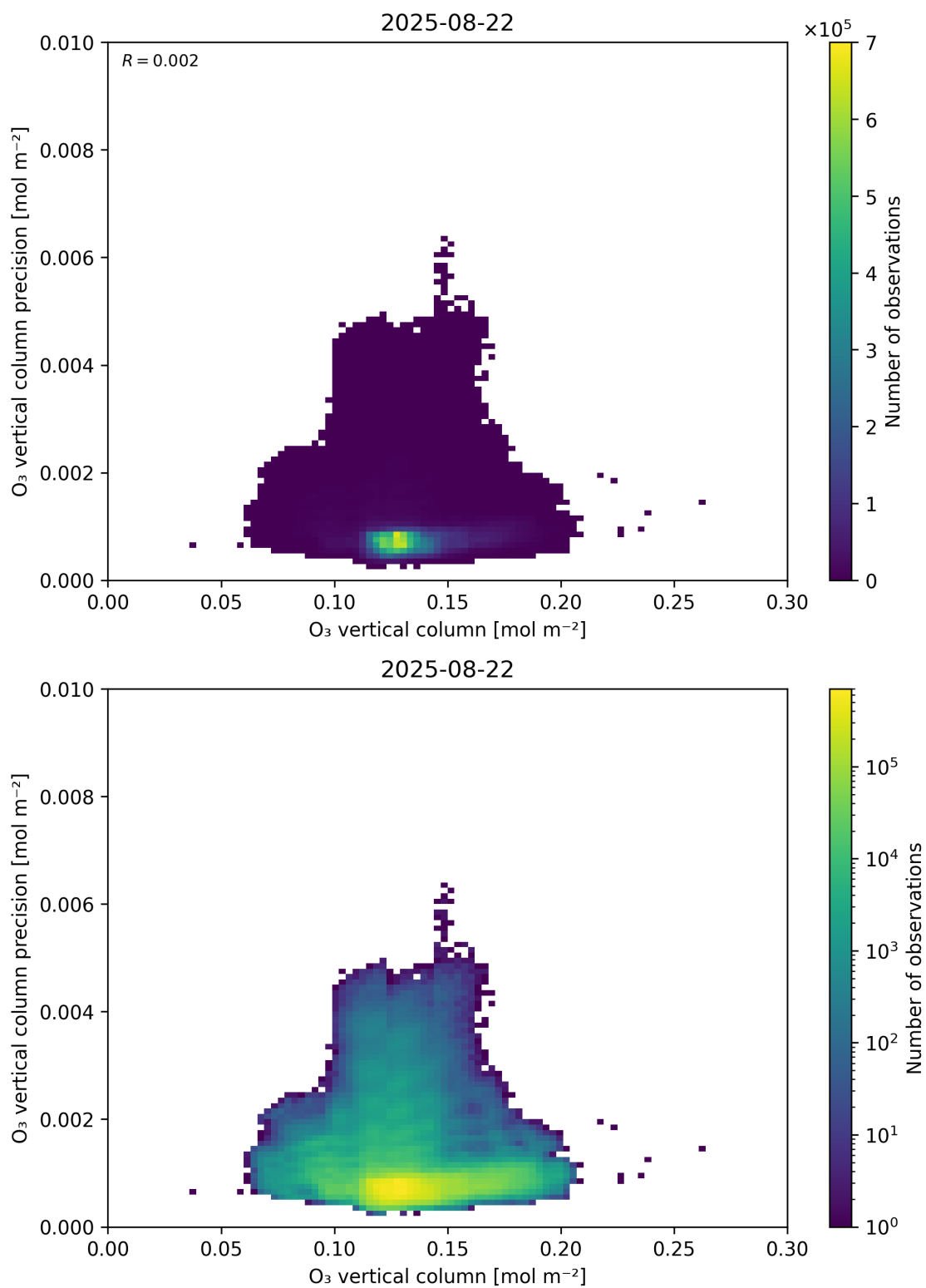
Figure 41: Scatter density plot of “O 3 vertical column” against “O 3 vertical column precision” for 2025-08-21 to 2025-08-23.
