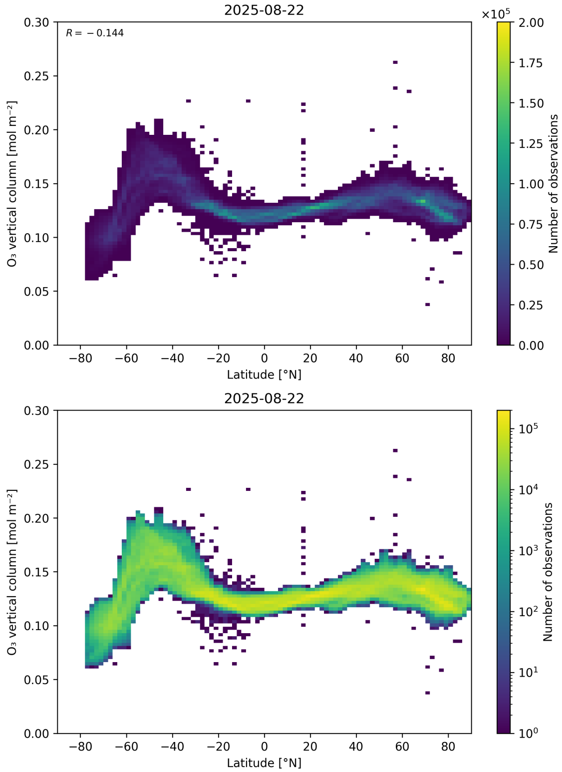
Figure 36: Scatter density plot of “Latitude” against “O 3 vertical column” for 2025-08-21 to 2025-08-23.
