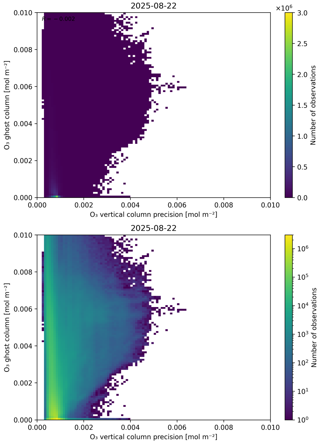
Figure 43: Scatter density plot of “ \text{O}_3 vertical column precision” against “ \text{O}_3 ghost column” for 2025-08-21 to 2025-08-23.
