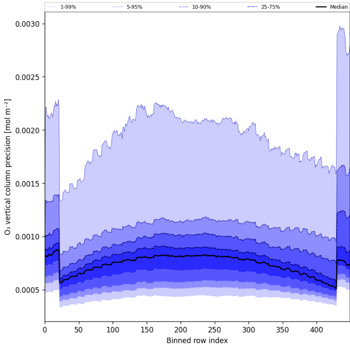
Figure 29: Along track statistics of “O 3 vertical column precision” for 2025-08-21 to 2025-08-23
