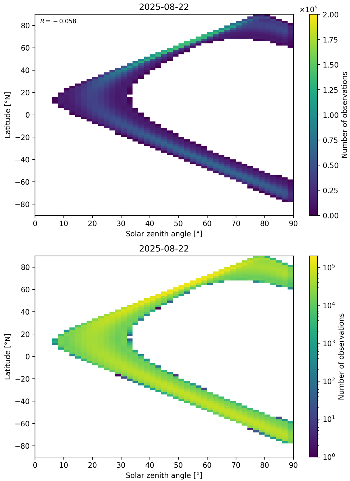
Figure 44: Scatter density plot of “Solar zenith angle” against “Latitude” for 2025-08-21 to 2025-08-23.
