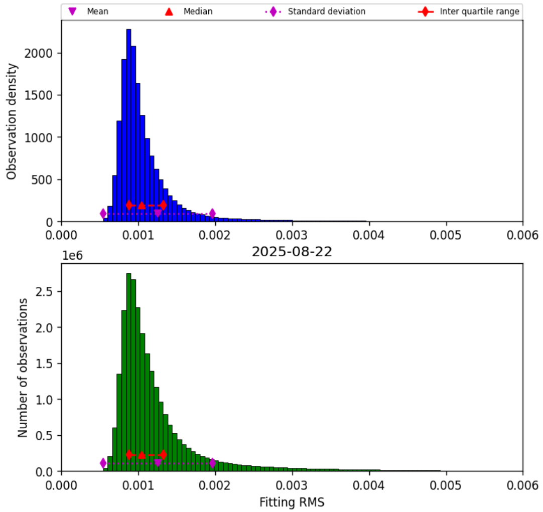
Figure 23: Histogram of “Fitting RMS” for 2025-08-21 to 2025-08-23
