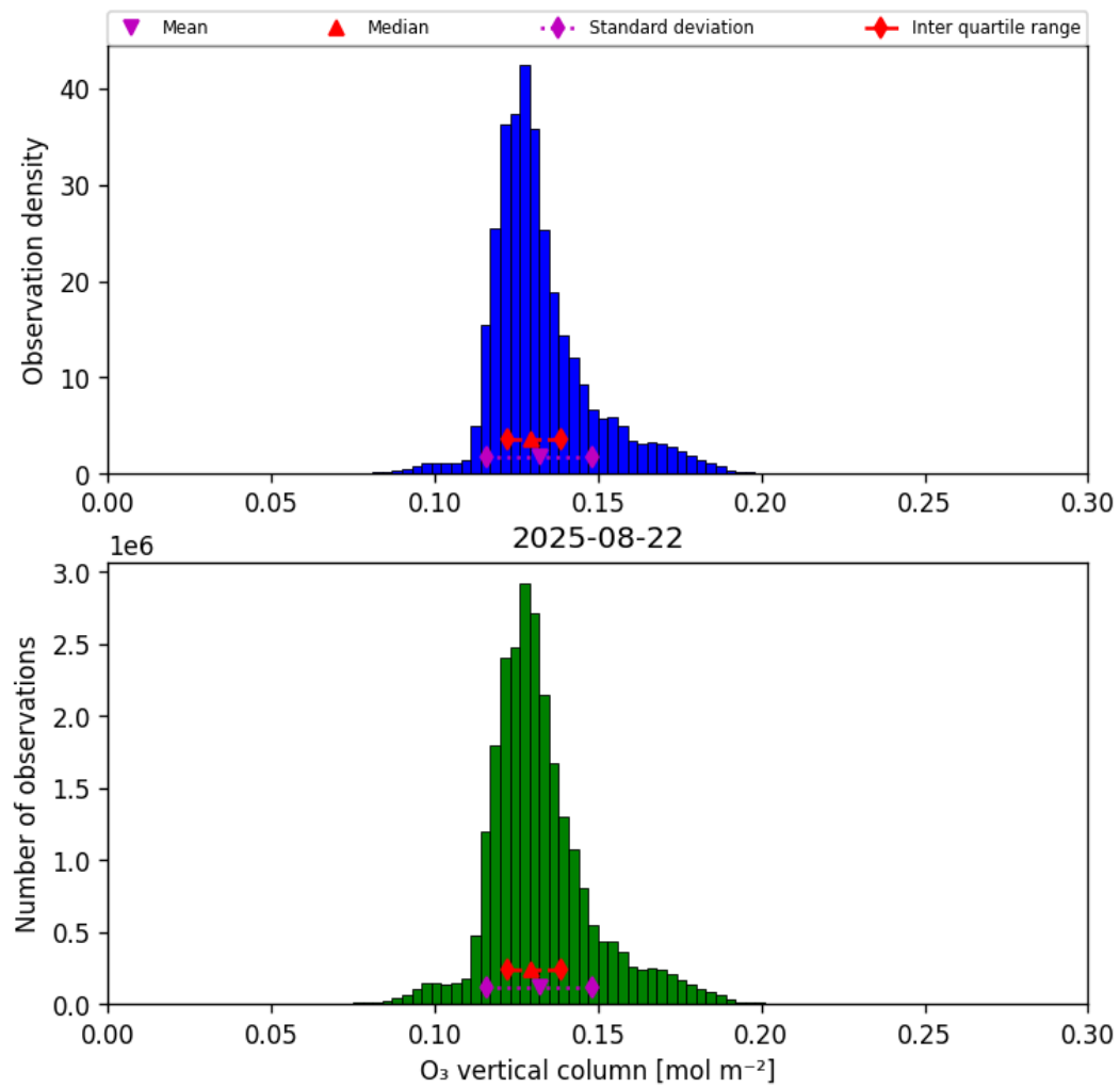
Figure 21: Histogram of “O 3 vertical column” for 2025-08-21 to 2025-08-23
