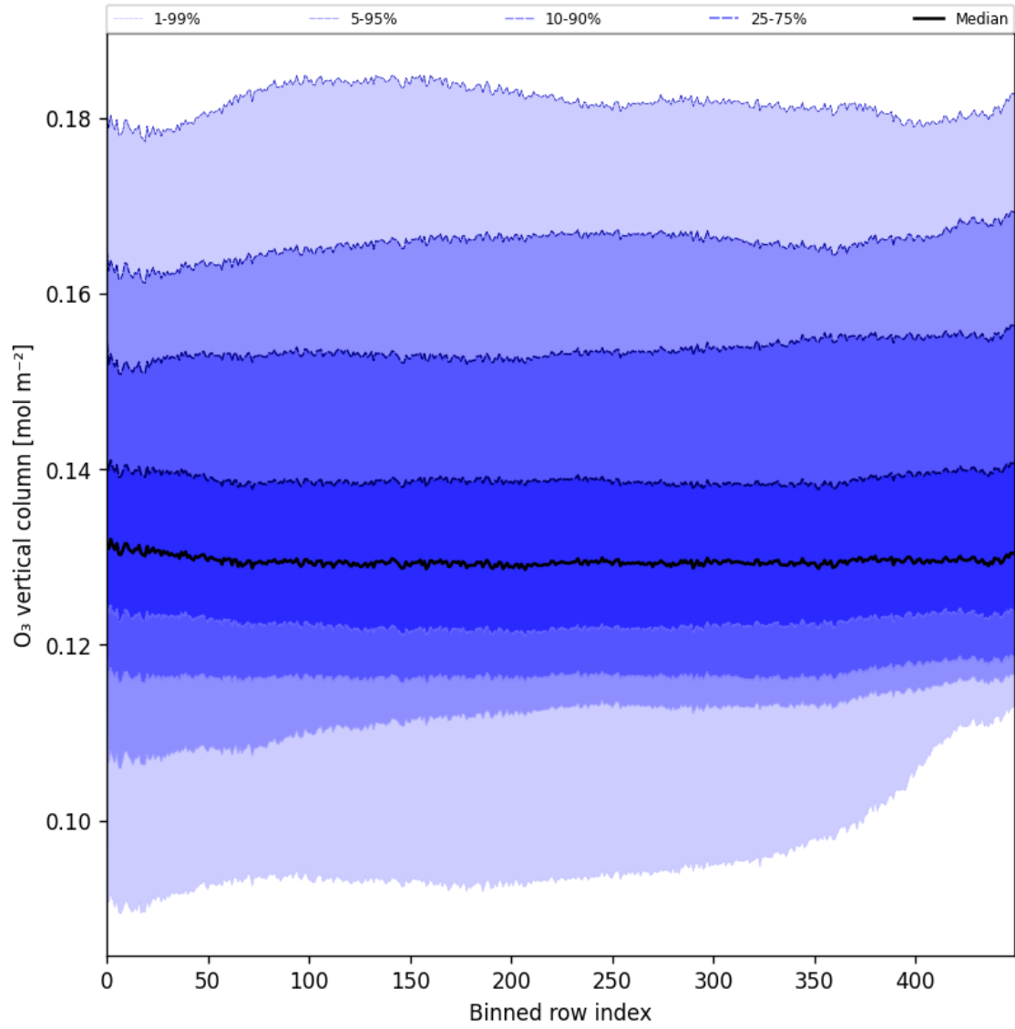
Figure 28: Along track statistics of “O 3 vertical column” for 2025-08-21 to 2025-08-23
