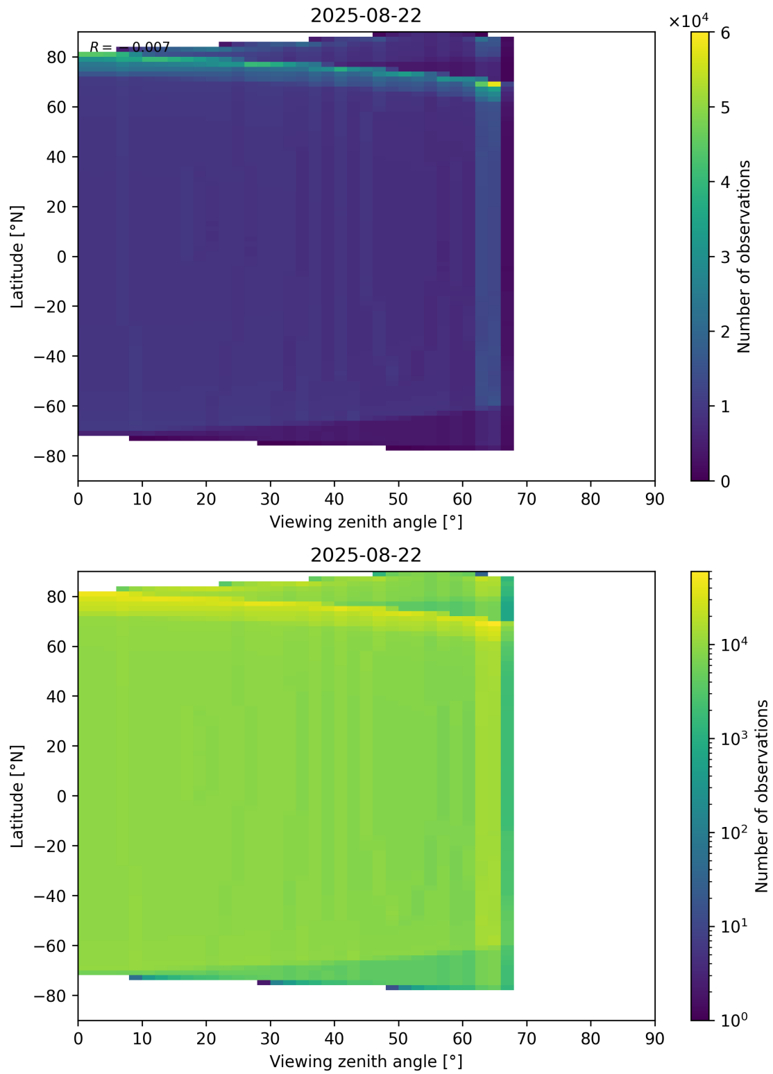
Figure 49: Scatter density plot of “Viewing zenith angle” against “Latitude” for 2025-08-21 to 2025-08-23.
