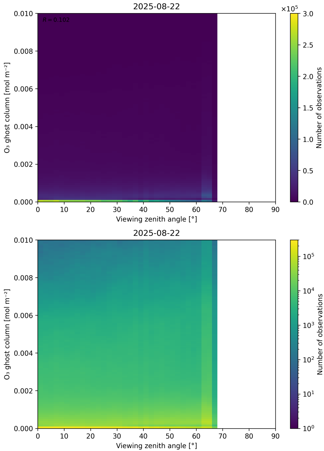
Figure 51: Scatter density plot of “Viewing zenith angle” against “O 3 ghost column” for 2025-08-21 to 2025-08-23.
