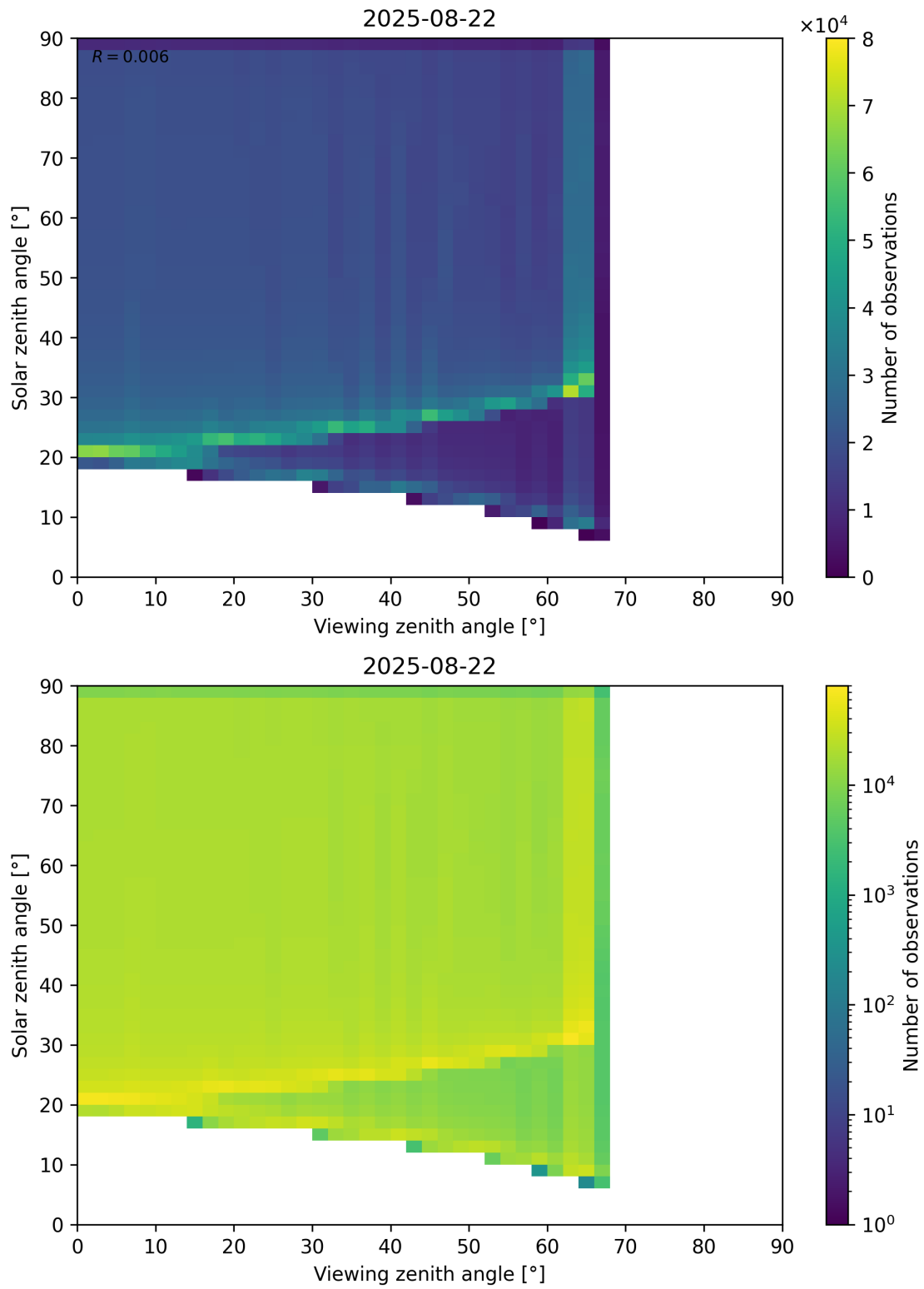
Figure 54: Scatter density plot of “Viewing zenith angle” against “Solar zenith angle” for 2025-08-21 to 2025-08-23.
