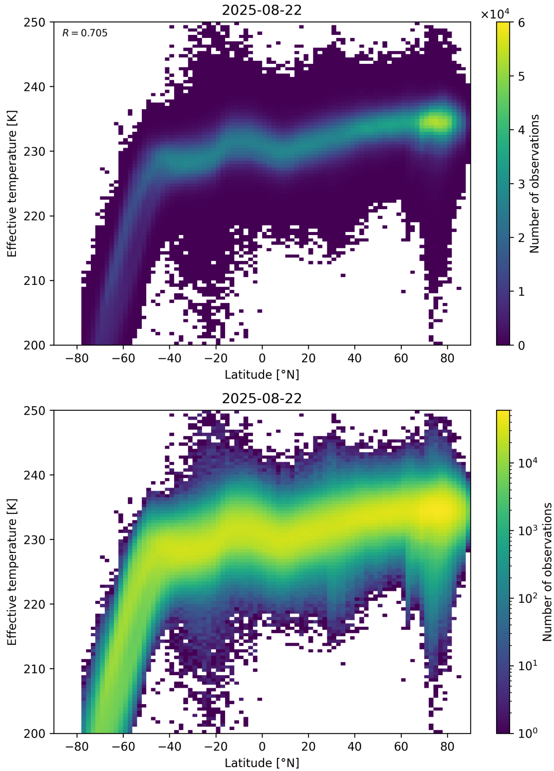
Figure 34: Scatter density plot of “Latitude” against “Effective temperature” for 2025-08-21 to 2025-08-23.
