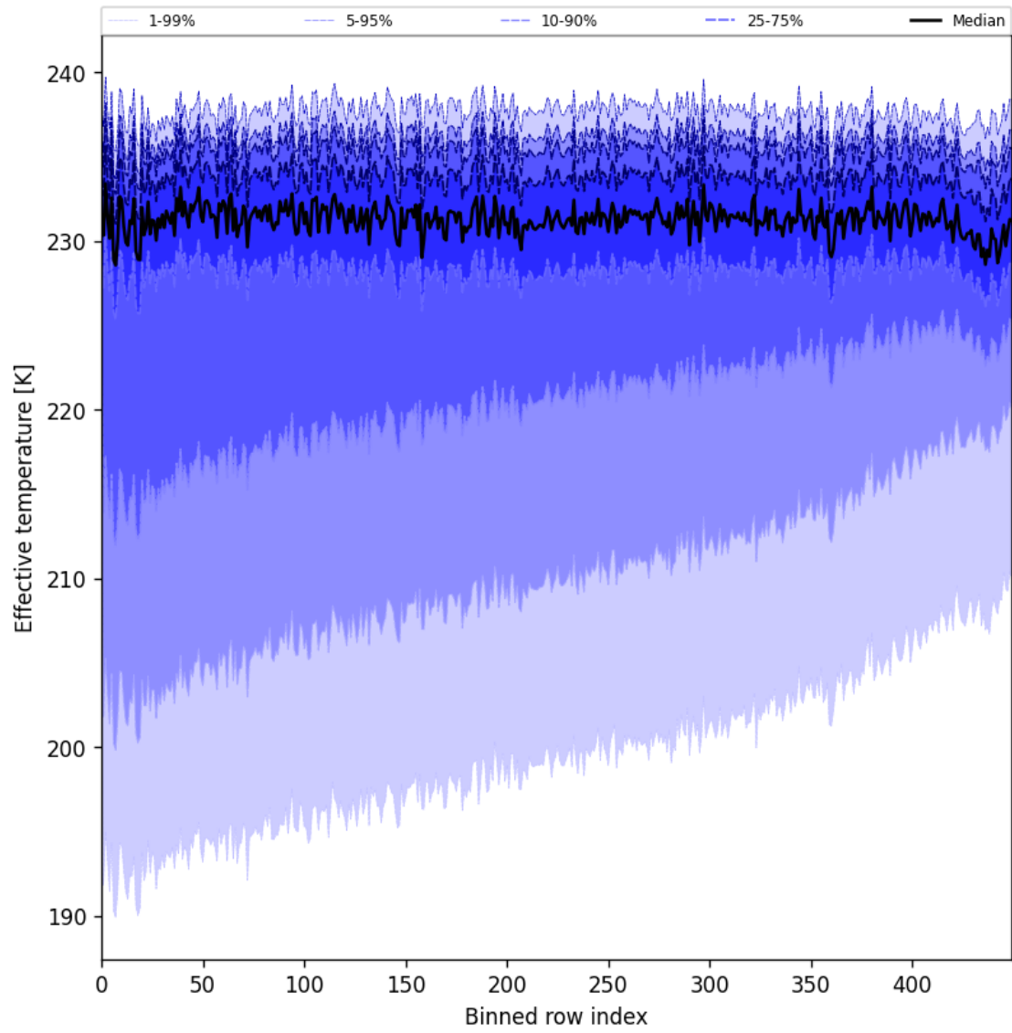
Figure 31: Along track statistics of “Effective temperature” for 2025-08-21 to 2025-08-23
