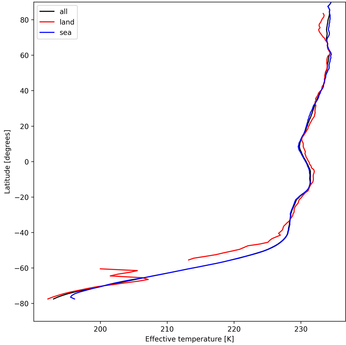
Figure 17: Zonal average of "Effective temperature" for 2025-08-21 to 2025-08-23.
