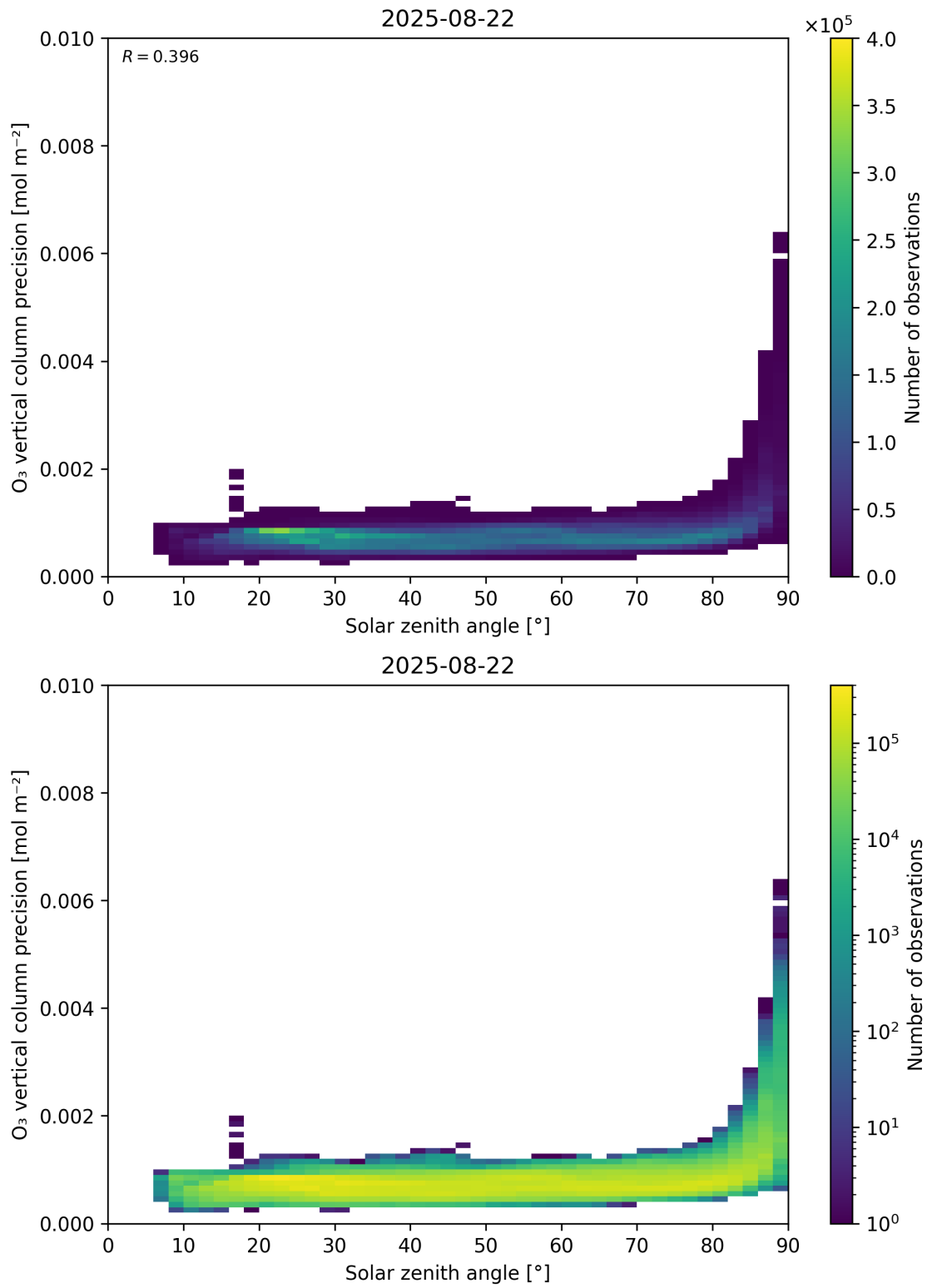
Figure 48: Scatter density plot of “Solar zenith angle” against “O 3 vertical column precision” for 2025-08-21 to 2025-08-23.
