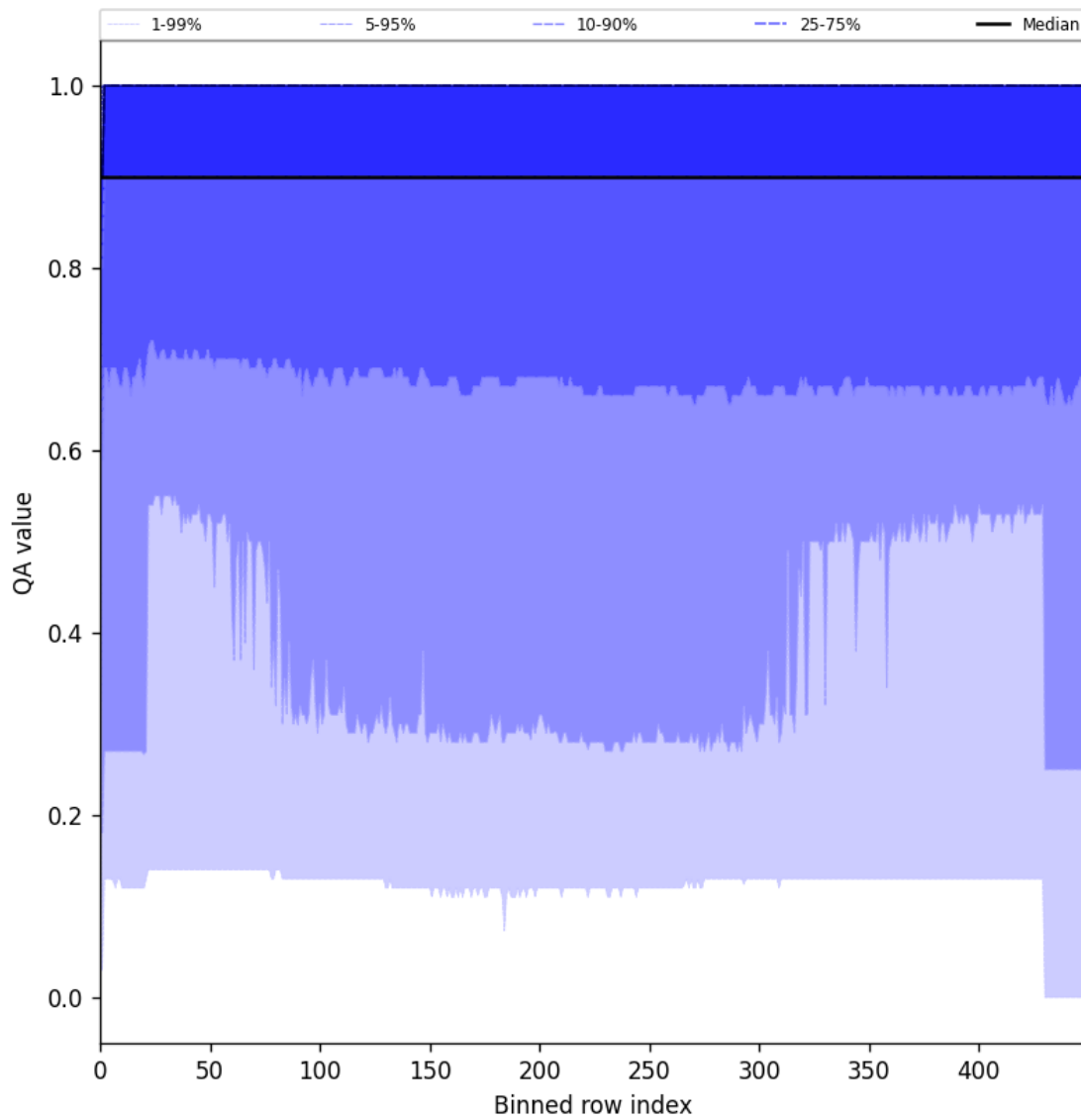
Figure 27: Along track statistics of “QA value” for 2025-08-21 to 2025-08-23
