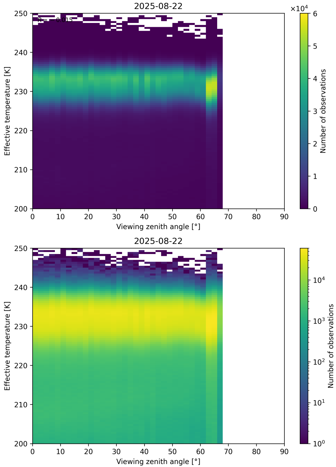
Figure 50: Scatter density plot of “Viewing zenith angle” against “Effective temperature” for 2025-08-21 to 2025-08-23.
