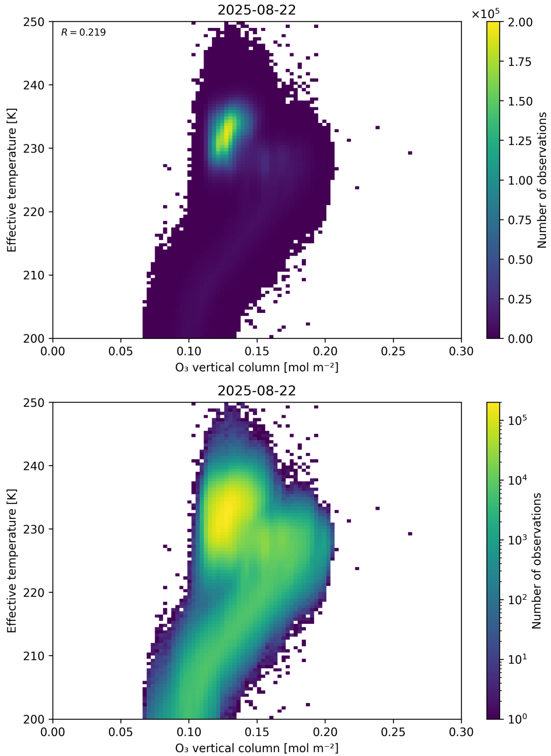
Figure 39: Scatter density plot of “O 3 vertical column” against “Effective temperature” for 2025-08-21 to 2025-08-23.
