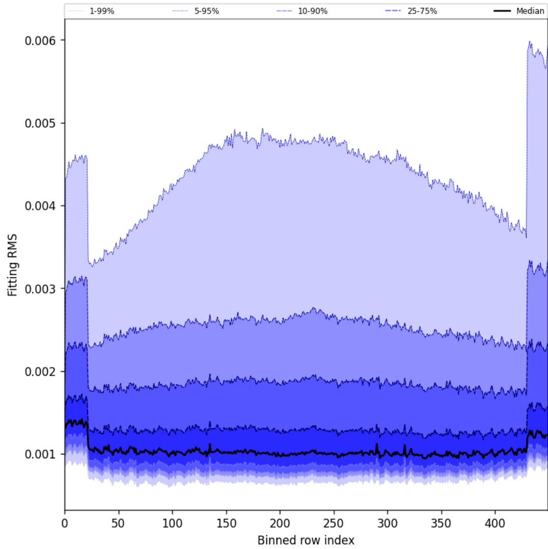
Figure 30: Along track statistics of “Fitting RMS” for 2025-08-21 to 2025-08-23
