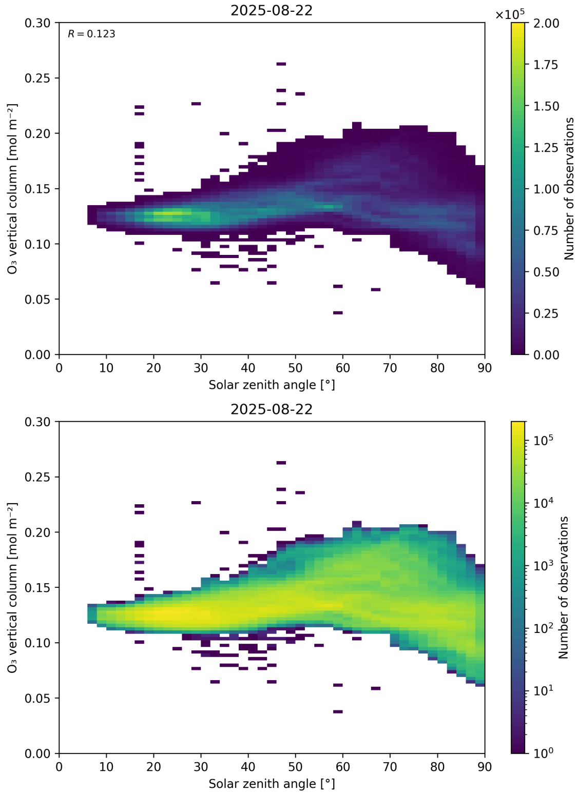
Figure 47: Scatter density plot of “Solar zenith angle” against “O 3 vertical column” for 2025-08-21 to 2025-08-23.
