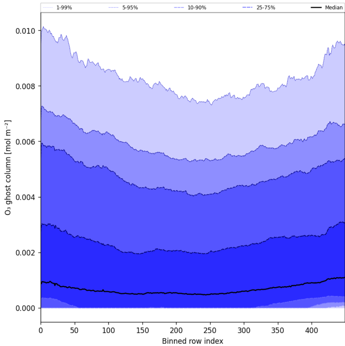
Figure 32: Along track statistics of “O 3 ghost column” for 2025-08-21 to 2025-08-23
