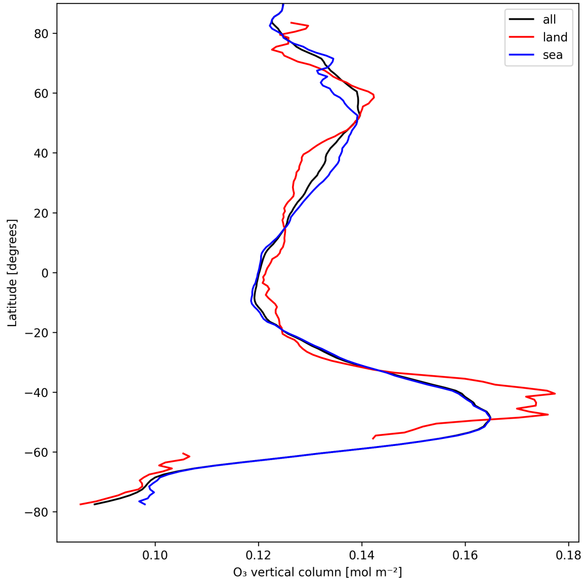
Figure 14: Zonal average of “O 3 vertical column” for 2025-08-21 to 2025-08-23.
