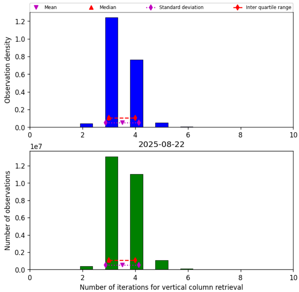
Figure 26: Histogram of “Number of iterations for vertical column retrieval” for 2025-08-21 to 2025-08-23
