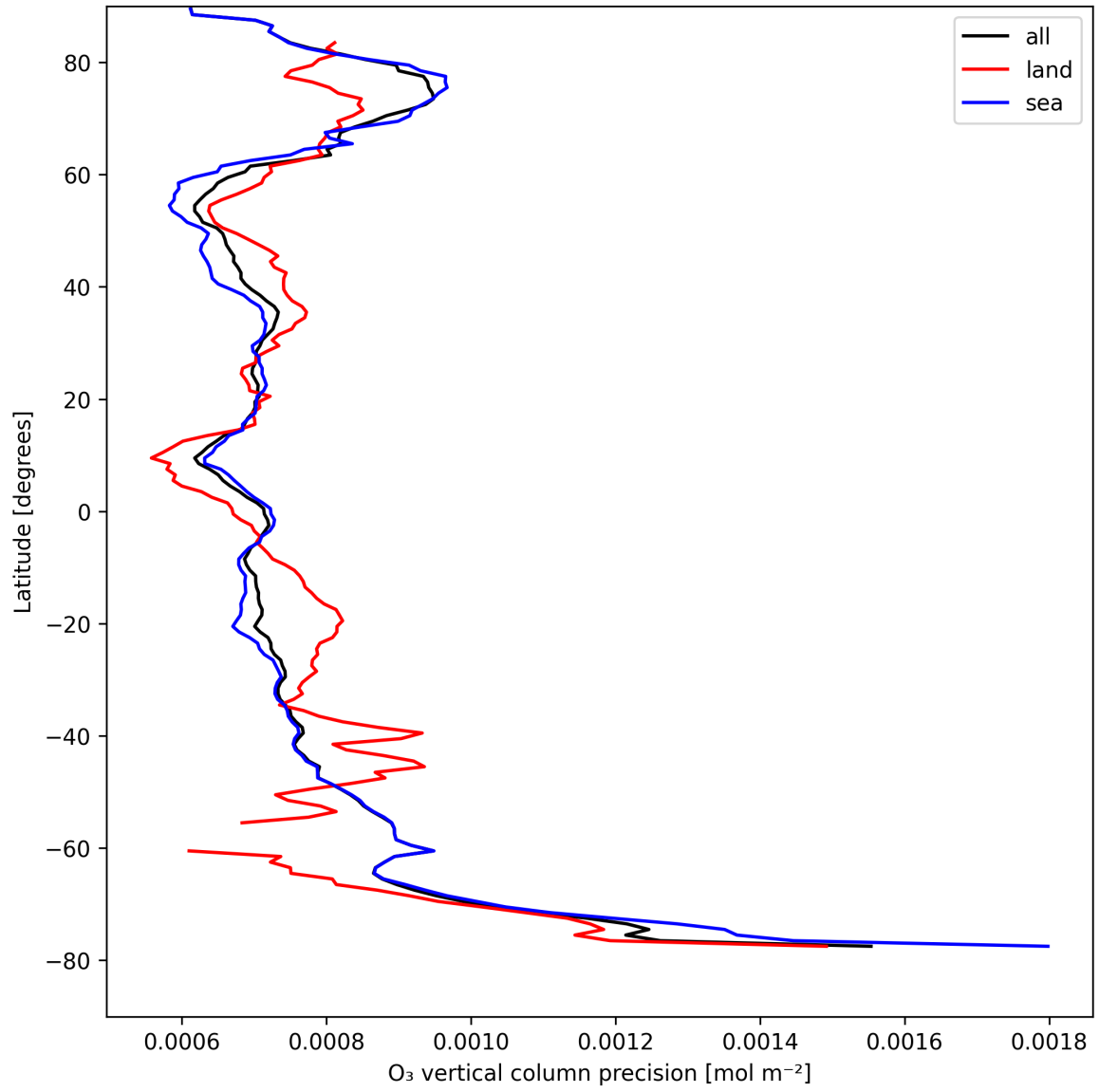
Figure 15: Zonal average of "O 3 vertical column precision" for 2025-08-21 to 2025-08-23.
