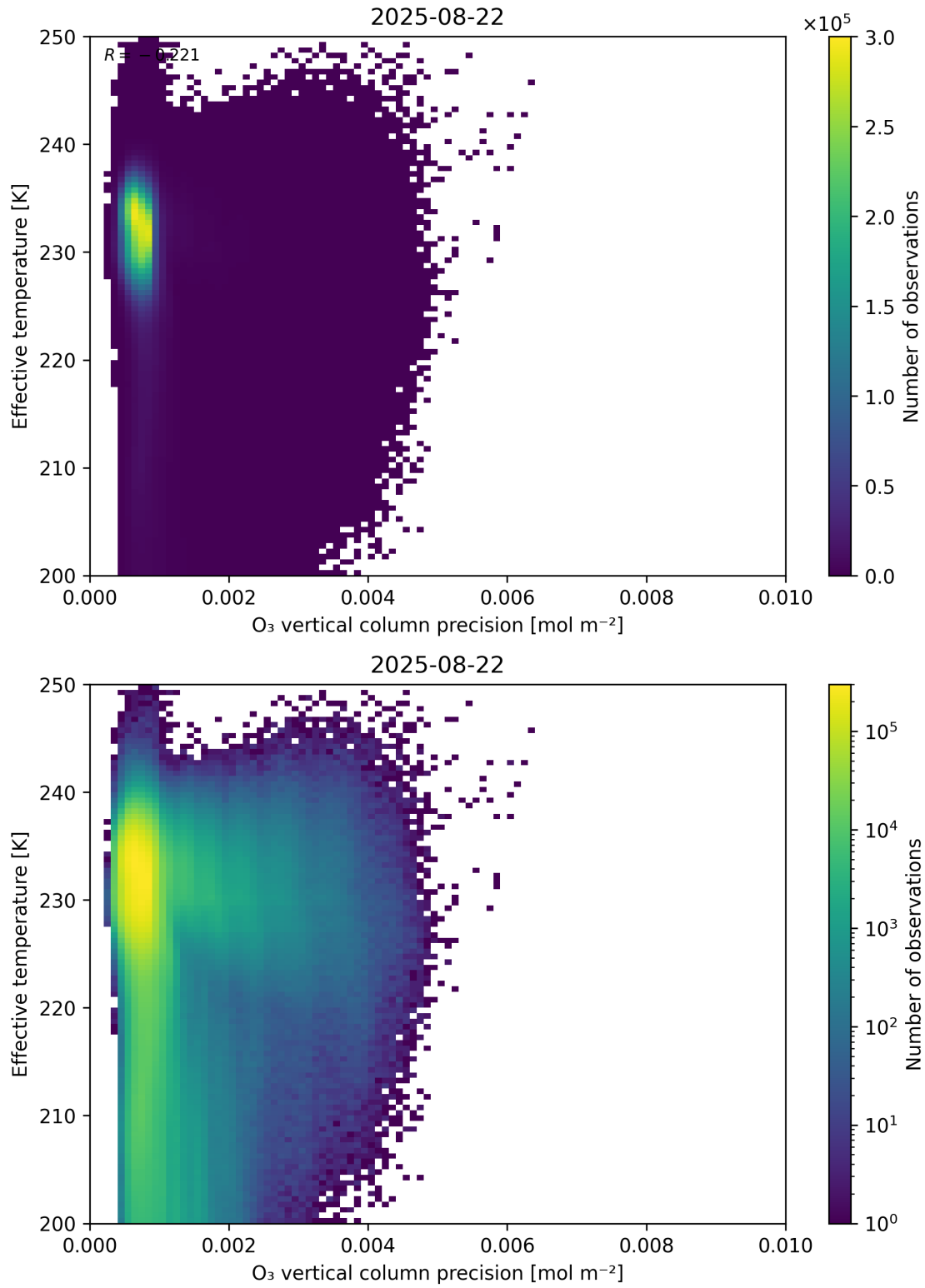
Figure 42: Scatter density plot of “O 3 vertical column precision” against “Effective temperature” for 2025-08-21 to 2025-08-23.
