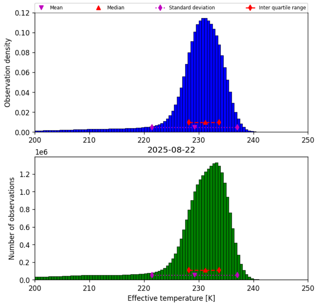
Figure 24: Histogram of “Effective temperature” for 2025-08-21 to 2025-08-23
