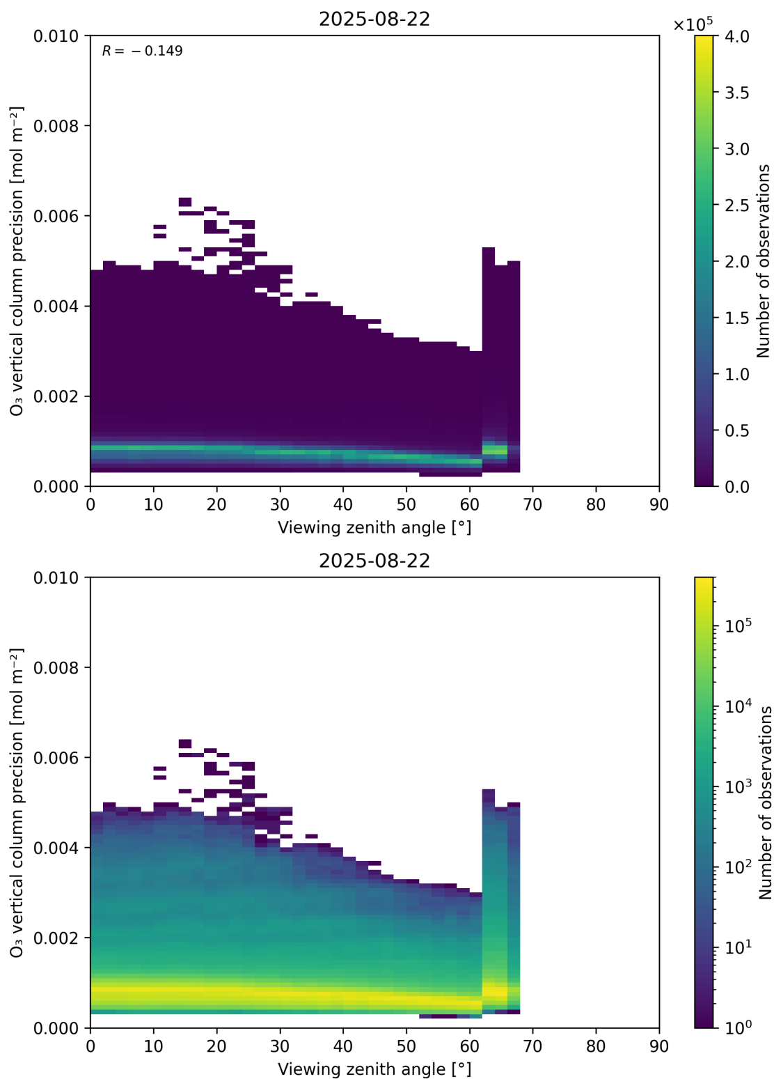
Figure 53: Scatter density plot of “Viewing zenith angle” against “O 3 vertical column precision” for 2025-08-21 to 2025-08-23.
