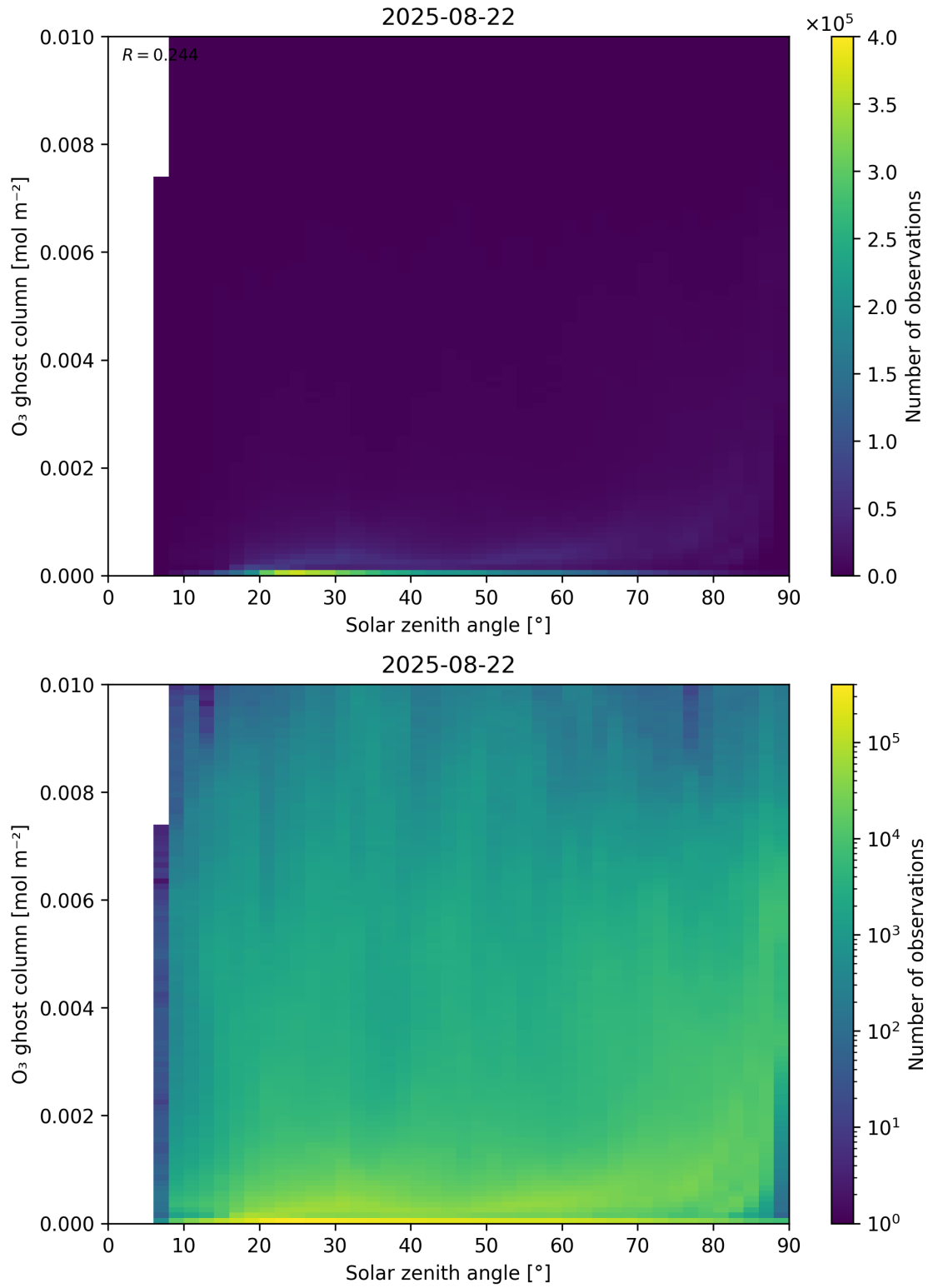
Figure 46: Scatter density plot of “Solar zenith angle” against “O 3 ghost column” for 2025-08-21 to 2025-08-23.
