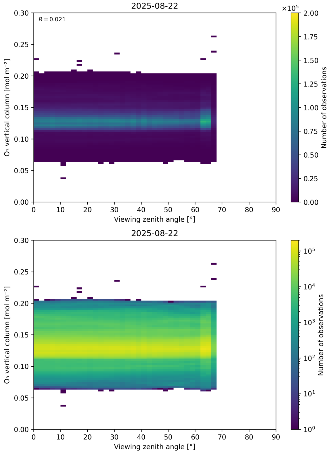
Figure 52: Scatter density plot of “Viewing zenith angle” against “O 3 vertical column” for 2025-08-21 to 2025-08-23.
