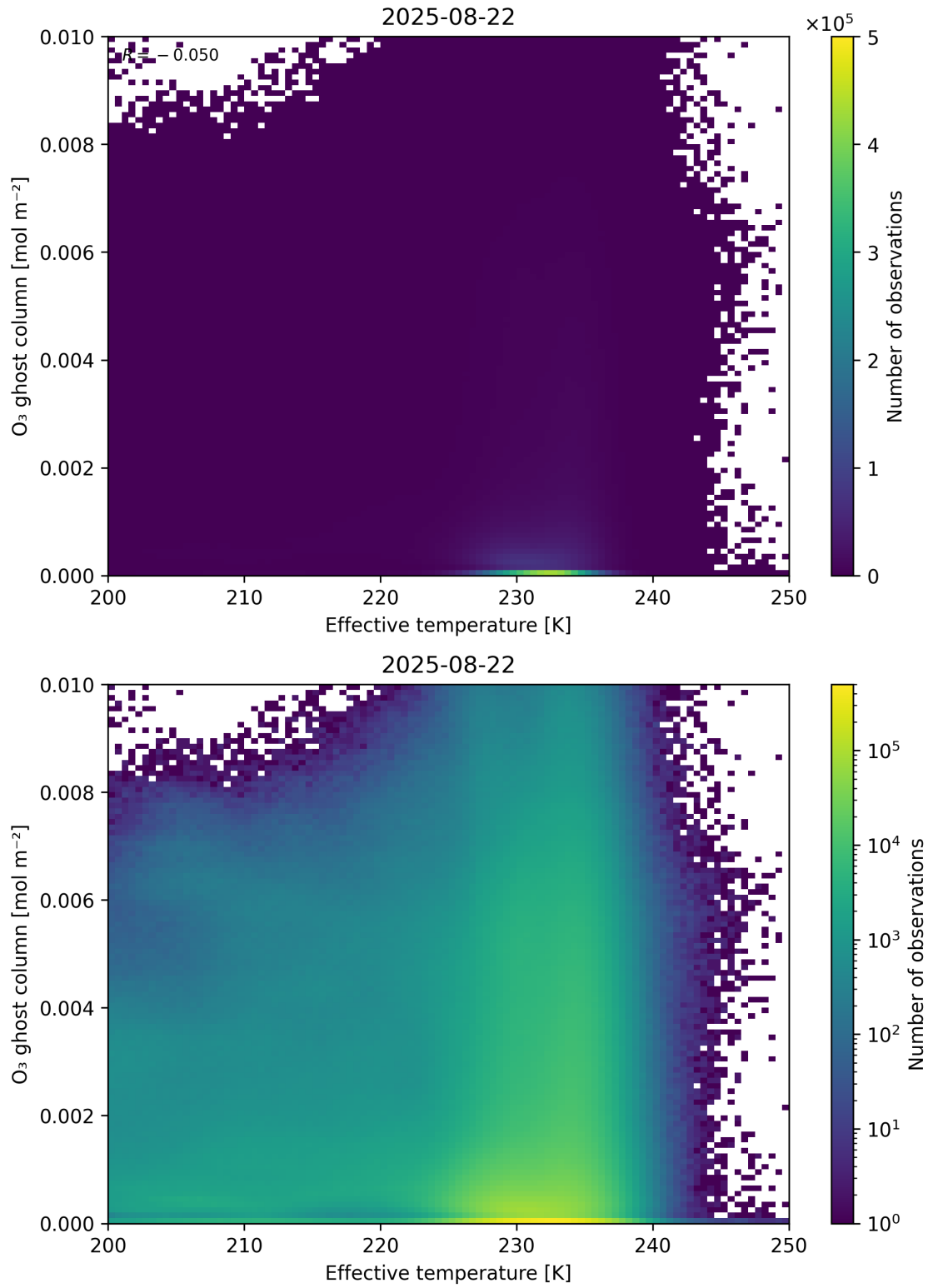
Figure 38: Scatter density plot of “Effective temperature” against “O 3 ghost column” for 2025-08-21 to 2025-08-23.
