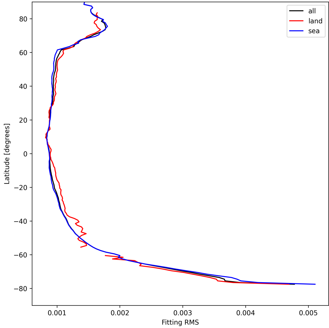
Figure 16: Zonal average of “Fitting RMS” for 2025-08-21 to 2025-08-23.
