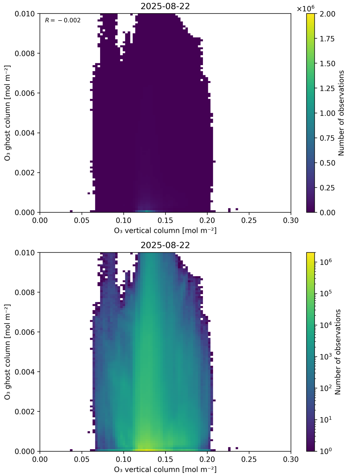
Figure 40: Scatter density plot of “O 3 vertical column” against “O 3 ghost column” for 2025-08-21 to 2025-08-23.
