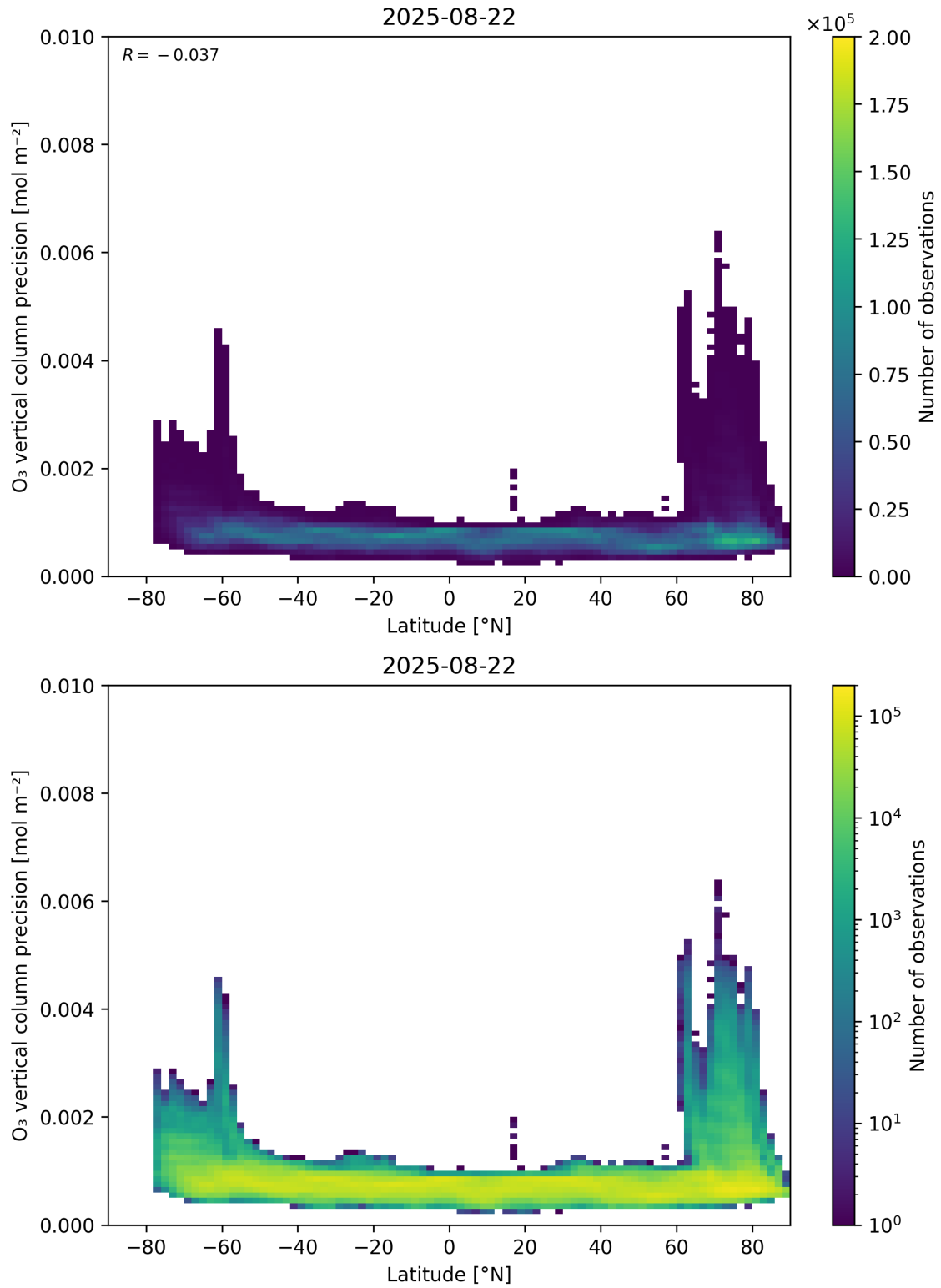
Figure 37: Scatter density plot of “Latitude” against “O 3 vertical column precision” for 2025-08-21 to 2025-08-23.
