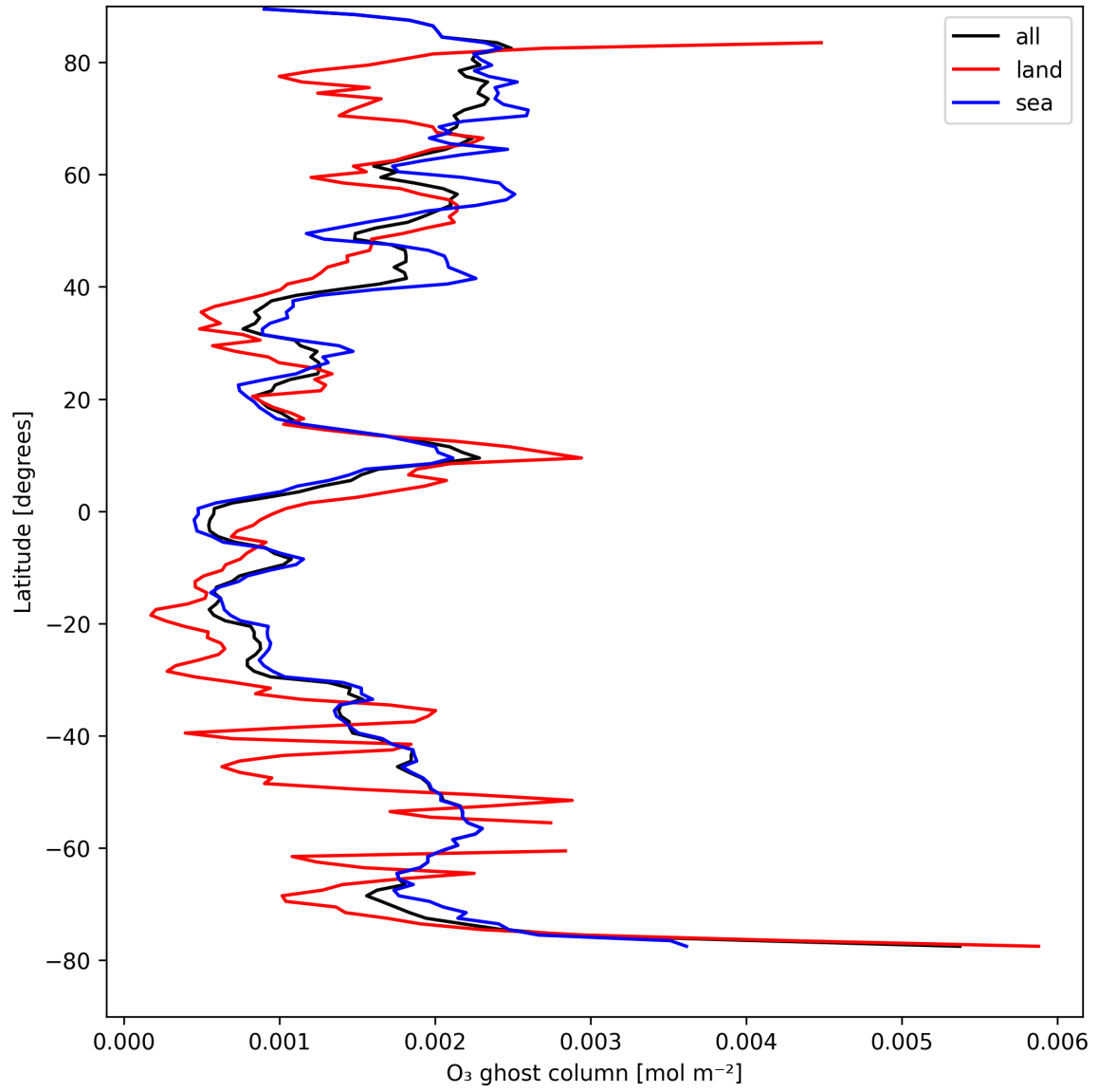
Figure 18: Zonal average of “O 3 ghost column” for 2025-08-21 to 2025-08-23.
