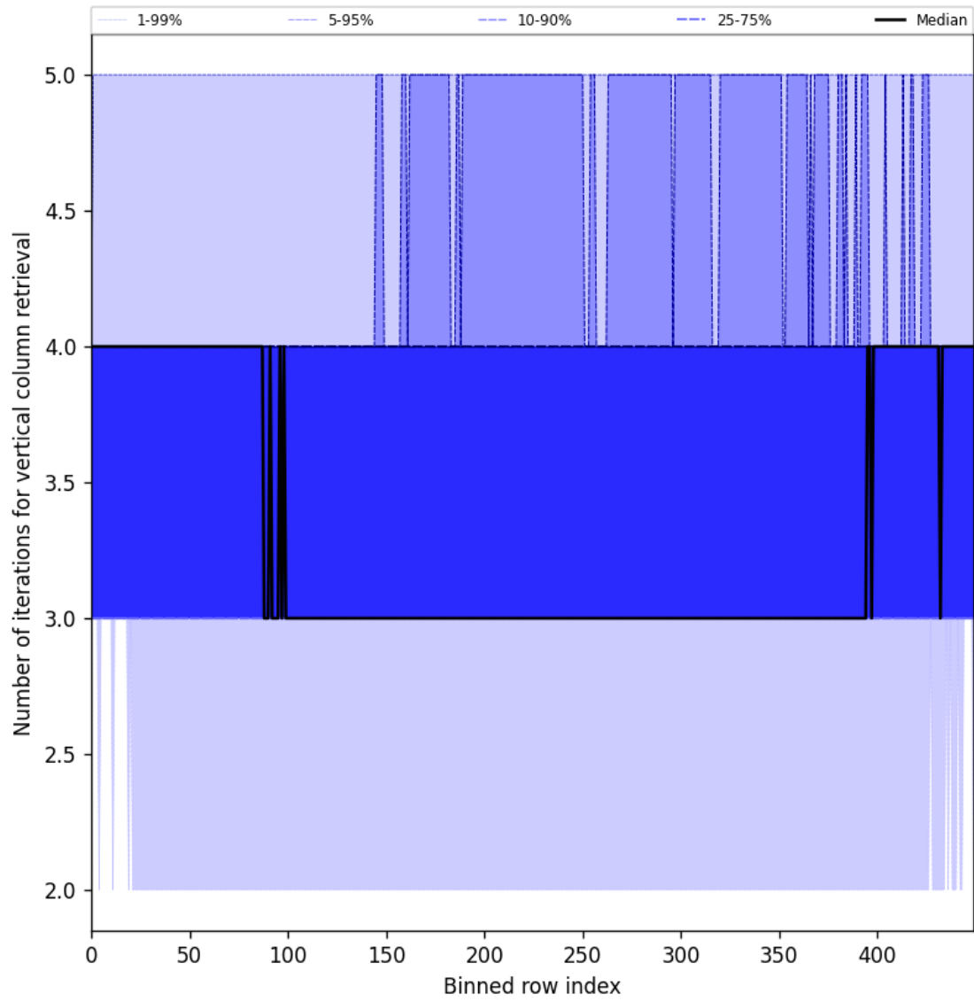
Figure 33: Along track statistics of “Number of iterations for vertical column retrieval” for 2025-08-21 to 2025-08-23
