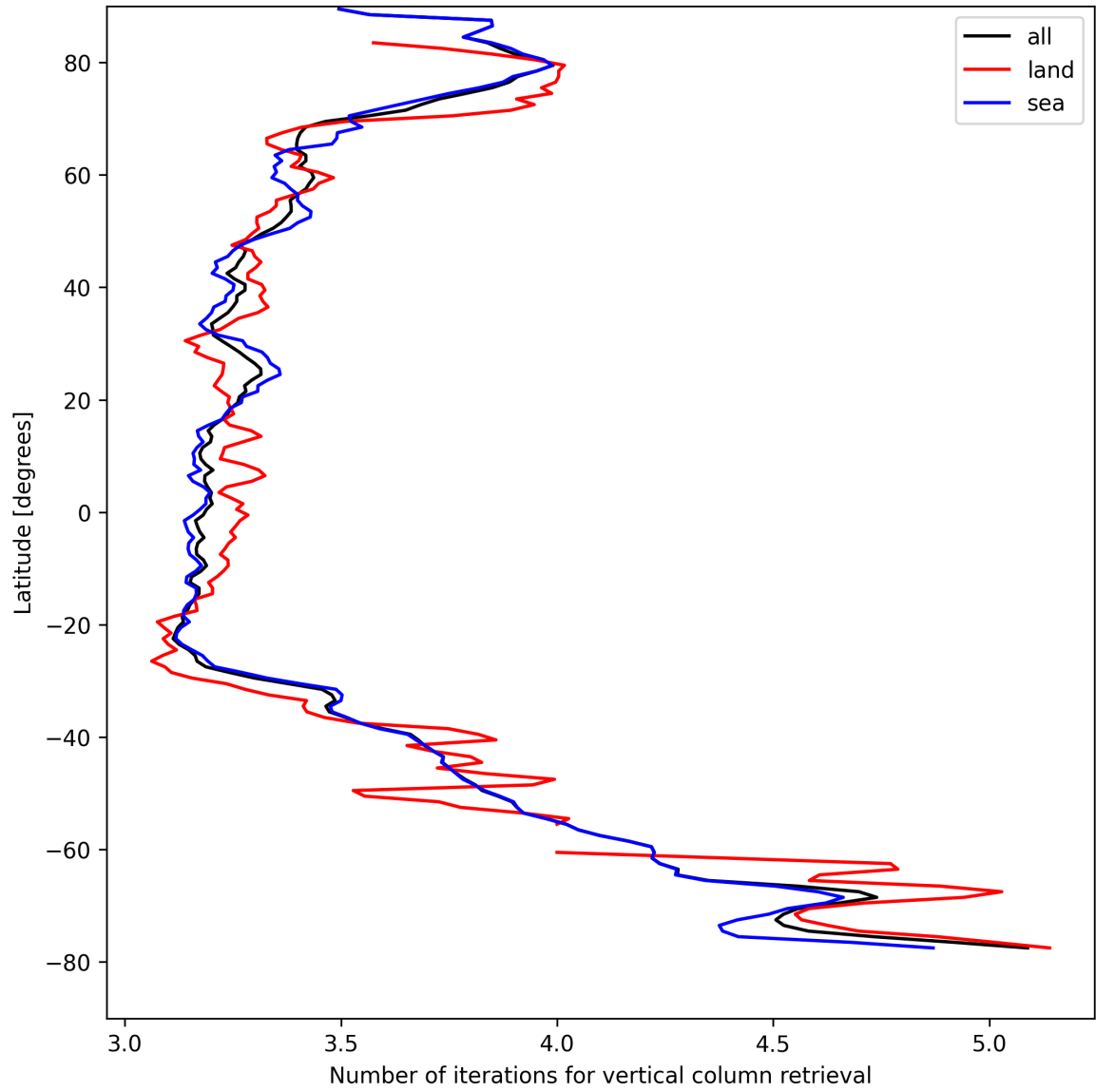
Figure 19: Zonal average of “Number of iterations for vertical column retrieval” for 2025-08-21 to 2025-08-23.
