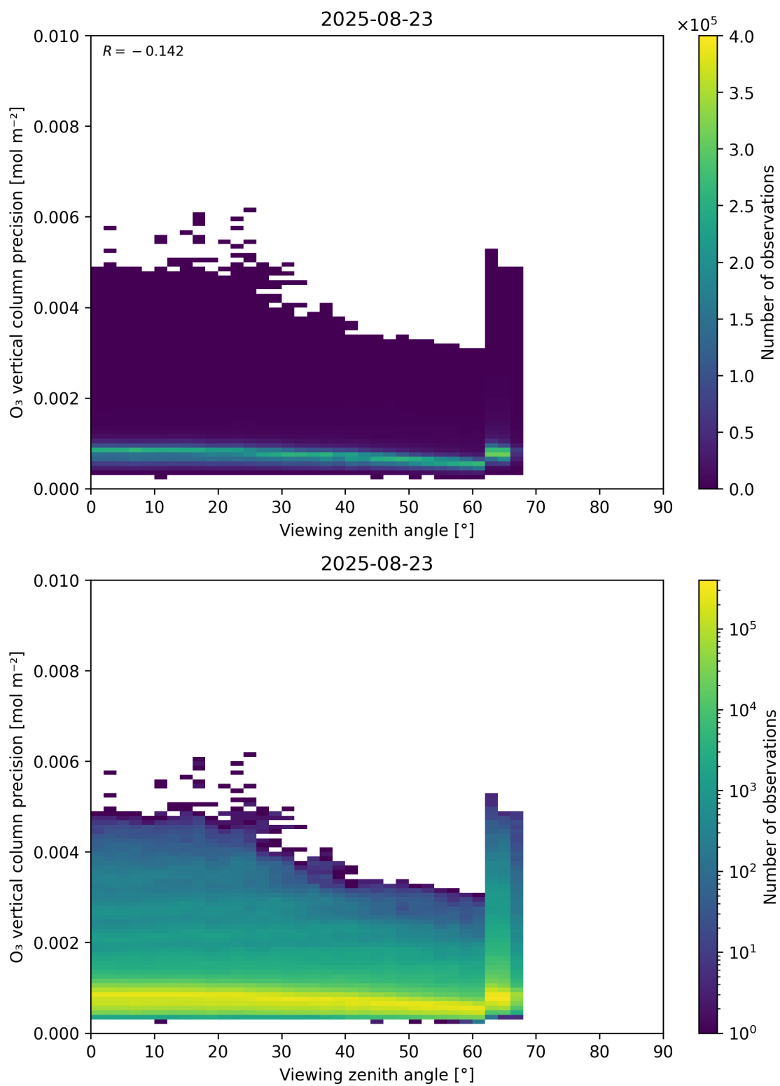
Figure 53: Scatter density plot of “Viewing zenith angle” against “O 3 vertical column precision” for 2025-08-22 to 2025-08-24.
