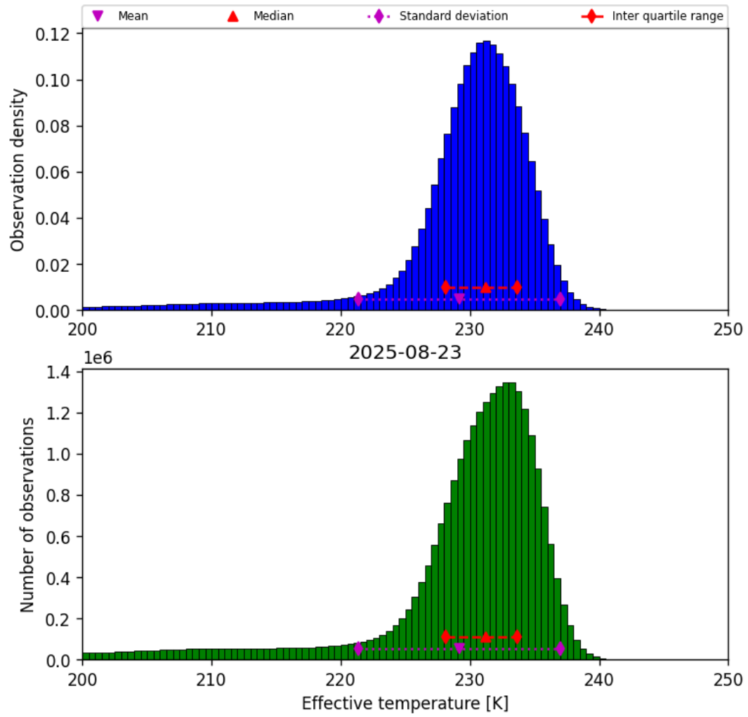
Figure 24: Histogram of “Effective temperature” for 2025-08-22 to 2025-08-24
