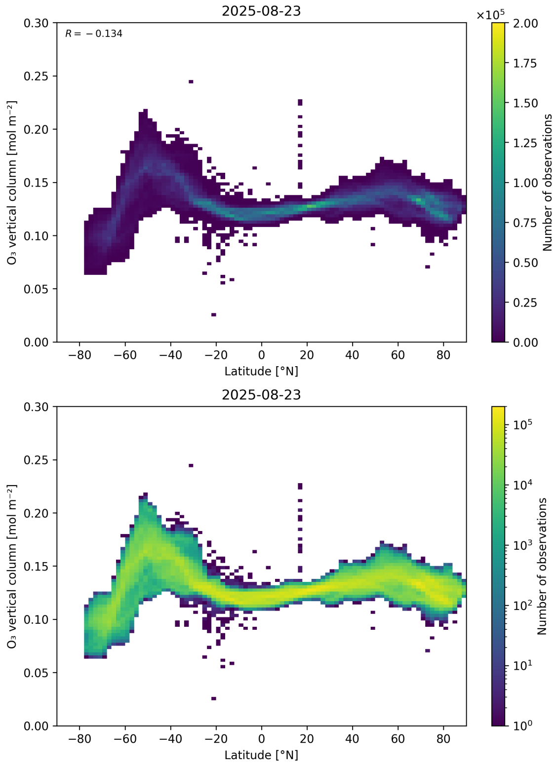
Figure 36: Scatter density plot of “Latitude” against “O 3 vertical column” for 2025-08-22 to 2025-08-24.
