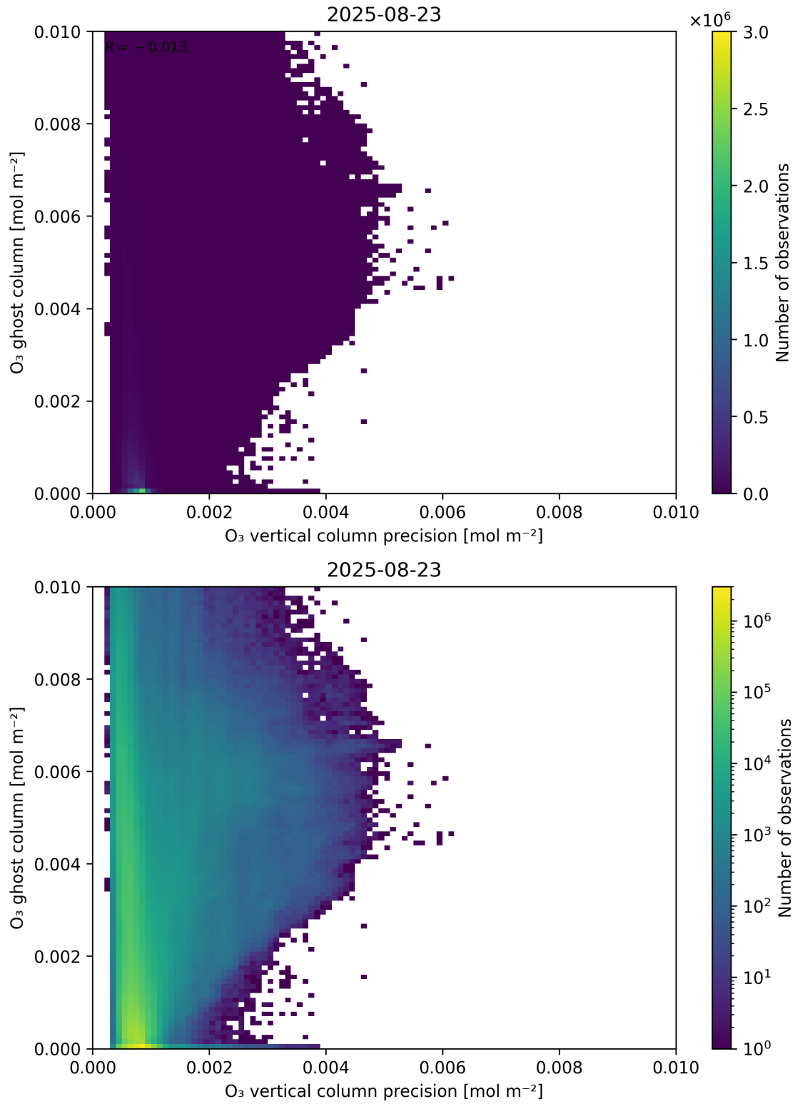
Figure 43: Scatter density plot of “ \text{O}_3 vertical column precision” against “ \text{O}_3 ghost column” for 2025-08-22 to 2025-08-24.
