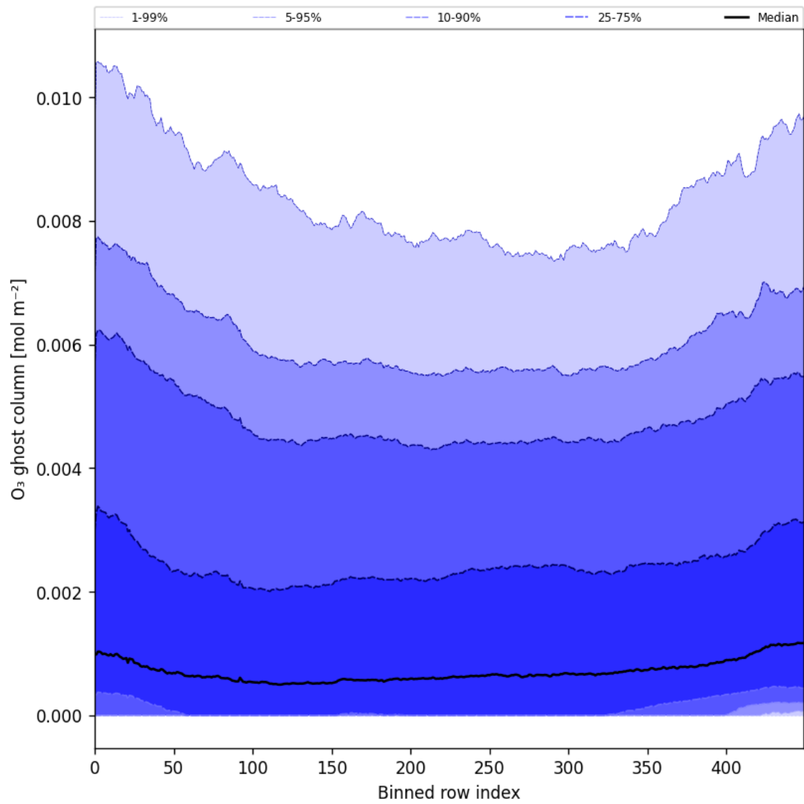
Figure 32: Along track statistics of “O 3 ghost column” for 2025-08-22 to 2025-08-24
