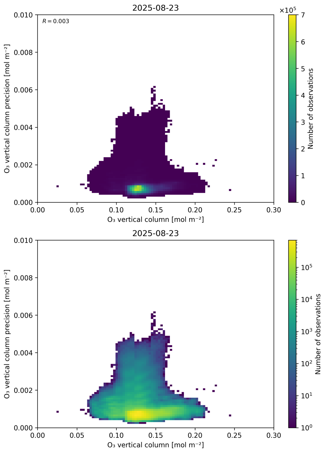
Figure 41: Scatter density plot of “O 3 vertical column” against “O 3 vertical column precision” for 2025-08-22 to 2025-08-24.
