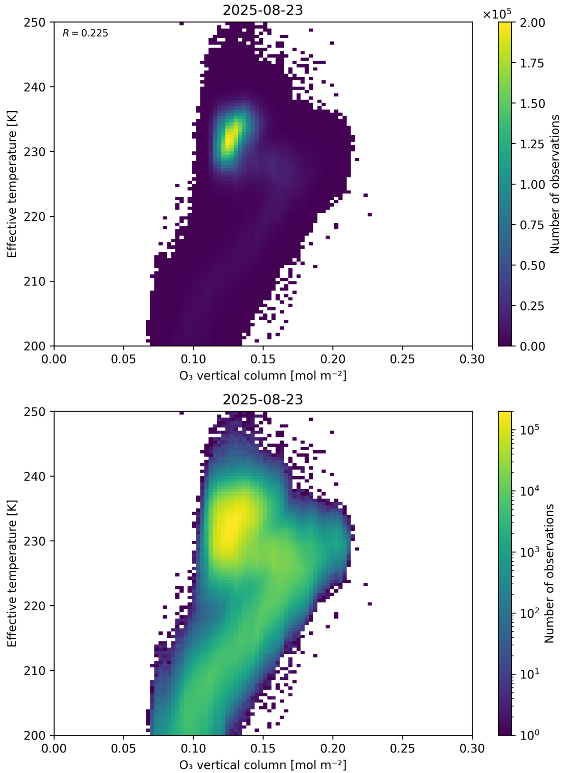
Figure 39: Scatter density plot of “O 3 vertical column” against “Effective temperature” for 2025-08-22 to 2025-08-24.
