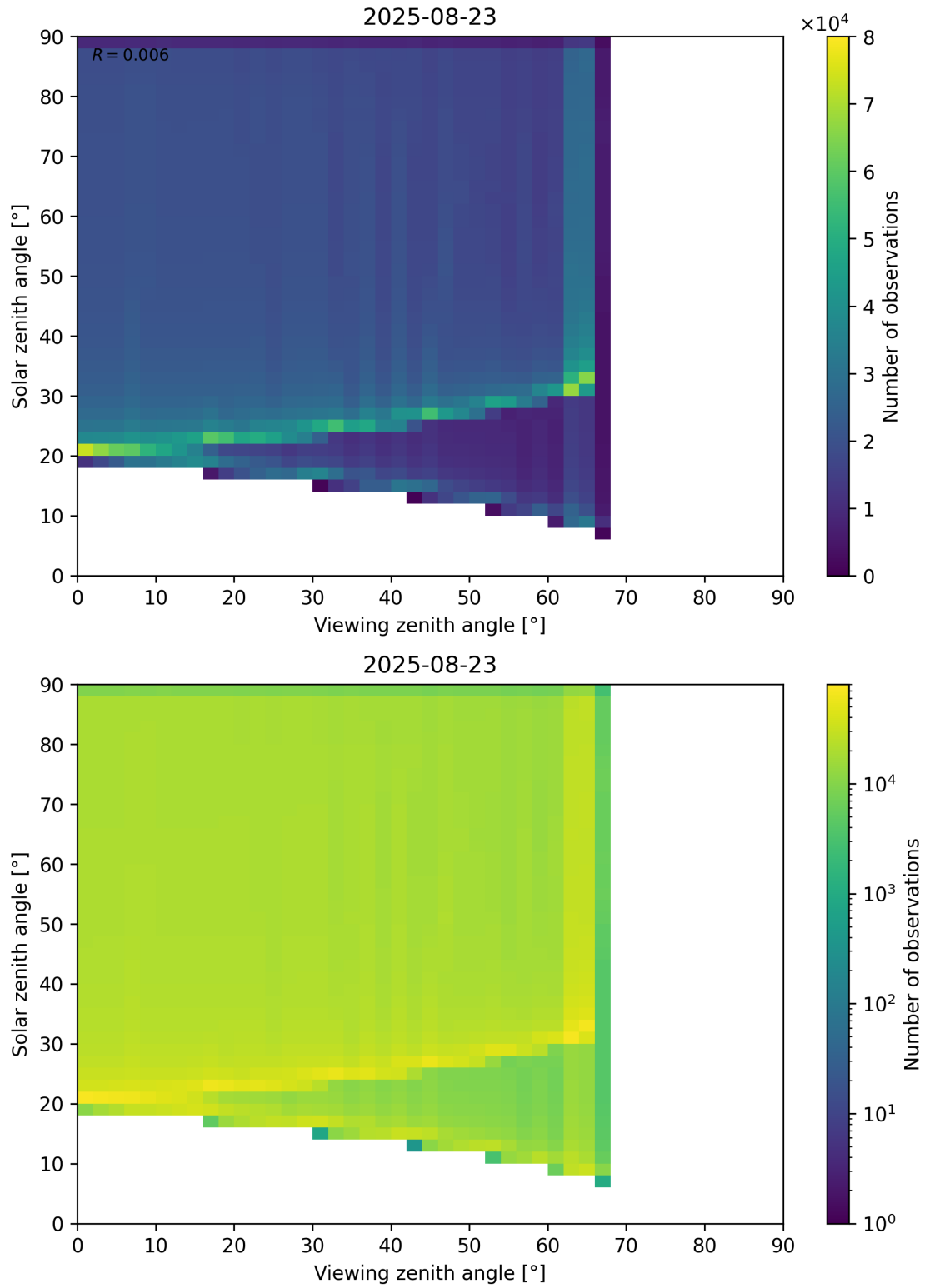
Figure 54: Scatter density plot of “Viewing zenith angle” against “Solar zenith angle” for 2025-08-22 to 2025-08-24.
