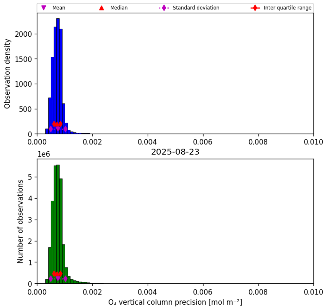
Figure 22: Histogram of “O 3 vertical column precision” for 2025-08-22 to 2025-08-24
