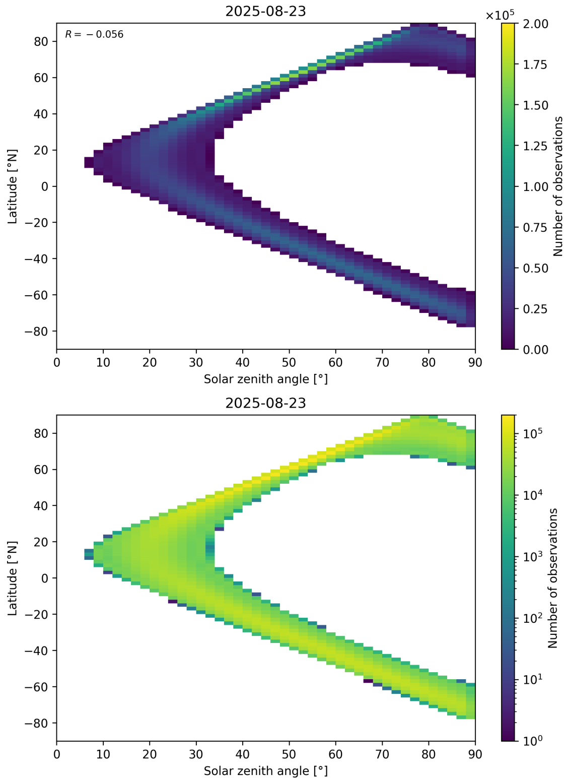
Figure 44: Scatter density plot of “Solar zenith angle” against “Latitude” for 2025-08-22 to 2025-08-24.
