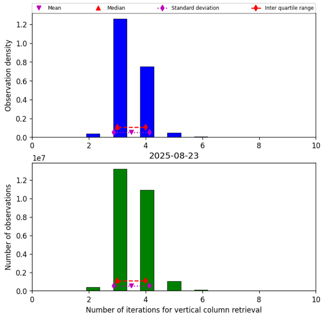
Figure 26: Histogram of “Number of iterations for vertical column retrieval” for 2025-08-22 to 2025-08-24
