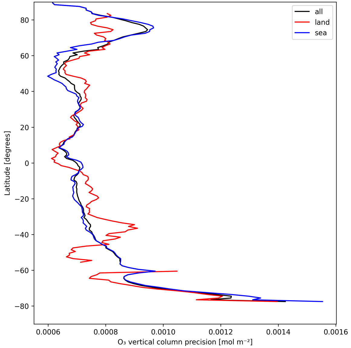
Figure 15: Zonal average of “O 3 vertical column precision” for 2025-08-22 to 2025-08-24.
