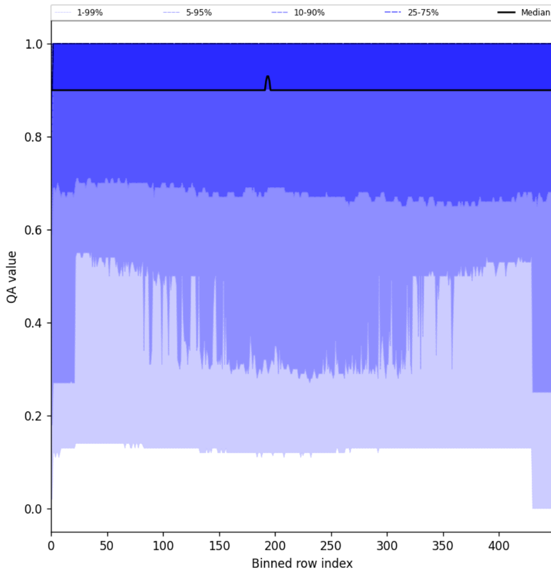
Figure 27: Along track statistics of “QA value” for 2025-08-22 to 2025-08-24
