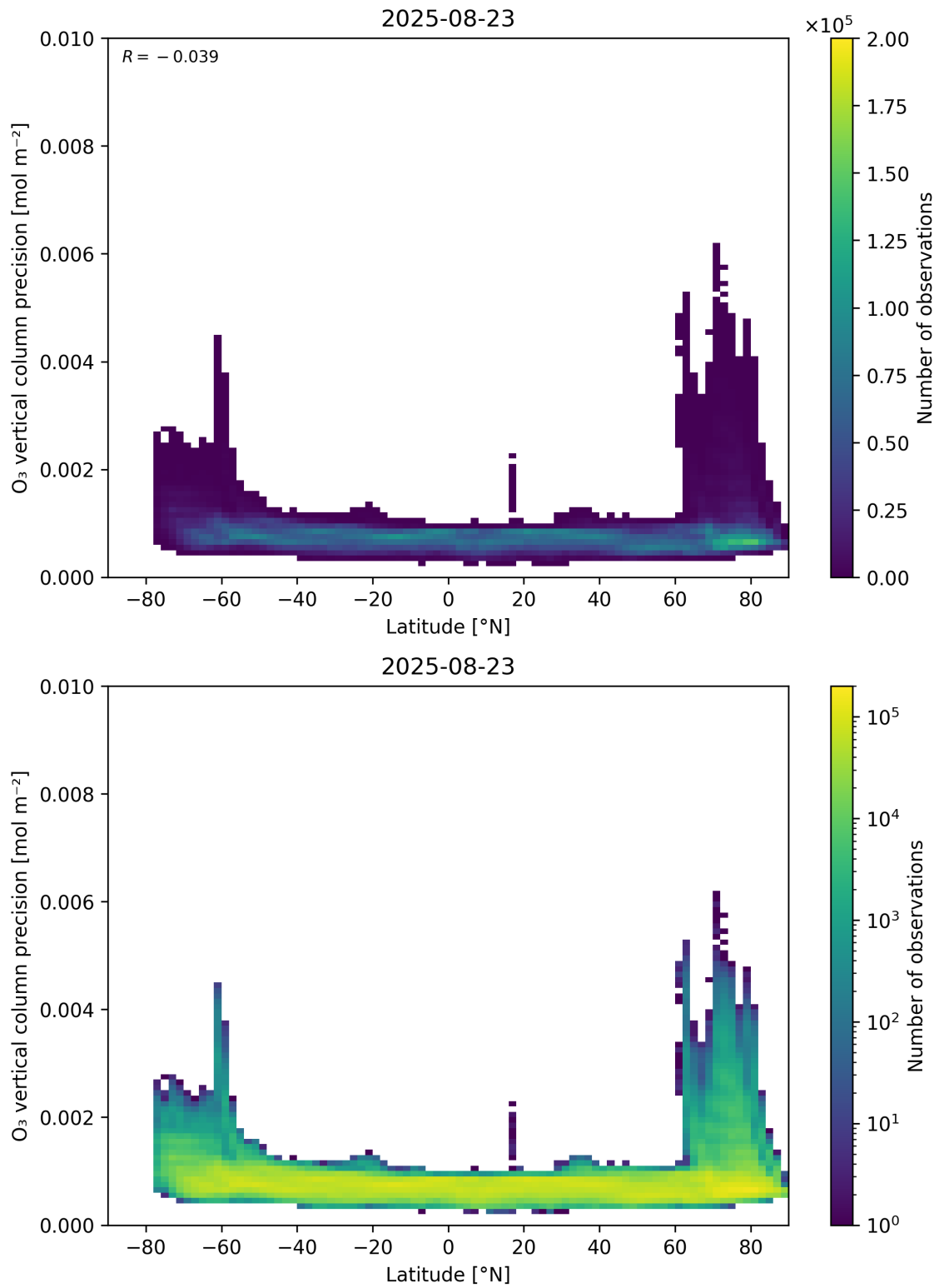
Figure 37: Scatter density plot of “Latitude” against “O 3 vertical column precision” for 2025-08-22 to 2025-08-24.
