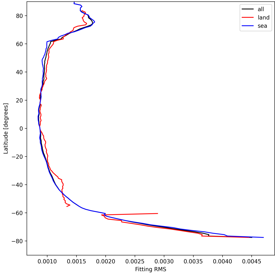
Figure 16: Zonal average of “Fitting RMS” for 2025-08-22 to 2025-08-24.
