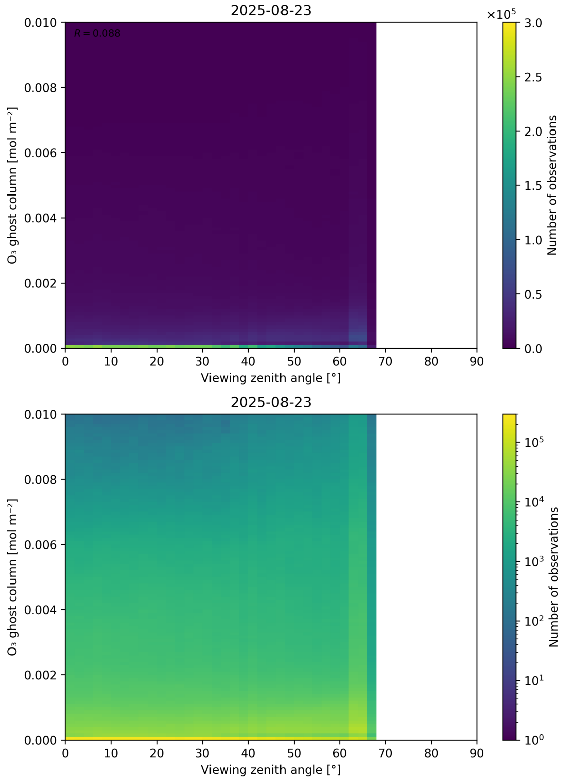
Figure 51: Scatter density plot of “Viewing zenith angle” against “O 3 ghost column” for 2025-08-22 to 2025-08-24.
