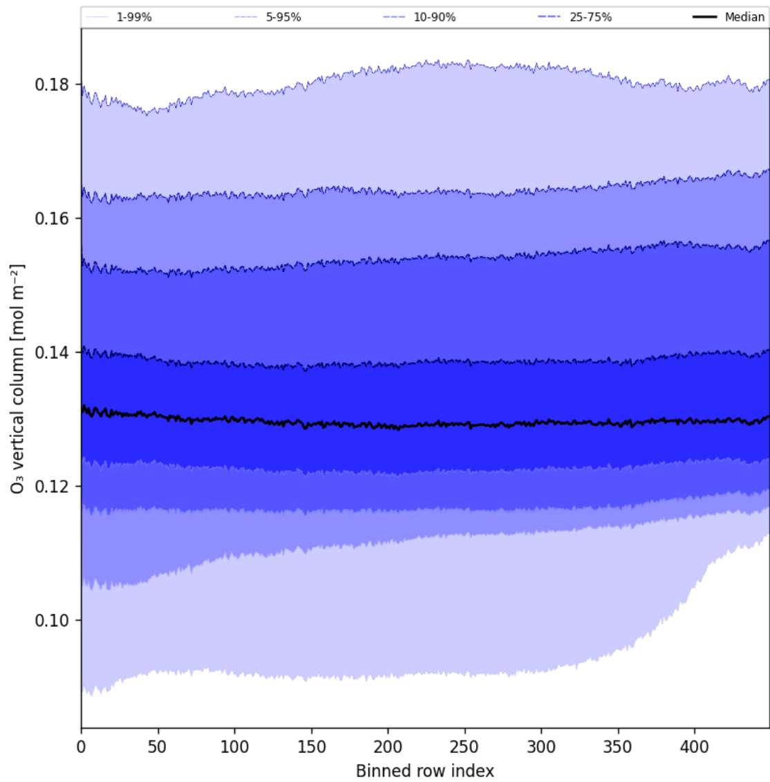
Figure 28: Along track statistics of “O 3 vertical column” for 2025-08-22 to 2025-08-24
