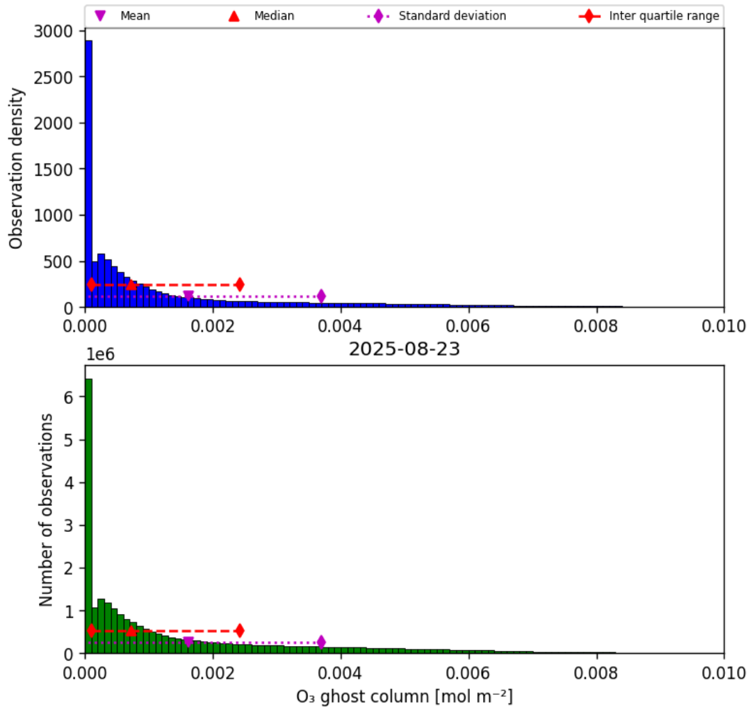
Figure 25: Histogram of “O 3 ghost column” for 2025-08-22 to 2025-08-24
