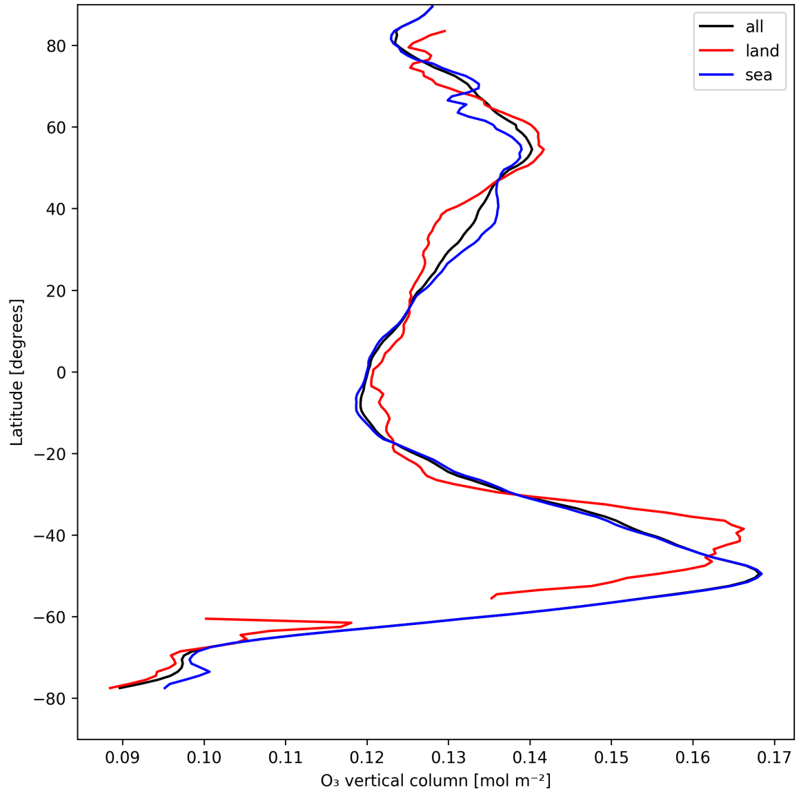
Figure 14: Zonal average of “O 3 vertical column” for 2025-08-22 to 2025-08-24.
