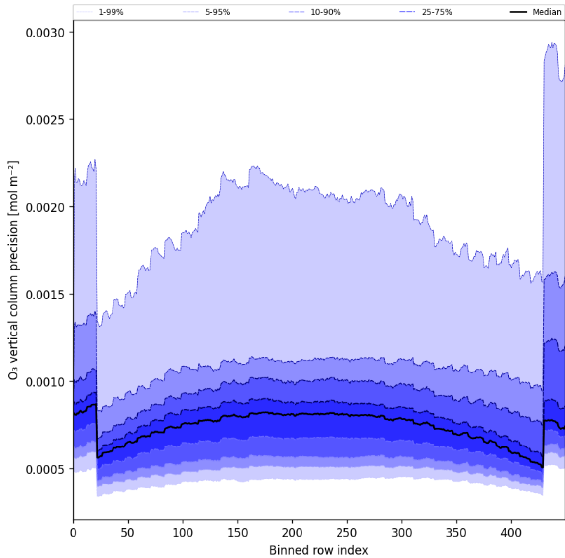
Figure 29: Along track statistics of “O 3 vertical column precision” for 2025-08-22 to 2025-08-24
