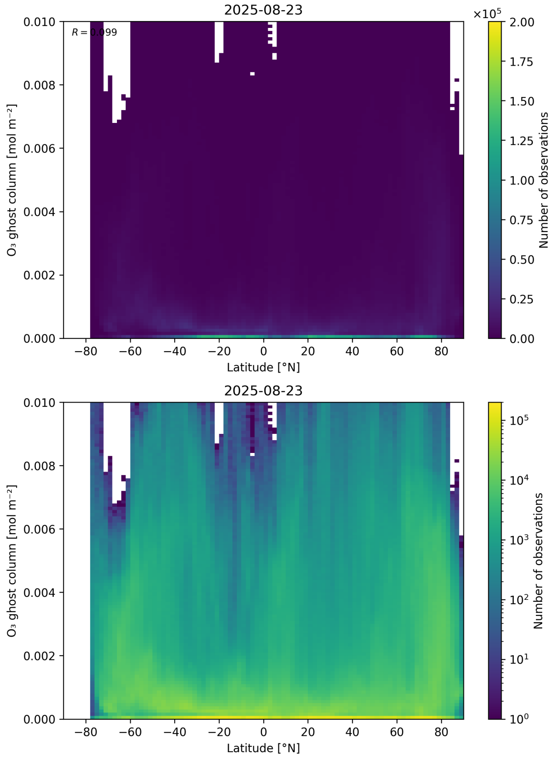
Figure 35: Scatter density plot of “Latitude” against “O 3 ghost column” for 2025-08-22 to 2025-08-24.
