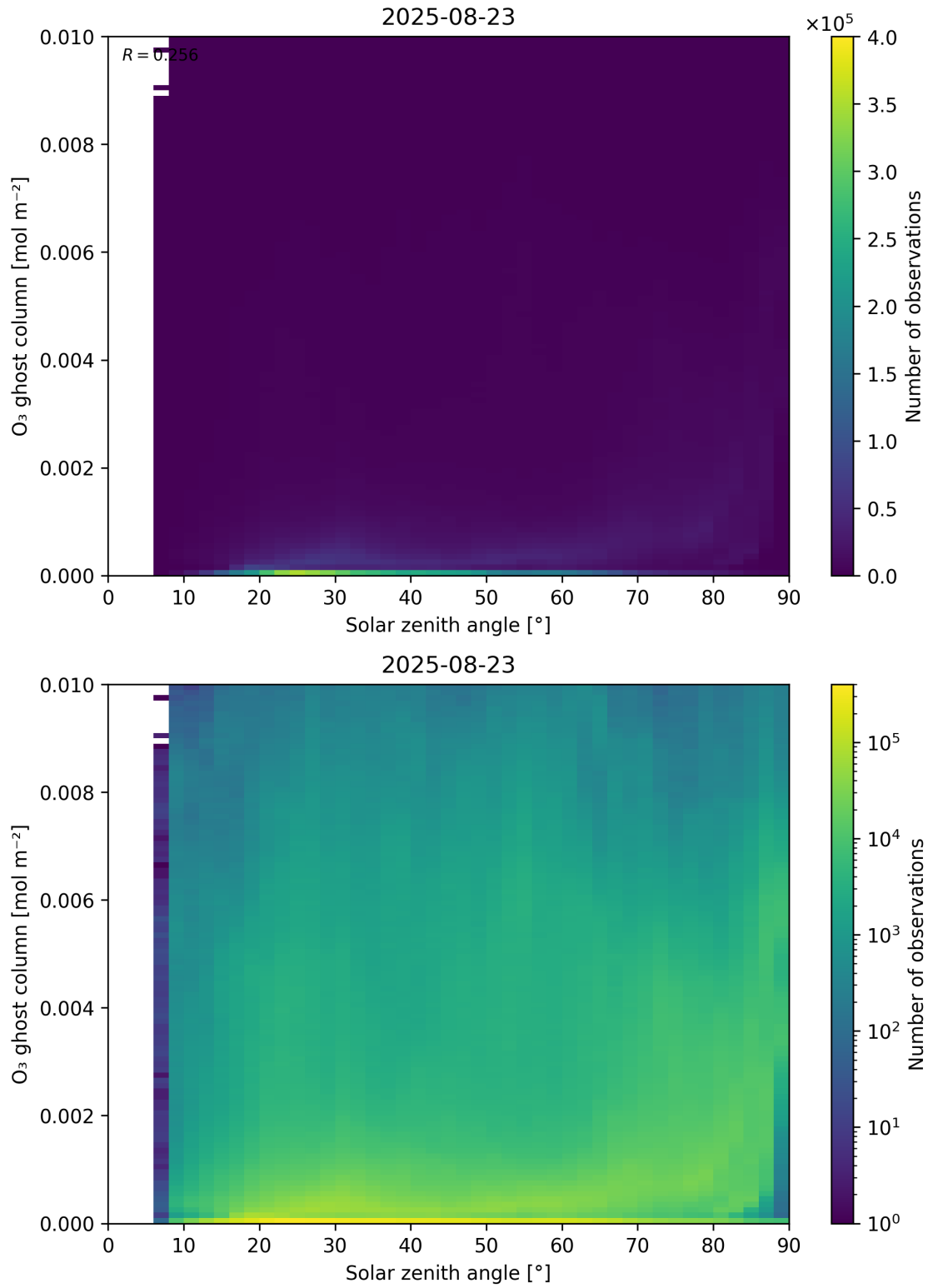
Figure 46: Scatter density plot of “Solar zenith angle” against “O 3 ghost column” for 2025-08-22 to 2025-08-24.
