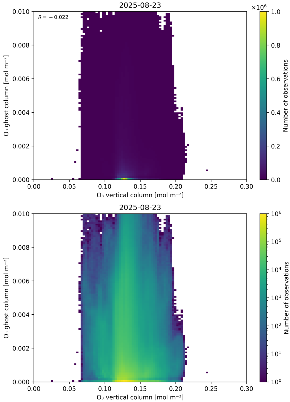
Figure 40: Scatter density plot of “O 3 vertical column” against “O 3 ghost column” for 2025-08-22 to 2025-08-24.
