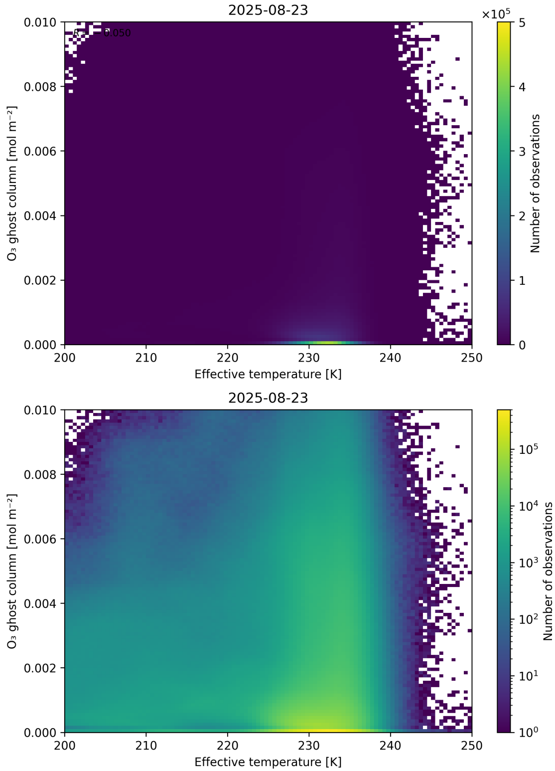
Figure 38: Scatter density plot of “Effective temperature” against “O 3 ghost column” for 2025-08-22 to 2025-08-24.
