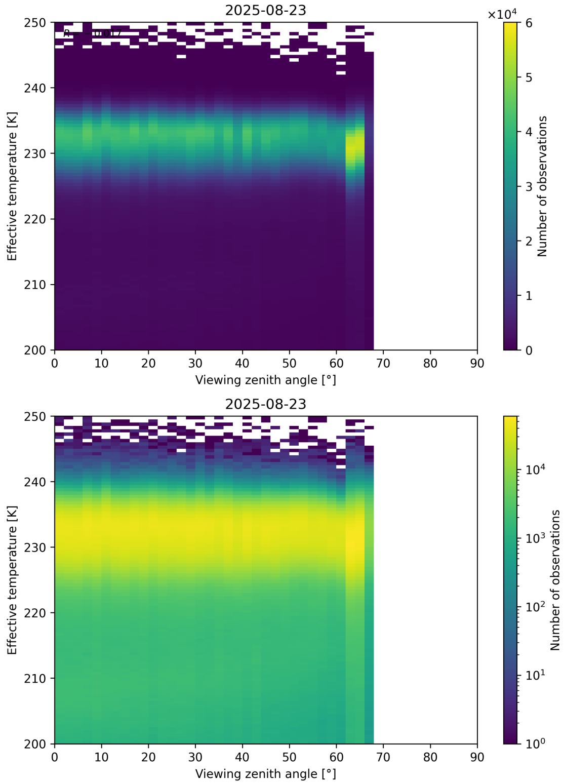
Figure 50: Scatter density plot of “Viewing zenith angle” against “Effective temperature” for 2025-08-22 to 2025-08-24.
