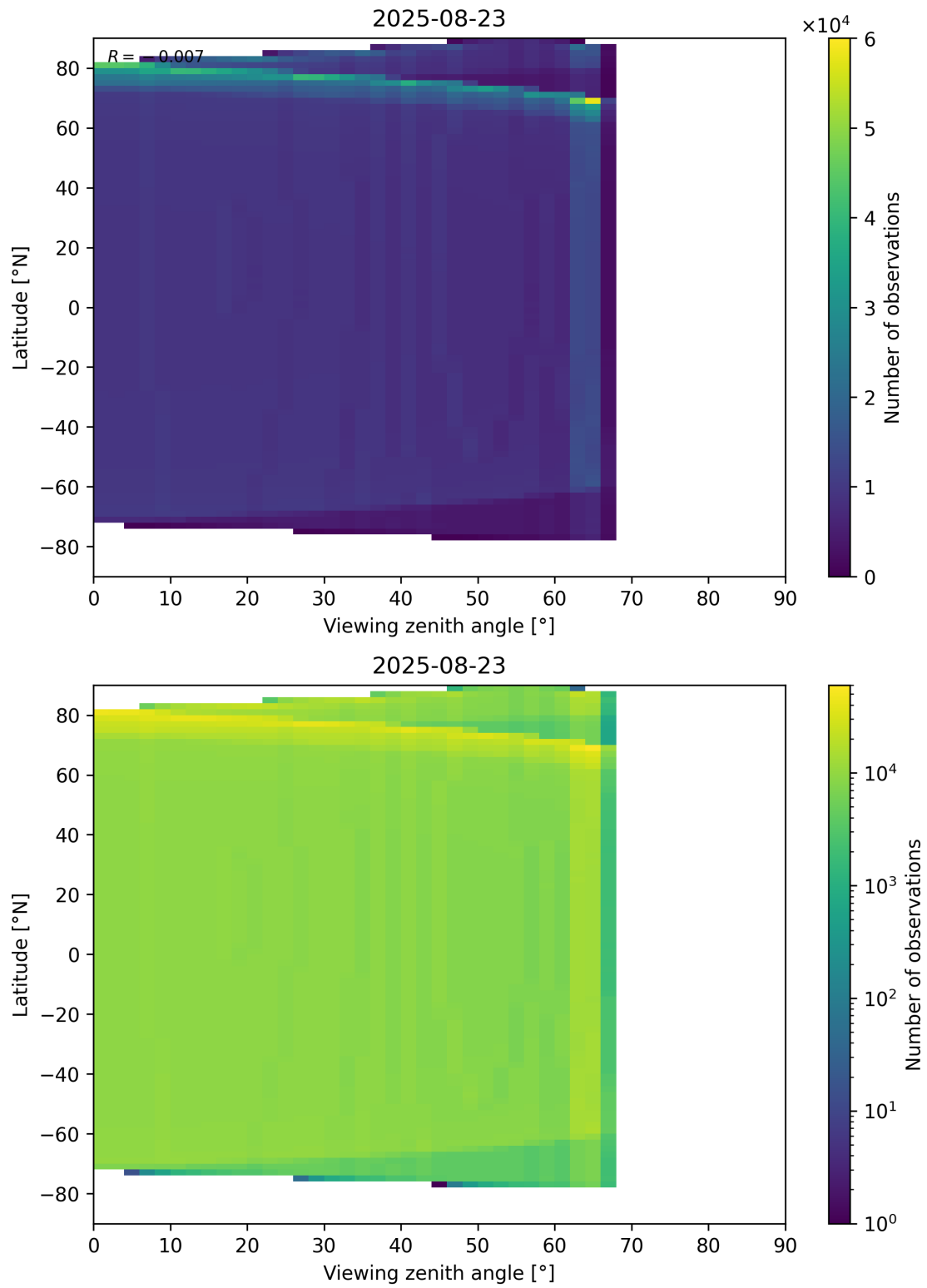
Figure 49: Scatter density plot of “Viewing zenith angle” against “Latitude” for 2025-08-22 to 2025-08-24.
