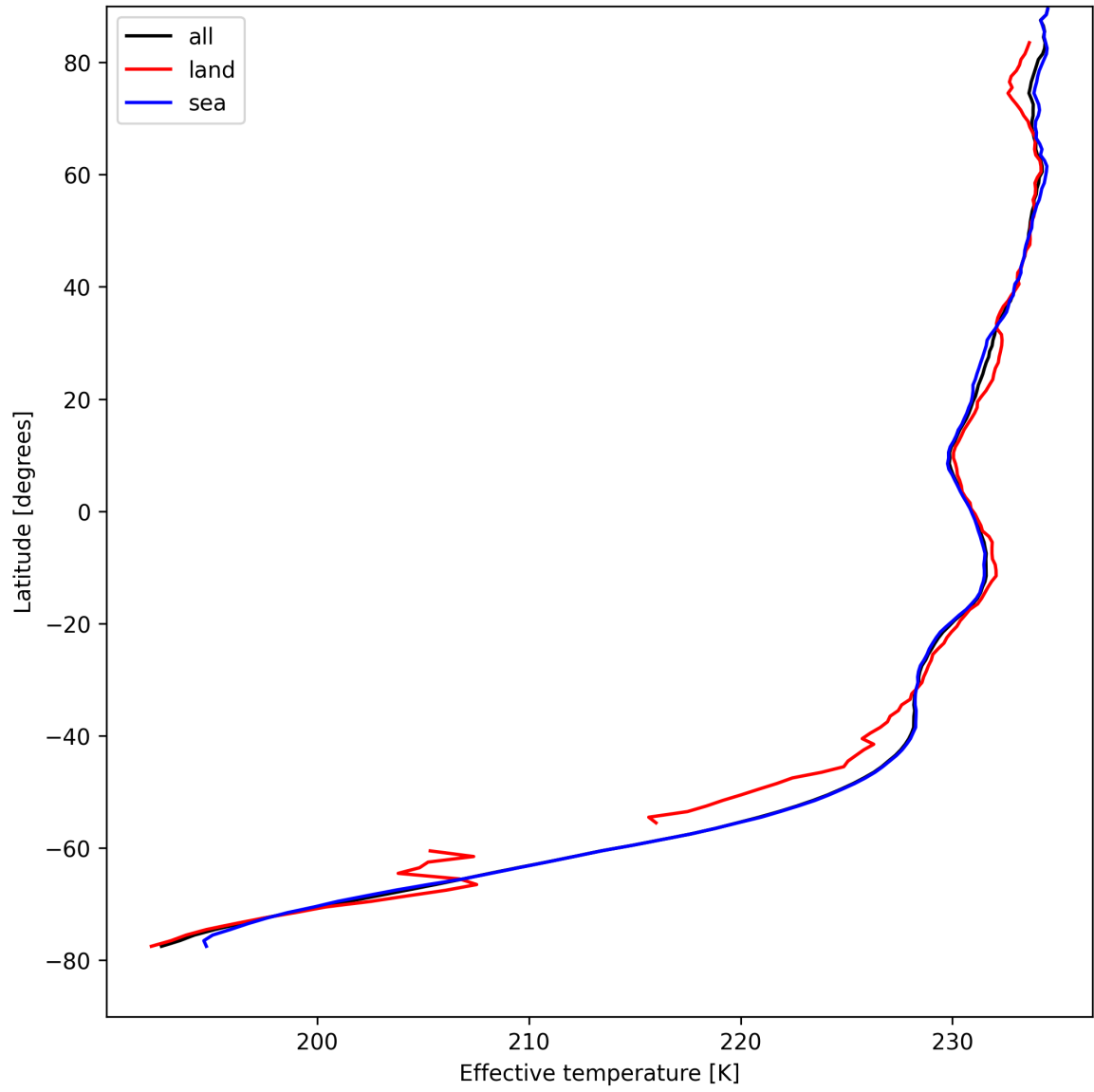
Figure 17: Zonal average of "Effective temperature" for 2025-08-22 to 2025-08-24.
