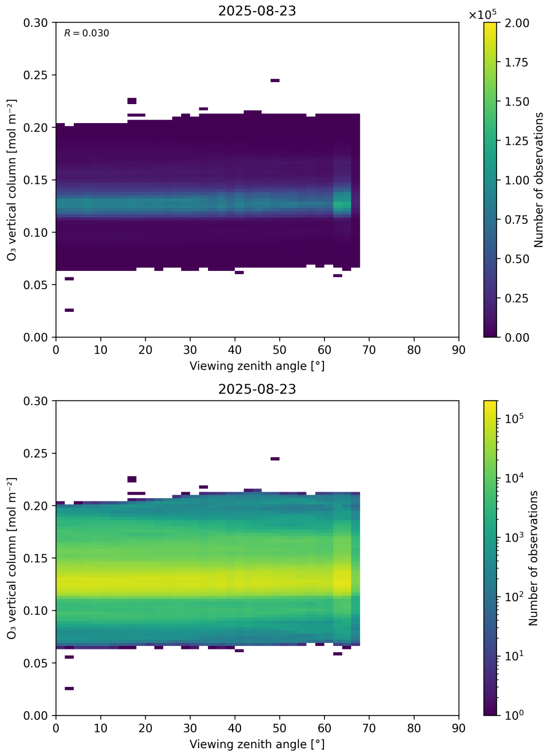
Figure 52: Scatter density plot of “Viewing zenith angle” against “O 3 vertical column” for 2025-08-22 to 2025-08-24.
