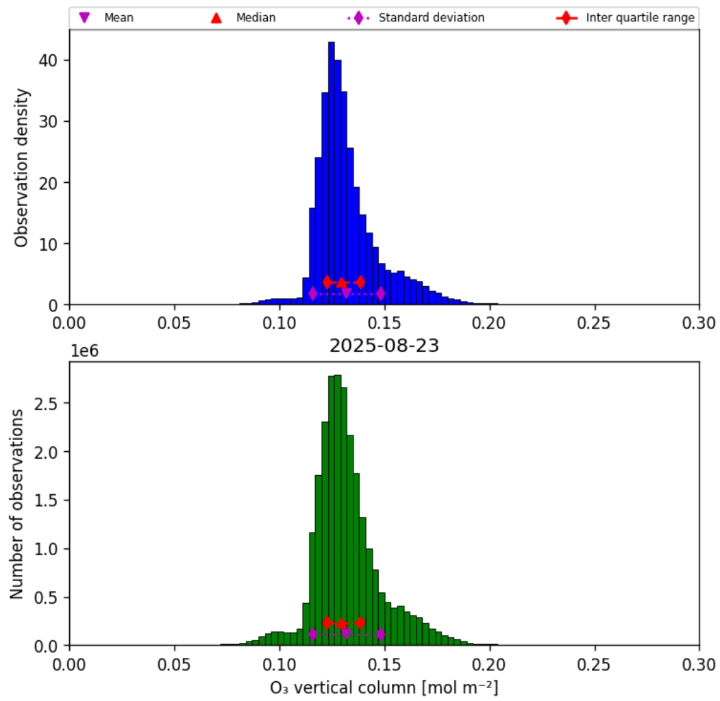
Figure 21: Histogram of “O 3 vertical column” for 2025-08-22 to 2025-08-24
