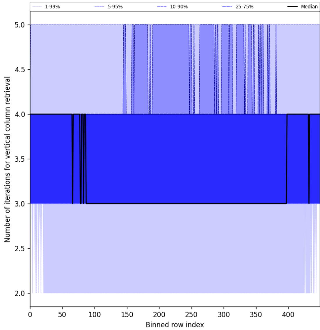
Figure 33: Along track statistics of “Number of iterations for vertical column retrieval” for 2025-08-22 to 2025-08-24
