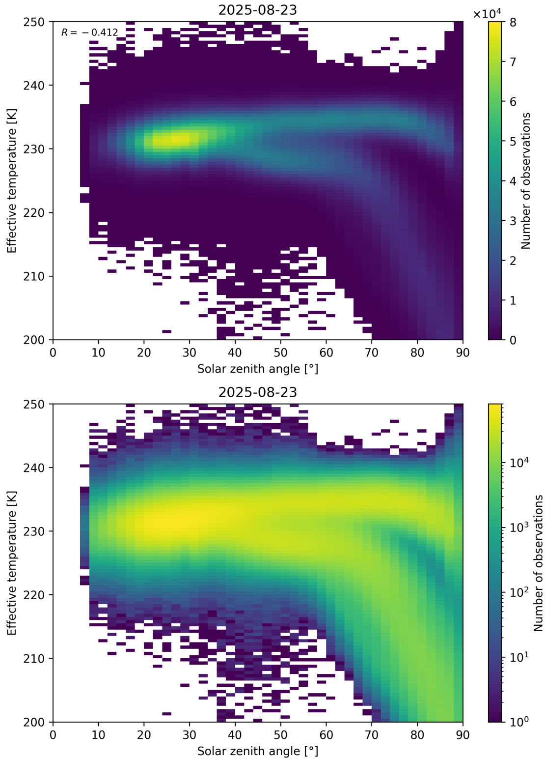
Figure 45: Scatter density plot of “Solar zenith angle” against “Effective temperature” for 2025-08-22 to 2025-08-24.
