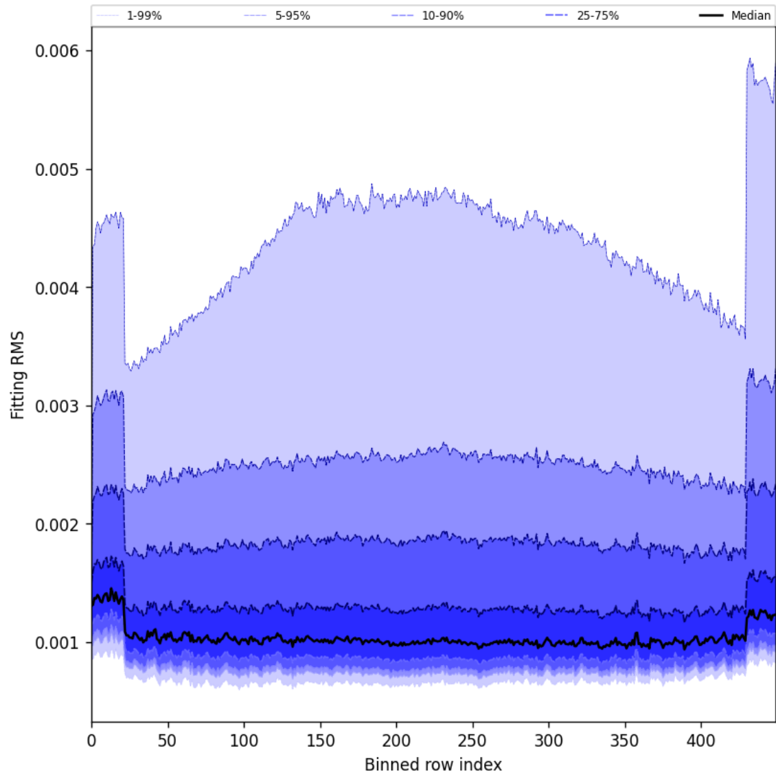
Figure 30: Along track statistics of “Fitting RMS” for 2025-08-22 to 2025-08-24
