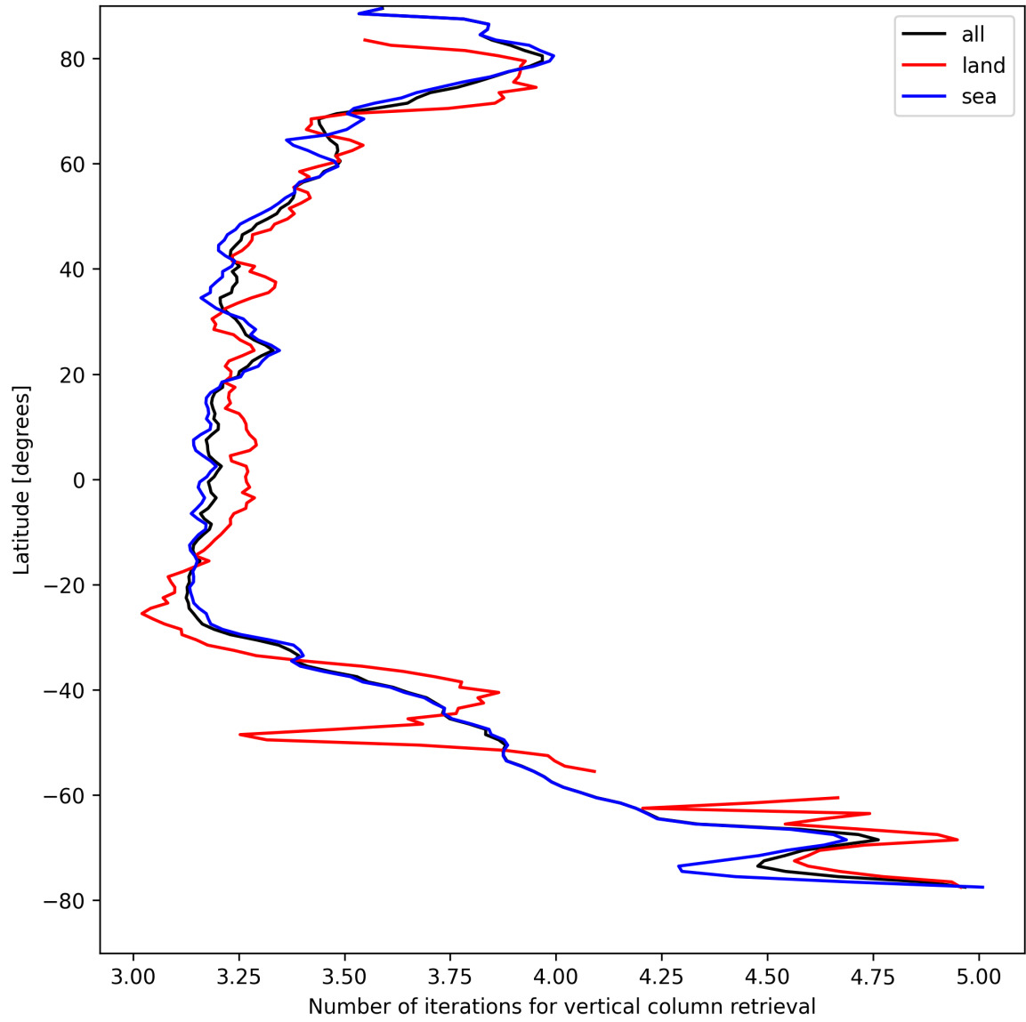
Figure 19: Zonal average of “Number of iterations for vertical column retrieval” for 2025-08-22 to 2025-08-24.
