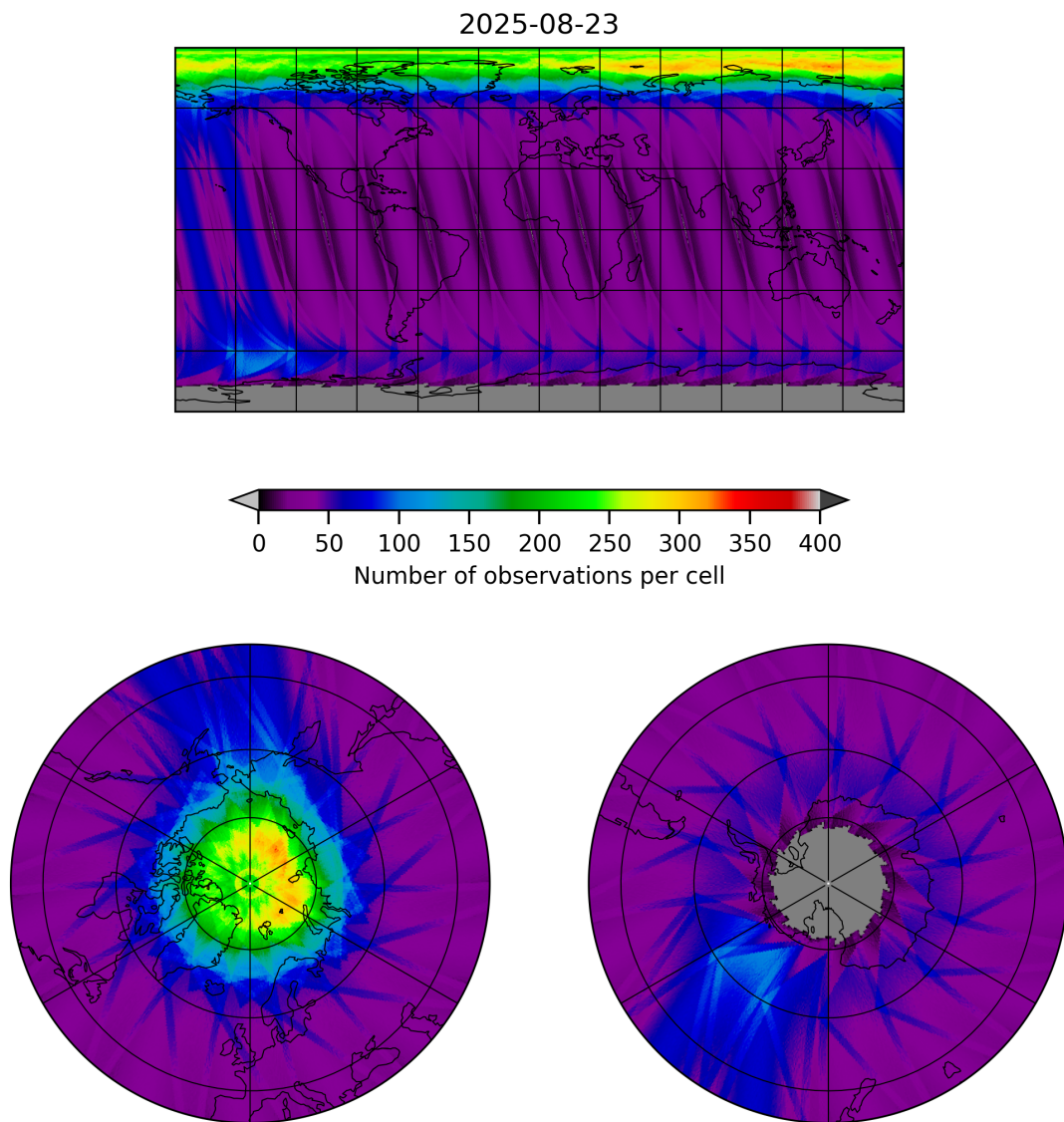
Figure 12: Map of the number of observations for 2025-08-22 to 2025-08-24
