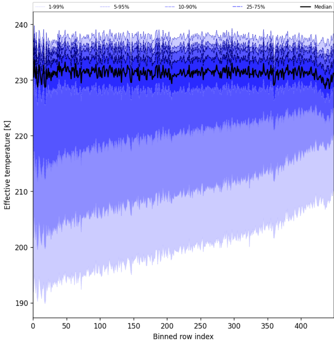
Figure 31: Along track statistics of “Effective temperature” for 2025-08-22 to 2025-08-24
