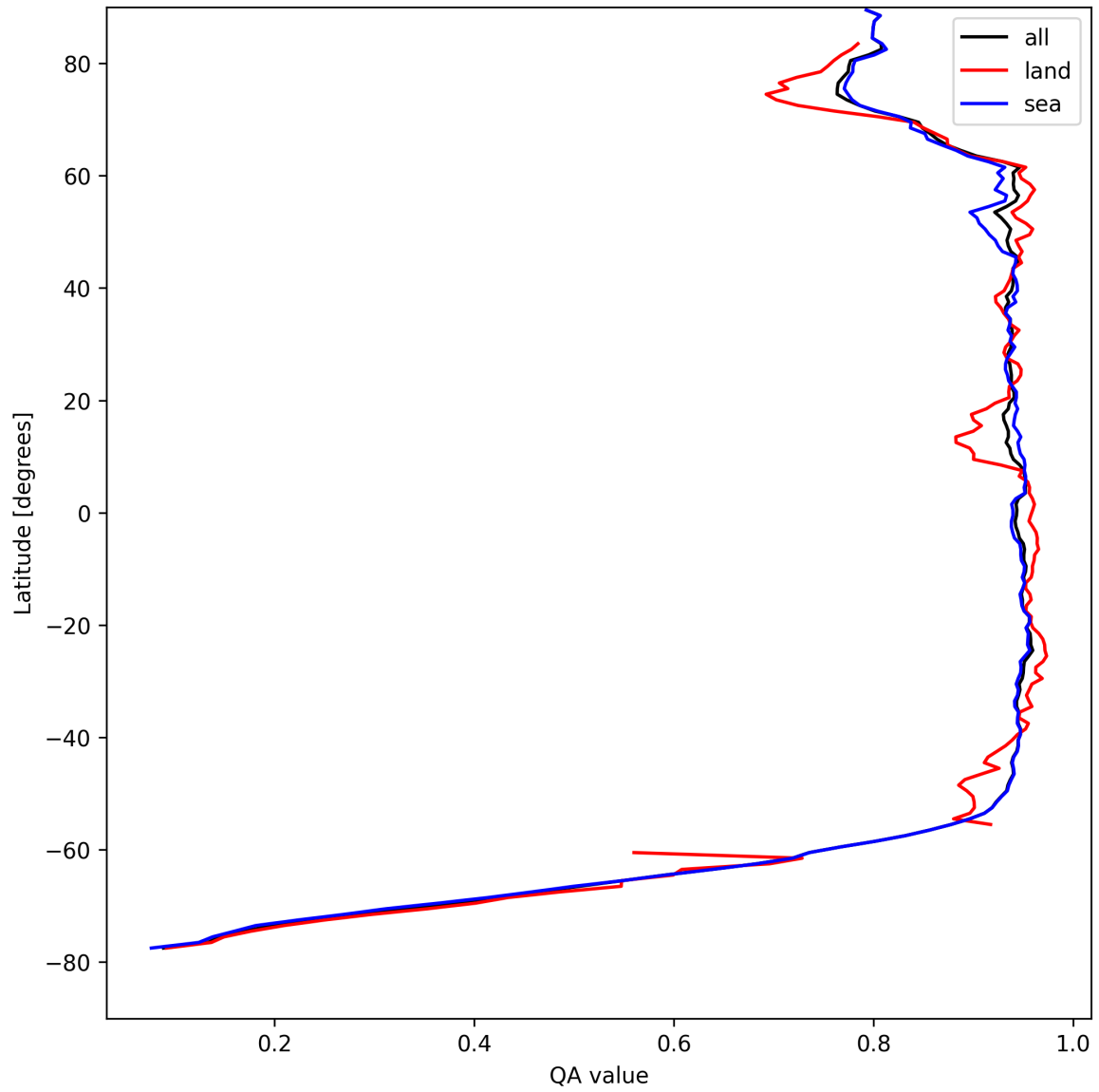
Figure 13: Zonal average of “QA value” for 2025-08-22 to 2025-08-24.
