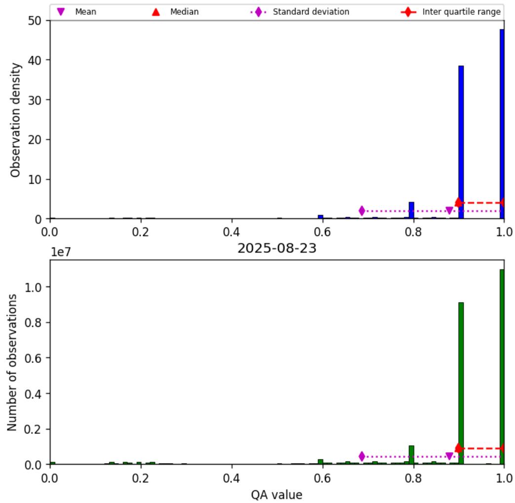
Figure 20: Histogram of “QA value” for 2025-08-22 to 2025-08-24
