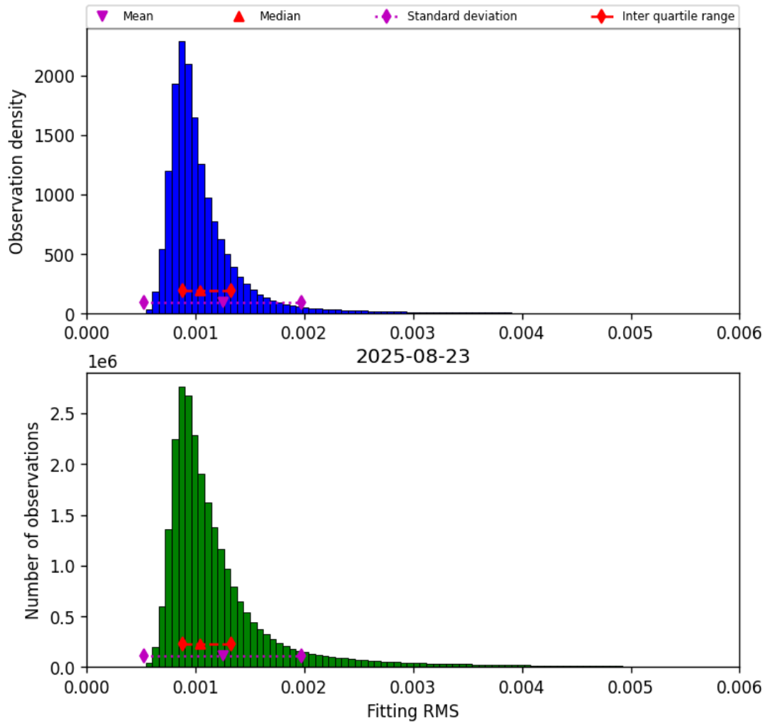
Figure 23: Histogram of “Fitting RMS” for 2025-08-22 to 2025-08-24
