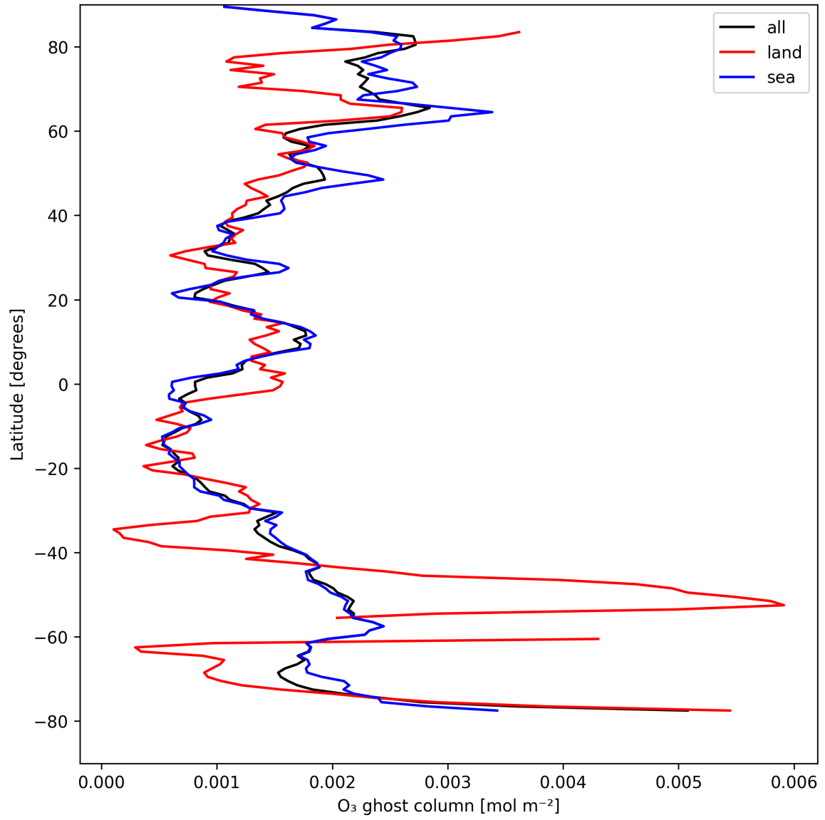
Figure 18: Zonal average of “O 3 ghost column” for 2025-08-22 to 2025-08-24.
