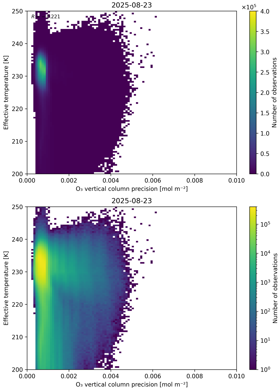
Figure 42: Scatter density plot of “O 3 vertical column precision” against “Effective temperature” for 2025-08-22 to 2025-08-24.
