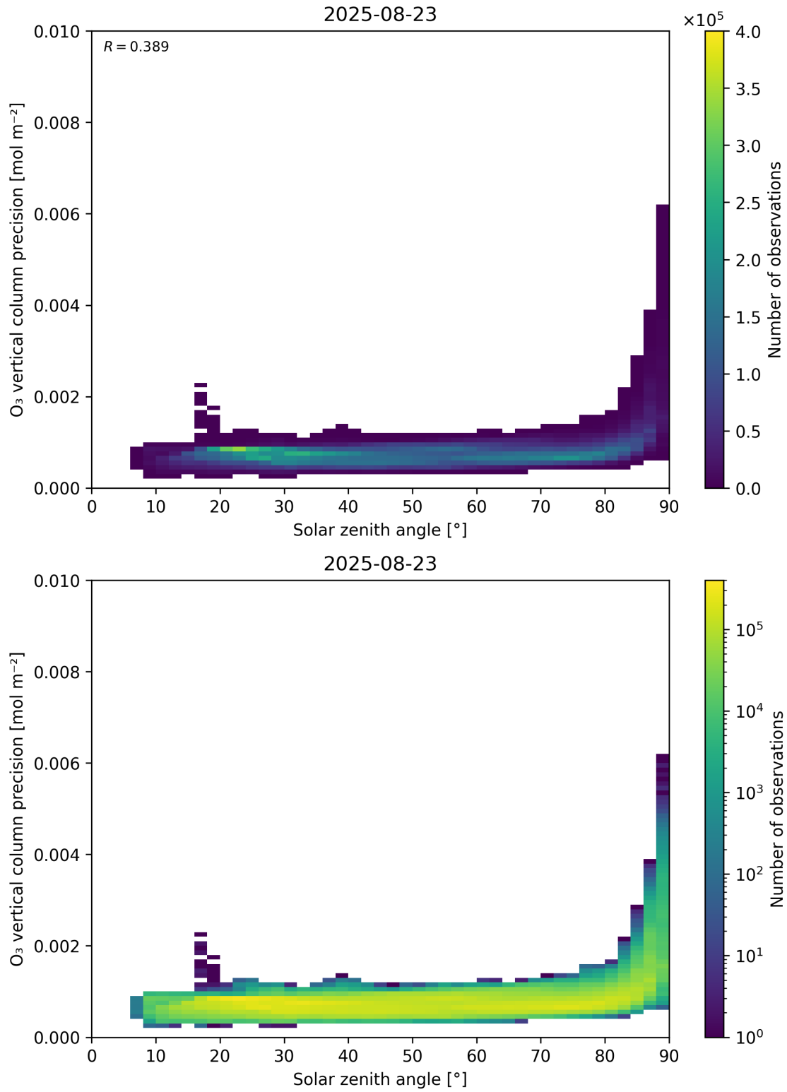
Figure 48: Scatter density plot of “Solar zenith angle” against “O 3 vertical column precision” for 2025-08-22 to 2025-08-24.
