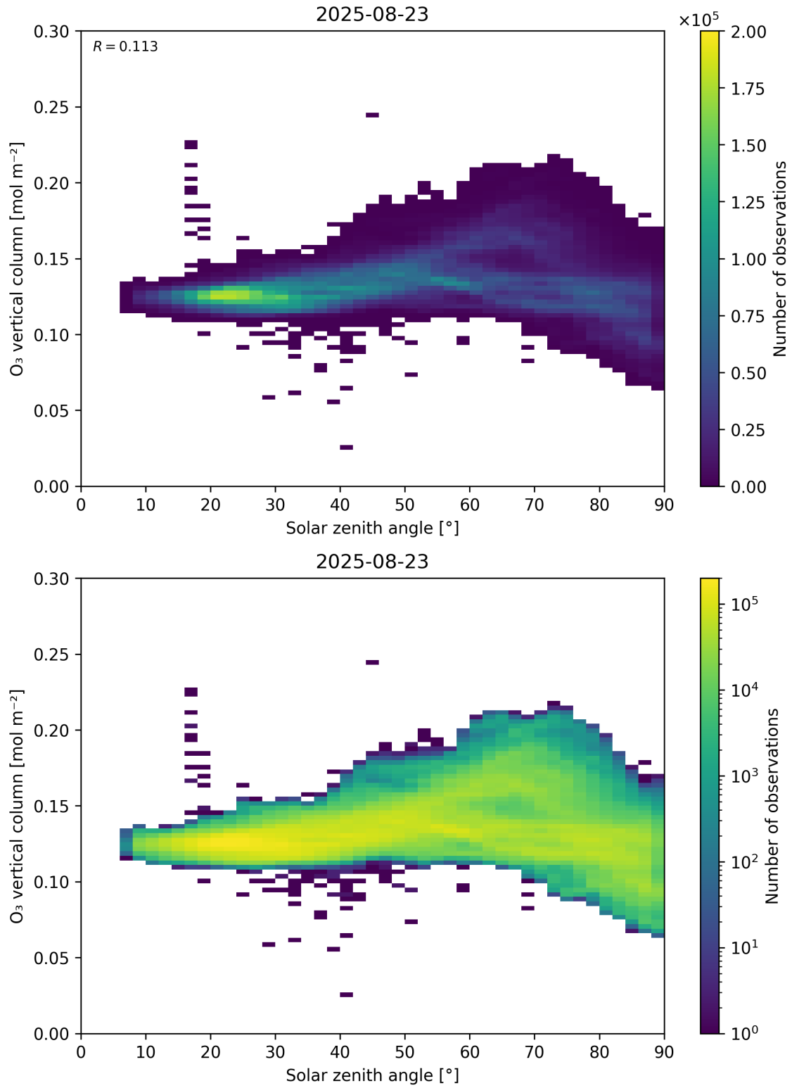
Figure 47: Scatter density plot of “Solar zenith angle” against “O 3 vertical column” for 2025-08-22 to 2025-08-24.
