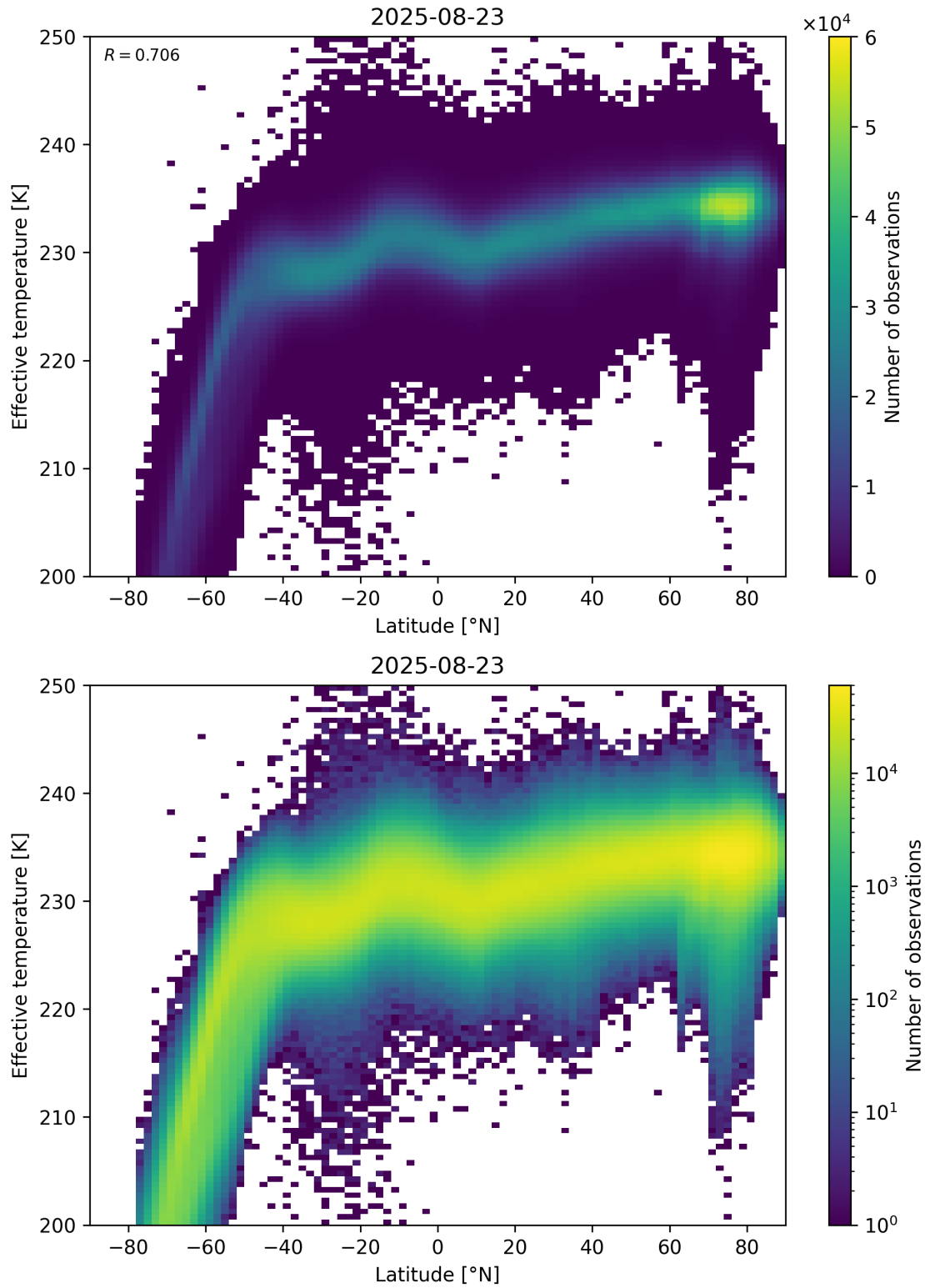
Figure 34: Scatter density plot of “Latitude” against “Effective temperature” for 2025-08-22 to 2025-08-24.
