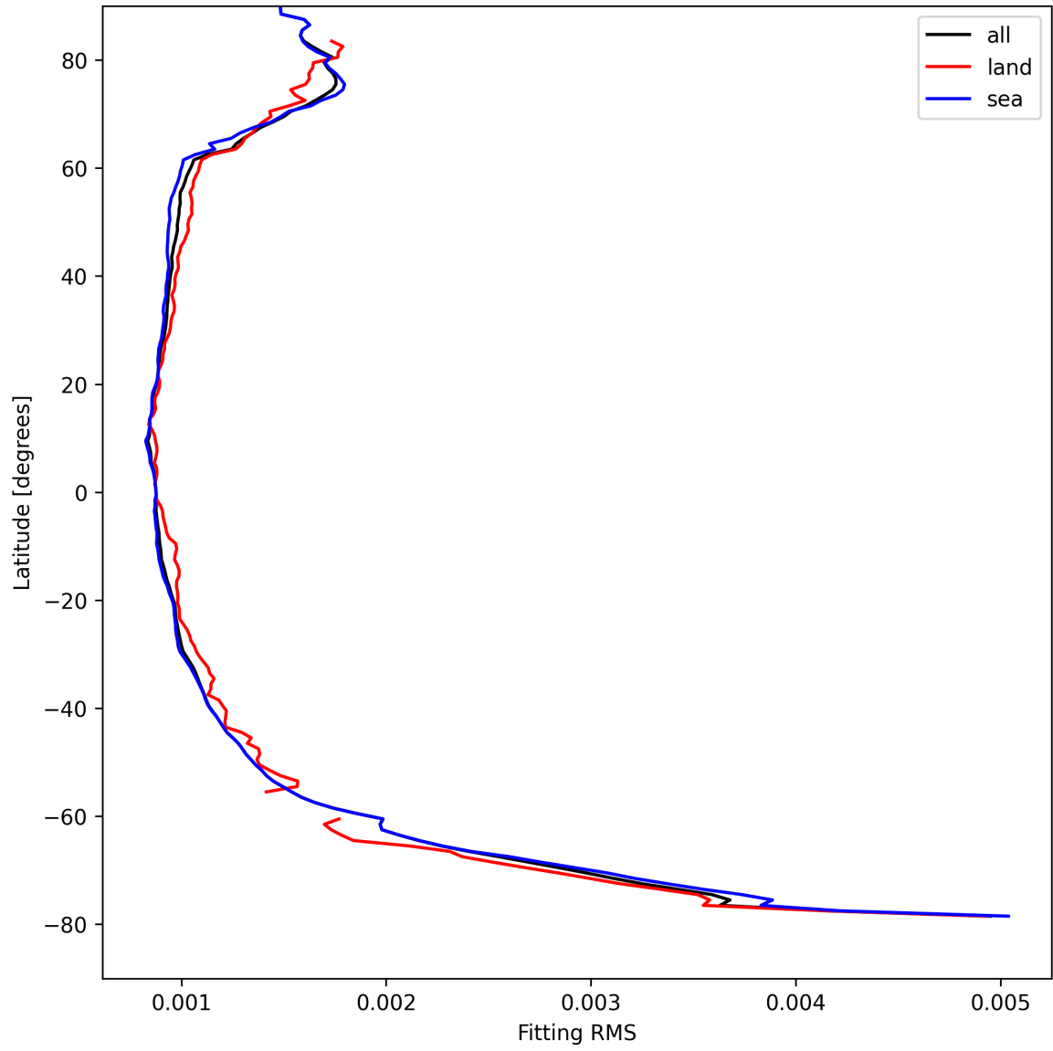
Figure 16: Zonal average of “Fitting RMS” for 2025-08-23 to 2025-08-25.
