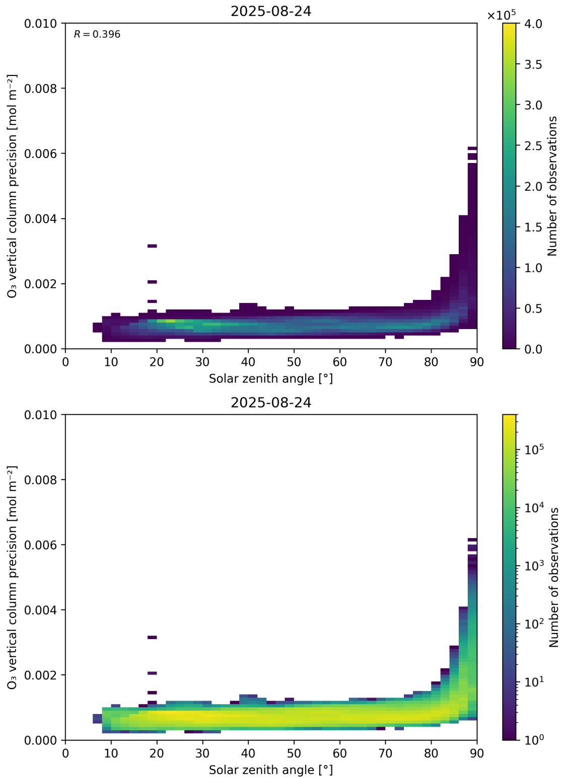
Figure 48: Scatter density plot of “Solar zenith angle” against “O 3 vertical column precision” for 2025-08-23 to 2025-08-25.
