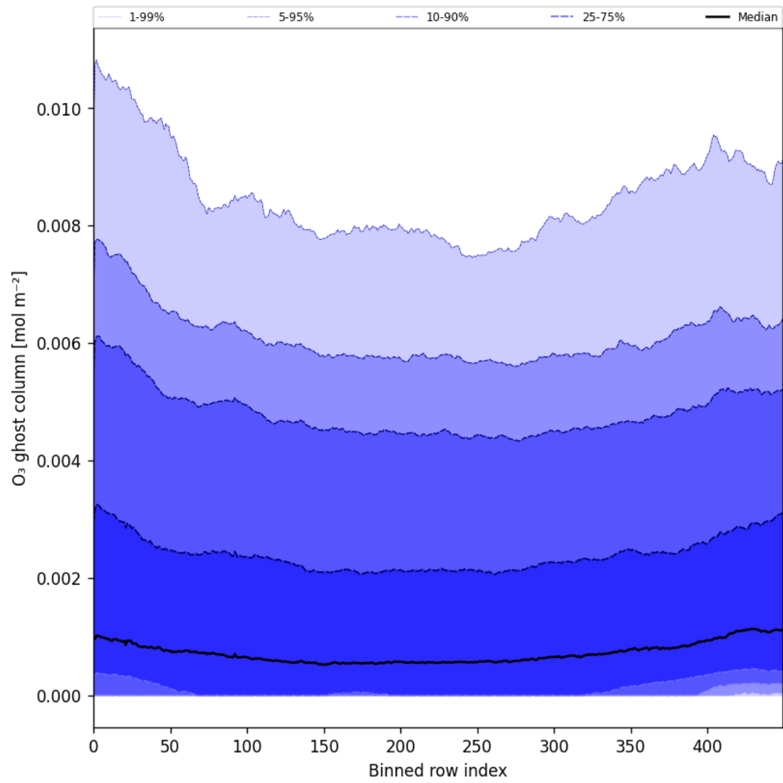
Figure 32: Along track statistics of “O 3 ghost column” for 2025-08-23 to 2025-08-25
