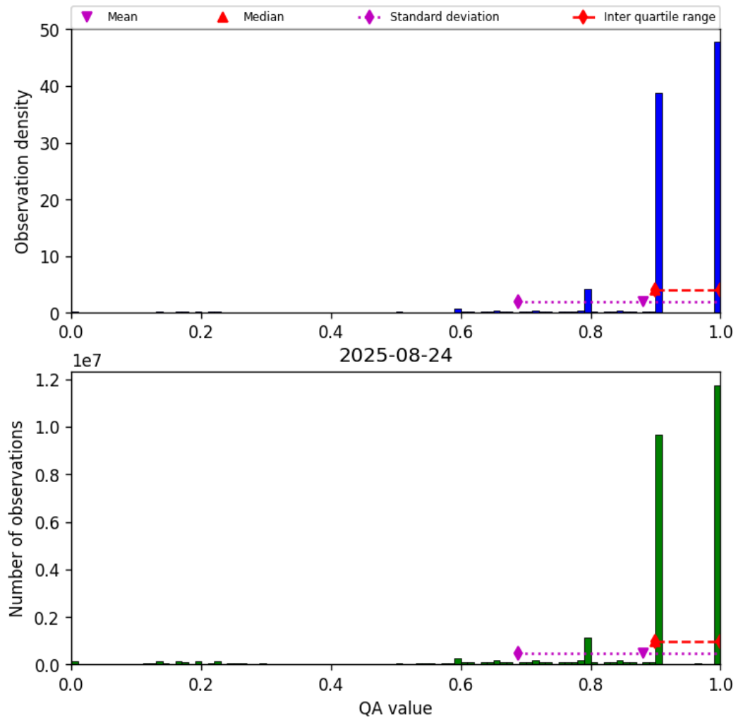
Figure 20: Histogram of “QA value” for 2025-08-23 to 2025-08-25
