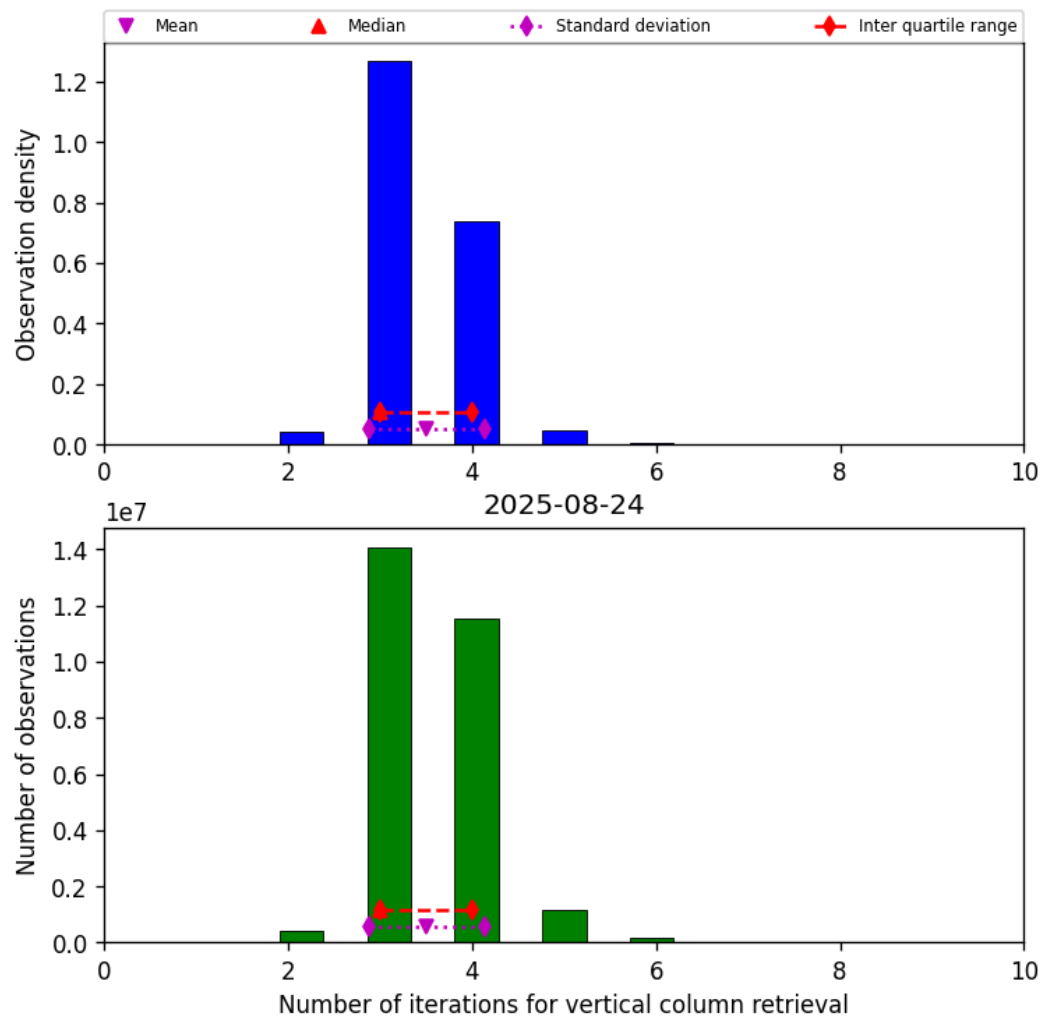
Figure 26: Histogram of “Number of iterations for vertical column retrieval” for 2025-08-23 to 2025-08-25
