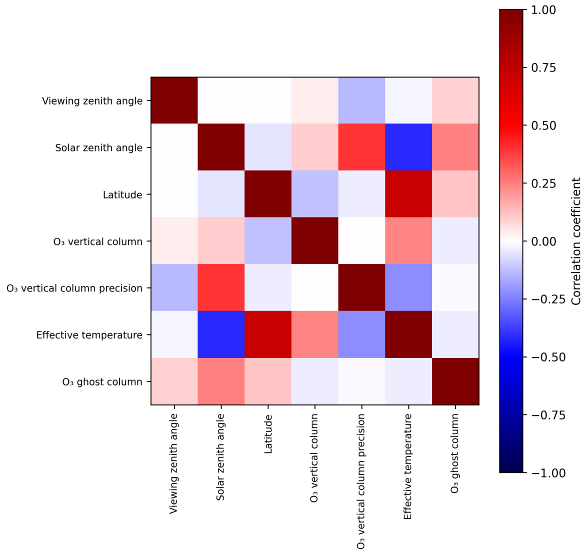
Figure 2: Map of correlation matrix for 2025-08-23 to 2025-08-25.
