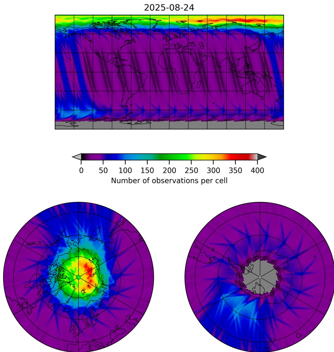
Figure 12: Map of the number of observations for 2025-08-23 to 2025-08-25
