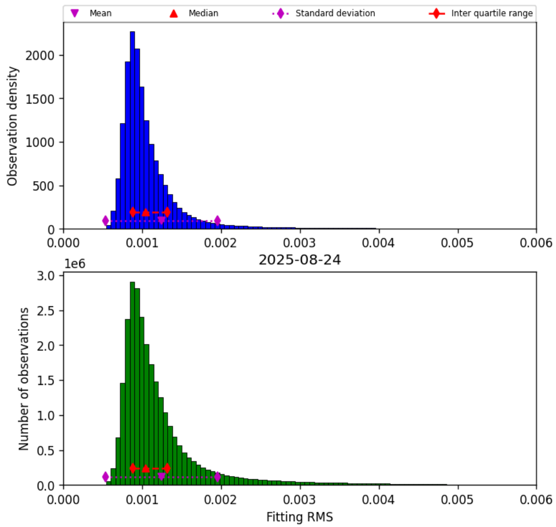
Figure 23: Histogram of “Fitting RMS” for 2025-08-23 to 2025-08-25
