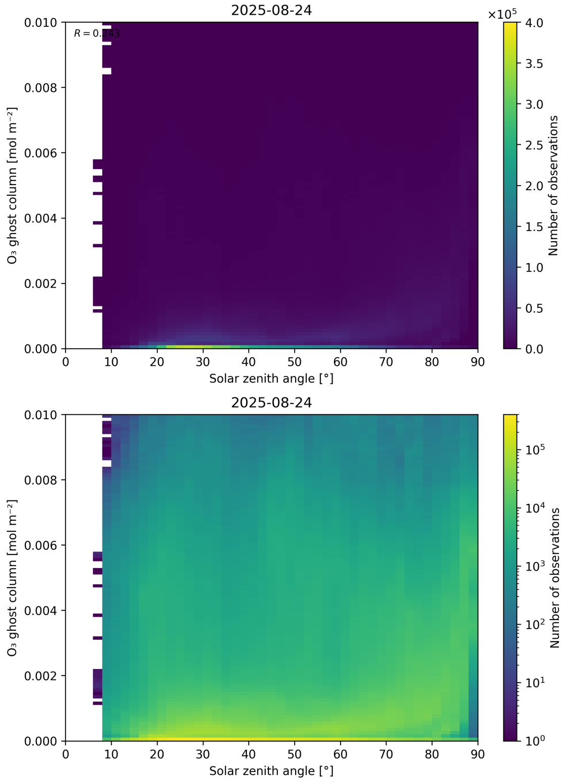
Figure 46: Scatter density plot of “Solar zenith angle” against “O 3 ghost column” for 2025-08-23 to 2025-08-25.
