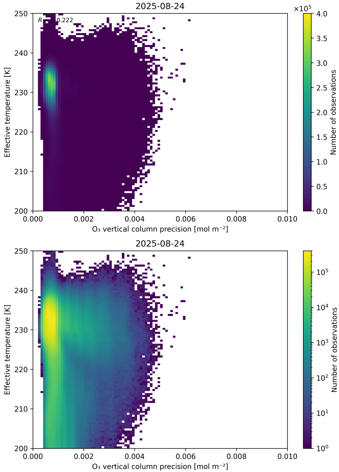
Figure 42: Scatter density plot of “ O_3 vertical column precision” against “Effective temperature” for 2025-08-23 to 2025-08-25.
