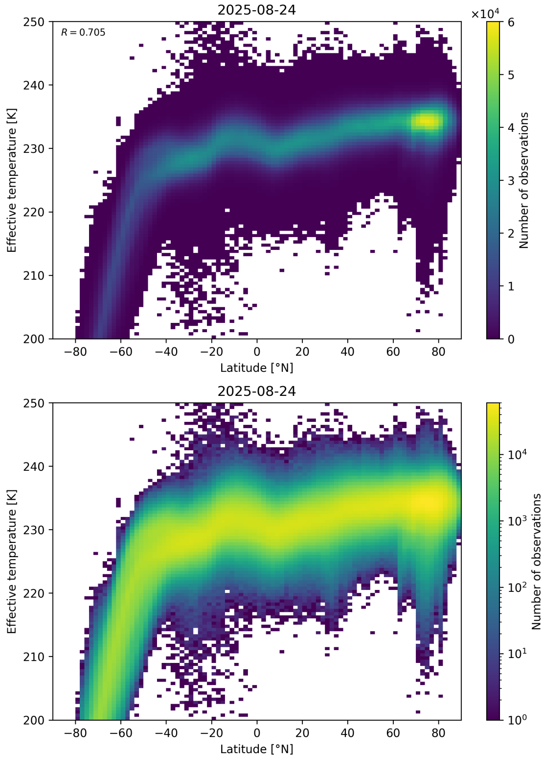
Figure 34: Scatter density plot of “Latitude” against “Effective temperature” for 2025-08-23 to 2025-08-25.
