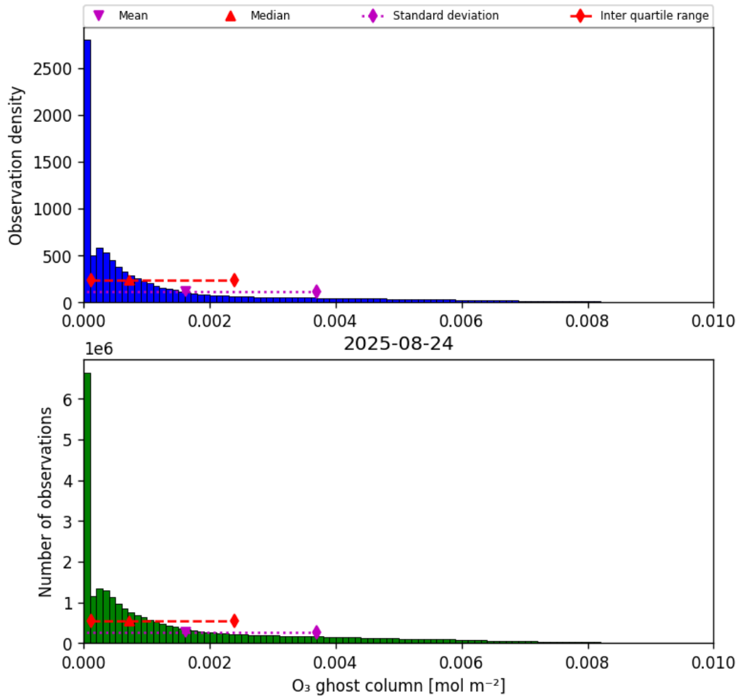
Figure 25: Histogram of “O 3 ghost column” for 2025-08-23 to 2025-08-25
