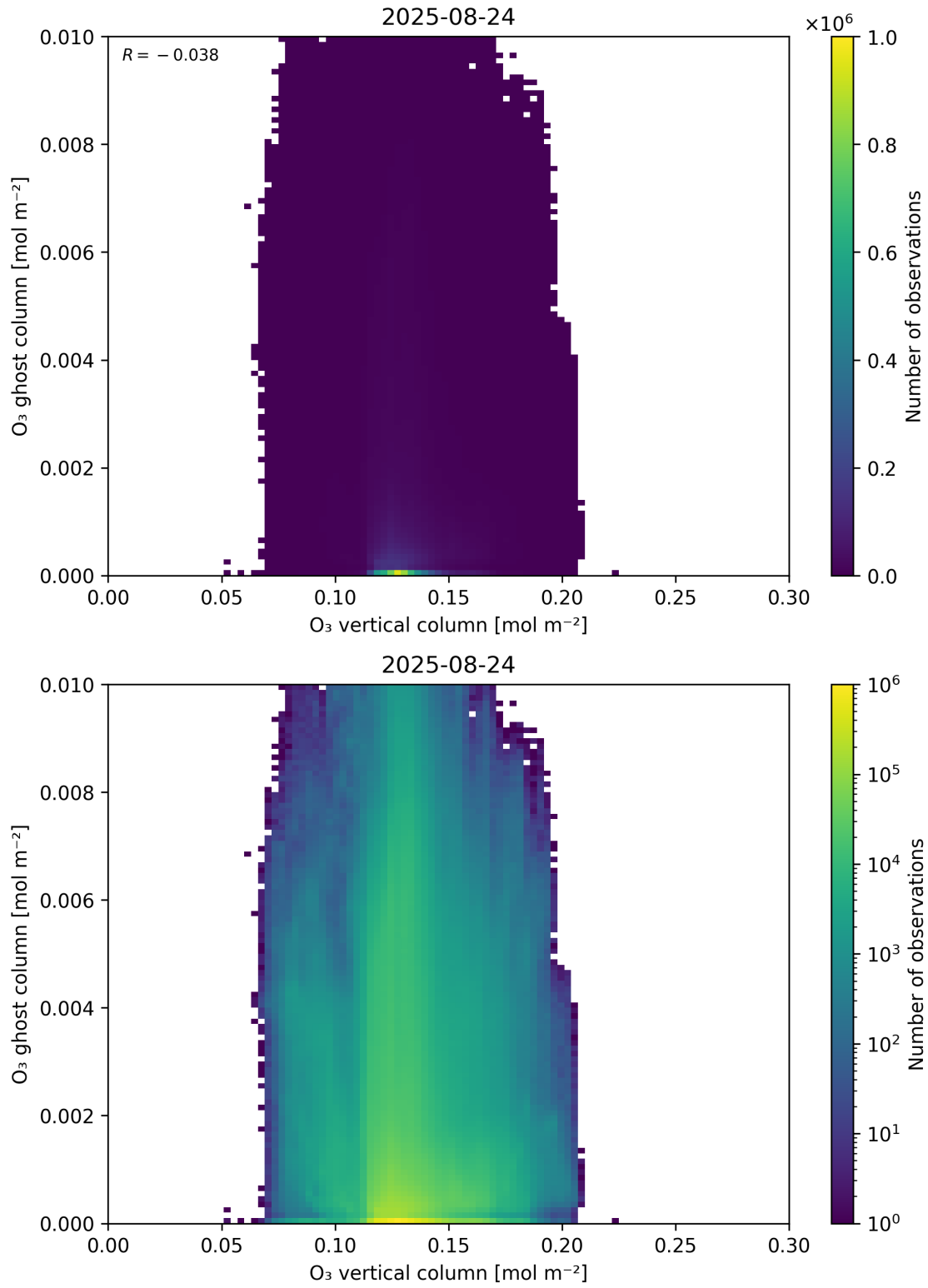
Figure 40: Scatter density plot of “O 3 vertical column” against “O 3 ghost column” for 2025-08-23 to 2025-08-25.
