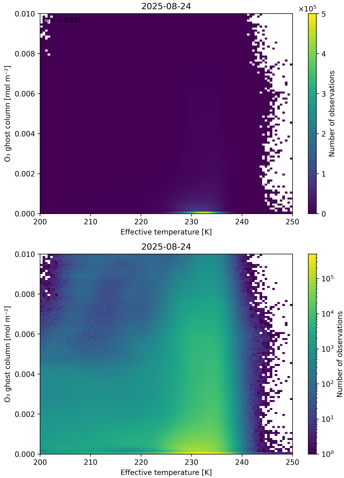
Figure 38: Scatter density plot of “Effective temperature” against “O 3 ghost column” for 2025-08-23 to 2025-08-25.
