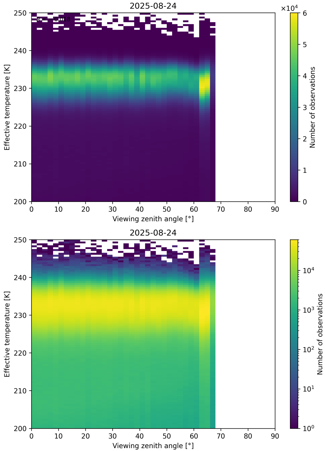
Figure 50: Scatter density plot of “Viewing zenith angle” against “Effective temperature” for 2025-08-23 to 2025-08-25.
