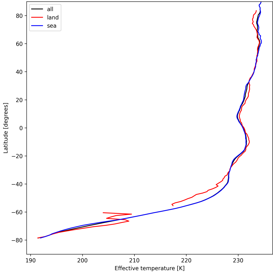
Figure 17: Zonal average of "Effective temperature" for 2025-08-23 to 2025-08-25.
