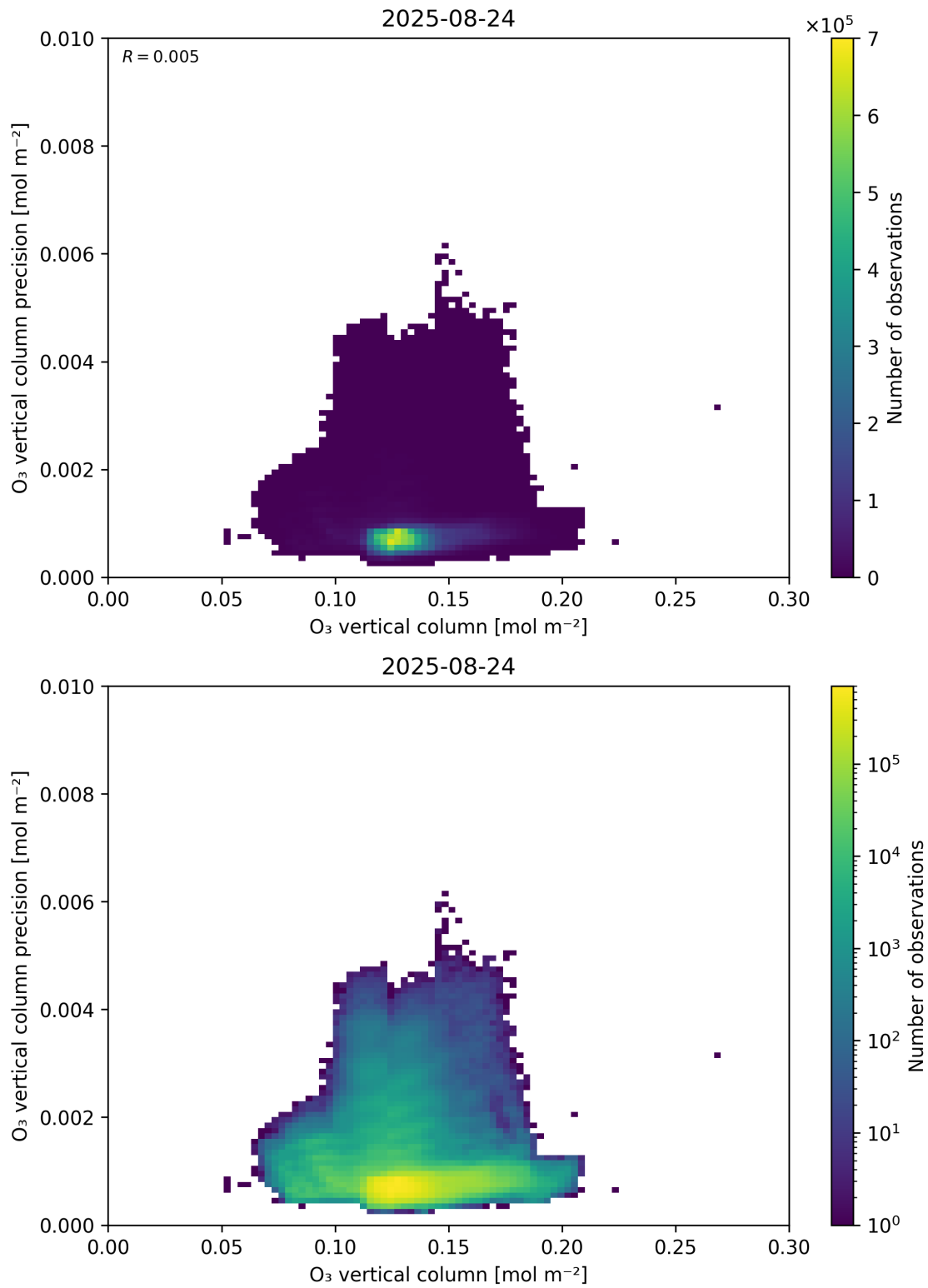
Figure 41: Scatter density plot of “O 3 vertical column” against “O 3 vertical column precision” for 2025-08-23 to 2025-08-25.
