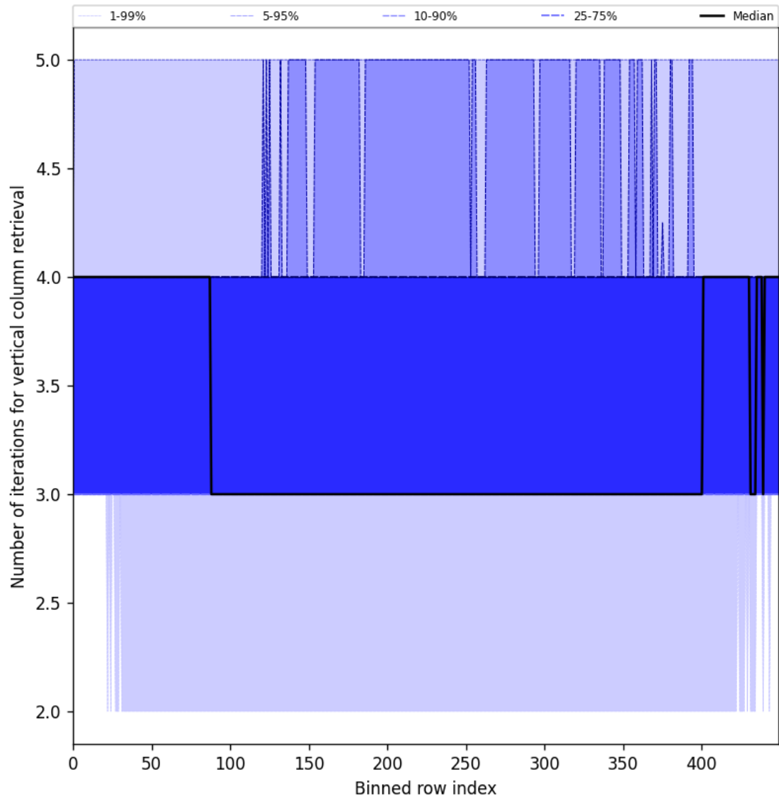
Figure 33: Along track statistics of “Number of iterations for vertical column retrieval” for 2025-08-23 to 2025-08-25
