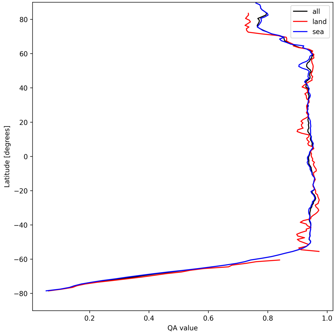
Figure 13: Zonal average of “QA value” for 2025-08-23 to 2025-08-25.
