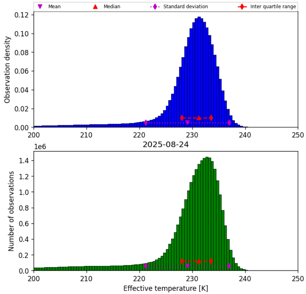
Figure 24: Histogram of “Effective temperature” for 2025-08-23 to 2025-08-25
