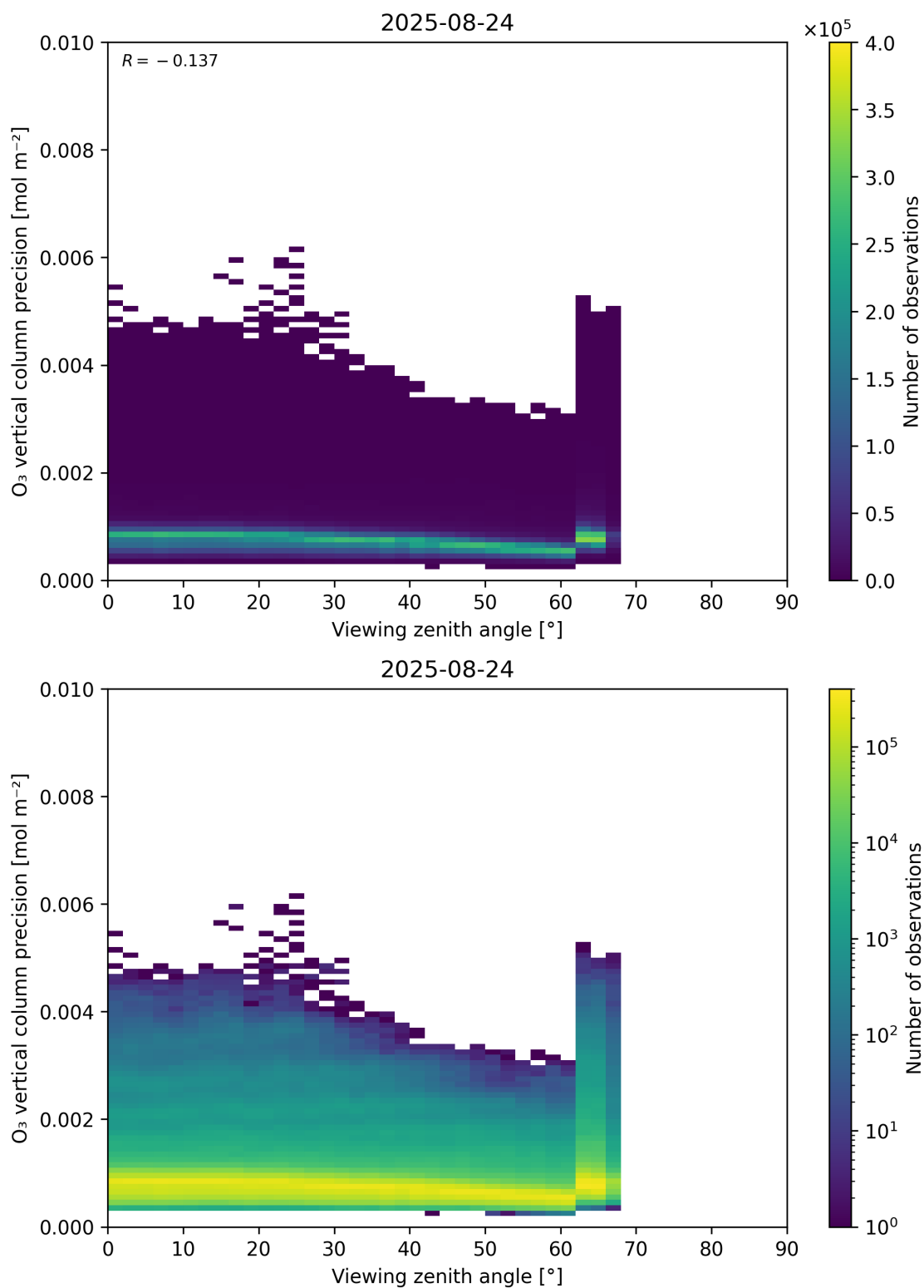
Figure 53: Scatter density plot of “Viewing zenith angle” against “O 3 vertical column precision” for 2025-08-23 to 2025-08-25.
