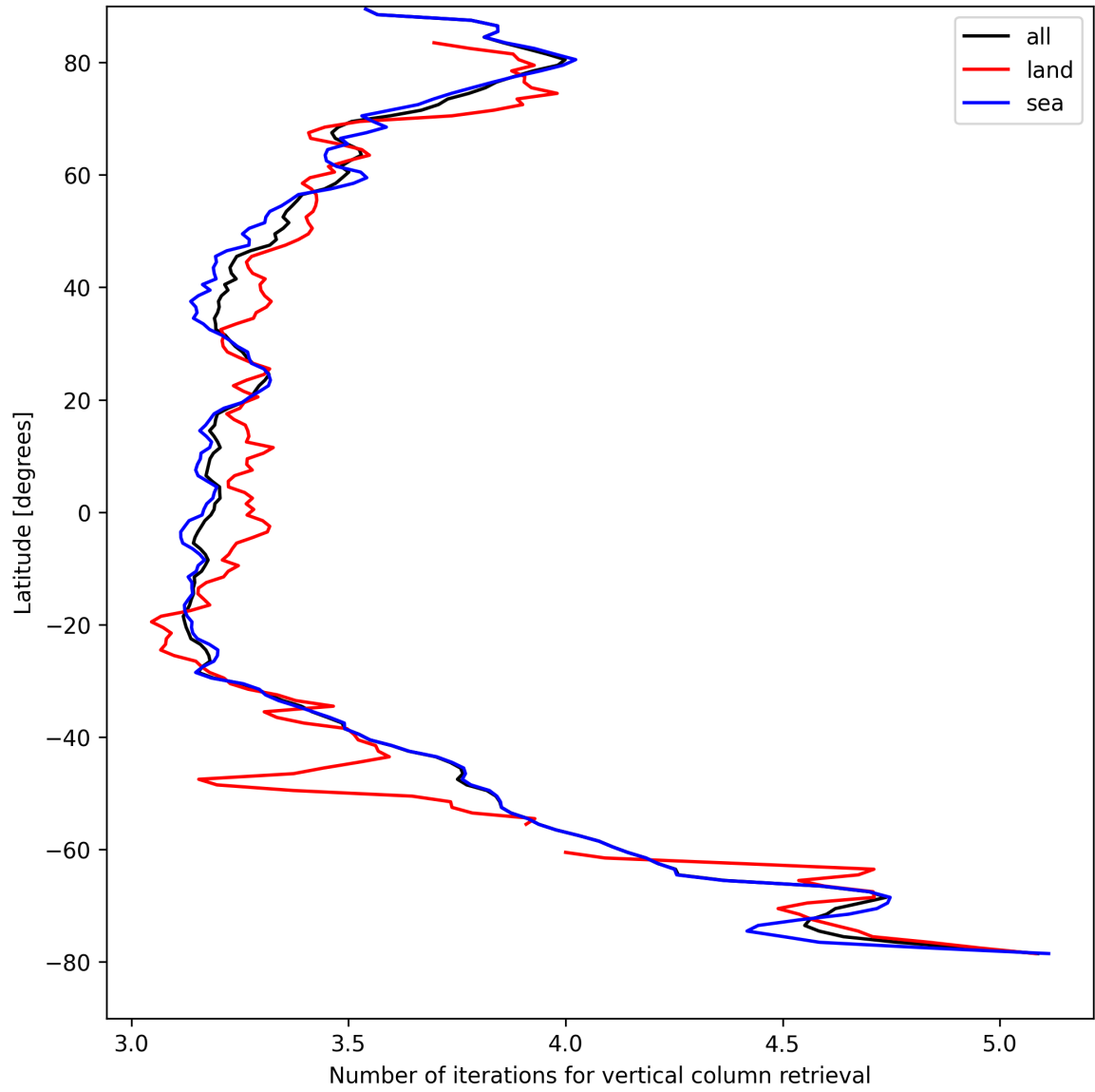
Figure 19: Zonal average of “Number of iterations for vertical column retrieval” for 2025-08-23 to 2025-08-25.
