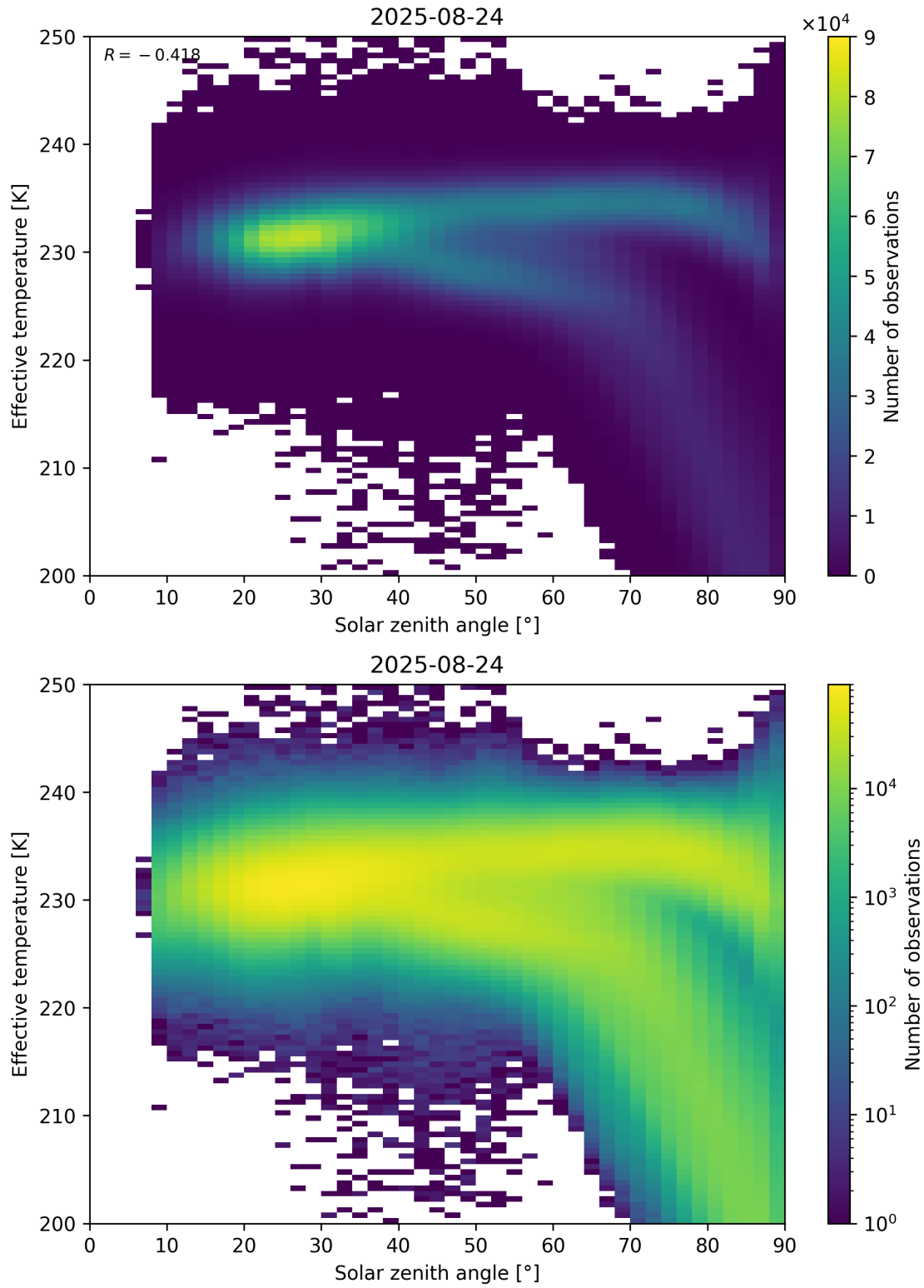
Figure 45: Scatter density plot of “Solar zenith angle” against “Effective temperature” for 2025-08-23 to 2025-08-25.
