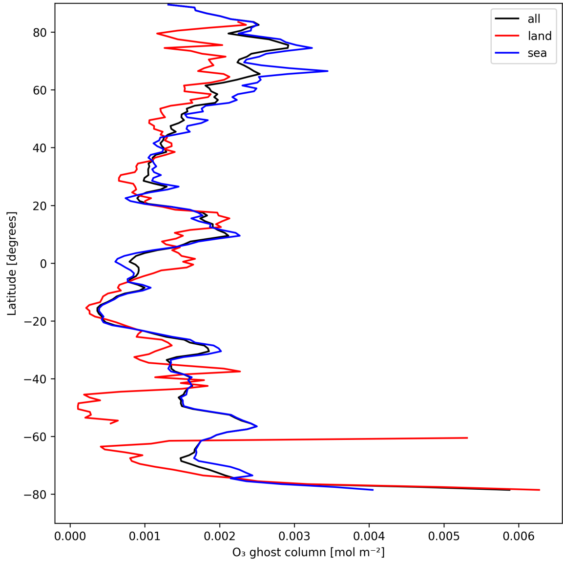
Figure 18: Zonal average of "O 3 ghost column" for 2025-08-23 to 2025-08-25.
