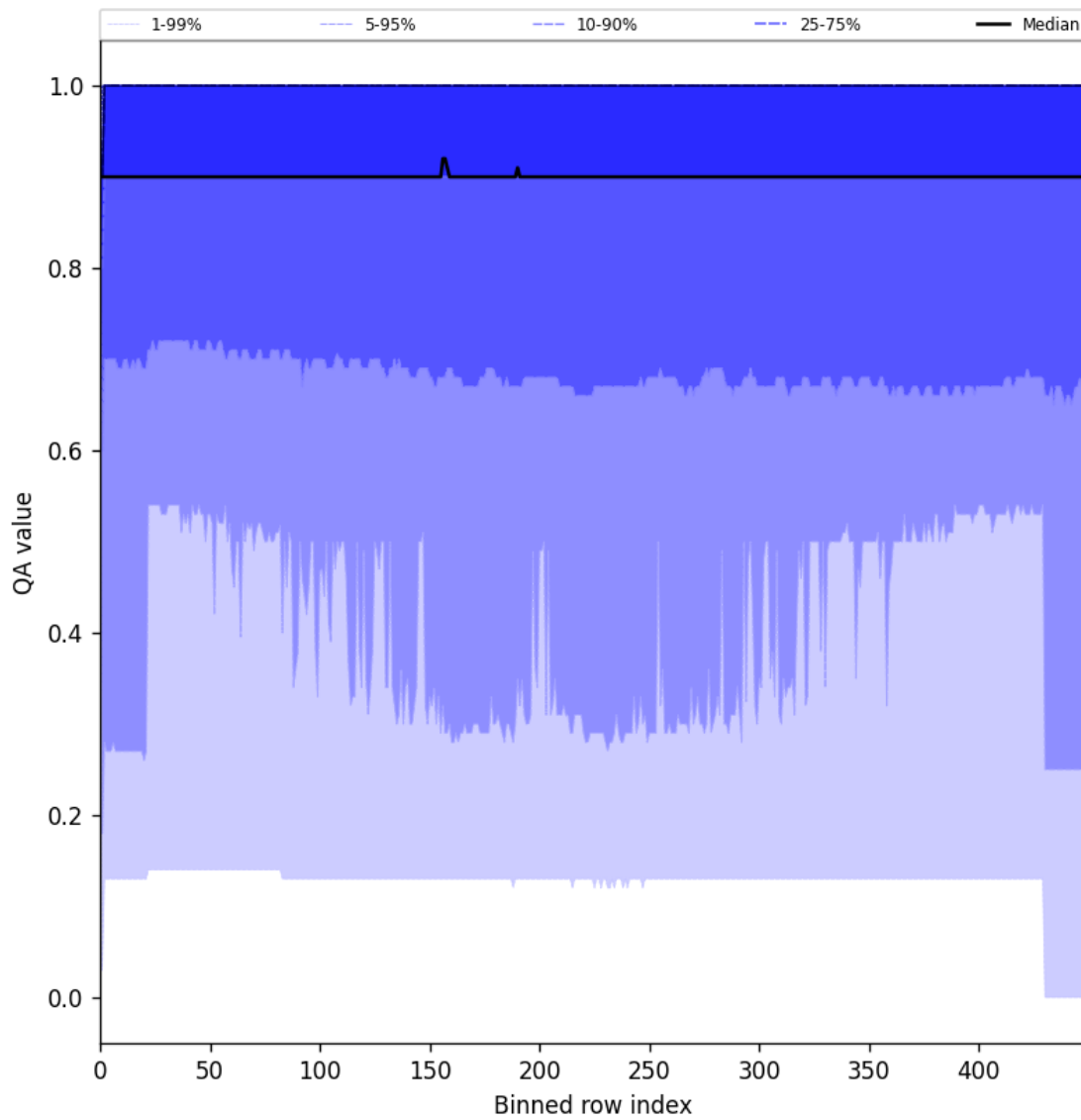
Figure 27: Along track statistics of “QA value” for 2025-08-23 to 2025-08-25
