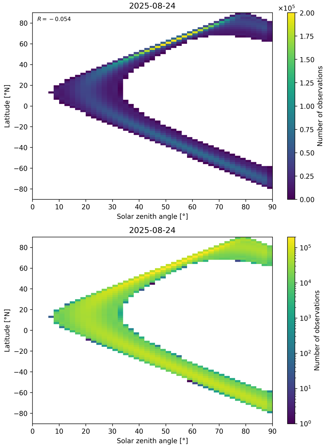
Figure 44: Scatter density plot of “Solar zenith angle” against “Latitude” for 2025-08-23 to 2025-08-25.
