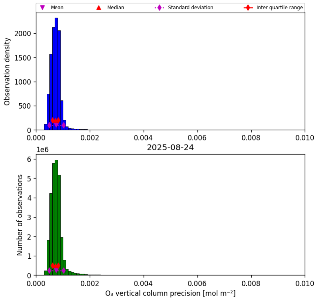
Figure 22: Histogram of “O 3 vertical column precision” for 2025-08-23 to 2025-08-25
