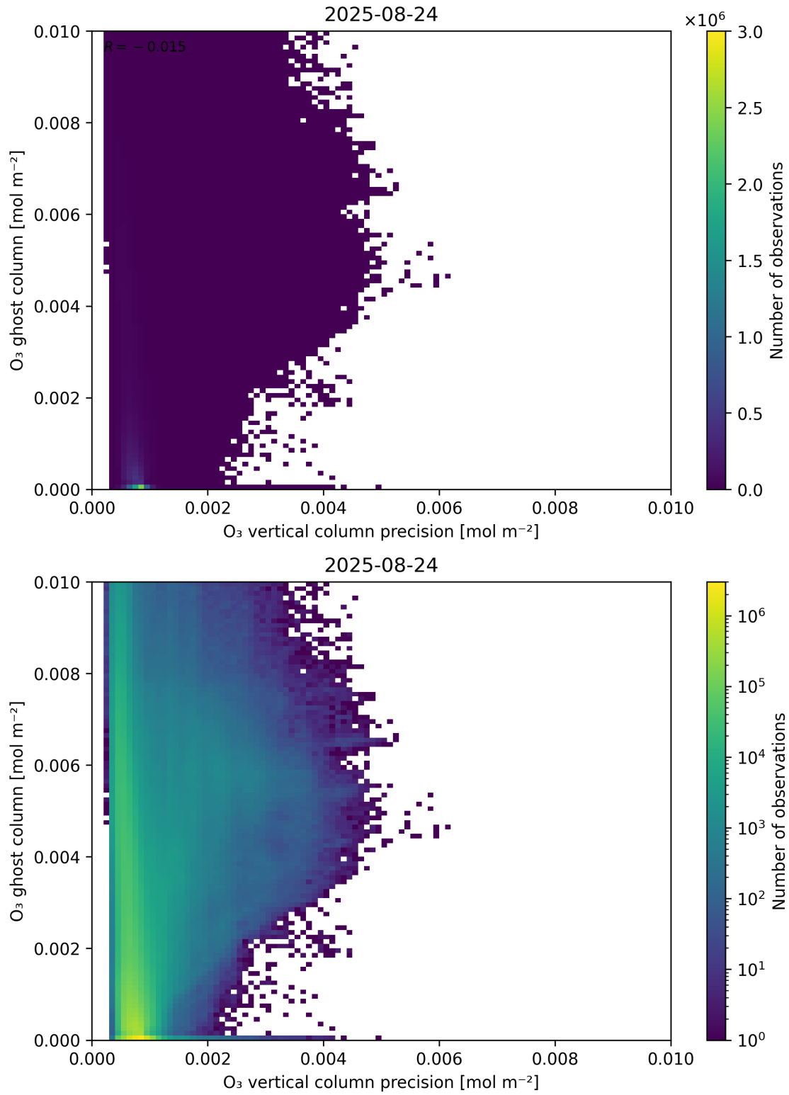
Figure 43: Scatter density plot of “ \text{O}_3 vertical column precision” against “ \text{O}_3 ghost column” for 2025-08-23 to 2025-08-25.
