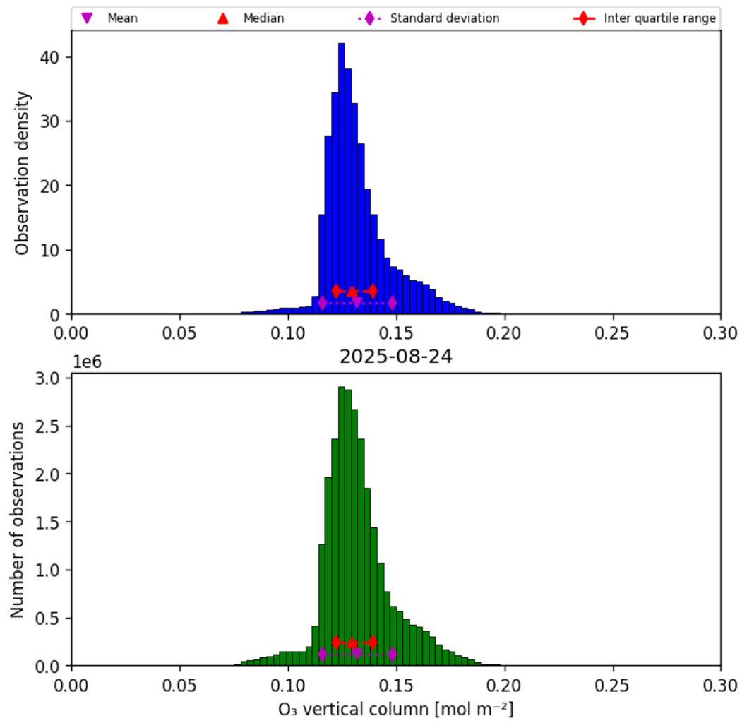
Figure 21: Histogram of “O 3 vertical column” for 2025-08-23 to 2025-08-25
