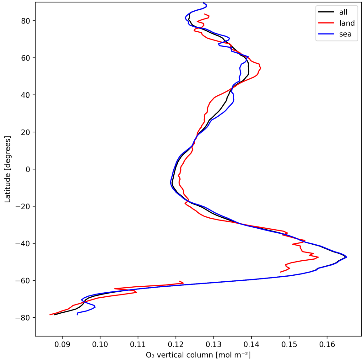
Figure 14: Zonal average of “O 3 vertical column” for 2025-08-23 to 2025-08-25.
