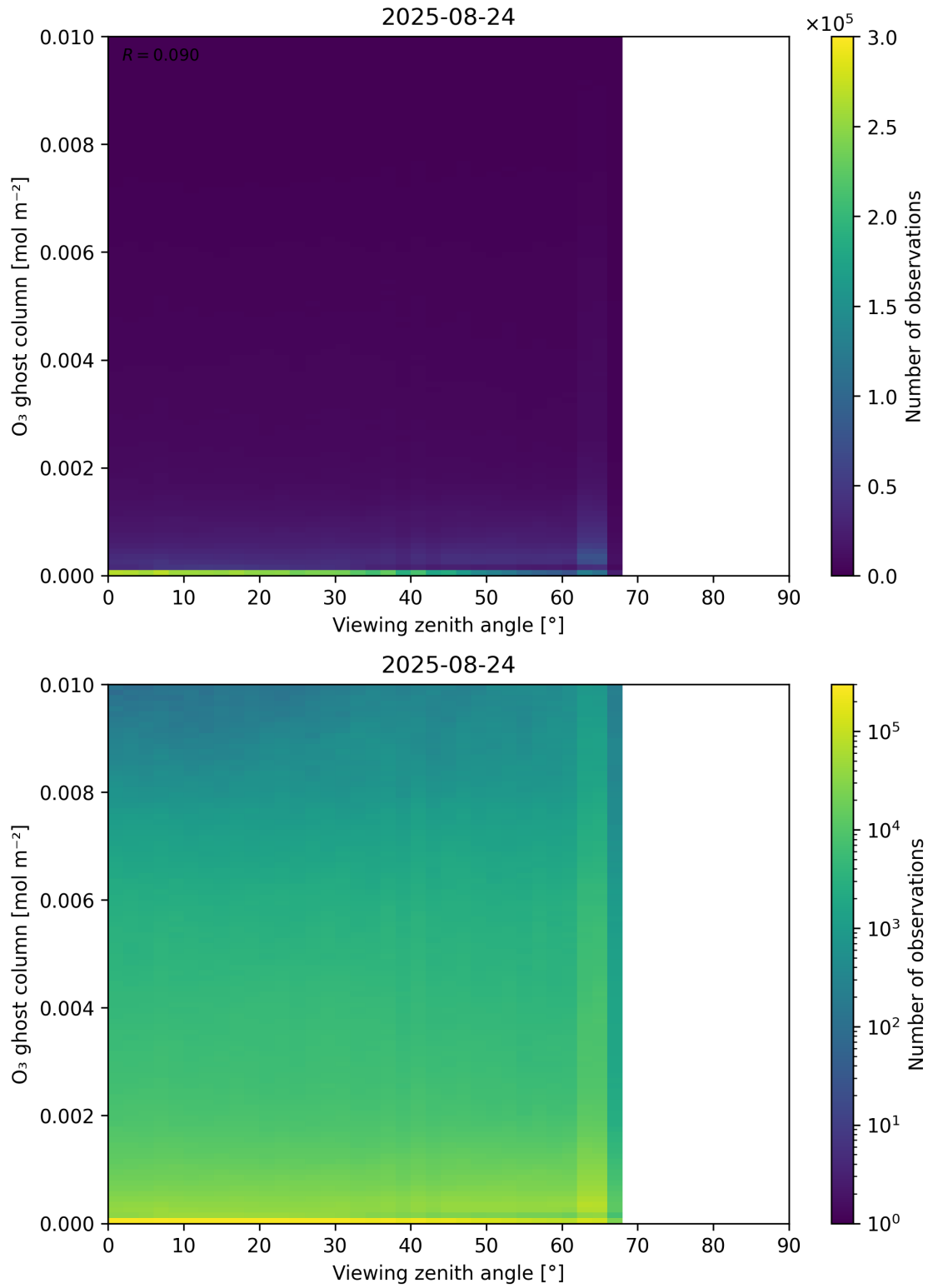
Figure 51: Scatter density plot of “Viewing zenith angle” against “O 3 ghost column” for 2025-08-23 to 2025-08-25.
