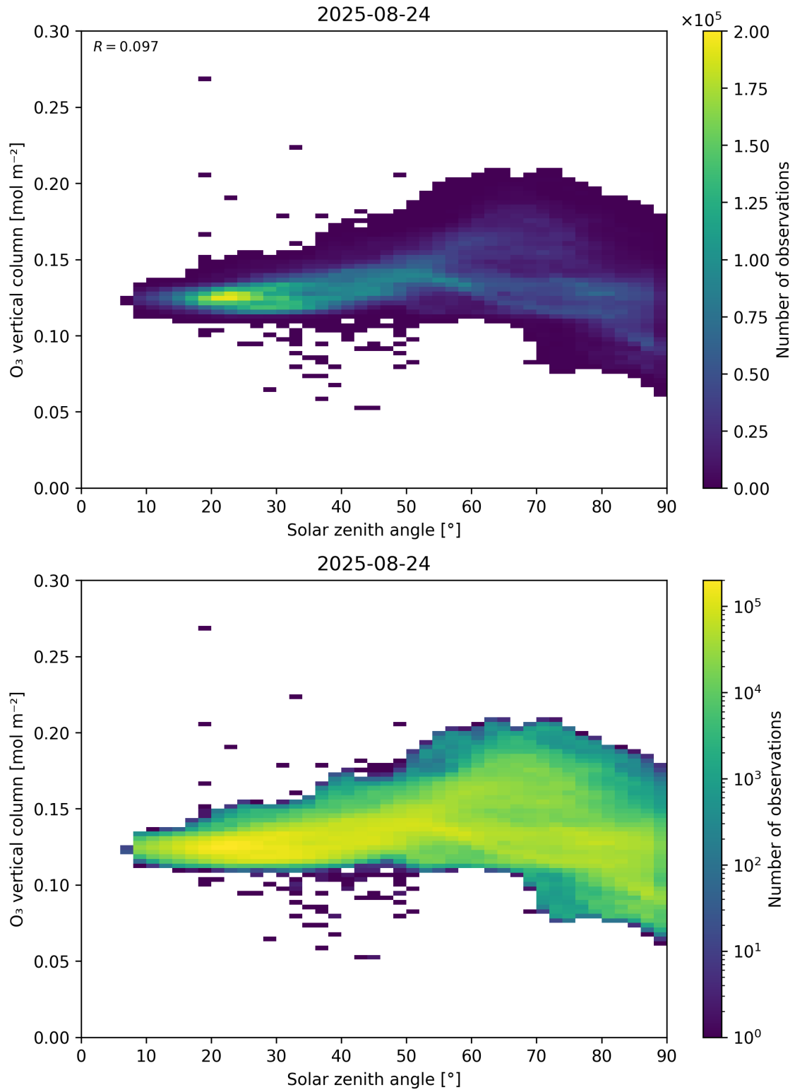
Figure 47: Scatter density plot of “Solar zenith angle” against “O 3 vertical column” for 2025-08-23 to 2025-08-25.
