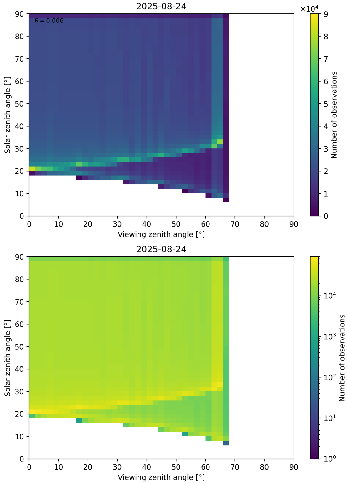
Figure 54: Scatter density plot of “Viewing zenith angle” against “Solar zenith angle” for 2025-08-23 to 2025-08-25.
