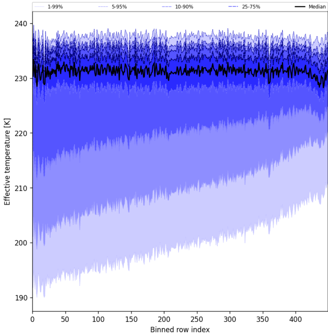
Figure 31: Along track statistics of “Effective temperature” for 2025-08-23 to 2025-08-25
