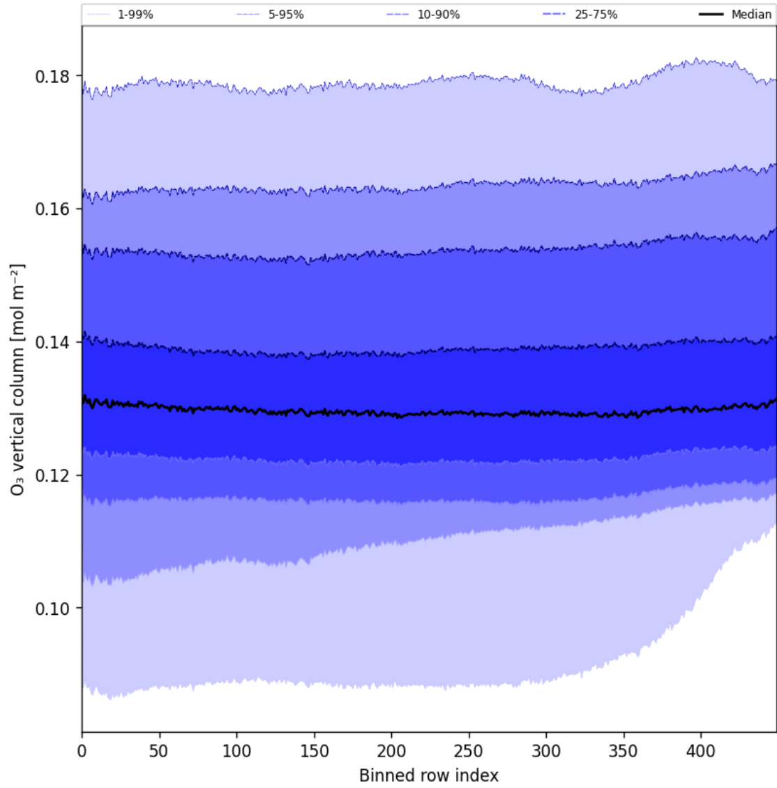
Figure 28: Along track statistics of “O 3 vertical column” for 2025-08-23 to 2025-08-25
