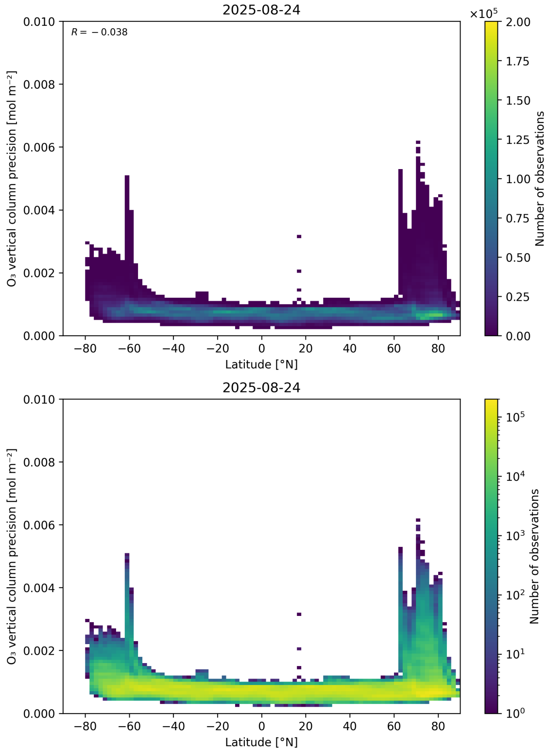
Figure 37: Scatter density plot of “Latitude” against “O 3 vertical column precision” for 2025-08-23 to 2025-08-25.
