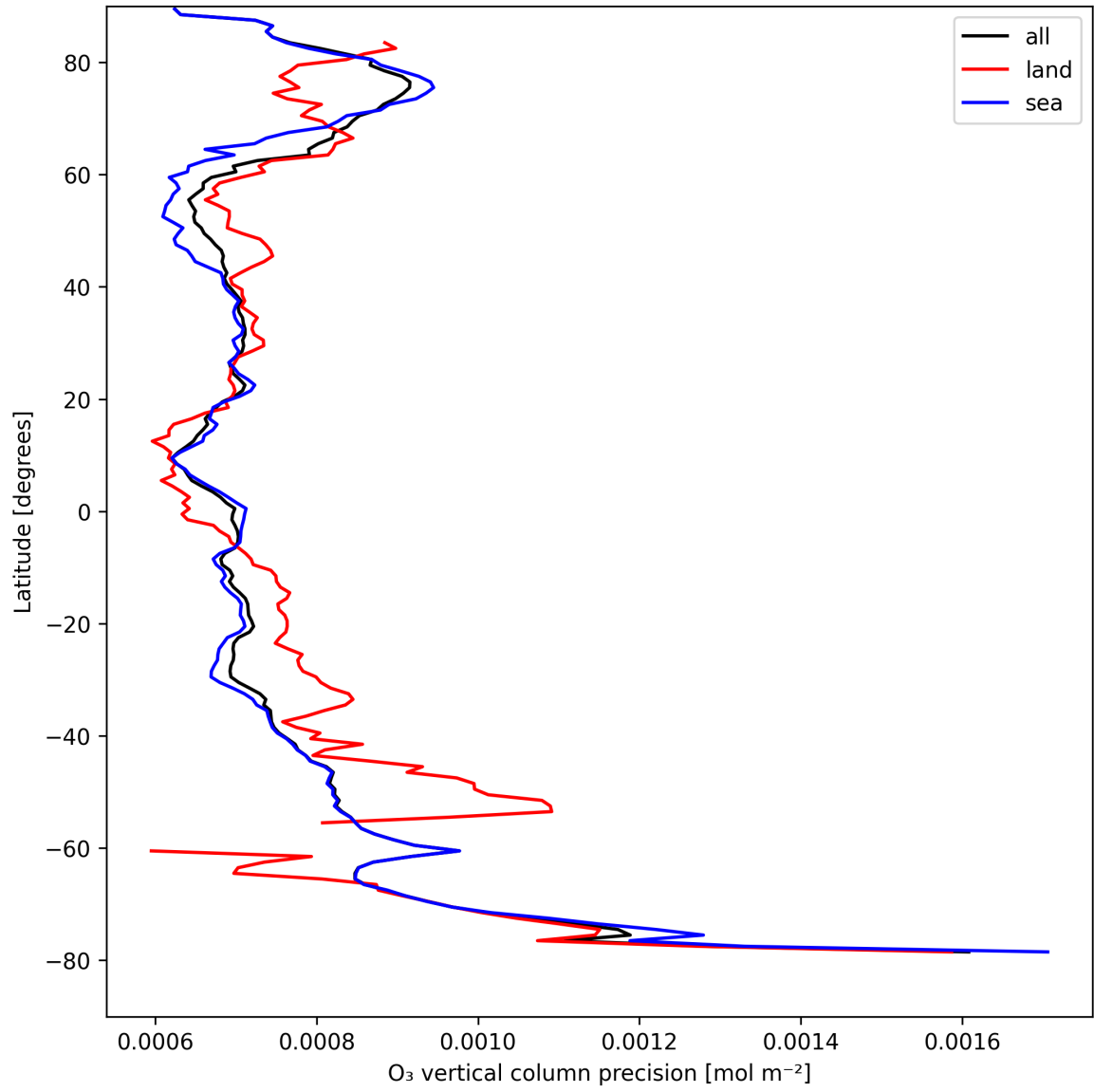
Figure 15: Zonal average of “O 3 vertical column precision” for 2025-08-23 to 2025-08-25.
