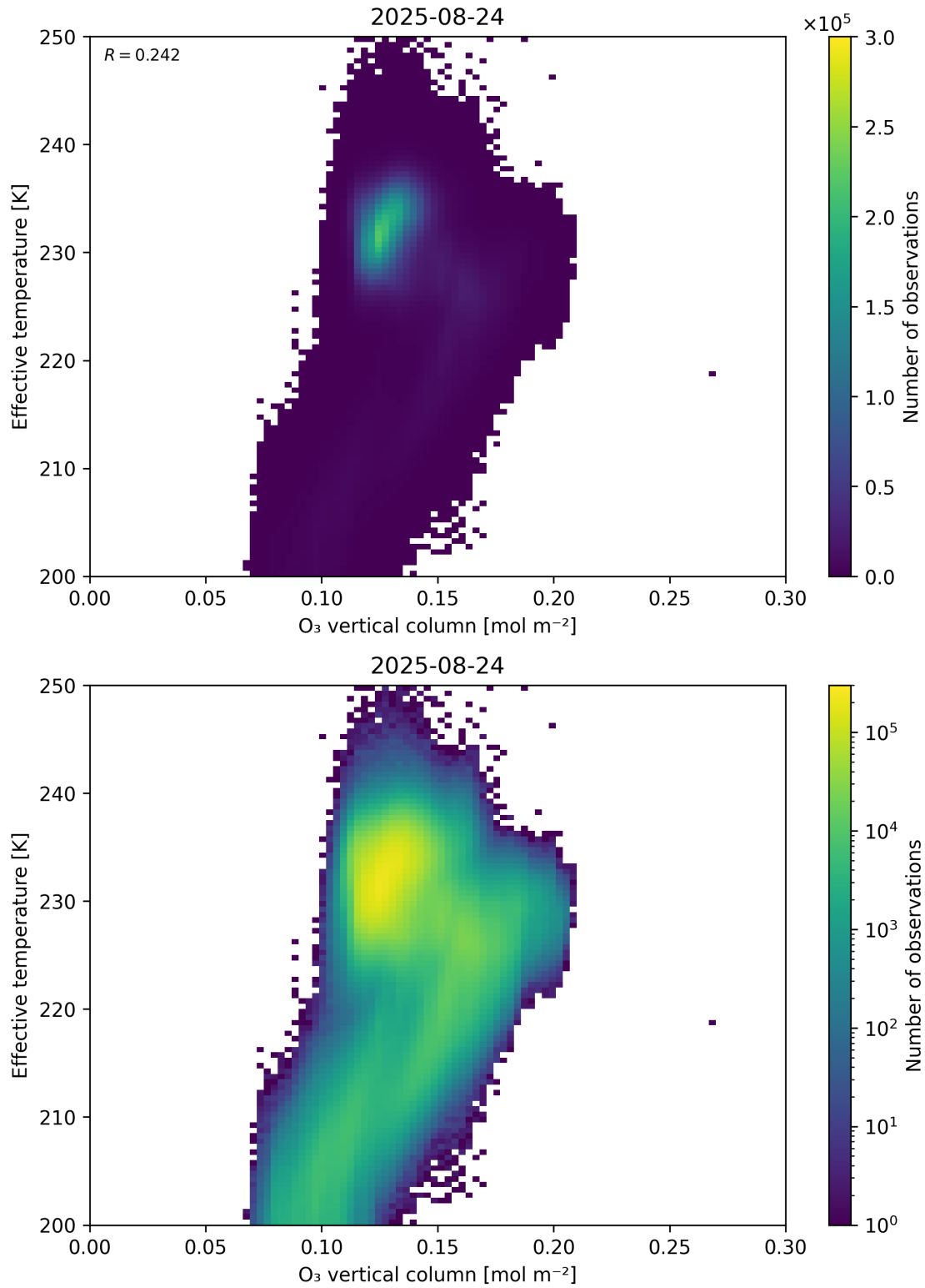
Figure 39: Scatter density plot of “O 3 vertical column” against “Effective temperature” for 2025-08-23 to 2025-08-25.
