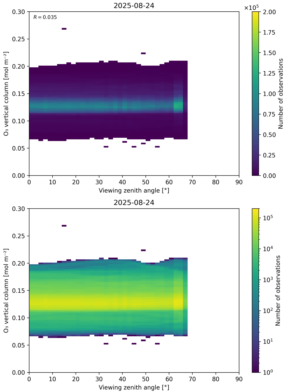
Figure 52: Scatter density plot of “Viewing zenith angle” against “O 3 vertical column” for 2025-08-23 to 2025-08-25.
