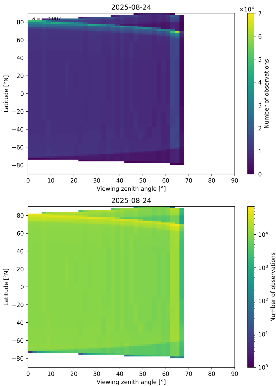
Figure 49: Scatter density plot of “Viewing zenith angle” against “Latitude” for 2025-08-23 to 2025-08-25.
