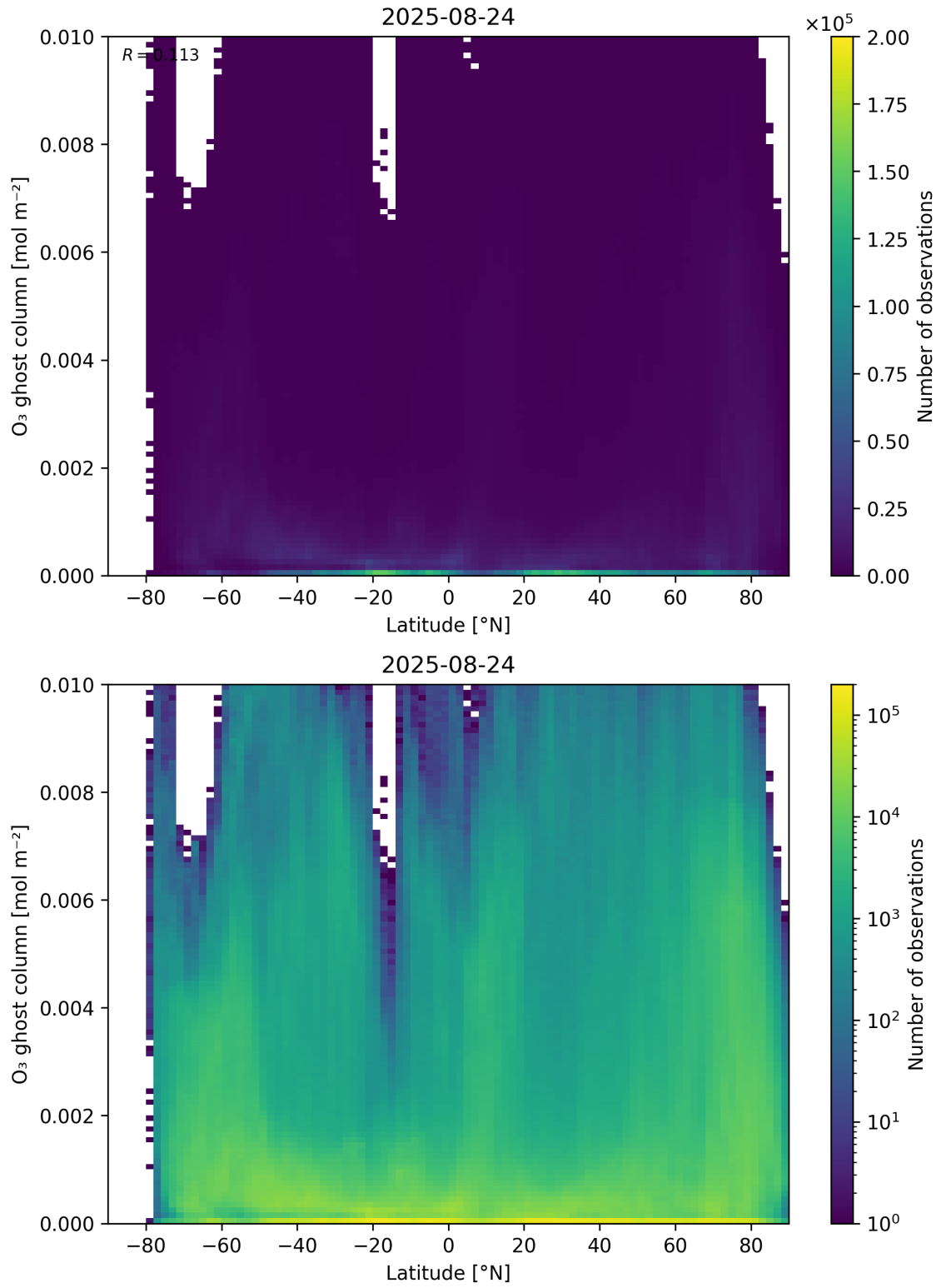
Figure 35: Scatter density plot of “Latitude” against “O 3 ghost column” for 2025-08-23 to 2025-08-25.
