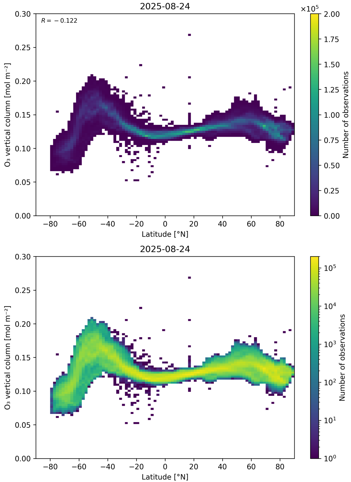
Figure 36: Scatter density plot of “Latitude” against “O 3 vertical column” for 2025-08-23 to 2025-08-25.
