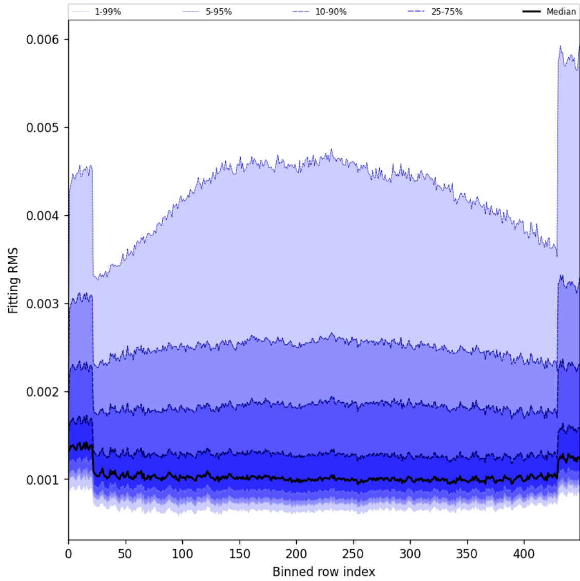
Figure 30: Along track statistics of “Fitting RMS” for 2025-08-23 to 2025-08-25
