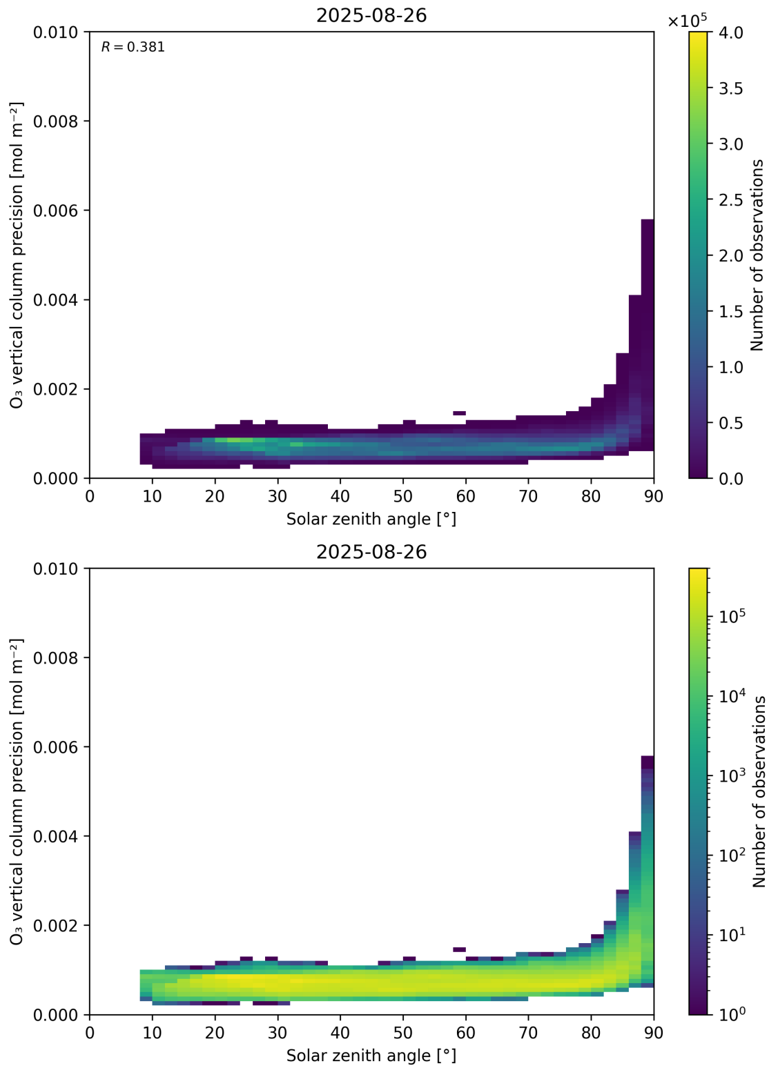
Figure 48: Scatter density plot of “Solar zenith angle” against “O 3 vertical column precision” for 2025-08-25 to 2025-08-27.
