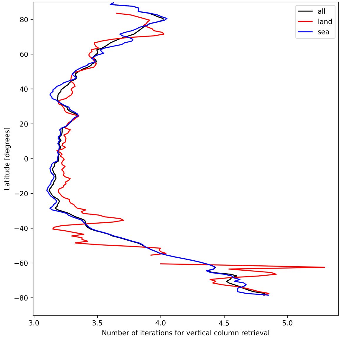
Figure 19: Zonal average of “Number of iterations for vertical column retrieval” for 2025-08-25 to 2025-08-27.
