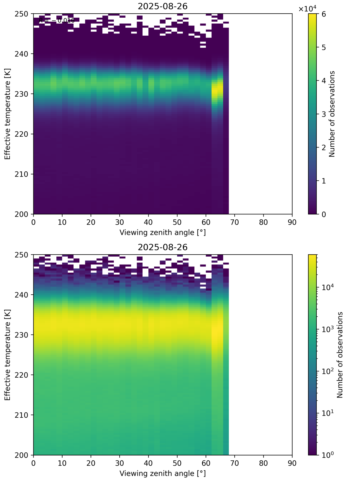
Figure 50: Scatter density plot of “Viewing zenith angle” against “Effective temperature” for 2025-08-25 to 2025-08-27.
