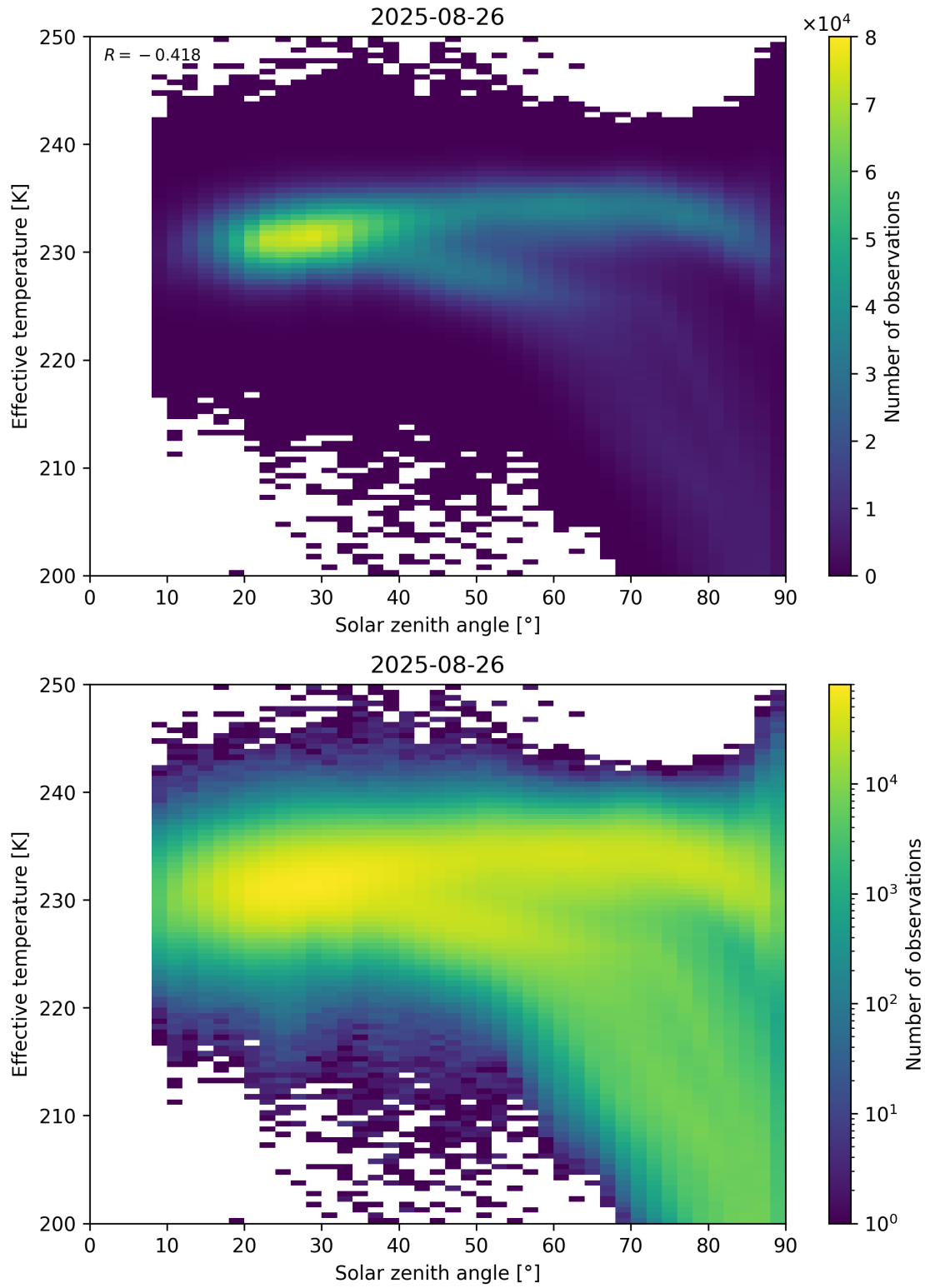
Figure 45: Scatter density plot of “Solar zenith angle” against “Effective temperature” for 2025-08-25 to 2025-08-27.
