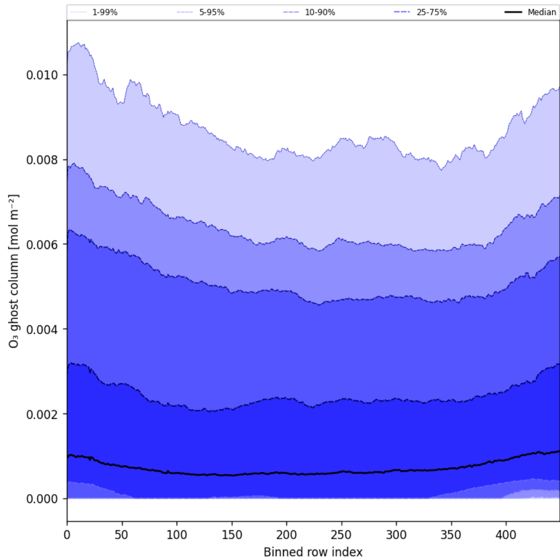
Figure 32: Along track statistics of “O 3 ghost column” for 2025-08-25 to 2025-08-27
