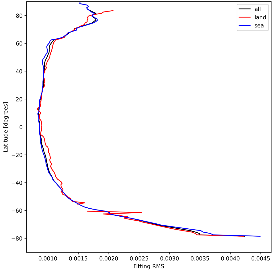
Figure 16: Zonal average of “Fitting RMS” for 2025-08-25 to 2025-08-27.
