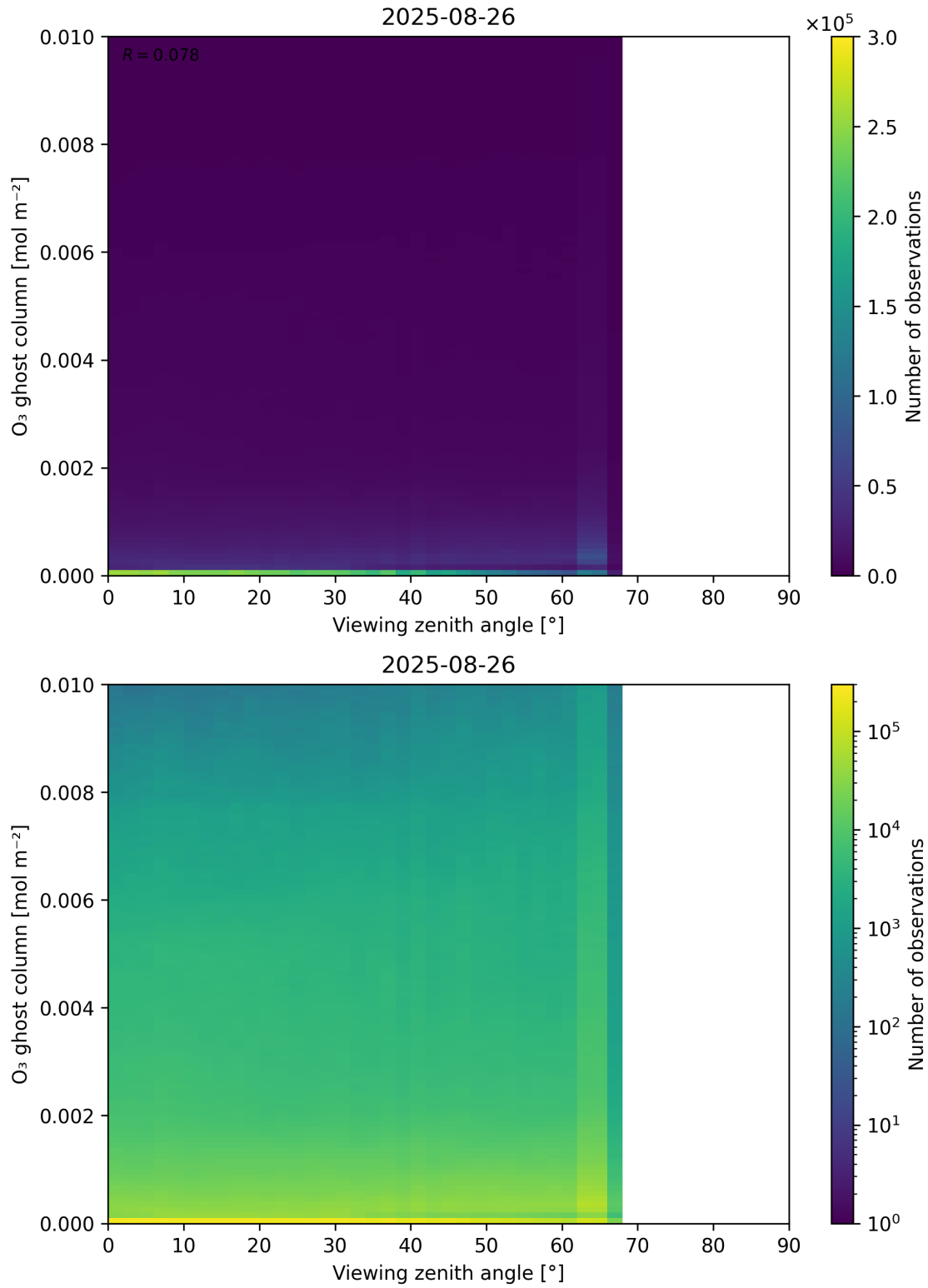
Figure 51: Scatter density plot of “Viewing zenith angle” against “O 3 ghost column” for 2025-08-25 to 2025-08-27.
