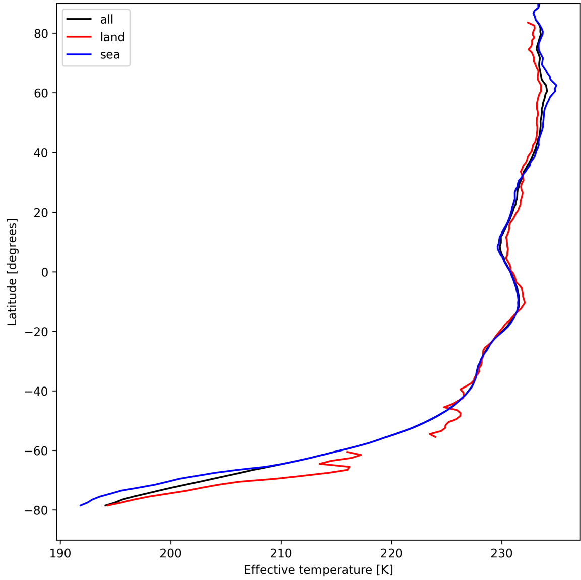
Figure 17: Zonal average of "Effective temperature" for 2025-08-25 to 2025-08-27.
