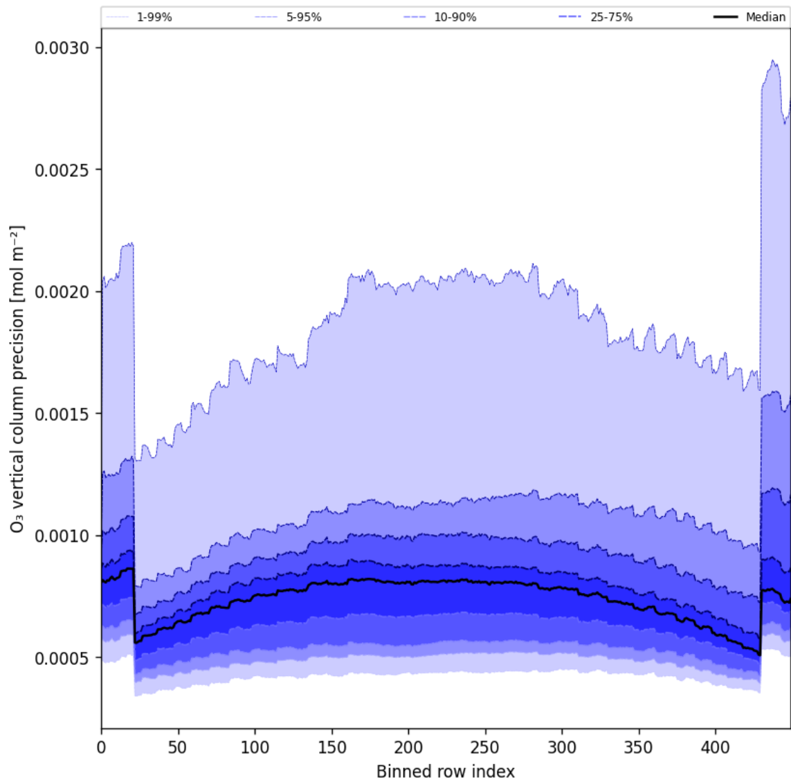
Figure 29: Along track statistics of “O 3 vertical column precision” for 2025-08-25 to 2025-08-27
