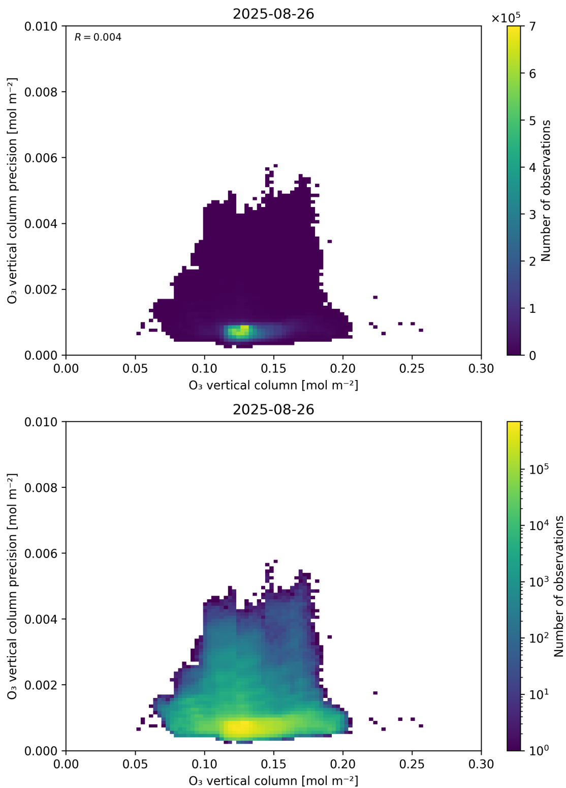
Figure 41: Scatter density plot of “O 3 vertical column” against “O 3 vertical column precision” for 2025-08-25 to 2025-08-27.
