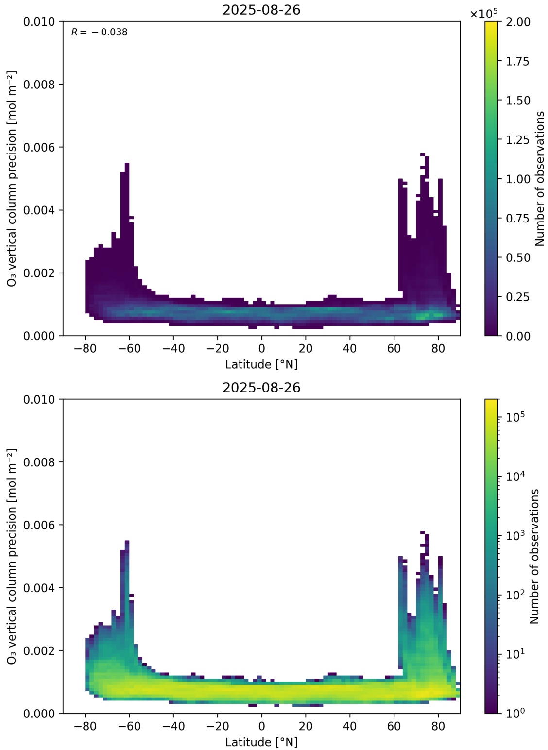
Figure 37: Scatter density plot of “Latitude” against “O 3 vertical column precision” for 2025-08-25 to 2025-08-27.
