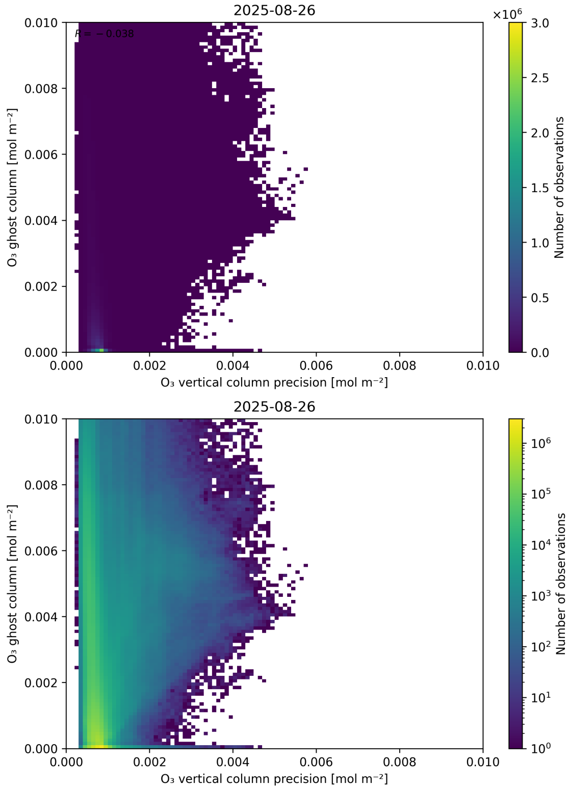
Figure 43: Scatter density plot of “O 3 vertical column precision” against “O 3 ghost column” for 2025-08-25 to 2025-08-27.
