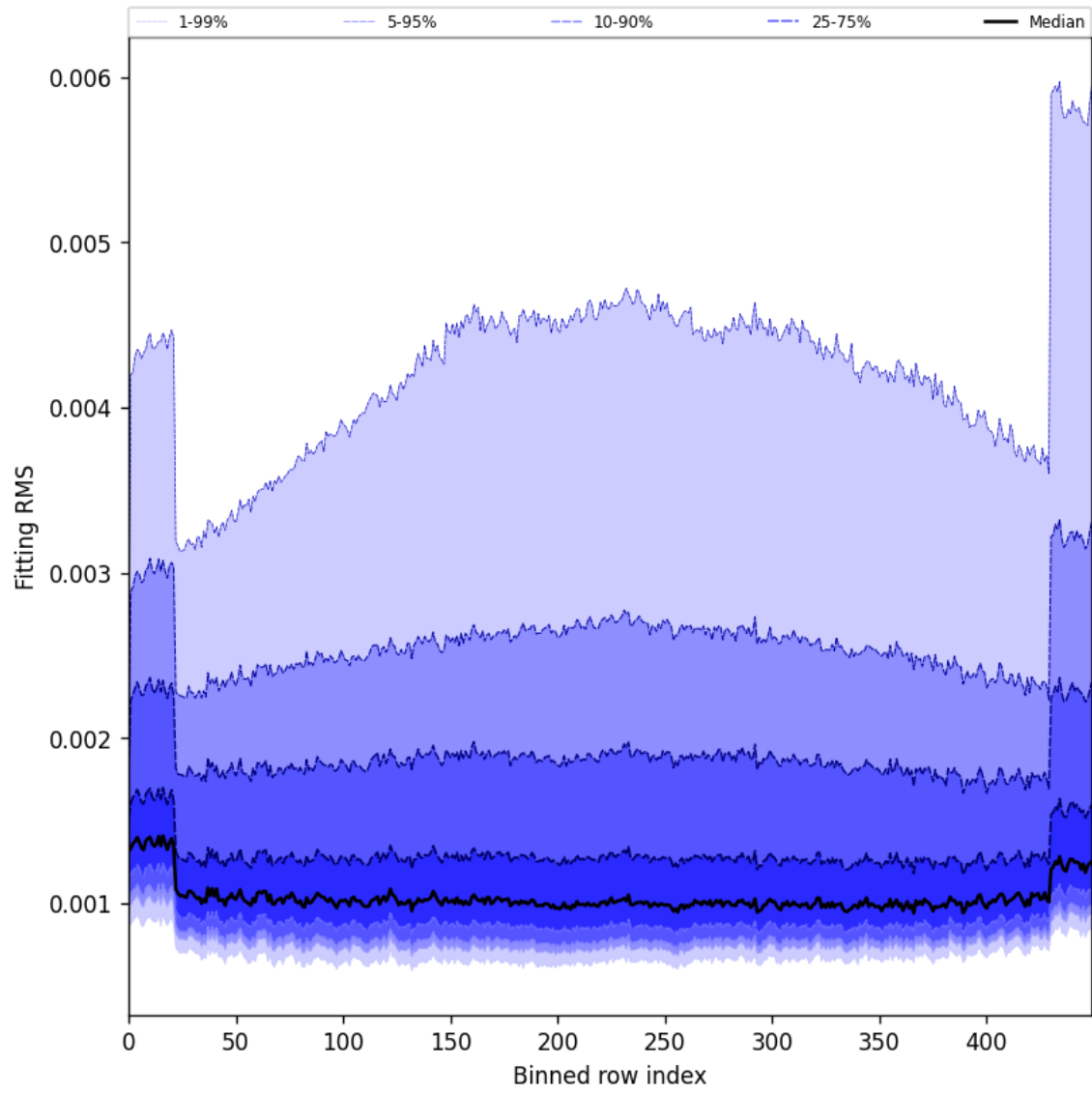
Figure 30: Along track statistics of “Fitting RMS” for 2025-08-25 to 2025-08-27
