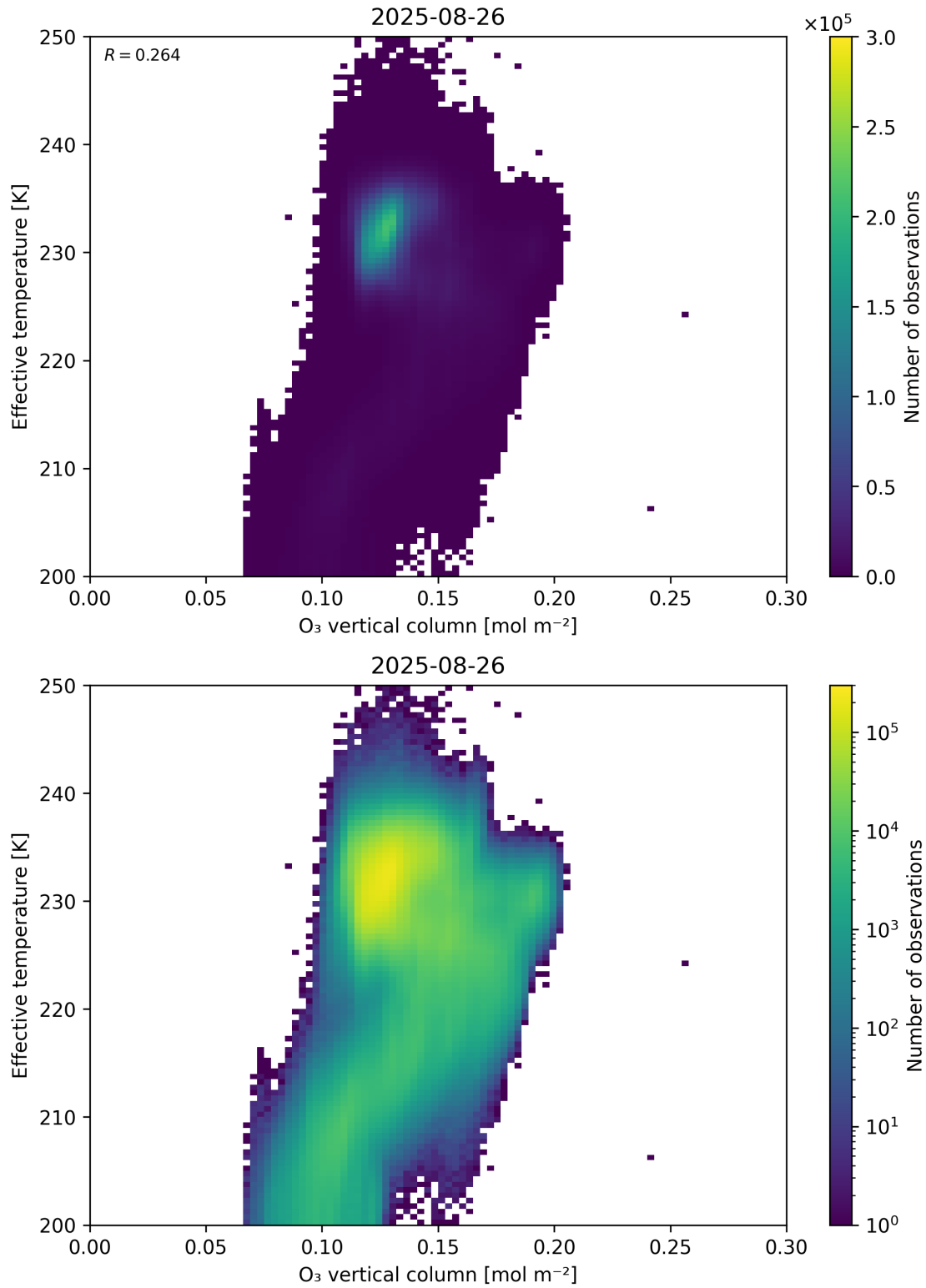
Figure 39: Scatter density plot of “O 3 vertical column” against “Effective temperature” for 2025-08-25 to 2025-08-27.
