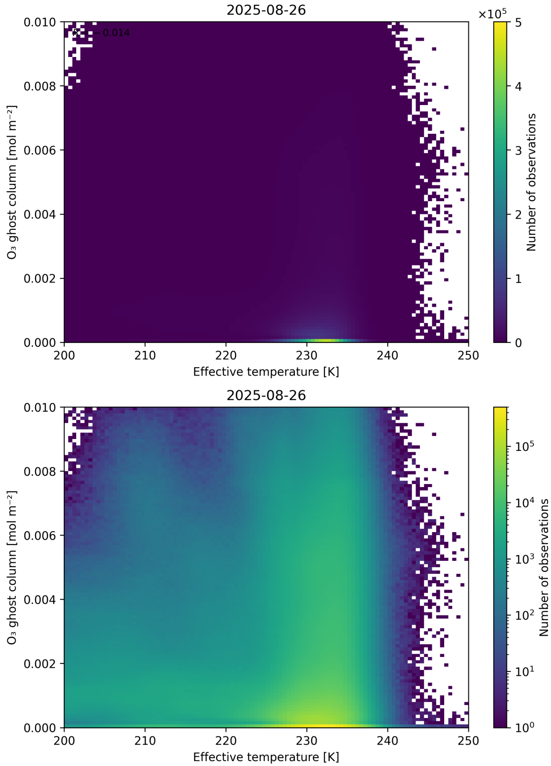
Figure 38: Scatter density plot of “Effective temperature” against “O 3 ghost column” for 2025-08-25 to 2025-08-27.
