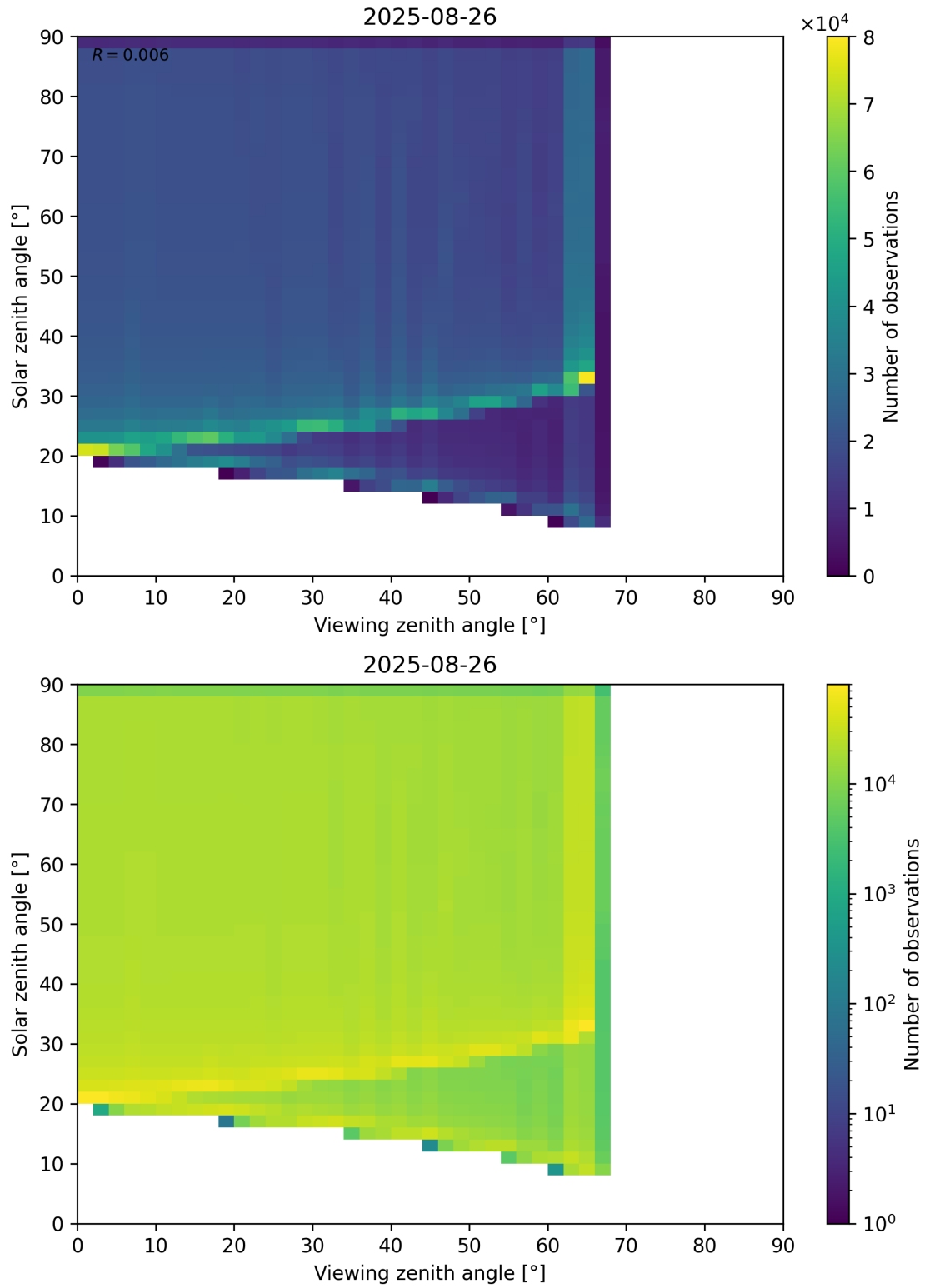
Figure 54: Scatter density plot of “Viewing zenith angle” against “Solar zenith angle” for 2025-08-25 to 2025-08-27.
