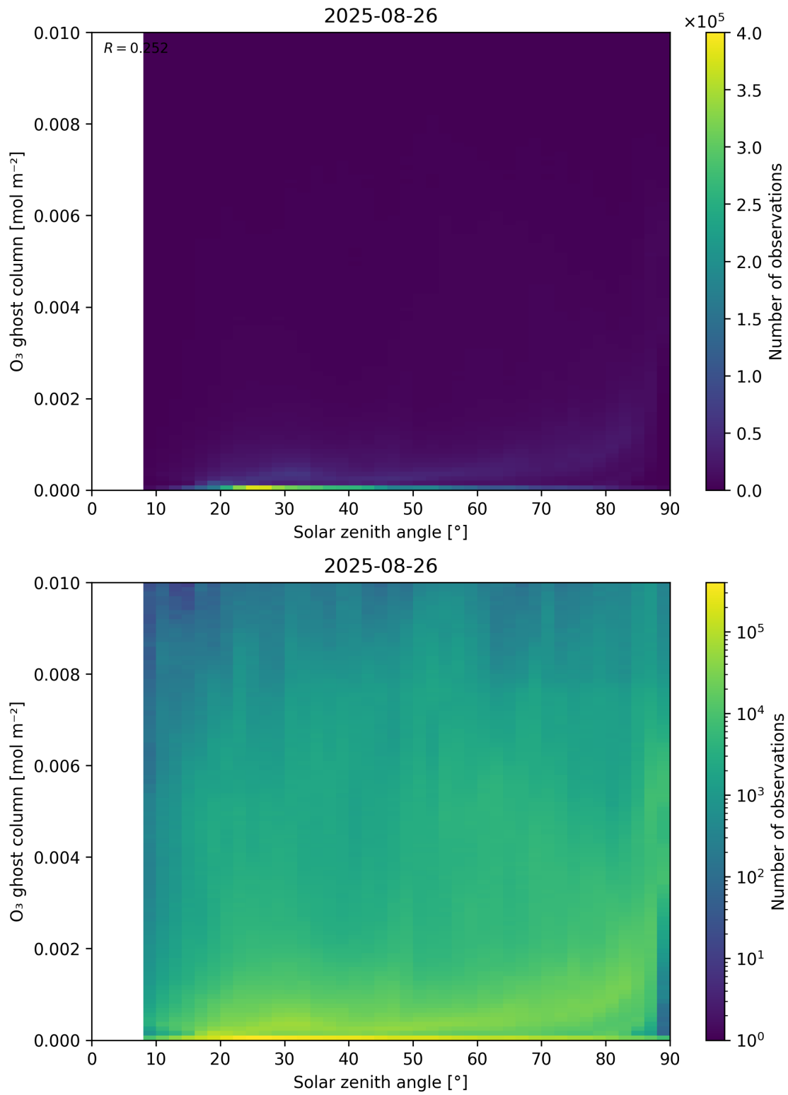
Figure 46: Scatter density plot of “Solar zenith angle” against “O 3 ghost column” for 2025-08-25 to 2025-08-27.
