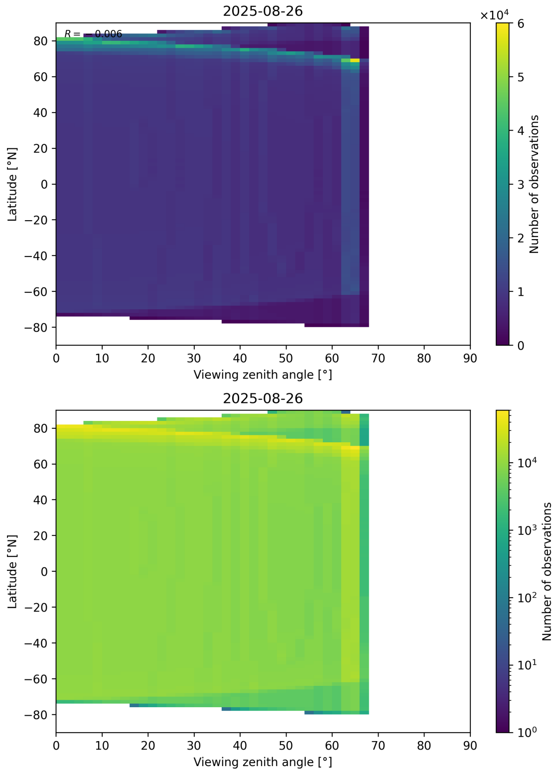
Figure 49: Scatter density plot of “Viewing zenith angle” against “Latitude” for 2025-08-25 to 2025-08-27.
