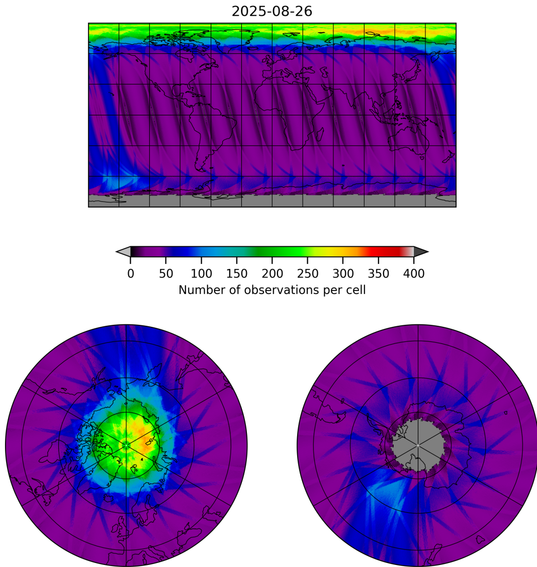
Figure 12: Map of the number of observations for 2025-08-25 to 2025-08-27
