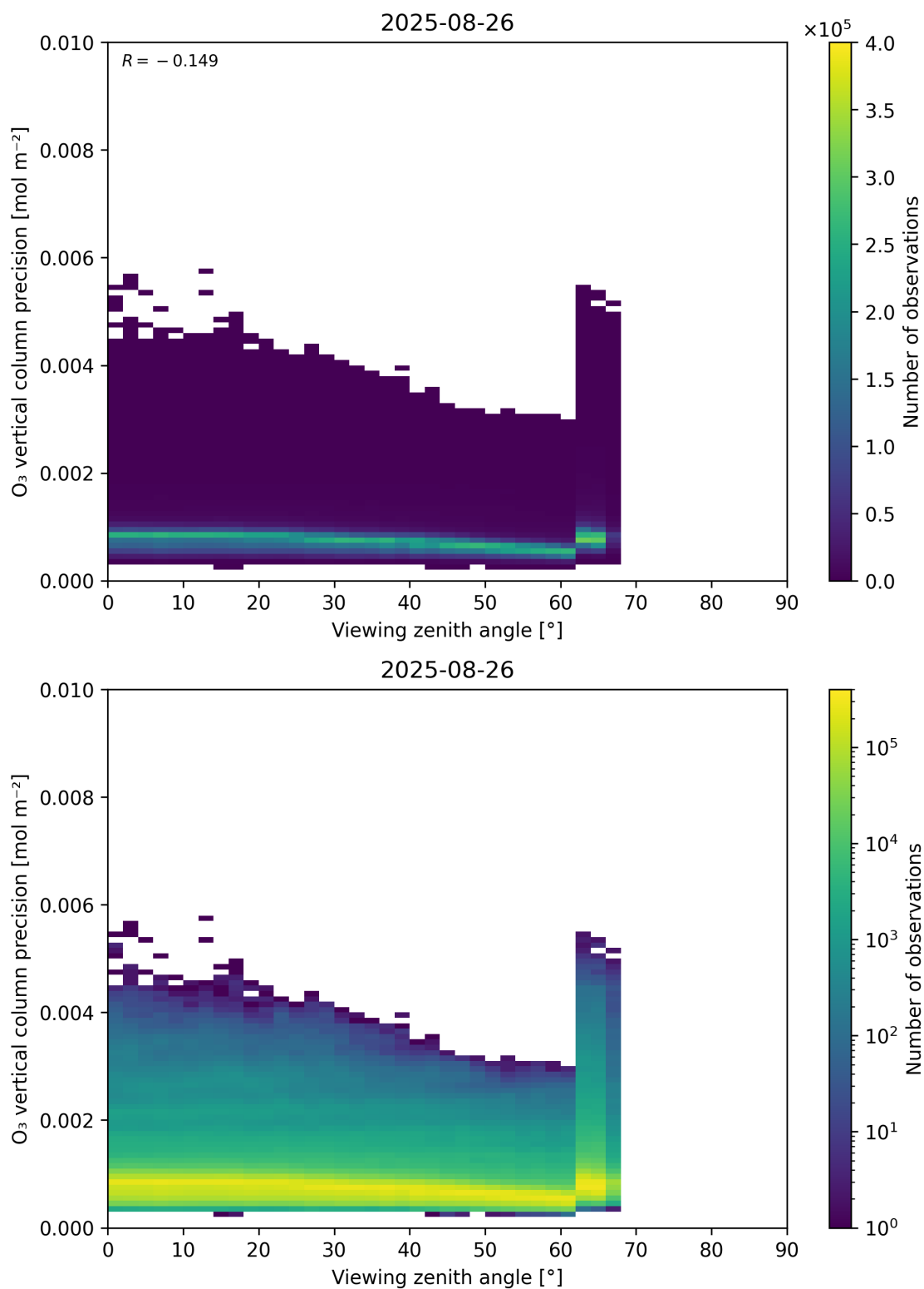
Figure 53: Scatter density plot of “Viewing zenith angle” against “O 3 vertical column precision” for 2025-08-25 to 2025-08-27.
