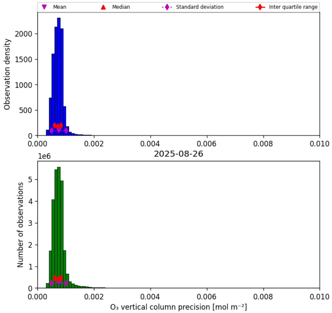
Figure 22: Histogram of “O 3 vertical column precision” for 2025-08-25 to 2025-08-27
