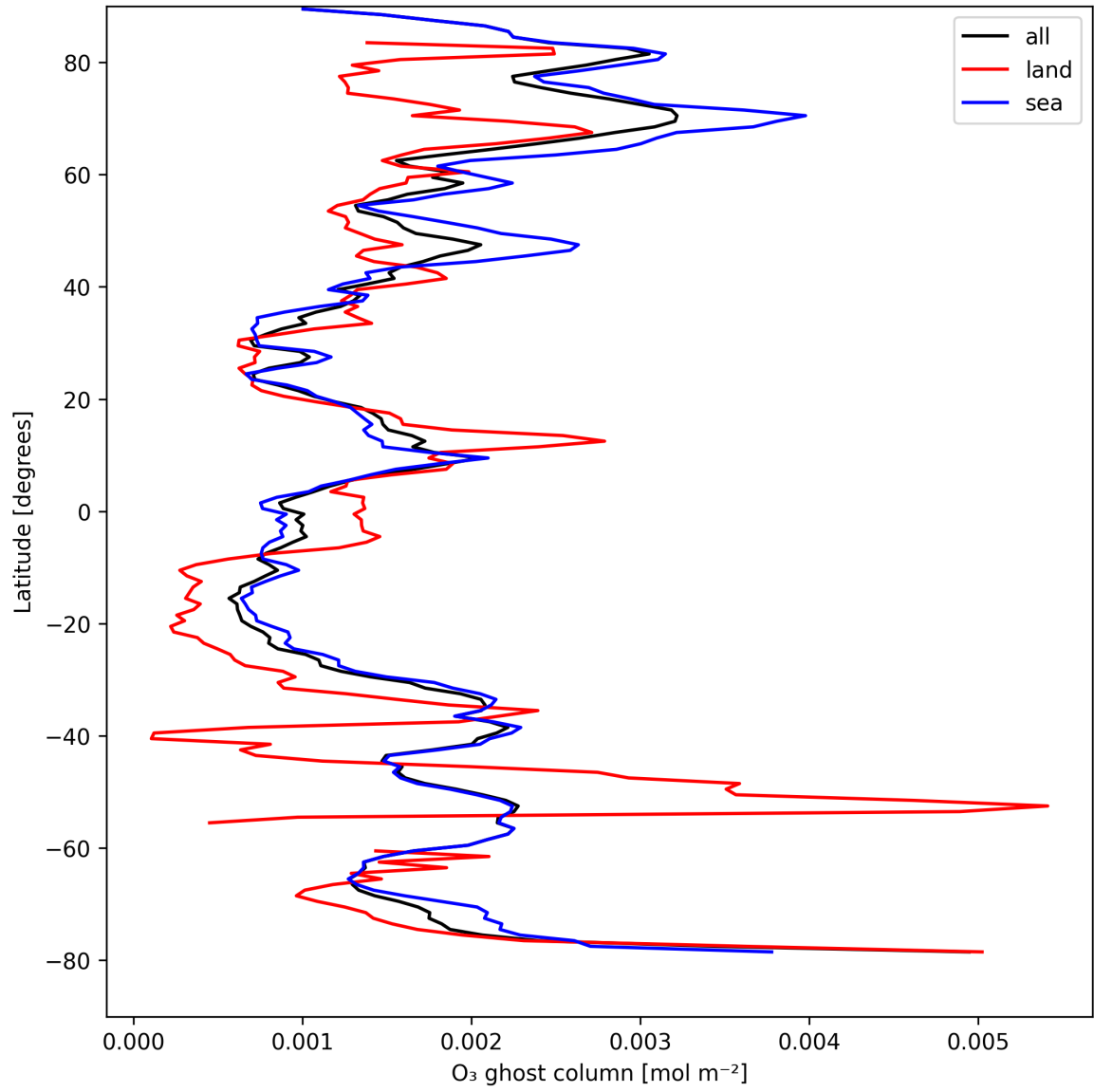
Figure 18: Zonal average of “O 3 ghost column” for 2025-08-25 to 2025-08-27.
