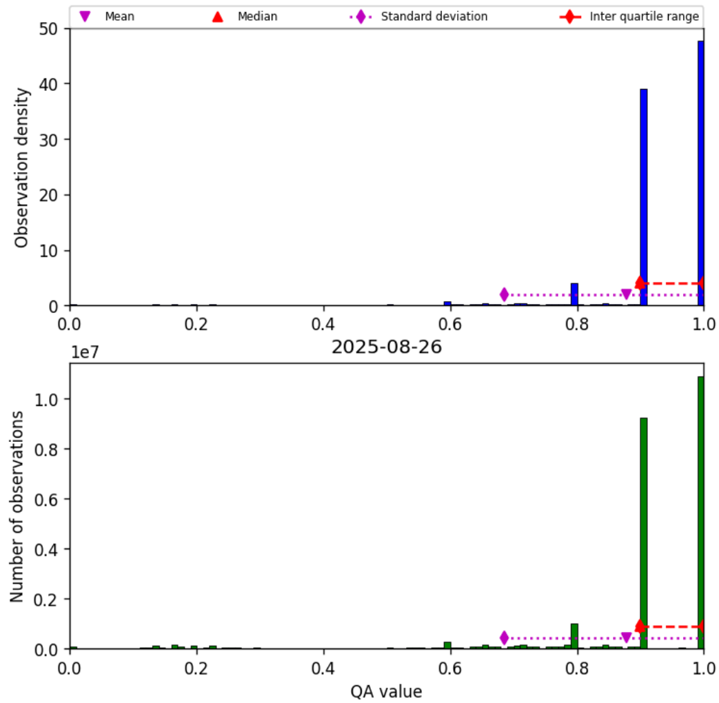
Figure 20: Histogram of “QA value” for 2025-08-25 to 2025-08-27
