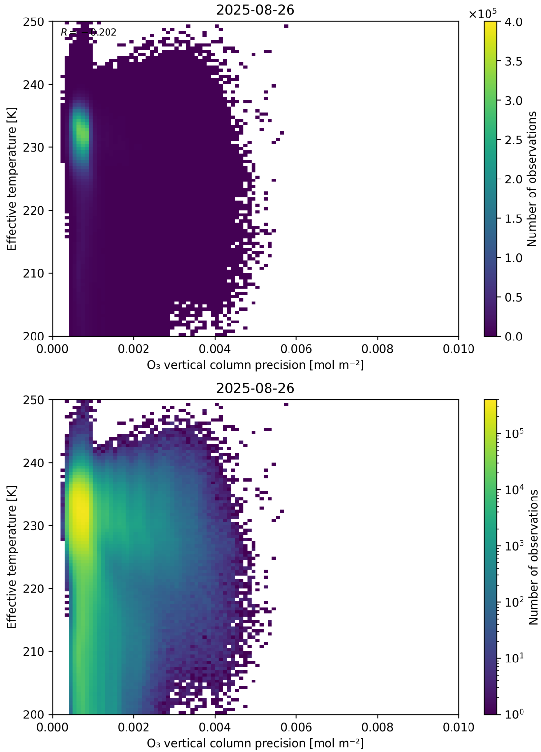
Figure 42: Scatter density plot of “O 3 vertical column precision” against “Effective temperature” for 2025-08-25 to 2025-08-27.
