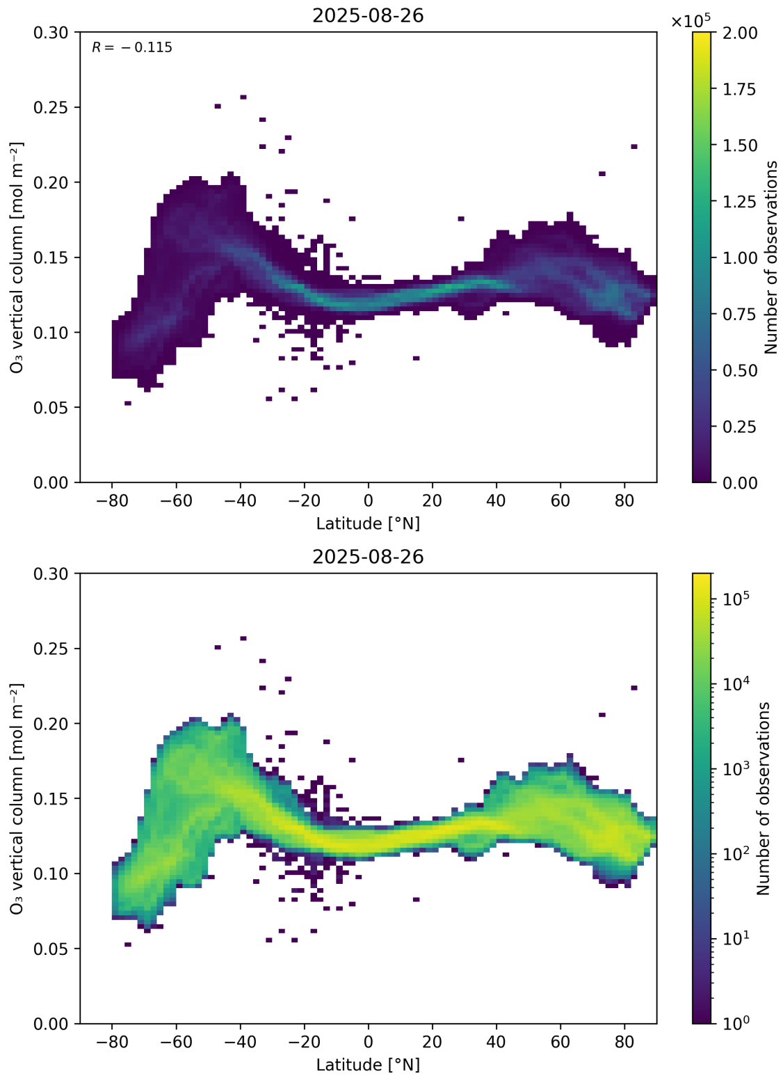
Figure 36: Scatter density plot of “Latitude” against “O 3 vertical column” for 2025-08-25 to 2025-08-27.
