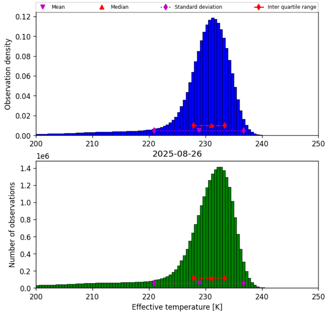
Figure 24: Histogram of “Effective temperature” for 2025-08-25 to 2025-08-27
