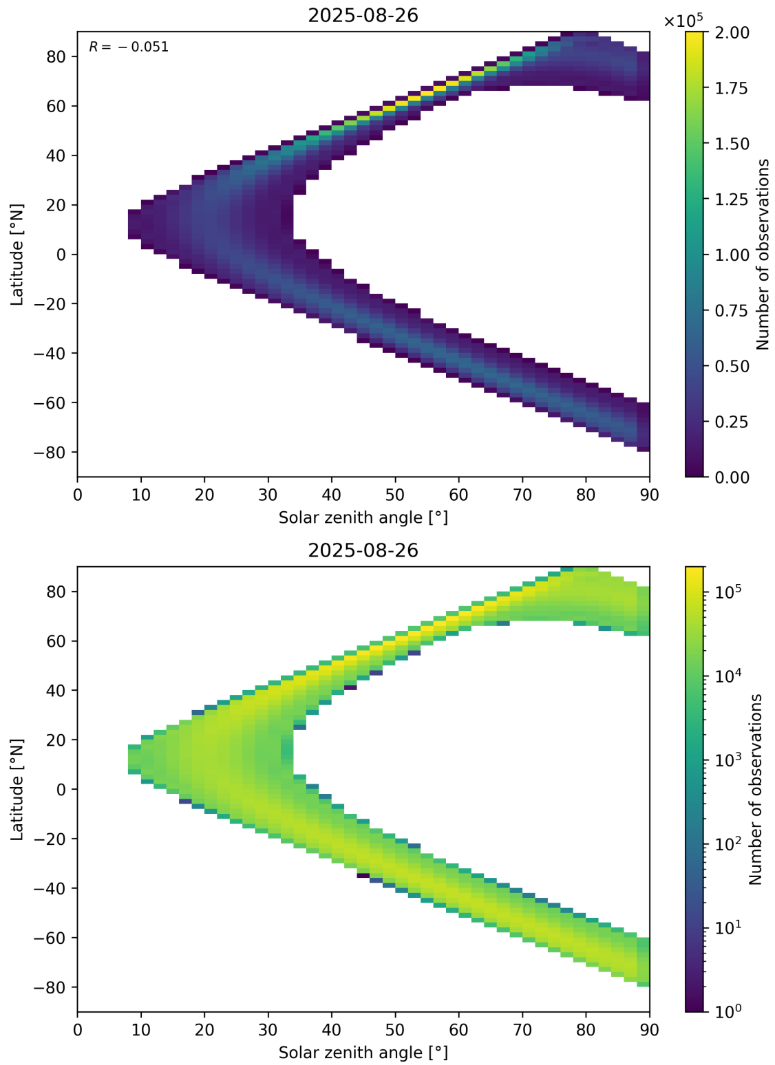
Figure 44: Scatter density plot of “Solar zenith angle” against “Latitude” for 2025-08-25 to 2025-08-27.
