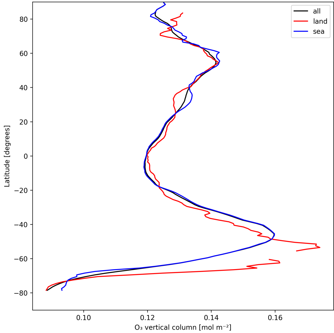
Figure 14: Zonal average of “O 3 vertical column” for 2025-08-25 to 2025-08-27.
