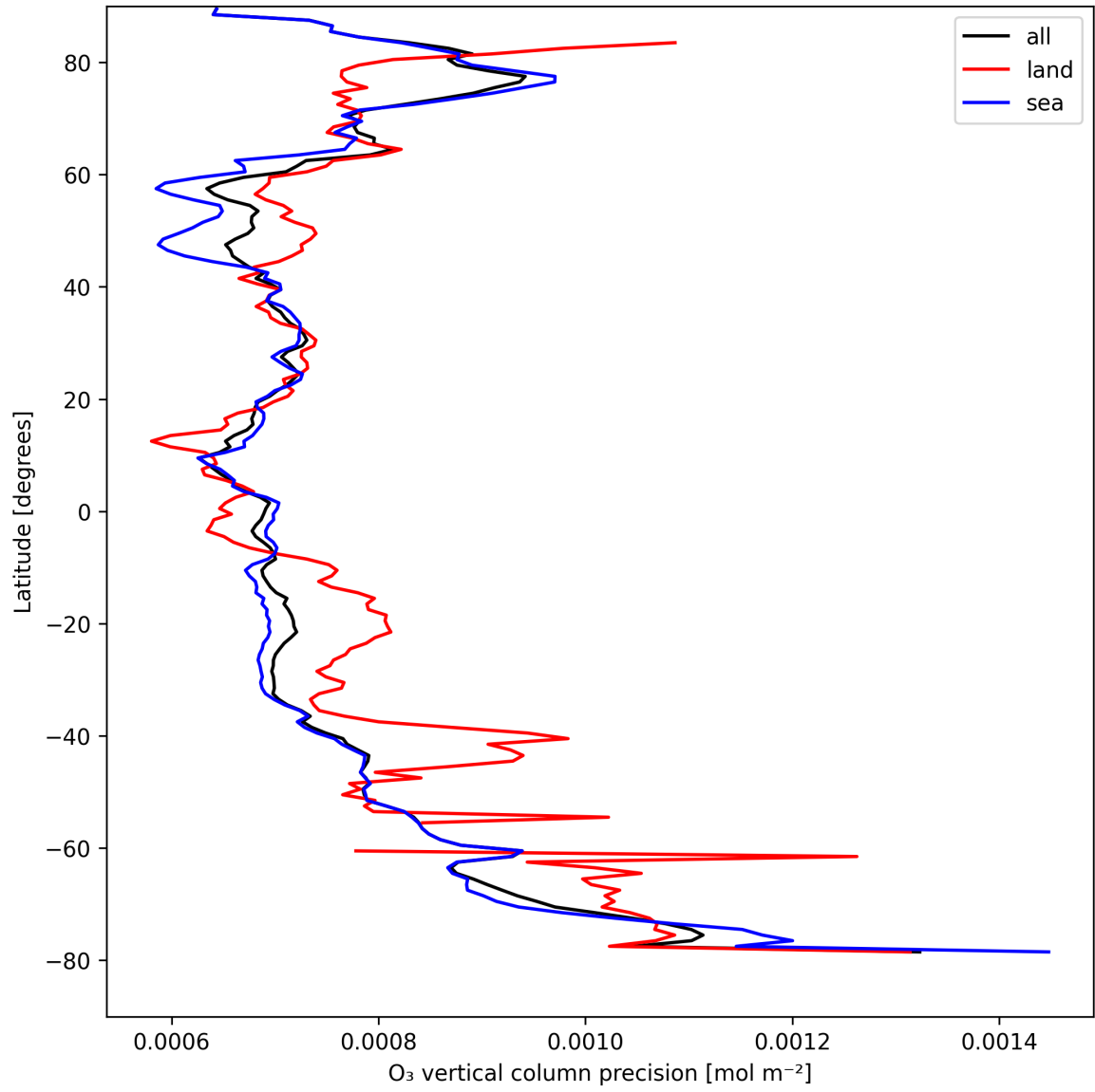
Figure 15: Zonal average of “O 3 vertical column precision” for 2025-08-25 to 2025-08-27.
