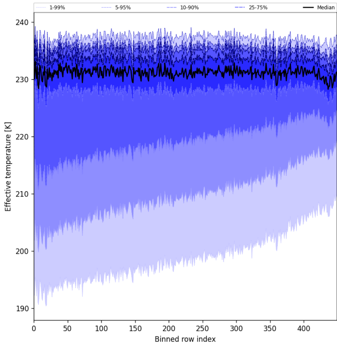
Figure 31: Along track statistics of “Effective temperature” for 2025-08-25 to 2025-08-27
