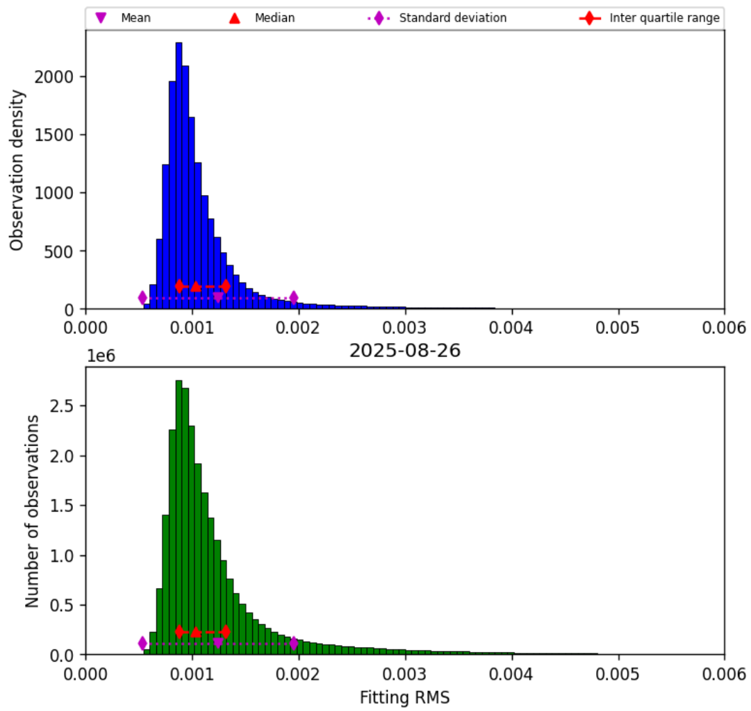
Figure 23: Histogram of “Fitting RMS” for 2025-08-25 to 2025-08-27
