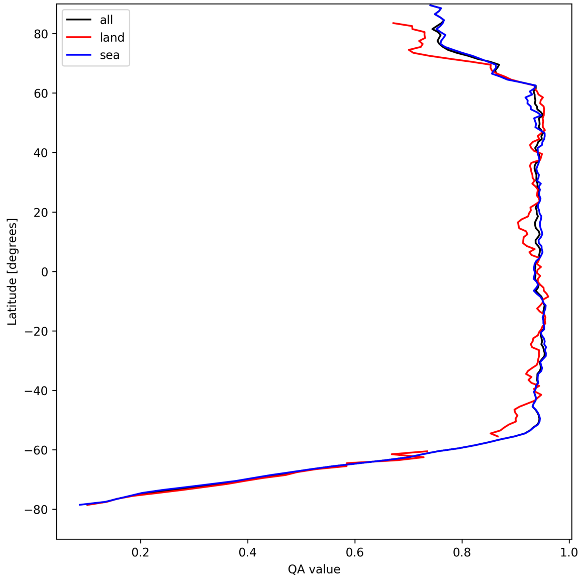
Figure 13: Zonal average of “QA value” for 2025-08-25 to 2025-08-27.
