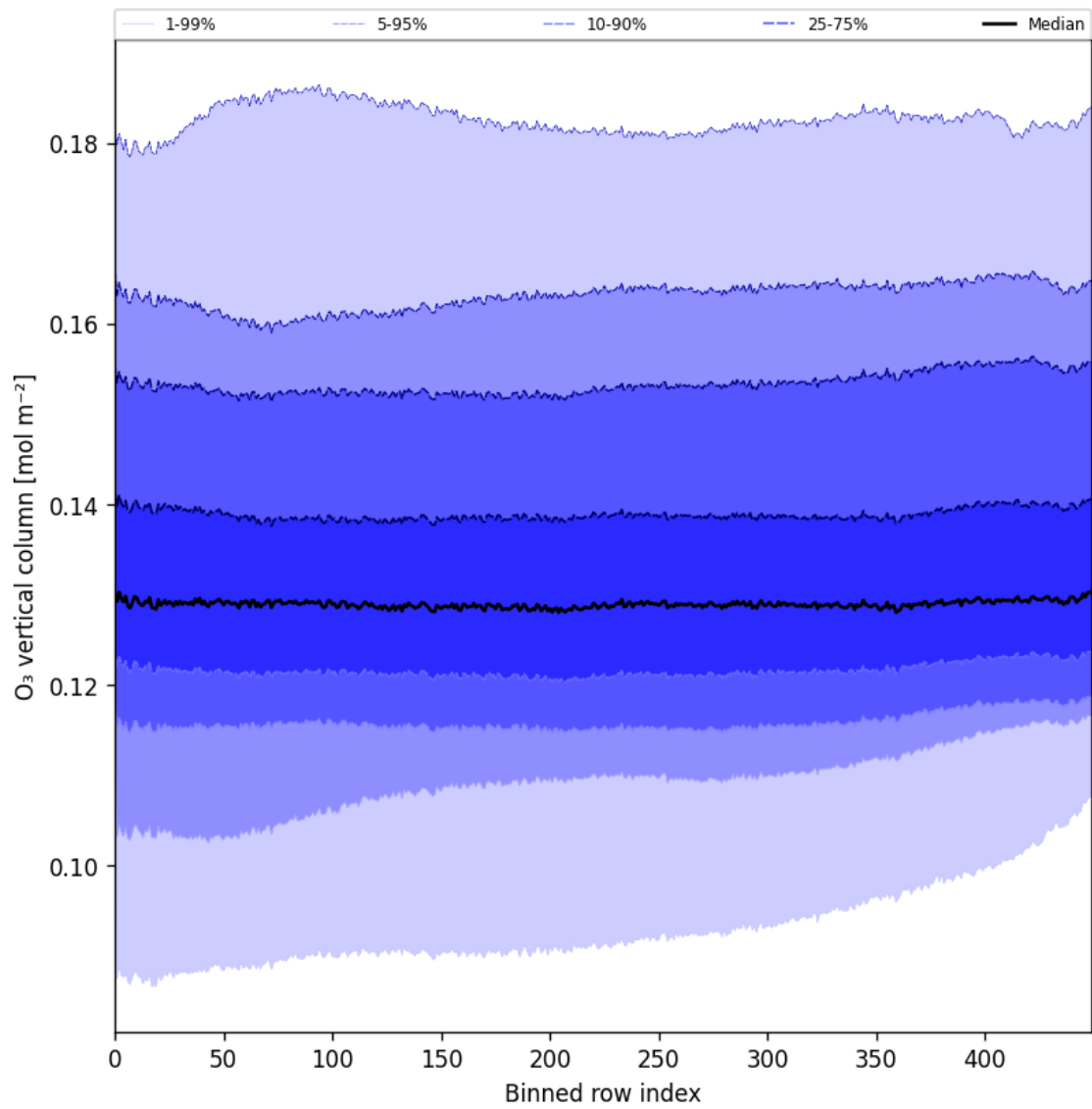
Figure 28: Along track statistics of “O 3 vertical column” for 2025-08-25 to 2025-08-27
