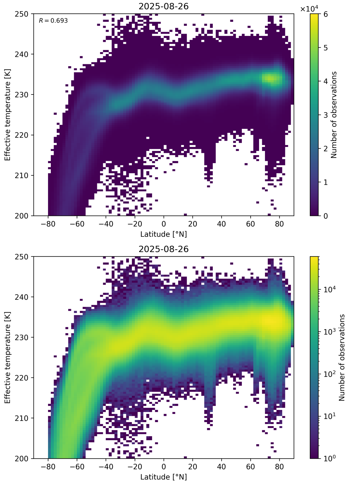
Figure 34: Scatter density plot of “Latitude” against “Effective temperature” for 2025-08-25 to 2025-08-27.
