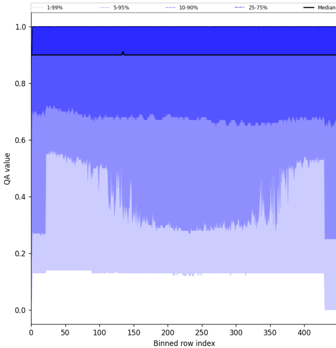
Figure 27: Along track statistics of “QA value” for 2025-08-25 to 2025-08-27
