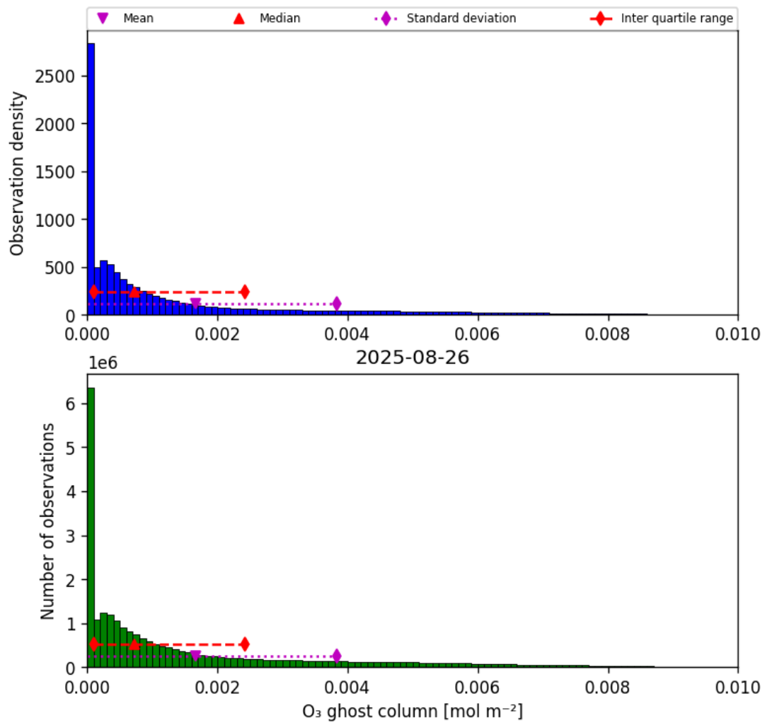
Figure 25: Histogram of "O 3 ghost column" for 2025-08-25 to 2025-08-27
