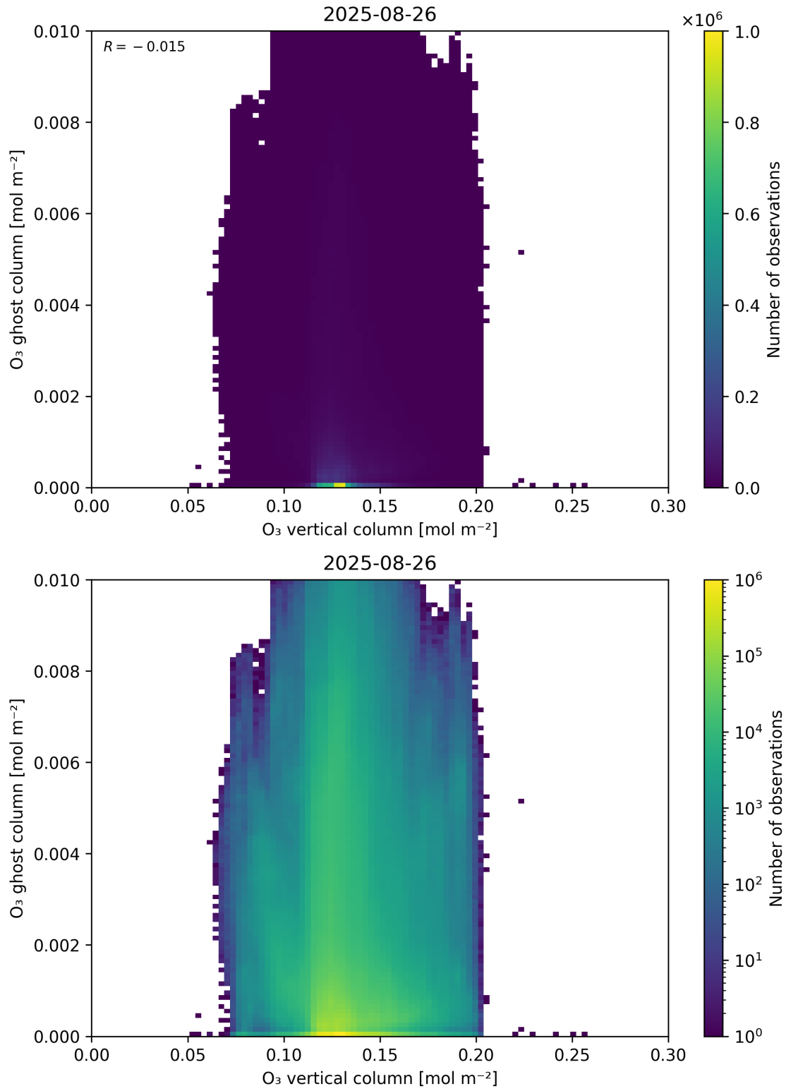
Figure 40: Scatter density plot of “O 3 vertical column” against “O 3 ghost column” for 2025-08-25 to 2025-08-27.
