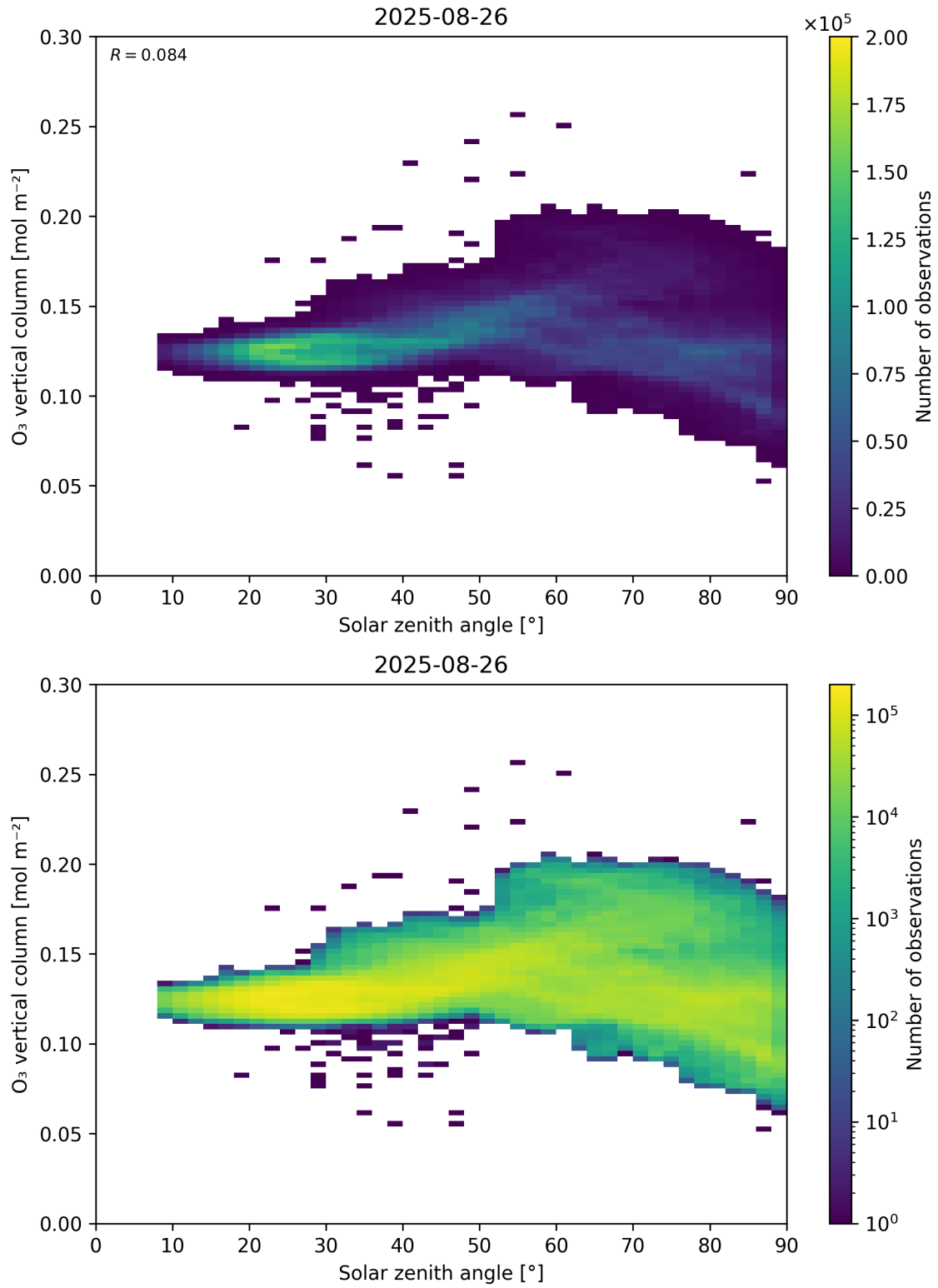
Figure 47: Scatter density plot of “Solar zenith angle” against “O 3 vertical column” for 2025-08-25 to 2025-08-27.
