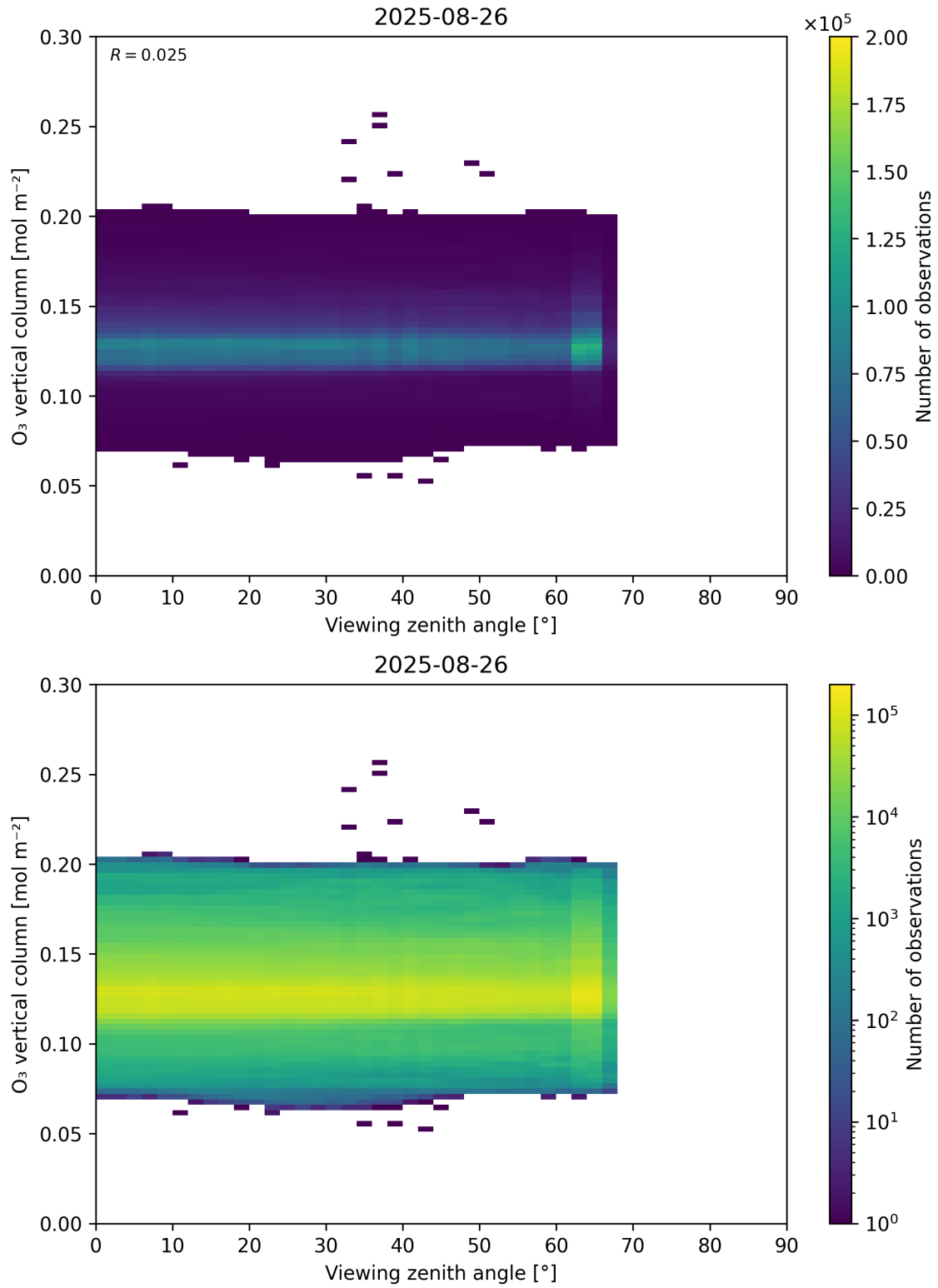
Figure 52: Scatter density plot of “Viewing zenith angle” against “O 3 vertical column” for 2025-08-25 to 2025-08-27.
