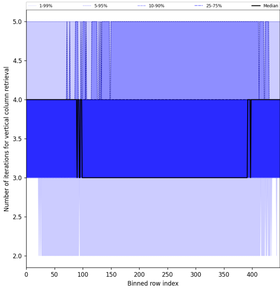
Figure 33: Along track statistics of “Number of iterations for vertical column retrieval” for 2025-08-25 to 2025-08-27
