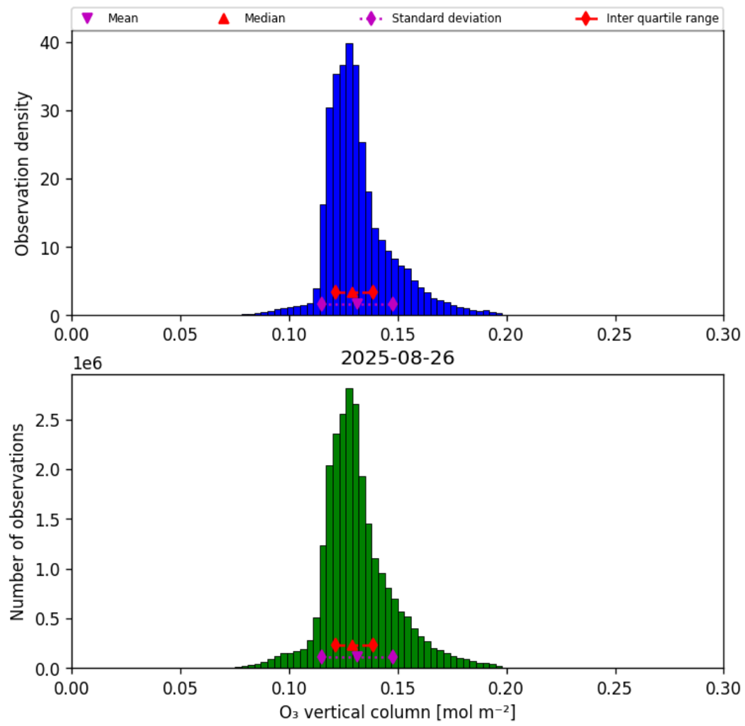
Figure 21: Histogram of “O 3 vertical column” for 2025-08-25 to 2025-08-27
