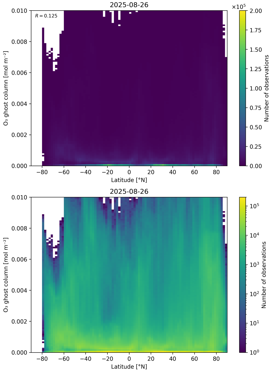
Figure 35: Scatter density plot of “Latitude” against “O 3 ghost column” for 2025-08-25 to 2025-08-27.
