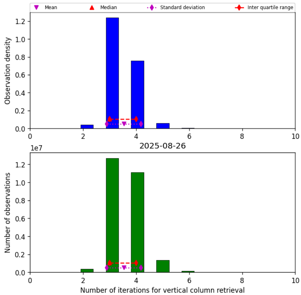
Figure 26: Histogram of “Number of iterations for vertical column retrieval” for 2025-08-25 to 2025-08-27
