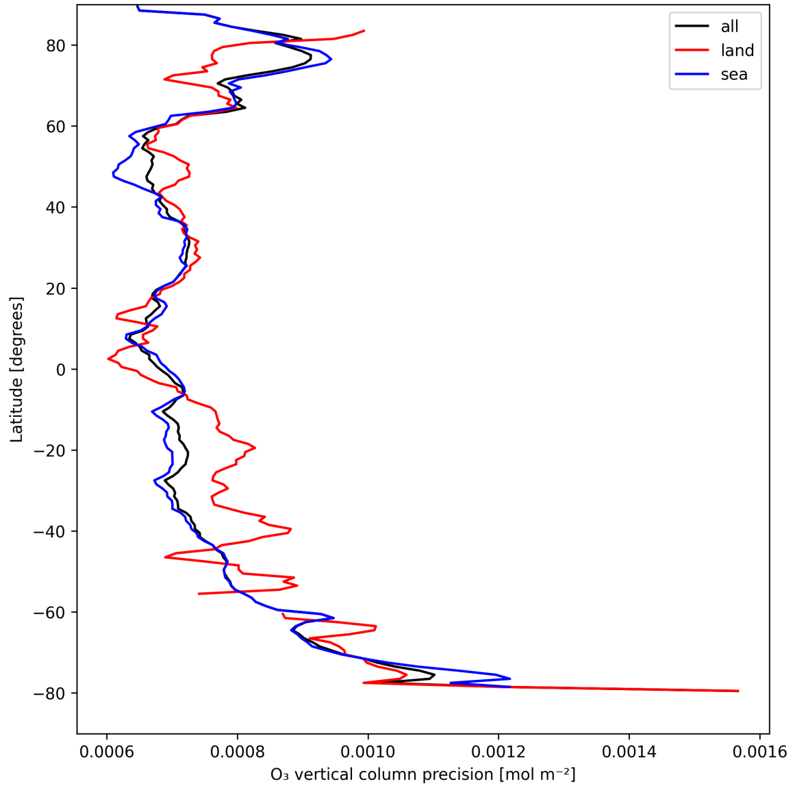
Figure 15: Zonal average of "O 3 vertical column precision" for 2025-08-26 to 2025-08-28.
