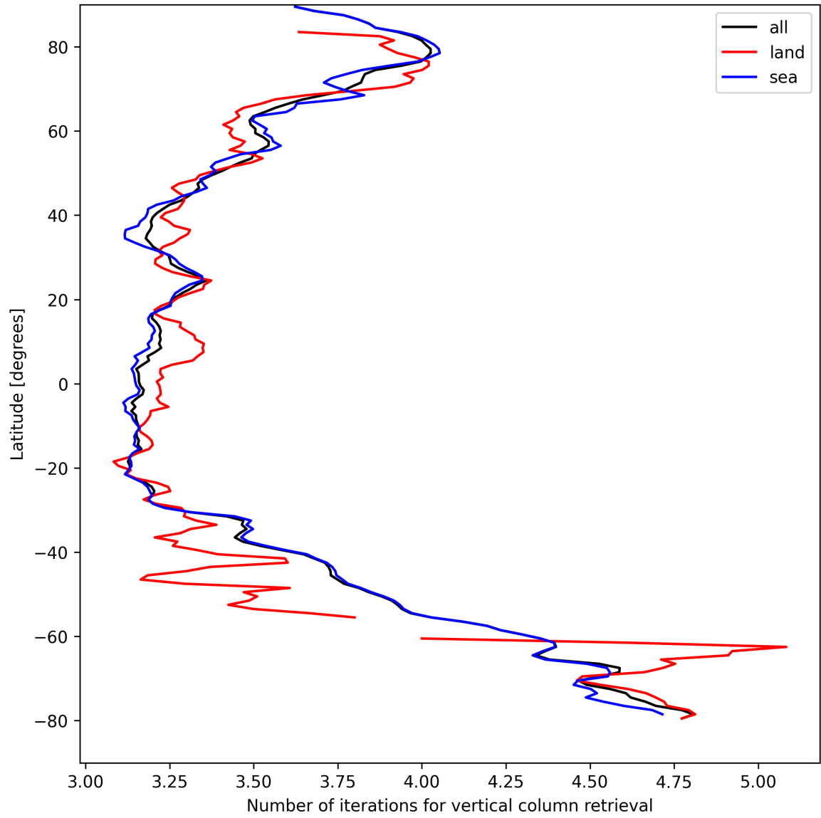
Figure 19: Zonal average of “Number of iterations for vertical column retrieval” for 2025-08-26 to 2025-08-28.
