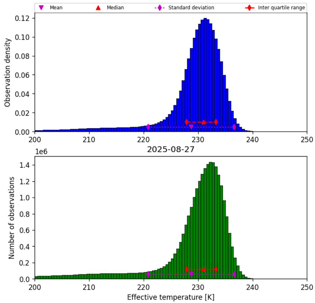
Figure 24: Histogram of “Effective temperature” for 2025-08-26 to 2025-08-28
