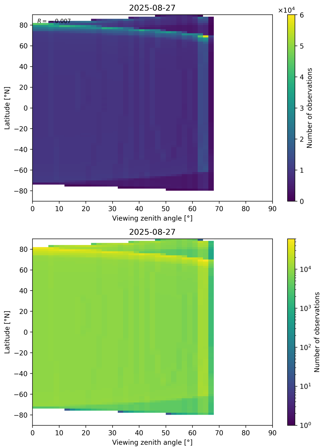
Figure 49: Scatter density plot of “Viewing zenith angle” against “Latitude” for 2025-08-26 to 2025-08-28.
