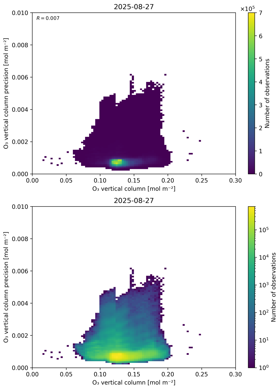
Figure 41: Scatter density plot of “O 3 vertical column” against “O 3 vertical column precision” for 2025-08-26 to 2025-08-28.
