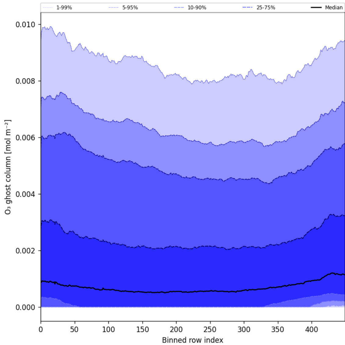
Figure 32: Along track statistics of “O 3 ghost column” for 2025-08-26 to 2025-08-28
