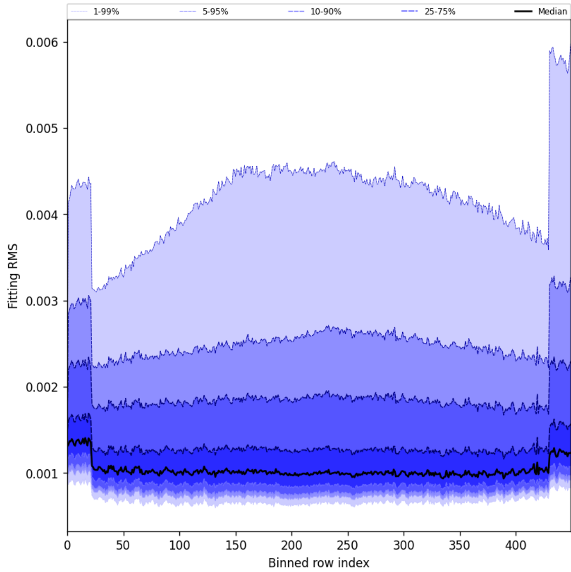
Figure 30: Along track statistics of “Fitting RMS” for 2025-08-26 to 2025-08-28
