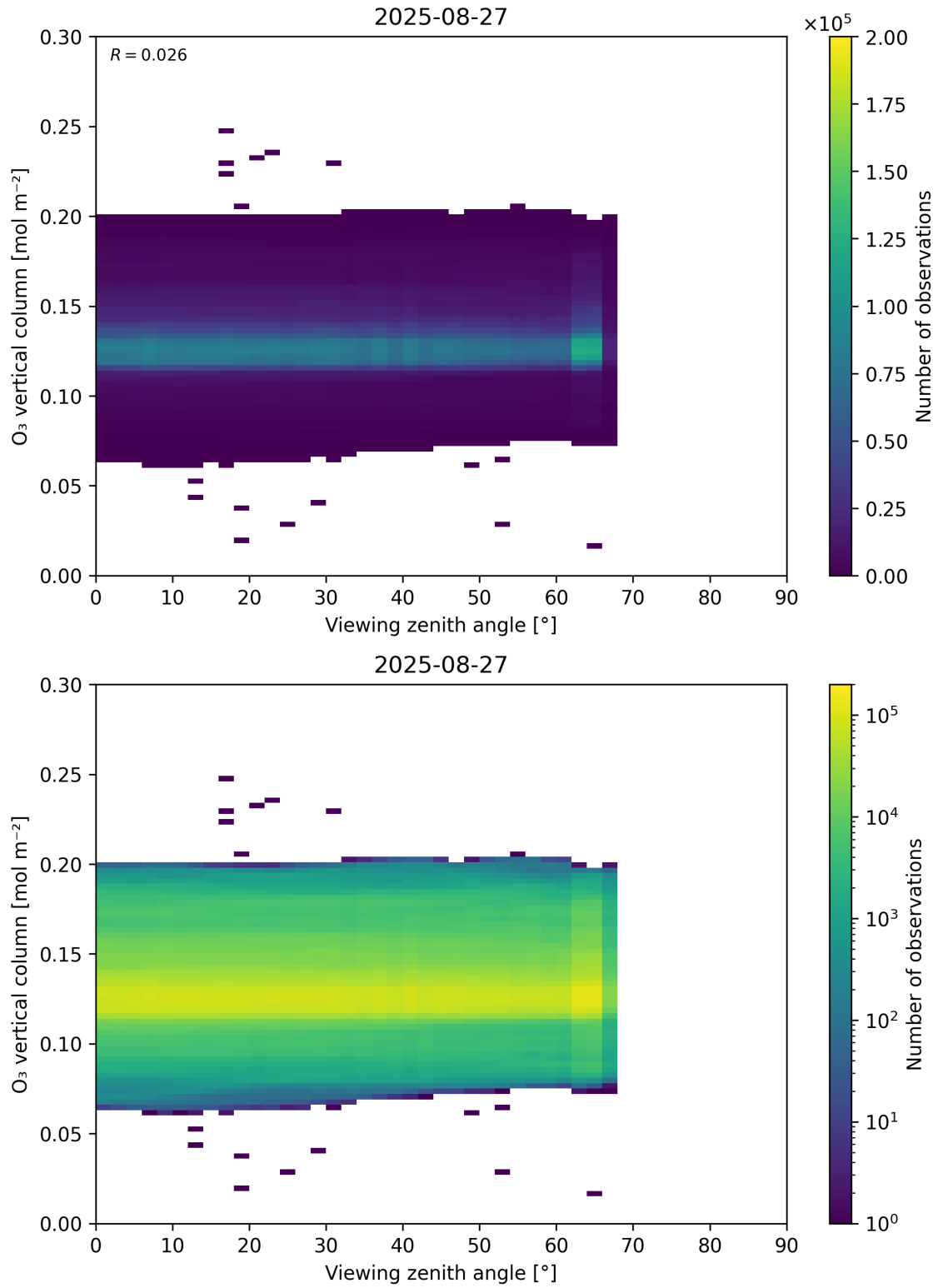
Figure 52: Scatter density plot of “Viewing zenith angle” against “O 3 vertical column” for 2025-08-26 to 2025-08-28.
