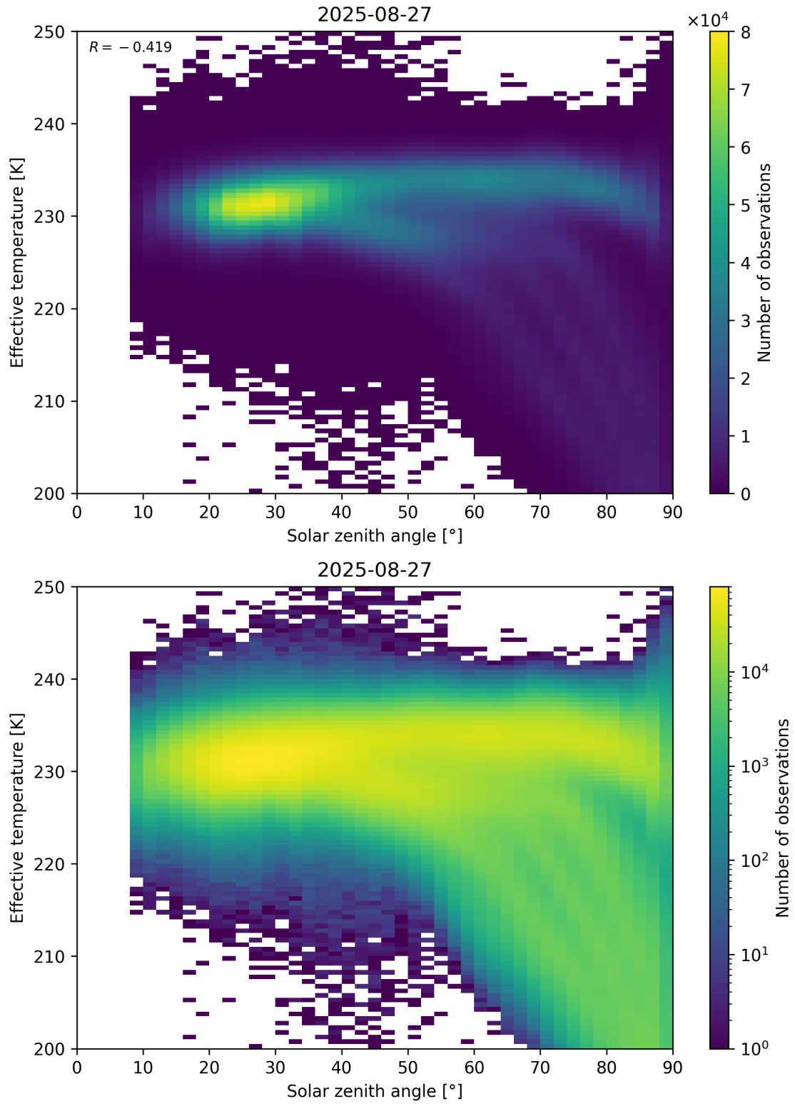
Figure 45: Scatter density plot of “Solar zenith angle” against “Effective temperature” for 2025-08-26 to 2025-08-28.
