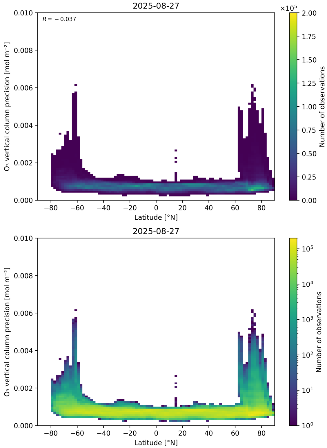
Figure 37: Scatter density plot of “Latitude” against “O 3 vertical column precision” for 2025-08-26 to 2025-08-28.
