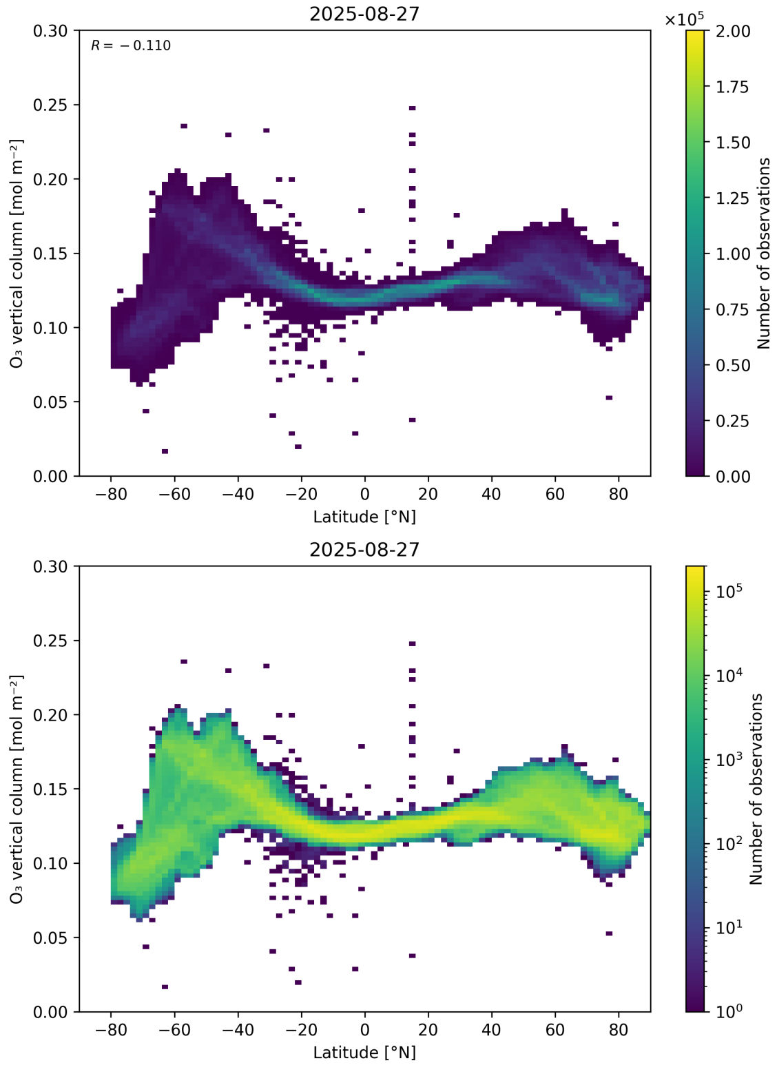
Figure 36: Scatter density plot of “Latitude” against “O 3 vertical column” for 2025-08-26 to 2025-08-28.
