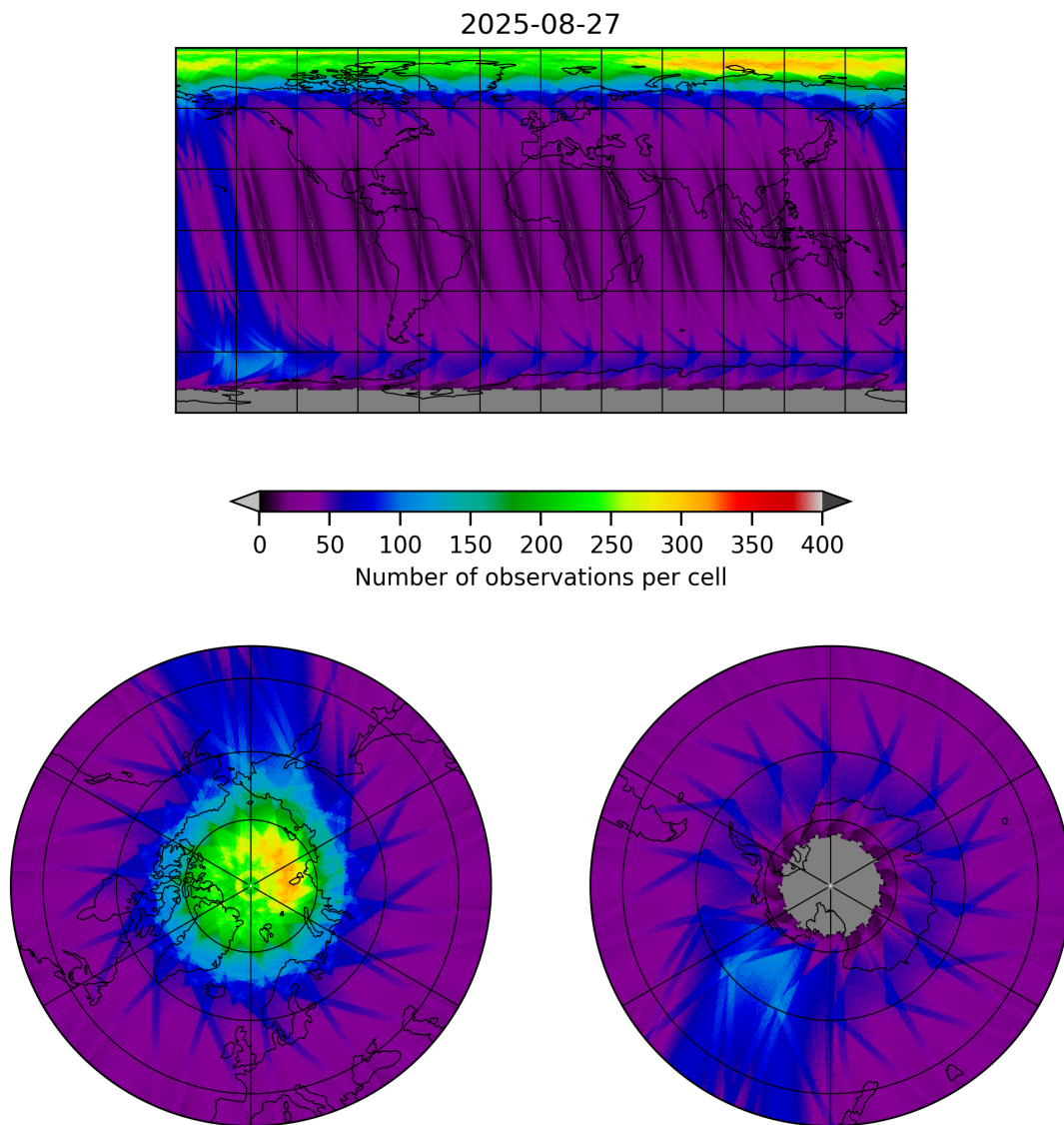
Figure 12: Map of the number of observations for 2025-08-26 to 2025-08-28
