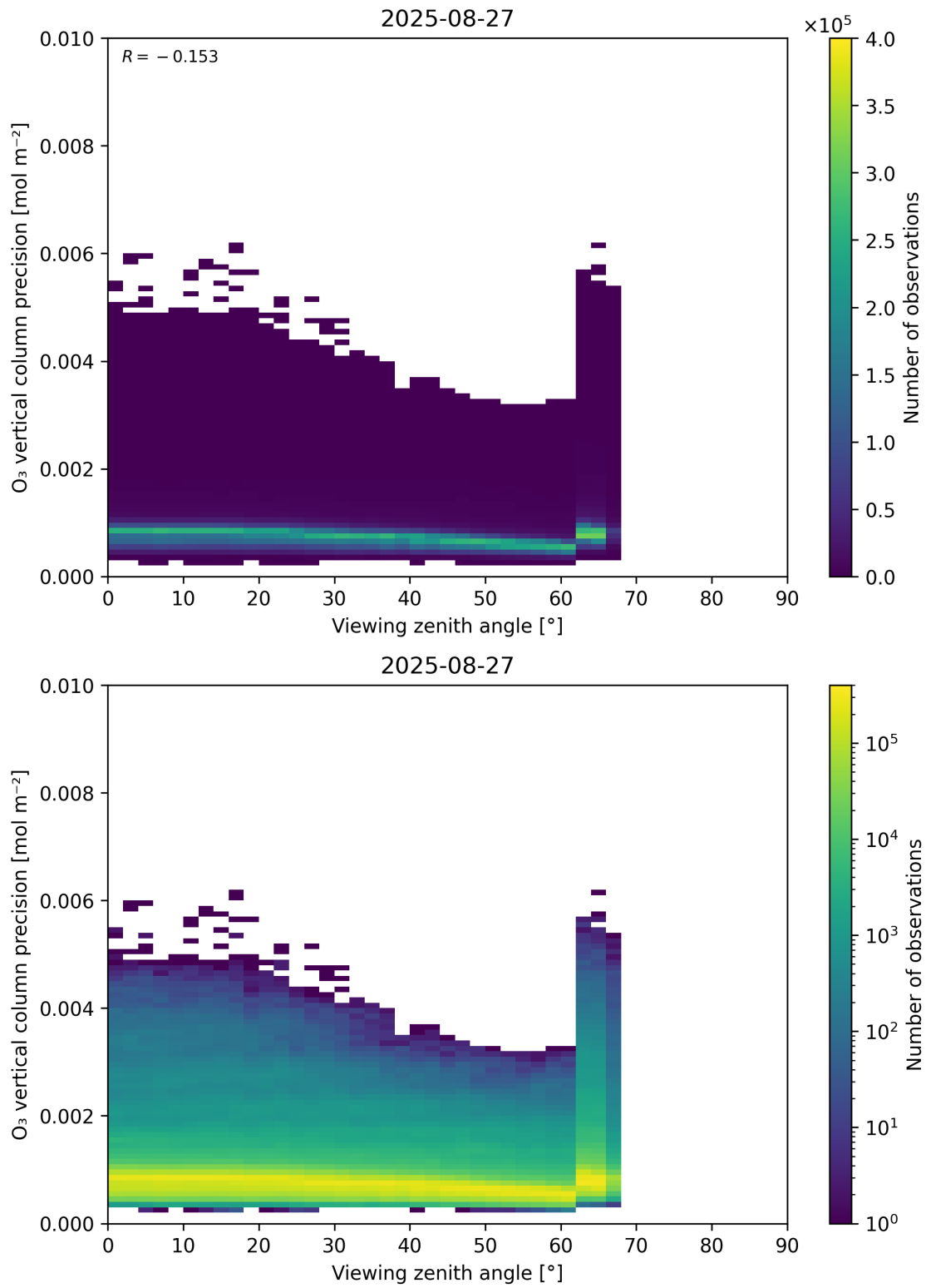
Figure 53: Scatter density plot of “Viewing zenith angle” against “O 3 vertical column precision” for 2025-08-26 to 2025-08-28.
