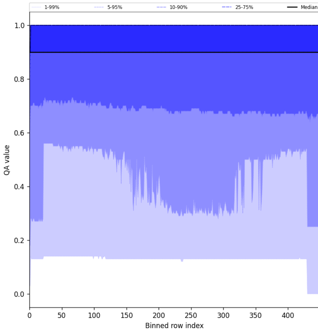
Figure 27: Along track statistics of “QA value” for 2025-08-26 to 2025-08-28
