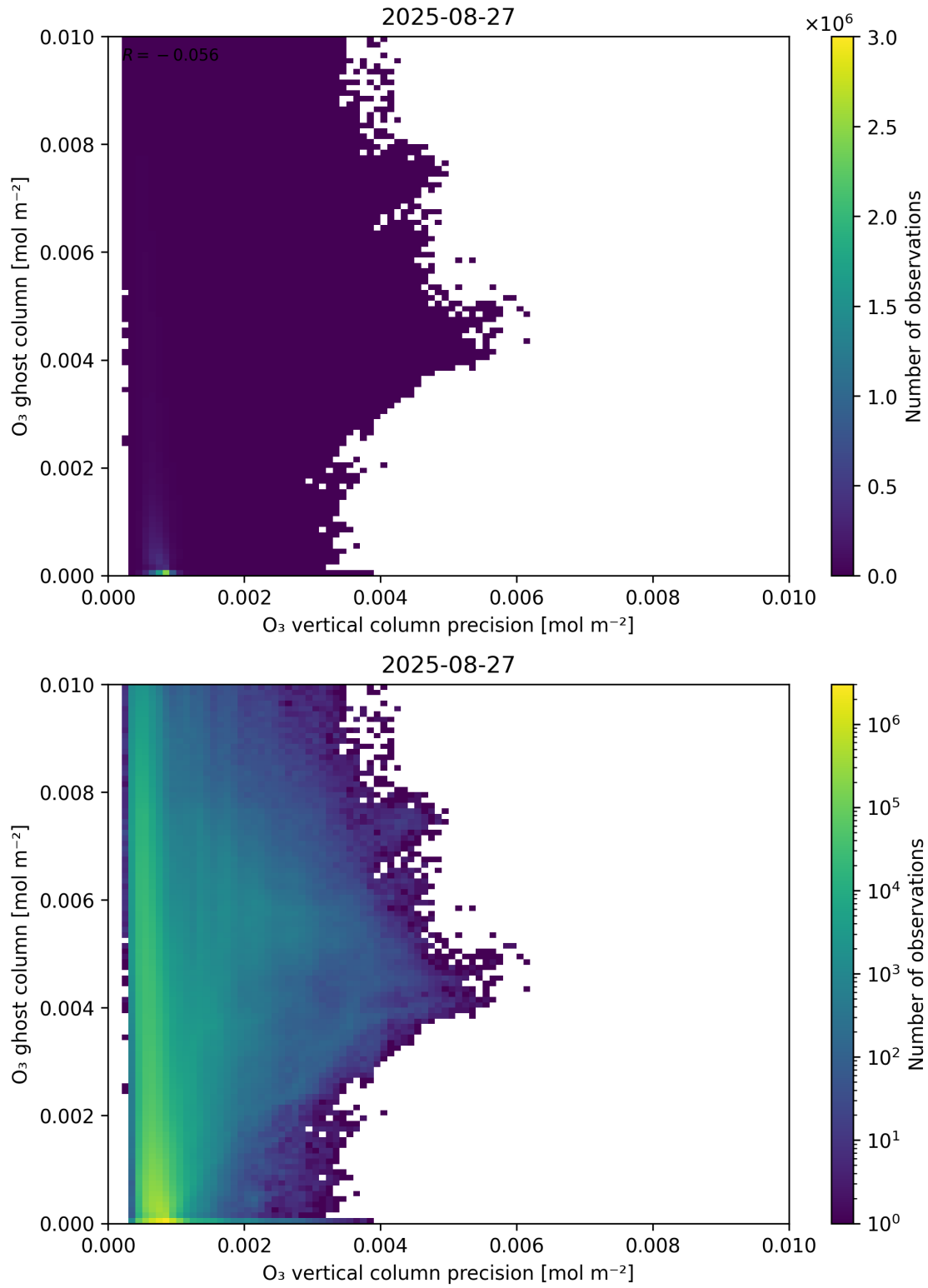
Figure 43: Scatter density plot of “ O_3 vertical column precision” against “ O_3 ghost column” for 2025-08-26 to 2025-08-28.
