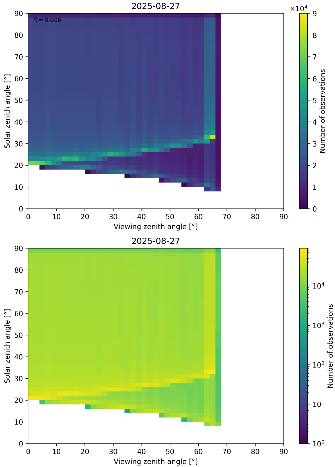
Figure 54: Scatter density plot of “Viewing zenith angle” against “Solar zenith angle” for 2025-08-26 to 2025-08-28.
