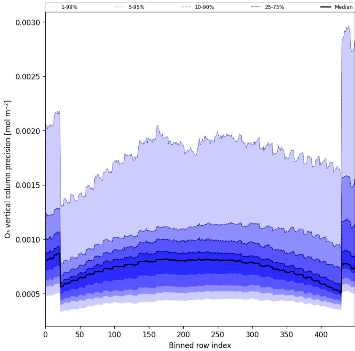
Figure 29: Along track statistics of “O 3 vertical column precision” for 2025-08-26 to 2025-08-28
