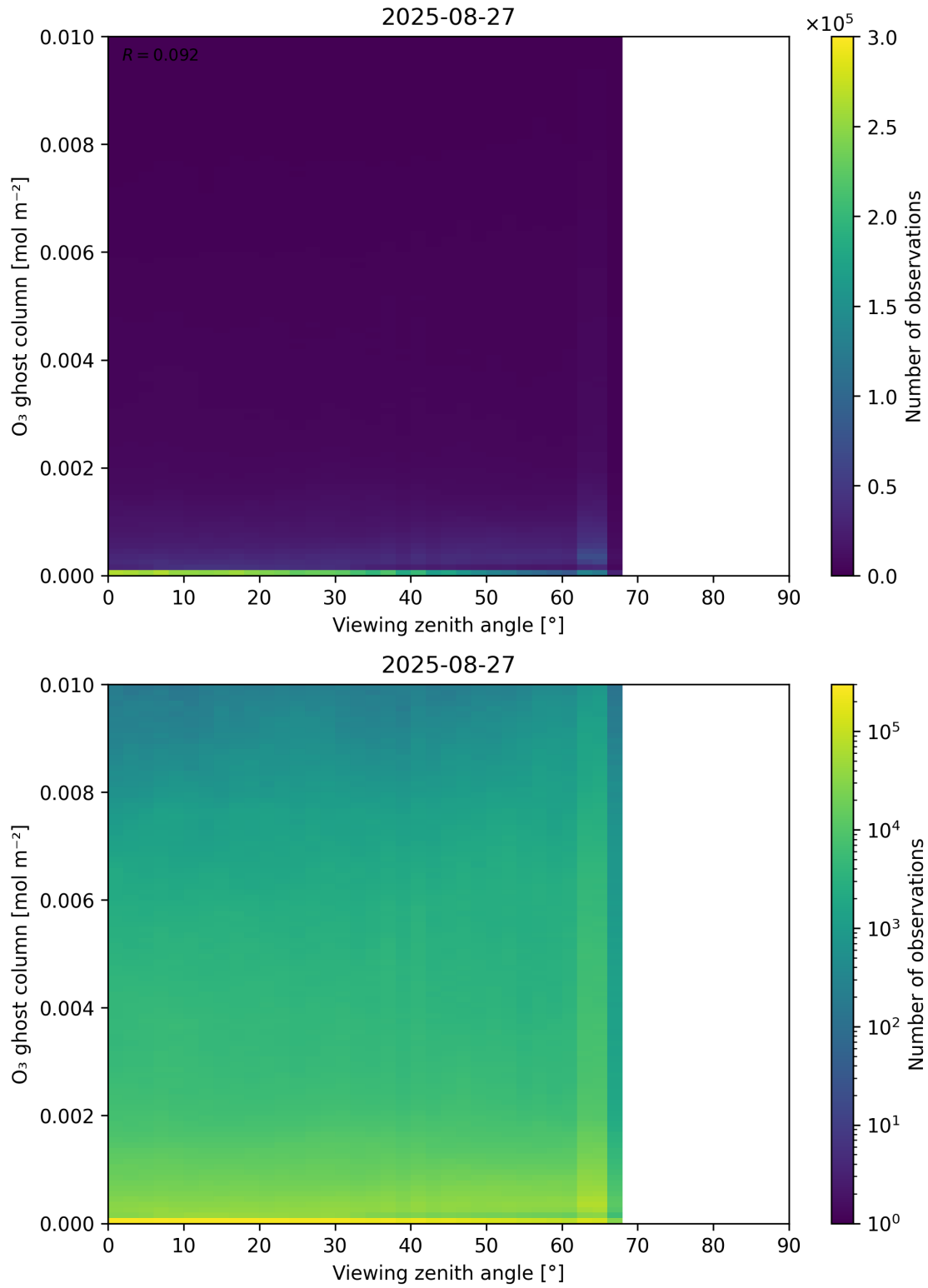
Figure 51: Scatter density plot of “Viewing zenith angle” against “O 3 ghost column” for 2025-08-26 to 2025-08-28.
