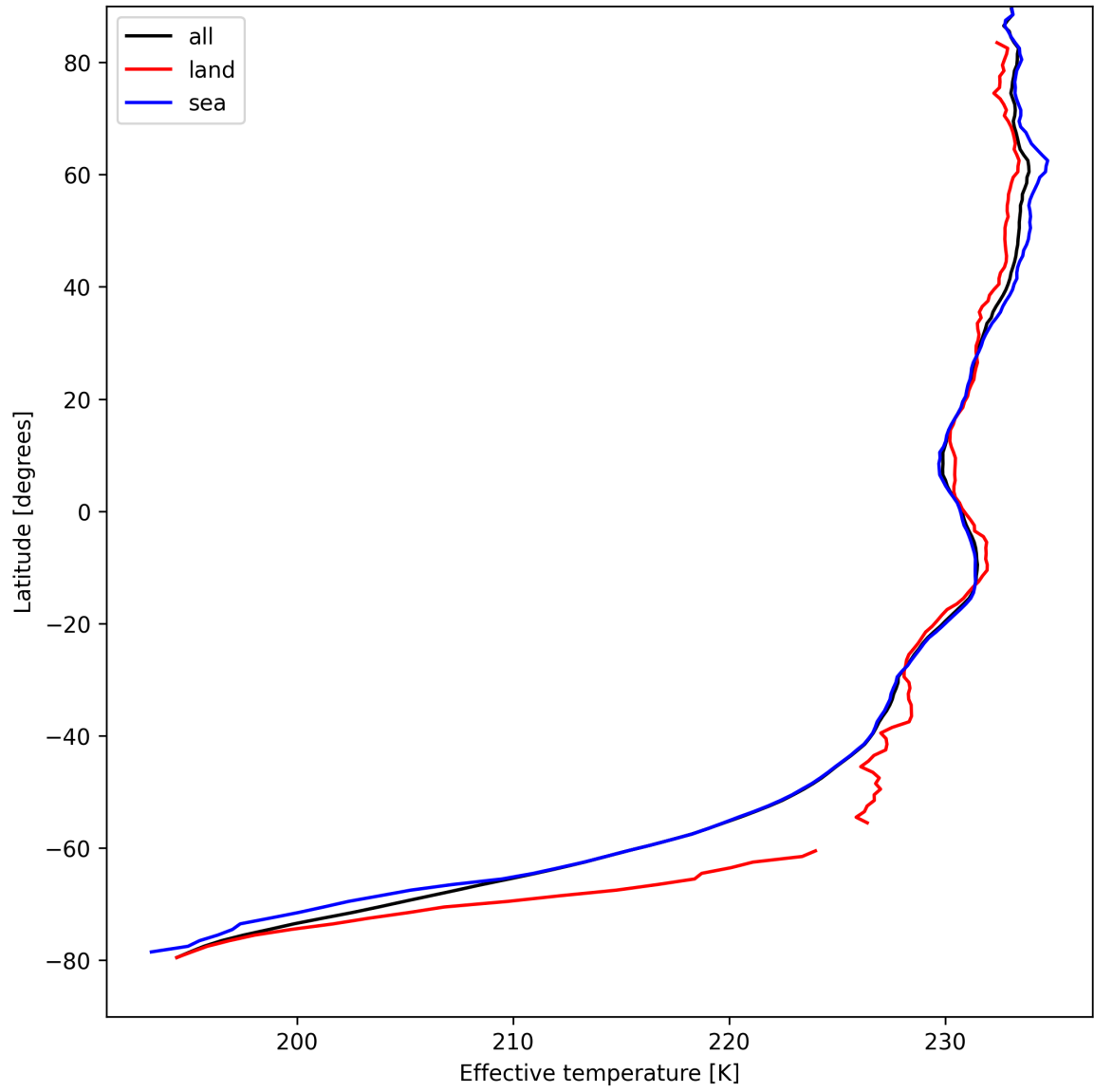
Figure 17: Zonal average of "Effective temperature" for 2025-08-26 to 2025-08-28.
