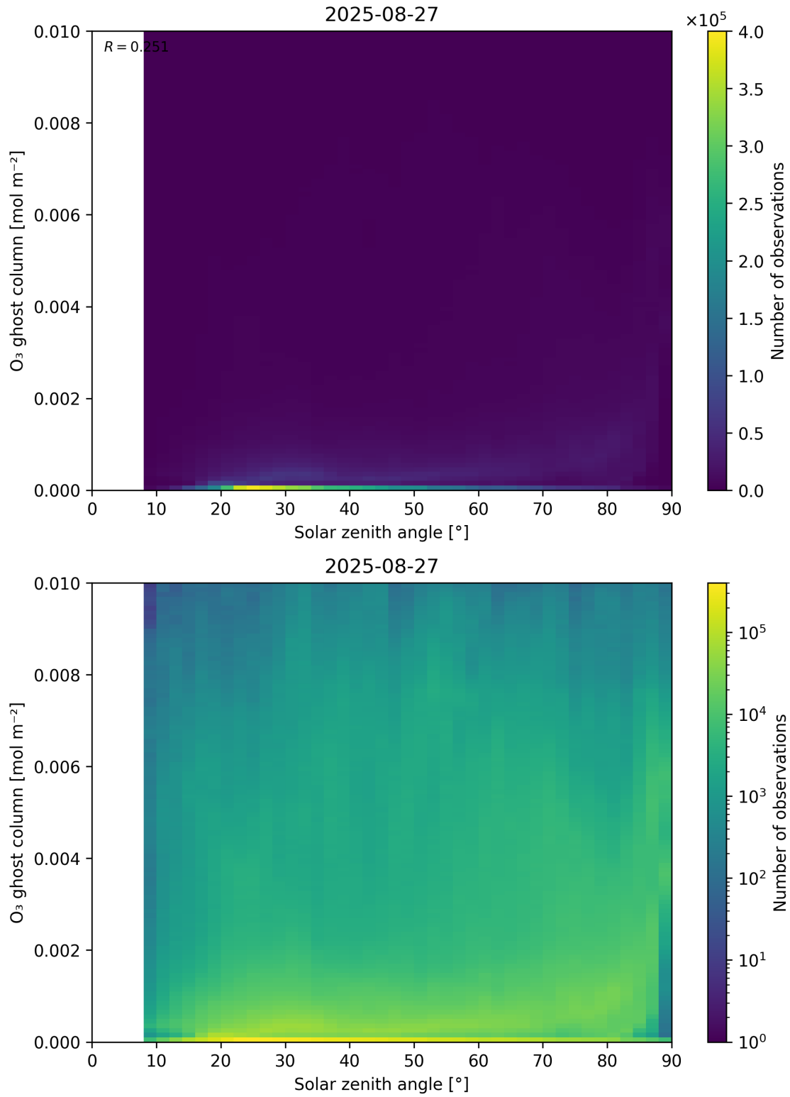
Figure 46: Scatter density plot of “Solar zenith angle” against “O 3 ghost column” for 2025-08-26 to 2025-08-28.
