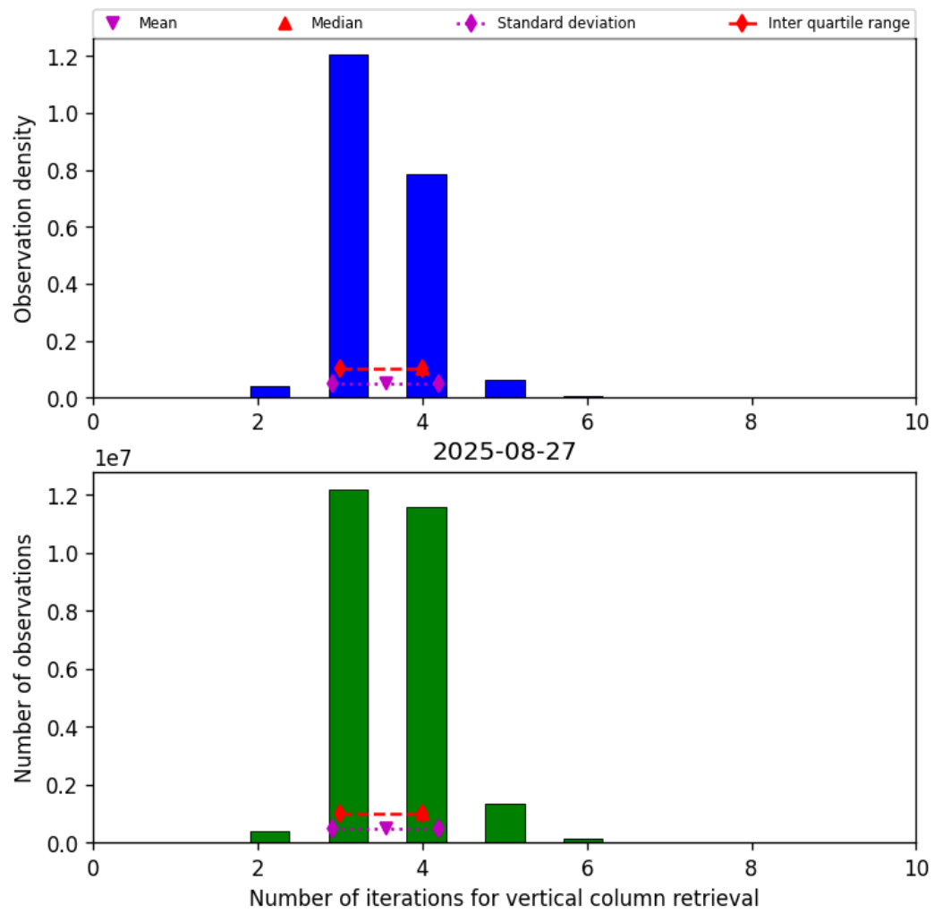
Figure 26: Histogram of “Number of iterations for vertical column retrieval” for 2025-08-26 to 2025-08-28
