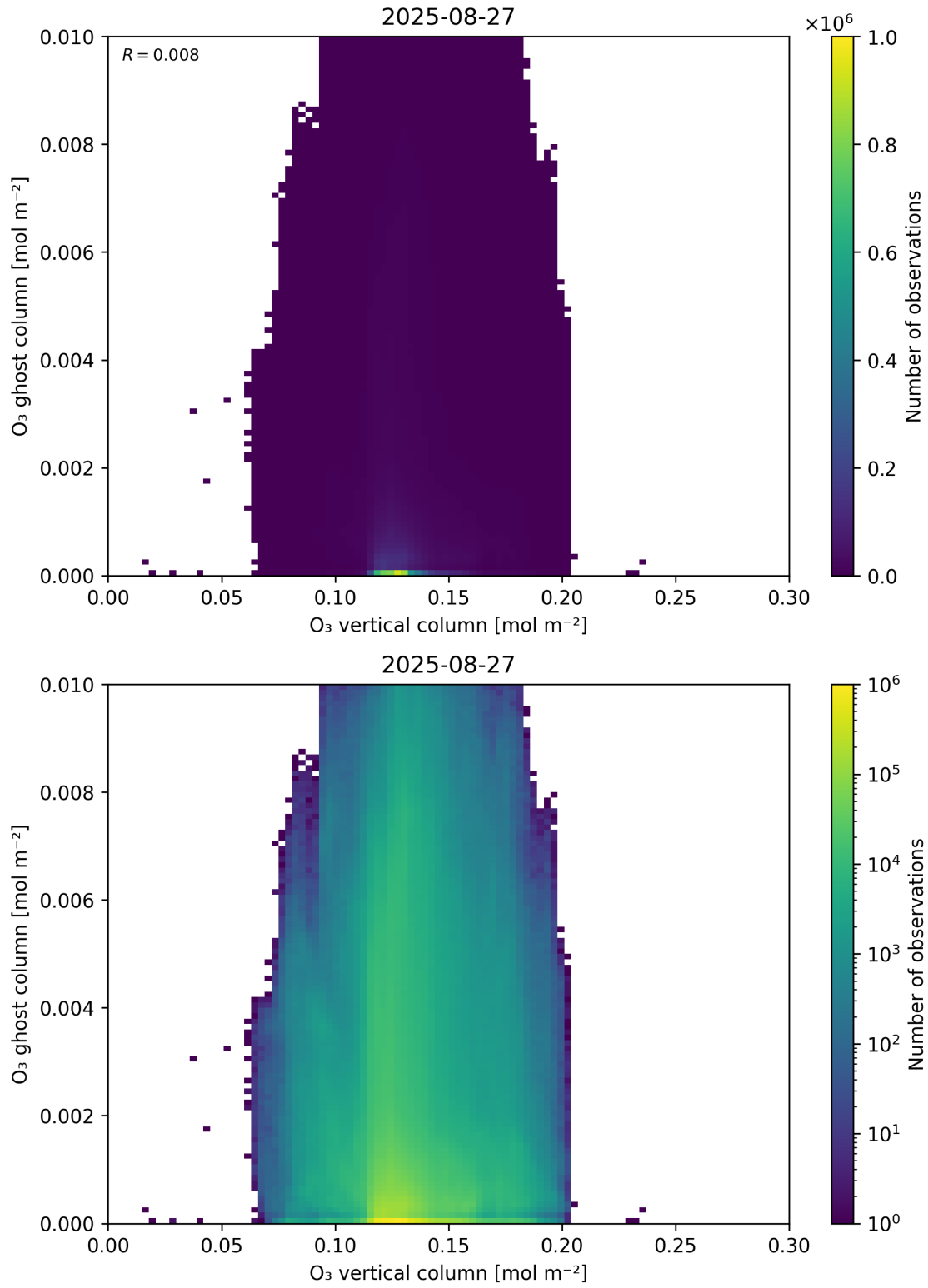
Figure 40: Scatter density plot of “O 3 vertical column” against “O 3 ghost column” for 2025-08-26 to 2025-08-28.
