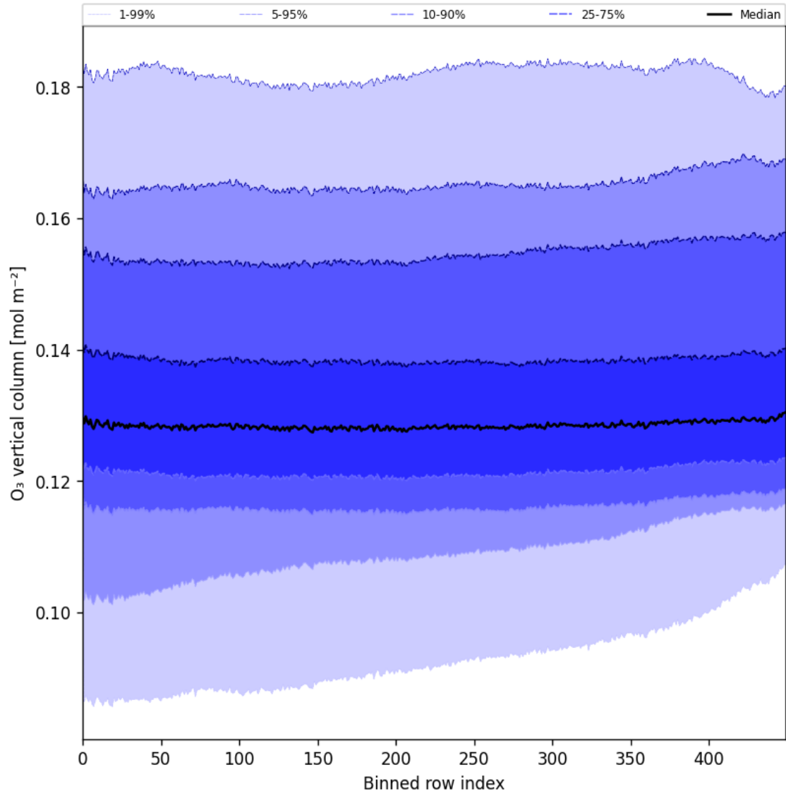
Figure 28: Along track statistics of “O 3 vertical column” for 2025-08-26 to 2025-08-28
