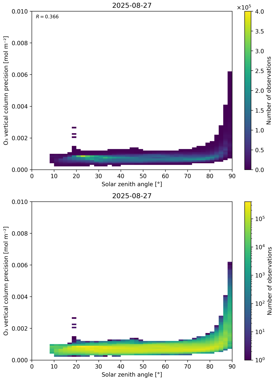
Figure 48: Scatter density plot of “Solar zenith angle” against “O 3 vertical column precision” for 2025-08-26 to 2025-08-28.
