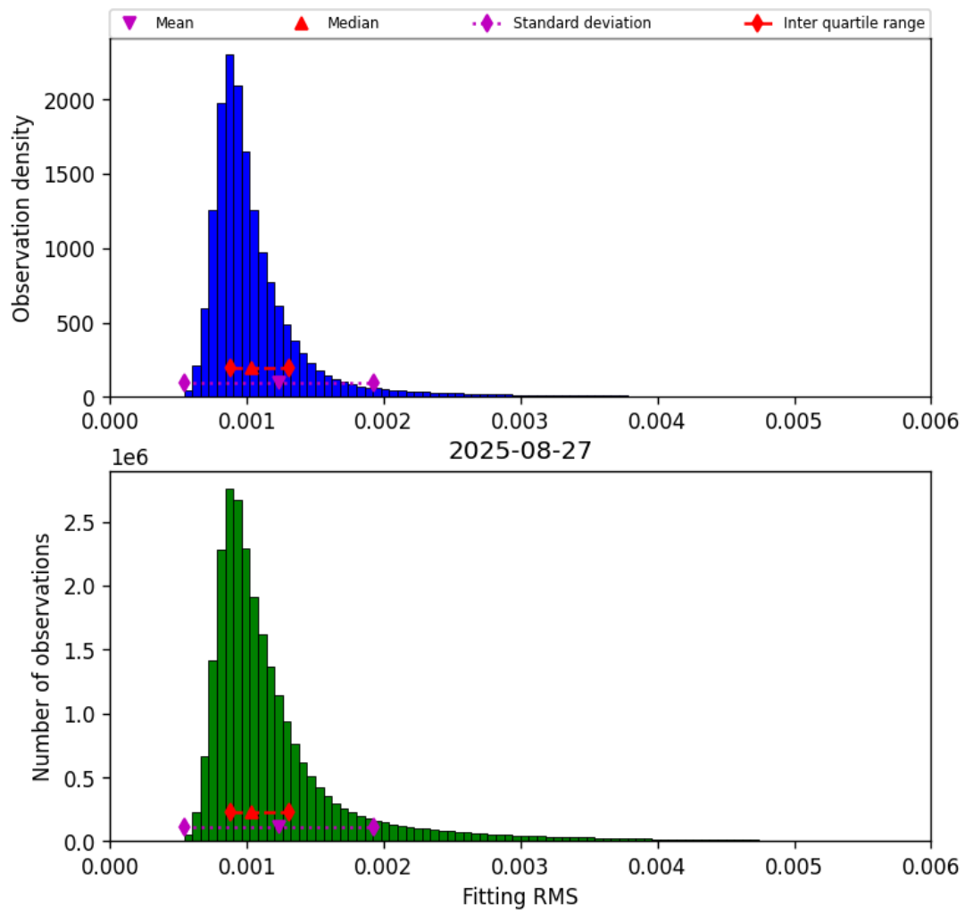
Figure 23: Histogram of “Fitting RMS” for 2025-08-26 to 2025-08-28
