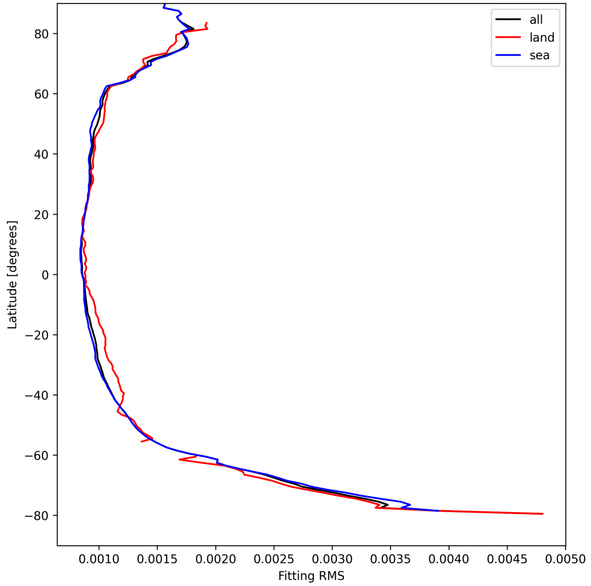
Figure 16: Zonal average of “Fitting RMS” for 2025-08-26 to 2025-08-28.
