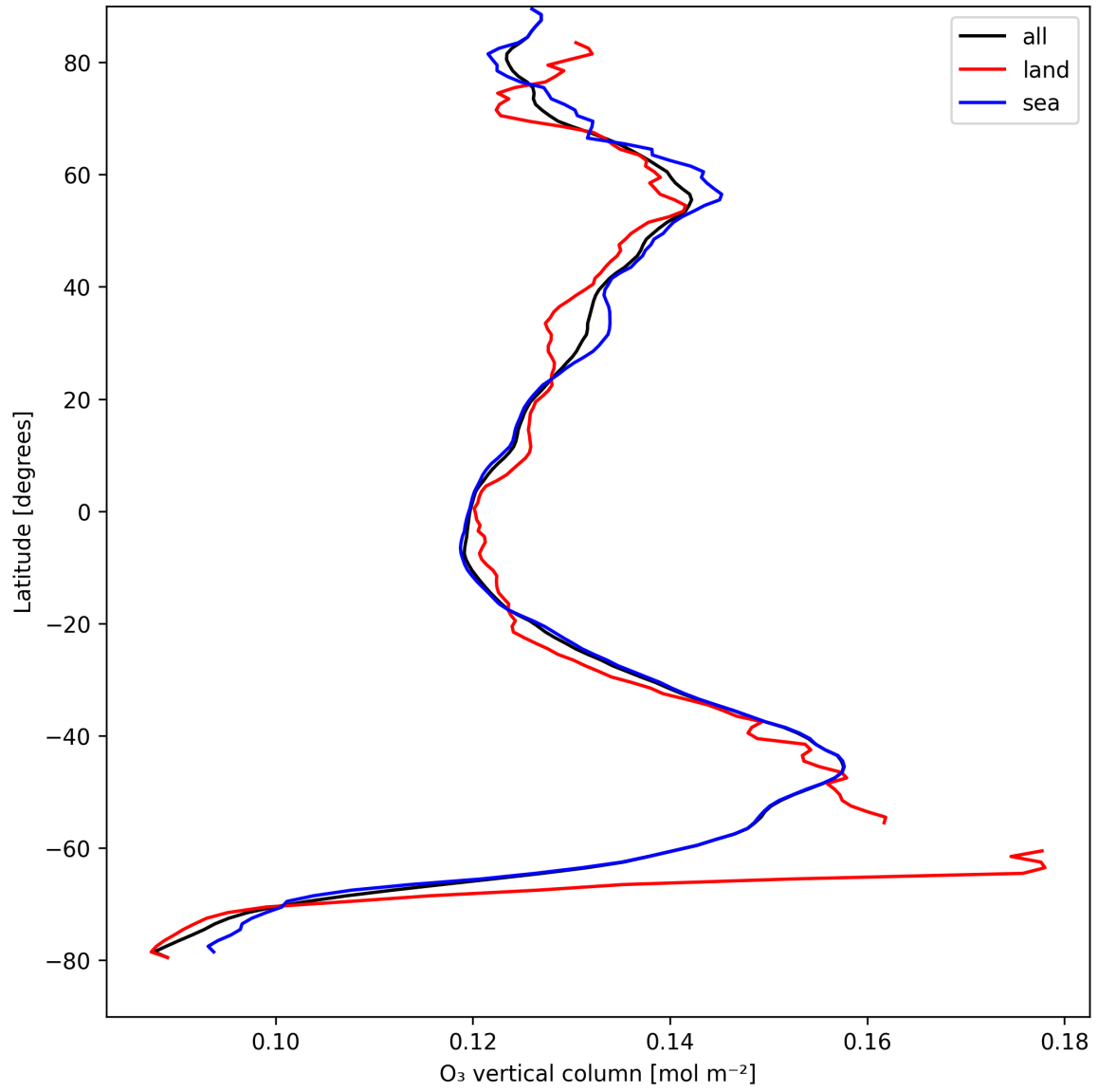
Figure 14: Zonal average of “O 3 vertical column” for 2025-08-26 to 2025-08-28.
