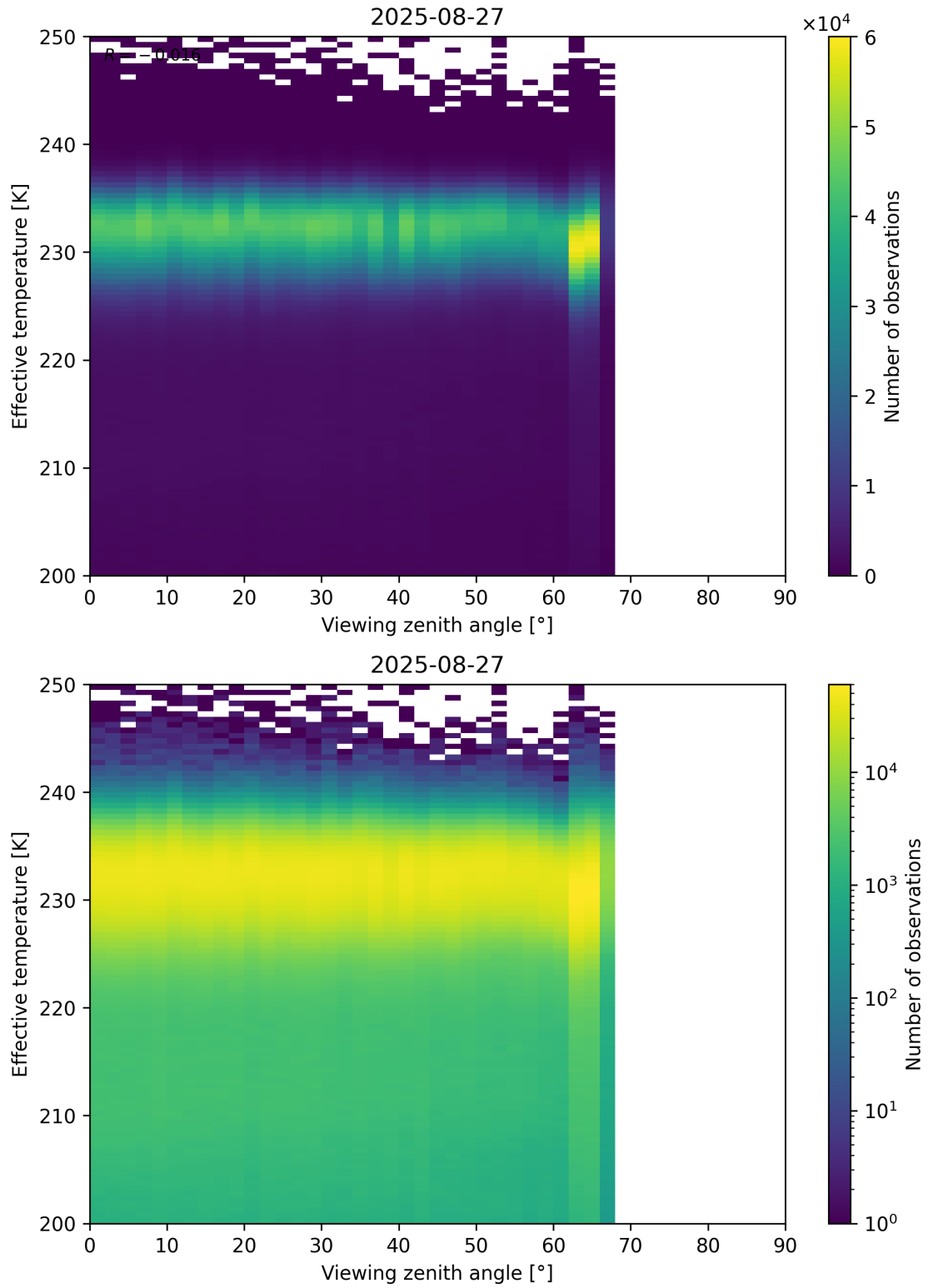
Figure 50: Scatter density plot of “Viewing zenith angle” against “Effective temperature” for 2025-08-26 to 2025-08-28.
