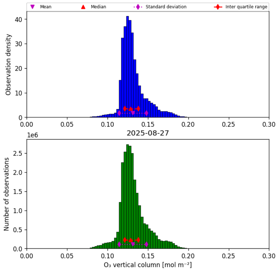
Figure 21: Histogram of “O 3 vertical column” for 2025-08-26 to 2025-08-28
