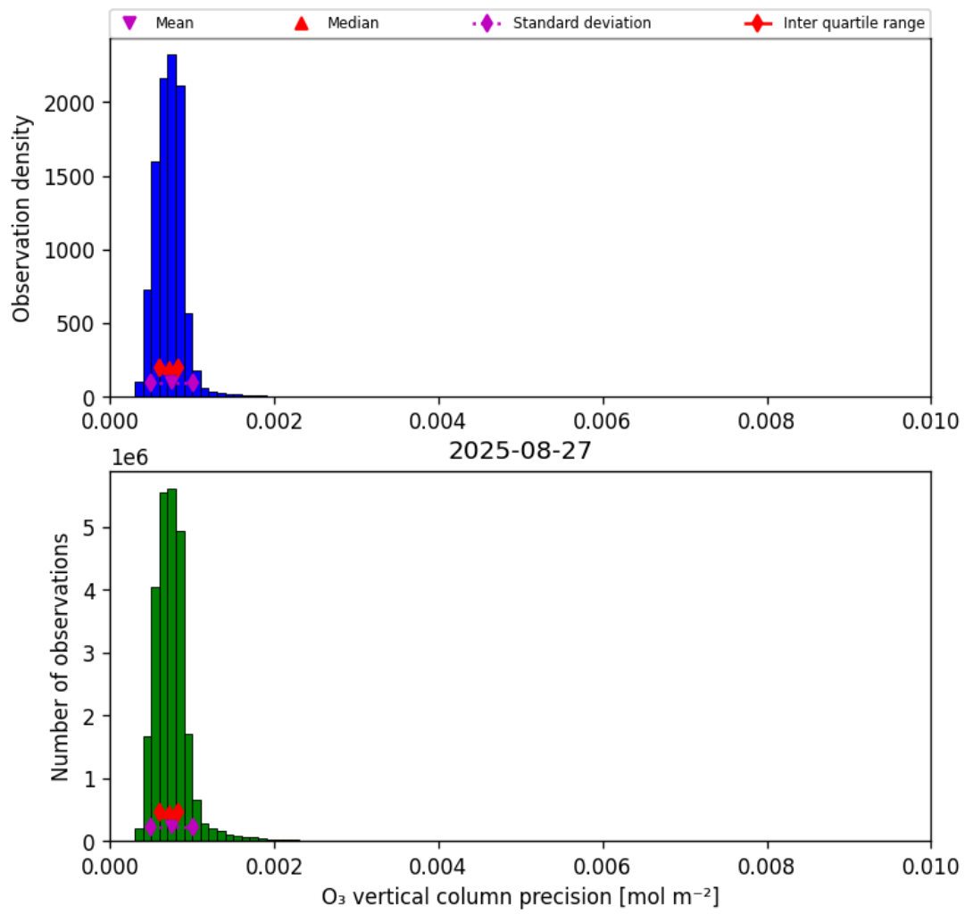
Figure 22: Histogram of “O 3 vertical column precision” for 2025-08-26 to 2025-08-28
