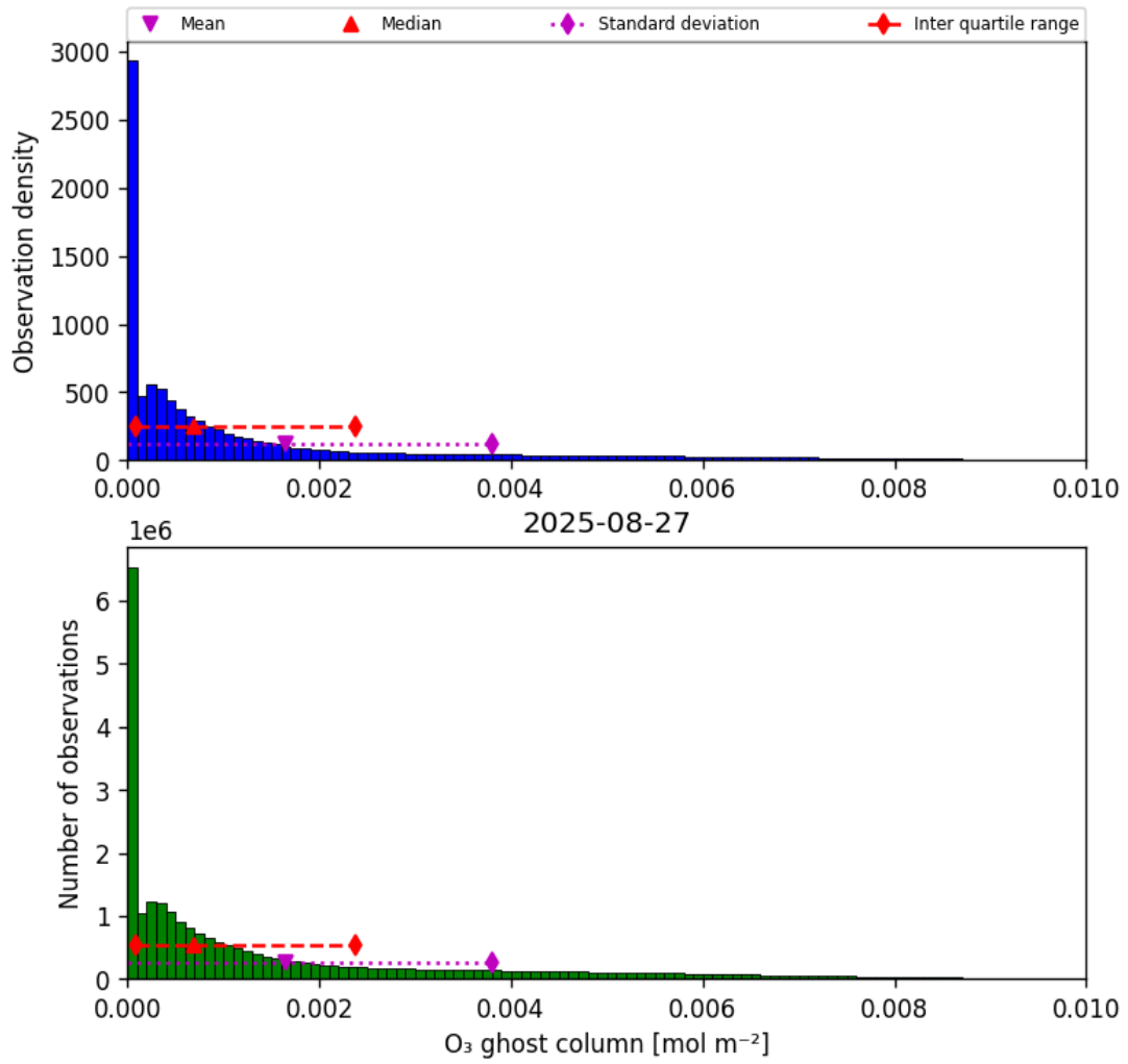
Figure 25: Histogram of "O 3 ghost column" for 2025-08-26 to 2025-08-28
