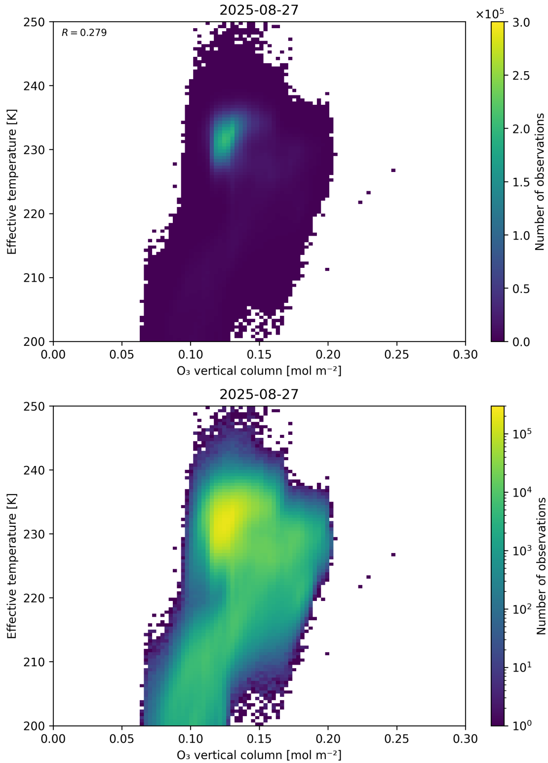
Figure 39: Scatter density plot of “O 3 vertical column” against “Effective temperature” for 2025-08-26 to 2025-08-28.
