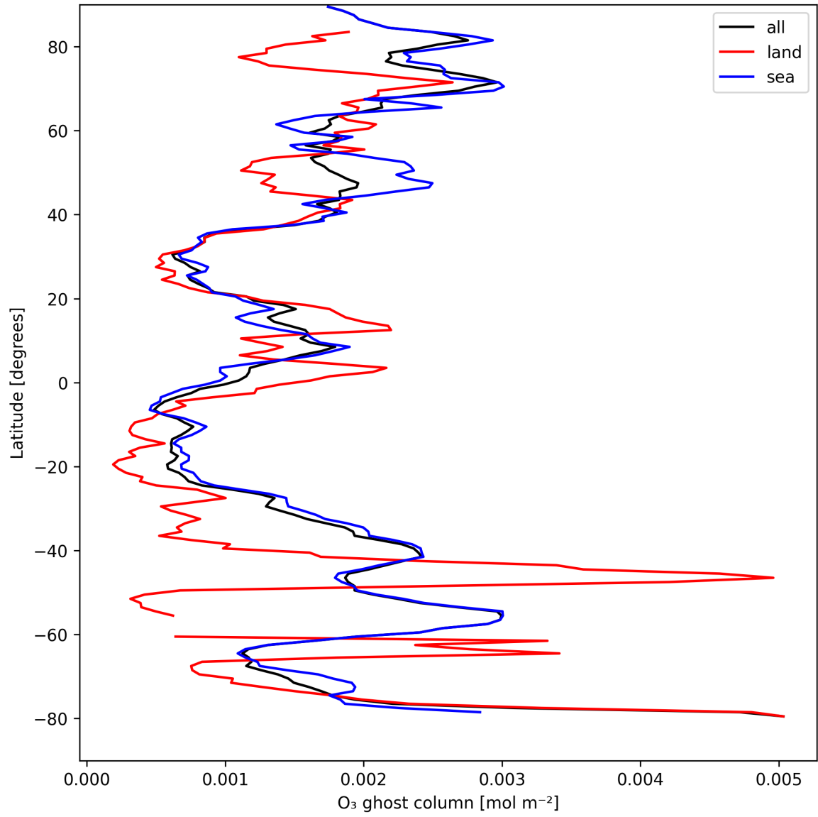
Figure 18: Zonal average of “O 3 ghost column” for 2025-08-26 to 2025-08-28.
