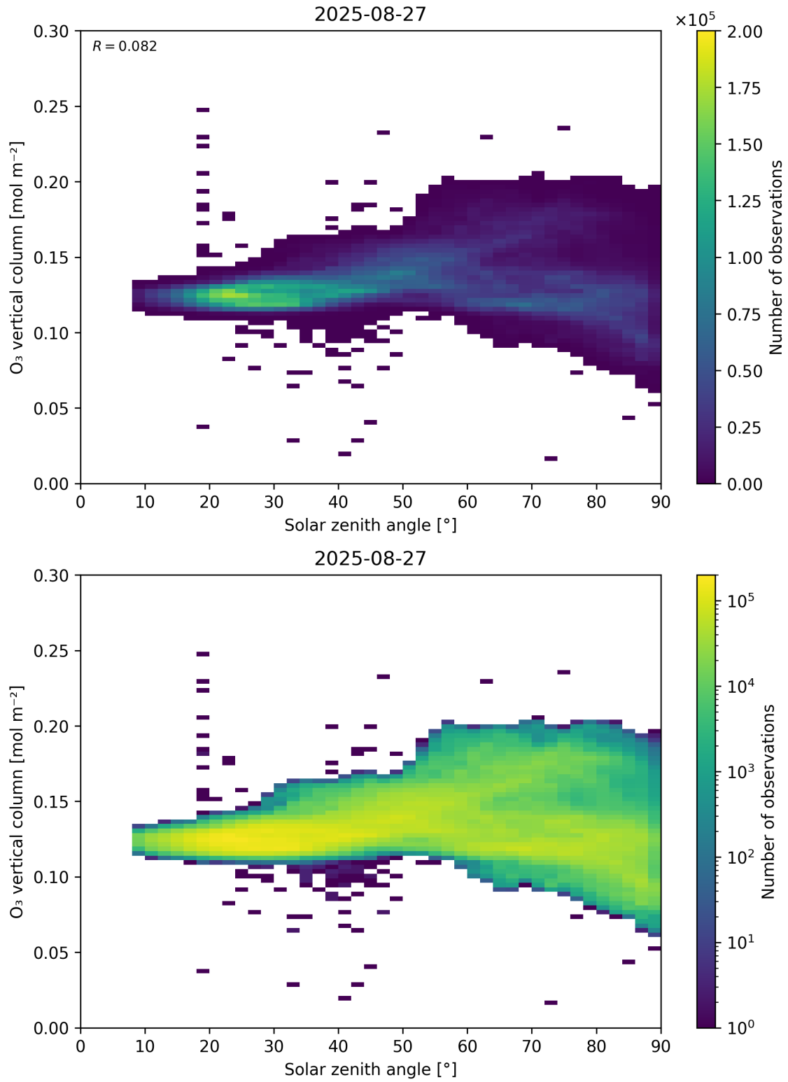
Figure 47: Scatter density plot of “Solar zenith angle” against “O 3 vertical column” for 2025-08-26 to 2025-08-28.
