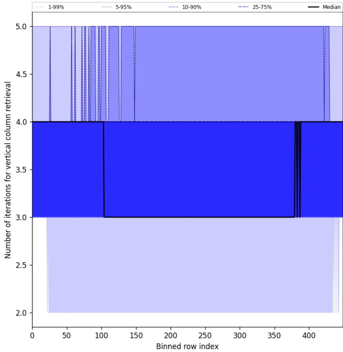
Figure 33: Along track statistics of “Number of iterations for vertical column retrieval” for 2025-08-26 to 2025-08-28
