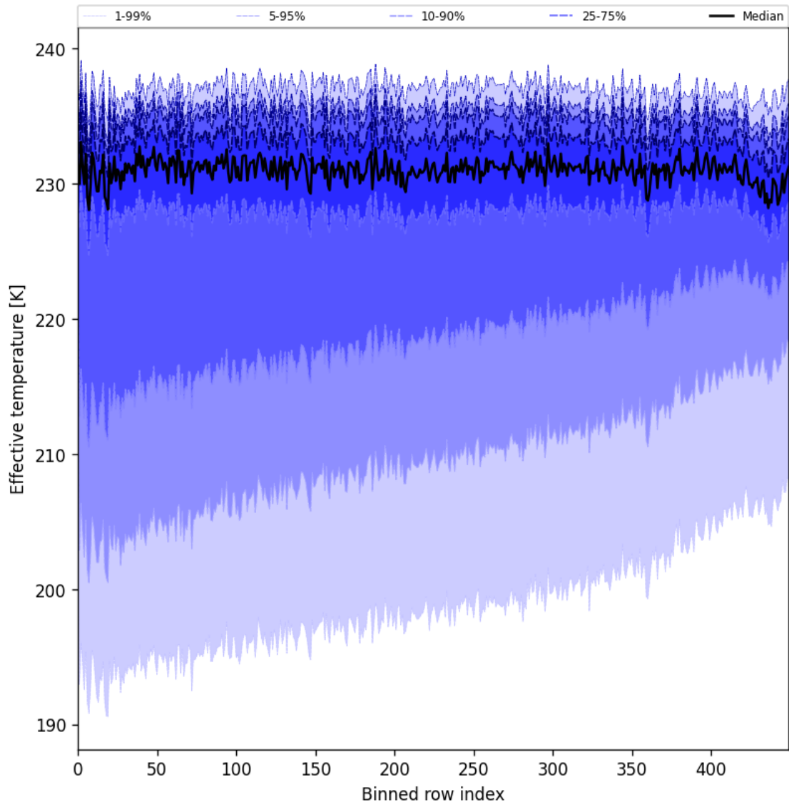
Figure 31: Along track statistics of “Effective temperature” for 2025-08-26 to 2025-08-28
