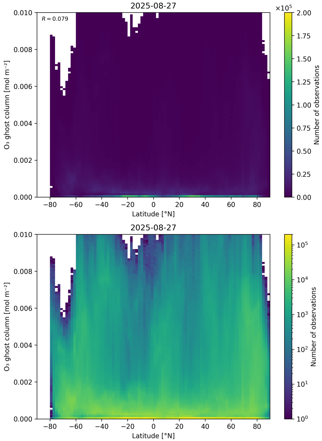
Figure 35: Scatter density plot of “Latitude” against “O 3 ghost column” for 2025-08-26 to 2025-08-28.
