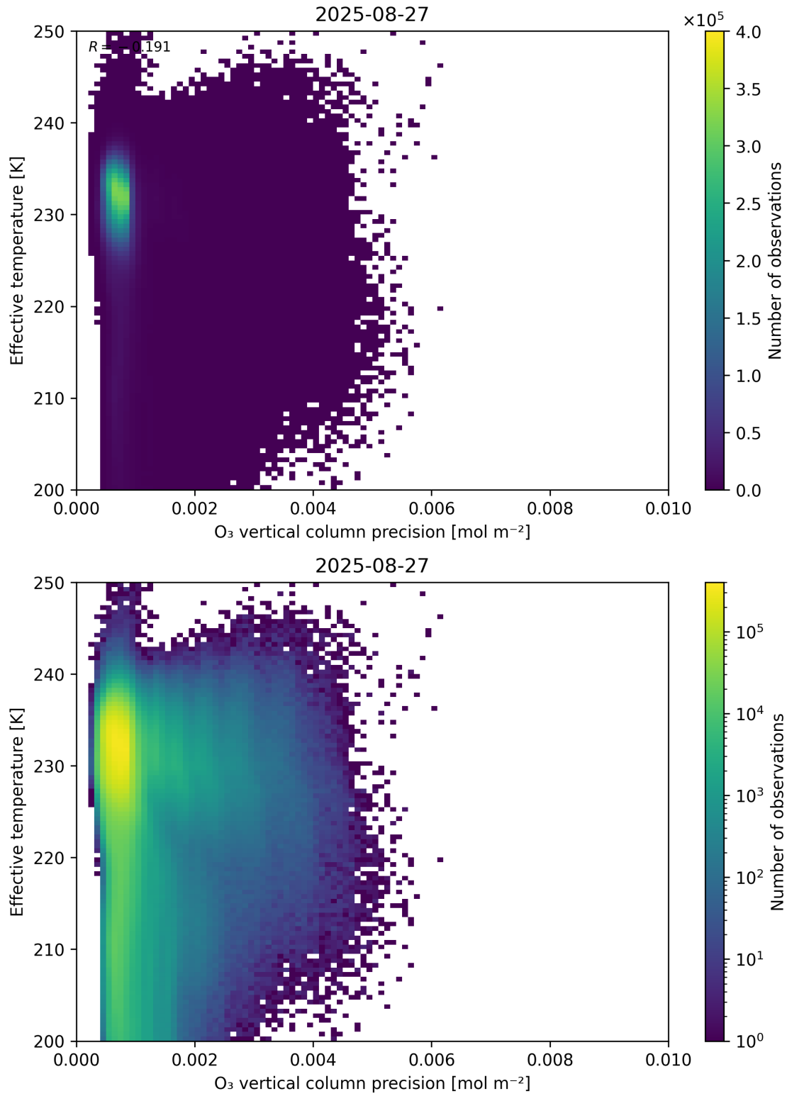
Figure 42: Scatter density plot of “O 3 vertical column precision” against “Effective temperature” for 2025-08-26 to 2025-08-28.
