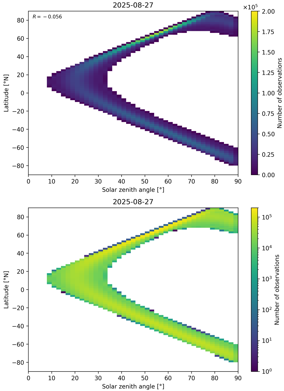
Figure 44: Scatter density plot of “Solar zenith angle” against “Latitude” for 2025-08-26 to 2025-08-28.
