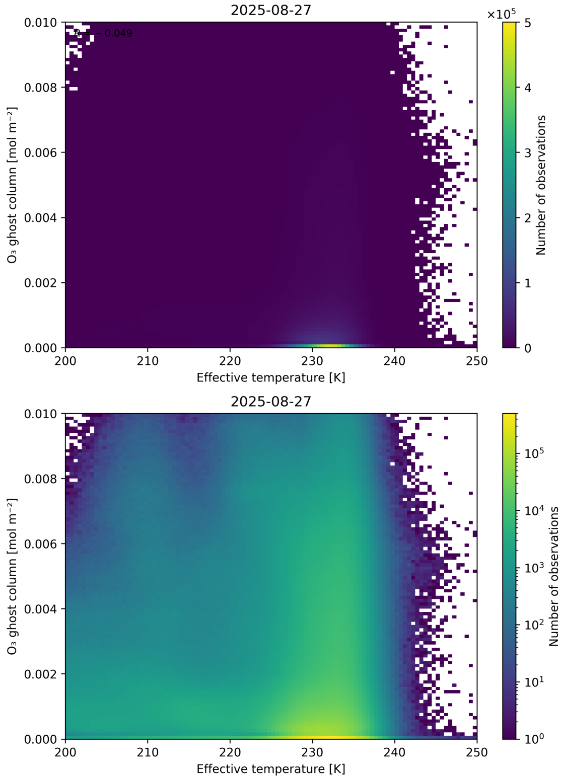
Figure 38: Scatter density plot of “Effective temperature” against “O 3 ghost column” for 2025-08-26 to 2025-08-28.
