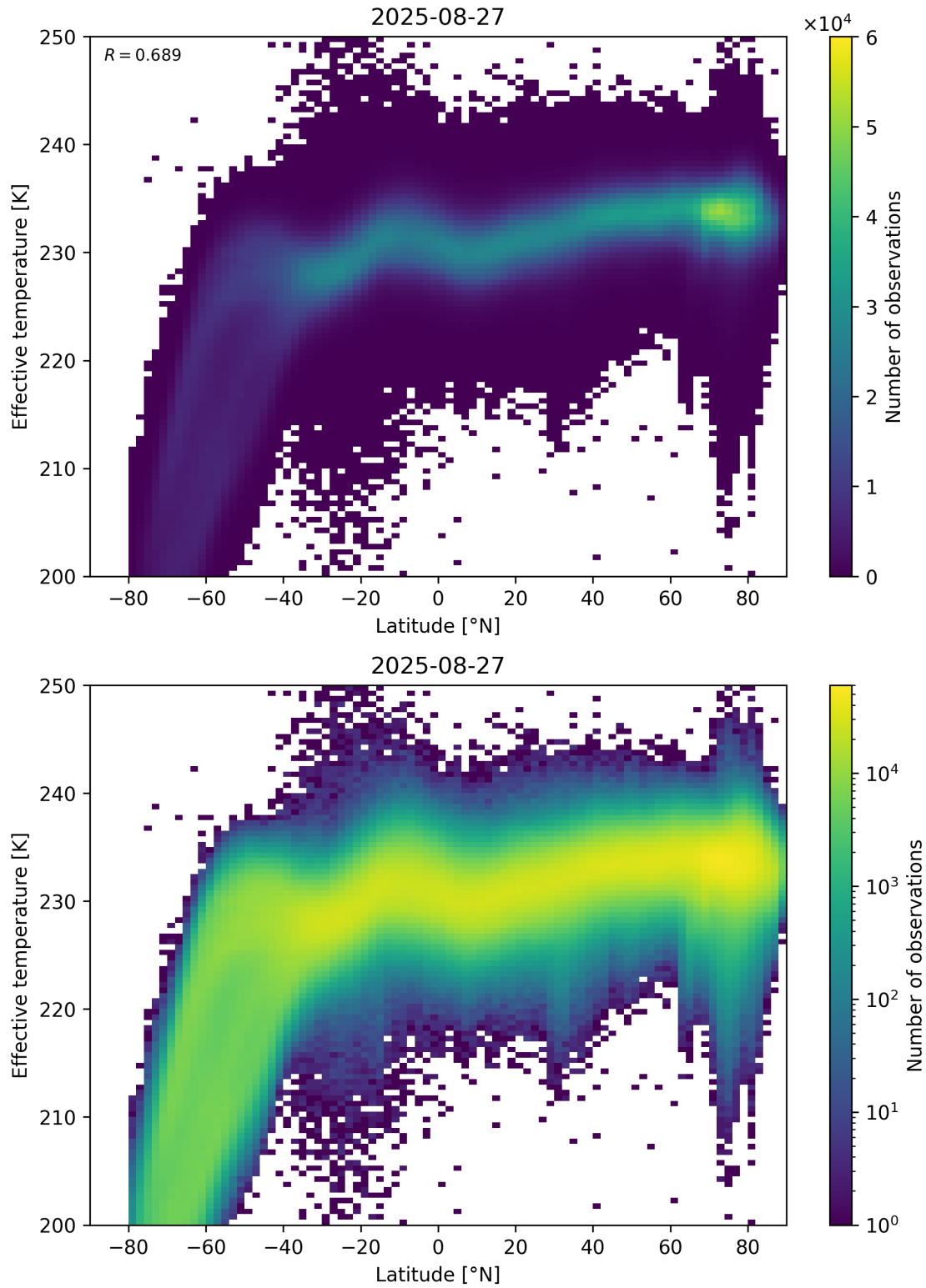
Figure 34: Scatter density plot of “Latitude” against “Effective temperature” for 2025-08-26 to 2025-08-28.
