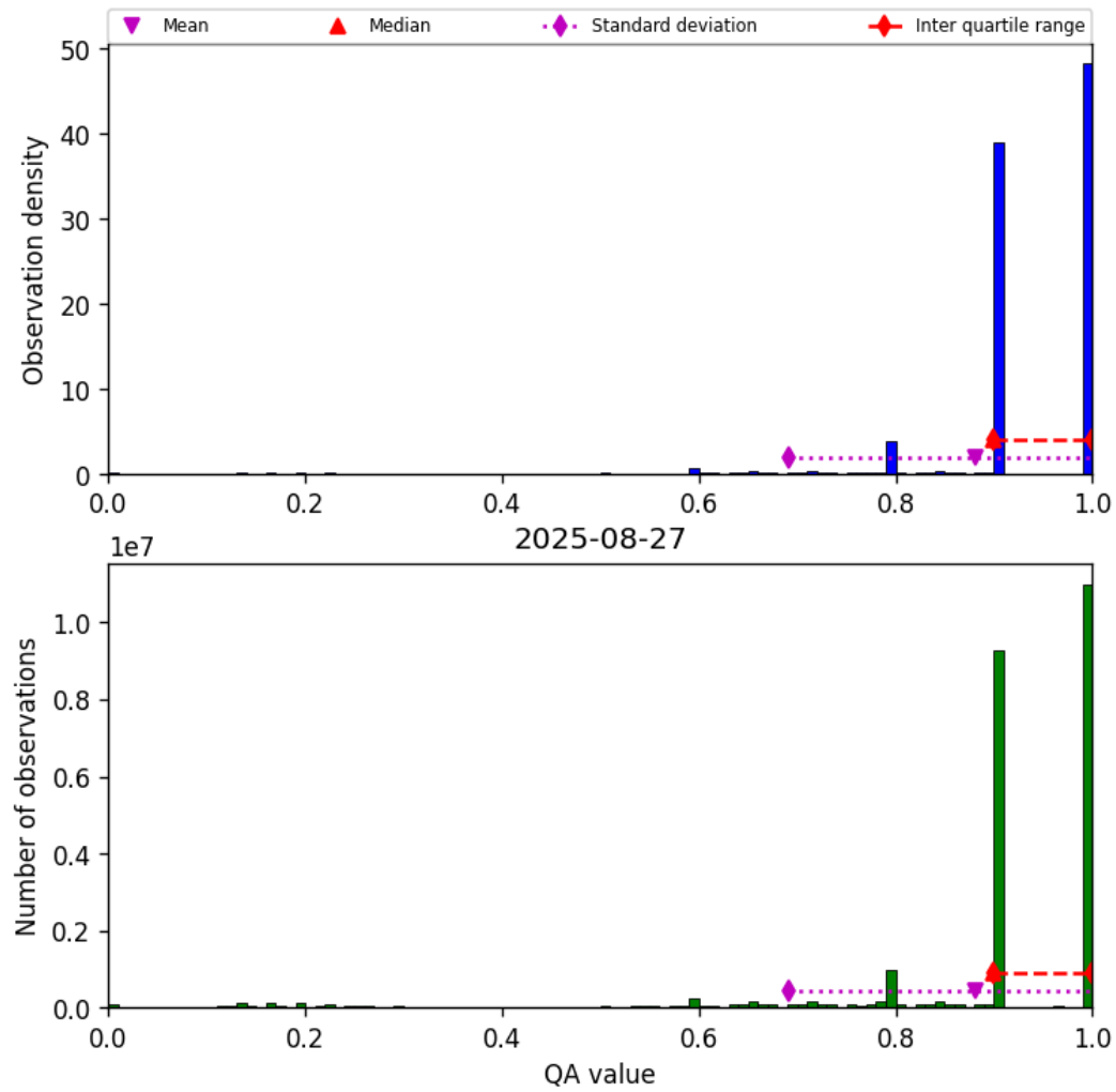
Figure 20: Histogram of “QA value” for 2025-08-26 to 2025-08-28
