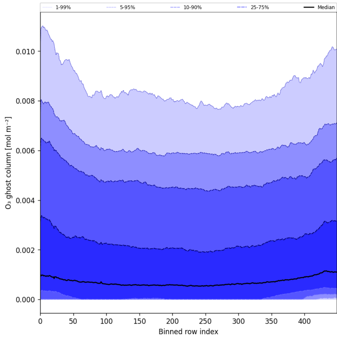
Figure 32: Along track statistics of “O 3 ghost column” for 2025-08-27 to 2025-08-29
