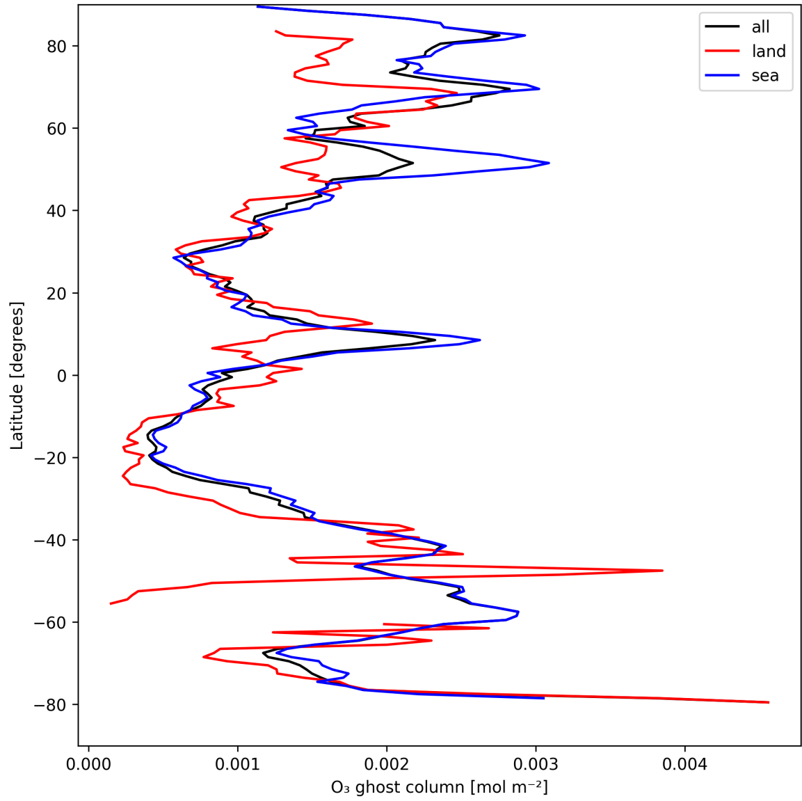
Figure 18: Zonal average of "O 3 ghost column" for 2025-08-27 to 2025-08-29.
