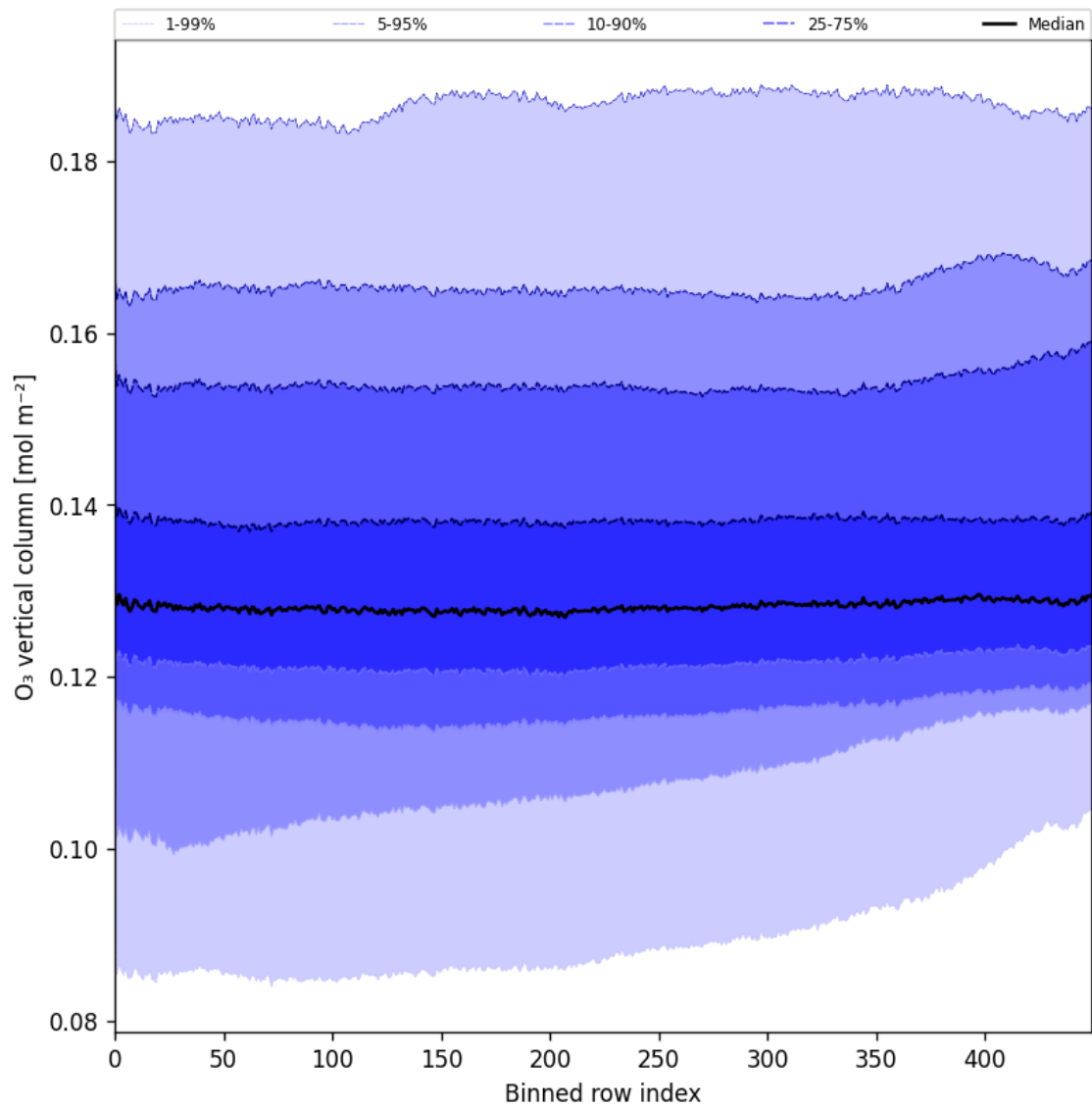
Figure 28: Along track statistics of “O 3 vertical column” for 2025-08-27 to 2025-08-29
