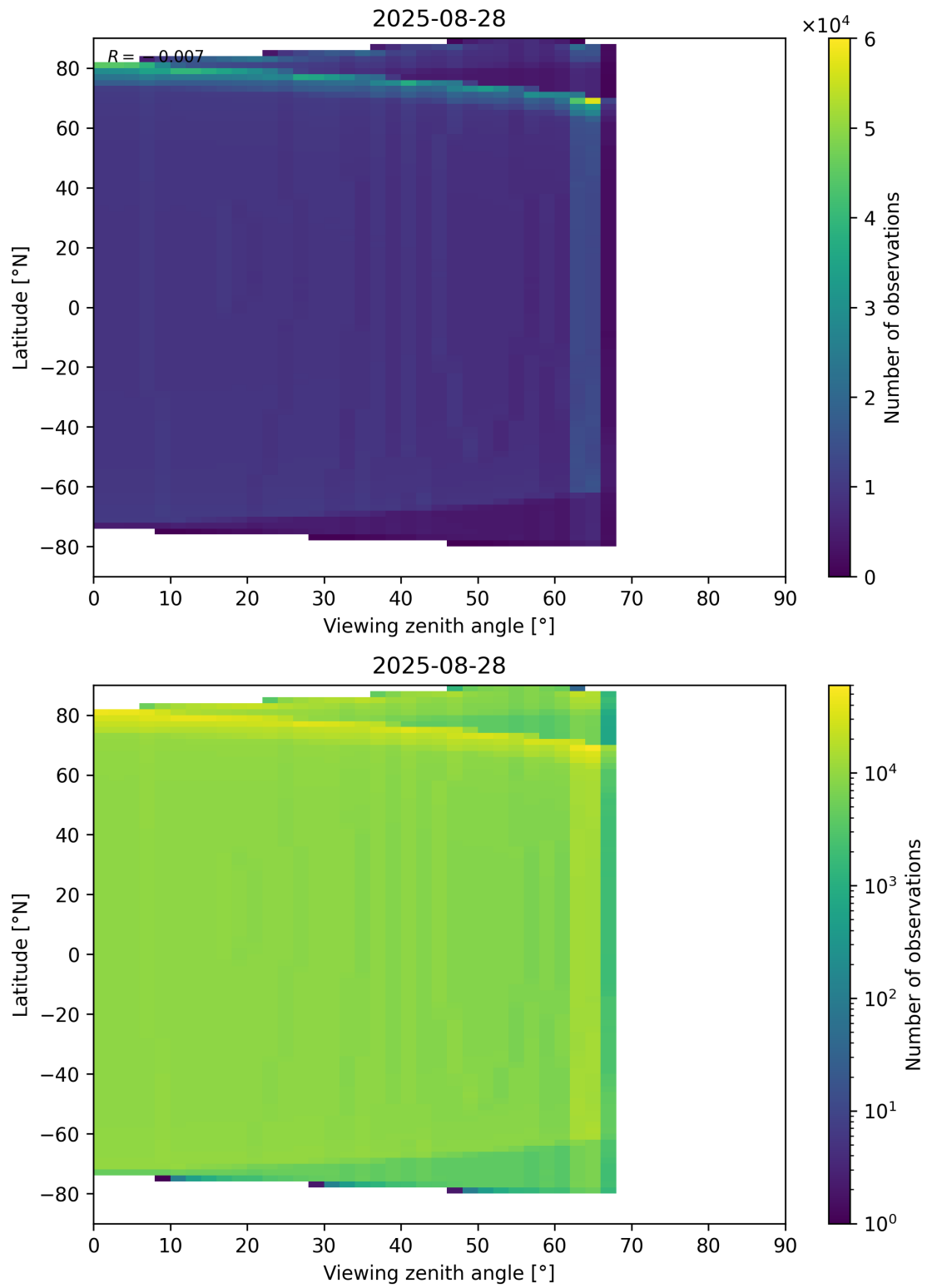
Figure 49: Scatter density plot of “Viewing zenith angle” against “Latitude” for 2025-08-27 to 2025-08-29.
