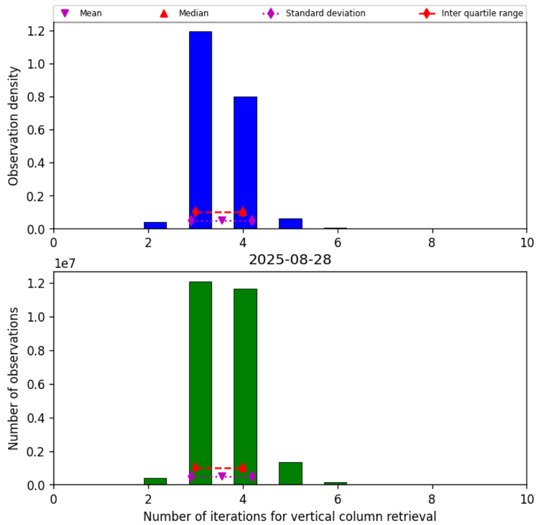
Figure 26: Histogram of “Number of iterations for vertical column retrieval” for 2025-08-27 to 2025-08-29
