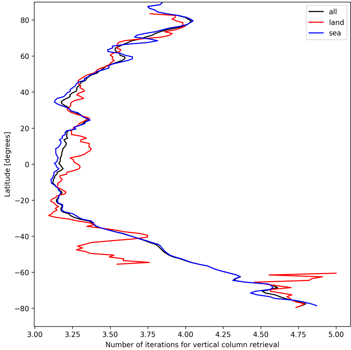
Figure 19: Zonal average of “Number of iterations for vertical column retrieval” for 2025-08-27 to 2025-08-29.
