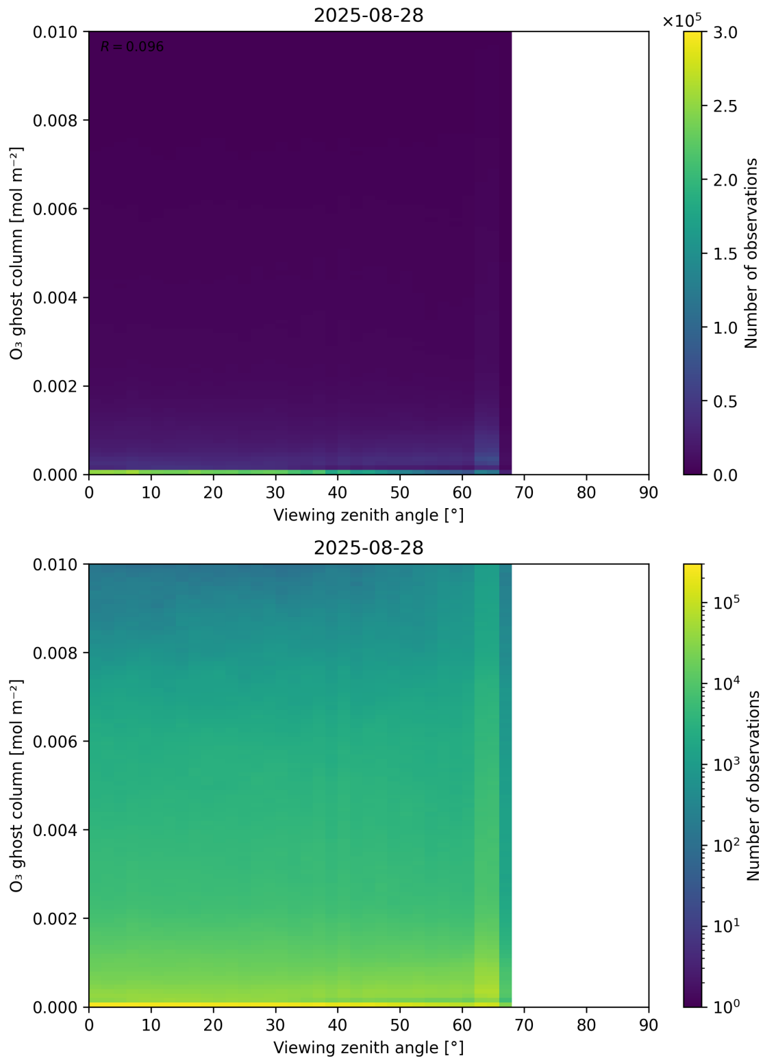
Figure 51: Scatter density plot of “Viewing zenith angle” against “O 3 ghost column” for 2025-08-27 to 2025-08-29.
