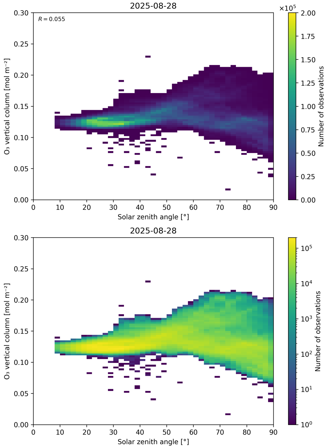
Figure 47: Scatter density plot of “Solar zenith angle” against “O 3 vertical column” for 2025-08-27 to 2025-08-29.
