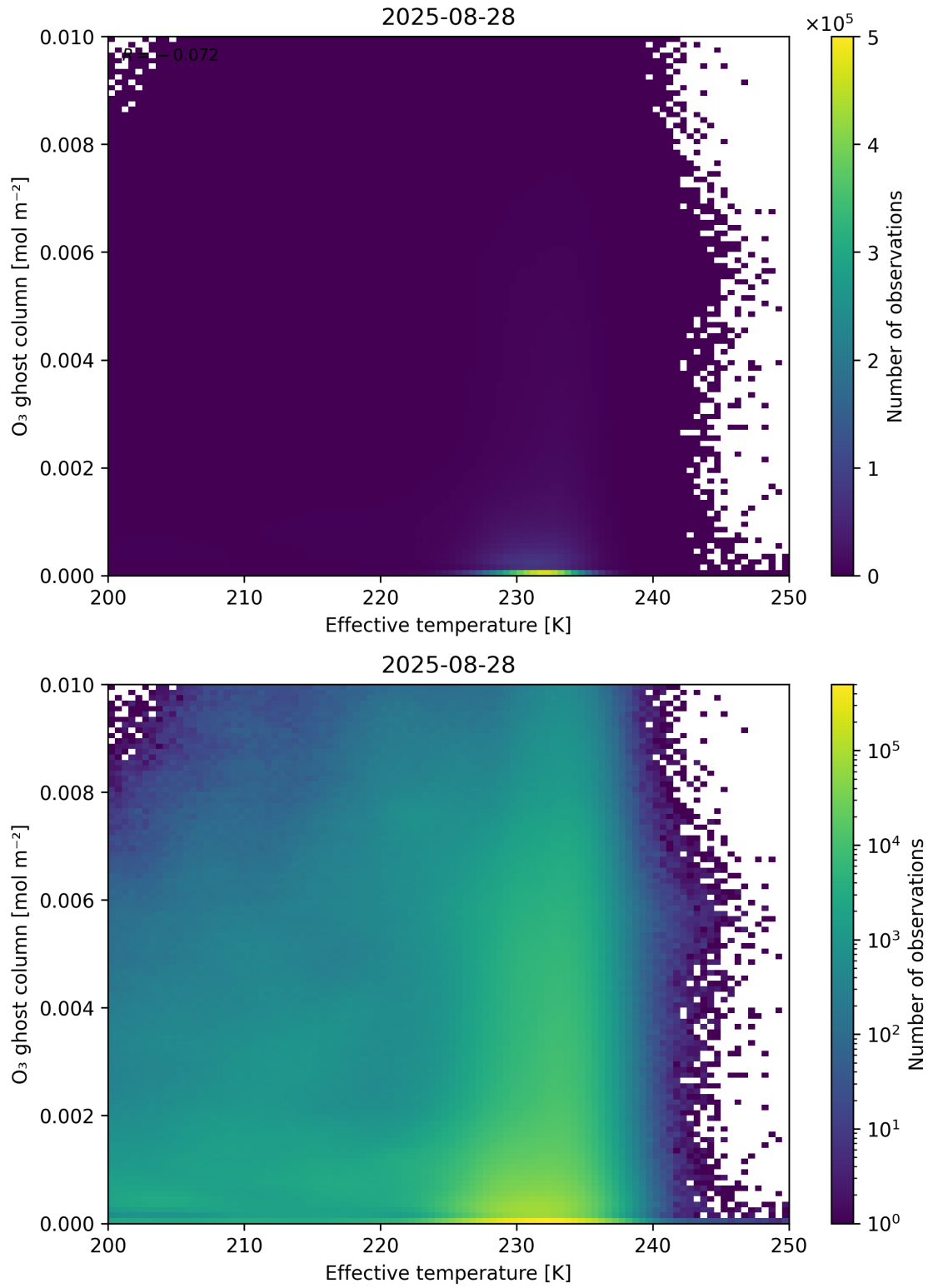
Figure 38: Scatter density plot of “Effective temperature” against “O 3 ghost column” for 2025-08-27 to 2025-08-29.
