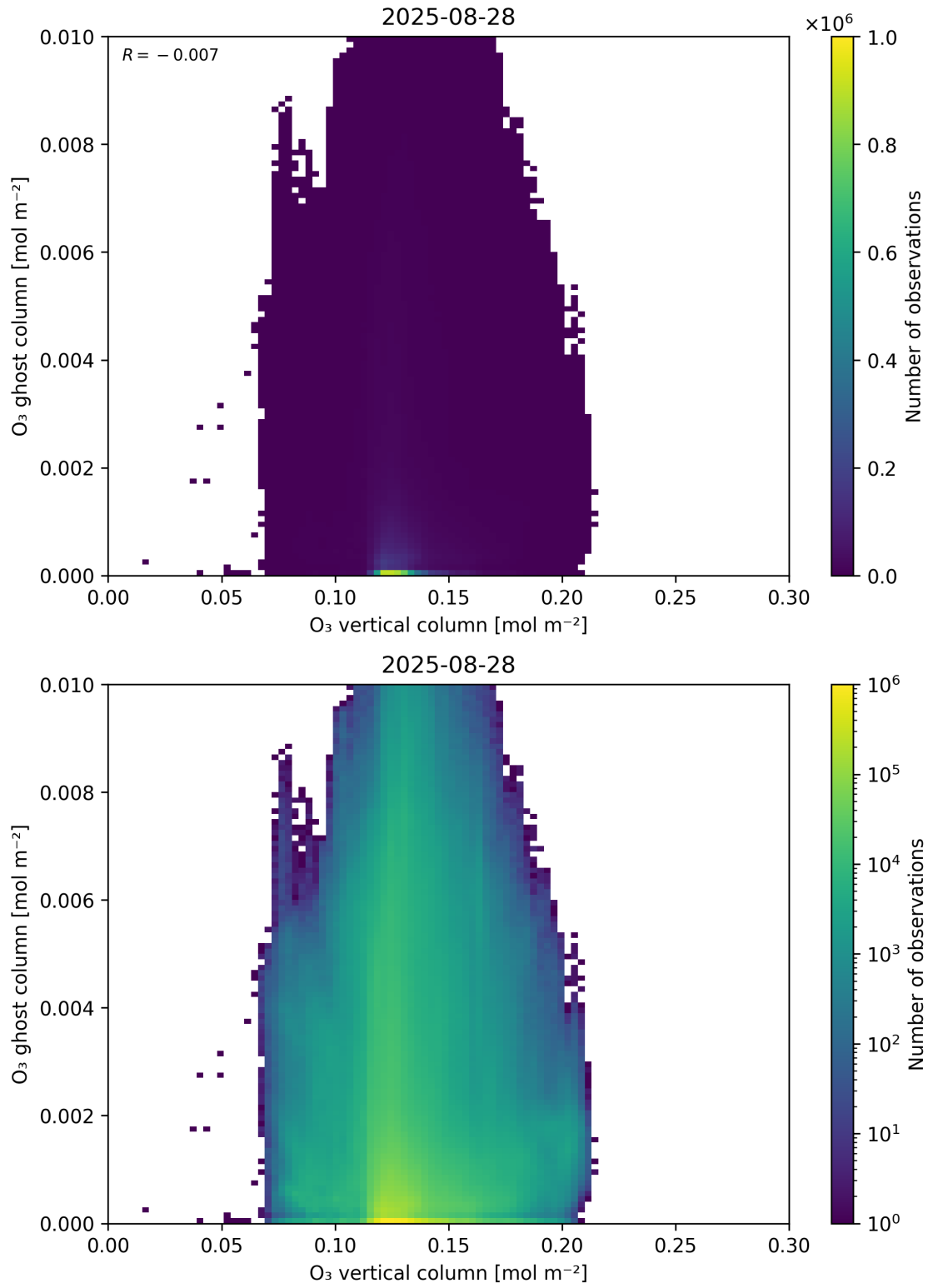
Figure 40: Scatter density plot of “O 3 vertical column” against “O 3 ghost column” for 2025-08-27 to 2025-08-29.
