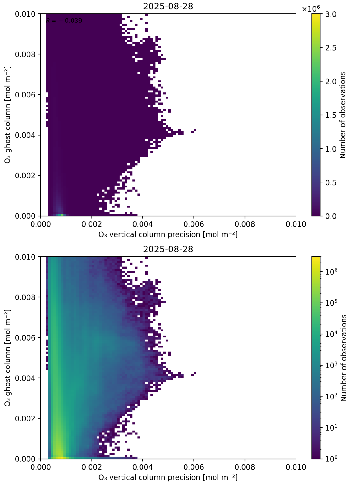
Figure 43: Scatter density plot of “O 3 vertical column precision” against “O 3 ghost column” for 2025-08-27 to 2025-08-29.
