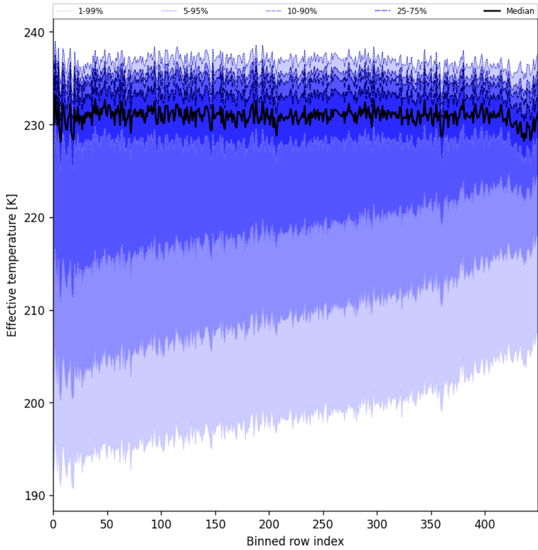
Figure 31: Along track statistics of “Effective temperature” for 2025-08-27 to 2025-08-29
