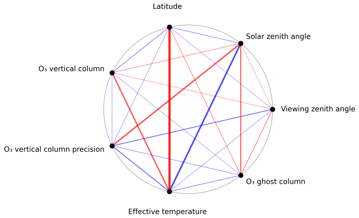
Figure 1: Map of correlation graph for 2025-08-27 to 2025-08-29.
