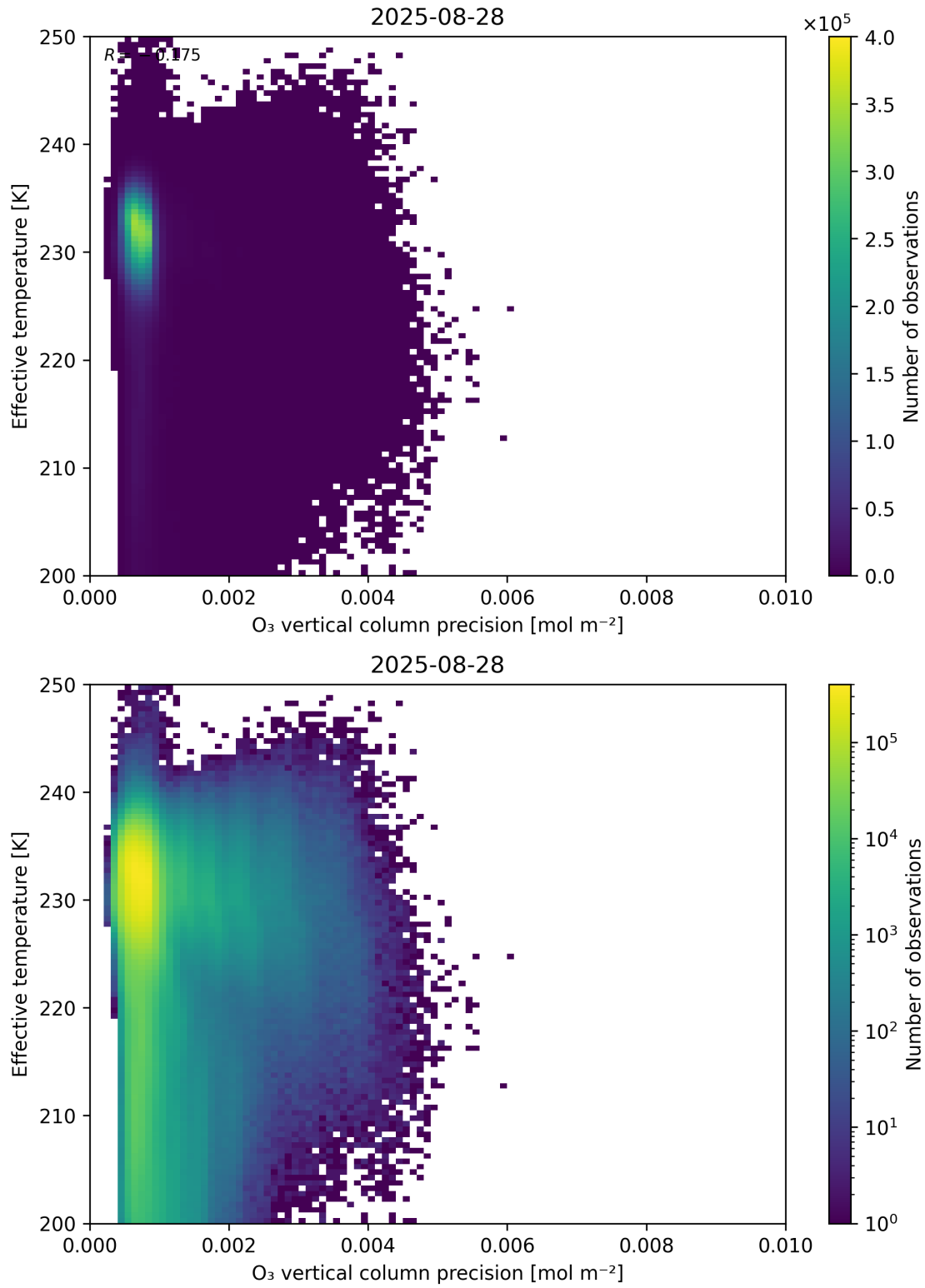
Figure 42: Scatter density plot of “O 3 vertical column precision” against “Effective temperature” for 2025-08-27 to 2025-08-29.
