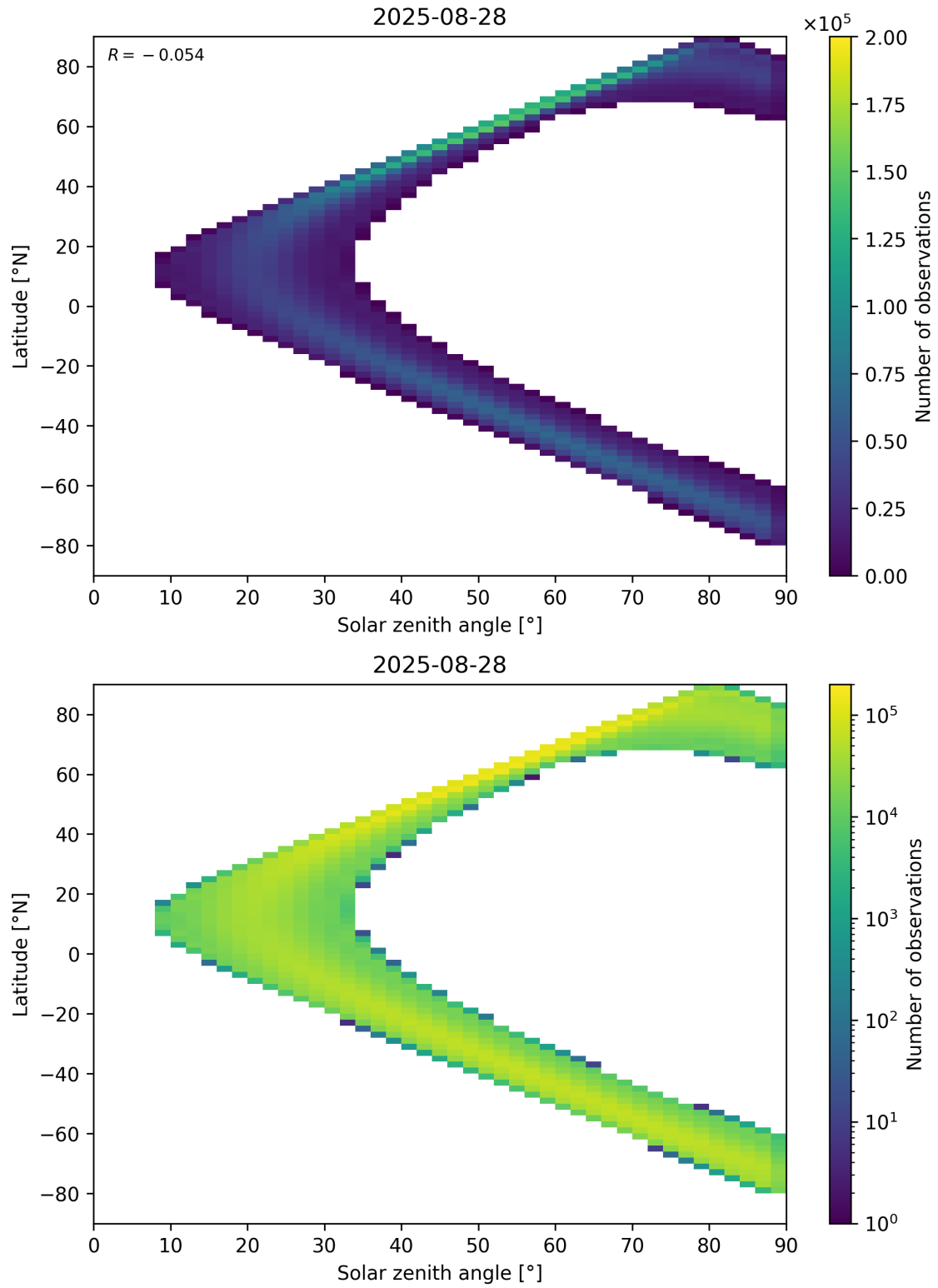
Figure 44: Scatter density plot of “Solar zenith angle” against “Latitude” for 2025-08-27 to 2025-08-29.
