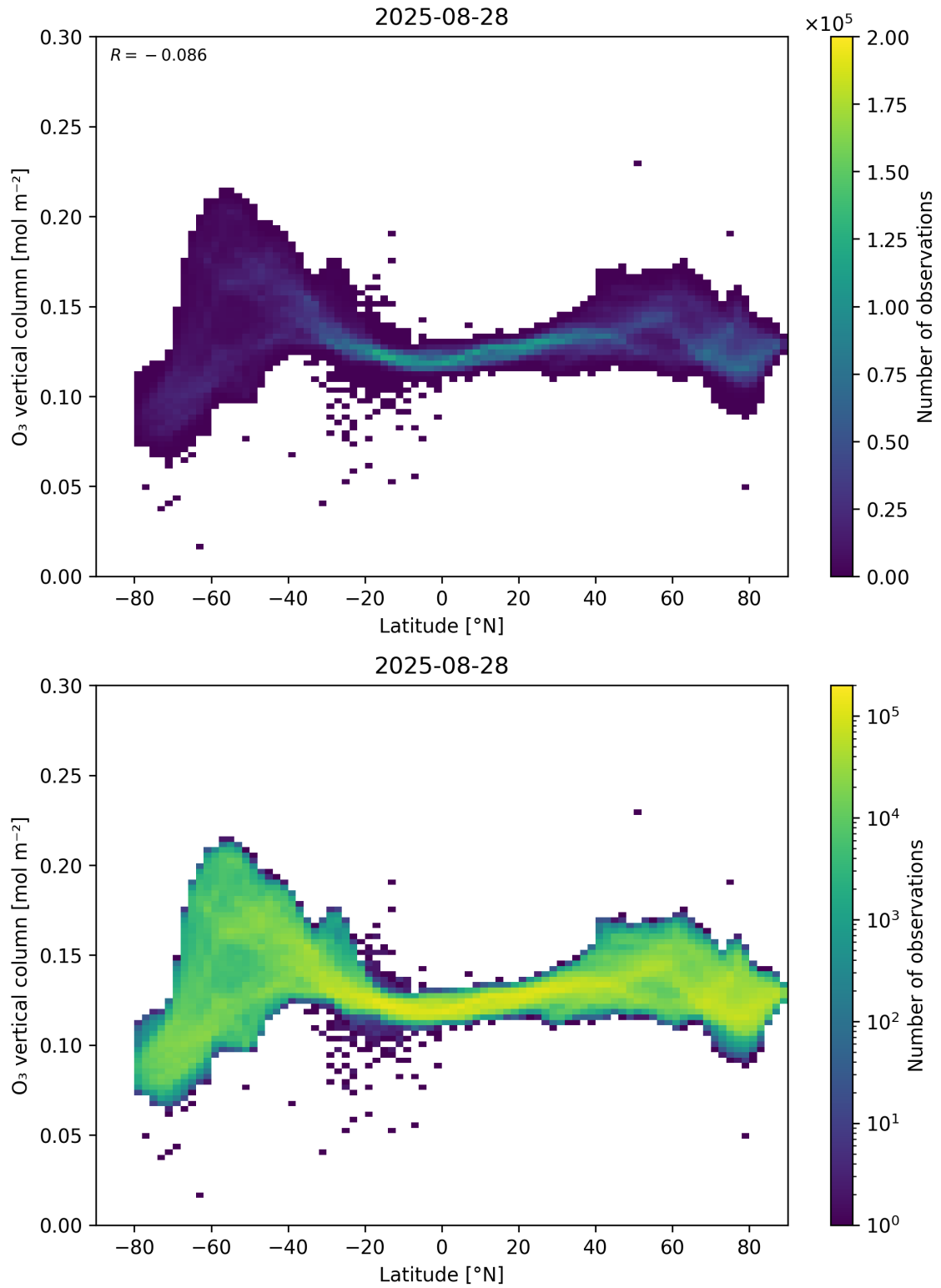
Figure 36: Scatter density plot of “Latitude” against “O 3 vertical column” for 2025-08-27 to 2025-08-29.
