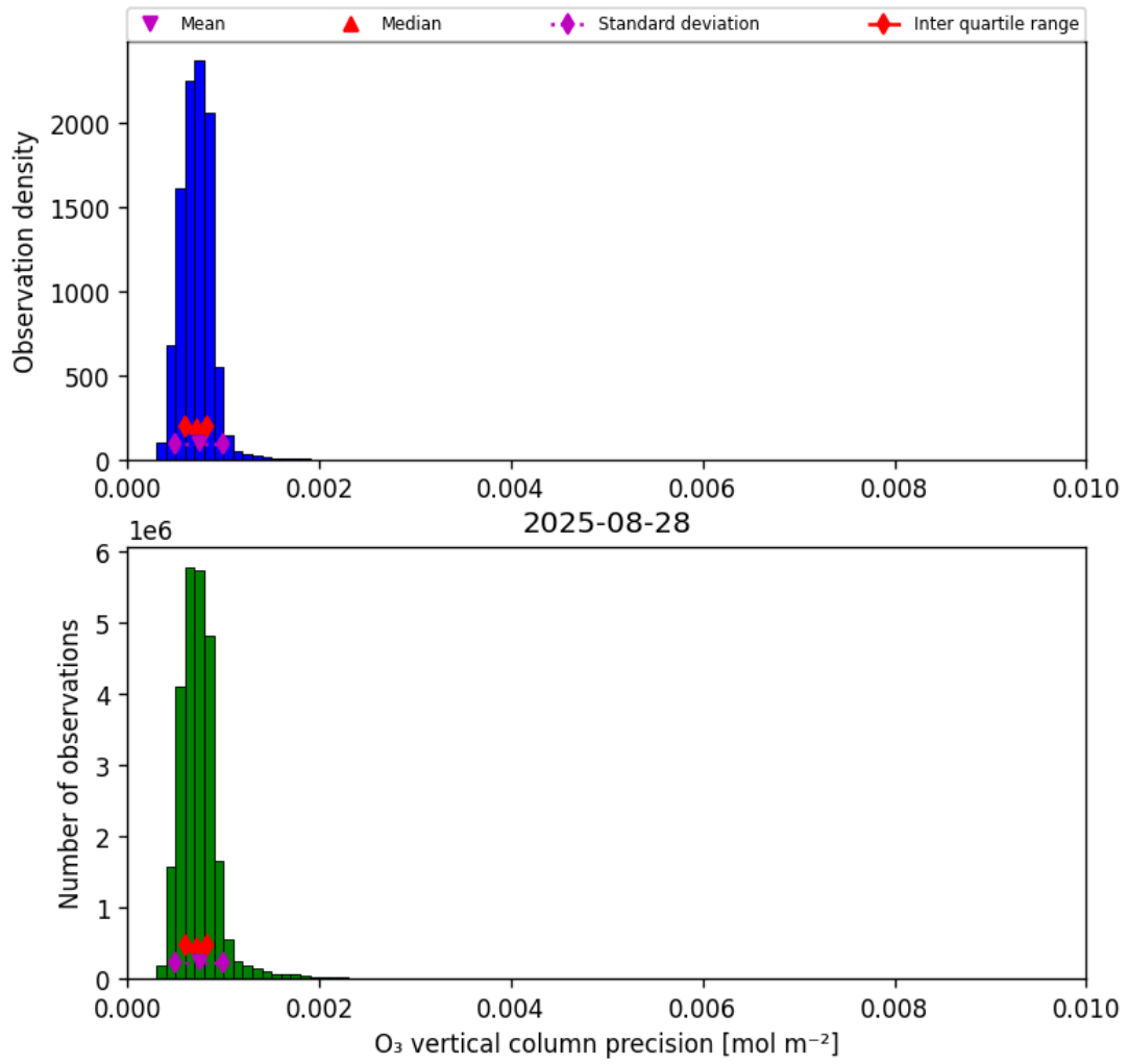
Figure 22: Histogram of “O 3 vertical column precision” for 2025-08-27 to 2025-08-29
