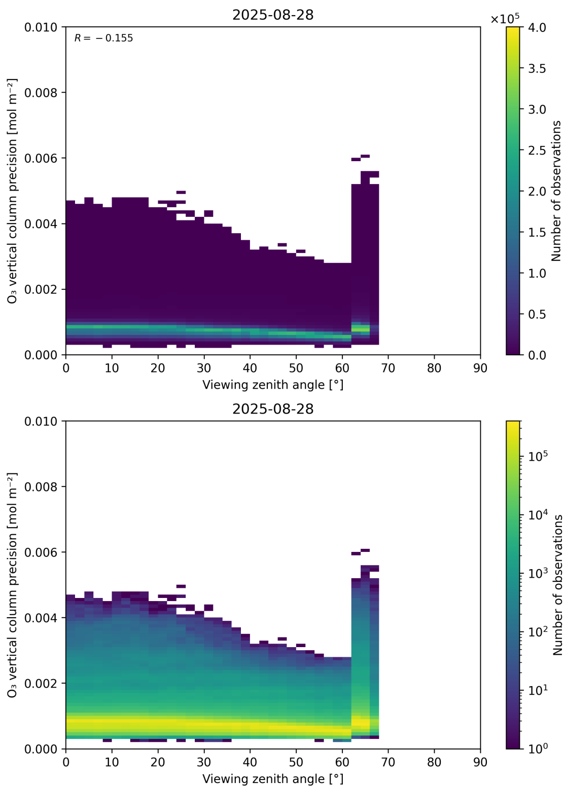
Figure 53: Scatter density plot of “Viewing zenith angle” against “O 3 vertical column precision” for 2025-08-27 to 2025-08-29.
