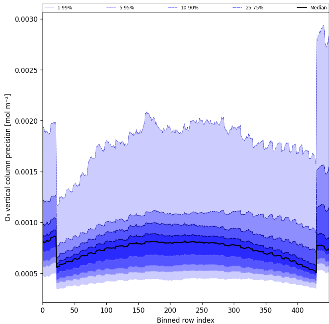
Figure 29: Along track statistics of “O 3 vertical column precision” for 2025-08-27 to 2025-08-29
