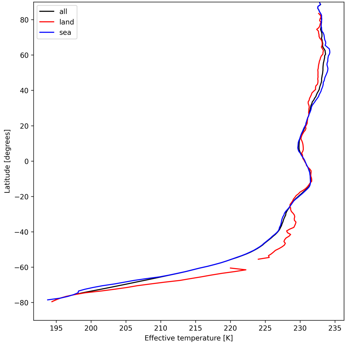
Figure 17: Zonal average of "Effective temperature" for 2025-08-27 to 2025-08-29.
