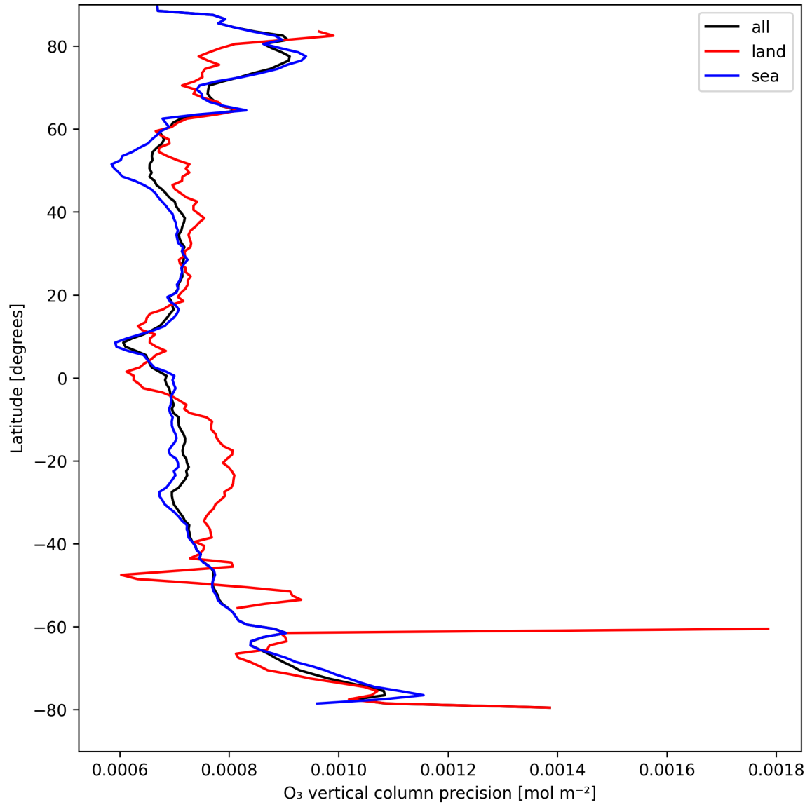
Figure 15: Zonal average of “O 3 vertical column precision” for 2025-08-27 to 2025-08-29.
