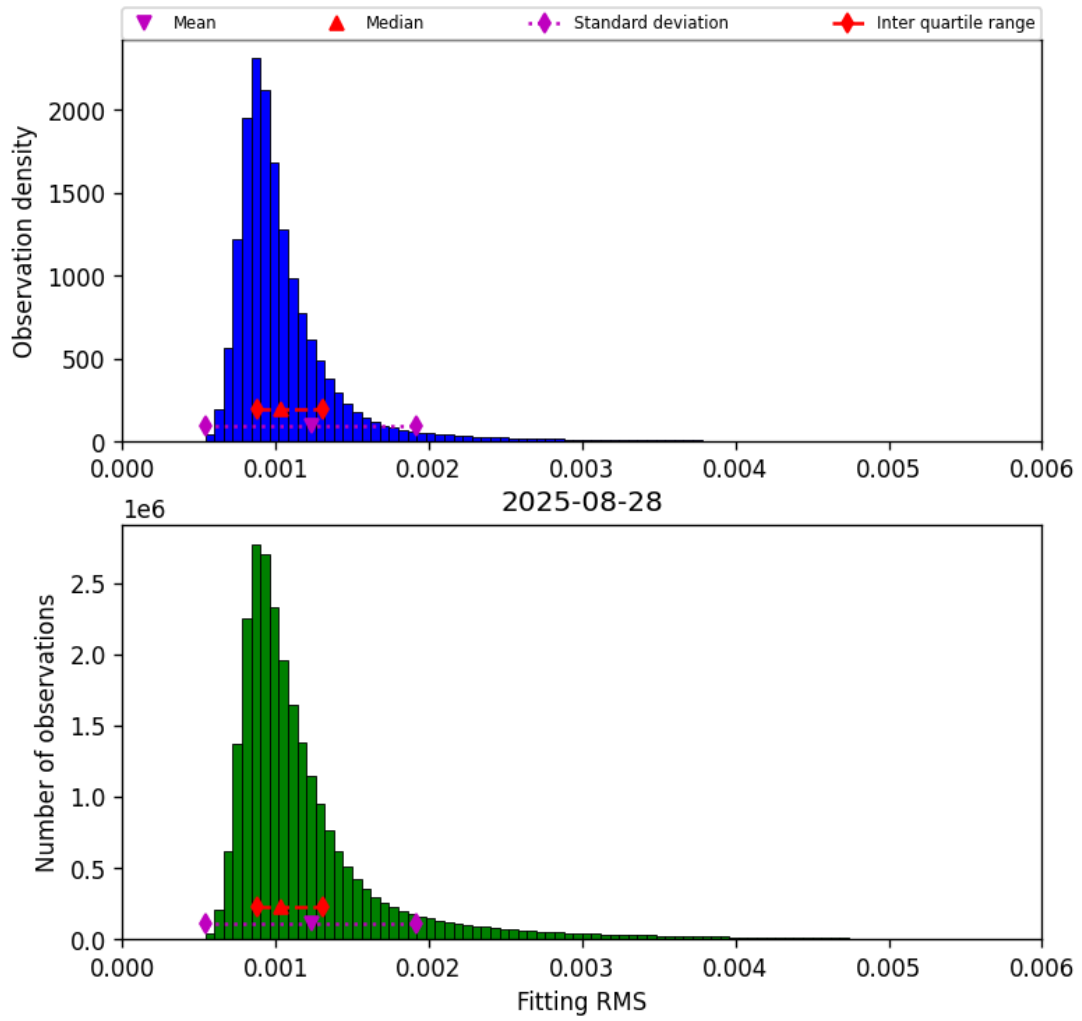
Figure 23: Histogram of “Fitting RMS” for 2025-08-27 to 2025-08-29
