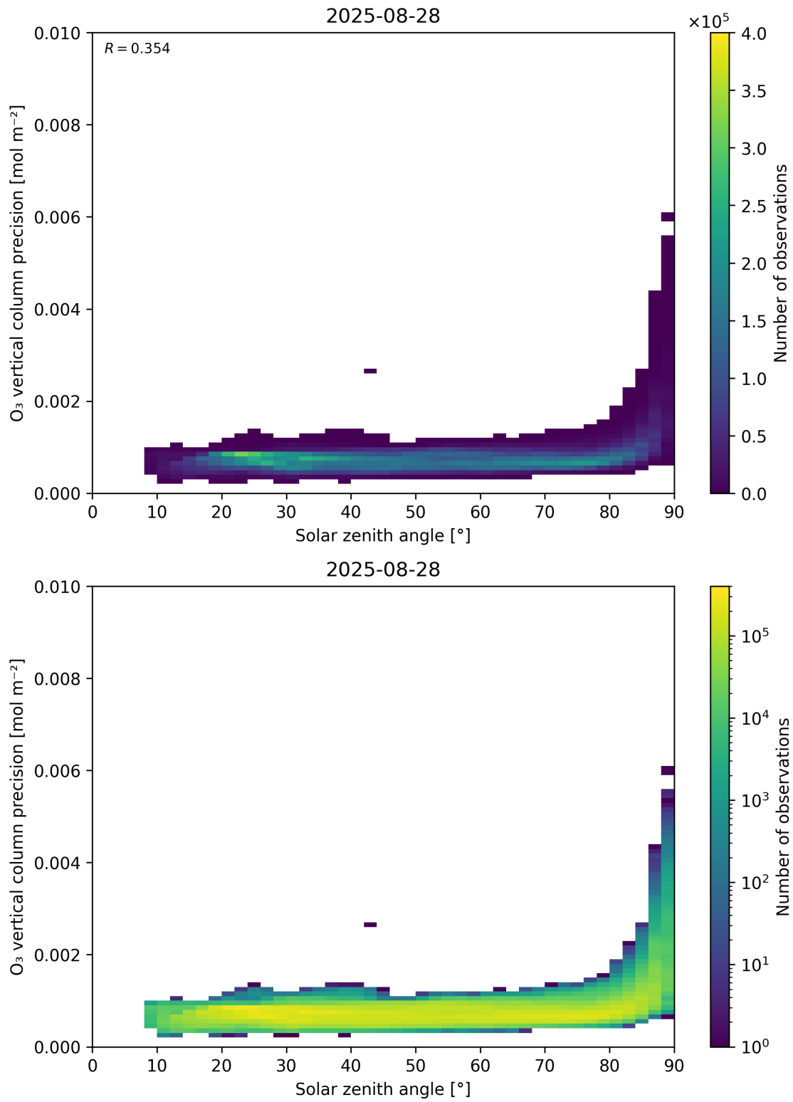
Figure 48: Scatter density plot of “Solar zenith angle” against “O 3 vertical column precision” for 2025-08-27 to 2025-08-29.
