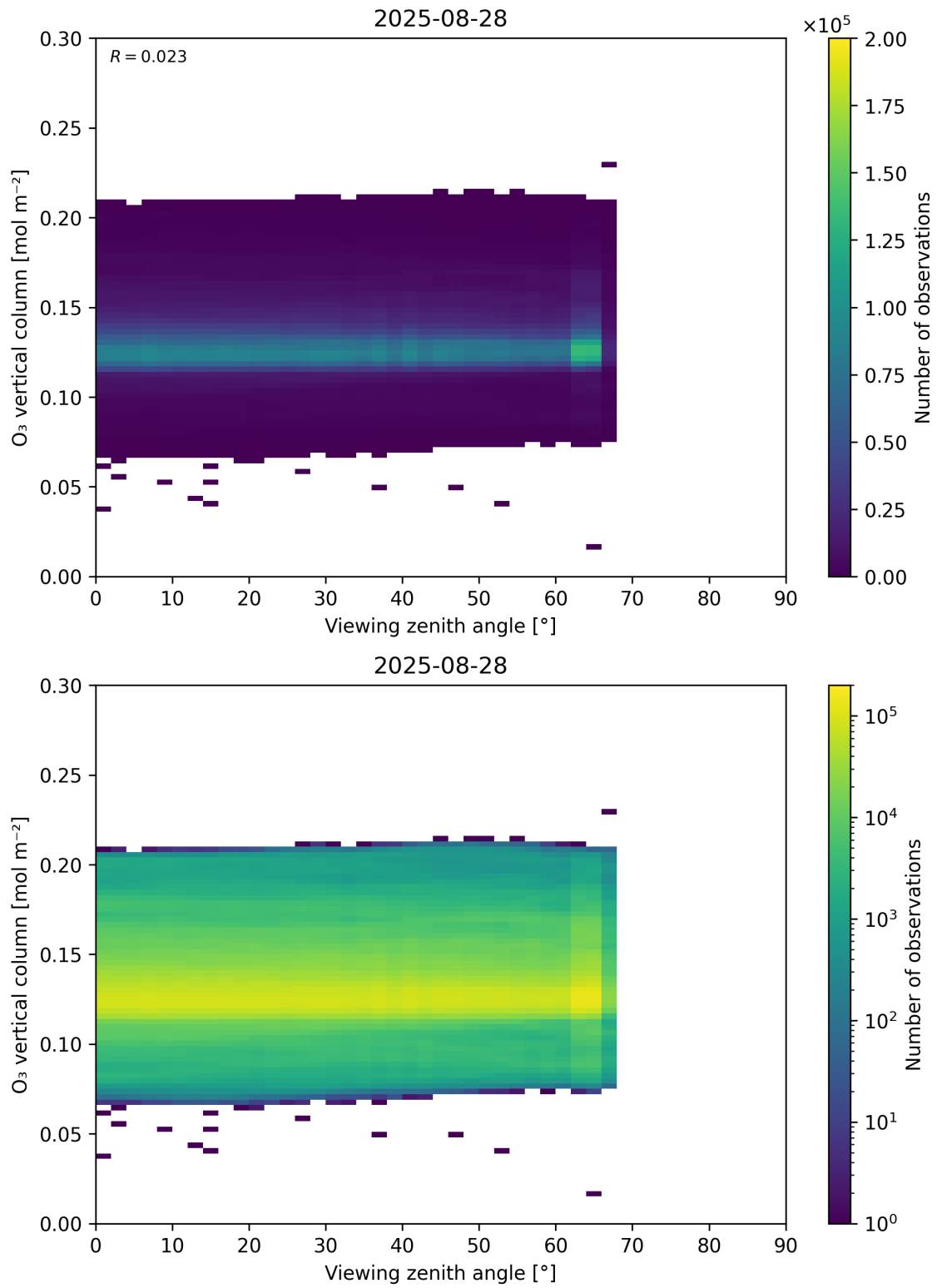
Figure 52: Scatter density plot of “Viewing zenith angle” against “O 3 vertical column” for 2025-08-27 to 2025-08-29.
