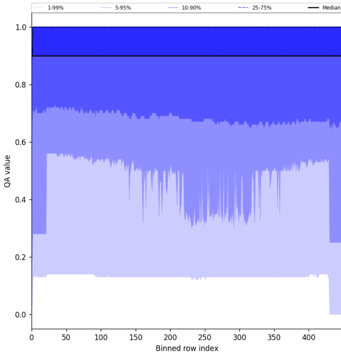
Figure 27: Along track statistics of “QA value” for 2025-08-27 to 2025-08-29
