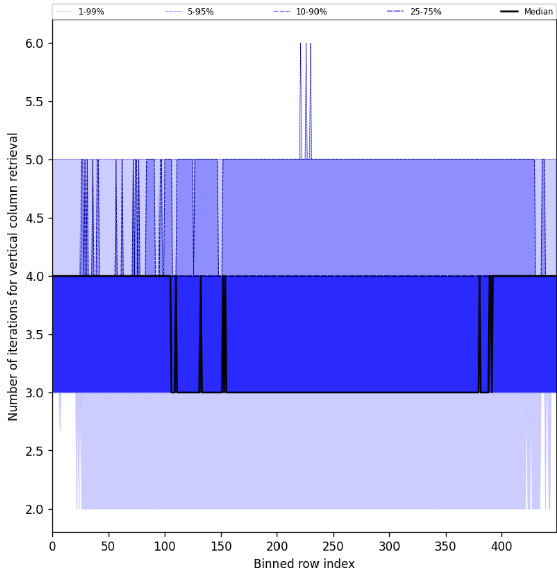
Figure 33: Along track statistics of “Number of iterations for vertical column retrieval” for 2025-08-27 to 2025-08-29
