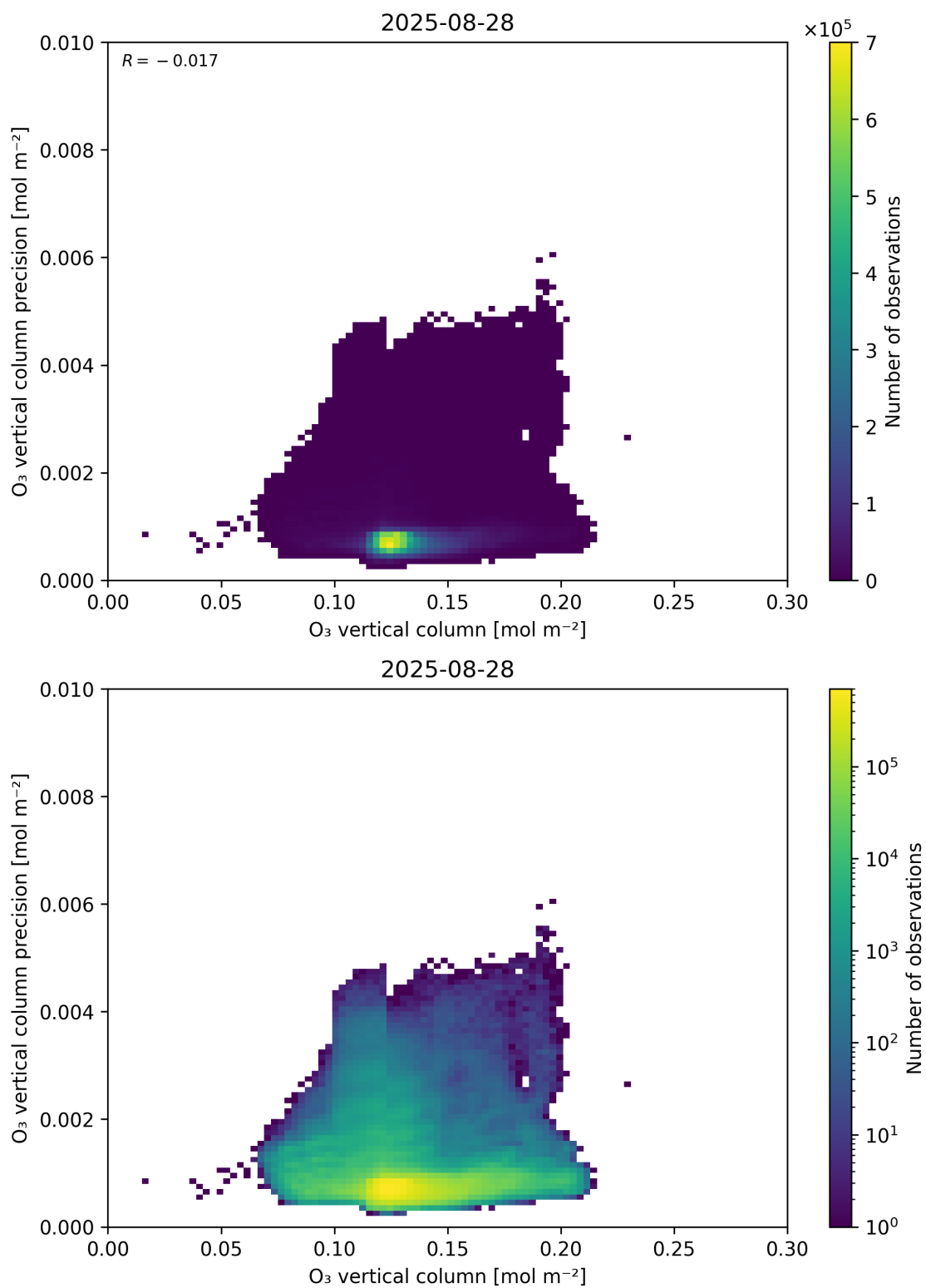
Figure 41: Scatter density plot of “O 3 vertical column” against “O 3 vertical column precision” for 2025-08-27 to 2025-08-29.
