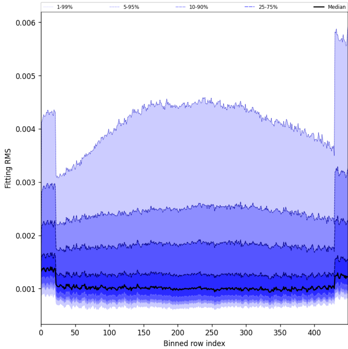
Figure 30: Along track statistics of “Fitting RMS” for 2025-08-27 to 2025-08-29
