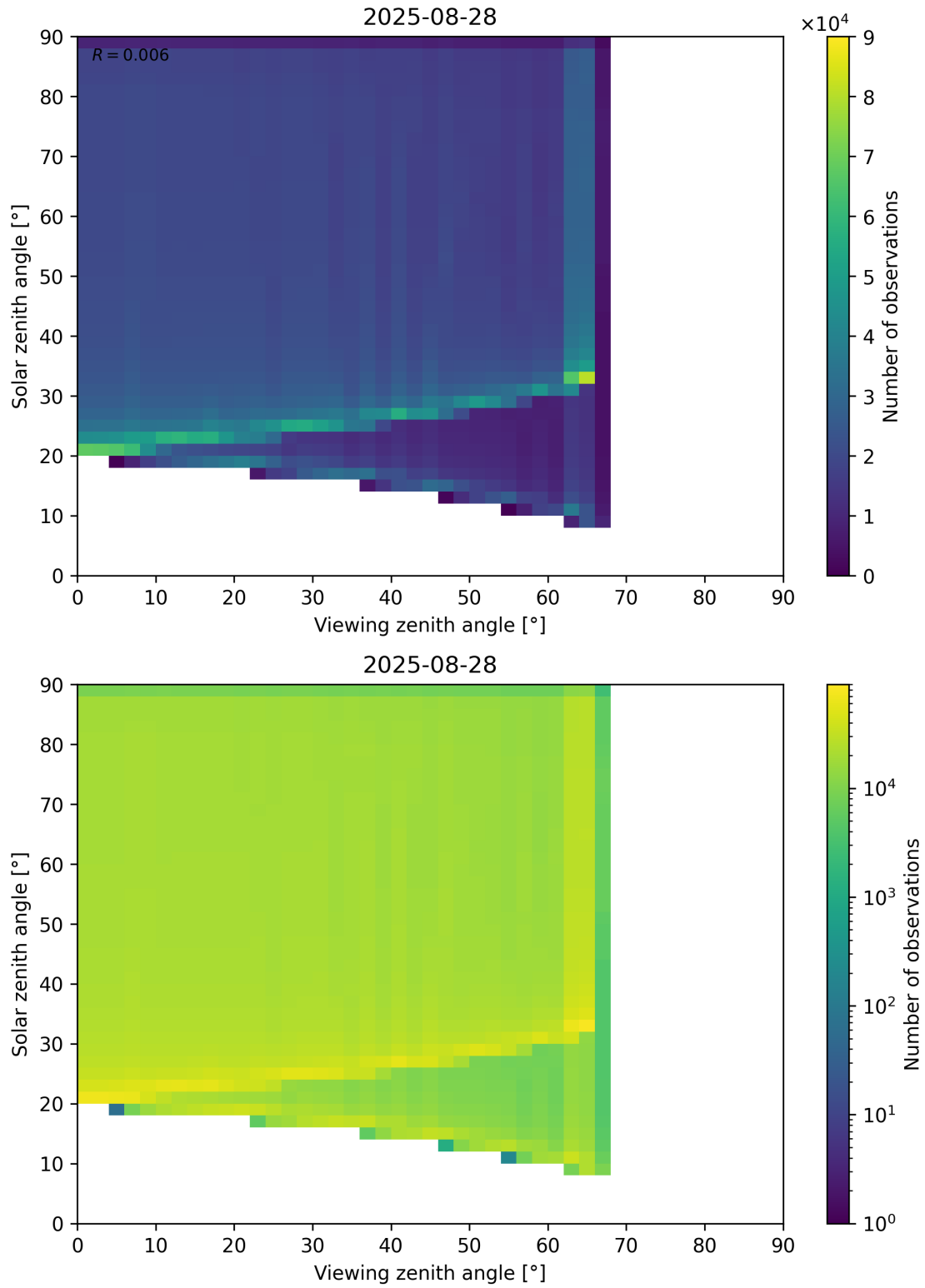
Figure 54: Scatter density plot of “Viewing zenith angle” against “Solar zenith angle” for 2025-08-27 to 2025-08-29.
