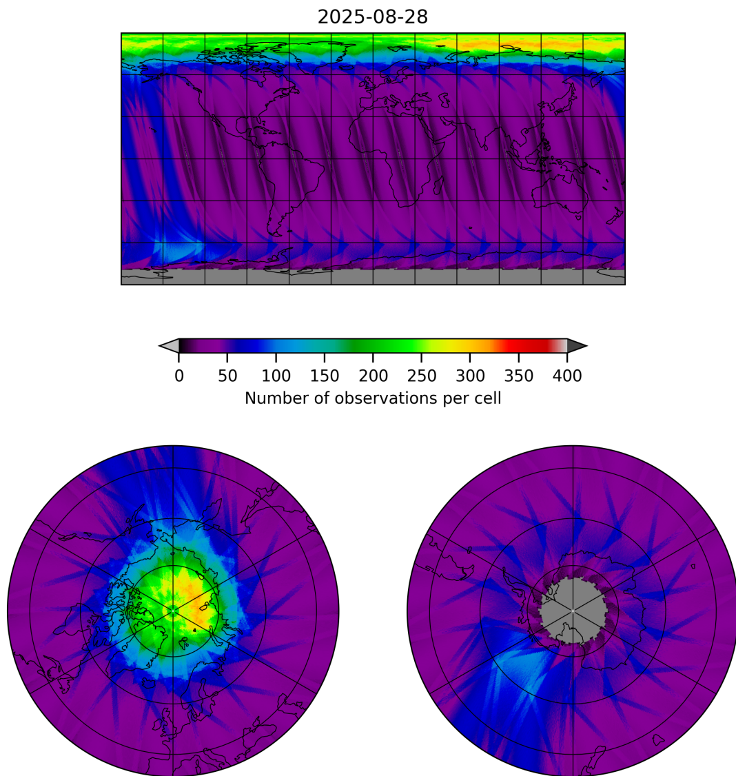
Figure 12: Map of the number of observations for 2025-08-27 to 2025-08-29
