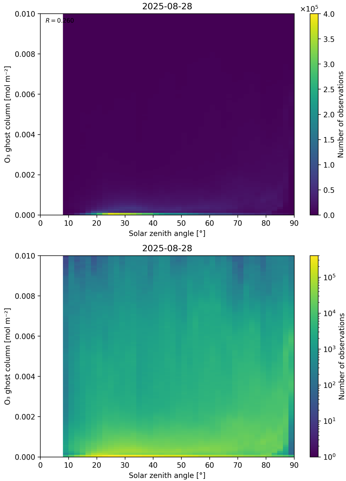
Figure 46: Scatter density plot of “Solar zenith angle” against “O 3 ghost column” for 2025-08-27 to 2025-08-29.
