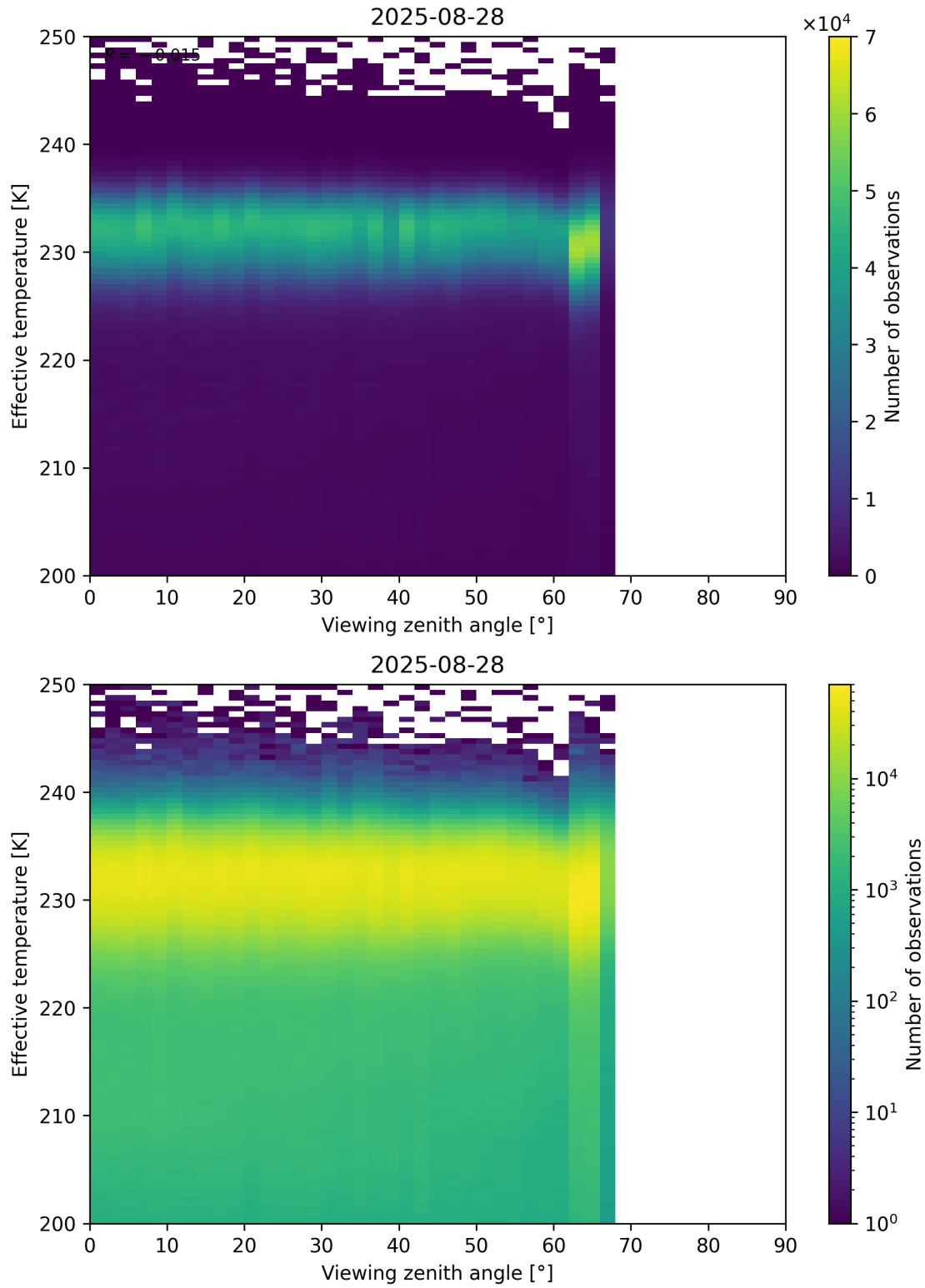
Figure 50: Scatter density plot of “Viewing zenith angle” against “Effective temperature” for 2025-08-27 to 2025-08-29.
