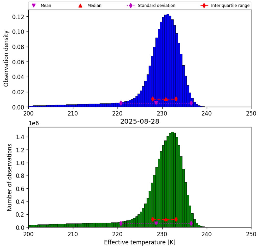
Figure 24: Histogram of “Effective temperature” for 2025-08-27 to 2025-08-29
