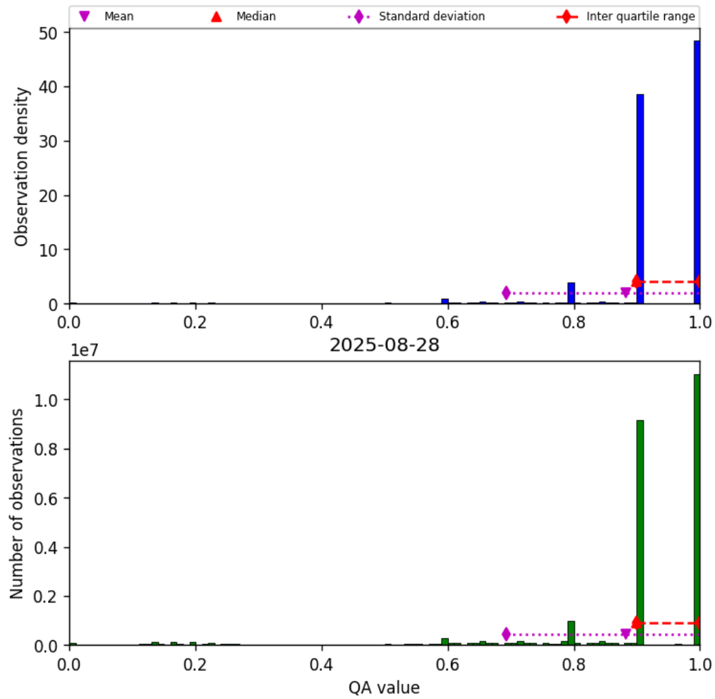
Figure 20: Histogram of “QA value” for 2025-08-27 to 2025-08-29
