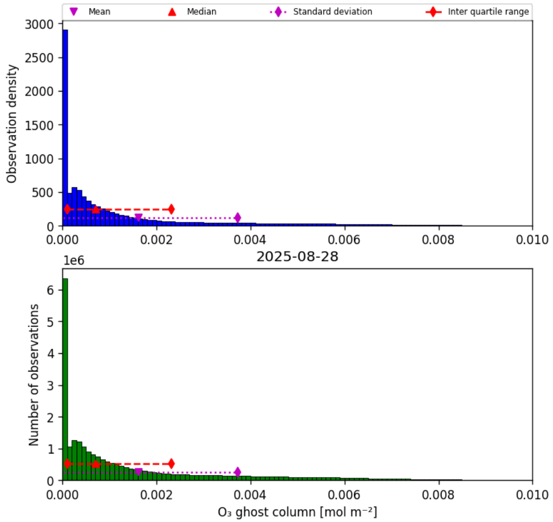
Figure 25: Histogram of “O 3 ghost column” for 2025-08-27 to 2025-08-29
