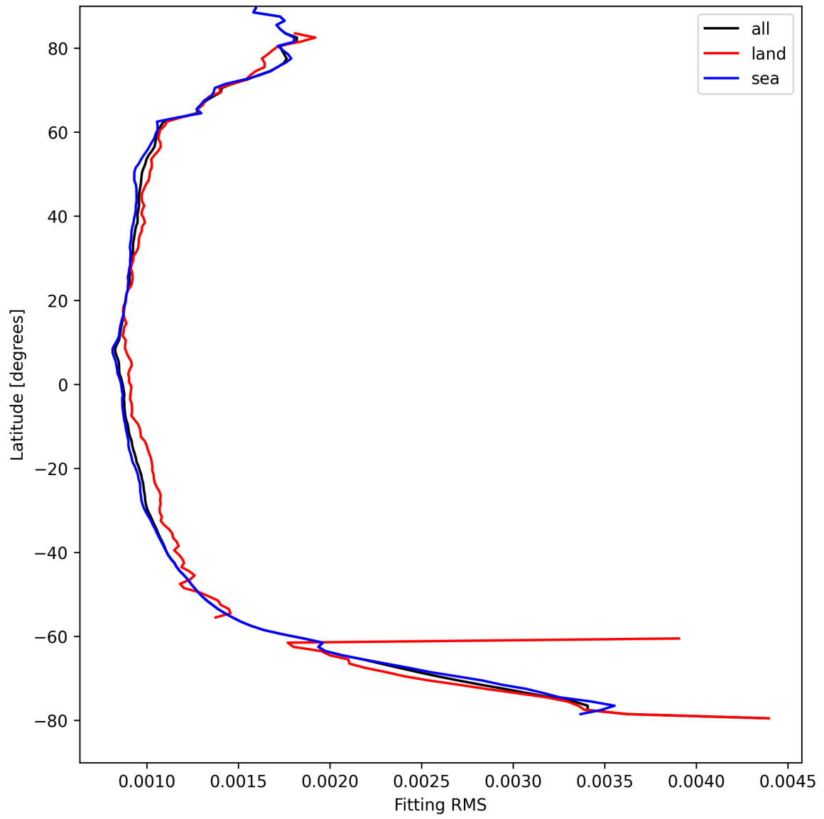
Figure 16: Zonal average of “Fitting RMS” for 2025-08-27 to 2025-08-29.
