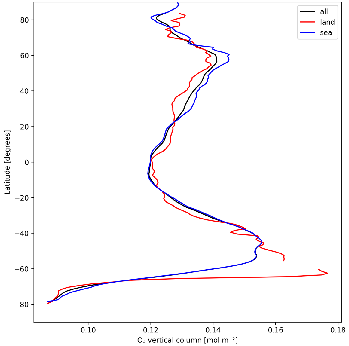
Figure 14: Zonal average of “O 3 vertical column” for 2025-08-27 to 2025-08-29.
