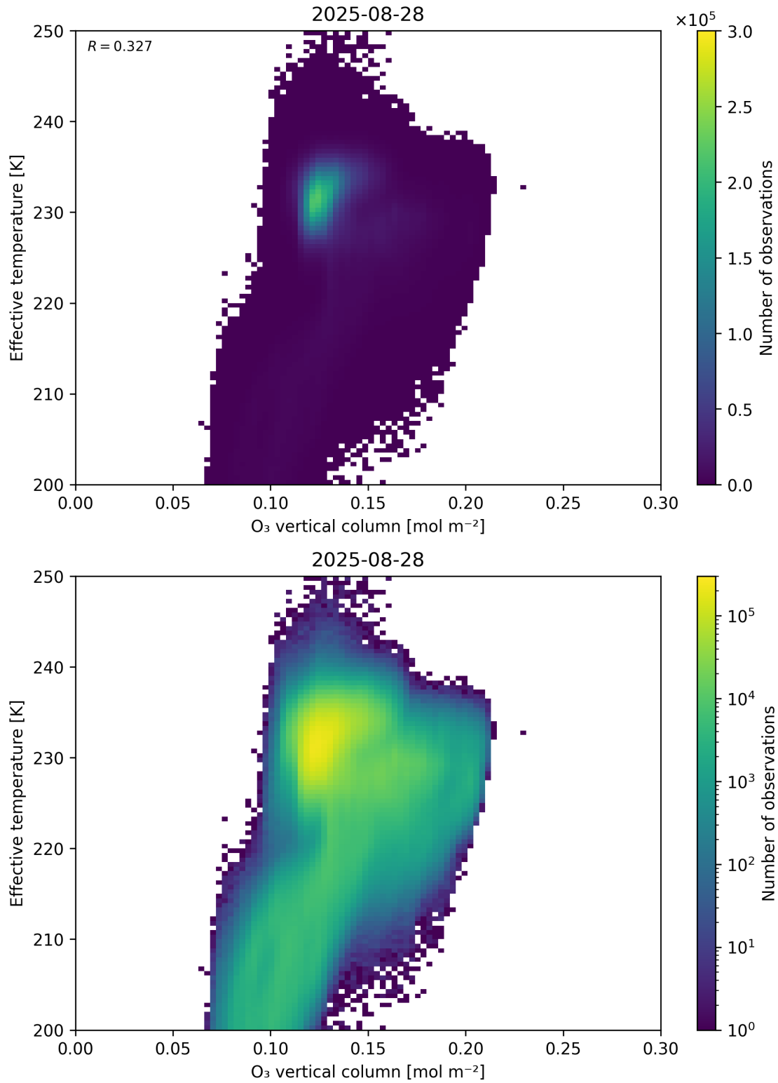
Figure 39: Scatter density plot of “O 3 vertical column” against “Effective temperature” for 2025-08-27 to 2025-08-29.
