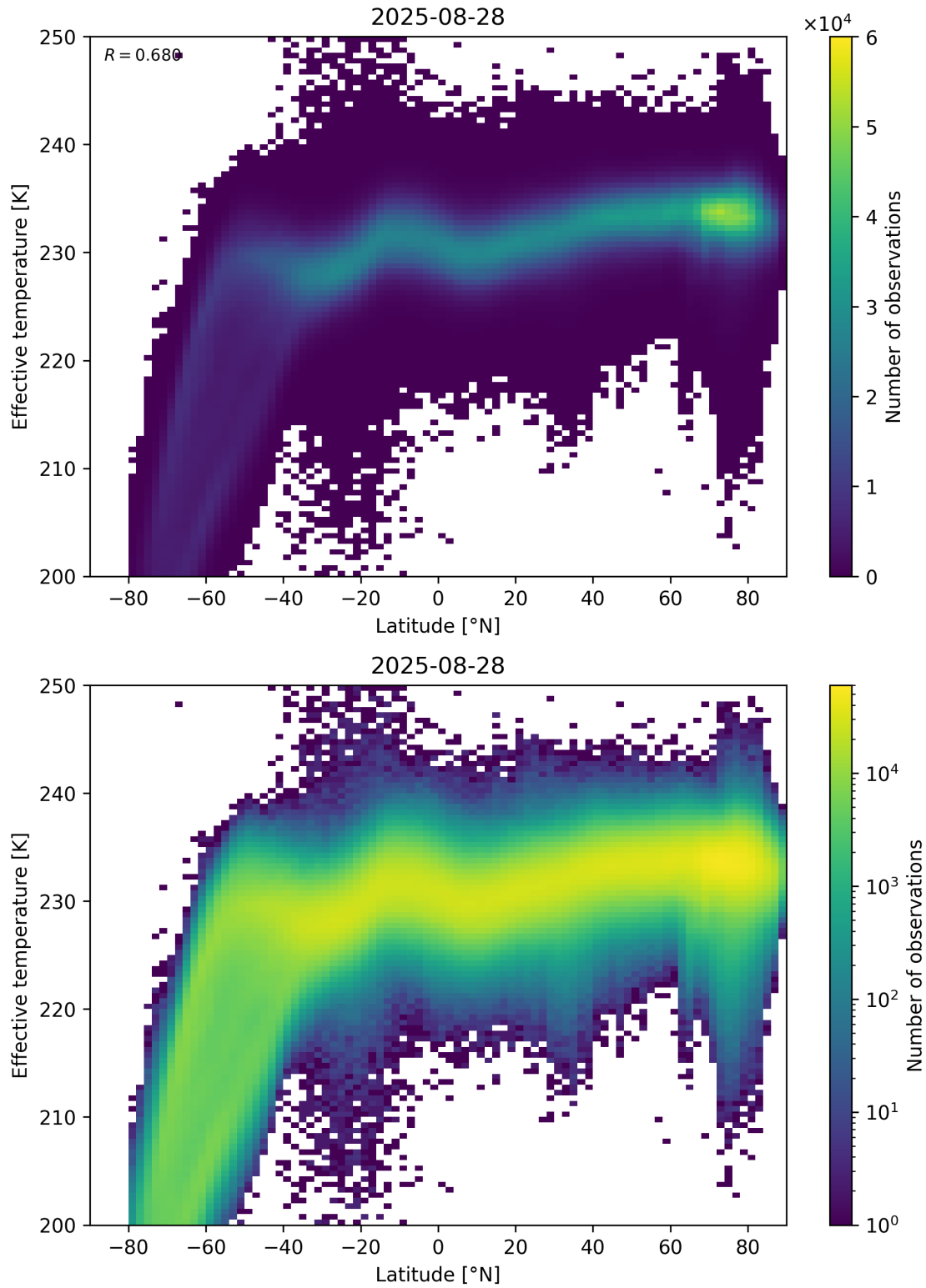
Figure 34: Scatter density plot of “Latitude” against “Effective temperature” for 2025-08-27 to 2025-08-29.
