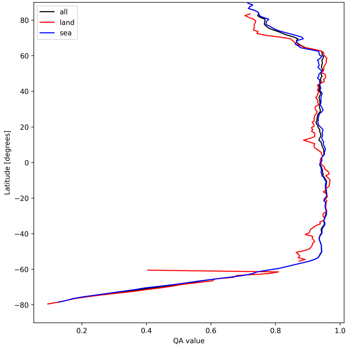
Figure 13: Zonal average of “QA value” for 2025-08-27 to 2025-08-29.
