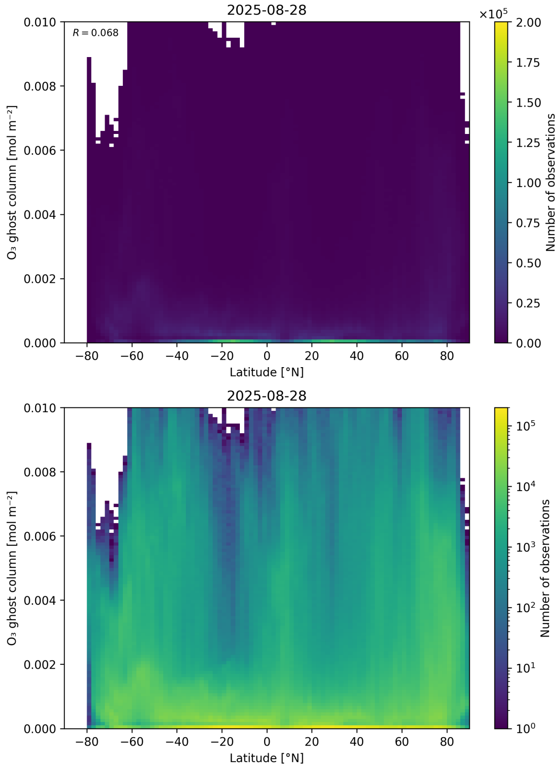
Figure 35: Scatter density plot of “Latitude” against “O 3 ghost column” for 2025-08-27 to 2025-08-29.
