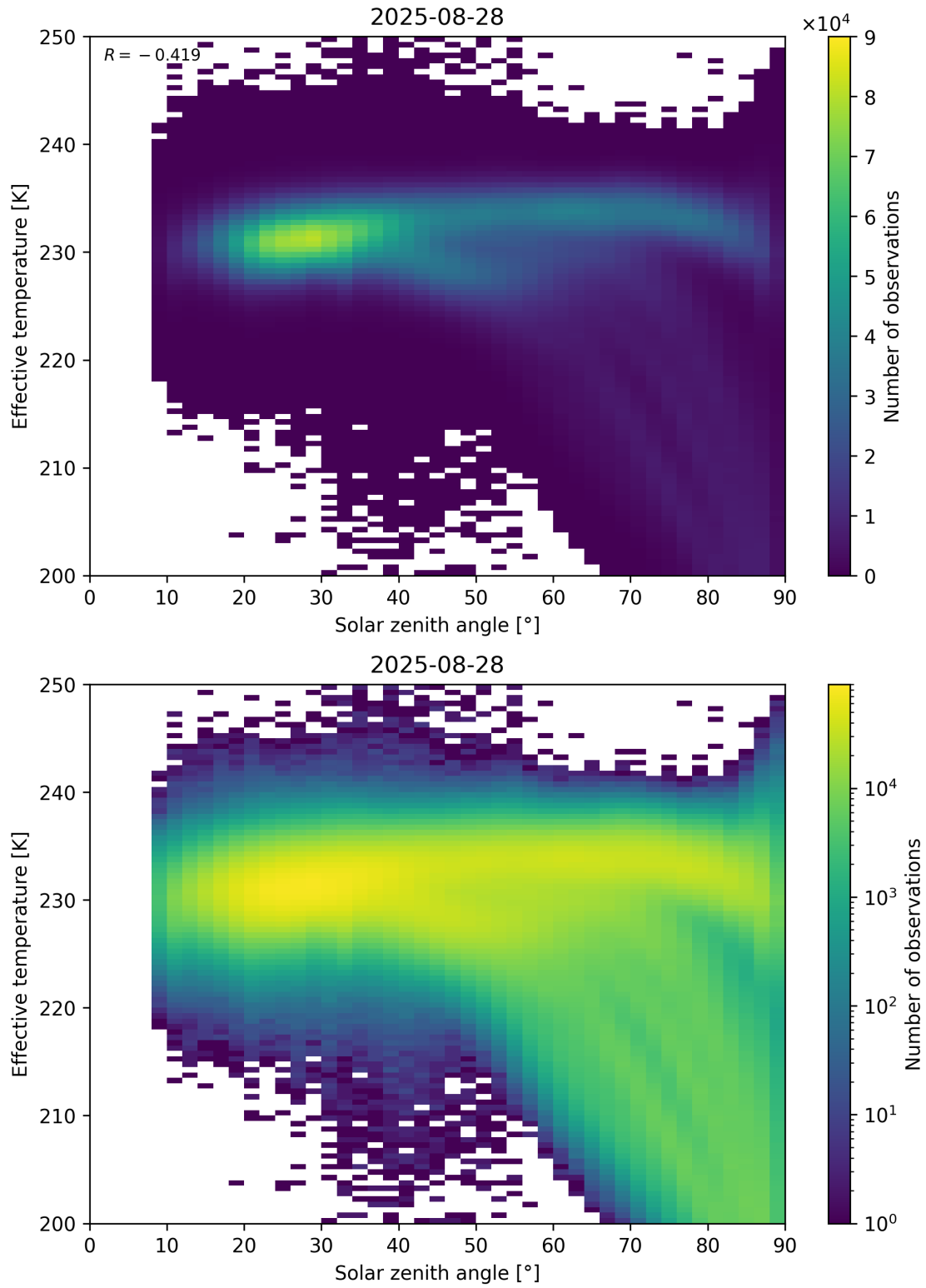
Figure 45: Scatter density plot of “Solar zenith angle” against “Effective temperature” for 2025-08-27 to 2025-08-29.
