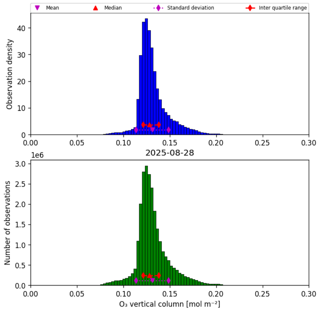
Figure 21: Histogram of “O 3 vertical column” for 2025-08-27 to 2025-08-29
