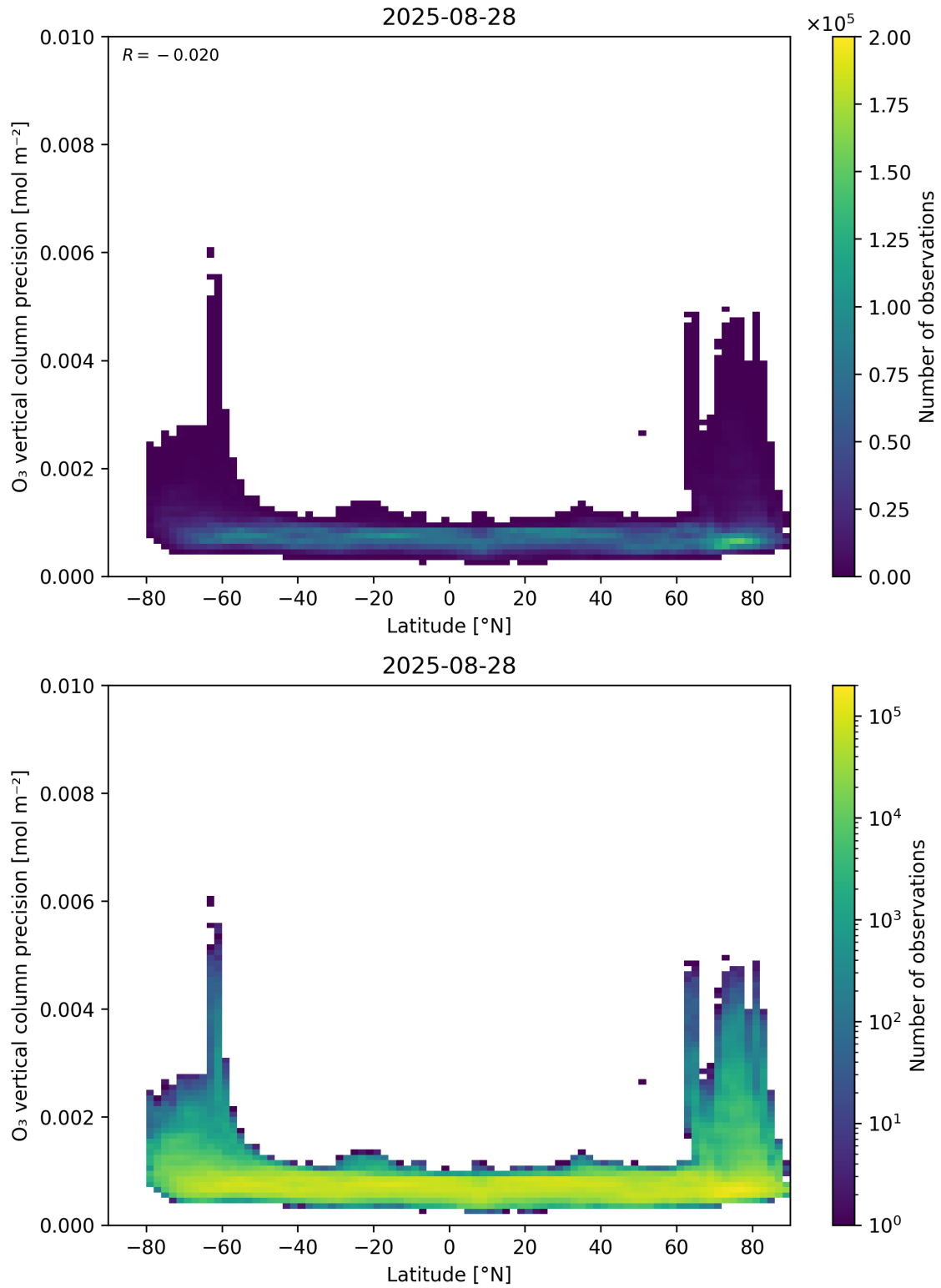
Figure 37: Scatter density plot of “Latitude” against “O 3 vertical column precision” for 2025-08-27 to 2025-08-29.
