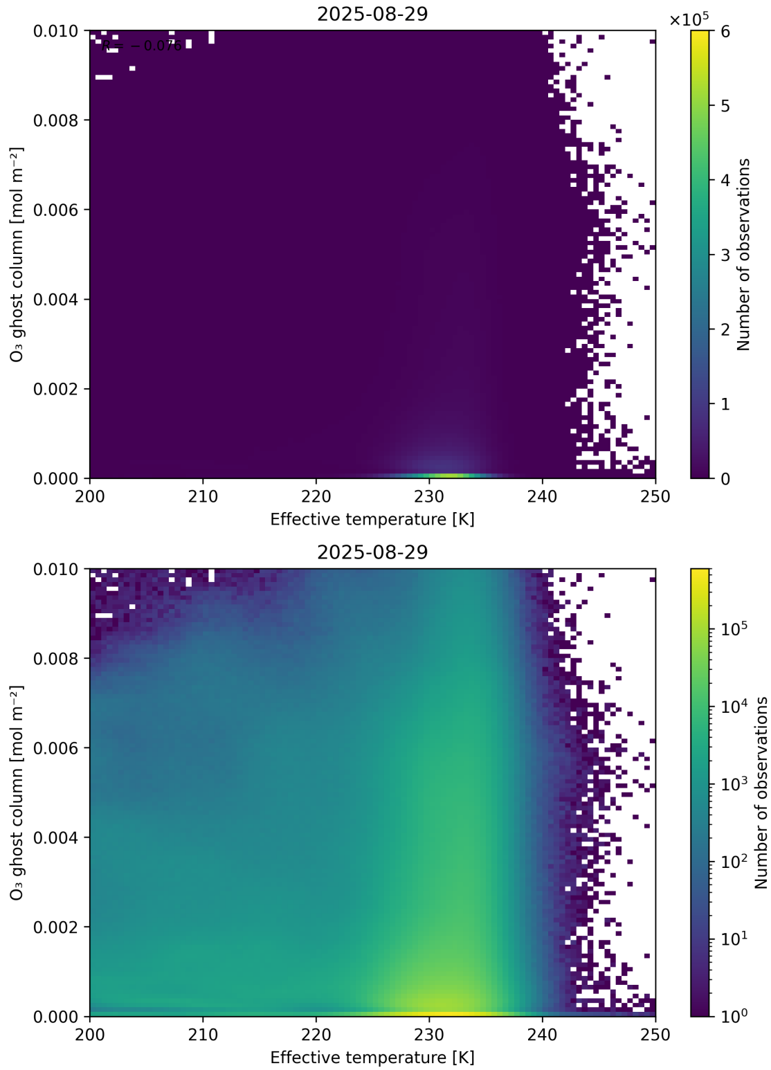
Figure 38: Scatter density plot of “Effective temperature” against “O 3 ghost column” for 2025-08-28 to 2025-08-30.
