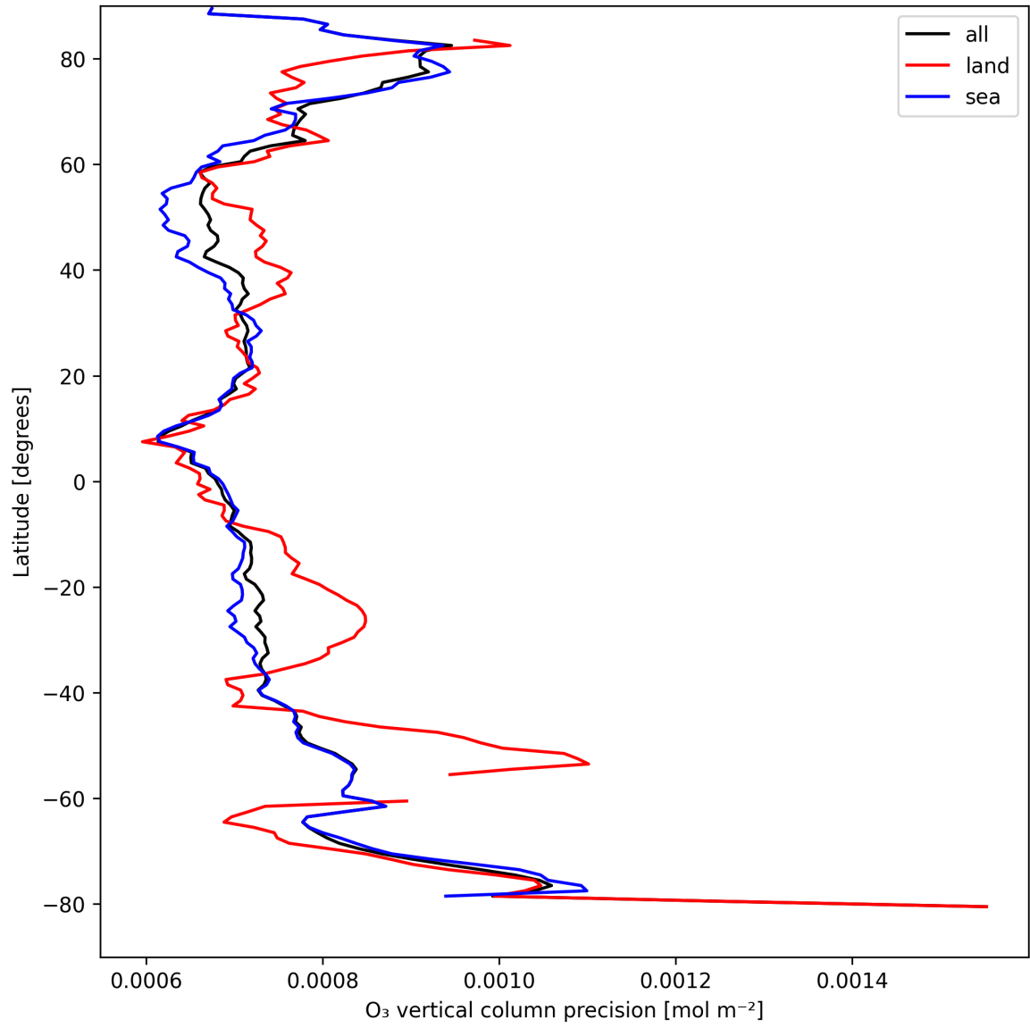
Figure 15: Zonal average of “O 3 vertical column precision” for 2025-08-28 to 2025-08-30.
