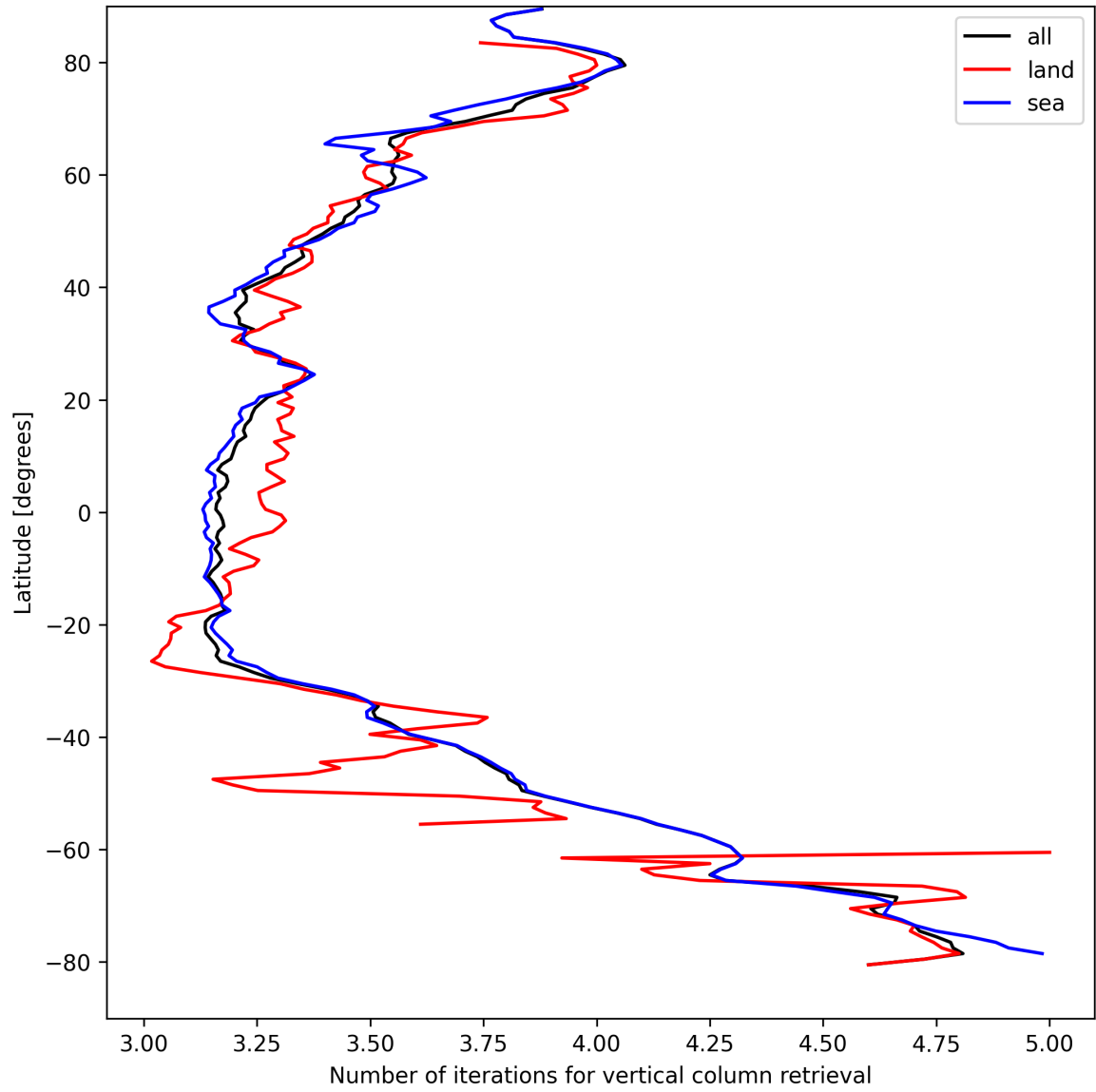
Figure 19: Zonal average of “Number of iterations for vertical column retrieval” for 2025-08-28 to 2025-08-30.
