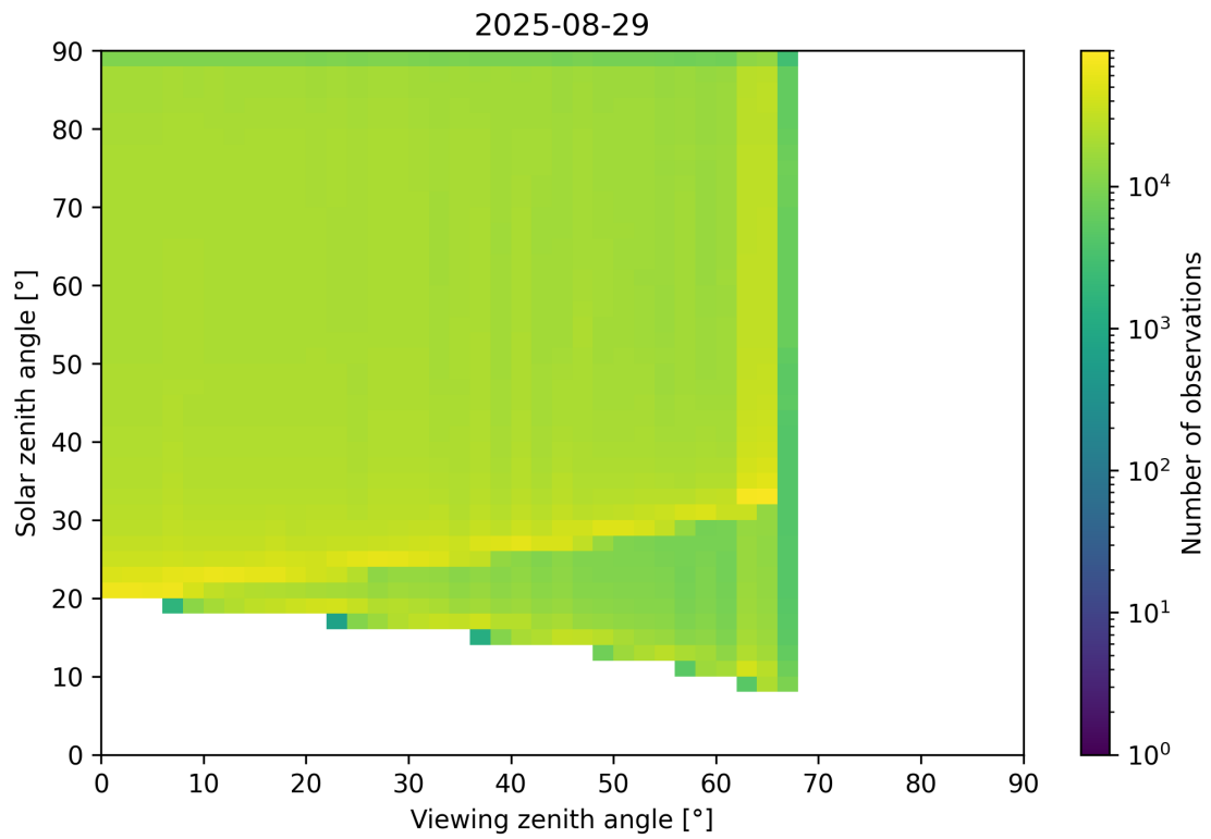
Figure 54: Scatter density plot of “Viewing zenith angle” against “Solar zenith angle” for 2025-08-28 to 2025-08-30.
