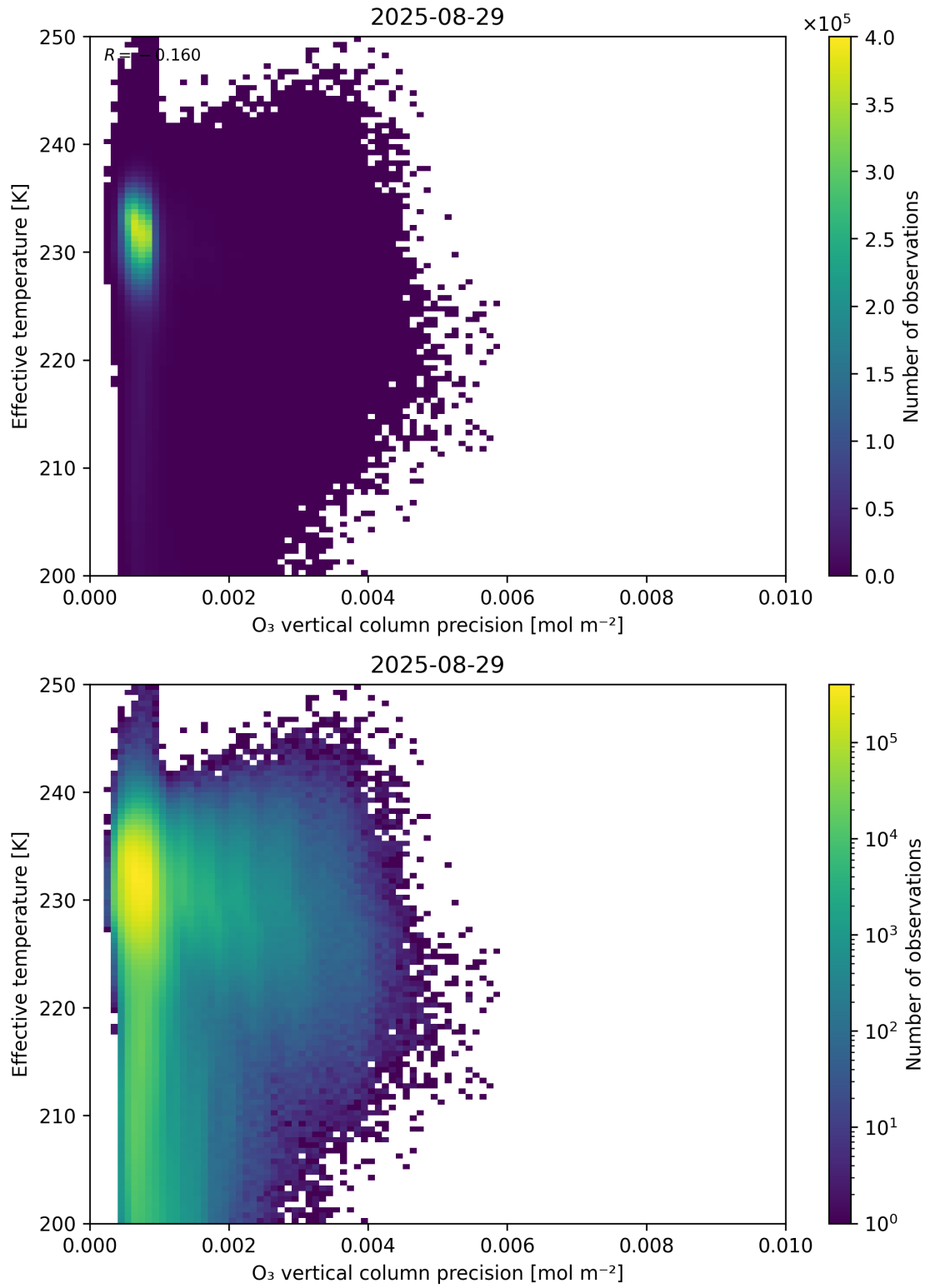
Figure 42: Scatter density plot of “O 3 vertical column precision” against “Effective temperature” for 2025-08-28 to 2025-08-30.
