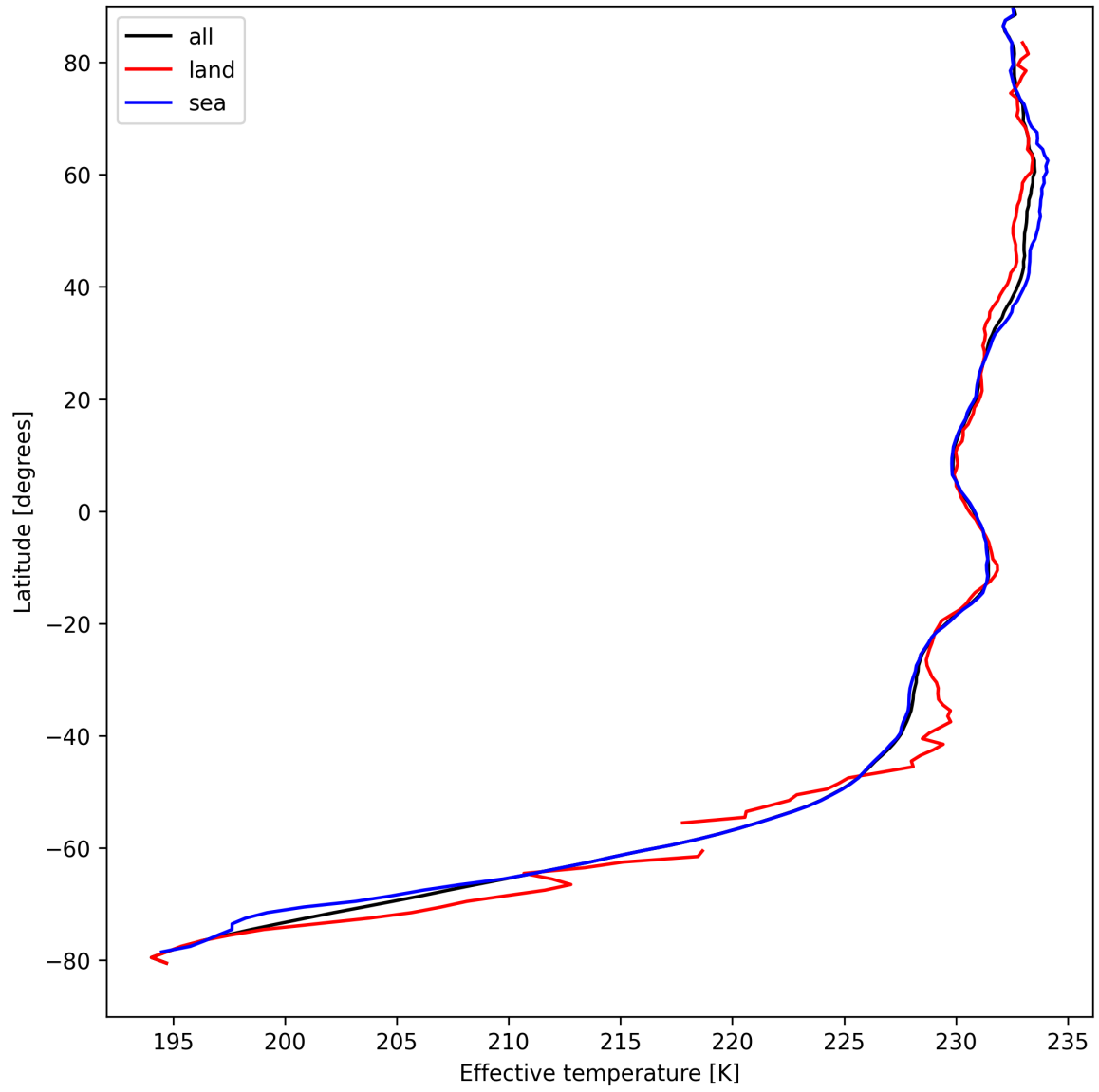
Figure 17: Zonal average of "Effective temperature" for 2025-08-28 to 2025-08-30.
