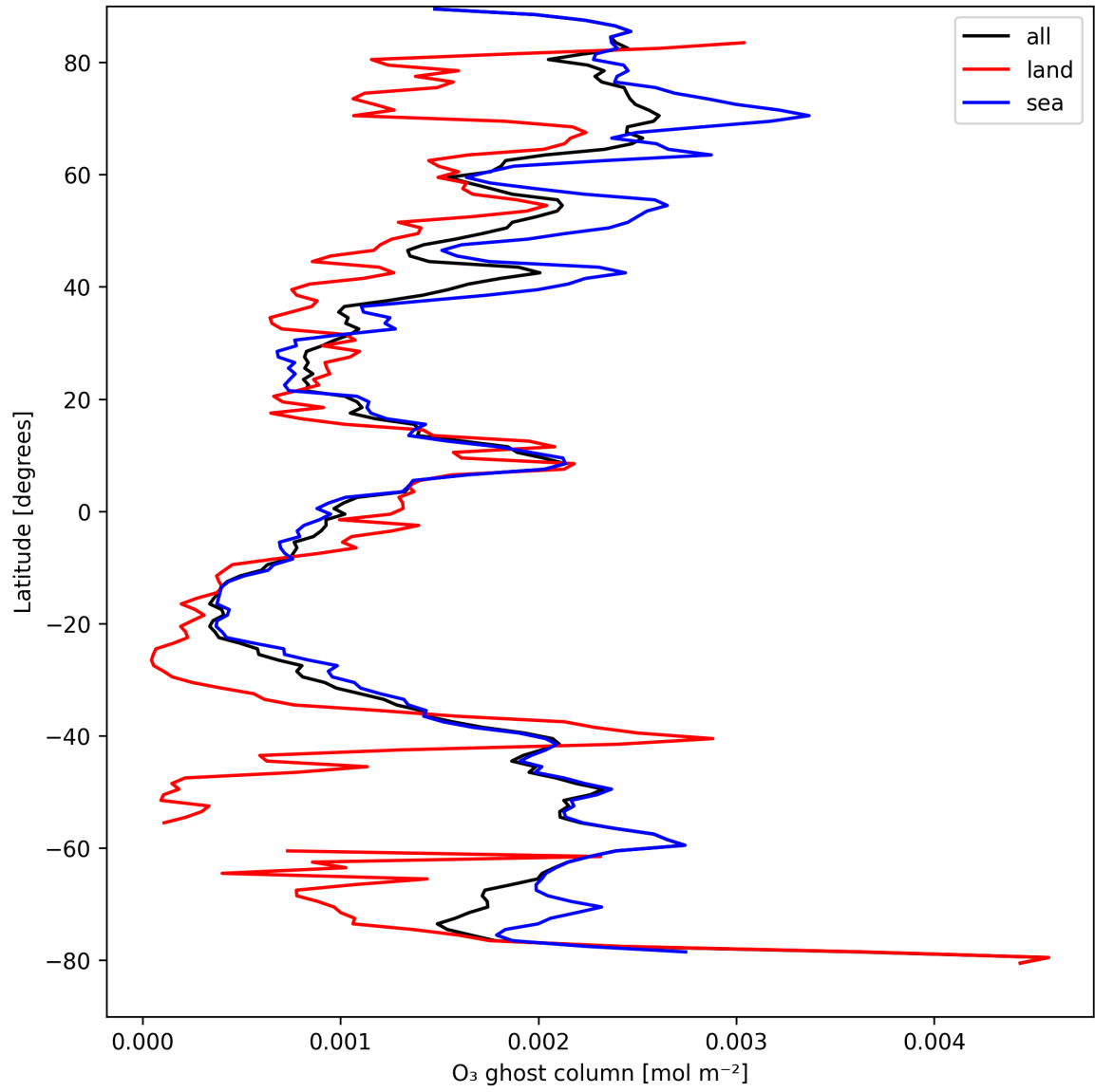
Figure 18: Zonal average of "O 3 ghost column" for 2025-08-28 to 2025-08-30.
