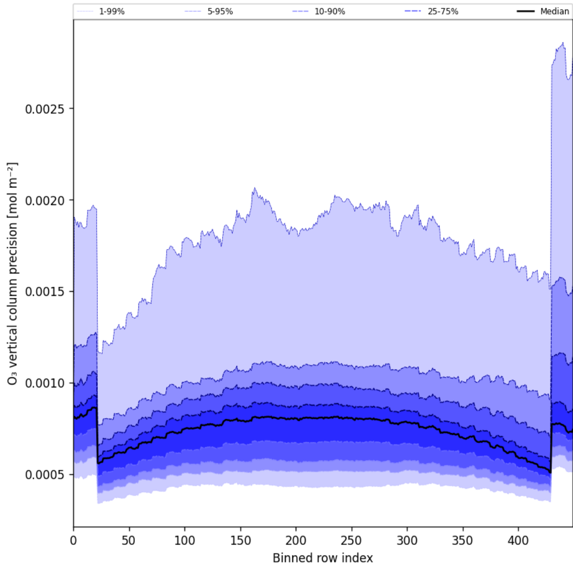
Figure 29: Along track statistics of “O 3 vertical column precision” for 2025-08-28 to 2025-08-30
