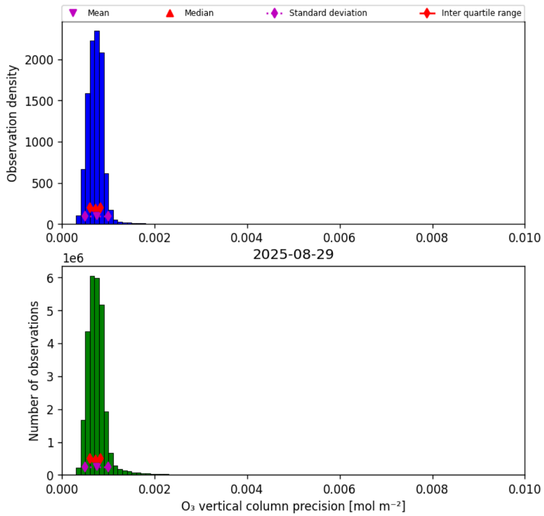
Figure 22: Histogram of “O 3 vertical column precision” for 2025-08-28 to 2025-08-30
