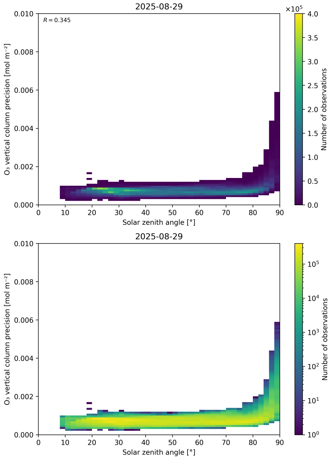
Figure 48: Scatter density plot of “Solar zenith angle” against “O 3 vertical column precision” for 2025-08-28 to 2025-08-30.
