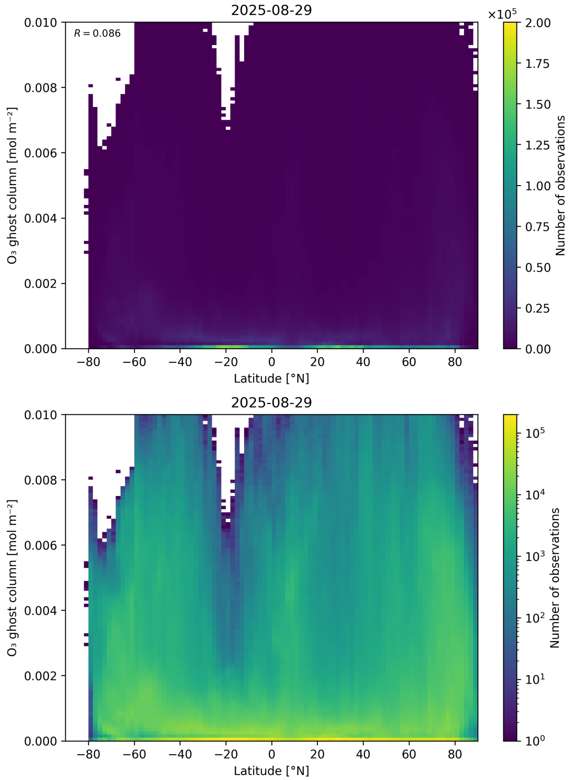
Figure 35: Scatter density plot of “Latitude” against “O 3 ghost column” for 2025-08-28 to 2025-08-30.
