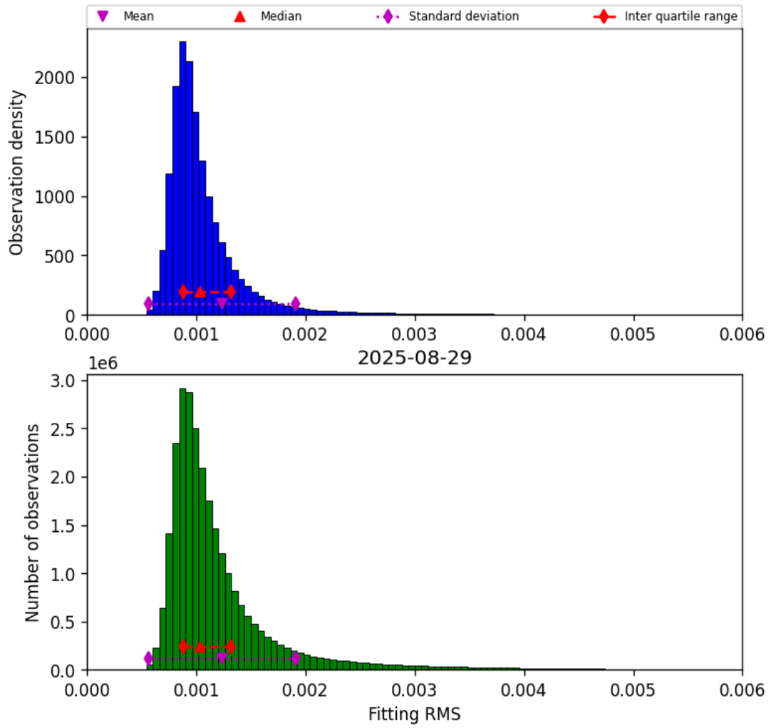
Figure 23: Histogram of “Fitting RMS” for 2025-08-28 to 2025-08-30
