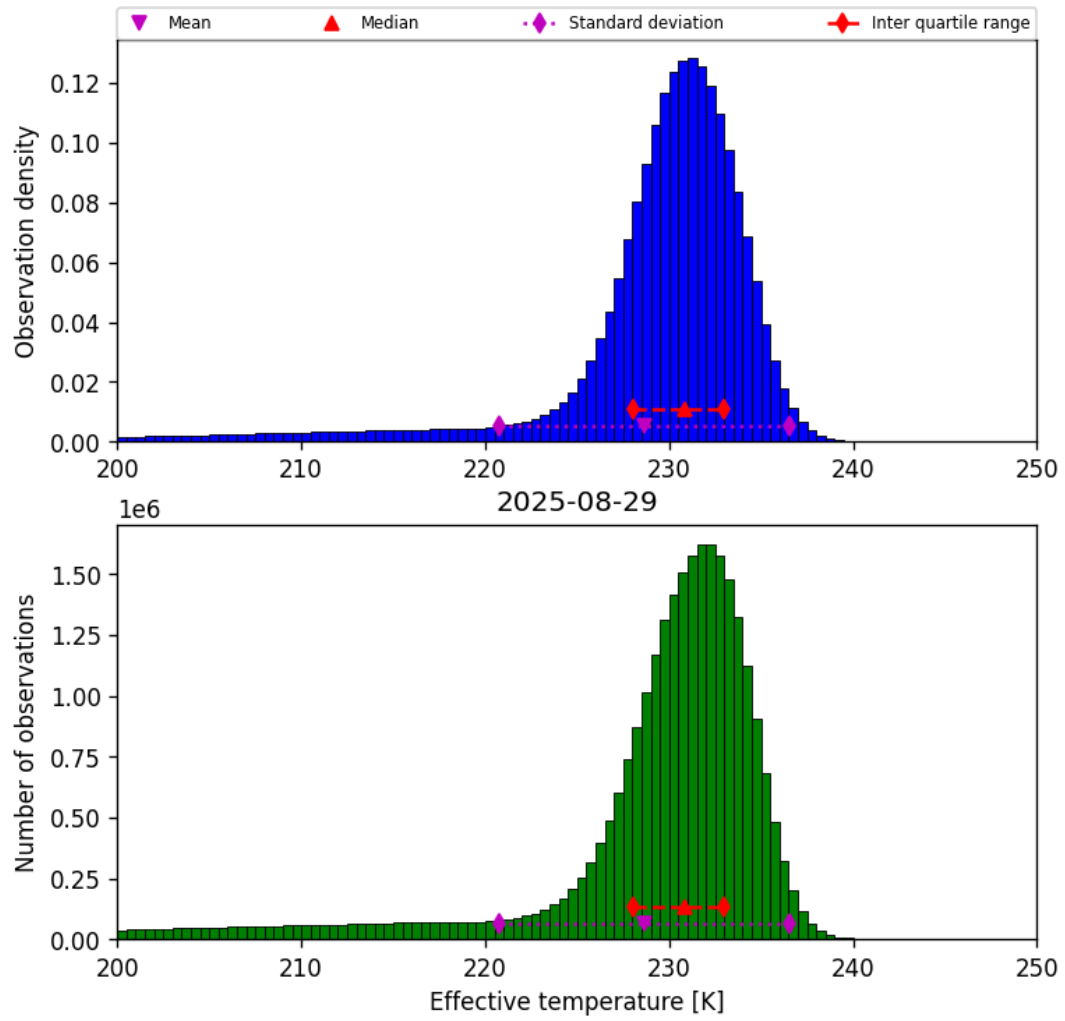
Figure 24: Histogram of “Effective temperature” for 2025-08-28 to 2025-08-30
