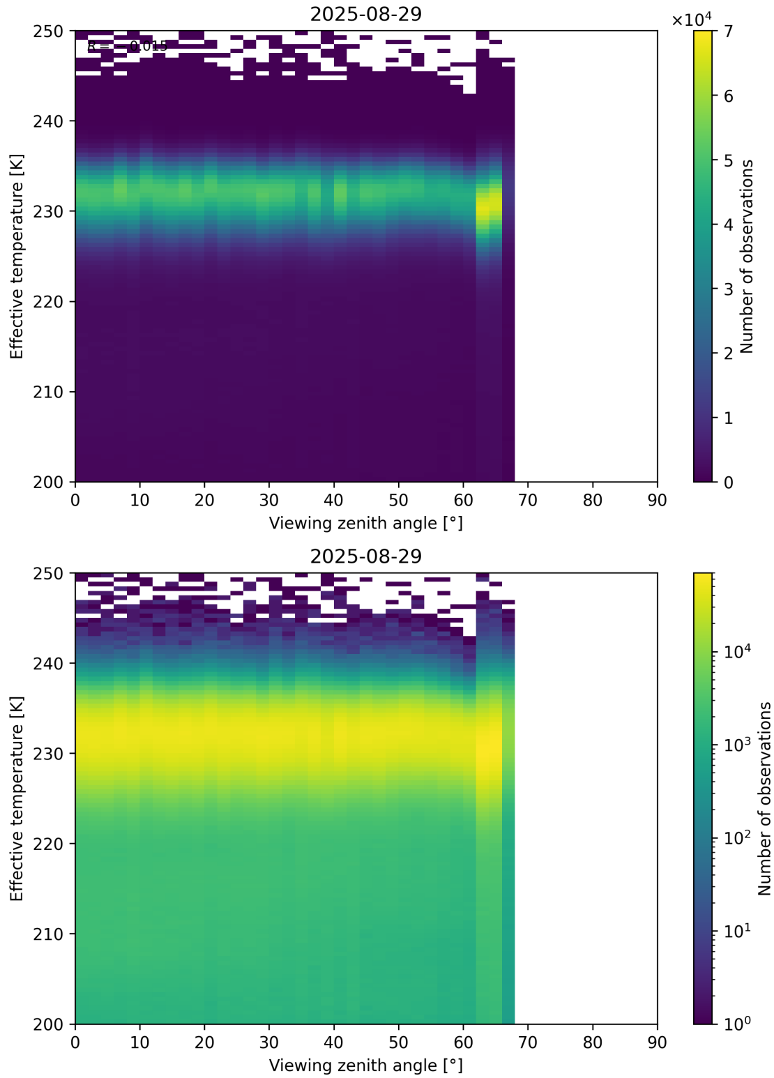
Figure 50: Scatter density plot of “Viewing zenith angle” against “Effective temperature” for 2025-08-28 to 2025-08-30.
