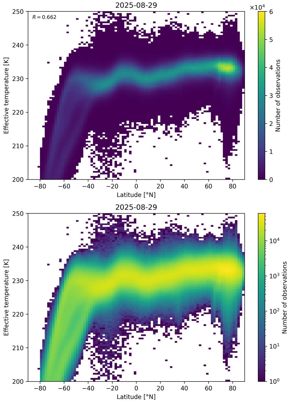
Figure 34: Scatter density plot of “Latitude” against “Effective temperature” for 2025-08-28 to 2025-08-30.
