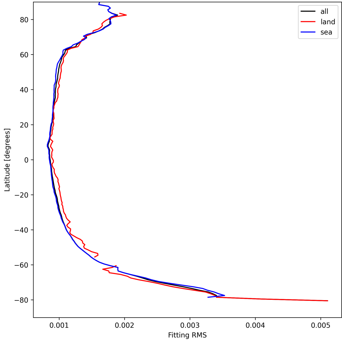
Figure 16: Zonal average of “Fitting RMS” for 2025-08-28 to 2025-08-30.
