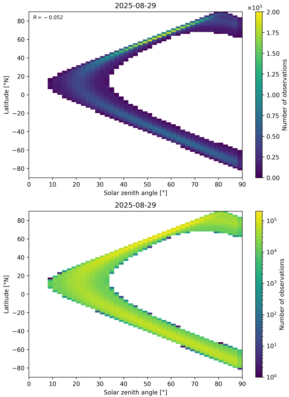
Figure 44: Scatter density plot of “Solar zenith angle” against “Latitude” for 2025-08-28 to 2025-08-30.
