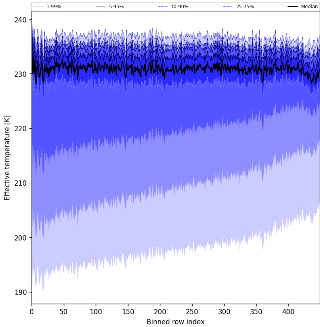
Figure 31: Along track statistics of “Effective temperature” for 2025-08-28 to 2025-08-30
