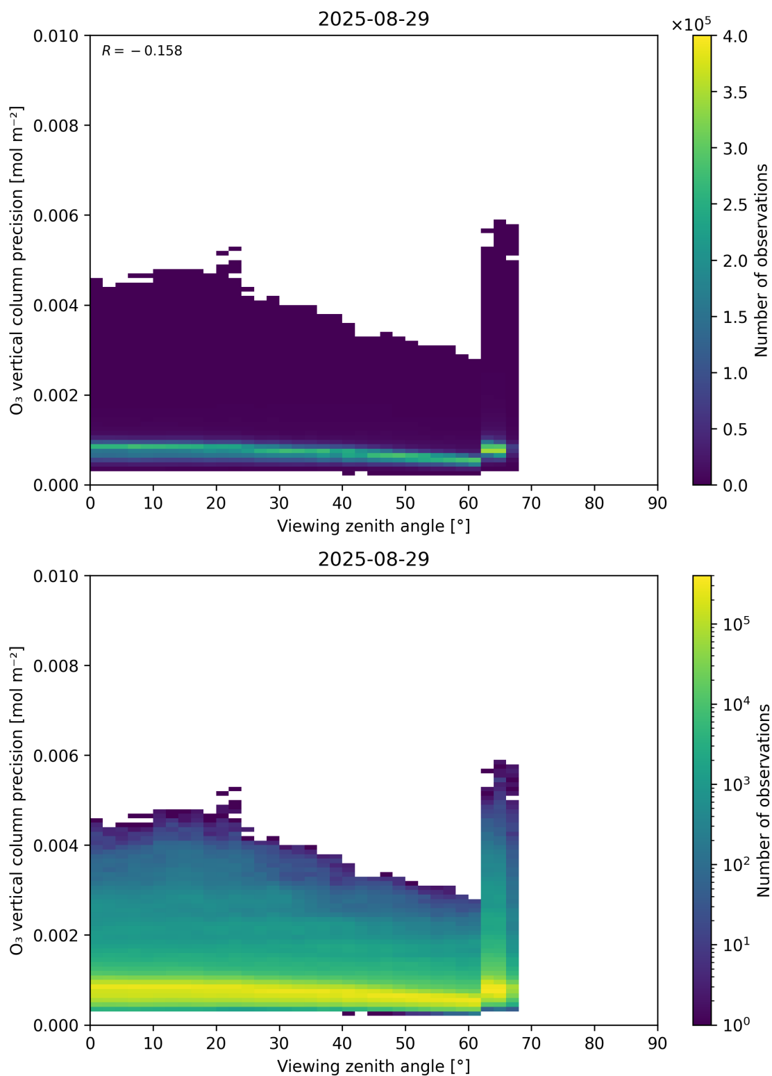
Figure 53: Scatter density plot of “Viewing zenith angle” against “O 3 vertical column precision” for 2025-08-28 to 2025-08-30.
