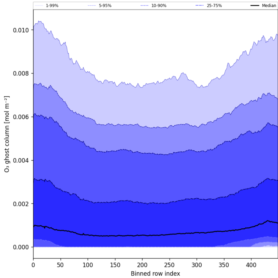
Figure 32: Along track statistics of “O 3 ghost column” for 2025-08-28 to 2025-08-30
