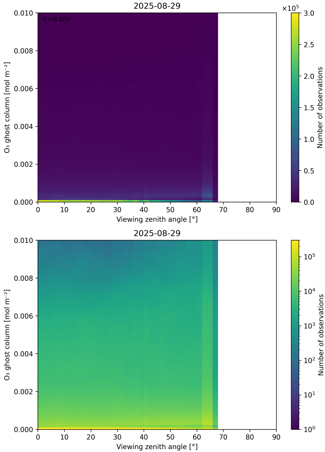
Figure 51: Scatter density plot of “Viewing zenith angle” against “O 3 ghost column” for 2025-08-28 to 2025-08-30.
