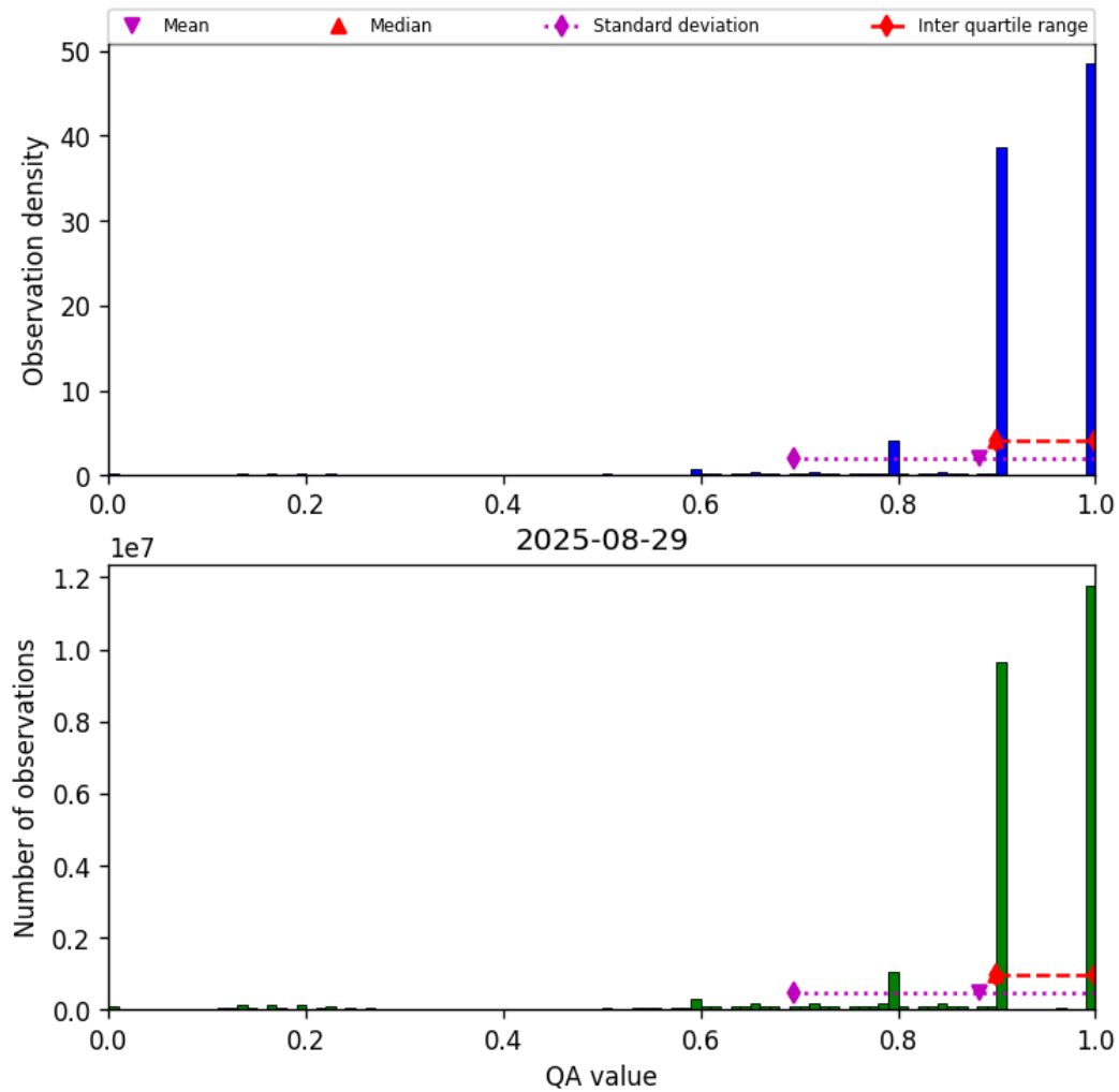
Figure 20: Histogram of “QA value” for 2025-08-28 to 2025-08-30
