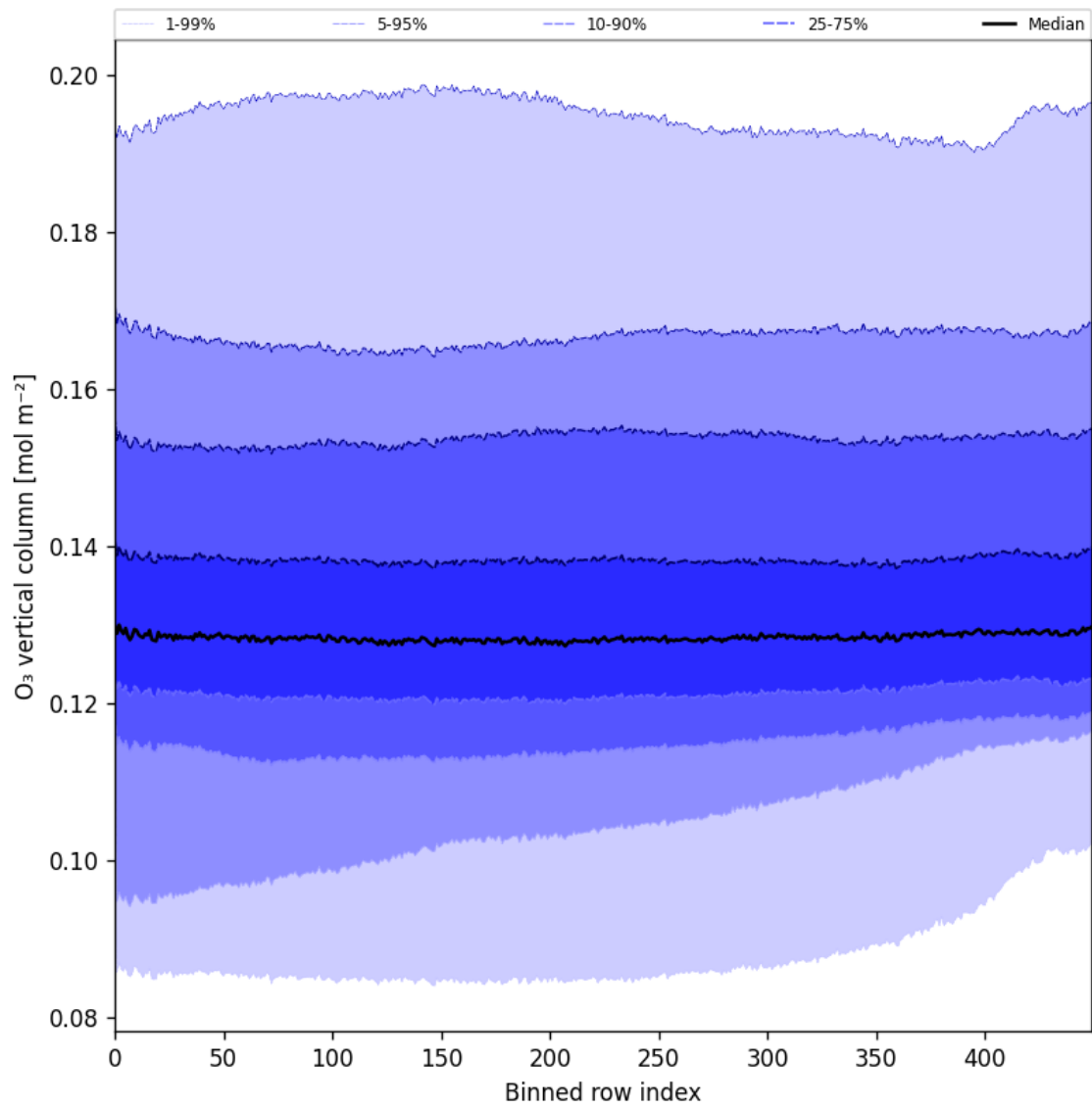
Figure 28: Along track statistics of “O 3 vertical column” for 2025-08-28 to 2025-08-30
