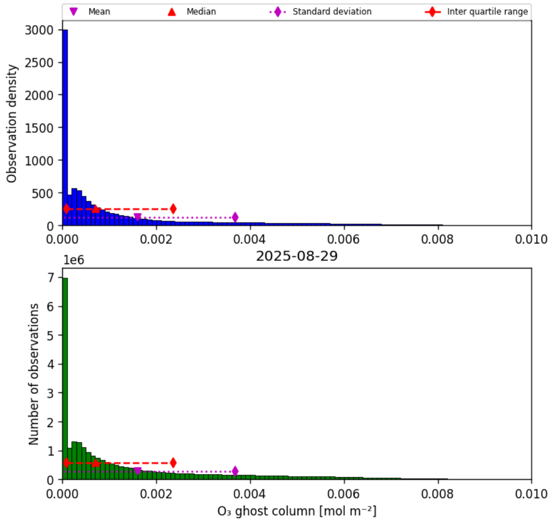
Figure 25: Histogram of “O 3 ghost column” for 2025-08-28 to 2025-08-30
