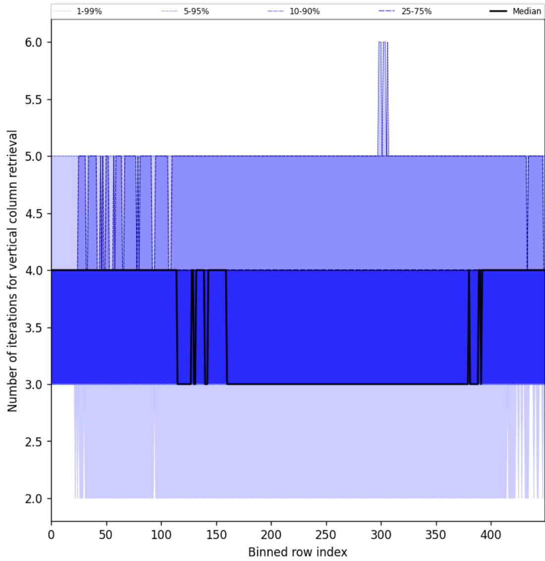
Figure 33: Along track statistics of “Number of iterations for vertical column retrieval” for 2025-08-28 to 2025-08-30
