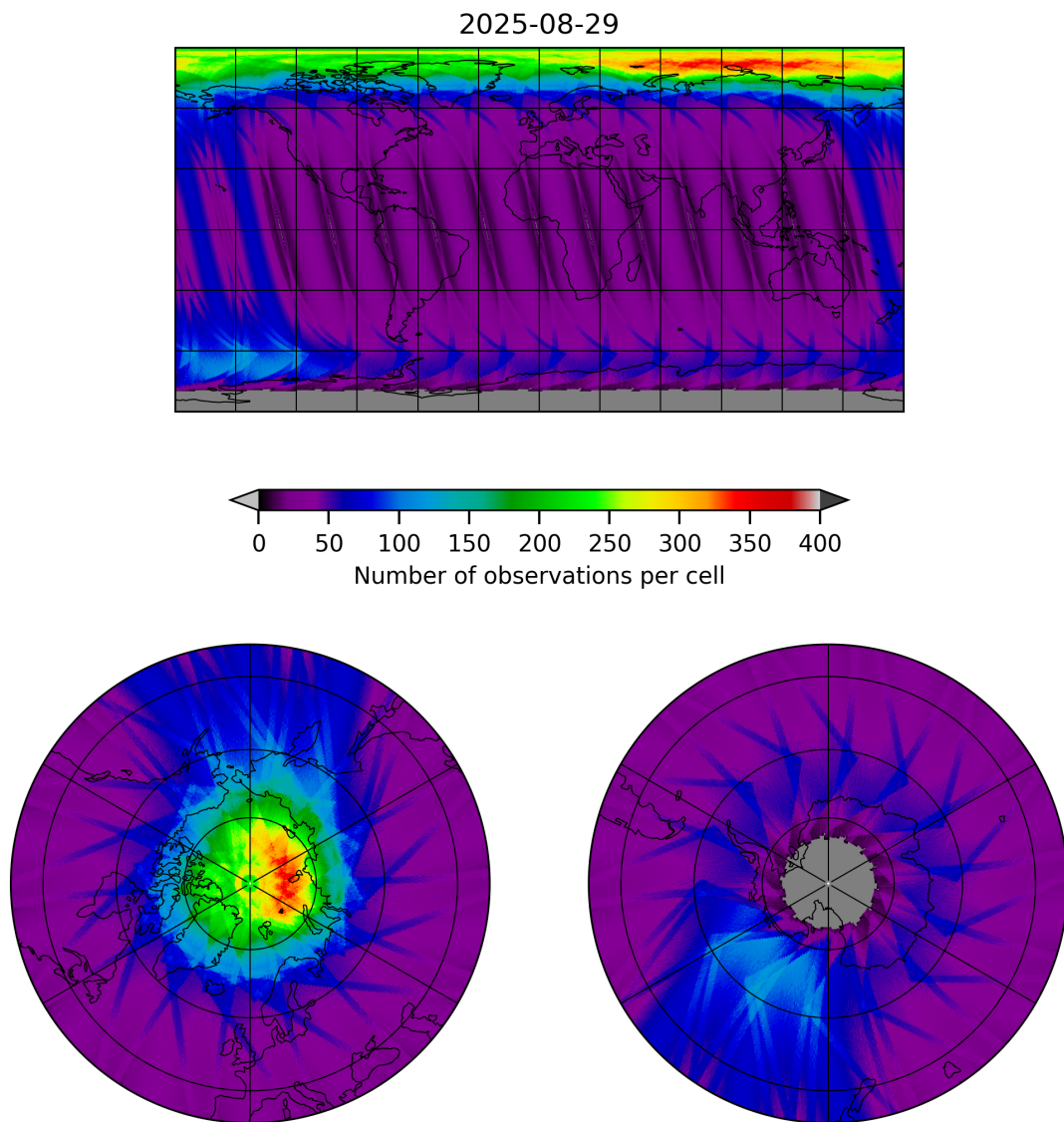
Figure 12: Map of the number of observations for 2025-08-28 to 2025-08-30
