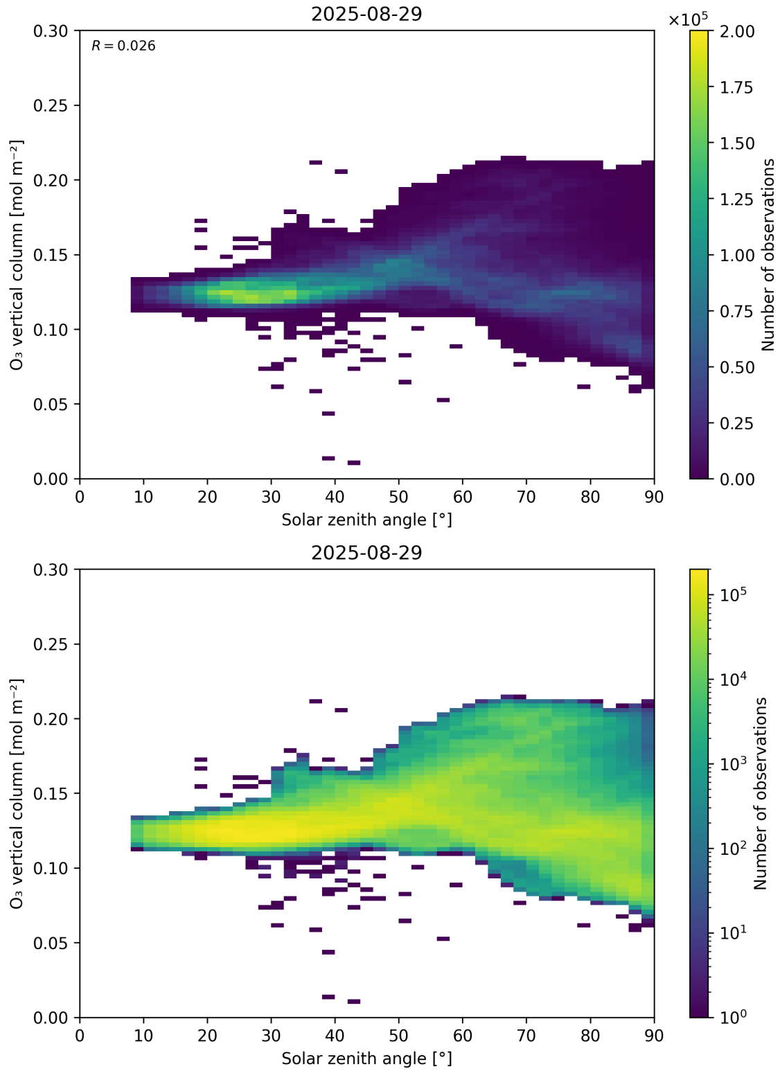
Figure 47: Scatter density plot of “Solar zenith angle” against “O 3 vertical column” for 2025-08-28 to 2025-08-30.
