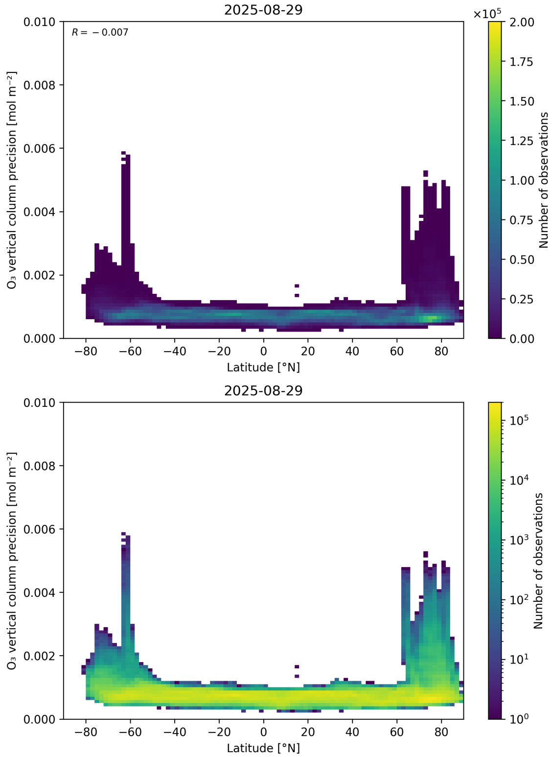
Figure 37: Scatter density plot of “Latitude” against “O 3 vertical column precision” for 2025-08-28 to 2025-08-30.
