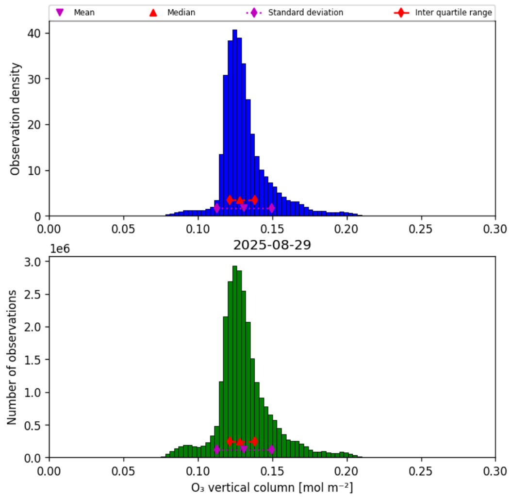
Figure 21: Histogram of “O 3 vertical column” for 2025-08-28 to 2025-08-30
