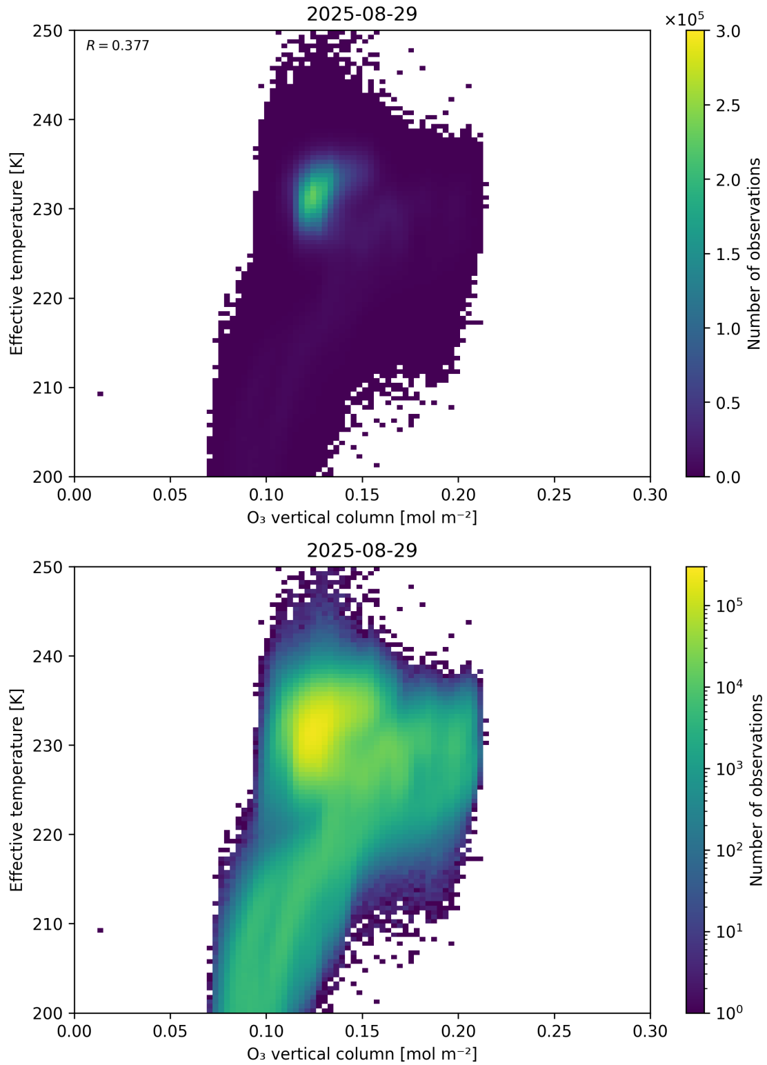
Figure 39: Scatter density plot of “O 3 vertical column” against “Effective temperature” for 2025-08-28 to 2025-08-30.
