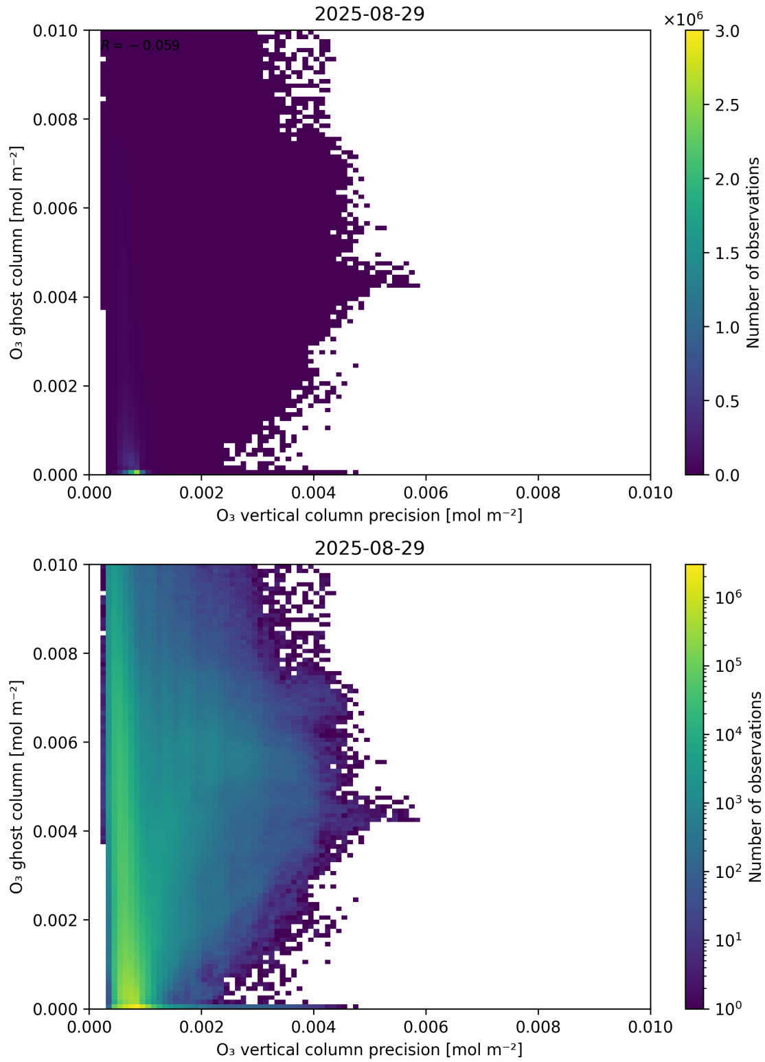
Figure 43: Scatter density plot of “ \text{O}_3 vertical column precision” against “ \text{O}_3 ghost column” for 2025-08-28 to 2025-08-30.
