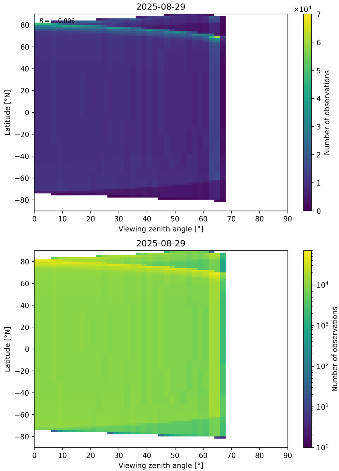
Figure 49: Scatter density plot of “Viewing zenith angle” against “Latitude” for 2025-08-28 to 2025-08-30.
