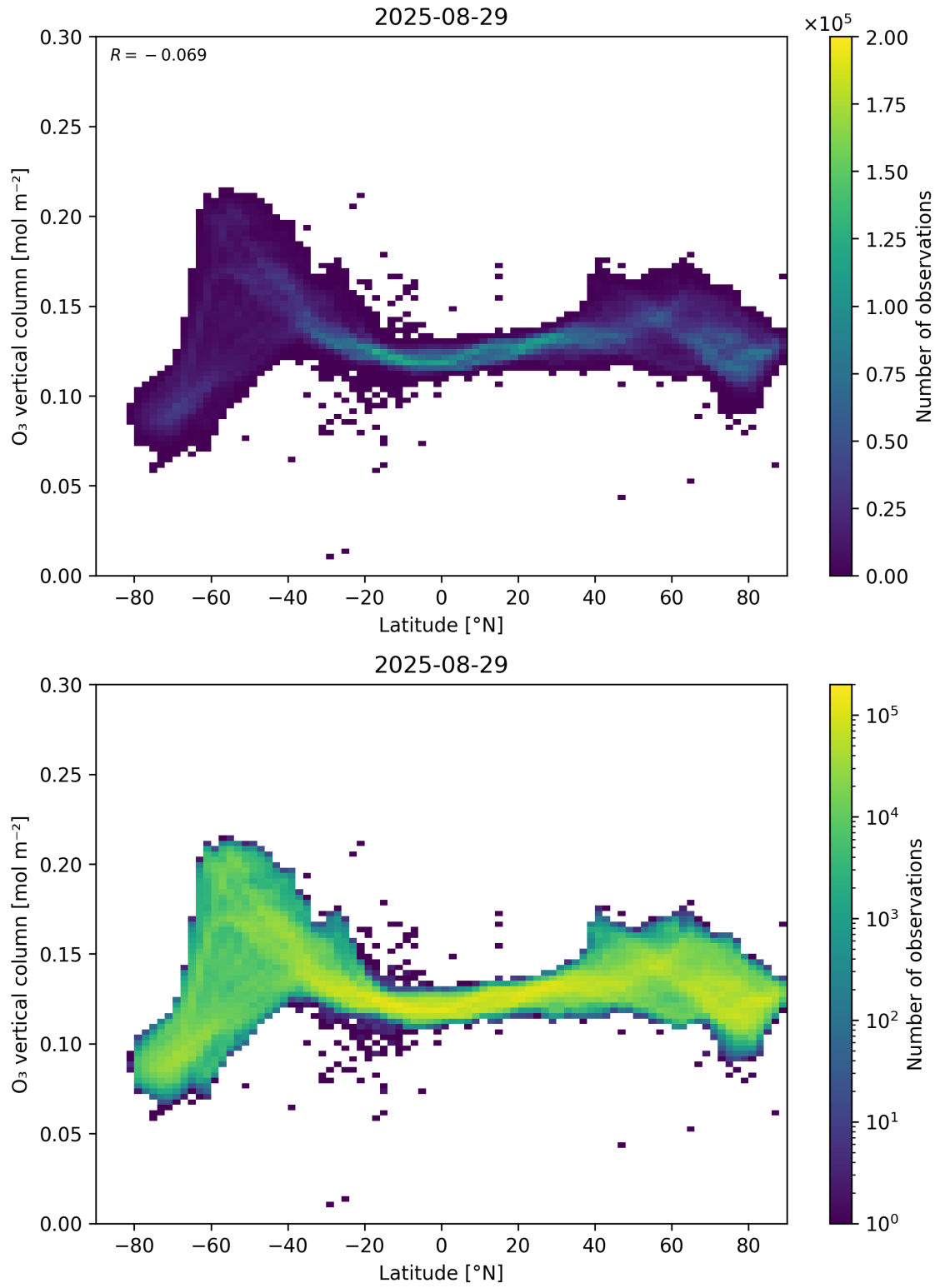
Figure 36: Scatter density plot of “Latitude” against “O 3 vertical column” for 2025-08-28 to 2025-08-30.
