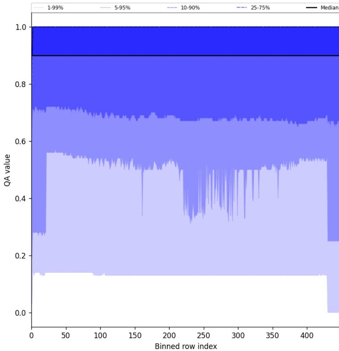
Figure 27: Along track statistics of “QA value” for 2025-08-28 to 2025-08-30
