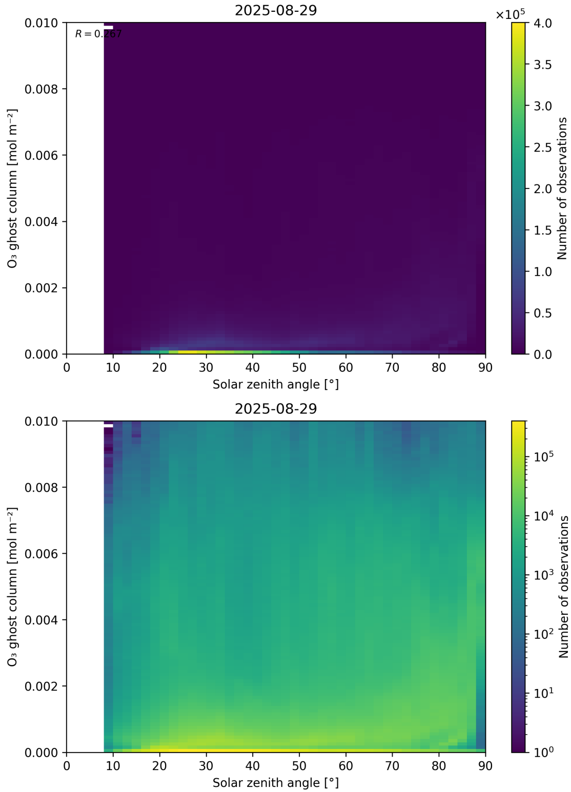
Figure 46: Scatter density plot of “Solar zenith angle” against “O 3 ghost column” for 2025-08-28 to 2025-08-30.
