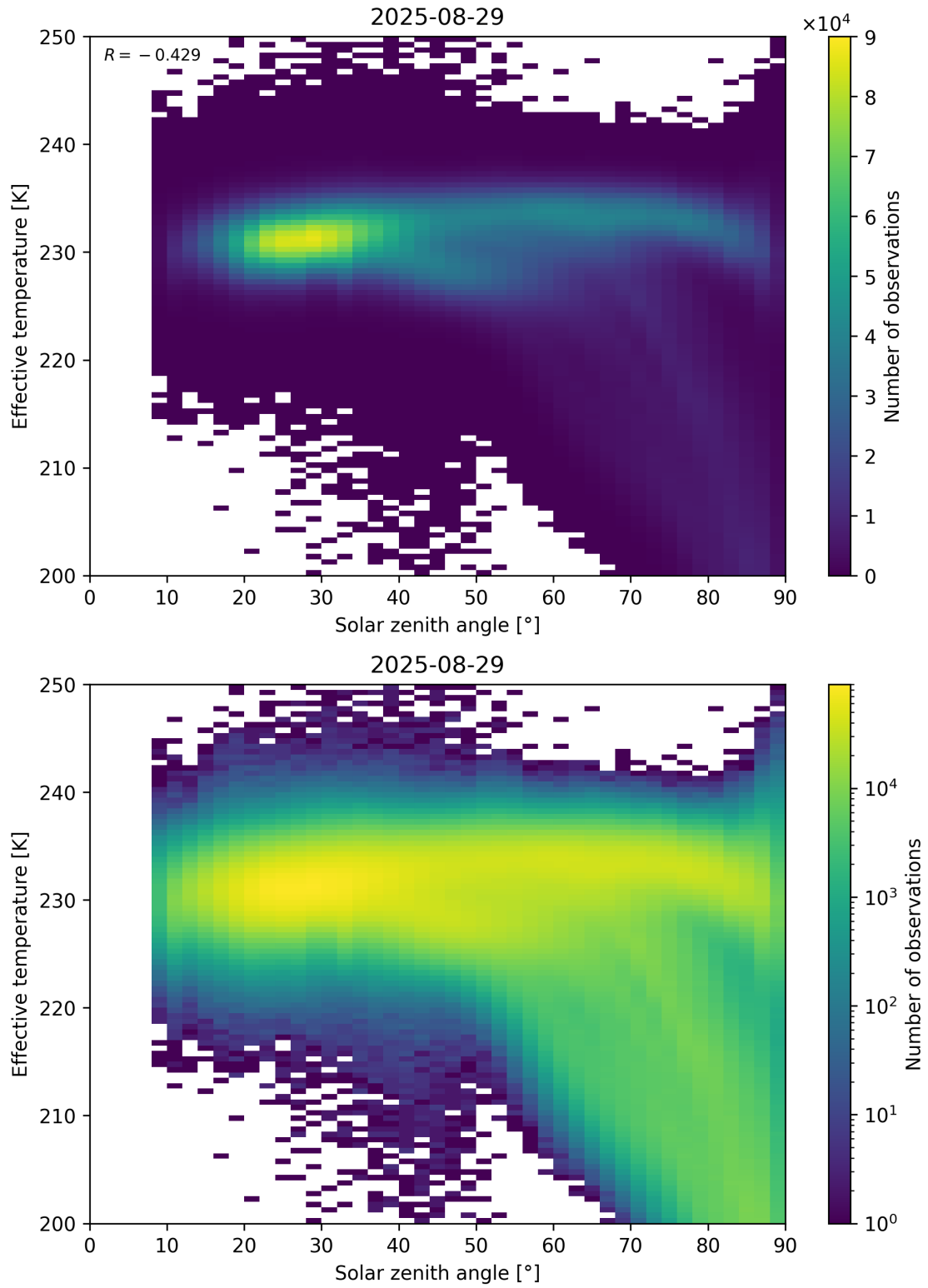
Figure 45: Scatter density plot of “Solar zenith angle” against “Effective temperature” for 2025-08-28 to 2025-08-30.
