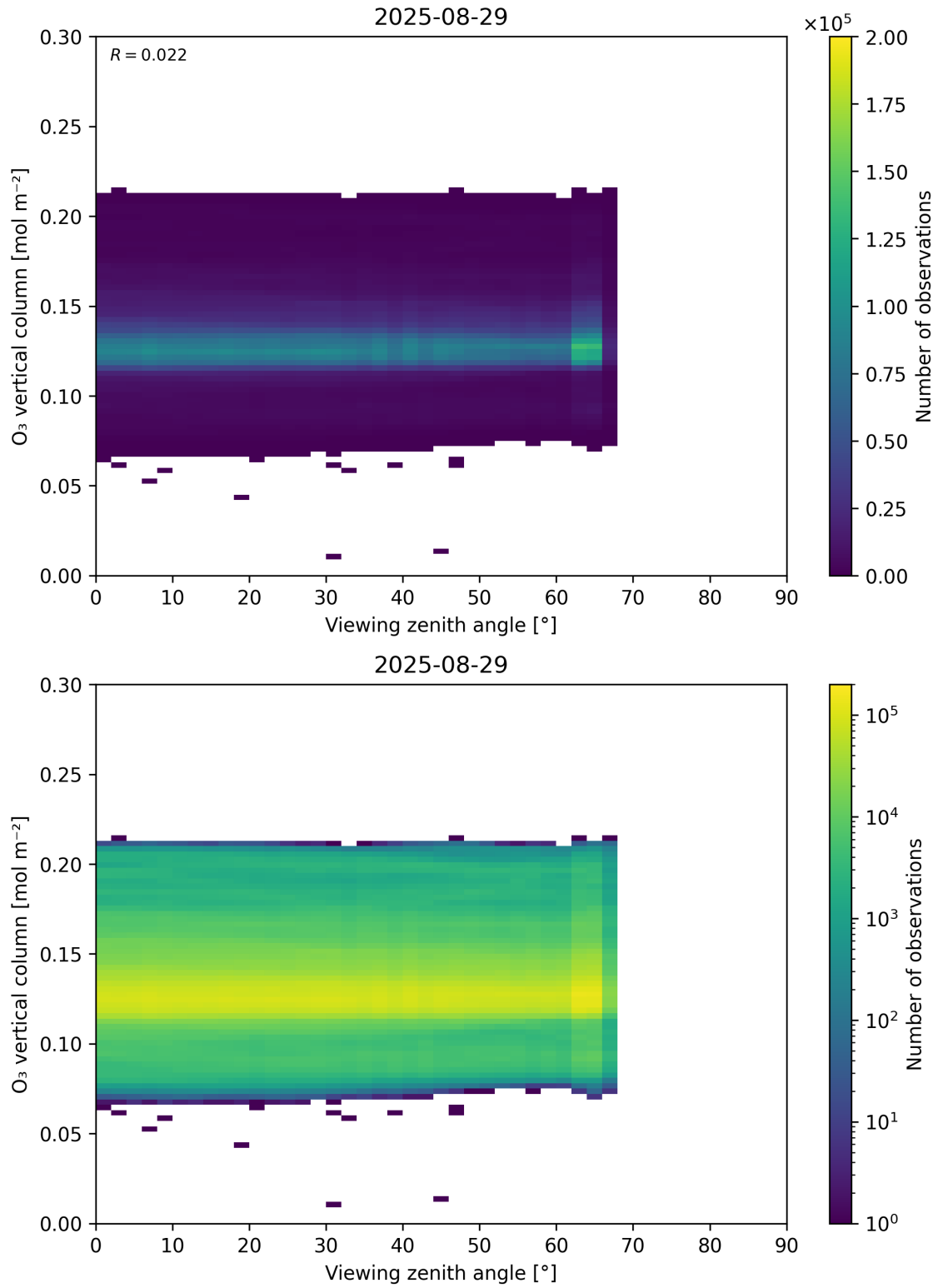
Figure 52: Scatter density plot of “Viewing zenith angle” against “O 3 vertical column” for 2025-08-28 to 2025-08-30.
