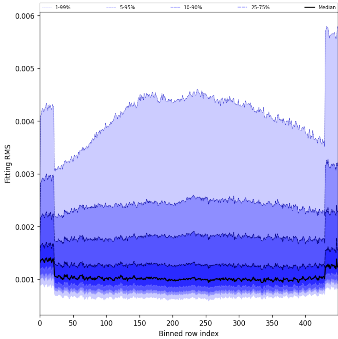
Figure 30: Along track statistics of “Fitting RMS” for 2025-08-28 to 2025-08-30
