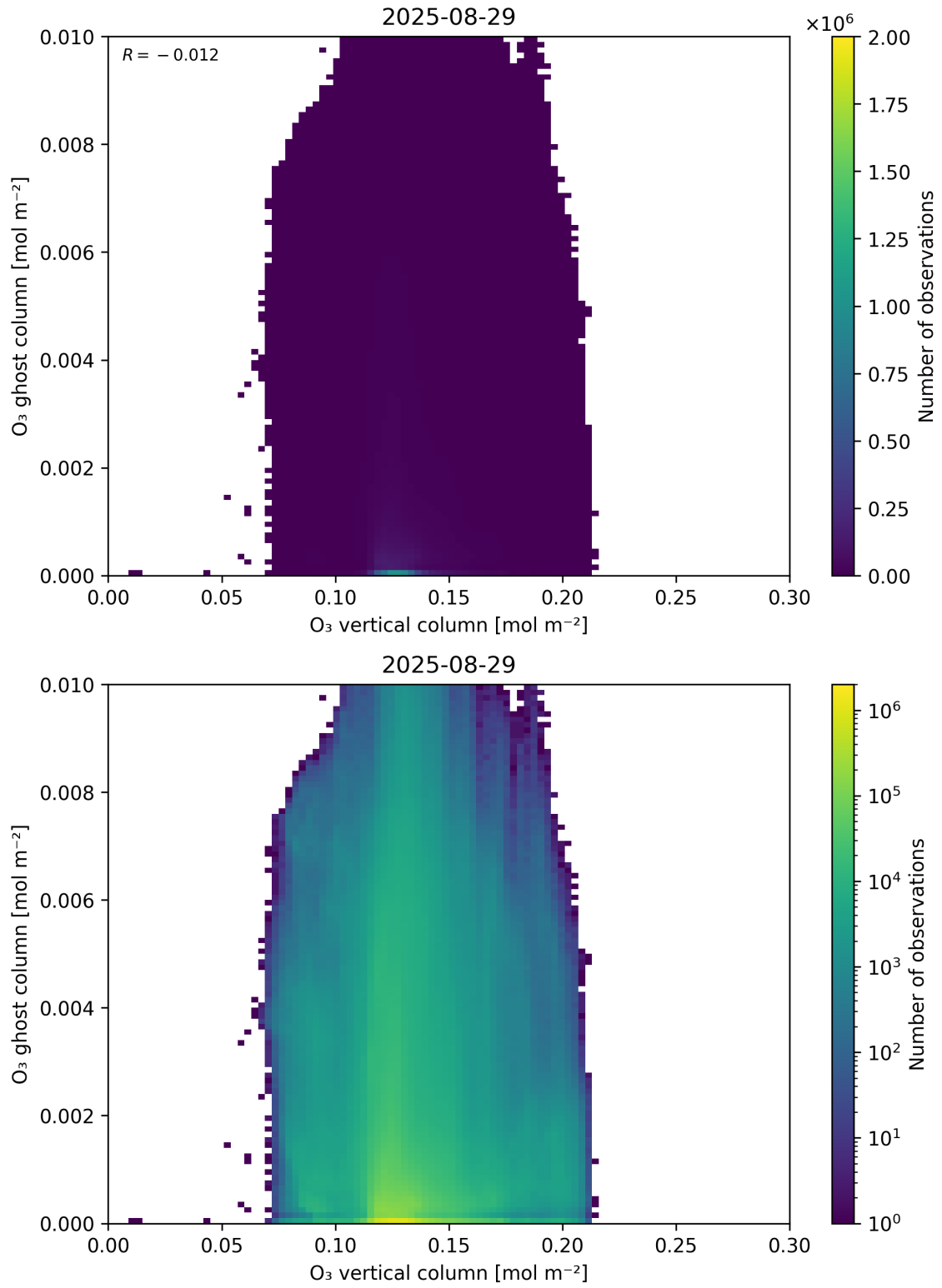
Figure 40: Scatter density plot of “O 3 vertical column” against “O 3 ghost column” for 2025-08-28 to 2025-08-30.
