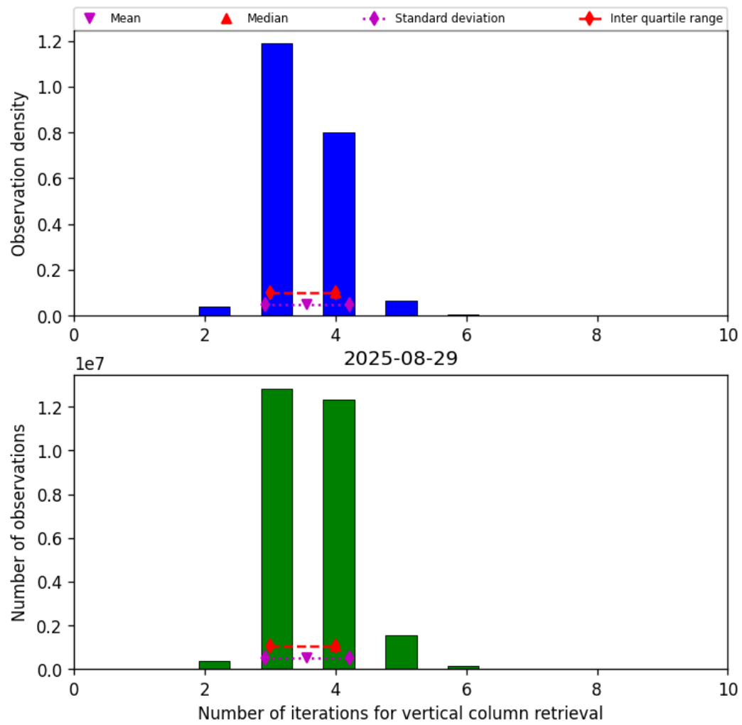
Figure 26: Histogram of “Number of iterations for vertical column retrieval” for 2025-08-28 to 2025-08-30
