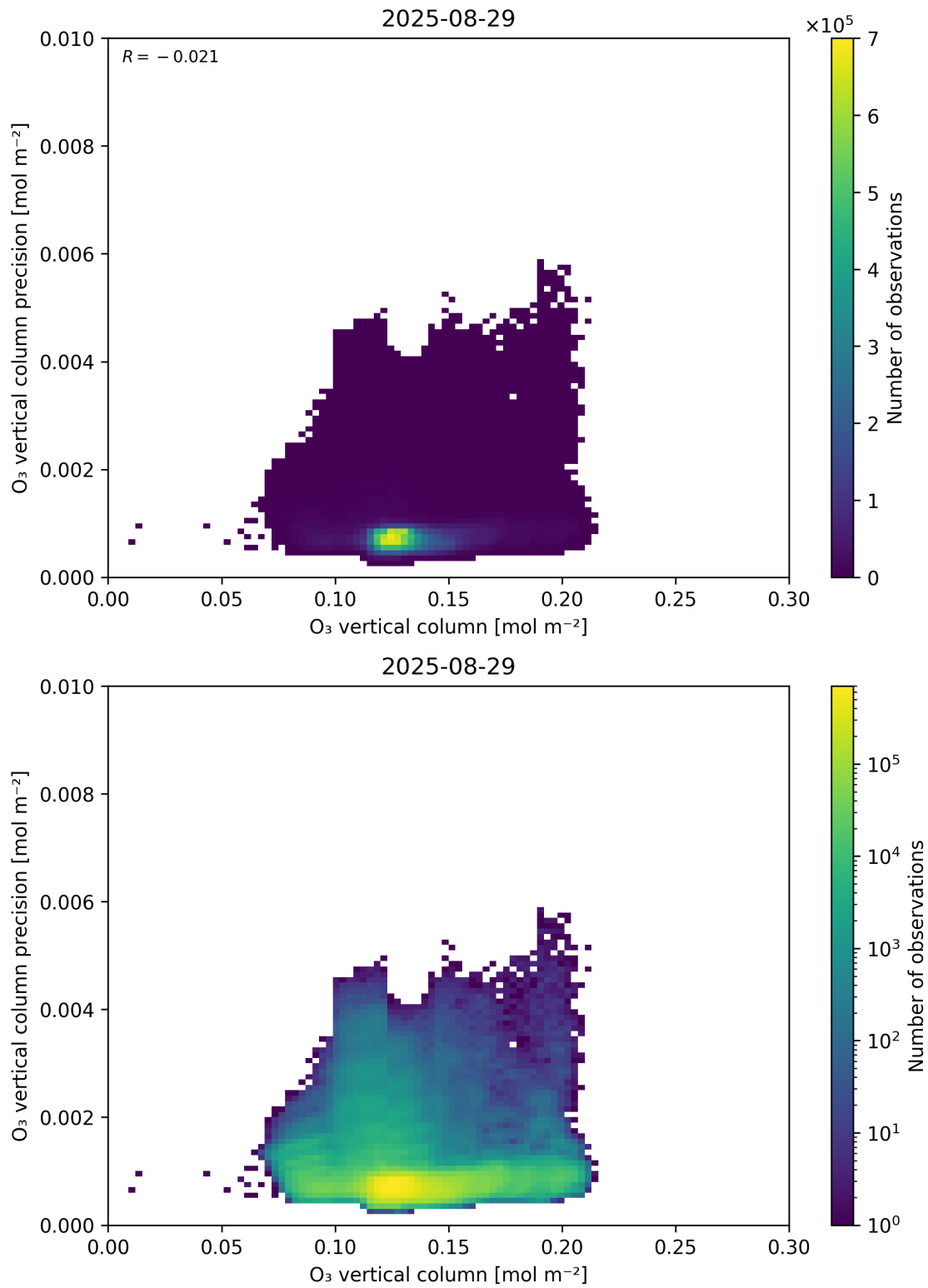
Figure 41: Scatter density plot of “O 3 vertical column” against “O 3 vertical column precision” for 2025-08-28 to 2025-08-30.
