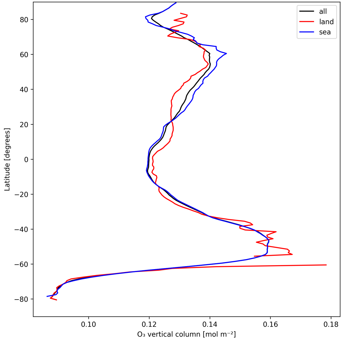
Figure 14: Zonal average of “O 3 vertical column” for 2025-08-28 to 2025-08-30.
