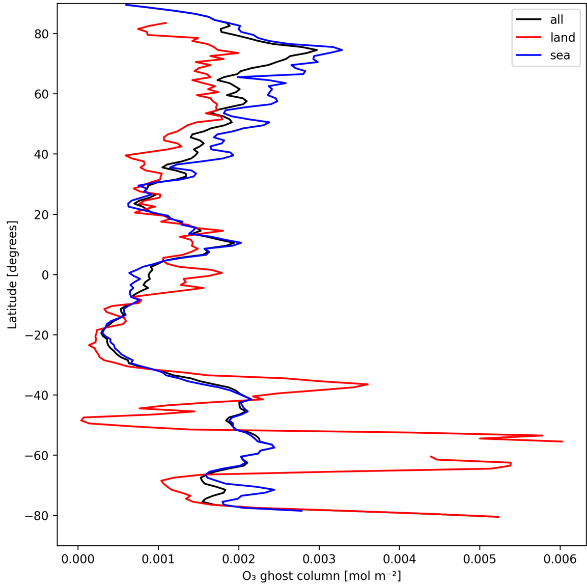
Figure 18: Zonal average of "O 3 ghost column" for 2025-08-30 to 2025-08-31.
