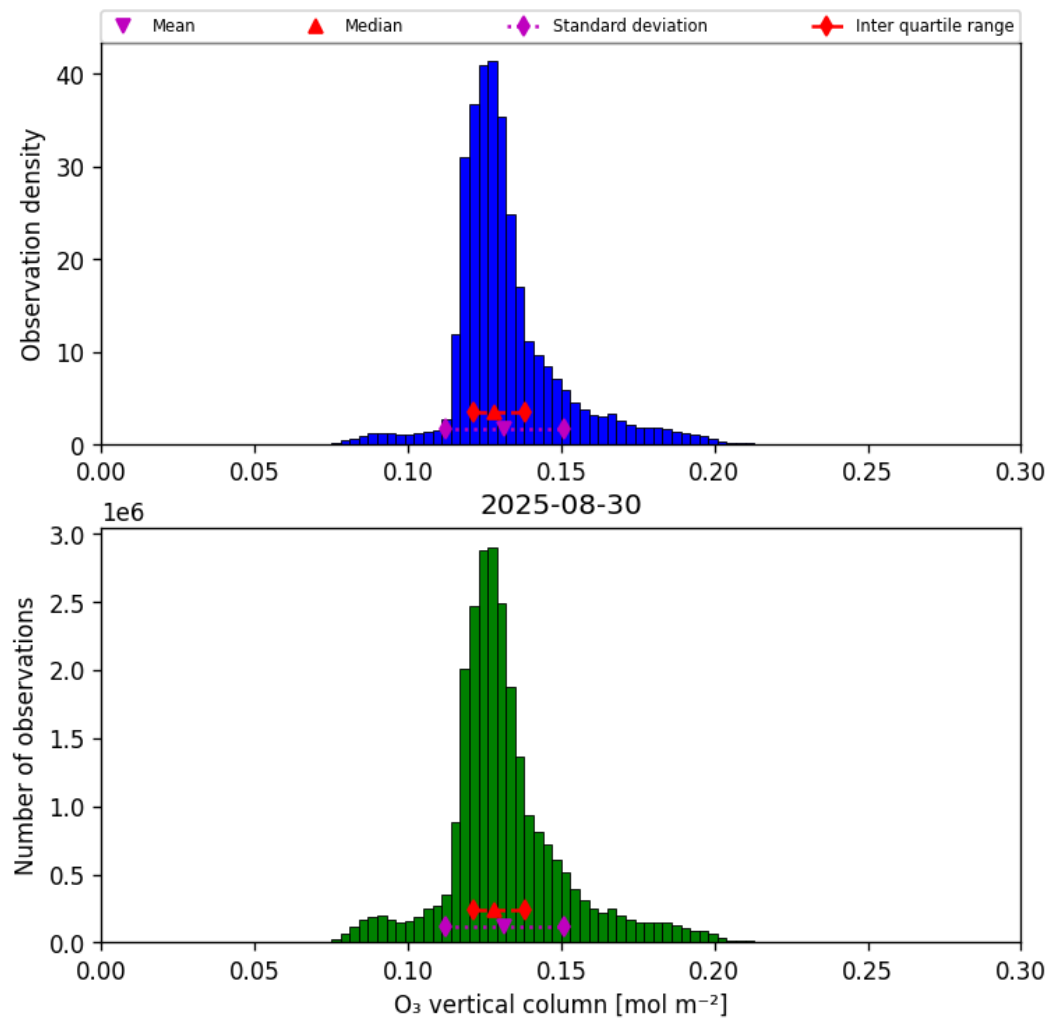
Figure 21: Histogram of “O 3 vertical column” for 2025-08-30 to 2025-08-31
