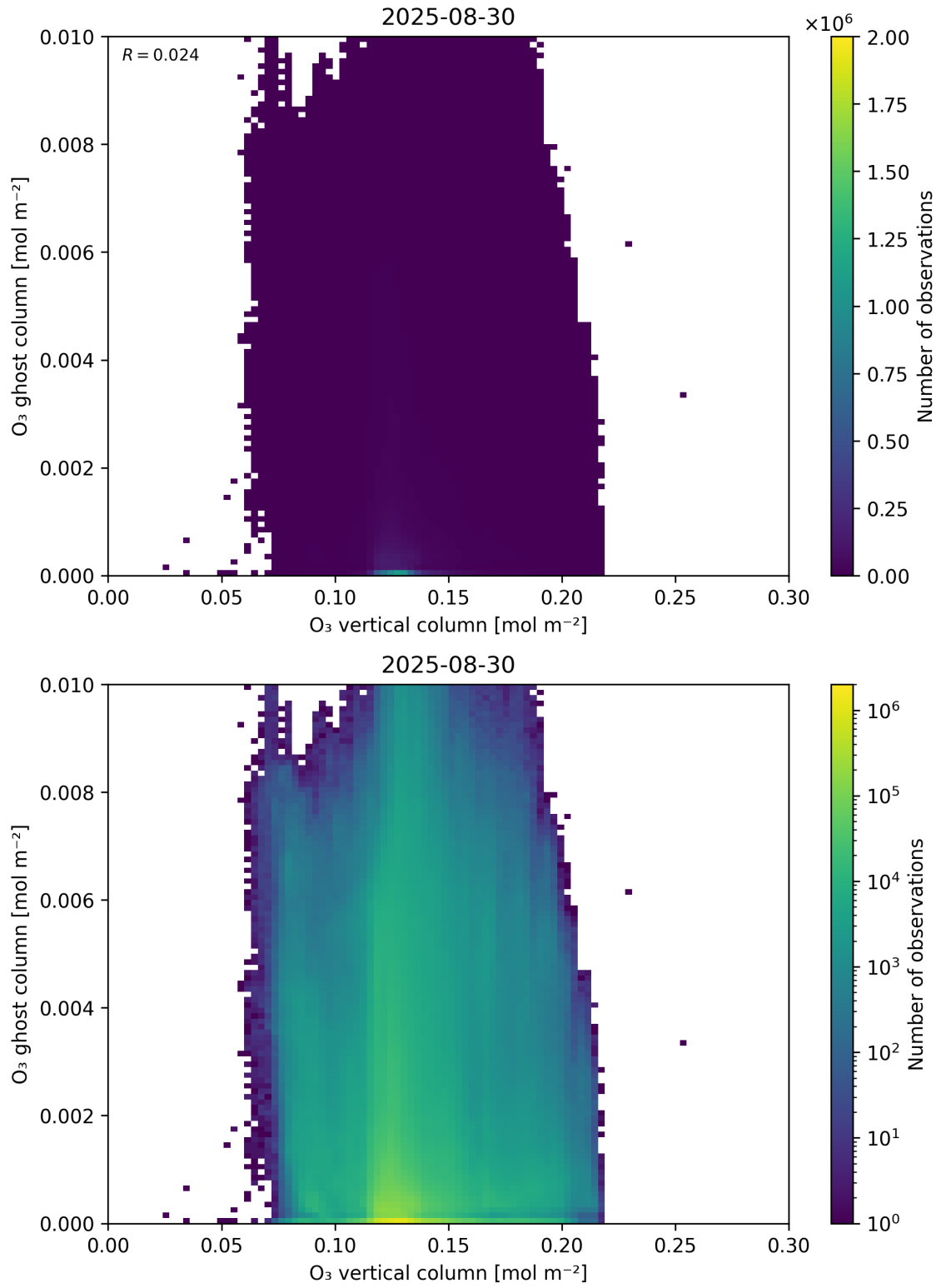
Figure 40: Scatter density plot of “O 3 vertical column” against “O 3 ghost column” for 2025-08-30 to 2025-08-31.
