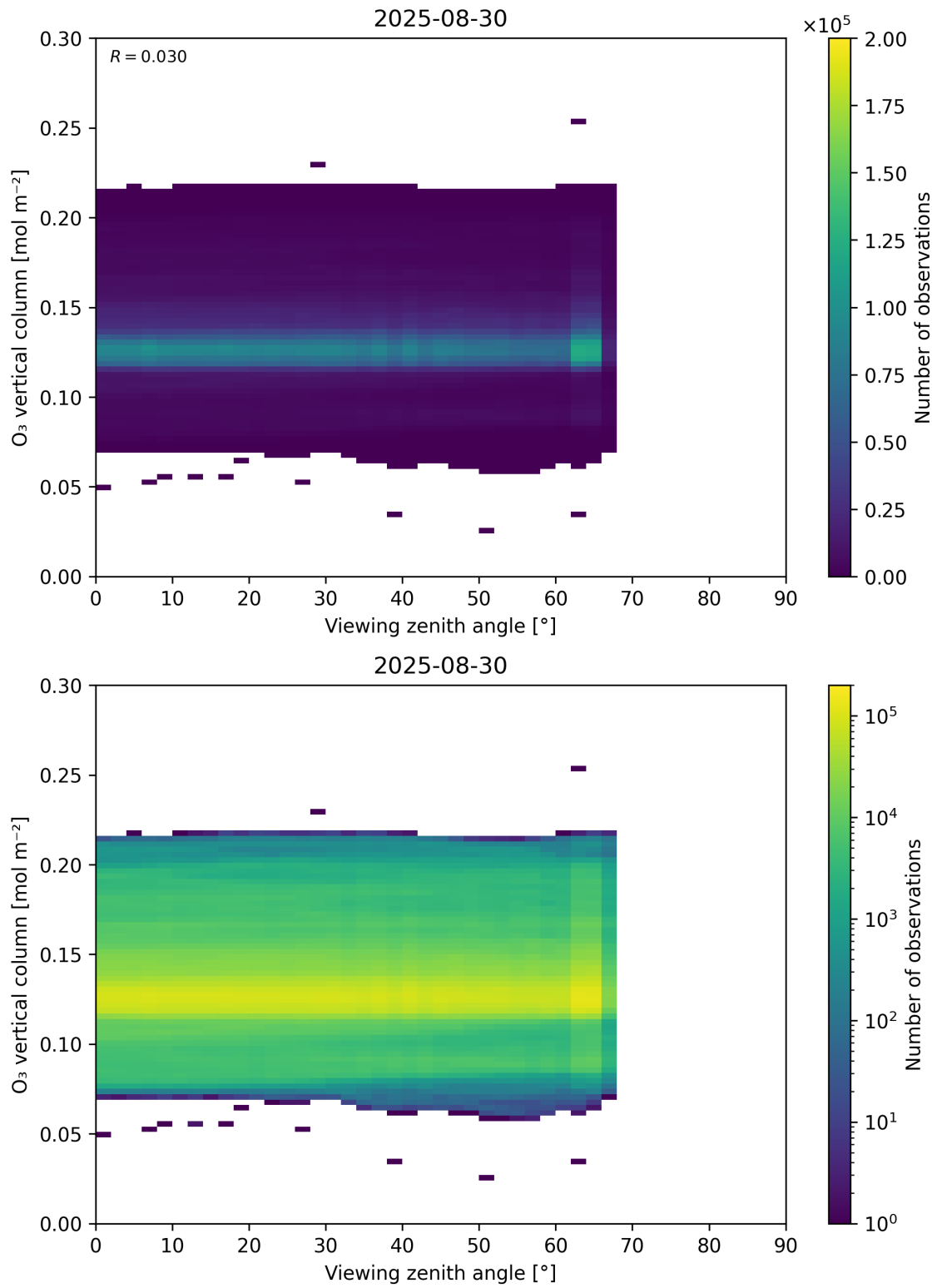
Figure 52: Scatter density plot of “Viewing zenith angle” against “O 3 vertical column” for 2025-08-30 to 2025-08-31.
