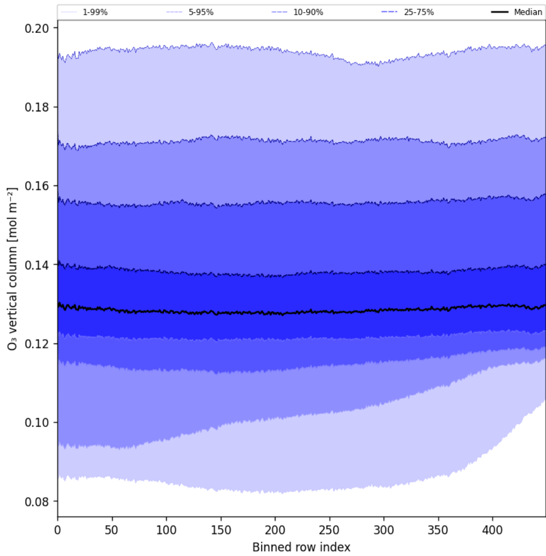
Figure 28: Along track statistics of “O 3 vertical column” for 2025-08-30 to 2025-08-31
