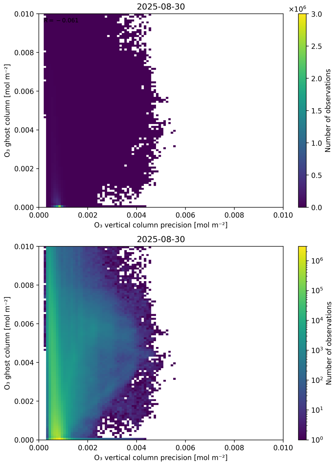
Figure 43: Scatter density plot of “ \text{O}_3 vertical column precision” against “ \text{O}_3 ghost column” for 2025-08-30 to 2025-08-31.
