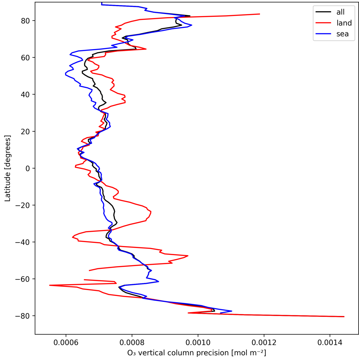
Figure 15: Zonal average of “O 3 vertical column precision” for 2025-08-30 to 2025-08-31.
