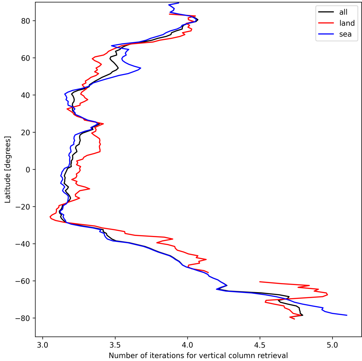
Figure 19: Zonal average of “Number of iterations for vertical column retrieval” for 2025-08-30 to 2025-08-31.
