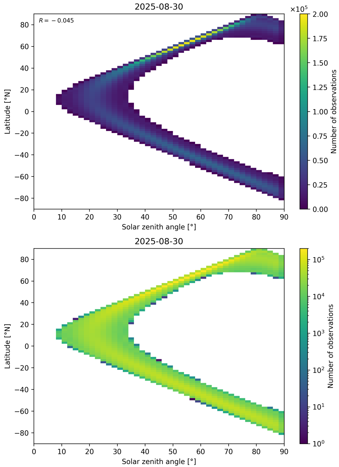
Figure 44: Scatter density plot of “Solar zenith angle” against “Latitude” for 2025-08-30 to 2025-08-31.
