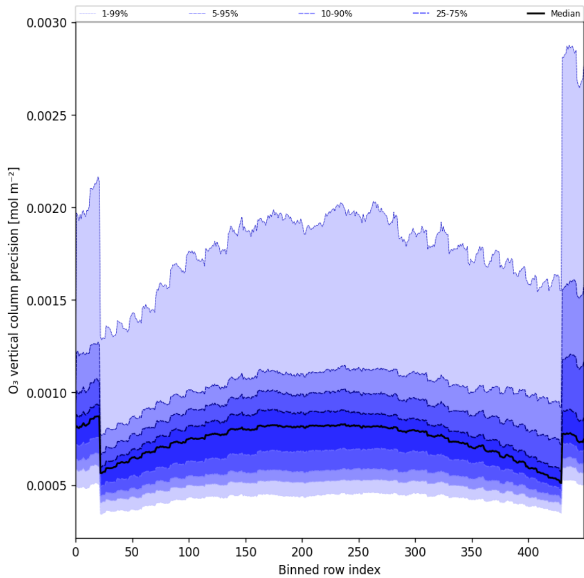
Figure 29: Along track statistics of “O 3 vertical column precision” for 2025-08-30 to 2025-08-31
