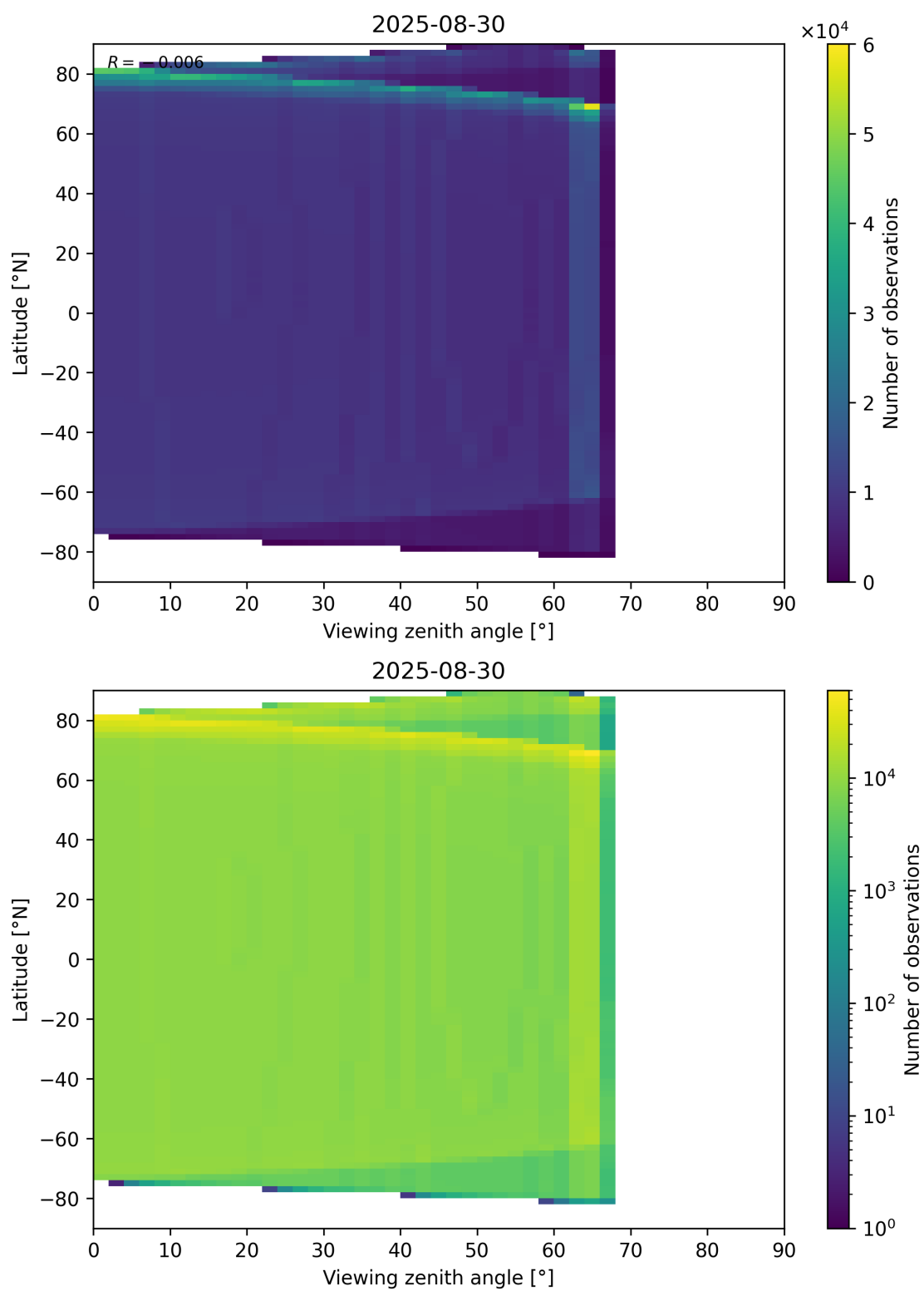
Figure 49: Scatter density plot of “Viewing zenith angle” against “Latitude” for 2025-08-30 to 2025-08-31.
