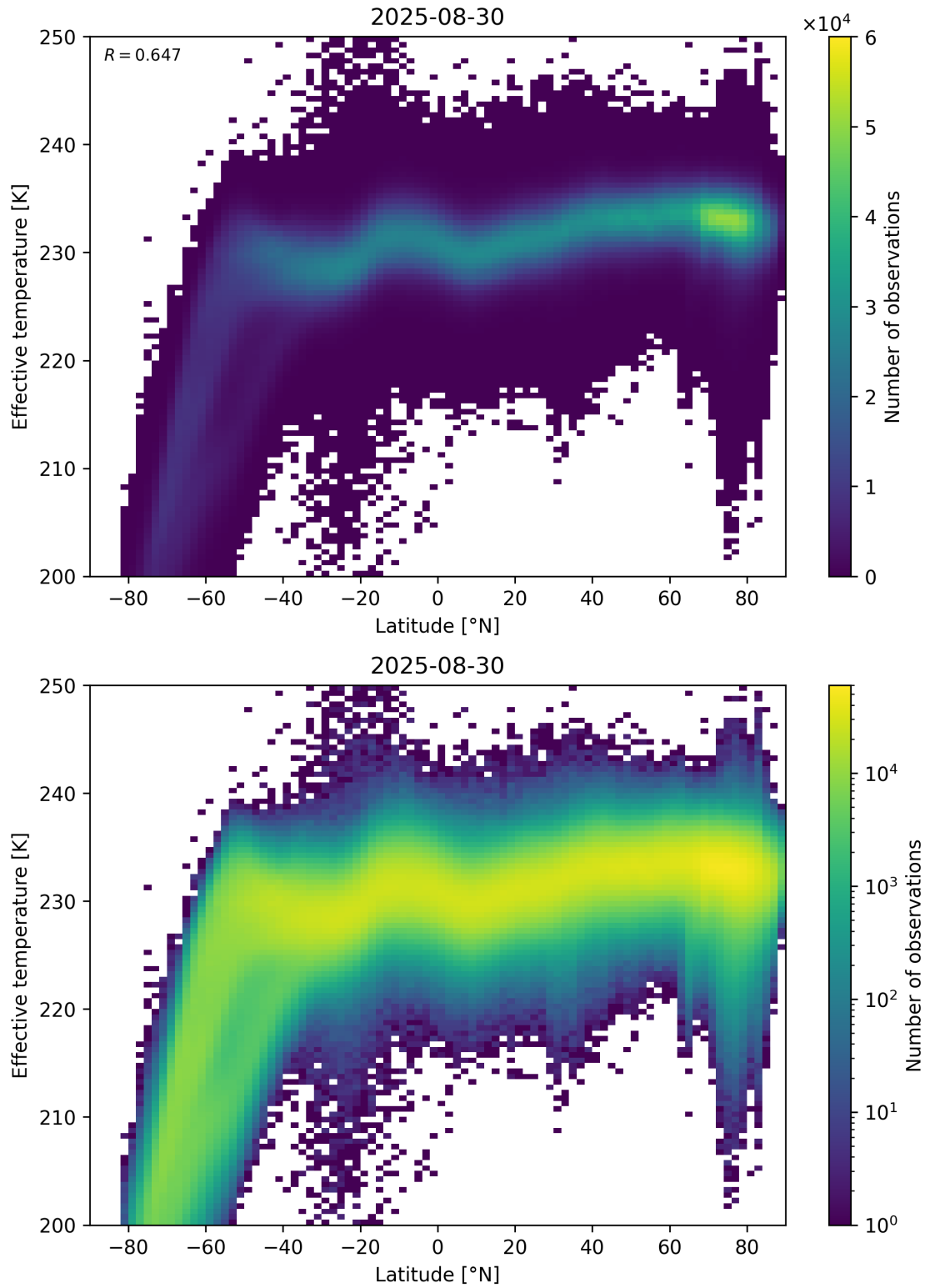
Figure 34: Scatter density plot of “Latitude” against “Effective temperature” for 2025-08-30 to 2025-08-31.
