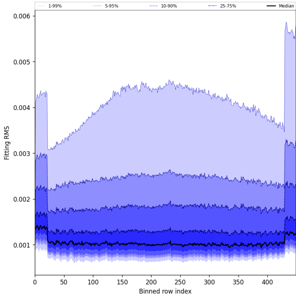
Figure 30: Along track statistics of “Fitting RMS” for 2025-08-30 to 2025-08-31
