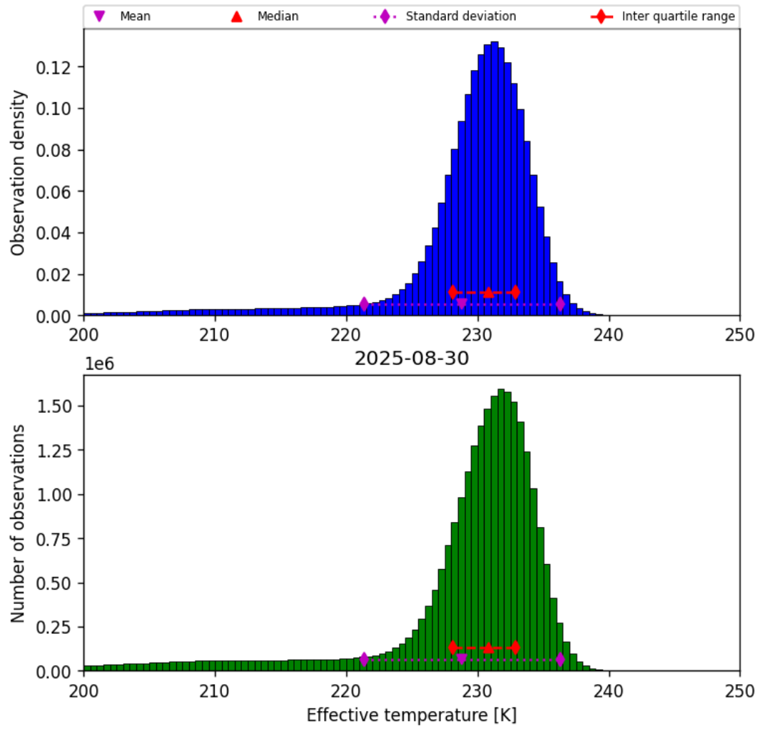
Figure 24: Histogram of “Effective temperature” for 2025-08-30 to 2025-08-31
