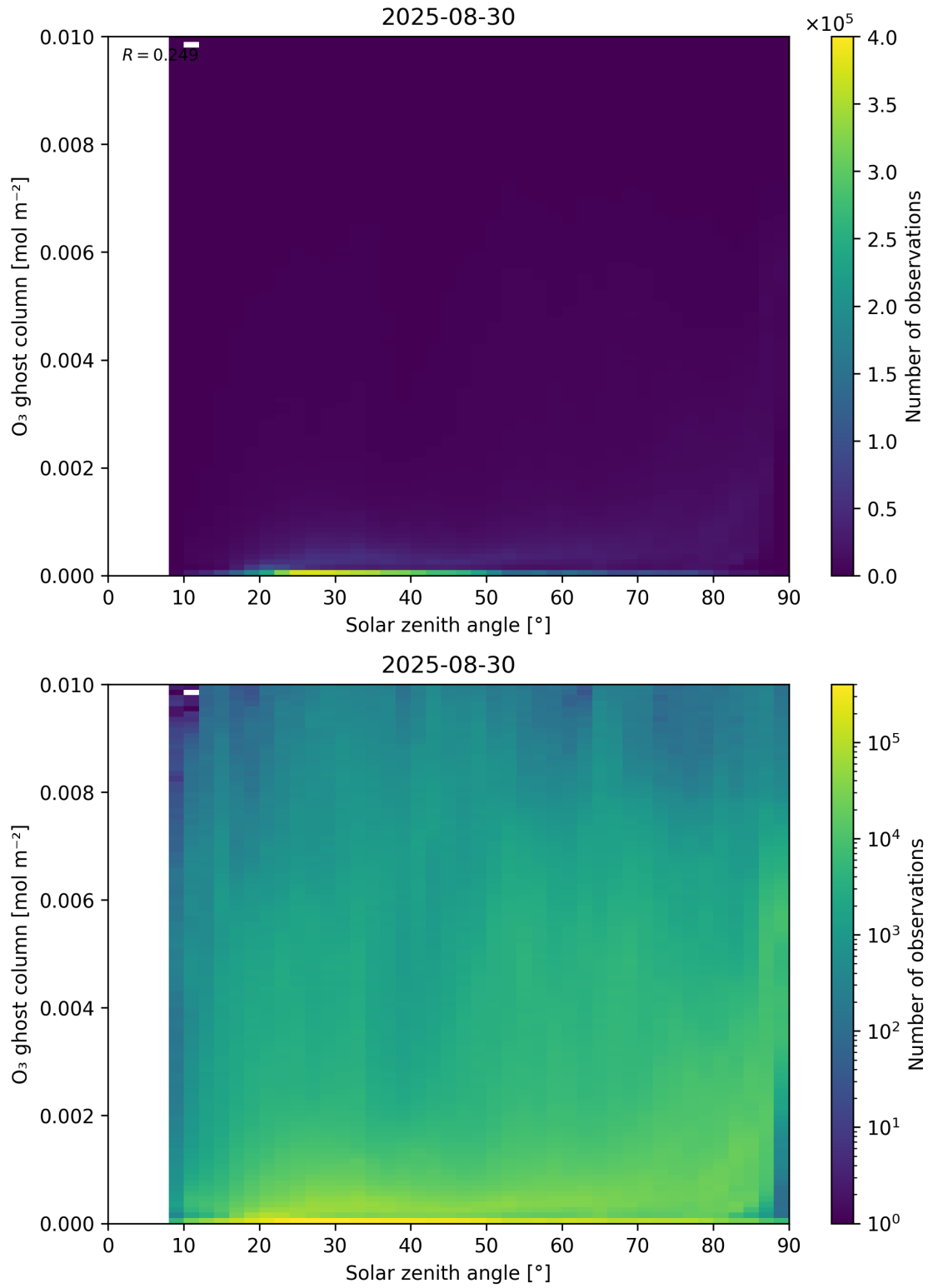
Figure 46: Scatter density plot of “Solar zenith angle” against “O 3 ghost column” for 2025-08-30 to 2025-08-31.
