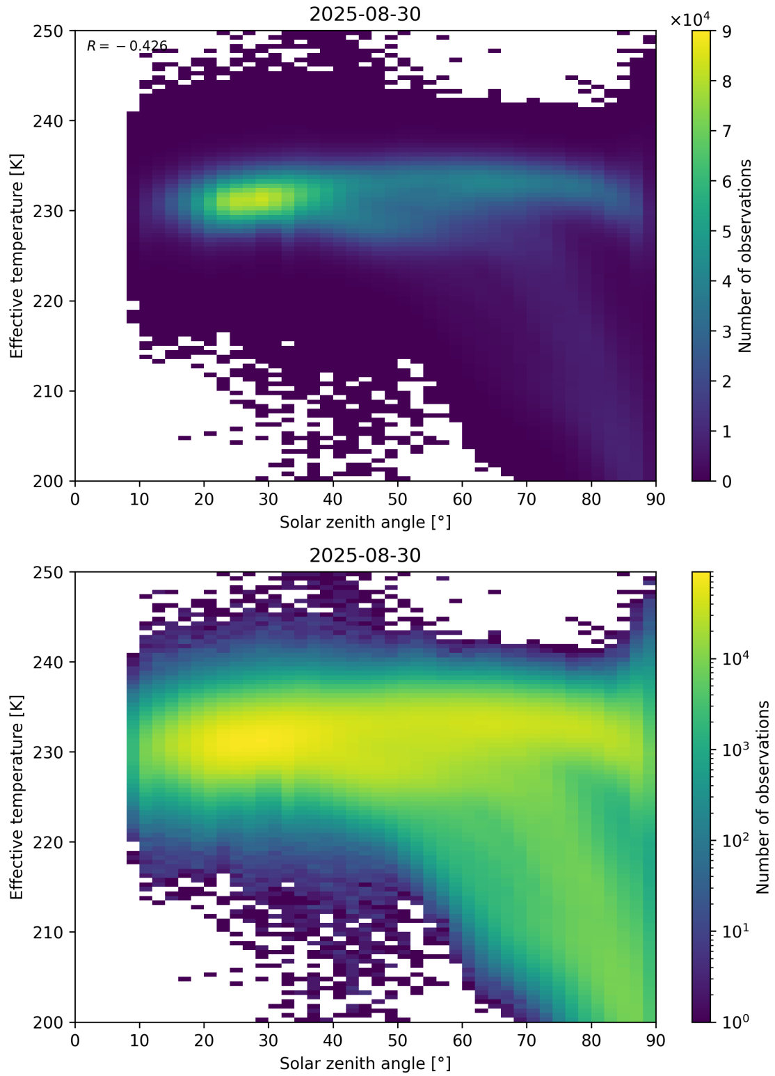
Figure 45: Scatter density plot of “Solar zenith angle” against “Effective temperature” for 2025-08-30 to 2025-08-31.
