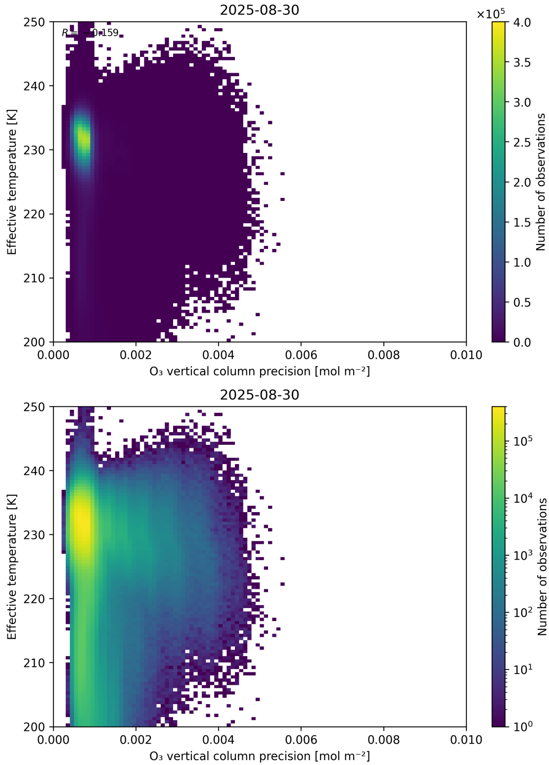
Figure 42: Scatter density plot of "O 3 vertical column precision" against "Effective temperature" for 2025-08-30 to 2025-08-31.
