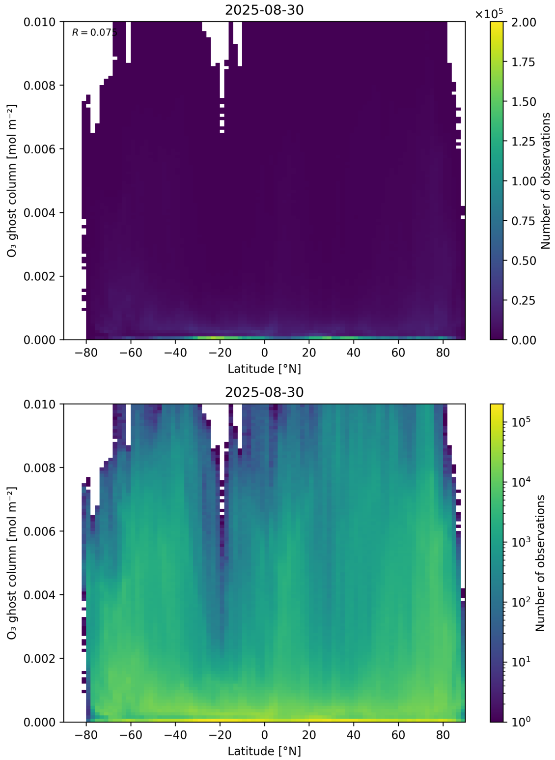
Figure 35: Scatter density plot of “Latitude” against “O 3 ghost column” for 2025-08-30 to 2025-08-31.
