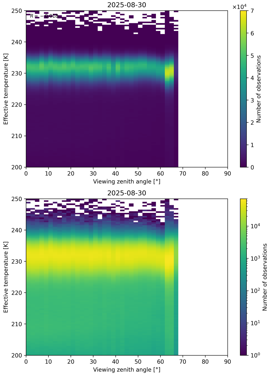
Figure 50: Scatter density plot of “Viewing zenith angle” against “Effective temperature” for 2025-08-30 to 2025-08-31.
