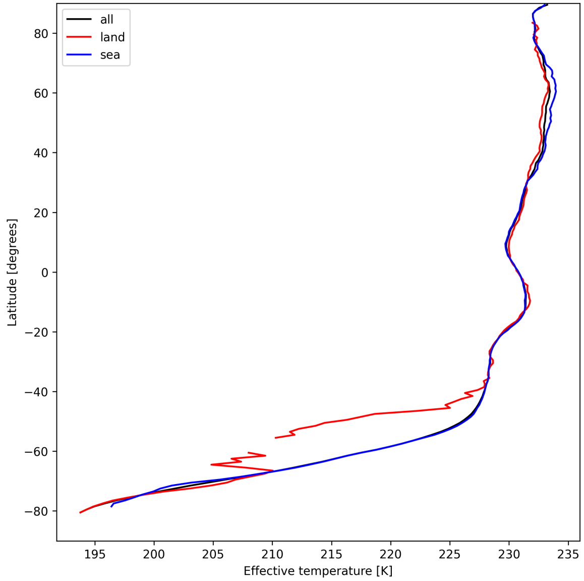
Figure 17: Zonal average of "Effective temperature" for 2025-08-30 to 2025-08-31.
