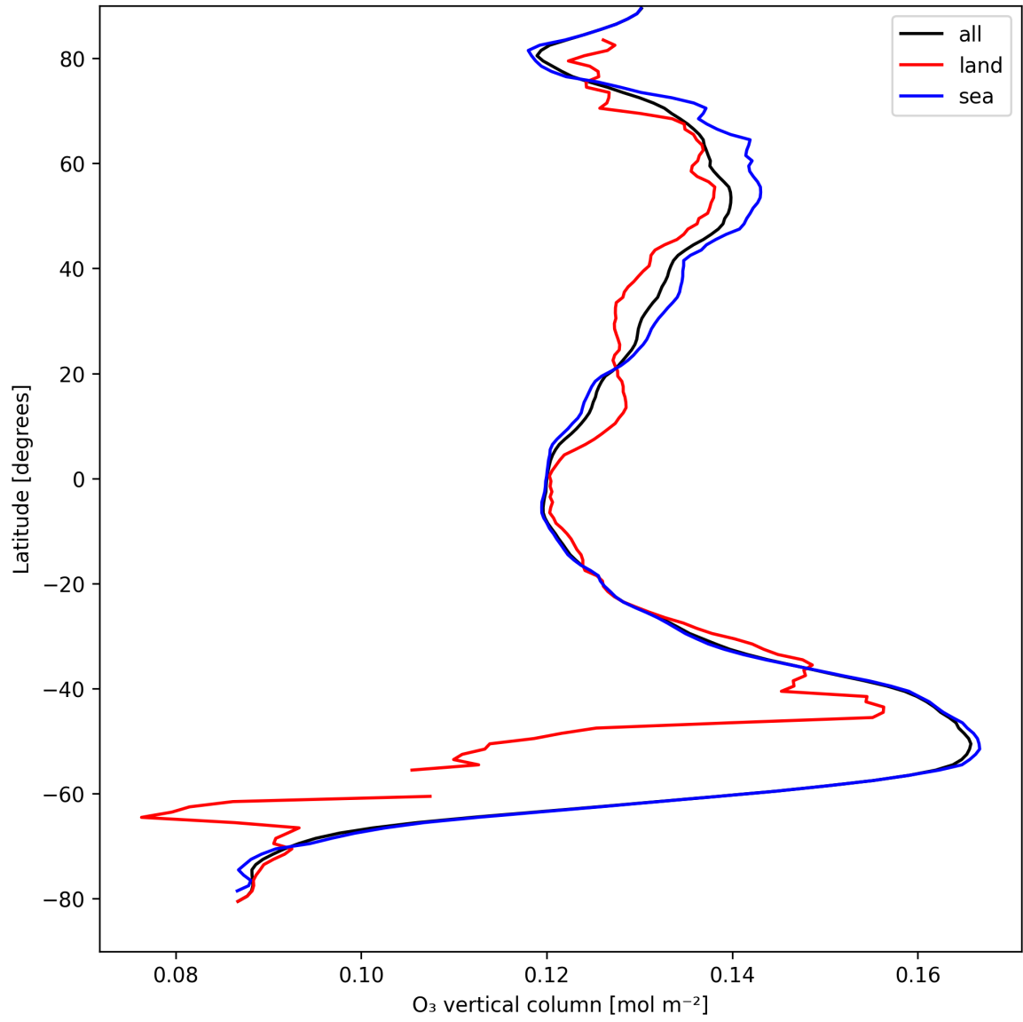
Figure 14: Zonal average of “O 3 vertical column” for 2025-08-30 to 2025-08-31.
