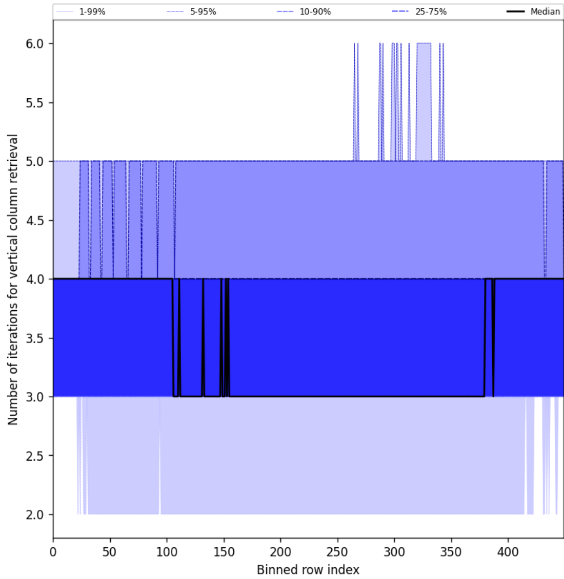
Figure 33: Along track statistics of “Number of iterations for vertical column retrieval” for 2025-08-30 to 2025-08-31
