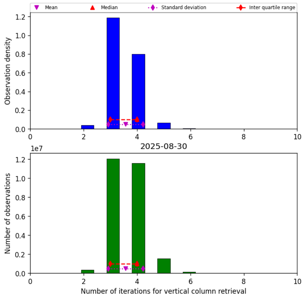
Figure 26: Histogram of “Number of iterations for vertical column retrieval” for 2025-08-30 to 2025-08-31
