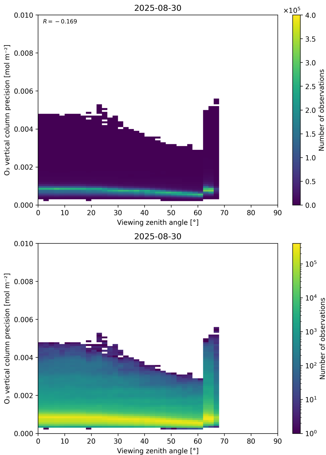
Figure 53: Scatter density plot of “Viewing zenith angle” against “O 3 vertical column precision” for 2025-08-30 to 2025-08-31.
