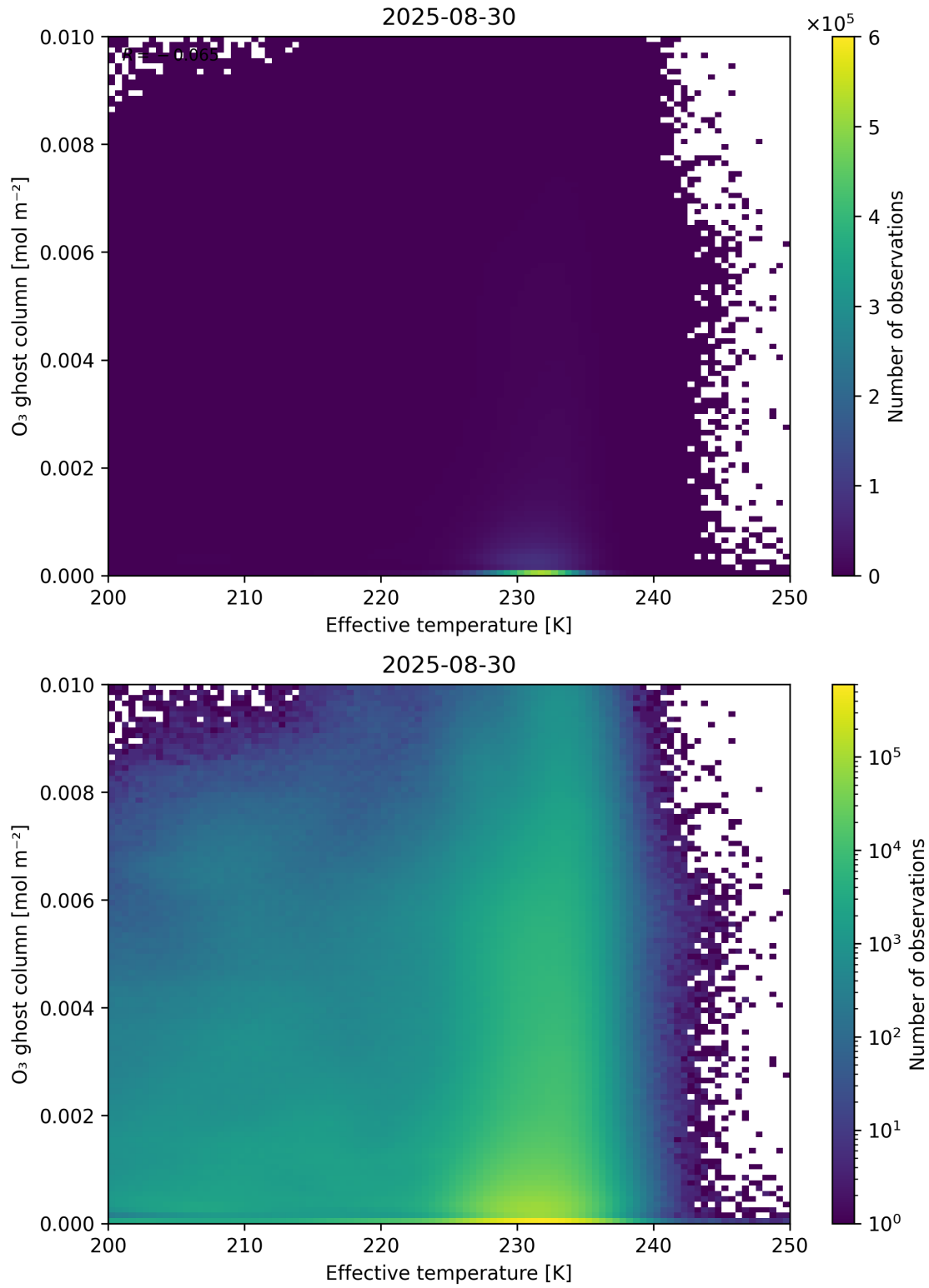
Figure 38: Scatter density plot of “Effective temperature” against “O 3 ghost column” for 2025-08-30 to 2025-08-31.
