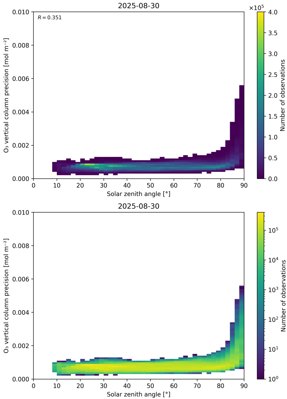
Figure 48: Scatter density plot of “Solar zenith angle” against “O 3 vertical column precision” for 2025-08-30 to 2025-08-31.
