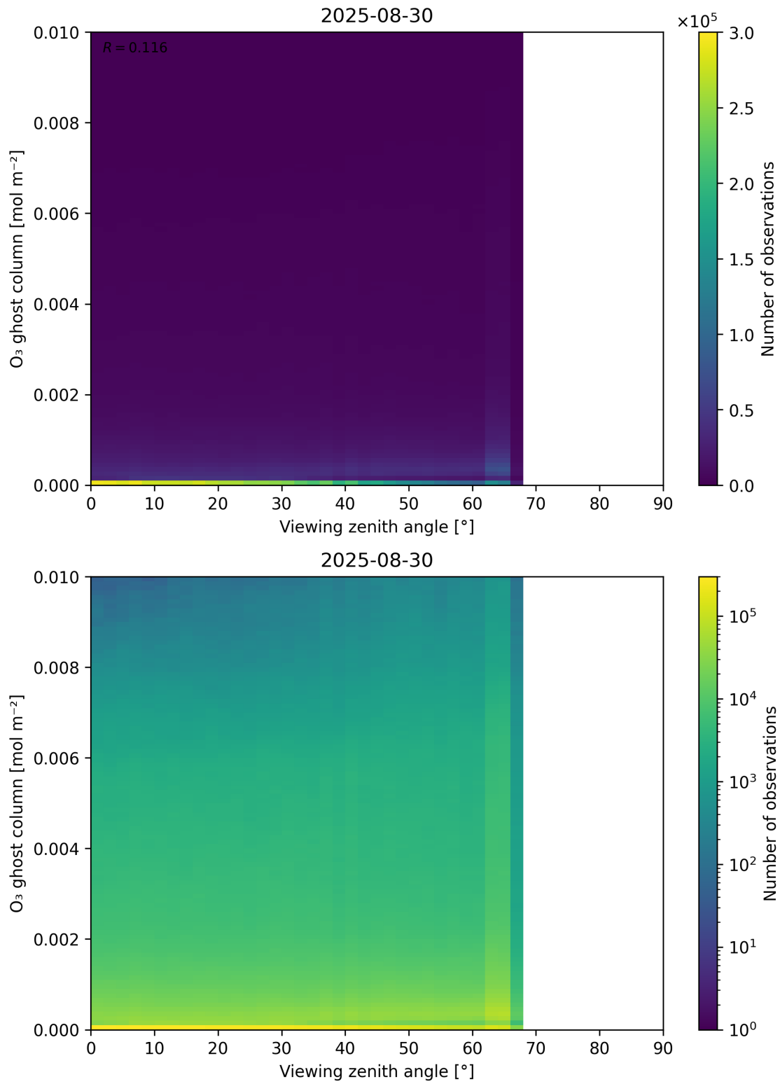
Figure 51: Scatter density plot of “Viewing zenith angle” against “O 3 ghost column” for 2025-08-30 to 2025-08-31.
