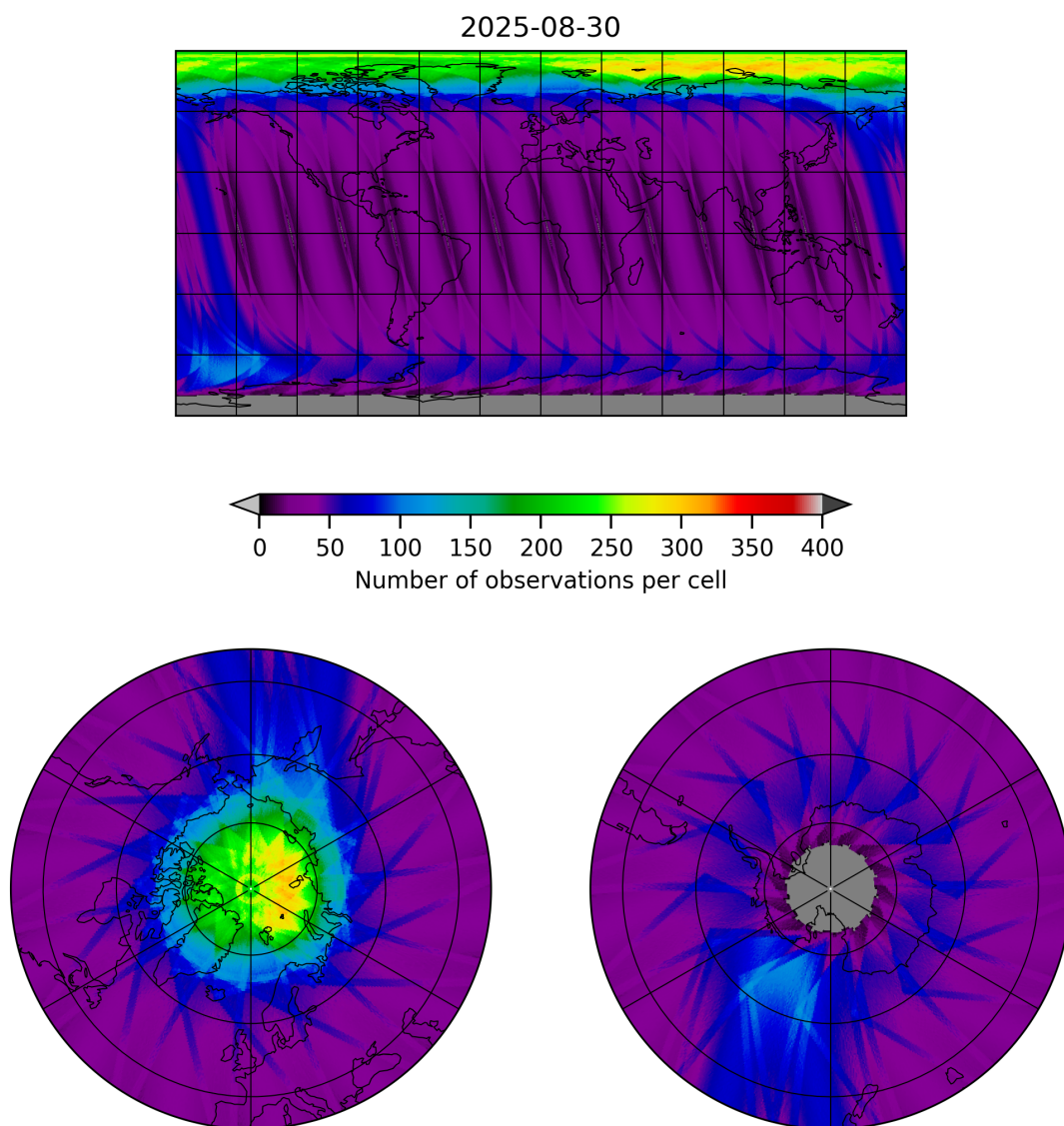
Figure 12: Map of the number of observations for 2025-08-30 to 2025-08-31
