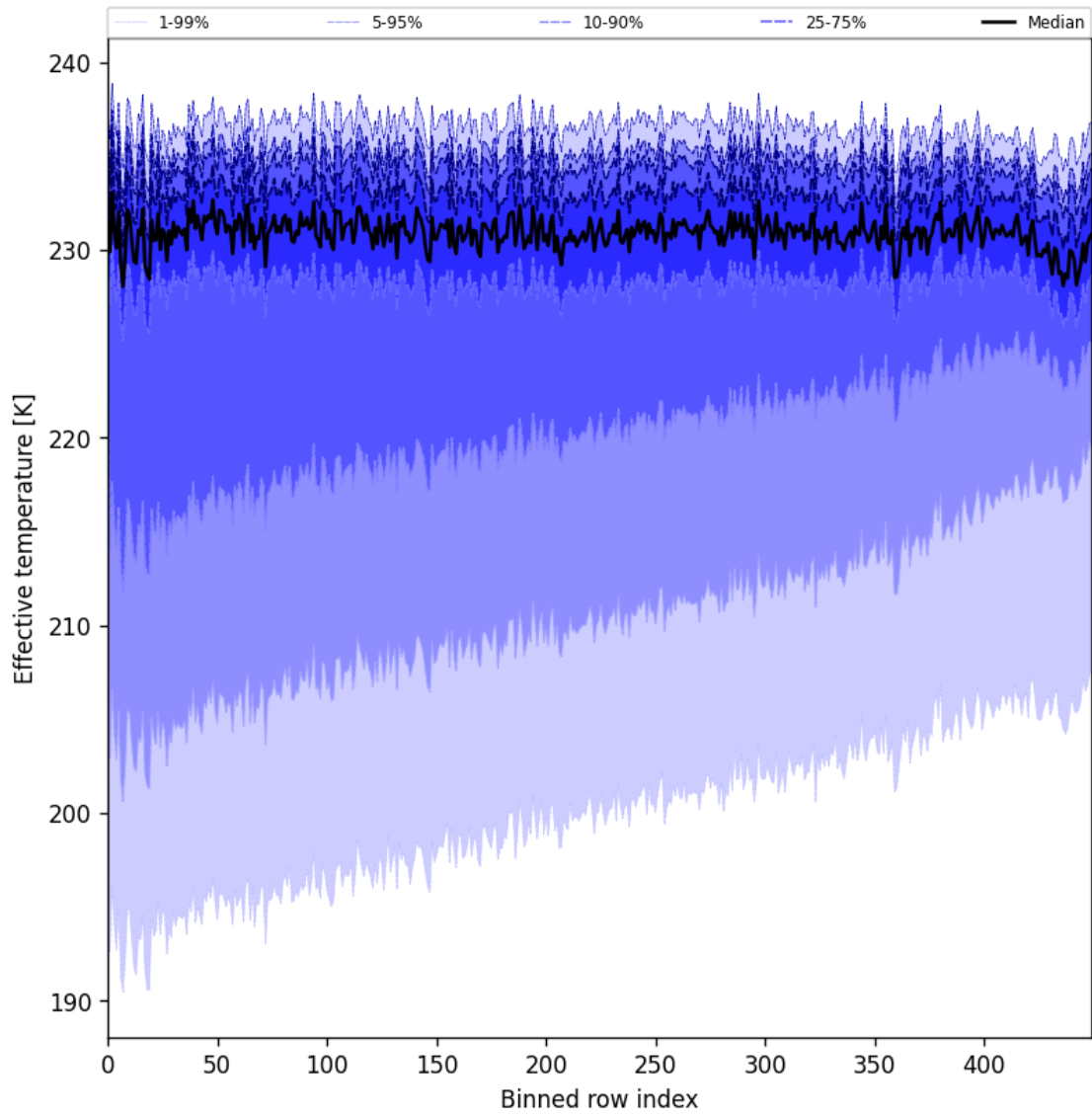
Figure 31: Along track statistics of “Effective temperature” for 2025-08-30 to 2025-08-31
