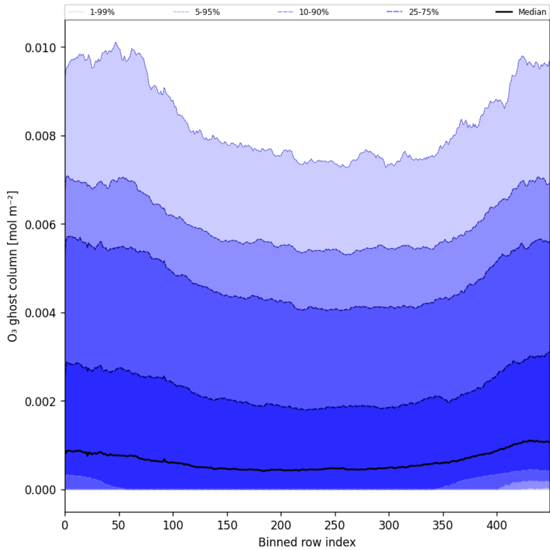
Figure 32: Along track statistics of “O 3 ghost column” for 2025-08-30 to 2025-08-31
