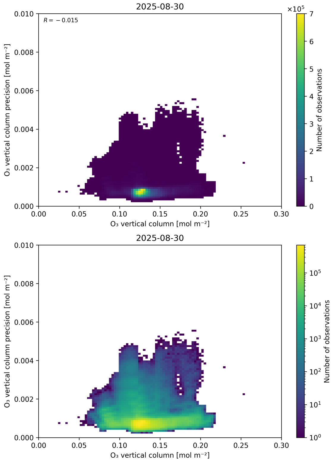
Figure 41: Scatter density plot of “O 3 vertical column” against “O 3 vertical column precision” for 2025-08-30 to 2025-08-31.
