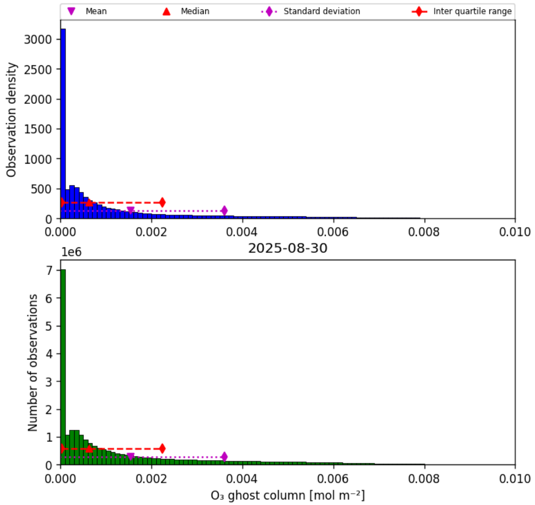
Figure 25: Histogram of "O 3 ghost column" for 2025-08-30 to 2025-08-31
