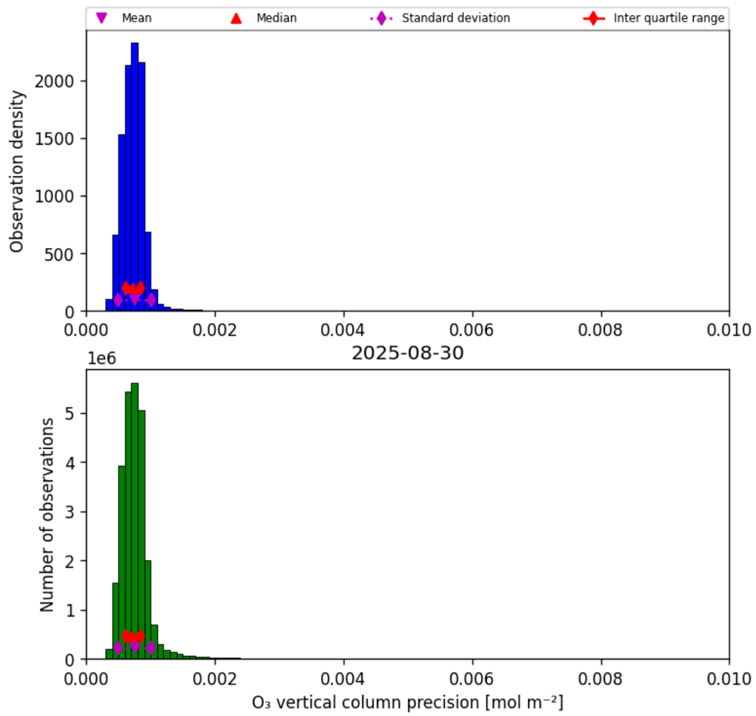
Figure 22: Histogram of “O 3 vertical column precision” for 2025-08-30 to 2025-08-31
