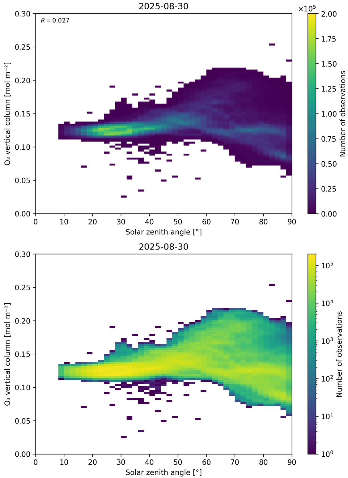
Figure 47: Scatter density plot of “Solar zenith angle” against “O 3 vertical column” for 2025-08-30 to 2025-08-31.
