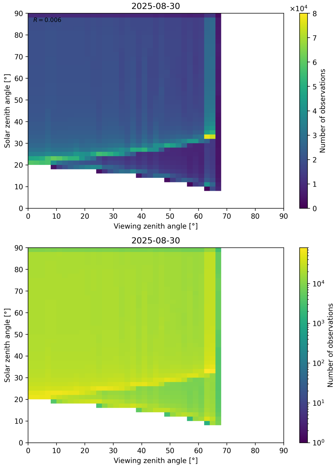
Figure 54: Scatter density plot of “Viewing zenith angle” against “Solar zenith angle” for 2025-08-30 to 2025-08-31.
