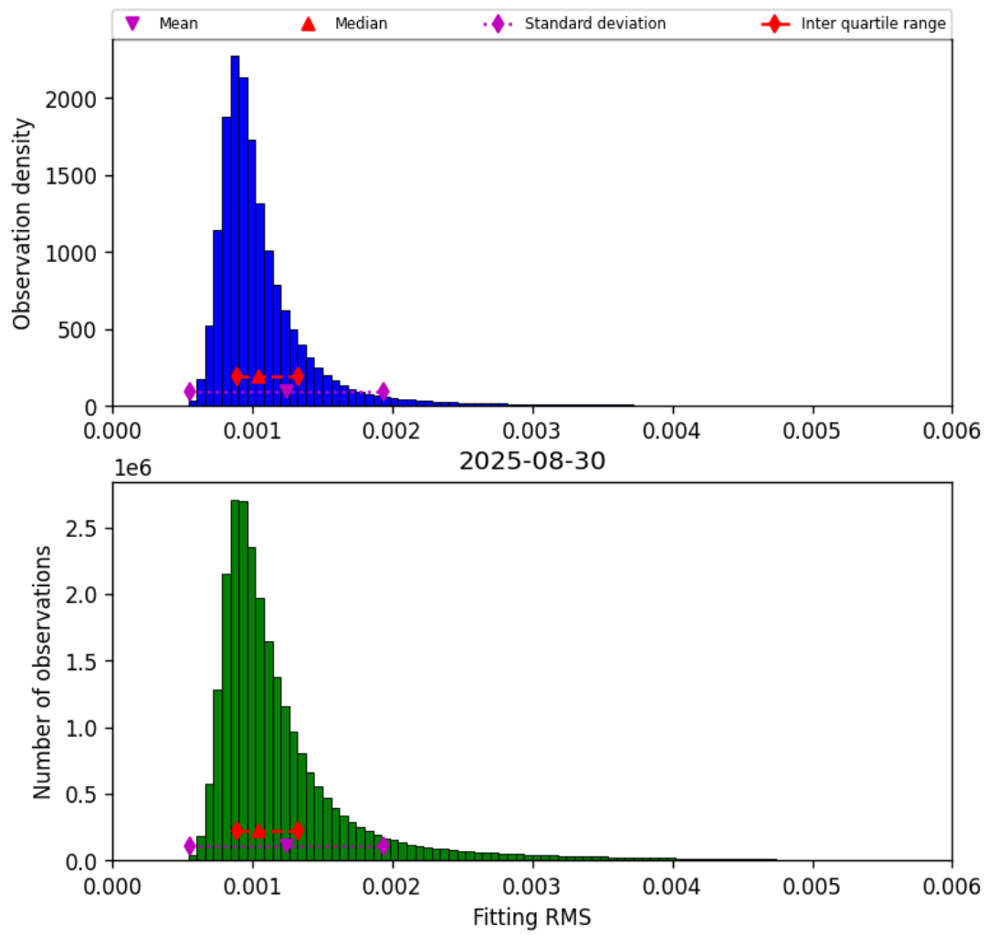
Figure 23: Histogram of “Fitting RMS” for 2025-08-30 to 2025-08-31
