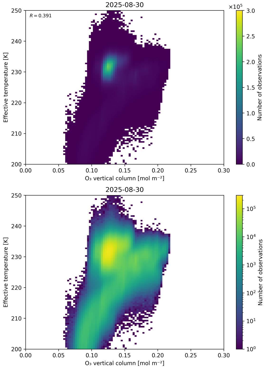
Figure 39: Scatter density plot of “O 3 vertical column” against “Effective temperature” for 2025-08-30 to 2025-08-31.
