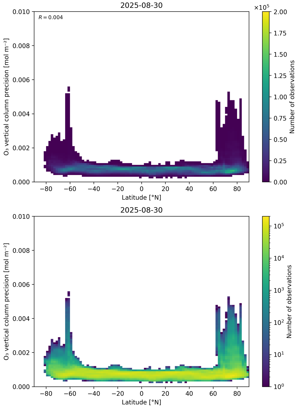
Figure 37: Scatter density plot of “Latitude” against “O 3 vertical column precision” for 2025-08-30 to 2025-08-31.
