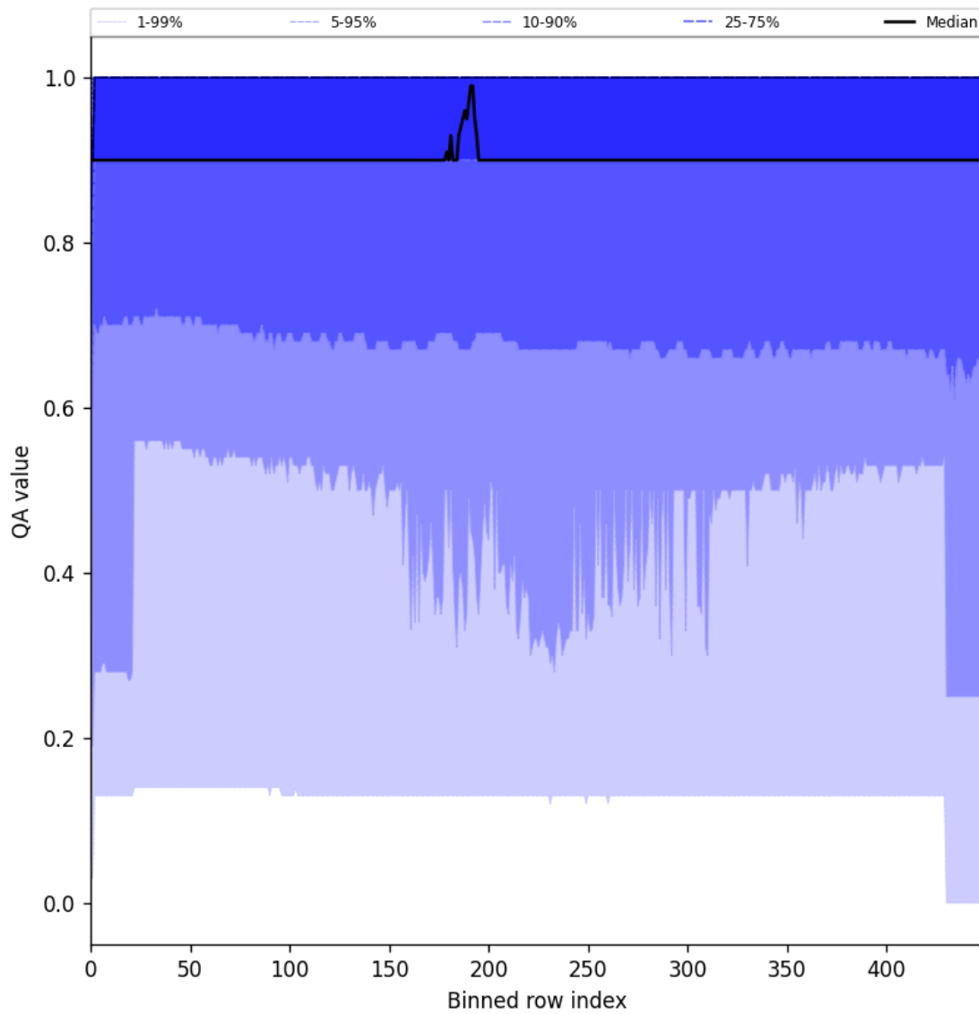
Figure 27: Along track statistics of “QA value” for 2025-08-30 to 2025-08-31
