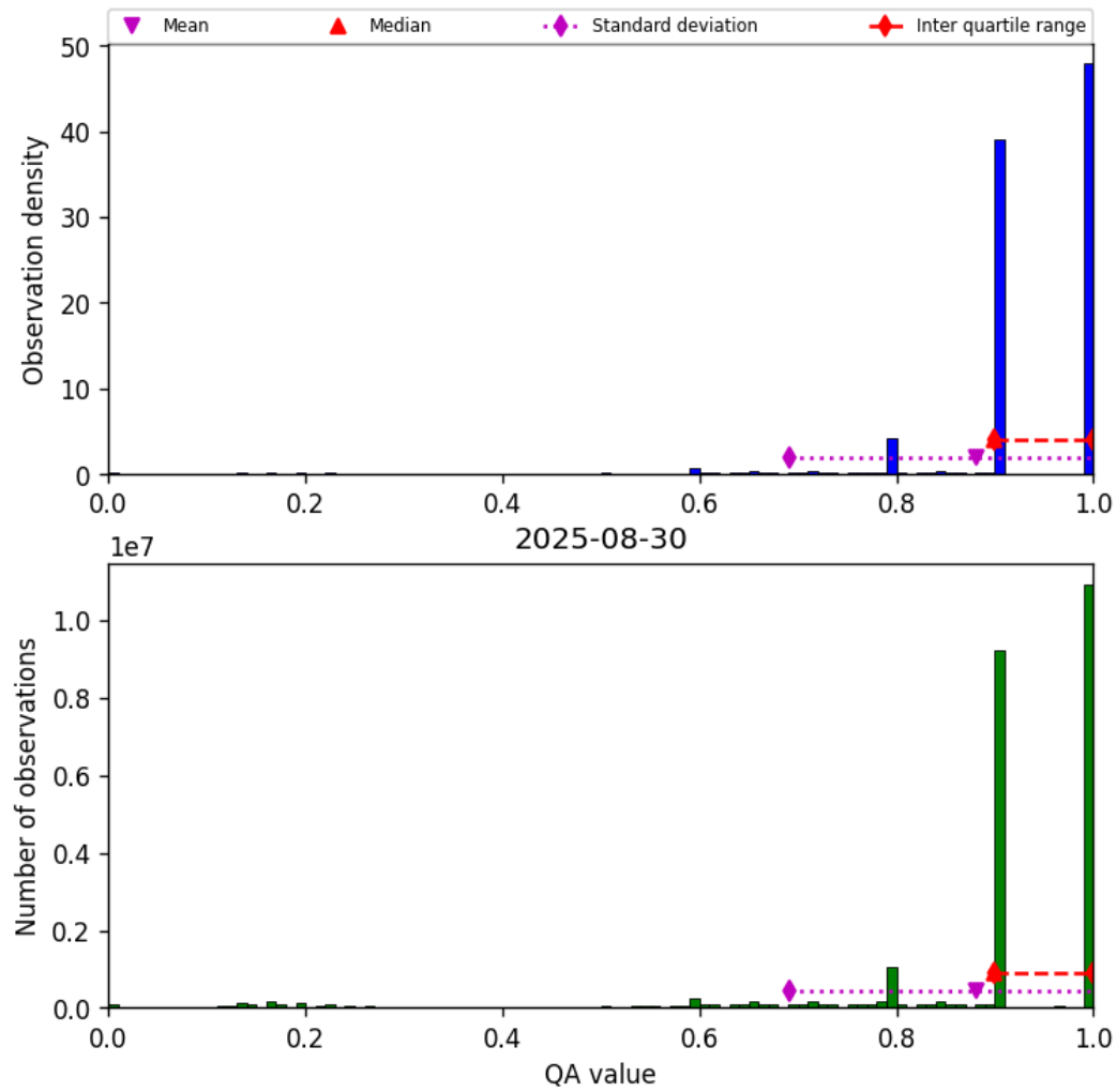
Figure 20: Histogram of “QA value” for 2025-08-30 to 2025-08-31
