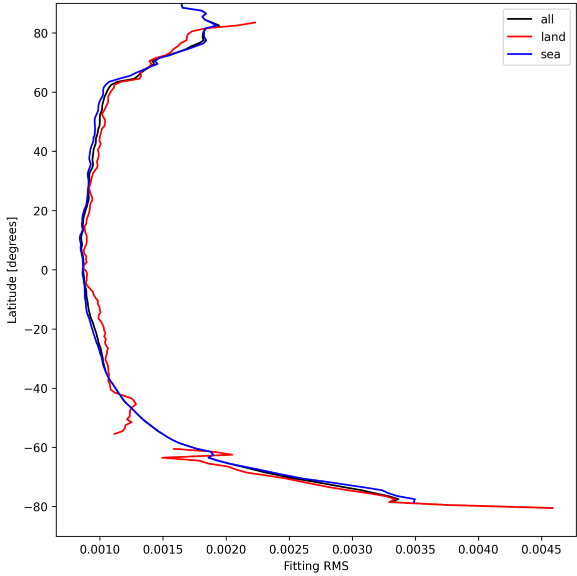
Figure 16: Zonal average of “Fitting RMS” for 2025-08-30 to 2025-08-31.
