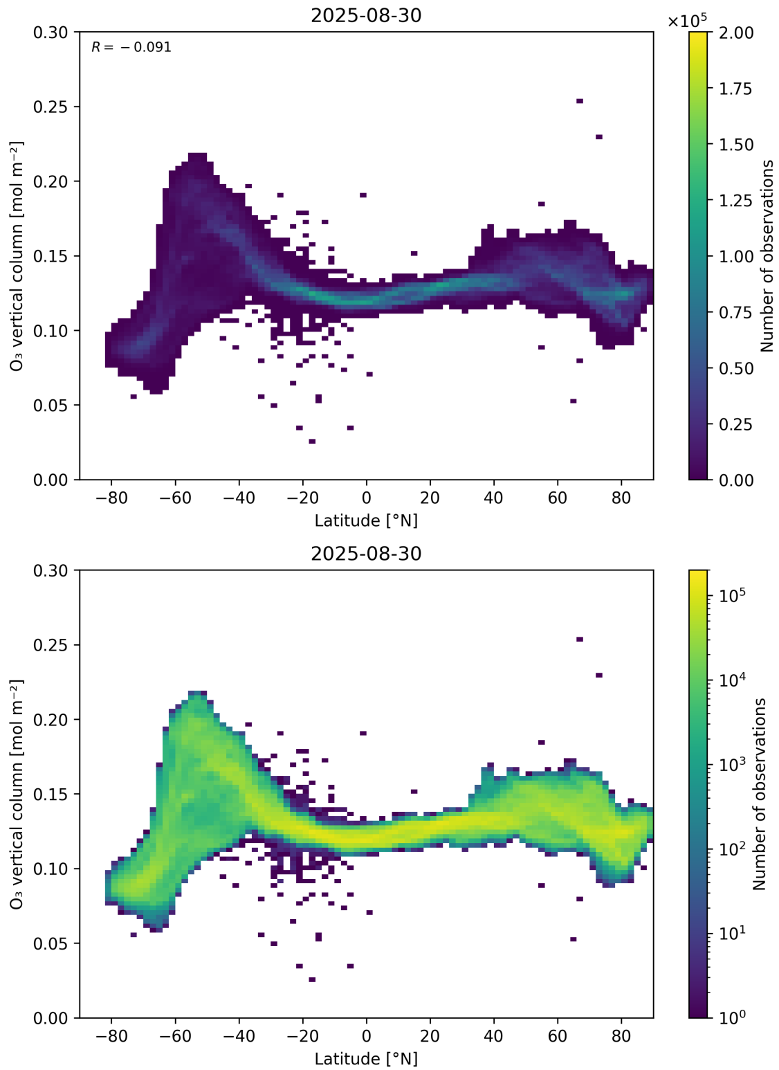
Figure 36: Scatter density plot of “Latitude” against “O 3 vertical column” for 2025-08-30 to 2025-08-31.
