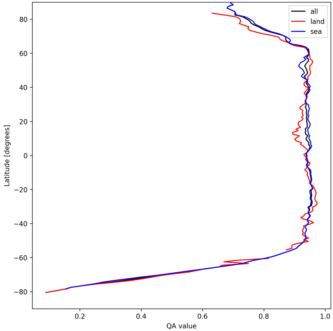
Figure 13: Zonal average of “QA value” for 2025-08-30 to 2025-08-31.
