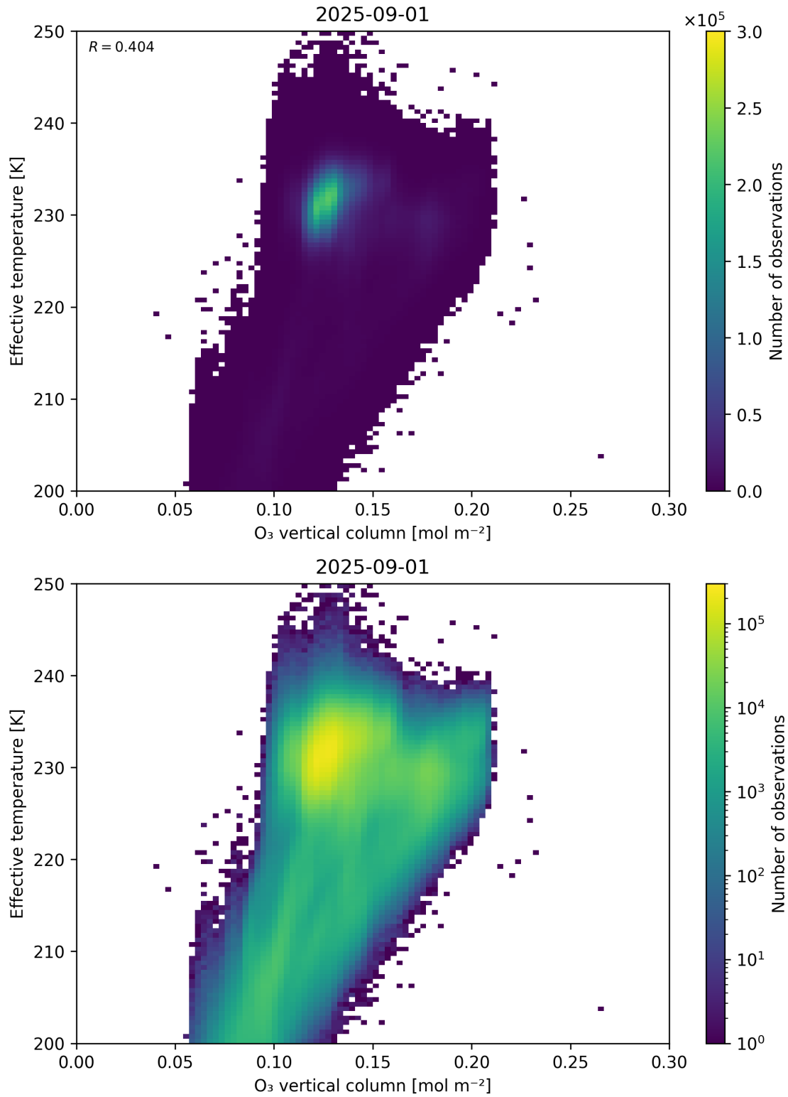
Figure 39: Scatter density plot of “O 3 vertical column” against “Effective temperature” for 2025-08-31 to 2025-09-02.
