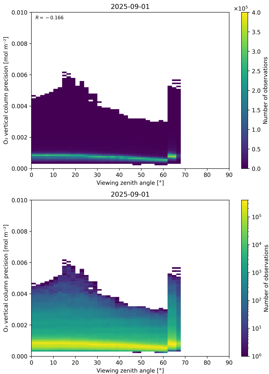
Figure 53: Scatter density plot of “Viewing zenith angle” against “O 3 vertical column precision” for 2025-08-31 to 2025-09-02.
