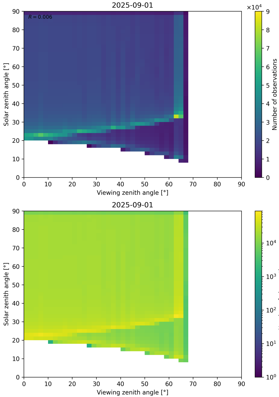
Figure 54: Scatter density plot of “Viewing zenith angle” against “Solar zenith angle” for 2025-08-31 to 2025-09-02.
