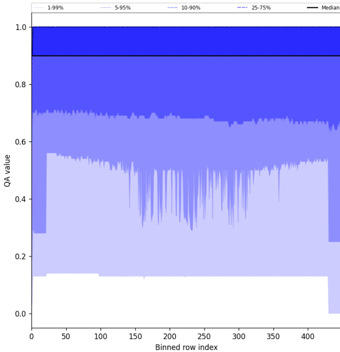
Figure 27: Along track statistics of “QA value” for 2025-08-31 to 2025-09-02
