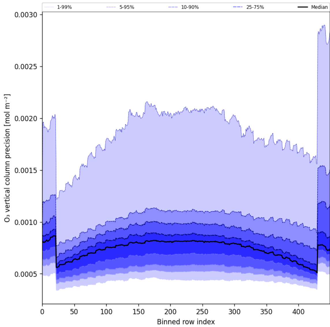
Figure 29: Along track statistics of “O 3 vertical column precision” for 2025-08-31 to 2025-09-02
