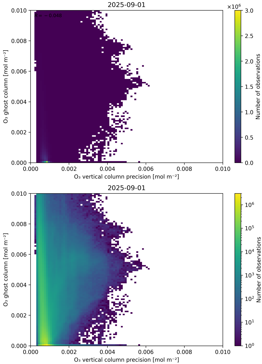
Figure 43: Scatter density plot of “O 3 vertical column precision” against “O 3 ghost column” for 2025-08-31 to 2025-09-02.
