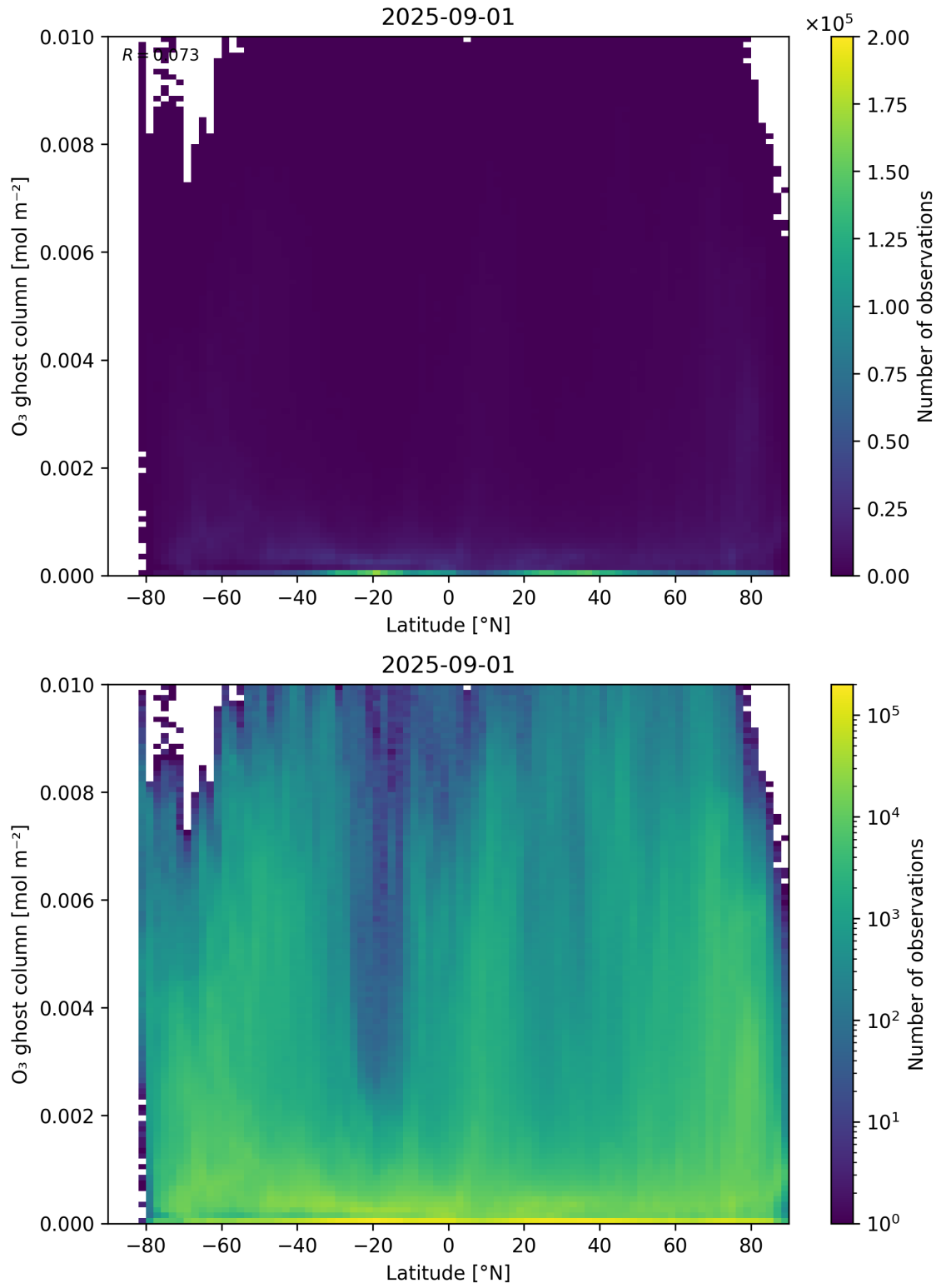
Figure 35: Scatter density plot of “Latitude” against “O 3 ghost column” for 2025-08-31 to 2025-09-02.
