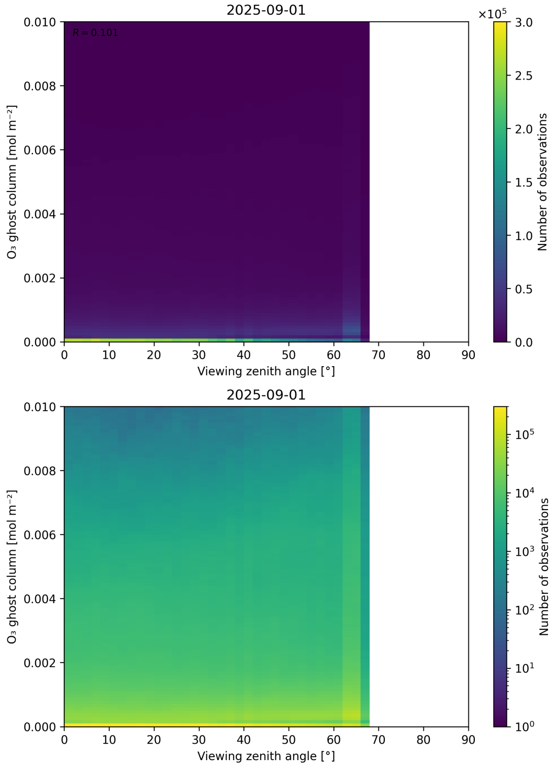
Figure 51: Scatter density plot of “Viewing zenith angle” against “O 3 ghost column” for 2025-08-31 to 2025-09-02.
