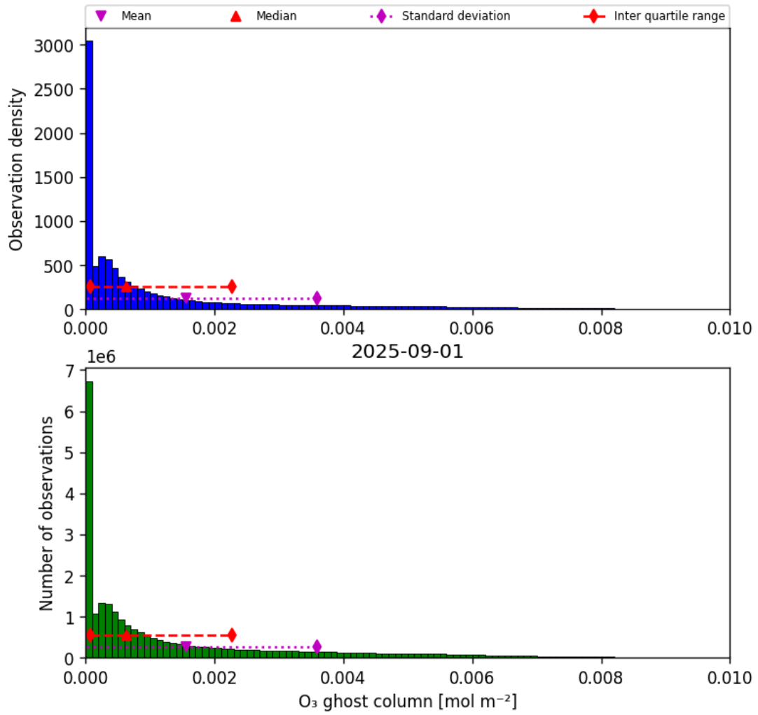
Figure 25: Histogram of "O 3 ghost column" for 2025-08-31 to 2025-09-02
