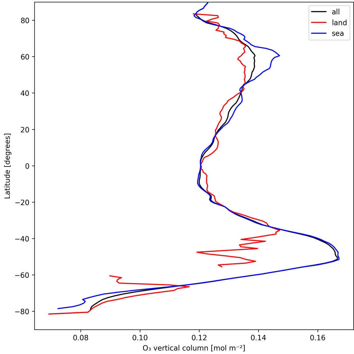
Figure 14: Zonal average of “O 3 vertical column” for 2025-08-31 to 2025-09-02.
