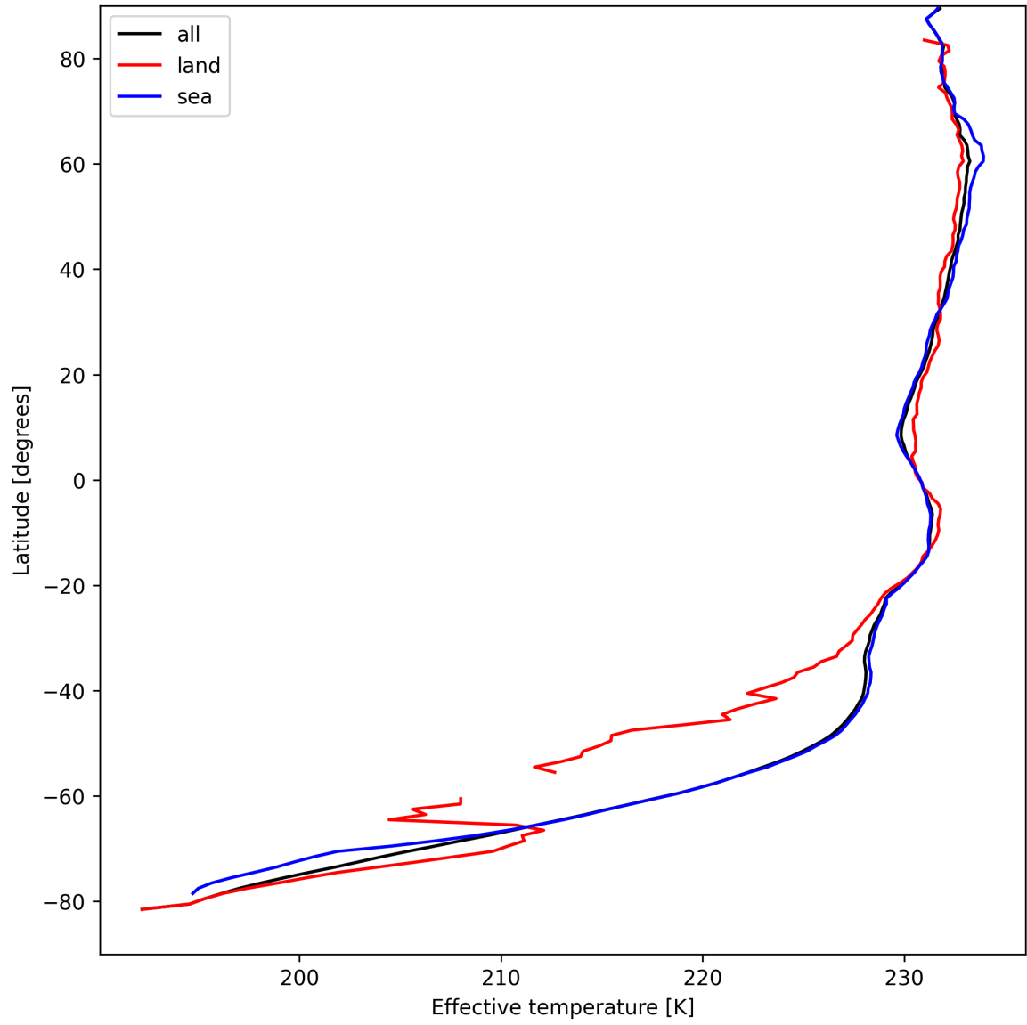
Figure 17: Zonal average of "Effective temperature" for 2025-08-31 to 2025-09-02.
