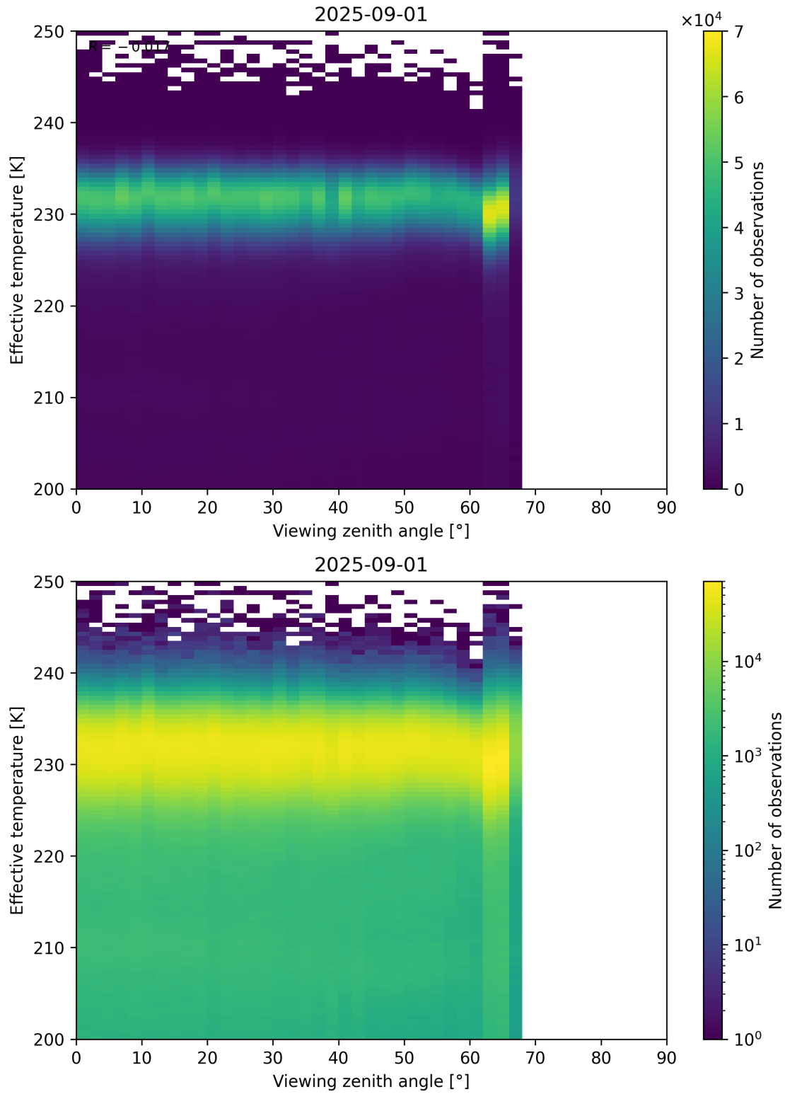
Figure 50: Scatter density plot of “Viewing zenith angle” against “Effective temperature” for 2025-08-31 to 2025-09-02.
