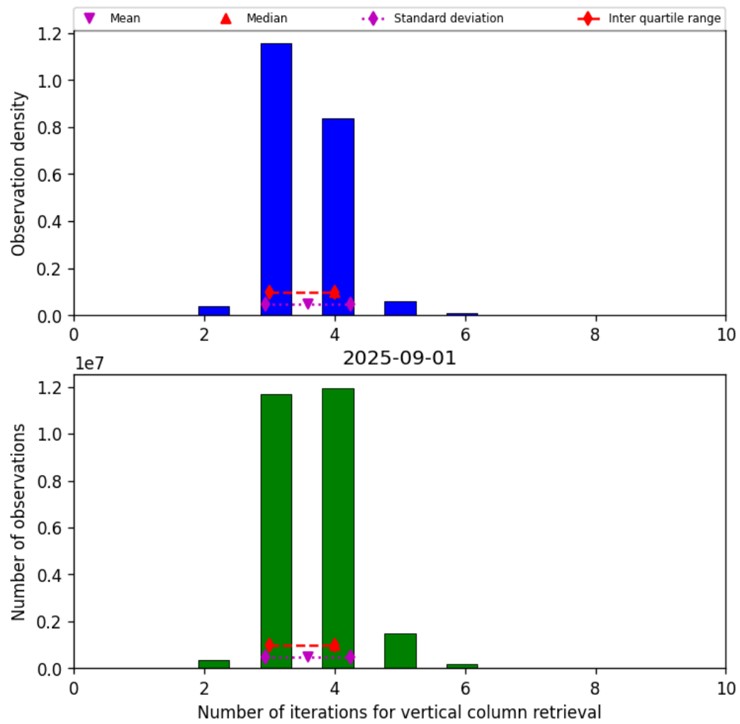
Figure 26: Histogram of “Number of iterations for vertical column retrieval” for 2025-08-31 to 2025-09-02
