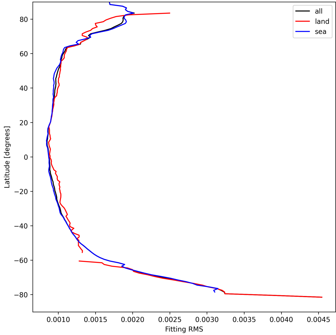
Figure 16: Zonal average of “Fitting RMS” for 2025-08-31 to 2025-09-02.
