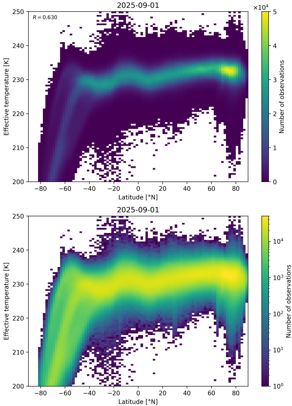
Figure 34: Scatter density plot of “Latitude” against “Effective temperature” for 2025-08-31 to 2025-09-02.
