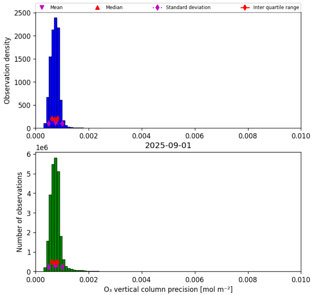
Figure 22: Histogram of “O 3 vertical column precision” for 2025-08-31 to 2025-09-02
