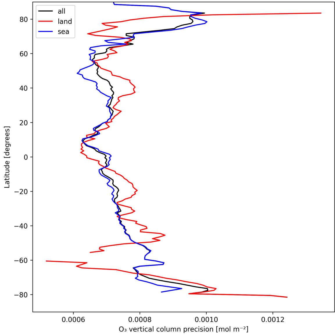
Figure 15: Zonal average of “O 3 vertical column precision” for 2025-08-31 to 2025-09-02.
