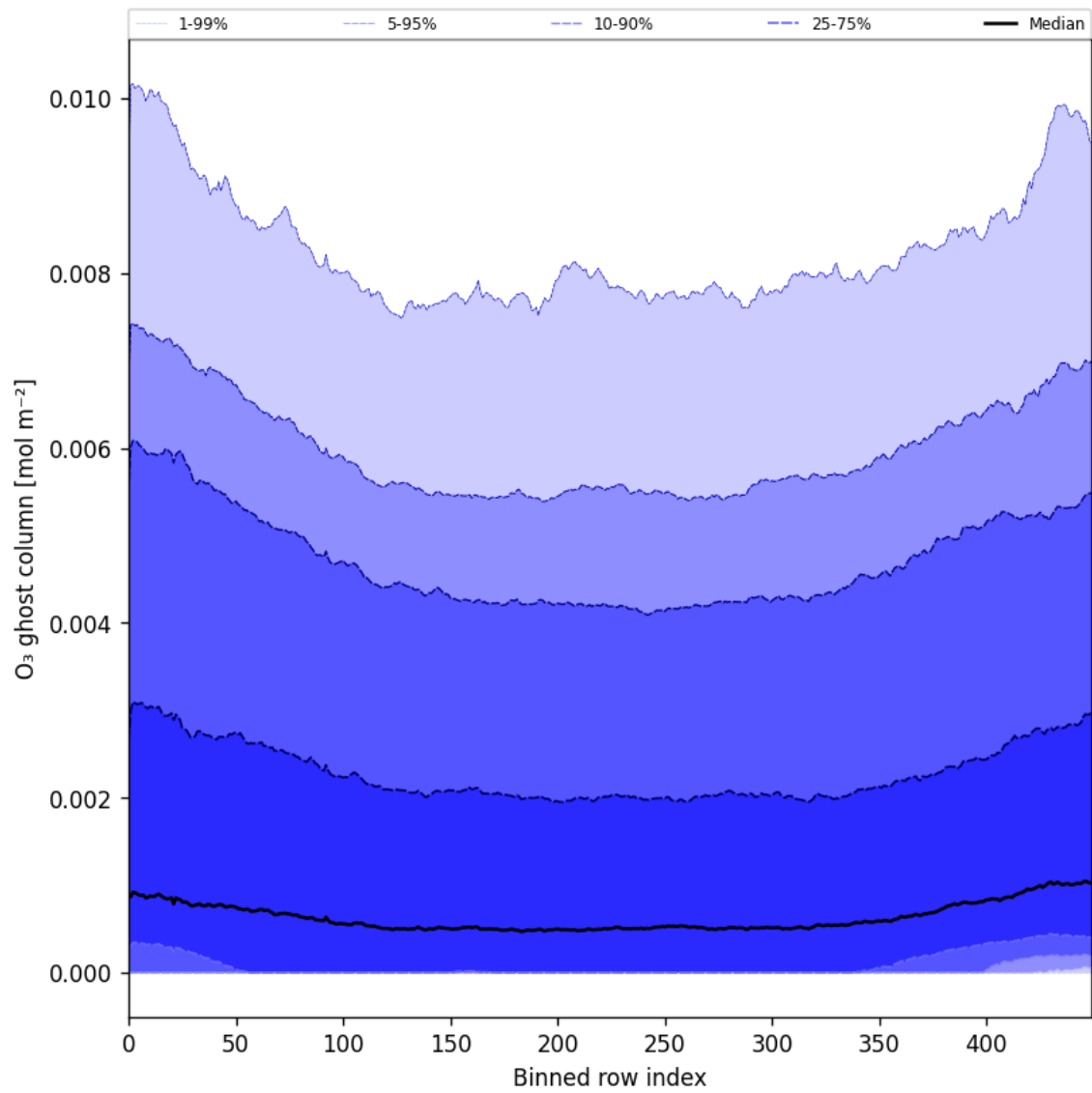
Figure 32: Along track statistics of “O 3 ghost column” for 2025-08-31 to 2025-09-02
