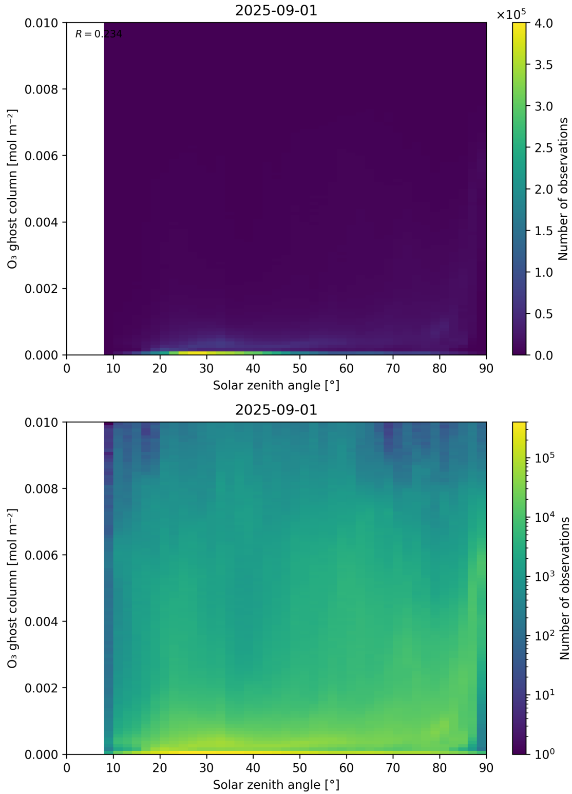
Figure 46: Scatter density plot of “Solar zenith angle” against “O 3 ghost column” for 2025-08-31 to 2025-09-02.
