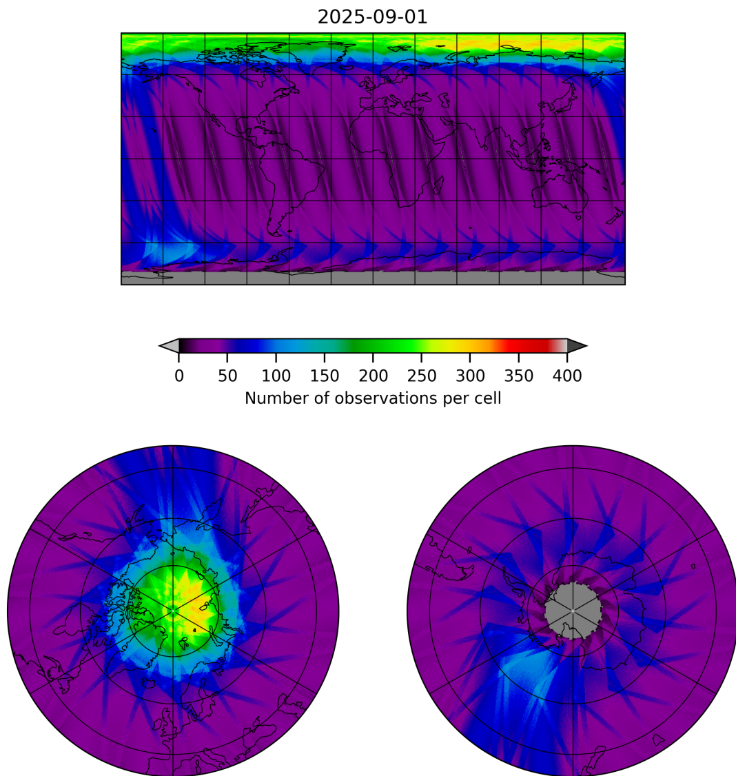
Figure 12: Map of the number of observations for 2025-08-31 to 2025-09-02
