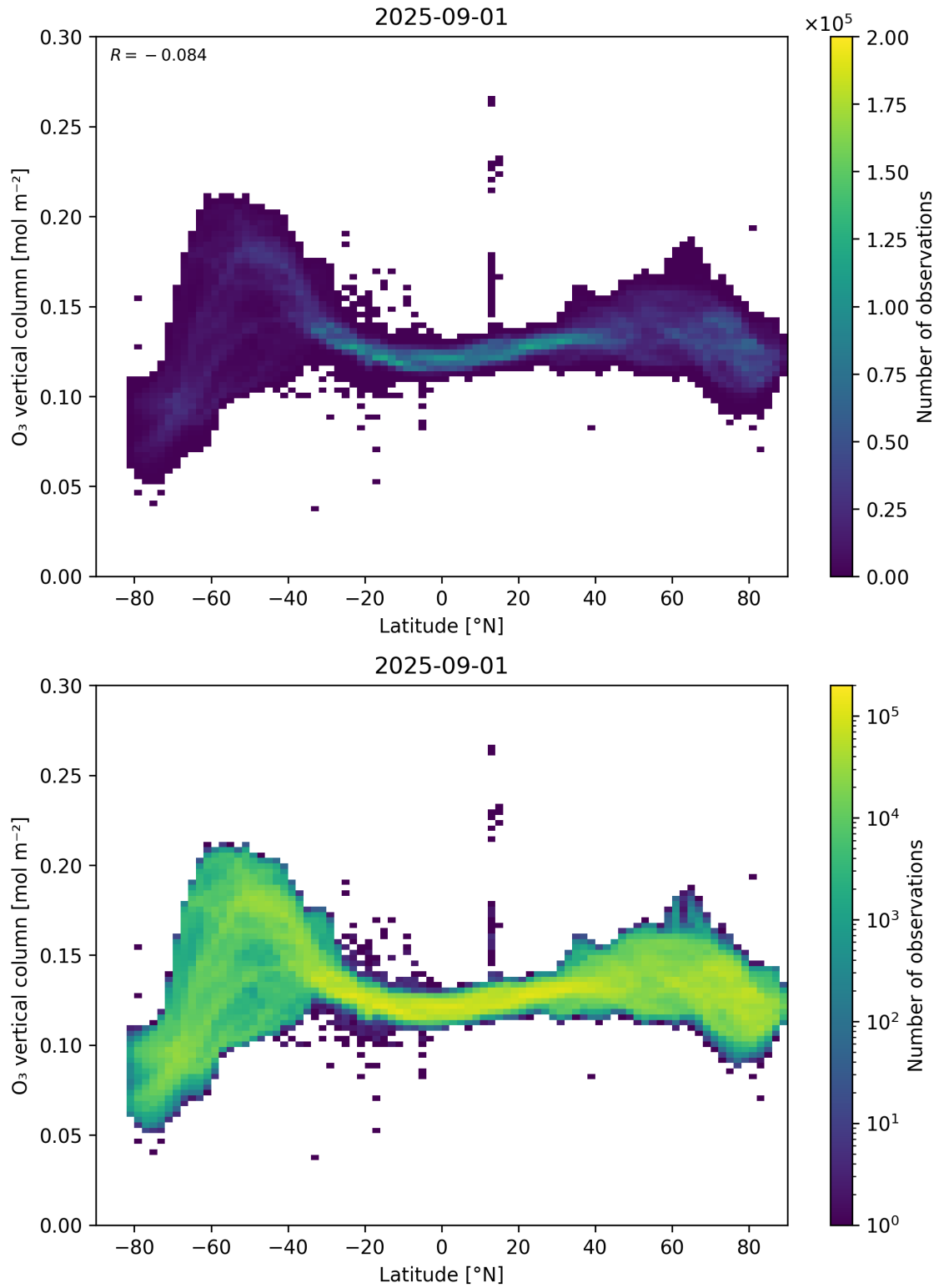
Figure 36: Scatter density plot of “Latitude” against “O 3 vertical column” for 2025-08-31 to 2025-09-02.
