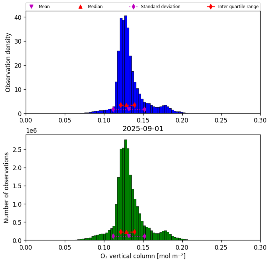
Figure 21: Histogram of “O 3 vertical column” for 2025-08-31 to 2025-09-02
