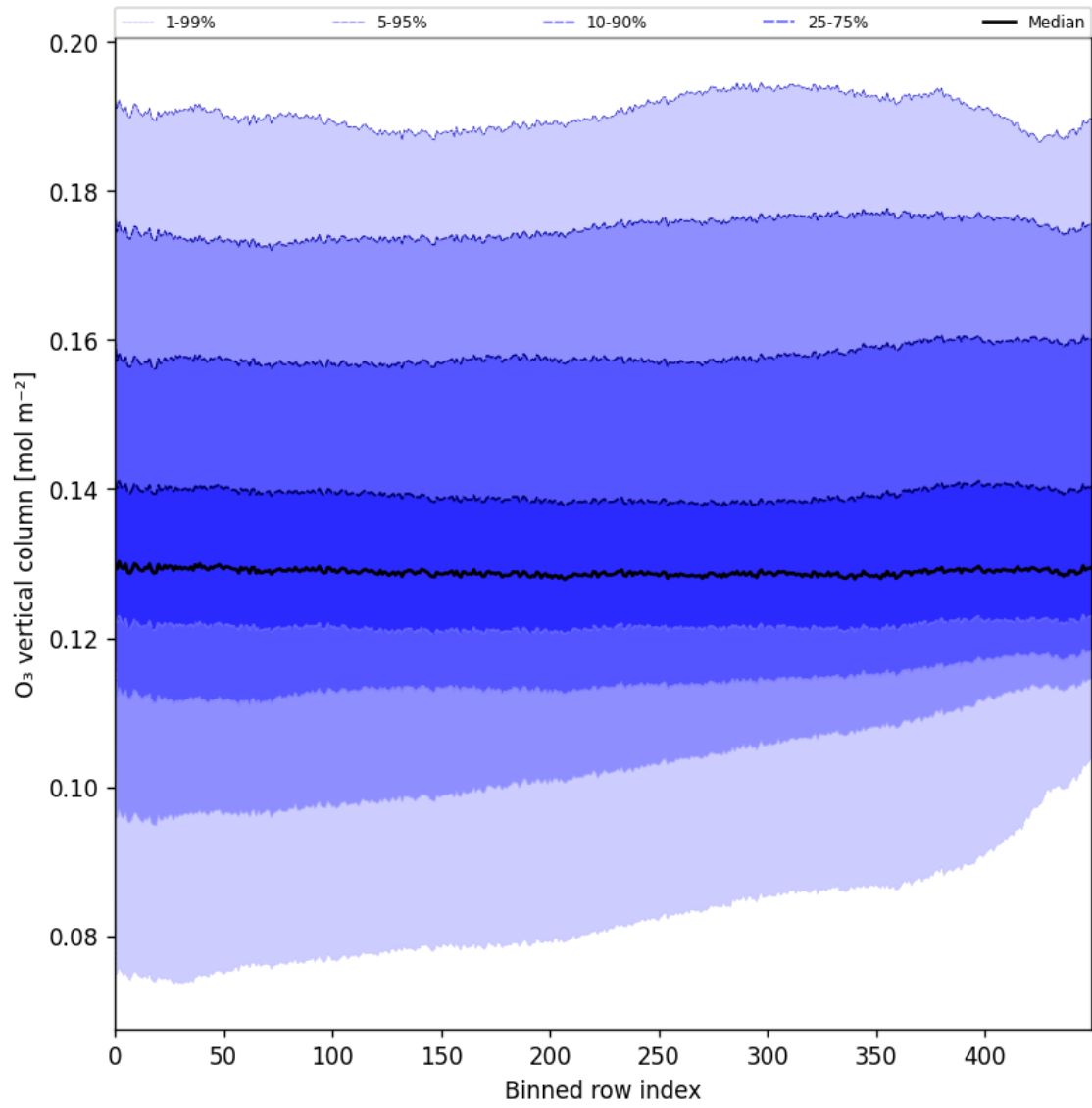
Figure 28: Along track statistics of “O 3 vertical column” for 2025-08-31 to 2025-09-02
