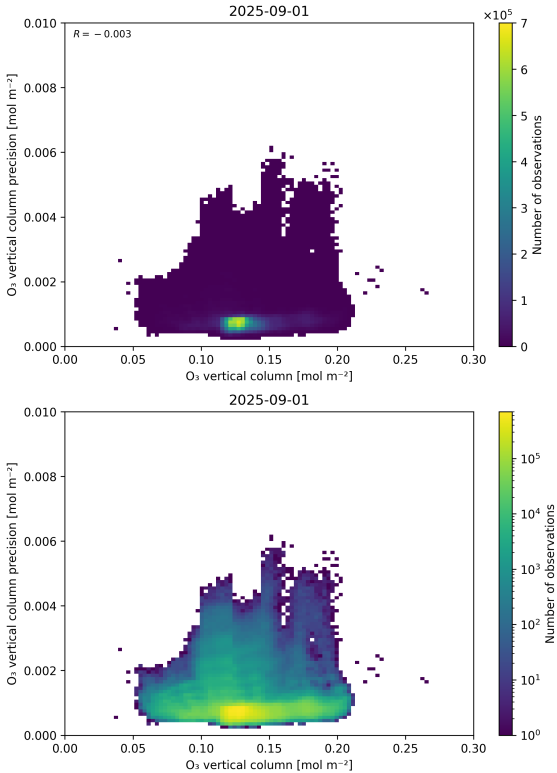
Figure 41: Scatter density plot of “O 3 vertical column” against “O 3 vertical column precision” for 2025-08-31 to 2025-09-02.
