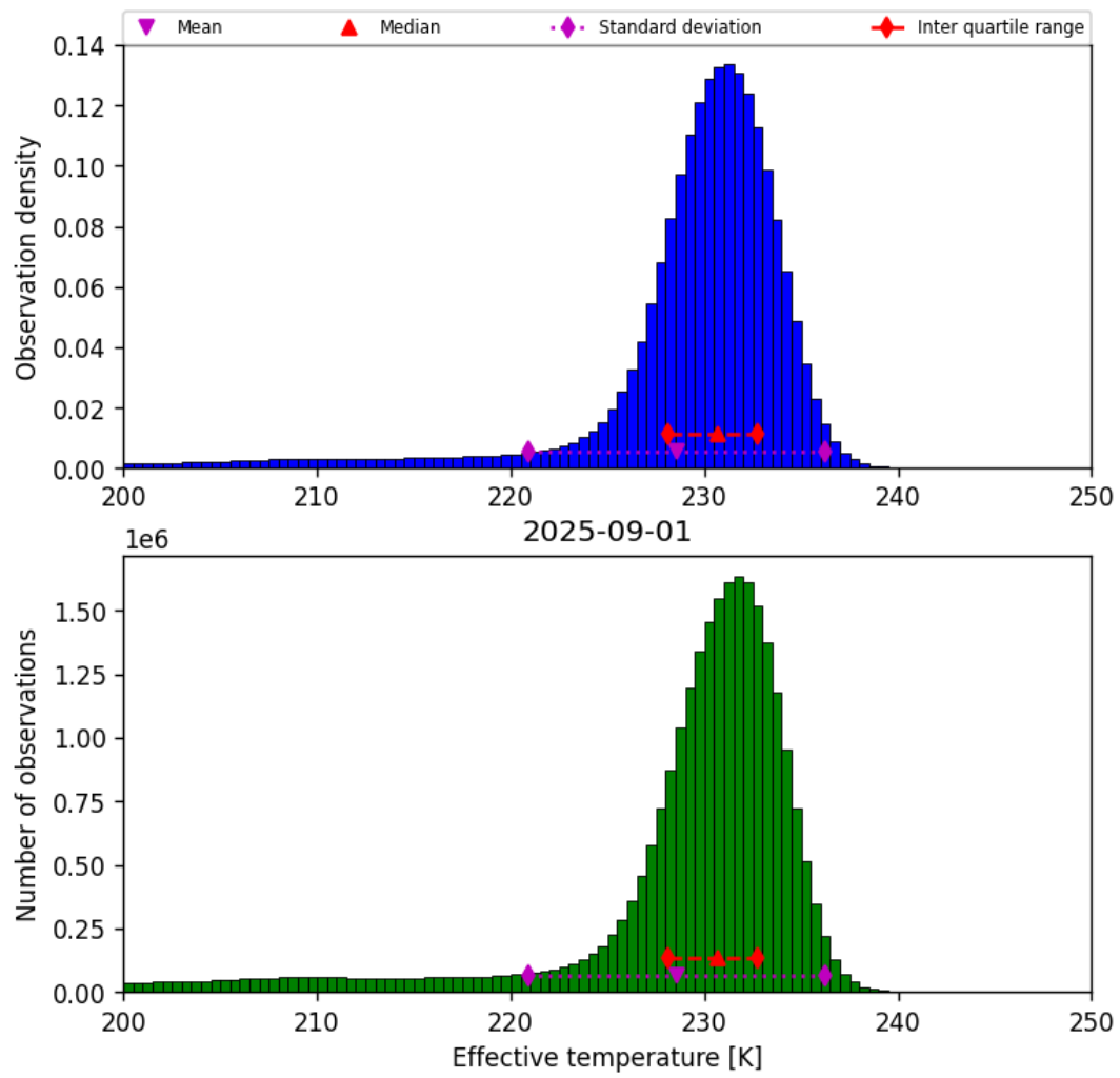
Figure 24: Histogram of “Effective temperature” for 2025-08-31 to 2025-09-02
