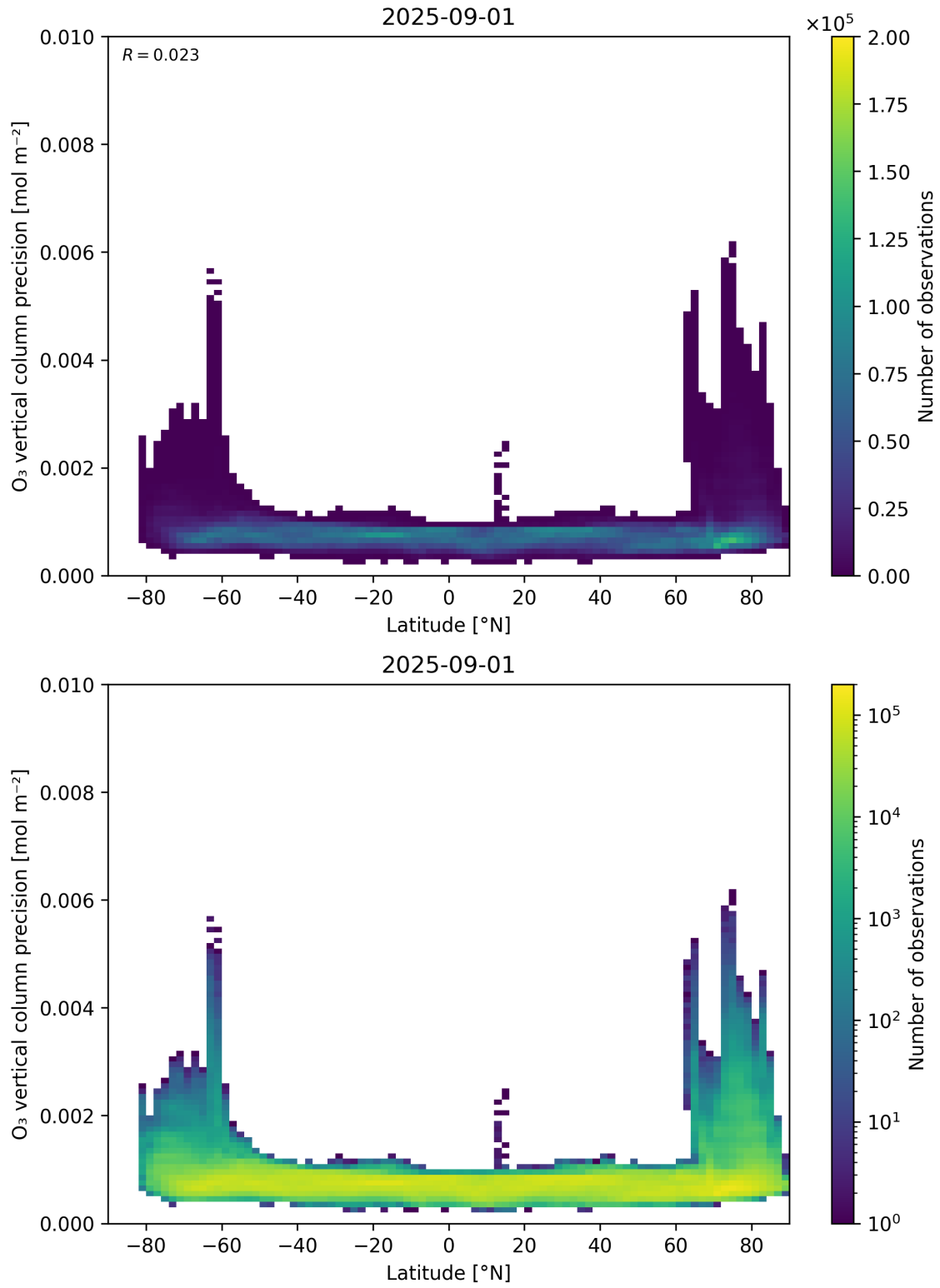
Figure 37: Scatter density plot of “Latitude” against “O 3 vertical column precision” for 2025-08-31 to 2025-09-02.
