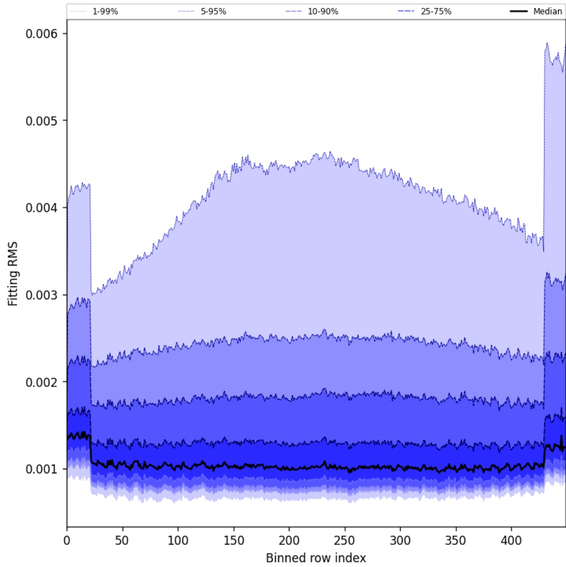
Figure 30: Along track statistics of “Fitting RMS” for 2025-08-31 to 2025-09-02
