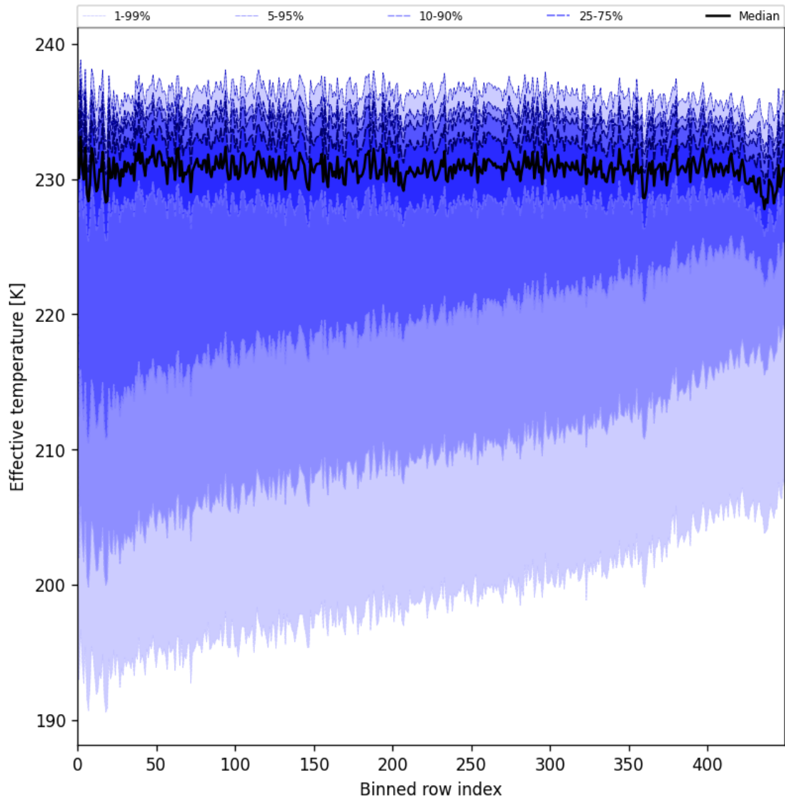
Figure 31: Along track statistics of “Effective temperature” for 2025-08-31 to 2025-09-02
