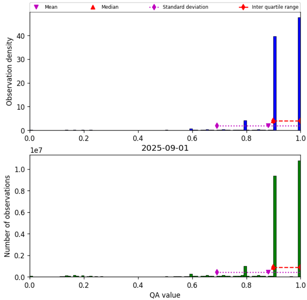
Figure 20: Histogram of “QA value” for 2025-08-31 to 2025-09-02
