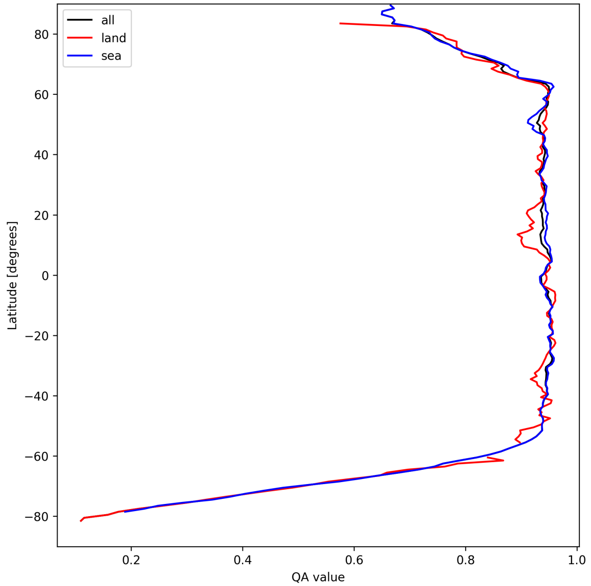
Figure 13: Zonal average of “QA value” for 2025-08-31 to 2025-09-02.
