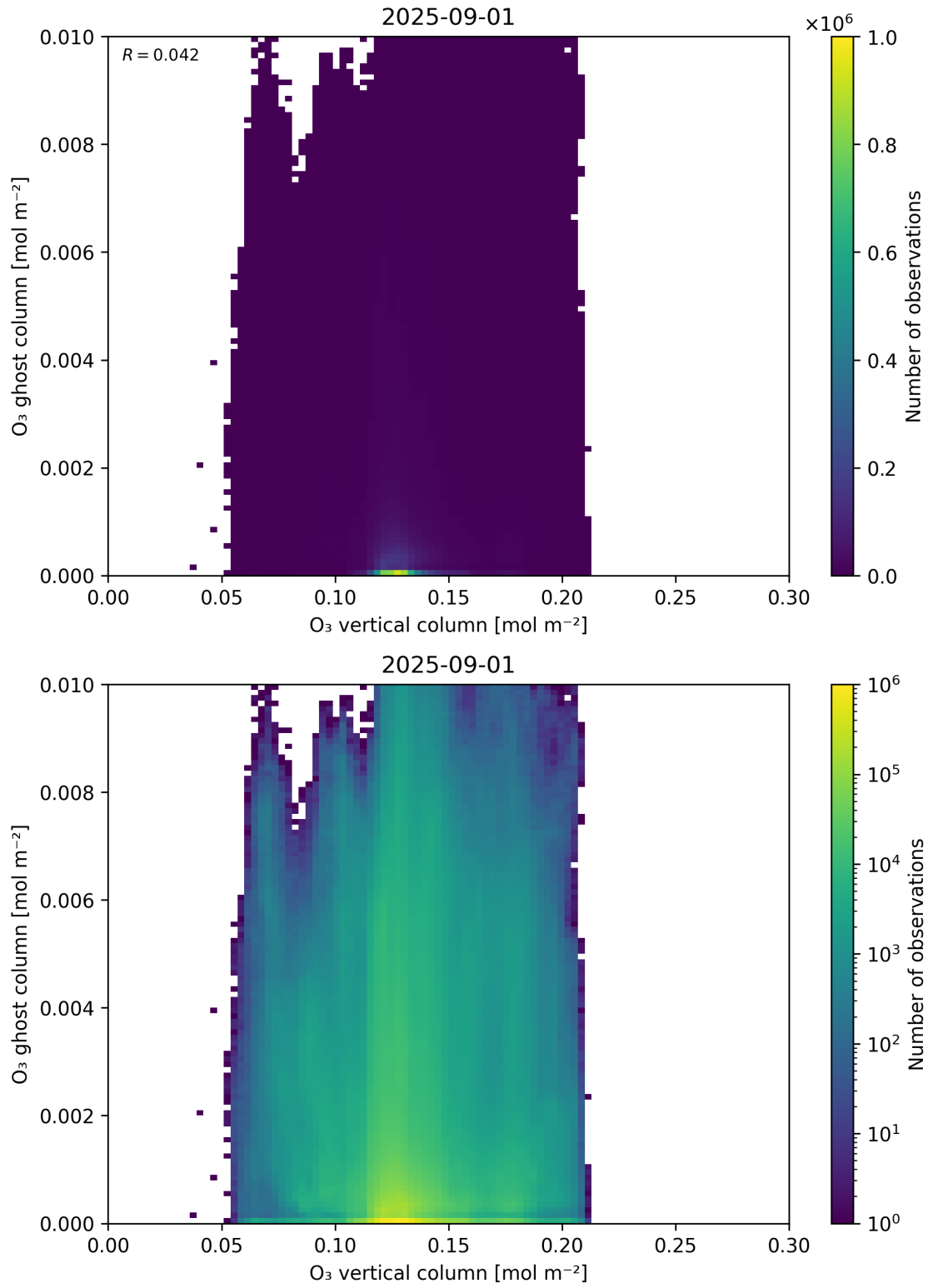
Figure 40: Scatter density plot of “O 3 vertical column” against “O 3 ghost column” for 2025-08-31 to 2025-09-02.
