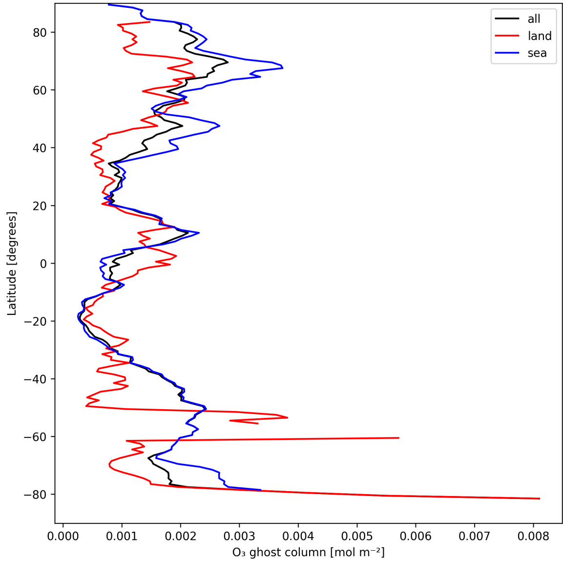
Figure 18: Zonal average of “O 3 ghost column” for 2025-08-31 to 2025-09-02.
