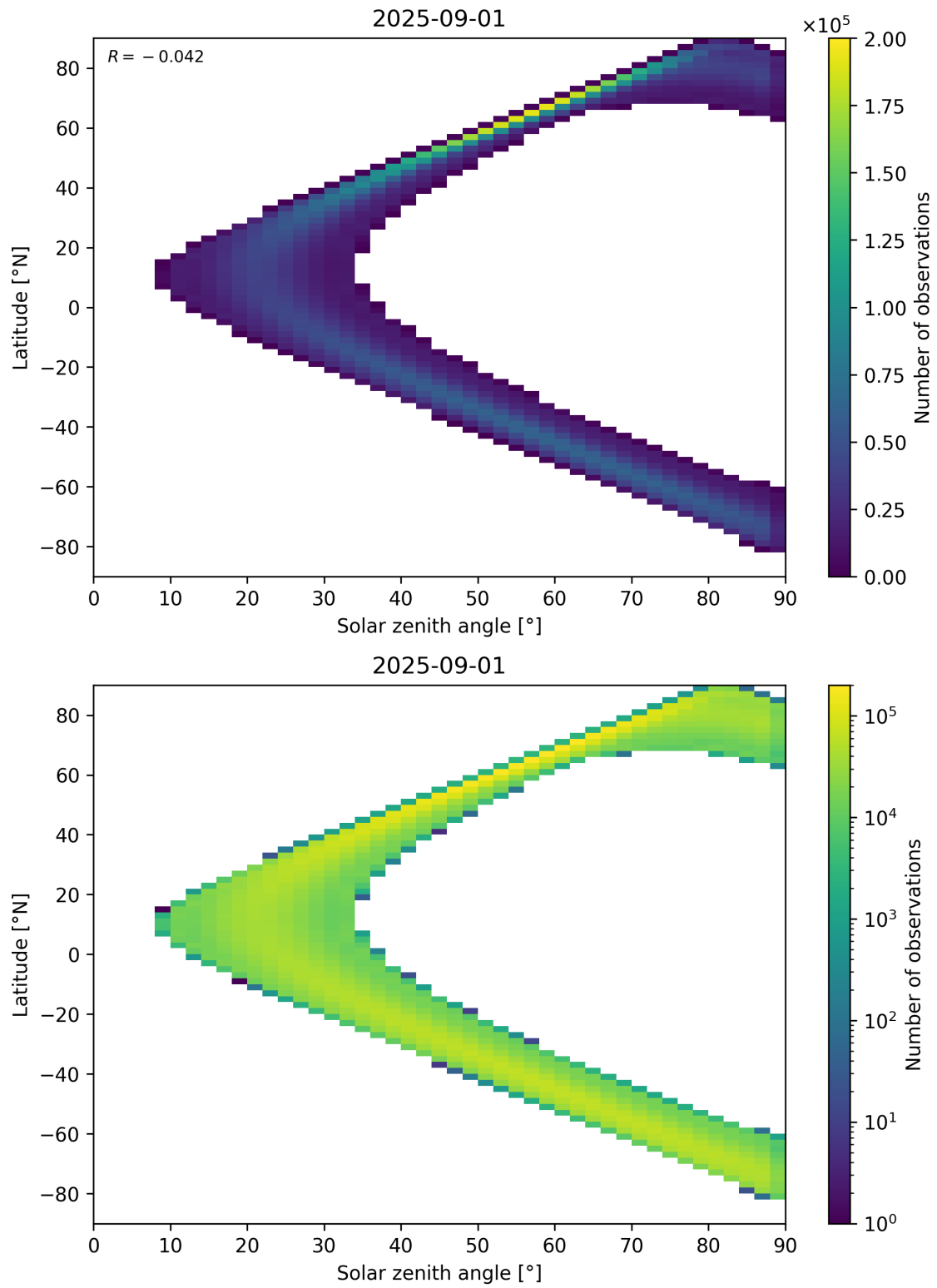
Figure 44: Scatter density plot of “Solar zenith angle” against “Latitude” for 2025-08-31 to 2025-09-02.
