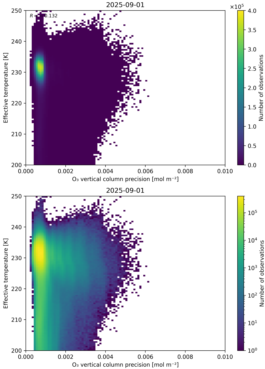
Figure 42: Scatter density plot of “O 3 vertical column precision” against “Effective temperature” for 2025-08-31 to 2025-09-02.
