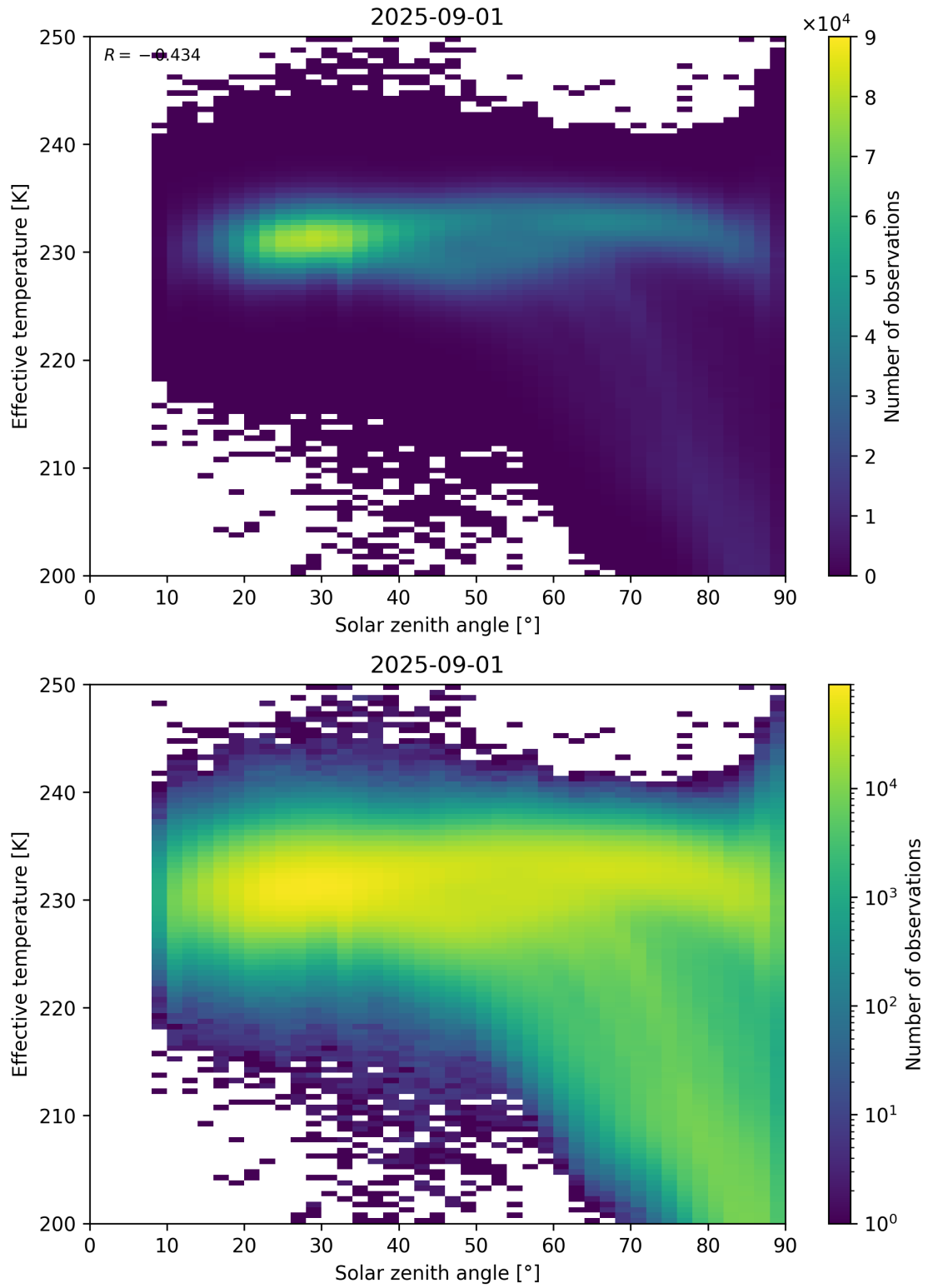
Figure 45: Scatter density plot of “Solar zenith angle” against “Effective temperature” for 2025-08-31 to 2025-09-02.
