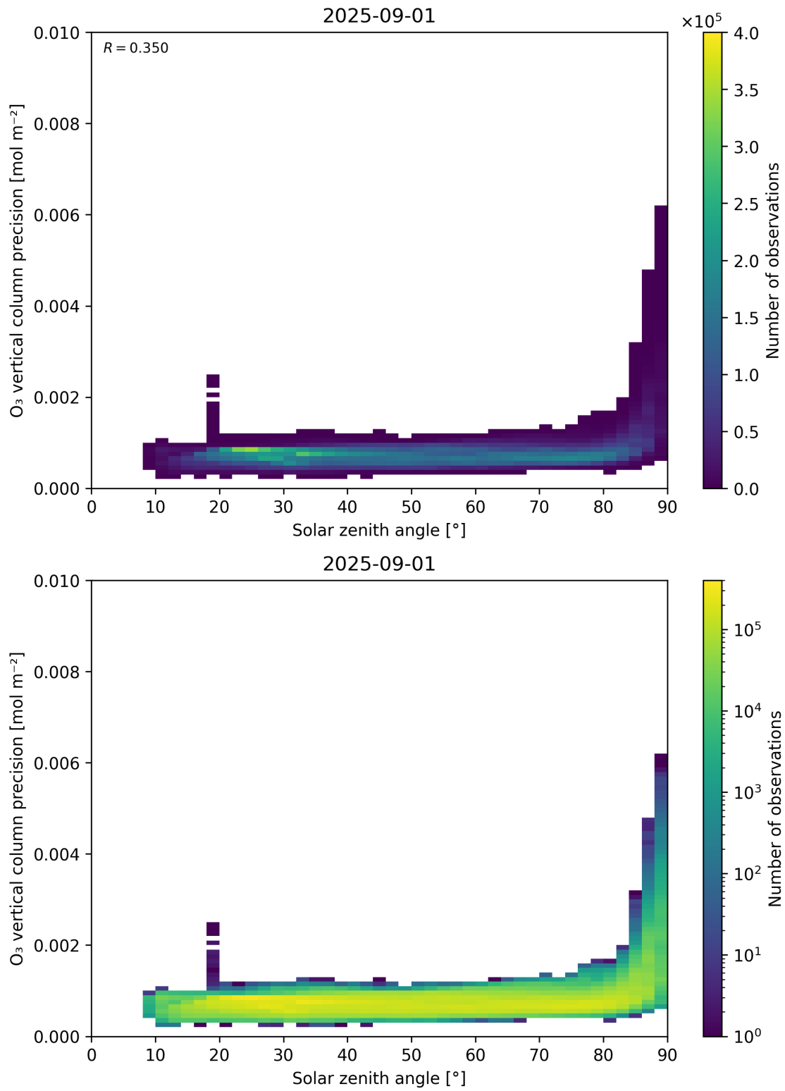
Figure 48: Scatter density plot of “Solar zenith angle” against “O 3 vertical column precision” for 2025-08-31 to 2025-09-02.
