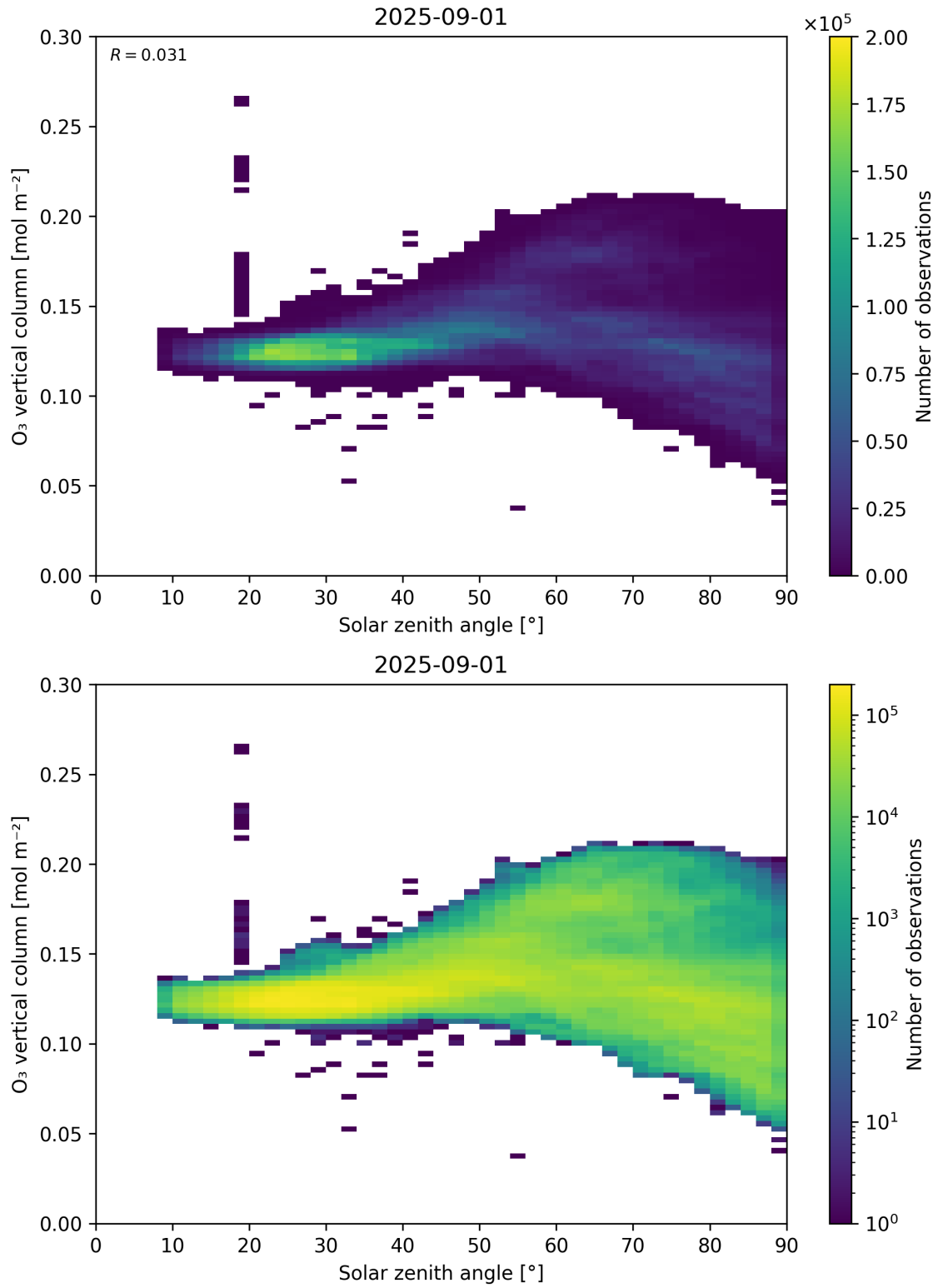
Figure 47: Scatter density plot of “Solar zenith angle” against “O 3 vertical column” for 2025-08-31 to 2025-09-02.
