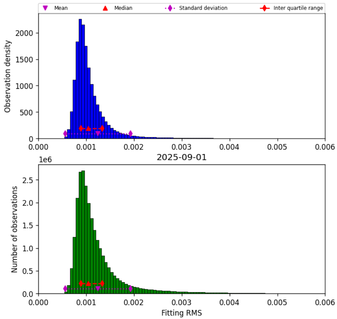
Figure 23: Histogram of “Fitting RMS” for 2025-08-31 to 2025-09-02
