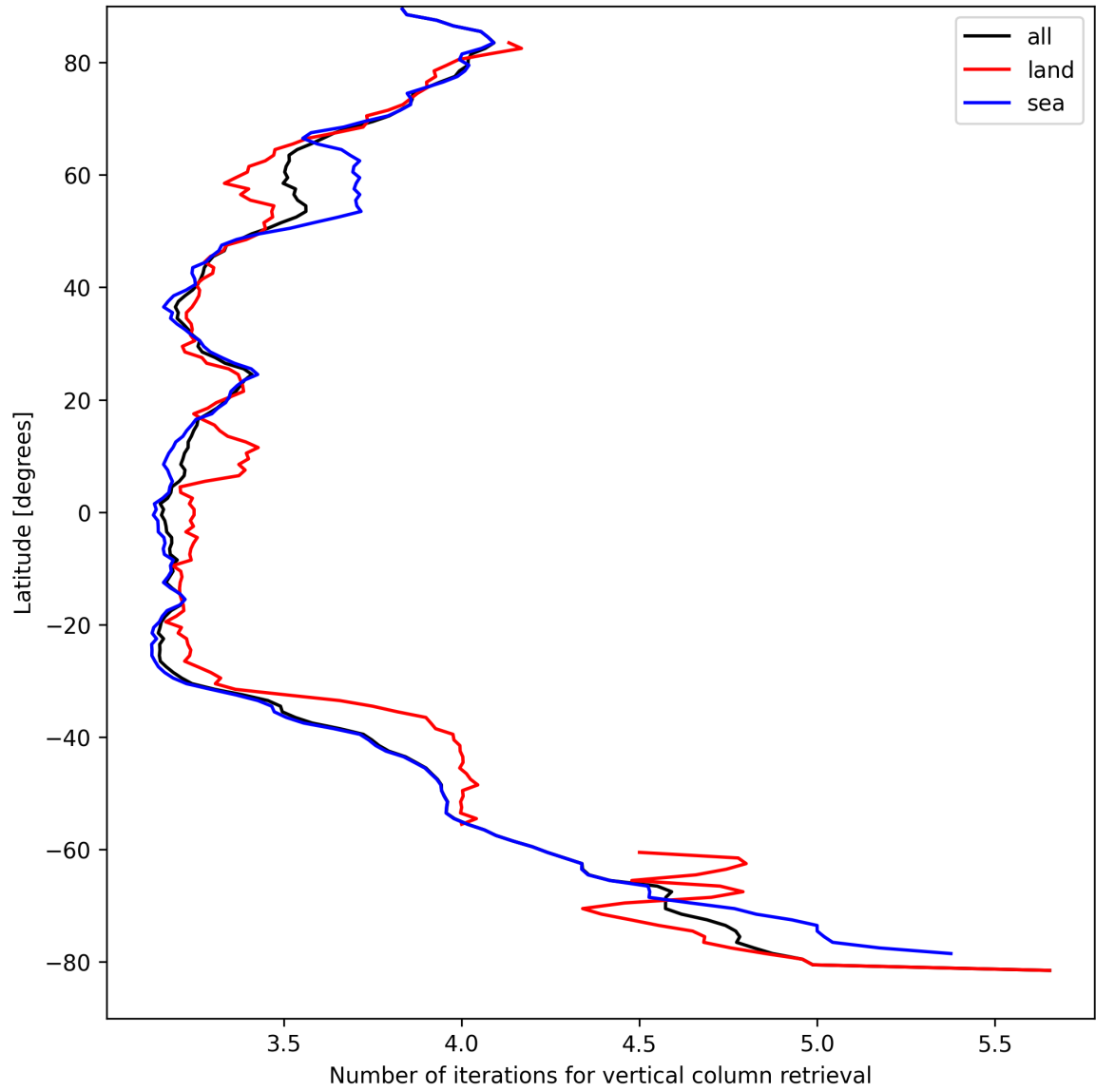
Figure 19: Zonal average of “Number of iterations for vertical column retrieval” for 2025-08-31 to 2025-09-02.
