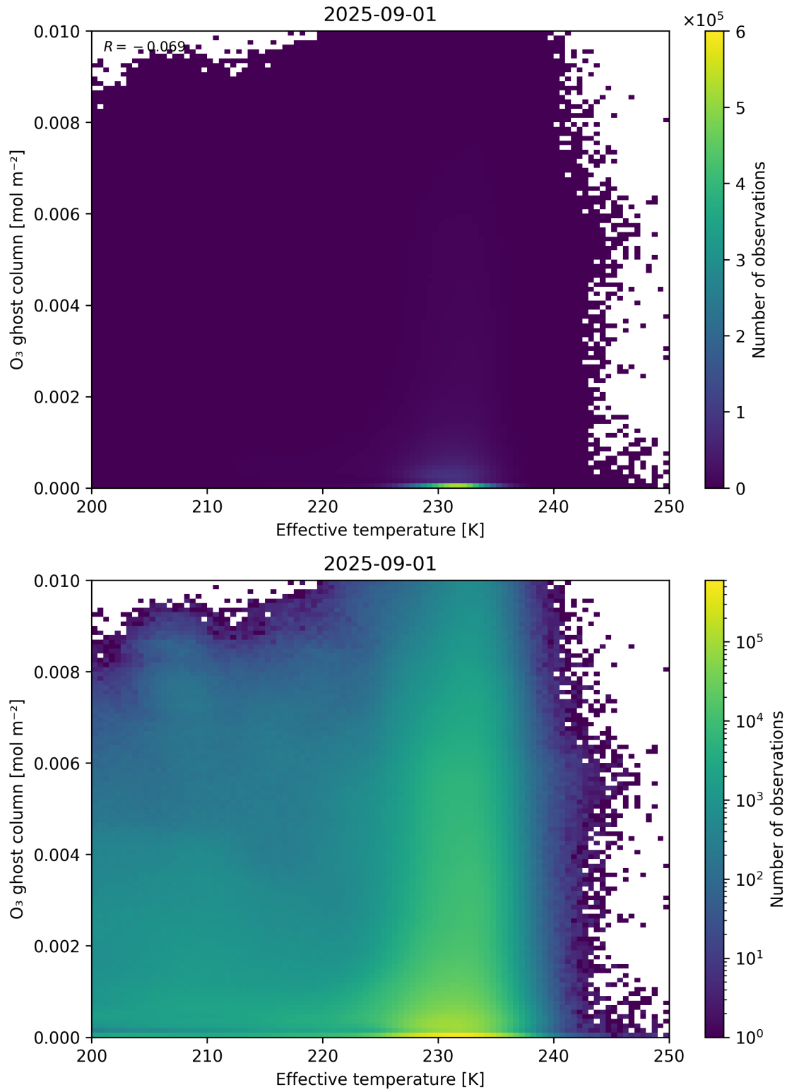
Figure 38: Scatter density plot of “Effective temperature” against “O 3 ghost column” for 2025-08-31 to 2025-09-02.
