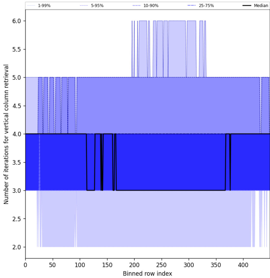
Figure 33: Along track statistics of “Number of iterations for vertical column retrieval” for 2025-08-31 to 2025-09-02
