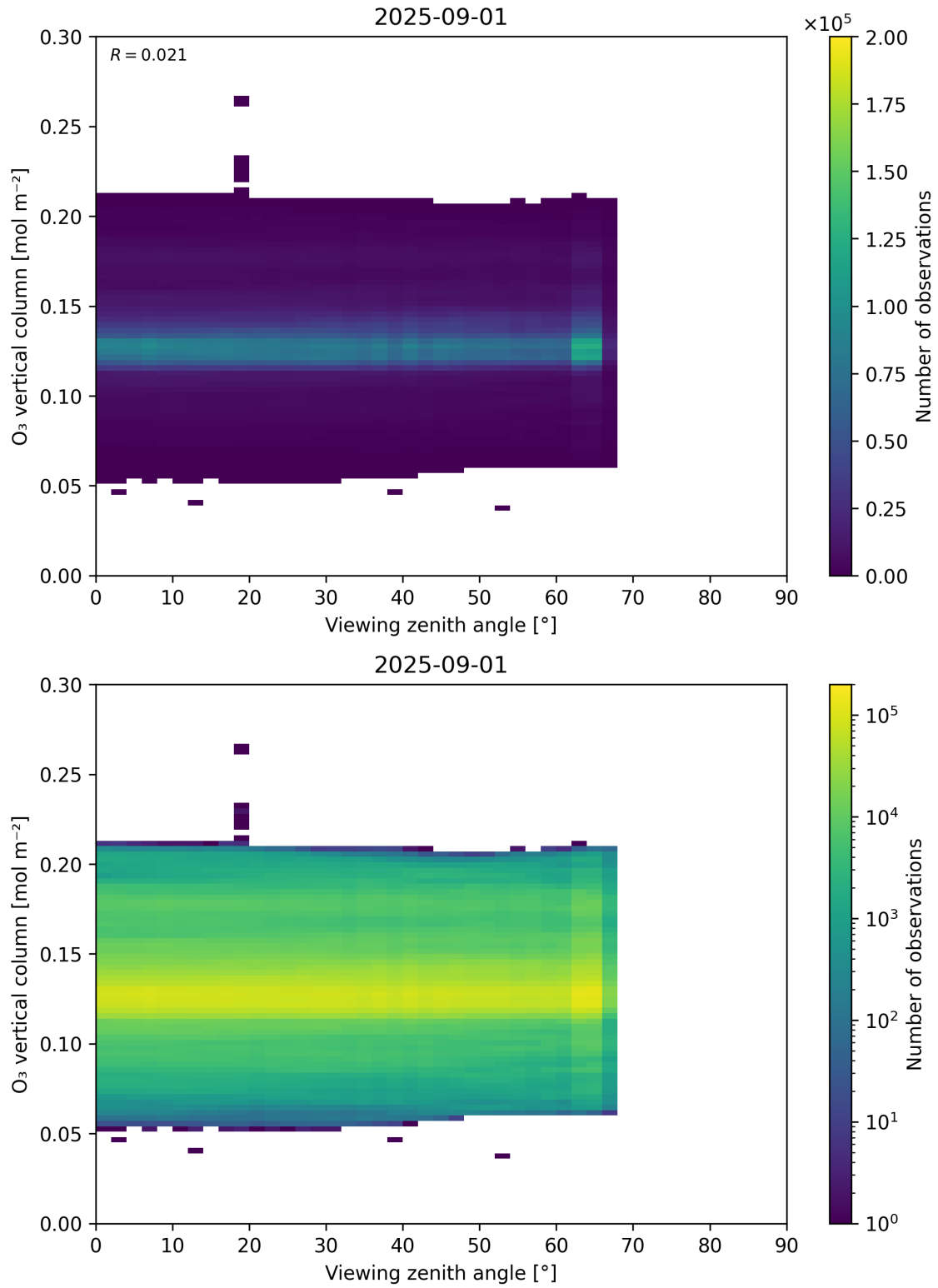
Figure 52: Scatter density plot of “Viewing zenith angle” against “O 3 vertical column” for 2025-08-31 to 2025-09-02.
