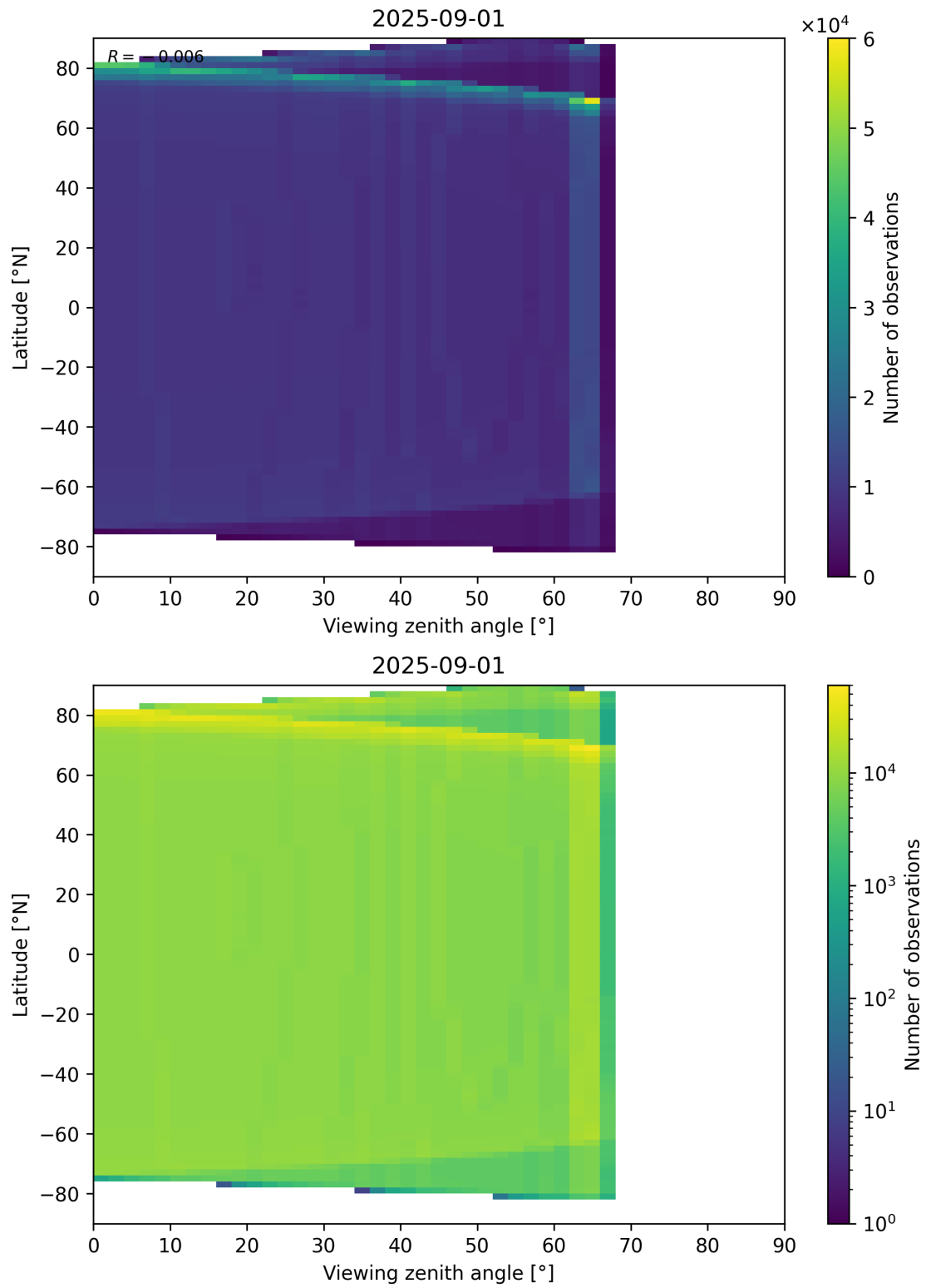
Figure 49: Scatter density plot of “Viewing zenith angle” against “Latitude” for 2025-08-31 to 2025-09-02.
