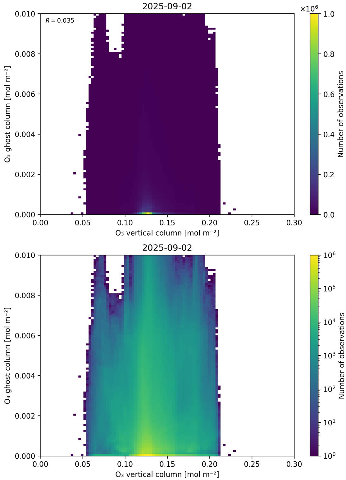
Figure 40: Scatter density plot of “O 3 vertical column” against “O 3 ghost column” for 2025-09-01 to 2025-09-03.
