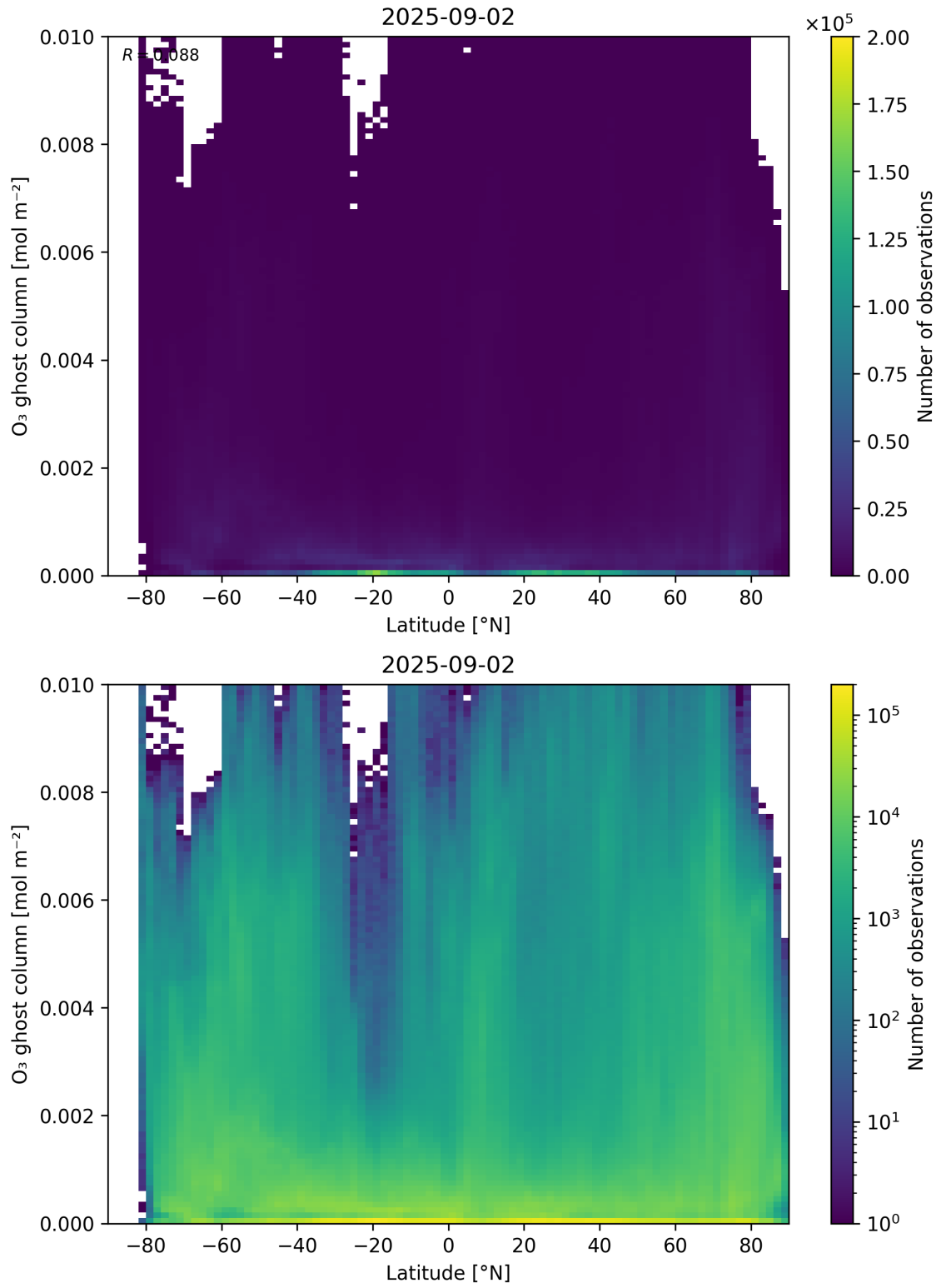
Figure 35: Scatter density plot of “Latitude” against “O 3 ghost column” for 2025-09-01 to 2025-09-03.
