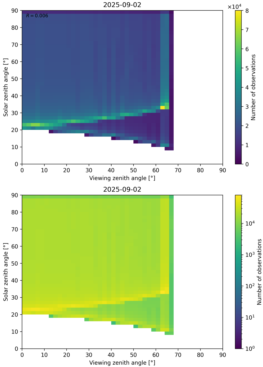
Figure 54: Scatter density plot of “Viewing zenith angle” against “Solar zenith angle” for 2025-09-01 to 2025-09-03.
