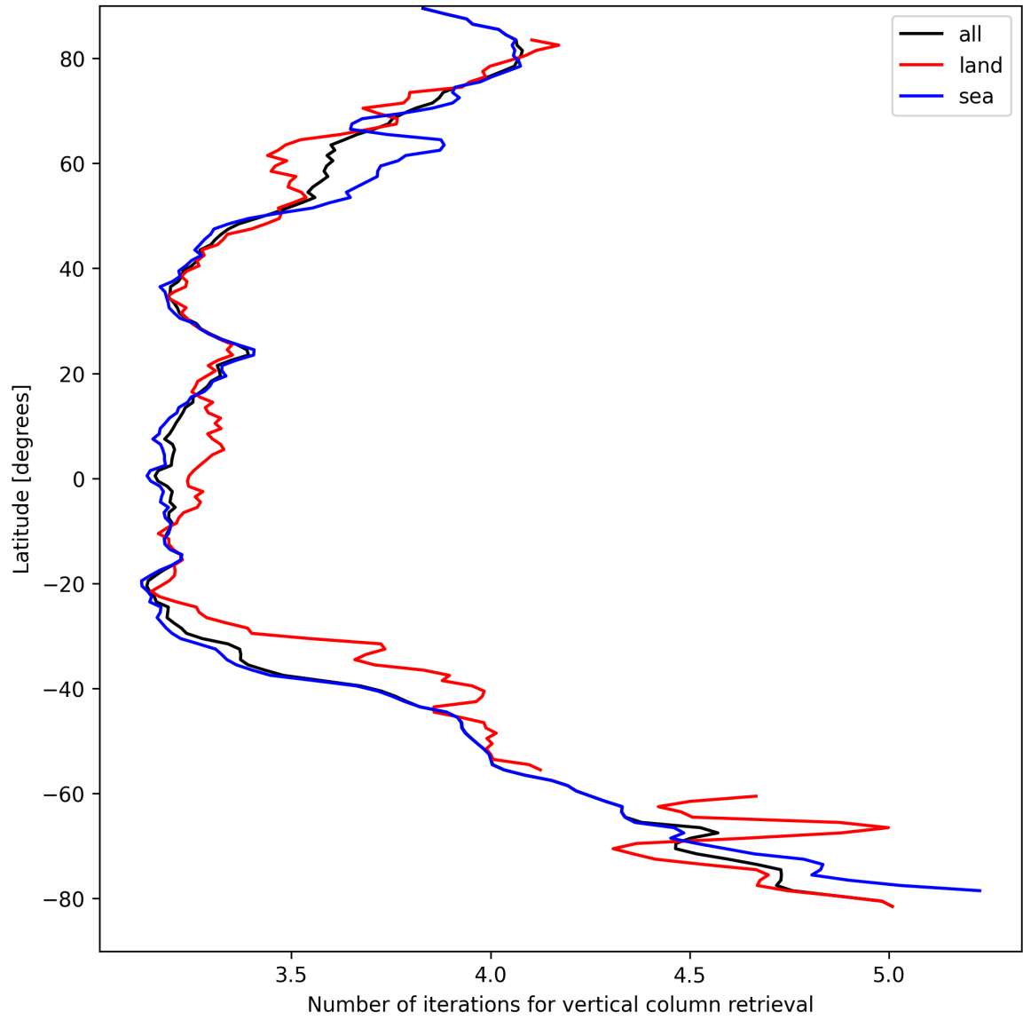
Figure 19: Zonal average of “Number of iterations for vertical column retrieval” for 2025-09-01 to 2025-09-03.
