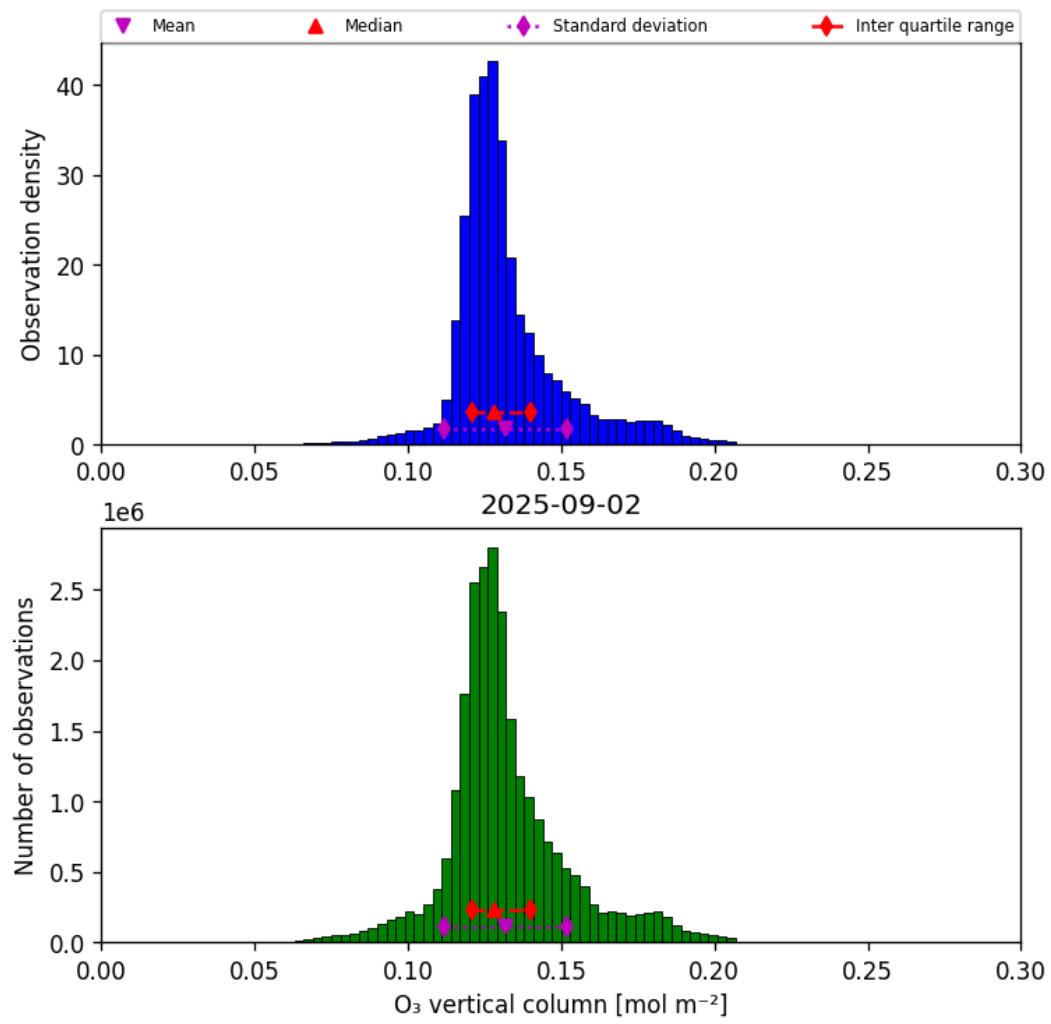
Figure 21: Histogram of “O 3 vertical column” for 2025-09-01 to 2025-09-03
