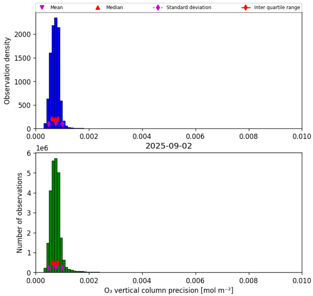
Figure 22: Histogram of “O 3 vertical column precision” for 2025-09-01 to 2025-09-03
