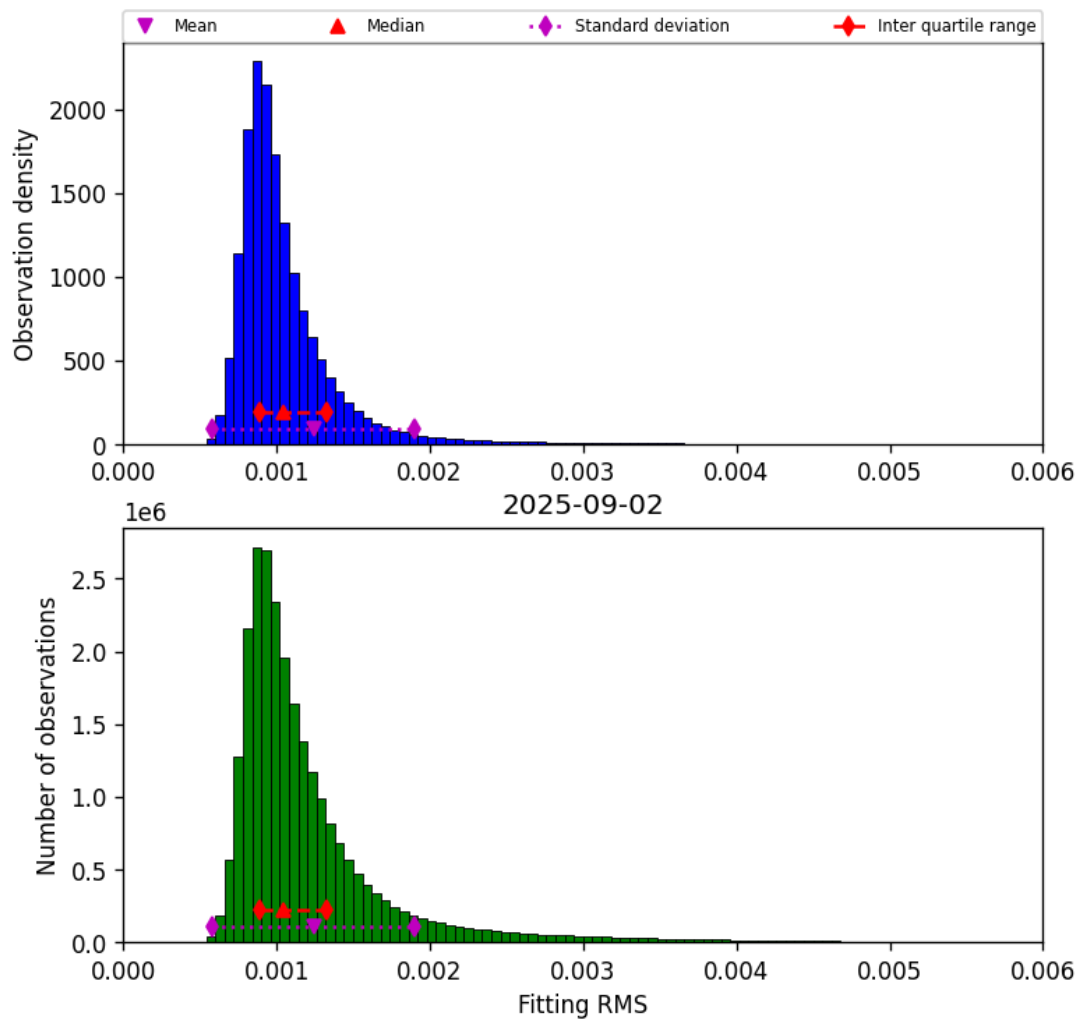
Figure 23: Histogram of “Fitting RMS” for 2025-09-01 to 2025-09-03
