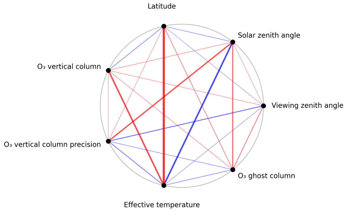
Figure 1: Map of correlation graph for 2025-09-01 to 2025-09-03.
