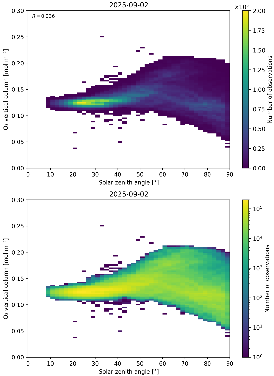
Figure 47: Scatter density plot of “Solar zenith angle” against “O 3 vertical column” for 2025-09-01 to 2025-09-03.
