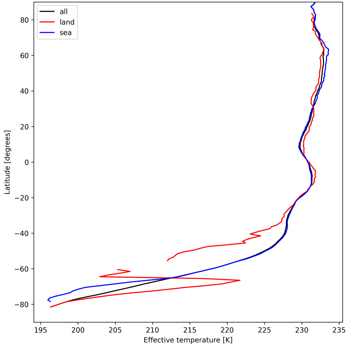
Figure 17: Zonal average of "Effective temperature" for 2025-09-01 to 2025-09-03.
