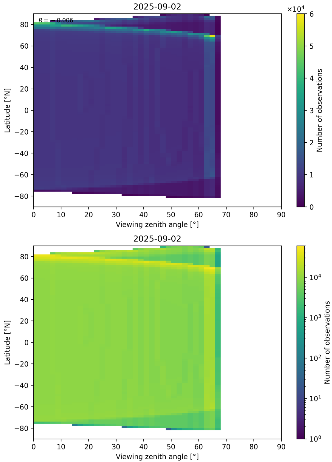
Figure 49: Scatter density plot of “Viewing zenith angle” against “Latitude” for 2025-09-01 to 2025-09-03.
