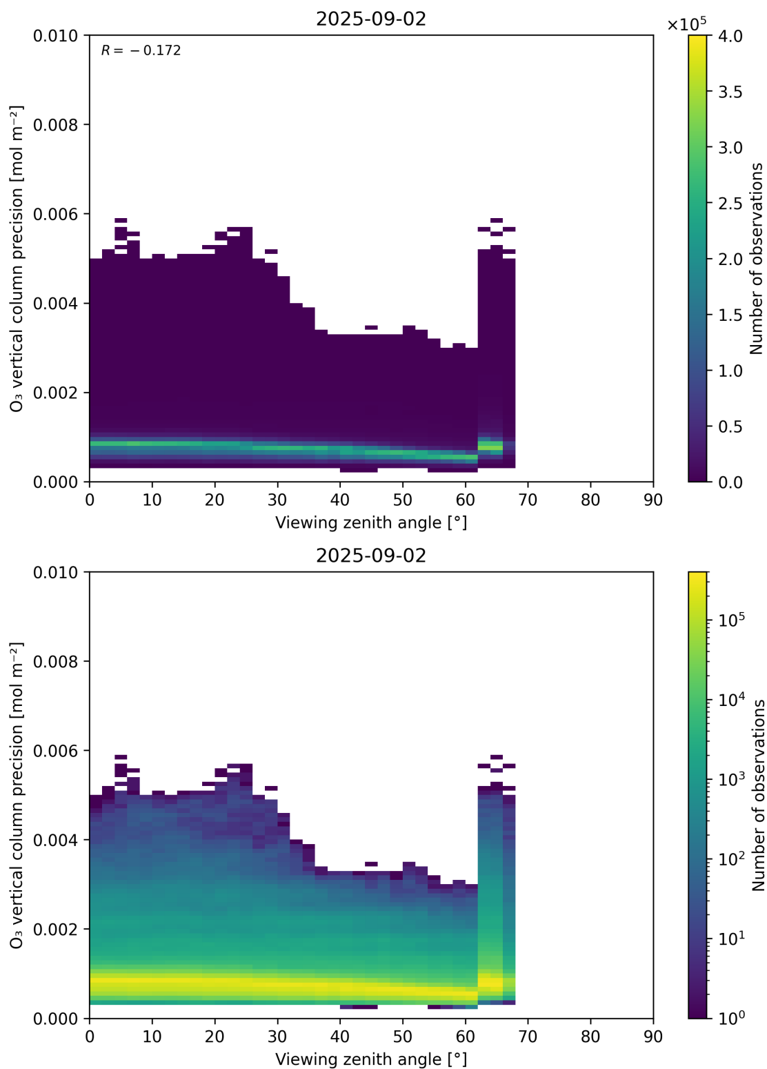
Figure 53: Scatter density plot of “Viewing zenith angle” against “O 3 vertical column precision” for 2025-09-01 to 2025-09-03.
