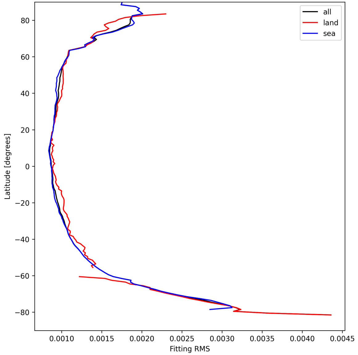
Figure 16: Zonal average of “Fitting RMS” for 2025-09-01 to 2025-09-03.
