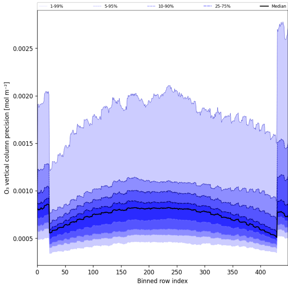
Figure 29: Along track statistics of “O 3 vertical column precision” for 2025-09-01 to 2025-09-03
