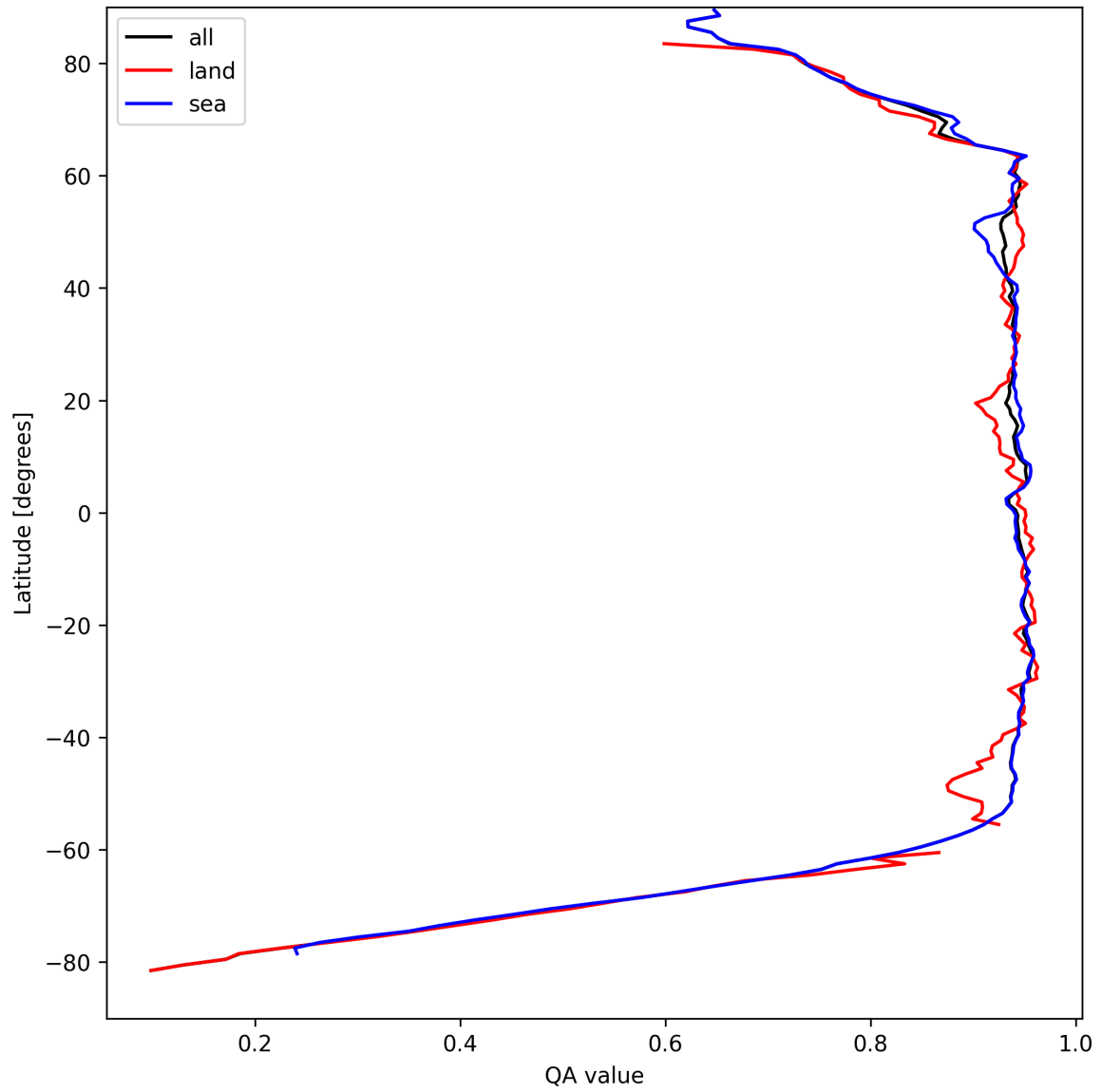
Figure 13: Zonal average of “QA value” for 2025-09-01 to 2025-09-03.
