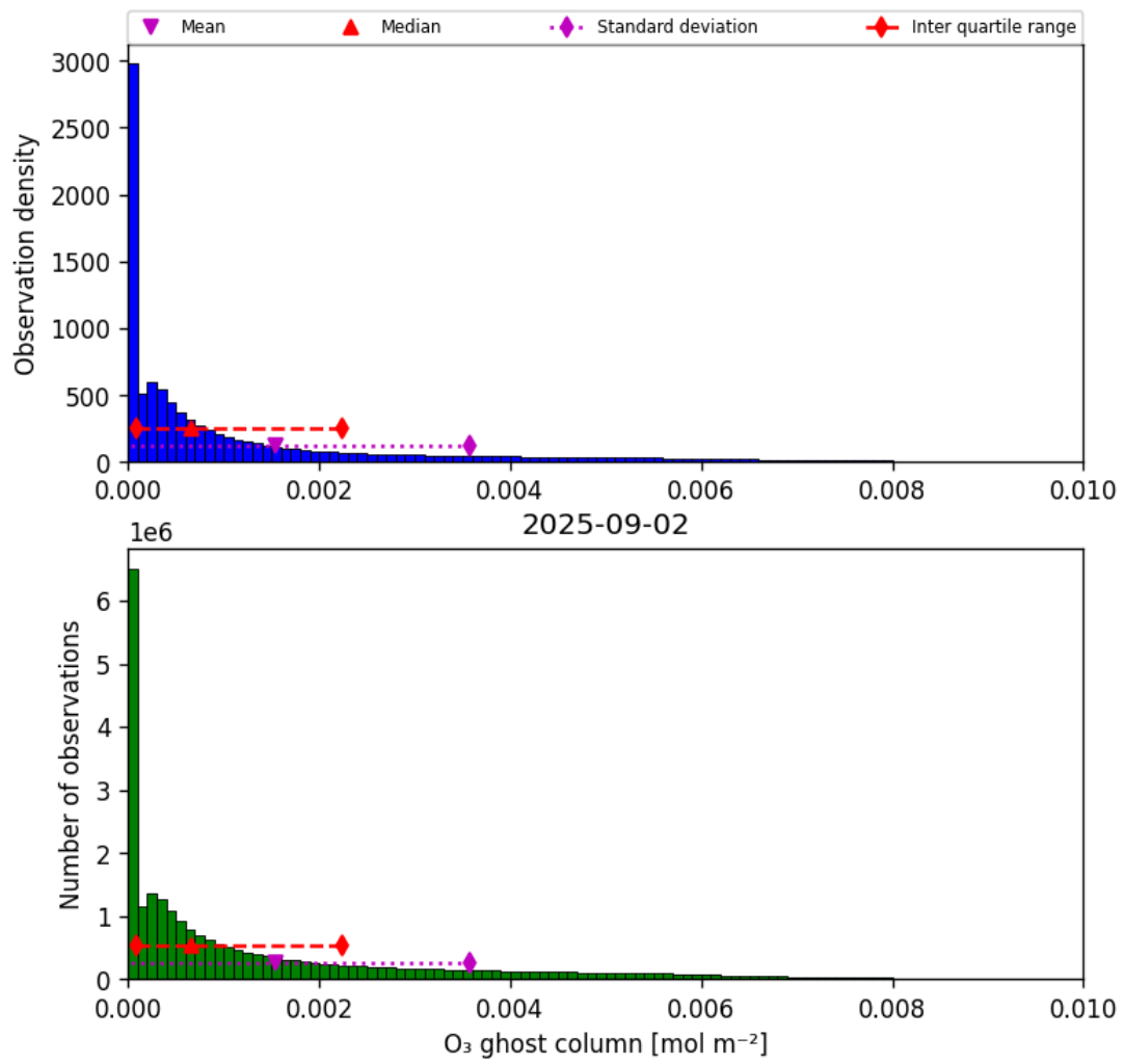
Figure 25: Histogram of “O 3 ghost column” for 2025-09-01 to 2025-09-03
