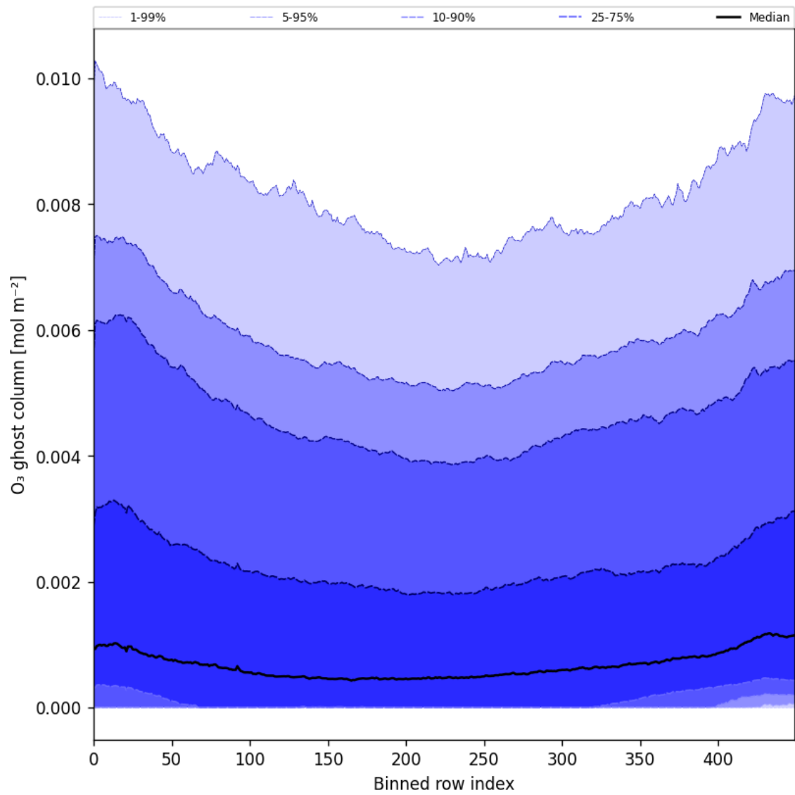
Figure 32: Along track statistics of “O 3 ghost column” for 2025-09-01 to 2025-09-03
