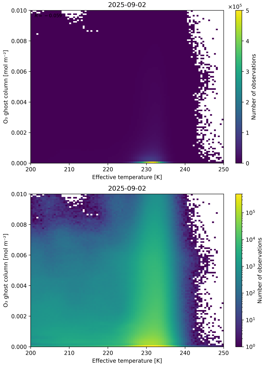
Figure 38: Scatter density plot of “Effective temperature” against “O 3 ghost column” for 2025-09-01 to 2025-09-03.
