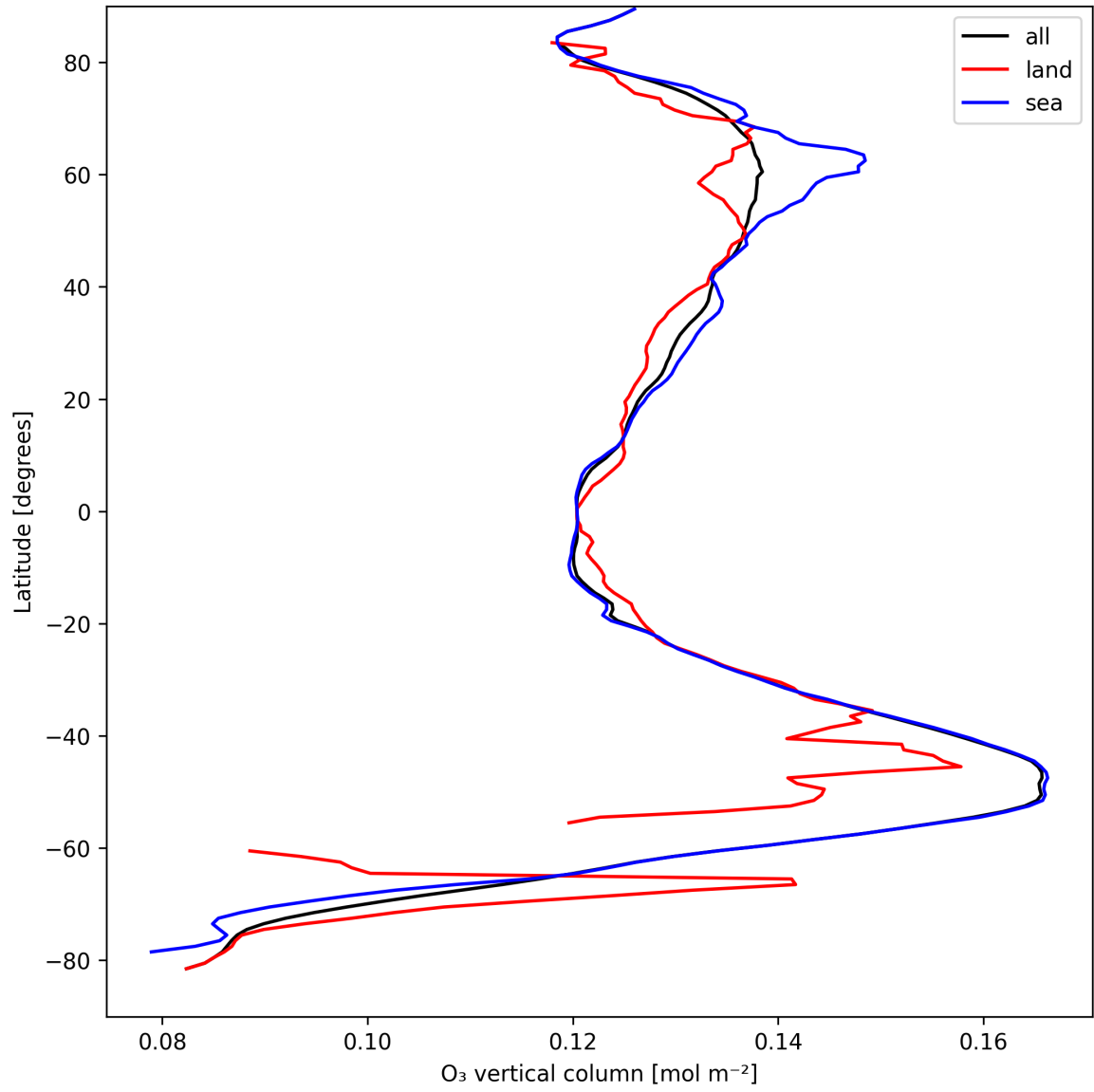
Figure 14: Zonal average of “O 3 vertical column” for 2025-09-01 to 2025-09-03.
