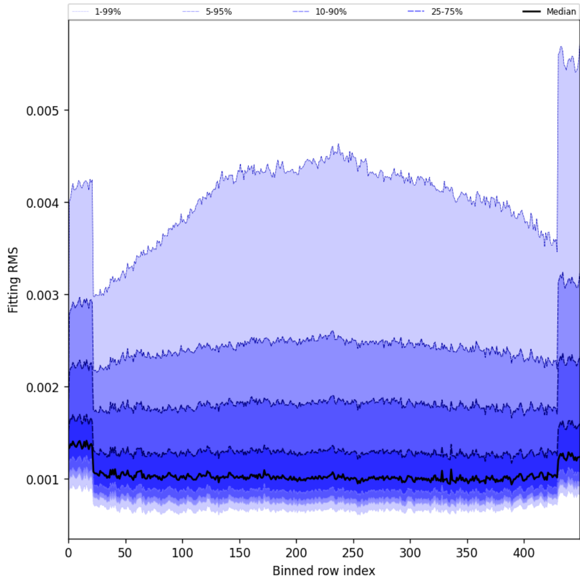
Figure 30: Along track statistics of “Fitting RMS” for 2025-09-01 to 2025-09-03
