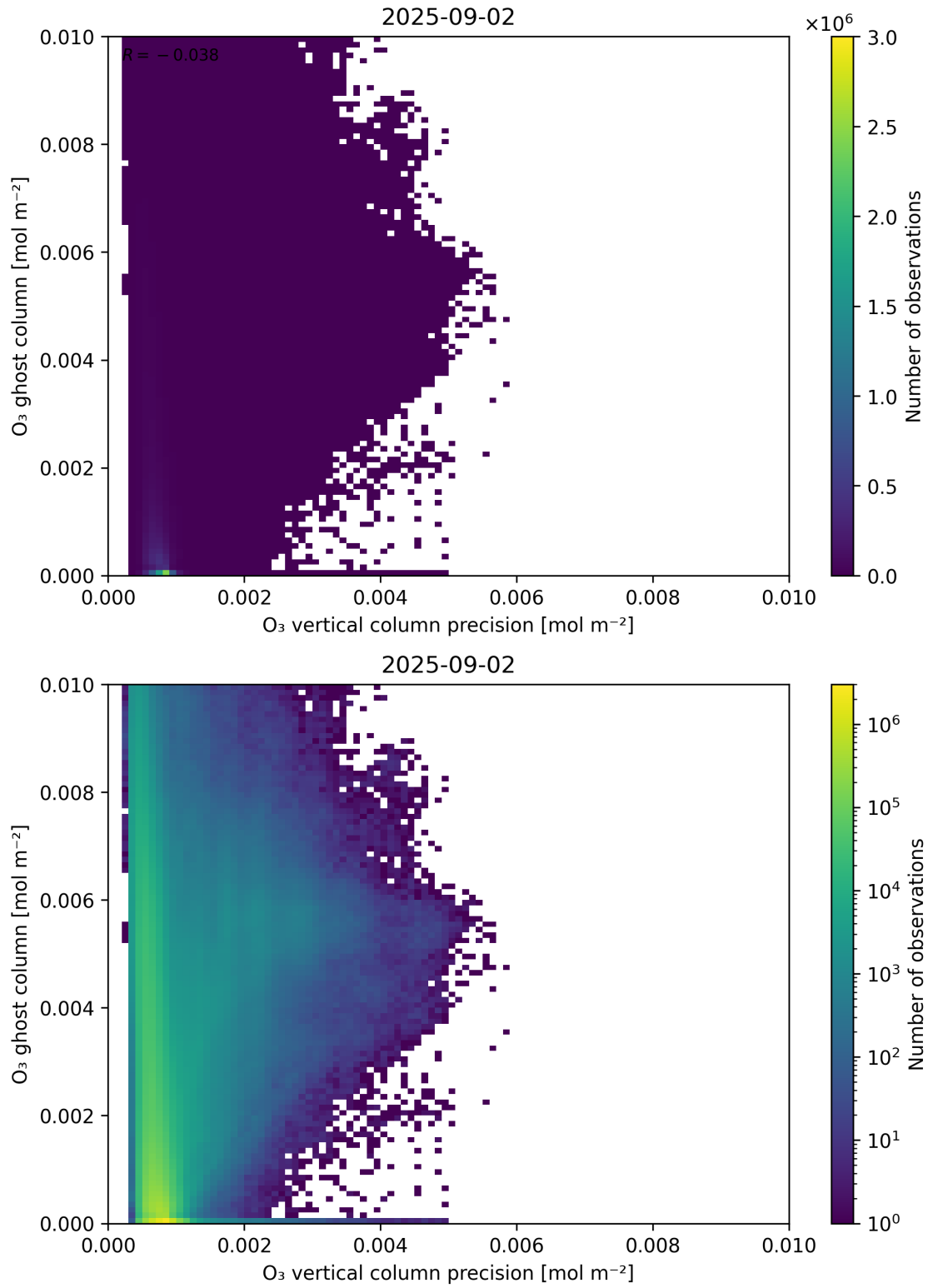
Figure 43: Scatter density plot of “O 3 vertical column precision” against “O 3 ghost column” for 2025-09-01 to 2025-09-03.
