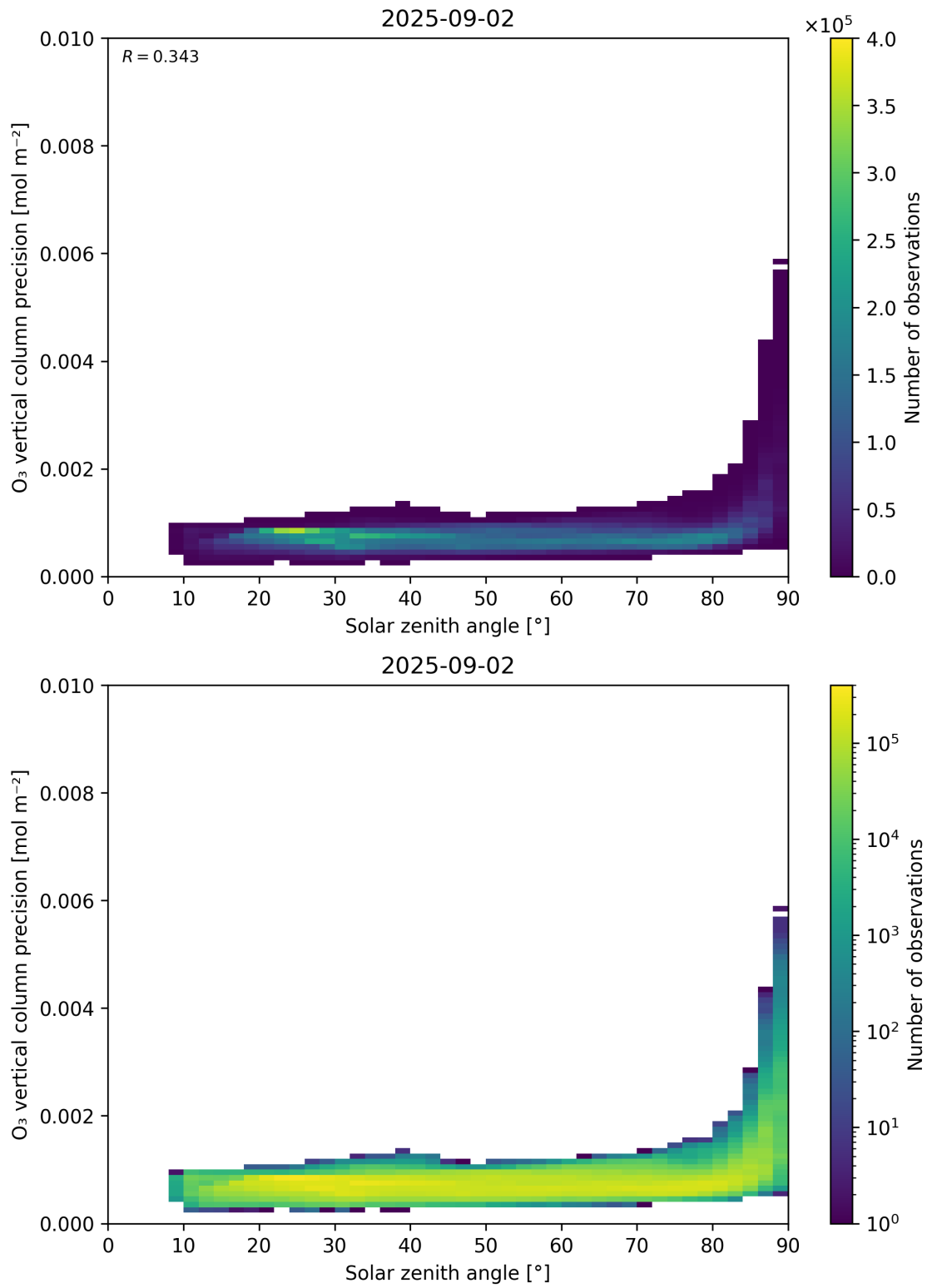
Figure 48: Scatter density plot of “Solar zenith angle” against “O 3 vertical column precision” for 2025-09-01 to 2025-09-03.
