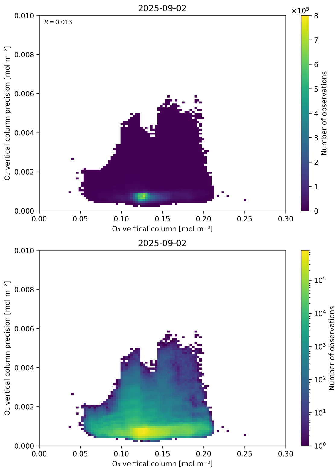
Figure 41: Scatter density plot of “O 3 vertical column” against “O 3 vertical column precision” for 2025-09-01 to 2025-09-03.
