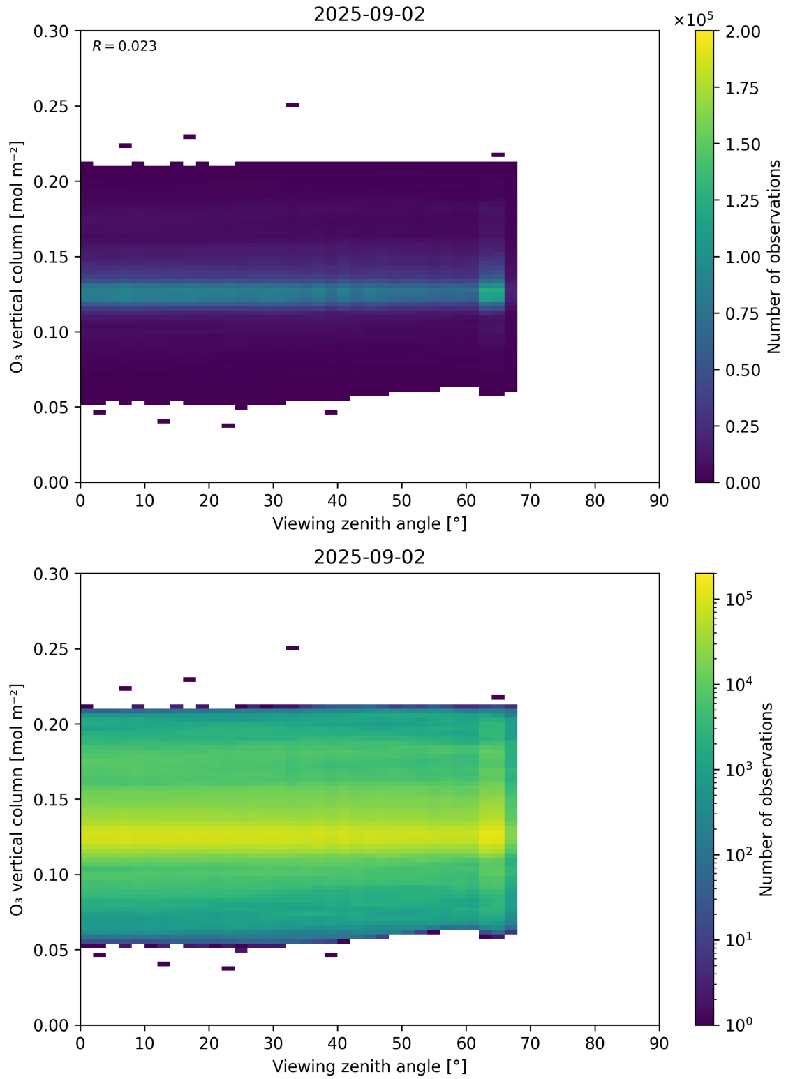
Figure 52: Scatter density plot of “Viewing zenith angle” against “O 3 vertical column” for 2025-09-01 to 2025-09-03.
