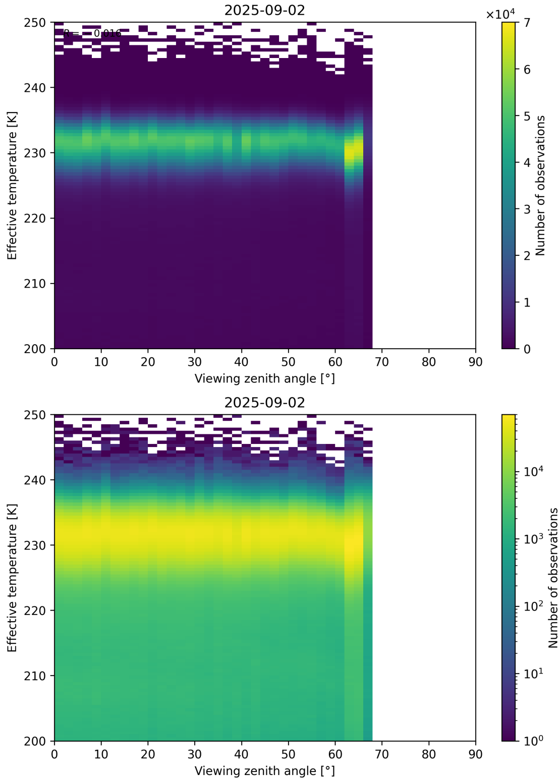
Figure 50: Scatter density plot of “Viewing zenith angle” against “Effective temperature” for 2025-09-01 to 2025-09-03.
