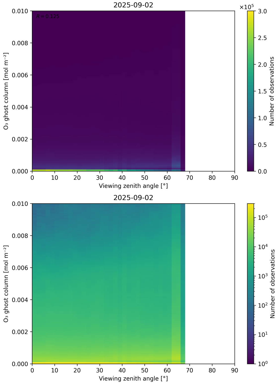
Figure 51: Scatter density plot of “Viewing zenith angle” against “O 3 ghost column” for 2025-09-01 to 2025-09-03.
