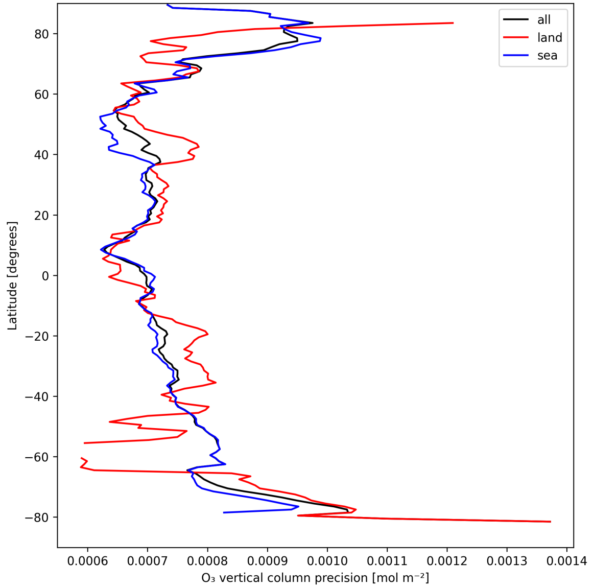
Figure 15: Zonal average of “O 3 vertical column precision” for 2025-09-01 to 2025-09-03.
