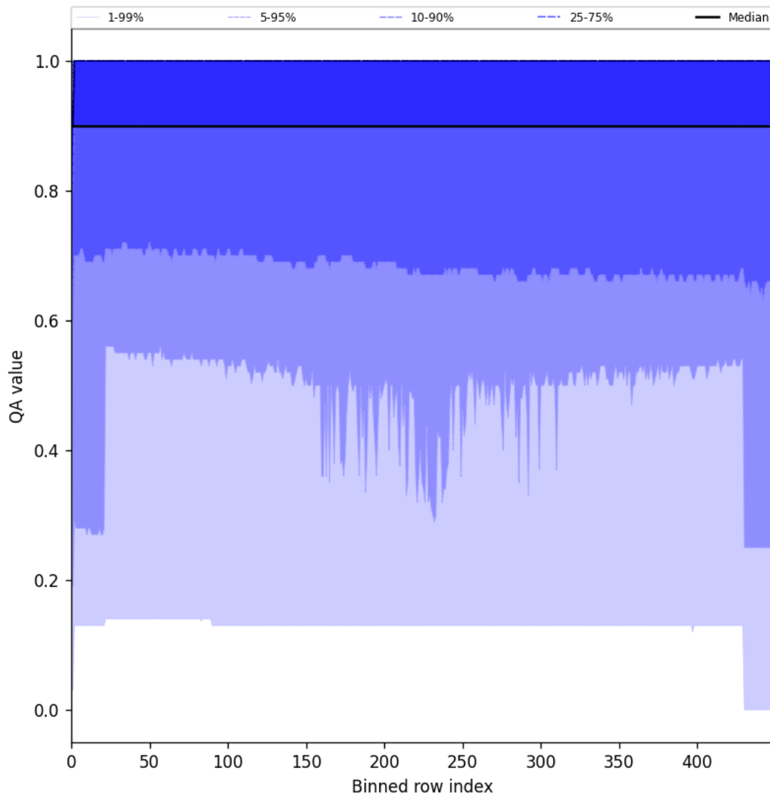
Figure 27: Along track statistics of “QA value” for 2025-09-01 to 2025-09-03
