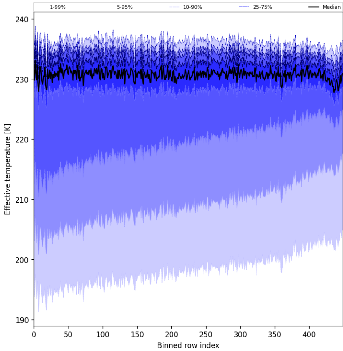
Figure 31: Along track statistics of “Effective temperature” for 2025-09-01 to 2025-09-03
