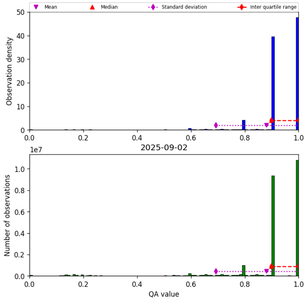
Figure 20: Histogram of “QA value” for 2025-09-01 to 2025-09-03
