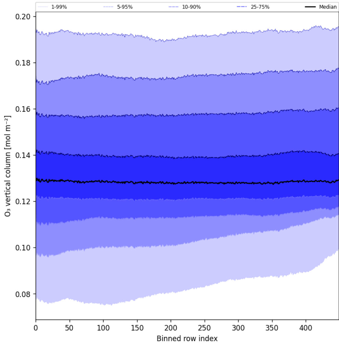
Figure 28: Along track statistics of “O 3 vertical column” for 2025-09-01 to 2025-09-03
