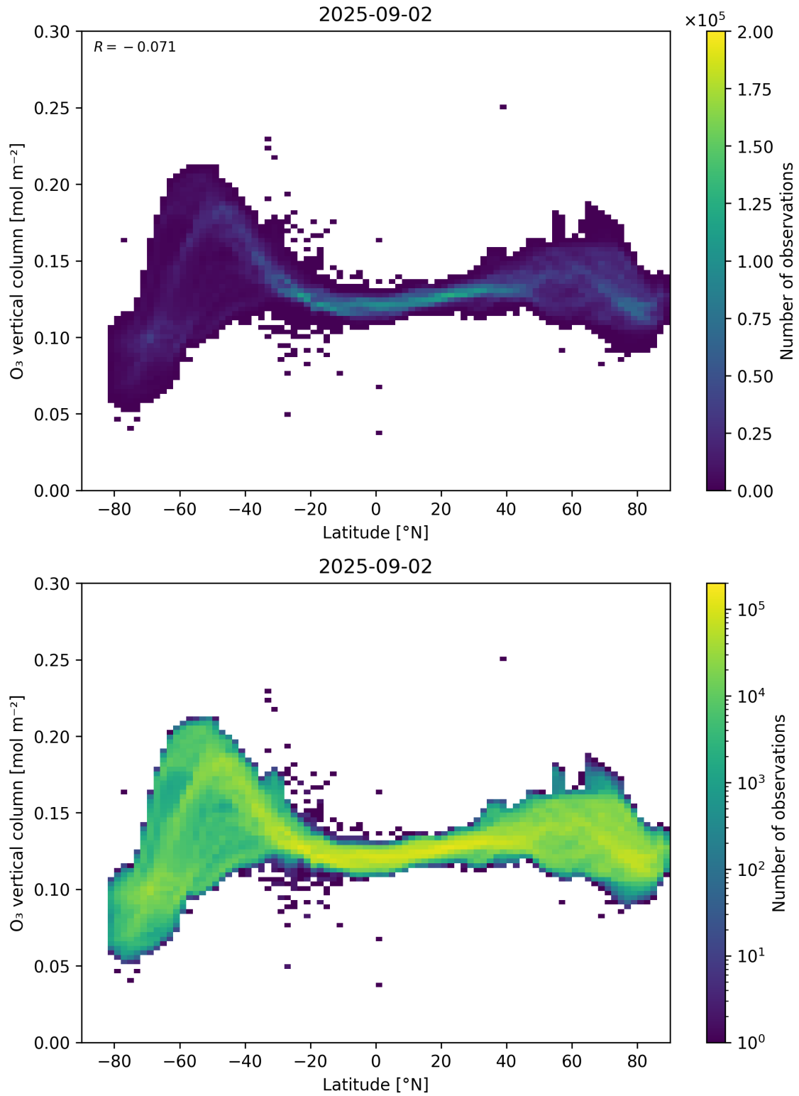
Figure 36: Scatter density plot of “Latitude” against “O 3 vertical column” for 2025-09-01 to 2025-09-03.
