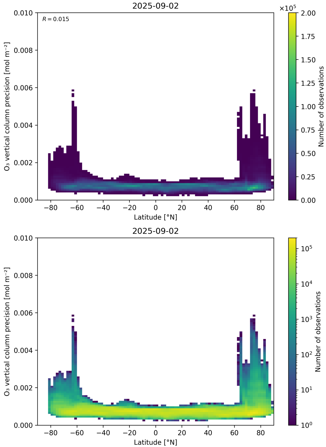
Figure 37: Scatter density plot of “Latitude” against “O 3 vertical column precision” for 2025-09-01 to 2025-09-03.
