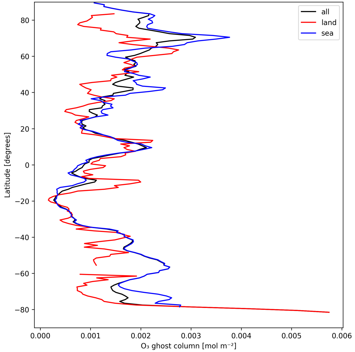
Figure 18: Zonal average of "O 3 ghost column" for 2025-09-01 to 2025-09-03.
