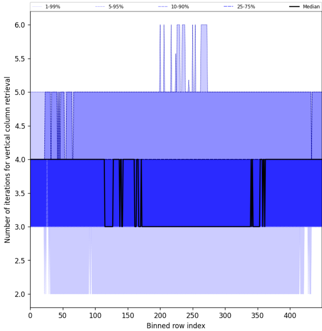
Figure 33: Along track statistics of “Number of iterations for vertical column retrieval” for 2025-09-01 to 2025-09-03
