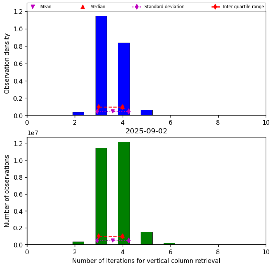
Figure 26: Histogram of “Number of iterations for vertical column retrieval” for 2025-09-01 to 2025-09-03
