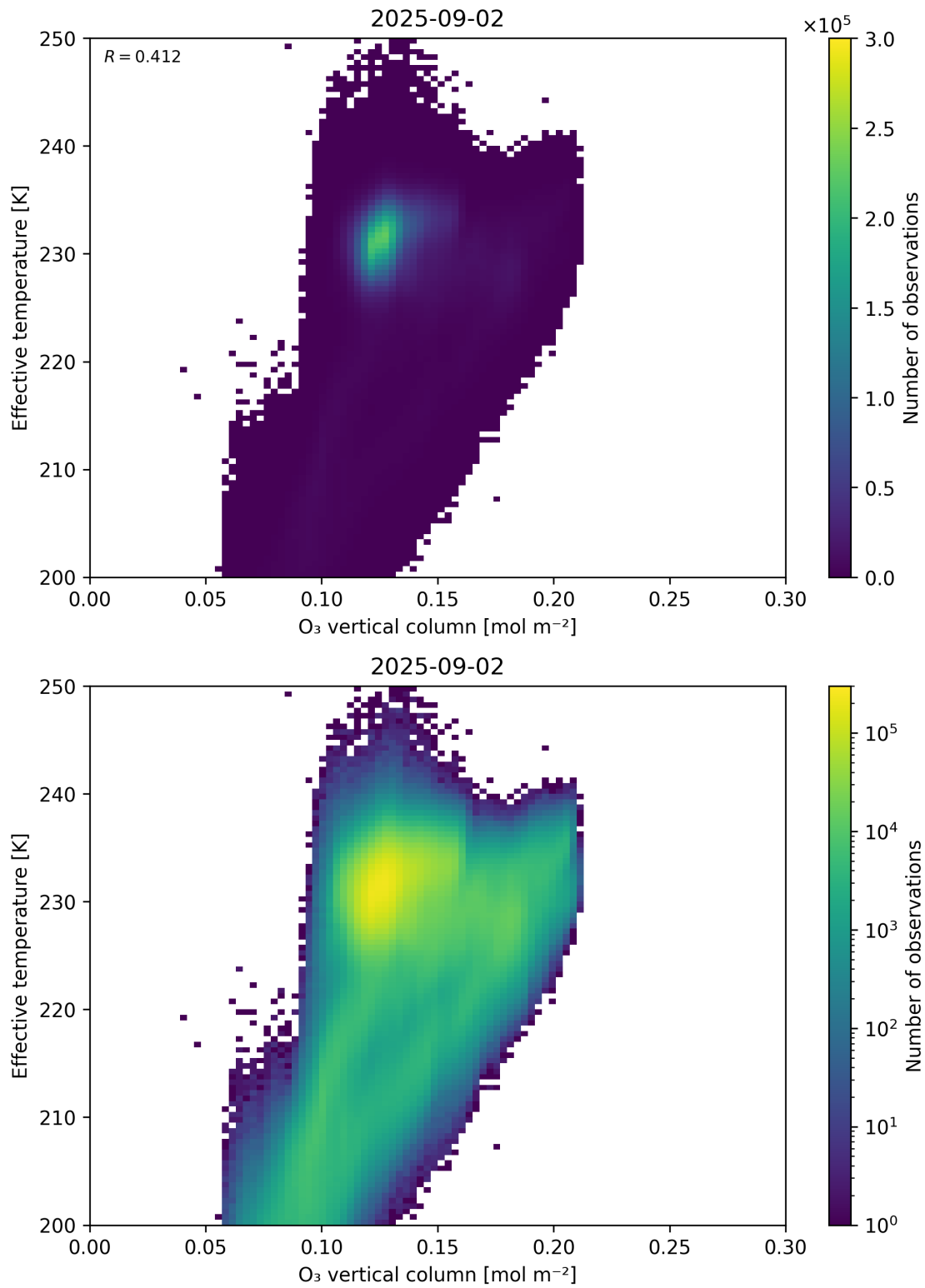
Figure 39: Scatter density plot of “O 3 vertical column” against “Effective temperature” for 2025-09-01 to 2025-09-03.
