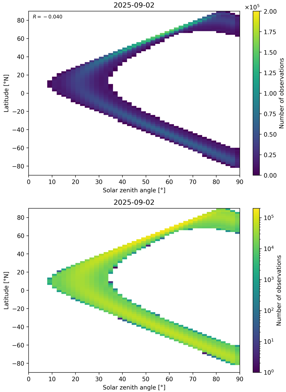
Figure 44: Scatter density plot of “Solar zenith angle” against “Latitude” for 2025-09-01 to 2025-09-03.
