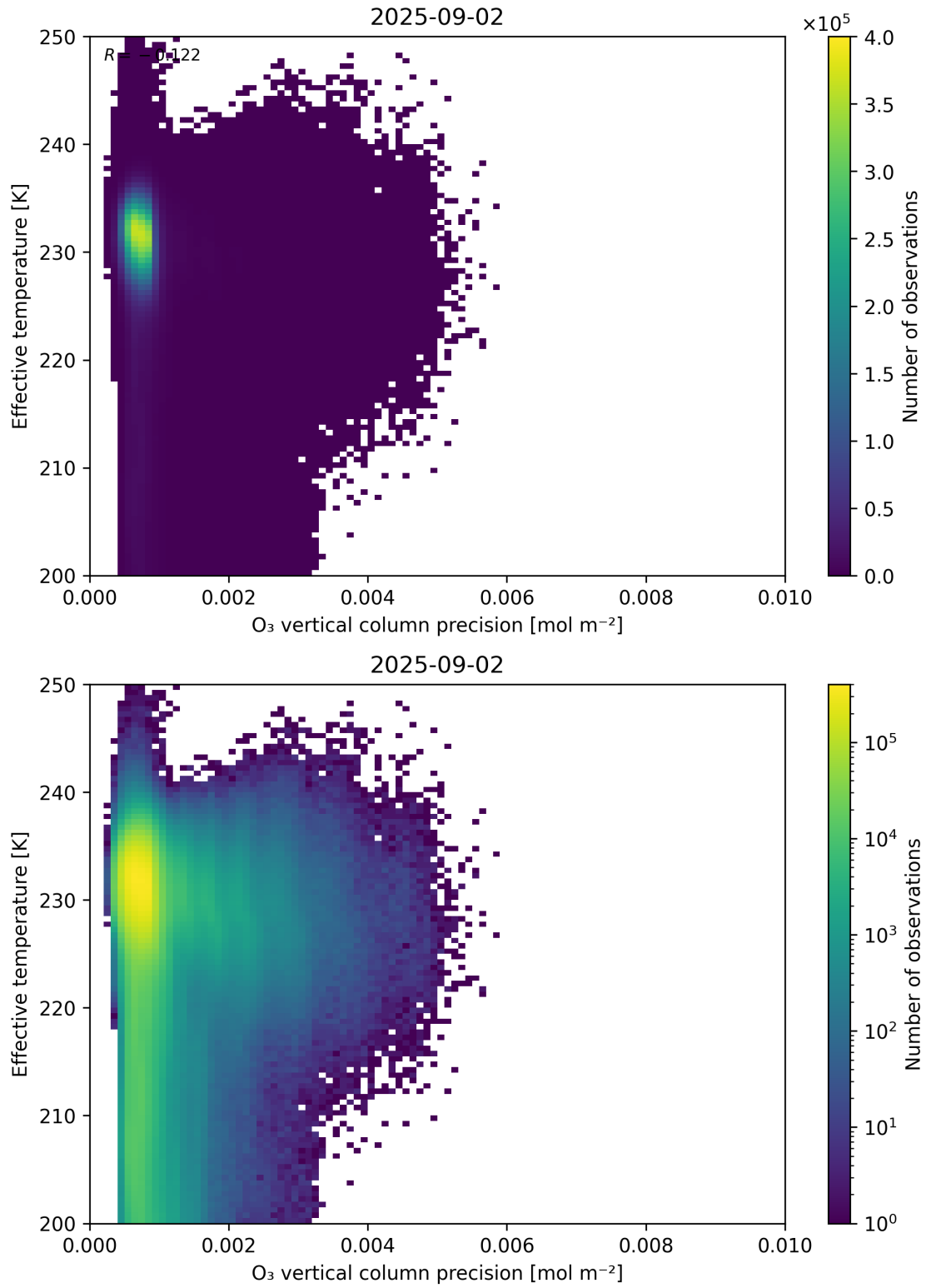
Figure 42: Scatter density plot of “O 3 vertical column precision” against “Effective temperature” for 2025-09-01 to 2025-09-03.
