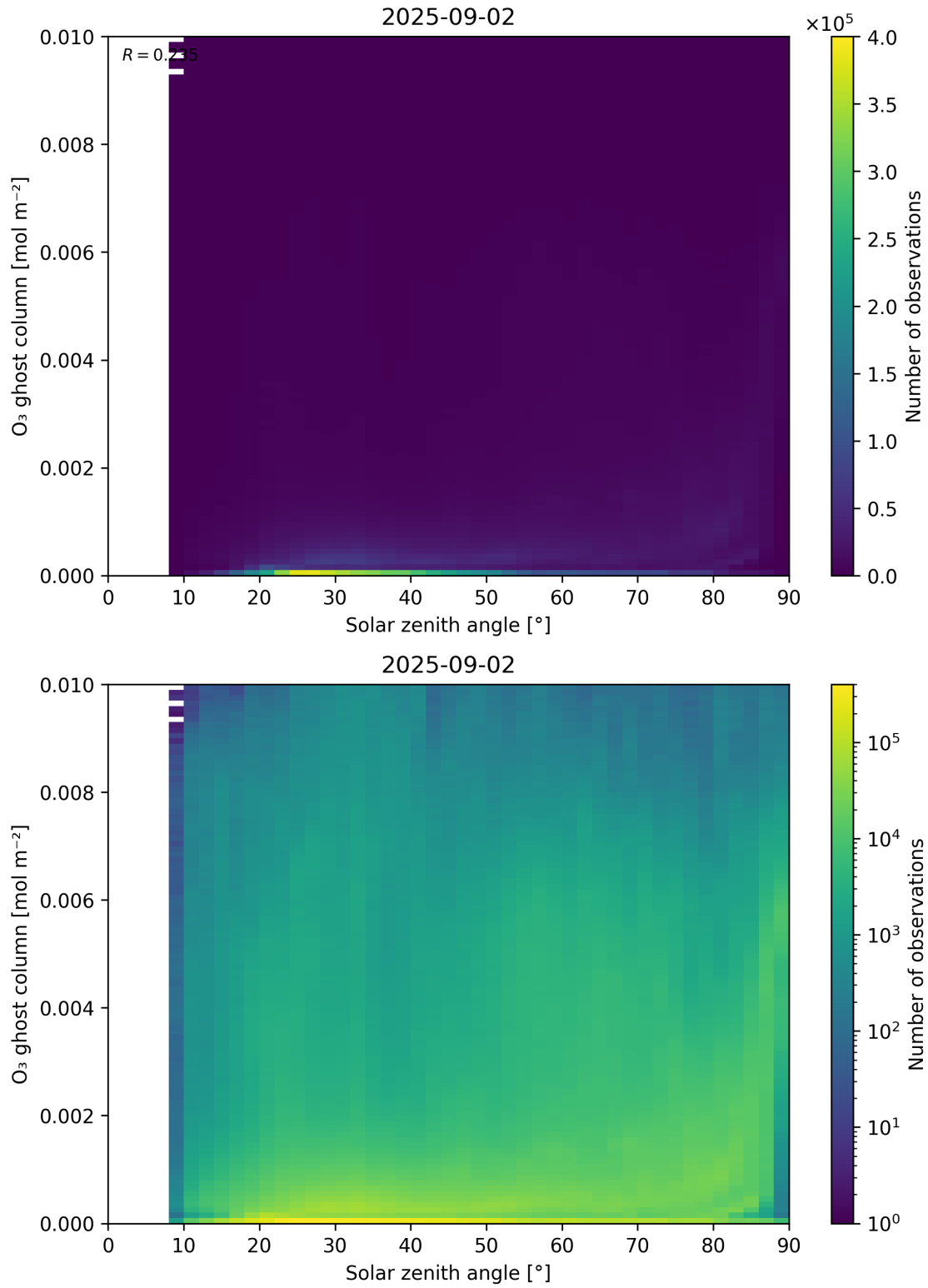
Figure 46: Scatter density plot of “Solar zenith angle” against “O 3 ghost column” for 2025-09-01 to 2025-09-03.
