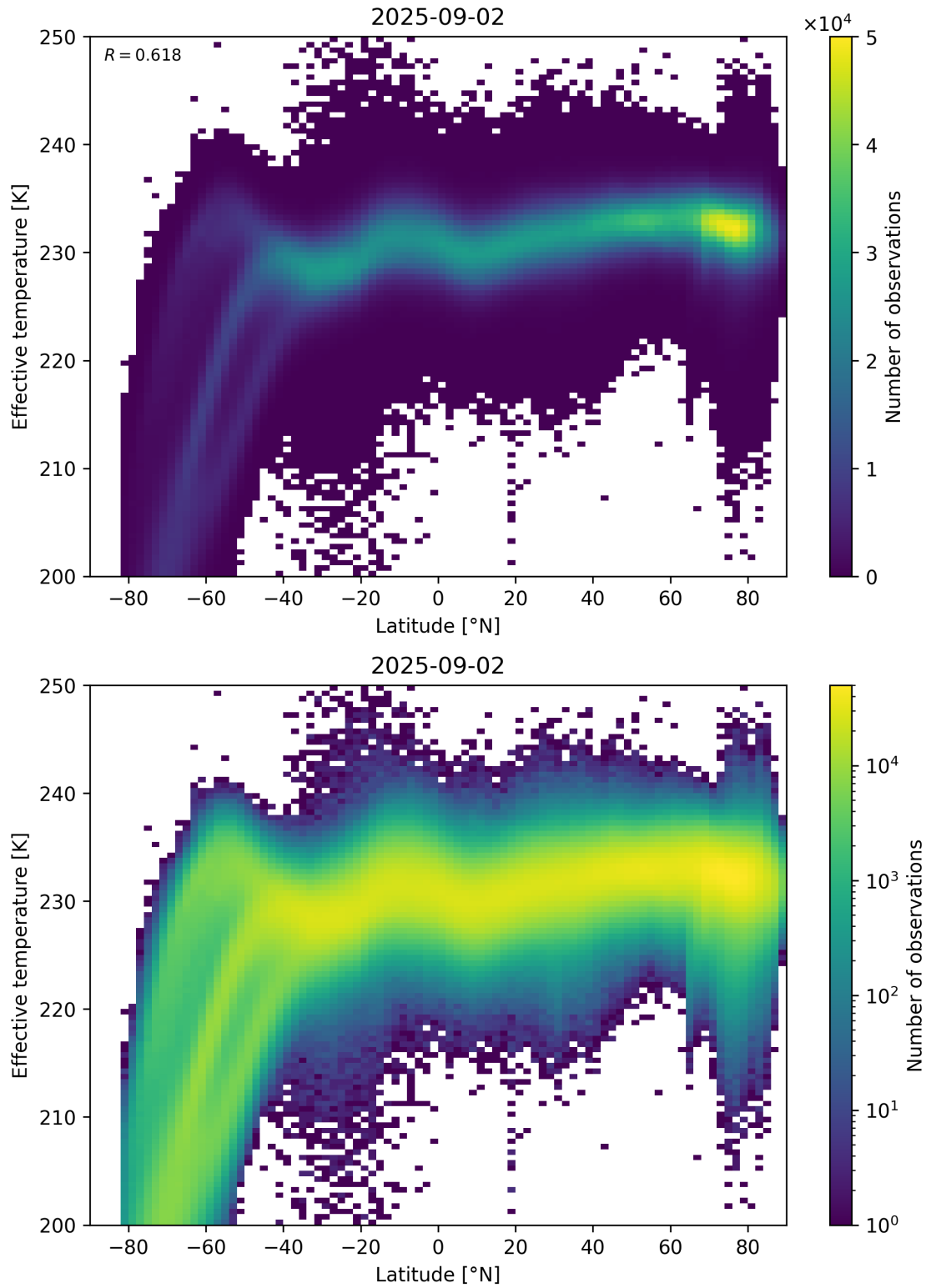
Figure 34: Scatter density plot of “Latitude” against “Effective temperature” for 2025-09-01 to 2025-09-03.
