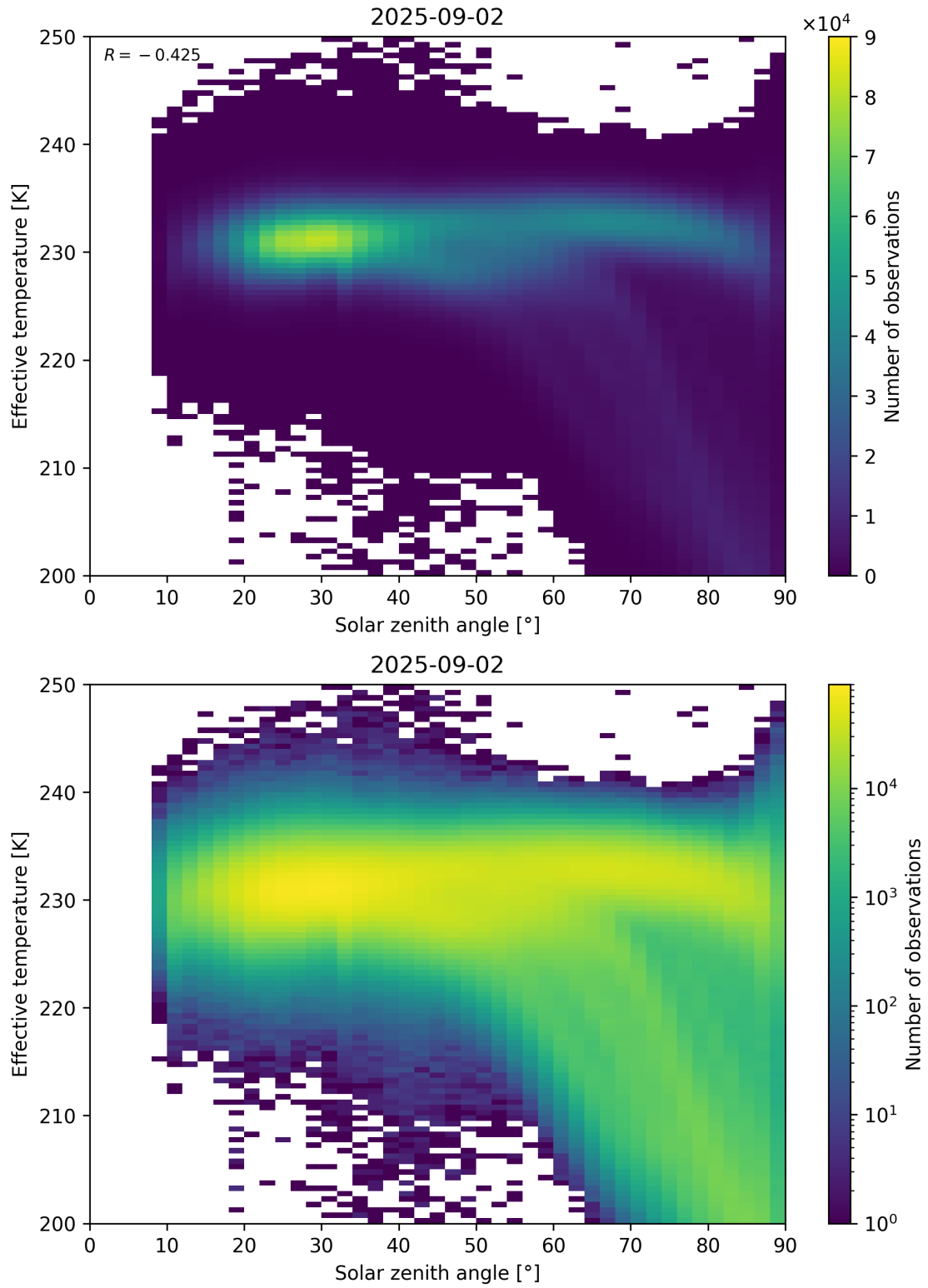
Figure 45: Scatter density plot of “Solar zenith angle” against “Effective temperature” for 2025-09-01 to 2025-09-03.
