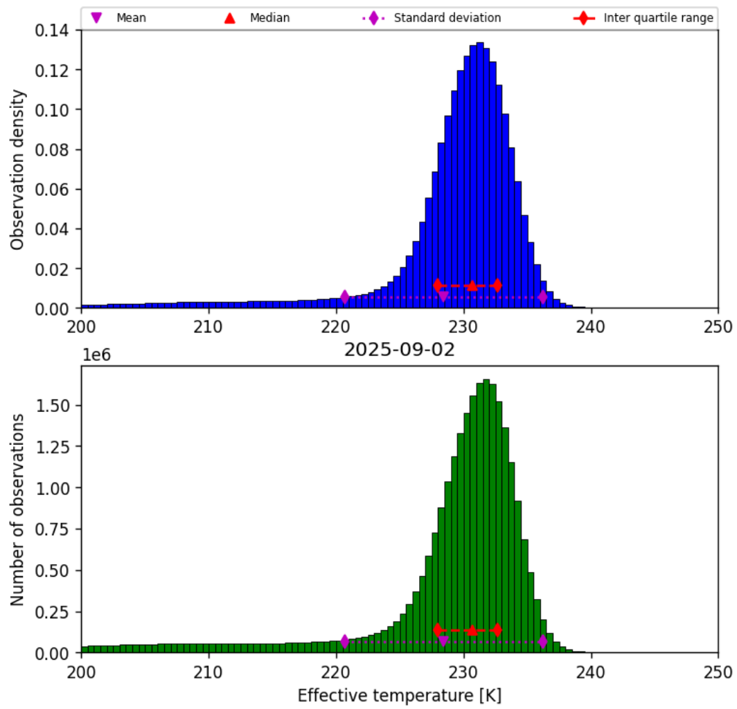
Figure 24: Histogram of “Effective temperature” for 2025-09-01 to 2025-09-03
