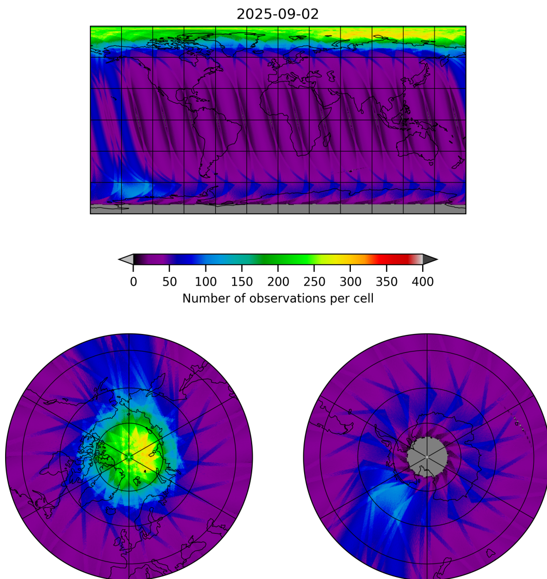
Figure 12: Map of the number of observations for 2025-09-01 to 2025-09-03
