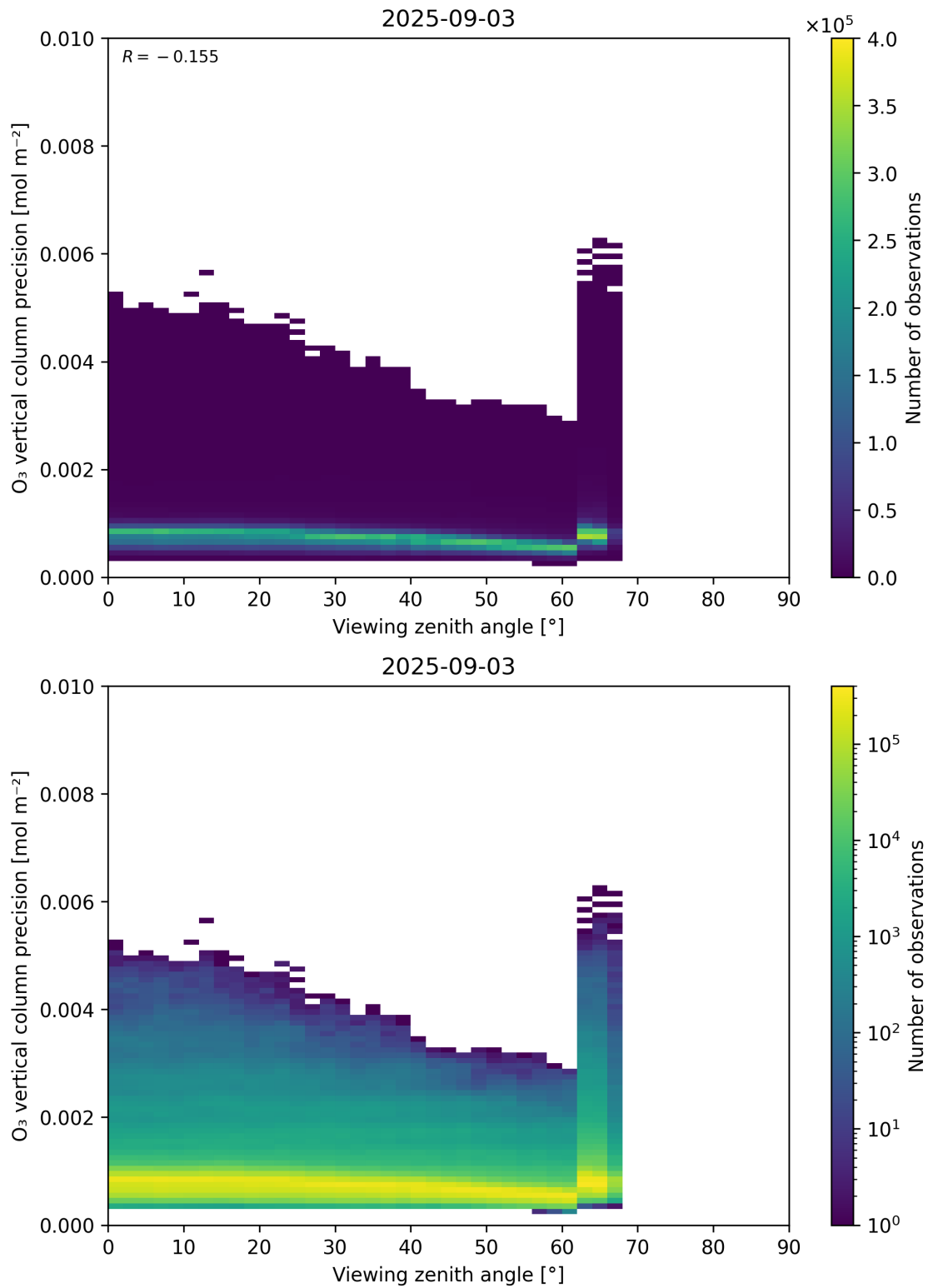
Figure 53: Scatter density plot of “Viewing zenith angle” against “O 3 vertical column precision” for 2025-09-02 to 2025-09-04.
