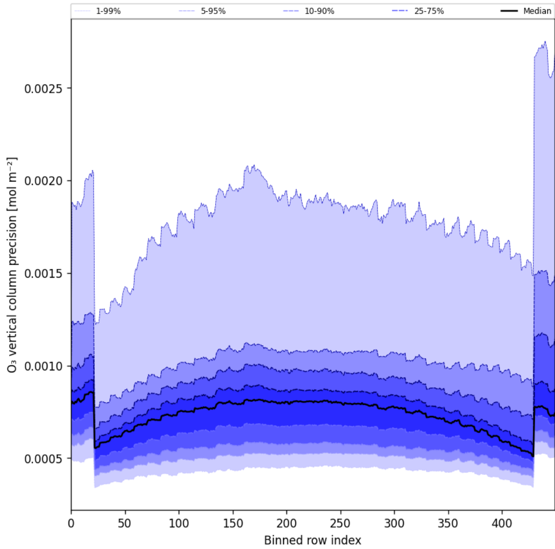
Figure 29: Along track statistics of “O 3 vertical column precision” for 2025-09-02 to 2025-09-04
