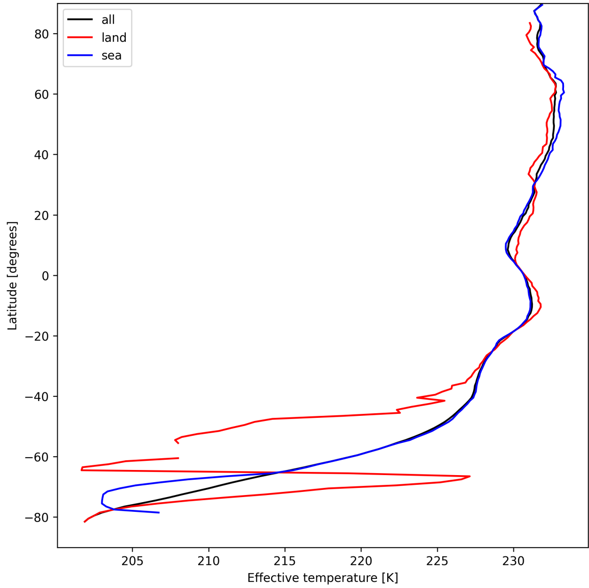
Figure 17: Zonal average of "Effective temperature" for 2025-09-02 to 2025-09-04.
