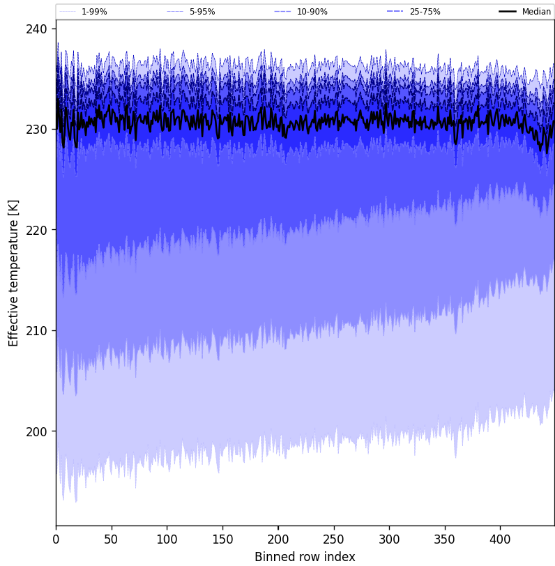
Figure 31: Along track statistics of “Effective temperature” for 2025-09-02 to 2025-09-04
