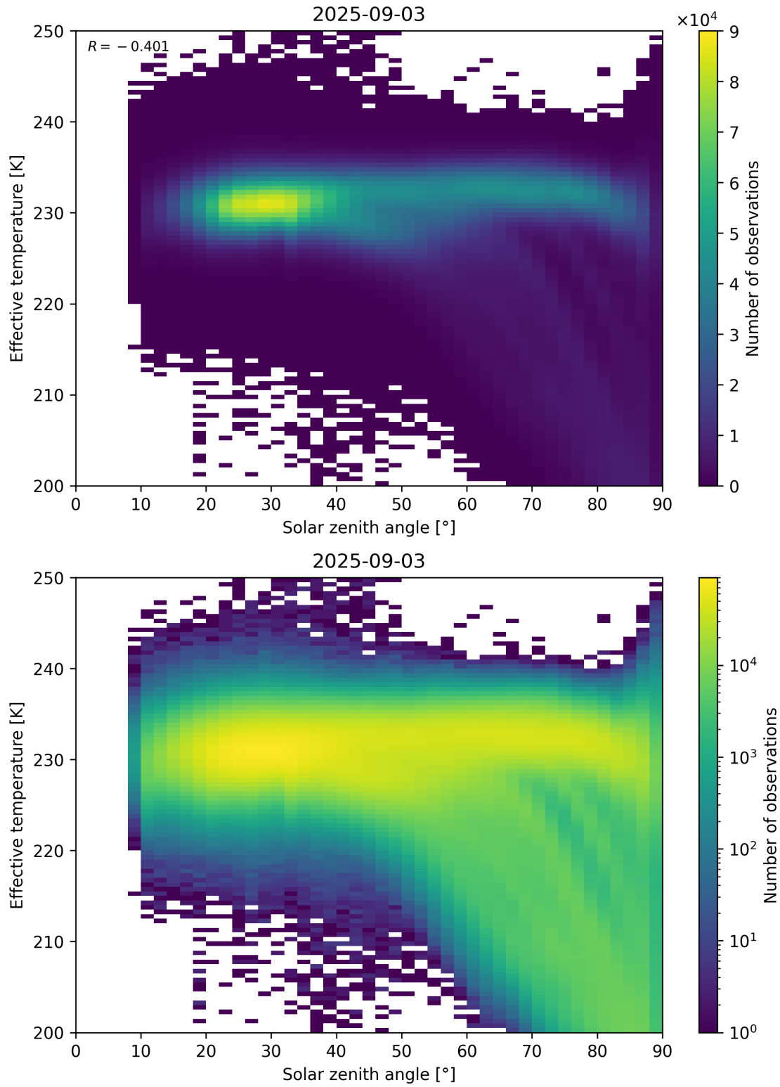
Figure 45: Scatter density plot of “Solar zenith angle” against “Effective temperature” for 2025-09-02 to 2025-09-04.
