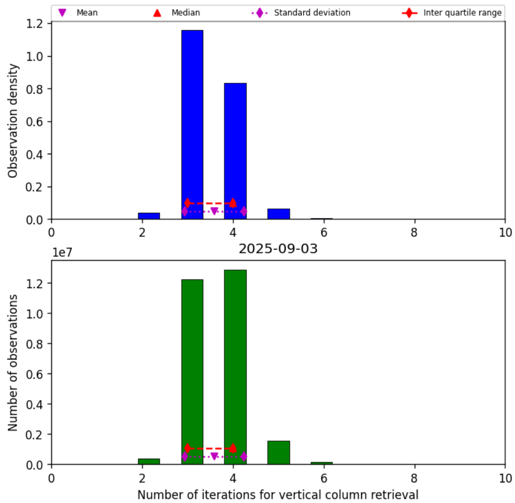
Figure 26: Histogram of “Number of iterations for vertical column retrieval” for 2025-09-02 to 2025-09-04
