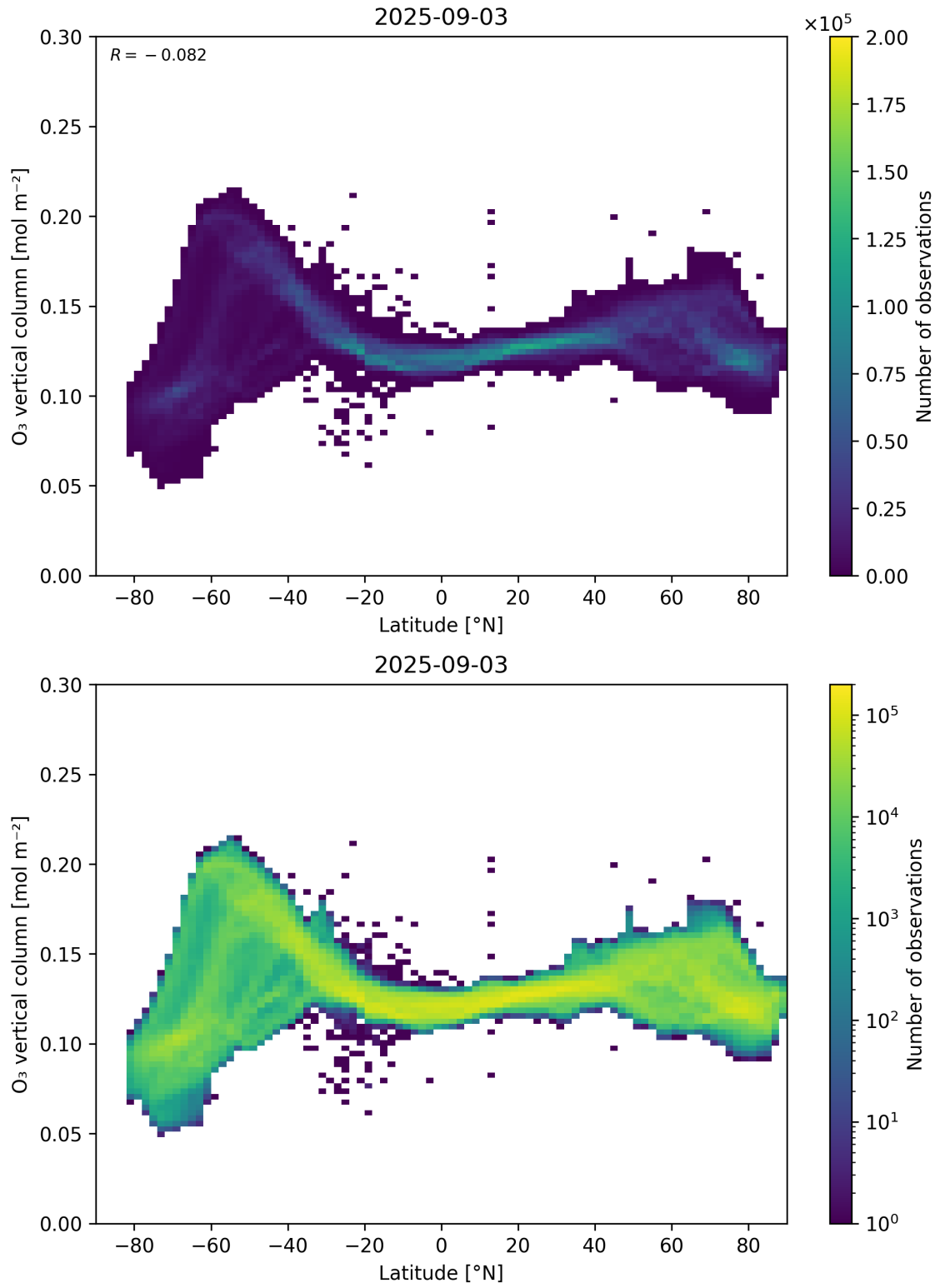
Figure 36: Scatter density plot of “Latitude” against “O 3 vertical column” for 2025-09-02 to 2025-09-04.
