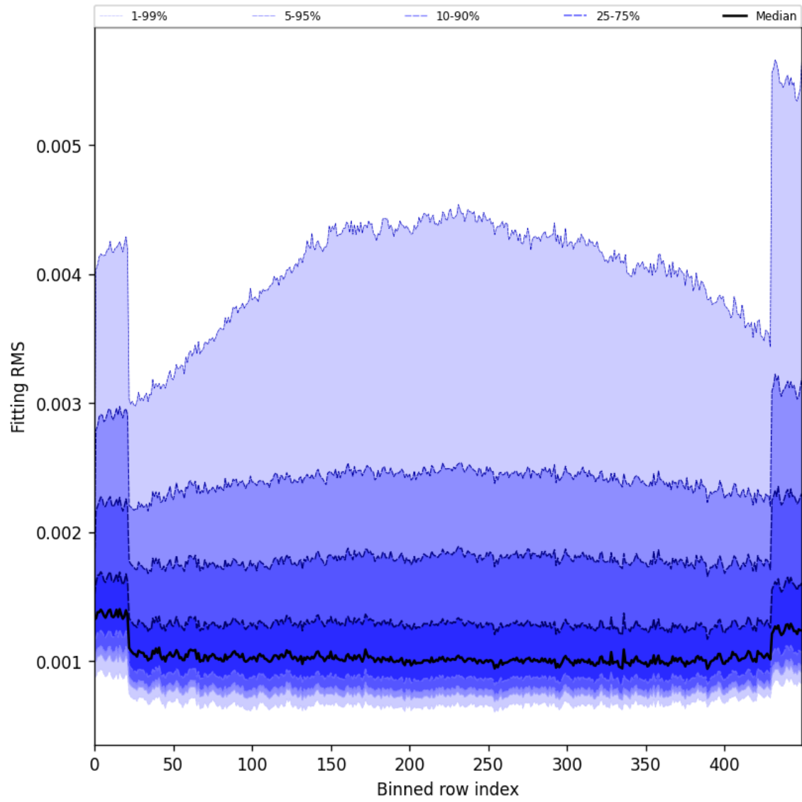
Figure 30: Along track statistics of “Fitting RMS” for 2025-09-02 to 2025-09-04
