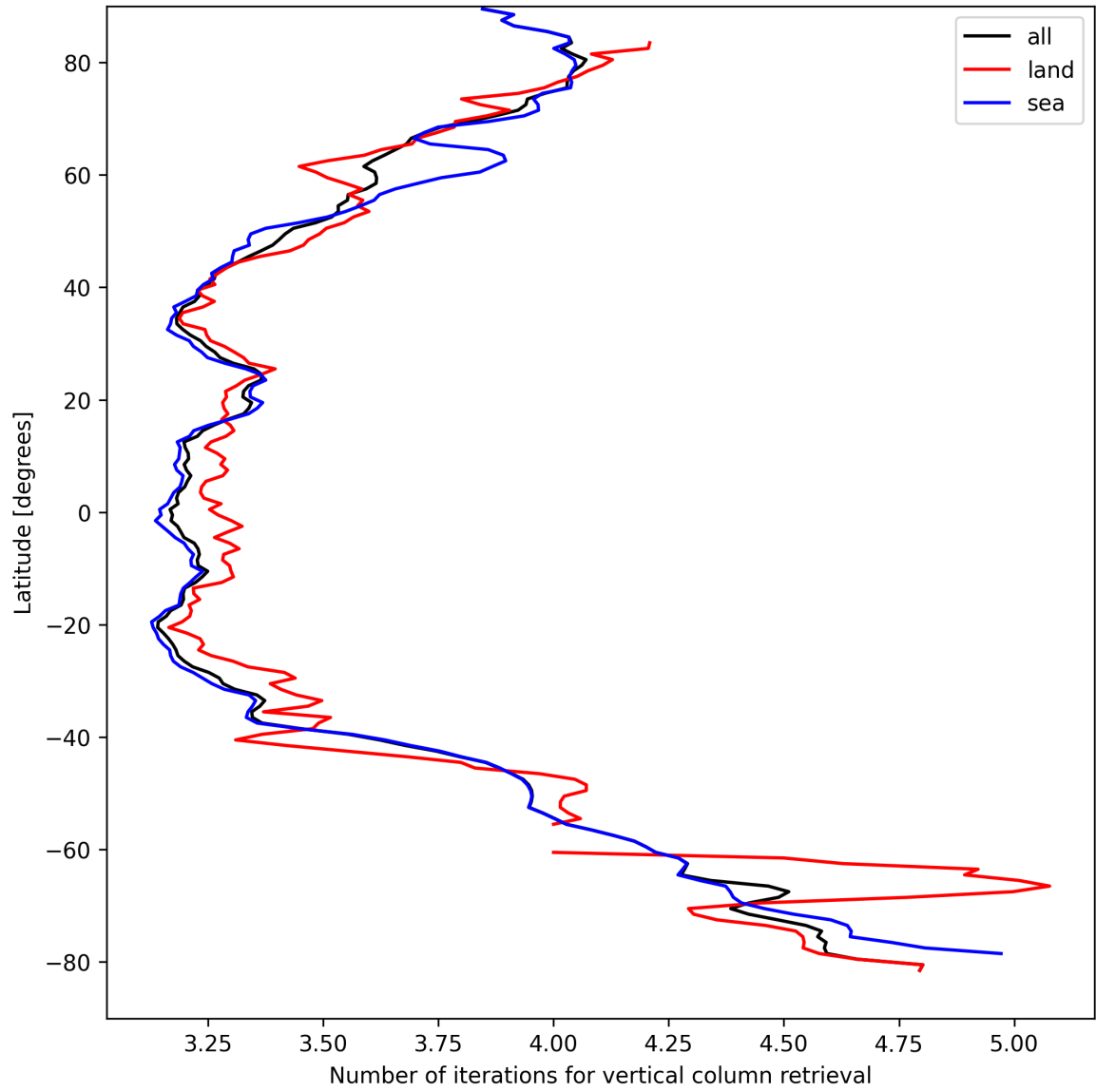
Figure 19: Zonal average of “Number of iterations for vertical column retrieval” for 2025-09-02 to 2025-09-04.
