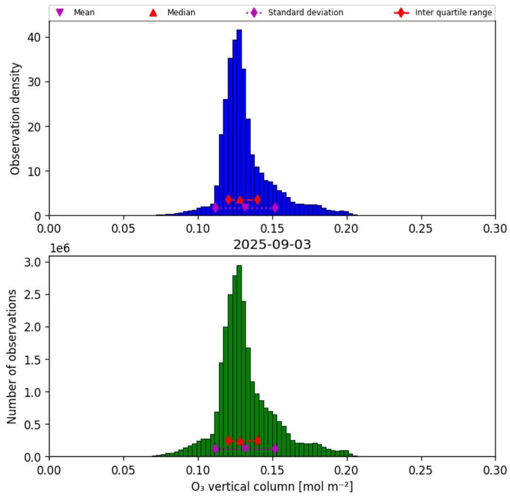
Figure 21: Histogram of “O 3 vertical column” for 2025-09-02 to 2025-09-04
