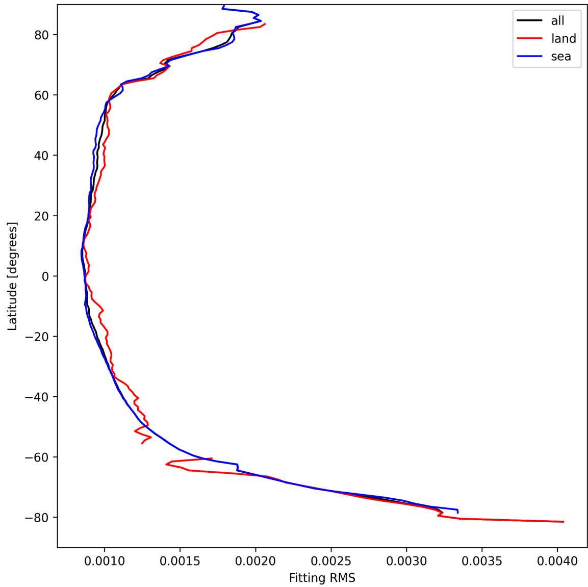
Figure 16: Zonal average of “Fitting RMS” for 2025-09-02 to 2025-09-04.
