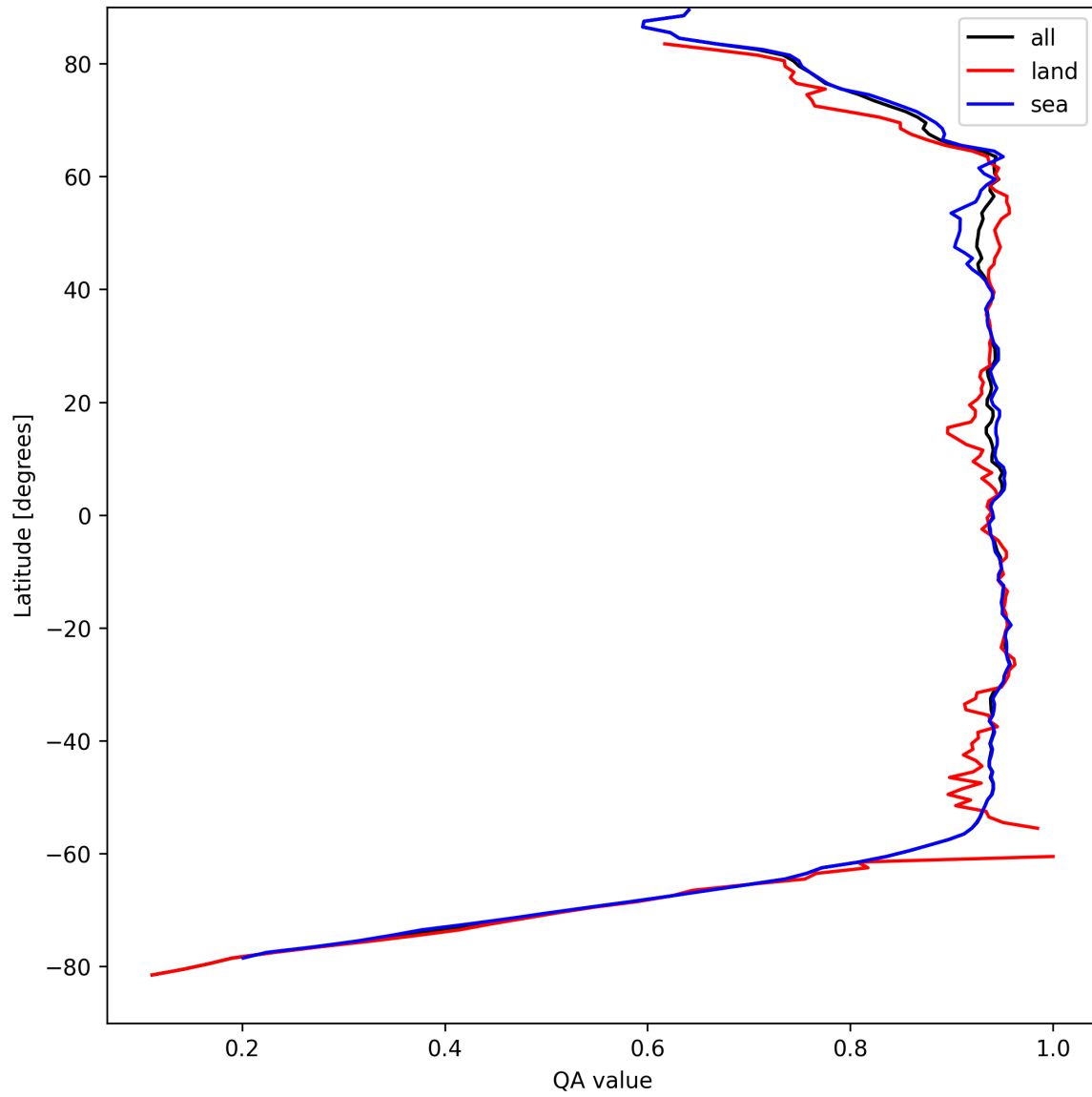
Figure 13: Zonal average of “QA value” for 2025-09-02 to 2025-09-04.
