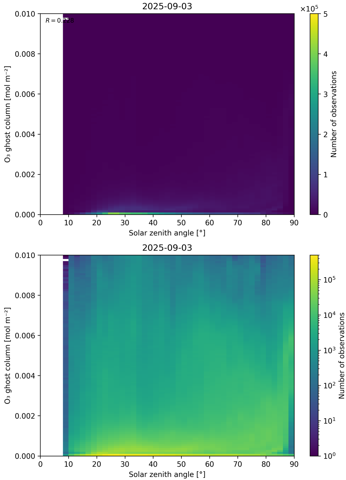
Figure 46: Scatter density plot of “Solar zenith angle” against “O 3 ghost column” for 2025-09-02 to 2025-09-04.
