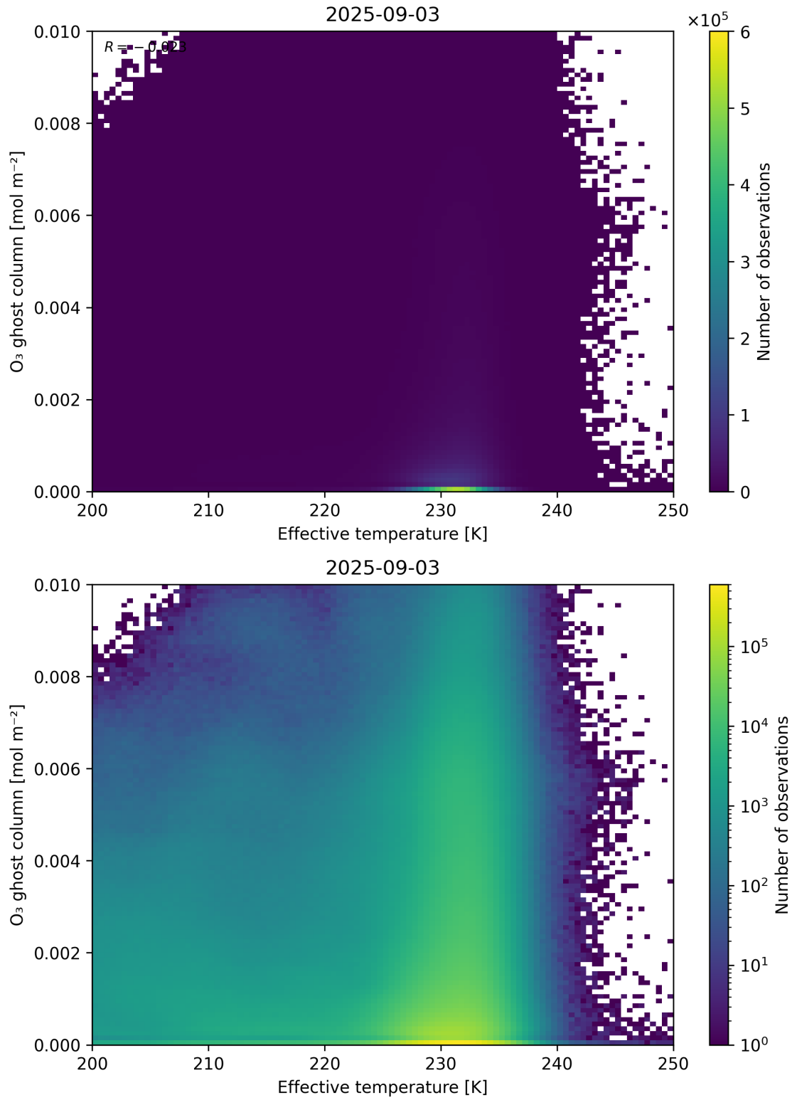
Figure 38: Scatter density plot of “Effective temperature” against “O 3 ghost column” for 2025-09-02 to 2025-09-04.
