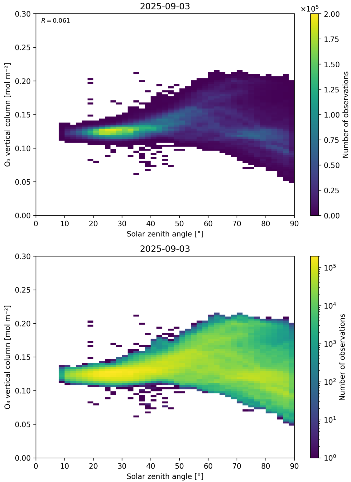
Figure 47: Scatter density plot of “Solar zenith angle” against “O 3 vertical column” for 2025-09-02 to 2025-09-04.
