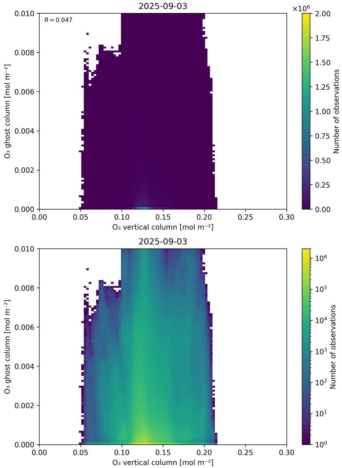
Figure 40: Scatter density plot of “O 3 vertical column” against “O 3 ghost column” for 2025-09-02 to 2025-09-04.
