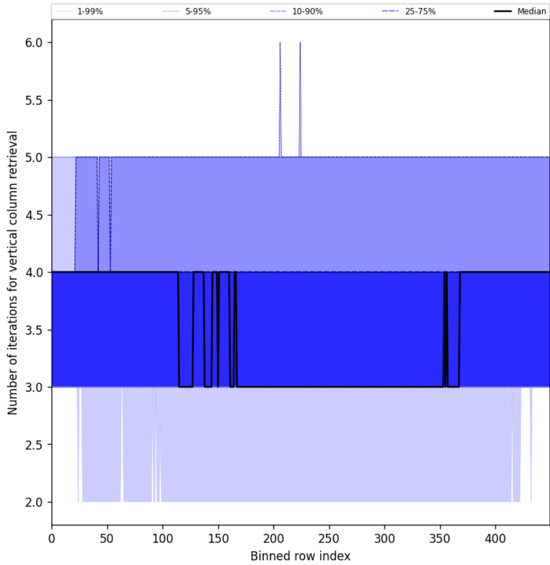
Figure 33: Along track statistics of “Number of iterations for vertical column retrieval” for 2025-09-02 to 2025-09-04
