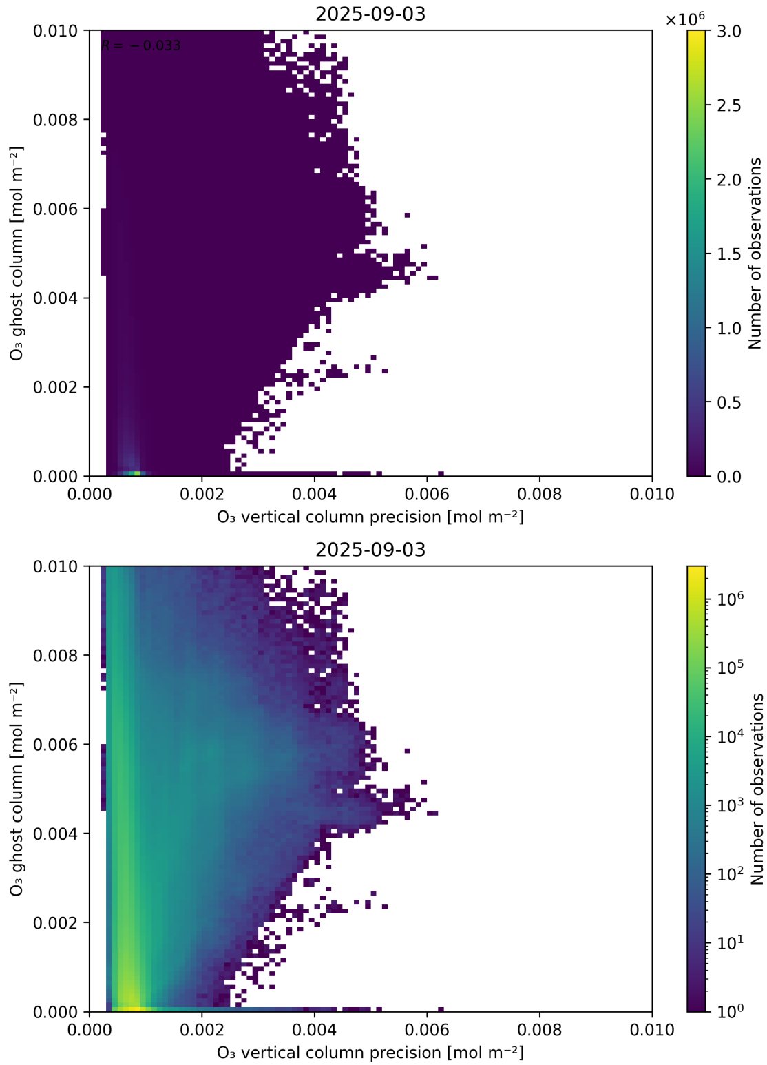
Figure 43: Scatter density plot of “O 3 vertical column precision” against “O 3 ghost column” for 2025-09-02 to 2025-09-04.
