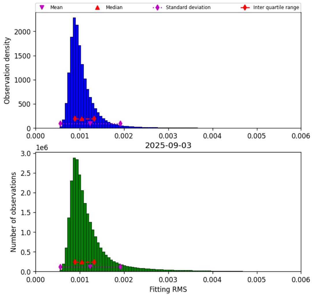
Figure 23: Histogram of “Fitting RMS” for 2025-09-02 to 2025-09-04
