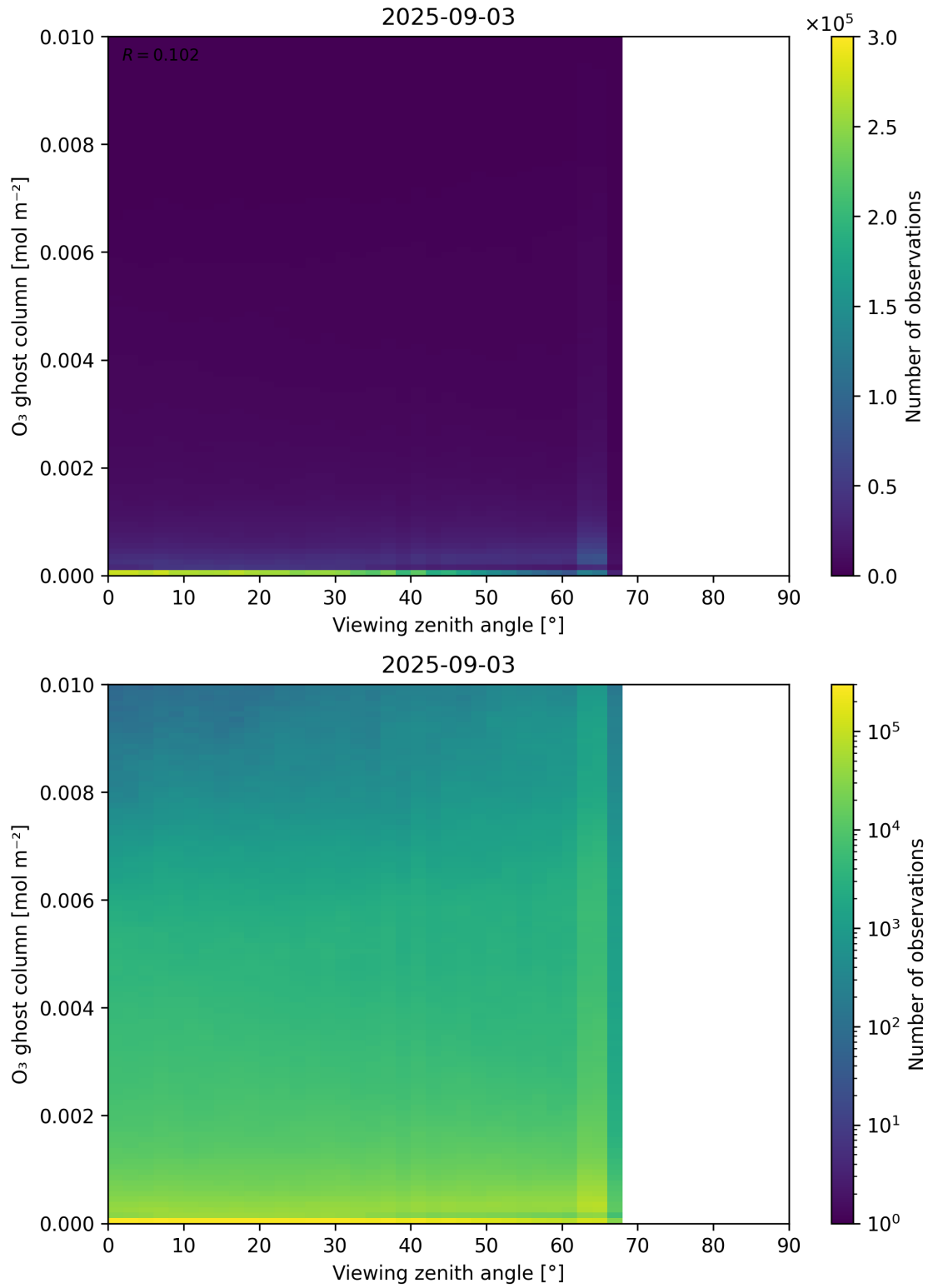
Figure 51: Scatter density plot of “Viewing zenith angle” against “O 3 ghost column” for 2025-09-02 to 2025-09-04.
