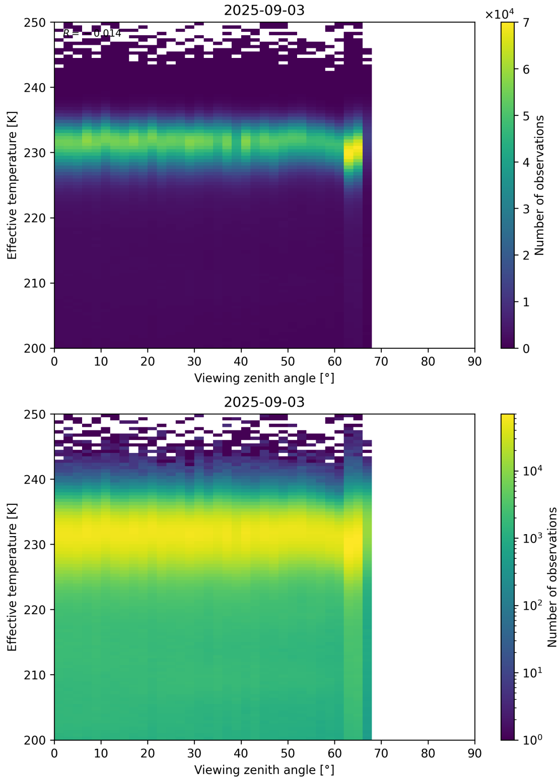
Figure 50: Scatter density plot of “Viewing zenith angle” against “Effective temperature” for 2025-09-02 to 2025-09-04.
