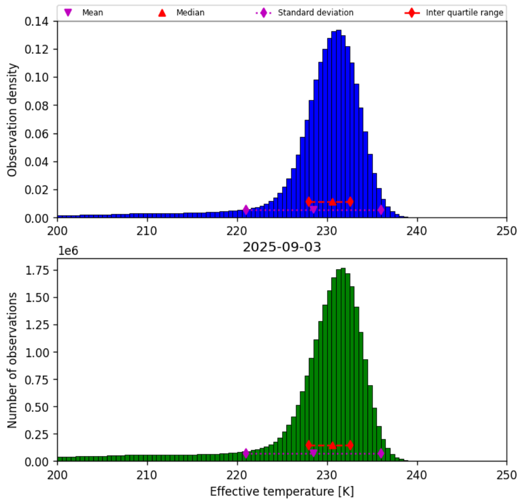
Figure 24: Histogram of “Effective temperature” for 2025-09-02 to 2025-09-04
