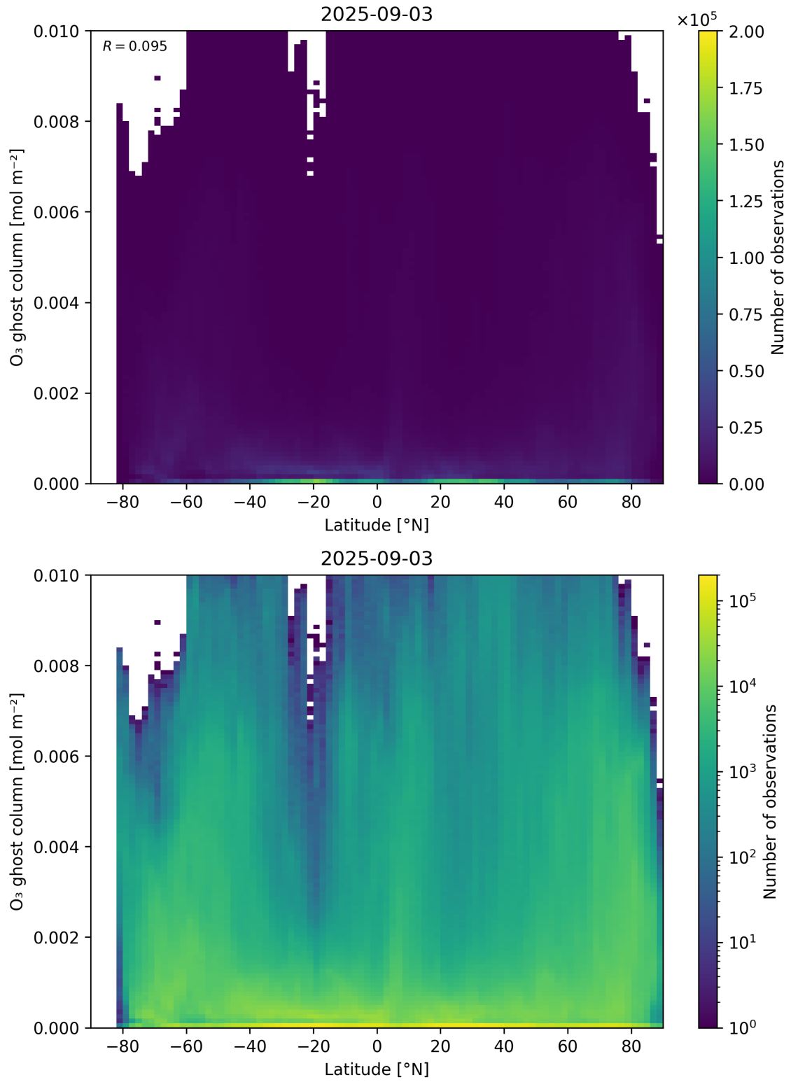
Figure 35: Scatter density plot of “Latitude” against “O 3 ghost column” for 2025-09-02 to 2025-09-04.
