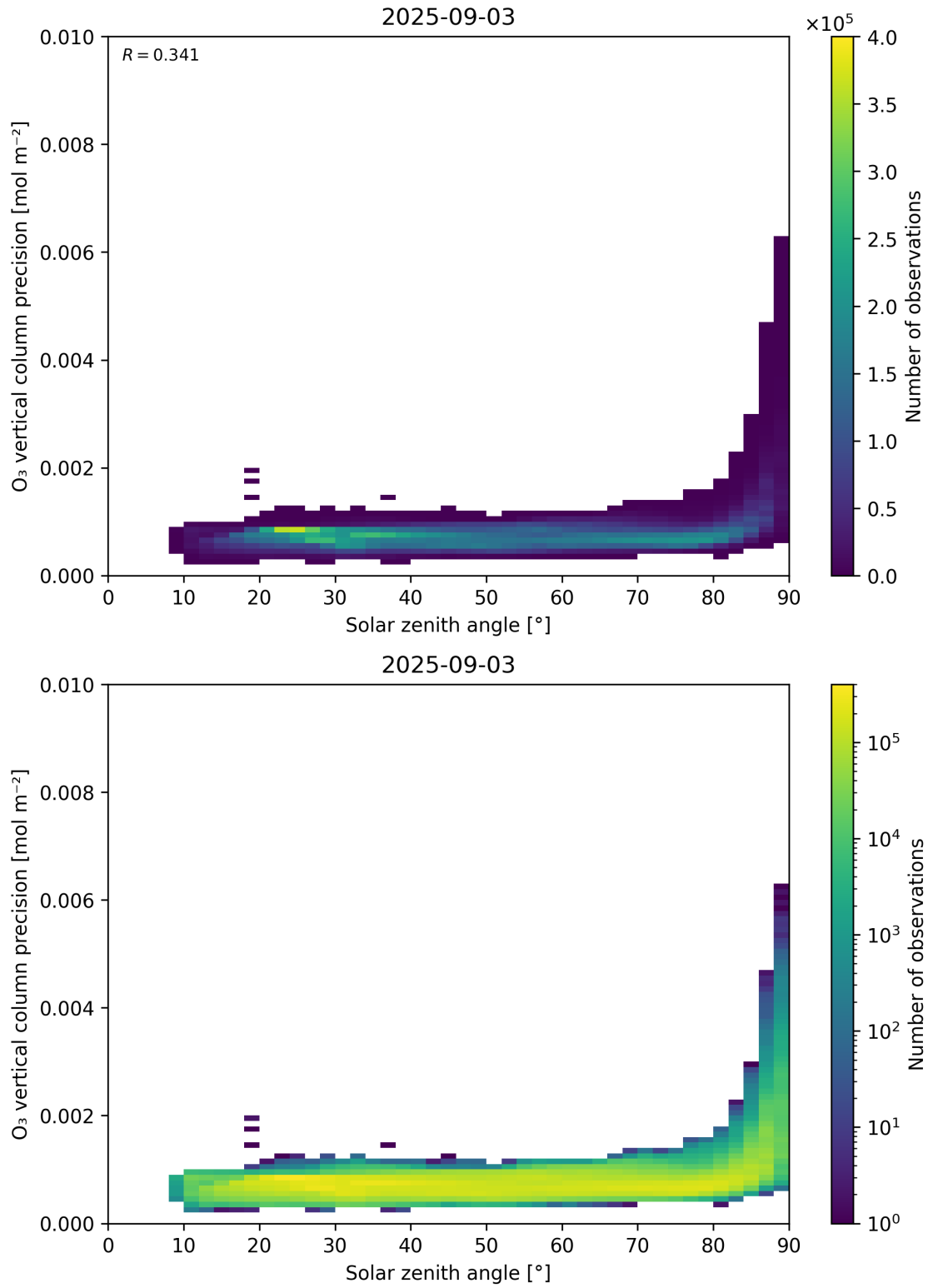
Figure 48: Scatter density plot of “Solar zenith angle” against “O 3 vertical column precision” for 2025-09-02 to 2025-09-04.
