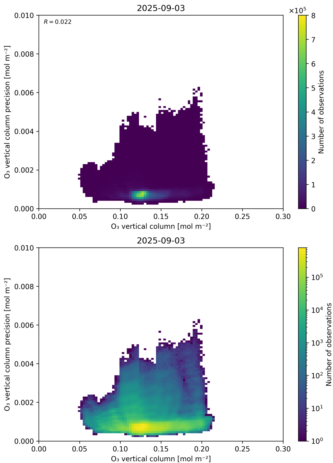
Figure 41: Scatter density plot of “O 3 vertical column” against “O 3 vertical column precision” for 2025-09-02 to 2025-09-04.
