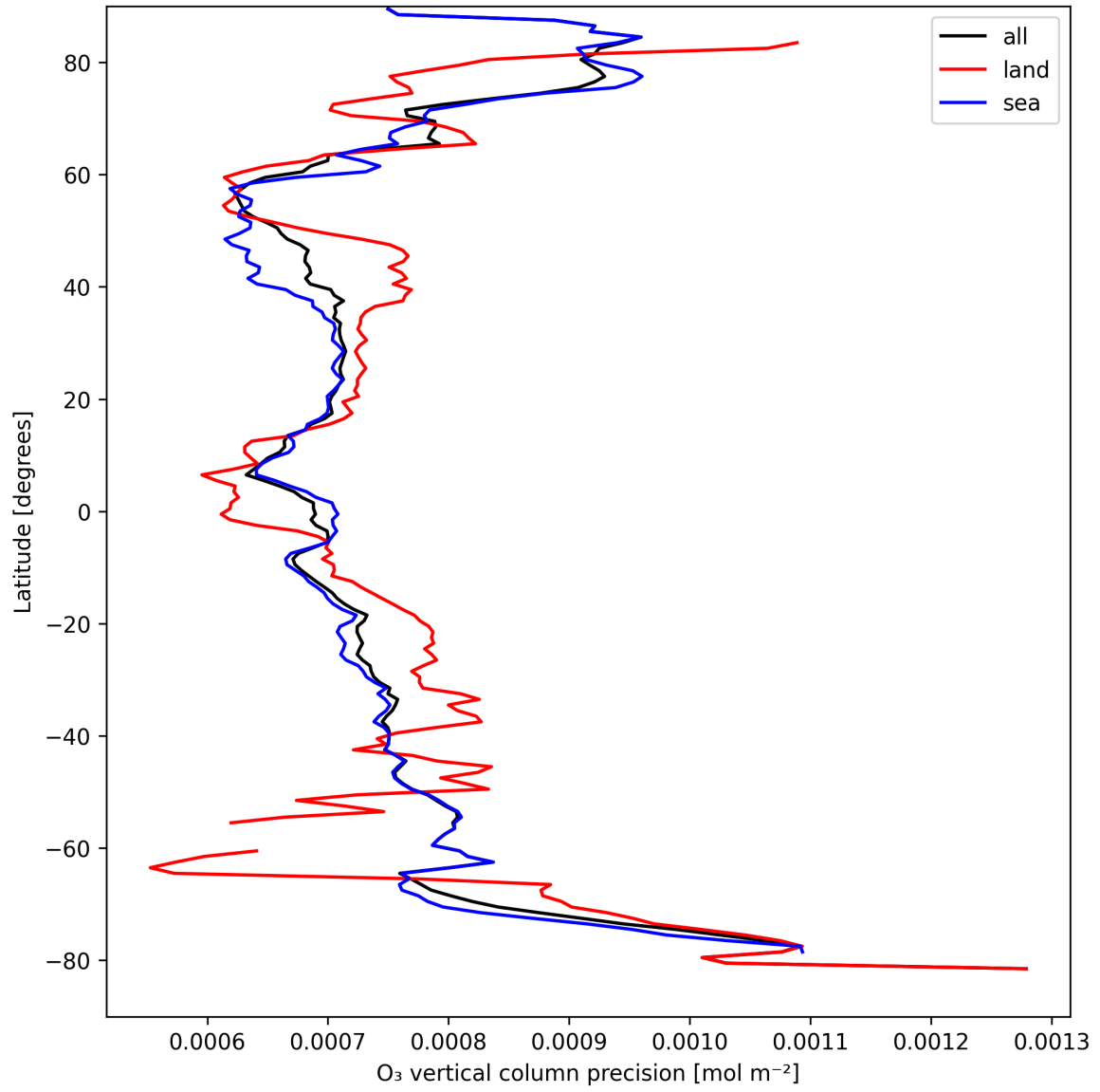
Figure 15: Zonal average of “O 3 vertical column precision” for 2025-09-02 to 2025-09-04.
