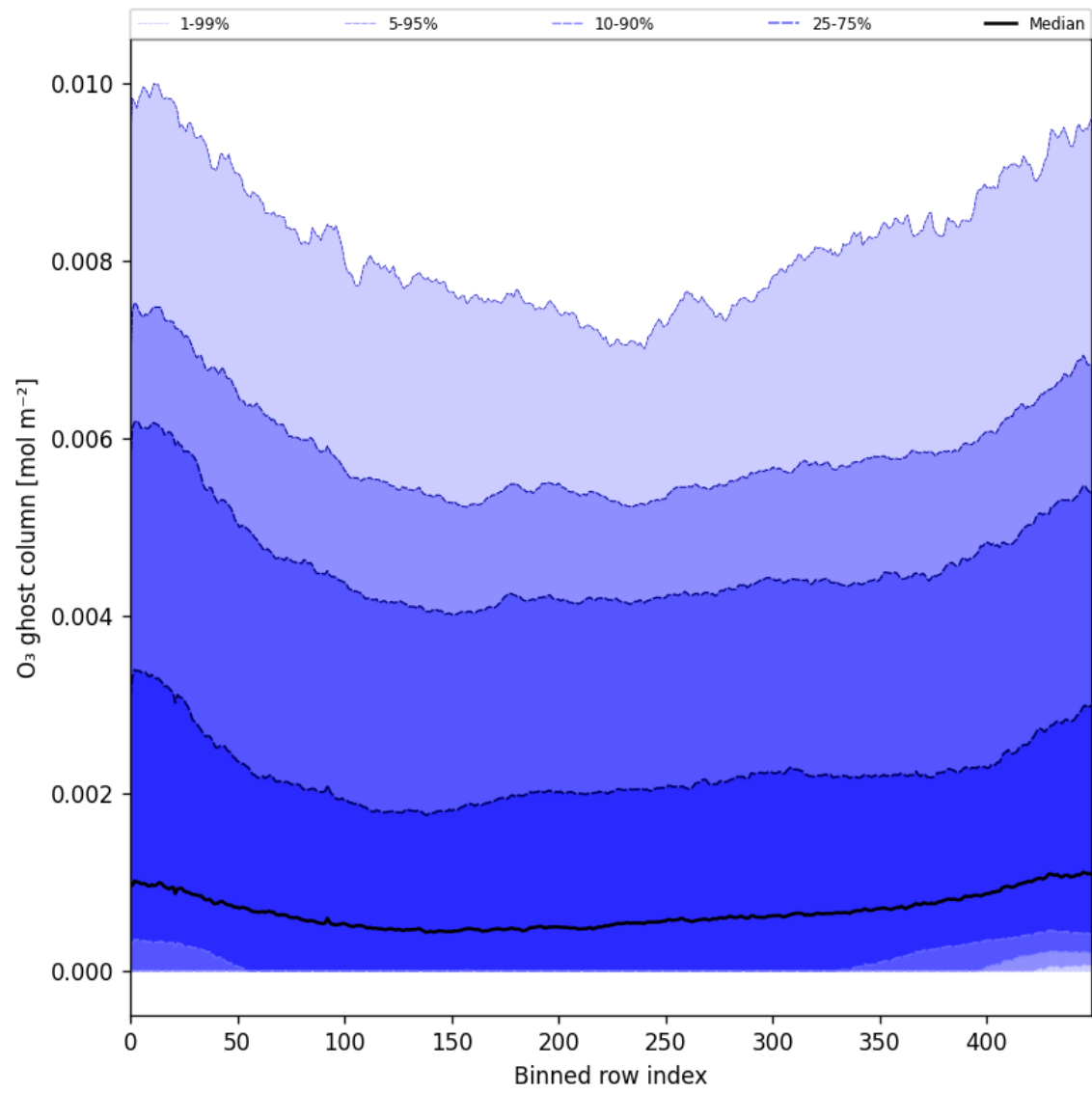
Figure 32: Along track statistics of “O 3 ghost column” for 2025-09-02 to 2025-09-04
