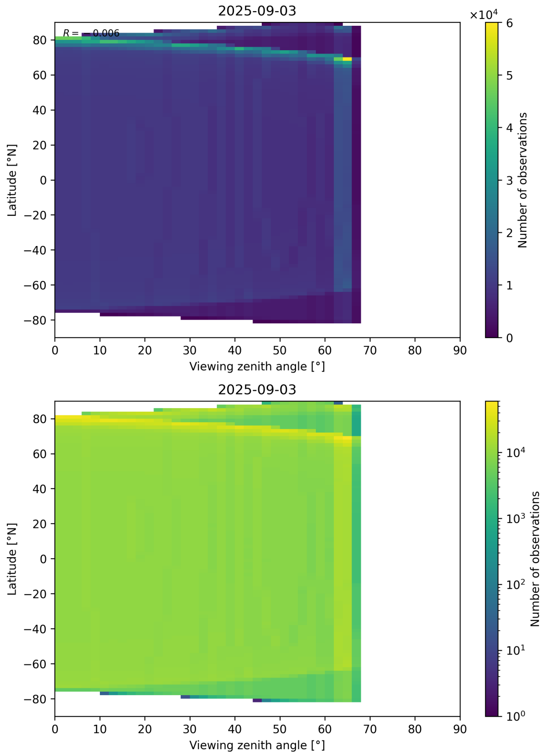
Figure 49: Scatter density plot of “Viewing zenith angle” against “Latitude” for 2025-09-02 to 2025-09-04.
