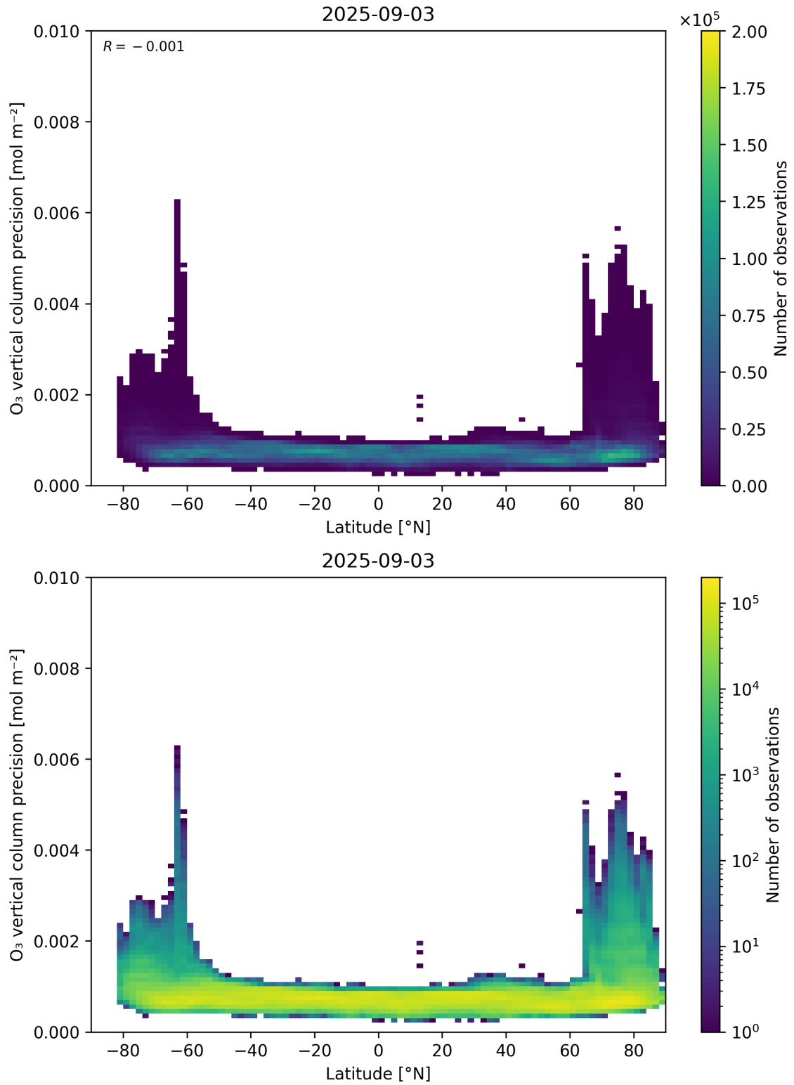
Figure 37: Scatter density plot of “Latitude” against “O 3 vertical column precision” for 2025-09-02 to 2025-09-04.
