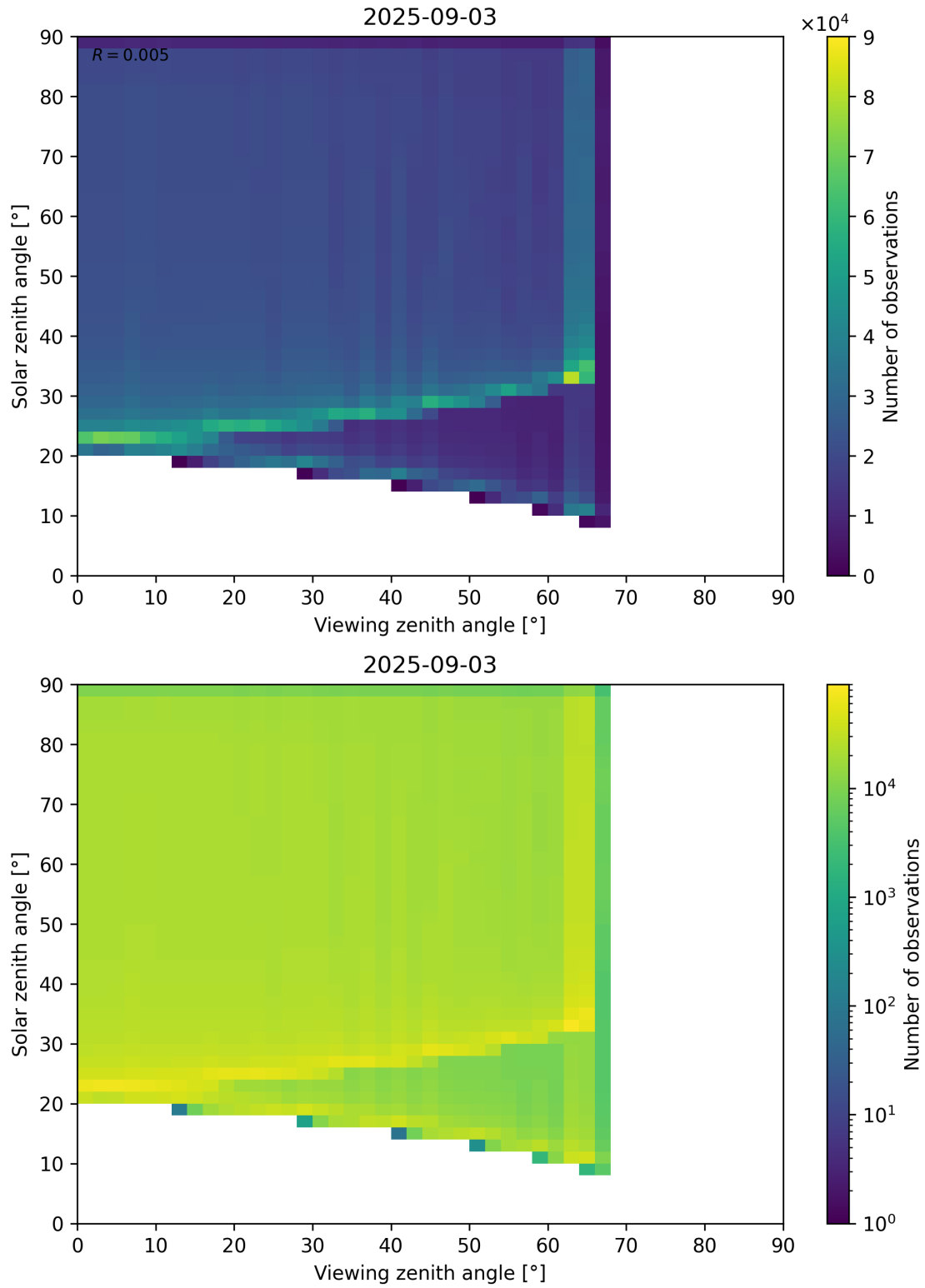
Figure 54: Scatter density plot of “Viewing zenith angle” against “Solar zenith angle” for 2025-09-02 to 2025-09-04.
