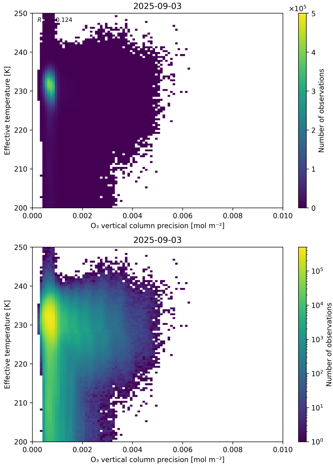
Figure 42: Scatter density plot of “ O_3 vertical column precision” against “Effective temperature” for 2025-09-02 to 2025-09-04.
