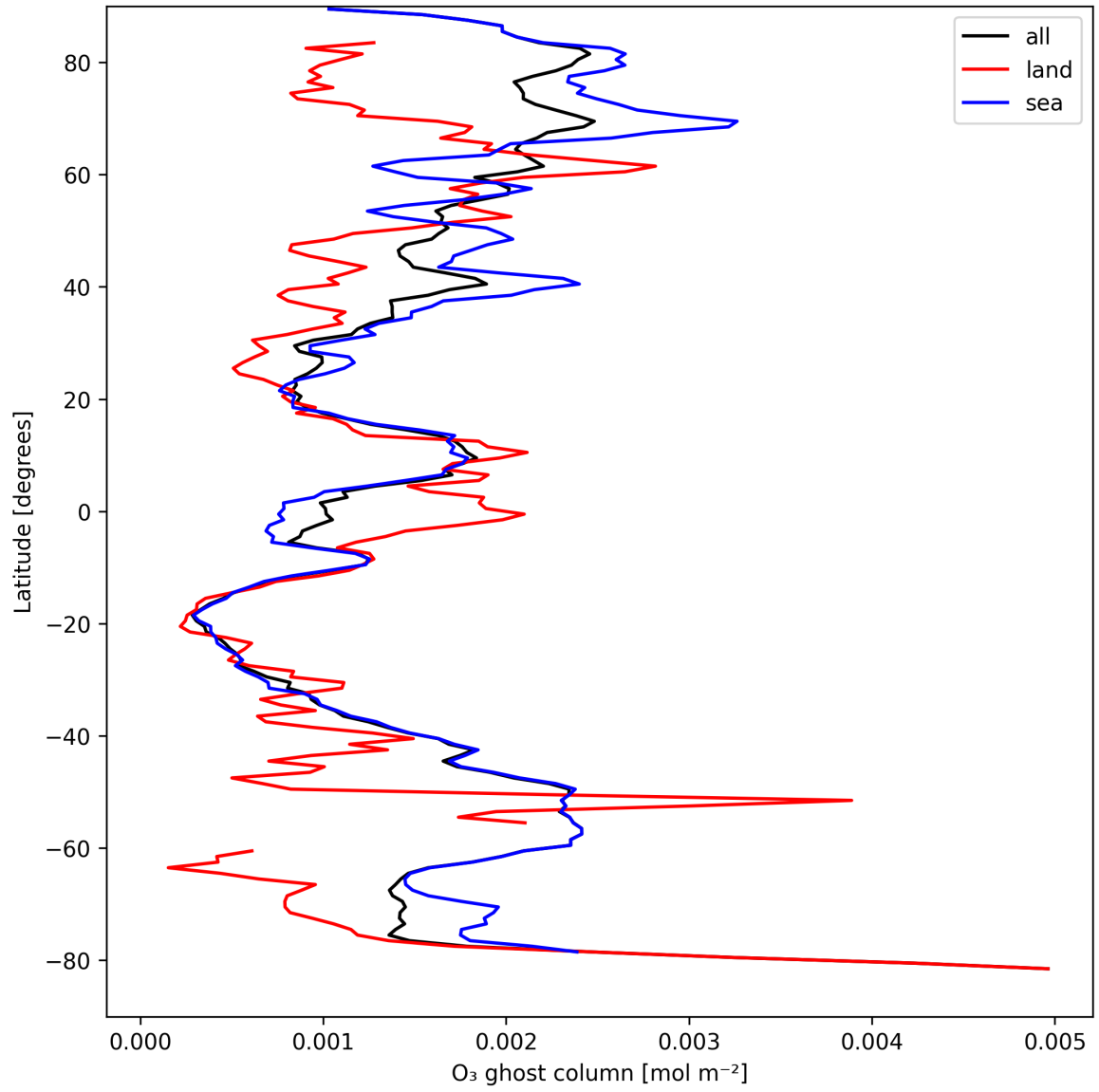
Figure 18: Zonal average of “O 3 ghost column” for 2025-09-02 to 2025-09-04.
