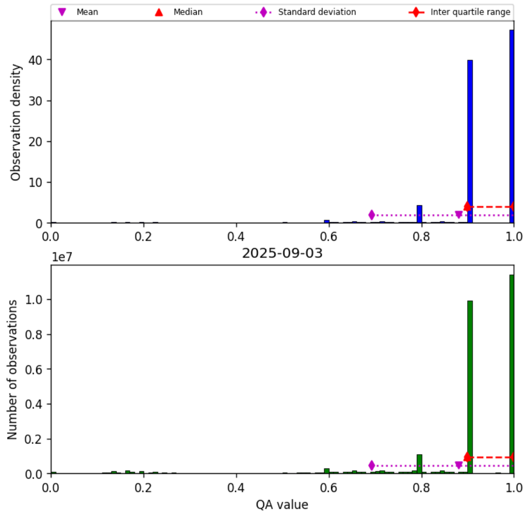
Figure 20: Histogram of “QA value” for 2025-09-02 to 2025-09-04
