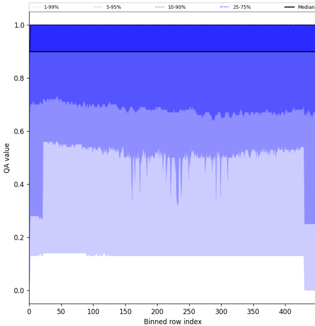
Figure 27: Along track statistics of “QA value” for 2025-09-02 to 2025-09-04
