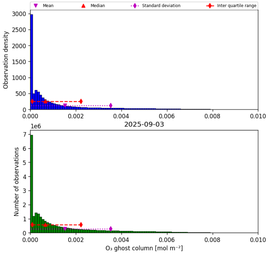
Figure 25: Histogram of “O 3 ghost column” for 2025-09-02 to 2025-09-04
