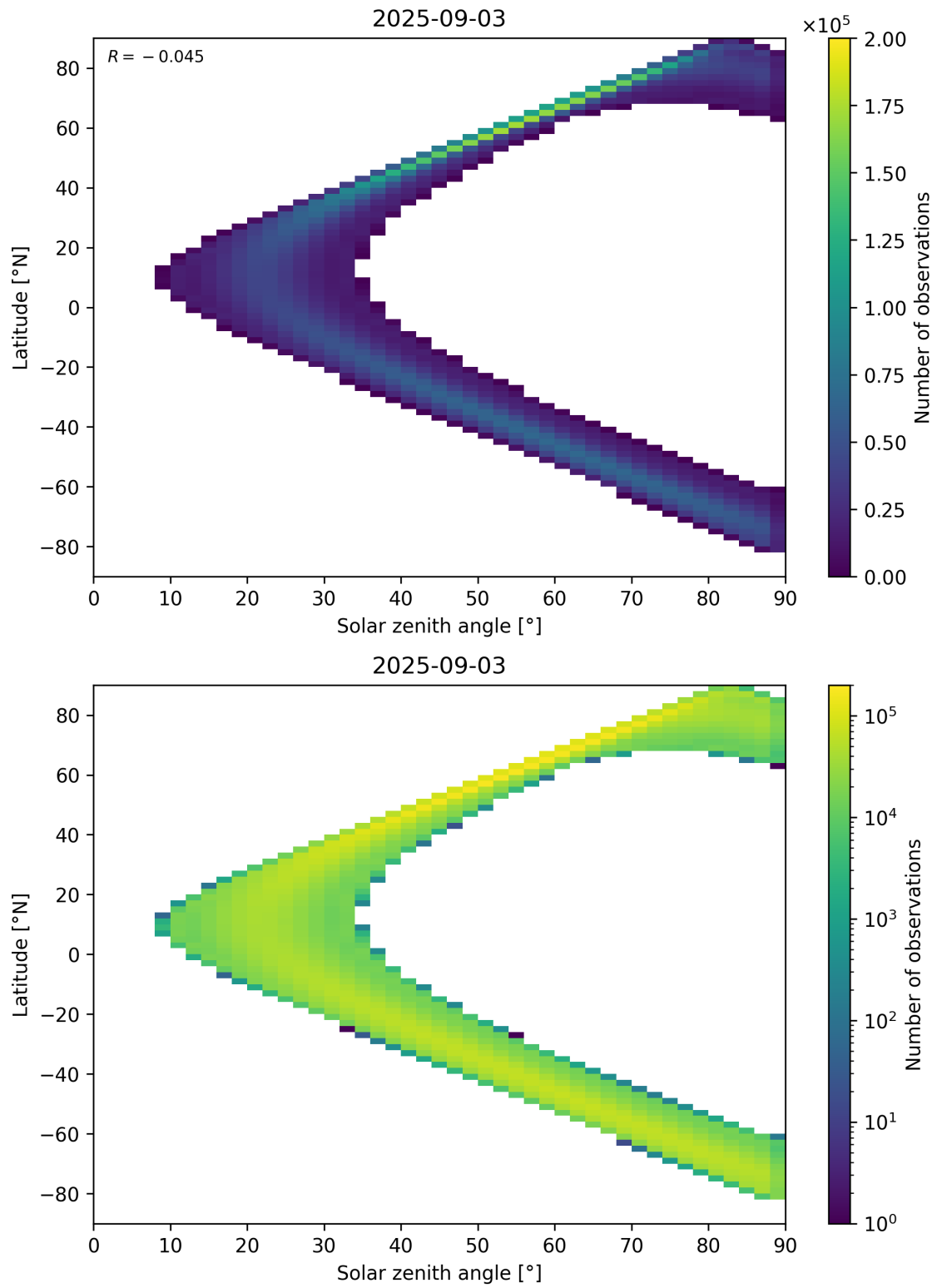
Figure 44: Scatter density plot of “Solar zenith angle” against “Latitude” for 2025-09-02 to 2025-09-04.
