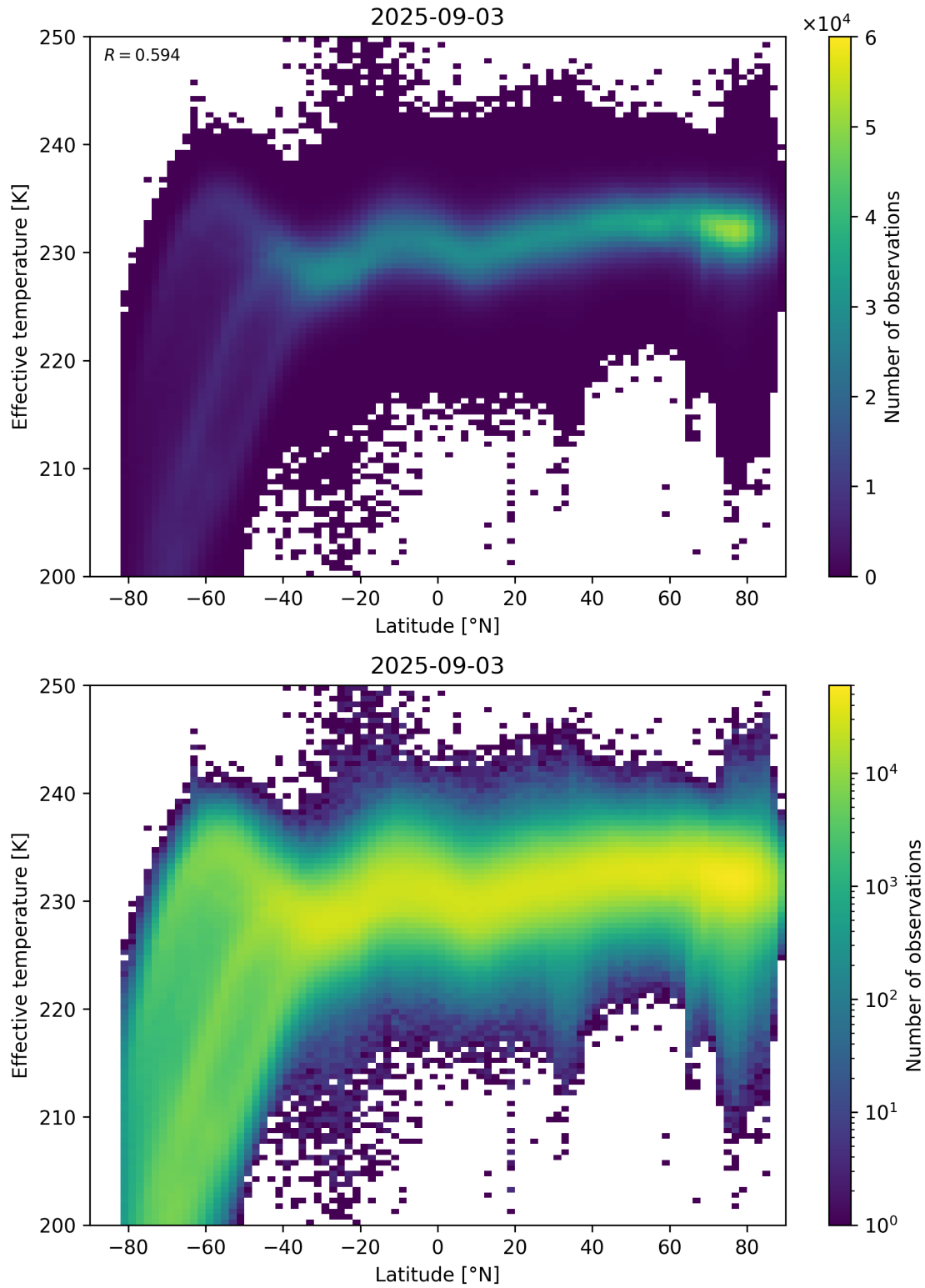
Figure 34: Scatter density plot of “Latitude” against “Effective temperature” for 2025-09-02 to 2025-09-04.
