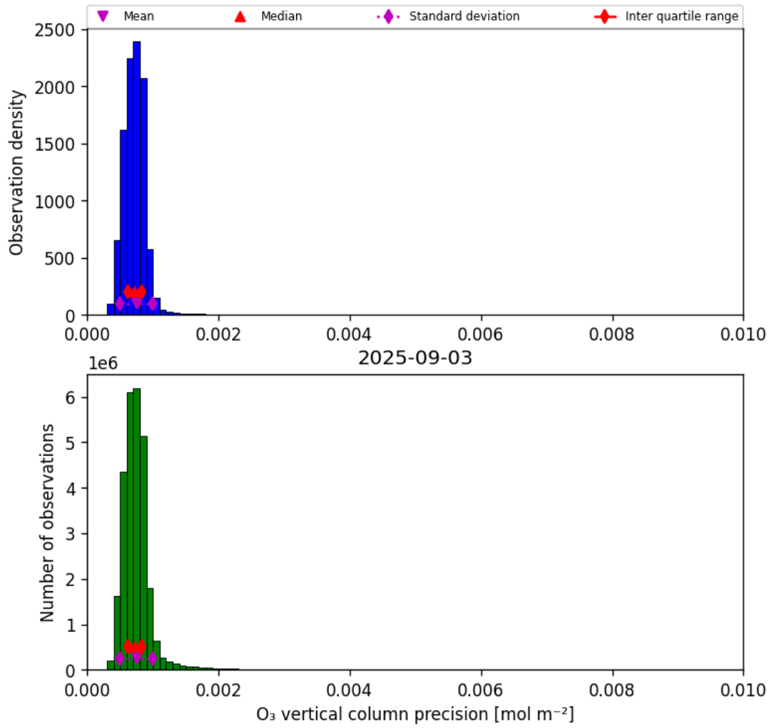
Figure 22: Histogram of “O 3 vertical column precision” for 2025-09-02 to 2025-09-04
