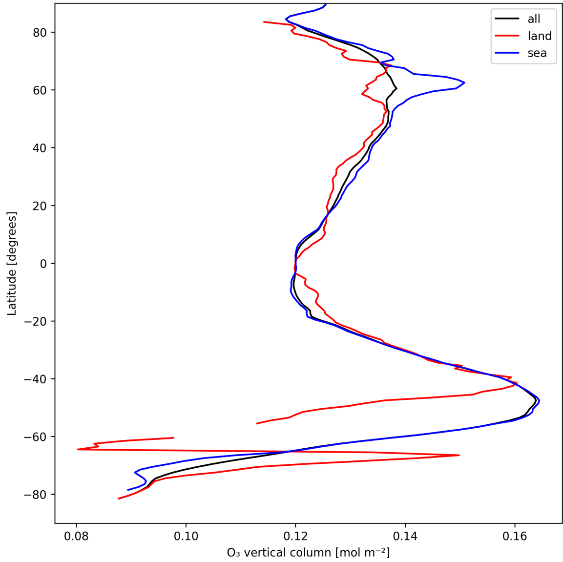
Figure 14: Zonal average of “O 3 vertical column” for 2025-09-02 to 2025-09-04.
