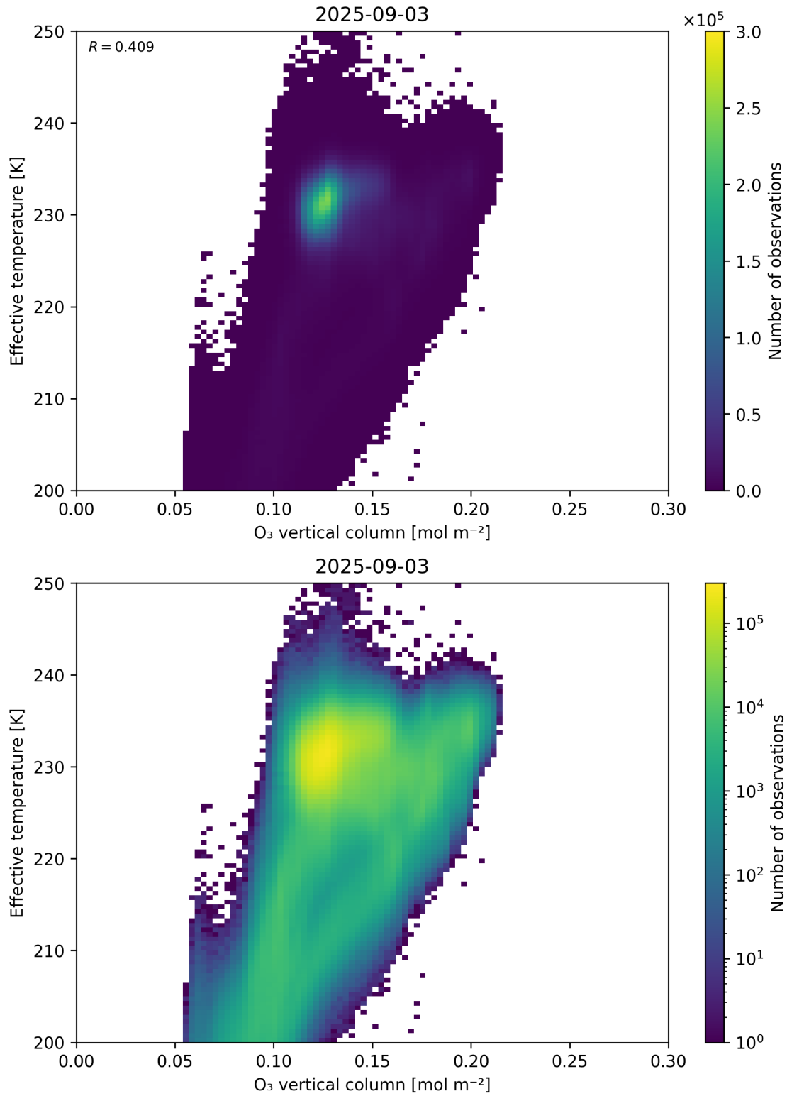
Figure 39: Scatter density plot of “O 3 vertical column” against “Effective temperature” for 2025-09-02 to 2025-09-04.
