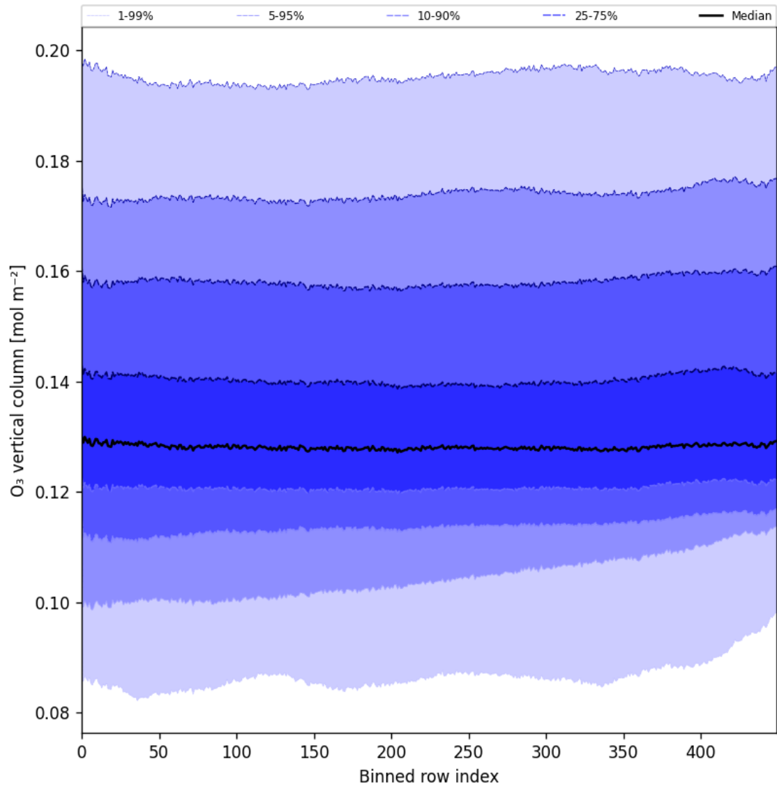
Figure 28: Along track statistics of “O 3 vertical column” for 2025-09-02 to 2025-09-04
