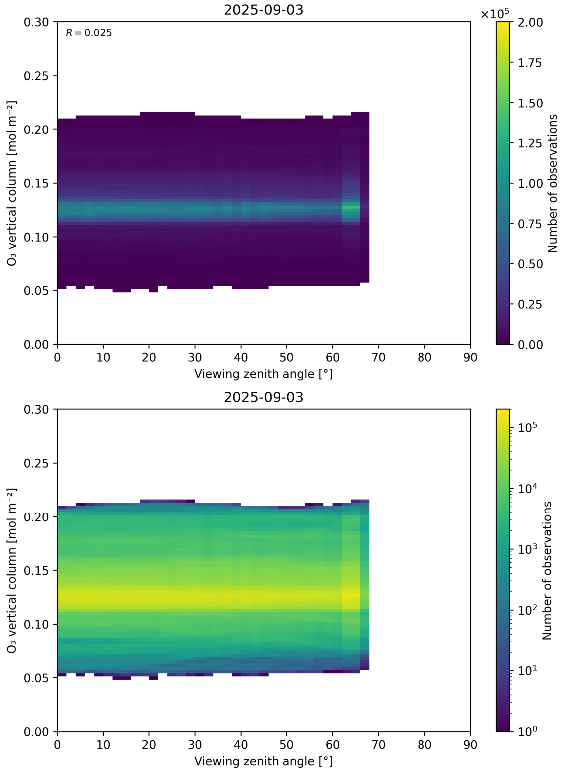
Figure 52: Scatter density plot of “Viewing zenith angle” against “O 3 vertical column” for 2025-09-02 to 2025-09-04.
