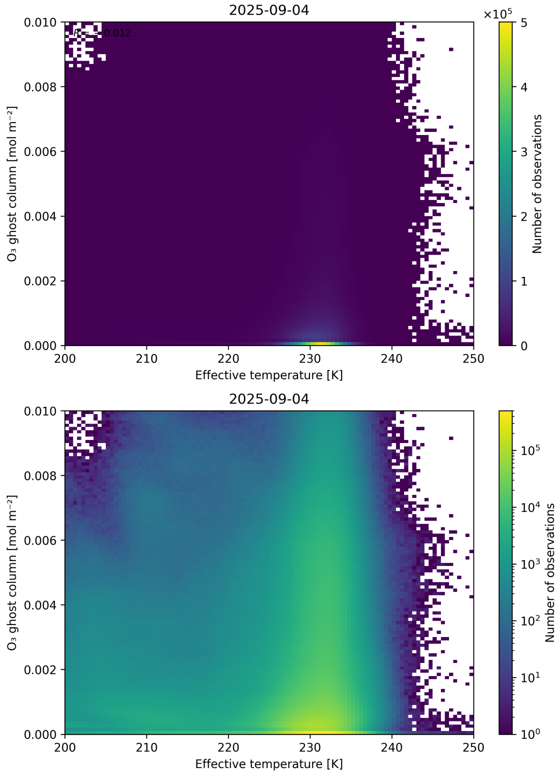
Figure 38: Scatter density plot of “Effective temperature” against “O 3 ghost column” for 2025-09-04 to 2025-09-05.
