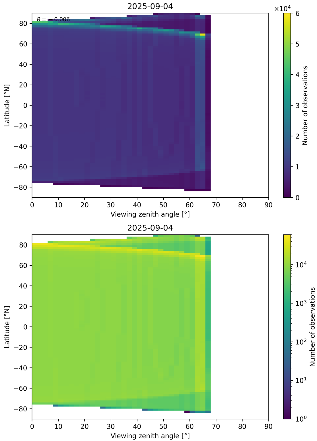
Figure 49: Scatter density plot of “Viewing zenith angle” against “Latitude” for 2025-09-04 to 2025-09-05.
