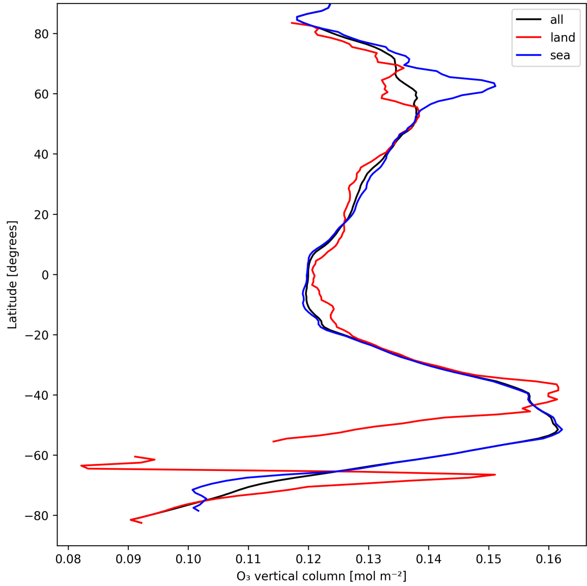
Figure 14: Zonal average of “O 3 vertical column” for 2025-09-04 to 2025-09-05.
