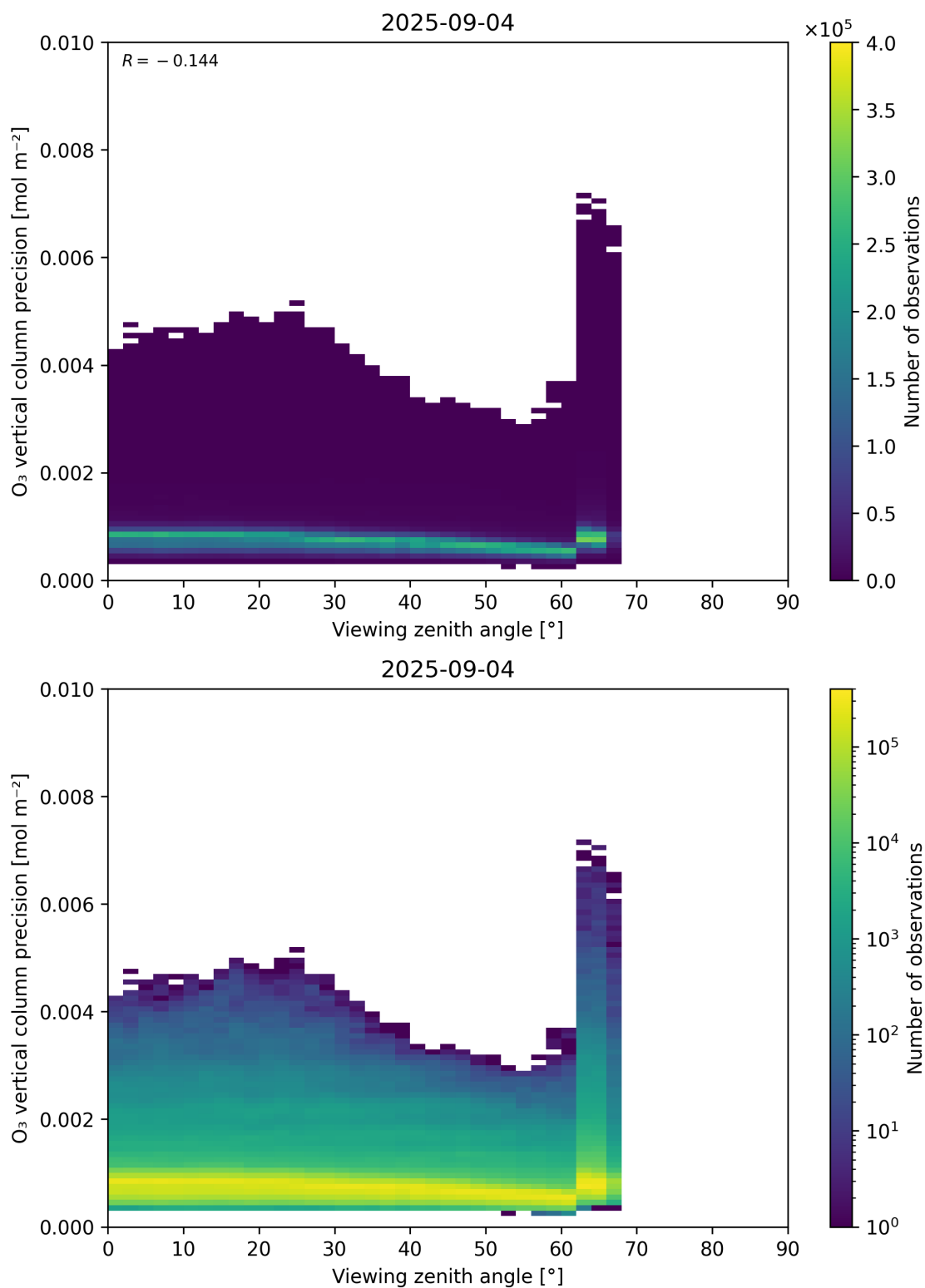
Figure 53: Scatter density plot of “Viewing zenith angle” against “O 3 vertical column precision” for 2025-09-04 to 2025-09-05.
