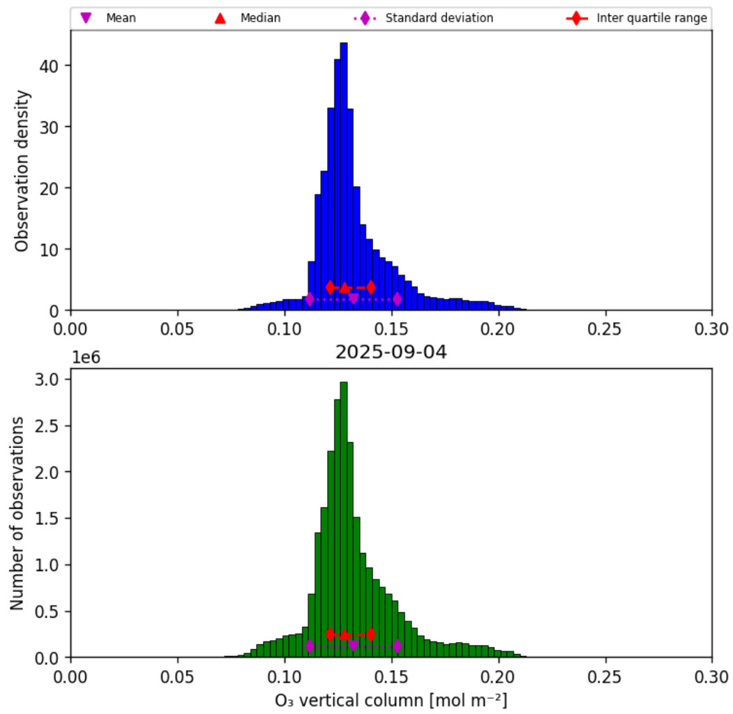
Figure 21: Histogram of “O 3 vertical column” for 2025-09-04 to 2025-09-05
