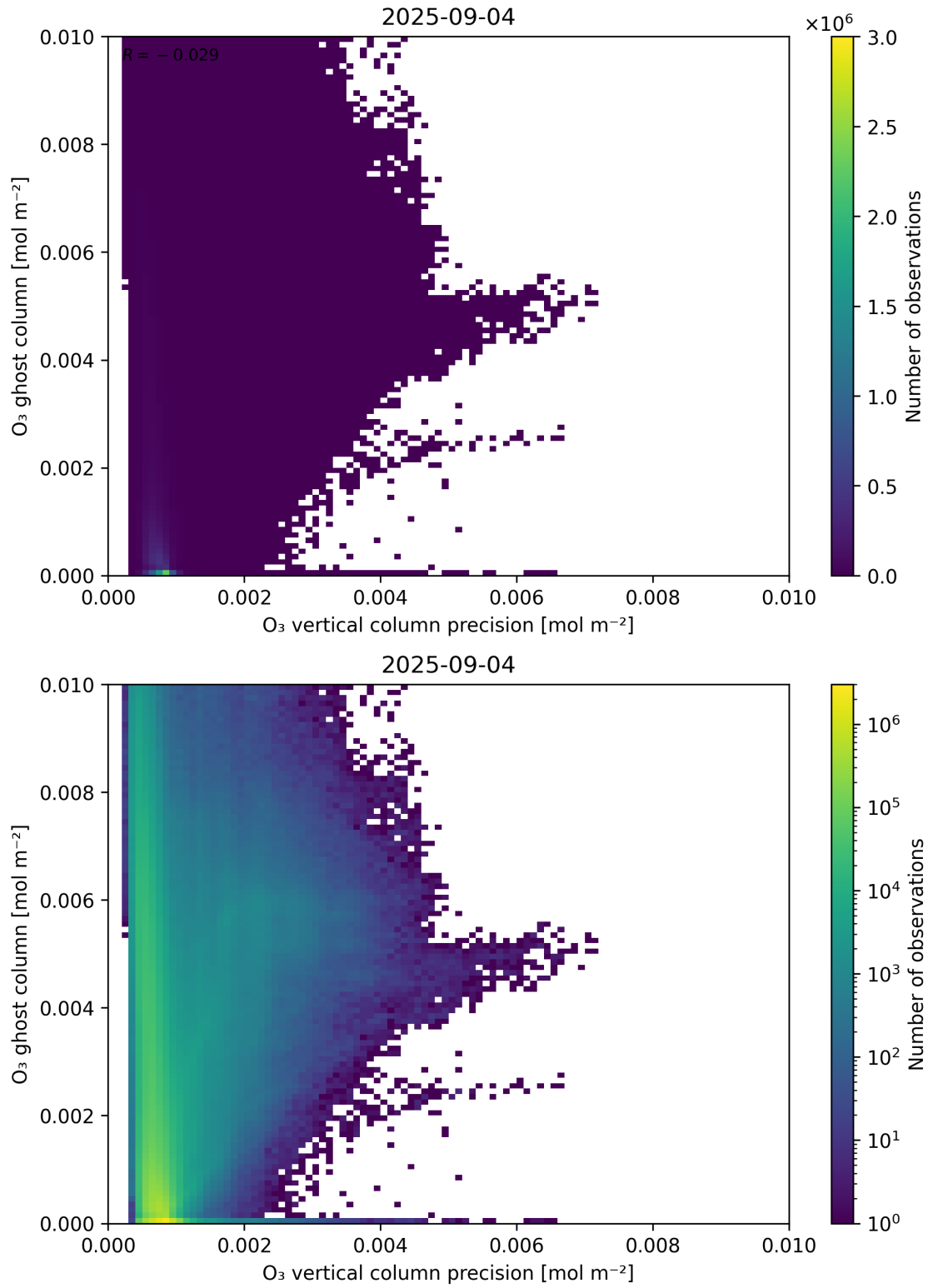
Figure 43: Scatter density plot of “ \text{O}_3 vertical column precision” against “ \text{O}_3 ghost column” for 2025-09-04 to 2025-09-05.
