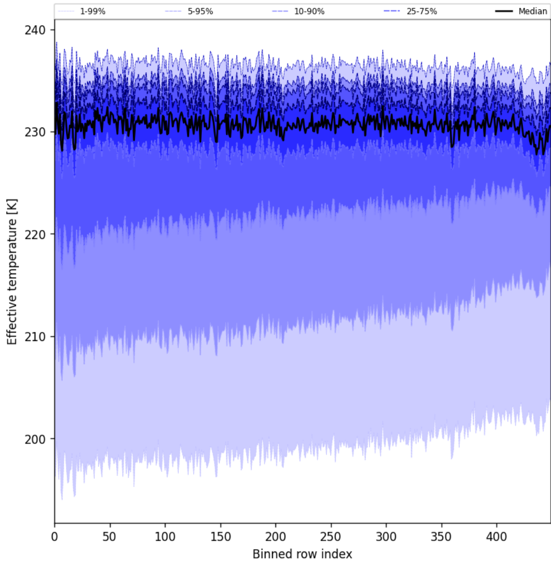
Figure 31: Along track statistics of "Effective temperature" for 2025-09-04 to 2025-09-05
