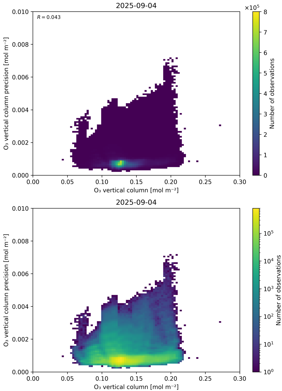
Figure 41: Scatter density plot of “O 3 vertical column” against “O 3 vertical column precision” for 2025-09-04 to 2025-09-05.
