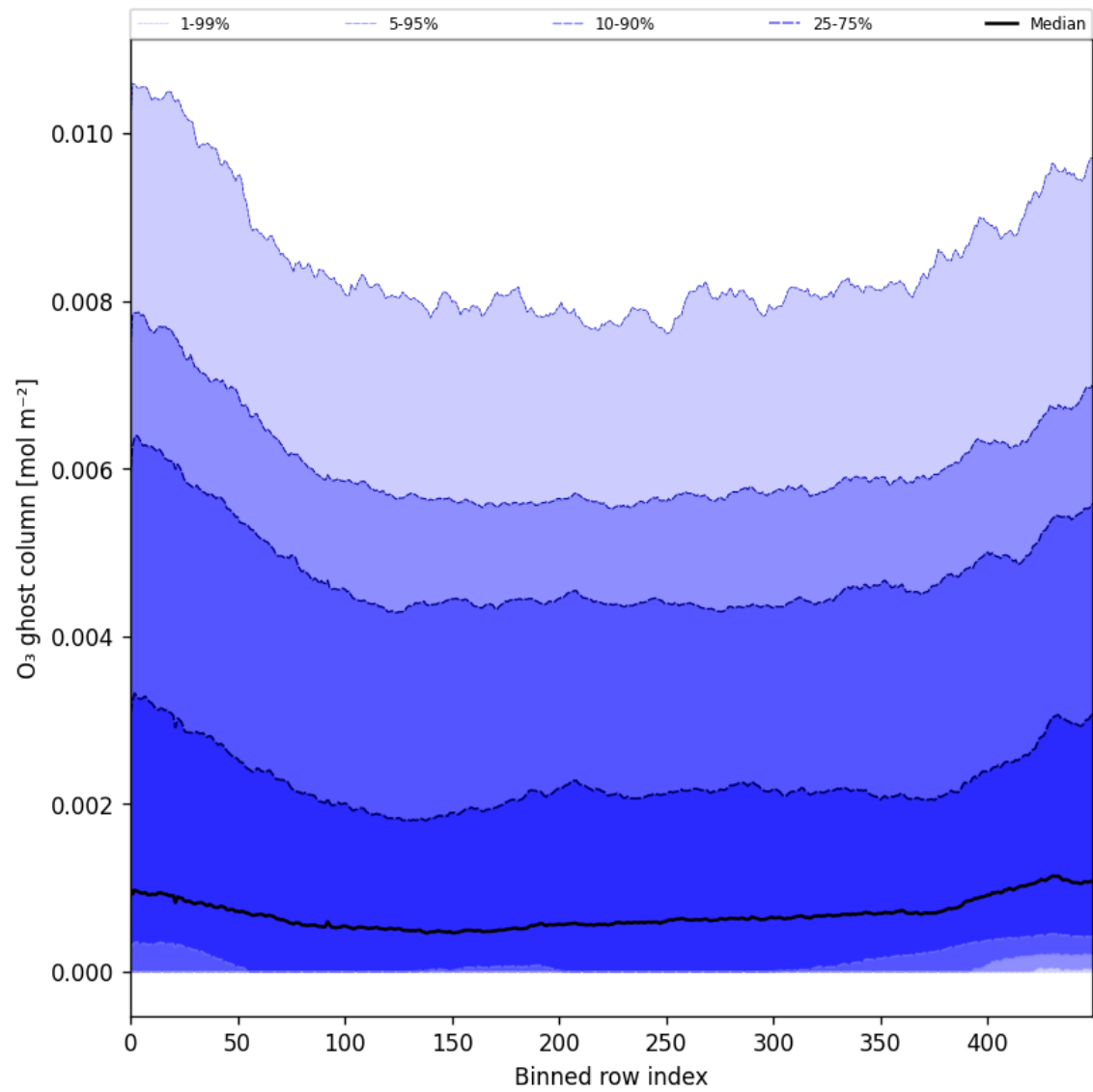
Figure 32: Along track statistics of “O 3 ghost column” for 2025-09-04 to 2025-09-05
