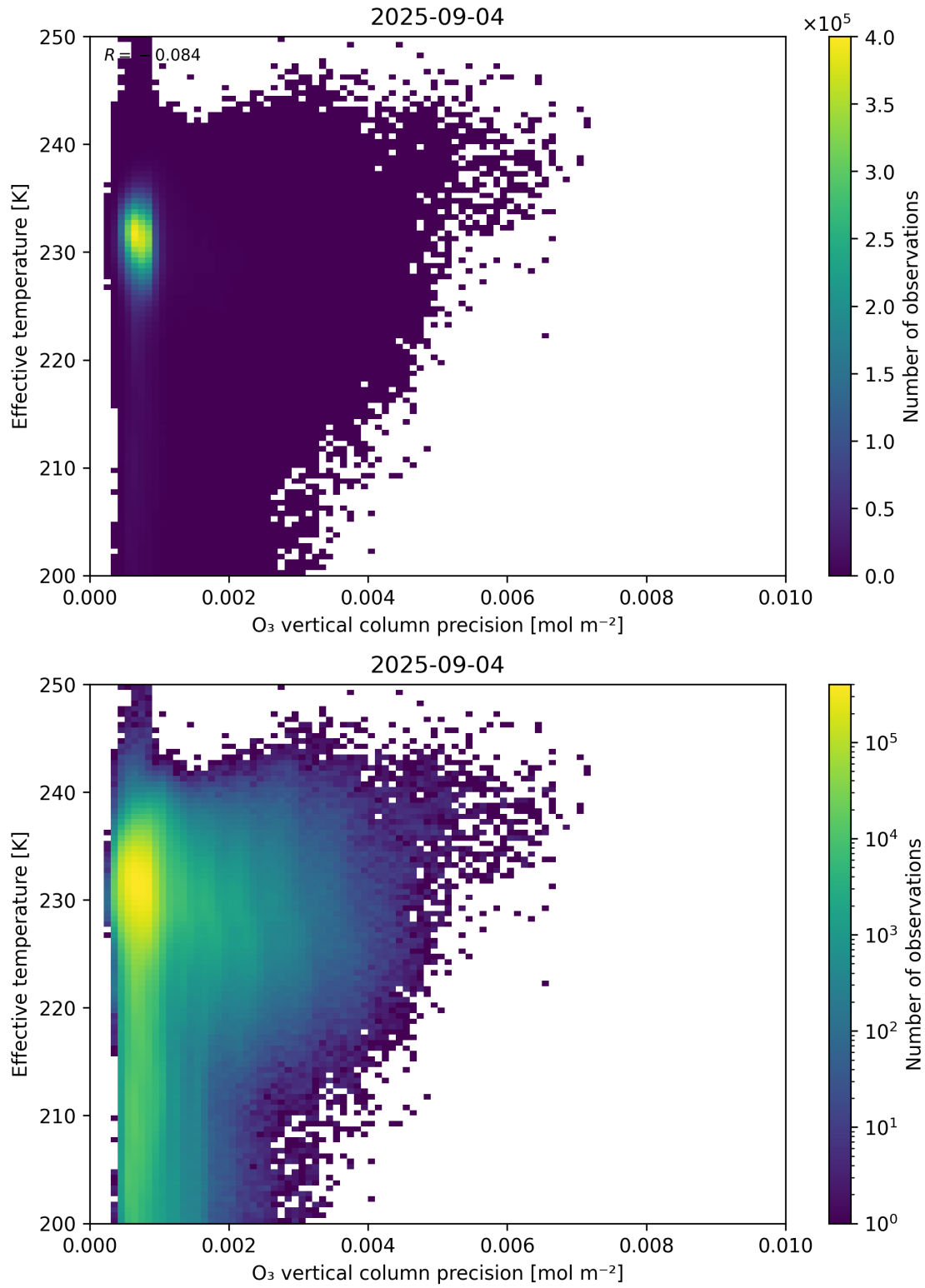
Figure 42: Scatter density plot of “O 3 vertical column precision” against “Effective temperature” for 2025-09-04 to 2025-09-05.
