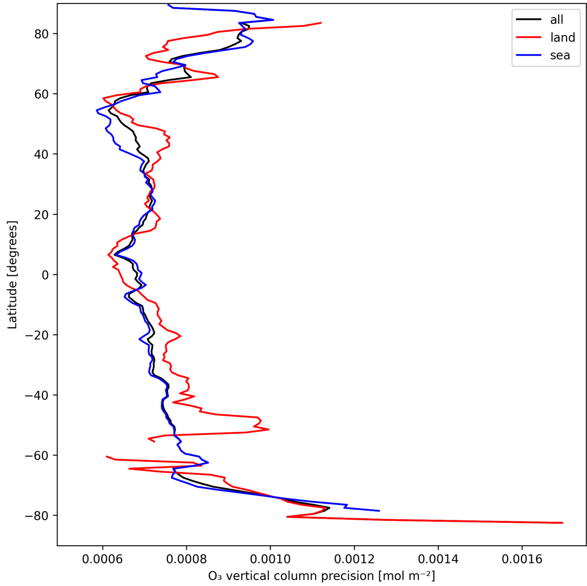
Figure 15: Zonal average of “O 3 vertical column precision” for 2025-09-04 to 2025-09-05.
