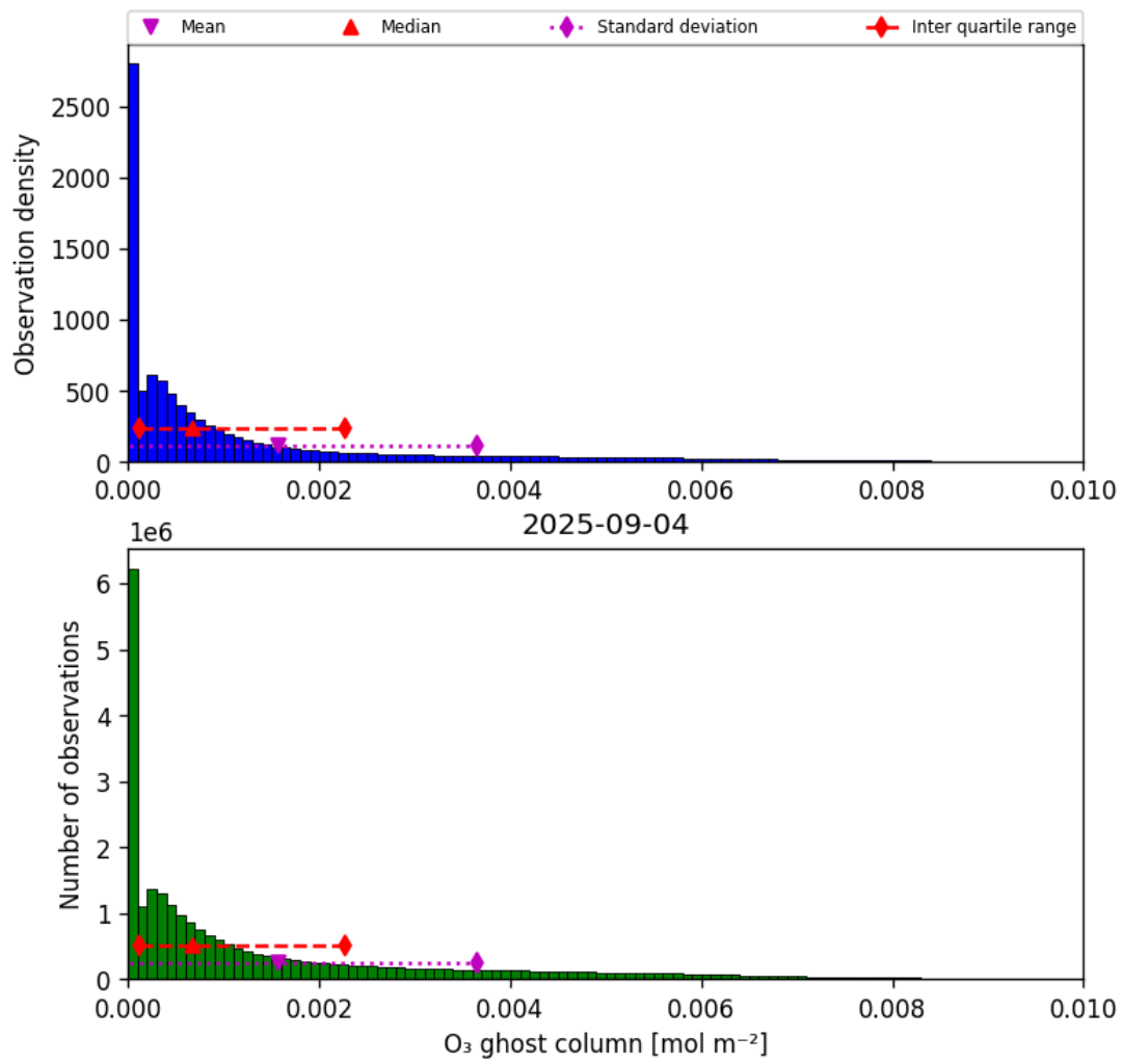
Figure 25: Histogram of “O 3 ghost column” for 2025-09-04 to 2025-09-05
