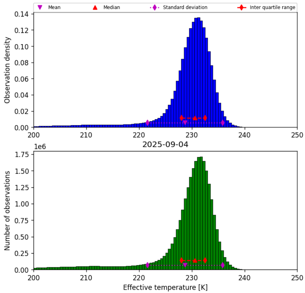
Figure 24: Histogram of “Effective temperature” for 2025-09-04 to 2025-09-05
