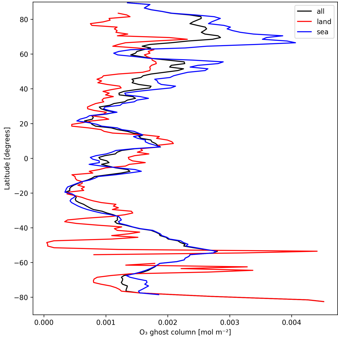
Figure 18: Zonal average of “O 3 ghost column” for 2025-09-04 to 2025-09-05.
