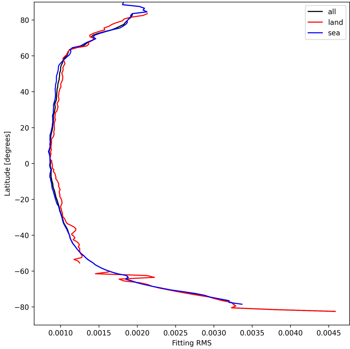
Figure 16: Zonal average of “Fitting RMS” for 2025-09-04 to 2025-09-05.
