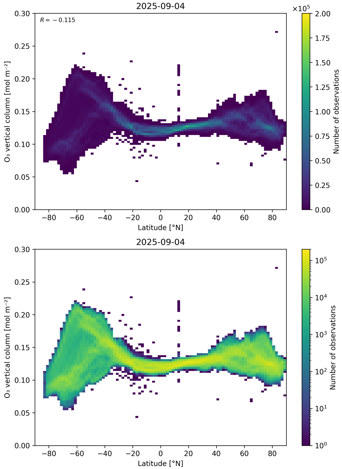
Figure 36: Scatter density plot of “Latitude” against “O 3 vertical column” for 2025-09-04 to 2025-09-05.
