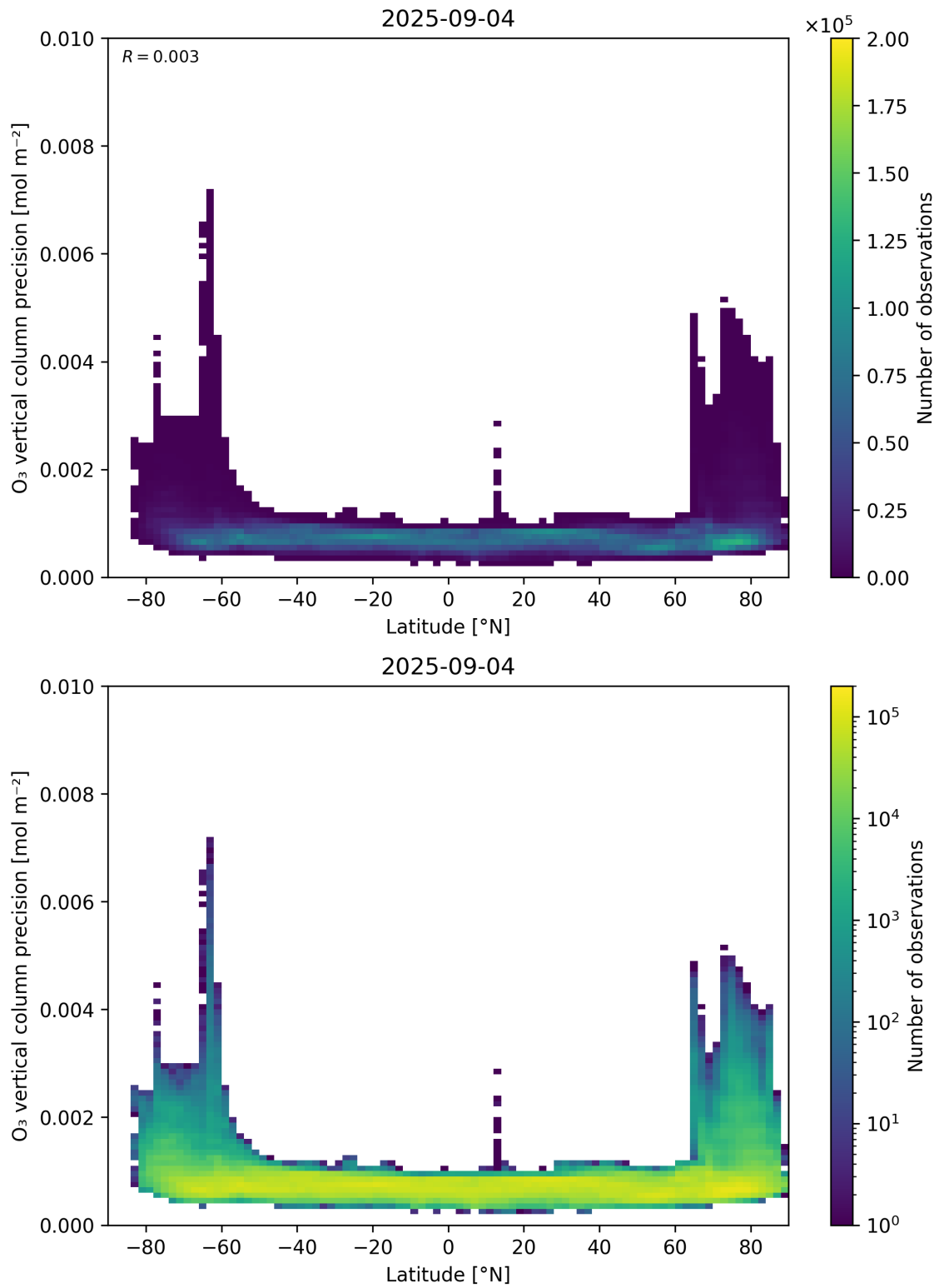
Figure 37: Scatter density plot of “Latitude” against “O 3 vertical column precision” for 2025-09-04 to 2025-09-05.
