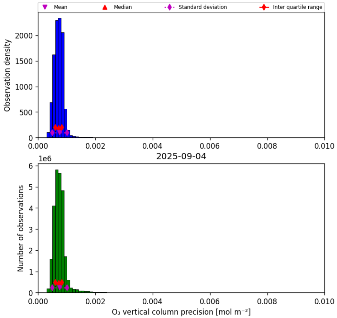
Figure 22: Histogram of “O 3 vertical column precision” for 2025-09-04 to 2025-09-05
