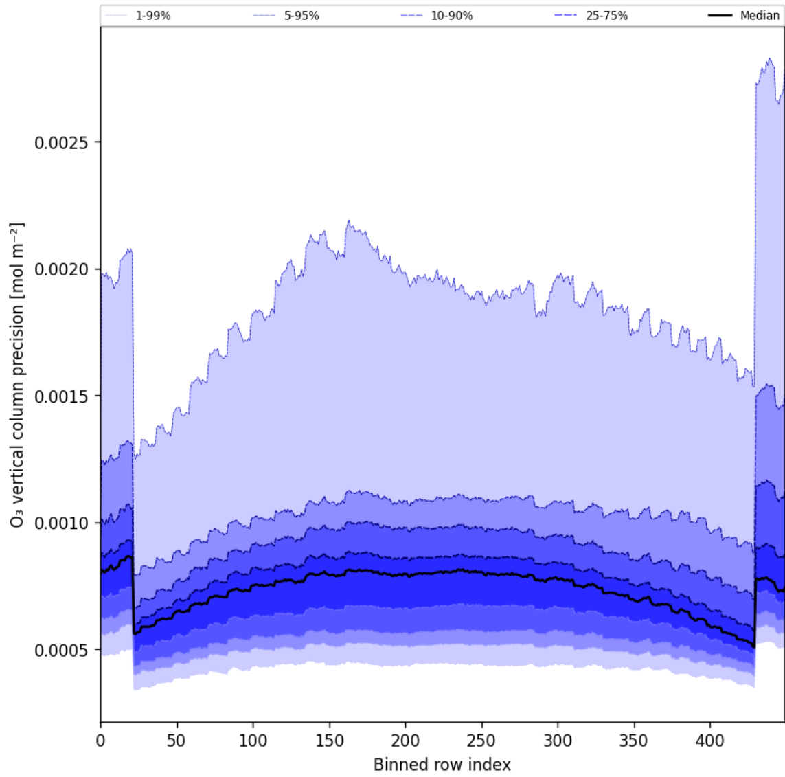
Figure 29: Along track statistics of “O 3 vertical column precision” for 2025-09-04 to 2025-09-05
