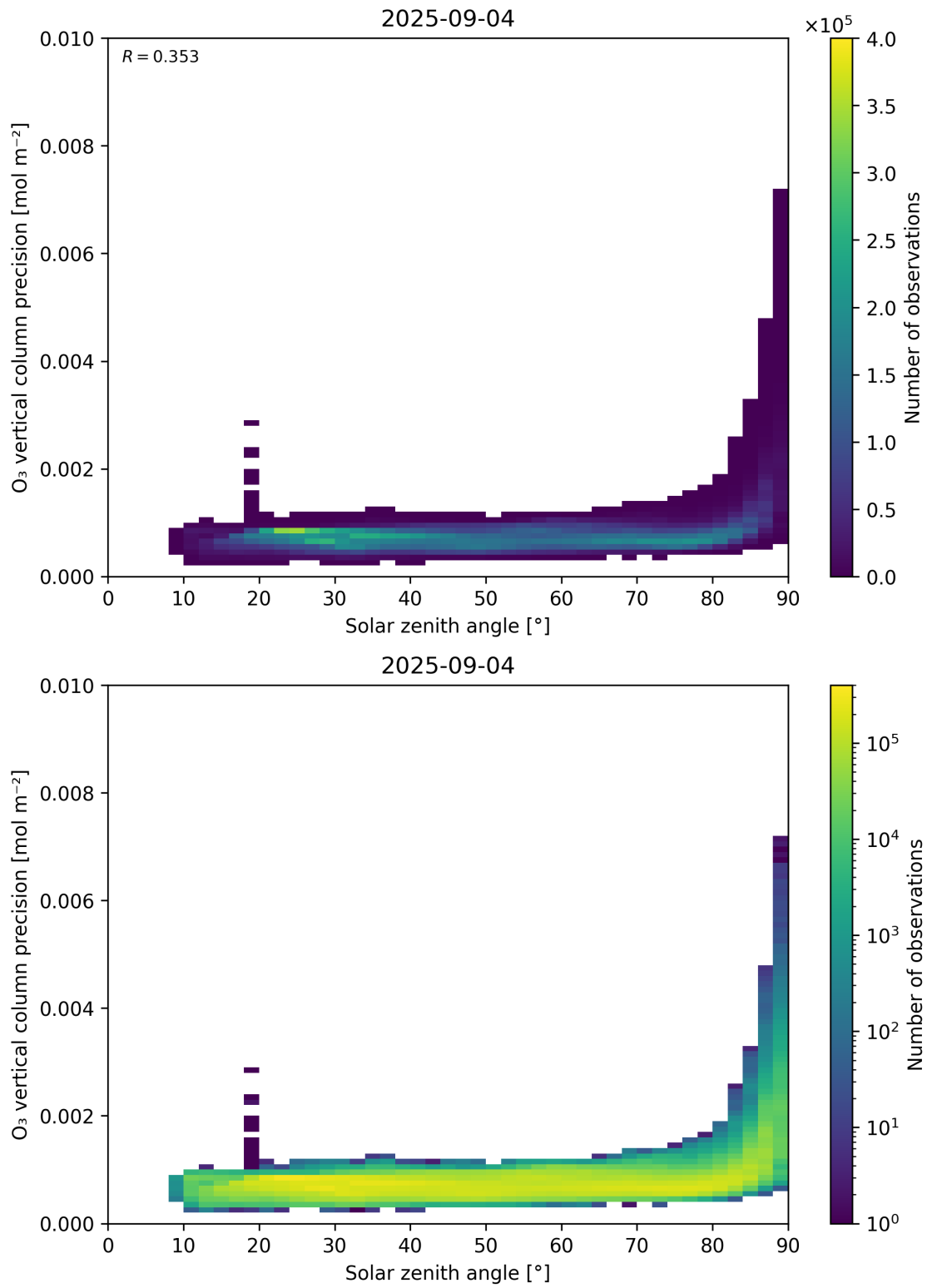
Figure 48: Scatter density plot of “Solar zenith angle” against “O 3 vertical column precision” for 2025-09-04 to 2025-09-05.
