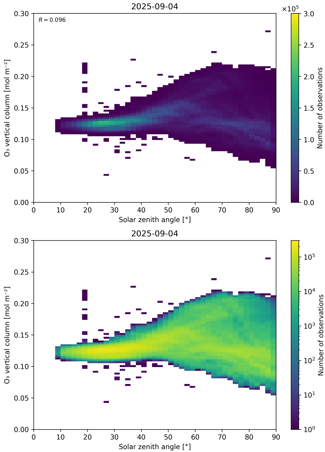
Figure 47: Scatter density plot of “Solar zenith angle” against “O 3 vertical column” for 2025-09-04 to 2025-09-05.
