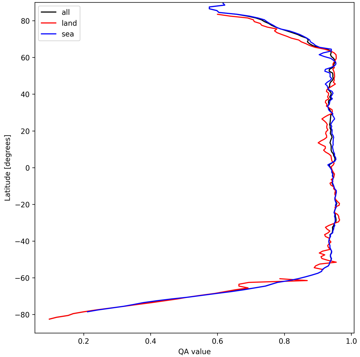
Figure 13: Zonal average of “QA value” for 2025-09-04 to 2025-09-05.
