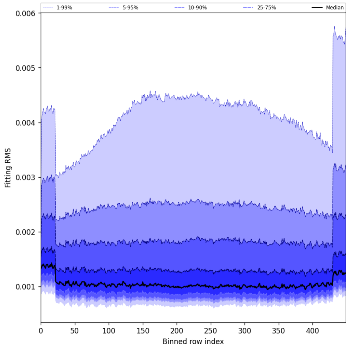
Figure 30: Along track statistics of “Fitting RMS” for 2025-09-04 to 2025-09-05
