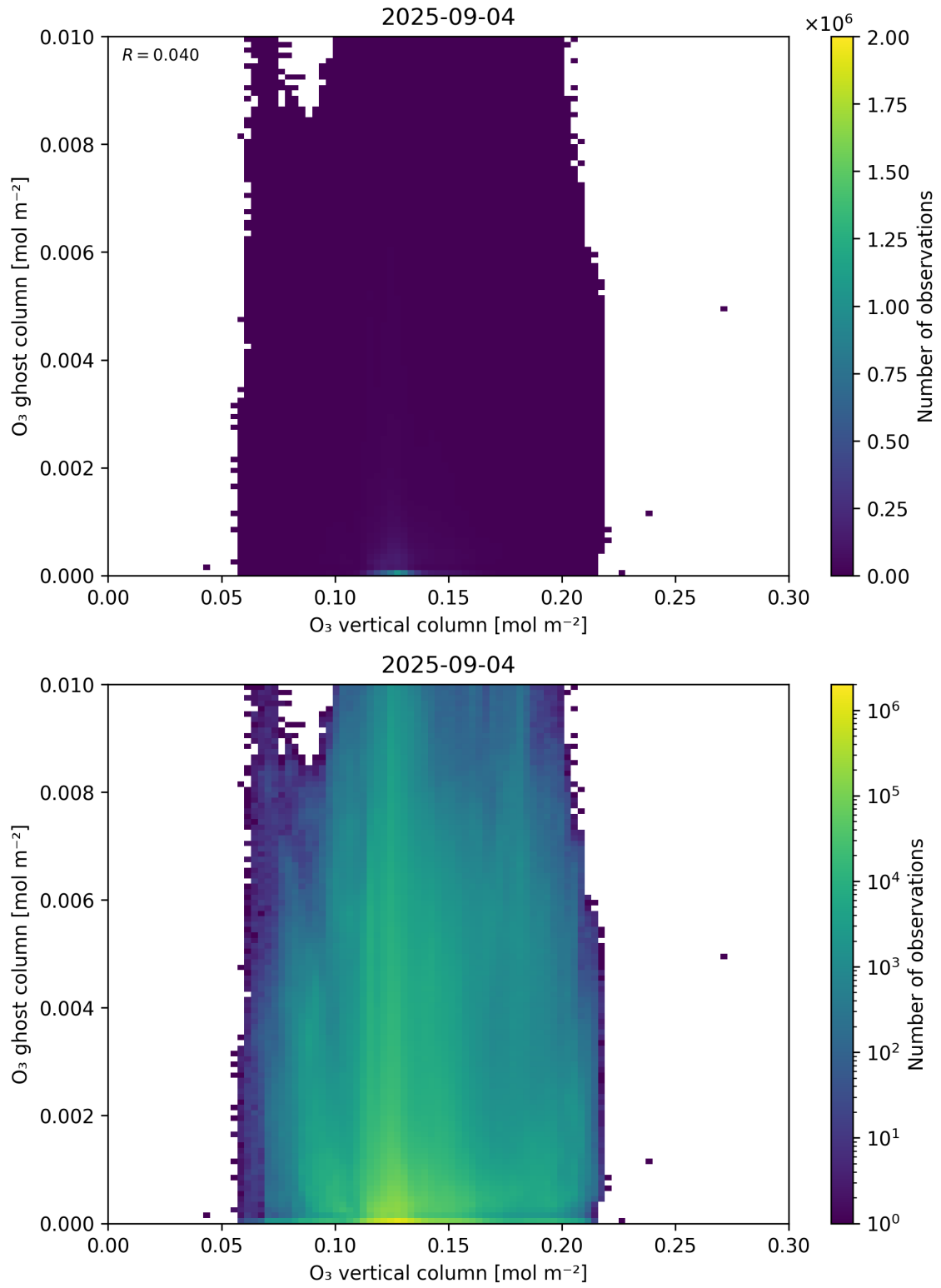
Figure 40: Scatter density plot of “O 3 vertical column” against “O 3 ghost column” for 2025-09-04 to 2025-09-05.
