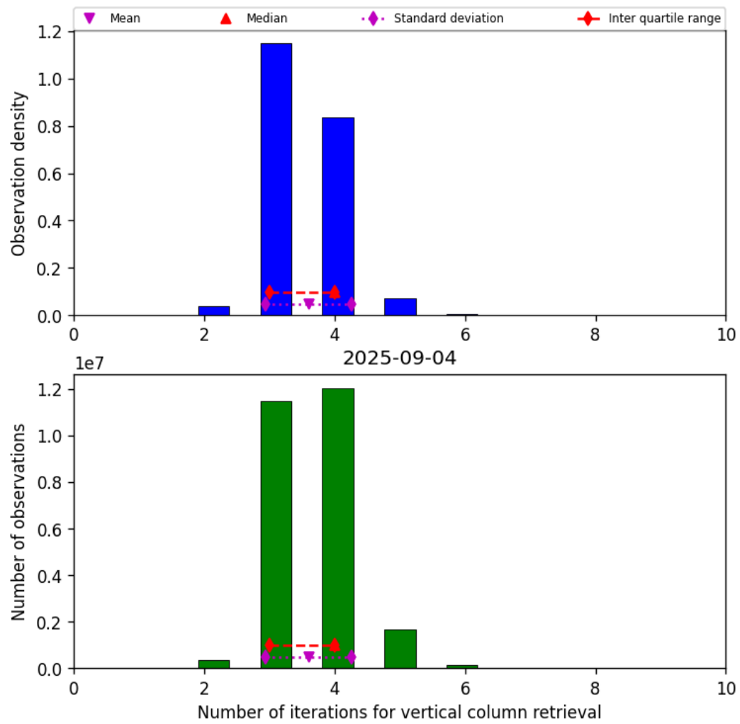
Figure 26: Histogram of “Number of iterations for vertical column retrieval” for 2025-09-04 to 2025-09-05
