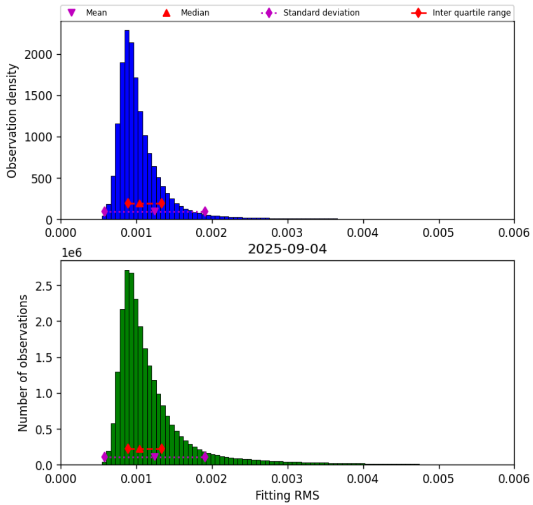
Figure 23: Histogram of “Fitting RMS” for 2025-09-04 to 2025-09-05
