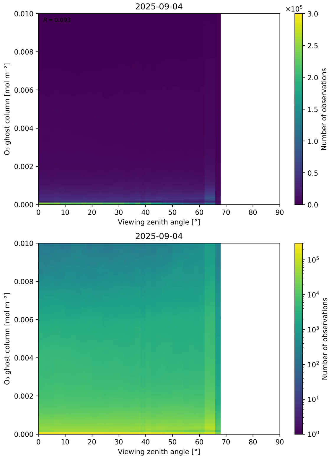
Figure 51: Scatter density plot of “Viewing zenith angle” against “O 3 ghost column” for 2025-09-04 to 2025-09-05.
