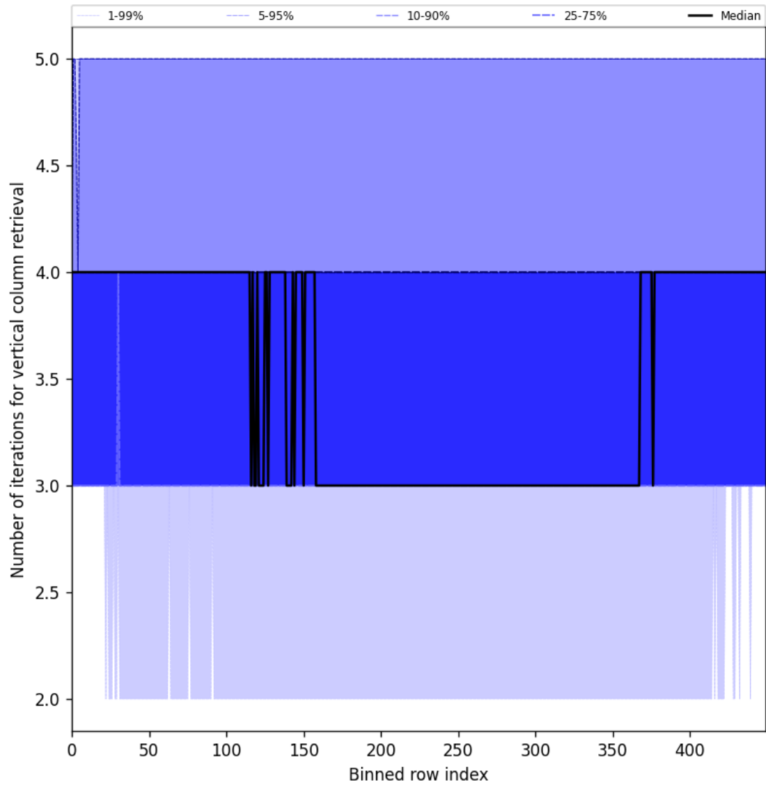
Figure 33: Along track statistics of “Number of iterations for vertical column retrieval” for 2025-09-04 to 2025-09-05
