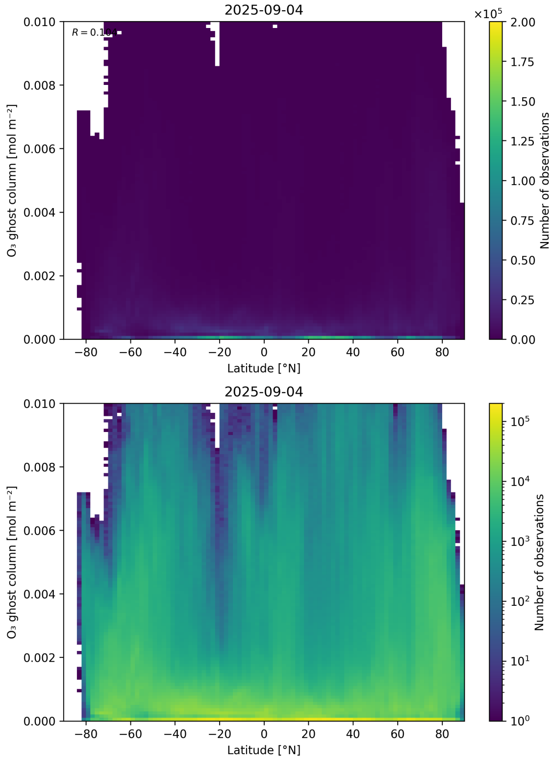
Figure 35: Scatter density plot of “Latitude” against “O 3 ghost column” for 2025-09-04 to 2025-09-05.
