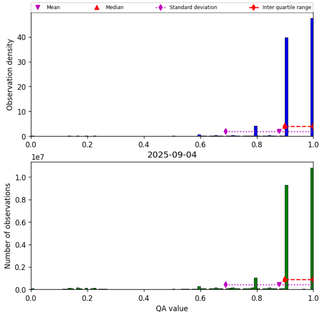
Figure 20: Histogram of “QA value” for 2025-09-04 to 2025-09-05
