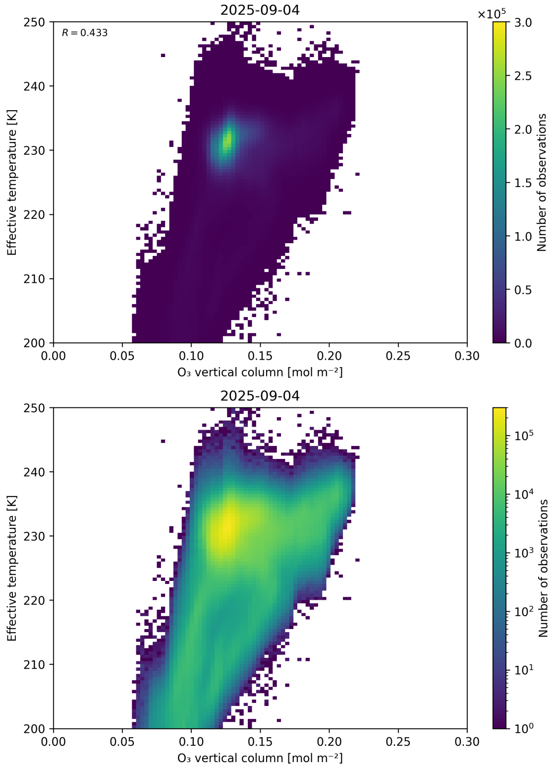
Figure 39: Scatter density plot of “O 3 vertical column” against “Effective temperature” for 2025-09-04 to 2025-09-05.
