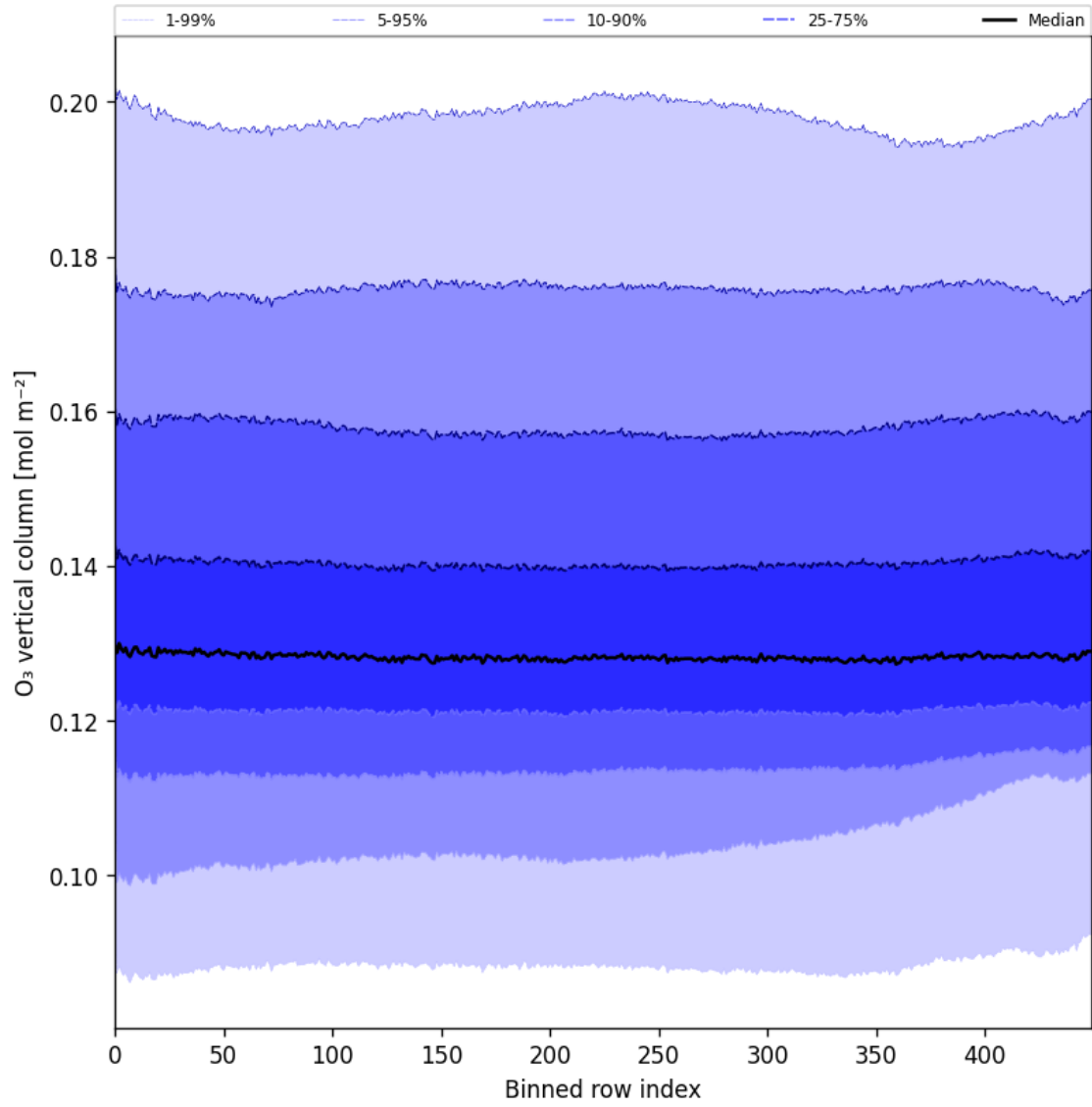
Figure 28: Along track statistics of “O 3 vertical column” for 2025-09-04 to 2025-09-05
