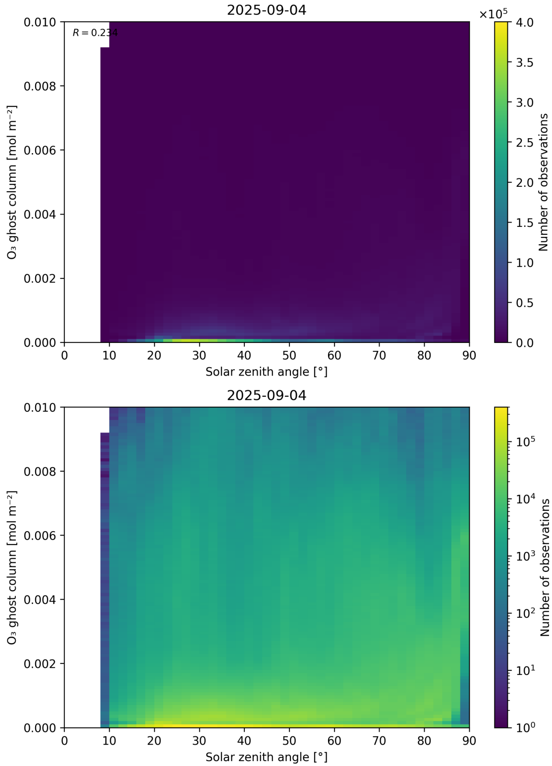
Figure 46: Scatter density plot of “Solar zenith angle” against “O 3 ghost column” for 2025-09-04 to 2025-09-05.
