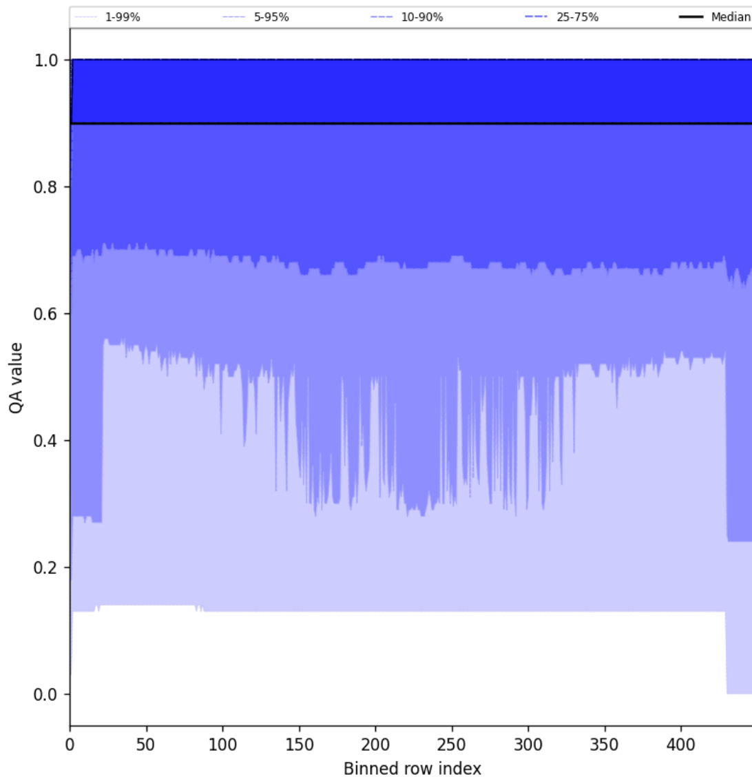
Figure 27: Along track statistics of “QA value” for 2025-09-04 to 2025-09-05
