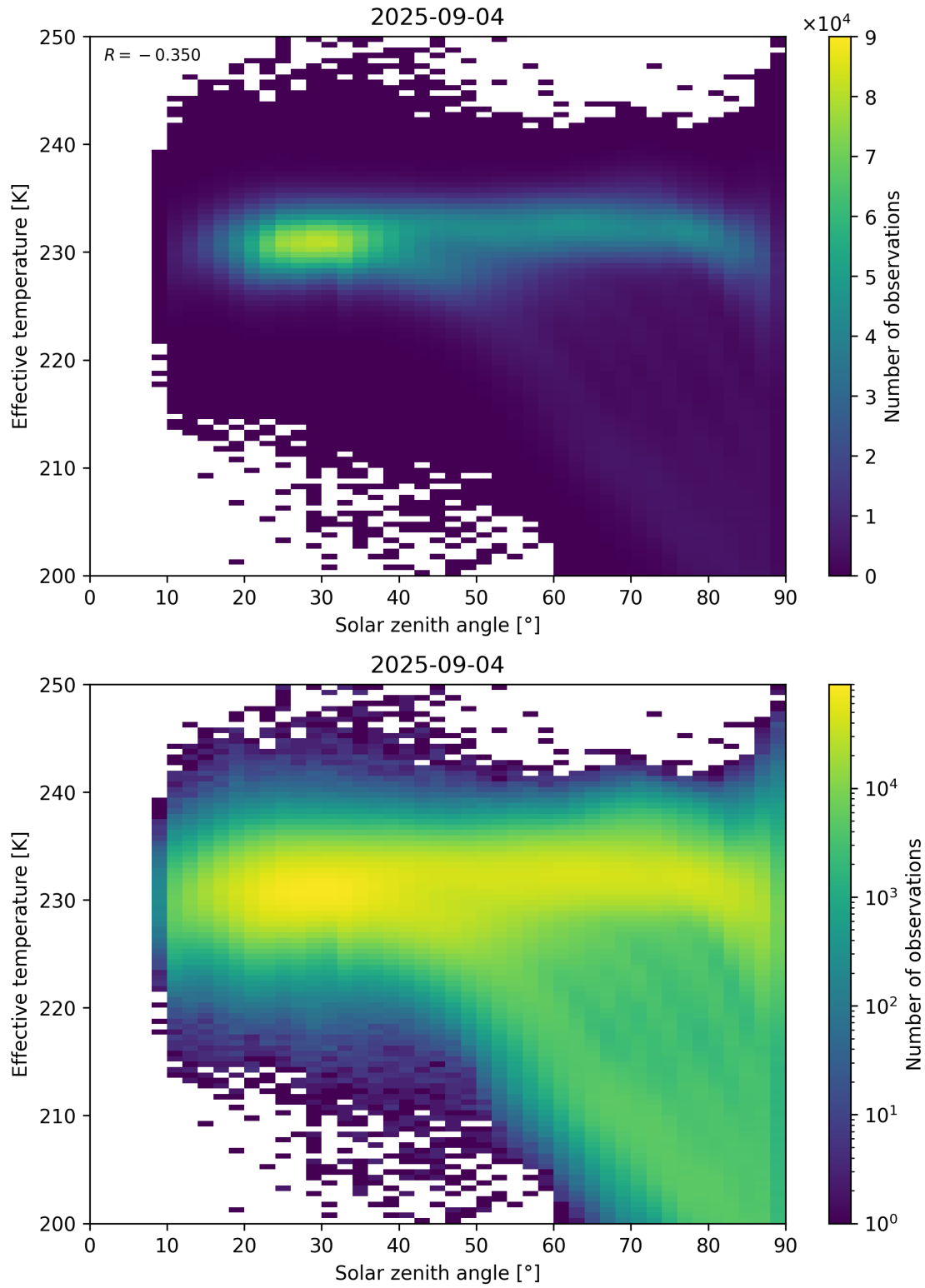
Figure 45: Scatter density plot of “Solar zenith angle” against “Effective temperature” for 2025-09-04 to 2025-09-05.
