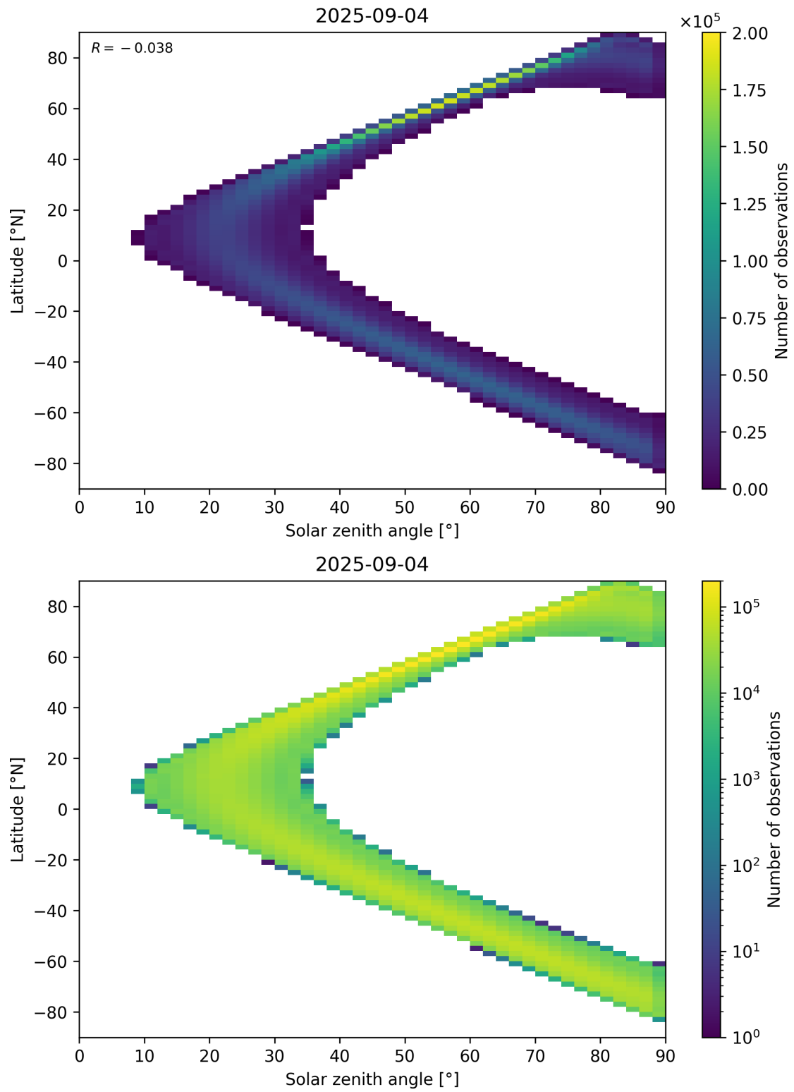
Figure 44: Scatter density plot of “Solar zenith angle” against “Latitude” for 2025-09-04 to 2025-09-05.
