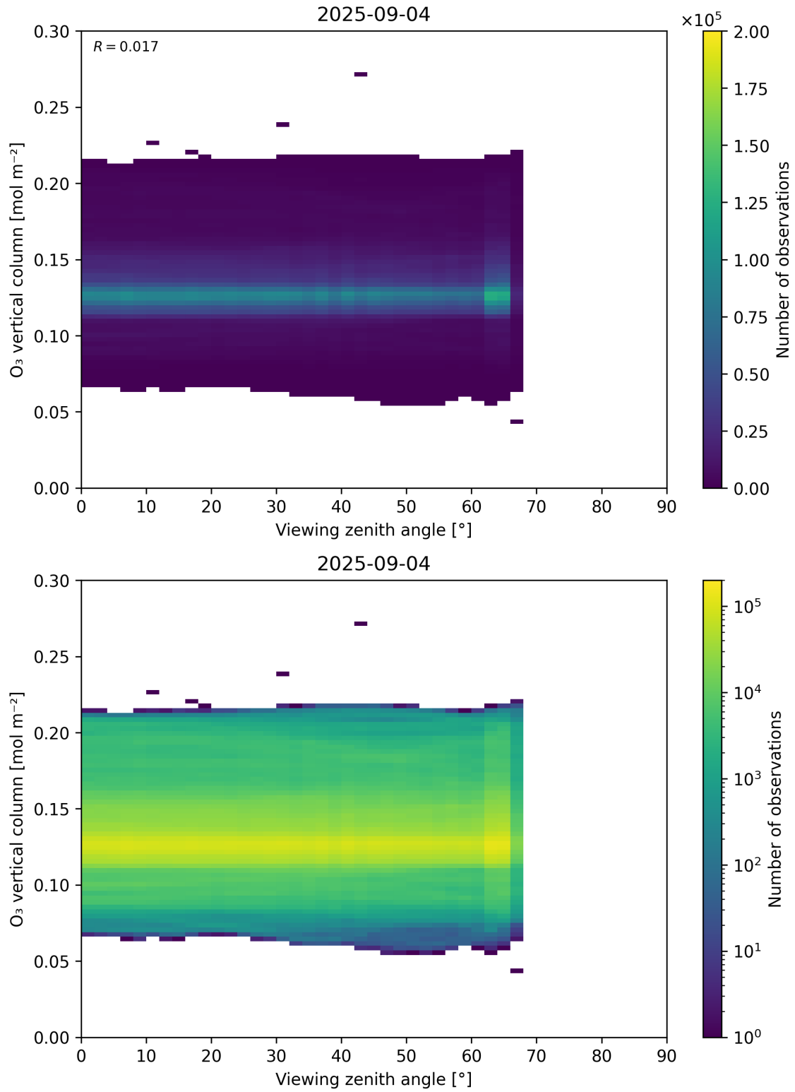
Figure 52: Scatter density plot of “Viewing zenith angle” against “O 3 vertical column” for 2025-09-04 to 2025-09-05.
