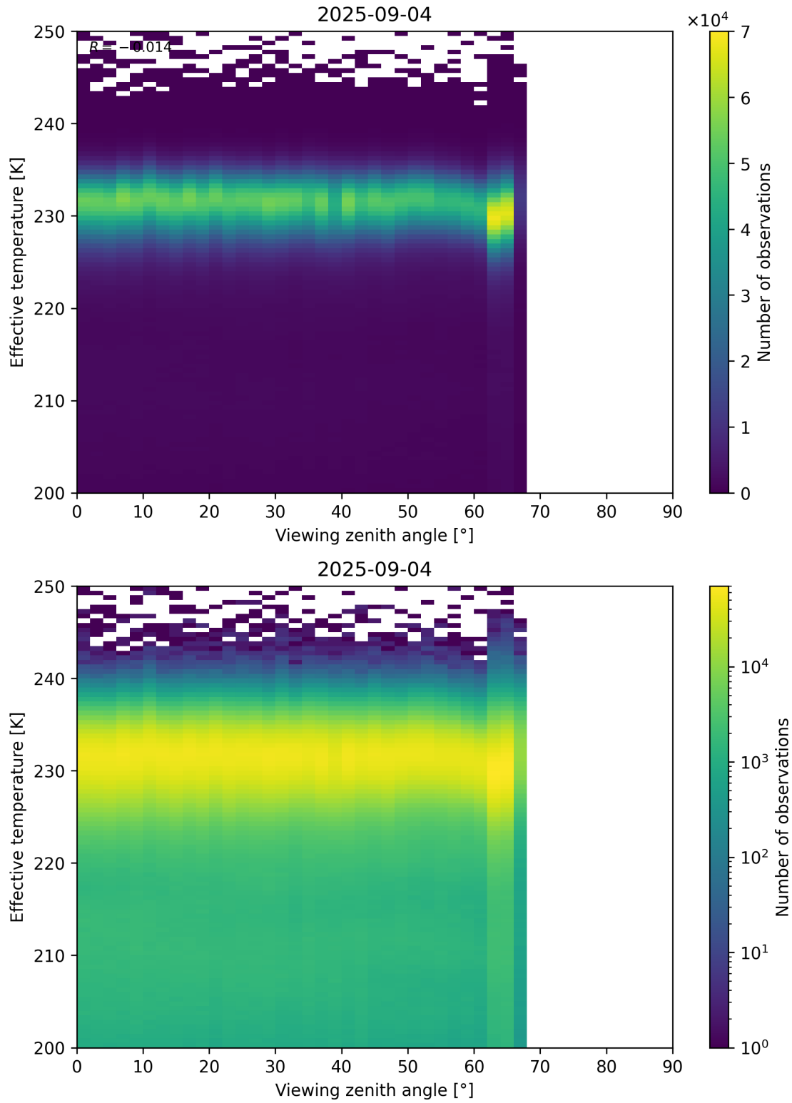
Figure 50: Scatter density plot of “Viewing zenith angle” against “Effective temperature” for 2025-09-04 to 2025-09-05.
