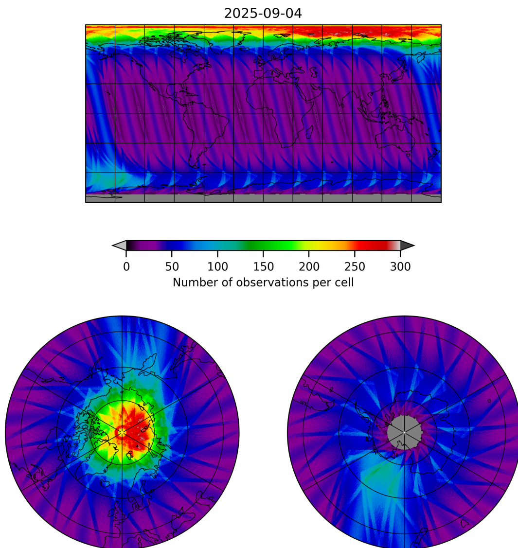
Figure 12: Map of the number of observations for 2025-09-04 to 2025-09-05
