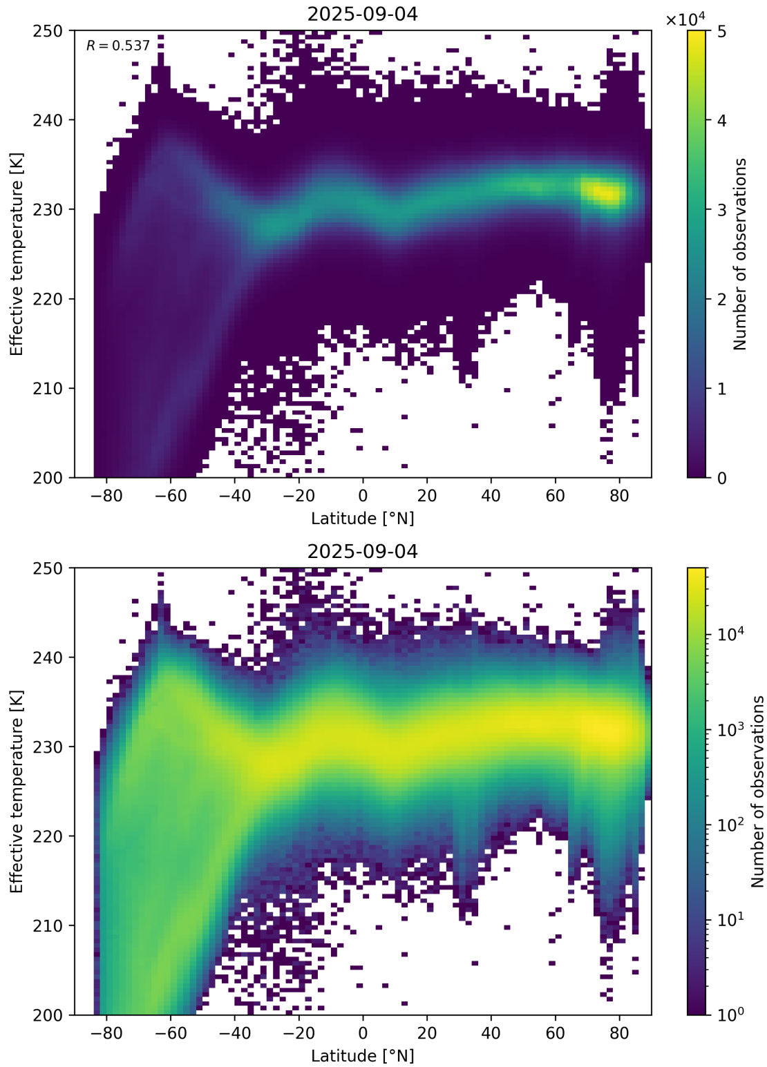
Figure 34: Scatter density plot of “Latitude” against “Effective temperature” for 2025-09-04 to 2025-09-05.
