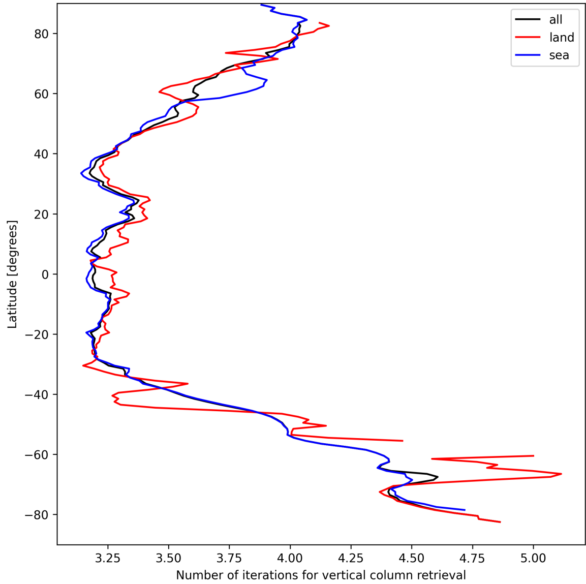
Figure 19: Zonal average of “Number of iterations for vertical column retrieval” for 2025-09-04 to 2025-09-05.
