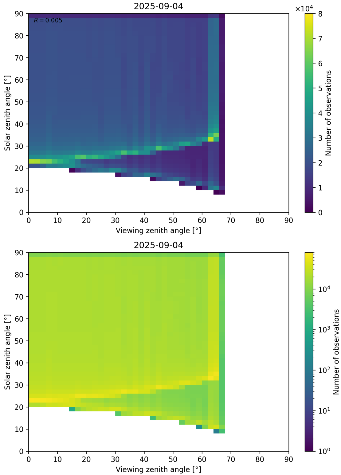
Figure 54: Scatter density plot of “Viewing zenith angle” against “Solar zenith angle” for 2025-09-04 to 2025-09-05.
