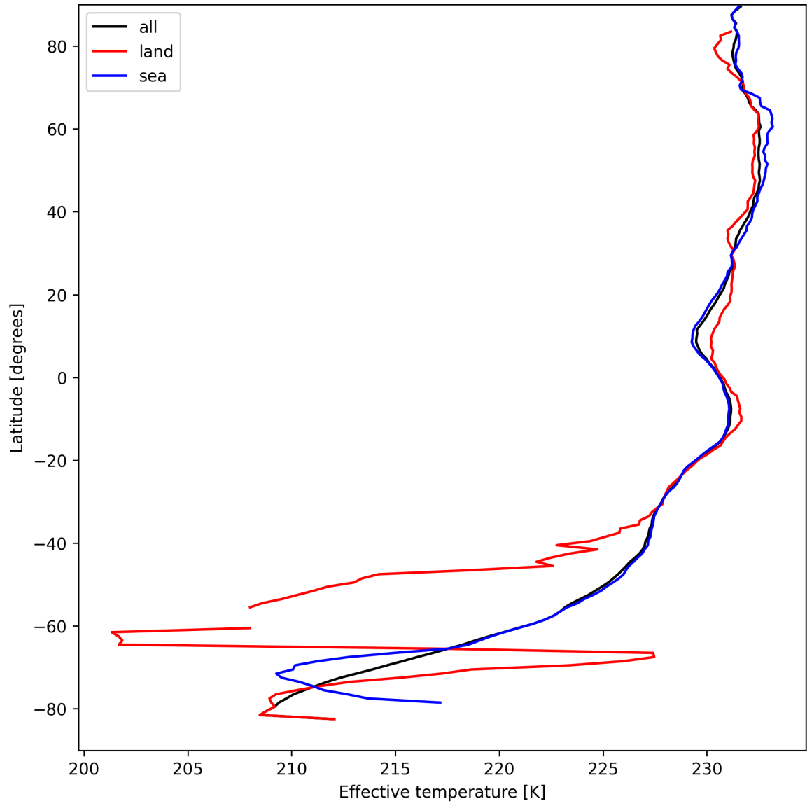
Figure 17: Zonal average of "Effective temperature" for 2025-09-04 to 2025-09-05.
