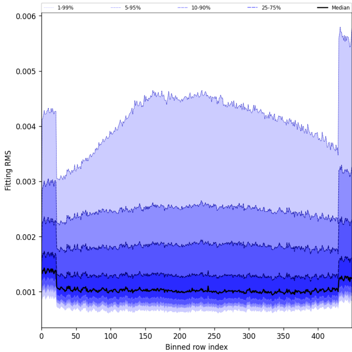
Figure 30: Along track statistics of “Fitting RMS” for 2025-09-04 to 2025-09-06
