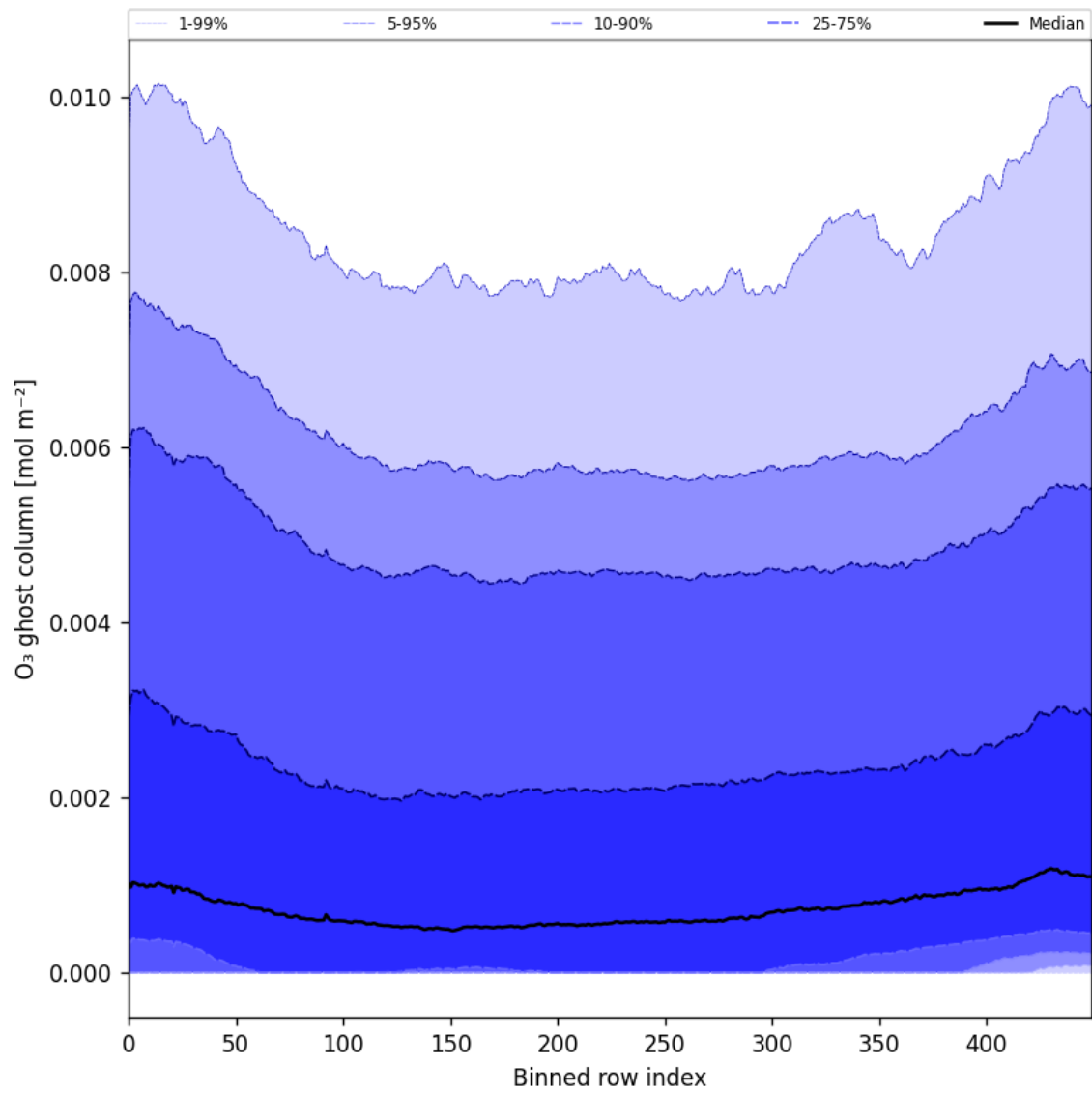
Figure 32: Along track statistics of “O 3 ghost column” for 2025-09-04 to 2025-09-06
