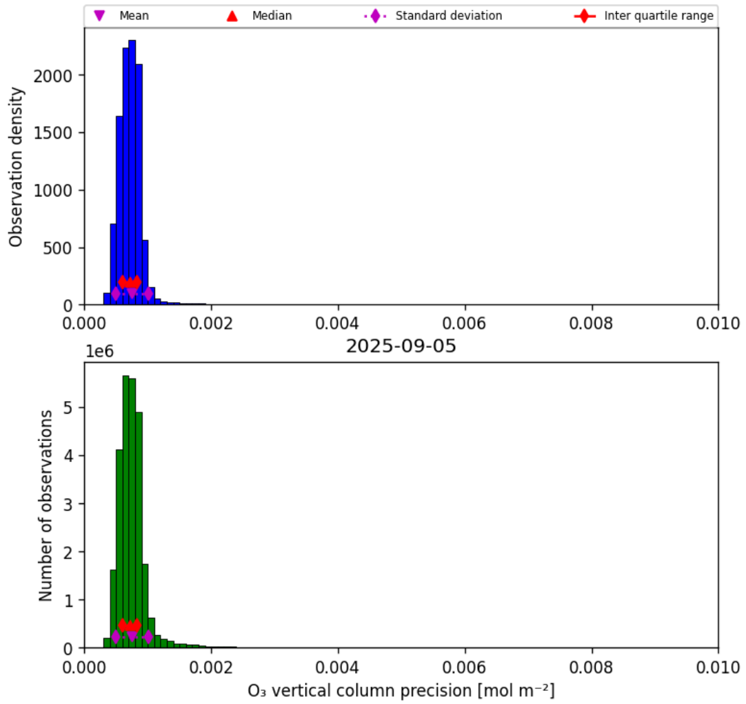
Figure 22: Histogram of “O 3 vertical column precision” for 2025-09-04 to 2025-09-06
