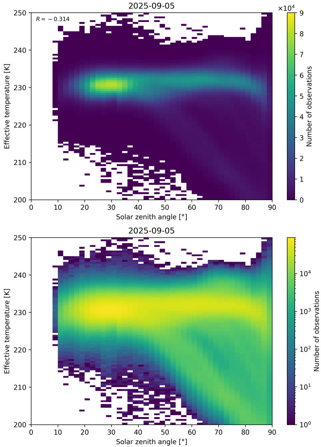
Figure 45: Scatter density plot of “Solar zenith angle” against “Effective temperature” for 2025-09-04 to 2025-09-06.
