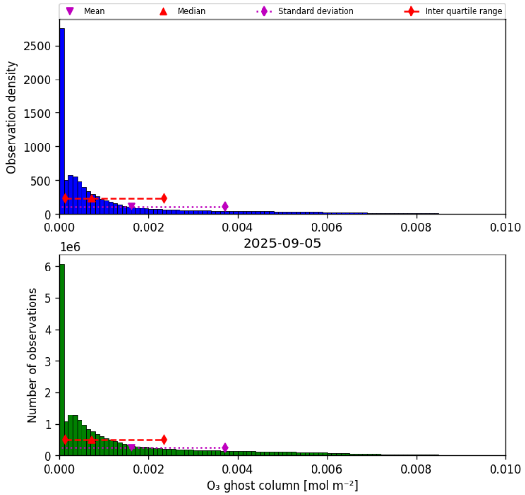
Figure 25: Histogram of “O 3 ghost column” for 2025-09-04 to 2025-09-06
