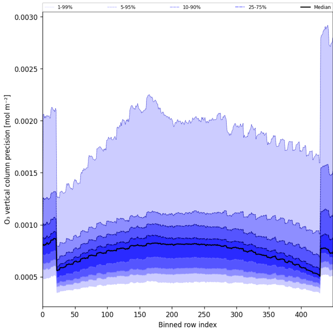
Figure 29: Along track statistics of “O 3 vertical column precision” for 2025-09-04 to 2025-09-06
