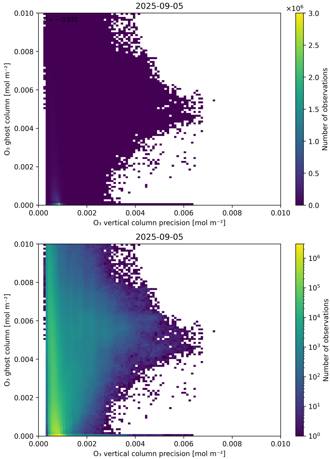
Figure 43: Scatter density plot of “O 3 vertical column precision” against “O 3 ghost column” for 2025-09-04 to 2025-09-06.
