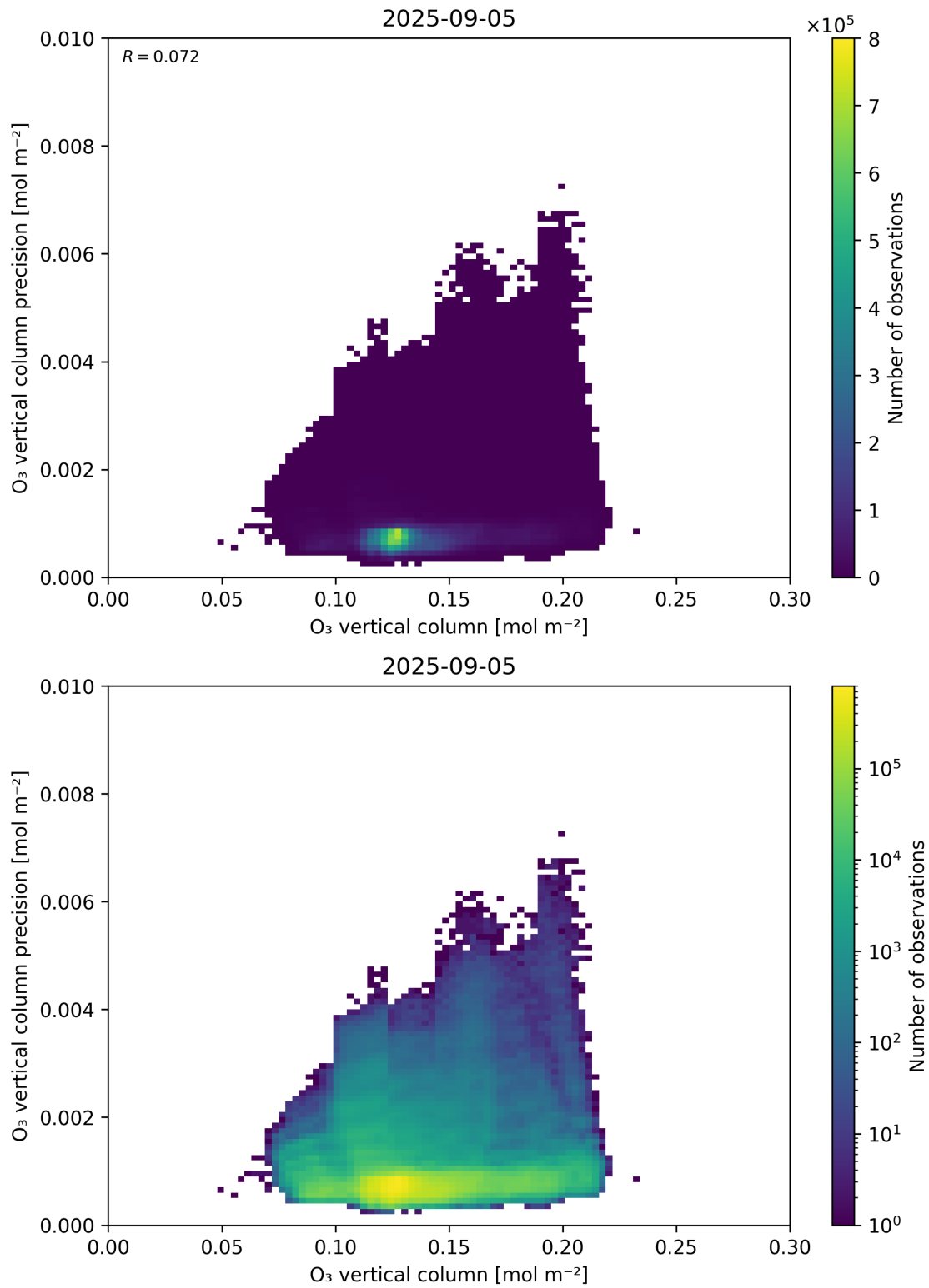
Figure 41: Scatter density plot of “O 3 vertical column” against “O 3 vertical column precision” for 2025-09-04 to 2025-09-06.
