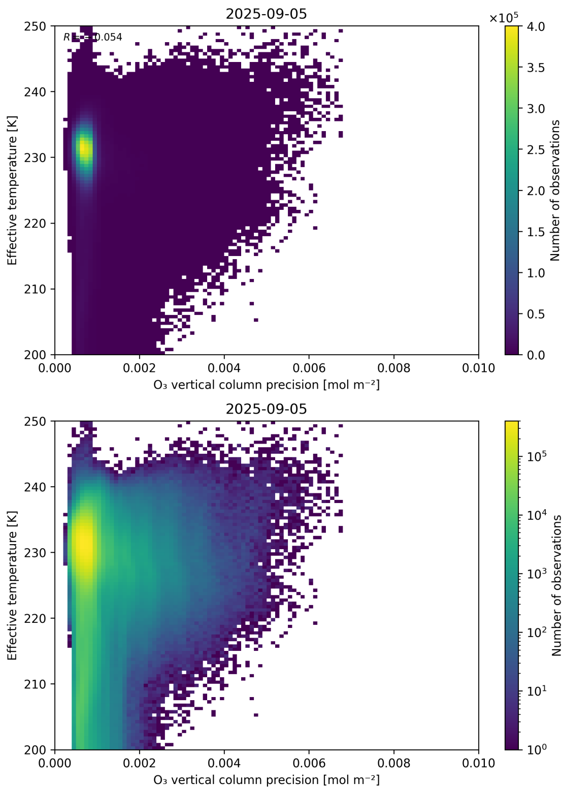
Figure 42: Scatter density plot of “O 3 vertical column precision” against “Effective temperature” for 2025-09-04 to 2025-09-06.
