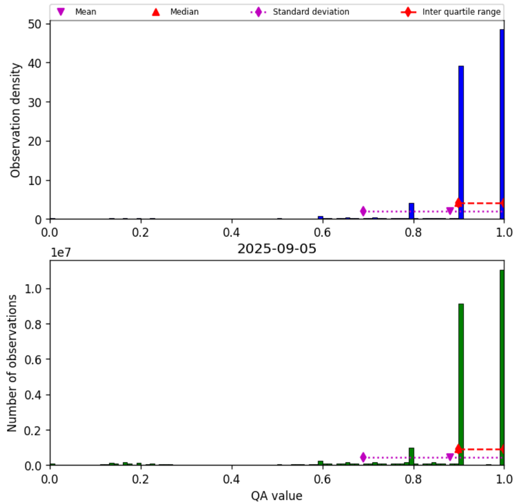
Figure 20: Histogram of “QA value” for 2025-09-04 to 2025-09-06
