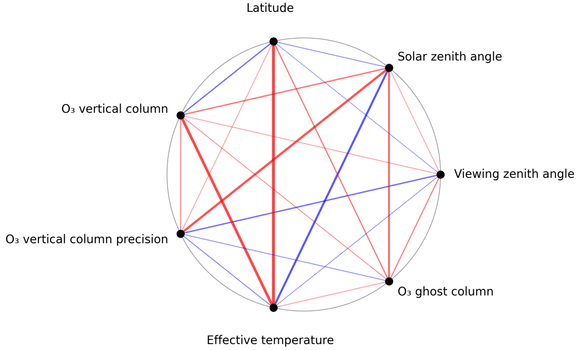
Figure 1: Map of correlation graph for 2025-09-04 to 2025-09-06.
