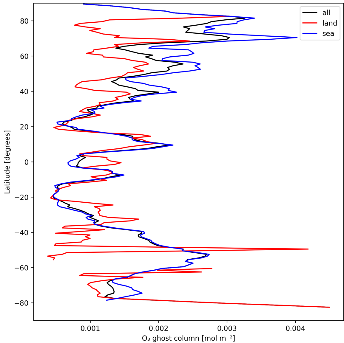
Figure 18: Zonal average of "O 3 ghost column" for 2025-09-04 to 2025-09-06.
