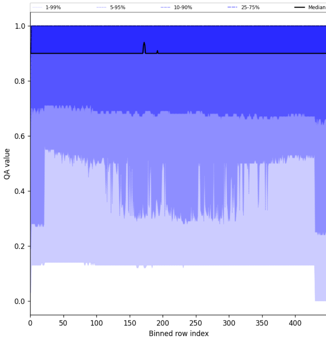
Figure 27: Along track statistics of “QA value” for 2025-09-04 to 2025-09-06
