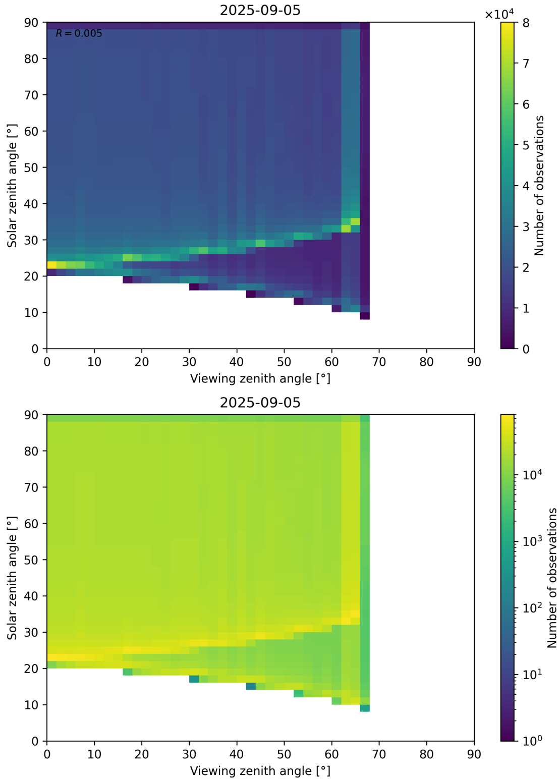
Figure 54: Scatter density plot of “Viewing zenith angle” against “Solar zenith angle” for 2025-09-04 to 2025-09-06.
