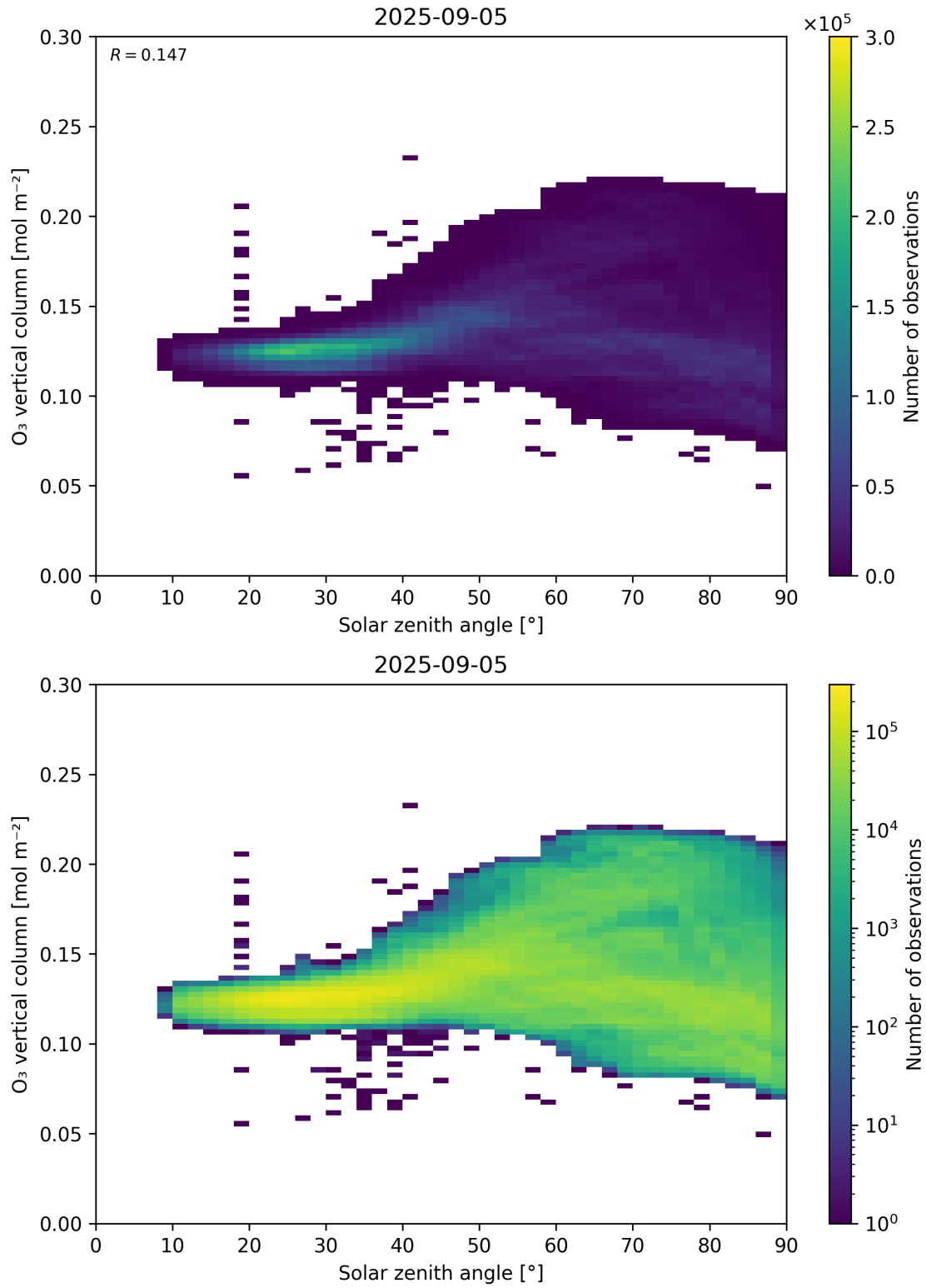
Figure 47: Scatter density plot of “Solar zenith angle” against “O 3 vertical column” for 2025-09-04 to 2025-09-06.
