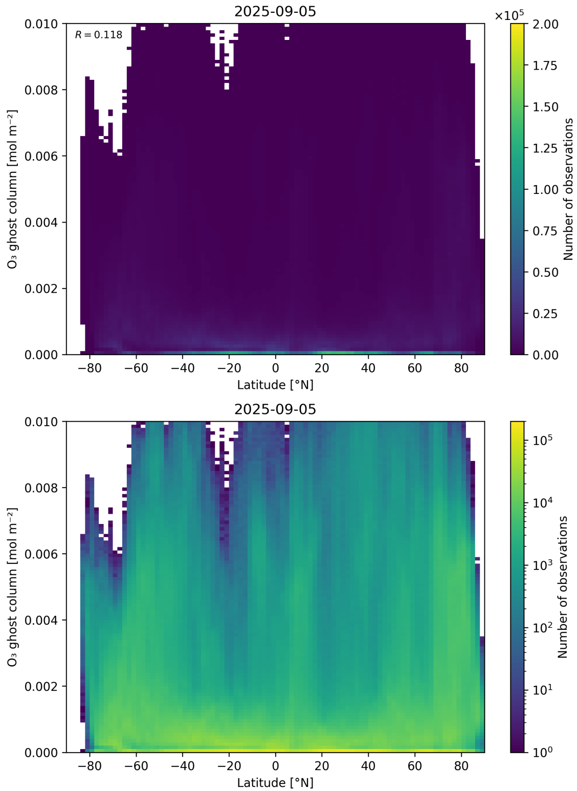
Figure 35: Scatter density plot of “Latitude” against “O 3 ghost column” for 2025-09-04 to 2025-09-06.
