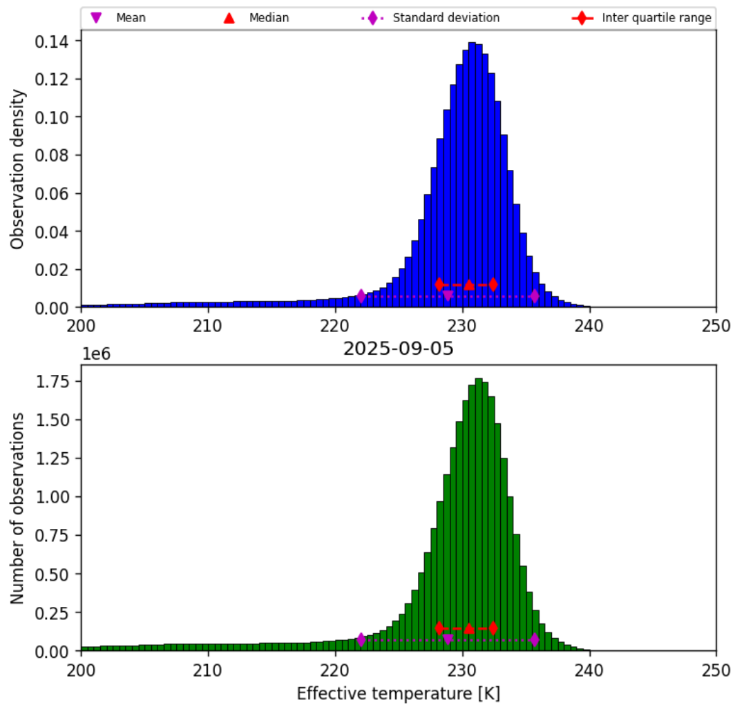
Figure 24: Histogram of “Effective temperature” for 2025-09-04 to 2025-09-06
