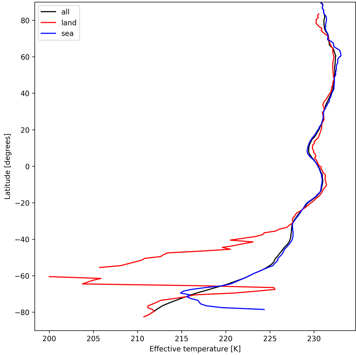
Figure 17: Zonal average of "Effective temperature" for 2025-09-04 to 2025-09-06.
