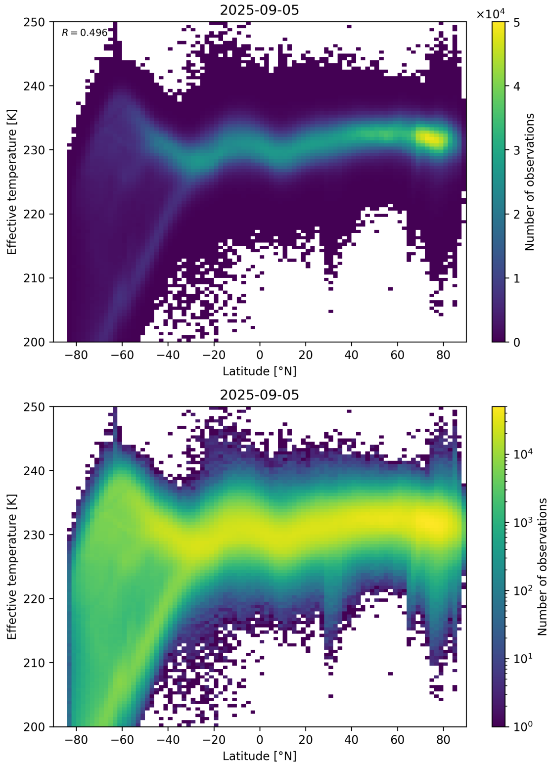
Figure 34: Scatter density plot of “Latitude” against “Effective temperature” for 2025-09-04 to 2025-09-06.
