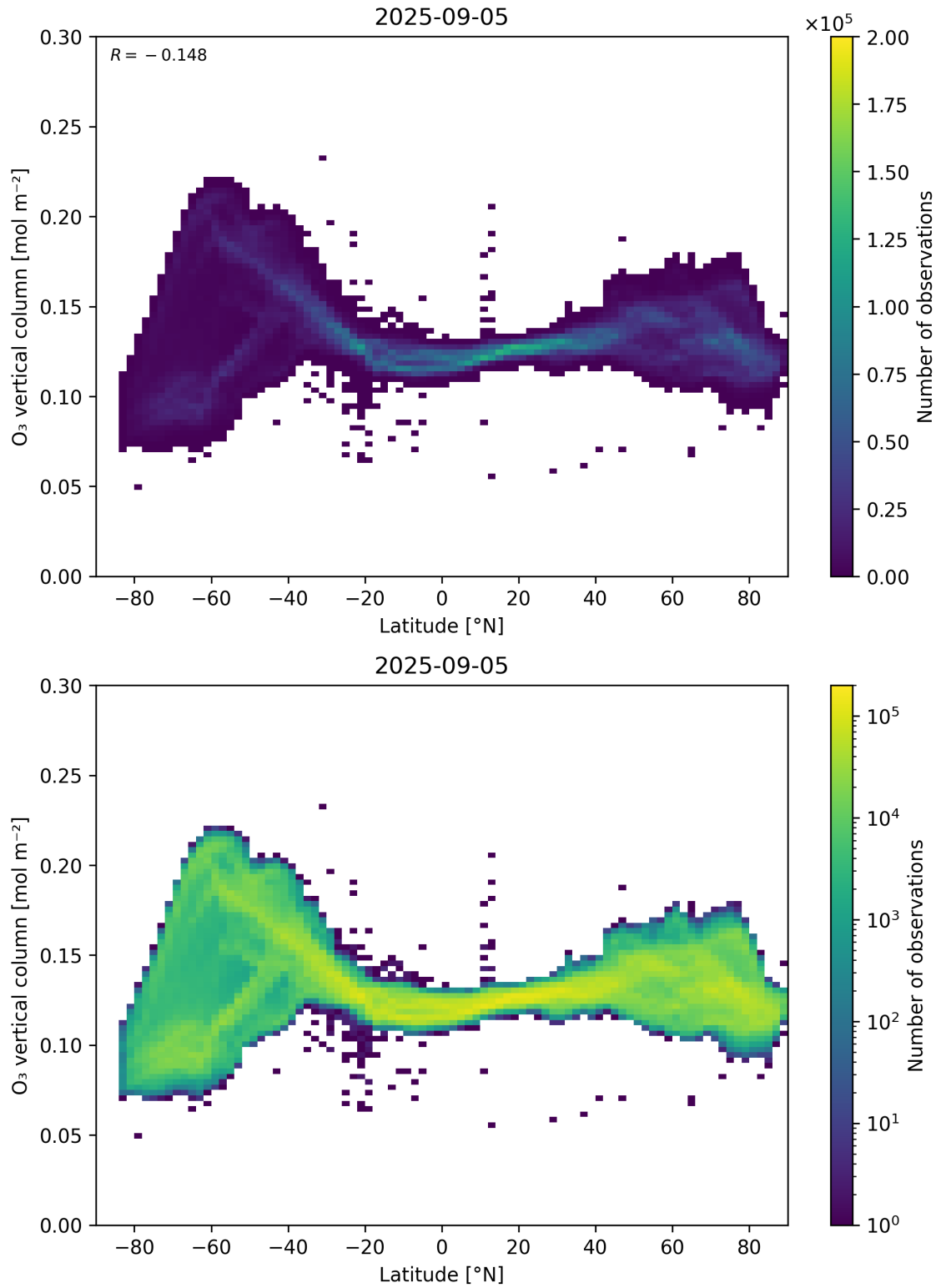
Figure 36: Scatter density plot of “Latitude” against “O 3 vertical column” for 2025-09-04 to 2025-09-06.
