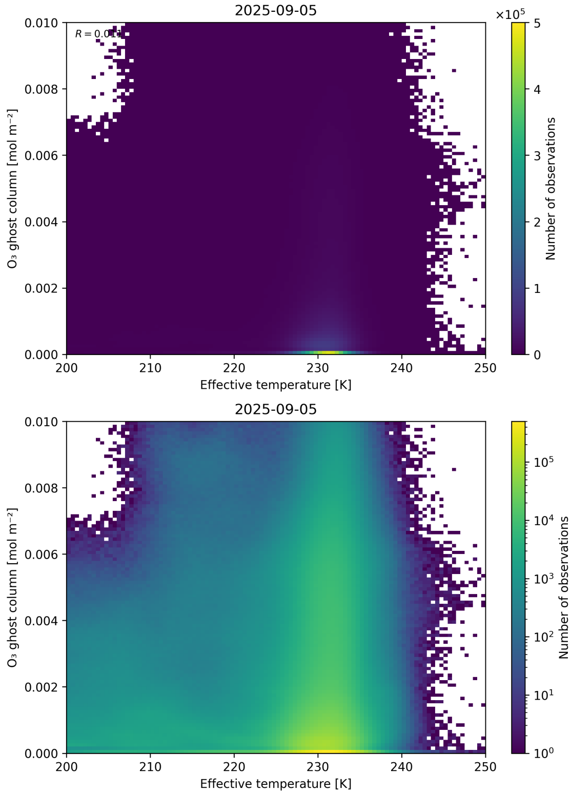
Figure 38: Scatter density plot of “Effective temperature” against “O 3 ghost column” for 2025-09-04 to 2025-09-06.
