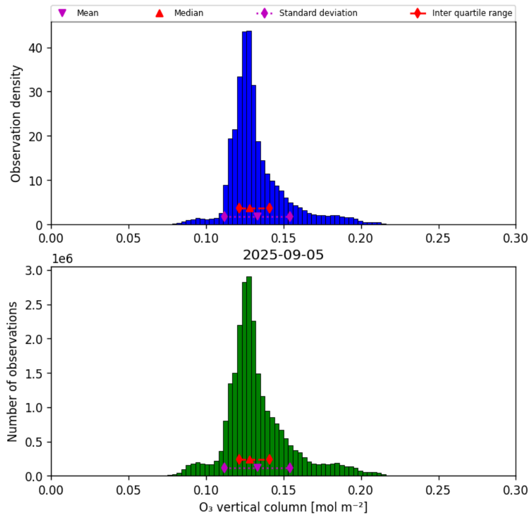
Figure 21: Histogram of “O 3 vertical column” for 2025-09-04 to 2025-09-06
