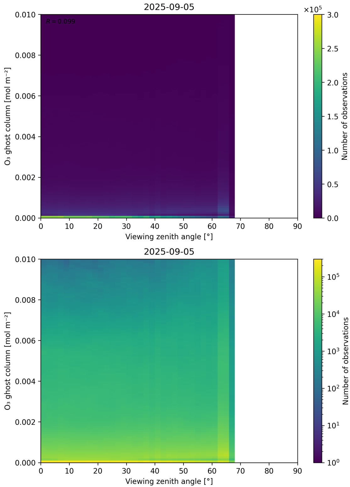
Figure 51: Scatter density plot of “Viewing zenith angle” against “O 3 ghost column” for 2025-09-04 to 2025-09-06.
