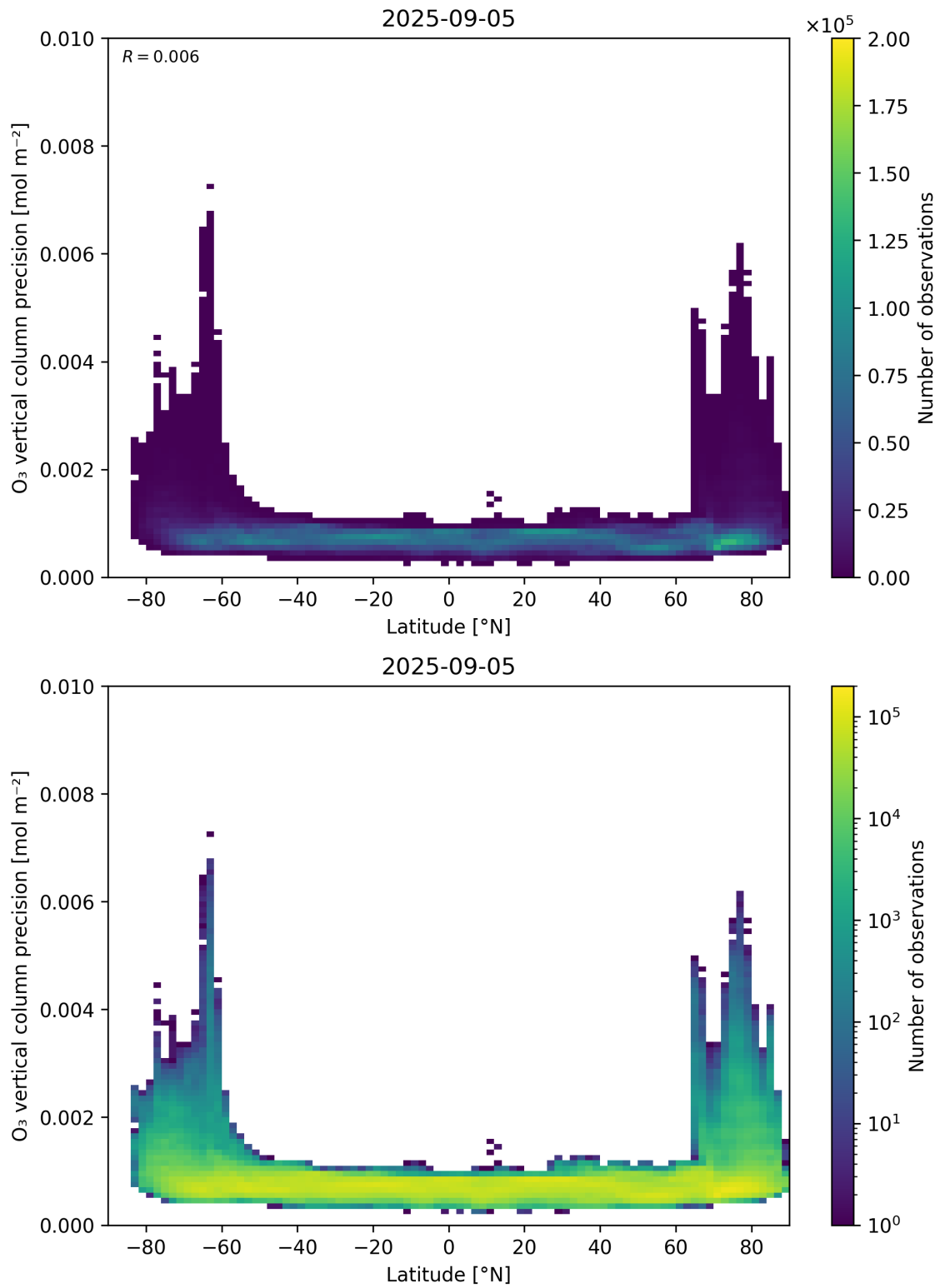
Figure 37: Scatter density plot of “Latitude” against “O 3 vertical column precision” for 2025-09-04 to 2025-09-06.
