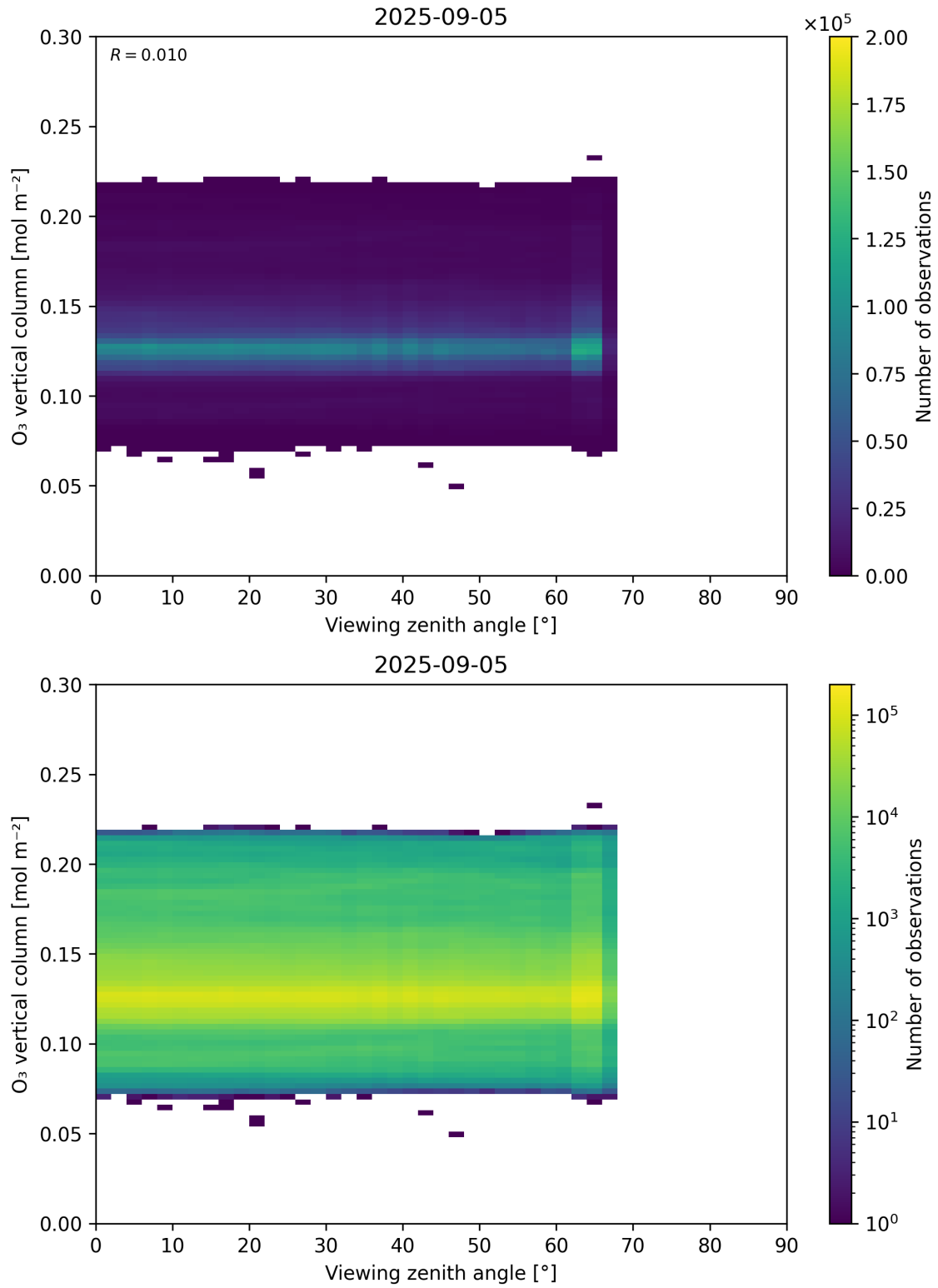
Figure 52: Scatter density plot of “Viewing zenith angle” against “O 3 vertical column” for 2025-09-04 to 2025-09-06.
