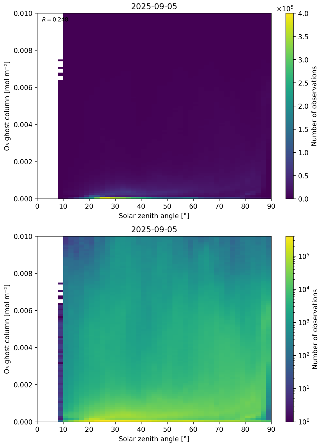
Figure 46: Scatter density plot of “Solar zenith angle” against “O 3 ghost column” for 2025-09-04 to 2025-09-06.
