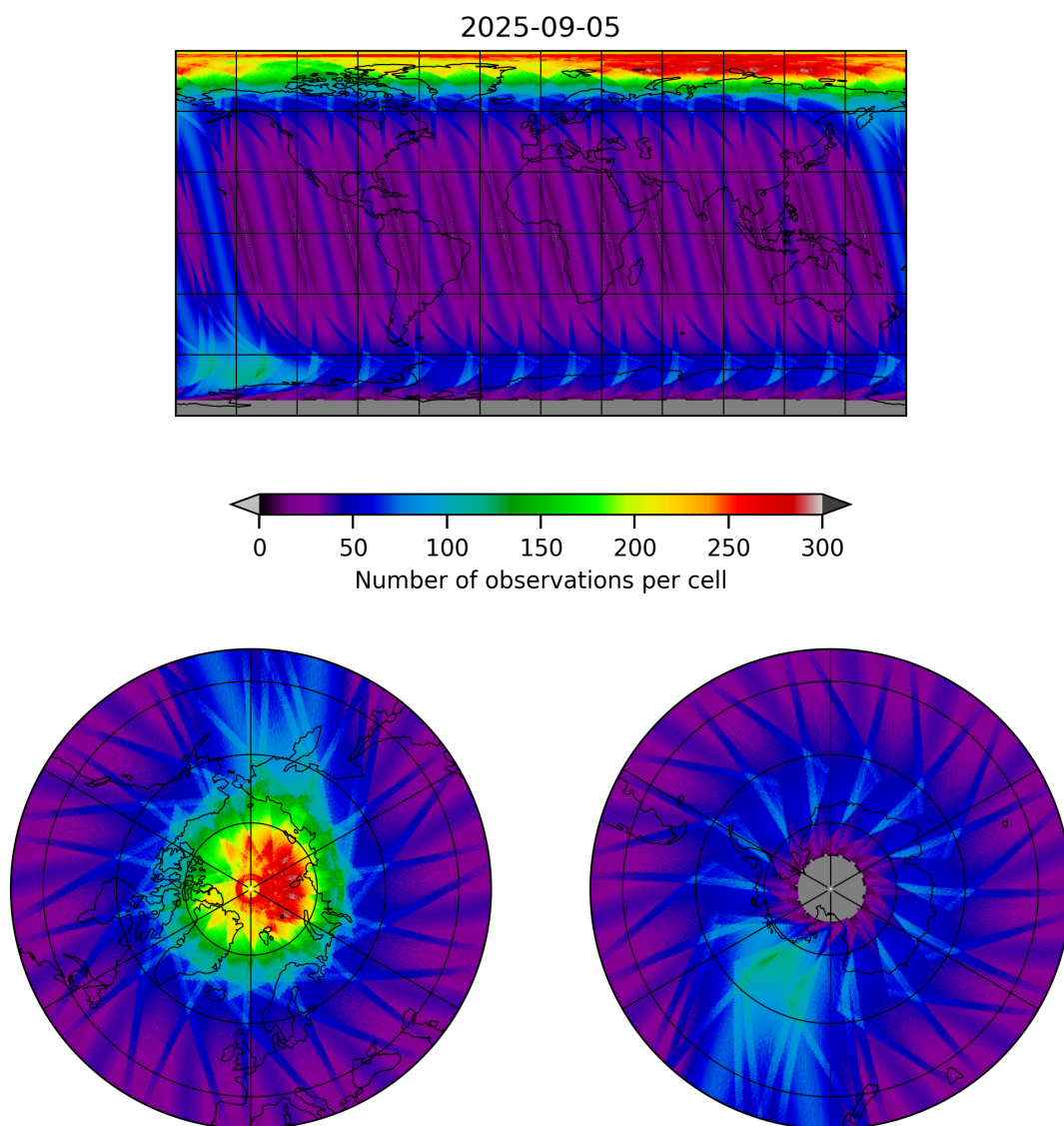
Figure 12: Map of the number of observations for 2025-09-04 to 2025-09-06
