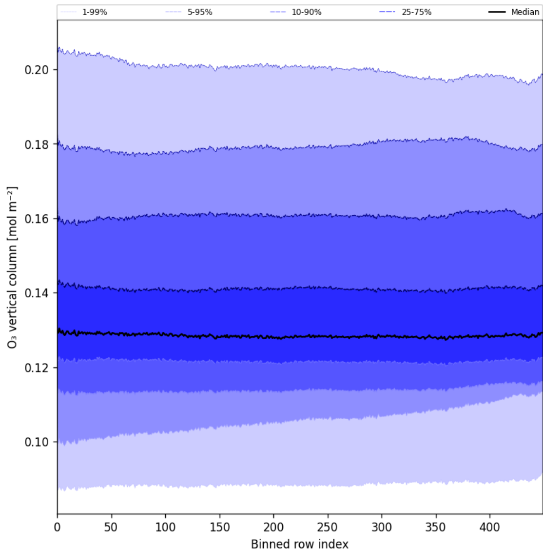
Figure 28: Along track statistics of “O 3 vertical column” for 2025-09-04 to 2025-09-06
