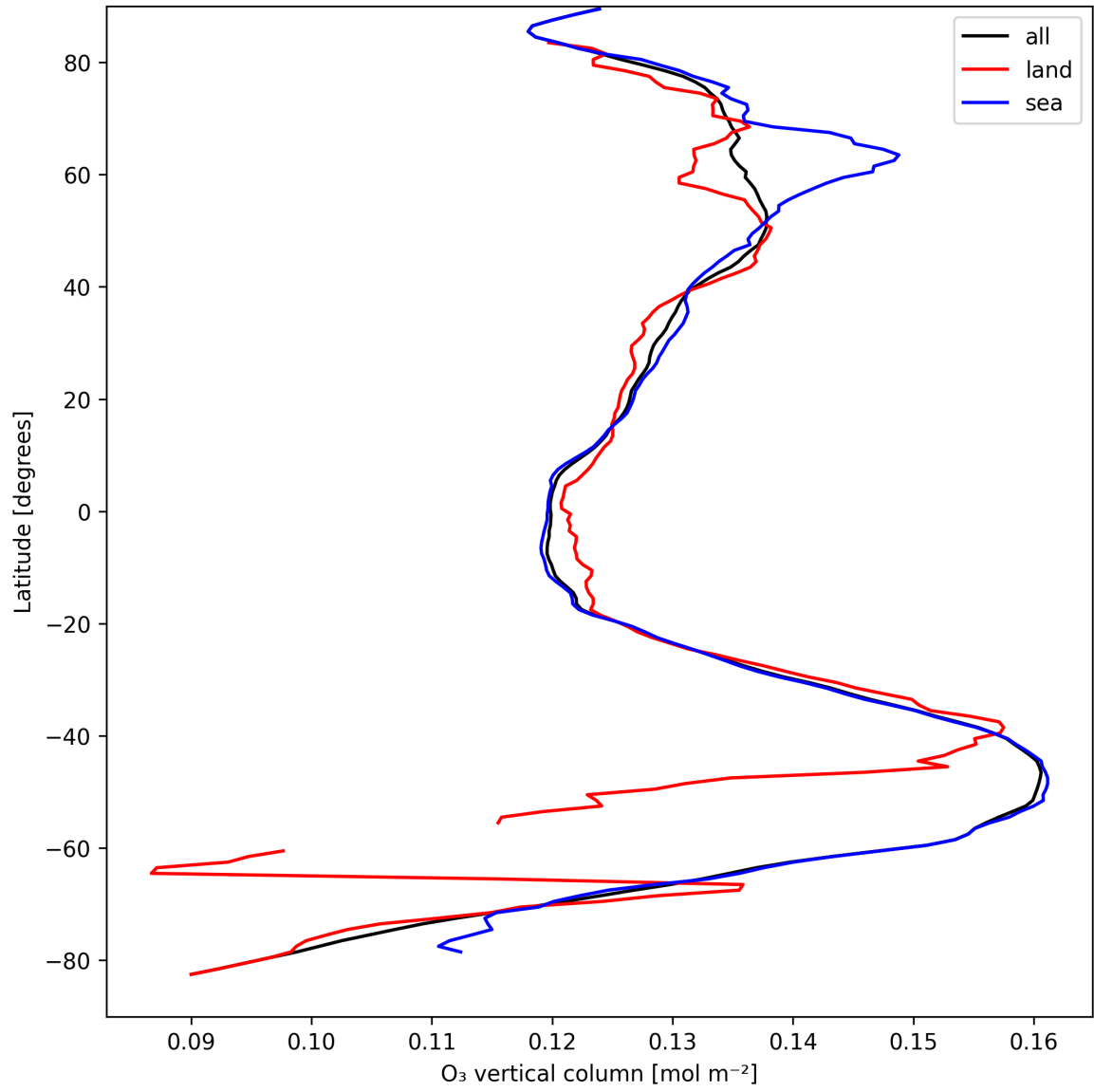
Figure 14: Zonal average of “O 3 vertical column” for 2025-09-04 to 2025-09-06.
