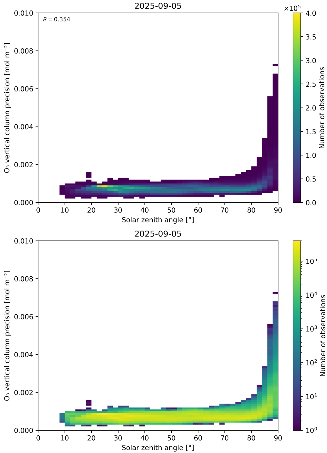
Figure 48: Scatter density plot of “Solar zenith angle” against “O 3 vertical column precision” for 2025-09-04 to 2025-09-06.
