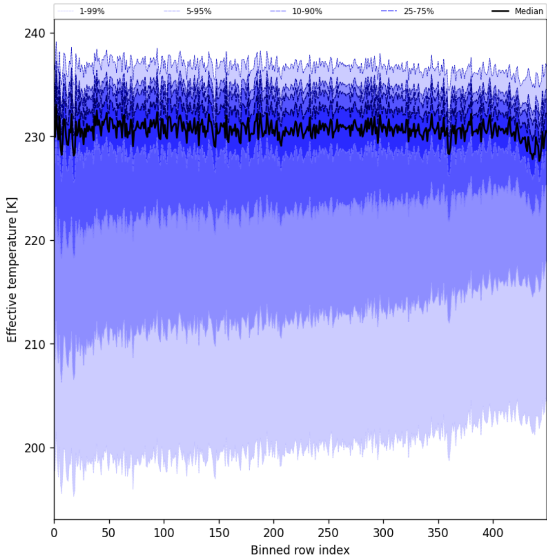
Figure 31: Along track statistics of “Effective temperature” for 2025-09-04 to 2025-09-06
