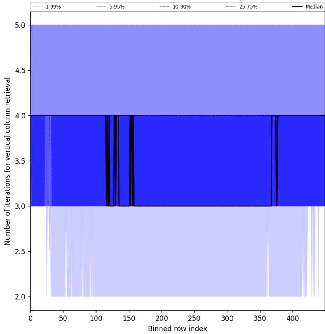
Figure 33: Along track statistics of “Number of iterations for vertical column retrieval” for 2025-09-04 to 2025-09-06
