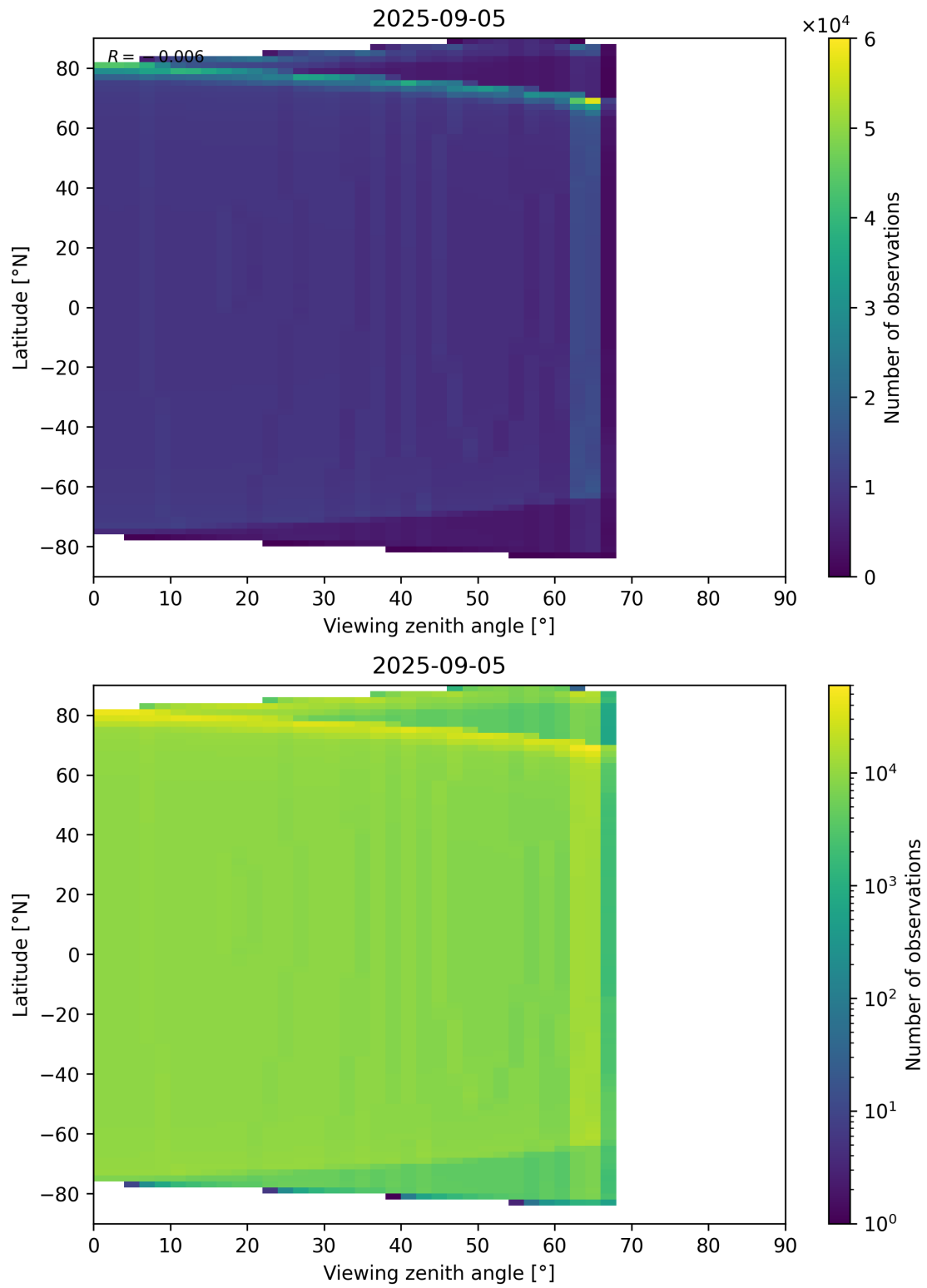
Figure 49: Scatter density plot of “Viewing zenith angle” against “Latitude” for 2025-09-04 to 2025-09-06.
