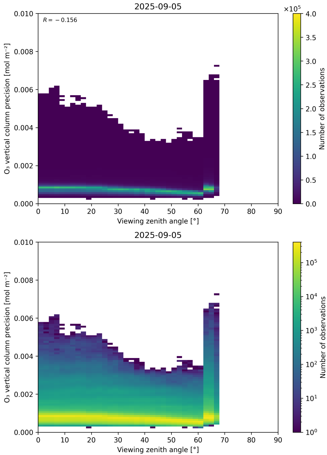
Figure 53: Scatter density plot of “Viewing zenith angle” against “O 3 vertical column precision” for 2025-09-04 to 2025-09-06.
