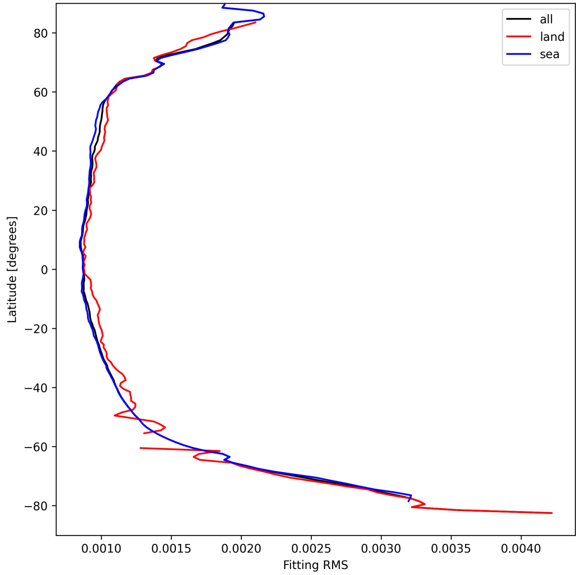
Figure 16: Zonal average of “Fitting RMS” for 2025-09-04 to 2025-09-06.
