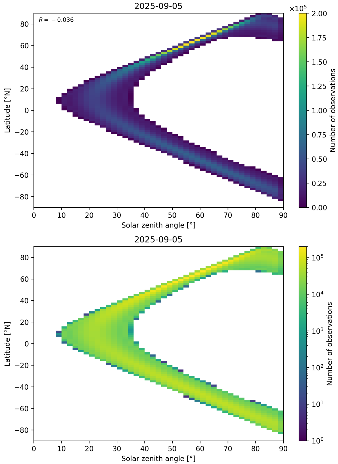
Figure 44: Scatter density plot of “Solar zenith angle” against “Latitude” for 2025-09-04 to 2025-09-06.
