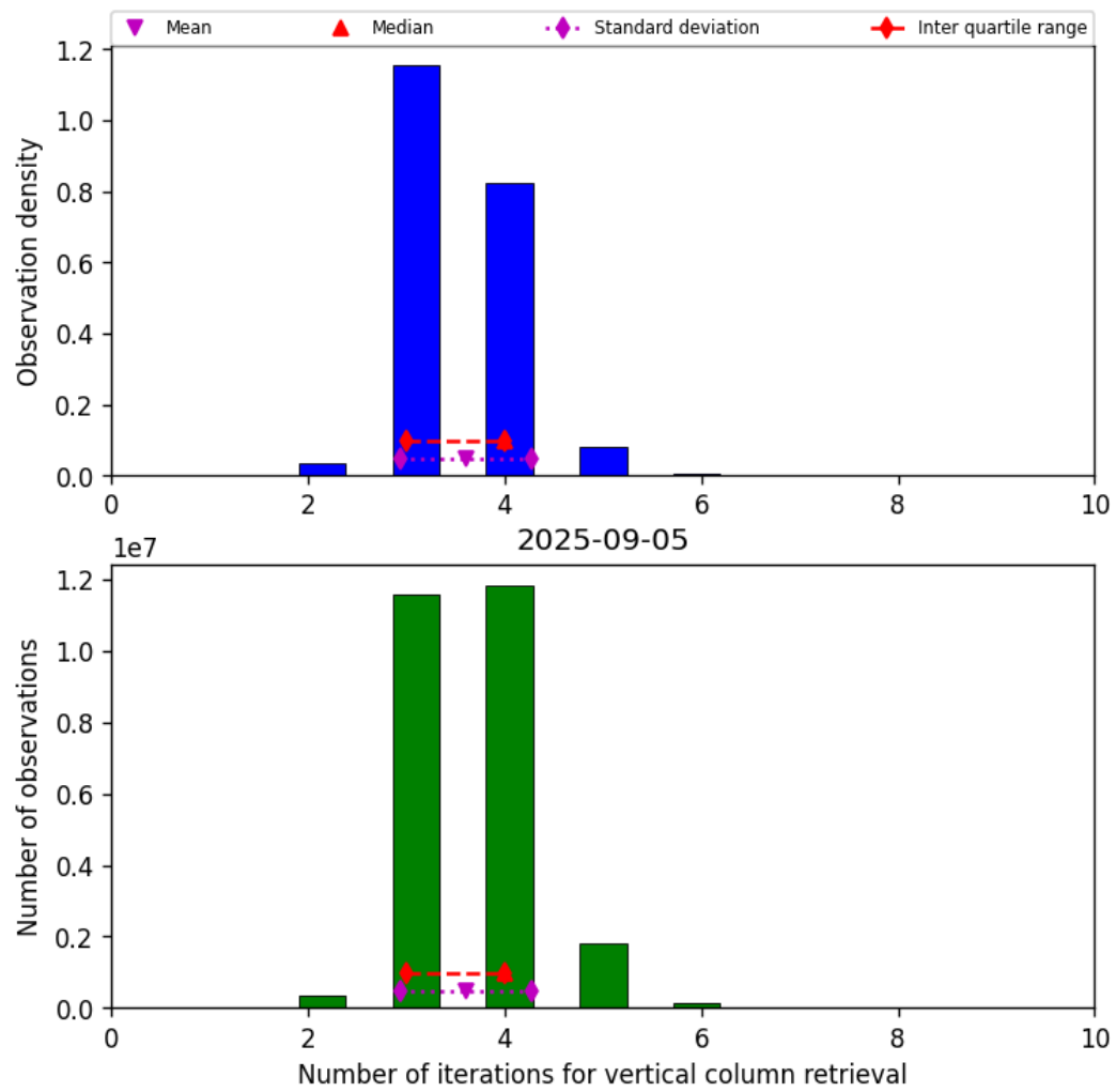
Figure 26: Histogram of “Number of iterations for vertical column retrieval” for 2025-09-04 to 2025-09-06
