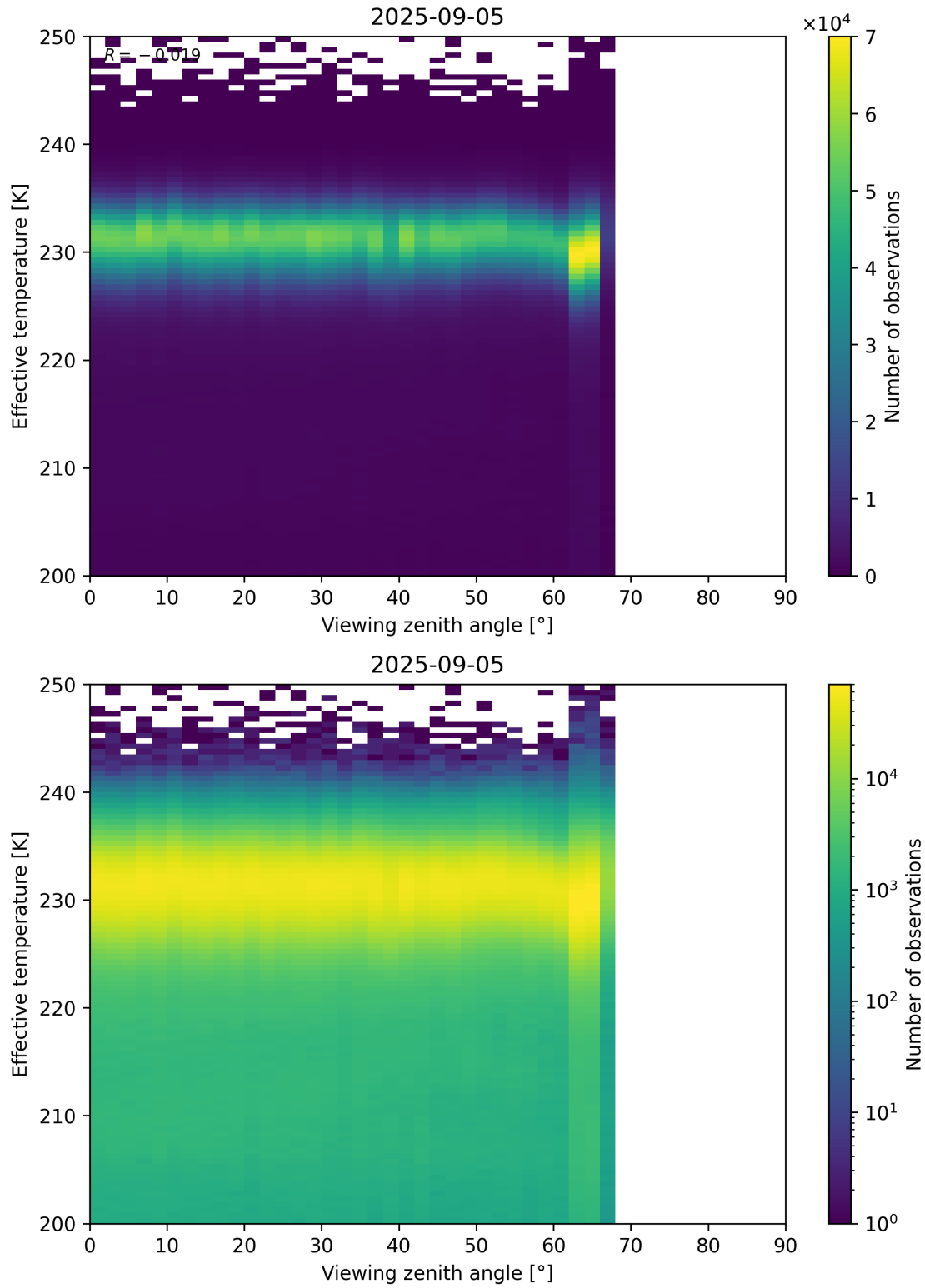
Figure 50: Scatter density plot of “Viewing zenith angle” against “Effective temperature” for 2025-09-04 to 2025-09-06.
