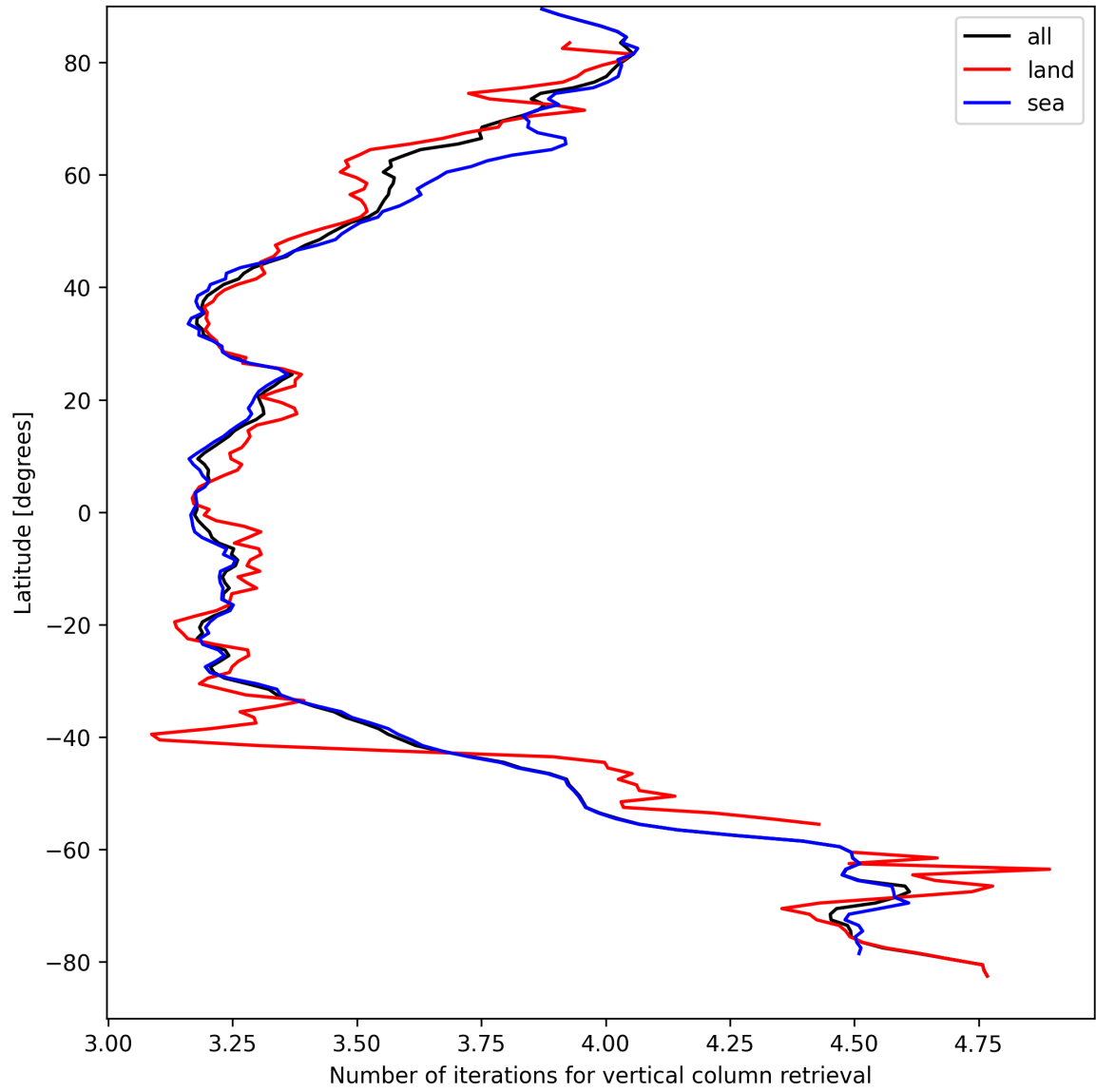
Figure 19: Zonal average of “Number of iterations for vertical column retrieval” for 2025-09-04 to 2025-09-06.
