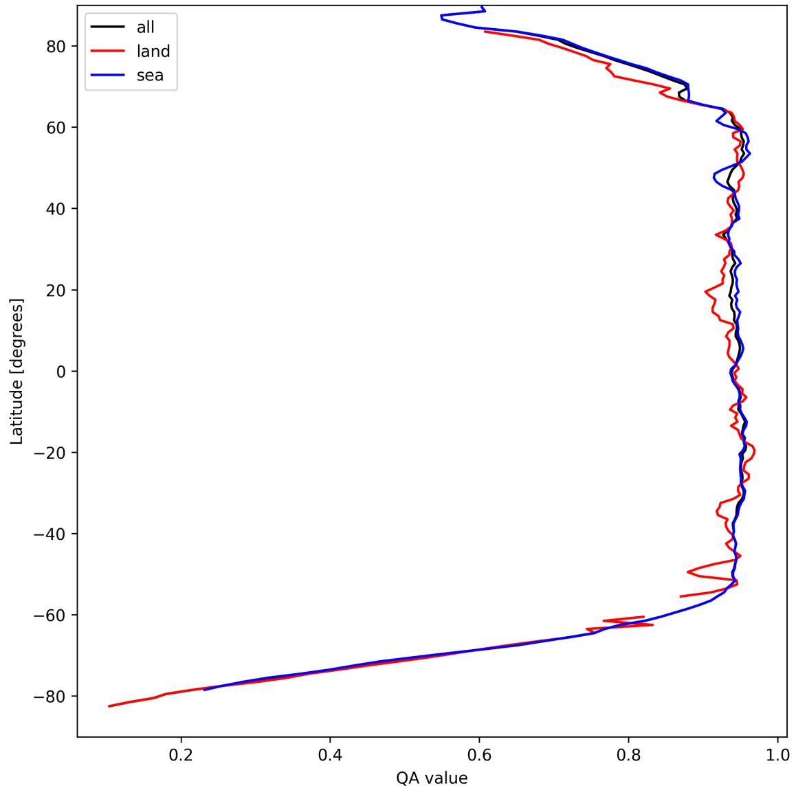
Figure 13: Zonal average of “QA value” for 2025-09-04 to 2025-09-06.
