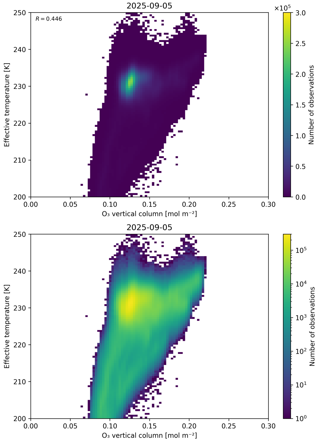
Figure 39: Scatter density plot of “O 3 vertical column” against “Effective temperature” for 2025-09-04 to 2025-09-06.
