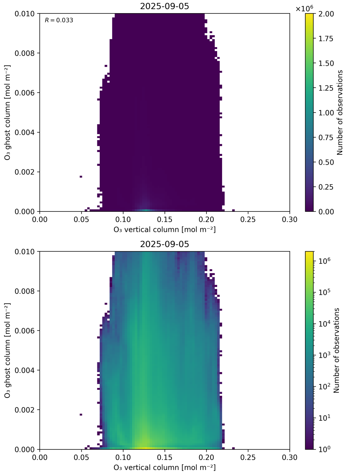
Figure 40: Scatter density plot of “O 3 vertical column” against “O 3 ghost column” for 2025-09-04 to 2025-09-06.
