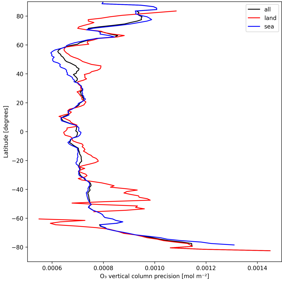
Figure 15: Zonal average of “O 3 vertical column precision” for 2025-09-04 to 2025-09-06.
