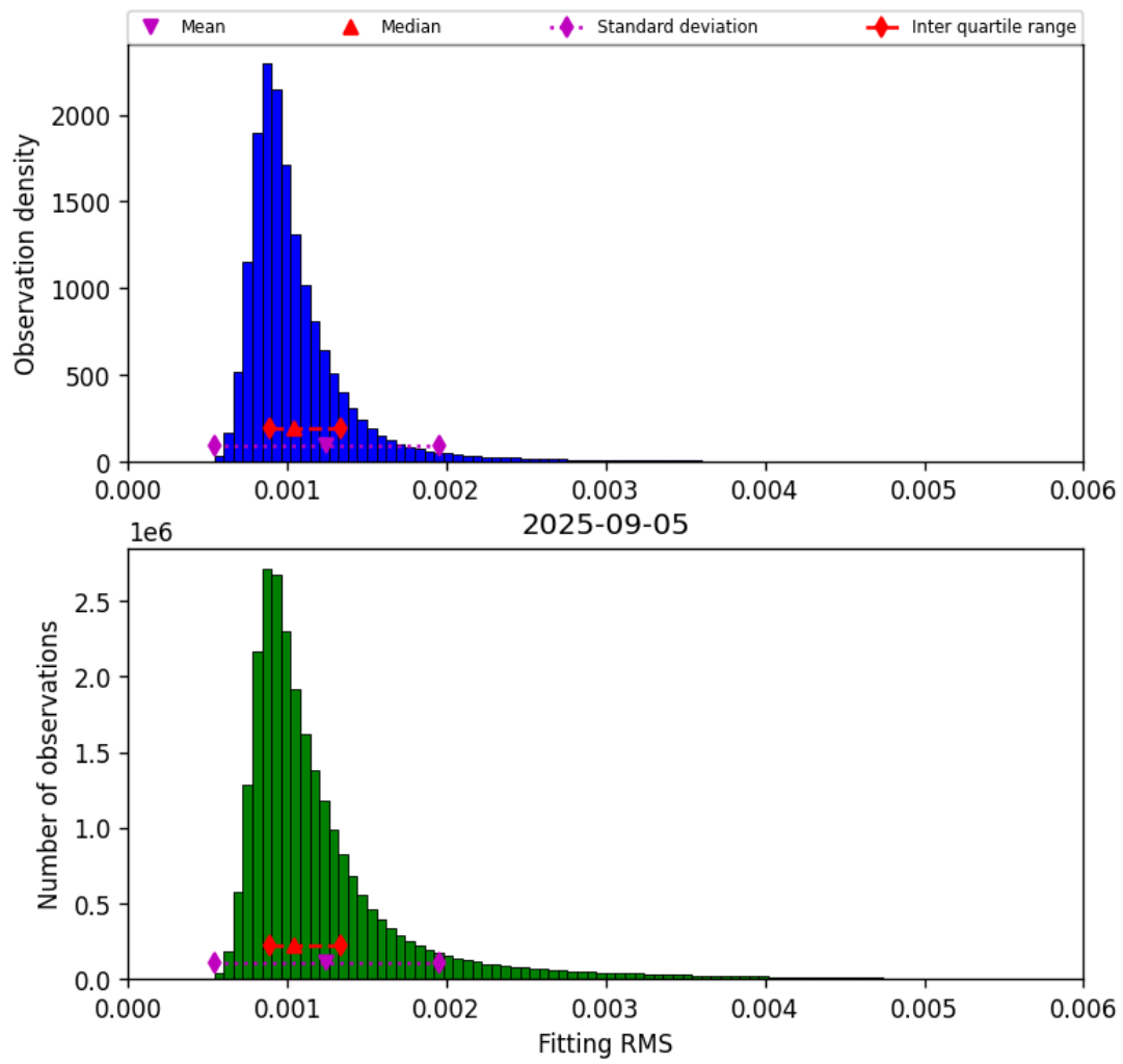
Figure 23: Histogram of “Fitting RMS” for 2025-09-04 to 2025-09-06
