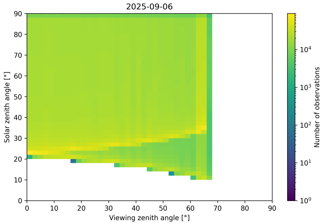
Figure 54: Scatter density plot of “Viewing zenith angle” against “Solar zenith angle” for 2025-09-05 to 2025-09-07.
