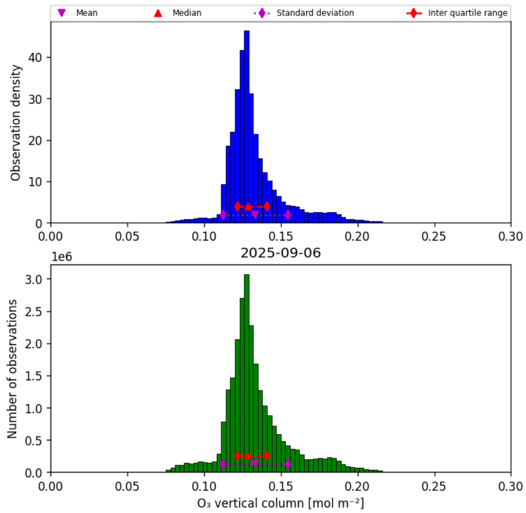
Figure 21: Histogram of “O 3 vertical column” for 2025-09-05 to 2025-09-07
