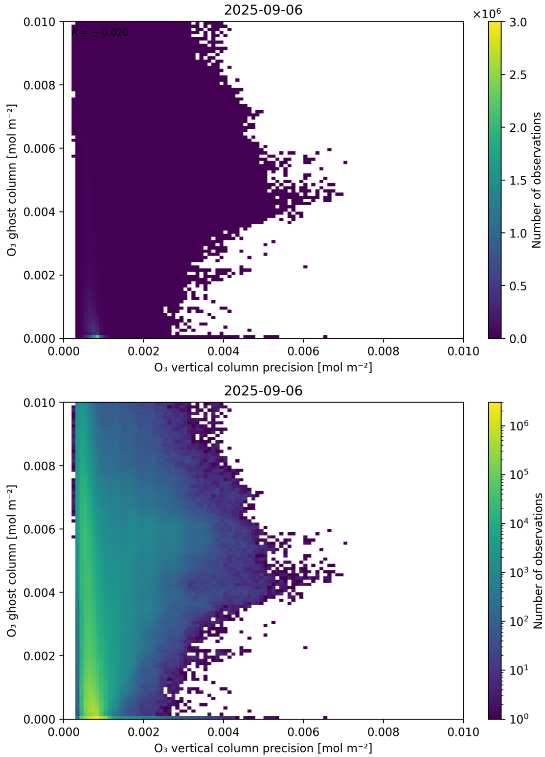
Figure 43: Scatter density plot of “ \text{O}_3 vertical column precision” against “ \text{O}_3 ghost column” for 2025-09-05 to 2025-09-07.
