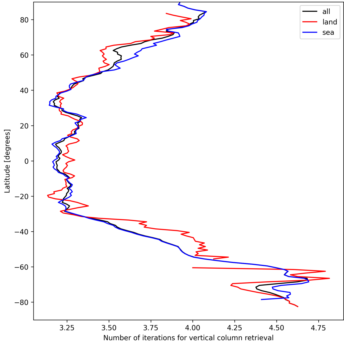
Figure 19: Zonal average of “Number of iterations for vertical column retrieval” for 2025-09-05 to 2025-09-07.
