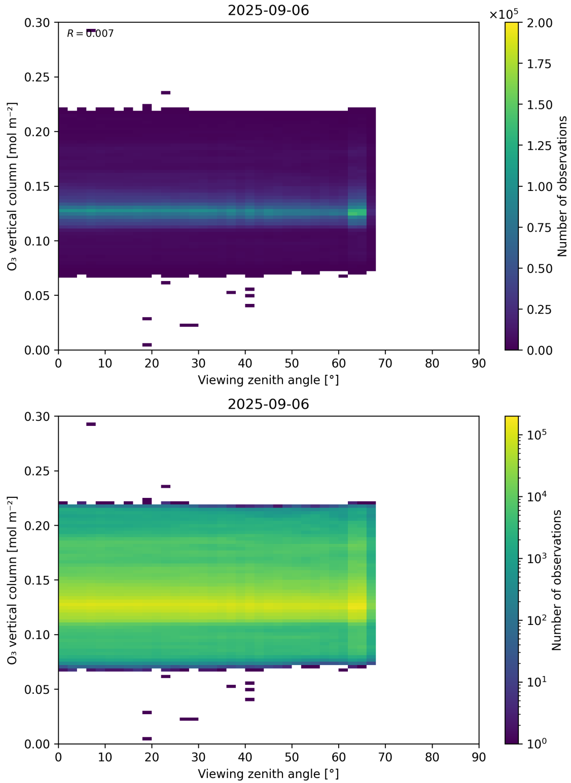
Figure 52: Scatter density plot of “Viewing zenith angle” against “O 3 vertical column” for 2025-09-05 to 2025-09-07.
