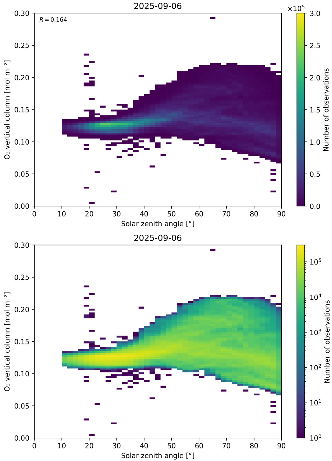
Figure 47: Scatter density plot of “Solar zenith angle” against “O 3 vertical column” for 2025-09-05 to 2025-09-07.
