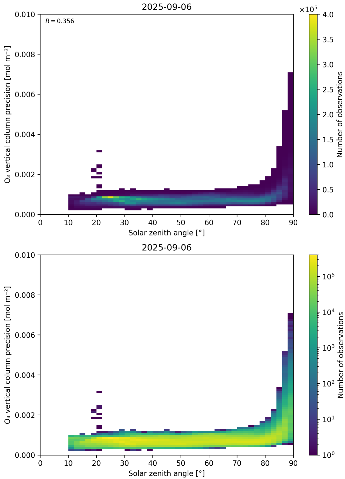
Figure 48: Scatter density plot of “Solar zenith angle” against “O 3 vertical column precision” for 2025-09-05 to 2025-09-07.
