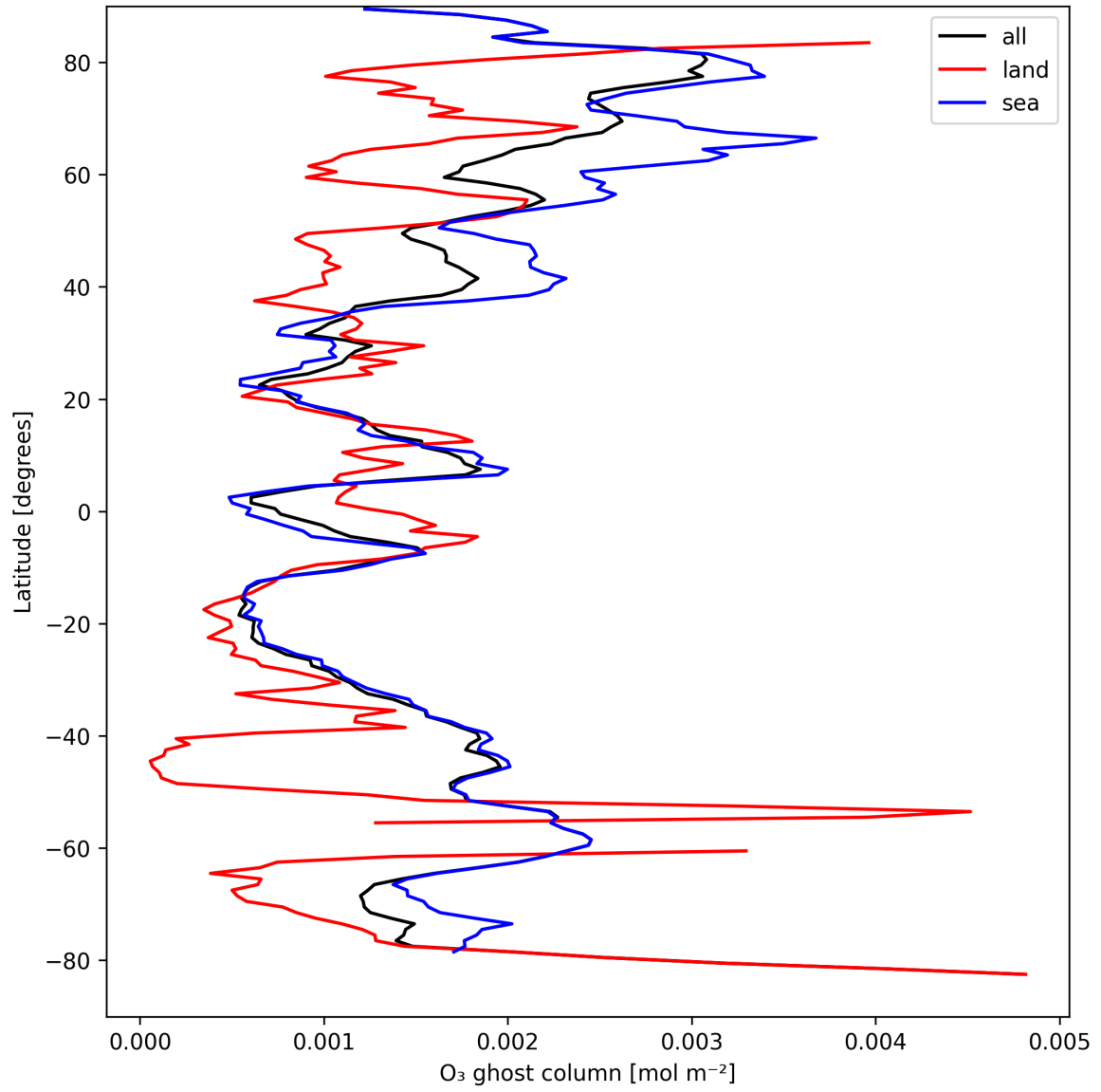
Figure 18: Zonal average of "O 3 ghost column" for 2025-09-05 to 2025-09-07.
