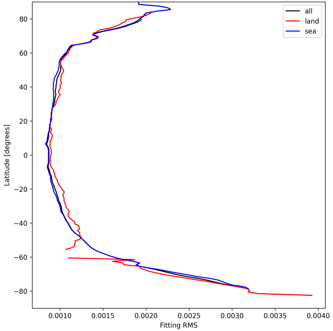
Figure 16: Zonal average of “Fitting RMS” for 2025-09-05 to 2025-09-07.
