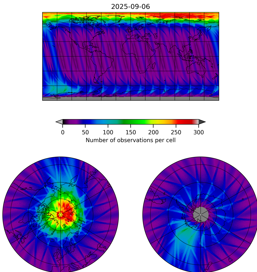
Figure 12: Map of the number of observations for 2025-09-05 to 2025-09-07
