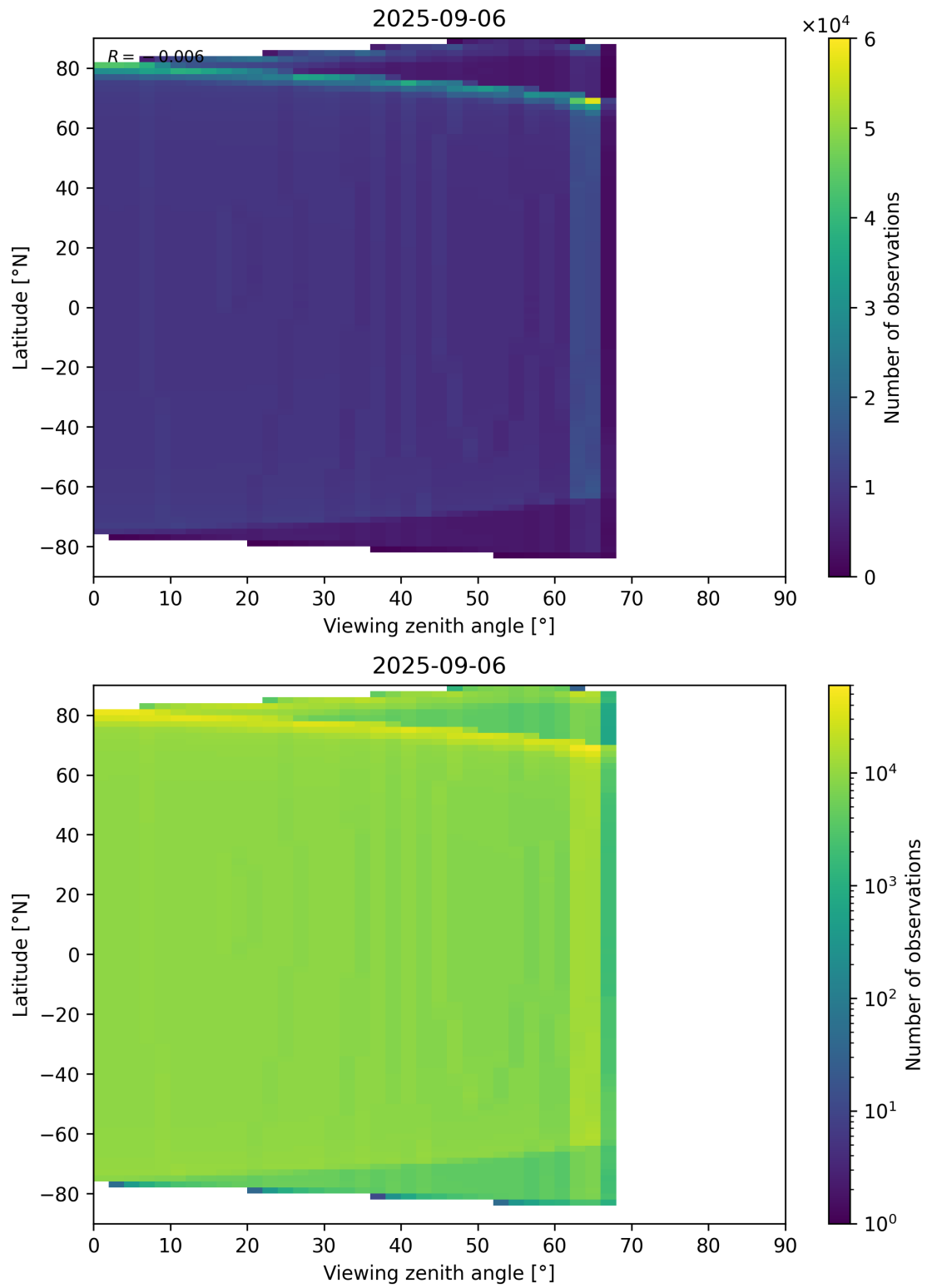
Figure 49: Scatter density plot of “Viewing zenith angle” against “Latitude” for 2025-09-05 to 2025-09-07.
