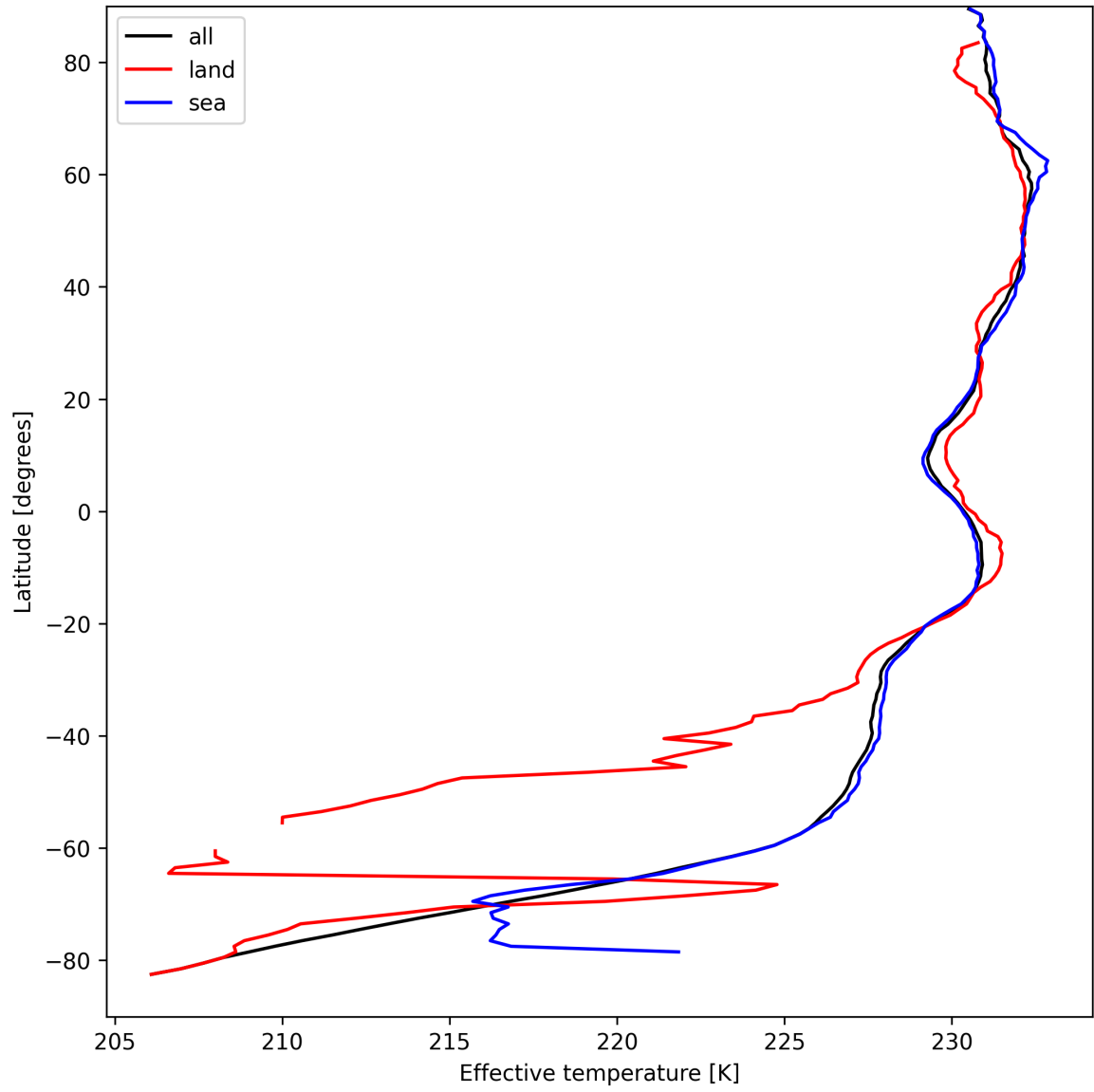
Figure 17: Zonal average of “Effective temperature” for 2025-09-05 to 2025-09-07.
