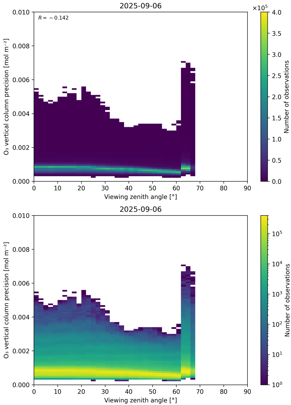
Figure 53: Scatter density plot of “Viewing zenith angle” against “O 3 vertical column precision” for 2025-09-05 to 2025-09-07.
