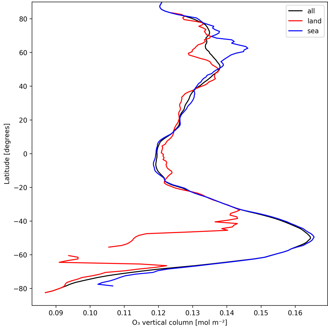
Figure 14: Zonal average of “O 3 vertical column” for 2025-09-05 to 2025-09-07.
