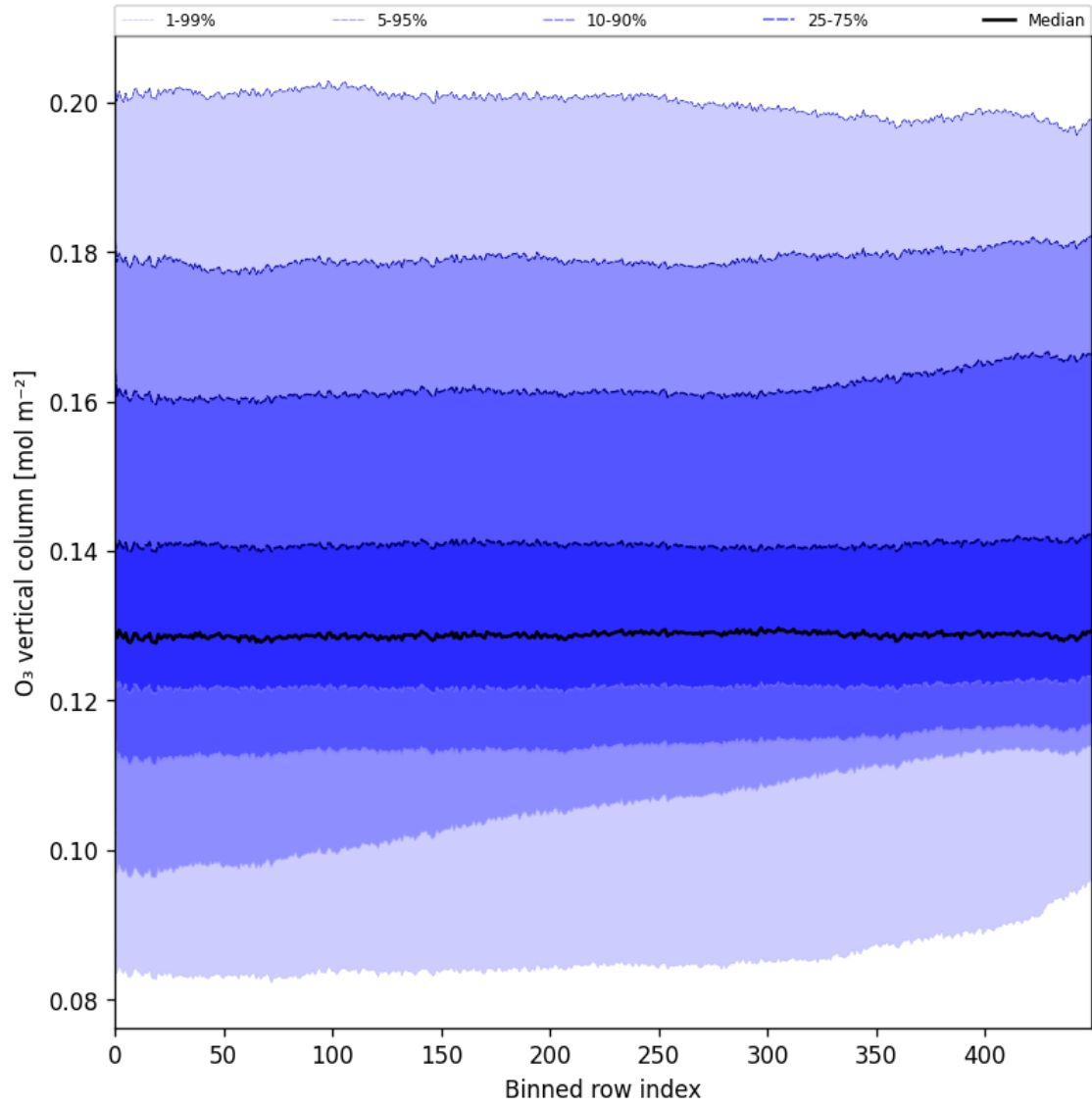
Figure 28: Along track statistics of “O 3 vertical column” for 2025-09-05 to 2025-09-07
