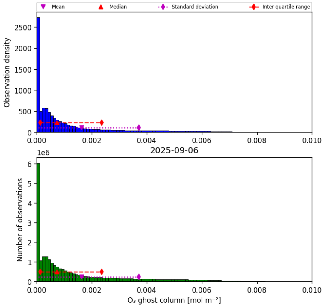
Figure 25: Histogram of “O 3 ghost column” for 2025-09-05 to 2025-09-07
