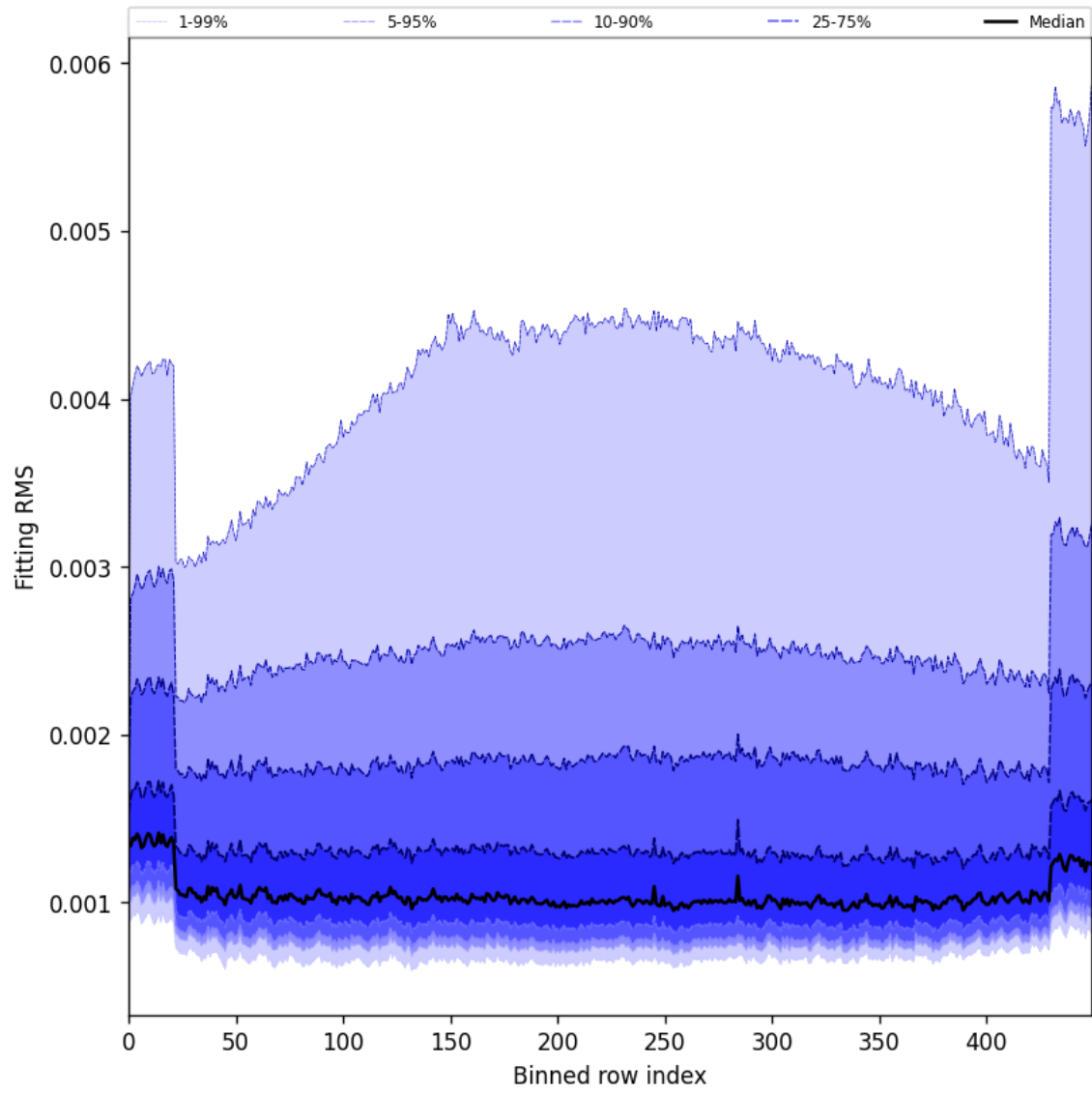
Figure 30: Along track statistics of “Fitting RMS” for 2025-09-05 to 2025-09-07
