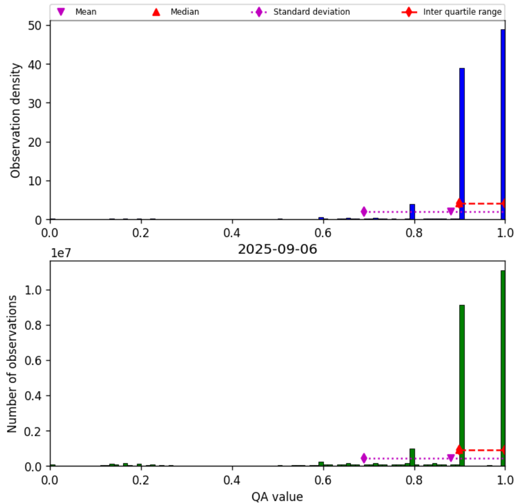
Figure 20: Histogram of “QA value” for 2025-09-05 to 2025-09-07
