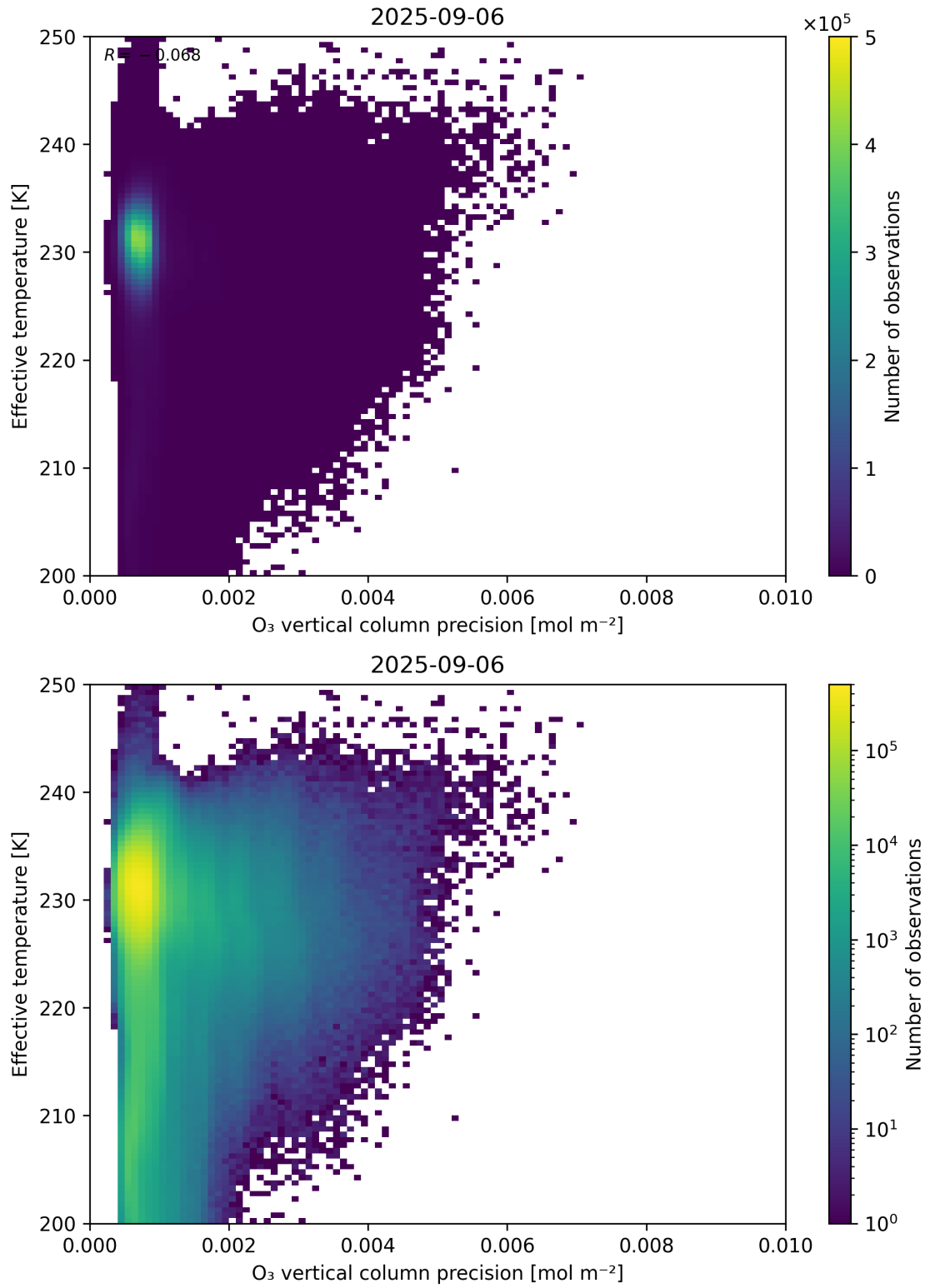
Figure 42: Scatter density plot of “ O_3 vertical column precision” against “Effective temperature” for 2025-09-05 to 2025-09-07.
