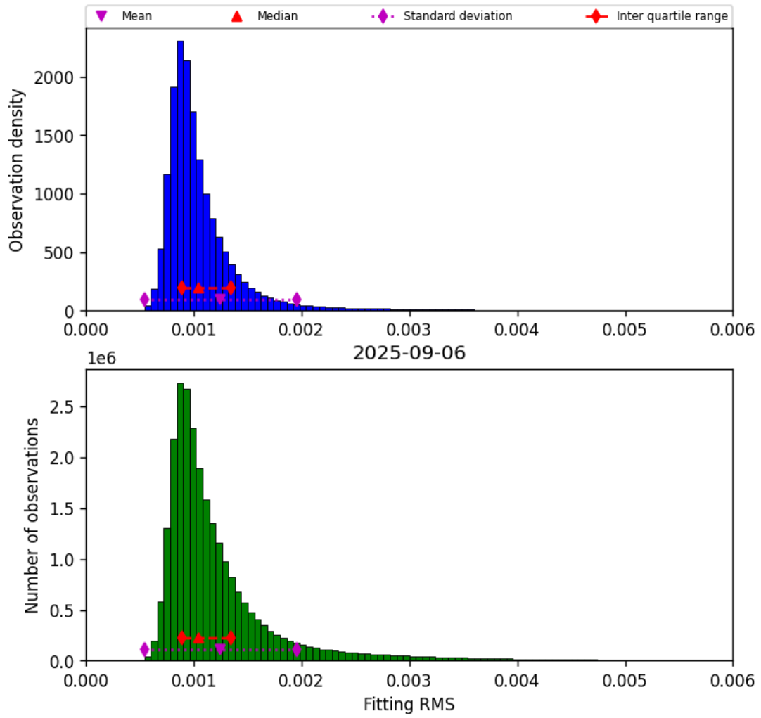
Figure 23: Histogram of “Fitting RMS” for 2025-09-05 to 2025-09-07
