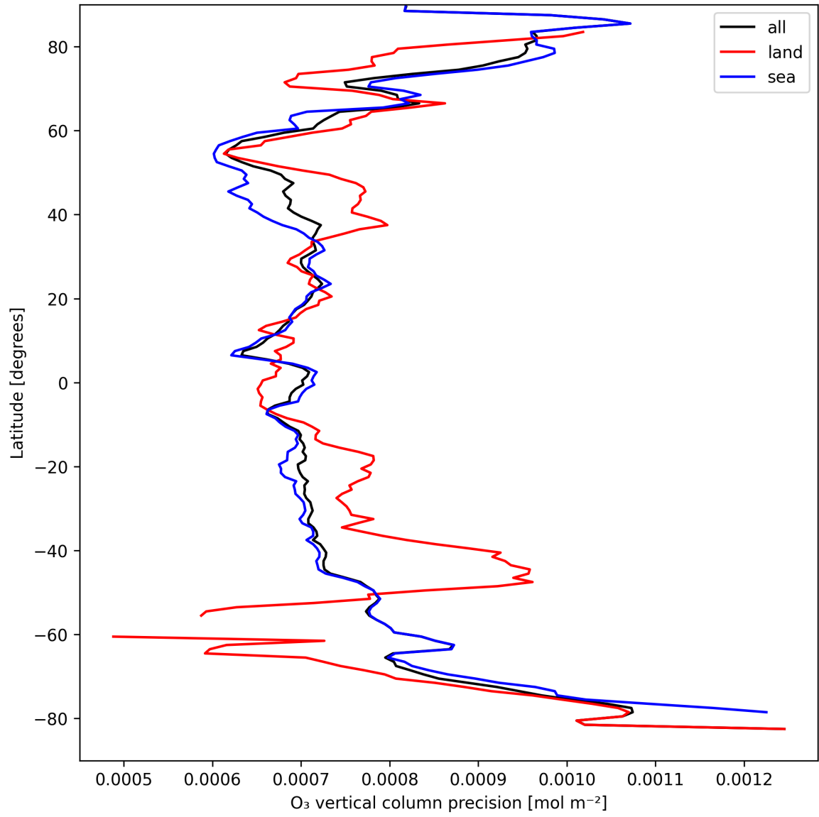
Figure 15: Zonal average of “O 3 vertical column precision” for 2025-09-05 to 2025-09-07.
