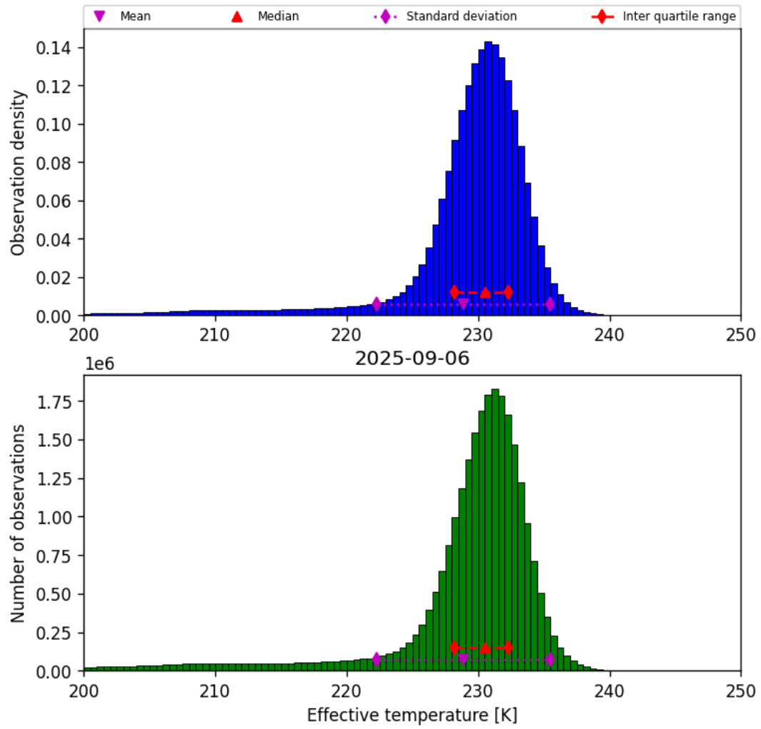
Figure 24: Histogram of “Effective temperature” for 2025-09-05 to 2025-09-07
