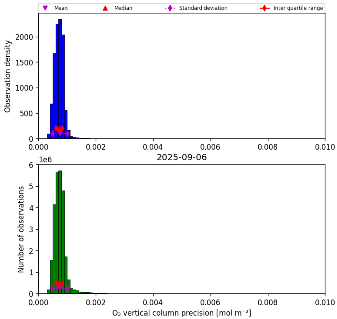
Figure 22: Histogram of "O 3 vertical column precision" for 2025-09-05 to 2025-09-07
