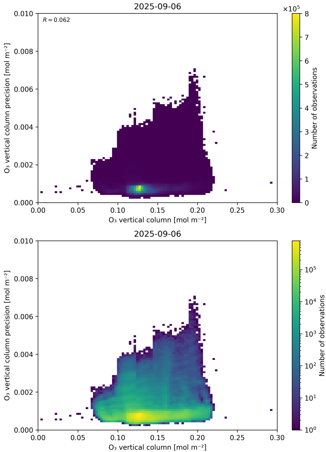
Figure 41: Scatter density plot of “O 3 vertical column” against “O 3 vertical column precision” for 2025-09-05 to 2025-09-07.
