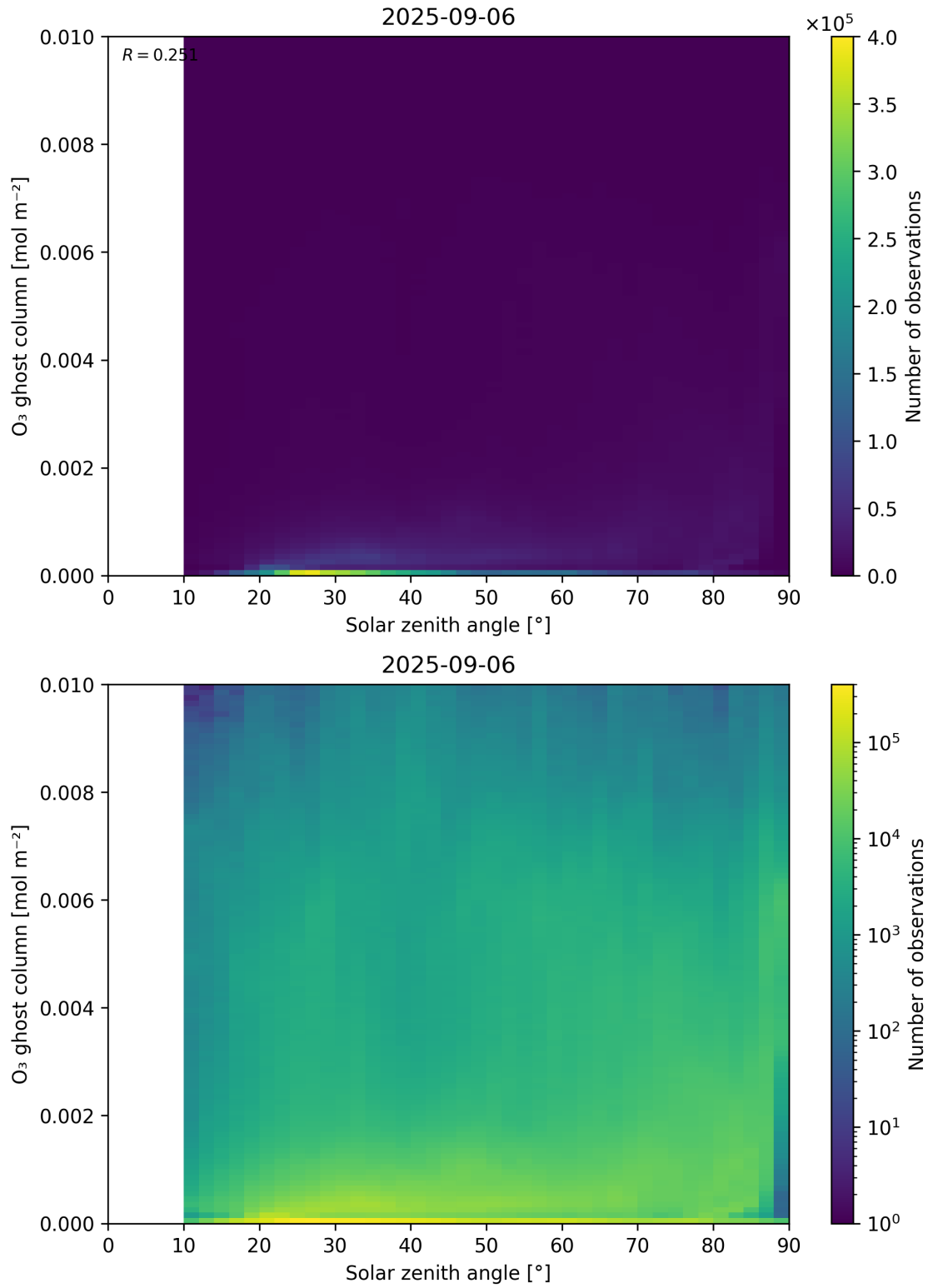
Figure 46: Scatter density plot of “Solar zenith angle” against “O 3 ghost column” for 2025-09-05 to 2025-09-07.
