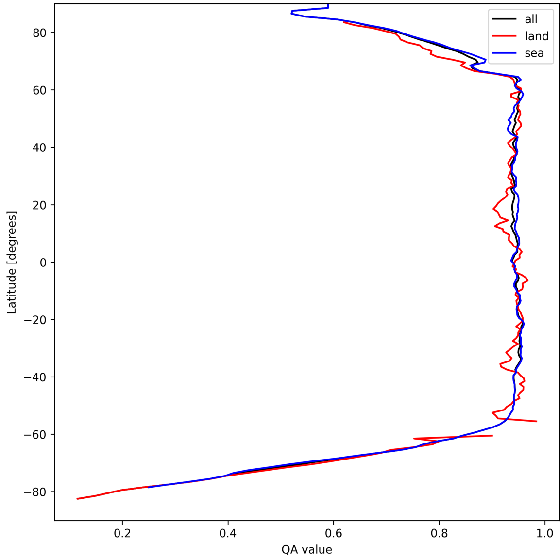
Figure 13: Zonal average of “QA value” for 2025-09-05 to 2025-09-07.
