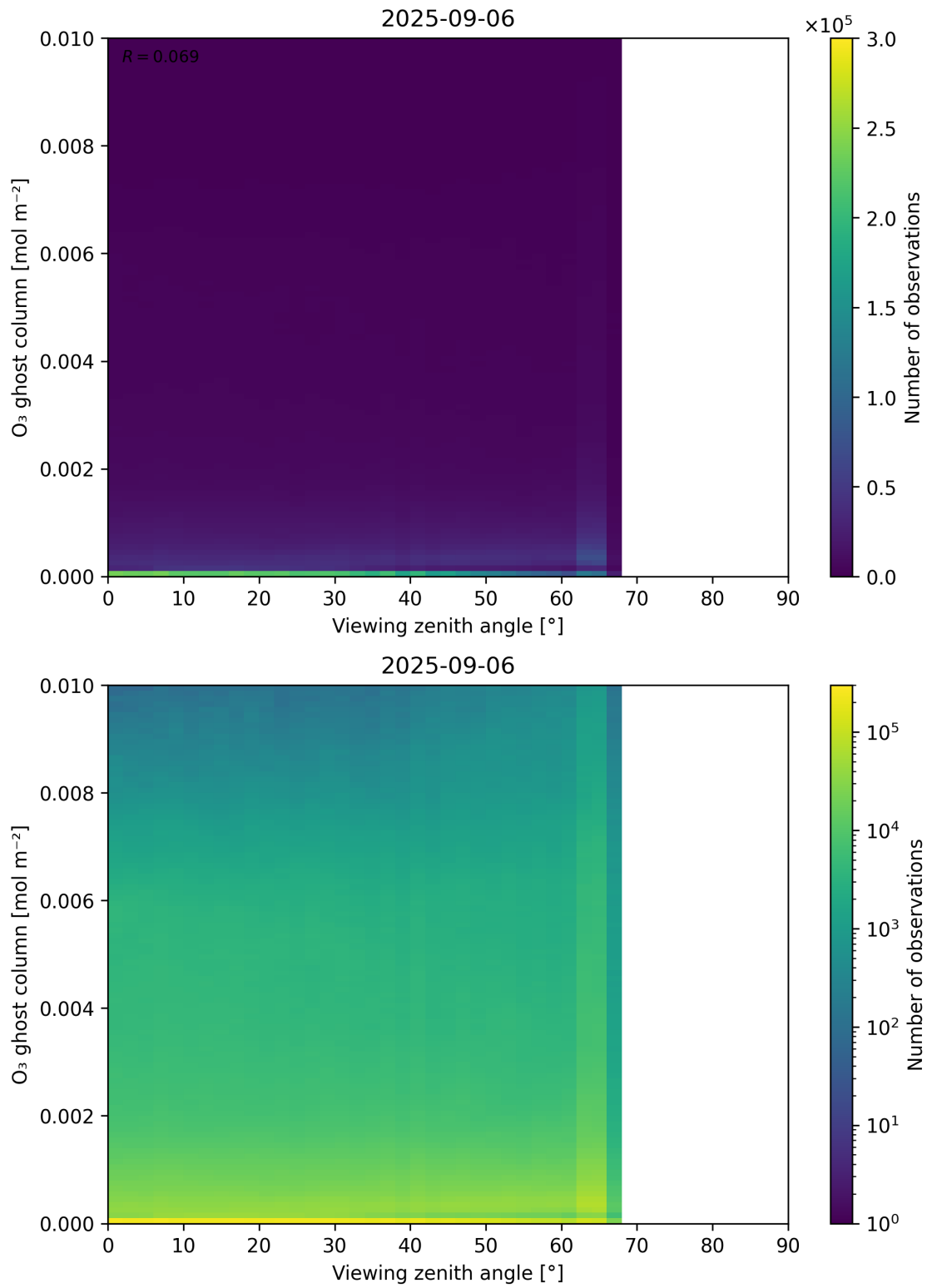
Figure 51: Scatter density plot of “Viewing zenith angle” against “O 3 ghost column” for 2025-09-05 to 2025-09-07.
