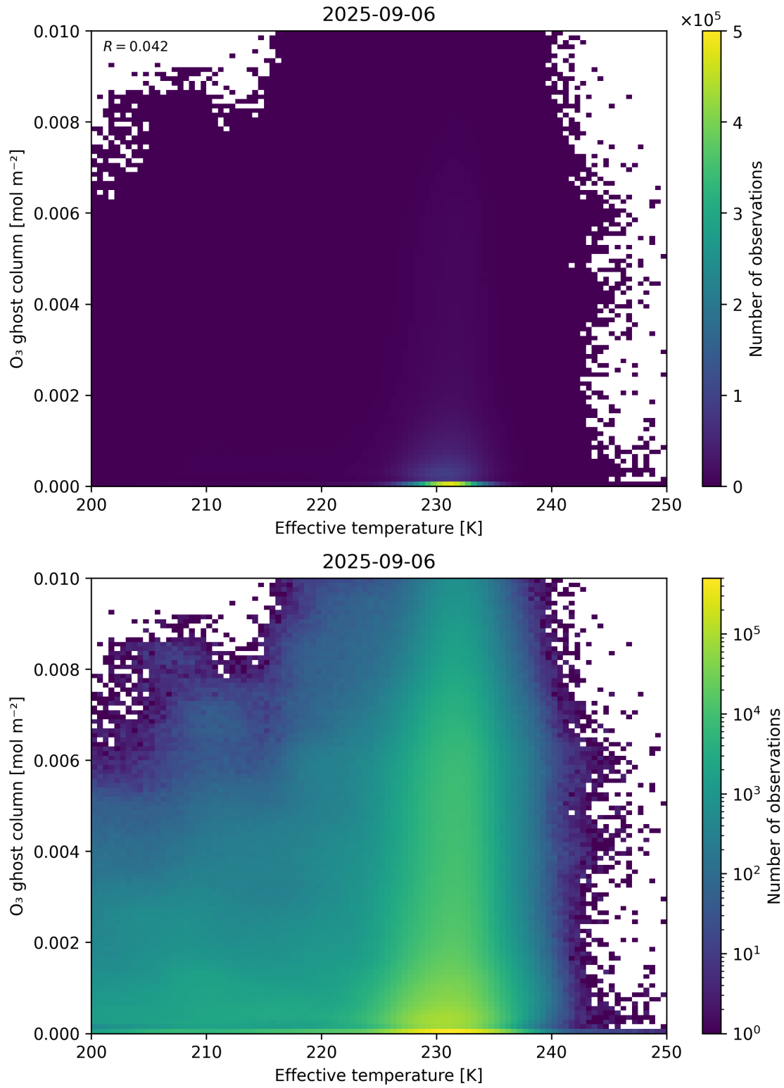
Figure 38: Scatter density plot of “Effective temperature” against “O 3 ghost column” for 2025-09-05 to 2025-09-07.
