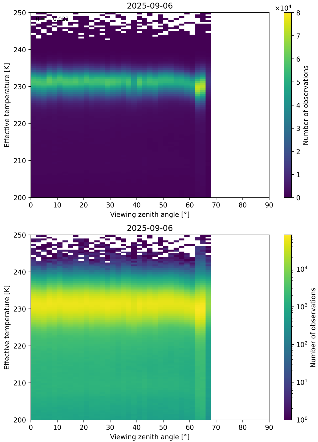
Figure 50: Scatter density plot of “Viewing zenith angle” against “Effective temperature” for 2025-09-05 to 2025-09-07.
