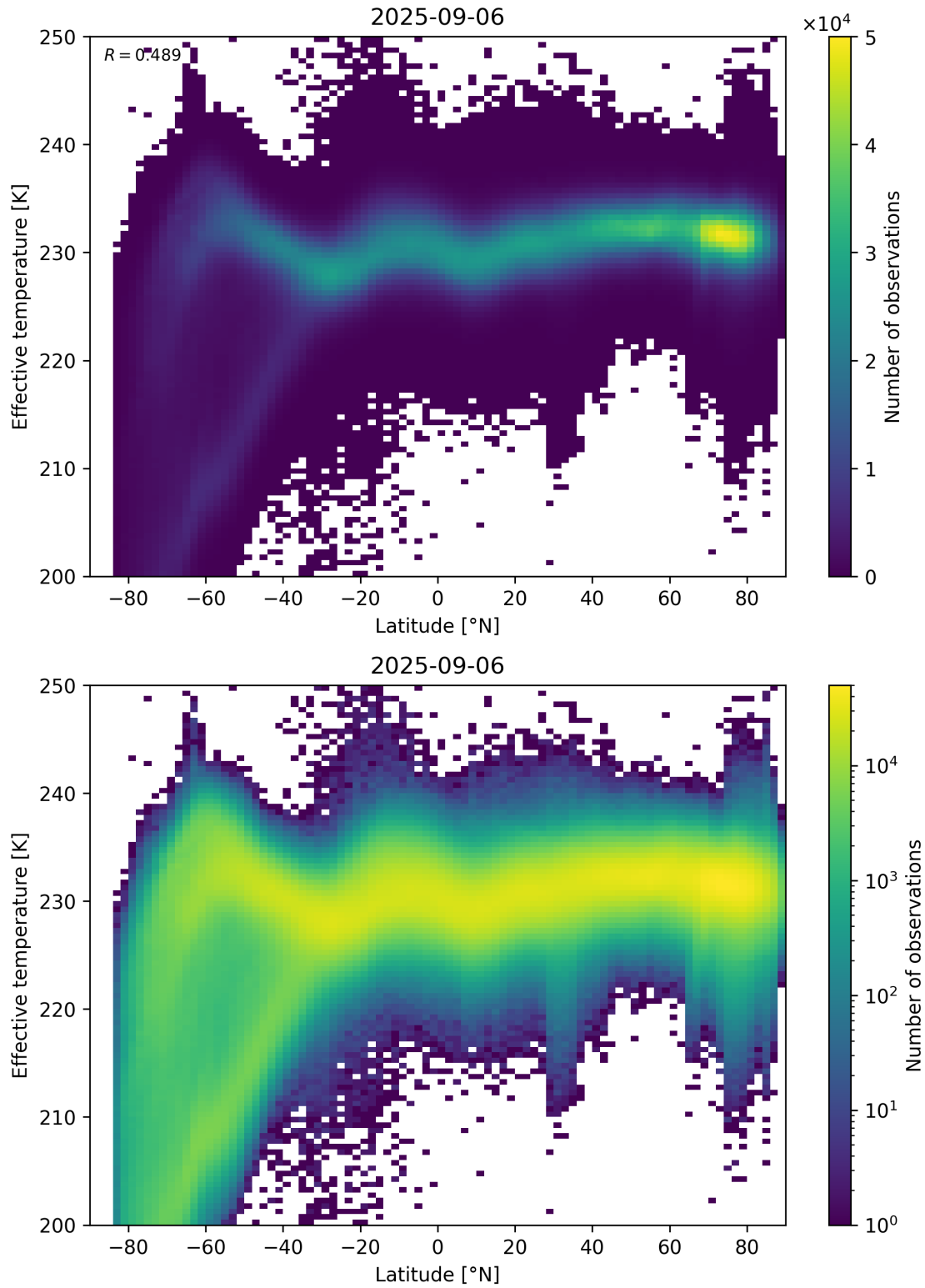
Figure 34: Scatter density plot of “Latitude” against “Effective temperature” for 2025-09-05 to 2025-09-07.
