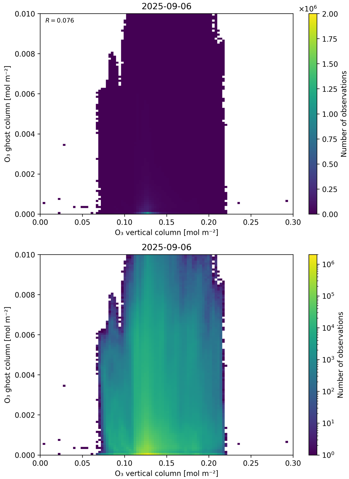
Figure 40: Scatter density plot of “O 3 vertical column” against “O 3 ghost column” for 2025-09-05 to 2025-09-07.
