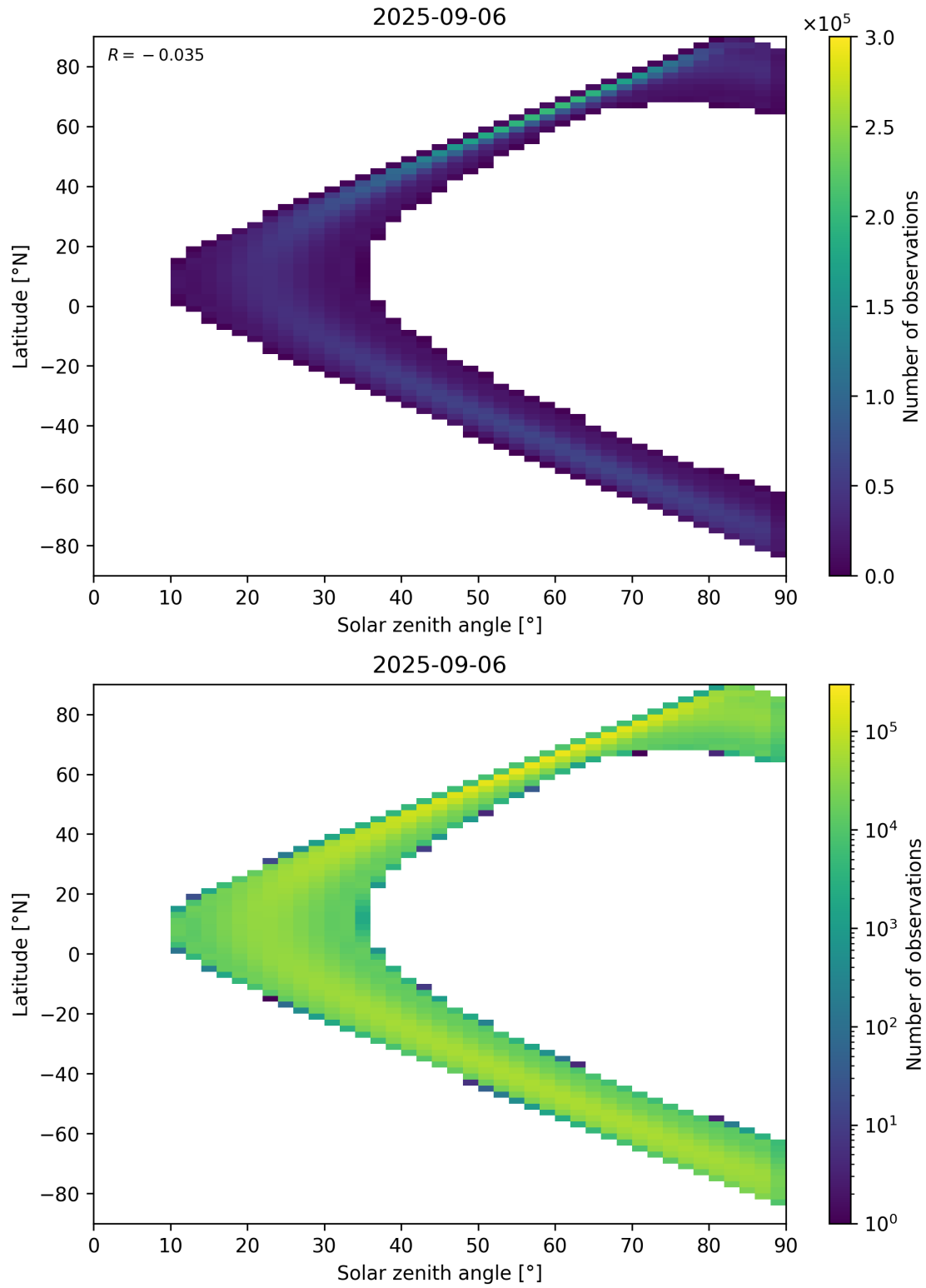
Figure 44: Scatter density plot of “Solar zenith angle” against “Latitude” for 2025-09-05 to 2025-09-07.
