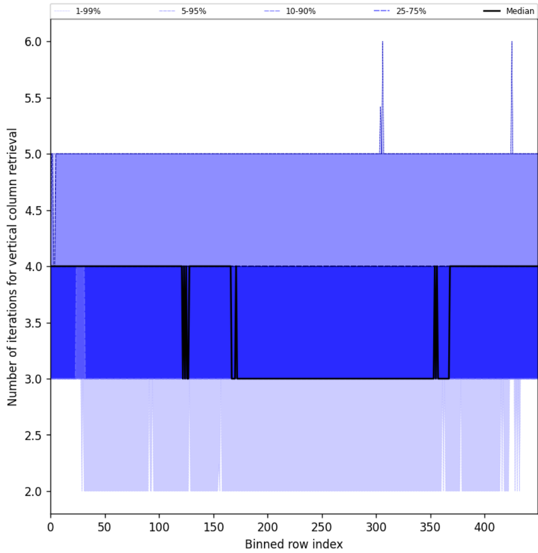
Figure 33: Along track statistics of “Number of iterations for vertical column retrieval” for 2025-09-05 to 2025-09-07
