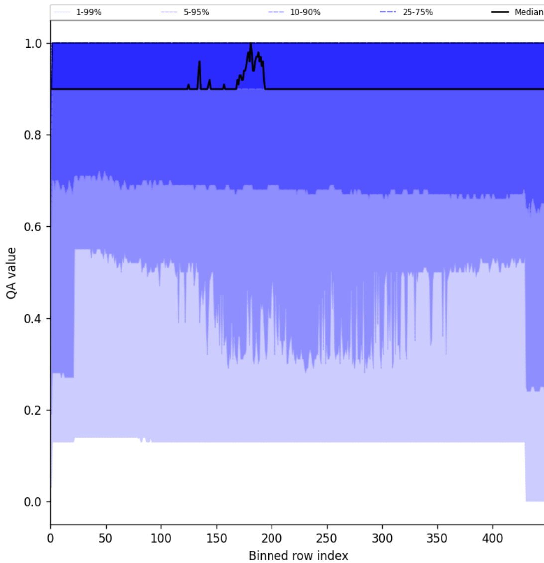
Figure 27: Along track statistics of “QA value” for 2025-09-05 to 2025-09-07
