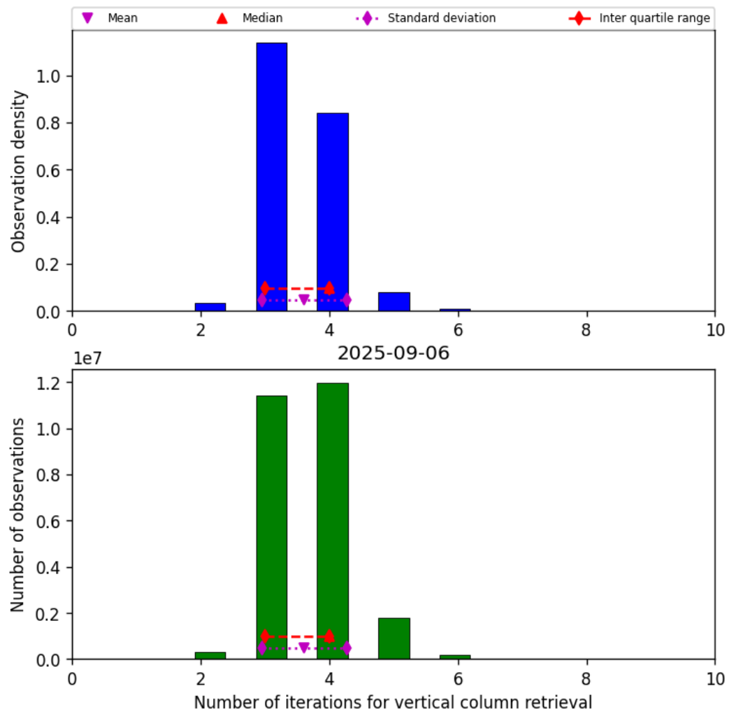
Figure 26: Histogram of “Number of iterations for vertical column retrieval” for 2025-09-05 to 2025-09-07
