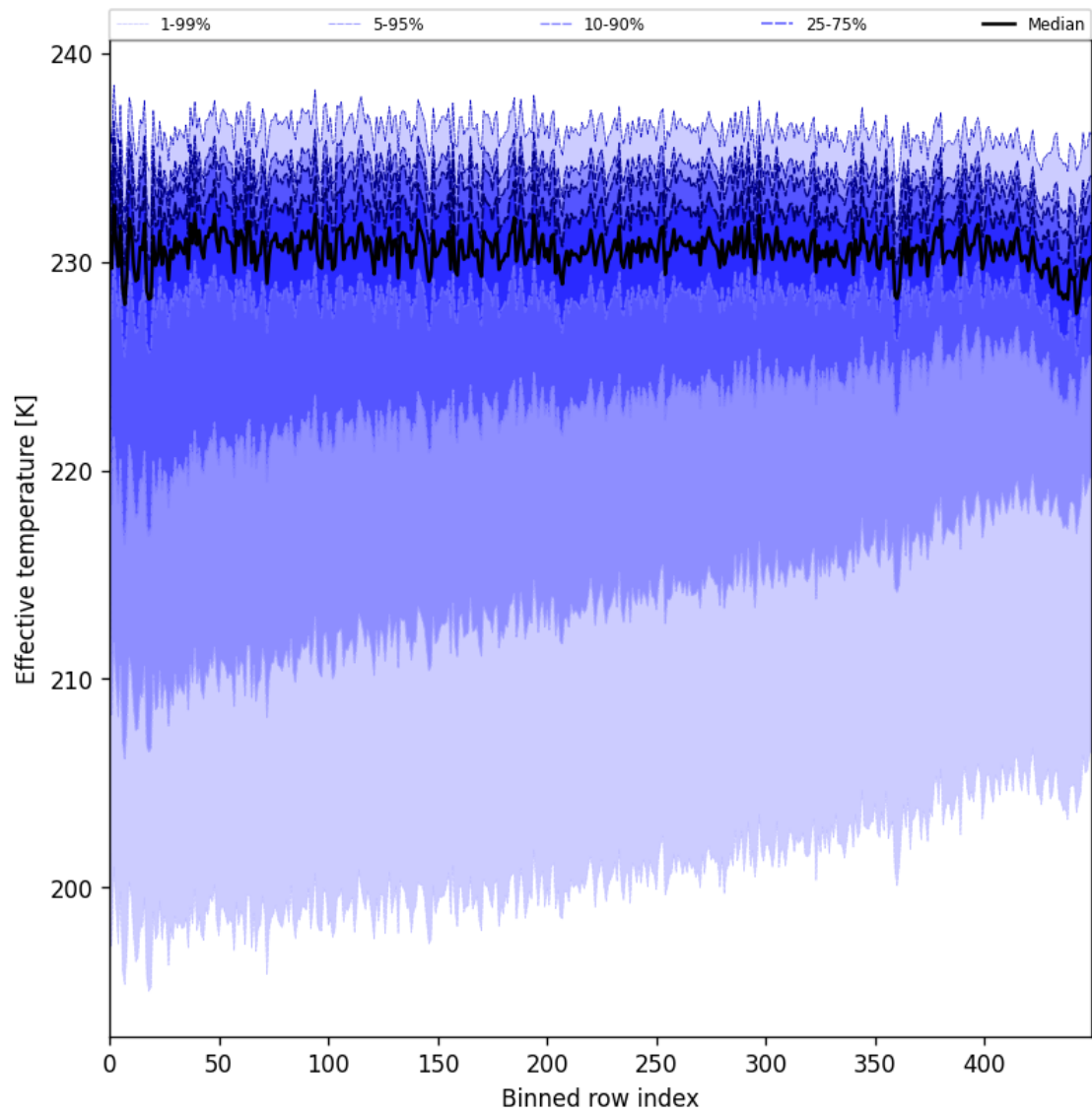
Figure 31: Along track statistics of “Effective temperature” for 2025-09-05 to 2025-09-07
