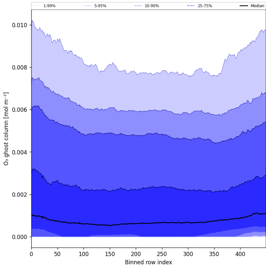
Figure 32: Along track statistics of “O 3 ghost column” for 2025-09-05 to 2025-09-07
