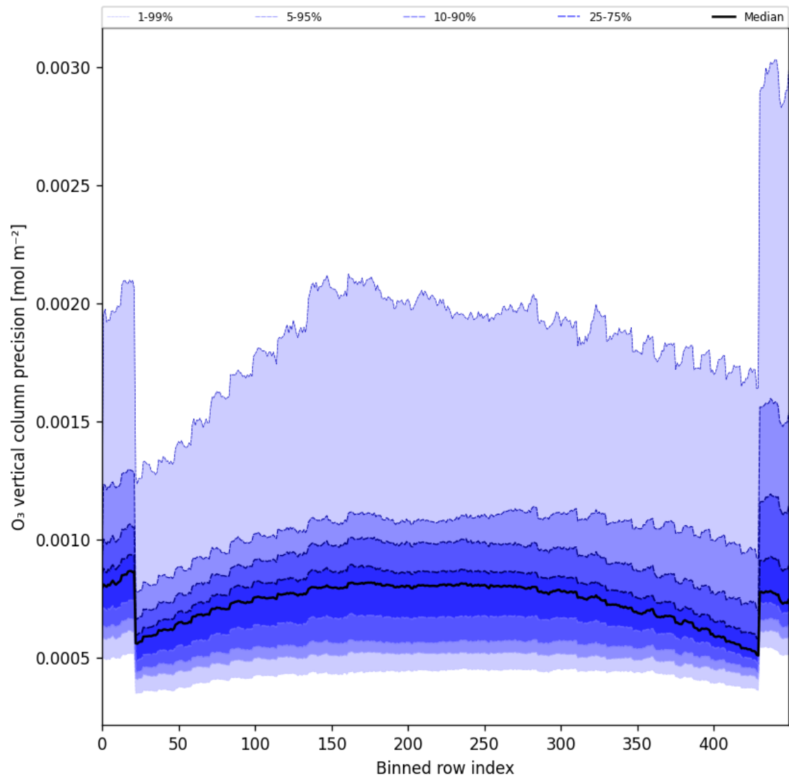
Figure 29: Along track statistics of “O 3 vertical column precision” for 2025-09-05 to 2025-09-07
