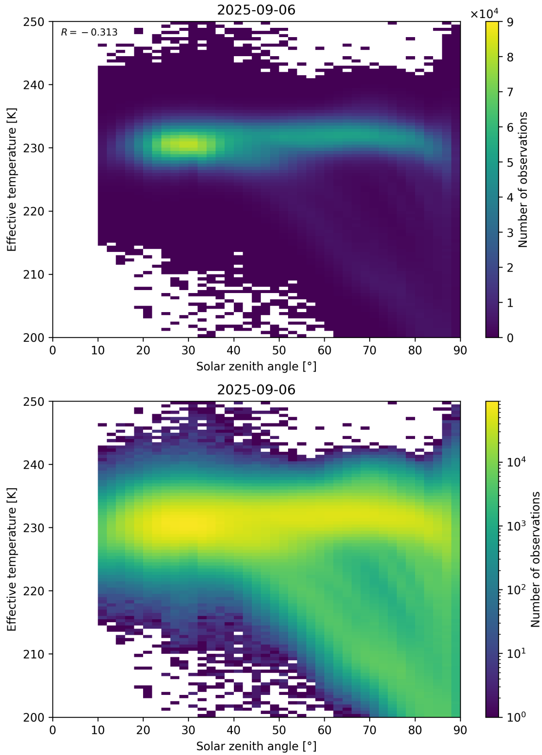
Figure 45: Scatter density plot of “Solar zenith angle” against “Effective temperature” for 2025-09-05 to 2025-09-07.
