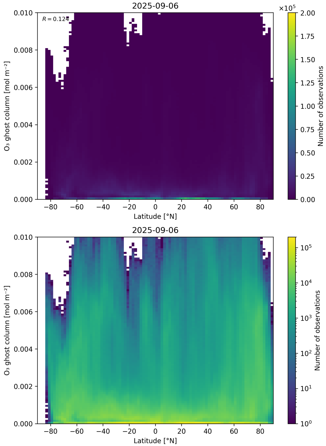
Figure 35: Scatter density plot of “Latitude” against “O 3 ghost column” for 2025-09-05 to 2025-09-07.
