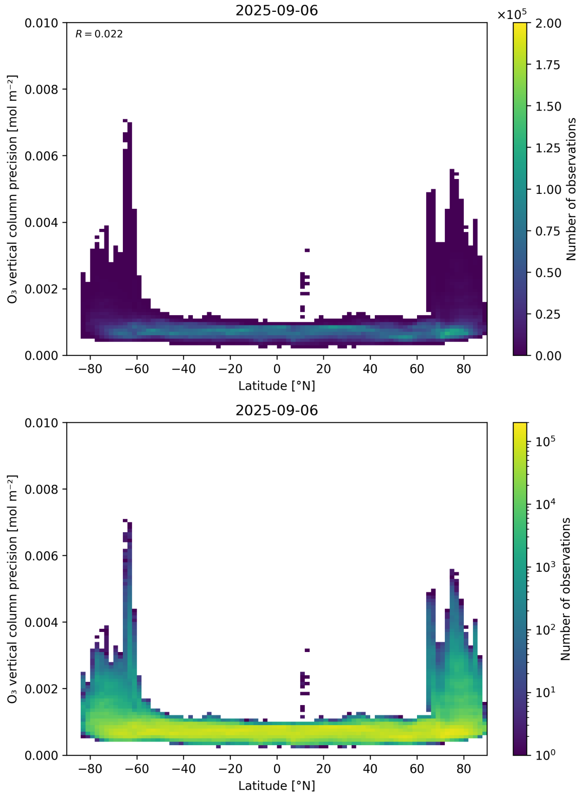
Figure 37: Scatter density plot of “Latitude” against “O 3 vertical column precision” for 2025-09-05 to 2025-09-07.
