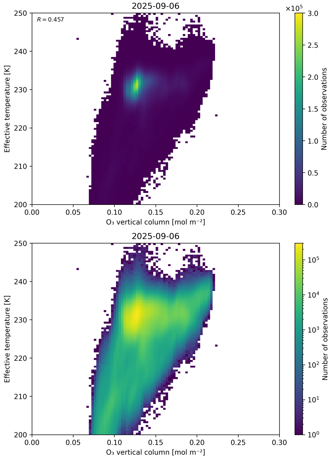
Figure 39: Scatter density plot of “O 3 vertical column” against “Effective temperature” for 2025-09-05 to 2025-09-07.
