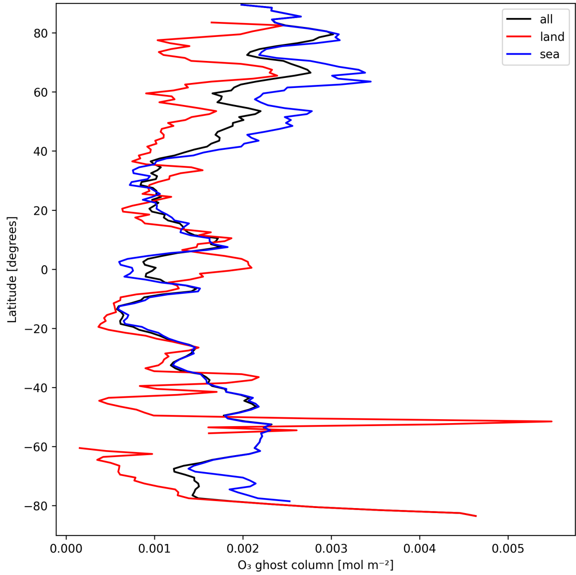
Figure 18: Zonal average of “O 3 ghost column” for 2025-09-06 to 2025-09-08.
