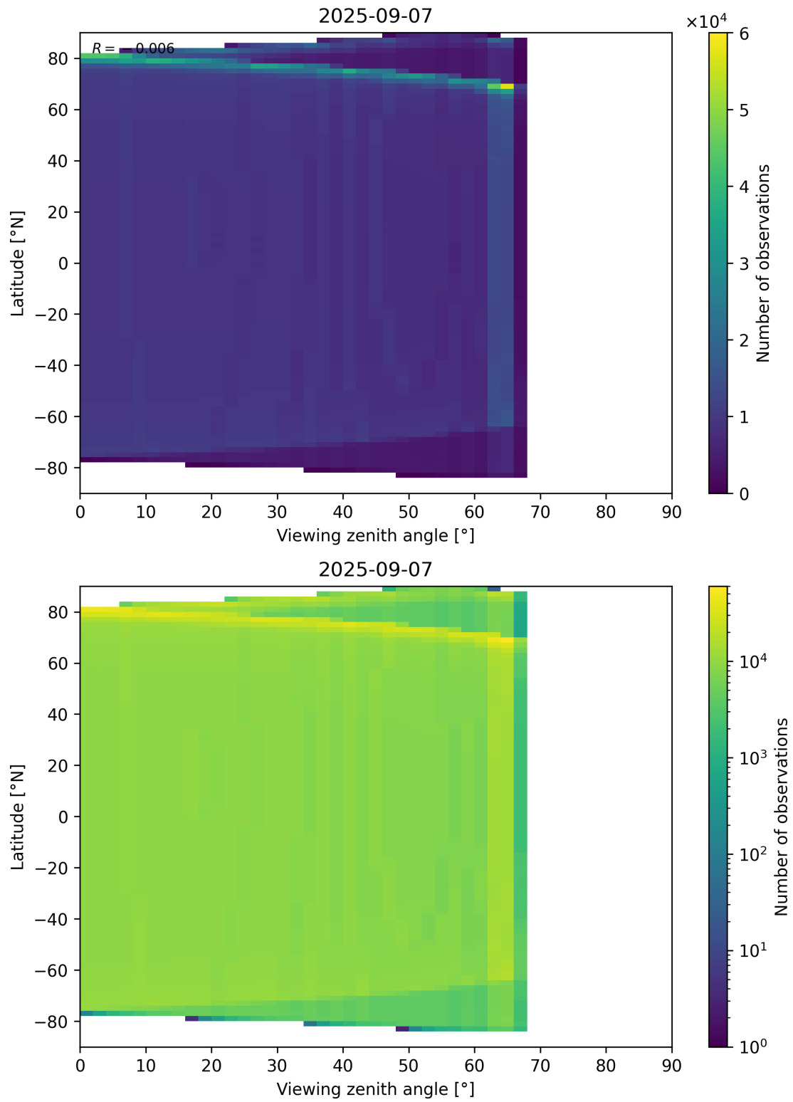
Figure 49: Scatter density plot of “Viewing zenith angle” against “Latitude” for 2025-09-06 to 2025-09-08.
