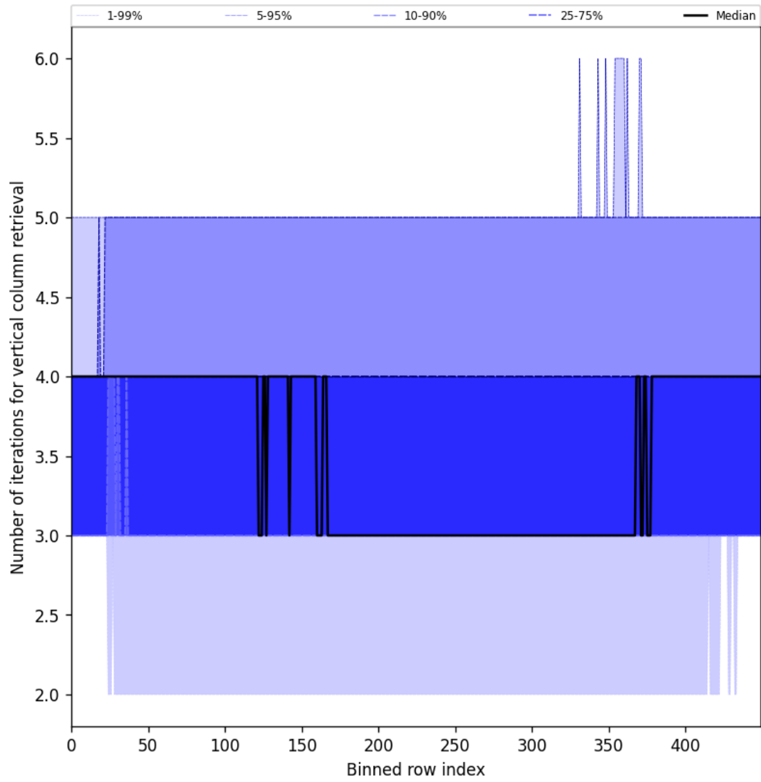
Figure 33: Along track statistics of “Number of iterations for vertical column retrieval” for 2025-09-06 to 2025-09-08
