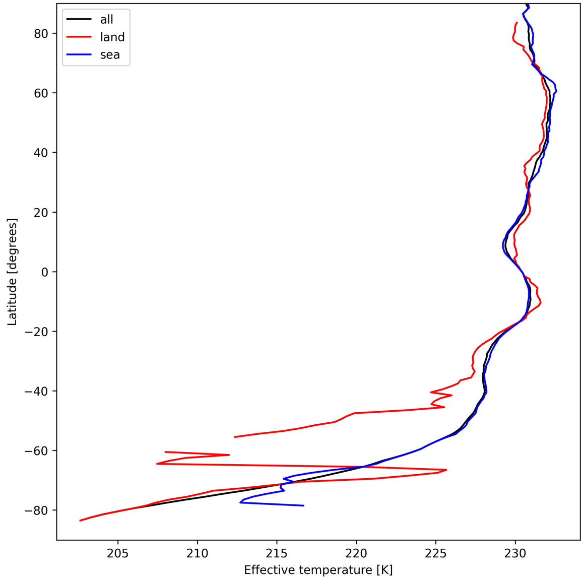
Figure 17: Zonal average of "Effective temperature" for 2025-09-06 to 2025-09-08.
