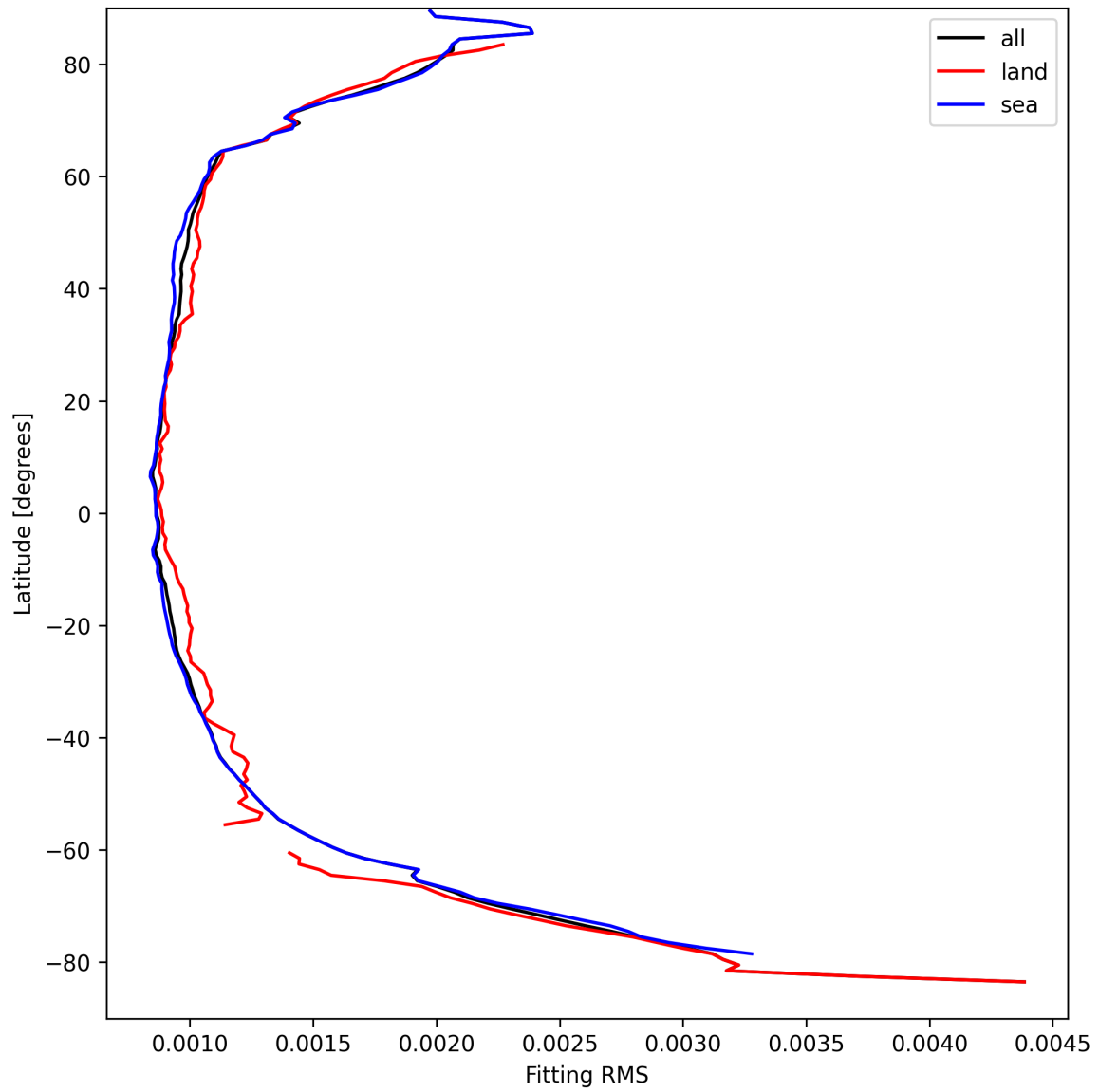
Figure 16: Zonal average of “Fitting RMS” for 2025-09-06 to 2025-09-08.
