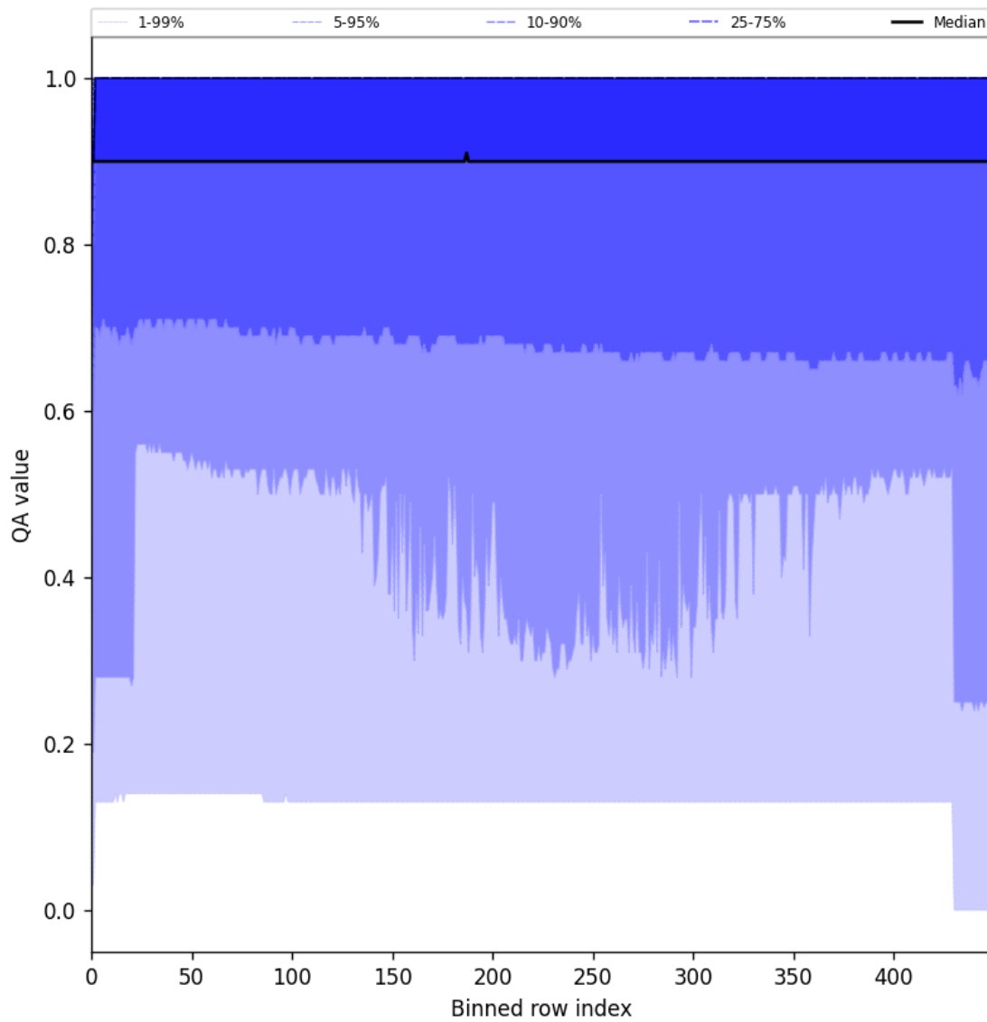
Figure 27: Along track statistics of “QA value” for 2025-09-06 to 2025-09-08
