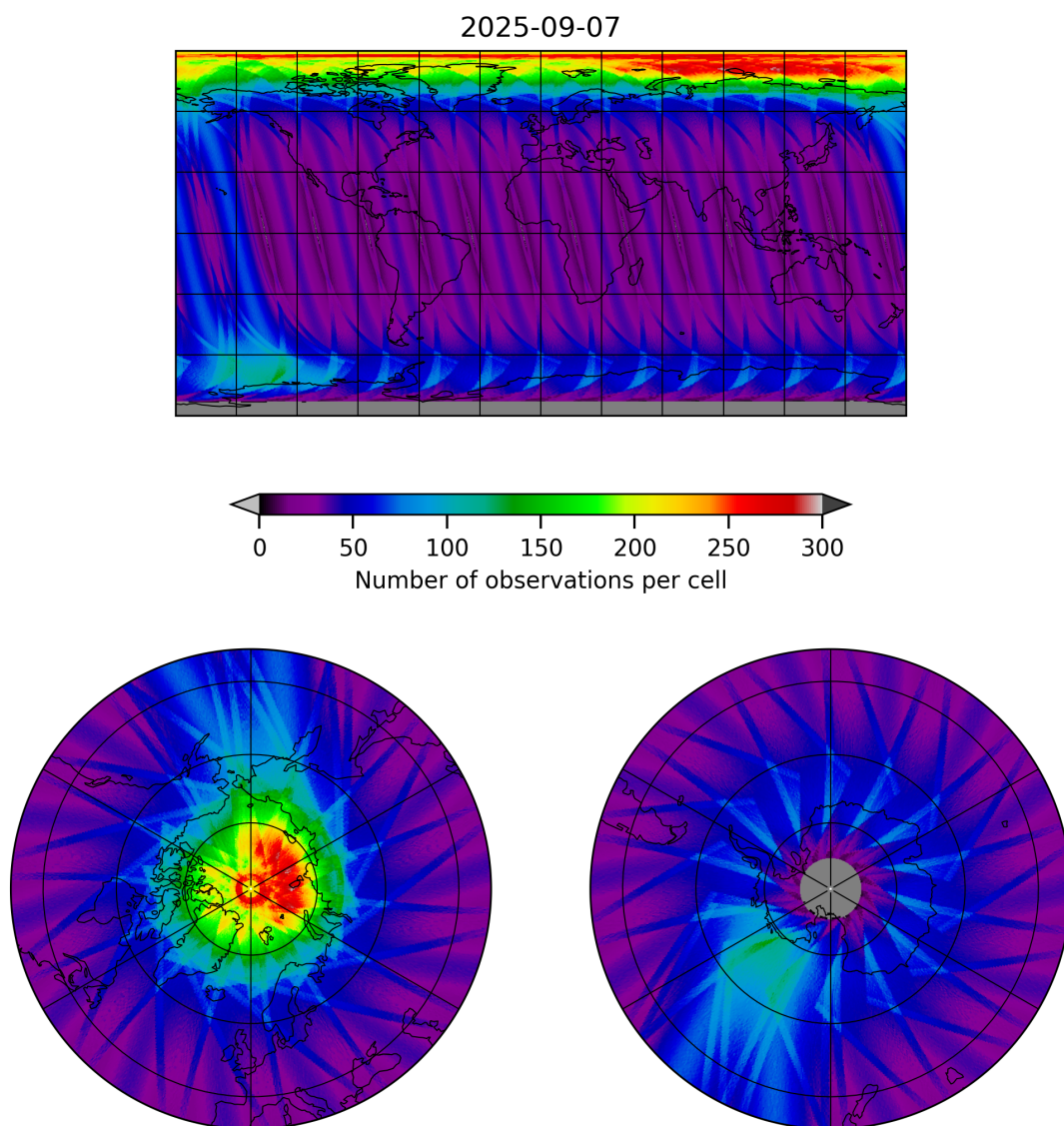
Figure 12: Map of the number of observations for 2025-09-06 to 2025-09-08
