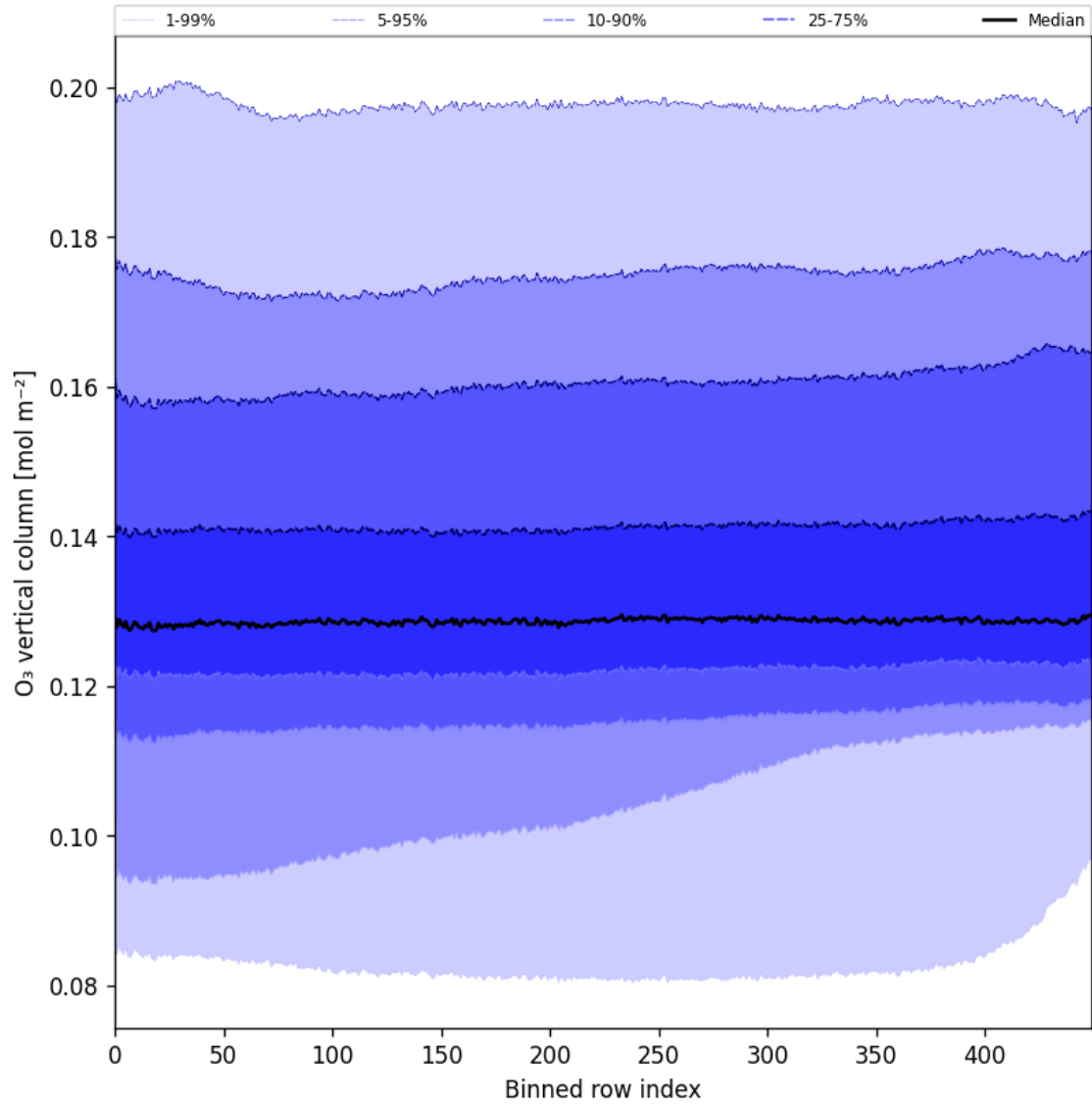
Figure 28: Along track statistics of “O 3 vertical column” for 2025-09-06 to 2025-09-08
