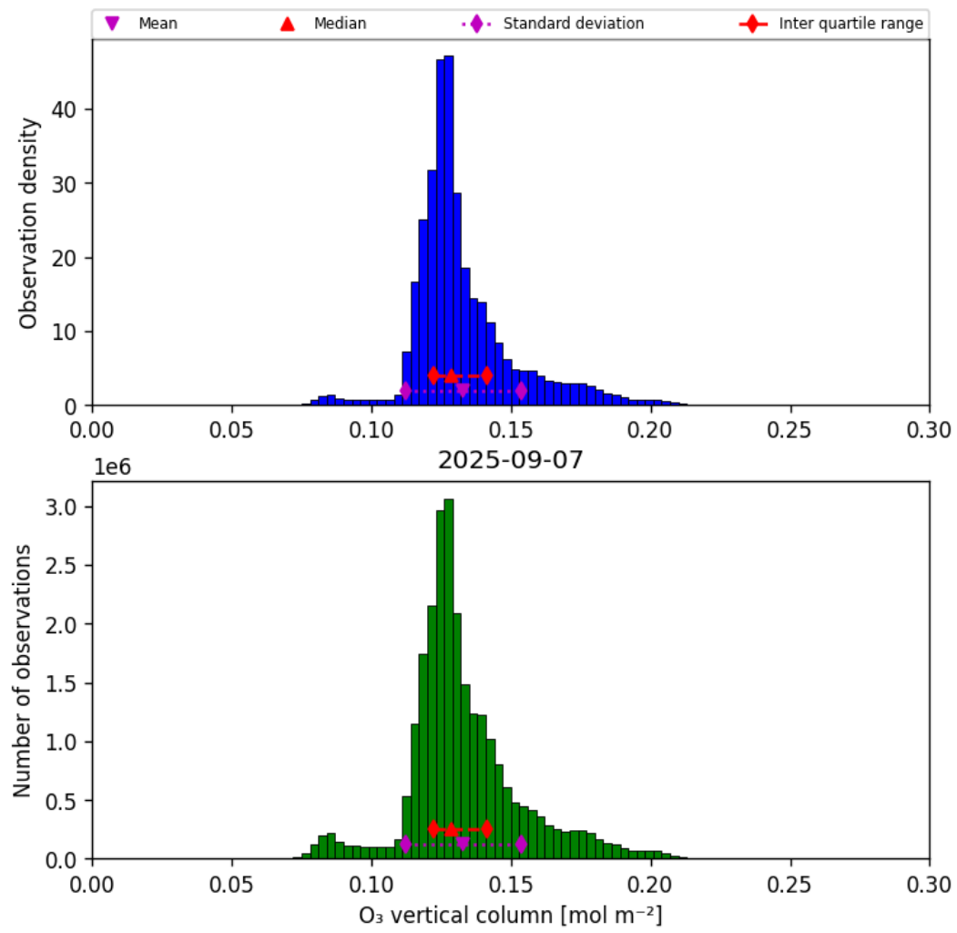
Figure 21: Histogram of “O 3 vertical column” for 2025-09-06 to 2025-09-08
