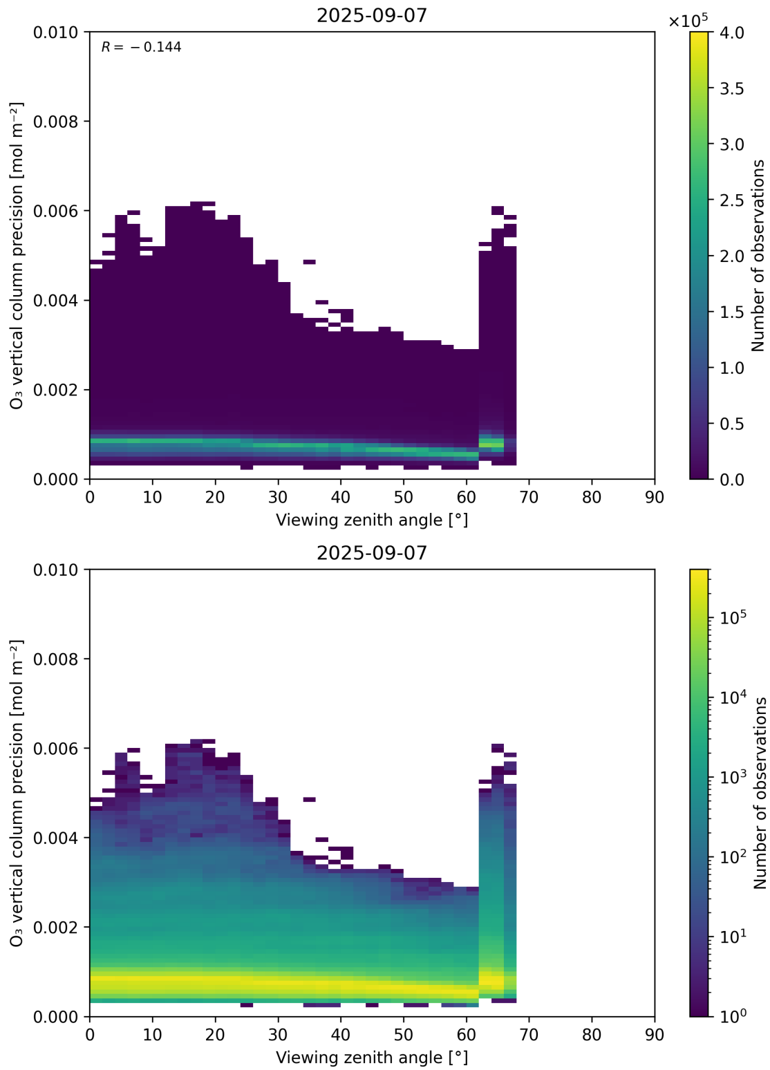
Figure 53: Scatter density plot of “Viewing zenith angle” against “O 3 vertical column precision” for 2025-09-06 to 2025-09-08.
