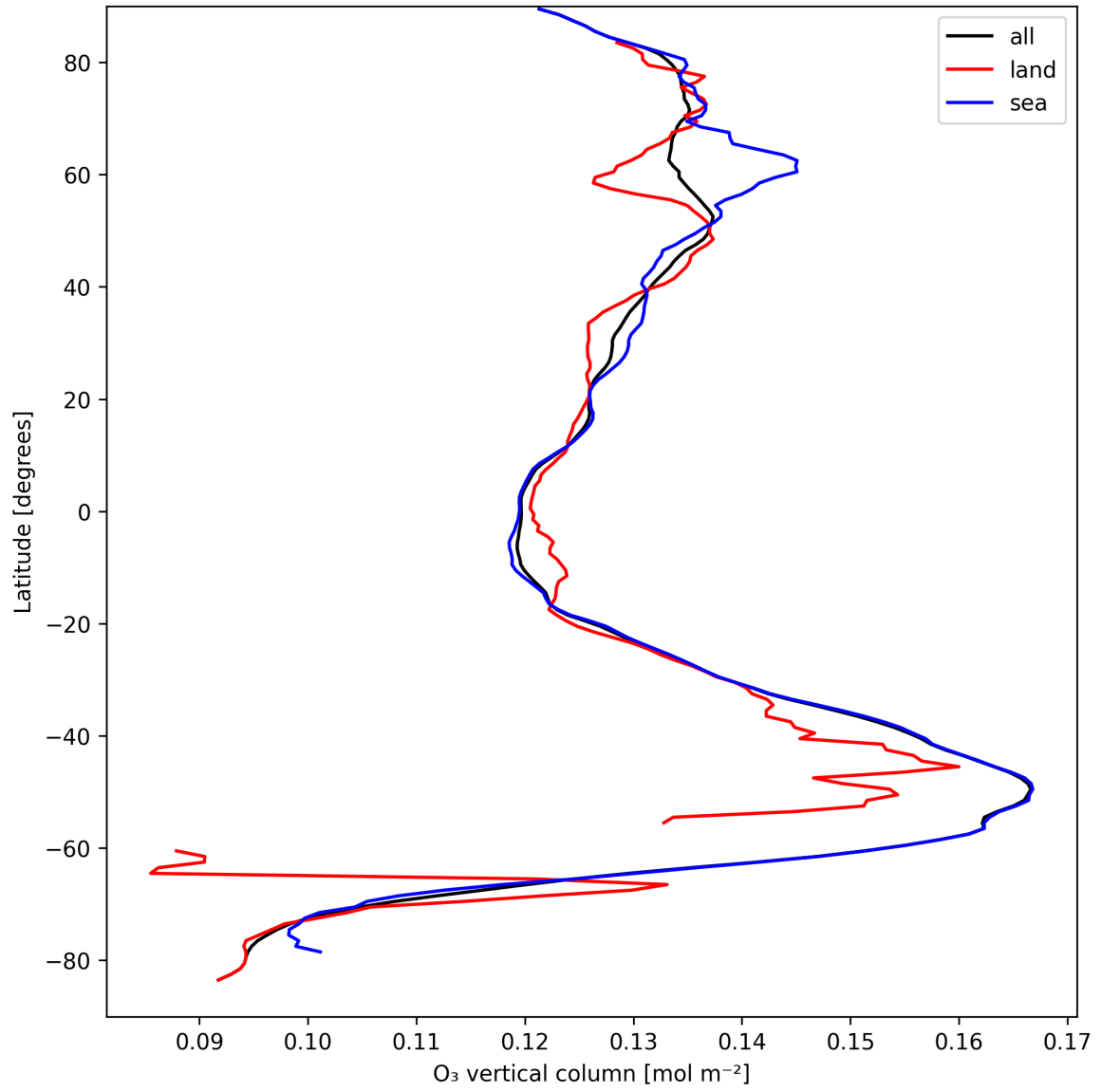
Figure 14: Zonal average of “O 3 vertical column” for 2025-09-06 to 2025-09-08.
