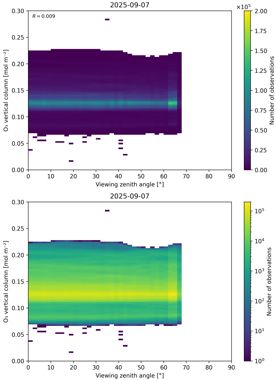
Figure 52: Scatter density plot of “Viewing zenith angle” against “O 3 vertical column” for 2025-09-06 to 2025-09-08.
