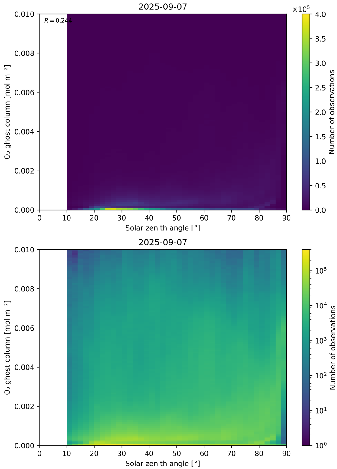
Figure 46: Scatter density plot of “Solar zenith angle” against “O 3 ghost column” for 2025-09-06 to 2025-09-08.
