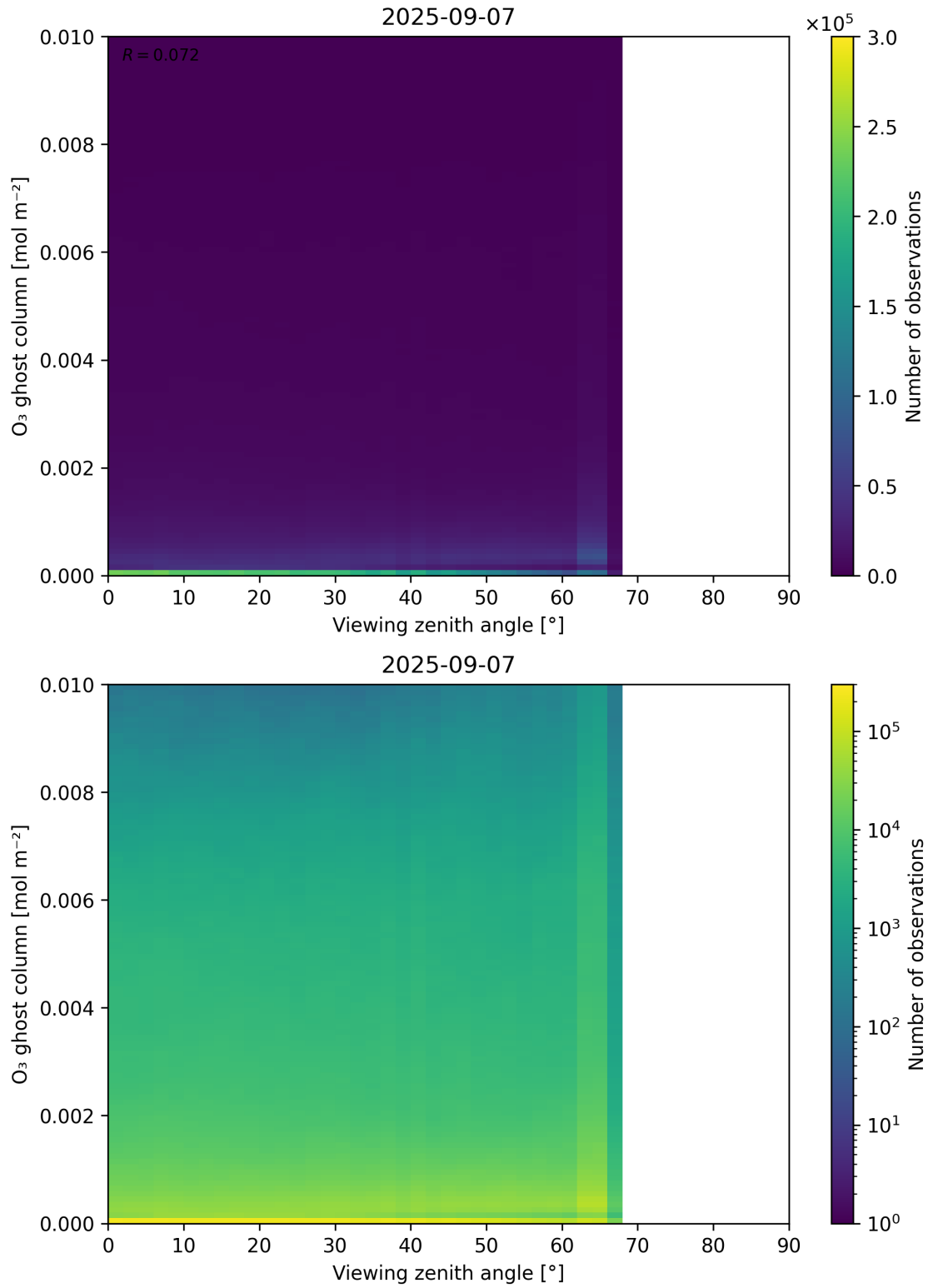
Figure 51: Scatter density plot of “Viewing zenith angle” against “O 3 ghost column” for 2025-09-06 to 2025-09-08.
