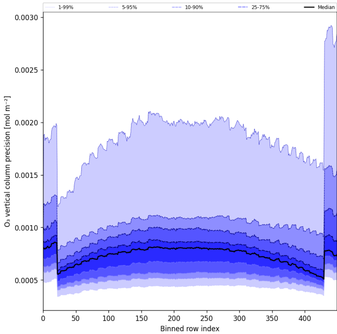
Figure 29: Along track statistics of “O 3 vertical column precision” for 2025-09-06 to 2025-09-08
