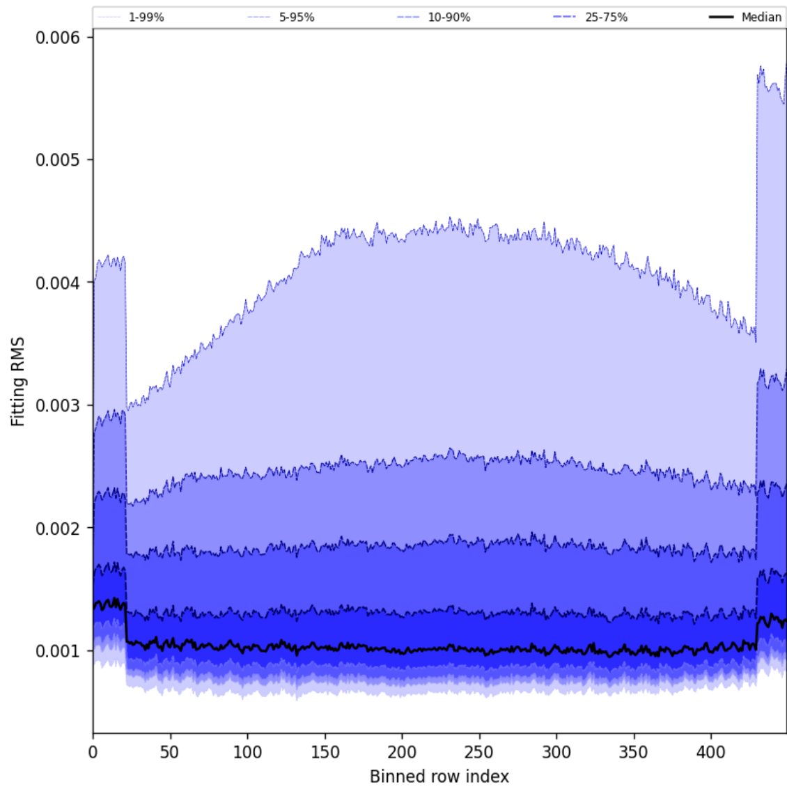
Figure 30: Along track statistics of “Fitting RMS” for 2025-09-06 to 2025-09-08
