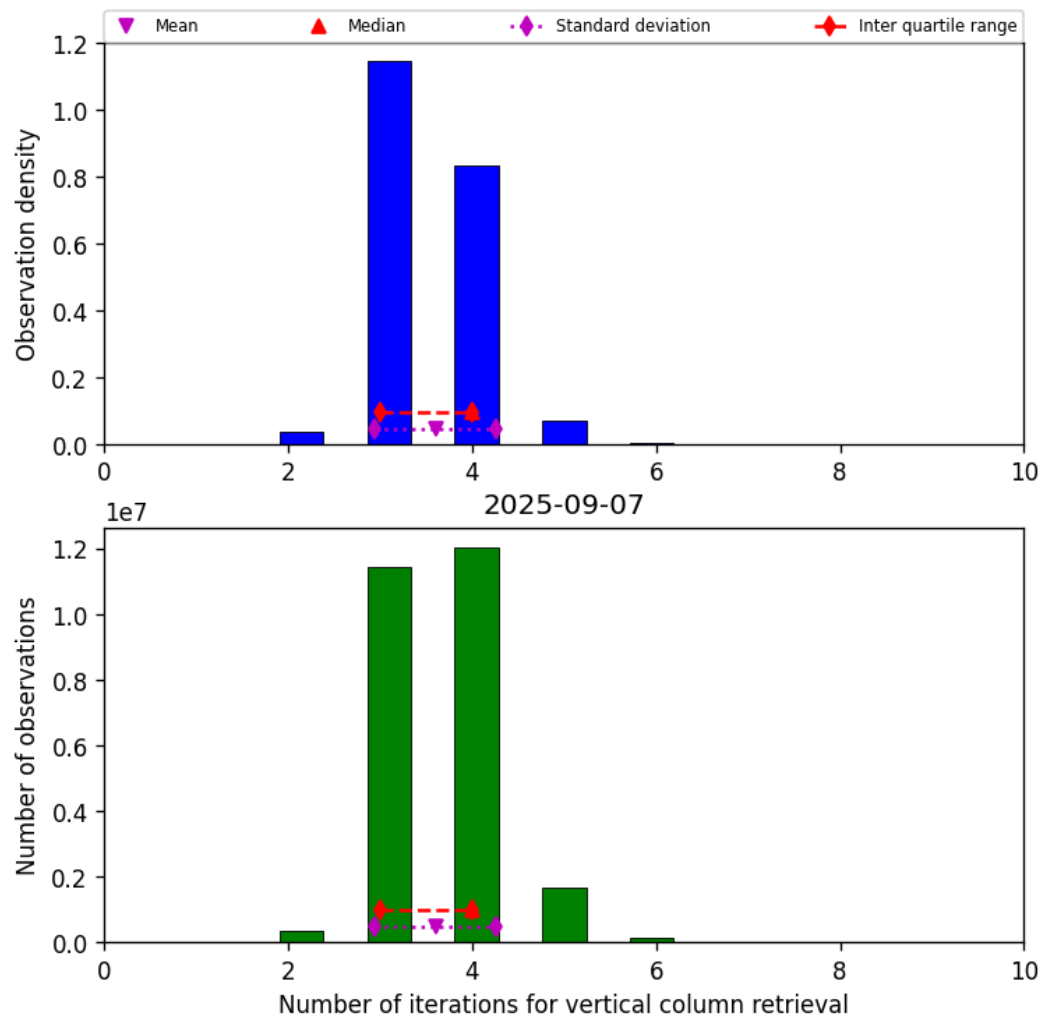
Figure 26: Histogram of “Number of iterations for vertical column retrieval” for 2025-09-06 to 2025-09-08
