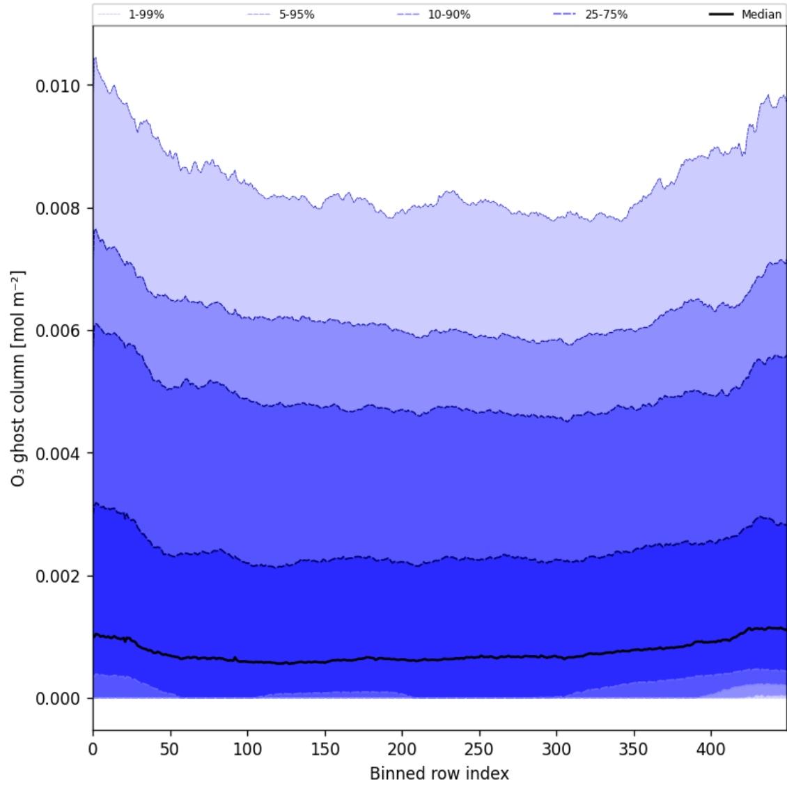
Figure 32: Along track statistics of “O 3 ghost column” for 2025-09-06 to 2025-09-08
