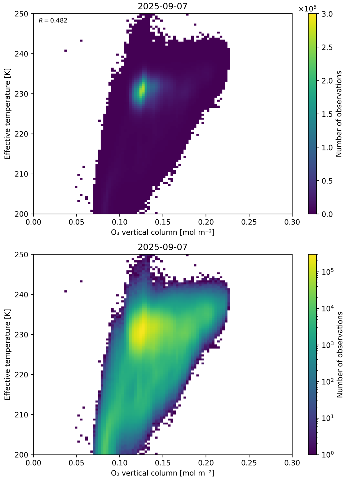
Figure 39: Scatter density plot of “O 3 vertical column” against “Effective temperature” for 2025-09-06 to 2025-09-08.
