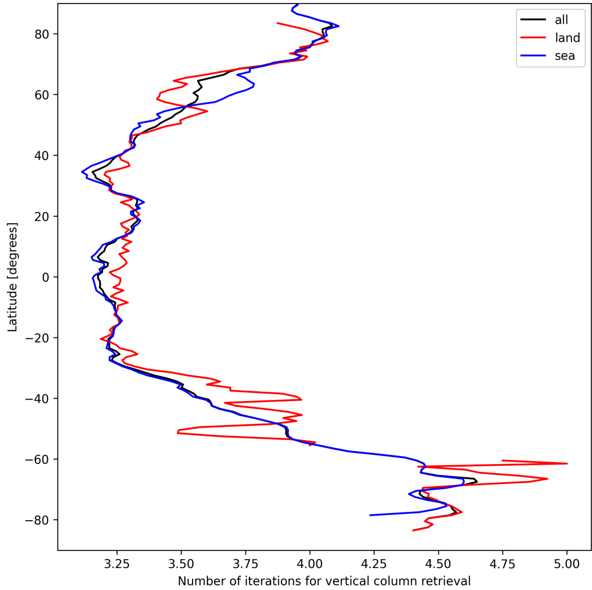
Figure 19: Zonal average of “Number of iterations for vertical column retrieval” for 2025-09-06 to 2025-09-08.
