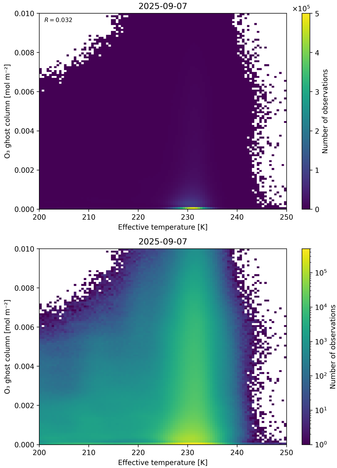
Figure 38: Scatter density plot of “Effective temperature” against “O 3 ghost column” for 2025-09-06 to 2025-09-08.
