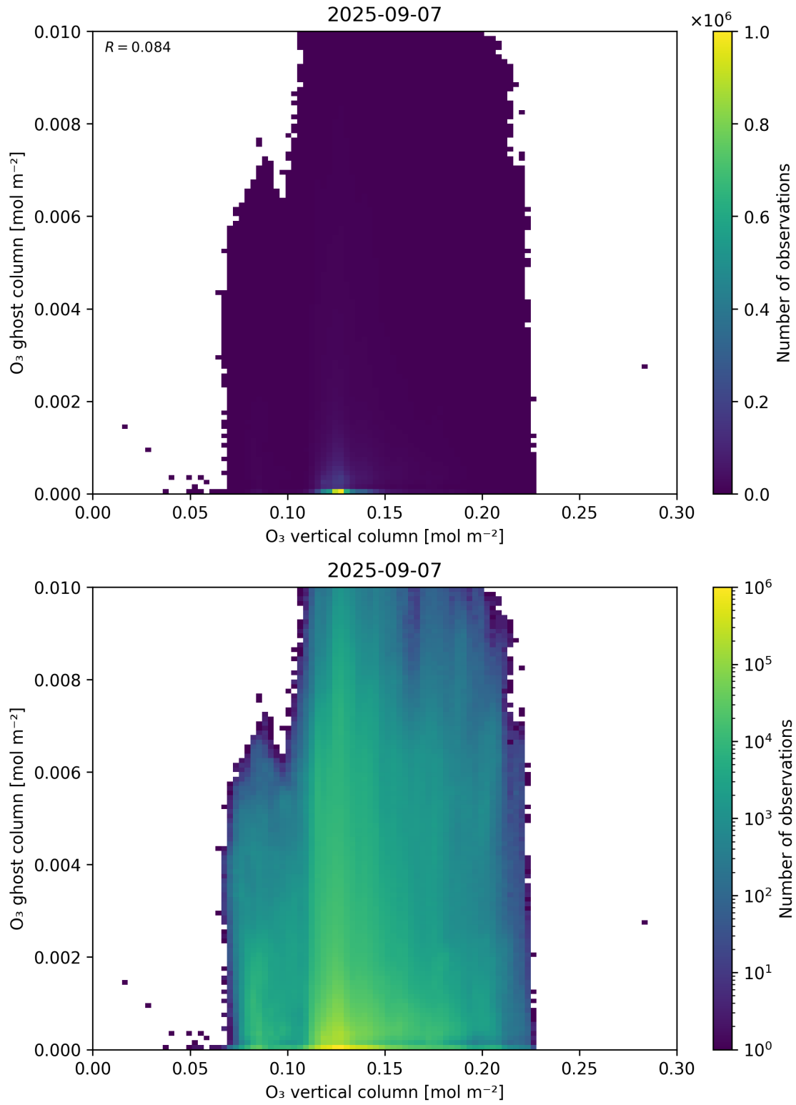
Figure 40: Scatter density plot of “O 3 vertical column” against “O 3 ghost column” for 2025-09-06 to 2025-09-08.
