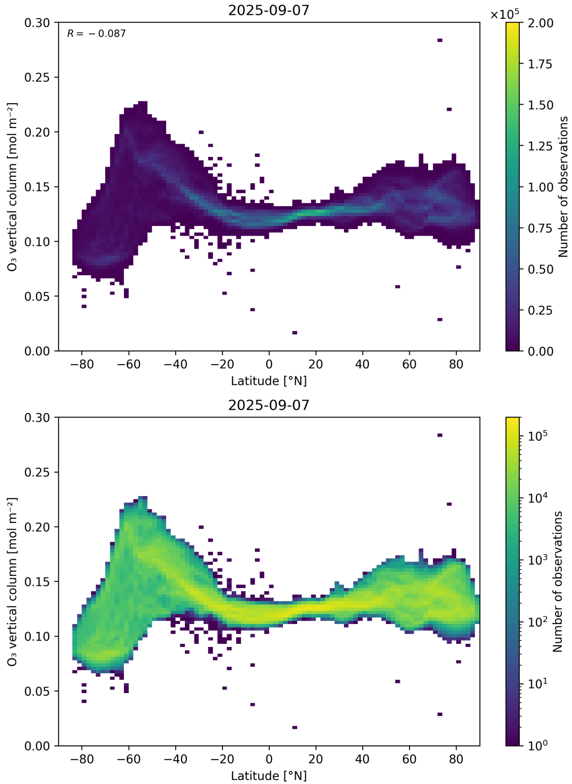
Figure 36: Scatter density plot of “Latitude” against “O 3 vertical column” for 2025-09-06 to 2025-09-08.
