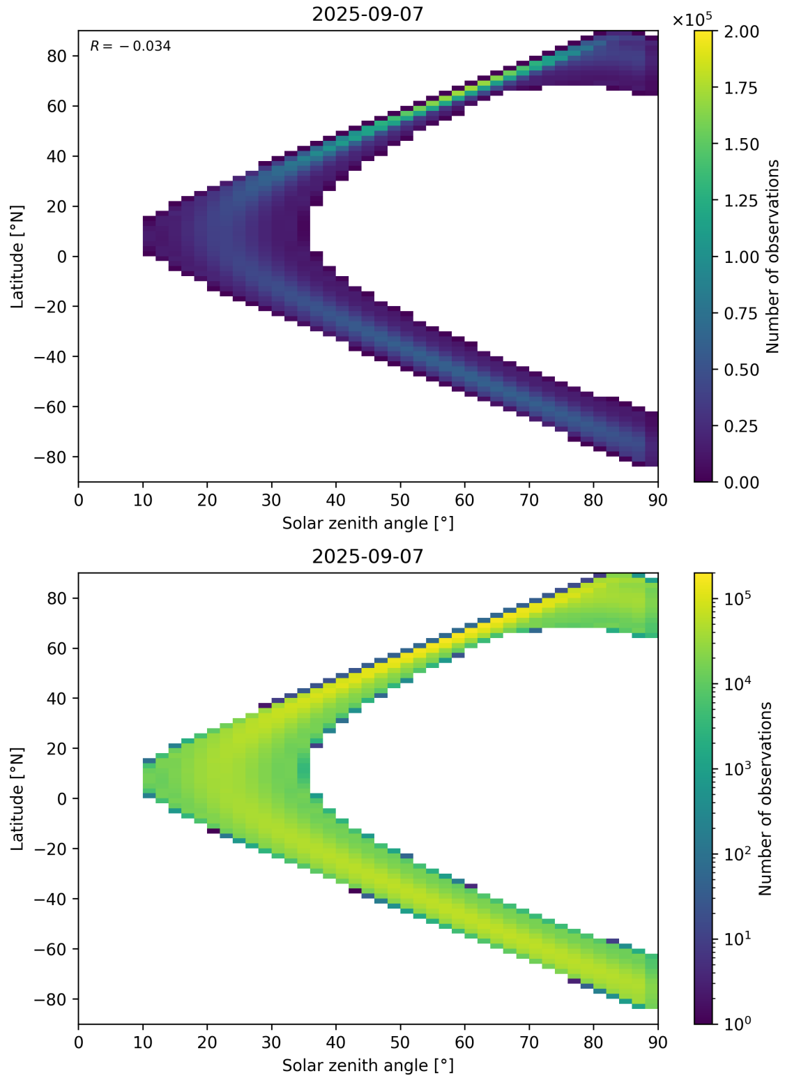
Figure 44: Scatter density plot of “Solar zenith angle” against “Latitude” for 2025-09-06 to 2025-09-08.
