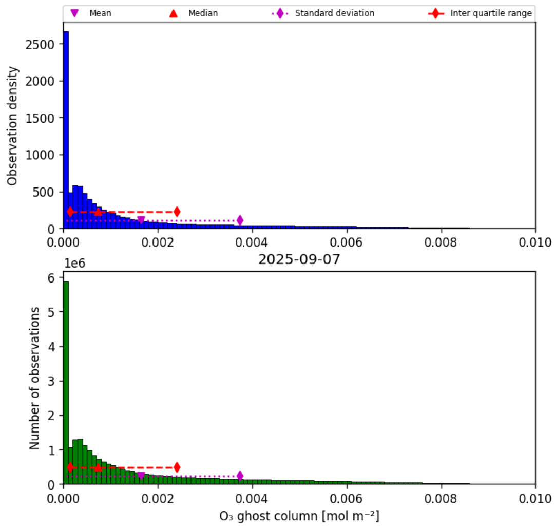
Figure 25: Histogram of “O 3 ghost column” for 2025-09-06 to 2025-09-08
