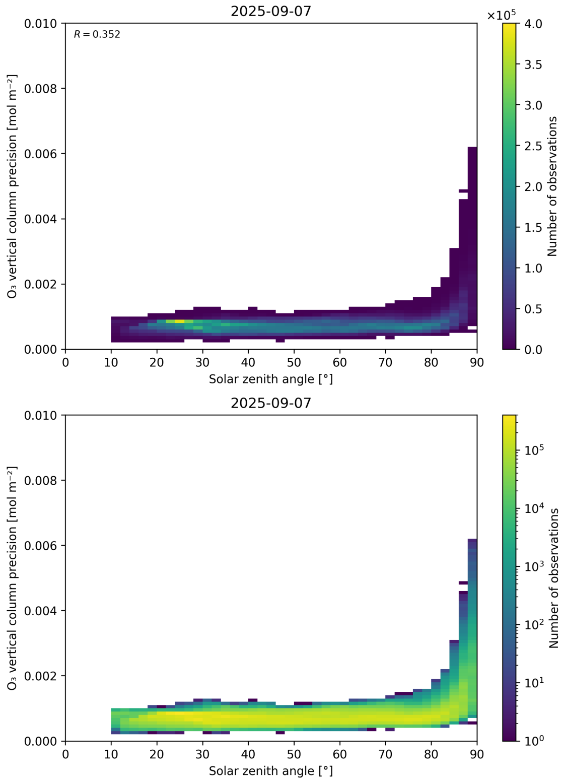
Figure 48: Scatter density plot of “Solar zenith angle” against “O 3 vertical column precision” for 2025-09-06 to 2025-09-08.
