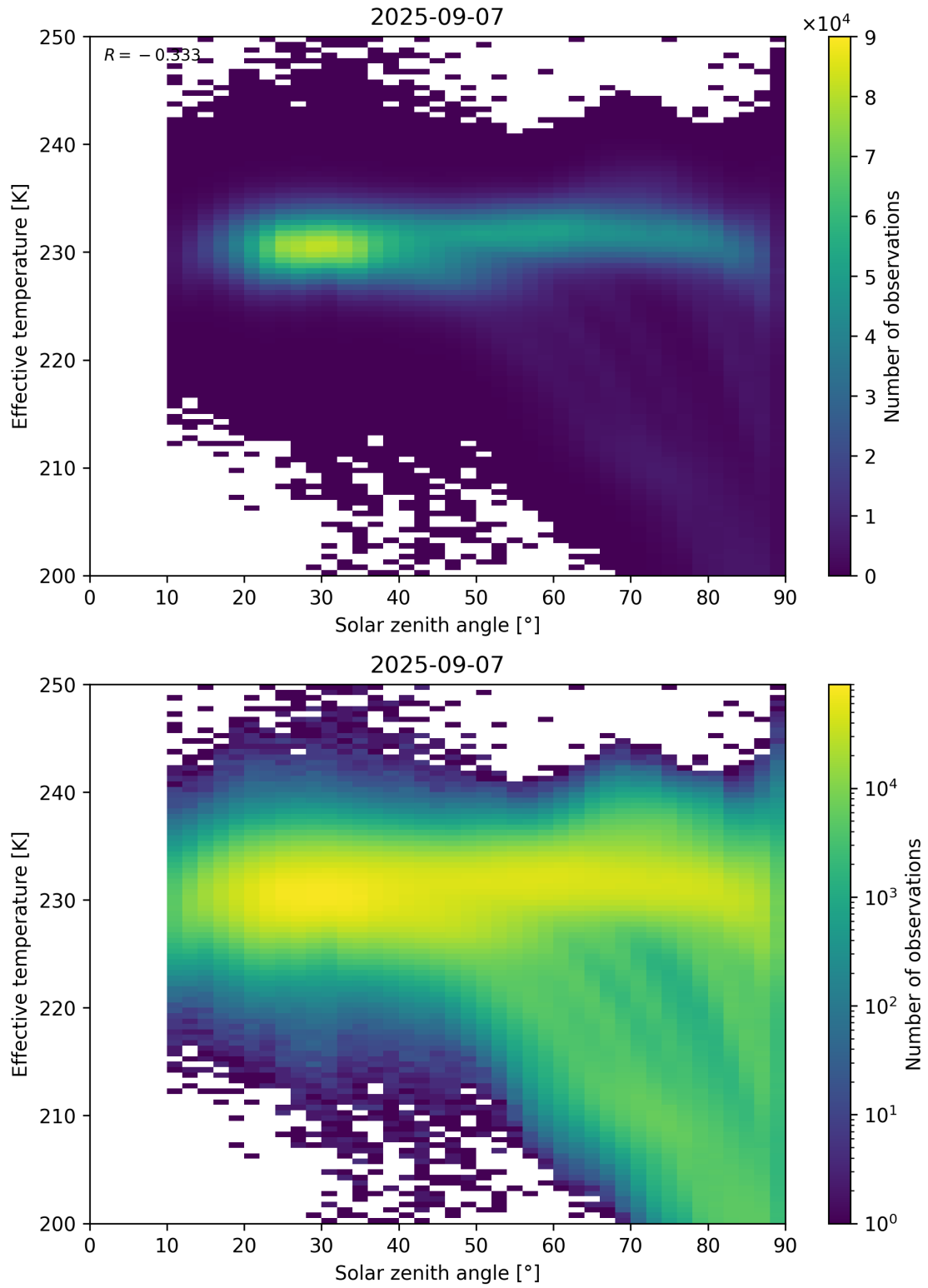
Figure 45: Scatter density plot of “Solar zenith angle” against “Effective temperature” for 2025-09-06 to 2025-09-08.
