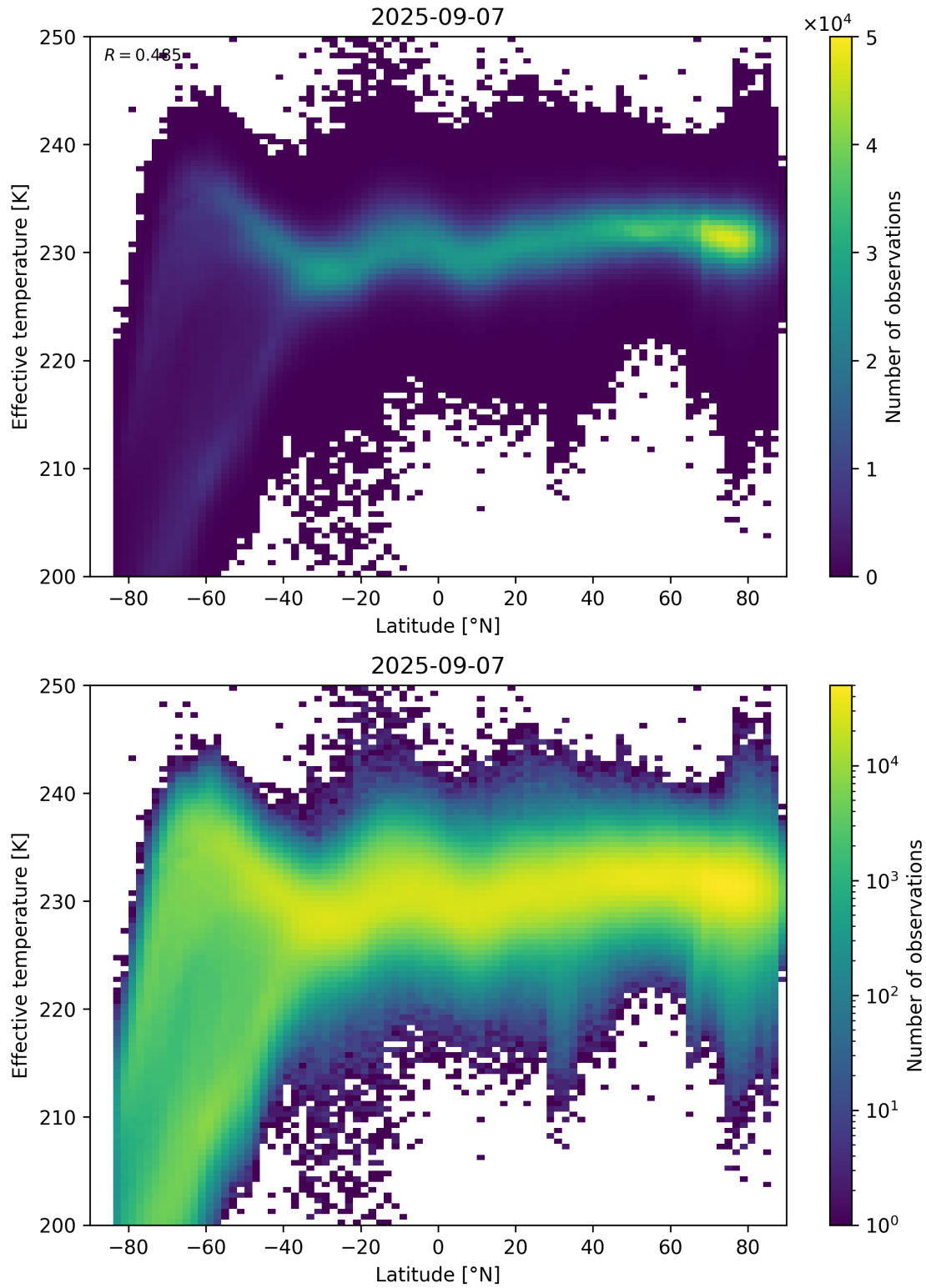
Figure 34: Scatter density plot of “Latitude” against “Effective temperature” for 2025-09-06 to 2025-09-08.
