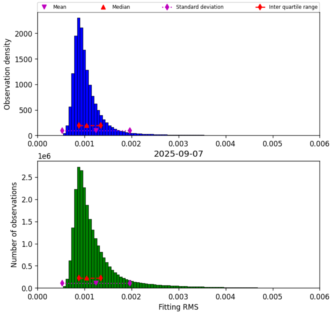
Figure 23: Histogram of “Fitting RMS” for 2025-09-06 to 2025-09-08
