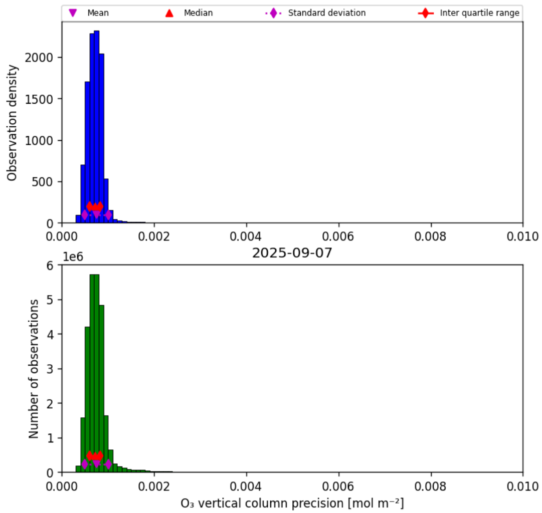
Figure 22: Histogram of “O 3 vertical column precision” for 2025-09-06 to 2025-09-08
