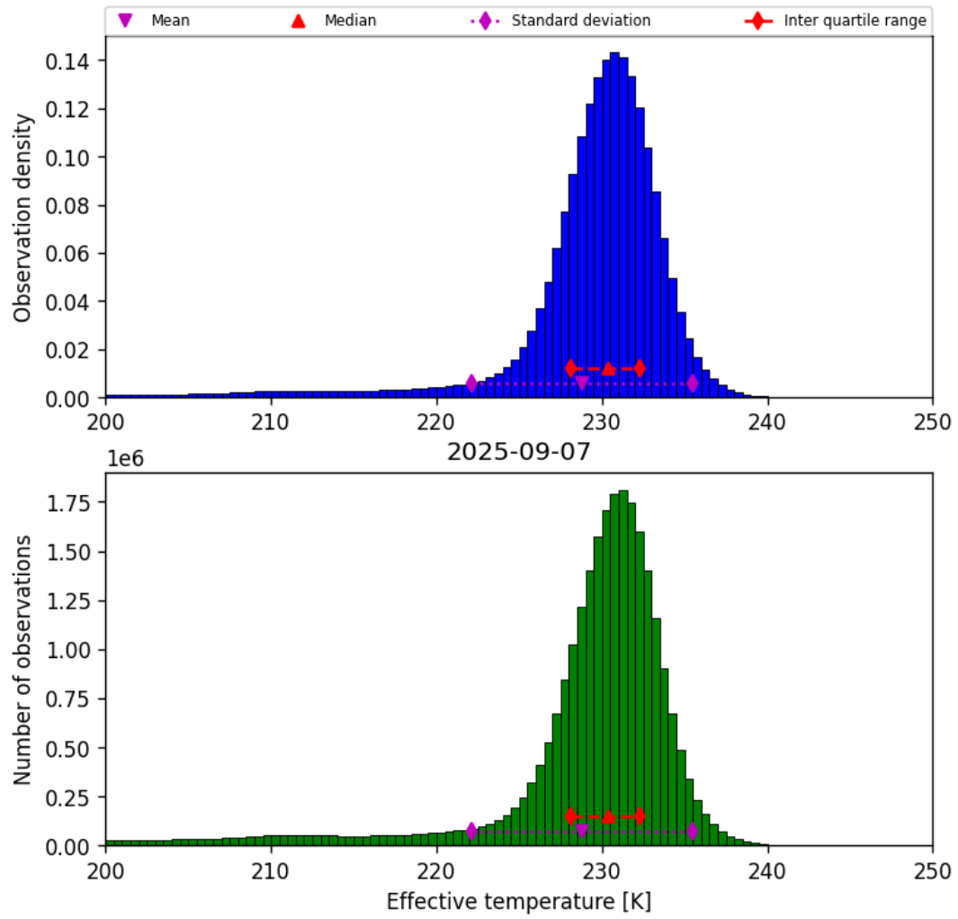
Figure 24: Histogram of “Effective temperature” for 2025-09-06 to 2025-09-08
