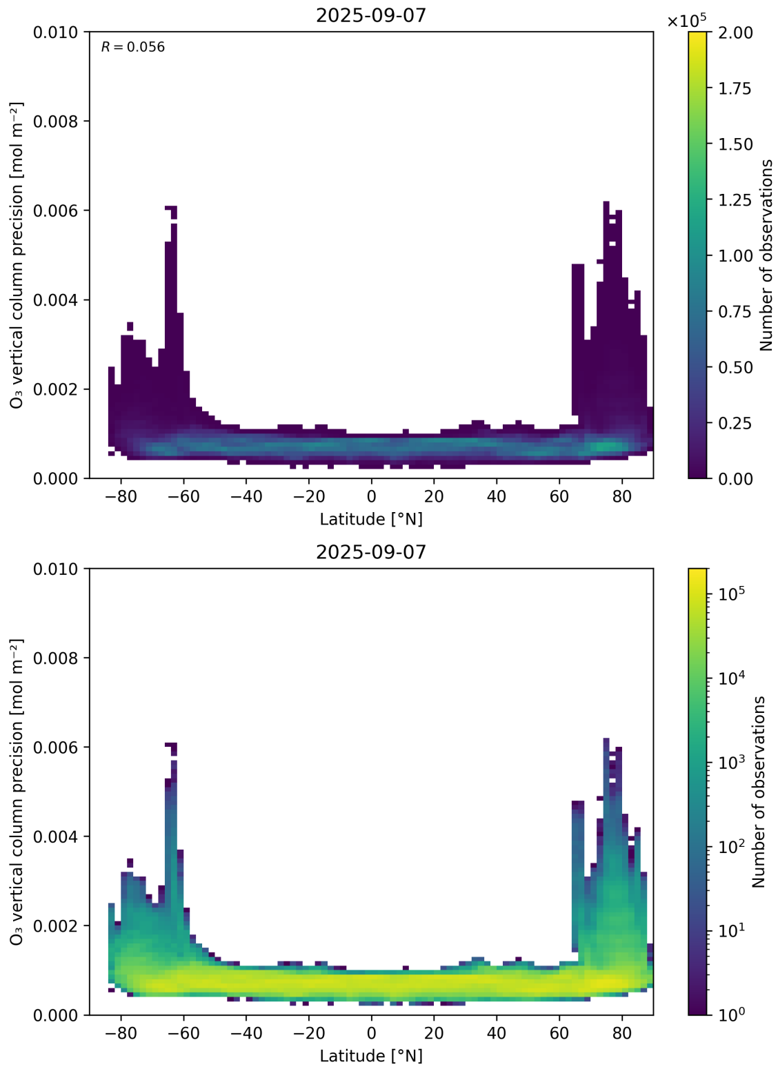
Figure 37: Scatter density plot of “Latitude” against “O 3 vertical column precision” for 2025-09-06 to 2025-09-08.
