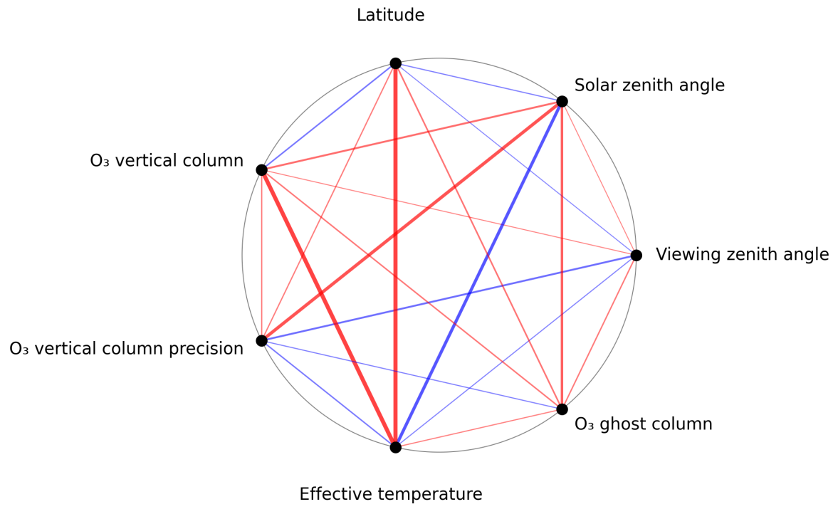
Figure 1: Map of correlation graph for 2025-09-06 to 2025-09-08.
