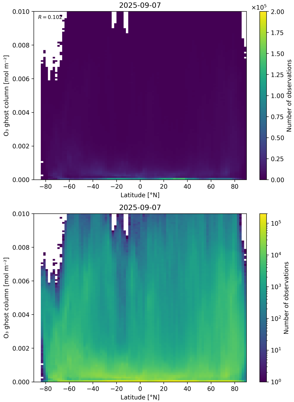
Figure 35: Scatter density plot of “Latitude” against “O 3 ghost column” for 2025-09-06 to 2025-09-08.
