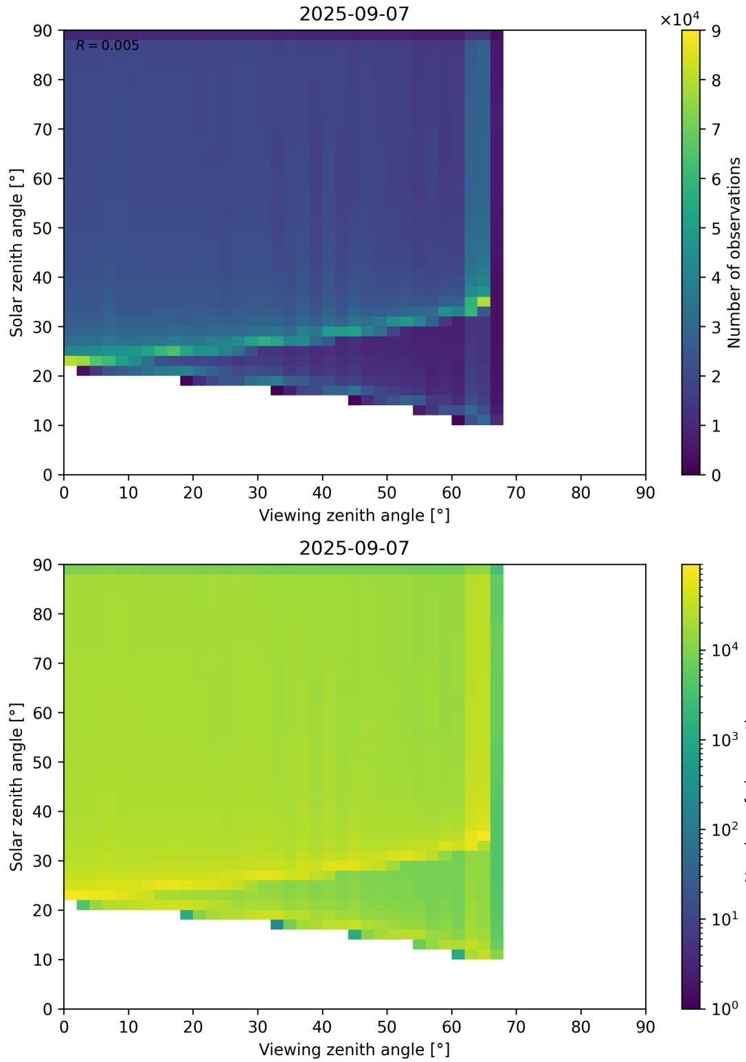
Figure 54: Scatter density plot of “Viewing zenith angle” against “Solar zenith angle” for 2025-09-06 to 2025-09-08.
