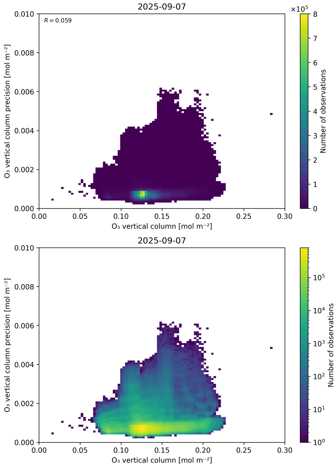
Figure 41: Scatter density plot of “O 3 vertical column” against “O 3 vertical column precision” for 2025-09-06 to 2025-09-08.
