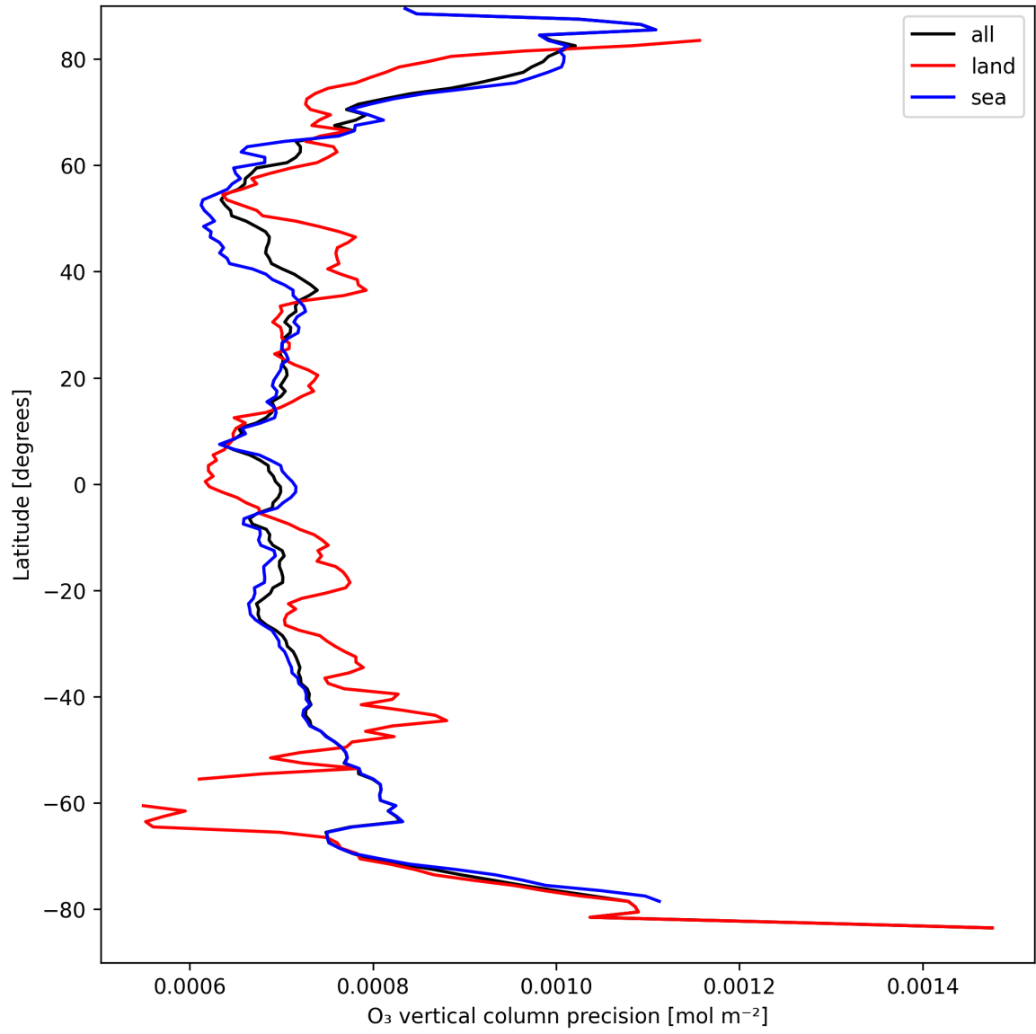
Figure 15: Zonal average of “O 3 vertical column precision” for 2025-09-06 to 2025-09-08.
