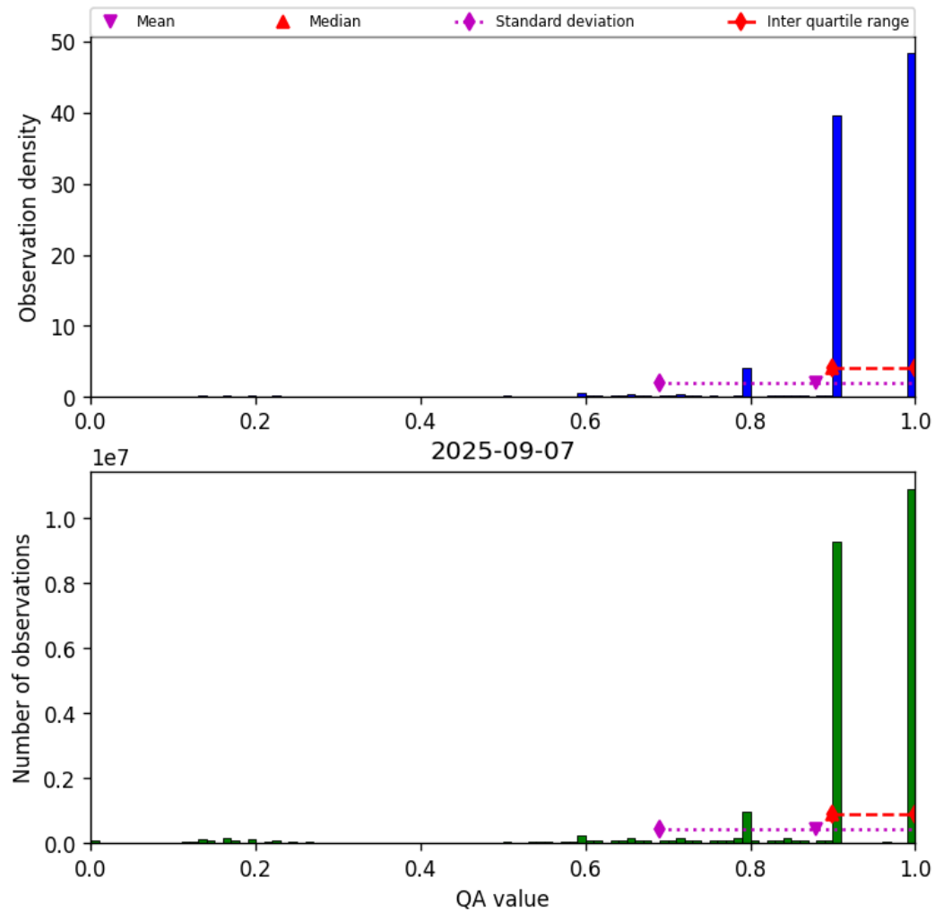
Figure 20: Histogram of “QA value” for 2025-09-06 to 2025-09-08
