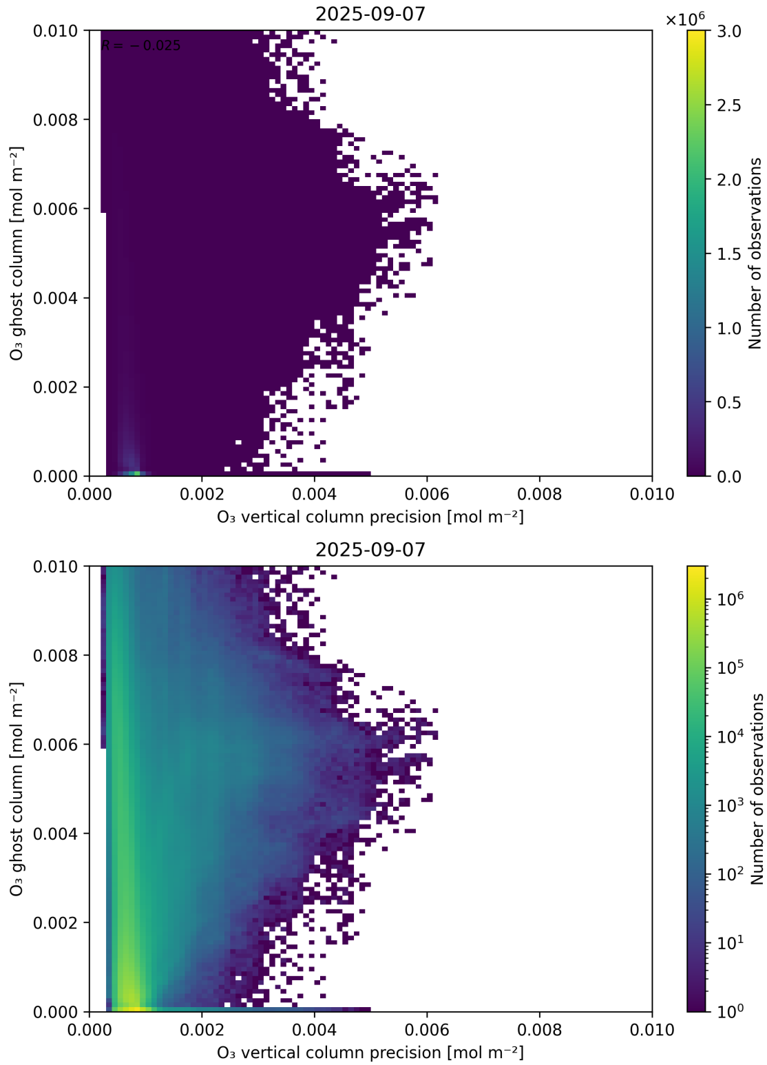
Figure 43: Scatter density plot of “O 3 vertical column precision” against “O 3 ghost column” for 2025-09-06 to 2025-09-08.
