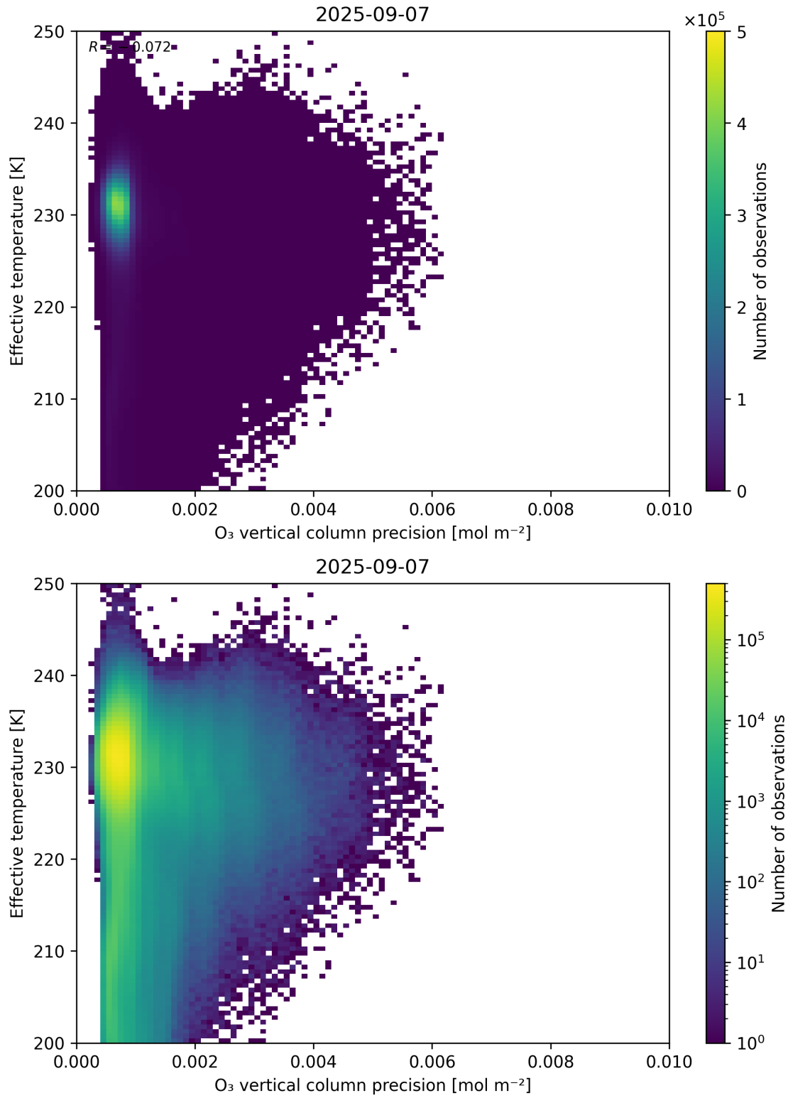
Figure 42: Scatter density plot of “O 3 vertical column precision” against “Effective temperature” for 2025-09-06 to 2025-09-08.
