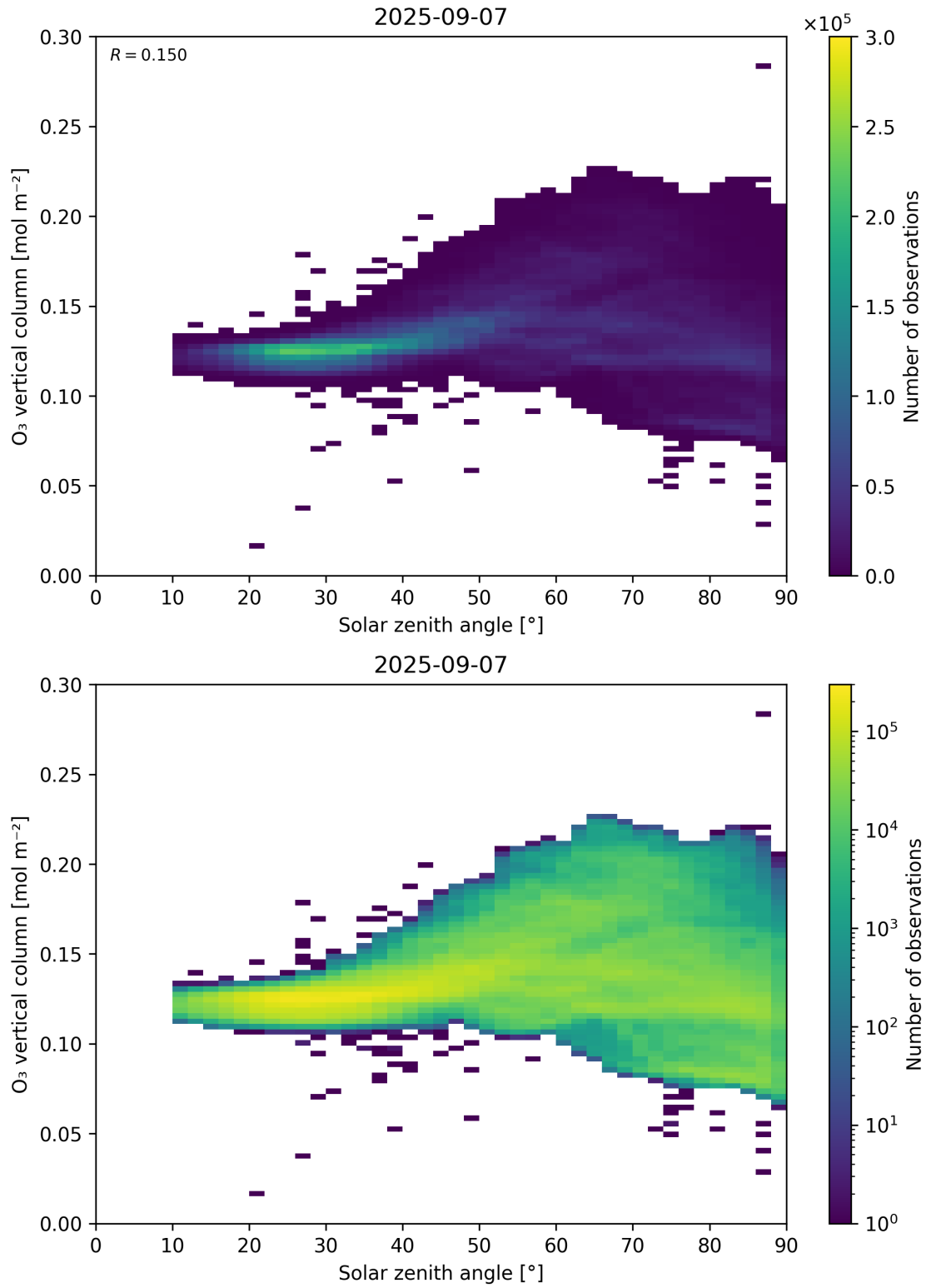
Figure 47: Scatter density plot of “Solar zenith angle” against “O 3 vertical column” for 2025-09-06 to 2025-09-08.
