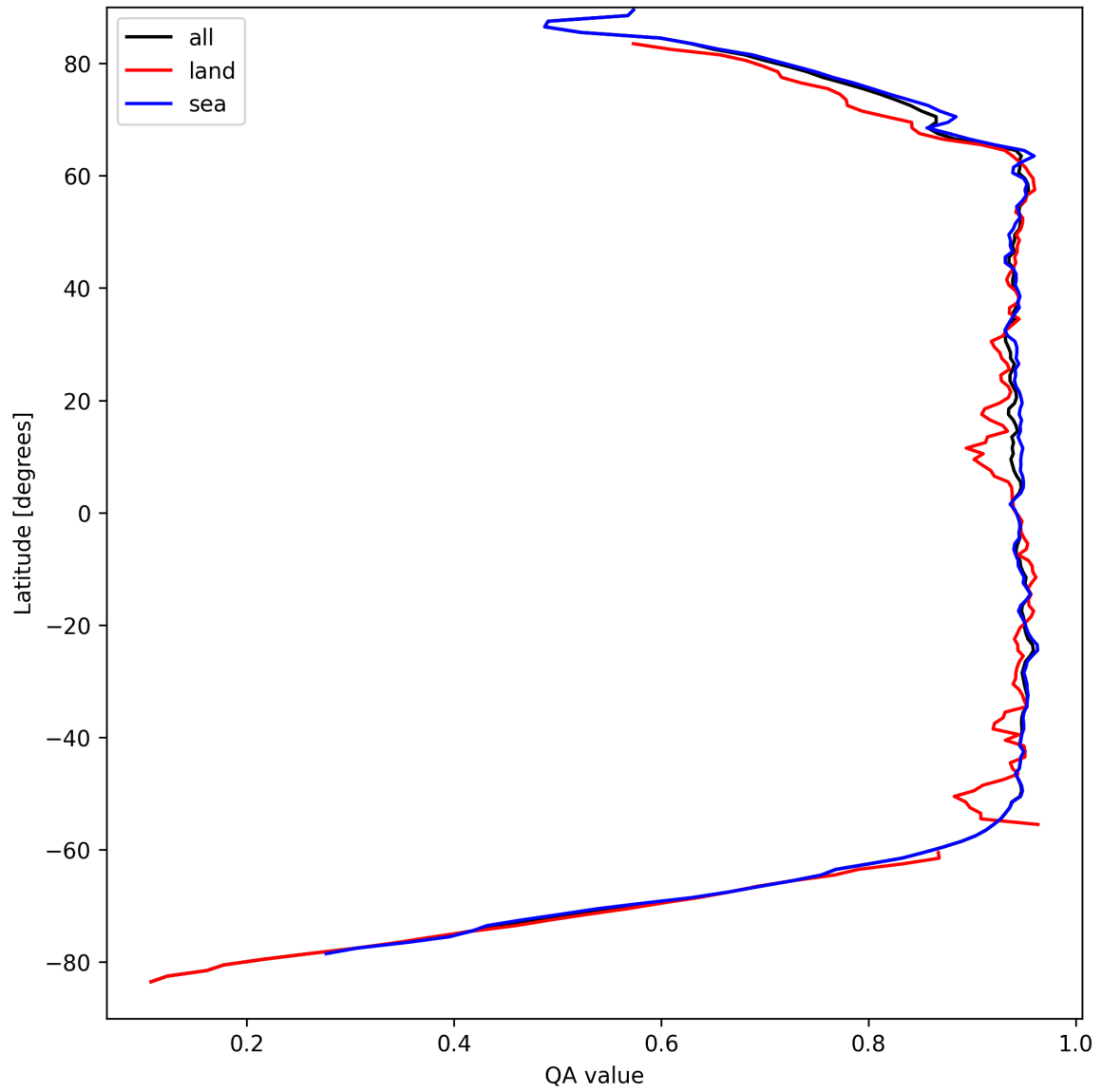
Figure 13: Zonal average of “QA value” for 2025-09-06 to 2025-09-08.
