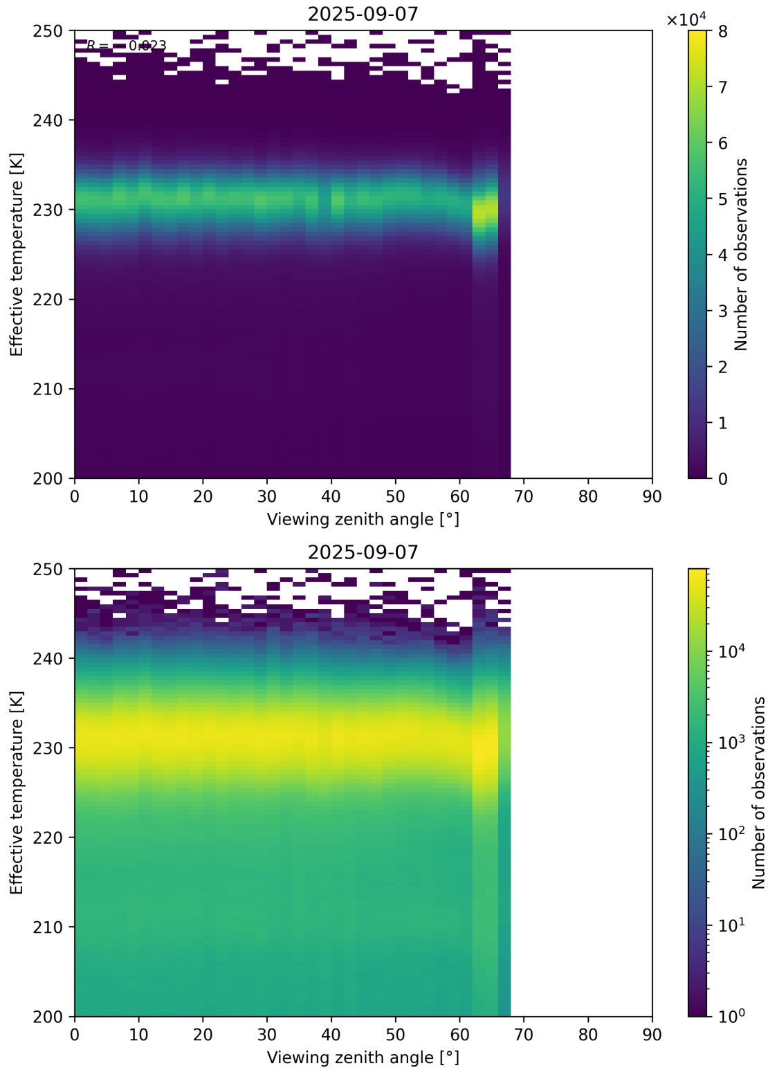
Figure 50: Scatter density plot of “Viewing zenith angle” against “Effective temperature” for 2025-09-06 to 2025-09-08.
