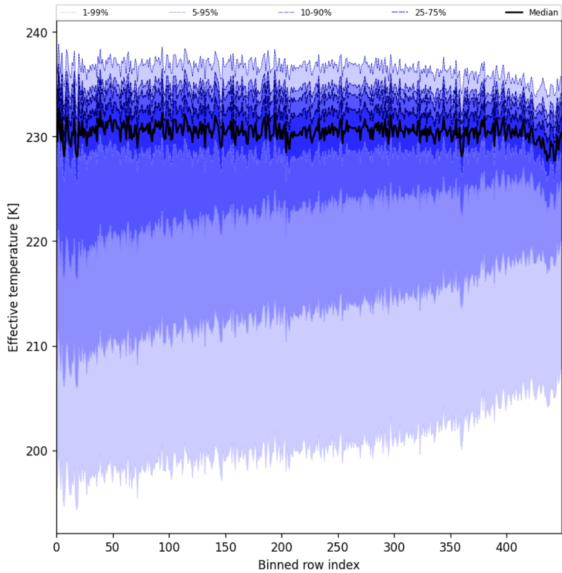
Figure 31: Along track statistics of “Effective temperature” for 2025-09-06 to 2025-09-08
