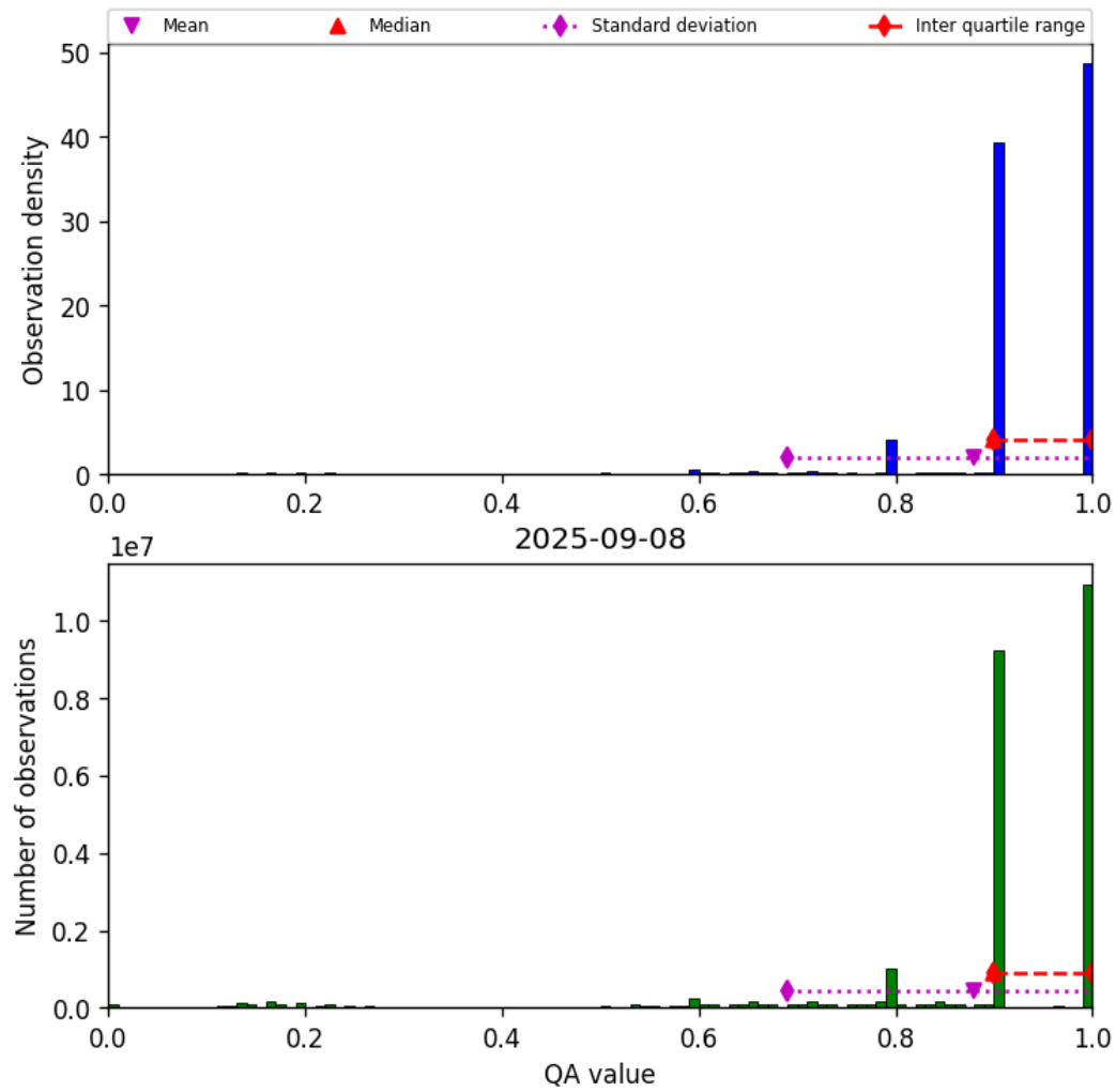
Figure 20: Histogram of “QA value” for 2025-09-07 to 2025-09-09
