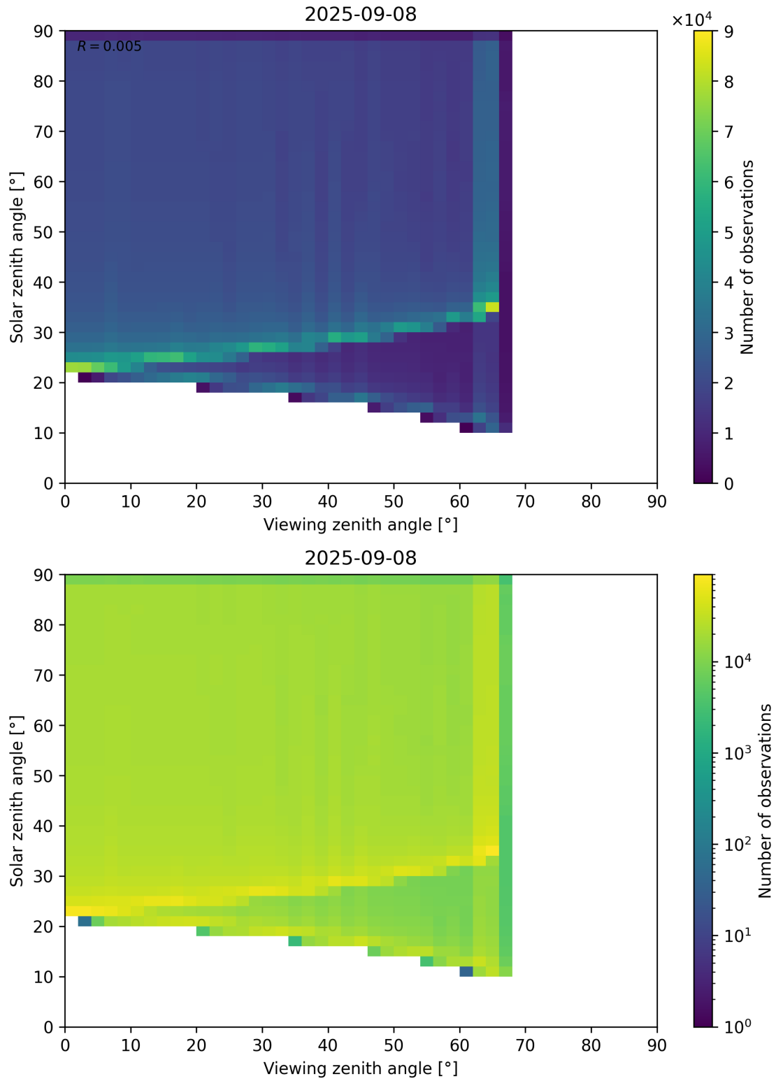
Figure 54: Scatter density plot of “Viewing zenith angle” against “Solar zenith angle” for 2025-09-07 to 2025-09-09.
