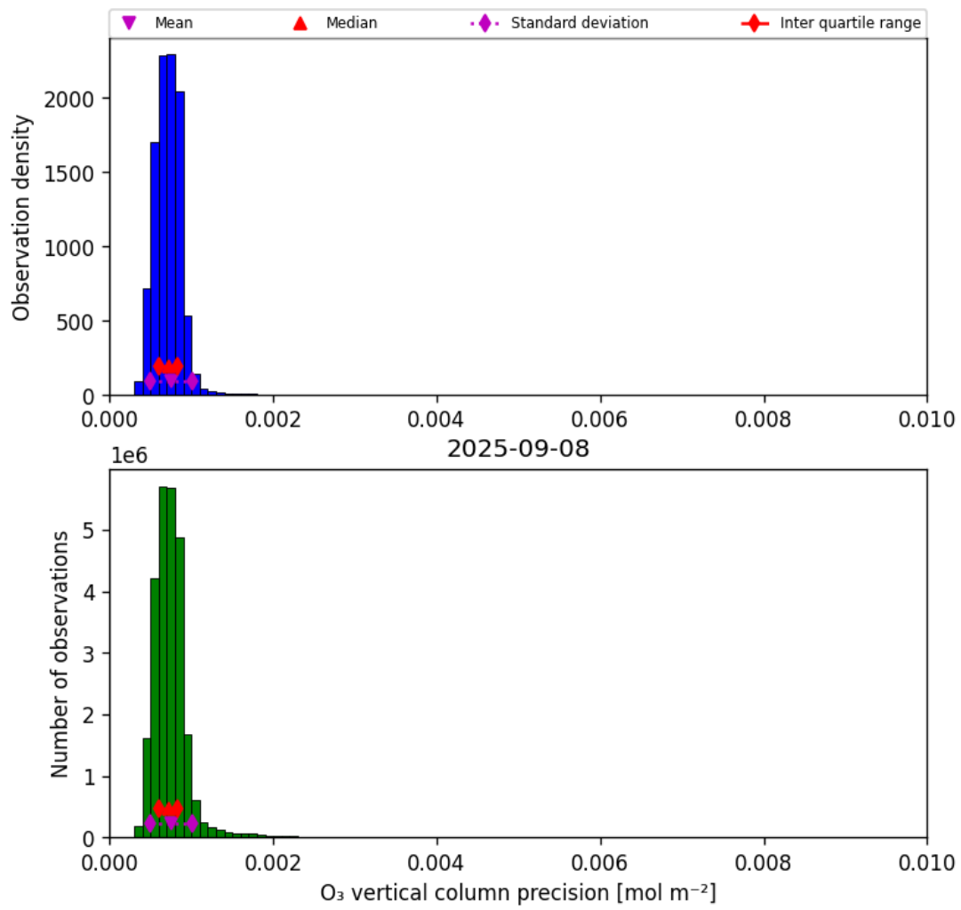
Figure 22: Histogram of "O 3 vertical column precision" for 2025-09-07 to 2025-09-09
