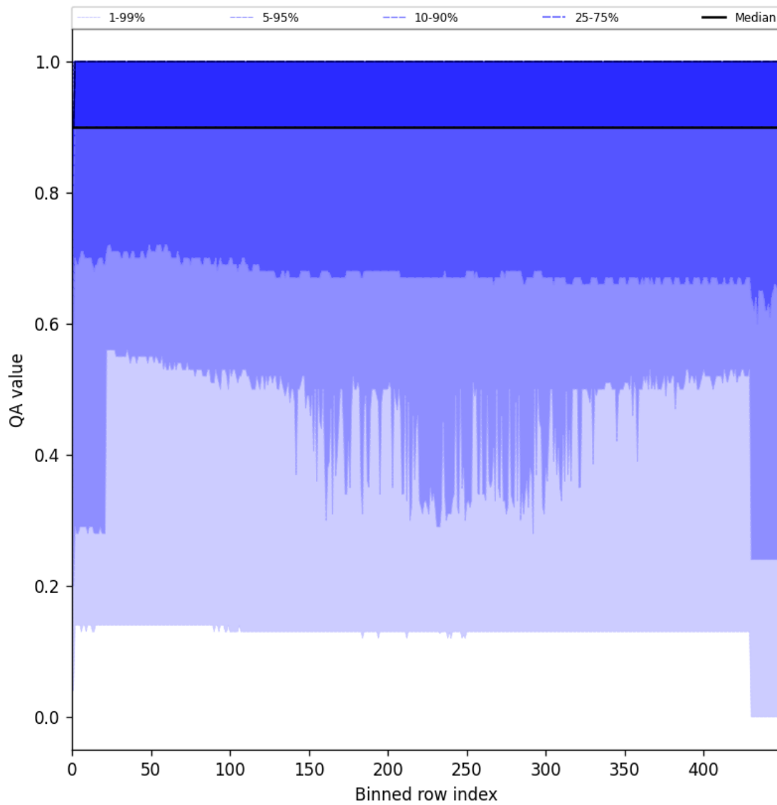
Figure 27: Along track statistics of “QA value” for 2025-09-07 to 2025-09-09
