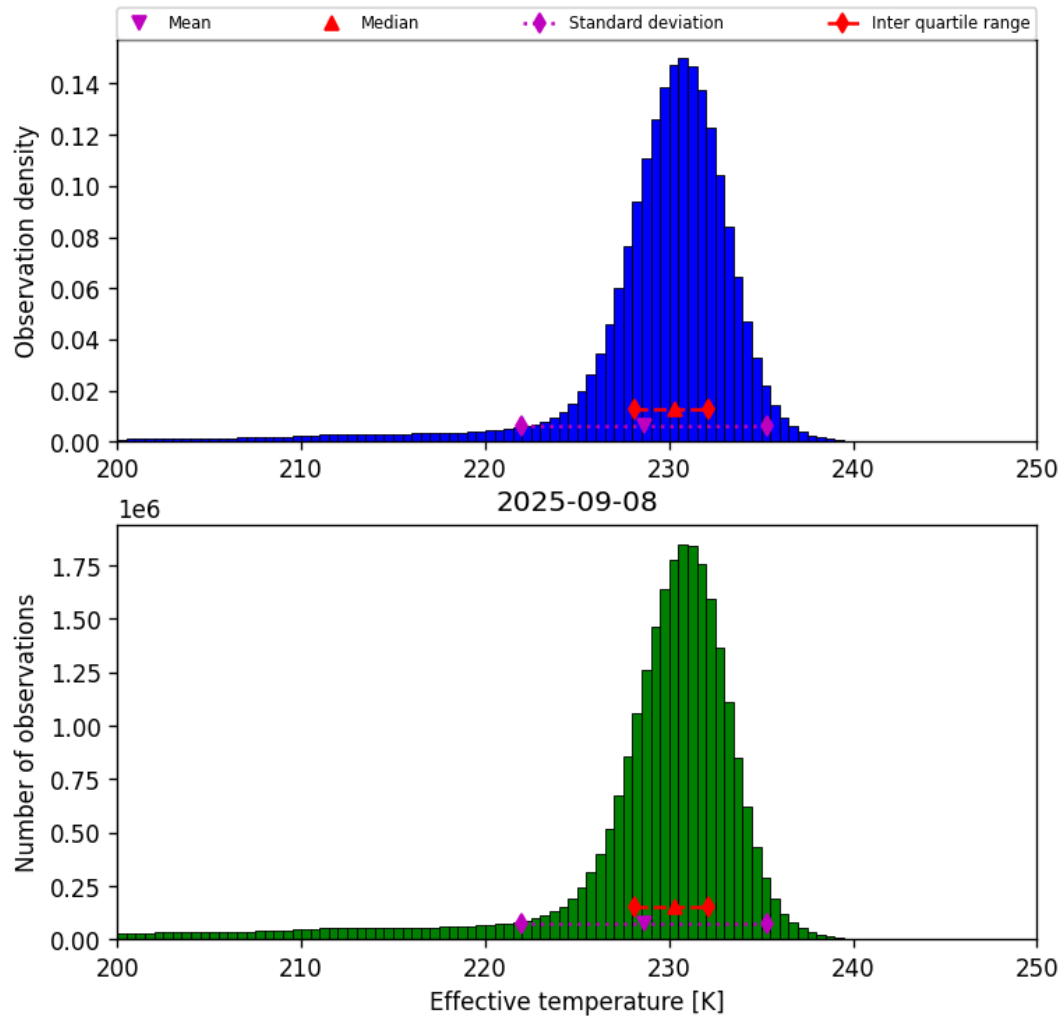
Figure 24: Histogram of “Effective temperature” for 2025-09-07 to 2025-09-09
