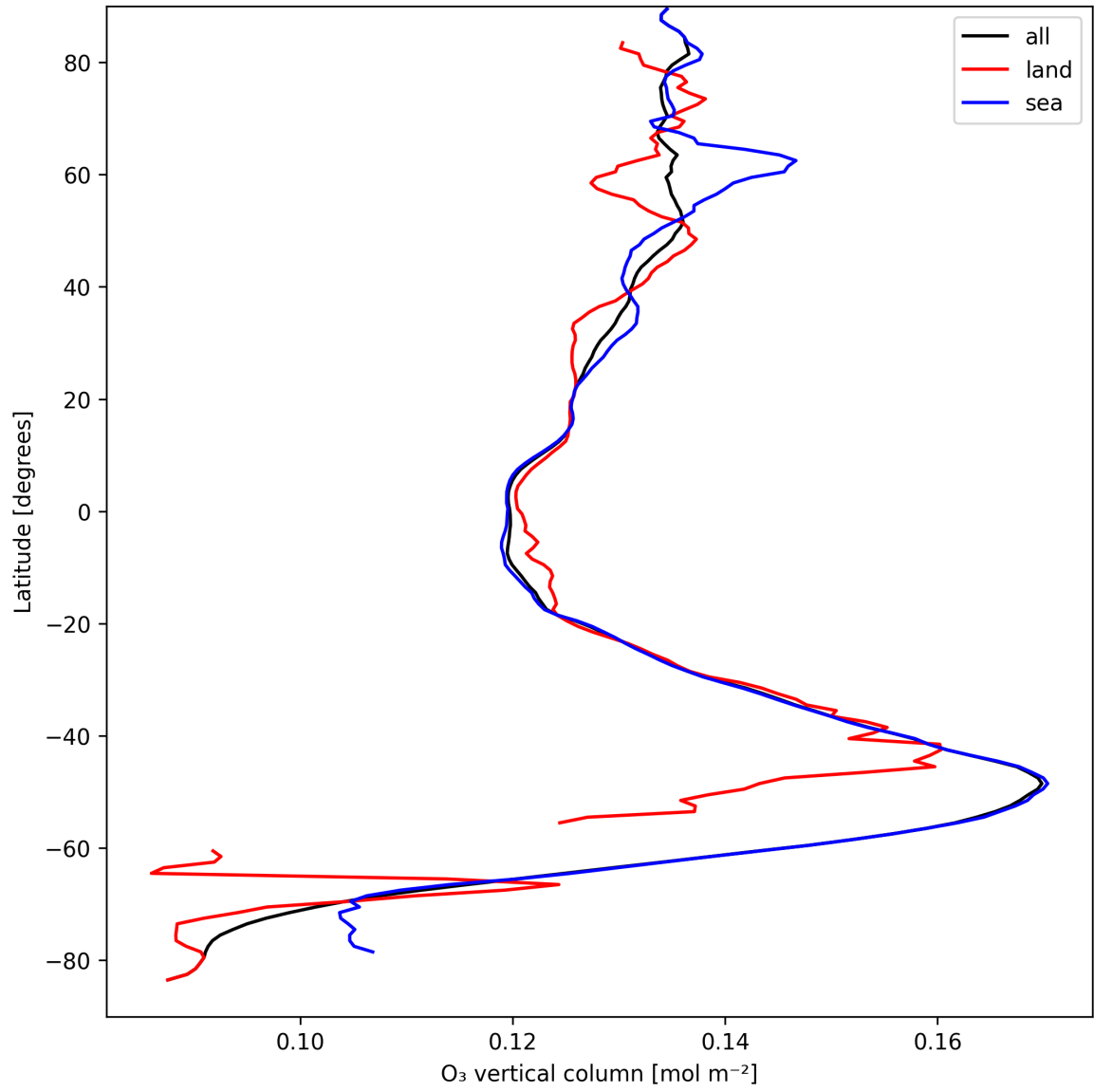
Figure 14: Zonal average of “O 3 vertical column” for 2025-09-07 to 2025-09-09.
