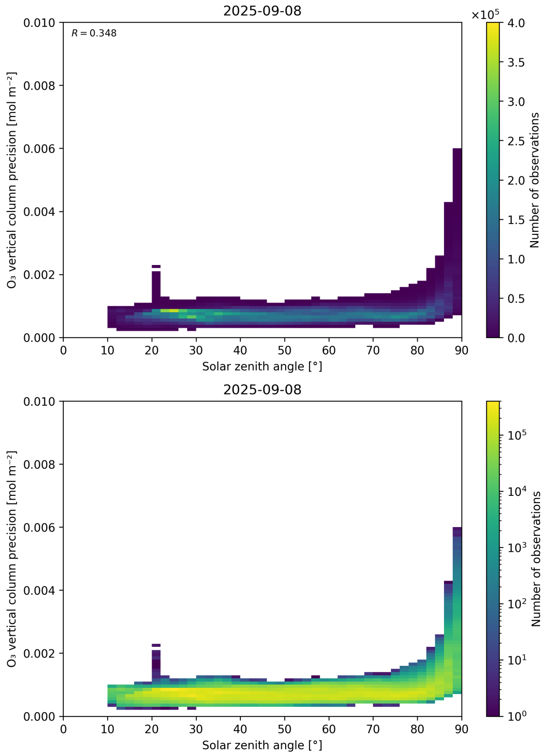
Figure 48: Scatter density plot of “Solar zenith angle” against “O 3 vertical column precision” for 2025-09-07 to 2025-09-09.
