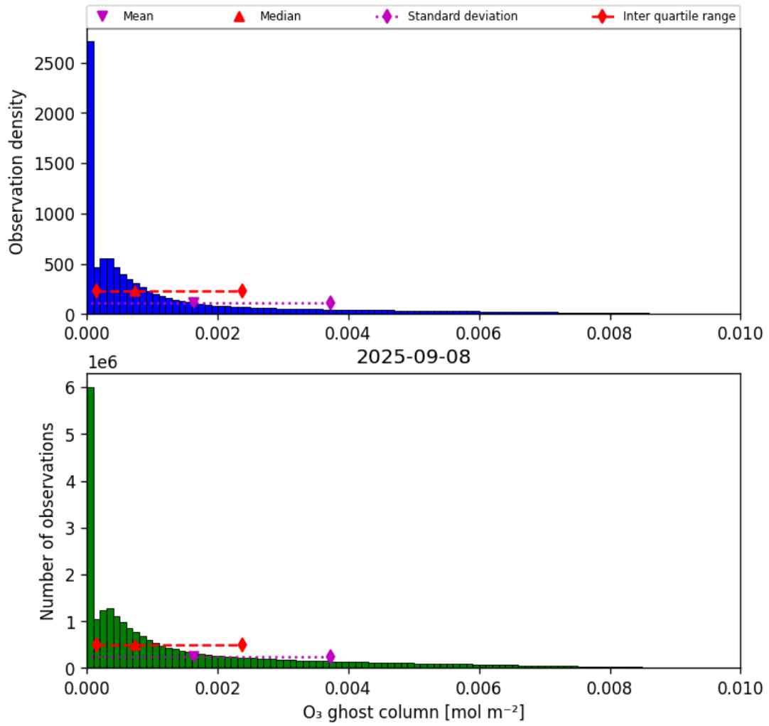
Figure 25: Histogram of “O 3 ghost column” for 2025-09-07 to 2025-09-09
