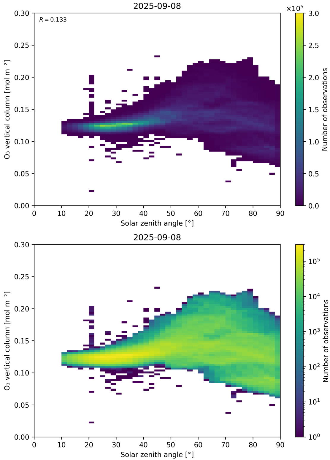
Figure 47: Scatter density plot of “Solar zenith angle” against “O 3 vertical column” for 2025-09-07 to 2025-09-09.
