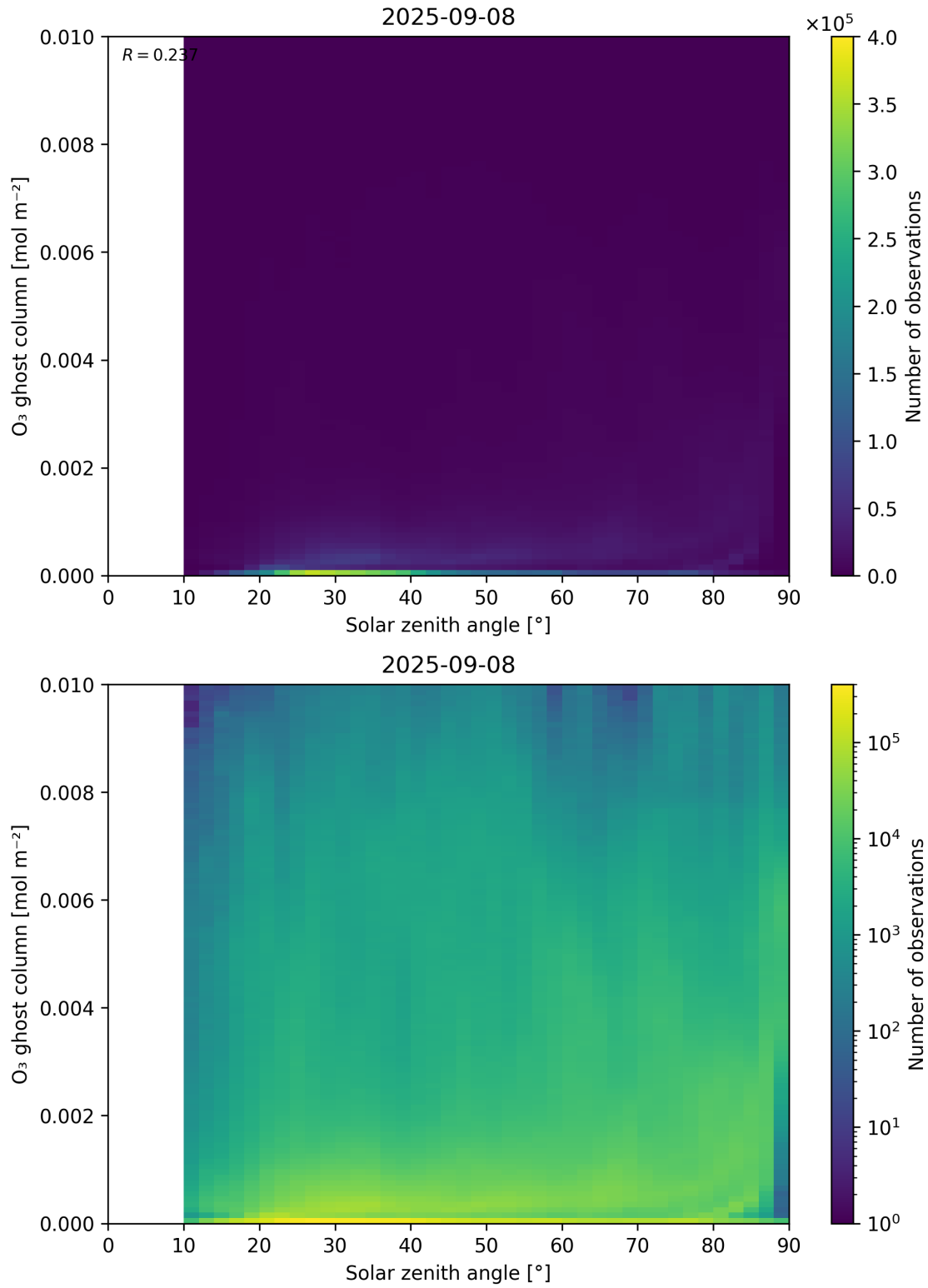
Figure 46: Scatter density plot of “Solar zenith angle” against “O 3 ghost column” for 2025-09-07 to 2025-09-09.
