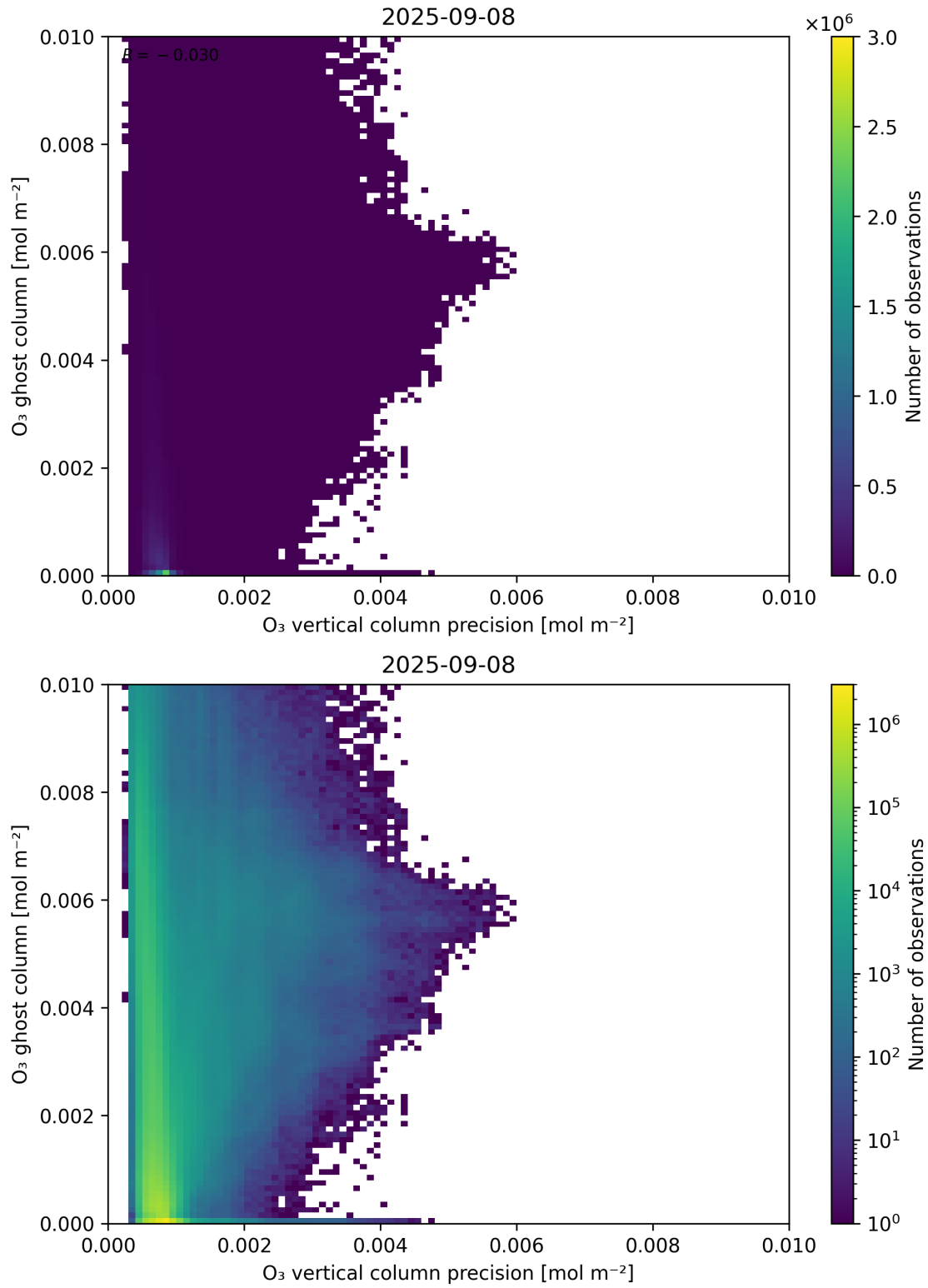
Figure 43: Scatter density plot of “O 3 vertical column precision” against “O 3 ghost column” for 2025-09-07 to 2025-09-09.
