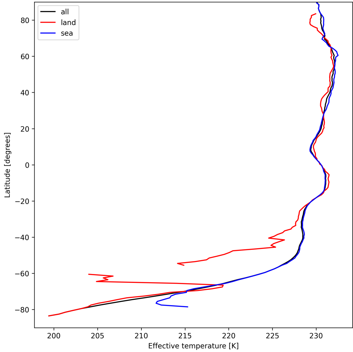
Figure 17: Zonal average of "Effective temperature" for 2025-09-07 to 2025-09-09.
