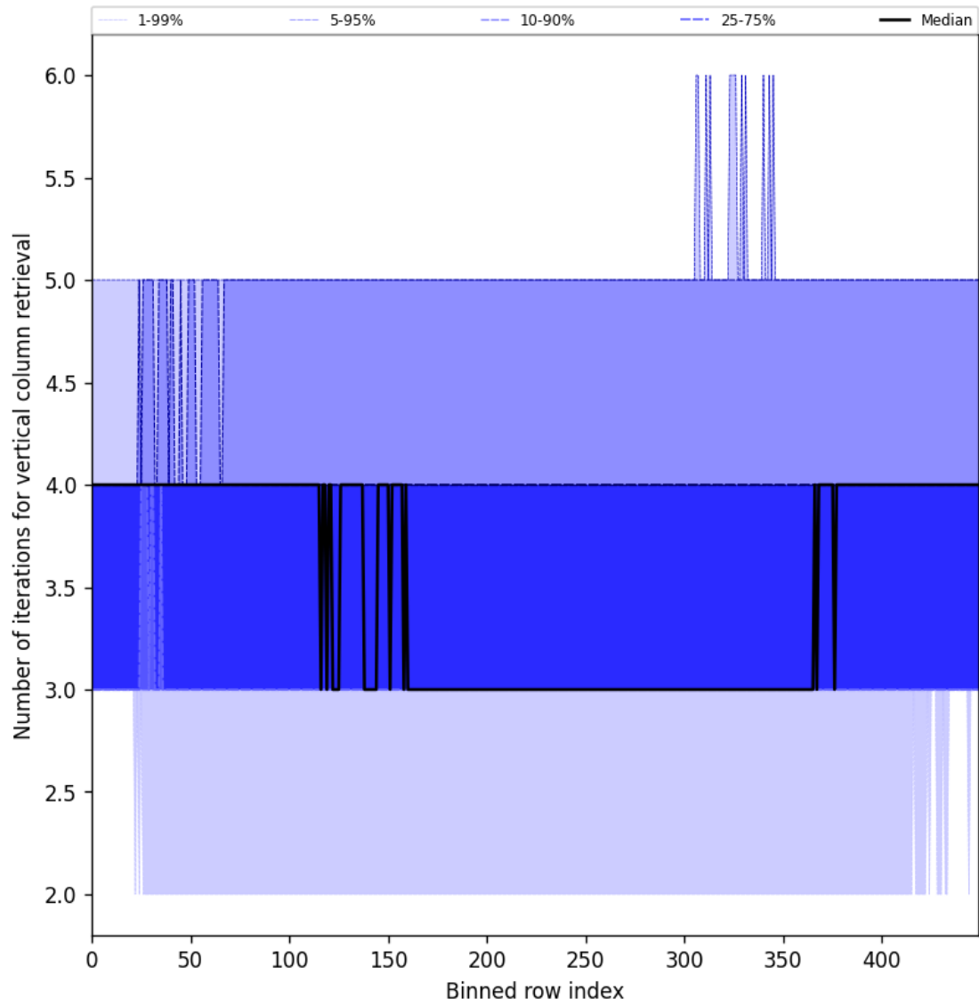
Figure 33: Along track statistics of “Number of iterations for vertical column retrieval” for 2025-09-07 to 2025-09-09
