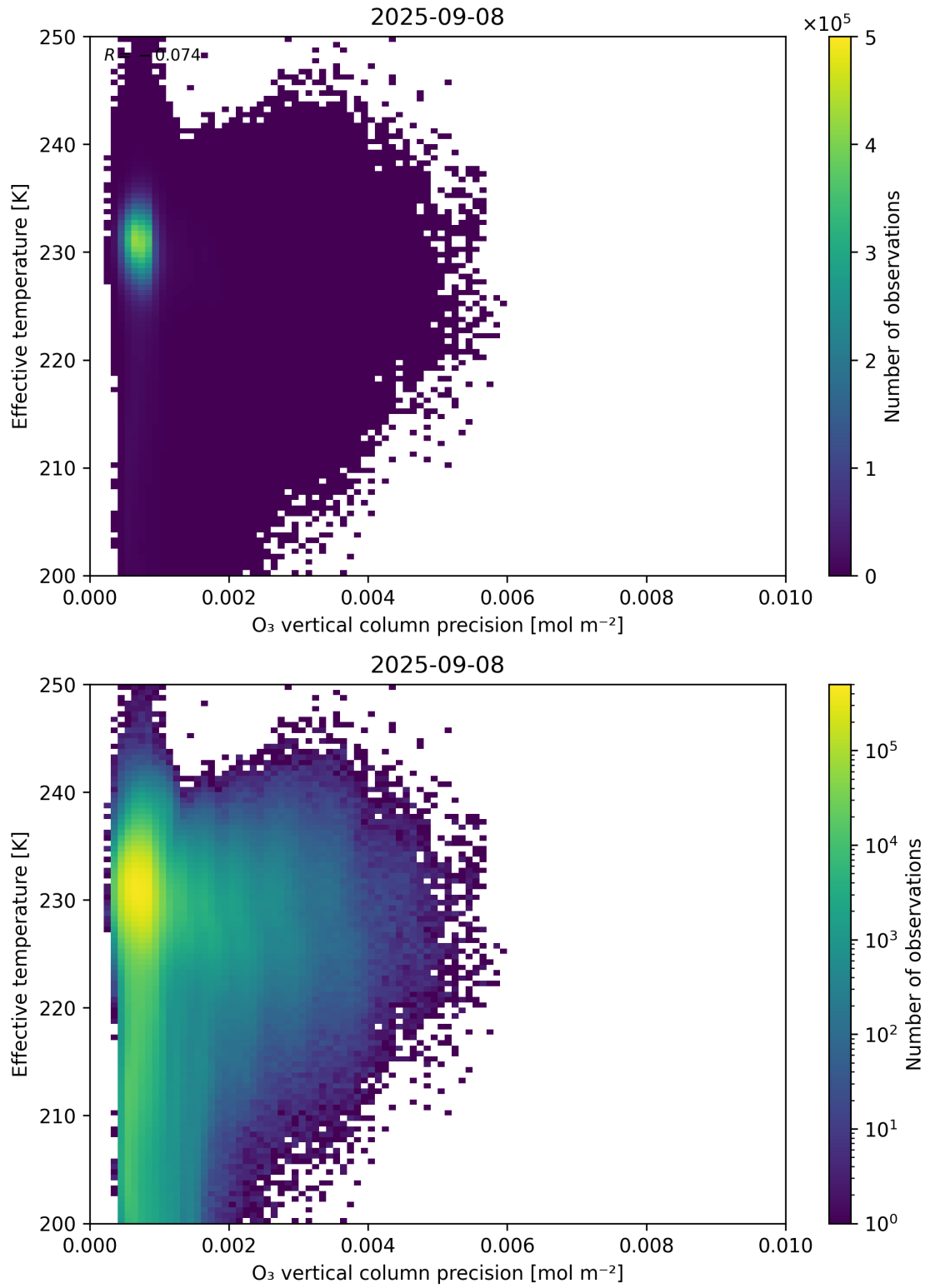
Figure 42: Scatter density plot of “ O_3 vertical column precision” against “Effective temperature” for 2025-09-07 to 2025-09-09.
