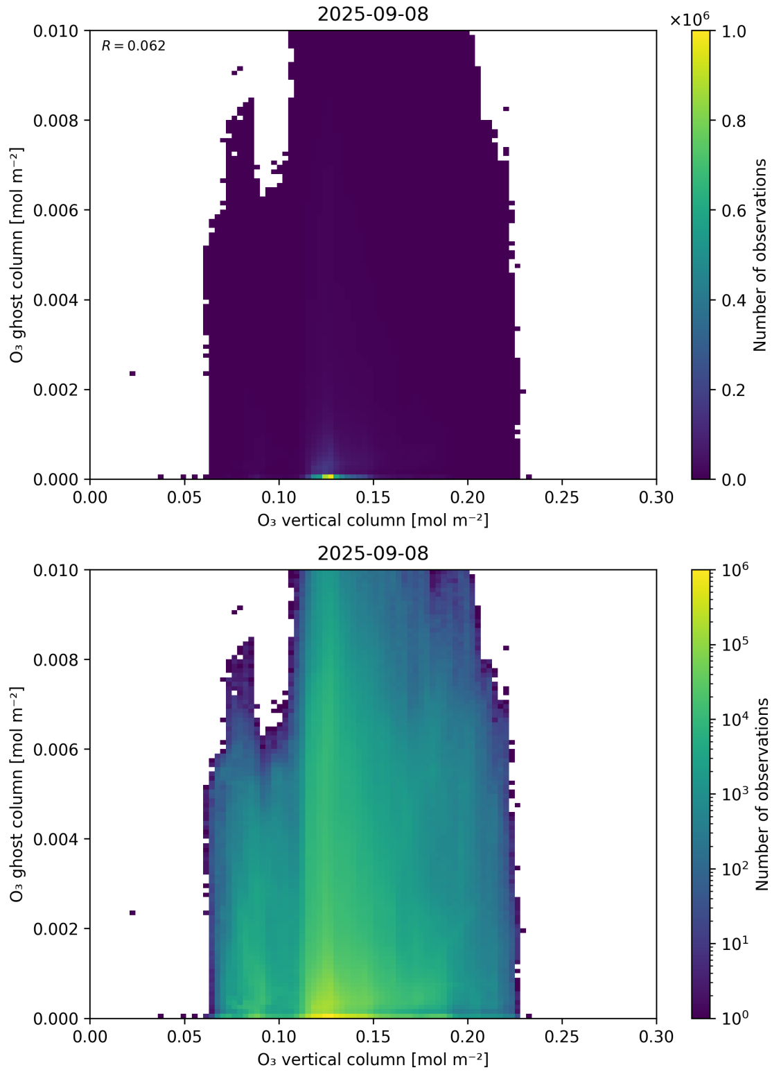
Figure 40: Scatter density plot of “O 3 vertical column” against “O 3 ghost column” for 2025-09-07 to 2025-09-09.
