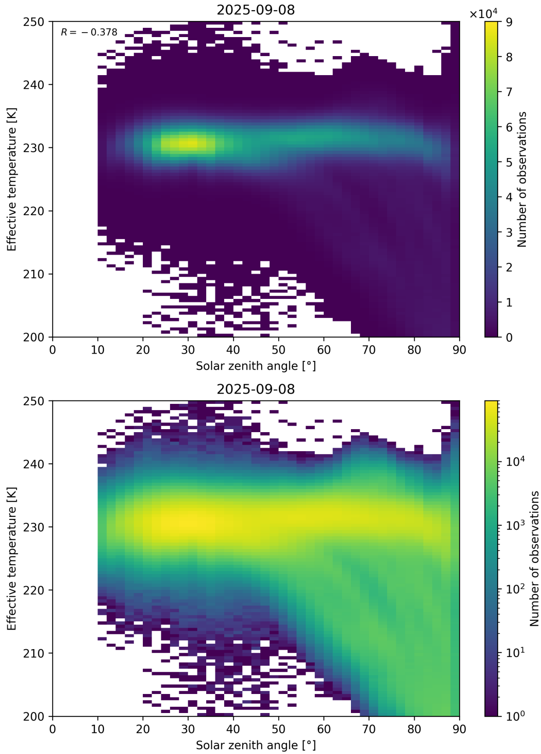
Figure 45: Scatter density plot of “Solar zenith angle” against “Effective temperature” for 2025-09-07 to 2025-09-09.
