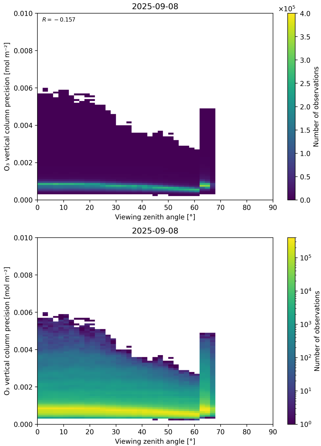
Figure 53: Scatter density plot of “Viewing zenith angle” against “O 3 vertical column precision” for 2025-09-07 to 2025-09-09.
