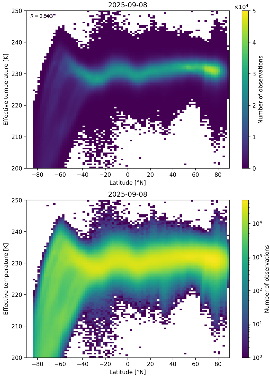
Figure 34: Scatter density plot of “Latitude” against “Effective temperature” for 2025-09-07 to 2025-09-09.
