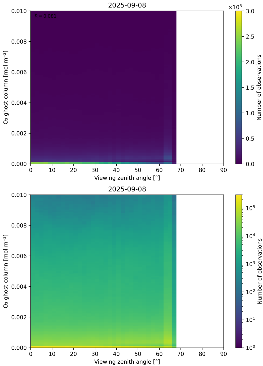
Figure 51: Scatter density plot of “Viewing zenith angle” against “O 3 ghost column” for 2025-09-07 to 2025-09-09.
