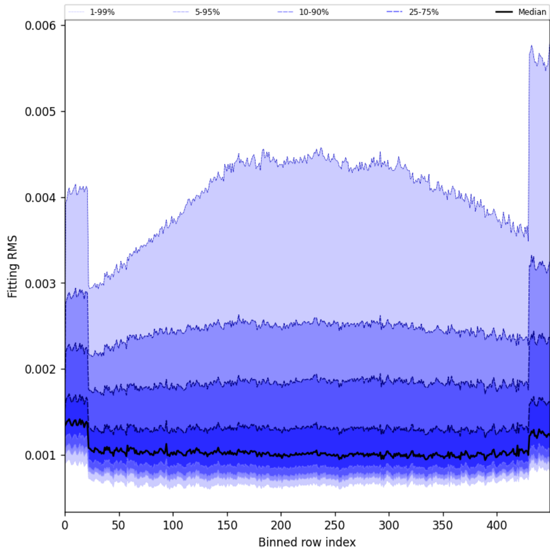
Figure 30: Along track statistics of “Fitting RMS” for 2025-09-07 to 2025-09-09
