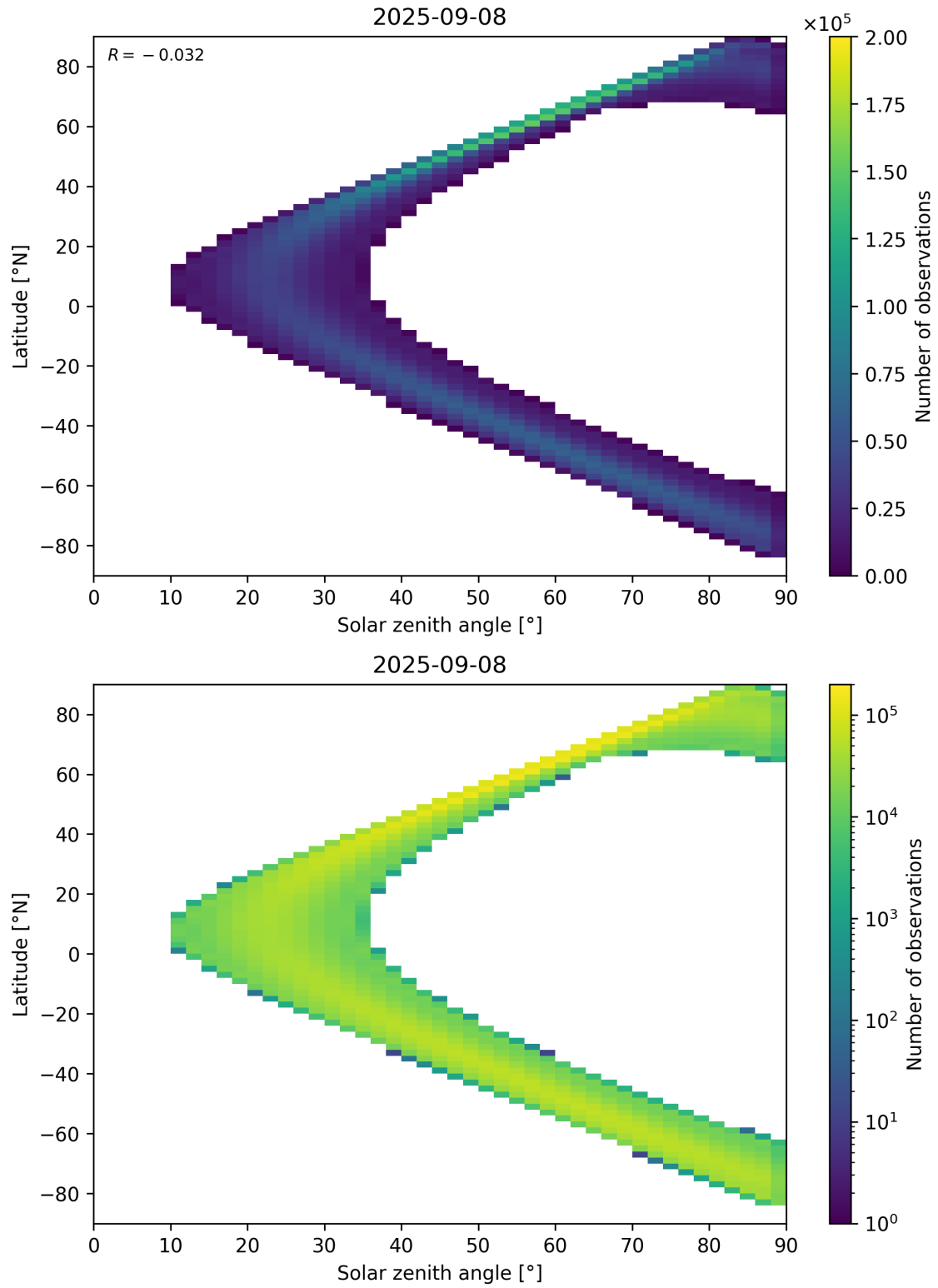
Figure 44: Scatter density plot of “Solar zenith angle” against “Latitude” for 2025-09-07 to 2025-09-09.
