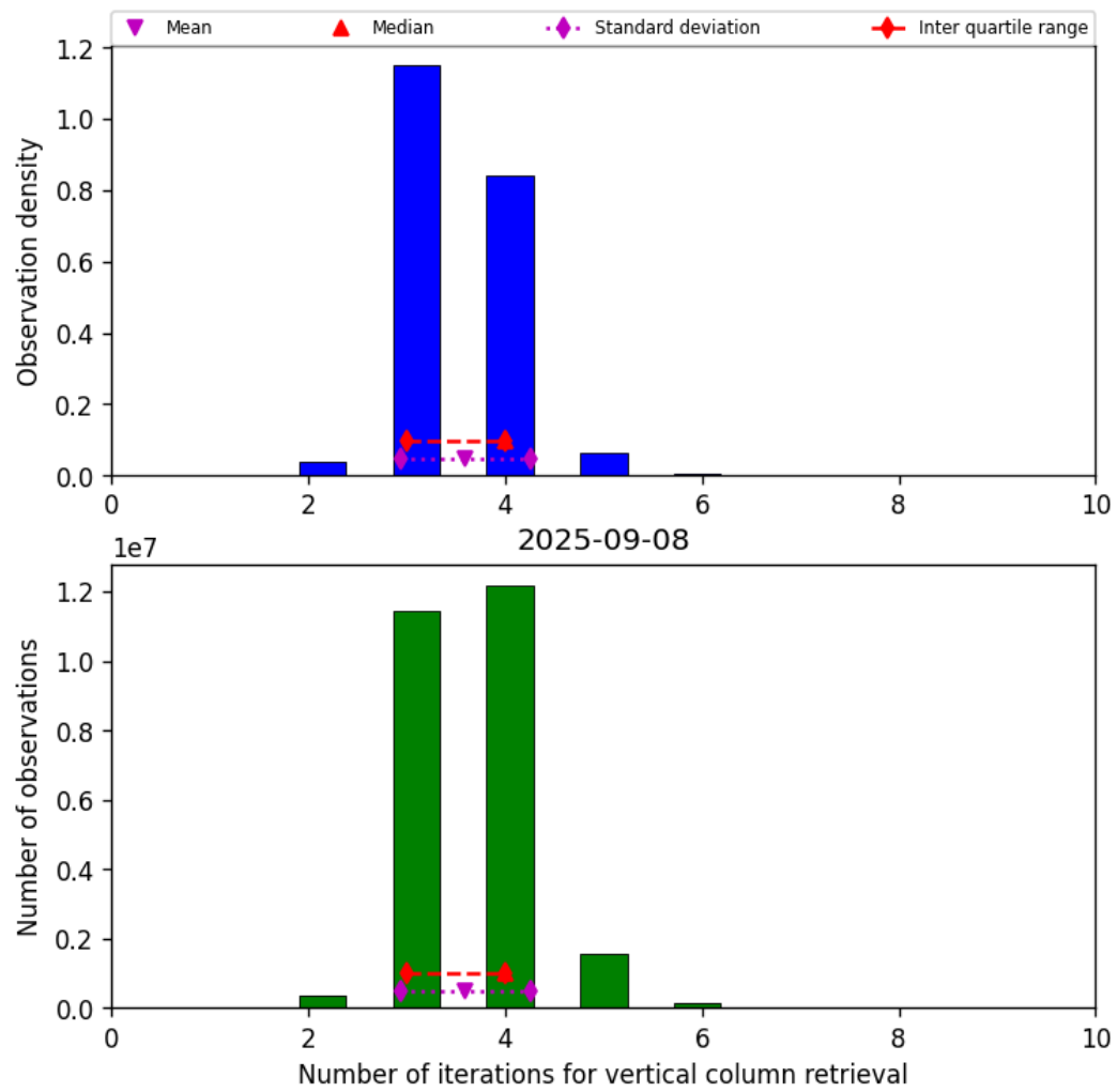
Figure 26: Histogram of “Number of iterations for vertical column retrieval” for 2025-09-07 to 2025-09-09
