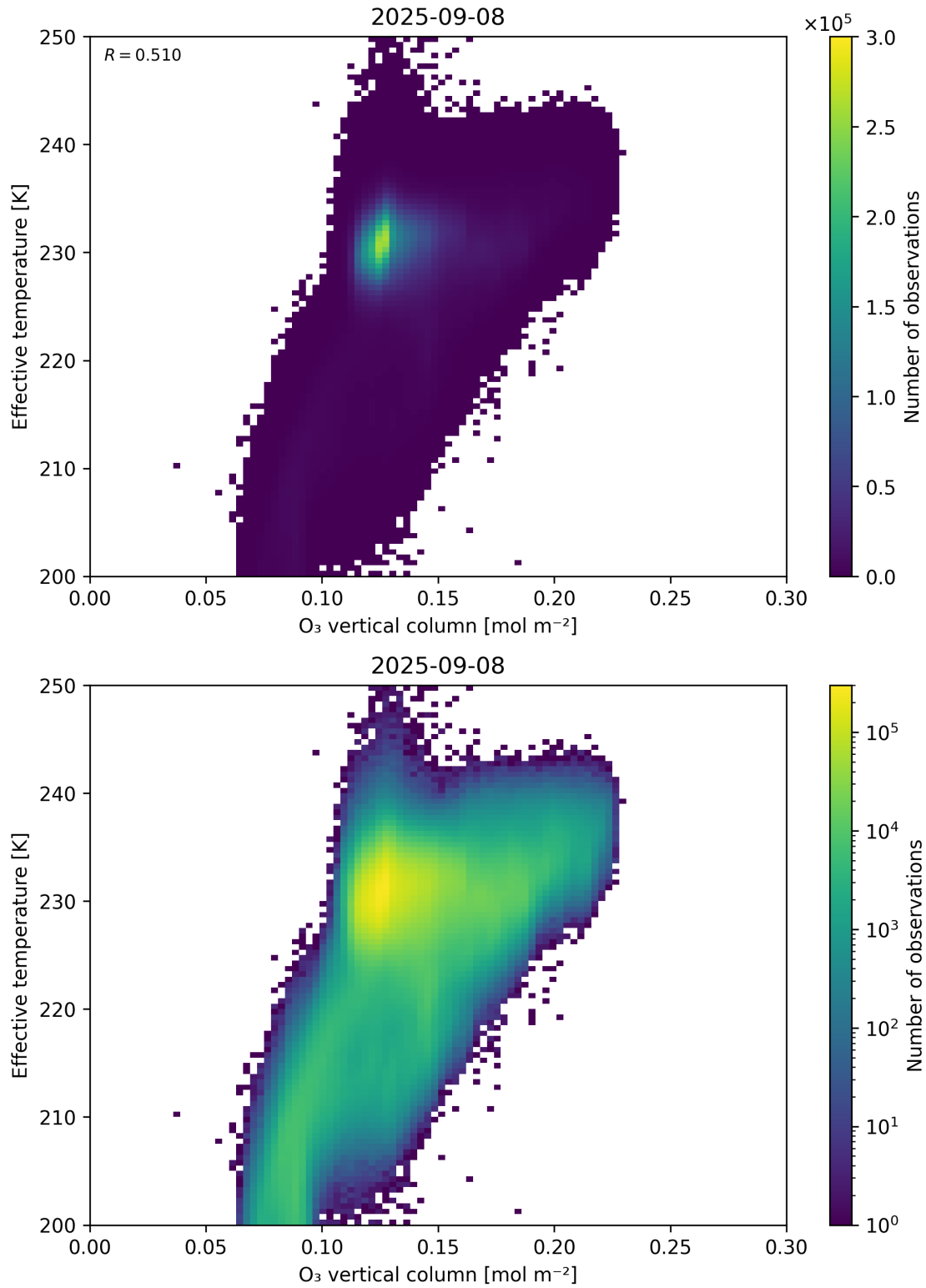
Figure 39: Scatter density plot of “O 3 vertical column” against “Effective temperature” for 2025-09-07 to 2025-09-09.
