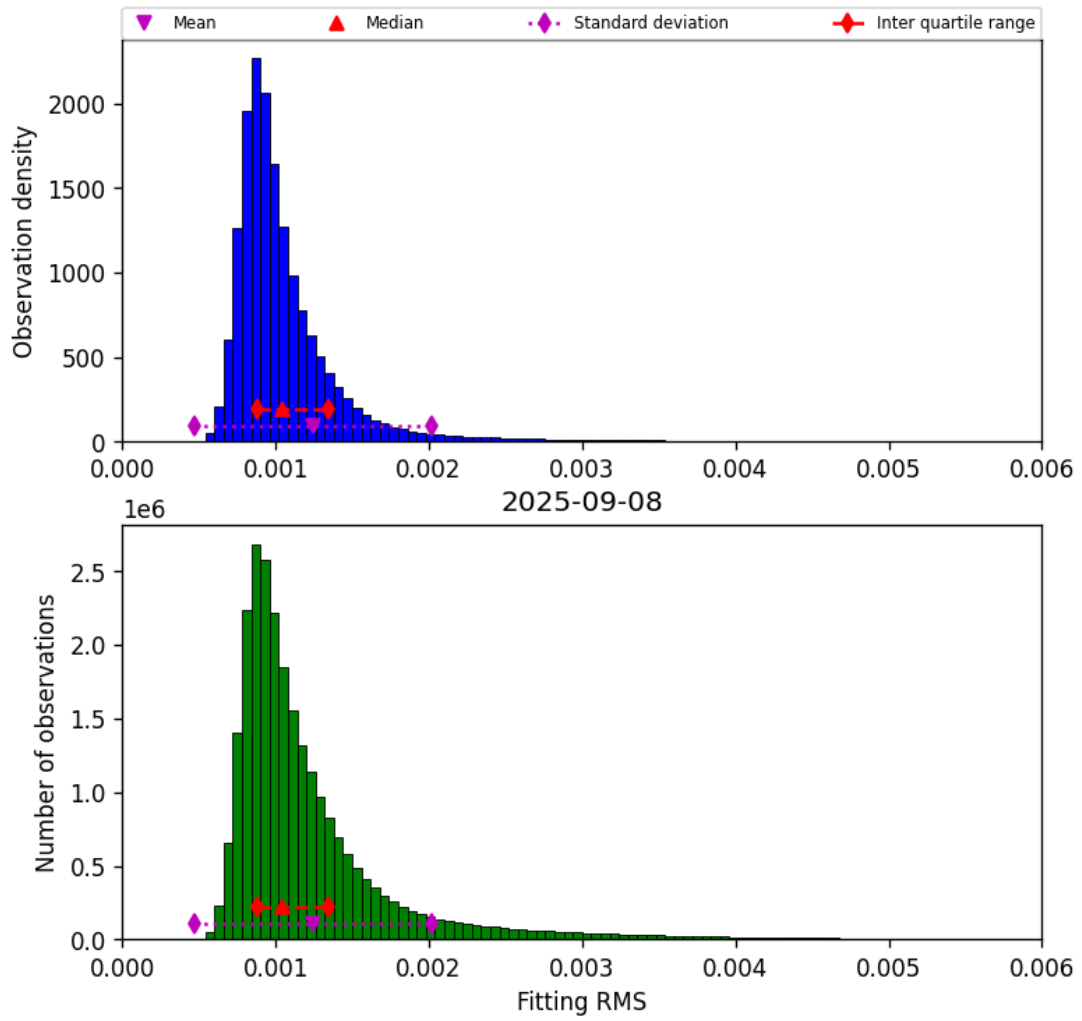
Figure 23: Histogram of “Fitting RMS” for 2025-09-07 to 2025-09-09
