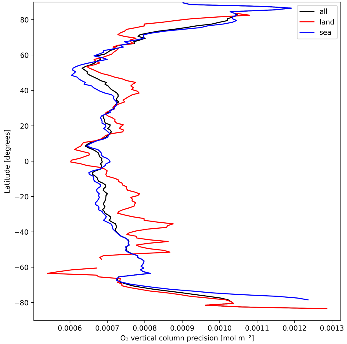
Figure 15: Zonal average of “O 3 vertical column precision” for 2025-09-07 to 2025-09-09.
