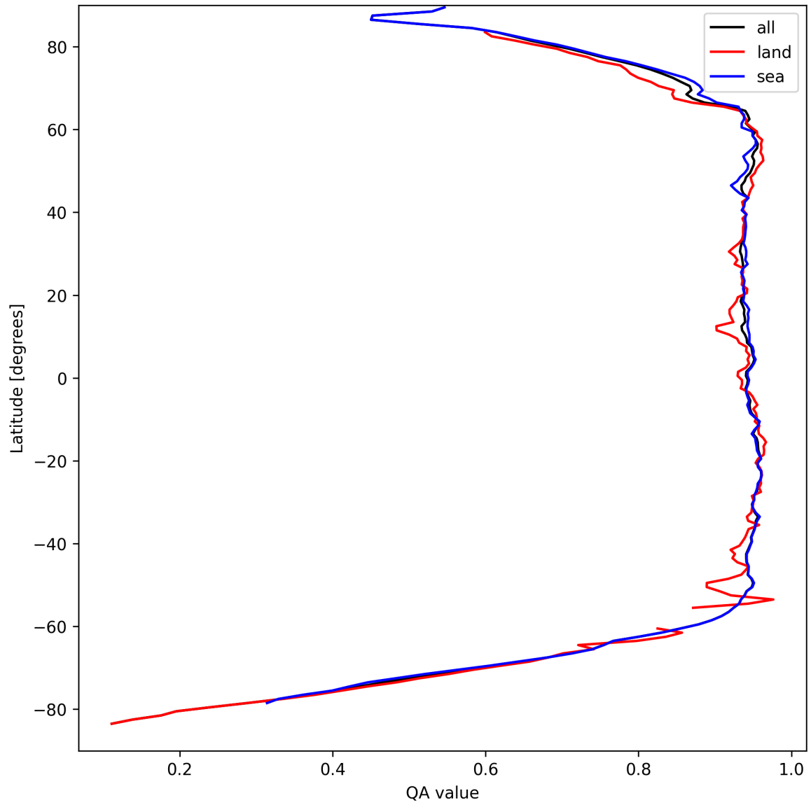
Figure 13: Zonal average of “QA value” for 2025-09-07 to 2025-09-09.
