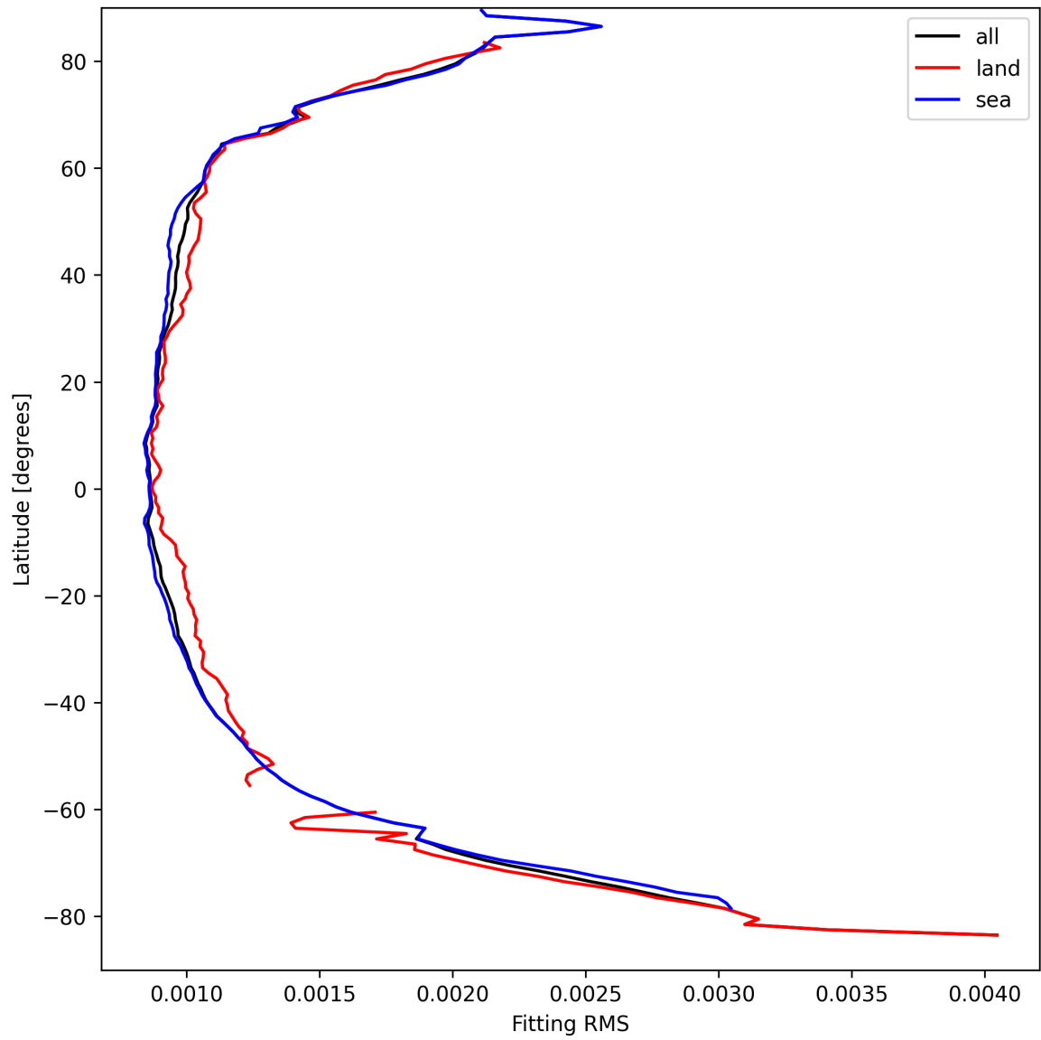
Figure 16: Zonal average of “Fitting RMS” for 2025-09-07 to 2025-09-09.
