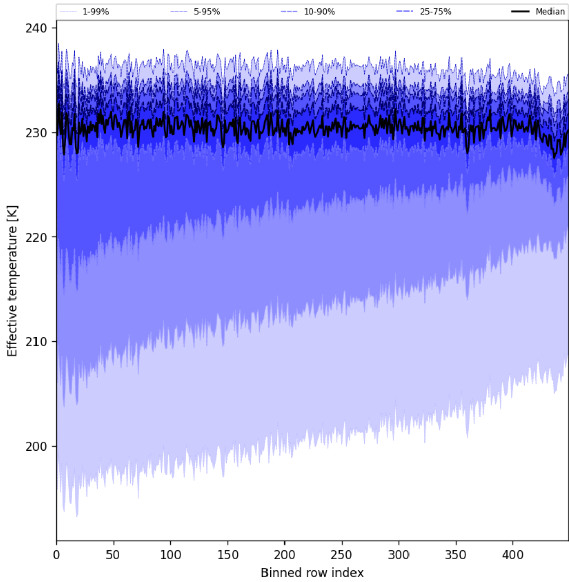
Figure 31: Along track statistics of “Effective temperature” for 2025-09-07 to 2025-09-09
