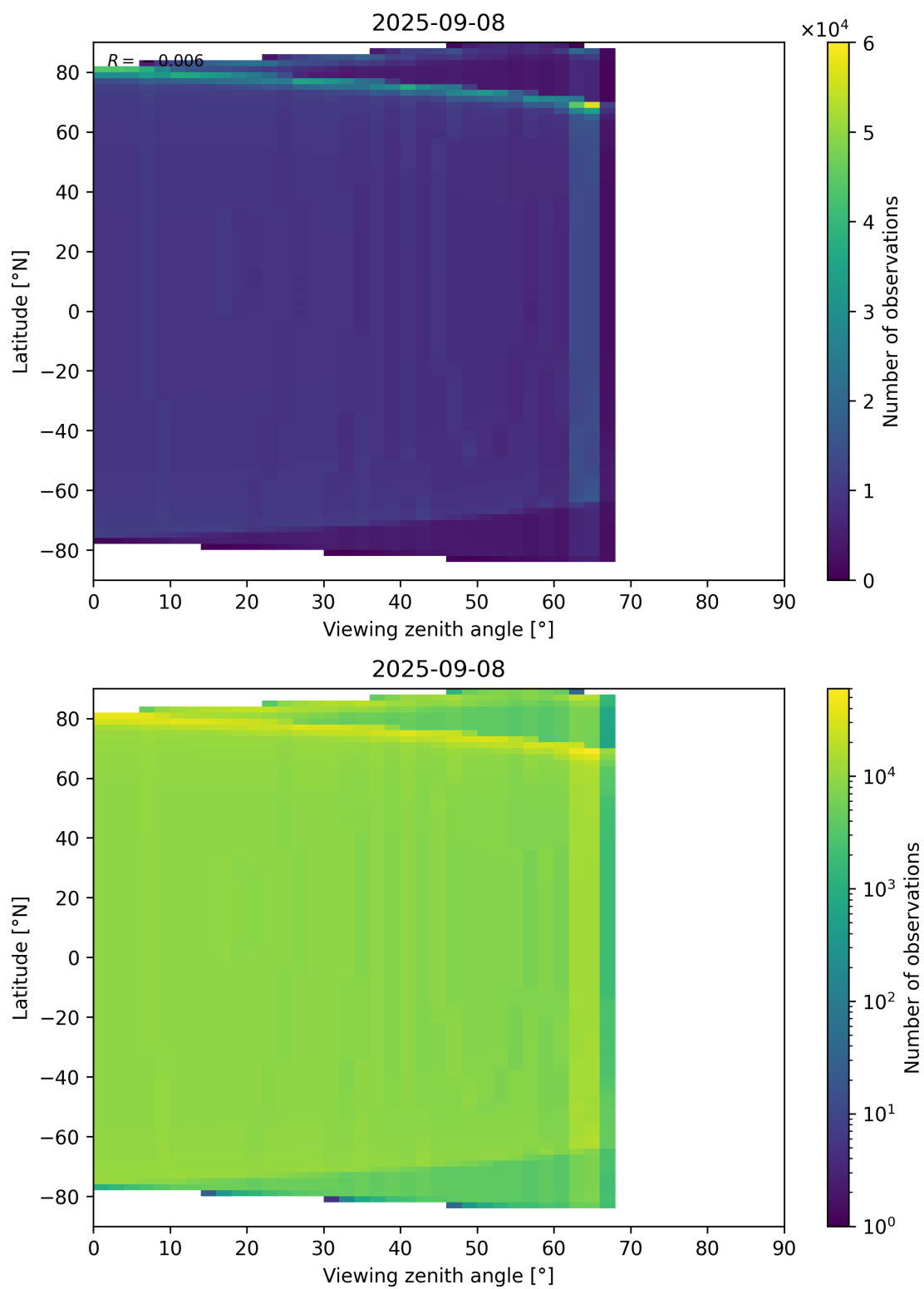
Figure 49: Scatter density plot of “Viewing zenith angle” against “Latitude” for 2025-09-07 to 2025-09-09.
