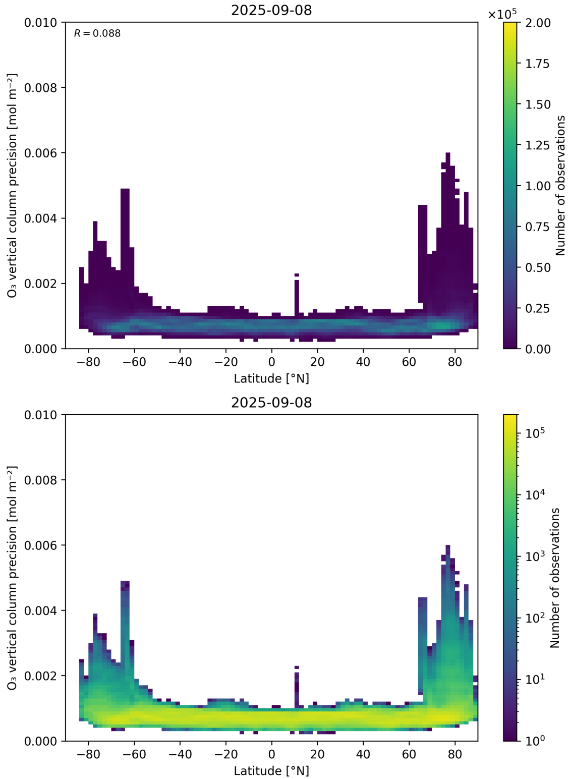
Figure 37: Scatter density plot of “Latitude” against “O 3 vertical column precision” for 2025-09-07 to 2025-09-09.
