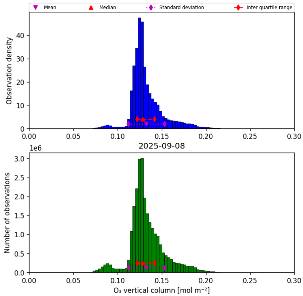
Figure 21: Histogram of “O 3 vertical column” for 2025-09-07 to 2025-09-09
