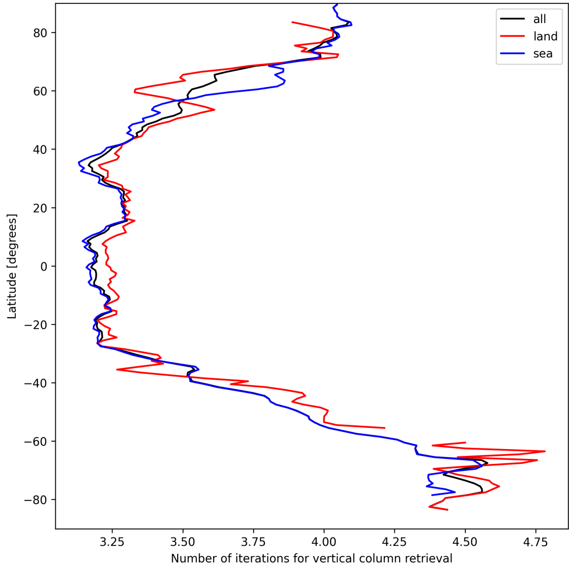
Figure 19: Zonal average of “Number of iterations for vertical column retrieval” for 2025-09-07 to 2025-09-09.
