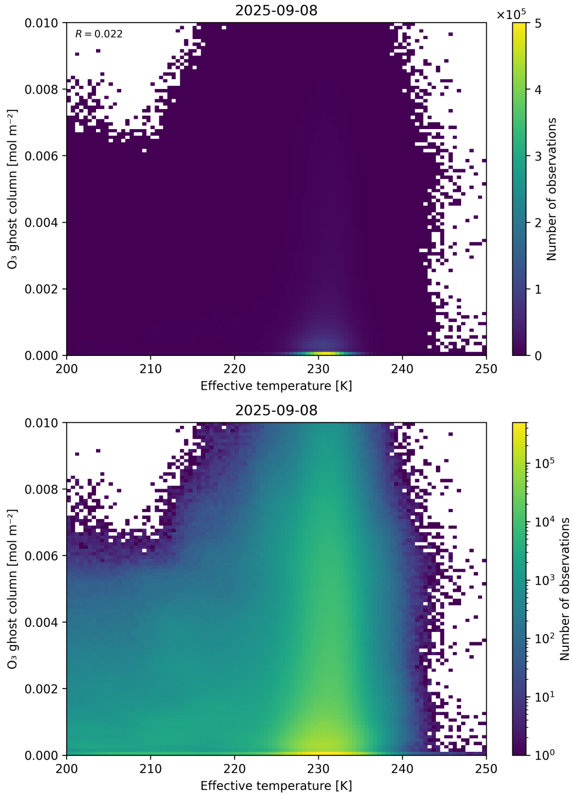
Figure 38: Scatter density plot of “Effective temperature” against “O 3 ghost column” for 2025-09-07 to 2025-09-09.
