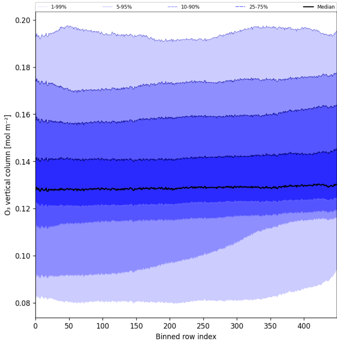
Figure 28: Along track statistics of “O 3 vertical column” for 2025-09-07 to 2025-09-09
