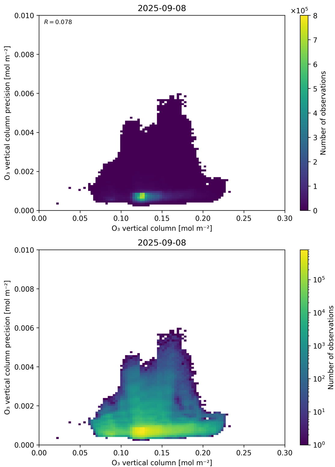
Figure 41: Scatter density plot of “O 3 vertical column” against “O 3 vertical column precision” for 2025-09-07 to 2025-09-09.
