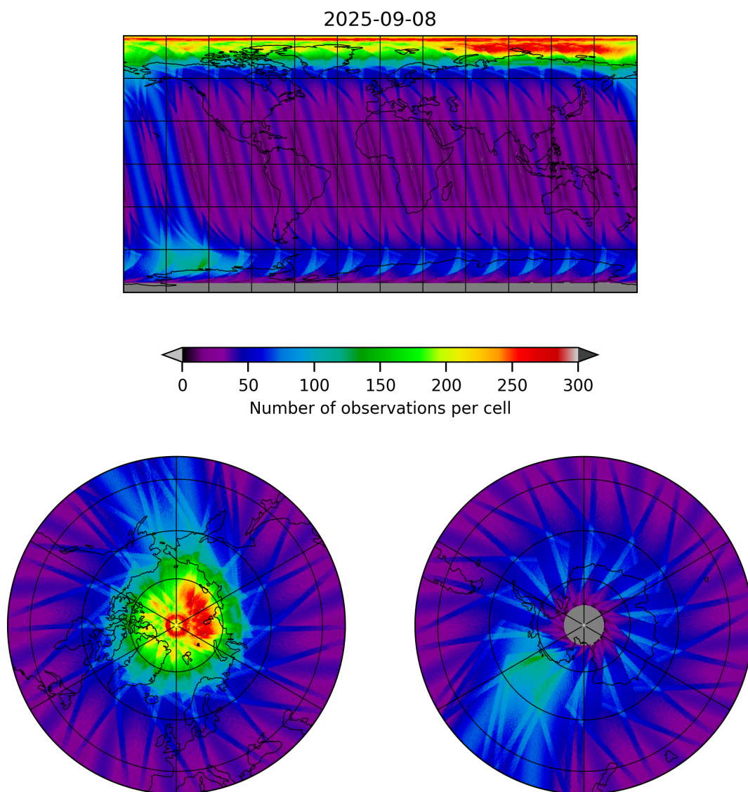
Figure 12: Map of the number of observations for 2025-09-07 to 2025-09-09
