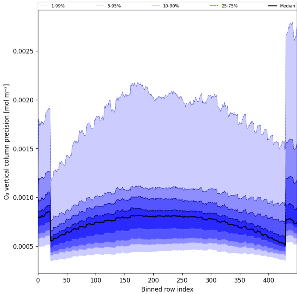
Figure 29: Along track statistics of “O 3 vertical column precision” for 2025-09-07 to 2025-09-09
