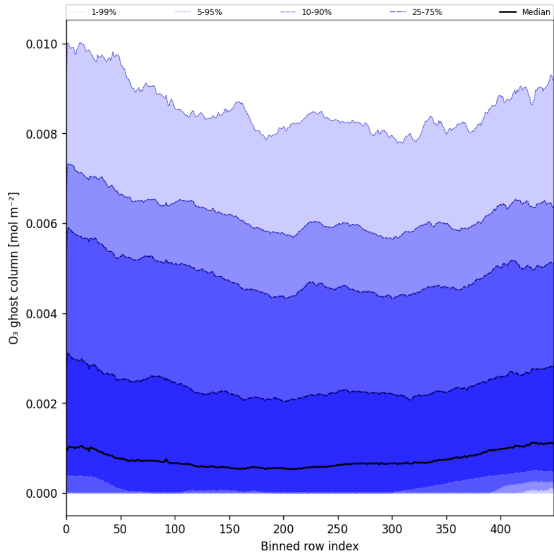
Figure 32: Along track statistics of “O 3 ghost column” for 2025-09-07 to 2025-09-09
