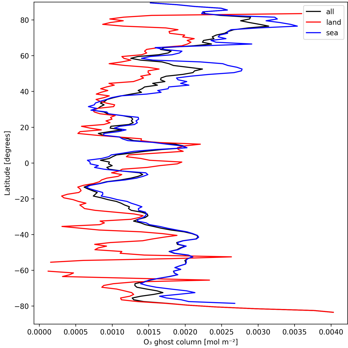
Figure 18: Zonal average of “O 3 ghost column” for 2025-09-07 to 2025-09-09.
