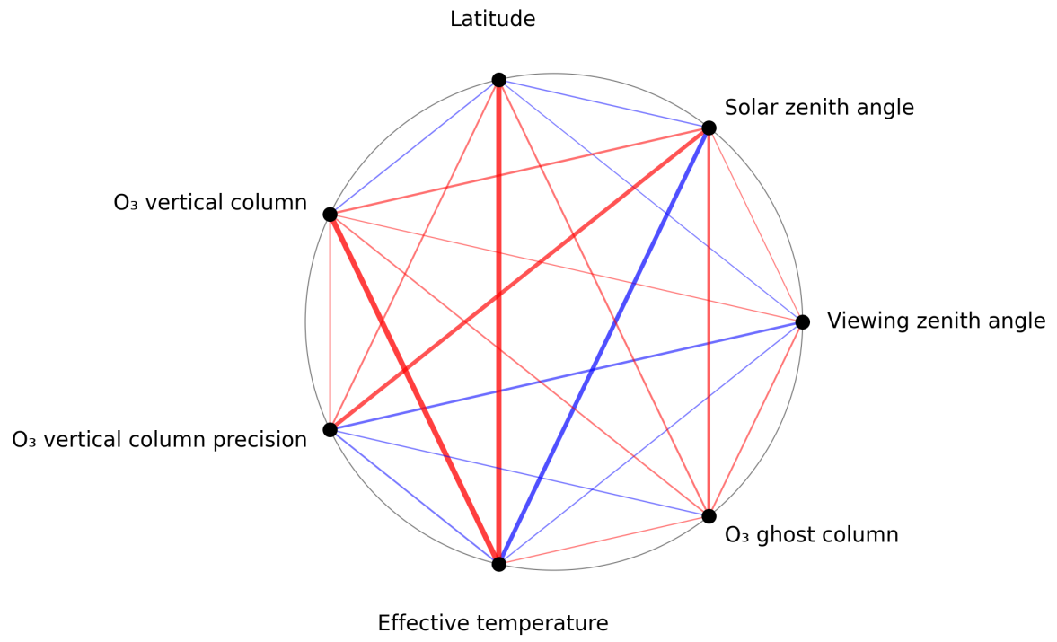
Figure 1: Map of correlation graph for 2025-09-07 to 2025-09-09.
