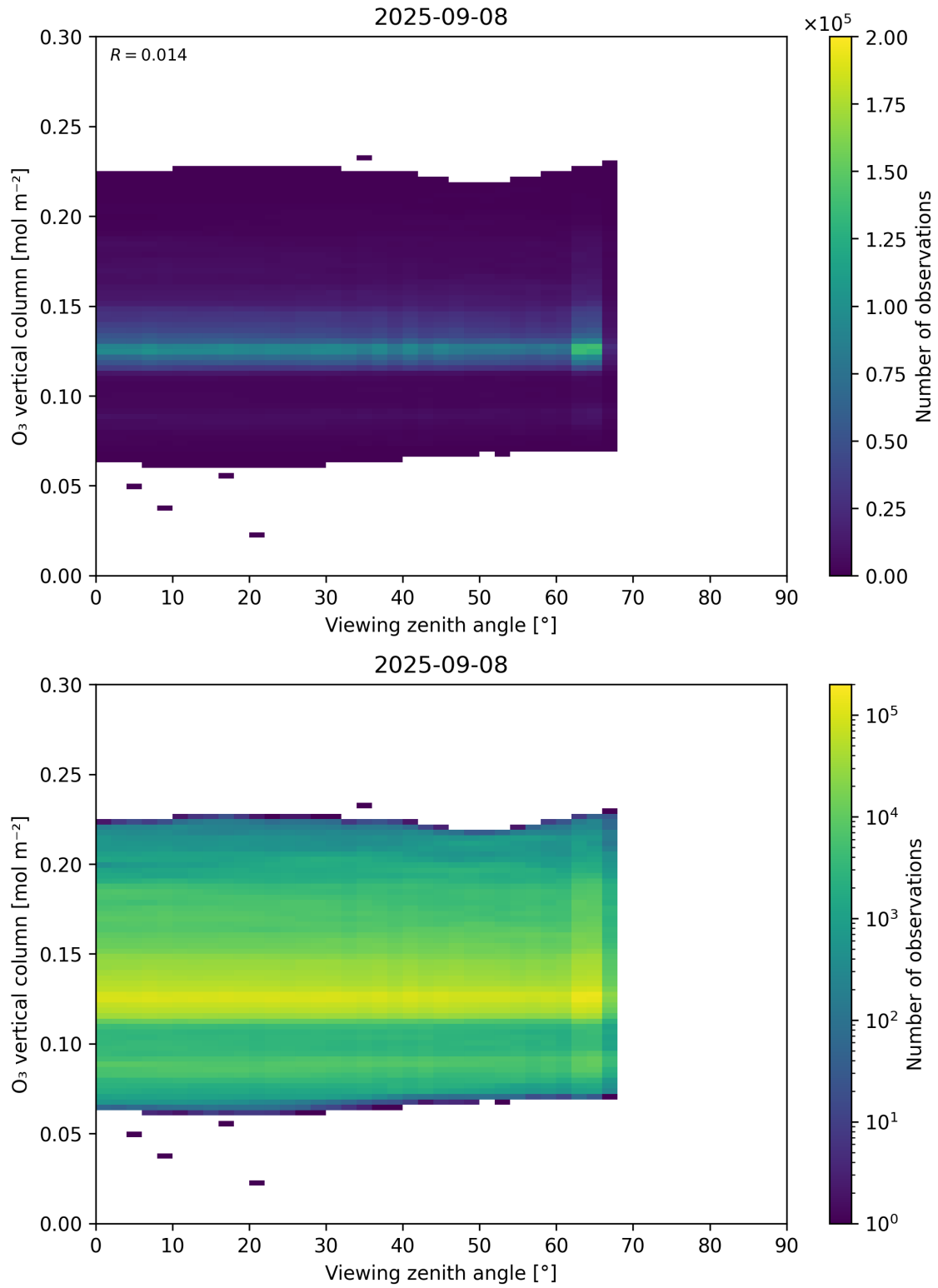
Figure 52: Scatter density plot of “Viewing zenith angle” against “O 3 vertical column” for 2025-09-07 to 2025-09-09.
