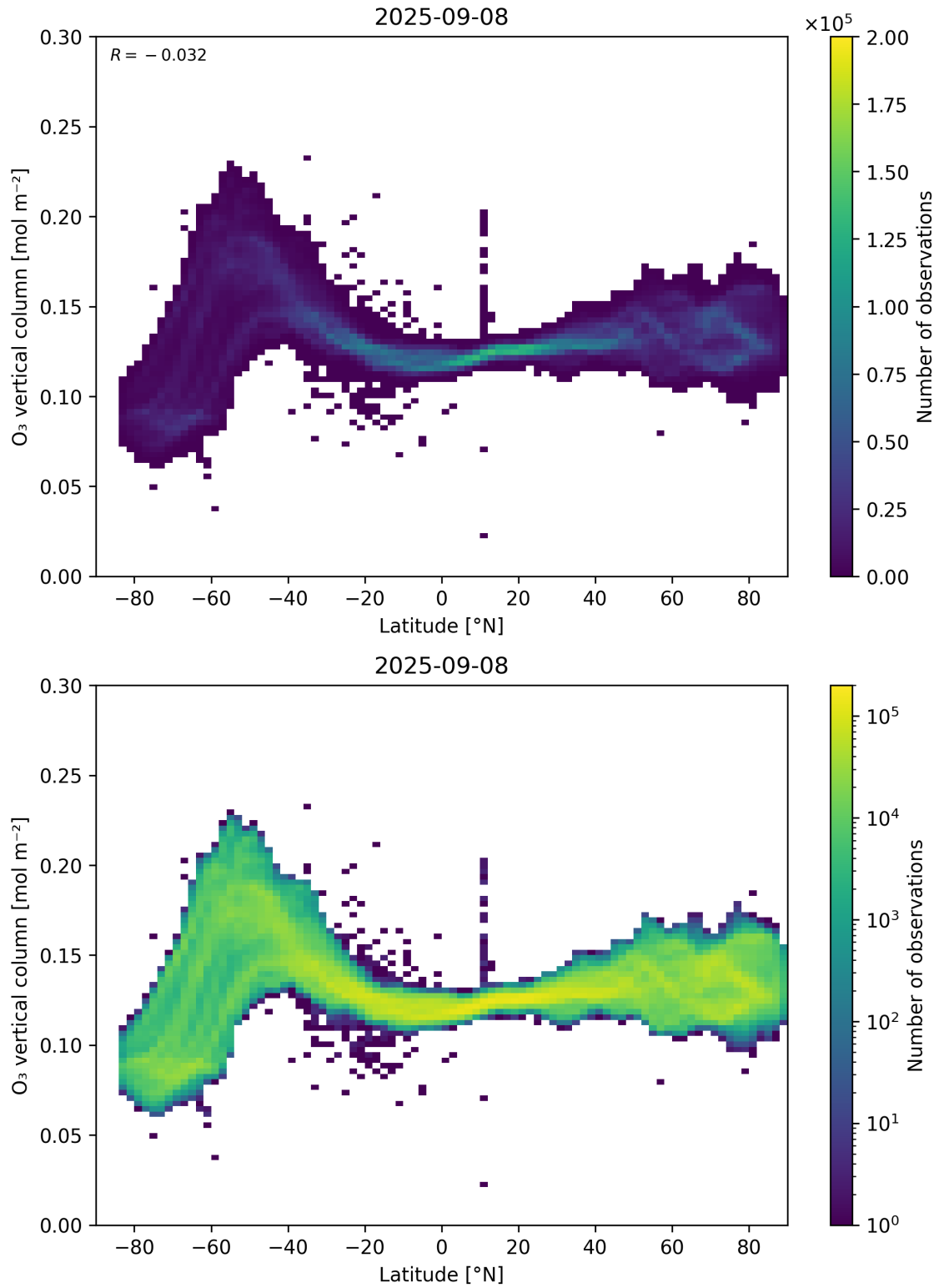
Figure 36: Scatter density plot of “Latitude” against “O 3 vertical column” for 2025-09-07 to 2025-09-09.
