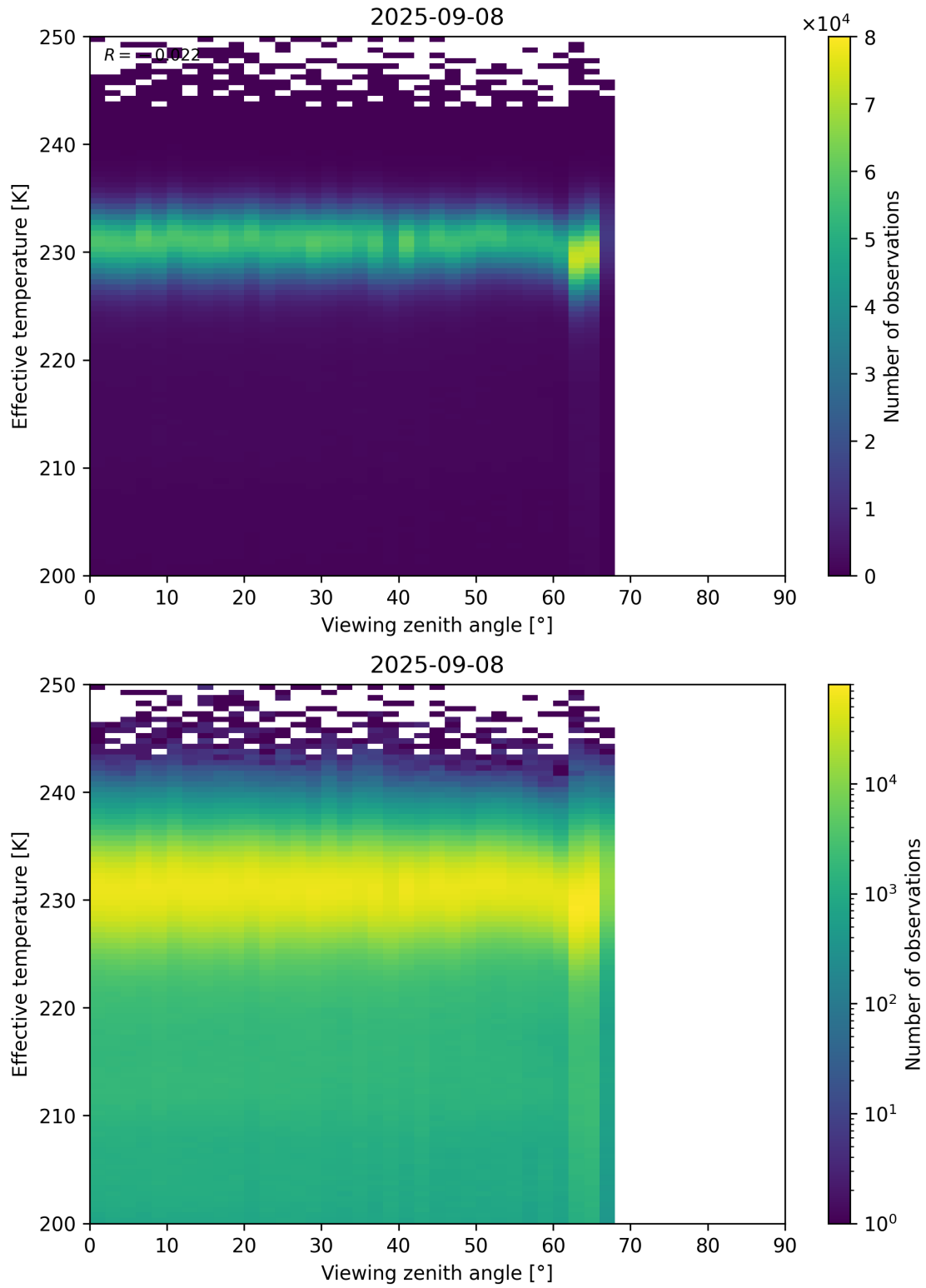
Figure 50: Scatter density plot of “Viewing zenith angle” against “Effective temperature” for 2025-09-07 to 2025-09-09.
