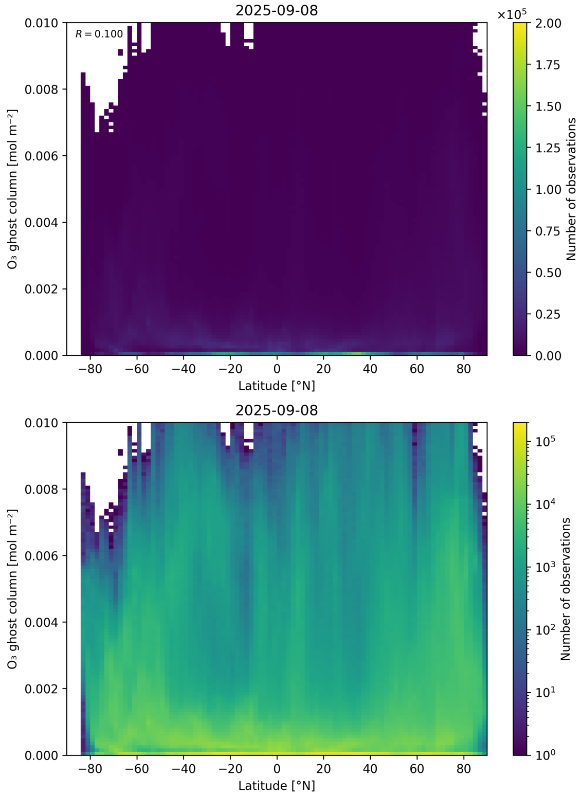
Figure 35: Scatter density plot of “Latitude” against “O 3 ghost column” for 2025-09-07 to 2025-09-09.
