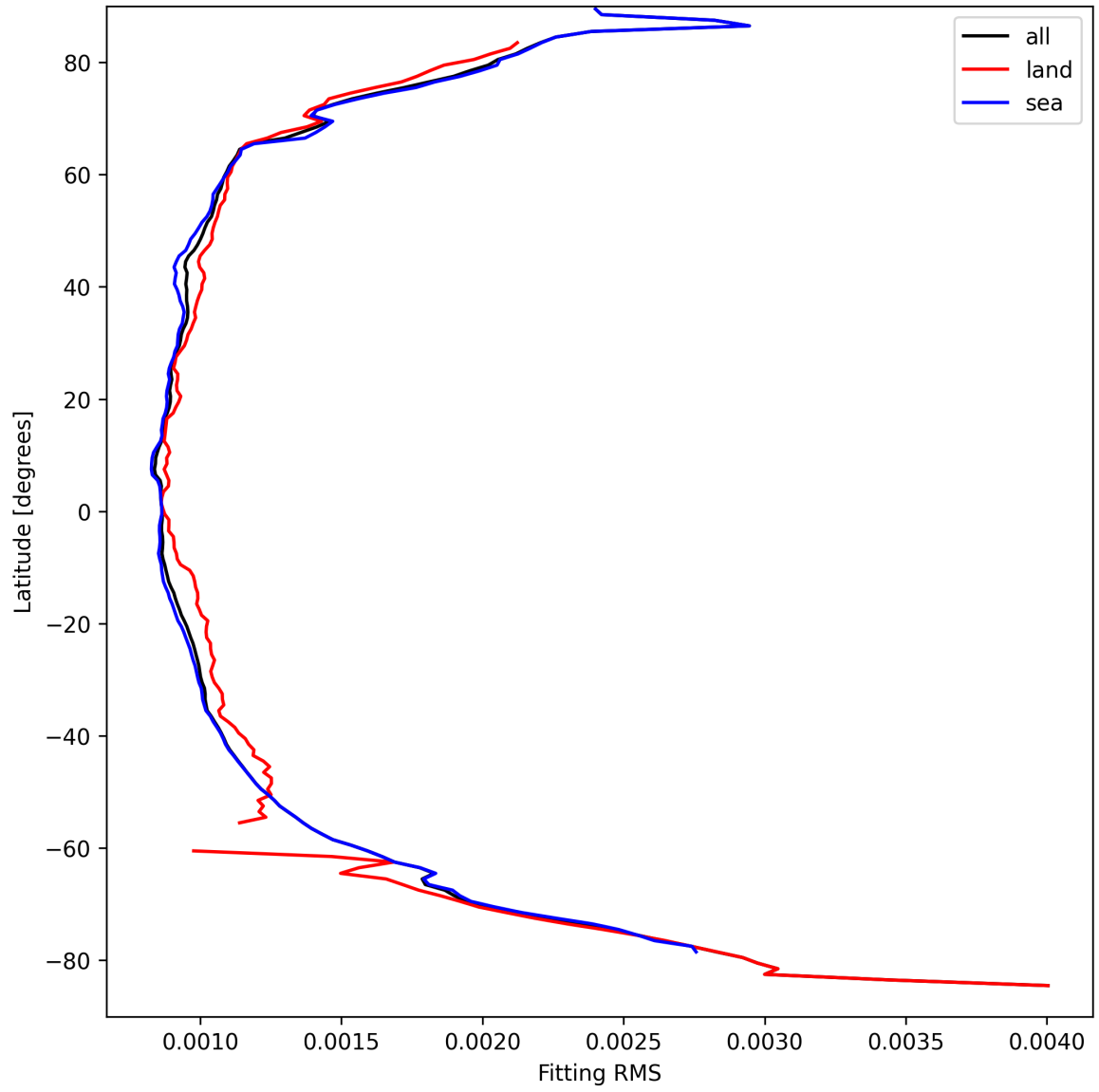
Figure 16: Zonal average of “Fitting RMS” for 2025-09-10 to 2025-09-11.
