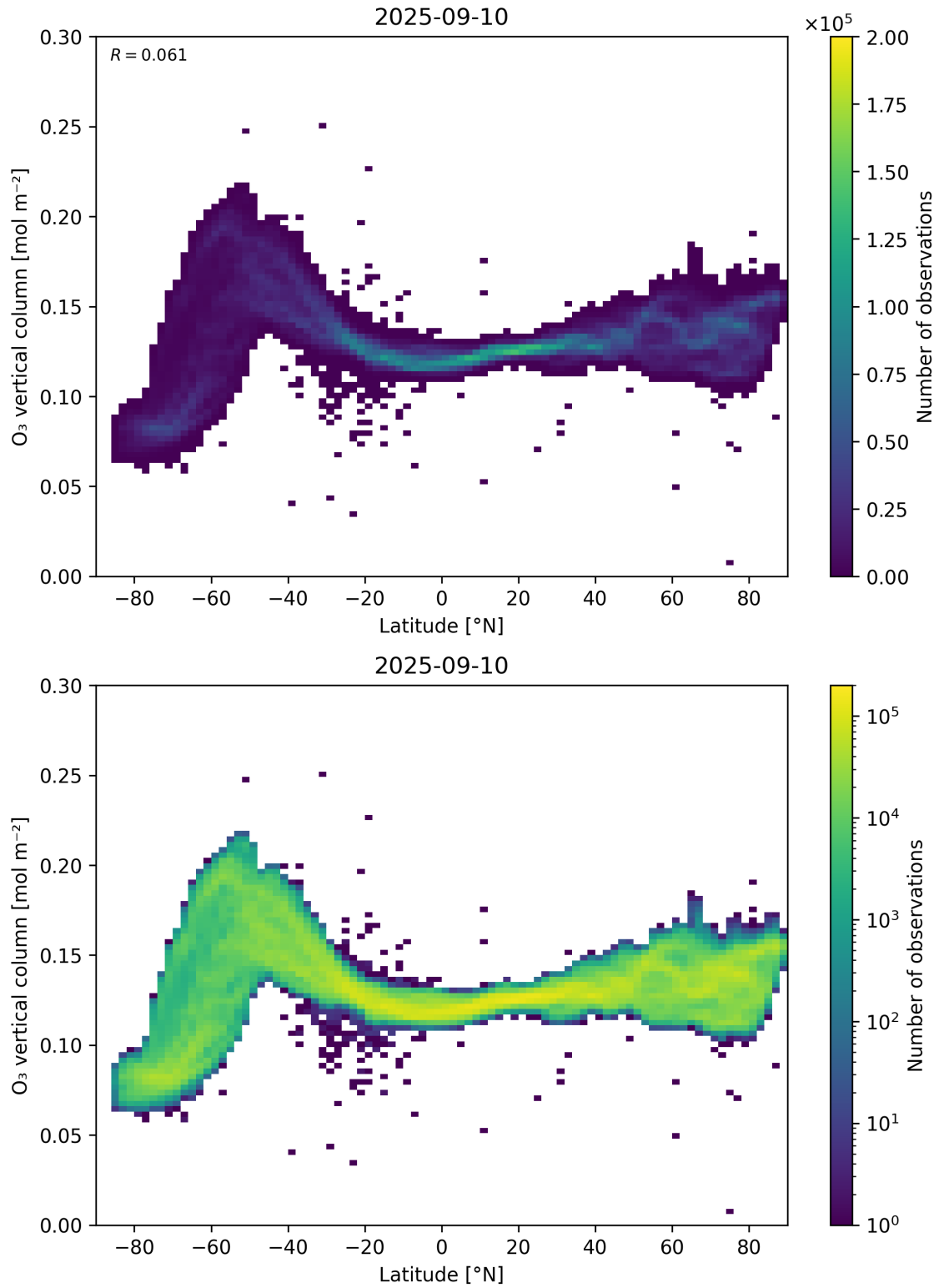
Figure 36: Scatter density plot of “Latitude” against “O 3 vertical column” for 2025-09-10 to 2025-09-11.
