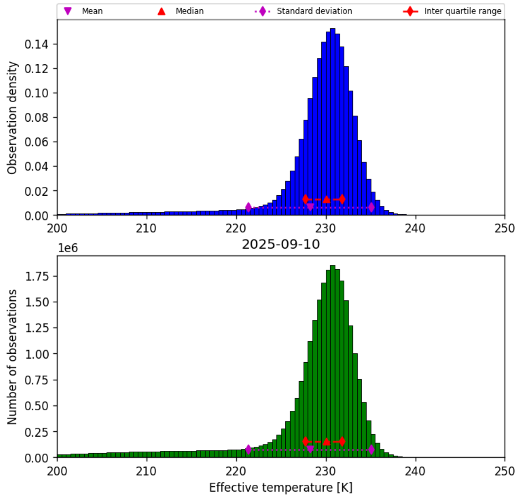
Figure 24: Histogram of “Effective temperature” for 2025-09-10 to 2025-09-11
