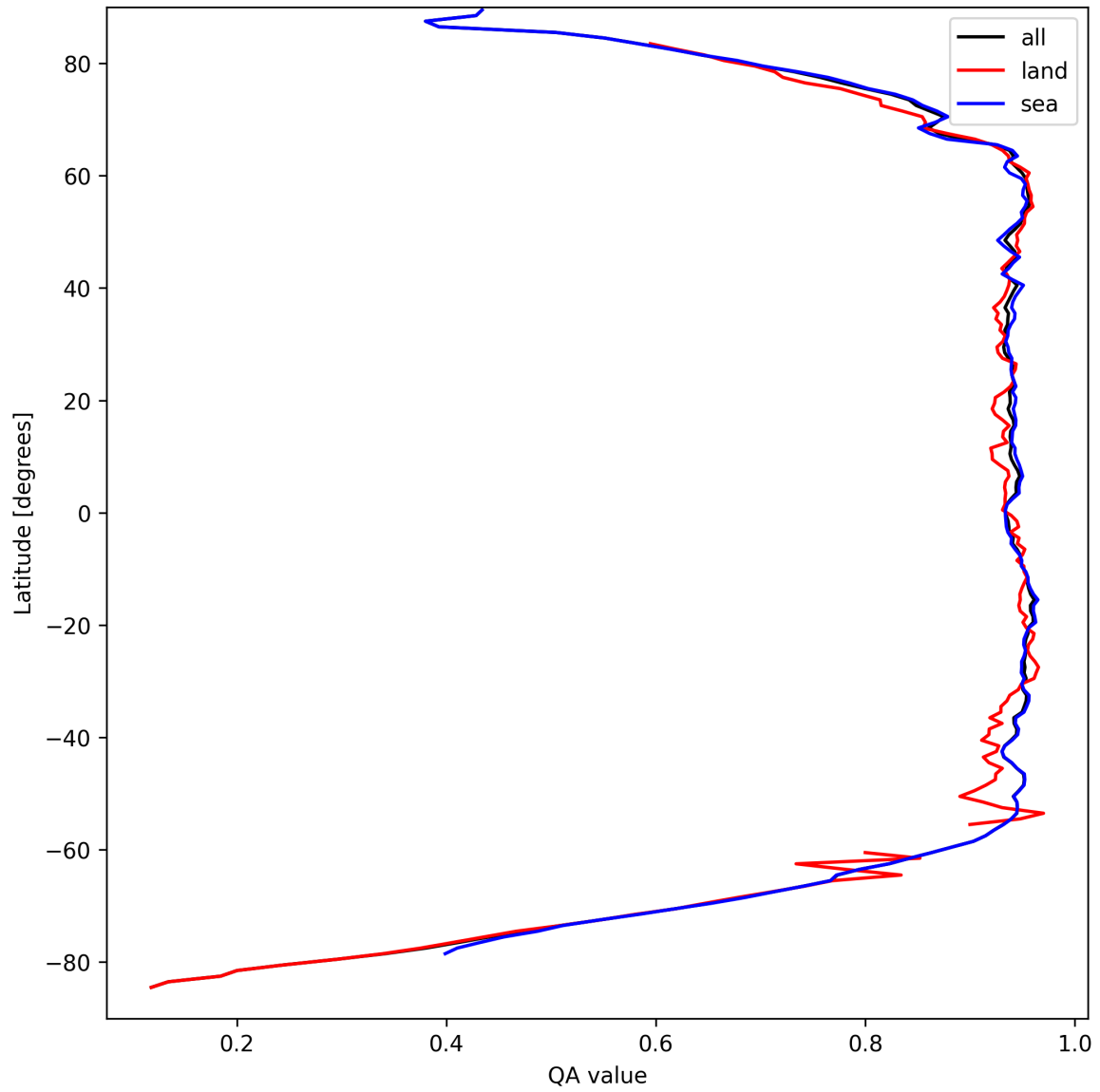
Figure 13: Zonal average of “QA value” for 2025-09-10 to 2025-09-11.
