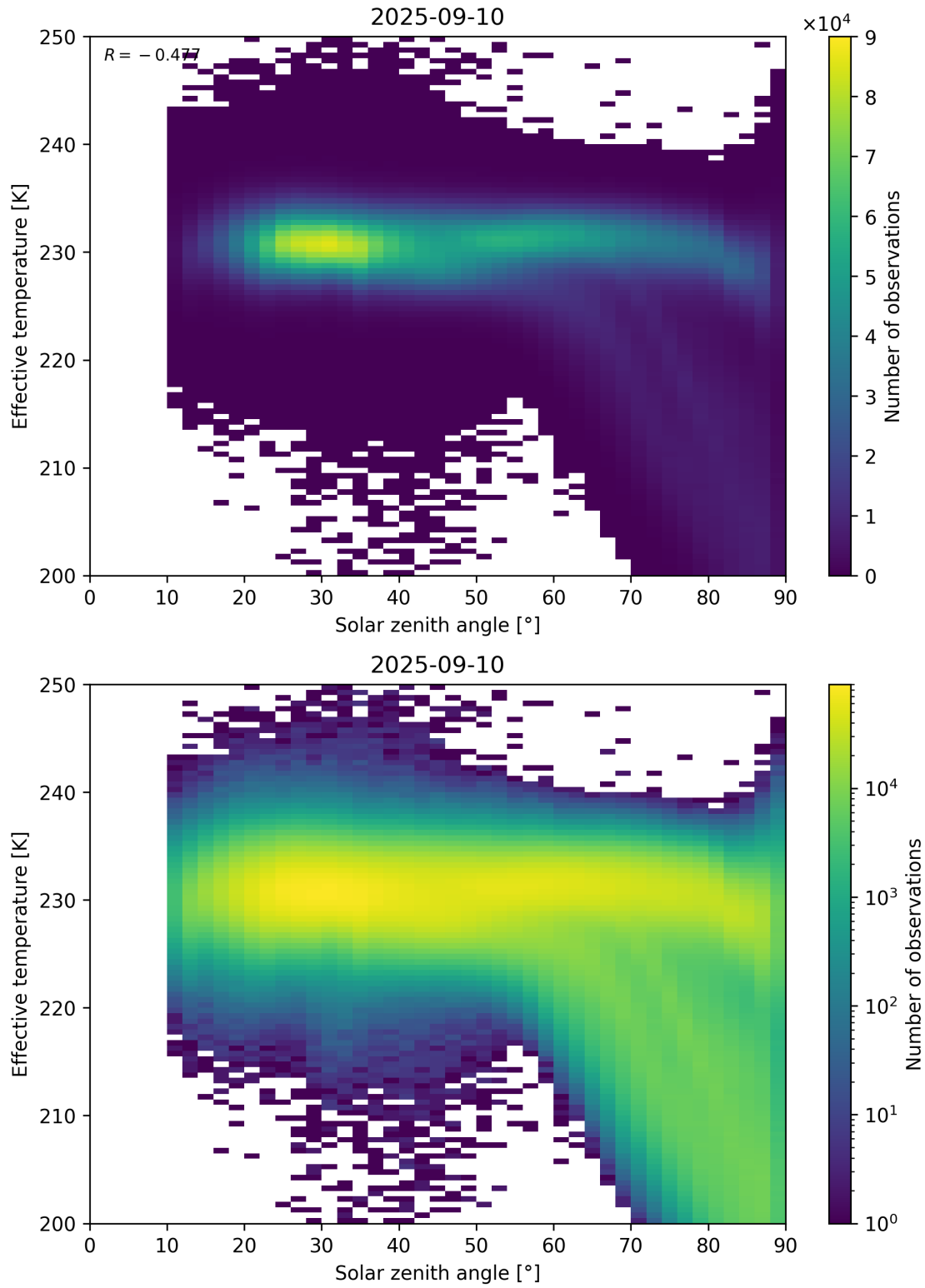
Figure 45: Scatter density plot of “Solar zenith angle” against “Effective temperature” for 2025-09-10 to 2025-09-11.
