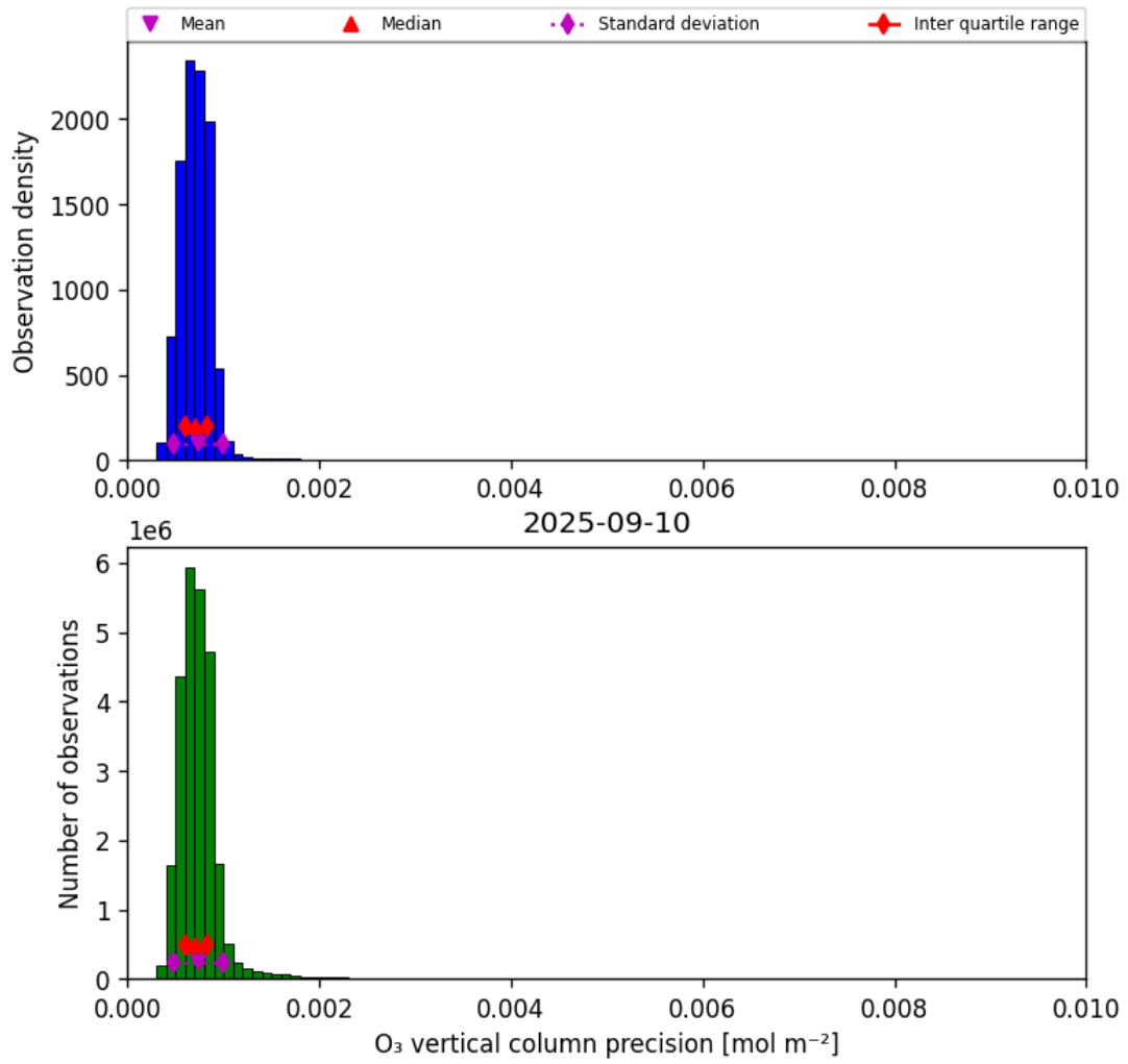
Figure 22: Histogram of “O 3 vertical column precision” for 2025-09-10 to 2025-09-11
