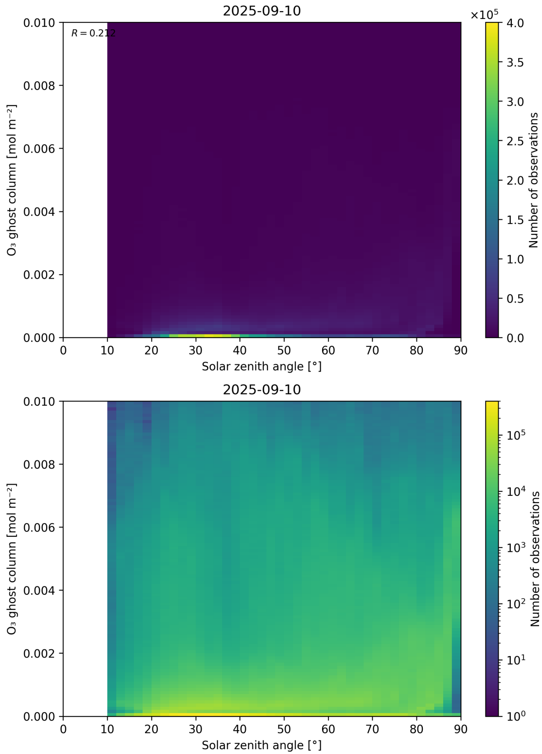
Figure 46: Scatter density plot of “Solar zenith angle” against “O 3 ghost column” for 2025-09-10 to 2025-09-11.
