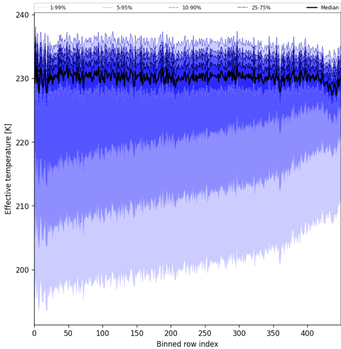
Figure 31: Along track statistics of “Effective temperature” for 2025-09-10 to 2025-09-11
