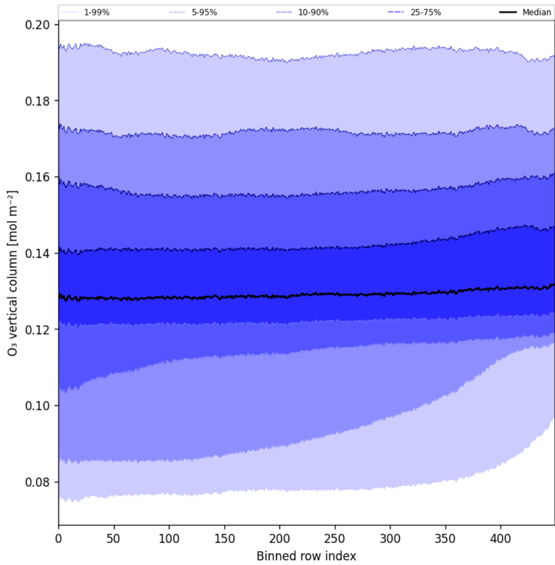
Figure 28: Along track statistics of “O 3 vertical column” for 2025-09-10 to 2025-09-11
