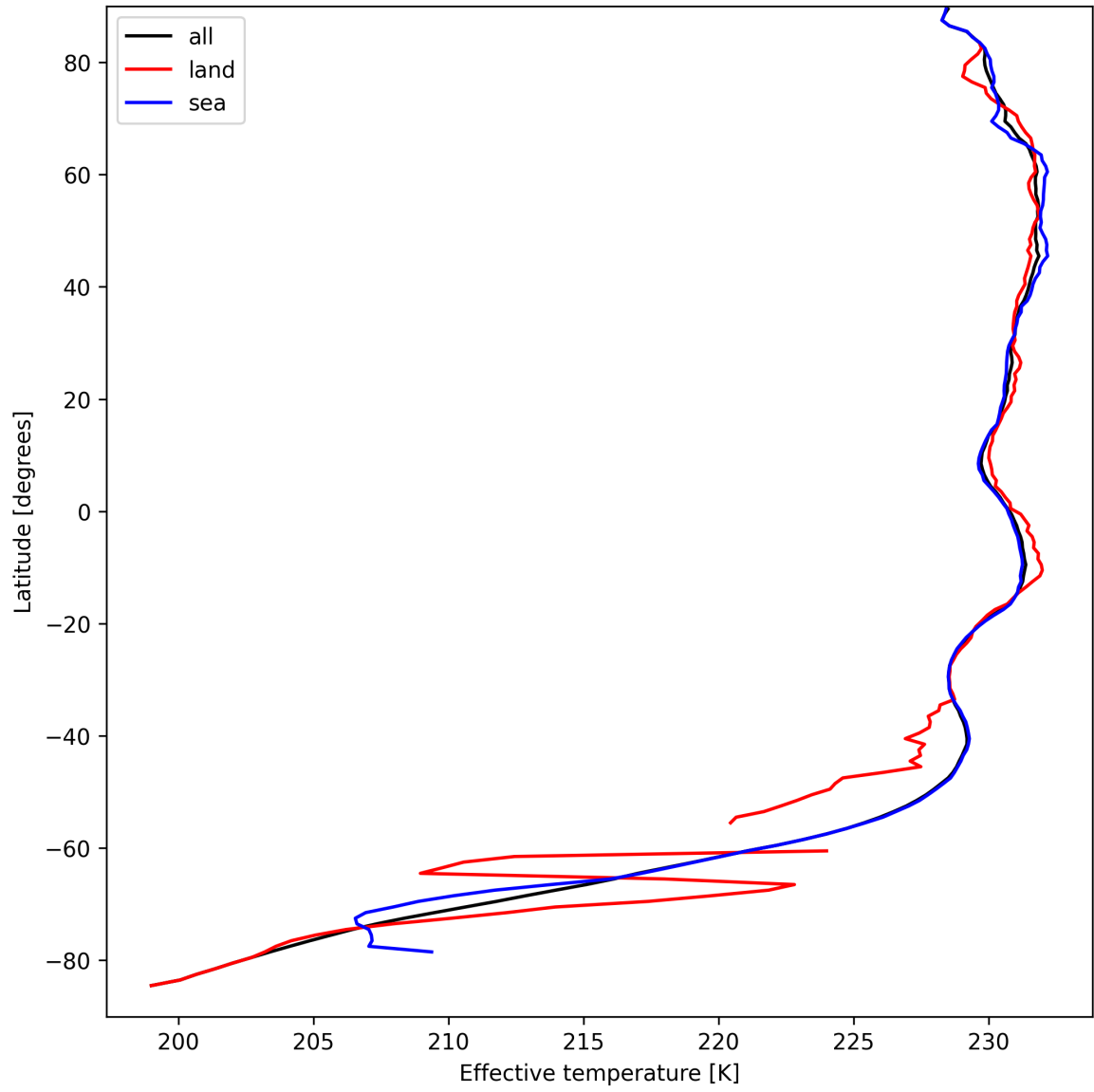
Figure 17: Zonal average of "Effective temperature" for 2025-09-10 to 2025-09-11.
