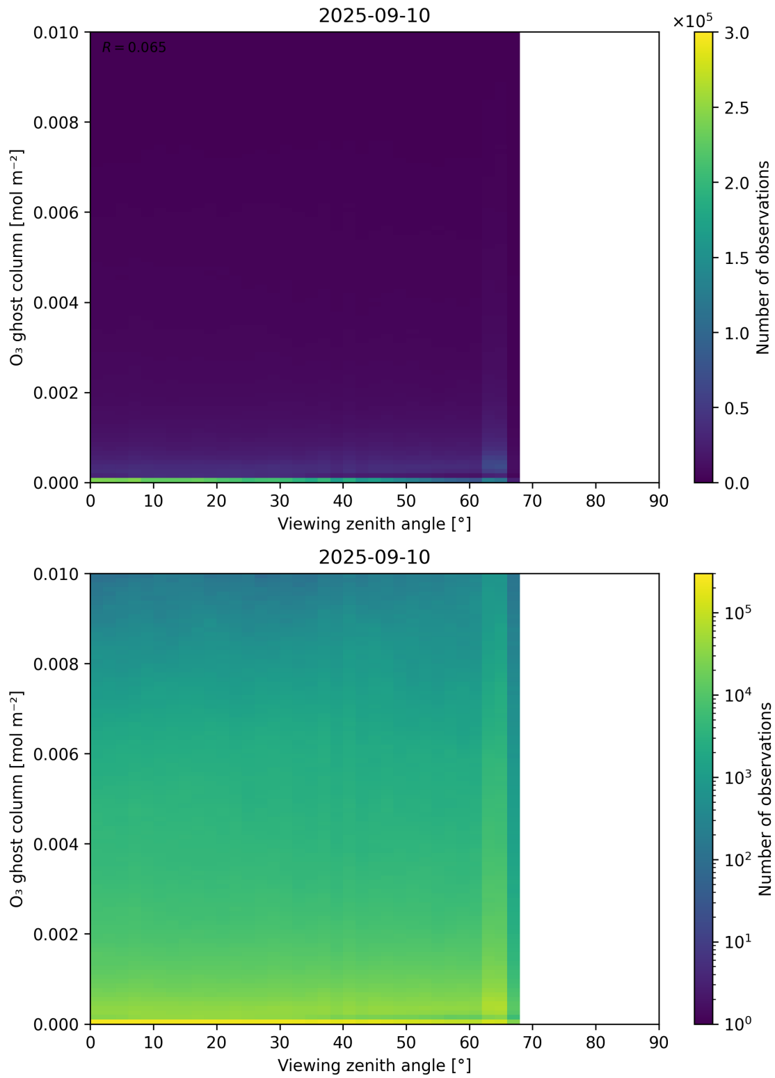
Figure 51: Scatter density plot of “Viewing zenith angle” against “O 3 ghost column” for 2025-09-10 to 2025-09-11.
