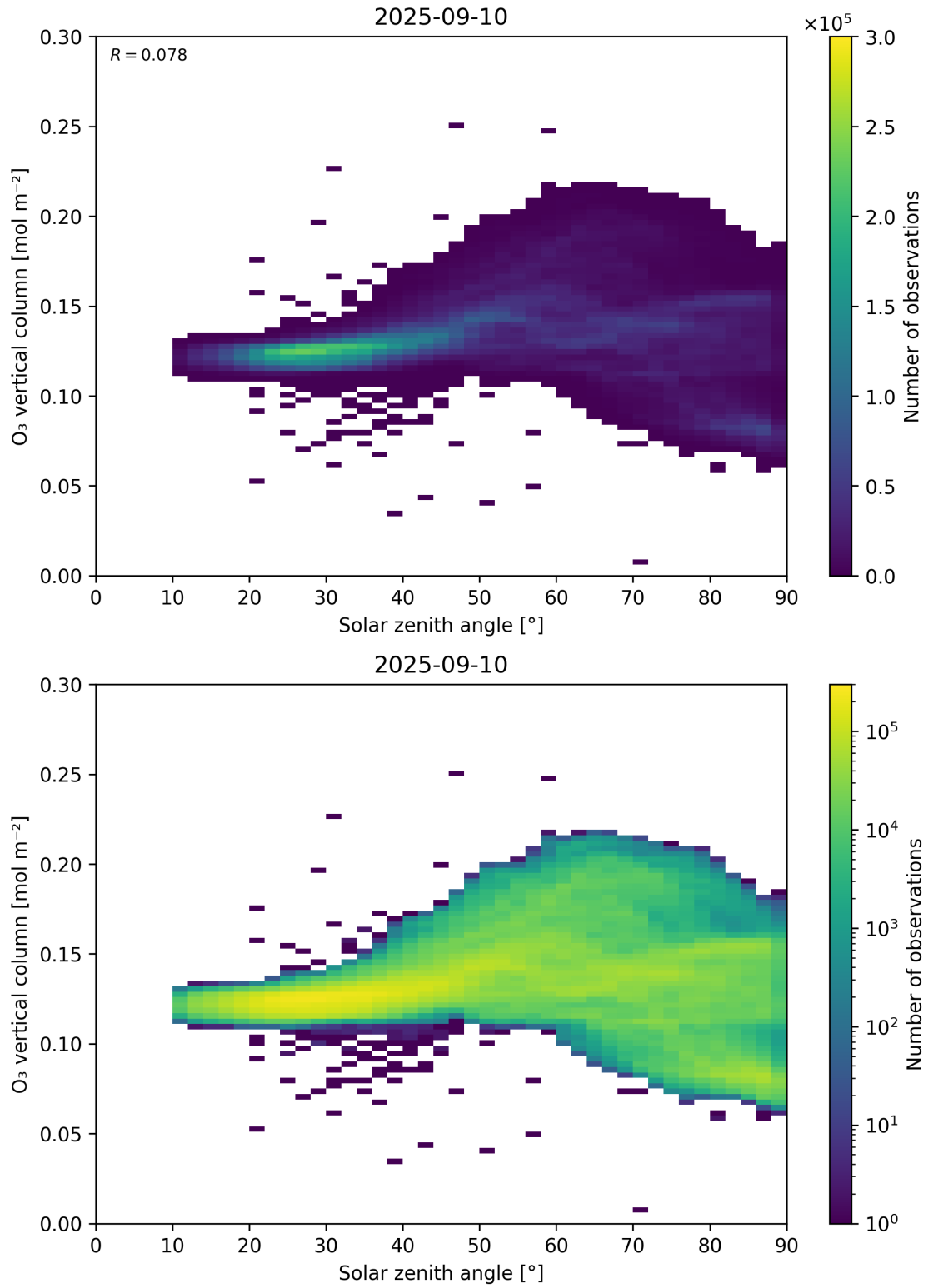
Figure 47: Scatter density plot of “Solar zenith angle” against “O 3 vertical column” for 2025-09-10 to 2025-09-11.
