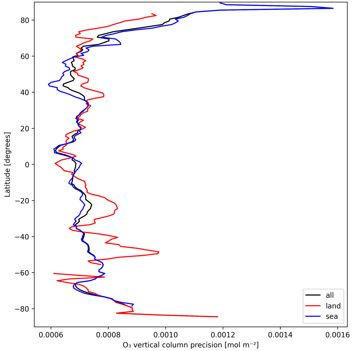
Figure 15: Zonal average of "O 3 vertical column precision" for 2025-09-10 to 2025-09-11.
