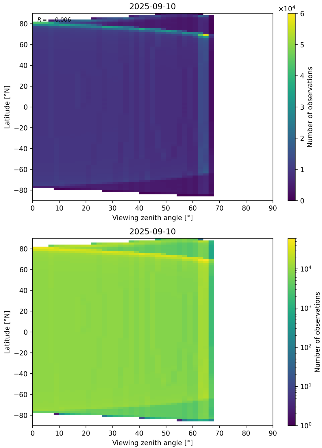
Figure 49: Scatter density plot of “Viewing zenith angle” against “Latitude” for 2025-09-10 to 2025-09-11.
