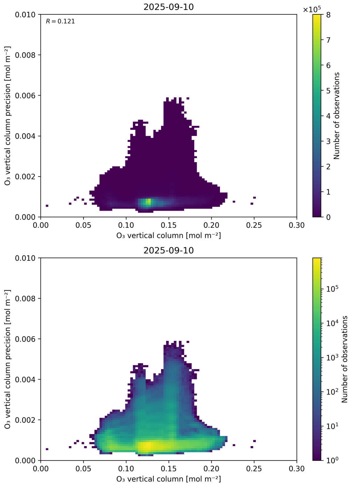
Figure 41: Scatter density plot of “O 3 vertical column” against “O 3 vertical column precision” for 2025-09-10 to 2025-09-11.
