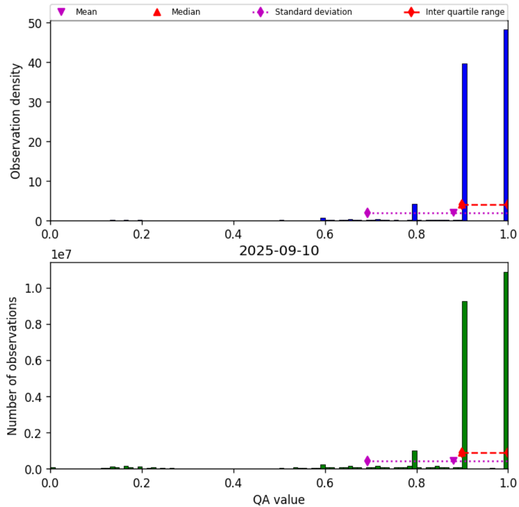
Figure 20: Histogram of “QA value” for 2025-09-10 to 2025-09-11
