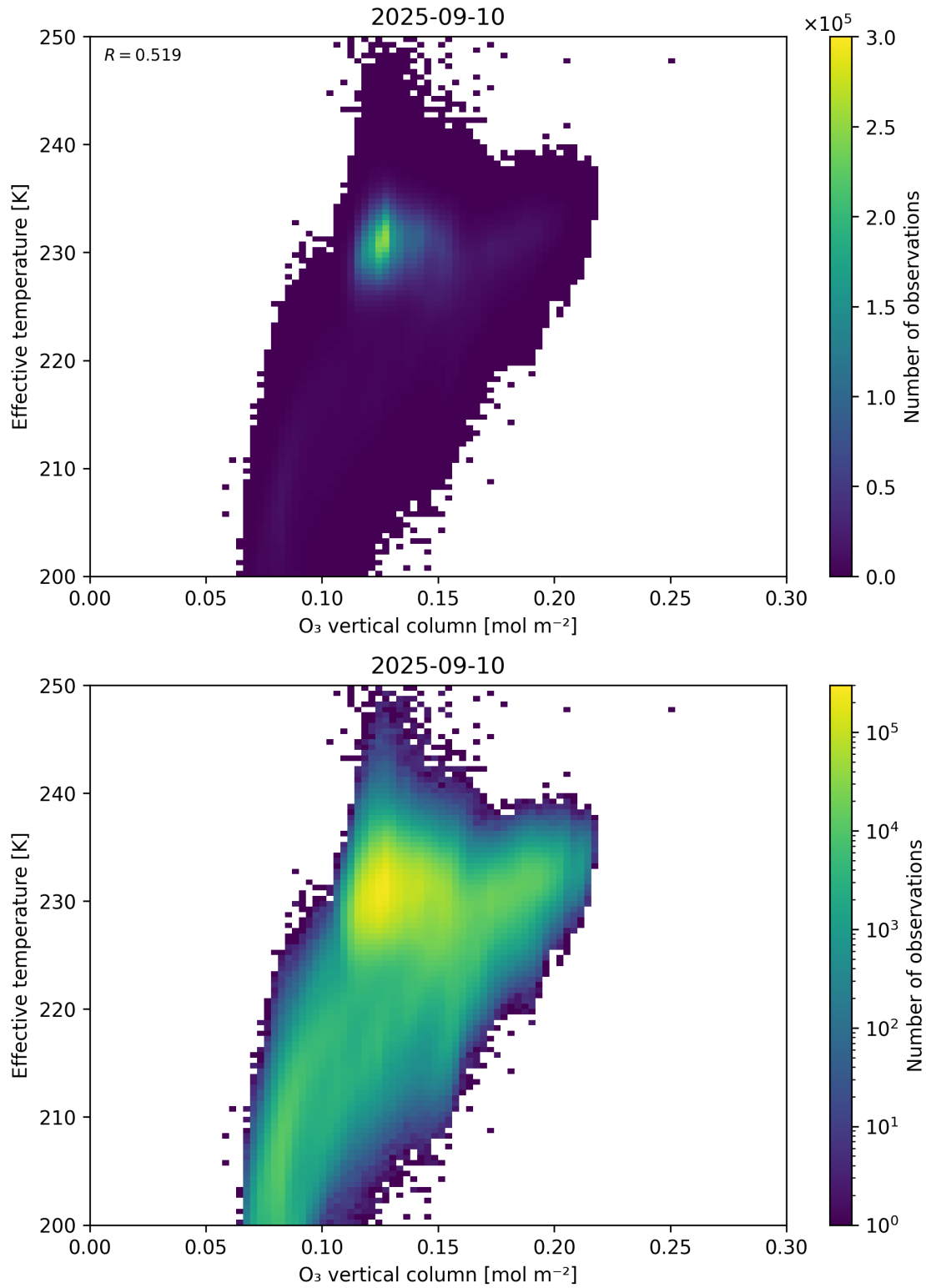
Figure 39: Scatter density plot of “O 3 vertical column” against “Effective temperature” for 2025-09-10 to 2025-09-11.
