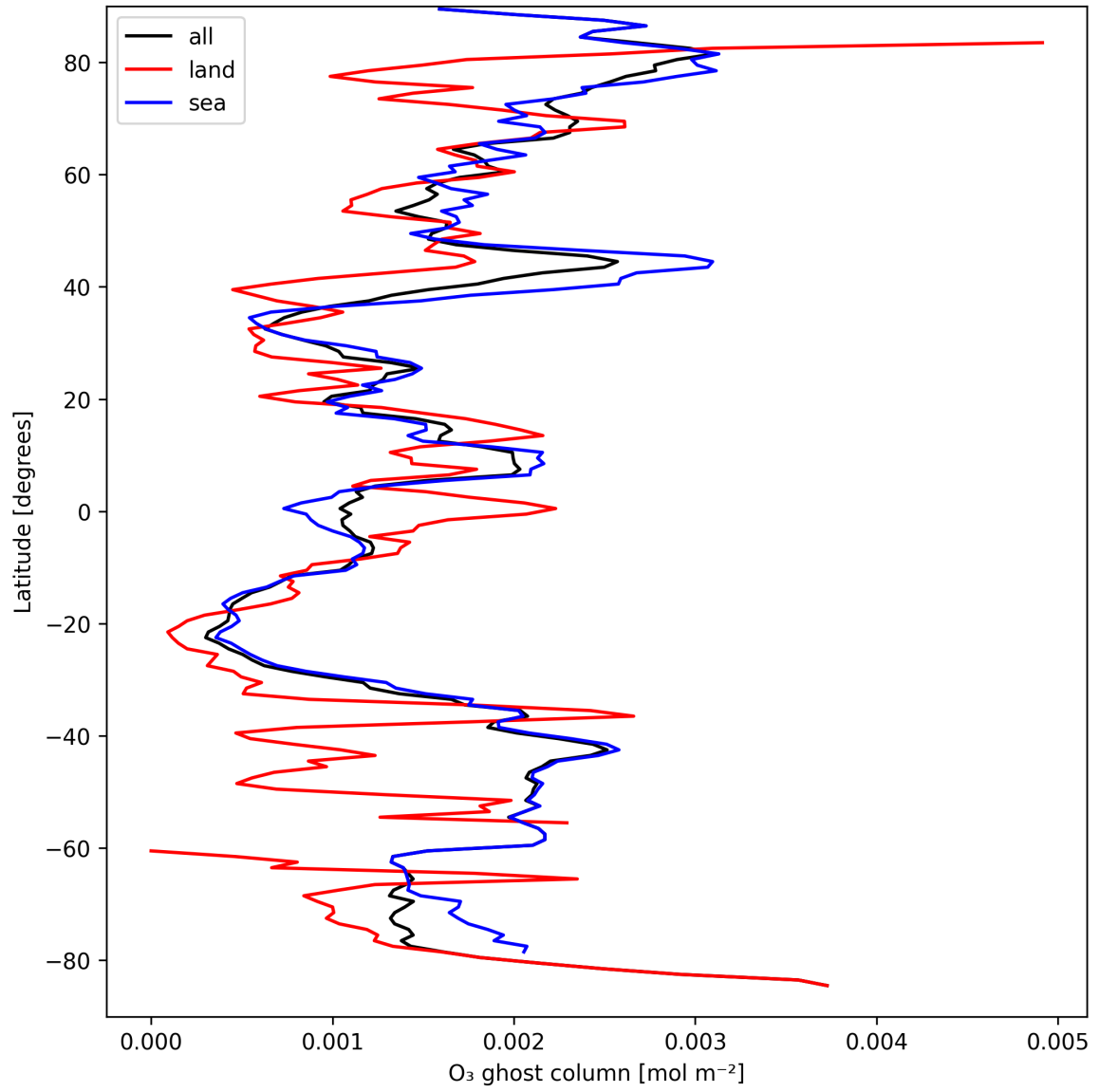
Figure 18: Zonal average of "O 3 ghost column" for 2025-09-10 to 2025-09-11.
