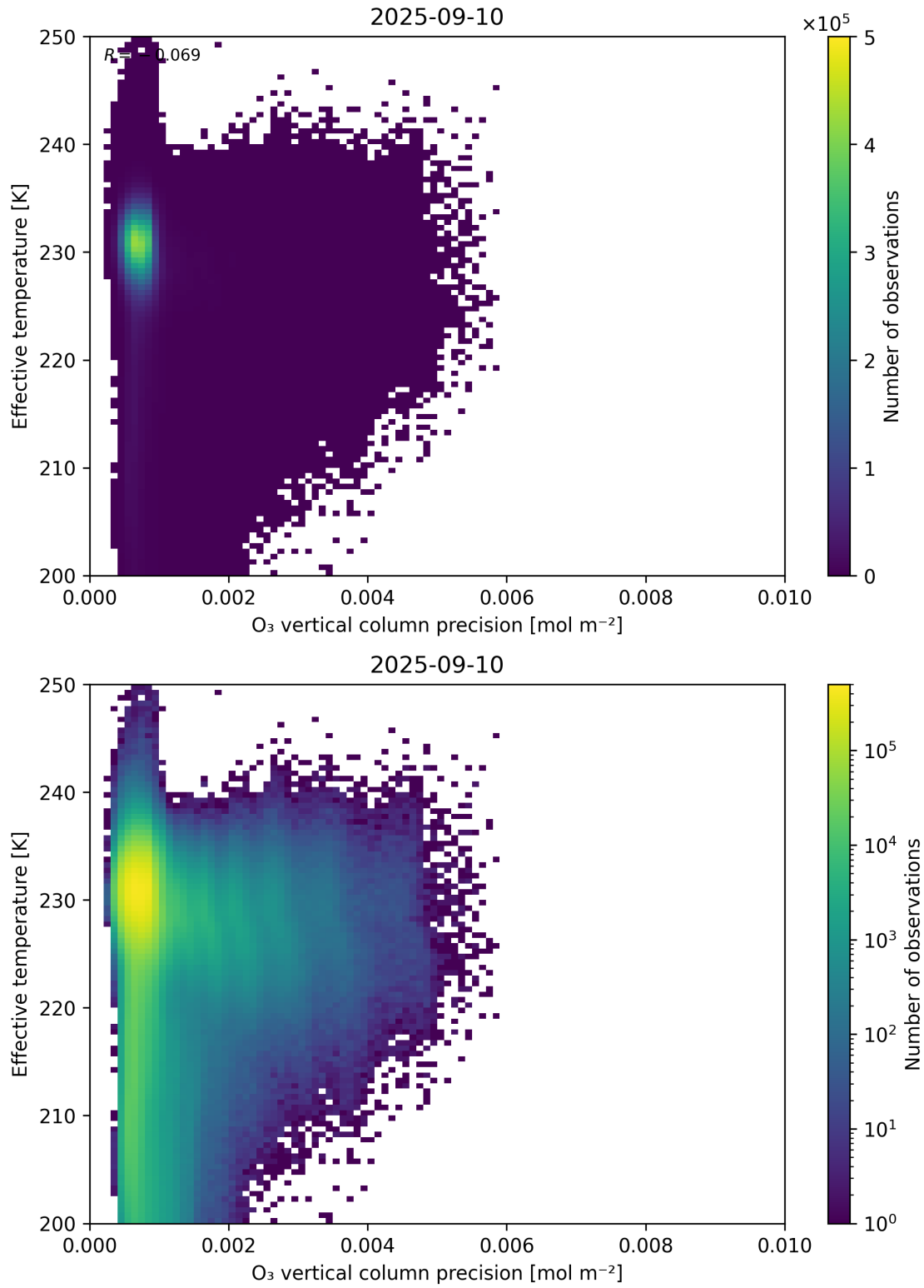
Figure 42: Scatter density plot of “O 3 vertical column precision” against “Effective temperature” for 2025-09-10 to 2025-09-11.
