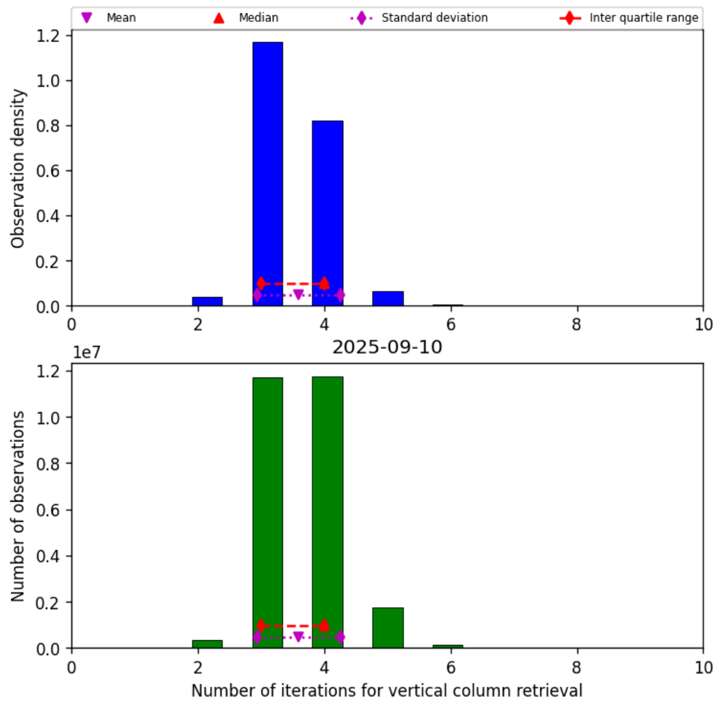
Figure 26: Histogram of “Number of iterations for vertical column retrieval” for 2025-09-10 to 2025-09-11
