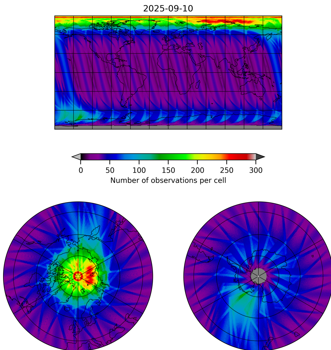
Figure 12: Map of the number of observations for 2025-09-10 to 2025-09-11
