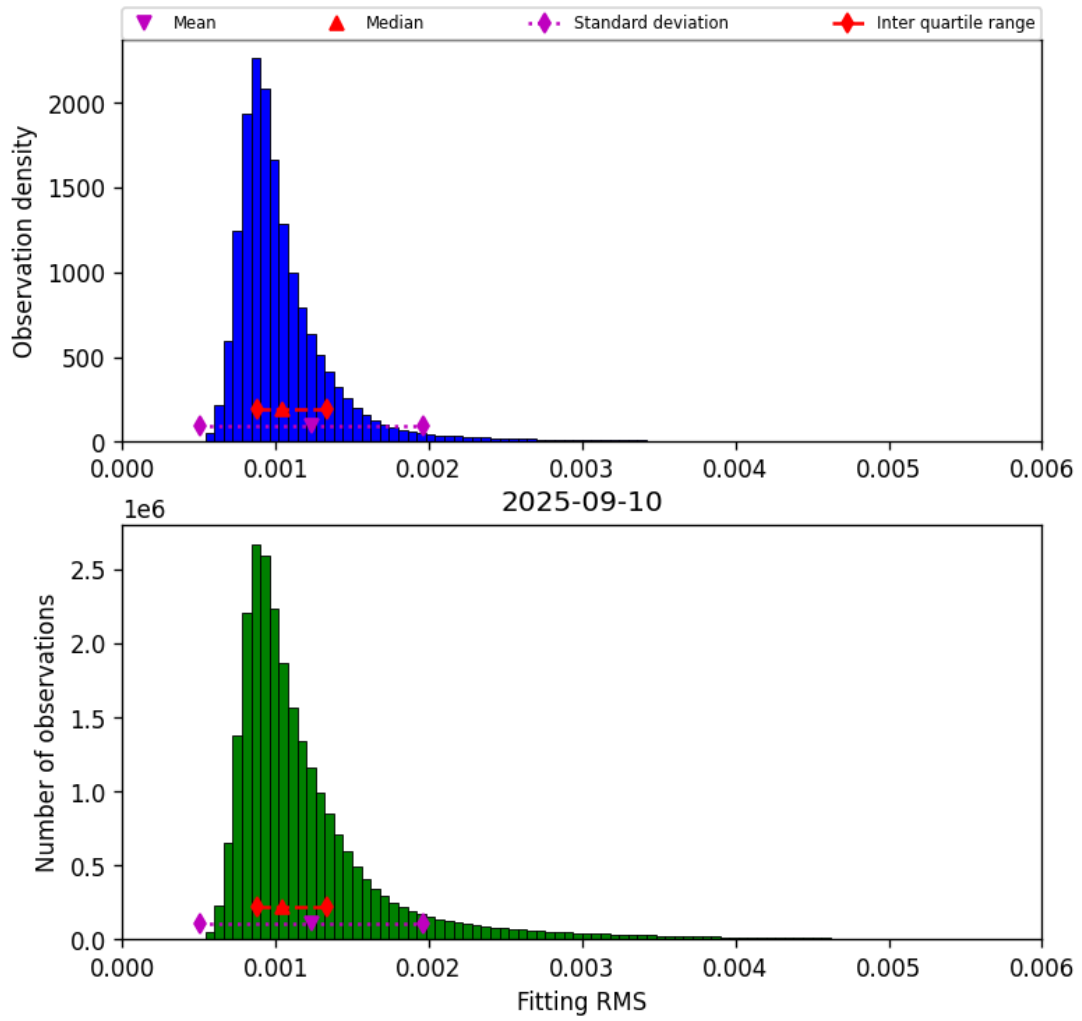
Figure 23: Histogram of “Fitting RMS” for 2025-09-10 to 2025-09-11
