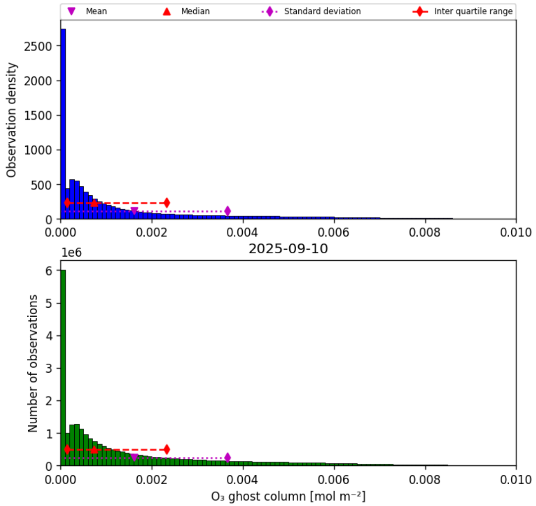
Figure 25: Histogram of “O 3 ghost column” for 2025-09-10 to 2025-09-11
