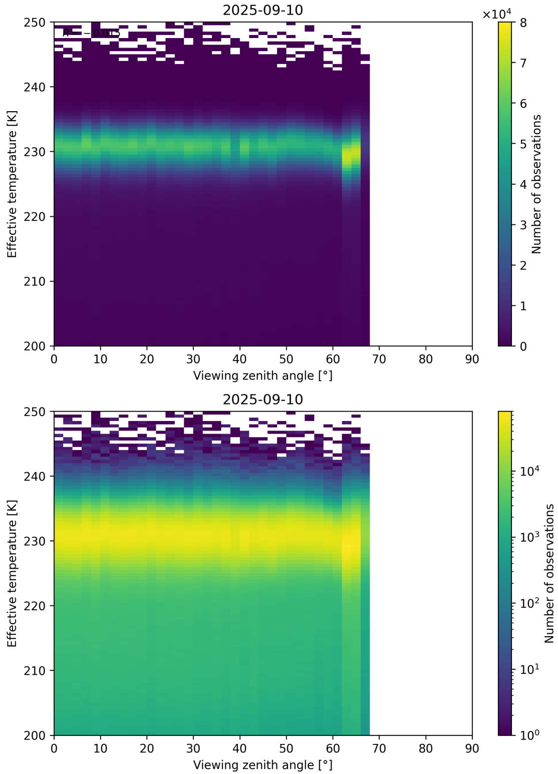
Figure 50: Scatter density plot of “Viewing zenith angle” against “Effective temperature” for 2025-09-10 to 2025-09-11.
