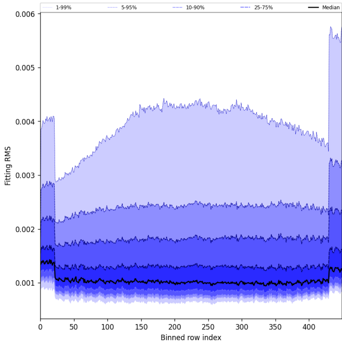
Figure 30: Along track statistics of “Fitting RMS” for 2025-09-10 to 2025-09-11
