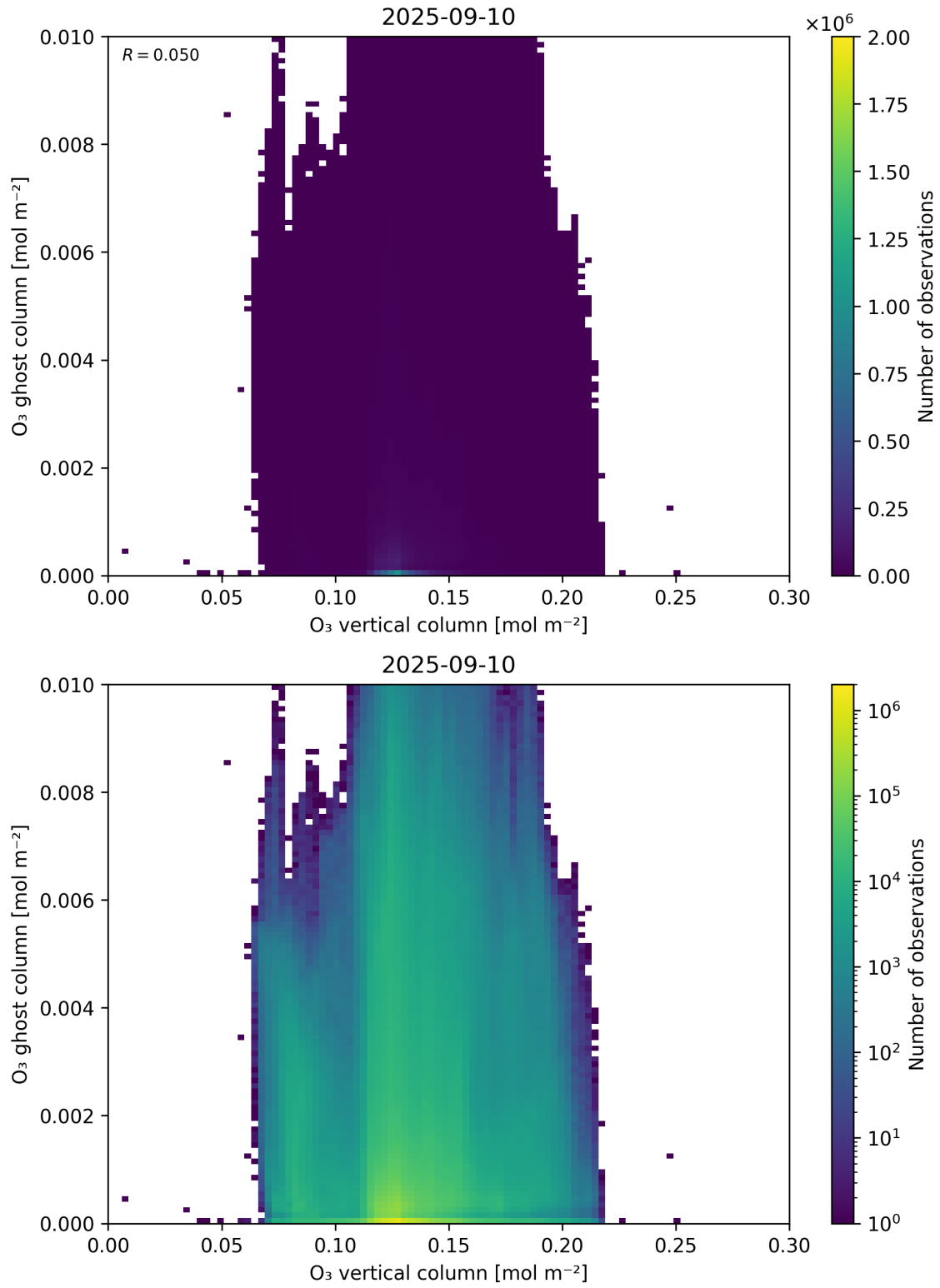
Figure 40: Scatter density plot of “O 3 vertical column” against “O 3 ghost column” for 2025-09-10 to 2025-09-11.
