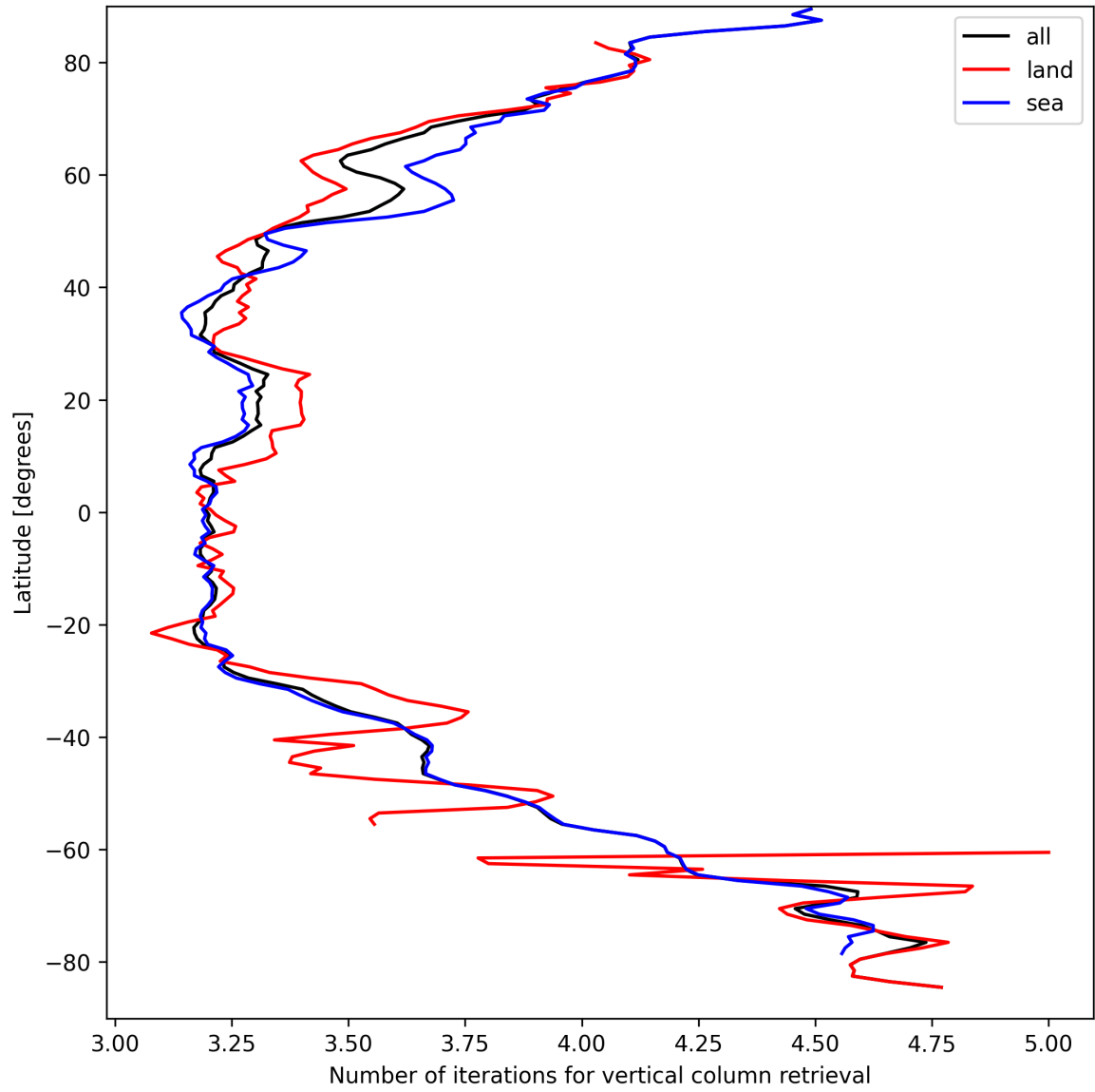
Figure 19: Zonal average of “Number of iterations for vertical column retrieval” for 2025-09-10 to 2025-09-11.
