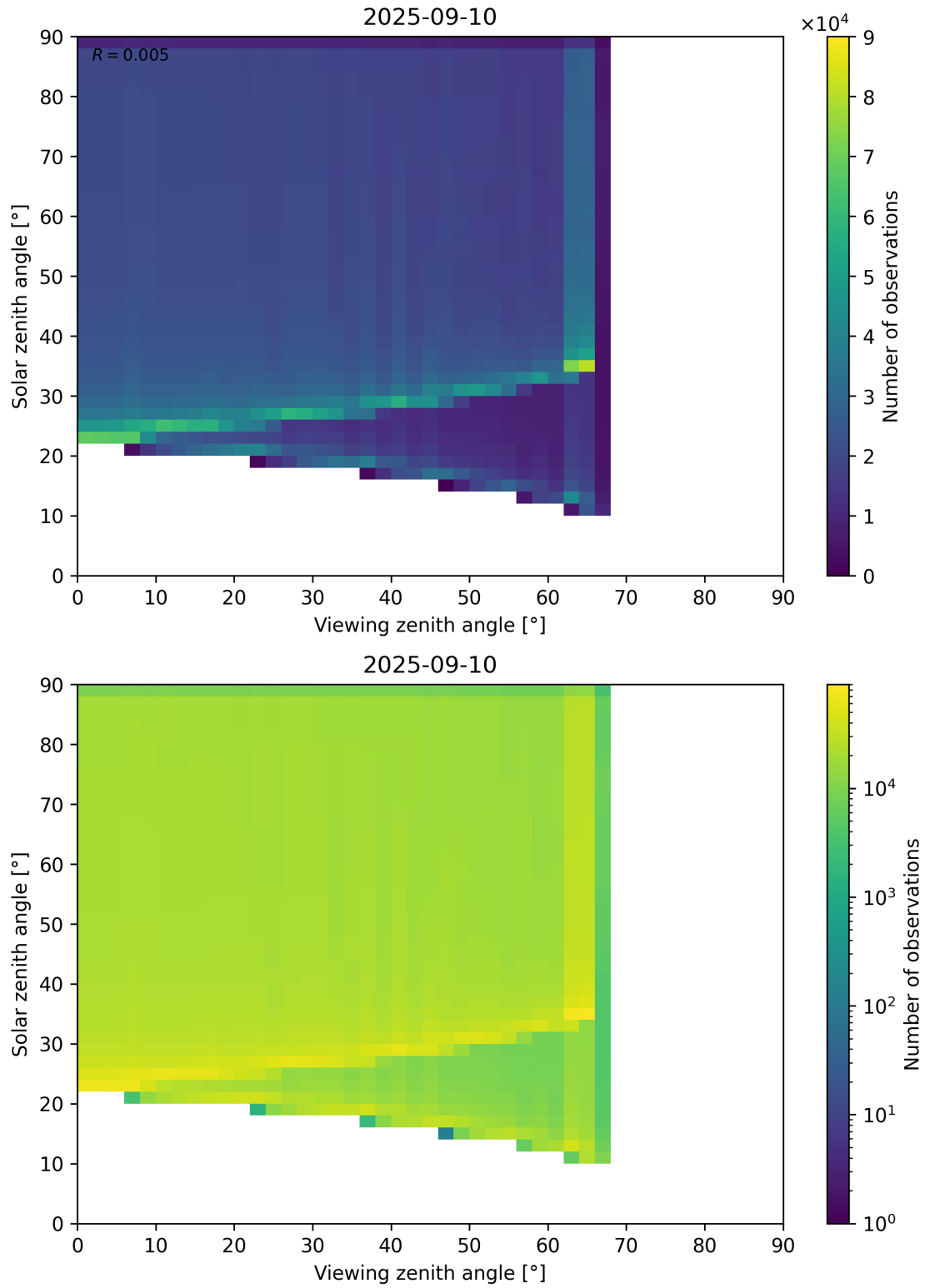
Figure 54: Scatter density plot of “Viewing zenith angle” against “Solar zenith angle” for 2025-09-10 to 2025-09-11.
