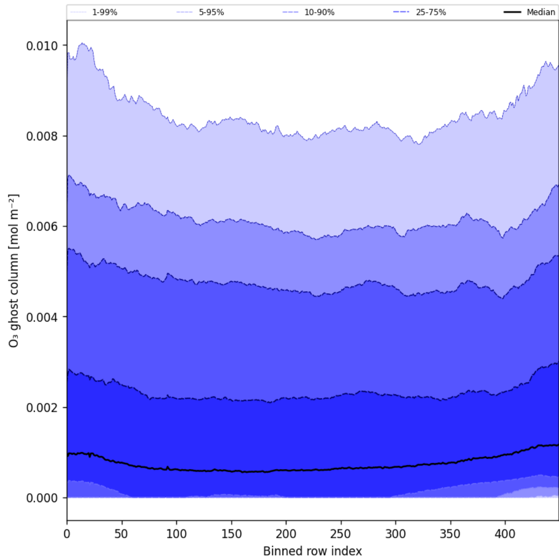
Figure 32: Along track statistics of “O 3 ghost column” for 2025-09-10 to 2025-09-11
