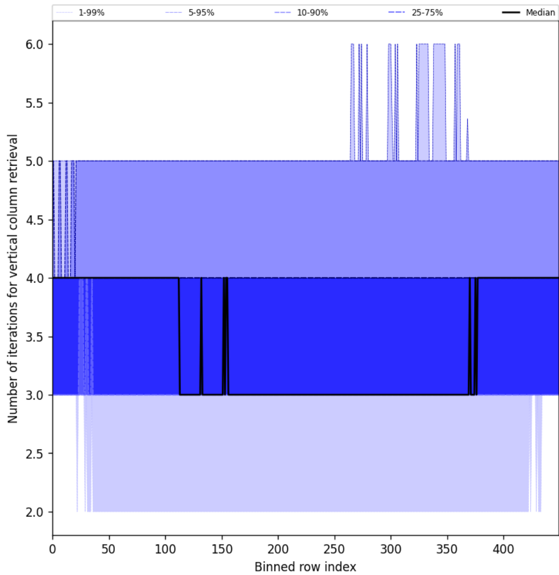
Figure 33: Along track statistics of “Number of iterations for vertical column retrieval” for 2025-09-10 to 2025-09-11
