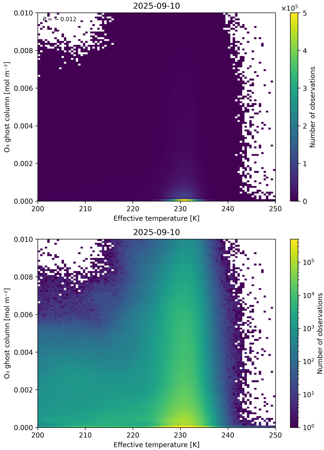
Figure 38: Scatter density plot of “Effective temperature” against “O 3 ghost column” for 2025-09-10 to 2025-09-11.
