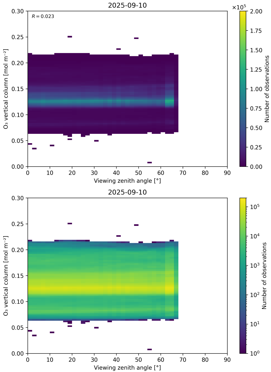
Figure 52: Scatter density plot of “Viewing zenith angle” against “O 3 vertical column” for 2025-09-10 to 2025-09-11.
