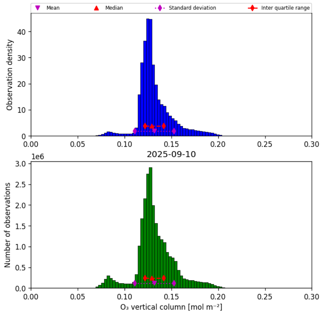
Figure 21: Histogram of “O 3 vertical column” for 2025-09-10 to 2025-09-11
