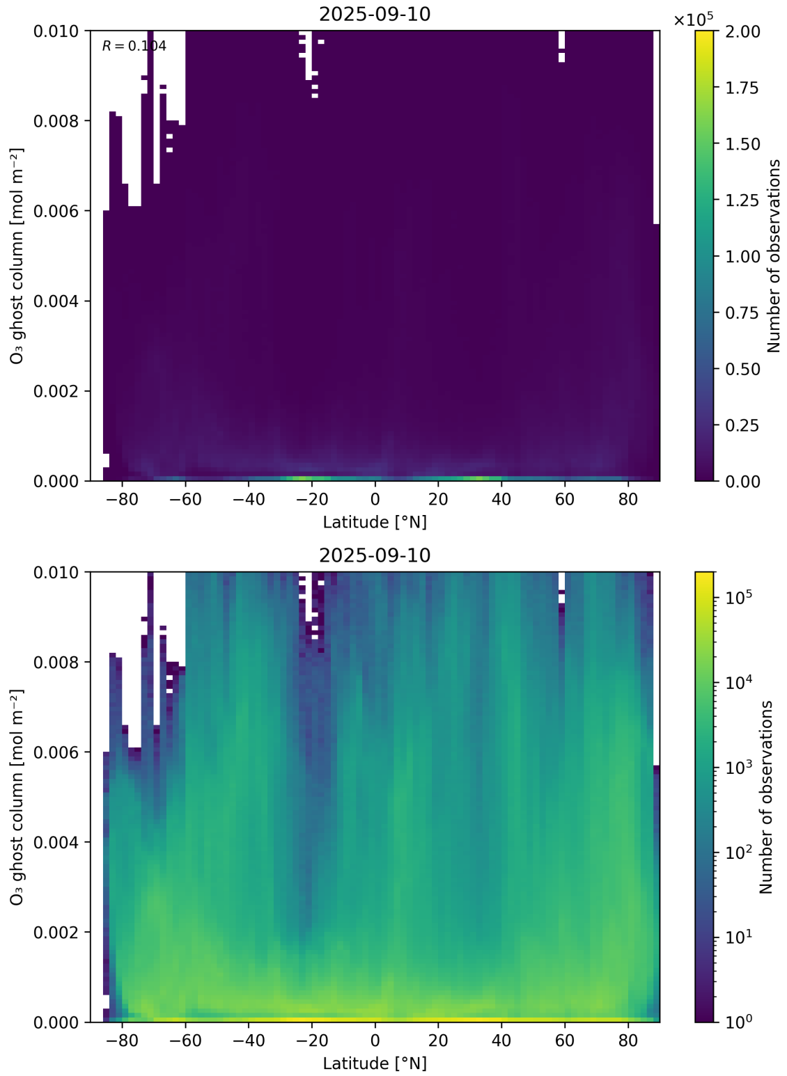
Figure 35: Scatter density plot of “Latitude” against “O 3 ghost column” for 2025-09-10 to 2025-09-11.
