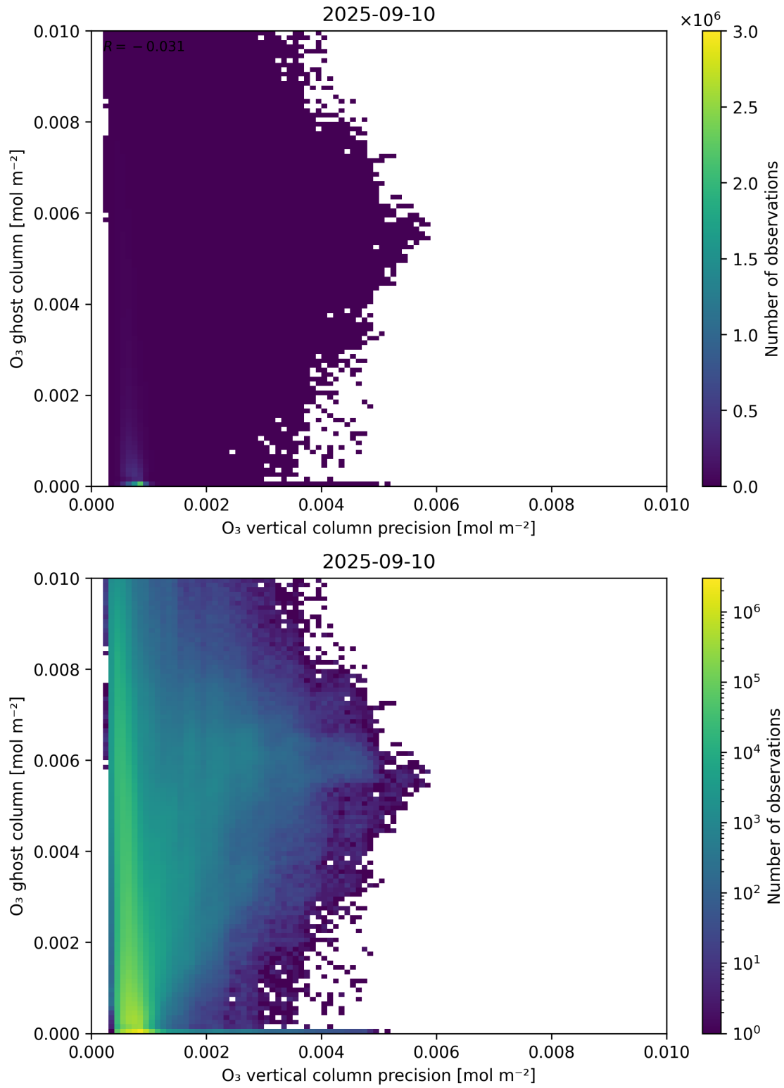
Figure 43: Scatter density plot of “ O_3 vertical column precision” against “ O_3 ghost column” for 2025-09-10 to 2025-09-11.
