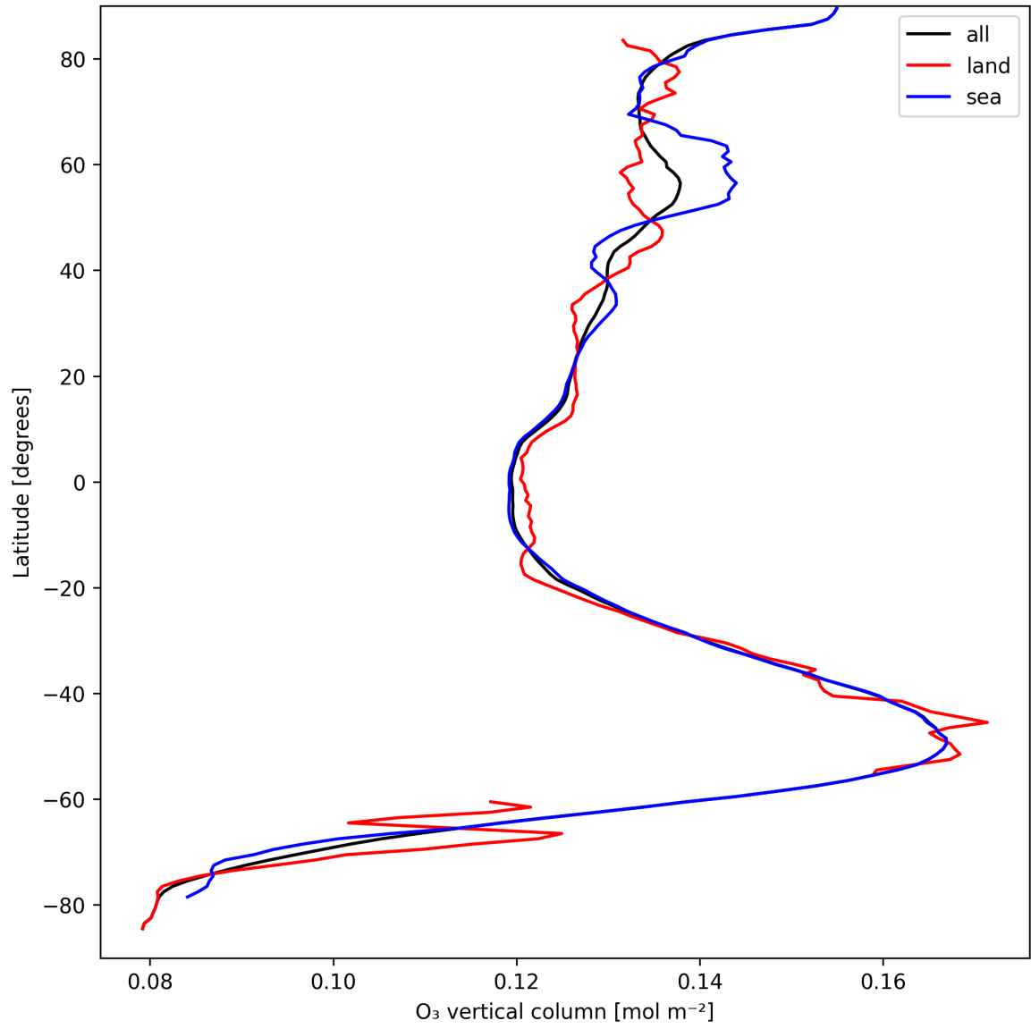
Figure 14: Zonal average of “O 3 vertical column” for 2025-09-10 to 2025-09-11.
