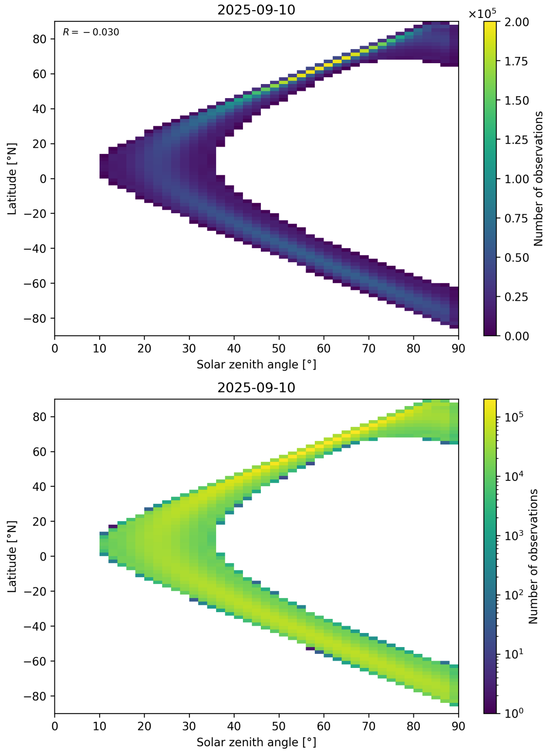
Figure 44: Scatter density plot of “Solar zenith angle” against “Latitude” for 2025-09-10 to 2025-09-11.
