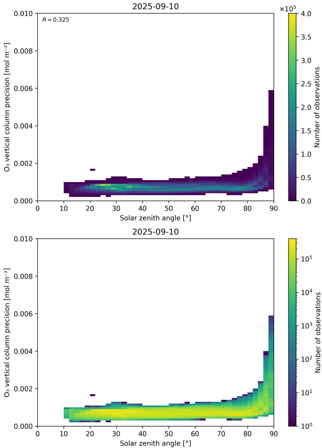
Figure 48: Scatter density plot of “Solar zenith angle” against “O 3 vertical column precision” for 2025-09-10 to 2025-09-11.
