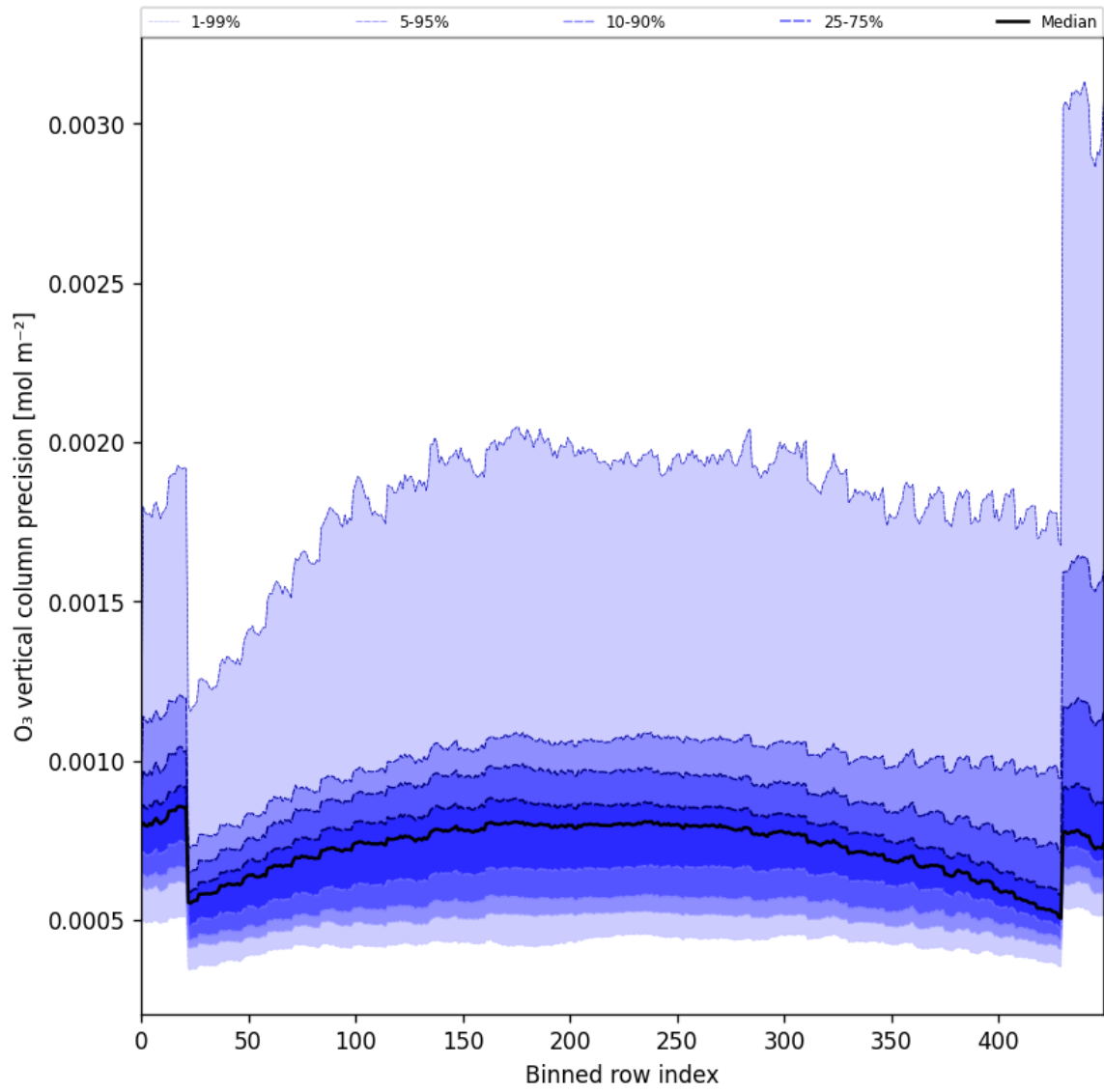
Figure 29: Along track statistics of “O 3 vertical column precision” for 2025-09-10 to 2025-09-11
