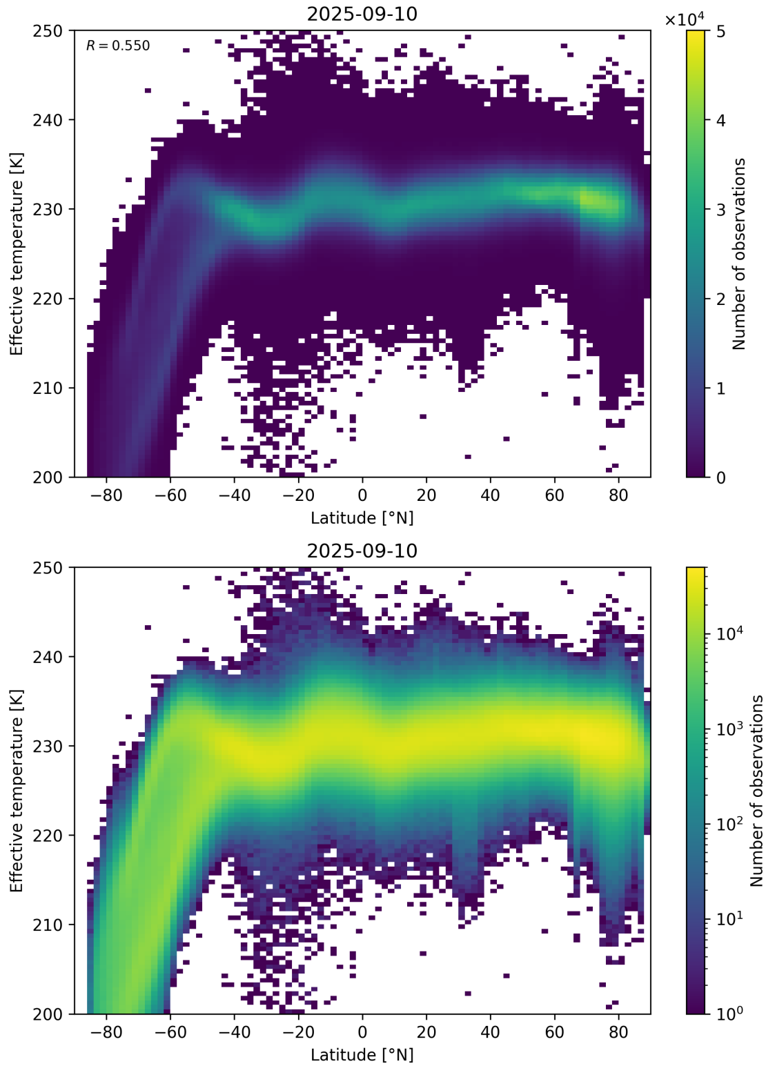
Figure 34: Scatter density plot of “Latitude” against “Effective temperature” for 2025-09-10 to 2025-09-11.
