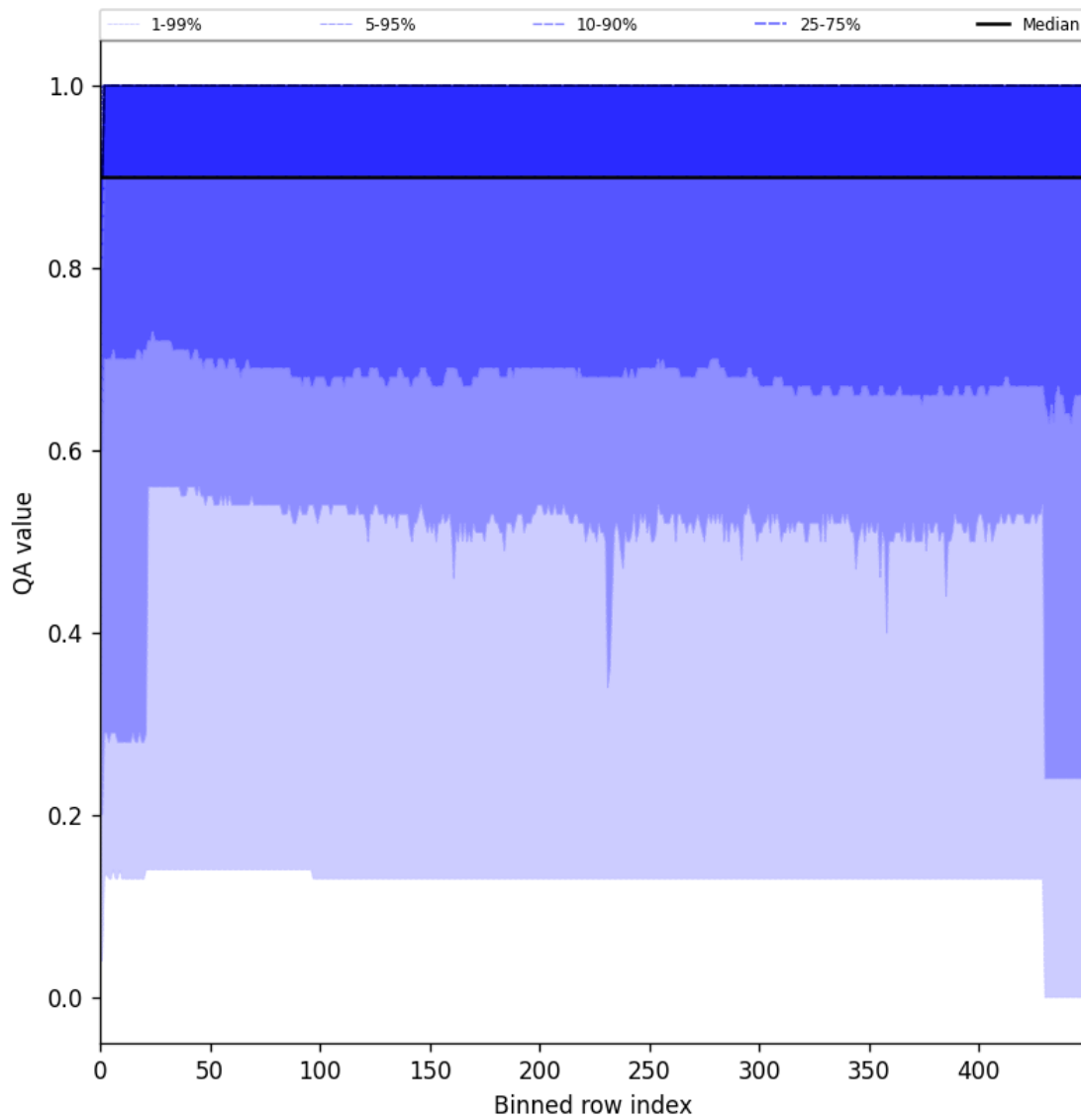
Figure 27: Along track statistics of “QA value” for 2025-09-10 to 2025-09-11
