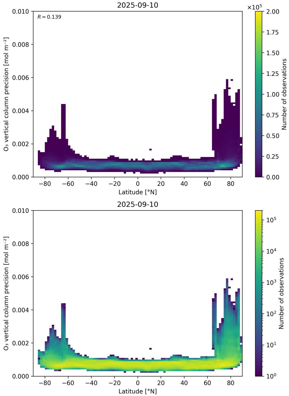
Figure 37: Scatter density plot of “Latitude” against “O 3 vertical column precision” for 2025-09-10 to 2025-09-11.
