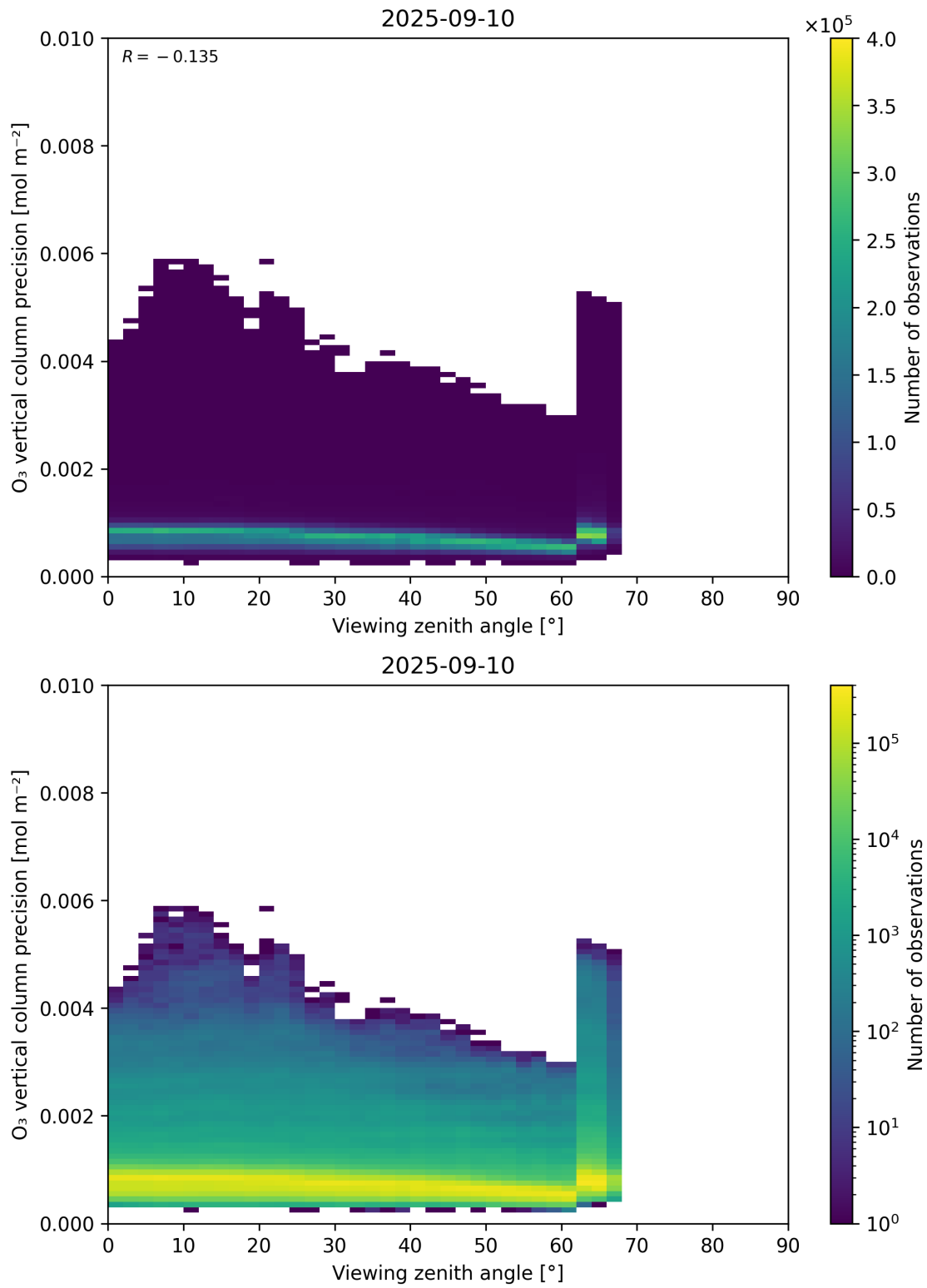
Figure 53: Scatter density plot of “Viewing zenith angle” against “O 3 vertical column precision” for 2025-09-10 to 2025-09-11.
