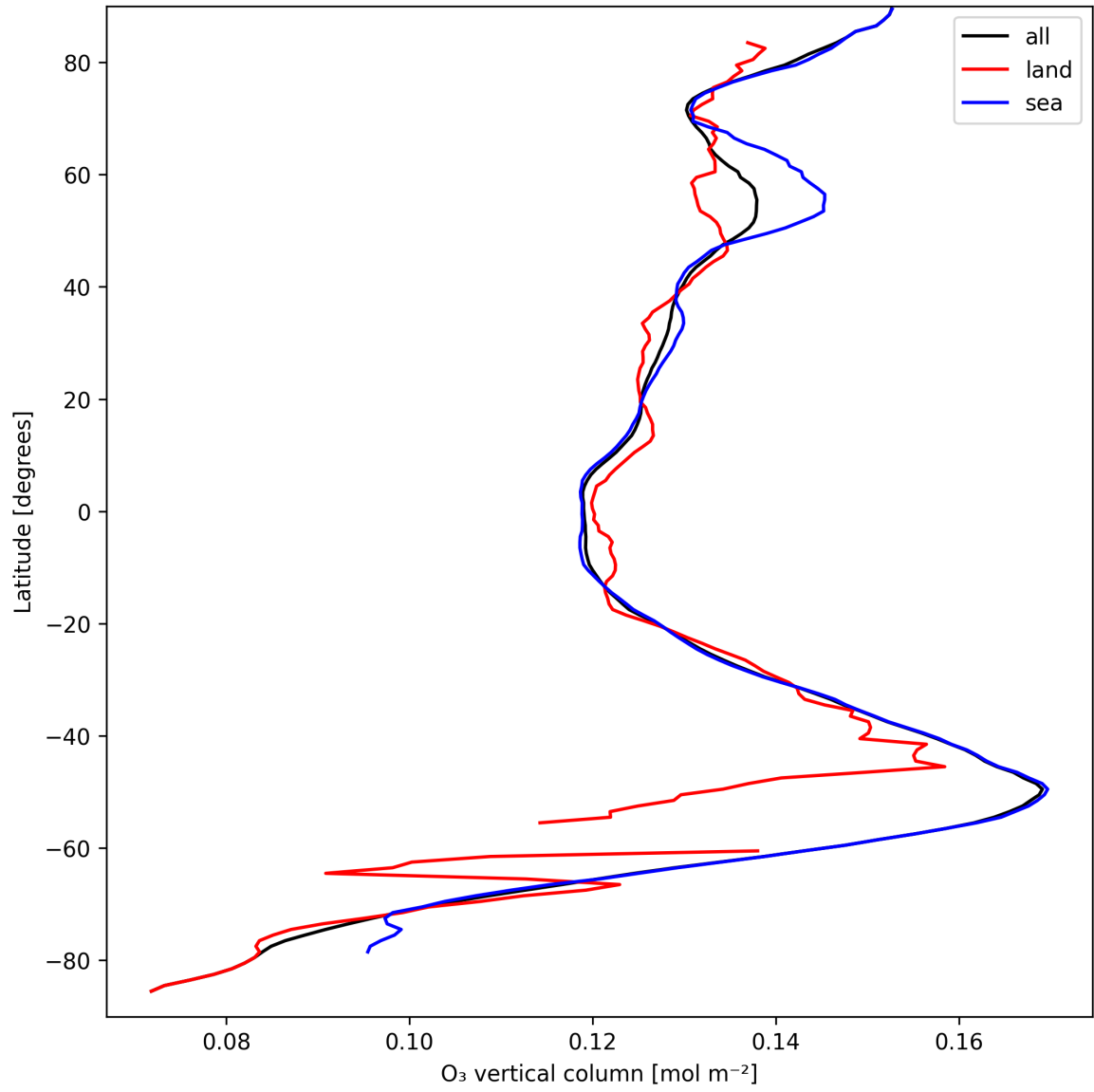
Figure 14: Zonal average of “O 3 vertical column” for 2025-09-11 to 2025-09-13.
