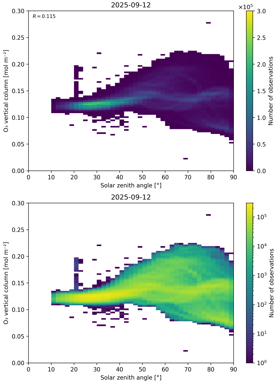
Figure 47: Scatter density plot of “Solar zenith angle” against “O 3 vertical column” for 2025-09-11 to 2025-09-13.
