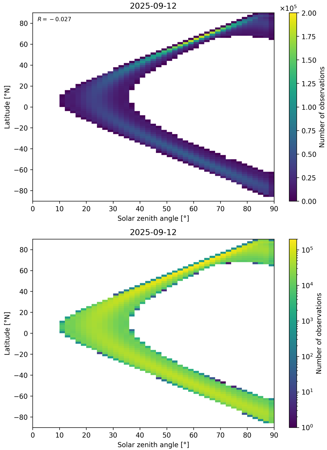
Figure 44: Scatter density plot of “Solar zenith angle” against “Latitude” for 2025-09-11 to 2025-09-13.
