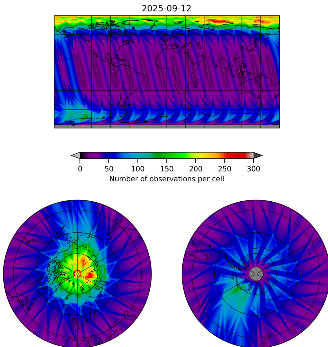
Figure 12: Map of the number of observations for 2025-09-11 to 2025-09-13
