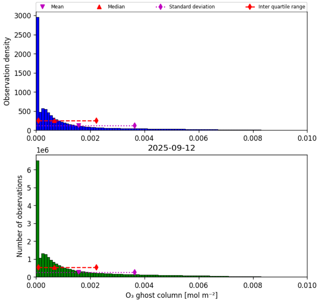
Figure 25: Histogram of “O 3 ghost column” for 2025-09-11 to 2025-09-13
