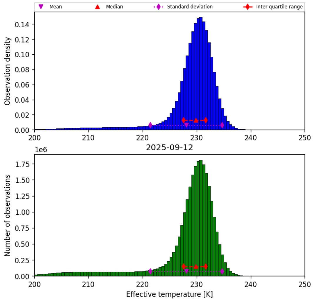
Figure 24: Histogram of “Effective temperature” for 2025-09-11 to 2025-09-13
