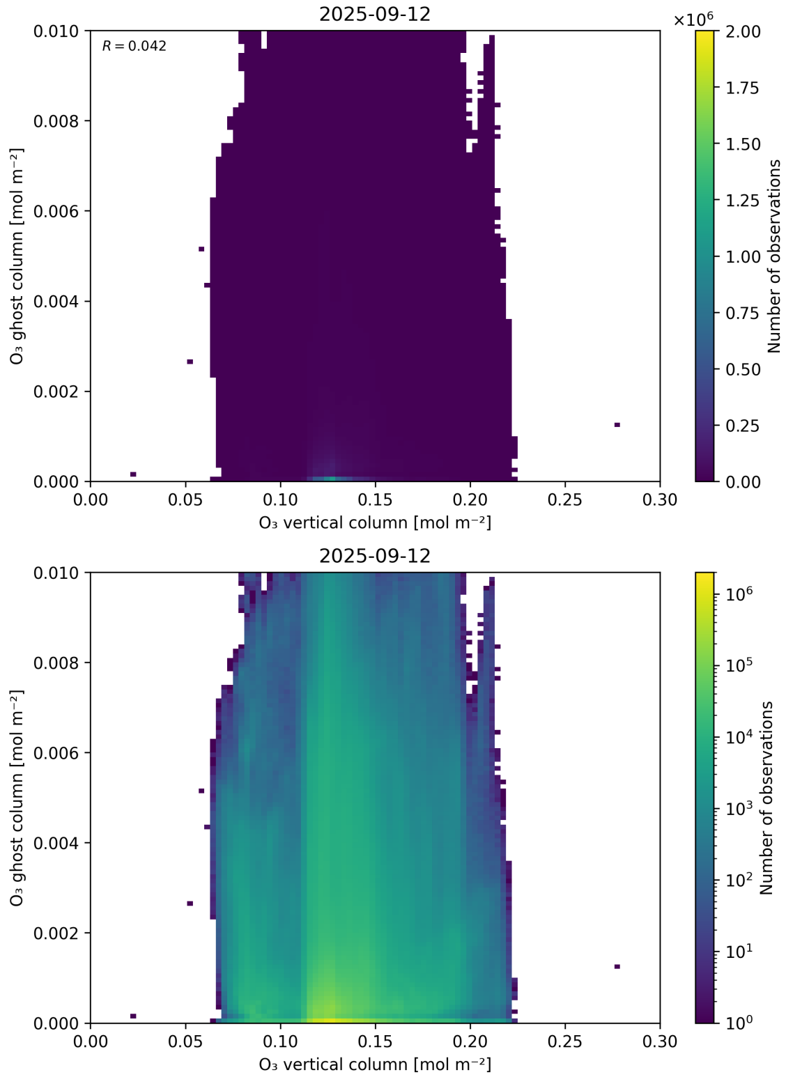
Figure 40: Scatter density plot of “O 3 vertical column” against “O 3 ghost column” for 2025-09-11 to 2025-09-13.
