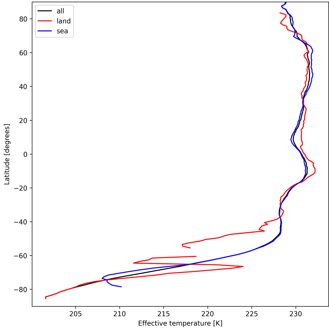
Figure 17: Zonal average of "Effective temperature" for 2025-09-11 to 2025-09-13.
