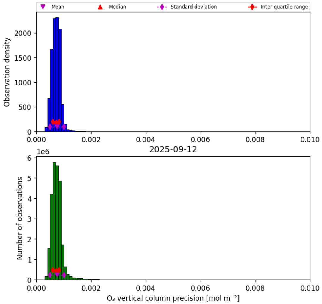
Figure 22: Histogram of “O 3 vertical column precision” for 2025-09-11 to 2025-09-13
