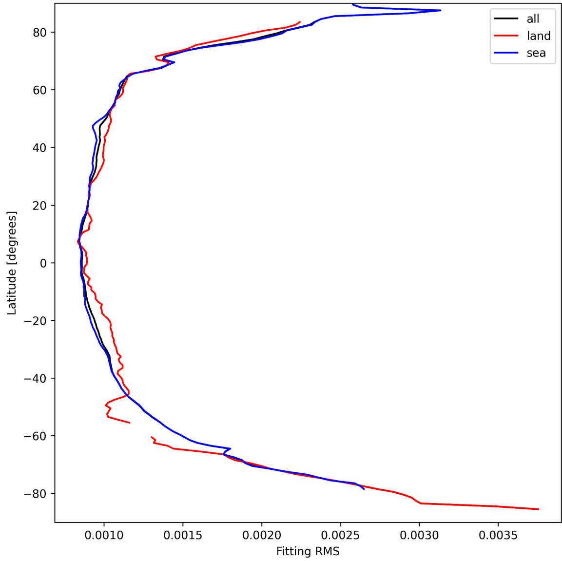
Figure 16: Zonal average of “Fitting RMS” for 2025-09-11 to 2025-09-13.
