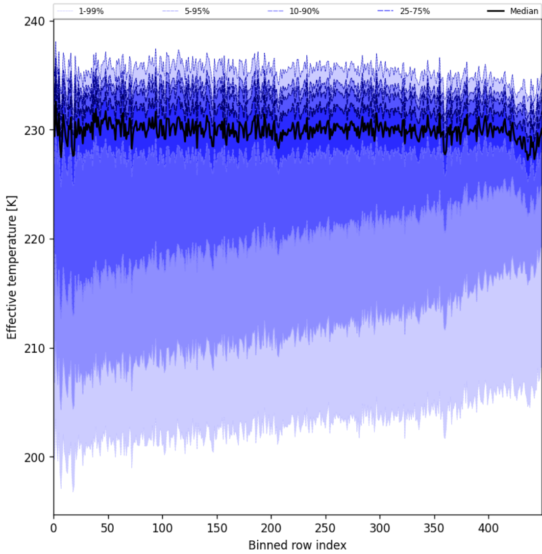
Figure 31: Along track statistics of “Effective temperature” for 2025-09-11 to 2025-09-13
