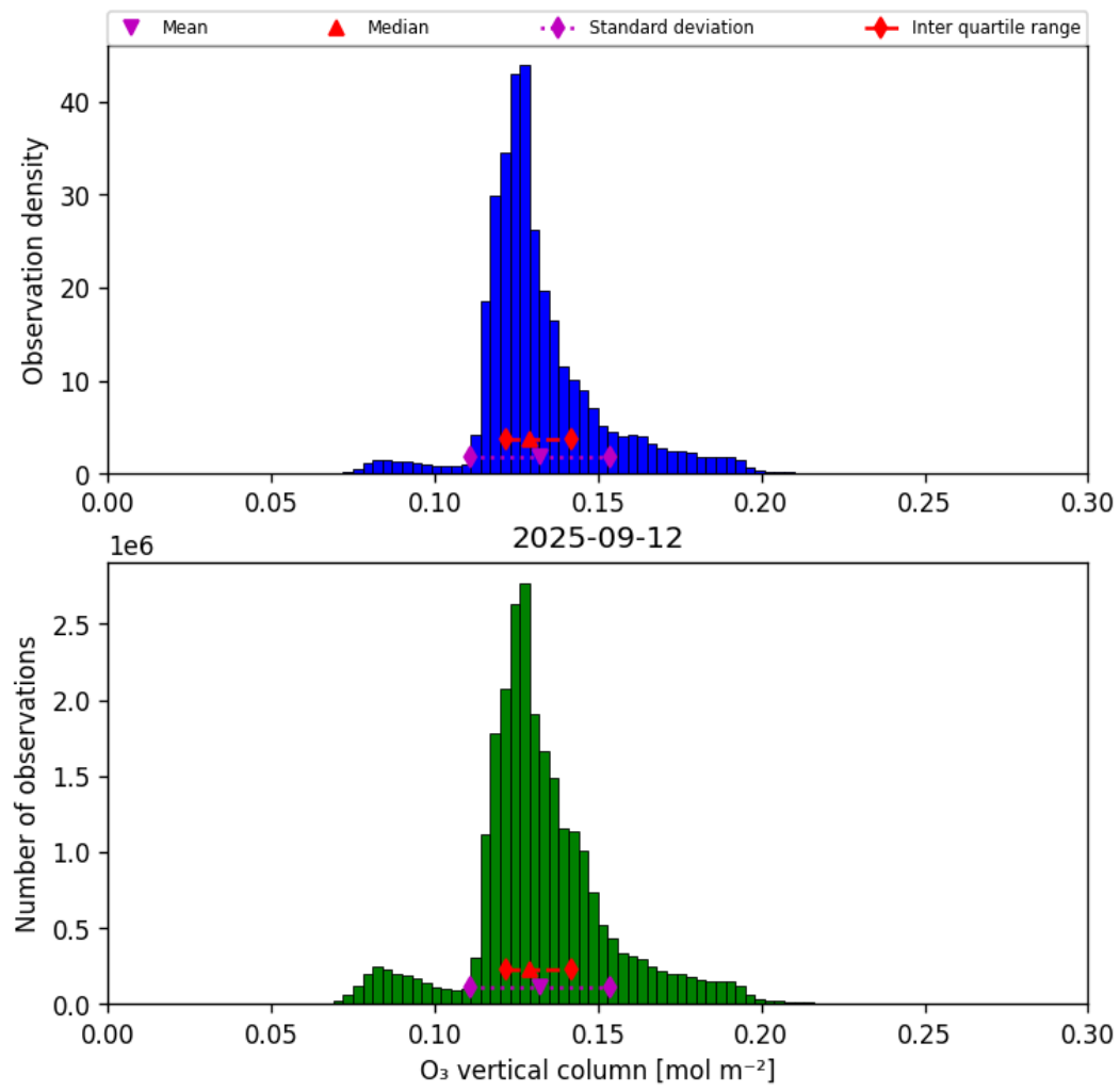
Figure 21: Histogram of “O 3 vertical column” for 2025-09-11 to 2025-09-13
