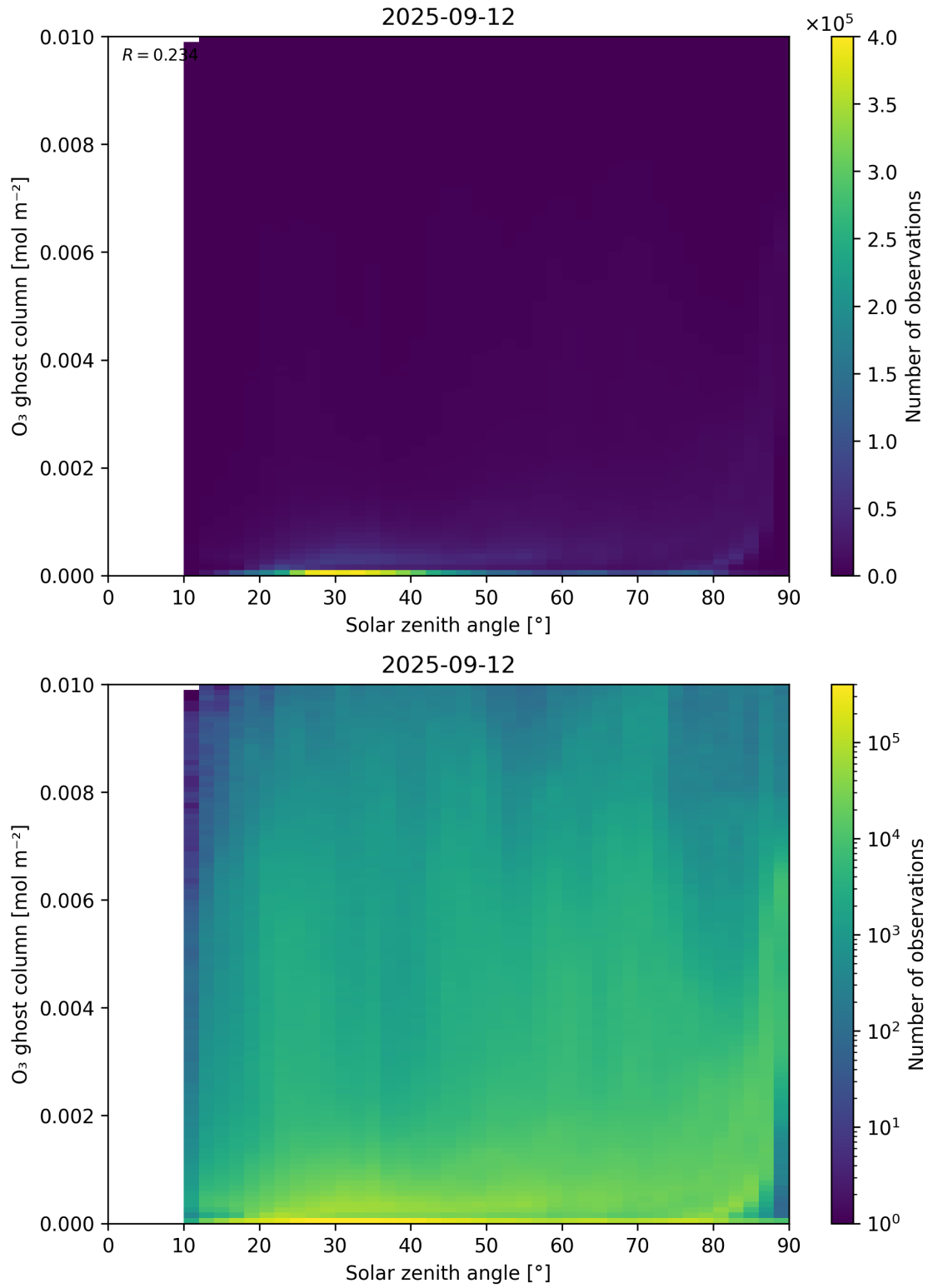
Figure 46: Scatter density plot of “Solar zenith angle” against “O 3 ghost column” for 2025-09-11 to 2025-09-13.
