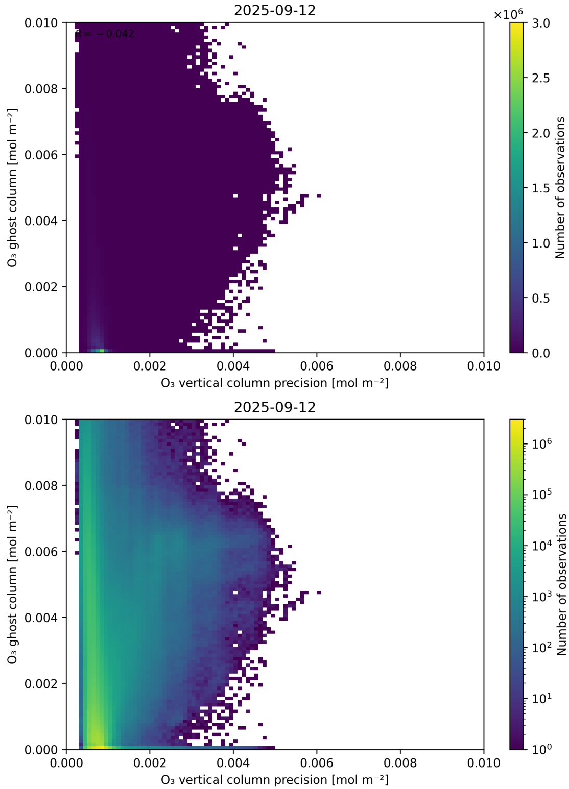
Figure 43: Scatter density plot of “O 3 vertical column precision” against “O 3 ghost column” for 2025-09-11 to 2025-09-13.
