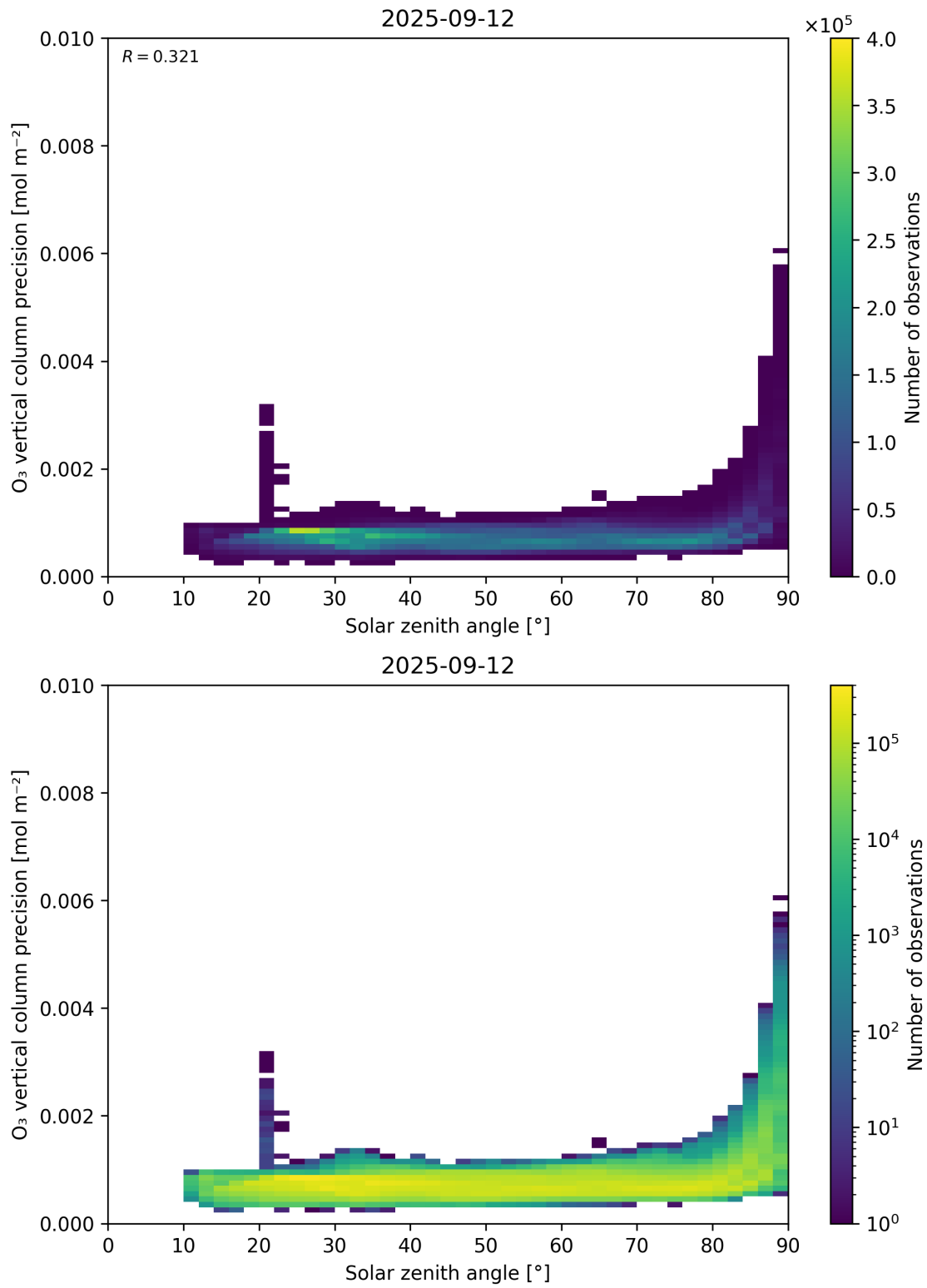
Figure 48: Scatter density plot of “Solar zenith angle” against “O 3 vertical column precision” for 2025-09-11 to 2025-09-13.
