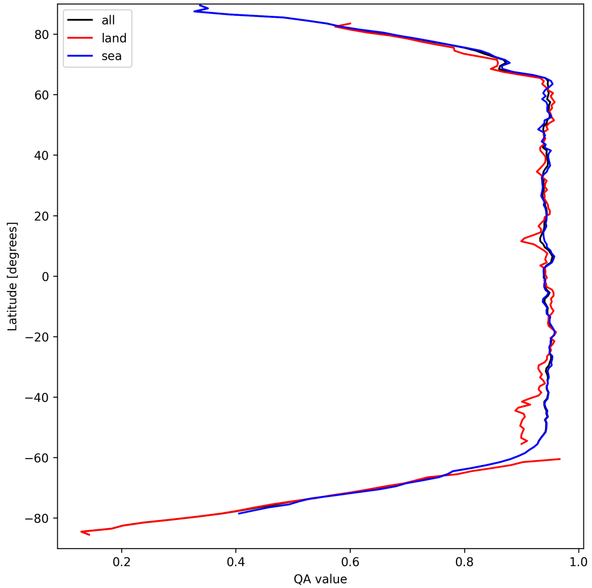
Figure 13: Zonal average of “QA value” for 2025-09-11 to 2025-09-13.
