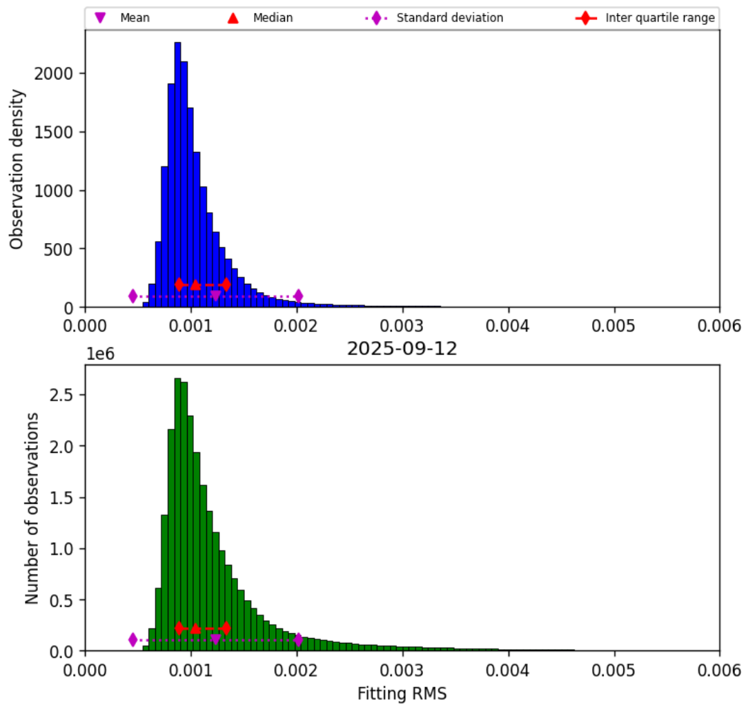
Figure 23: Histogram of “Fitting RMS” for 2025-09-11 to 2025-09-13
