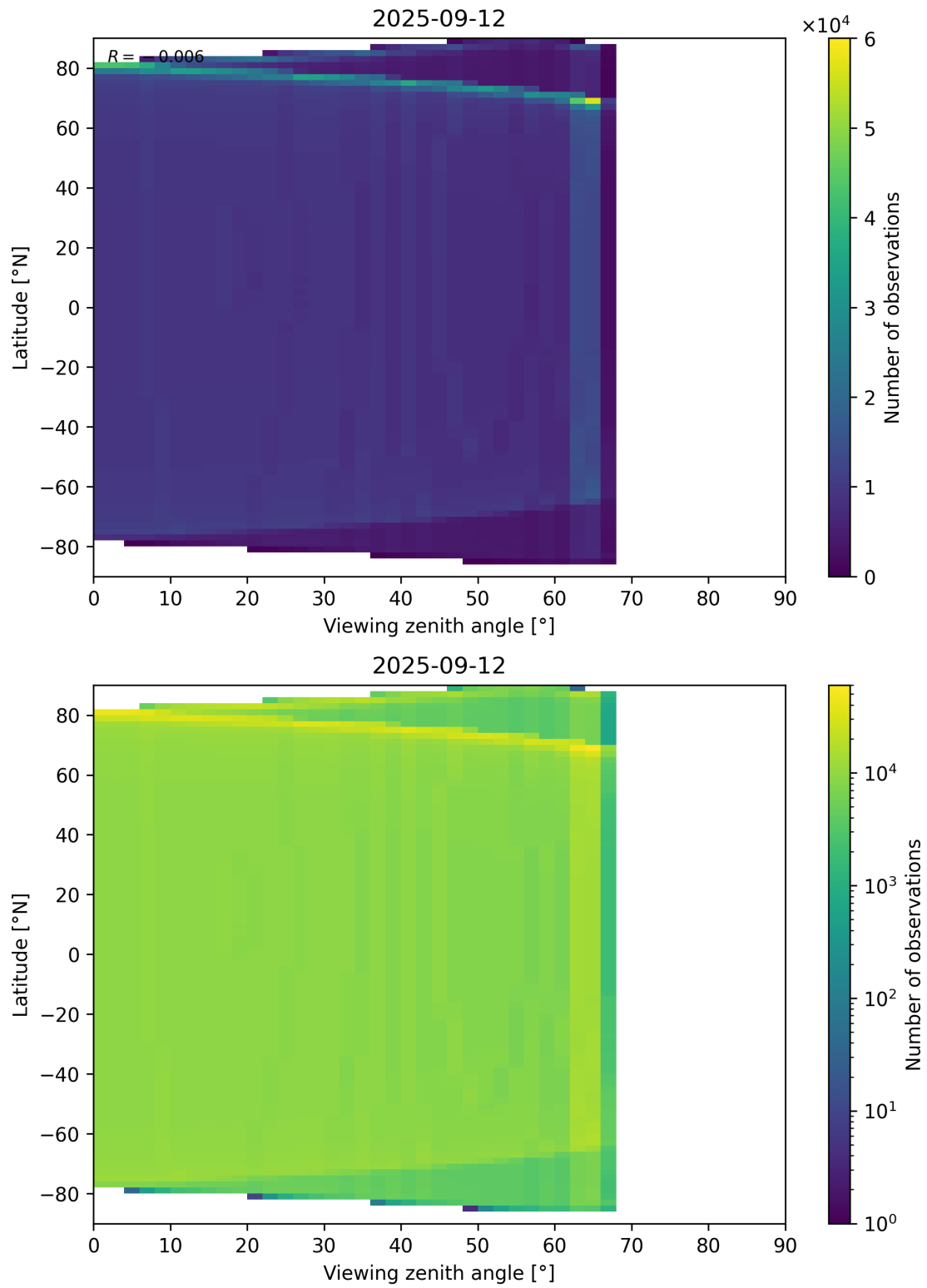
Figure 49: Scatter density plot of “Viewing zenith angle” against “Latitude” for 2025-09-11 to 2025-09-13.
