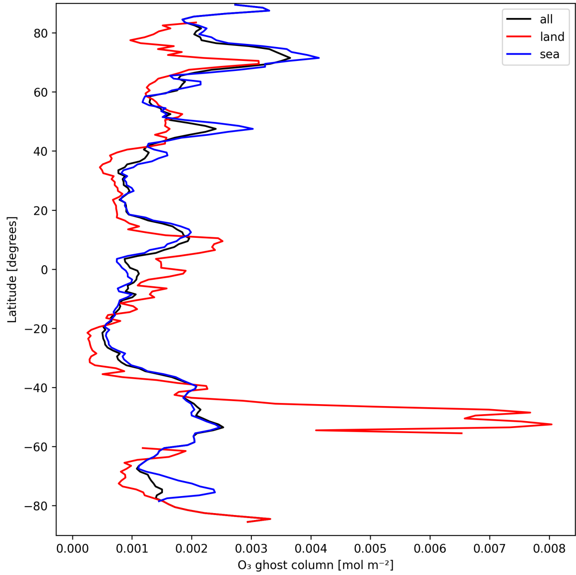
Figure 18: Zonal average of “O 3 ghost column” for 2025-09-11 to 2025-09-13.
