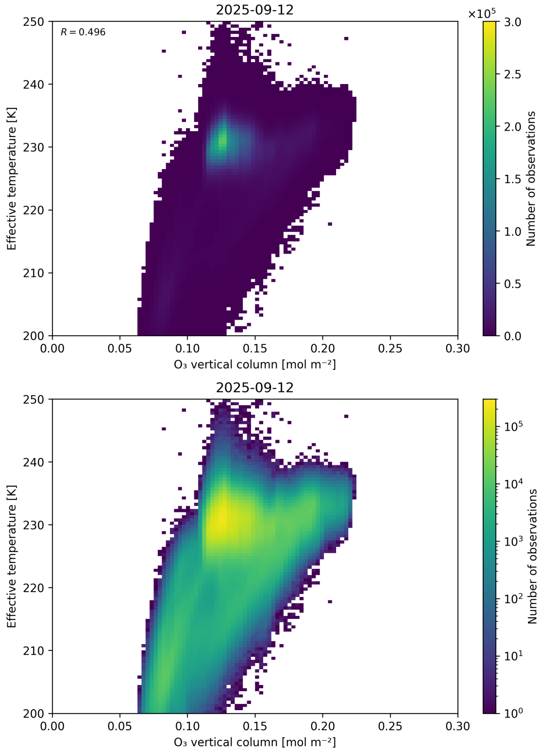
Figure 39: Scatter density plot of “O 3 vertical column” against “Effective temperature” for 2025-09-11 to 2025-09-13.
