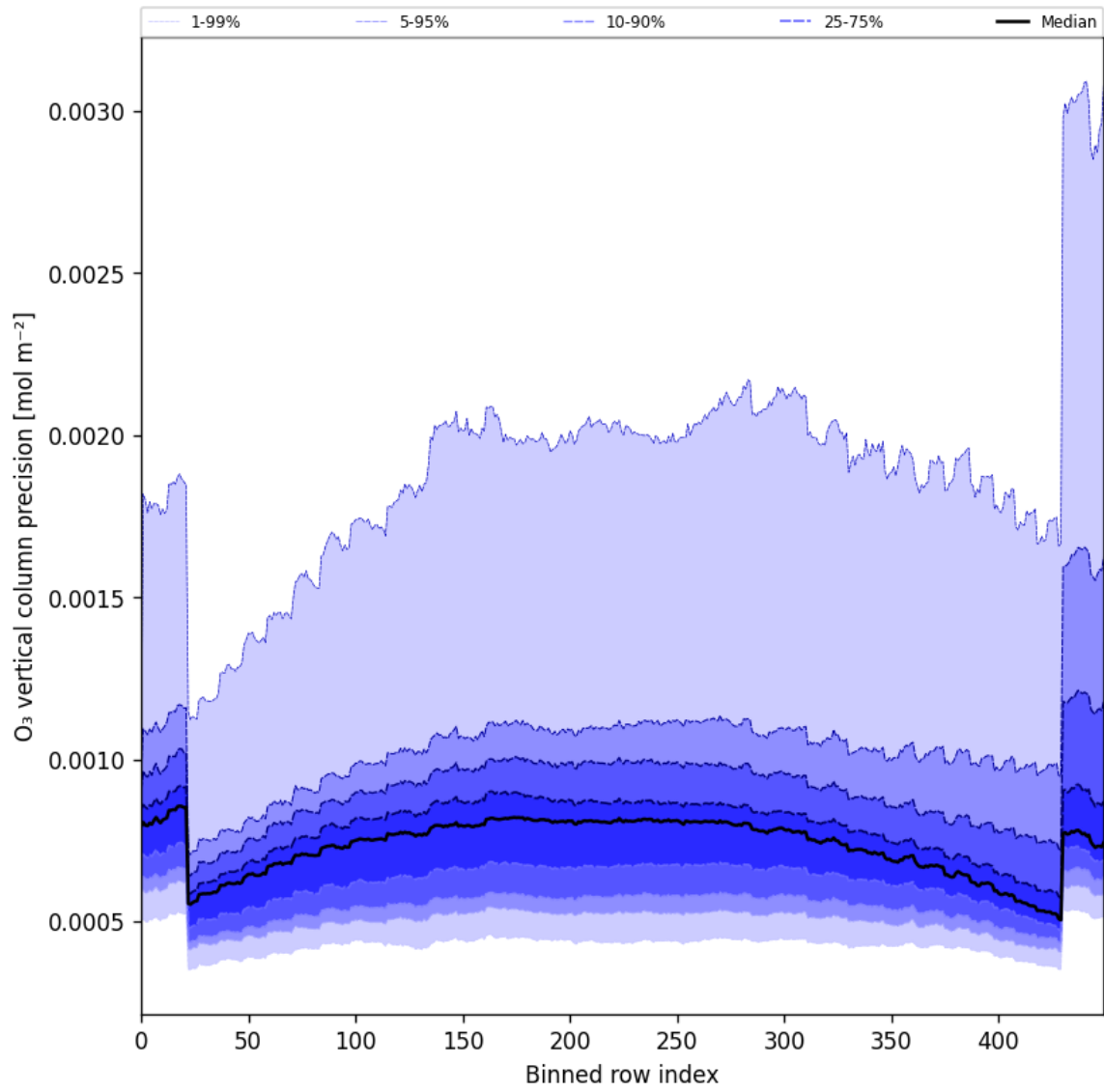
Figure 29: Along track statistics of “O 3 vertical column precision” for 2025-09-11 to 2025-09-13
