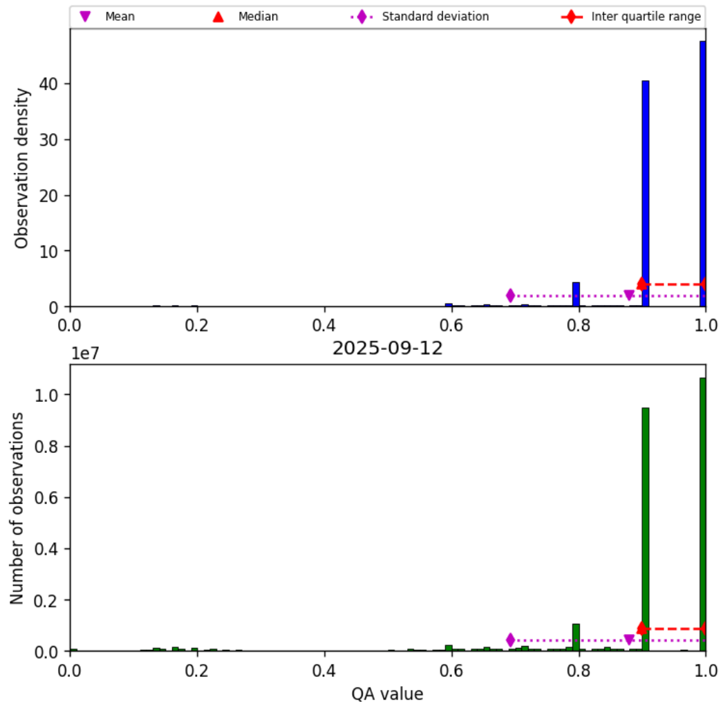
Figure 20: Histogram of “QA value” for 2025-09-11 to 2025-09-13
