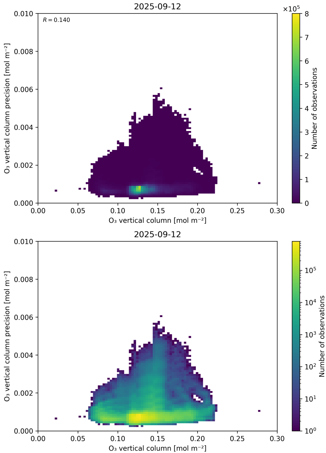
Figure 41: Scatter density plot of “O 3 vertical column” against “O 3 vertical column precision” for 2025-09-11 to 2025-09-13.
