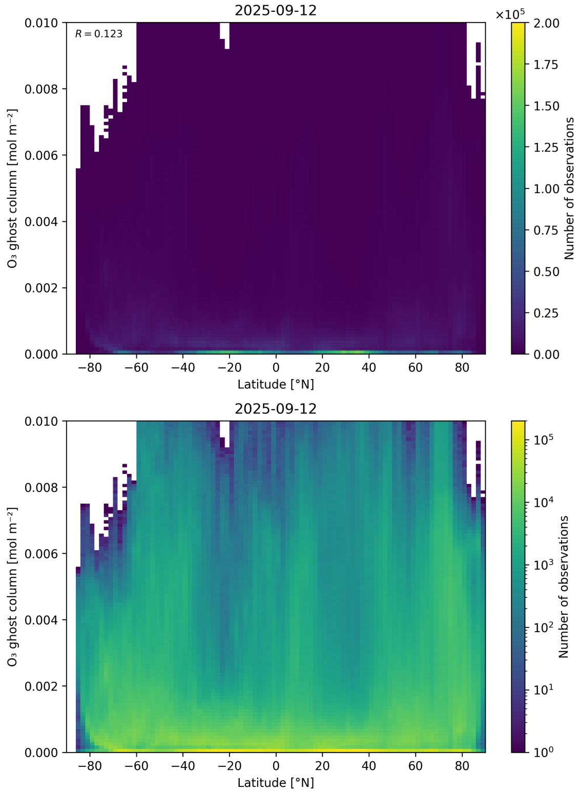
Figure 35: Scatter density plot of “Latitude” against “O 3 ghost column” for 2025-09-11 to 2025-09-13.
