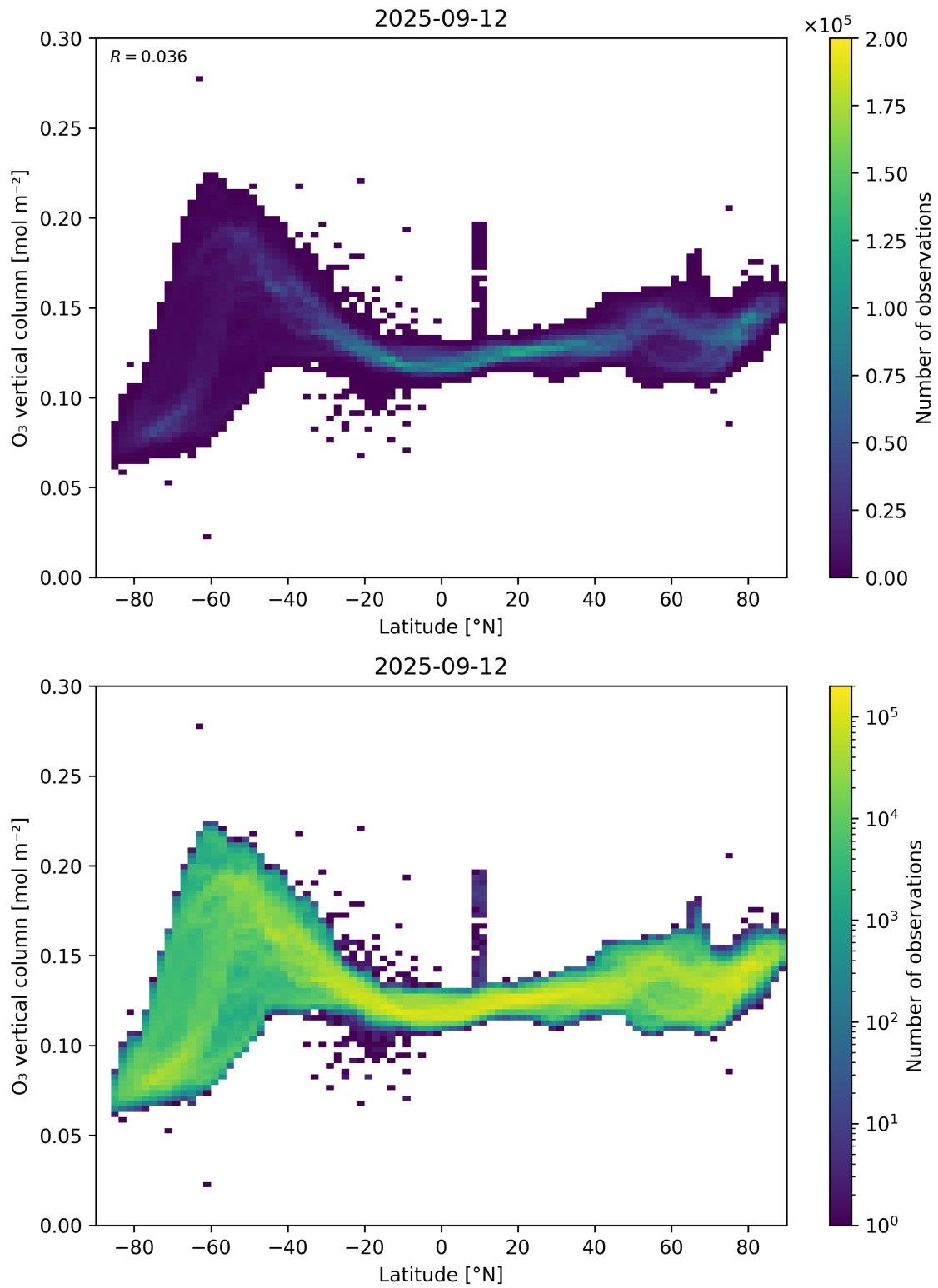
Figure 36: Scatter density plot of “Latitude” against “O 3 vertical column” for 2025-09-11 to 2025-09-13.
