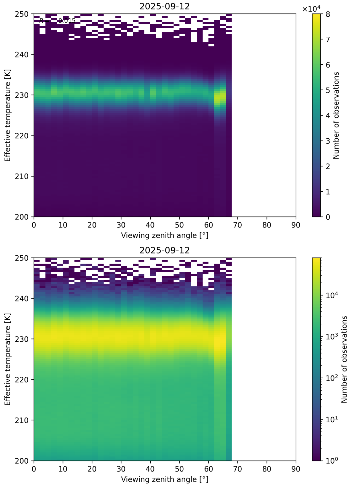
Figure 50: Scatter density plot of “Viewing zenith angle” against “Effective temperature” for 2025-09-11 to 2025-09-13.
