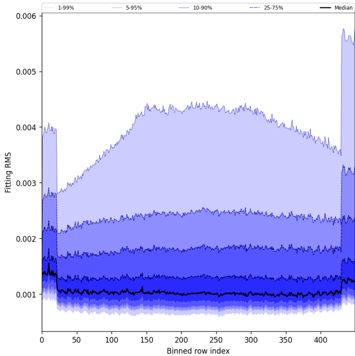
Figure 30: Along track statistics of “Fitting RMS” for 2025-09-11 to 2025-09-13
