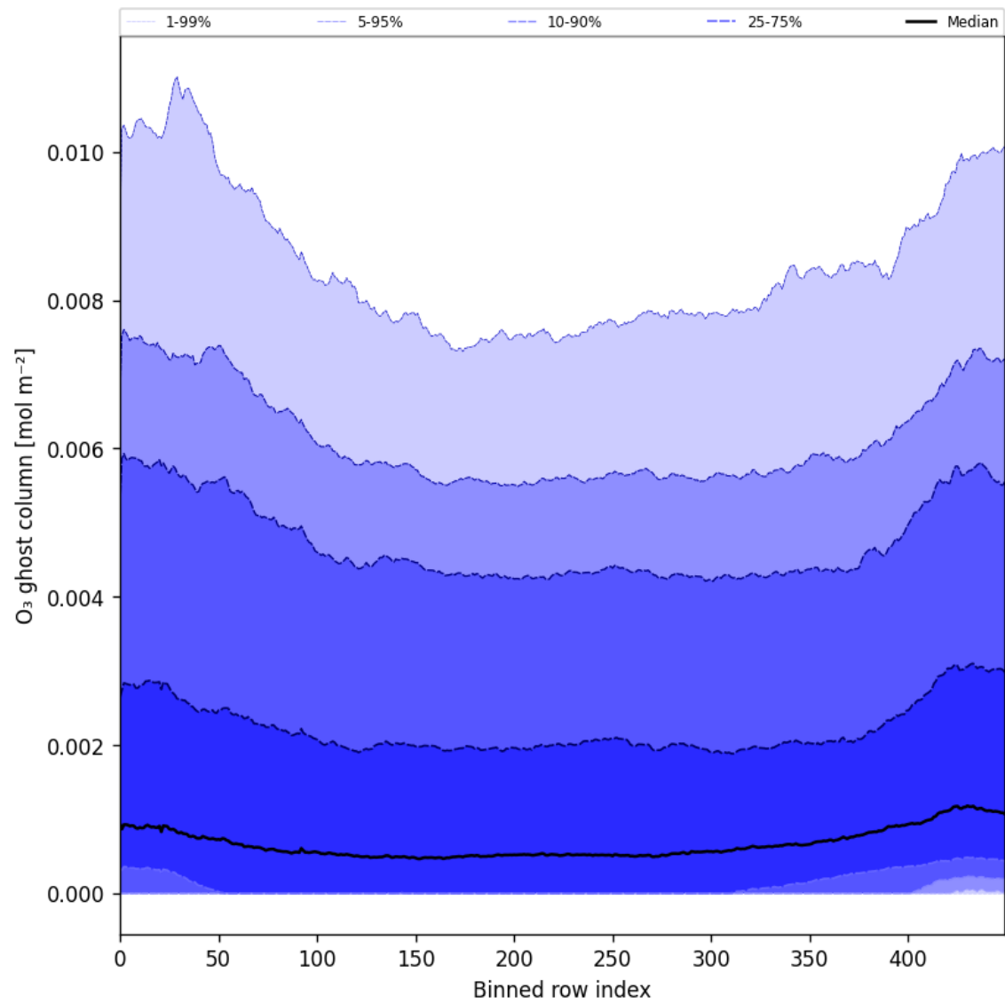
Figure 32: Along track statistics of “O 3 ghost column” for 2025-09-11 to 2025-09-13
