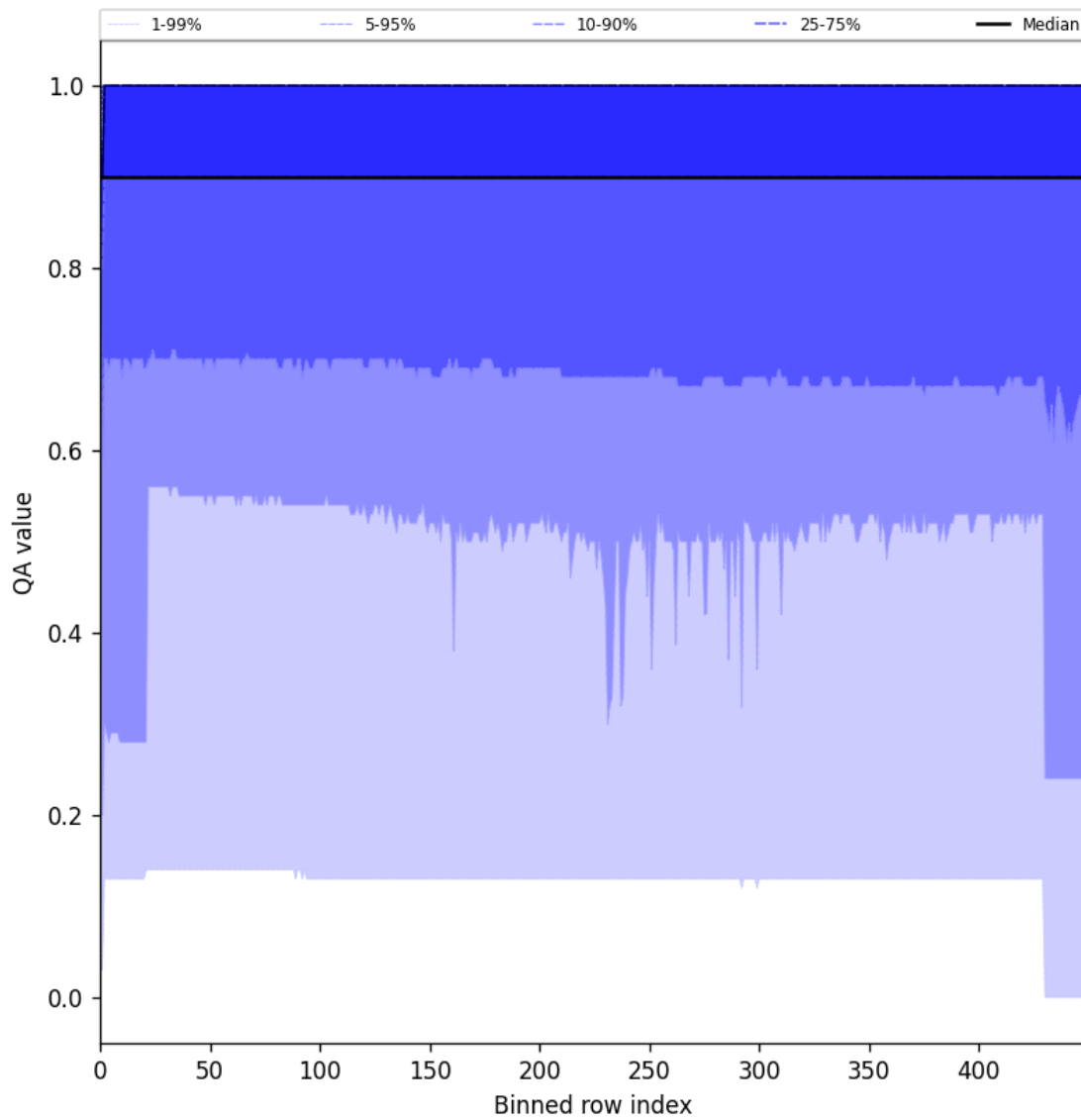
Figure 27: Along track statistics of “QA value” for 2025-09-11 to 2025-09-13
