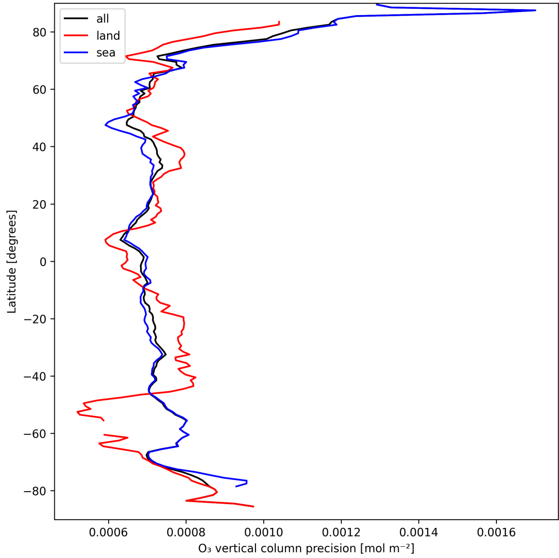
Figure 15: Zonal average of “O 3 vertical column precision” for 2025-09-11 to 2025-09-13.
