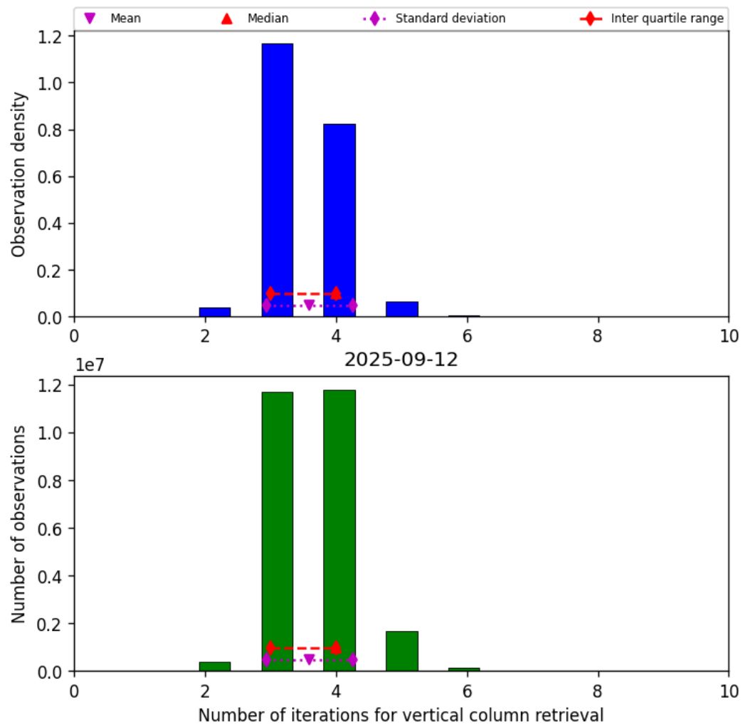
Figure 26: Histogram of “Number of iterations for vertical column retrieval” for 2025-09-11 to 2025-09-13
