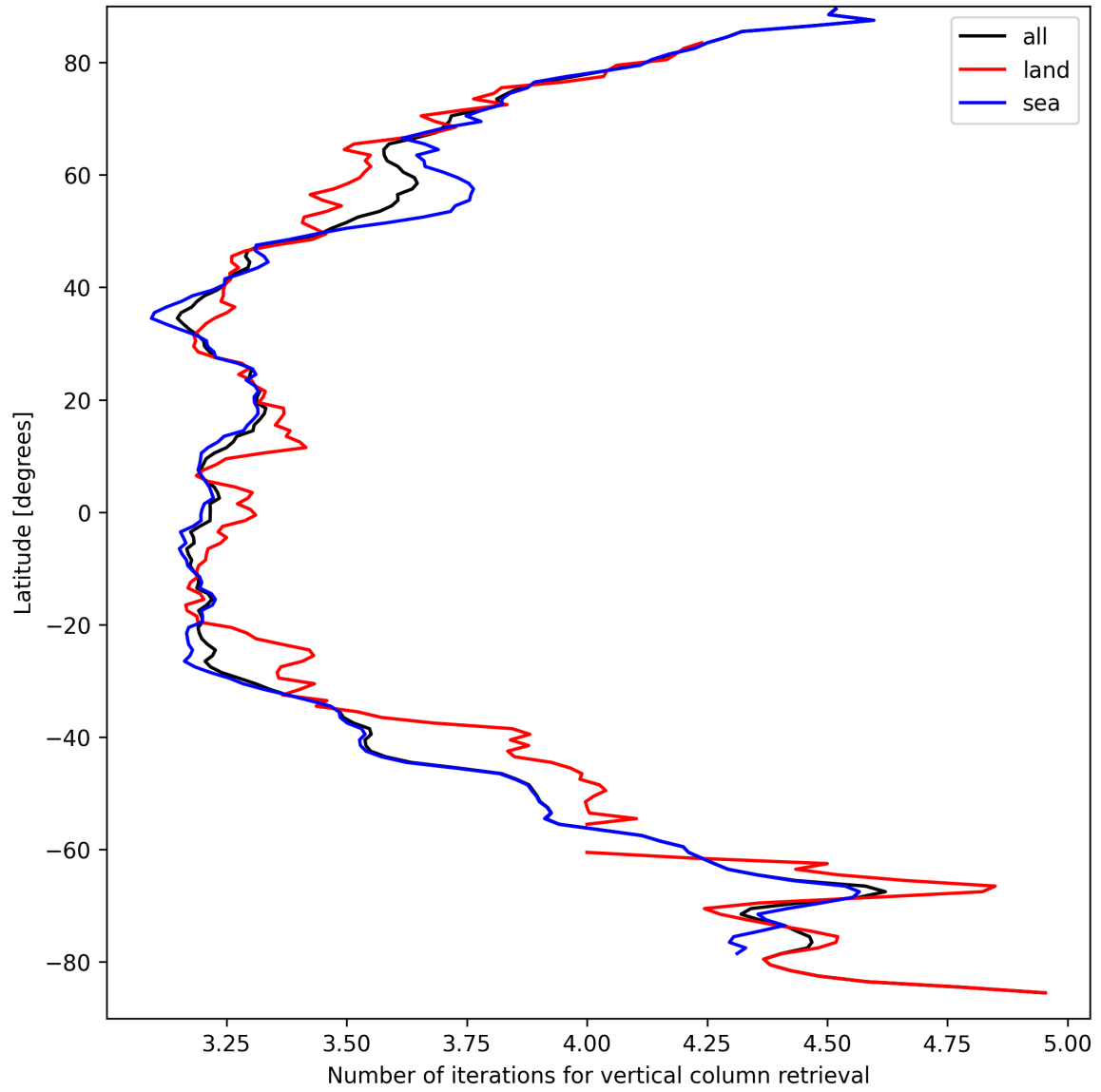
Figure 19: Zonal average of “Number of iterations for vertical column retrieval” for 2025-09-11 to 2025-09-13.
