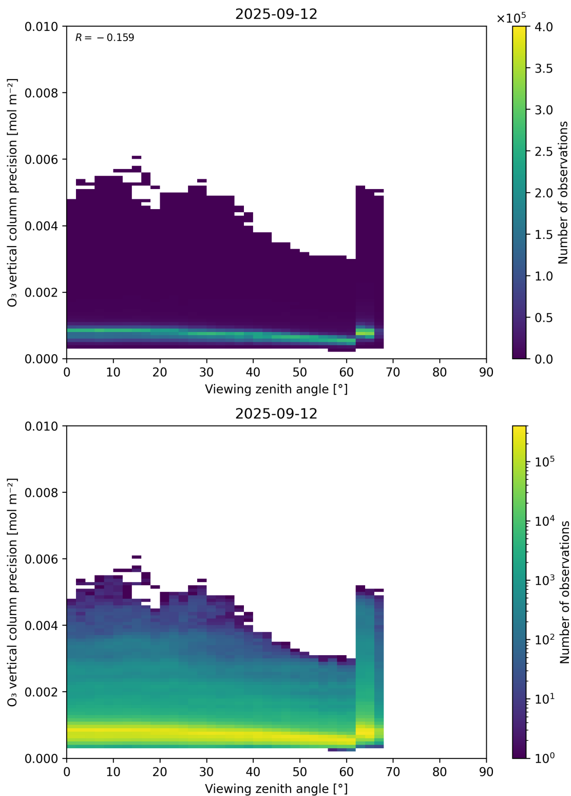
Figure 53: Scatter density plot of “Viewing zenith angle” against “O 3 vertical column precision” for 2025-09-11 to 2025-09-13.
