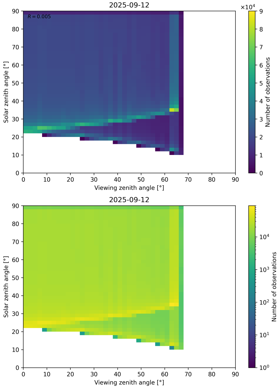
Figure 54: Scatter density plot of “Viewing zenith angle” against “Solar zenith angle” for 2025-09-11 to 2025-09-13.
