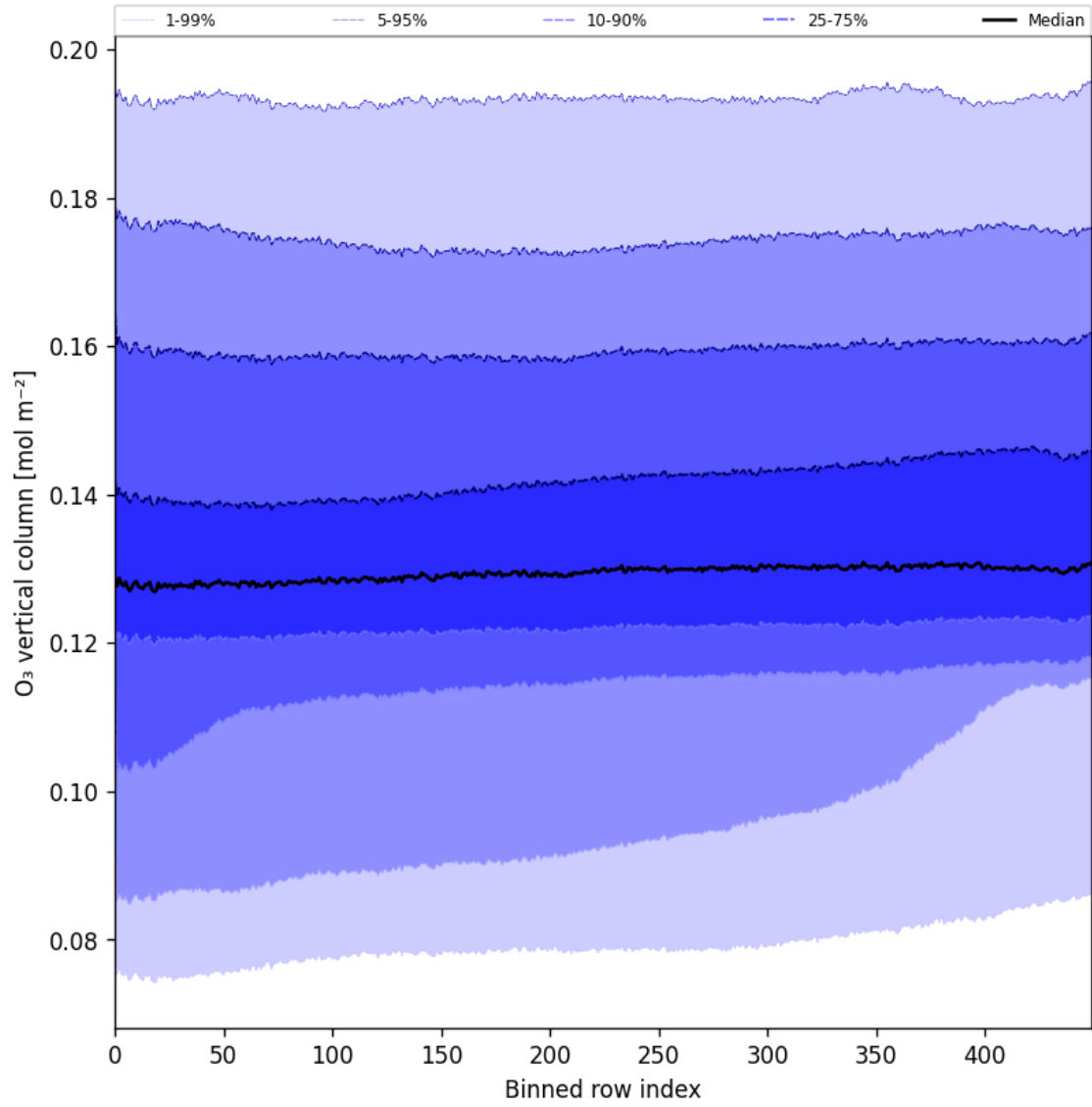
Figure 28: Along track statistics of “O 3 vertical column” for 2025-09-11 to 2025-09-13
