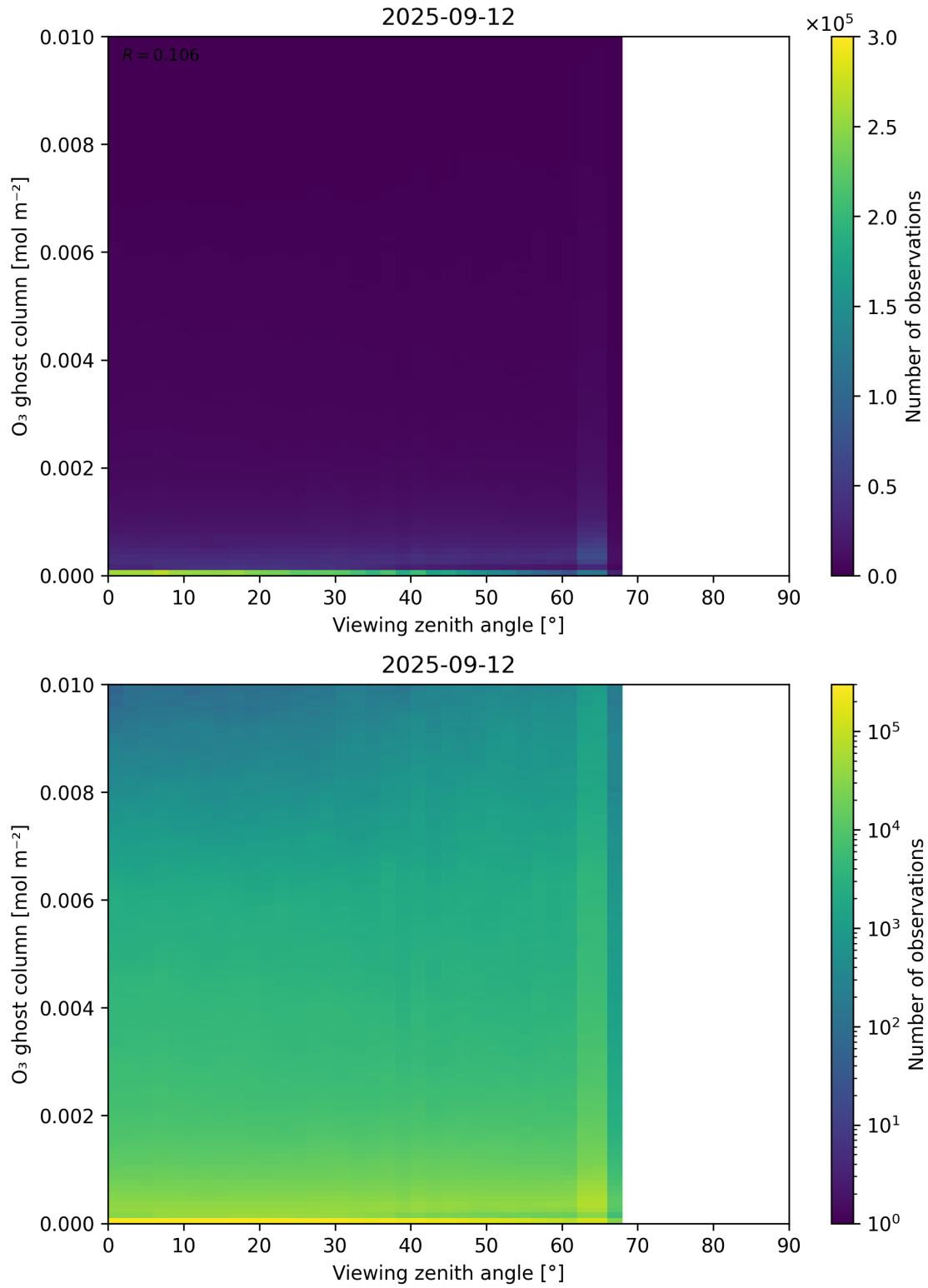
Figure 51: Scatter density plot of “Viewing zenith angle” against “O 3 ghost column” for 2025-09-11 to 2025-09-13.
