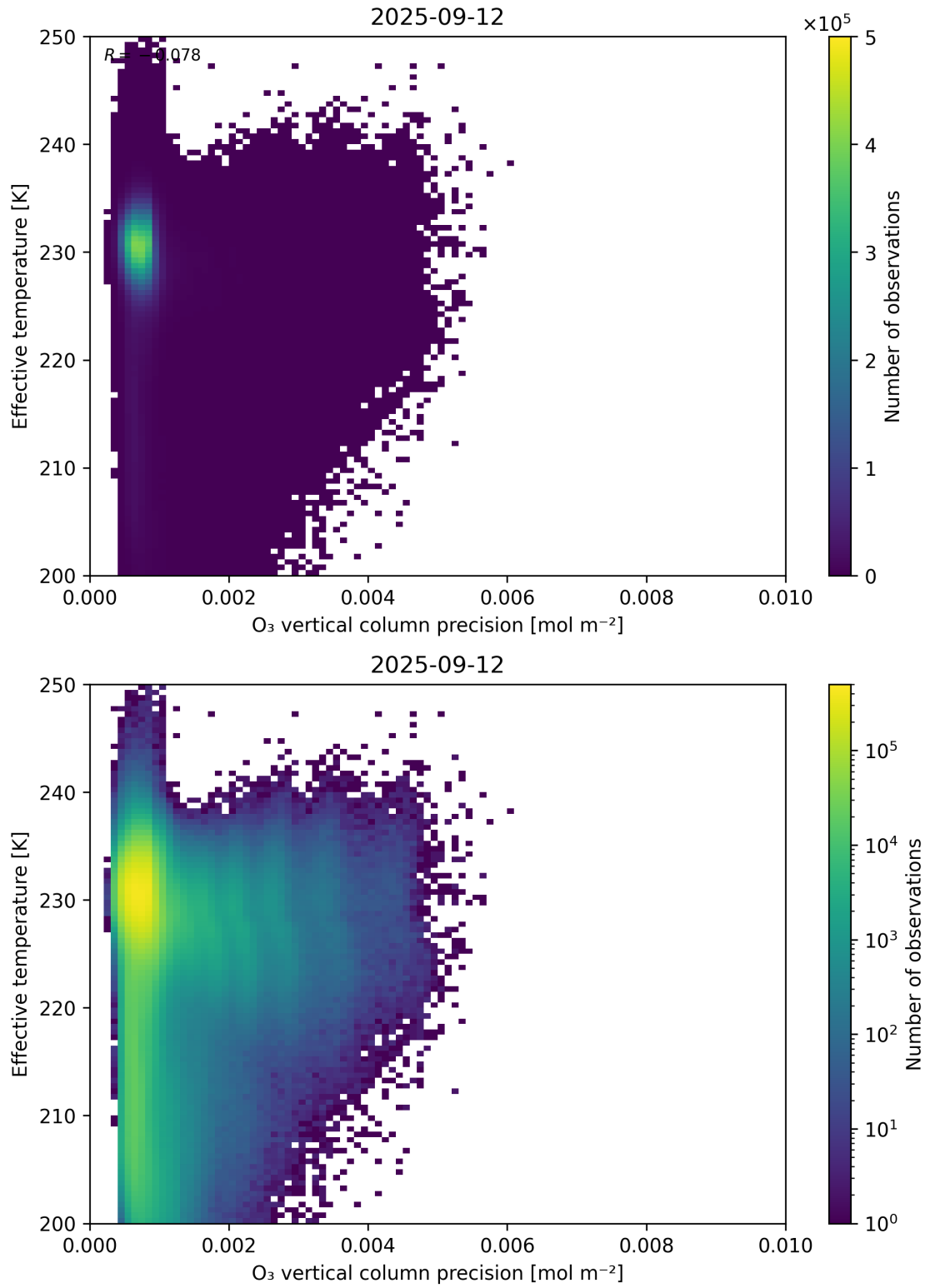
Figure 42: Scatter density plot of “O 3 vertical column precision” against “Effective temperature” for 2025-09-11 to 2025-09-13.
