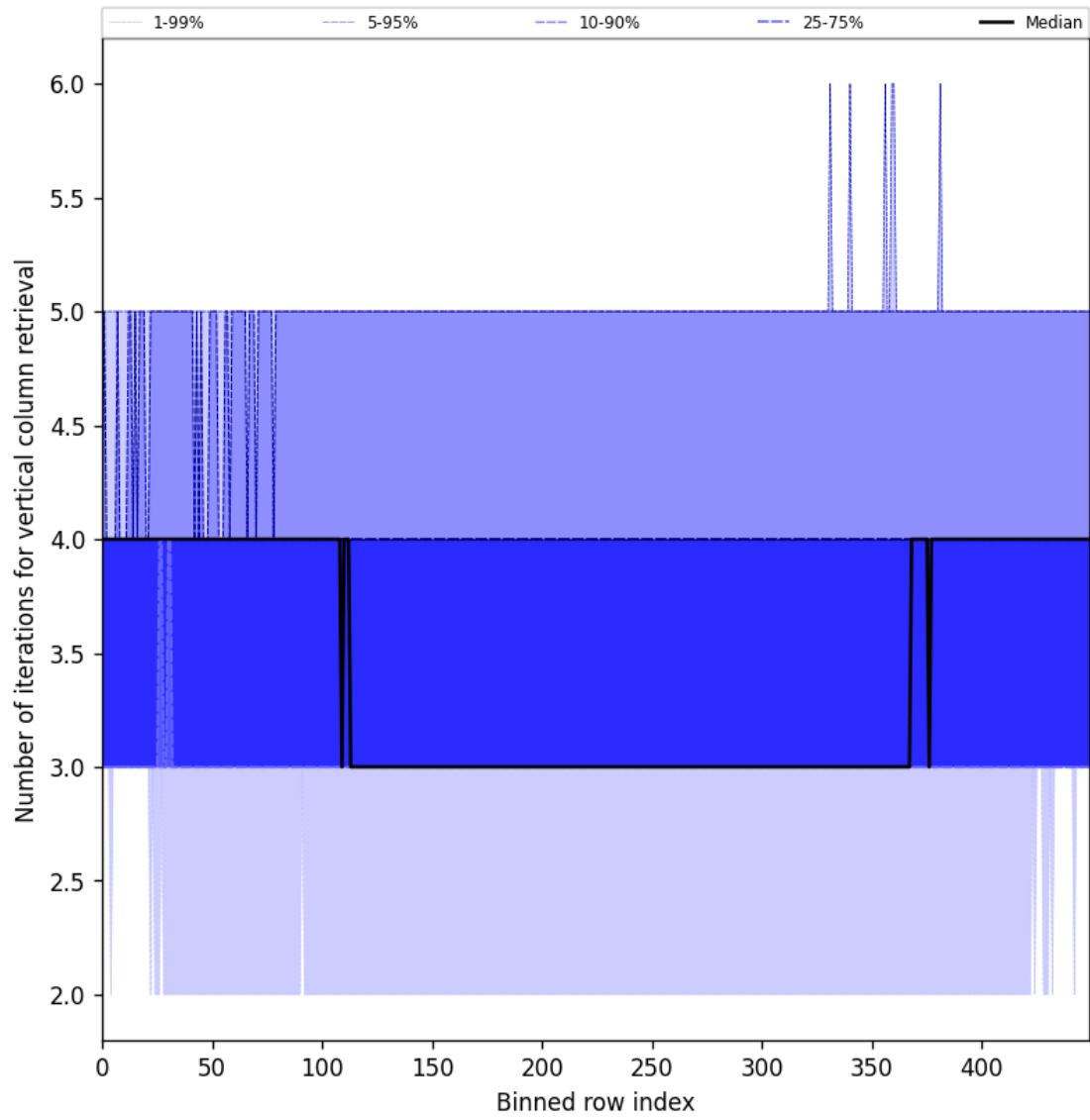
Figure 33: Along track statistics of “Number of iterations for vertical column retrieval” for 2025-09-11 to 2025-09-13
