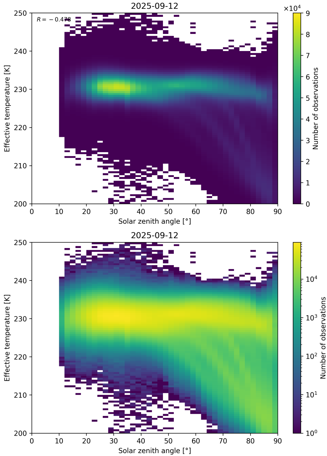
Figure 45: Scatter density plot of “Solar zenith angle” against “Effective temperature” for 2025-09-11 to 2025-09-13.
