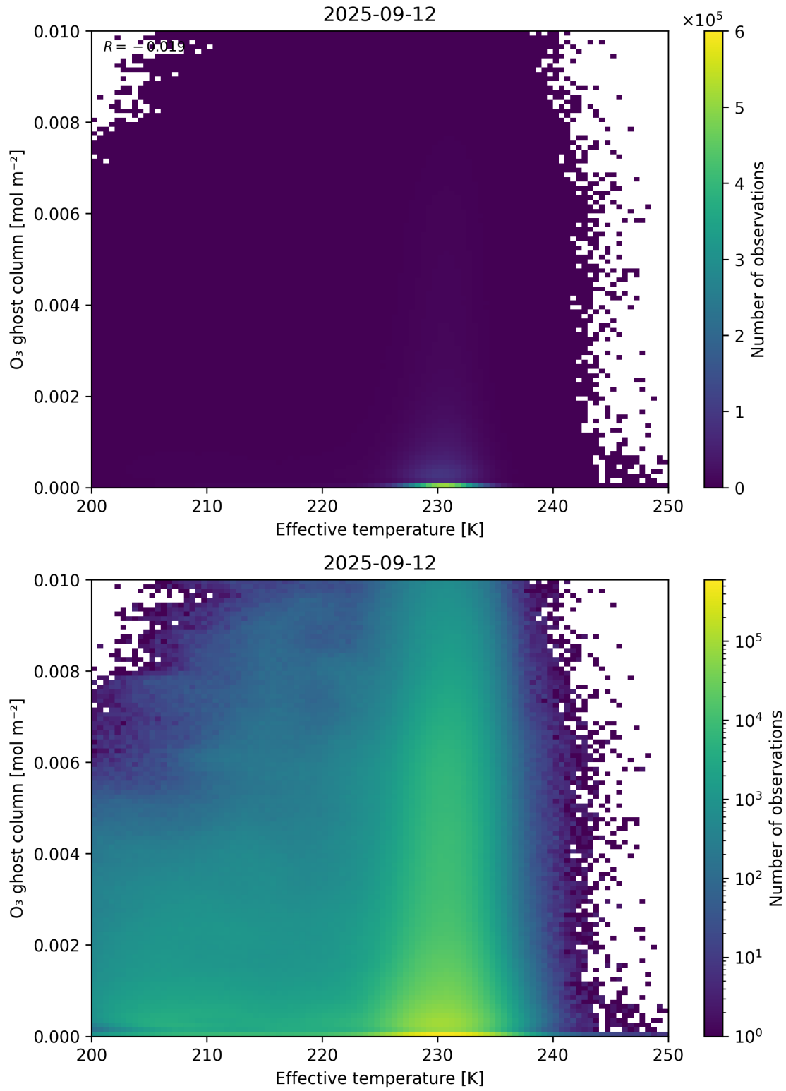
Figure 38: Scatter density plot of “Effective temperature” against “O 3 ghost column” for 2025-09-11 to 2025-09-13.
