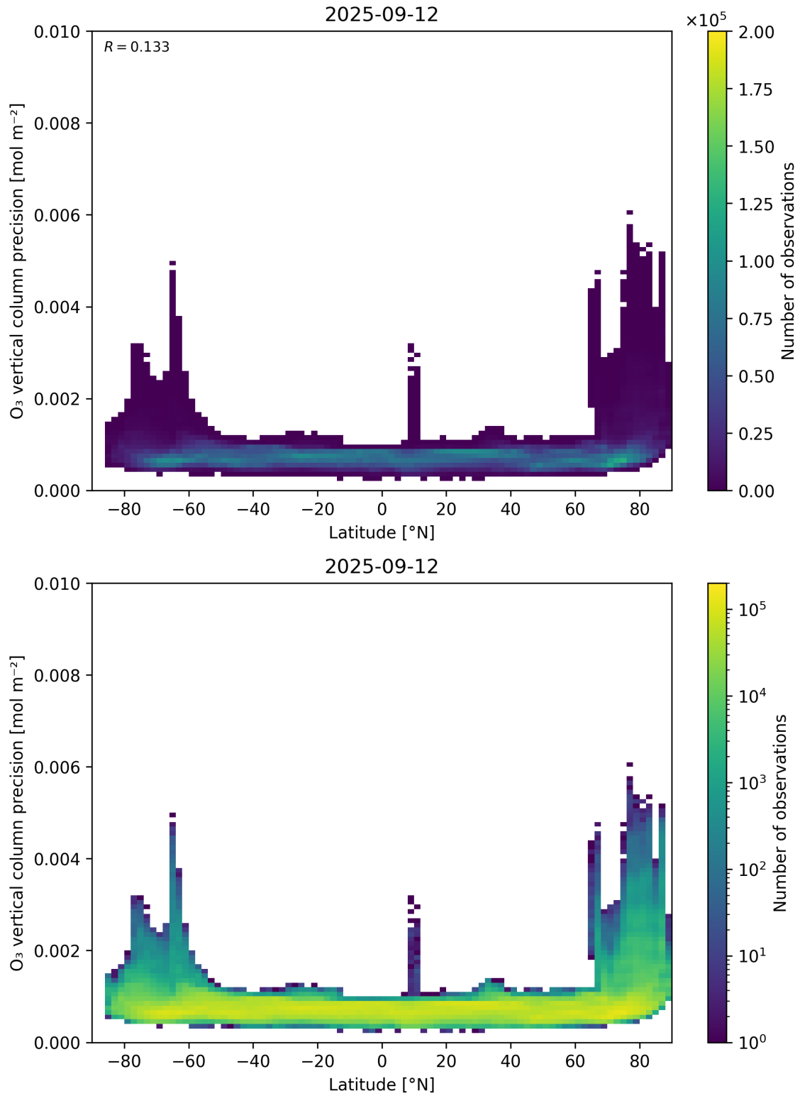
Figure 37: Scatter density plot of “Latitude” against “O 3 vertical column precision” for 2025-09-11 to 2025-09-13.
