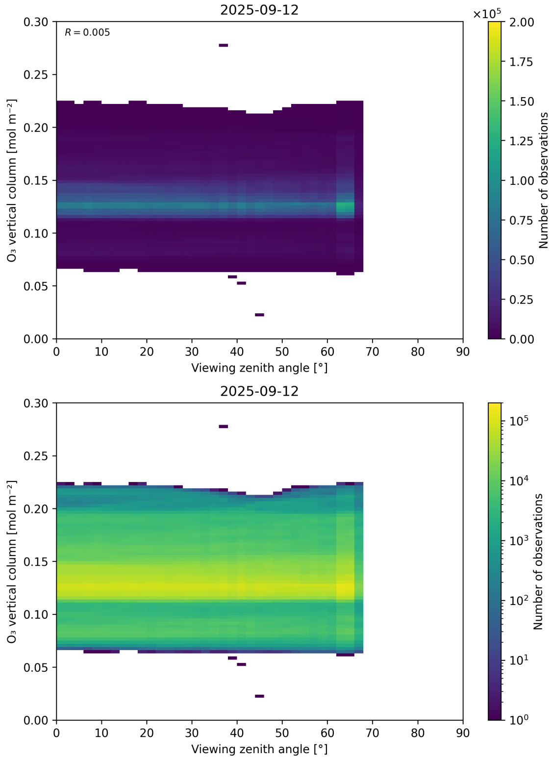
Figure 52: Scatter density plot of “Viewing zenith angle” against “O 3 vertical column” for 2025-09-11 to 2025-09-13.
