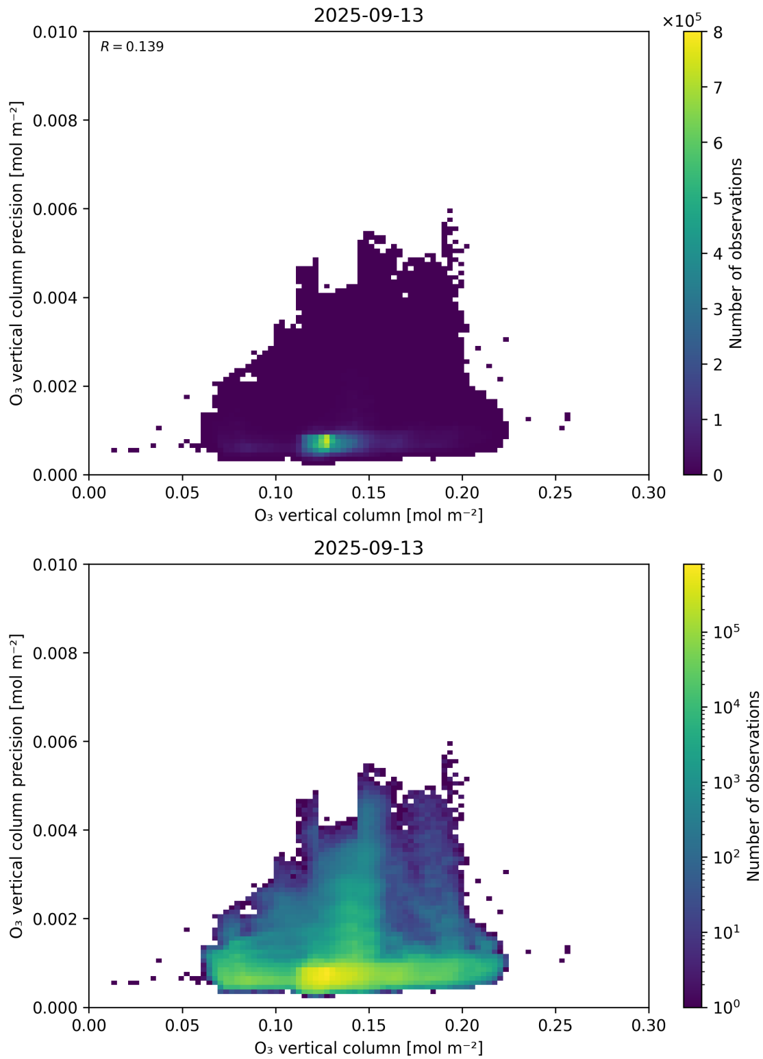
Figure 41: Scatter density plot of “O 3 vertical column” against “O 3 vertical column precision” for 2025-09-12 to 2025-09-14.
