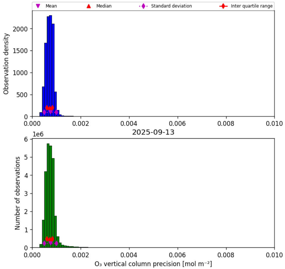
Figure 22: Histogram of “O 3 vertical column precision” for 2025-09-12 to 2025-09-14
