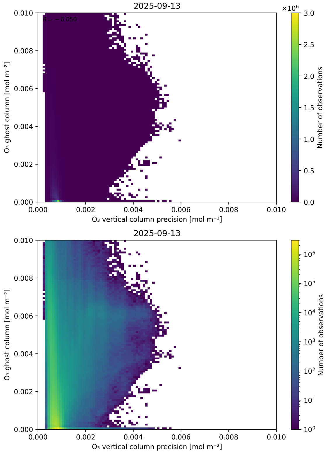
Figure 43: Scatter density plot of “ \text{O}_3 vertical column precision” against “ \text{O}_3 ghost column” for 2025-09-12 to 2025-09-14.
