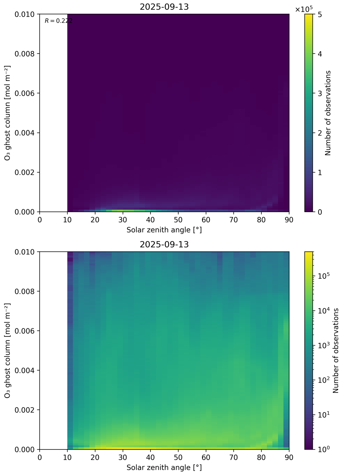
Figure 46: Scatter density plot of “Solar zenith angle” against “O 3 ghost column” for 2025-09-12 to 2025-09-14.
