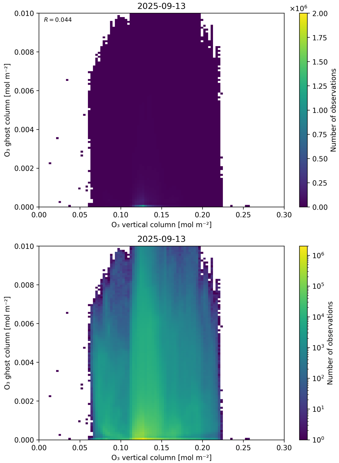
Figure 40: Scatter density plot of “O 3 vertical column” against “O 3 ghost column” for 2025-09-12 to 2025-09-14.
