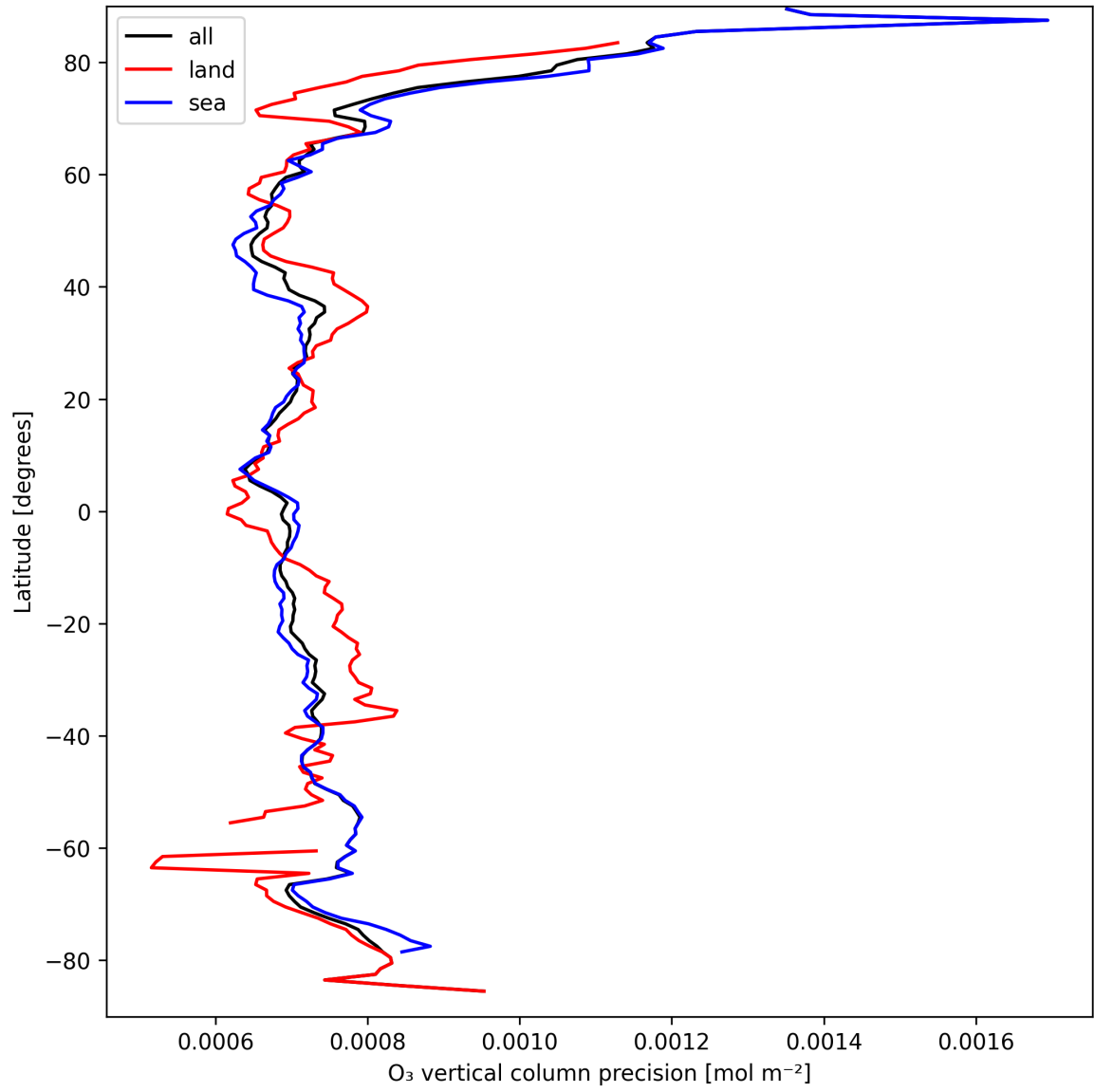
Figure 15: Zonal average of “O 3 vertical column precision” for 2025-09-12 to 2025-09-14.
