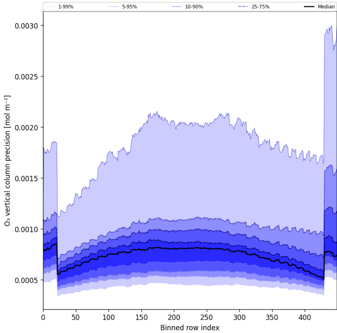
Figure 29: Along track statistics of “O 3 vertical column precision” for 2025-09-12 to 2025-09-14
