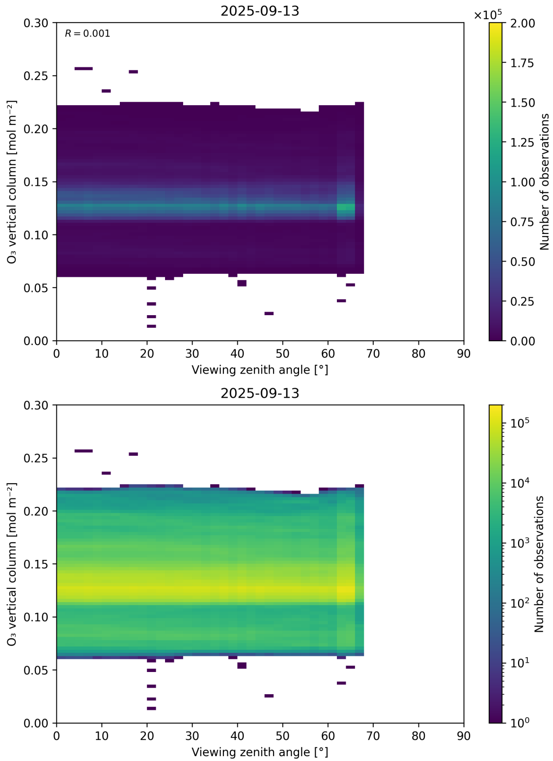
Figure 52: Scatter density plot of “Viewing zenith angle” against “O 3 vertical column” for 2025-09-12 to 2025-09-14.
