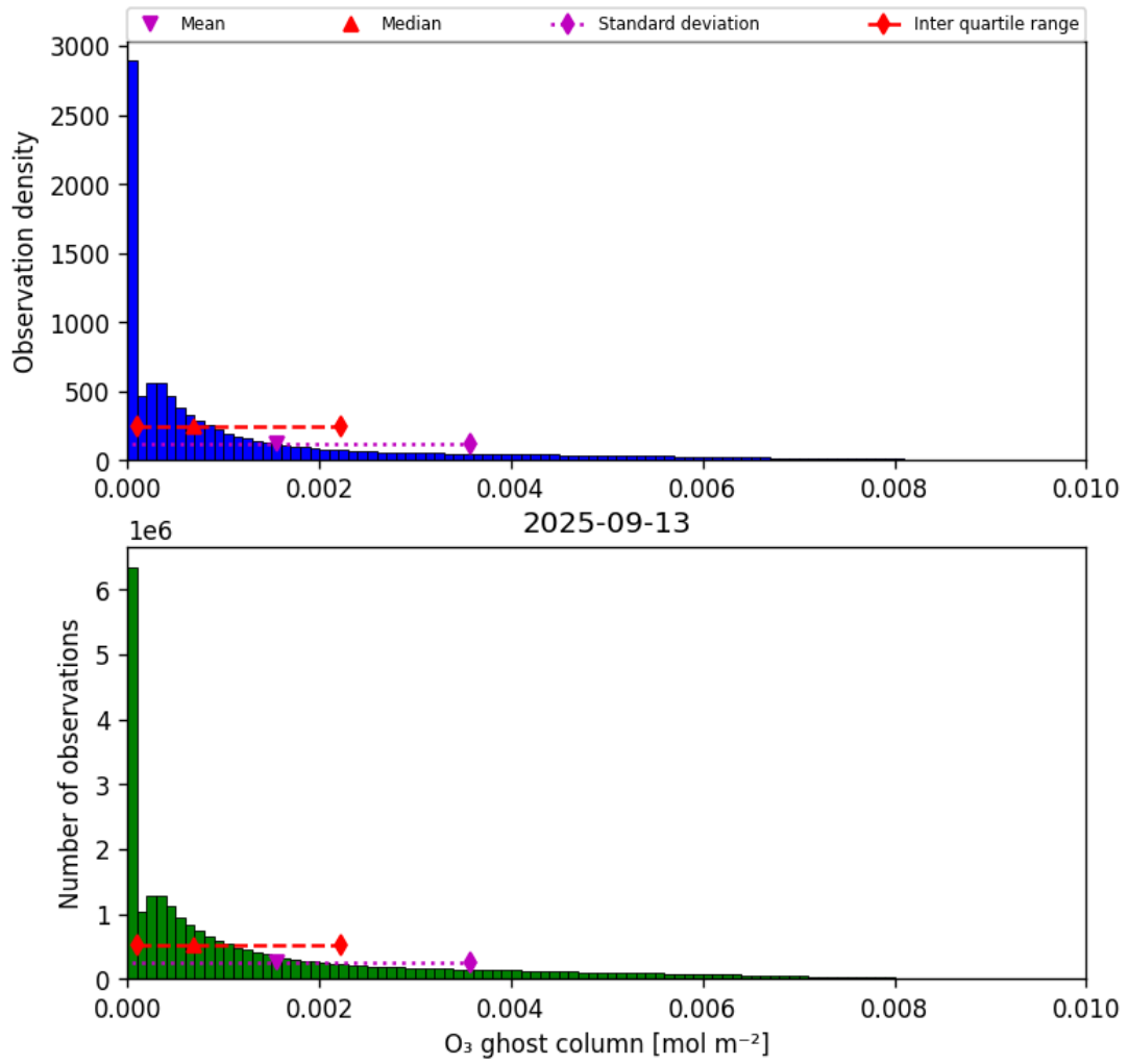
Figure 25: Histogram of “O 3 ghost column” for 2025-09-12 to 2025-09-14
