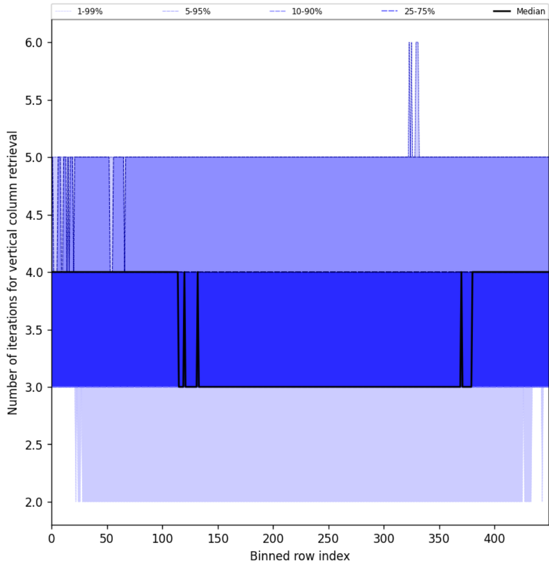
Figure 33: Along track statistics of “Number of iterations for vertical column retrieval” for 2025-09-12 to 2025-09-14
