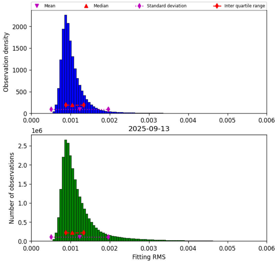
Figure 23: Histogram of “Fitting RMS” for 2025-09-12 to 2025-09-14
