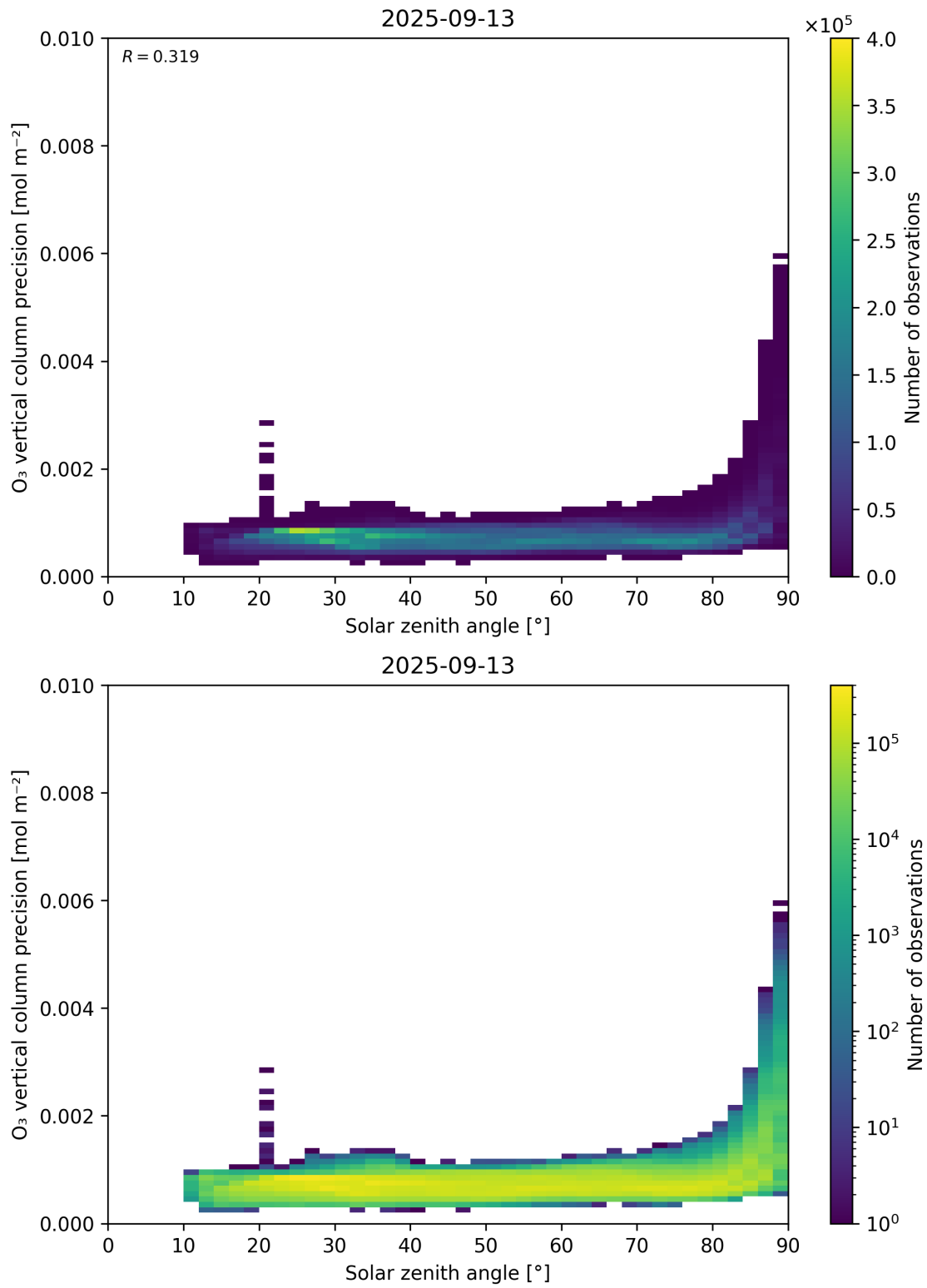
Figure 48: Scatter density plot of “Solar zenith angle” against “O 3 vertical column precision” for 2025-09-12 to 2025-09-14.
