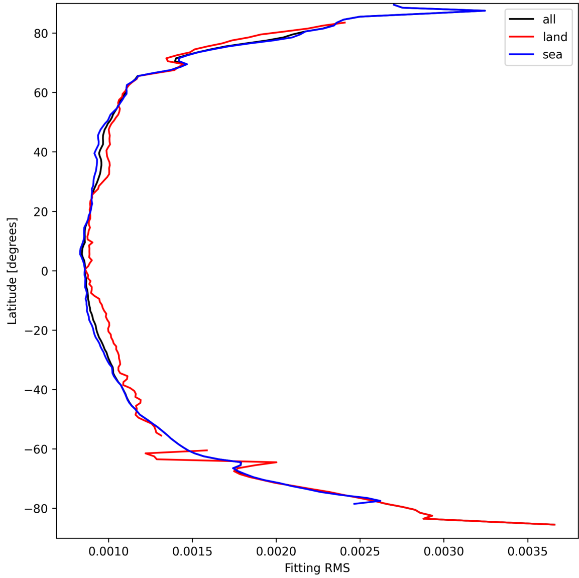
Figure 16: Zonal average of “Fitting RMS” for 2025-09-12 to 2025-09-14.
