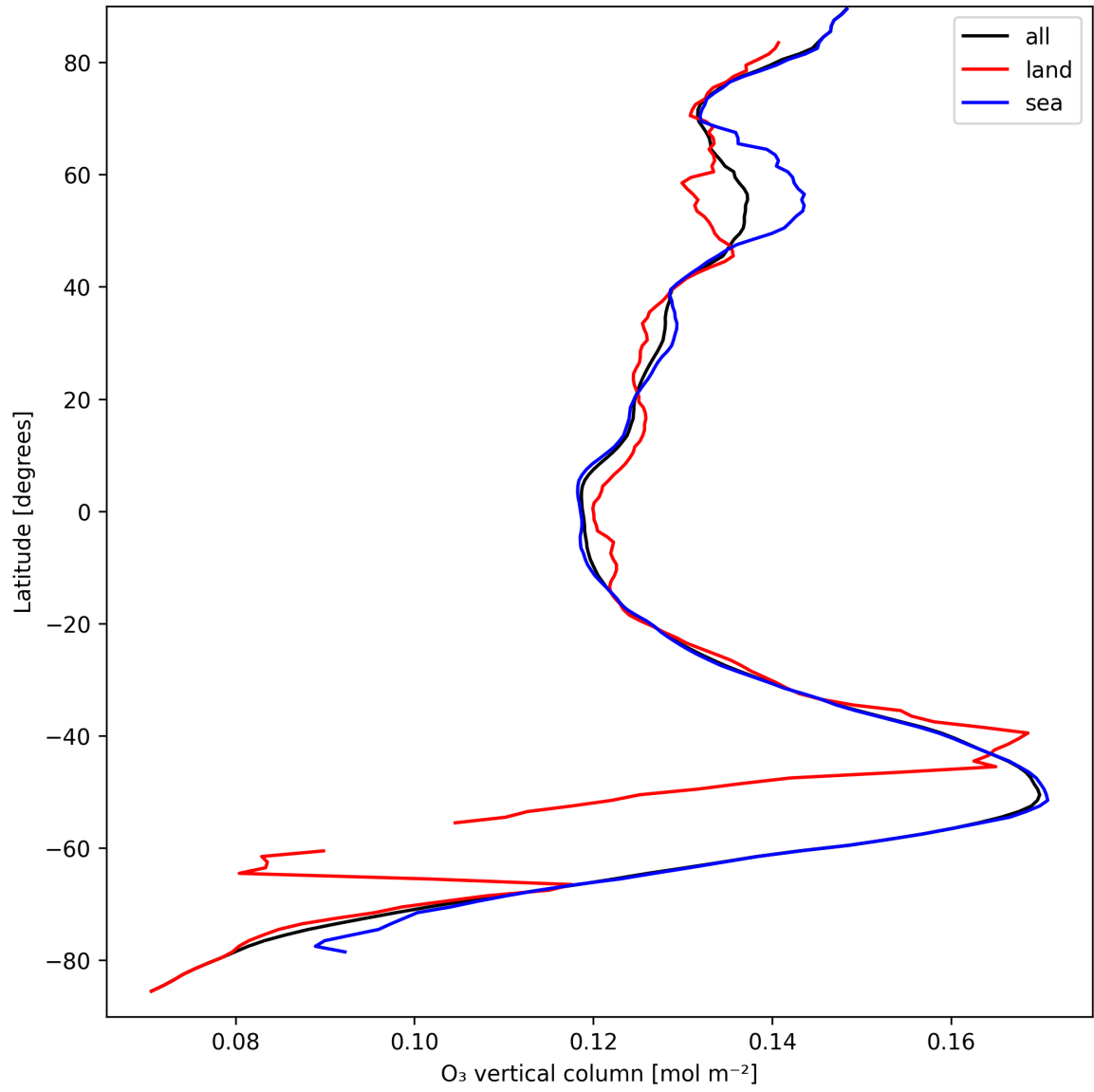
Figure 14: Zonal average of “O 3 vertical column” for 2025-09-12 to 2025-09-14.
