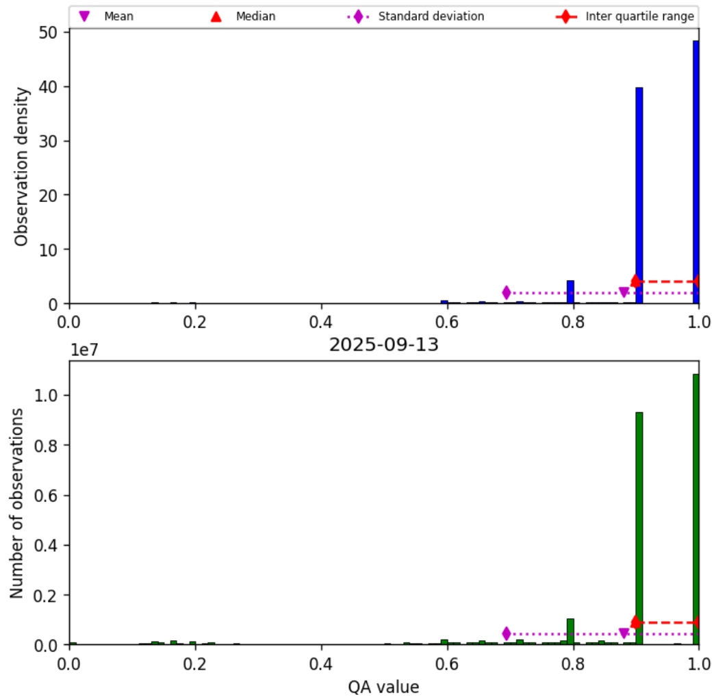
Figure 20: Histogram of “QA value” for 2025-09-12 to 2025-09-14
