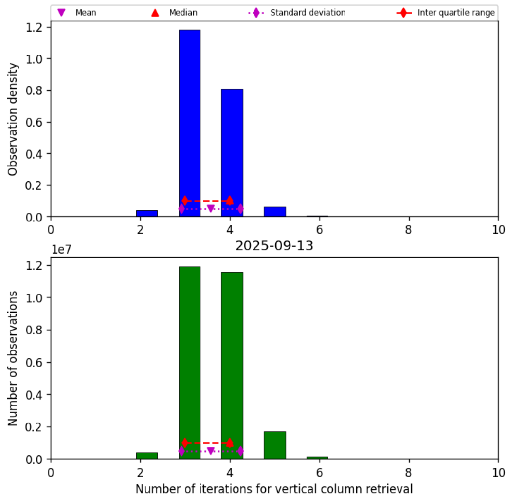
Figure 26: Histogram of “Number of iterations for vertical column retrieval” for 2025-09-12 to 2025-09-14
