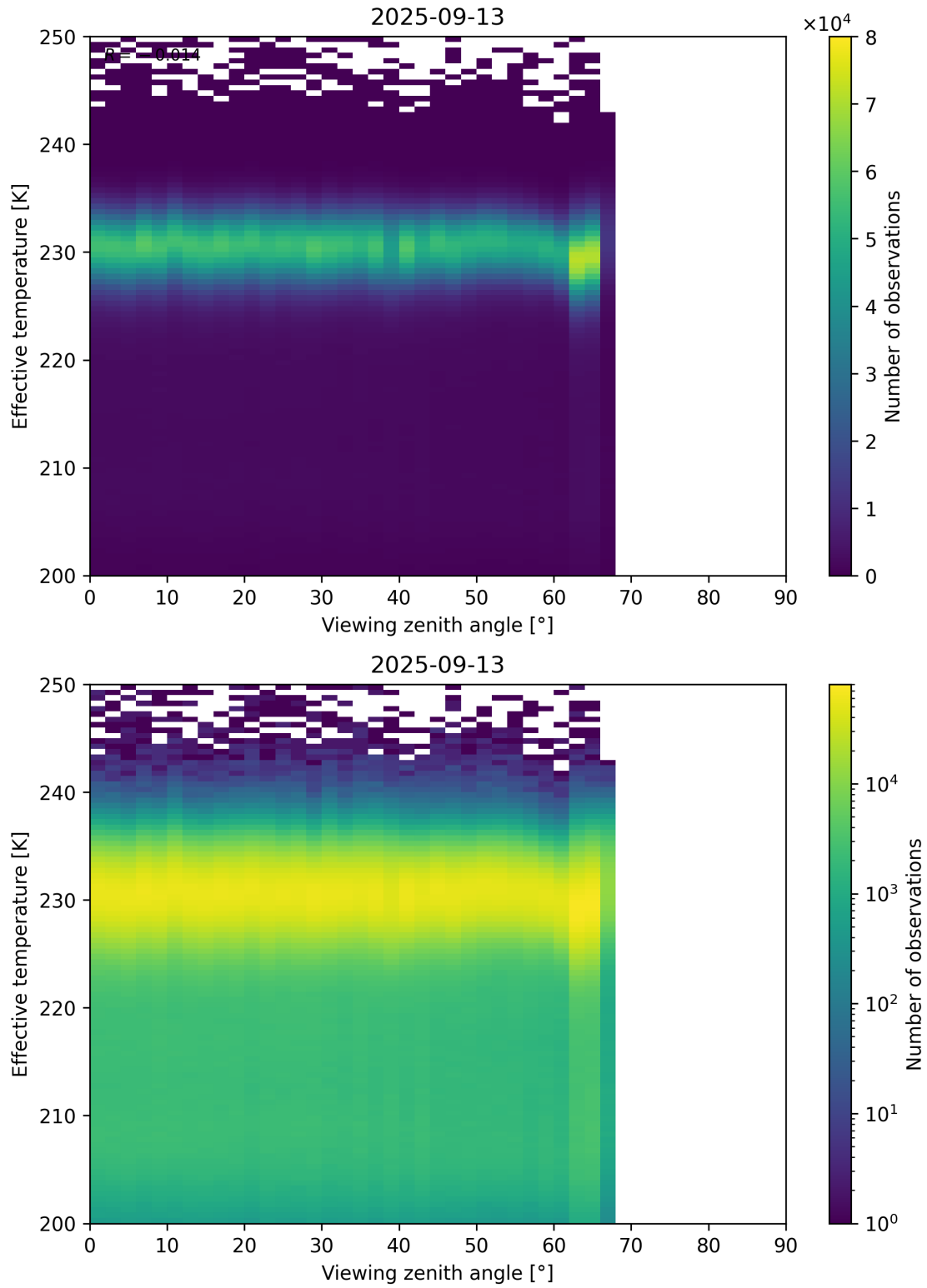
Figure 50: Scatter density plot of “Viewing zenith angle” against “Effective temperature” for 2025-09-12 to 2025-09-14.
