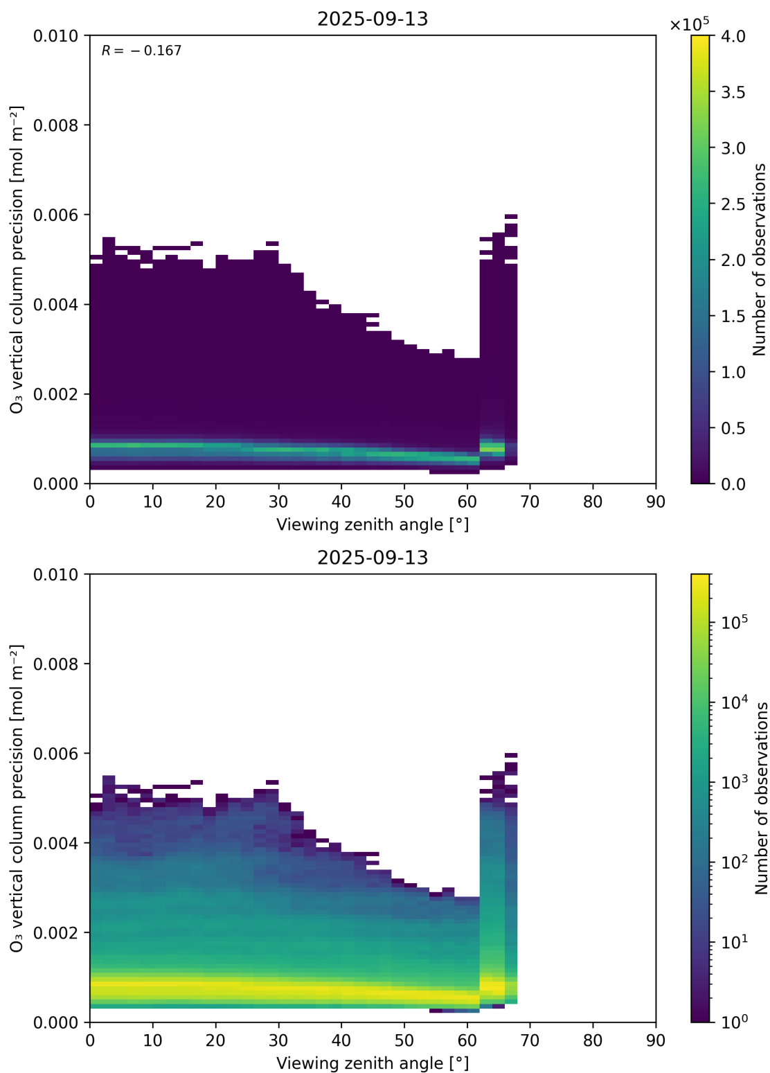
Figure 53: Scatter density plot of “Viewing zenith angle” against “O 3 vertical column precision” for 2025-09-12 to 2025-09-14.
