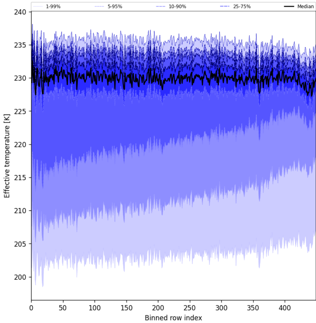
Figure 31: Along track statistics of “Effective temperature” for 2025-09-12 to 2025-09-14
