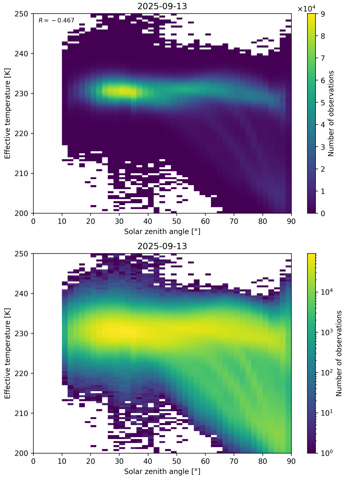
Figure 45: Scatter density plot of “Solar zenith angle” against “Effective temperature” for 2025-09-12 to 2025-09-14.
