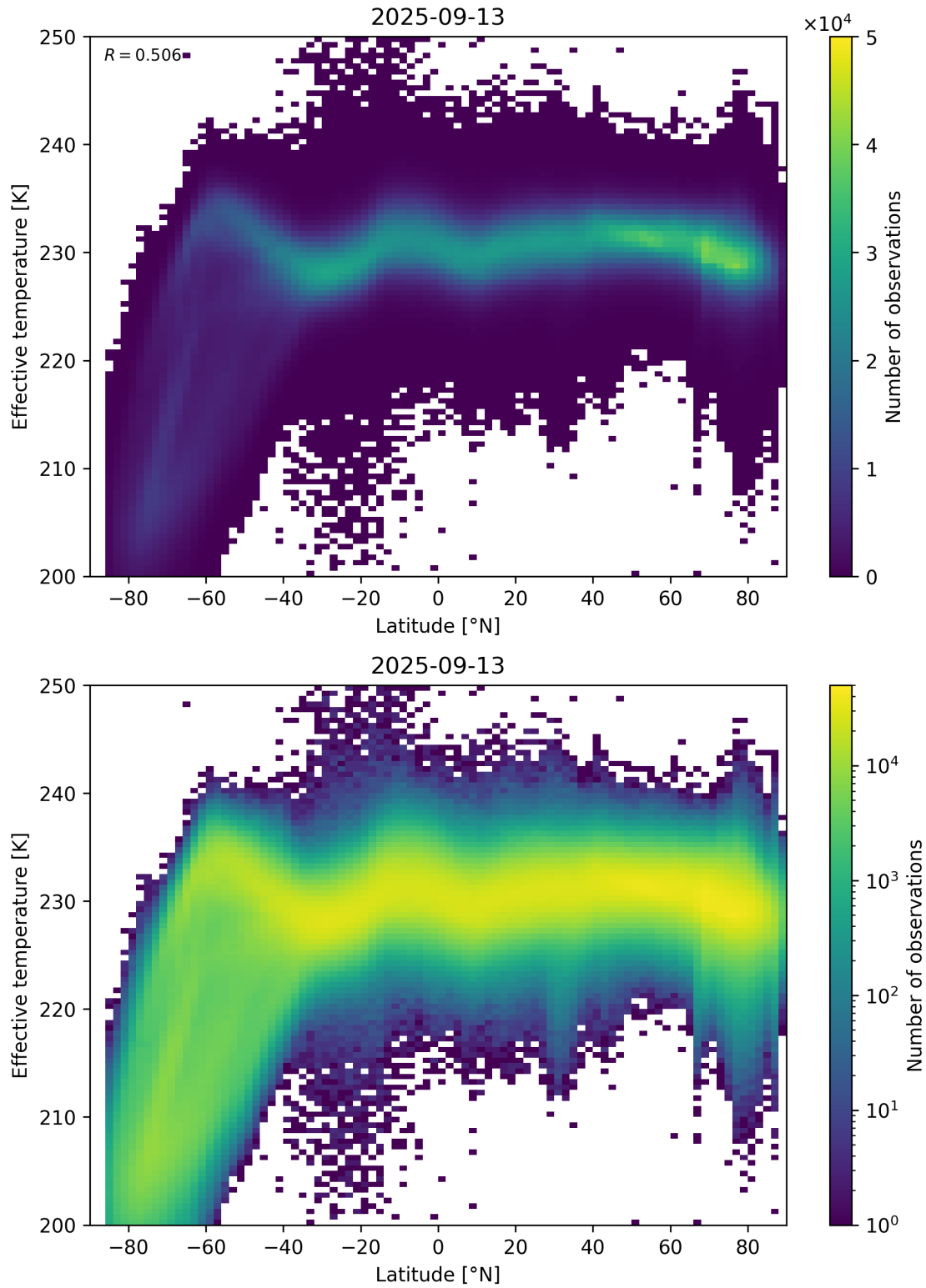
Figure 34: Scatter density plot of “Latitude” against “Effective temperature” for 2025-09-12 to 2025-09-14.
