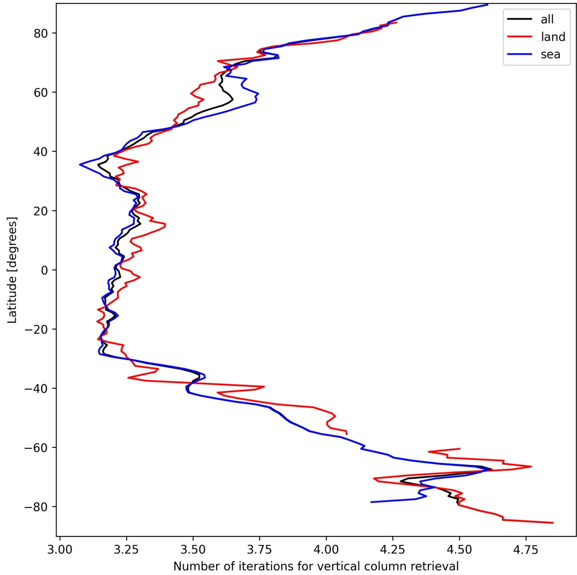
Figure 19: Zonal average of “Number of iterations for vertical column retrieval” for 2025-09-12 to 2025-09-14.
