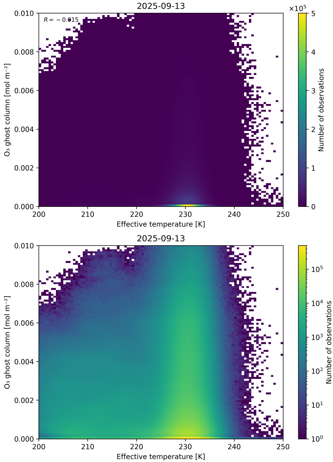
Figure 38: Scatter density plot of “Effective temperature” against “O 3 ghost column” for 2025-09-12 to 2025-09-14.
