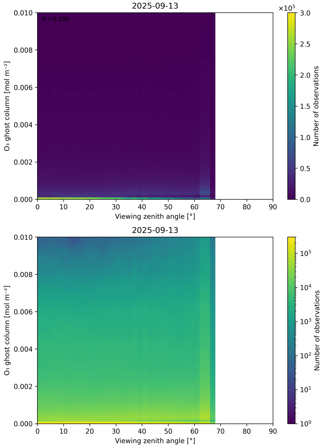
Figure 51: Scatter density plot of “Viewing zenith angle” against “O 3 ghost column” for 2025-09-12 to 2025-09-14.
