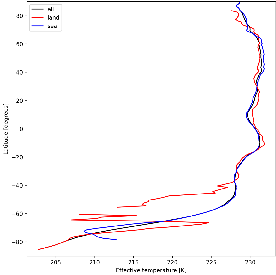
Figure 17: Zonal average of "Effective temperature" for 2025-09-12 to 2025-09-14.
