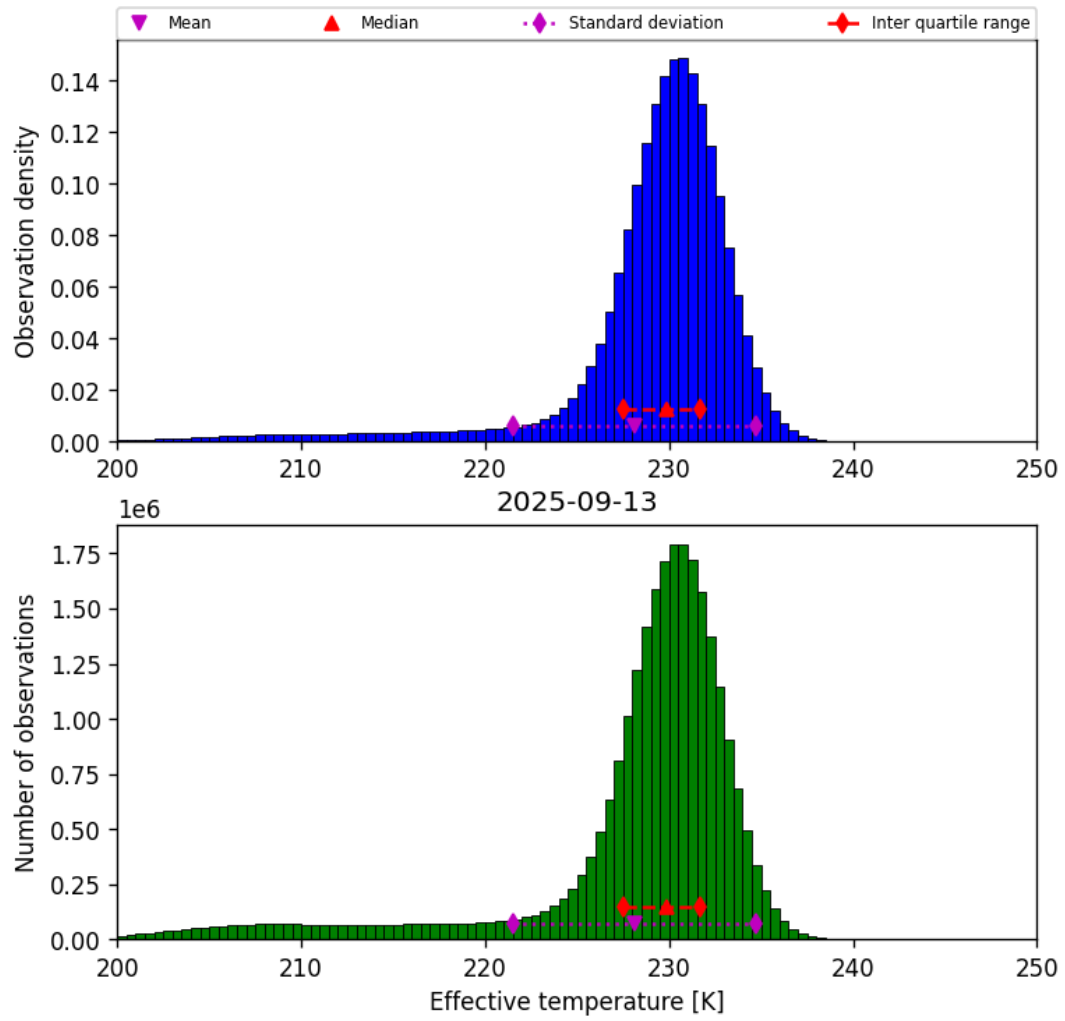
Figure 24: Histogram of “Effective temperature” for 2025-09-12 to 2025-09-14
