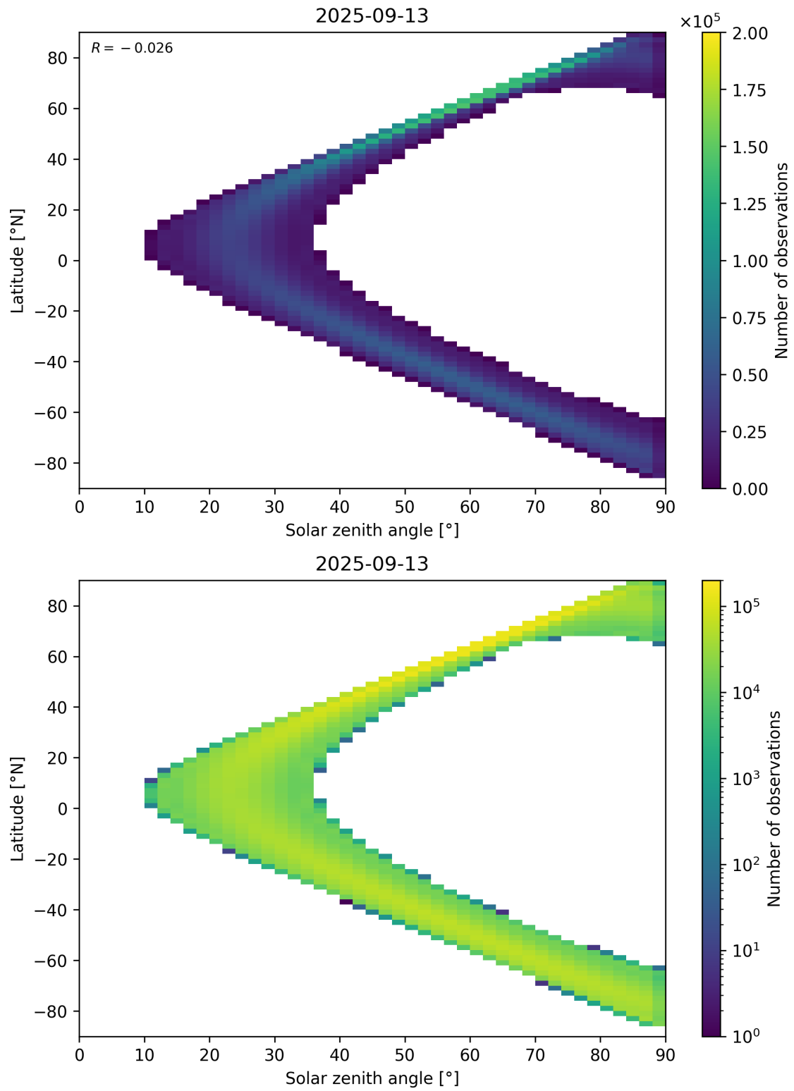
Figure 44: Scatter density plot of “Solar zenith angle” against “Latitude” for 2025-09-12 to 2025-09-14.
