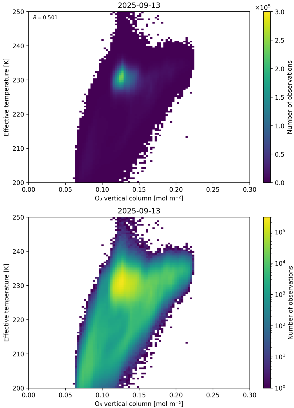
Figure 39: Scatter density plot of “O 3 vertical column” against “Effective temperature” for 2025-09-12 to 2025-09-14.
