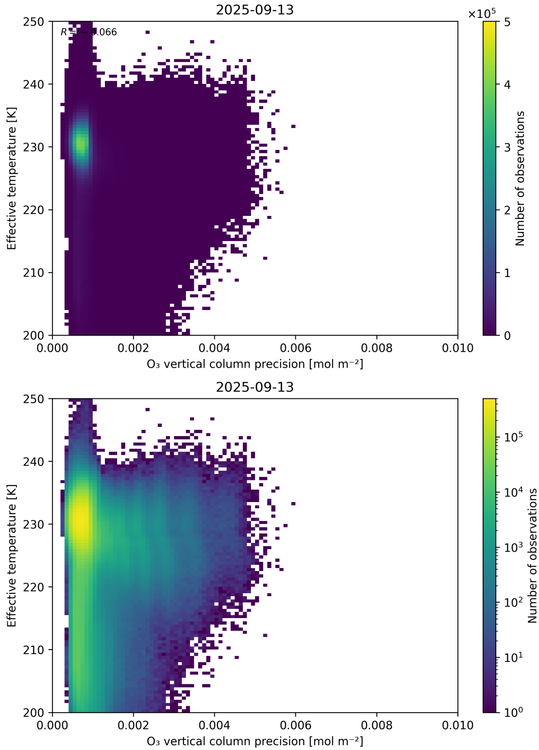
Figure 42: Scatter density plot of “O 3 vertical column precision” against “Effective temperature” for 2025-09-12 to 2025-09-14.
