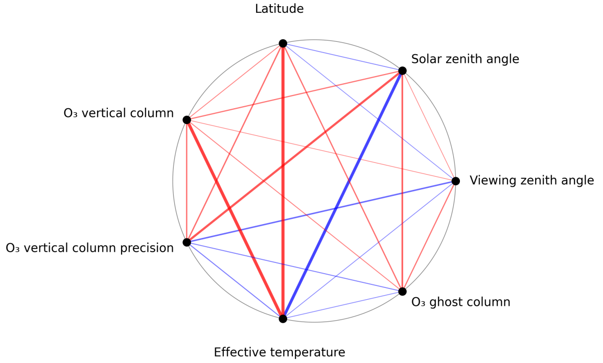
Figure 1: Map of correlation graph for 2025-09-12 to 2025-09-14.
