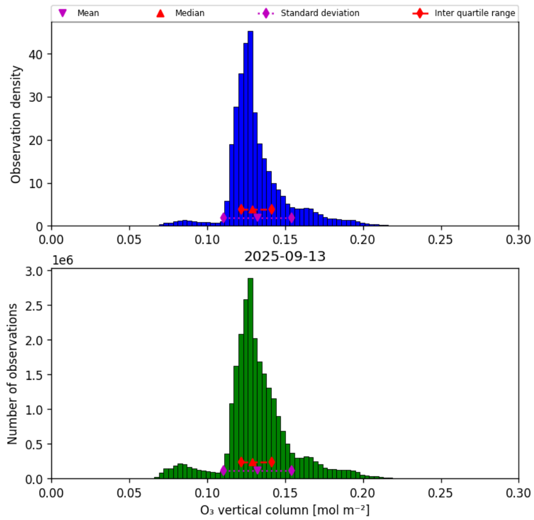
Figure 21: Histogram of “O 3 vertical column” for 2025-09-12 to 2025-09-14
