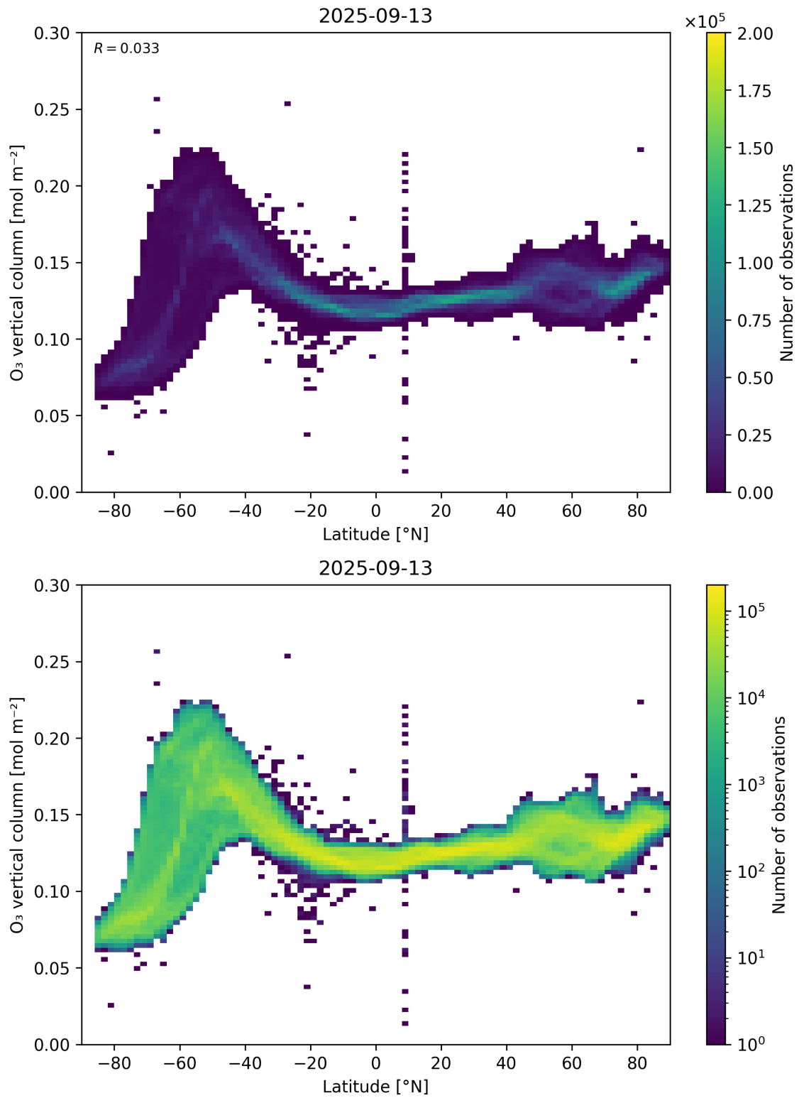
Figure 36: Scatter density plot of “Latitude” against “O 3 vertical column” for 2025-09-12 to 2025-09-14.
