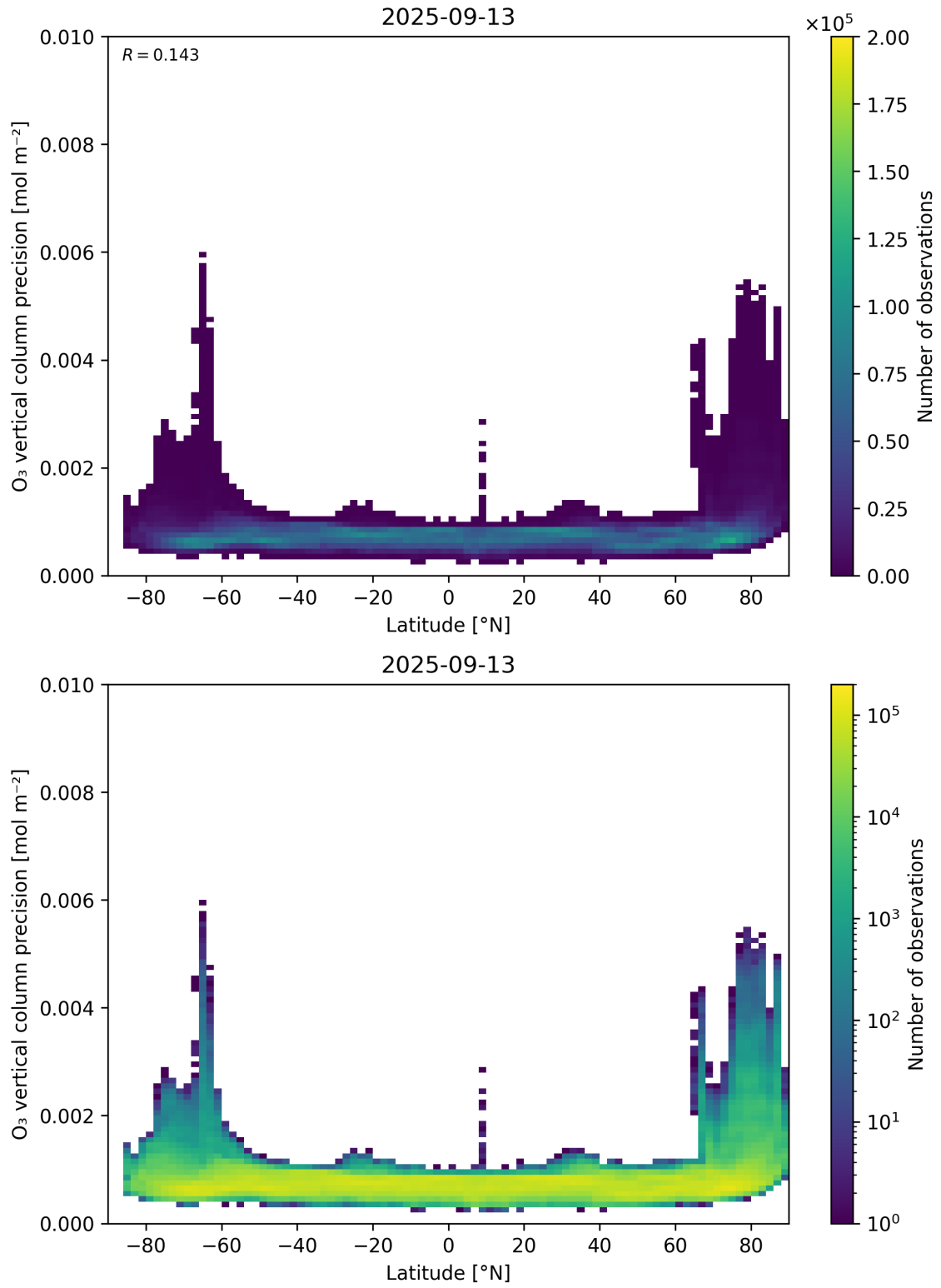
Figure 37: Scatter density plot of “Latitude” against “O 3 vertical column precision” for 2025-09-12 to 2025-09-14.
