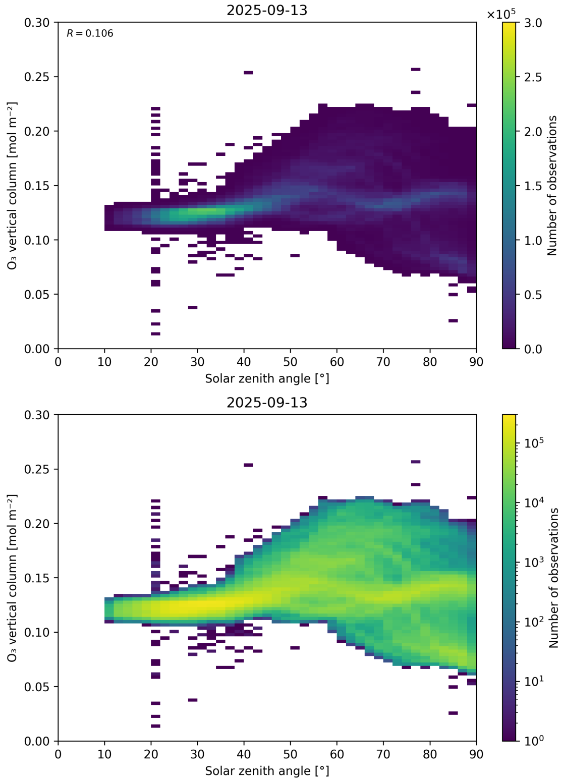
Figure 47: Scatter density plot of “Solar zenith angle” against “O 3 vertical column” for 2025-09-12 to 2025-09-14.
