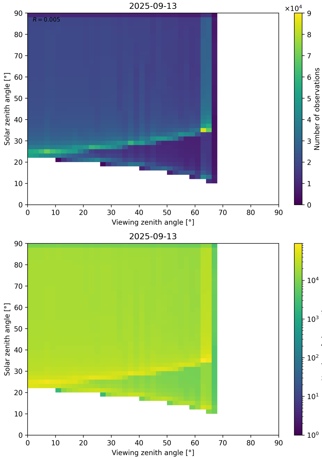
Figure 54: Scatter density plot of “Viewing zenith angle” against “Solar zenith angle” for 2025-09-12 to 2025-09-14.
