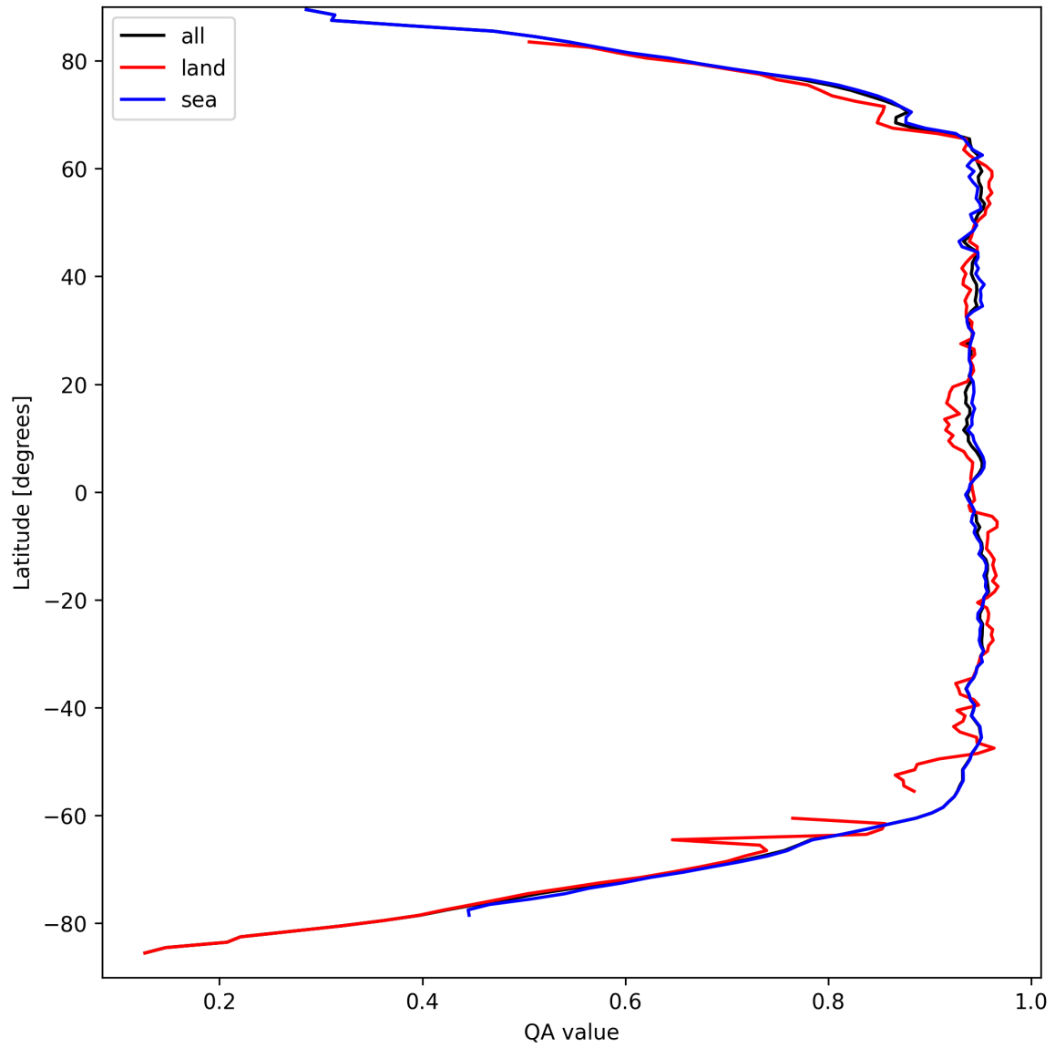
Figure 13: Zonal average of “QA value” for 2025-09-12 to 2025-09-14.
