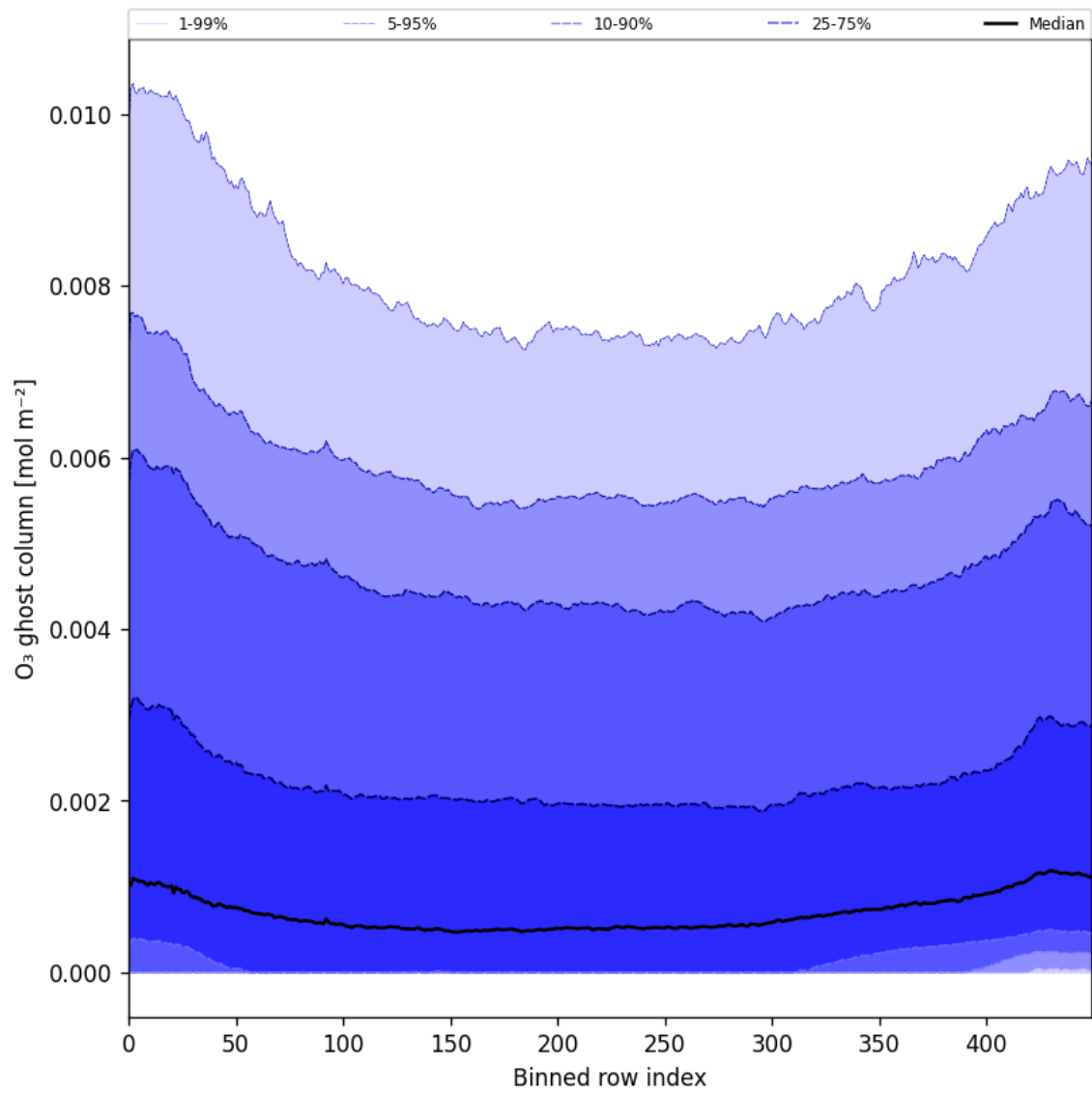
Figure 32: Along track statistics of “O 3 ghost column” for 2025-09-12 to 2025-09-14
