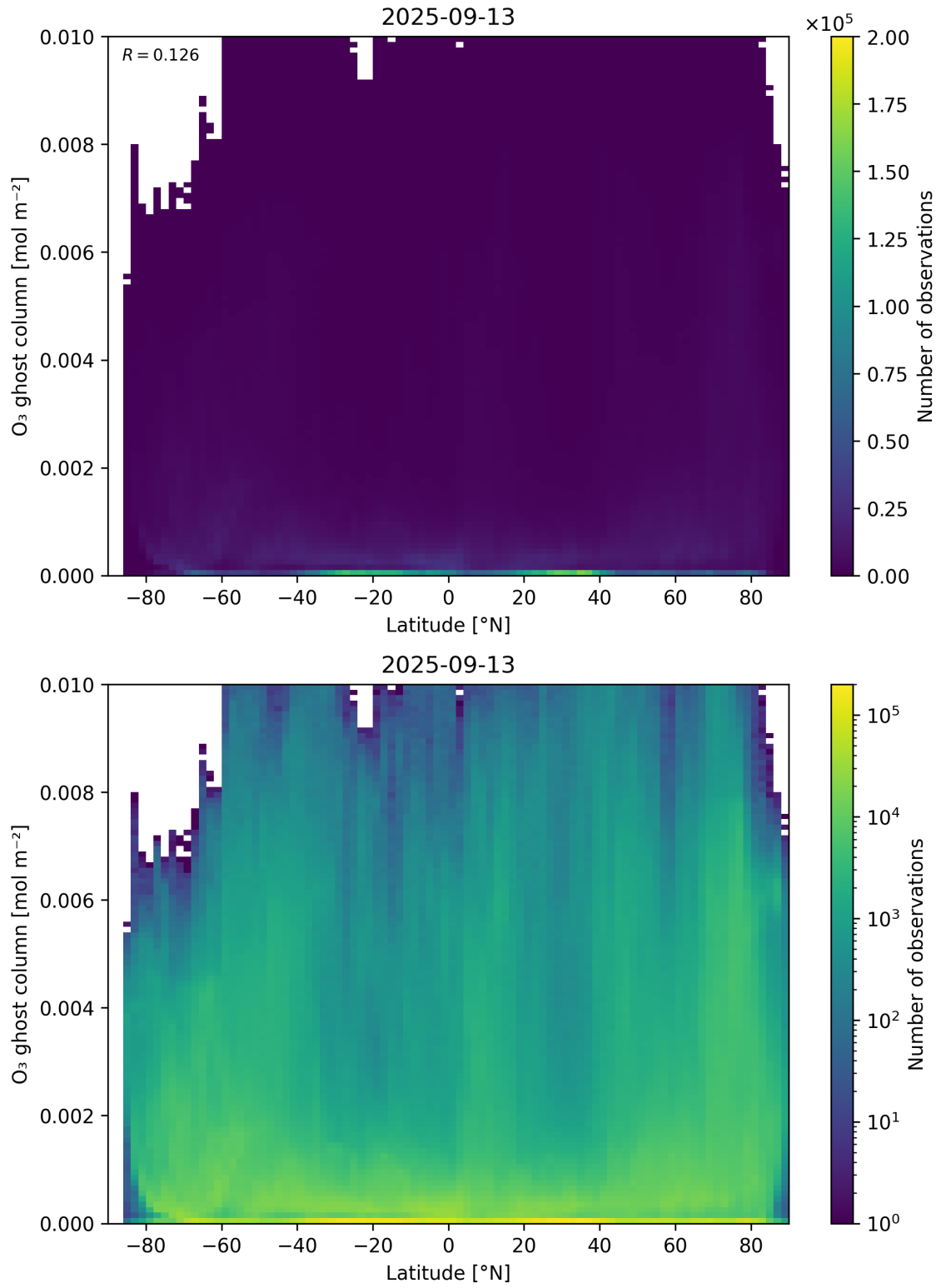
Figure 35: Scatter density plot of “Latitude” against “O 3 ghost column” for 2025-09-12 to 2025-09-14.
