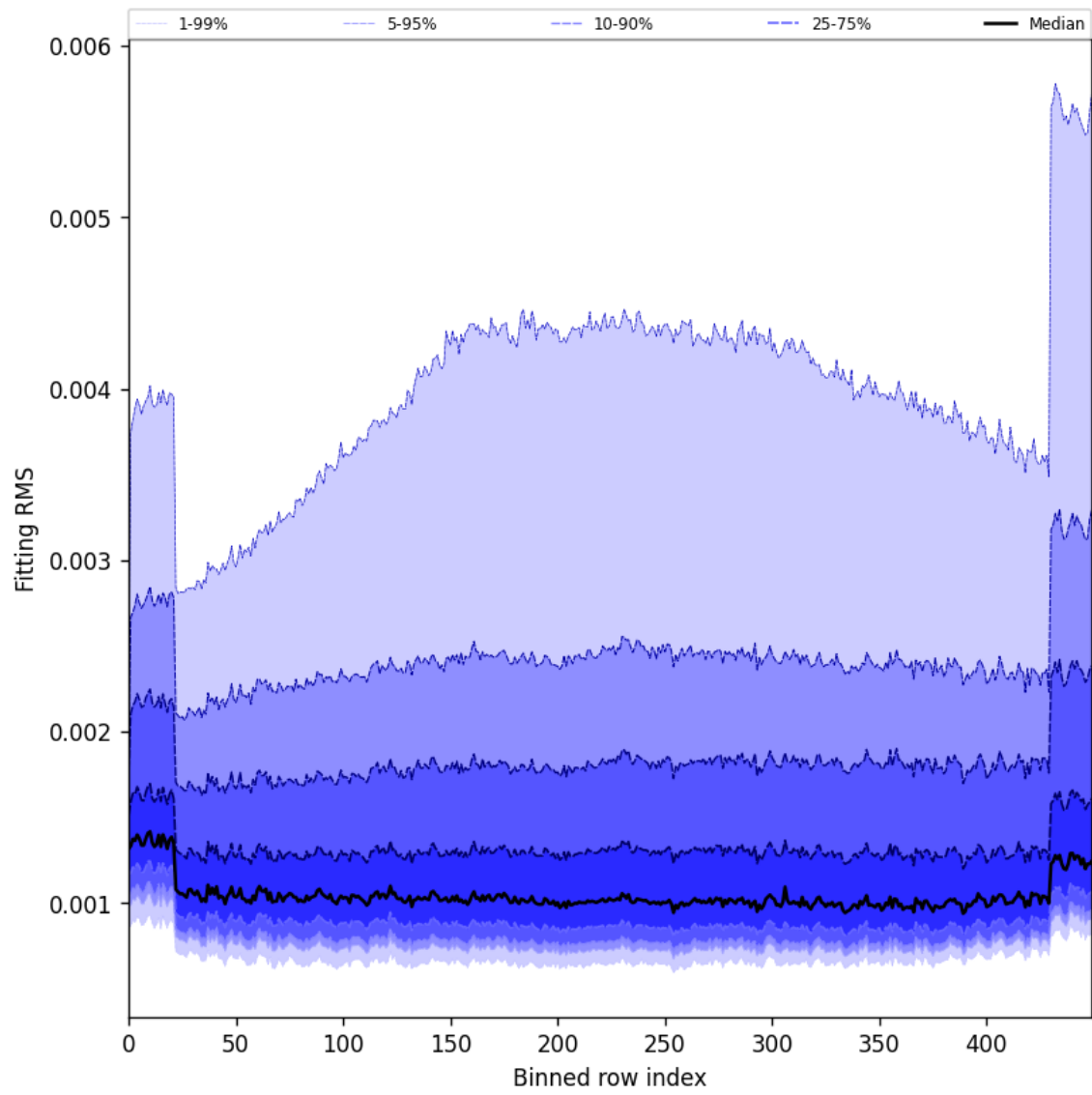
Figure 30: Along track statistics of “Fitting RMS” for 2025-09-12 to 2025-09-14
