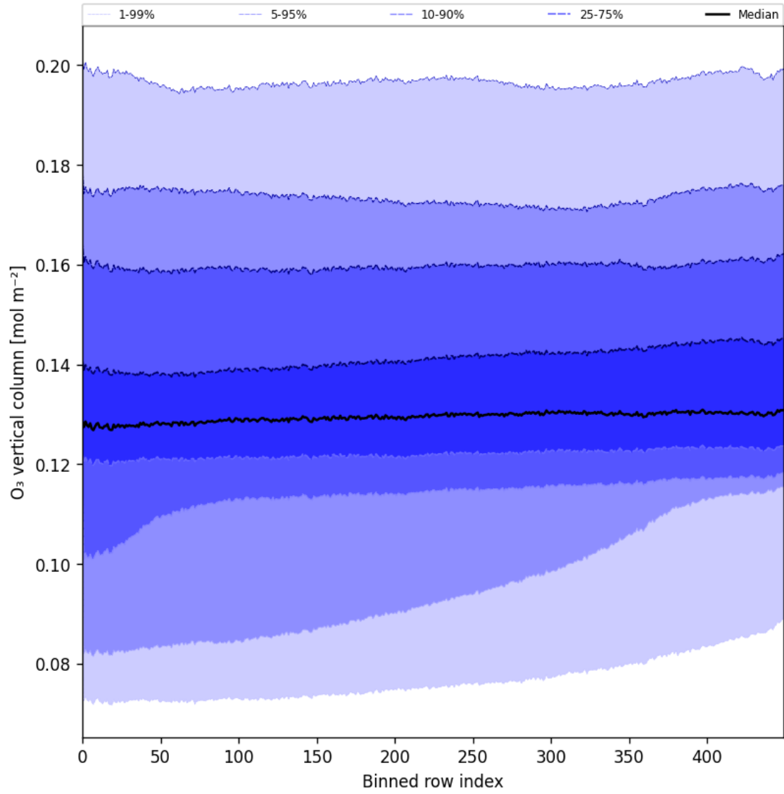
Figure 28: Along track statistics of "O 3 vertical column" for 2025-09-12 to 2025-09-14
