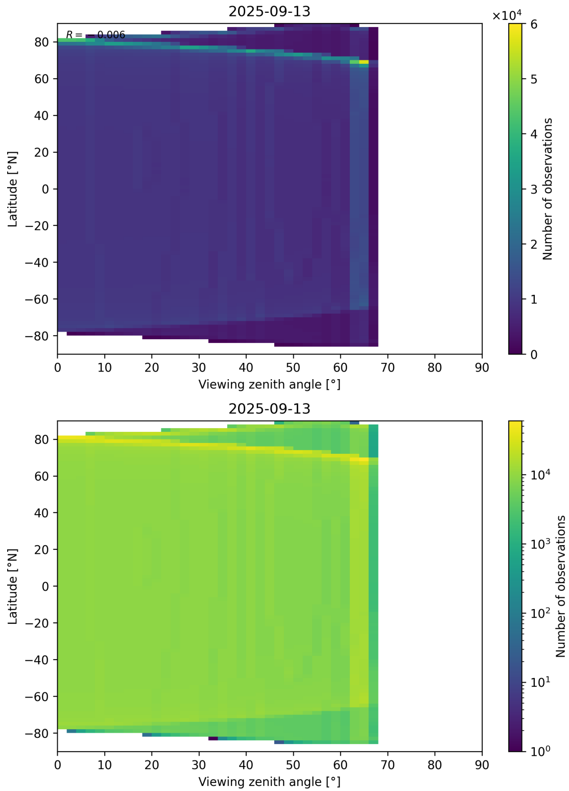
Figure 49: Scatter density plot of “Viewing zenith angle” against “Latitude” for 2025-09-12 to 2025-09-14.
