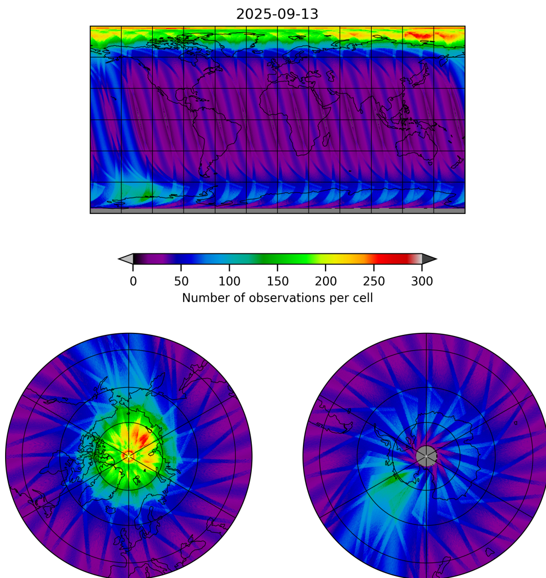
Figure 12: Map of the number of observations for 2025-09-12 to 2025-09-14
