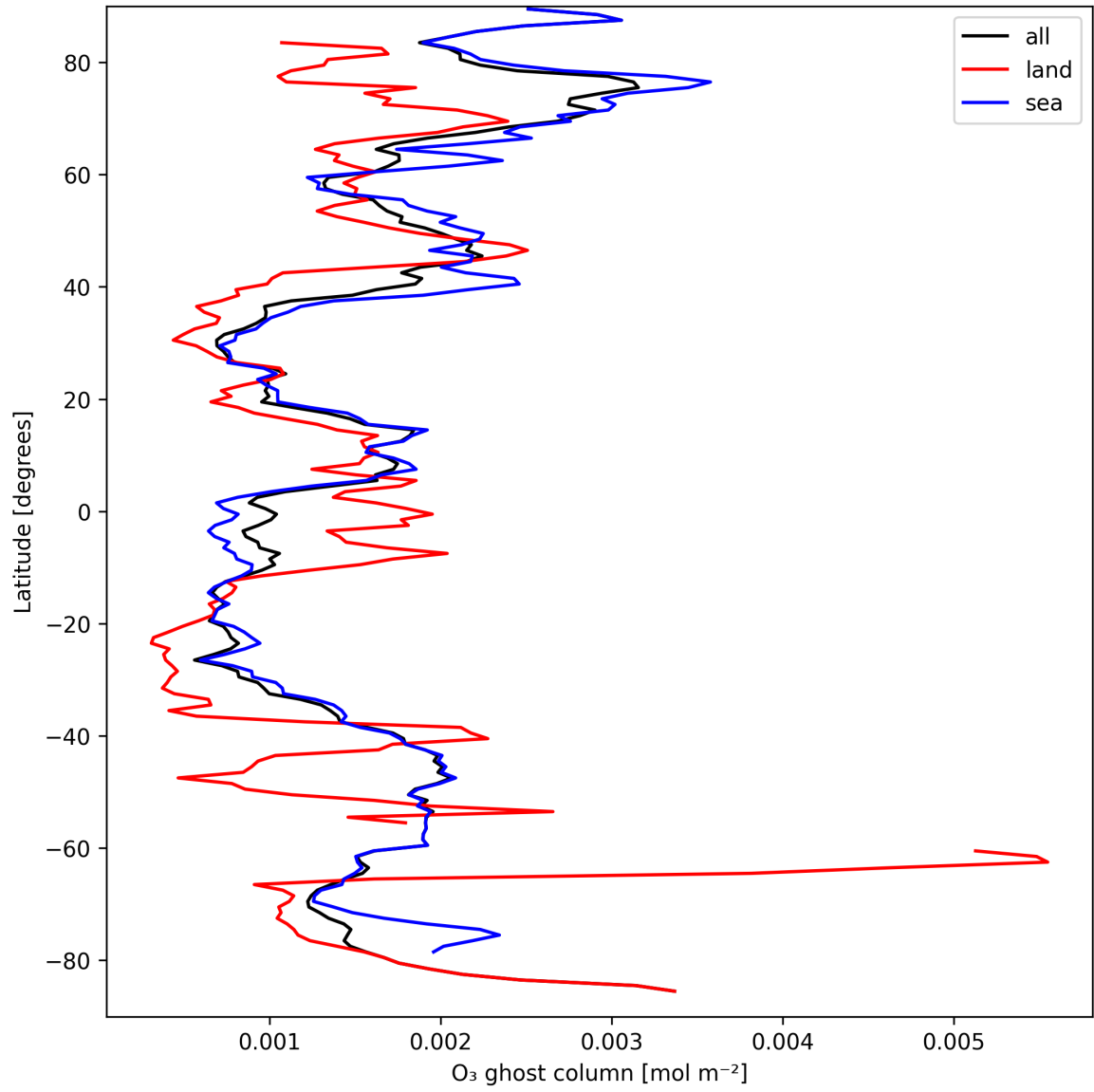
Figure 18: Zonal average of "O 3 ghost column" for 2025-09-12 to 2025-09-14.
