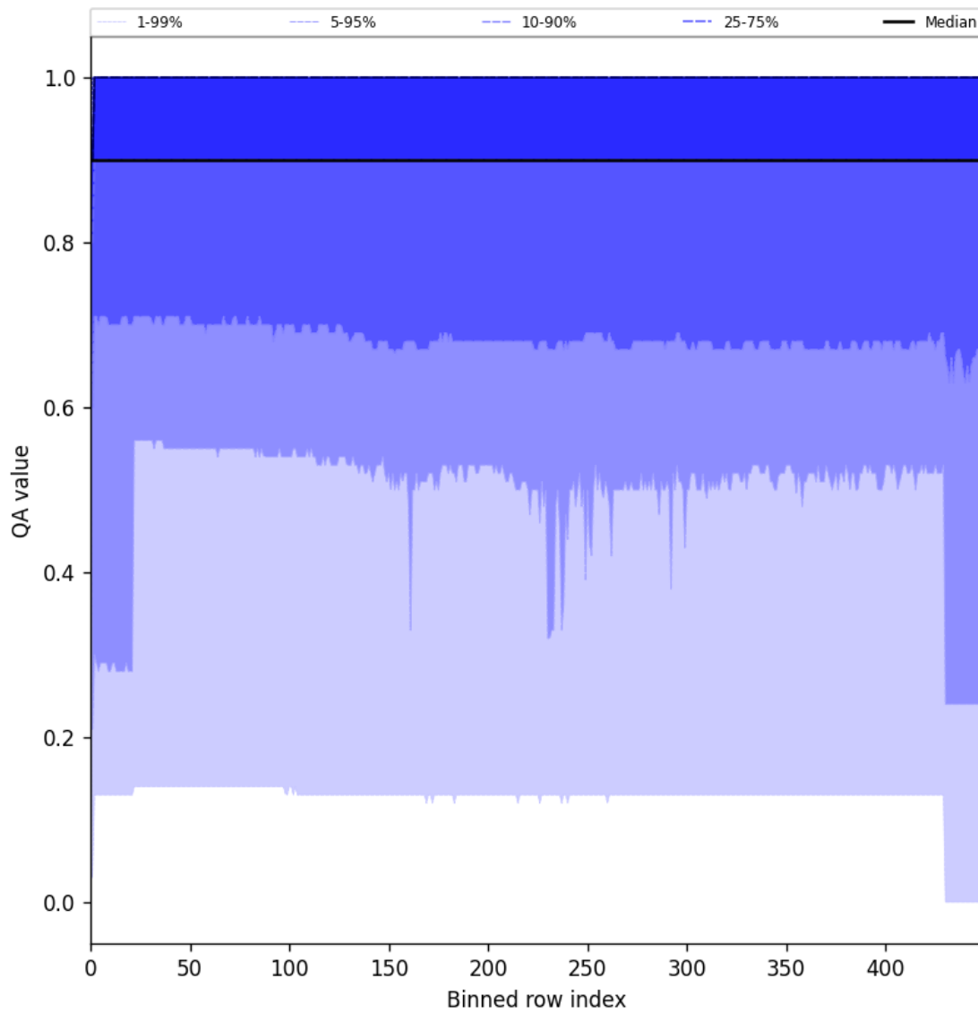
Figure 27: Along track statistics of “QA value” for 2025-09-12 to 2025-09-14
