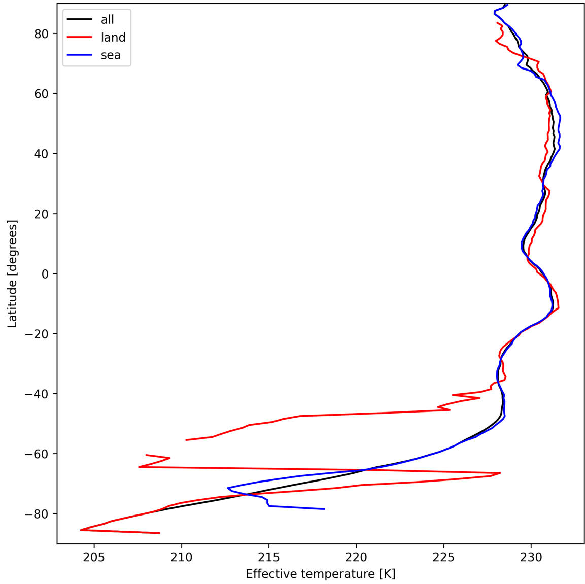
Figure 17: Zonal average of "Effective temperature" for 2025-09-13 to 2025-09-15.
