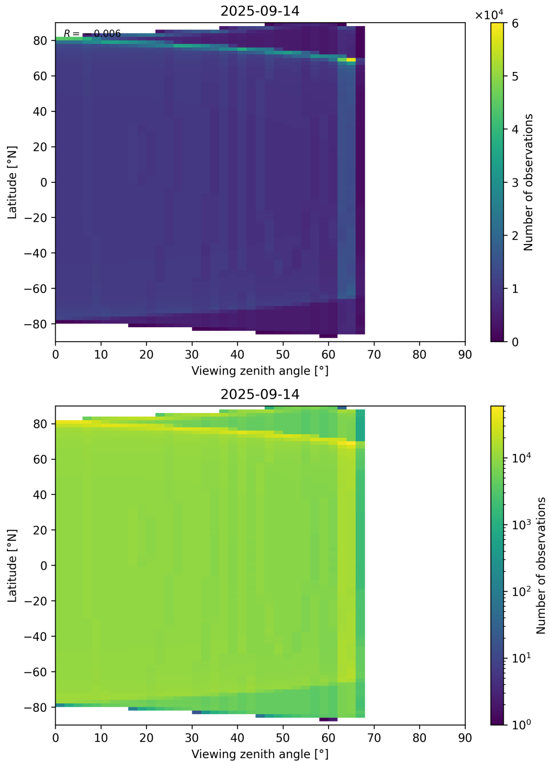
Figure 49: Scatter density plot of “Viewing zenith angle” against “Latitude” for 2025-09-13 to 2025-09-15.
