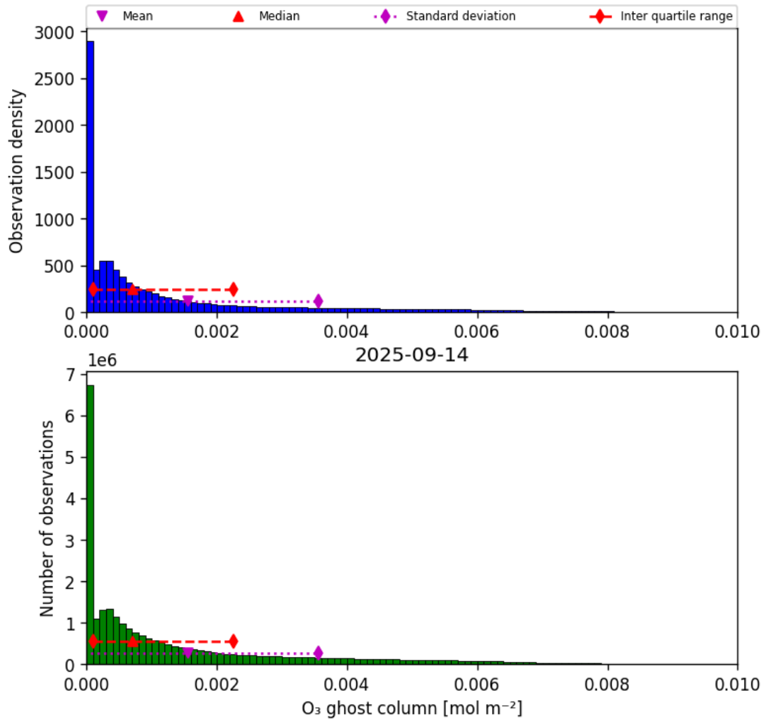
Figure 25: Histogram of “O 3 ghost column” for 2025-09-13 to 2025-09-15
