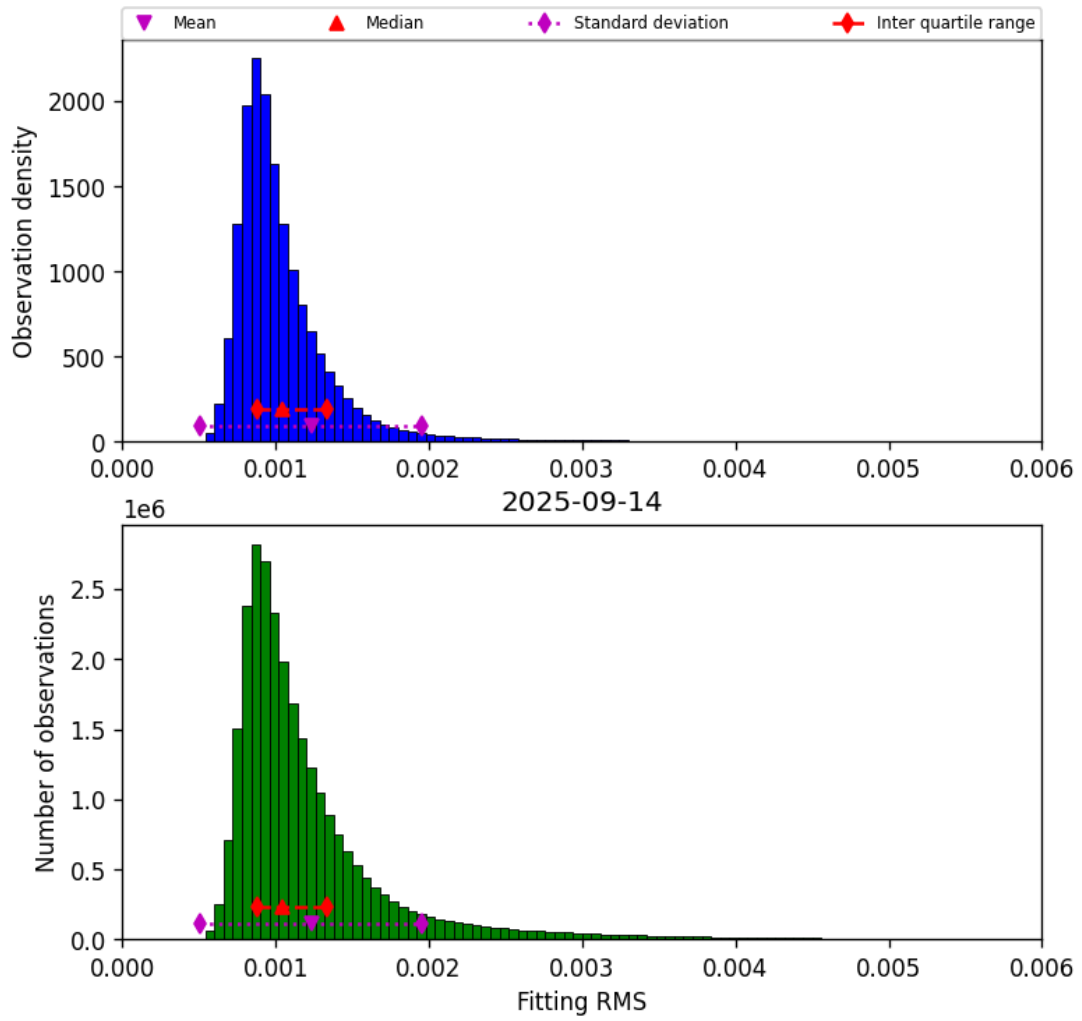
Figure 23: Histogram of “Fitting RMS” for 2025-09-13 to 2025-09-15
