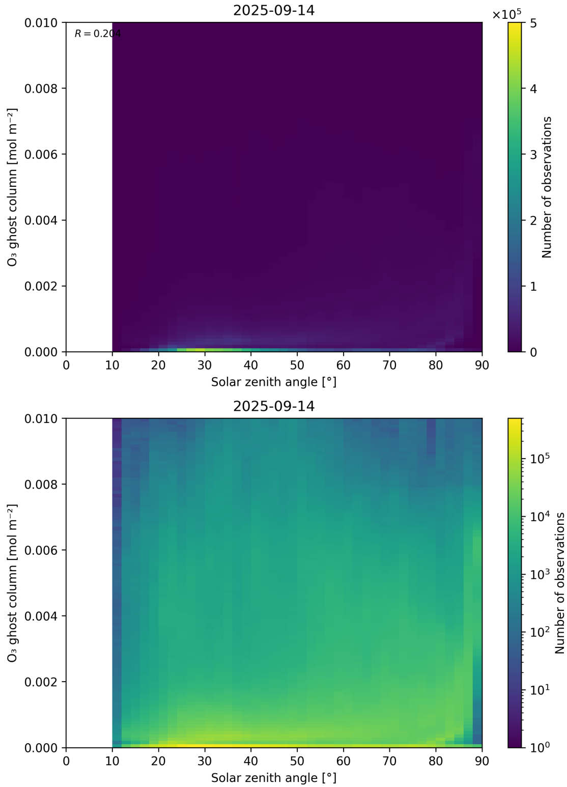
Figure 46: Scatter density plot of “Solar zenith angle” against “O 3 ghost column” for 2025-09-13 to 2025-09-15.
