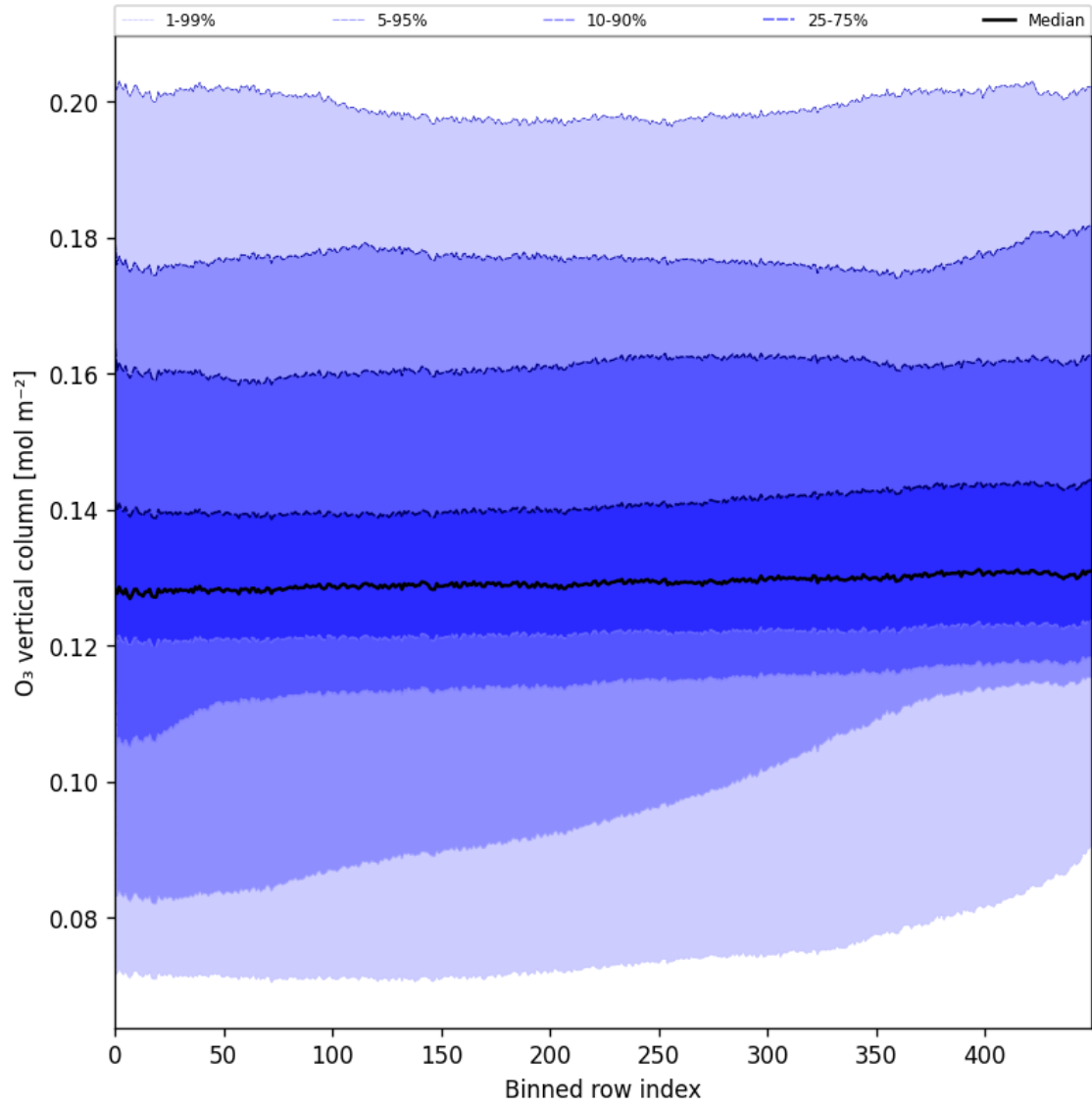
Figure 28: Along track statistics of “O 3 vertical column” for 2025-09-13 to 2025-09-15
