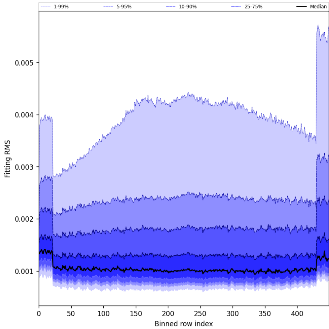
Figure 30: Along track statistics of “Fitting RMS” for 2025-09-13 to 2025-09-15
