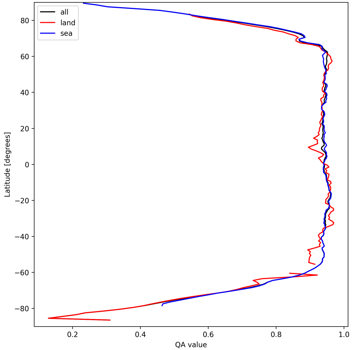
Figure 13: Zonal average of “QA value” for 2025-09-13 to 2025-09-15.
