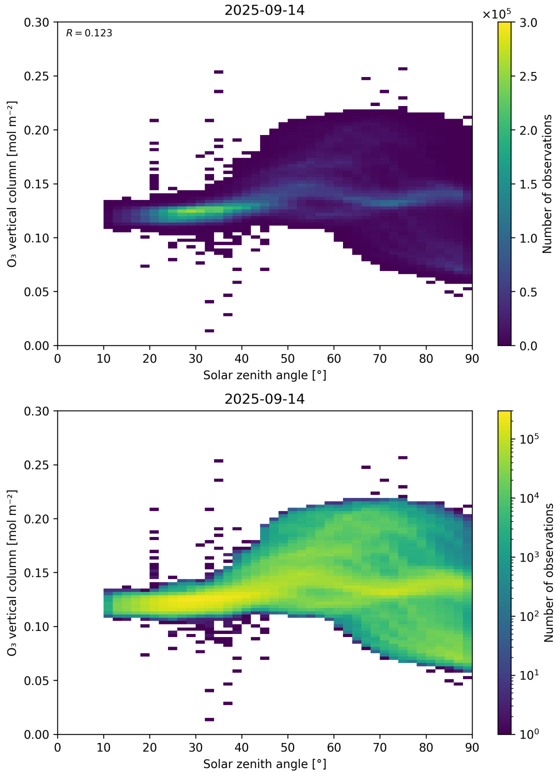
Figure 47: Scatter density plot of “Solar zenith angle” against “O 3 vertical column” for 2025-09-13 to 2025-09-15.
