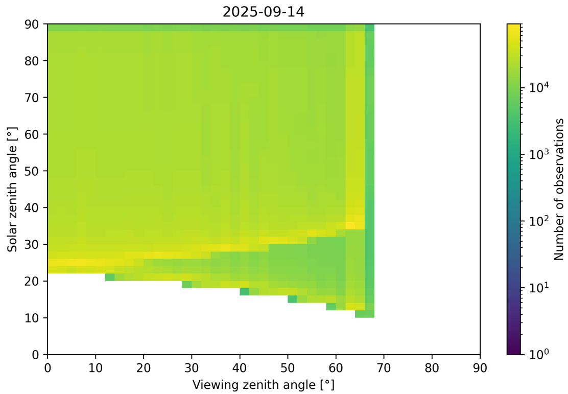
Figure 54: Scatter density plot of “Viewing zenith angle” against “Solar zenith angle” for 2025-09-13 to 2025-09-15.
