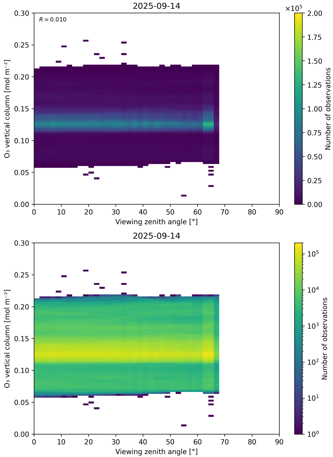
Figure 52: Scatter density plot of “Viewing zenith angle” against “O 3 vertical column” for 2025-09-13 to 2025-09-15.
