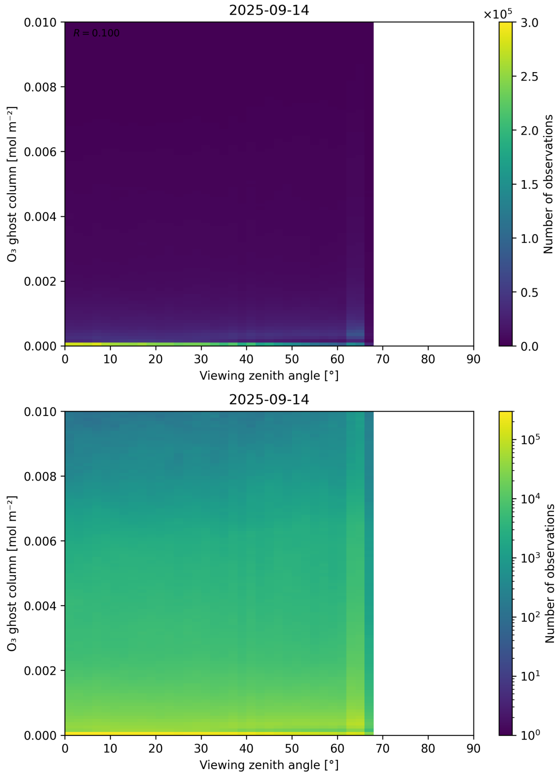
Figure 51: Scatter density plot of “Viewing zenith angle” against “O 3 ghost column” for 2025-09-13 to 2025-09-15.
