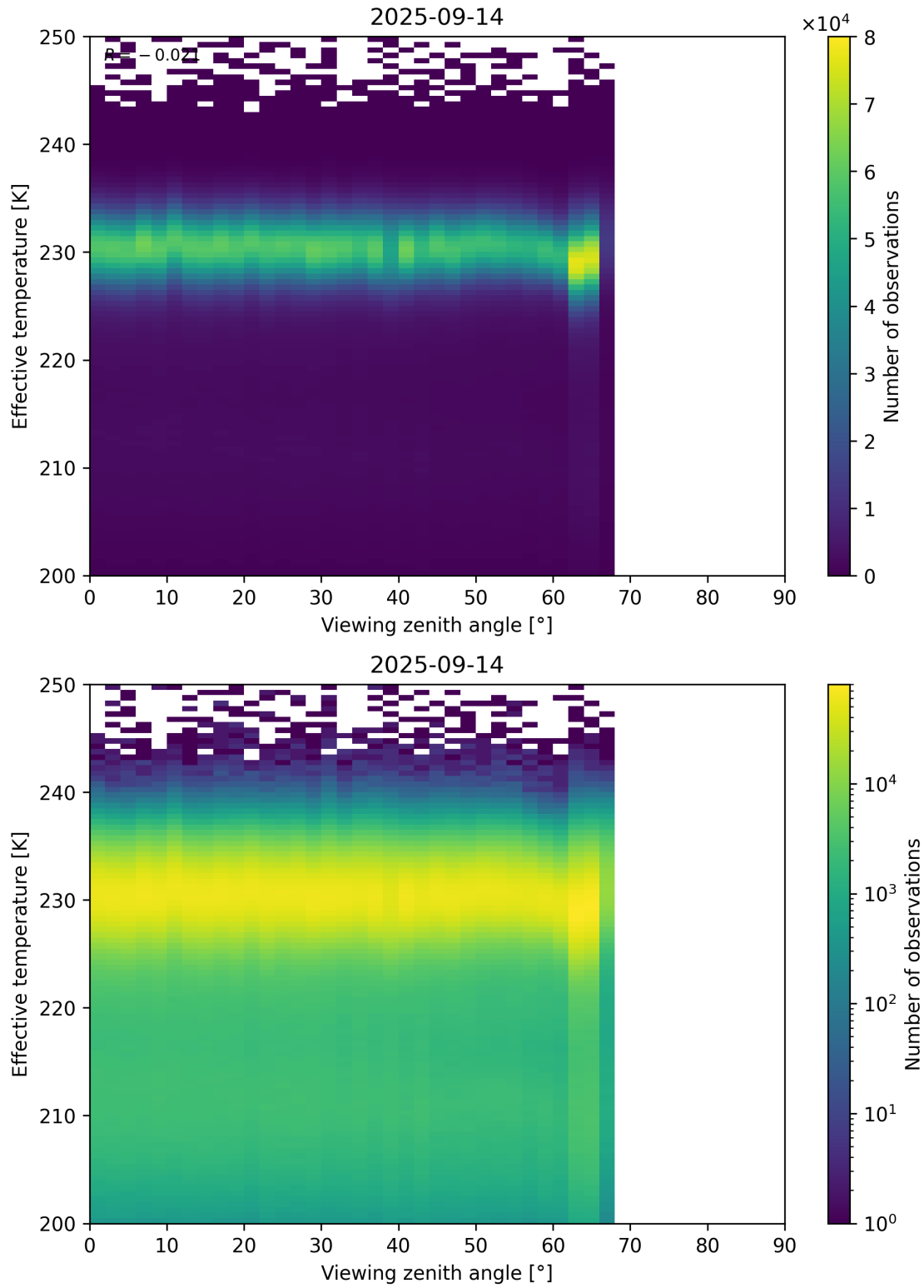
Figure 50: Scatter density plot of “Viewing zenith angle” against “Effective temperature” for 2025-09-13 to 2025-09-15.
