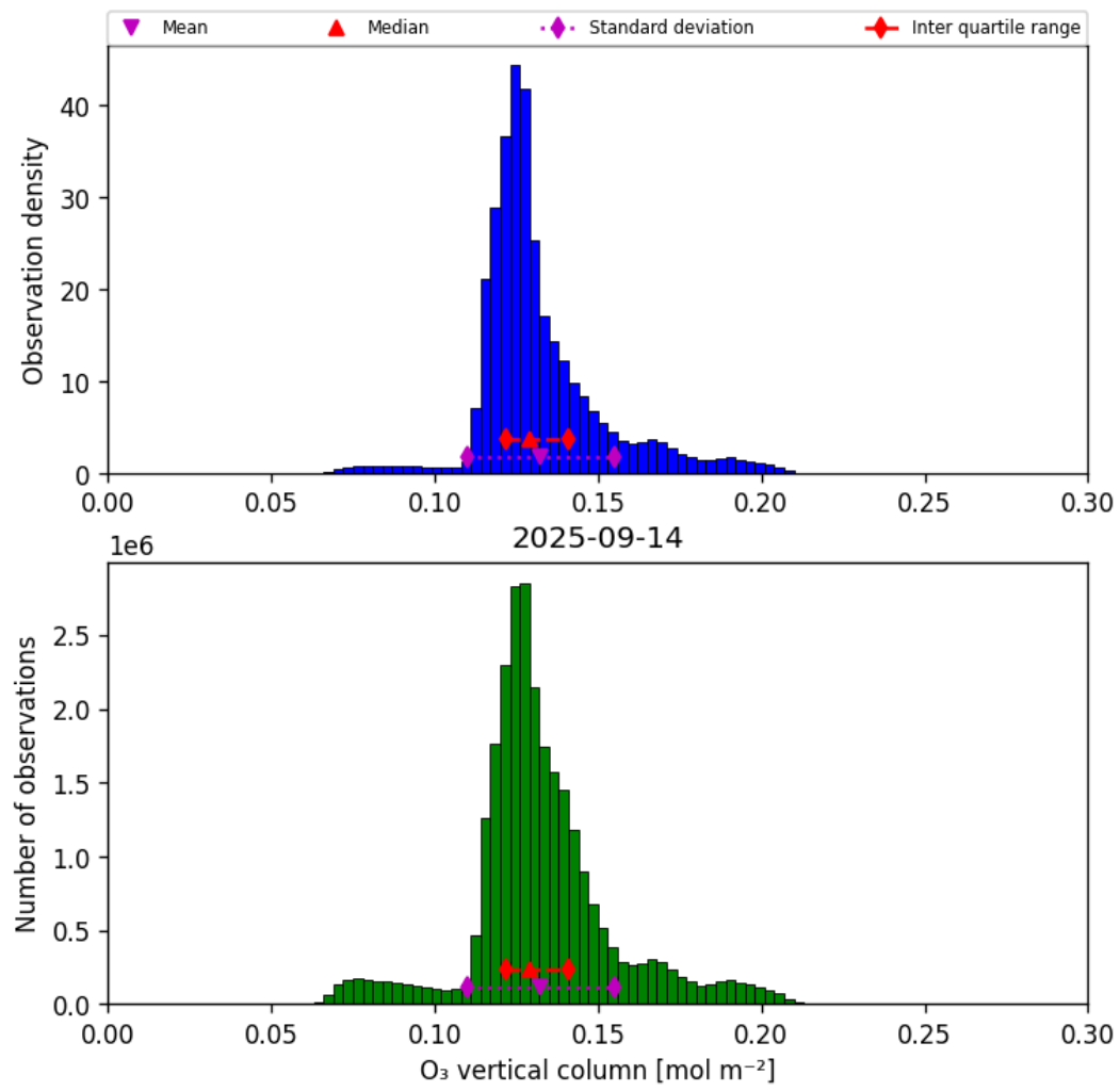
Figure 21: Histogram of “O 3 vertical column” for 2025-09-13 to 2025-09-15
