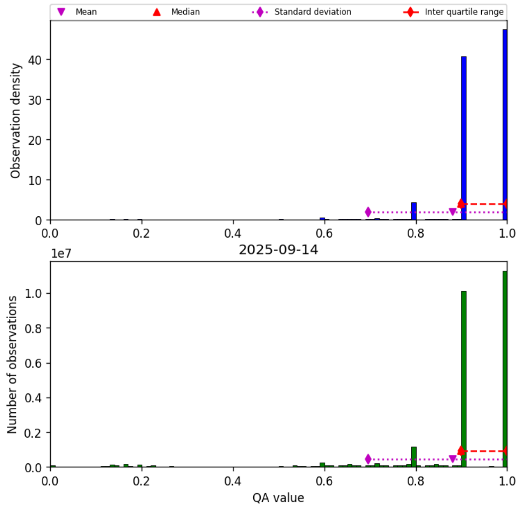
Figure 20: Histogram of “QA value” for 2025-09-13 to 2025-09-15
