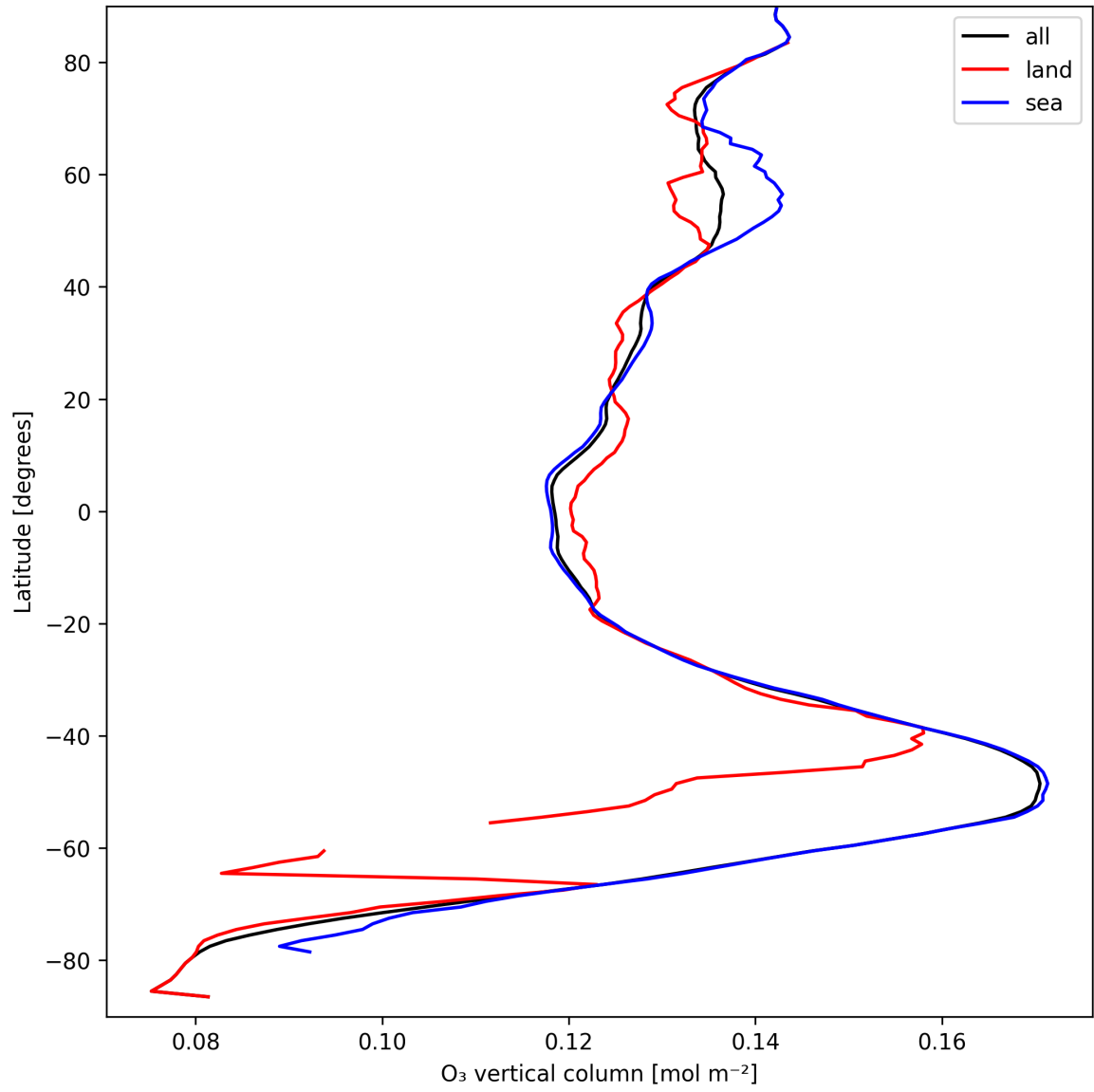
Figure 14: Zonal average of “O 3 vertical column” for 2025-09-13 to 2025-09-15.
