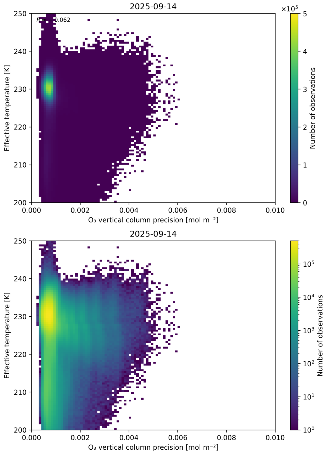
Figure 42: Scatter density plot of “O 3 vertical column precision” against “Effective temperature” for 2025-09-13 to 2025-09-15.
