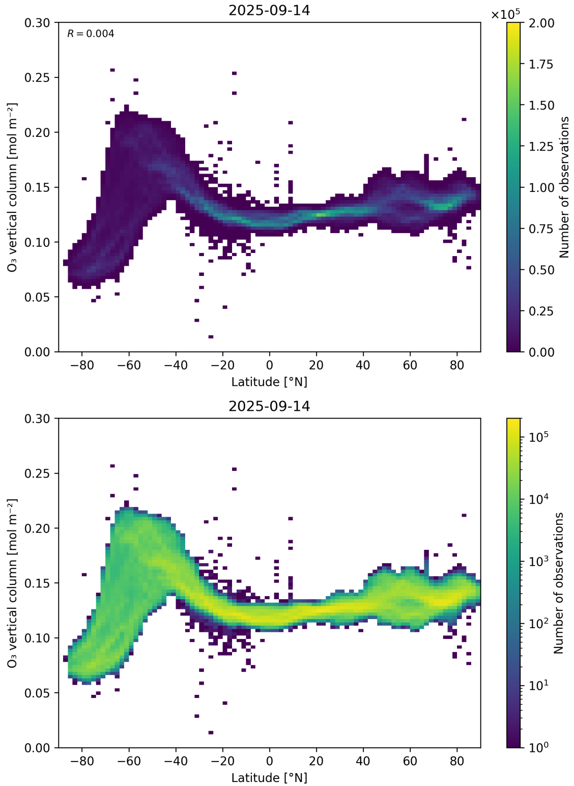
Figure 36: Scatter density plot of “Latitude” against “O 3 vertical column” for 2025-09-13 to 2025-09-15.
