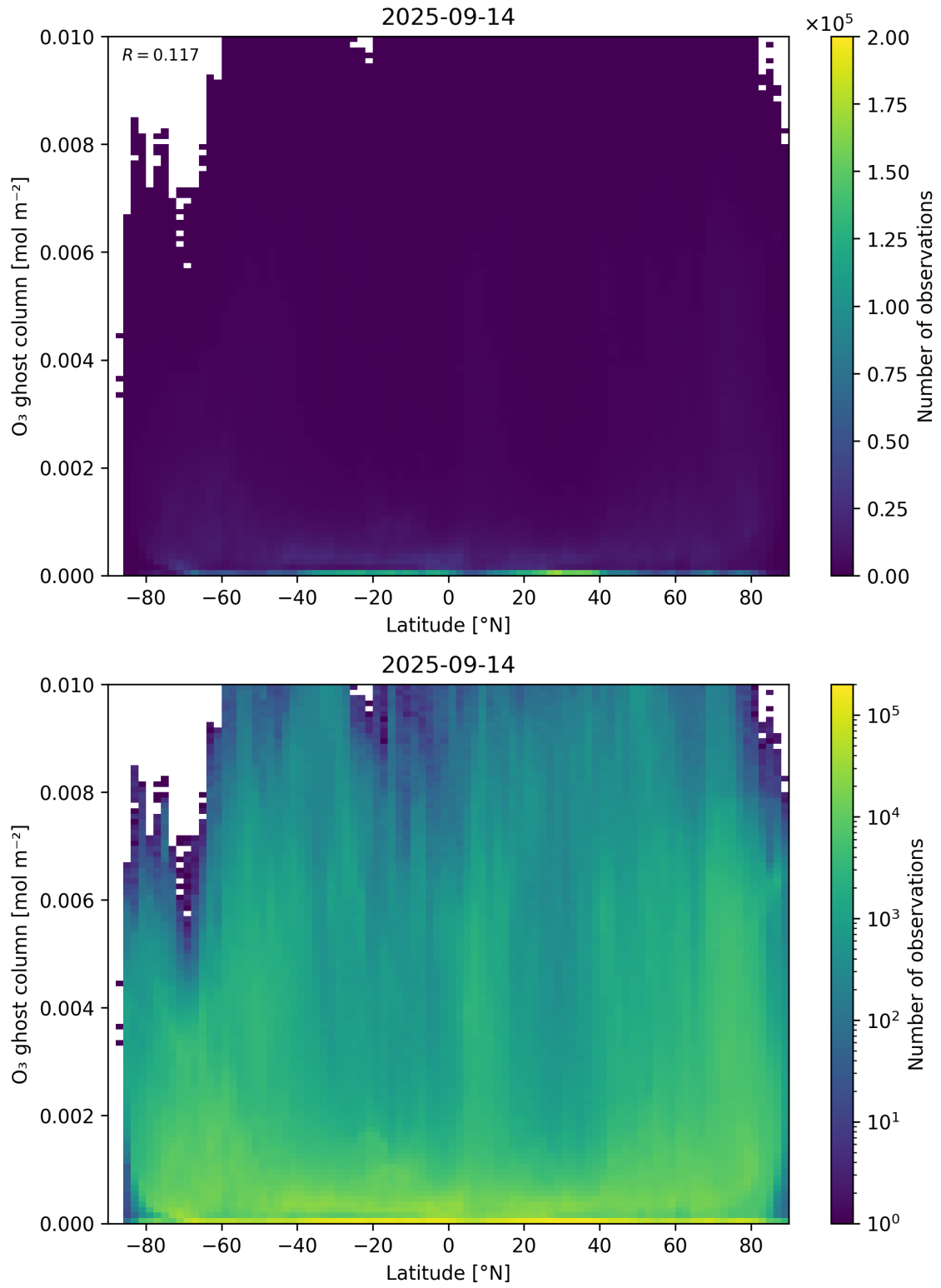
Figure 35: Scatter density plot of “Latitude” against “O 3 ghost column” for 2025-09-13 to 2025-09-15.
