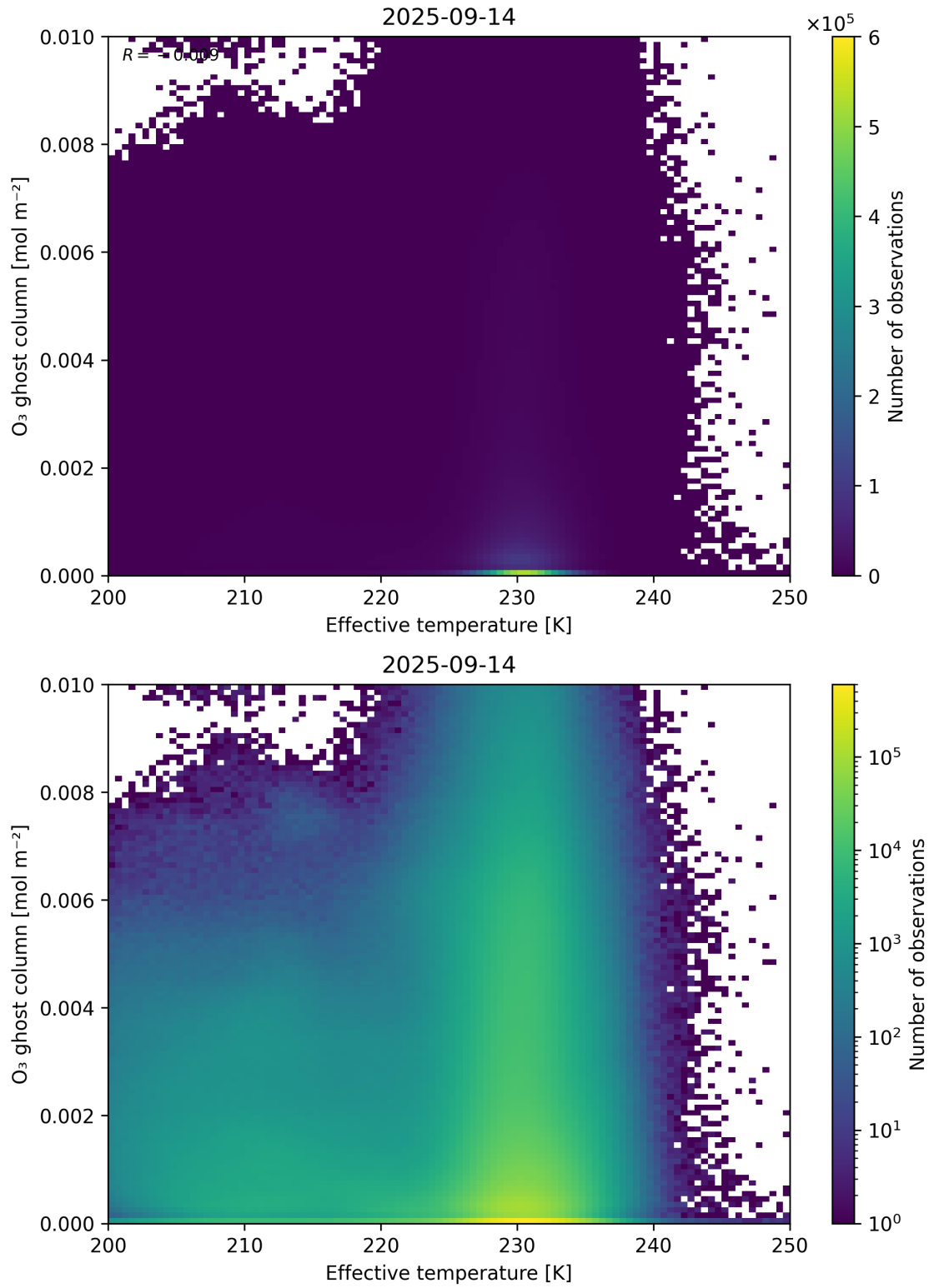
Figure 38: Scatter density plot of “Effective temperature” against “O 3 ghost column” for 2025-09-13 to 2025-09-15.
