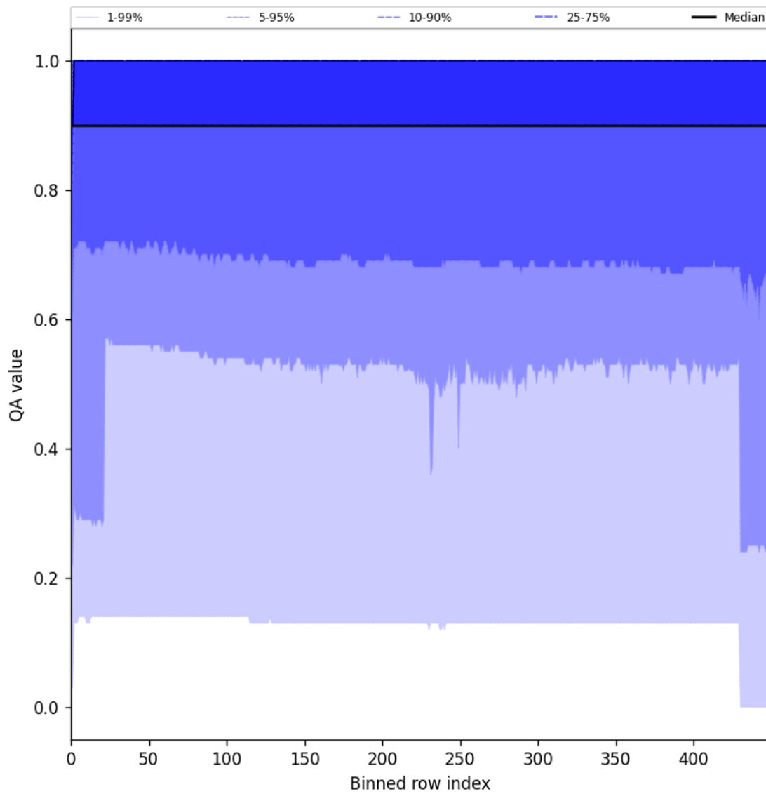
Figure 27: Along track statistics of “QA value” for 2025-09-13 to 2025-09-15
