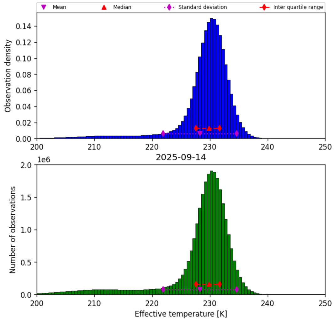
Figure 24: Histogram of “Effective temperature” for 2025-09-13 to 2025-09-15
