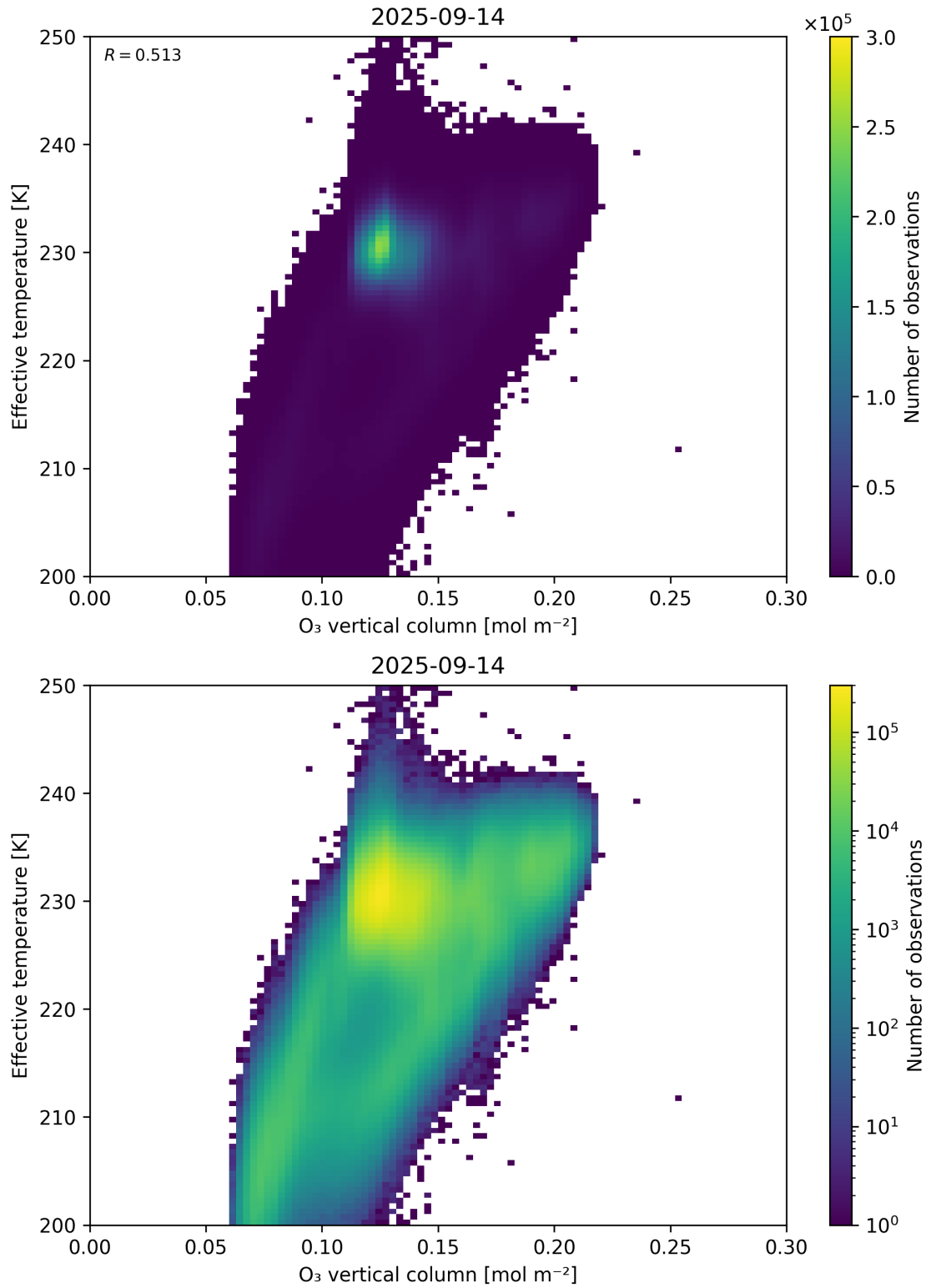
Figure 39: Scatter density plot of “O 3 vertical column” against “Effective temperature” for 2025-09-13 to 2025-09-15.
