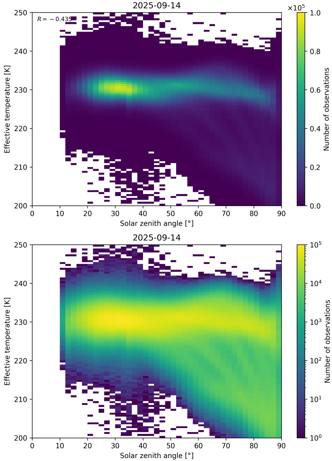
Figure 45: Scatter density plot of “Solar zenith angle” against “Effective temperature” for 2025-09-13 to 2025-09-15.
