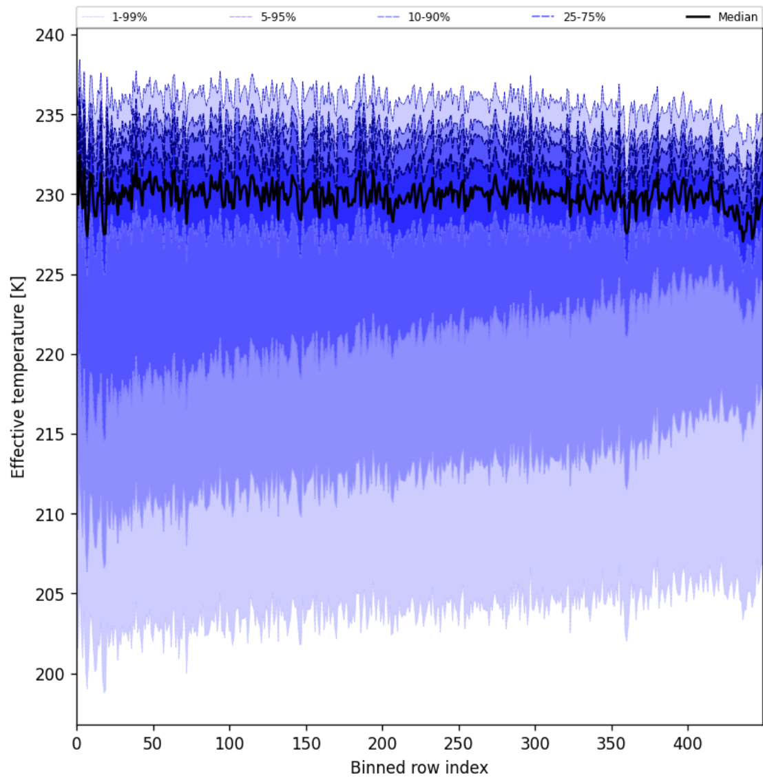
Figure 31: Along track statistics of “Effective temperature” for 2025-09-13 to 2025-09-15
