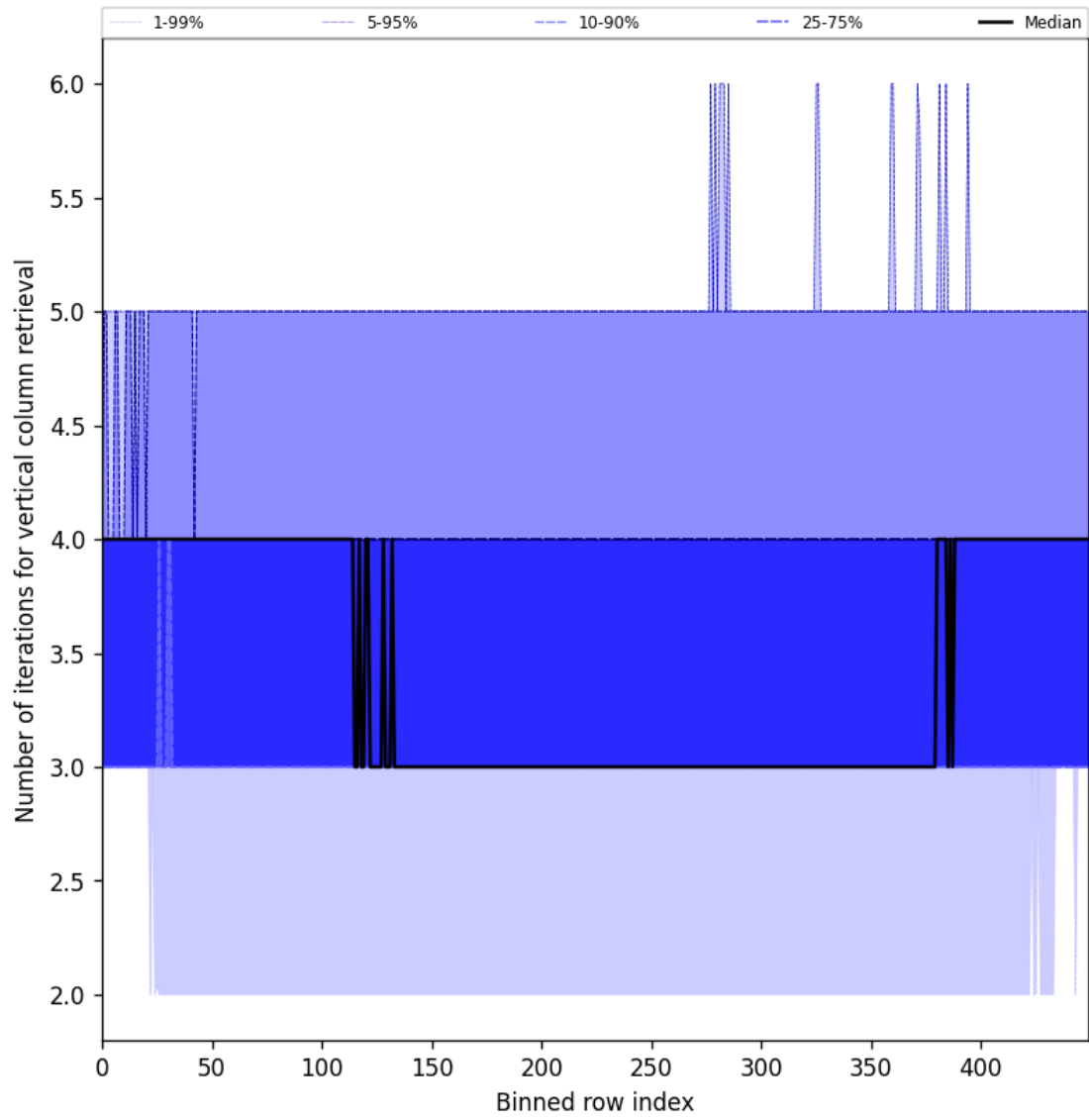
Figure 33: Along track statistics of “Number of iterations for vertical column retrieval” for 2025-09-13 to 2025-09-15
