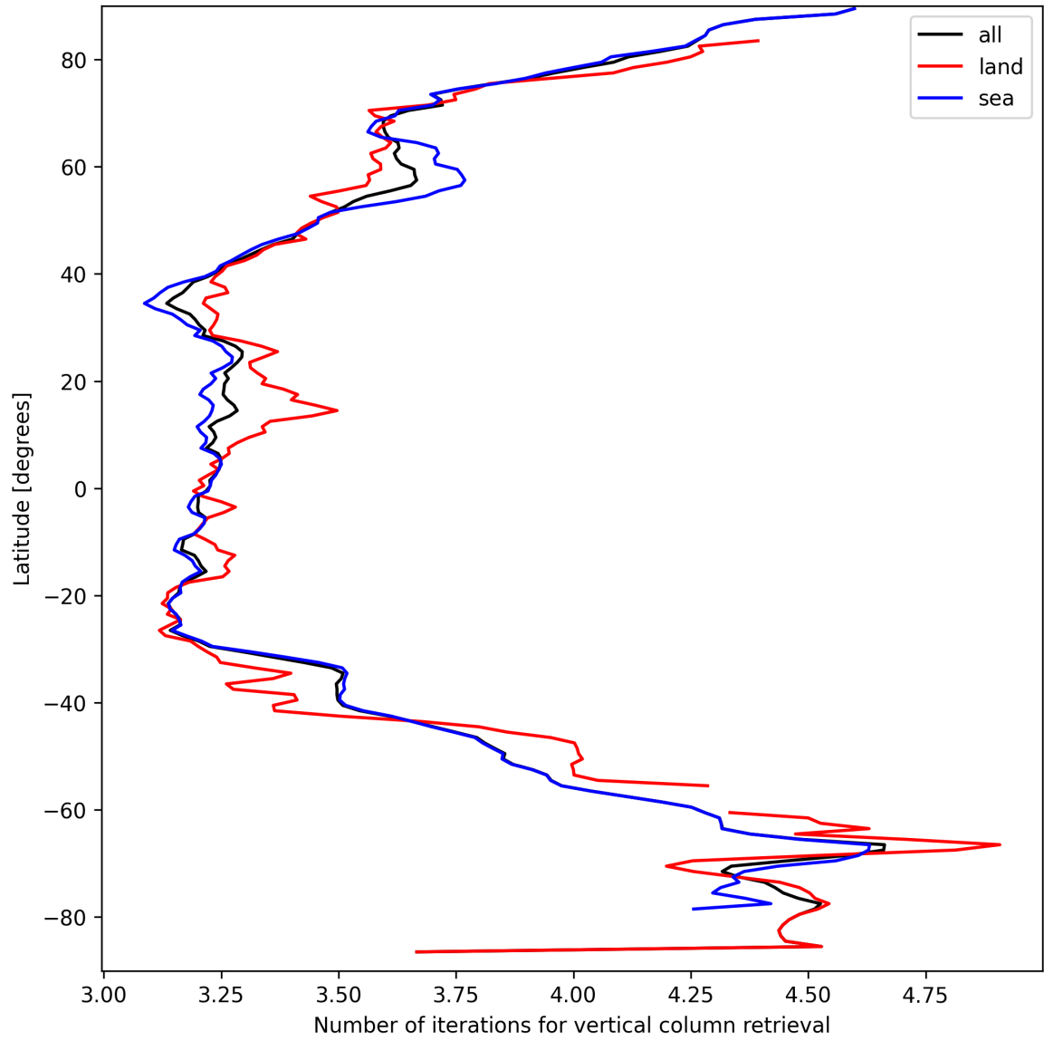
Figure 19: Zonal average of “Number of iterations for vertical column retrieval” for 2025-09-13 to 2025-09-15.
