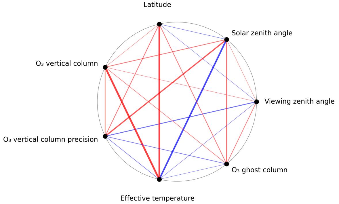
Figure 1: Map of correlation graph for 2025-09-13 to 2025-09-15.
