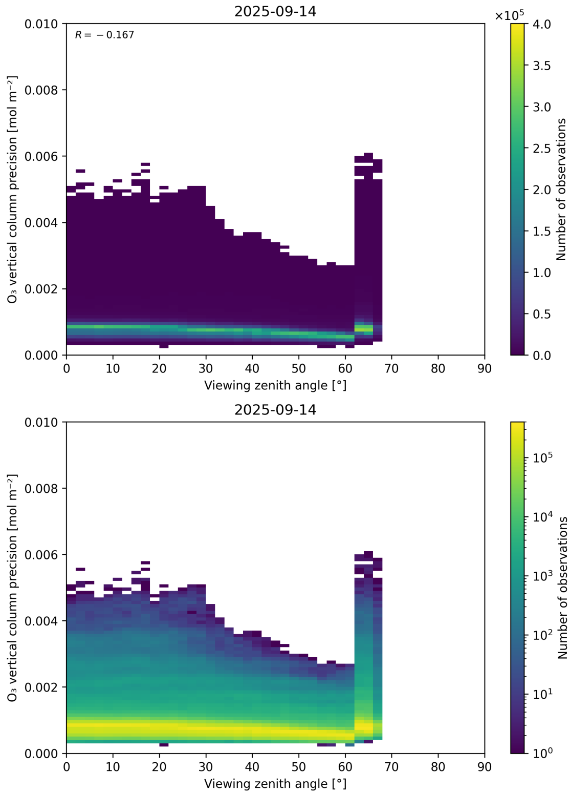
Figure 53: Scatter density plot of “Viewing zenith angle” against “O 3 vertical column precision” for 2025-09-13 to 2025-09-15.
