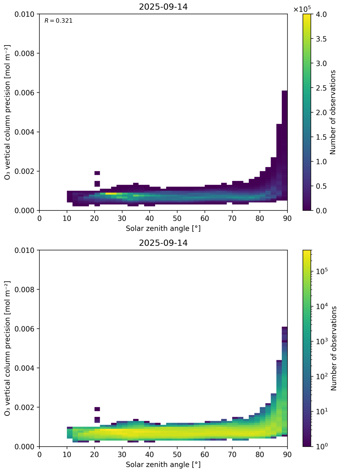
Figure 48: Scatter density plot of “Solar zenith angle” against “O 3 vertical column precision” for 2025-09-13 to 2025-09-15.
