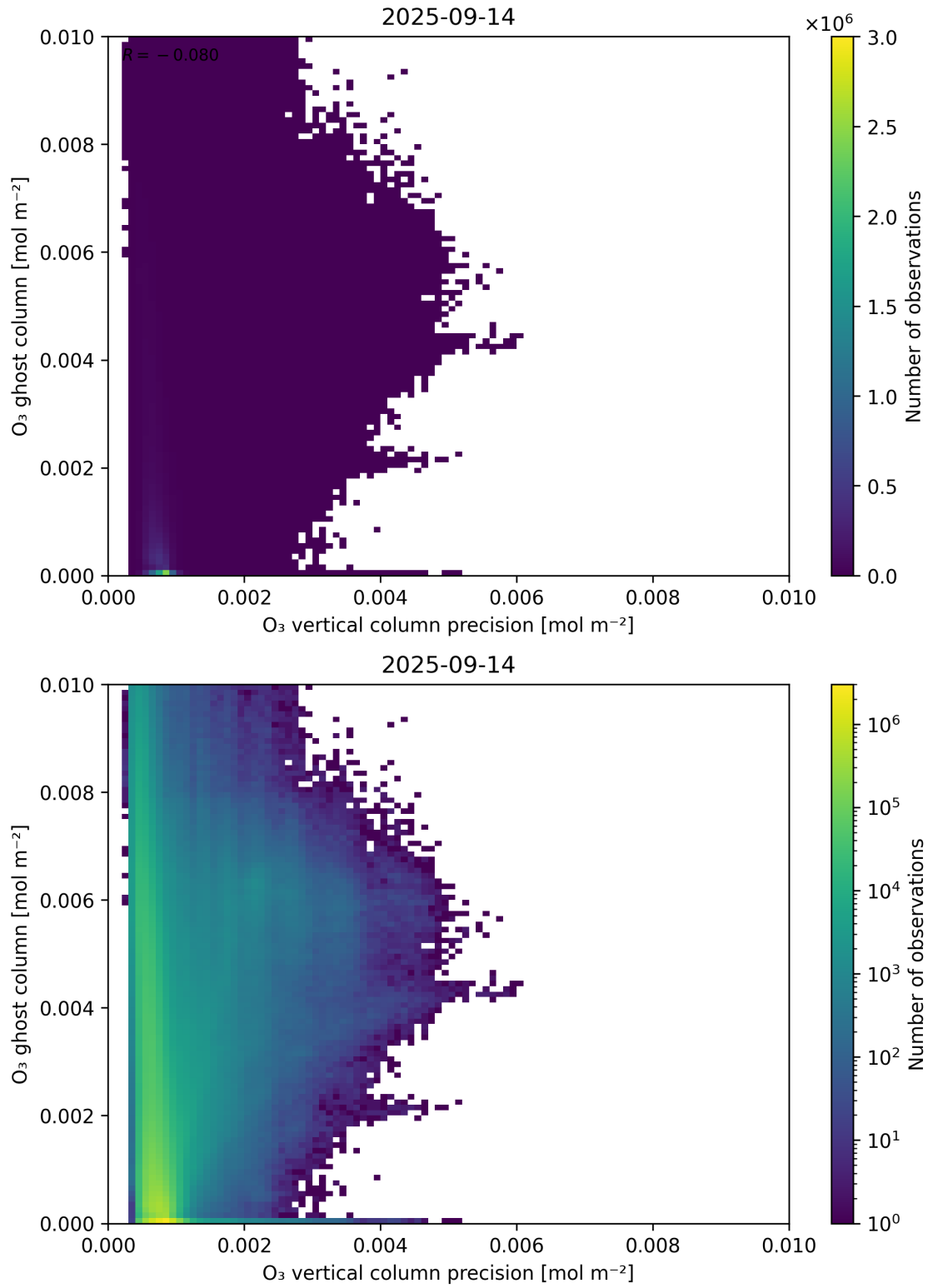
Figure 43: Scatter density plot of “ \text{O}_3 vertical column precision” against “ \text{O}_3 ghost column” for 2025-09-13 to 2025-09-15.
