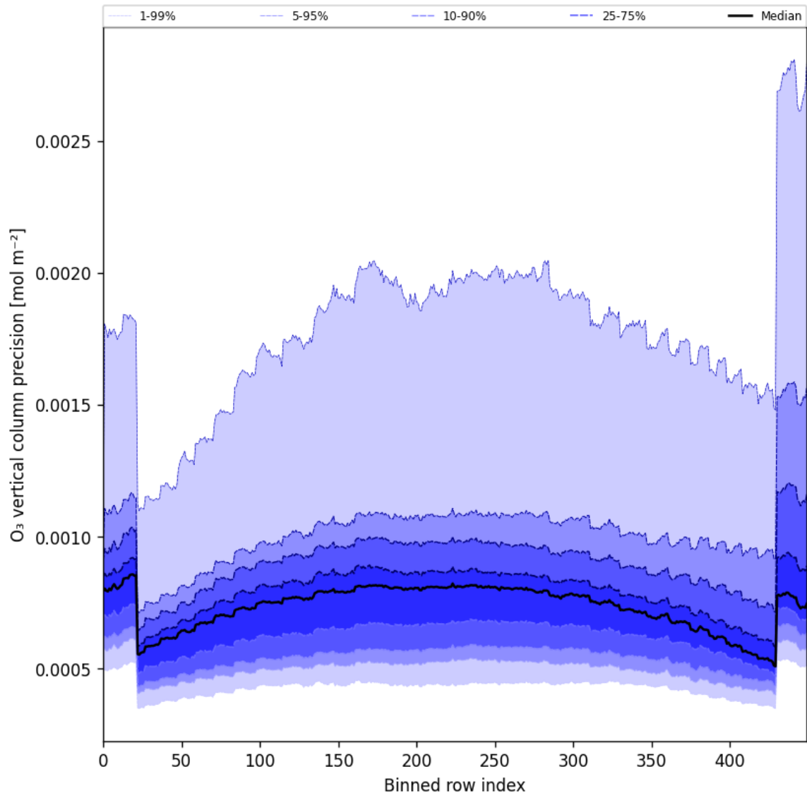
Figure 29: Along track statistics of “O 3 vertical column precision” for 2025-09-13 to 2025-09-15
