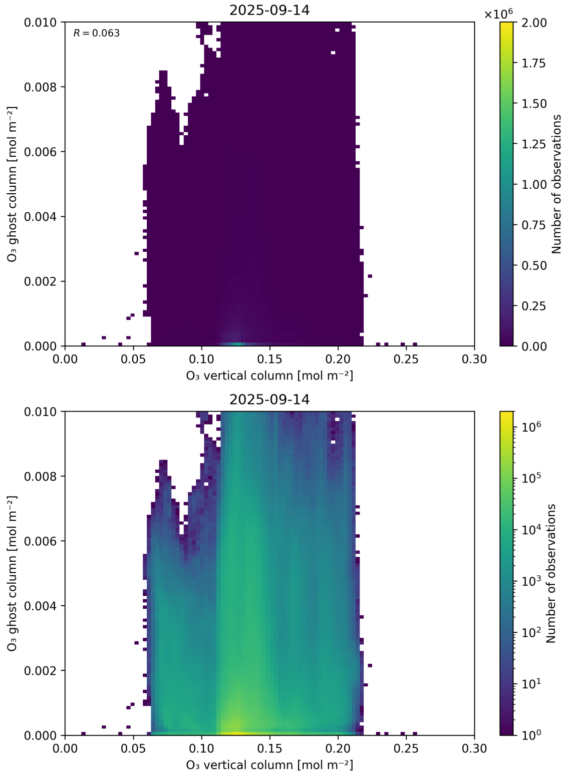
Figure 40: Scatter density plot of “O 3 vertical column” against “O 3 ghost column” for 2025-09-13 to 2025-09-15.
