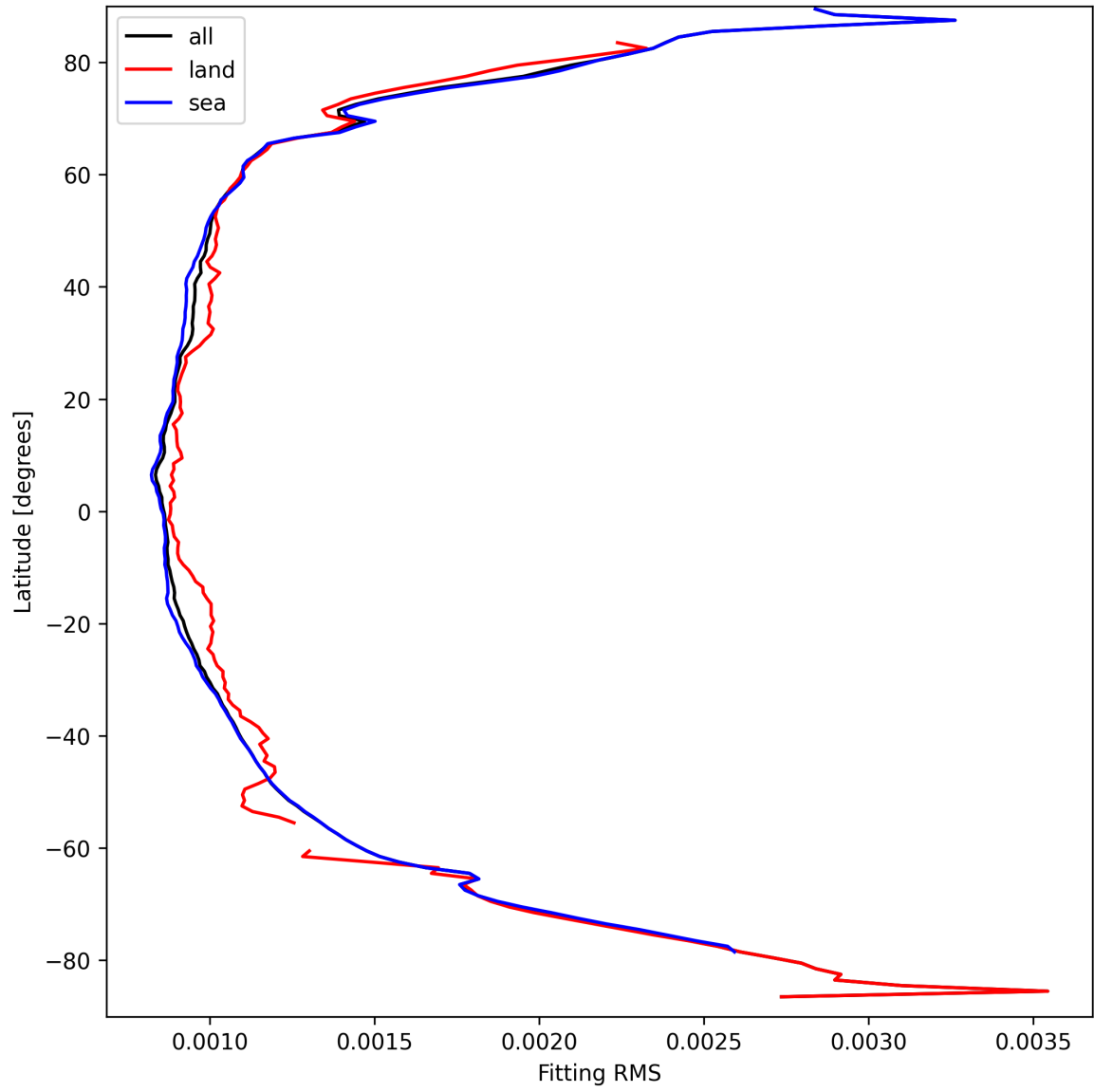
Figure 16: Zonal average of “Fitting RMS” for 2025-09-13 to 2025-09-15.
