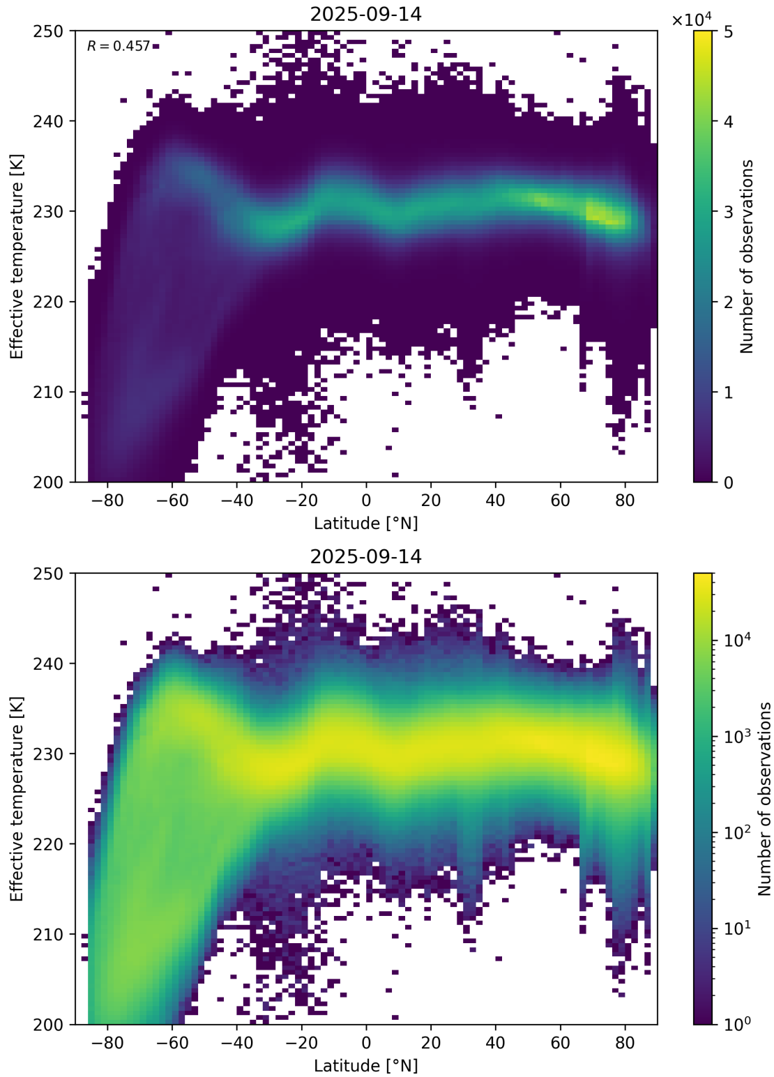
Figure 34: Scatter density plot of “Latitude” against “Effective temperature” for 2025-09-13 to 2025-09-15.
