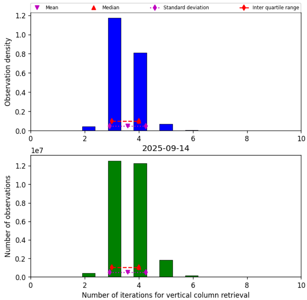
Figure 26: Histogram of “Number of iterations for vertical column retrieval” for 2025-09-13 to 2025-09-15
