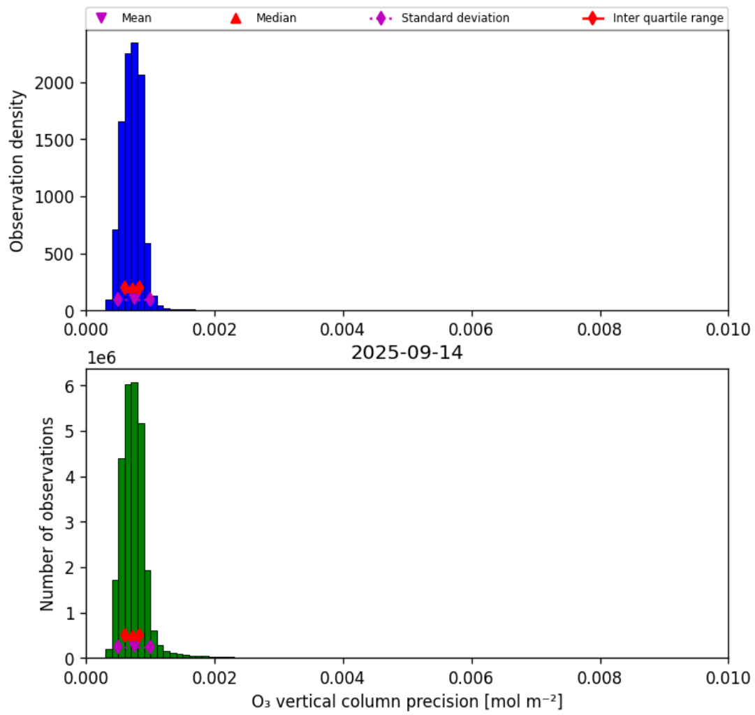
Figure 22: Histogram of “O 3 vertical column precision” for 2025-09-13 to 2025-09-15
