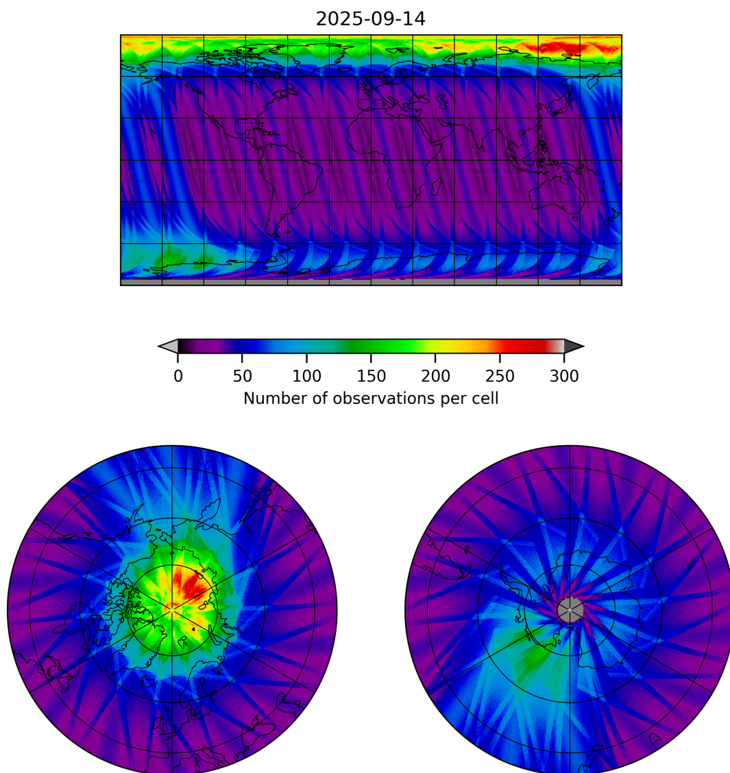
Figure 12: Map of the number of observations for 2025-09-13 to 2025-09-15
