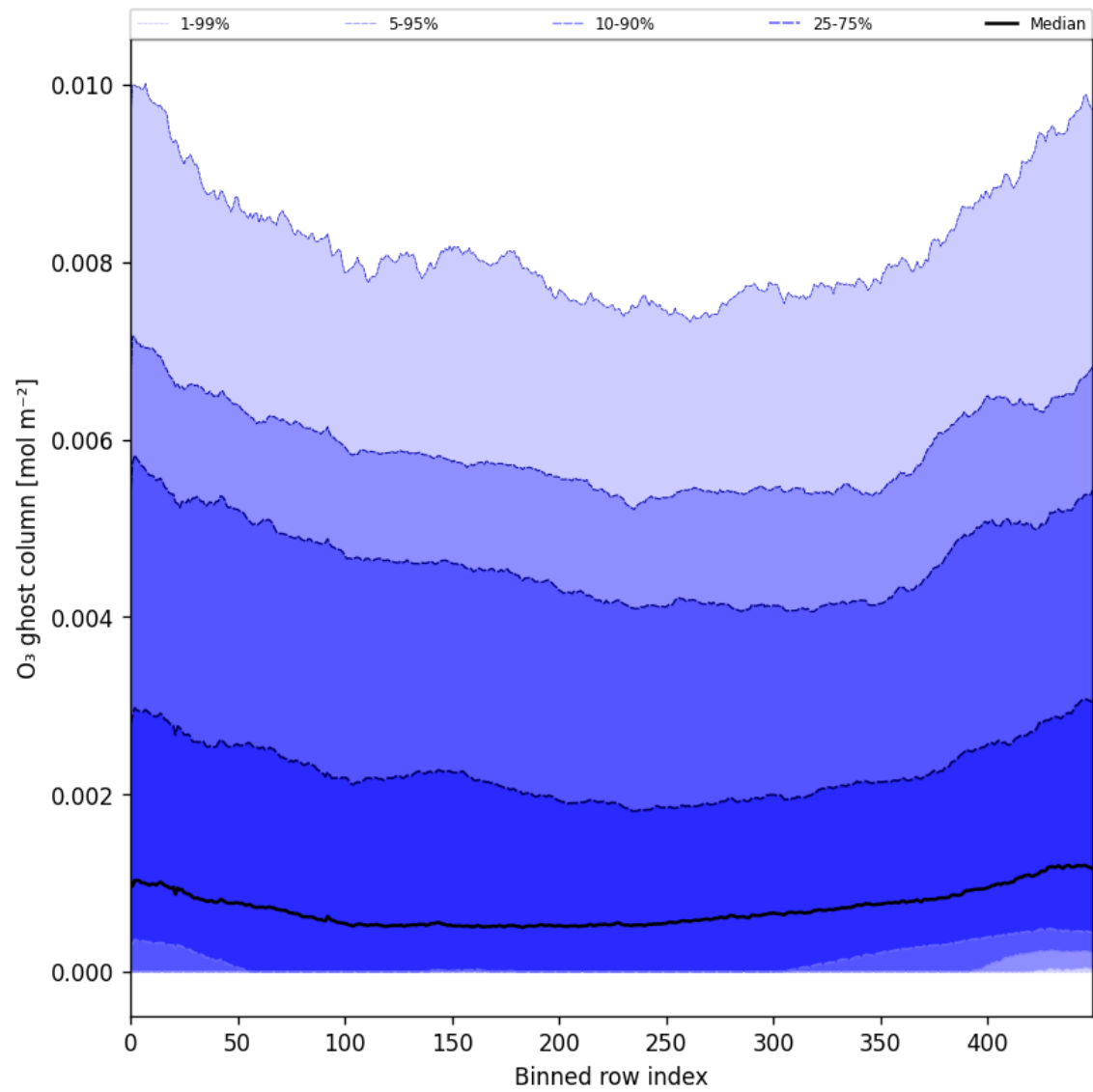
Figure 32: Along track statistics of “O 3 ghost column” for 2025-09-13 to 2025-09-15
