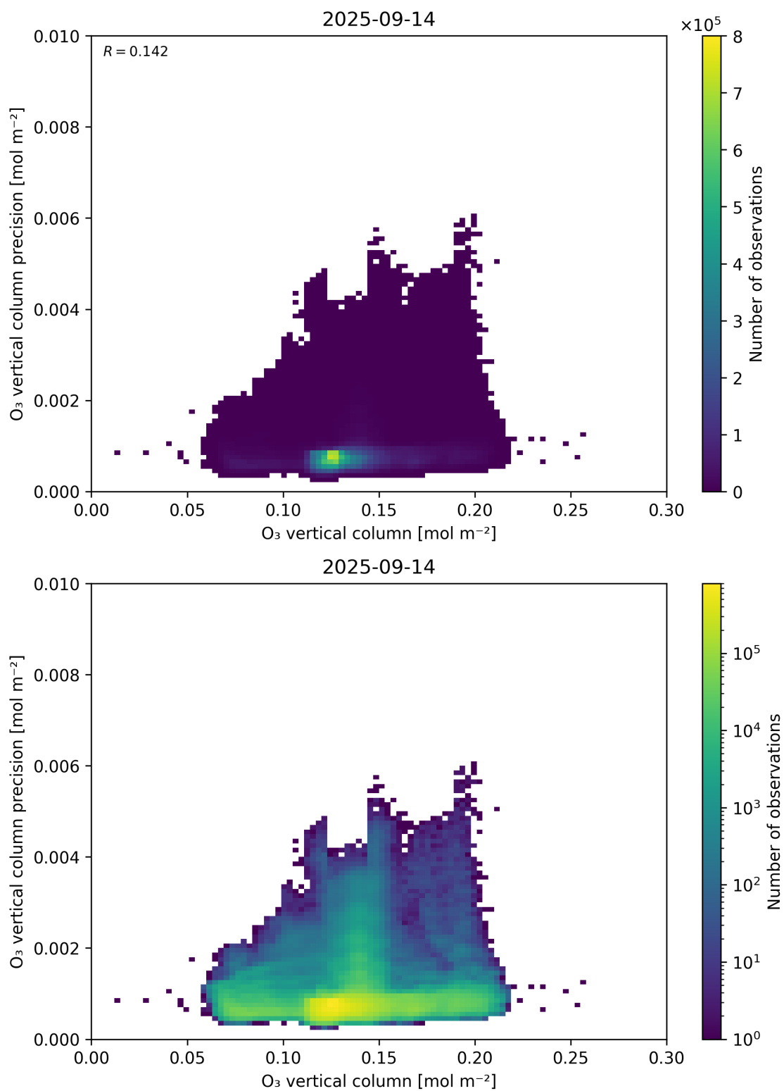
Figure 41: Scatter density plot of “O 3 vertical column” against “O 3 vertical column precision” for 2025-09-13 to 2025-09-15.
