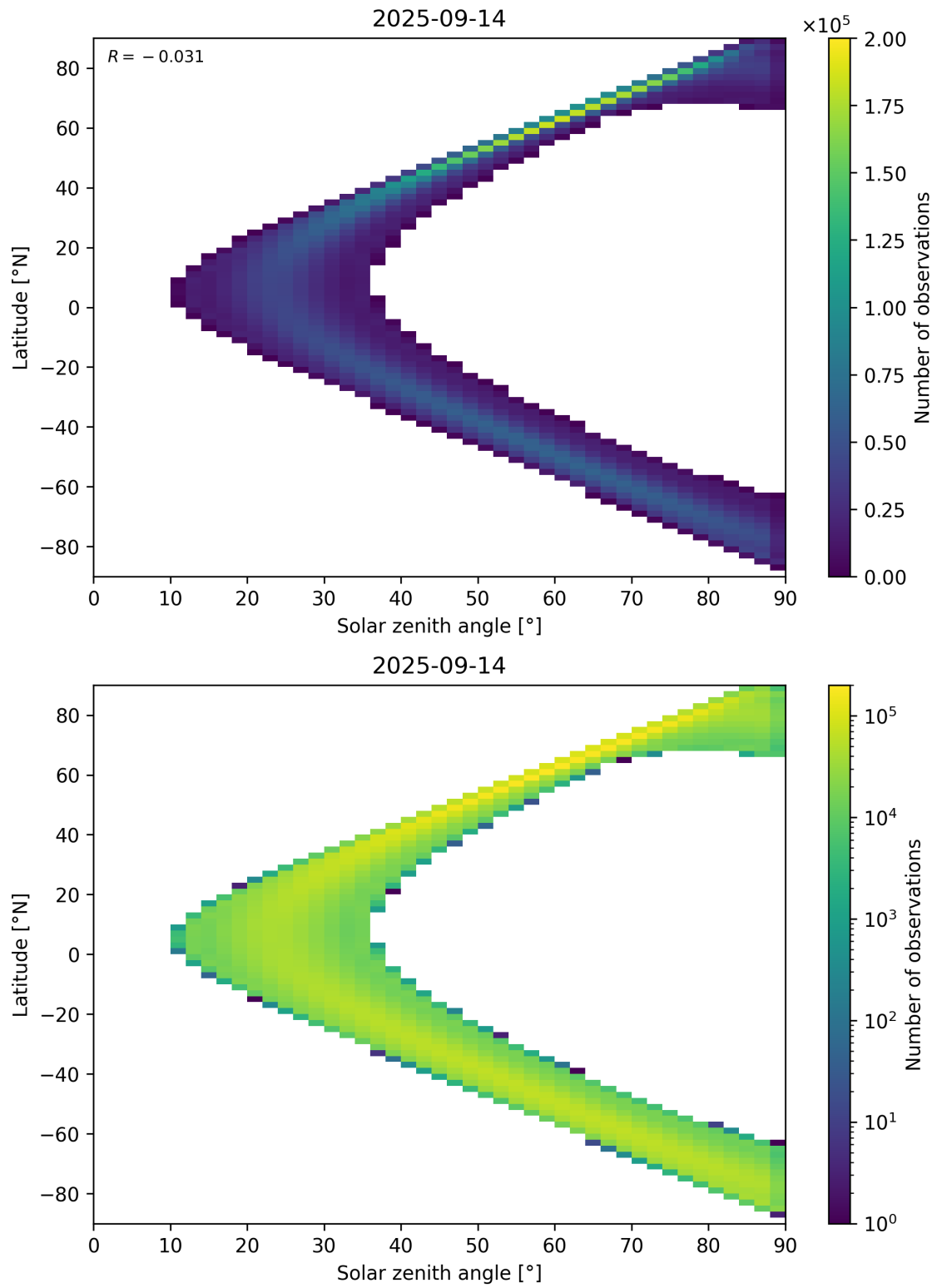
Figure 44: Scatter density plot of “Solar zenith angle” against “Latitude” for 2025-09-13 to 2025-09-15.
