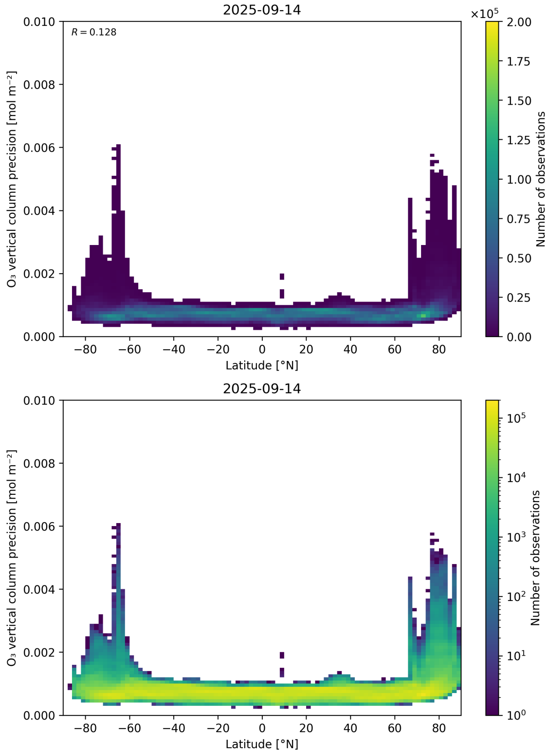
Figure 37: Scatter density plot of “Latitude” against “O 3 vertical column precision” for 2025-09-13 to 2025-09-15.
