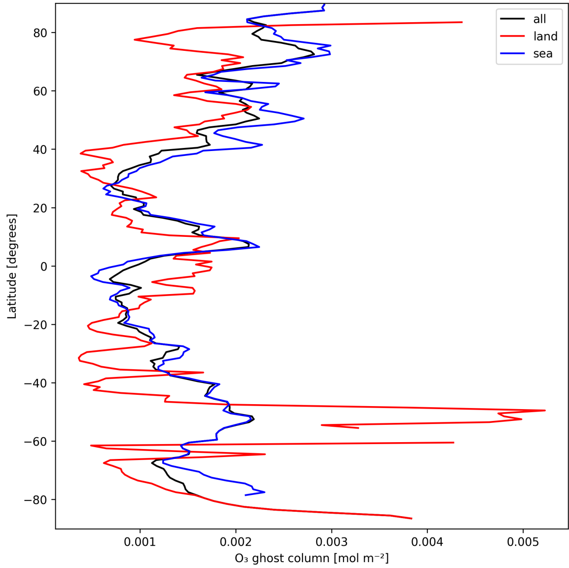
Figure 18: Zonal average of “O 3 ghost column” for 2025-09-13 to 2025-09-15.
