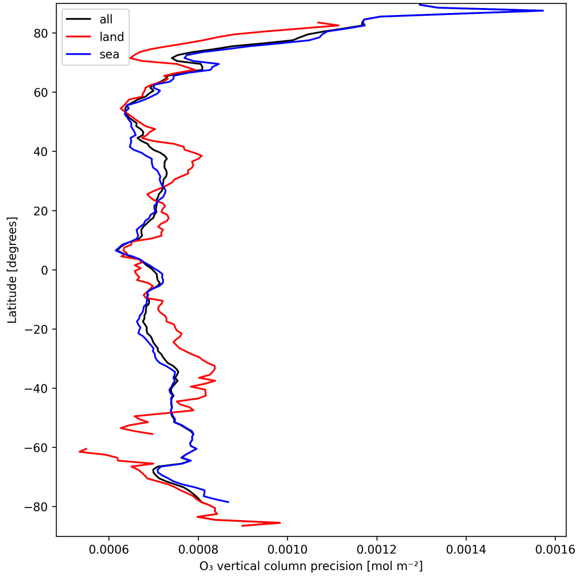
Figure 15: Zonal average of “O 3 vertical column precision” for 2025-09-13 to 2025-09-15.
