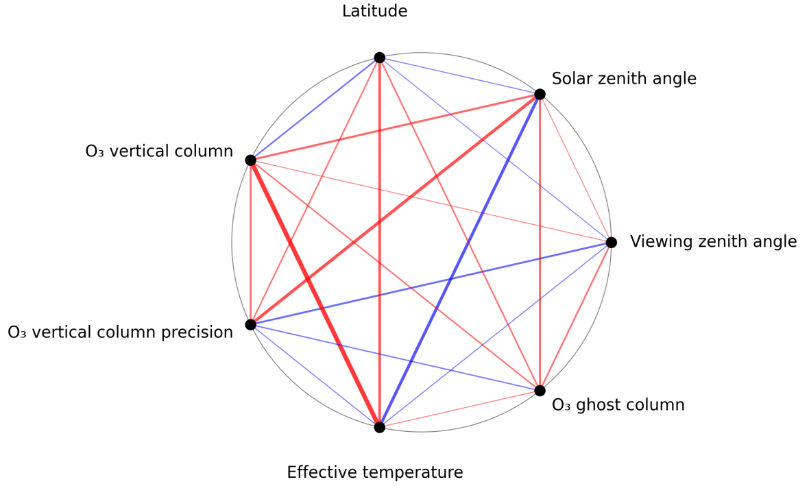
Figure 1: Map of correlation graph for 2025-09-16 to 2025-09-18.
