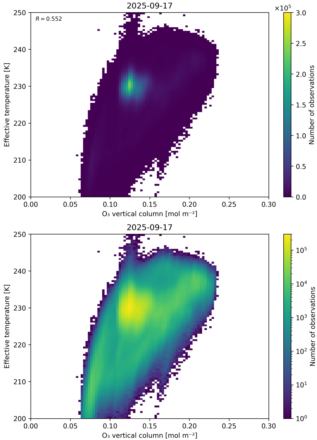
Figure 39: Scatter density plot of “O 3 vertical column” against “Effective temperature” for 2025-09-16 to 2025-09-18.
