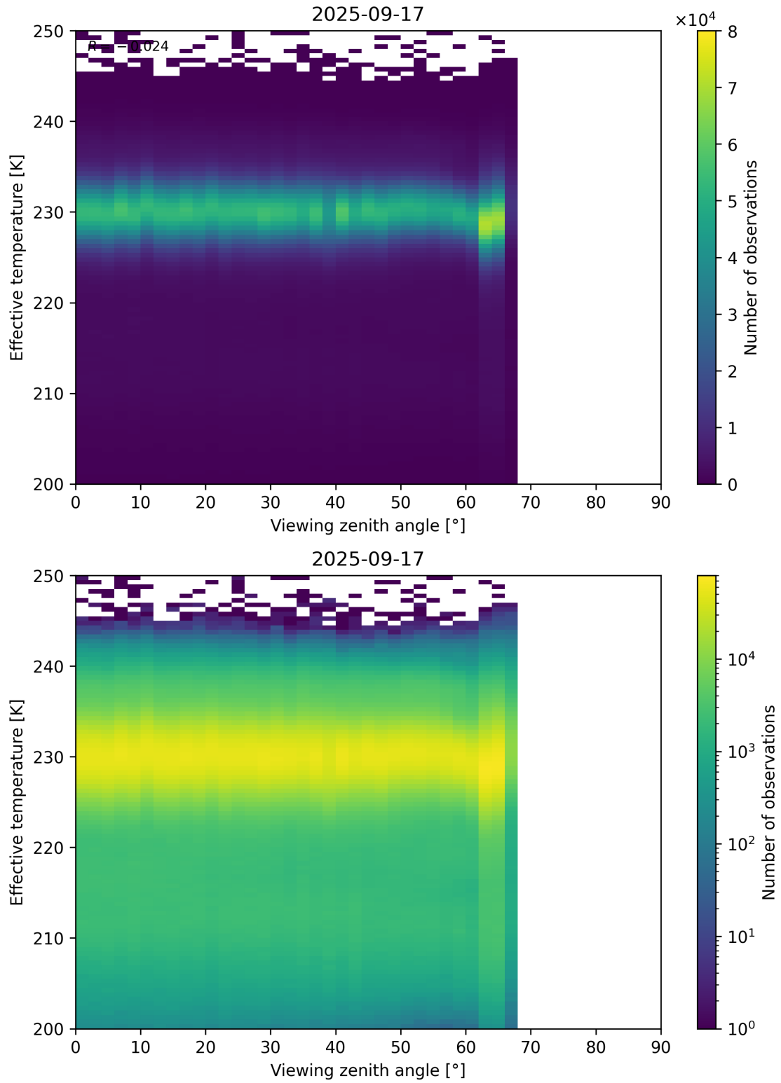
Figure 50: Scatter density plot of “Viewing zenith angle” against “Effective temperature” for 2025-09-16 to 2025-09-18.
