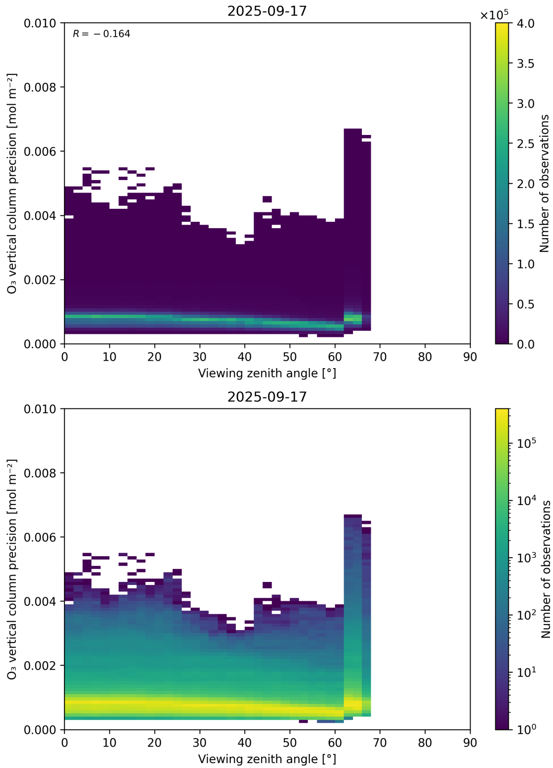
Figure 53: Scatter density plot of “Viewing zenith angle” against “O 3 vertical column precision” for 2025-09-16 to 2025-09-18.
