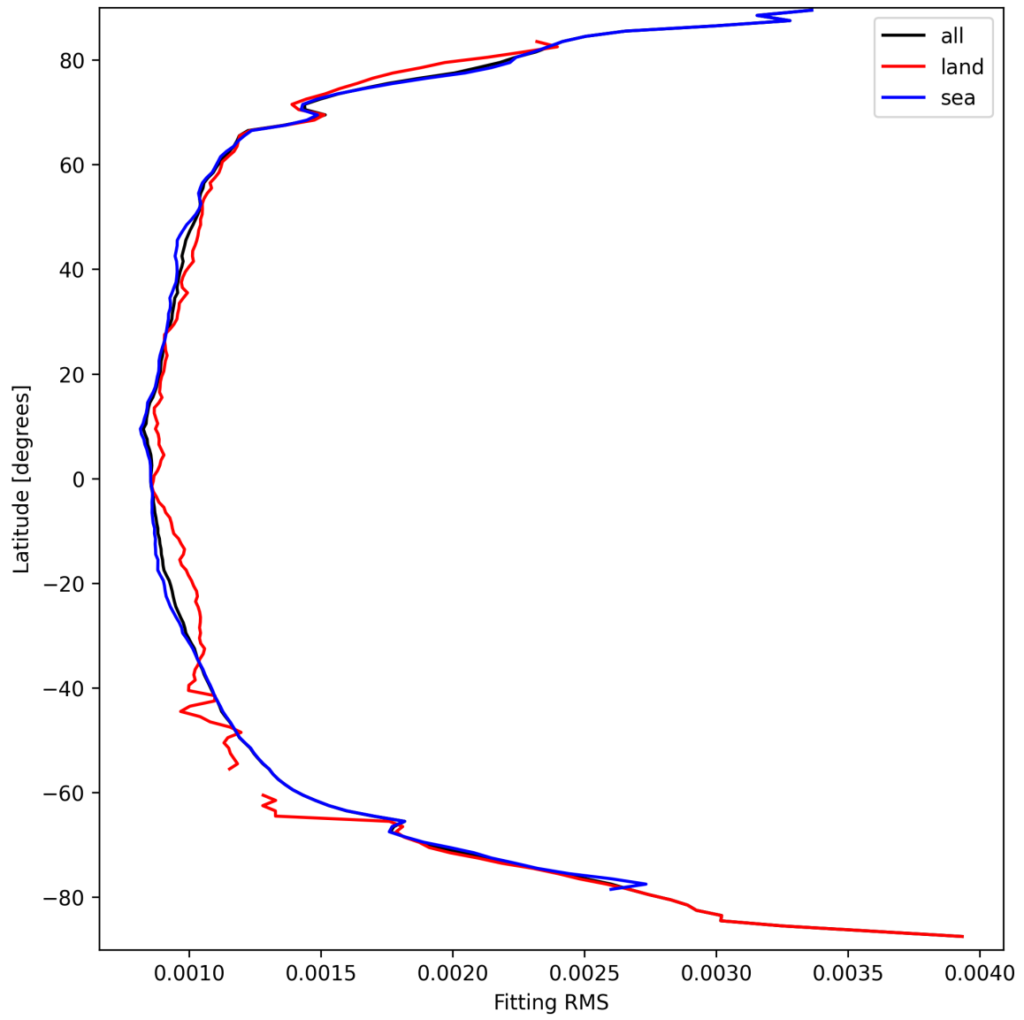
Figure 16: Zonal average of “Fitting RMS” for 2025-09-16 to 2025-09-18.
