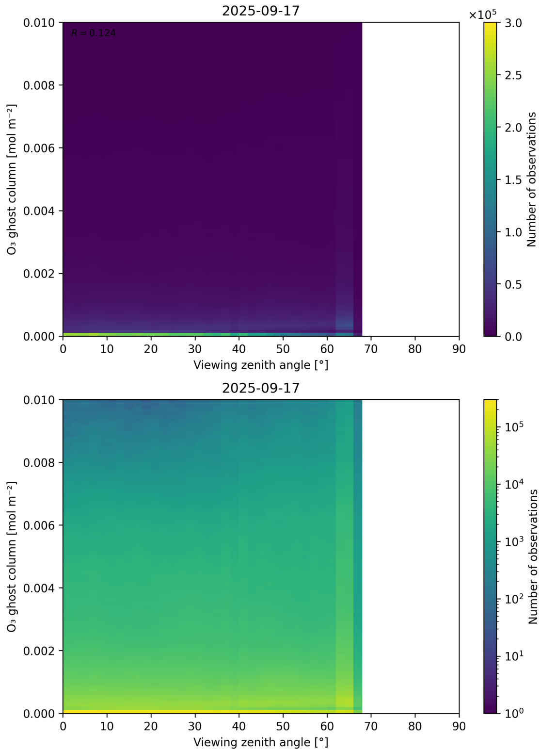
Figure 51: Scatter density plot of “Viewing zenith angle” against “O 3 ghost column” for 2025-09-16 to 2025-09-18.
