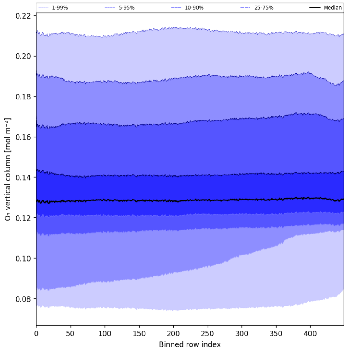
Figure 28: Along track statistics of “O 3 vertical column” for 2025-09-16 to 2025-09-18
