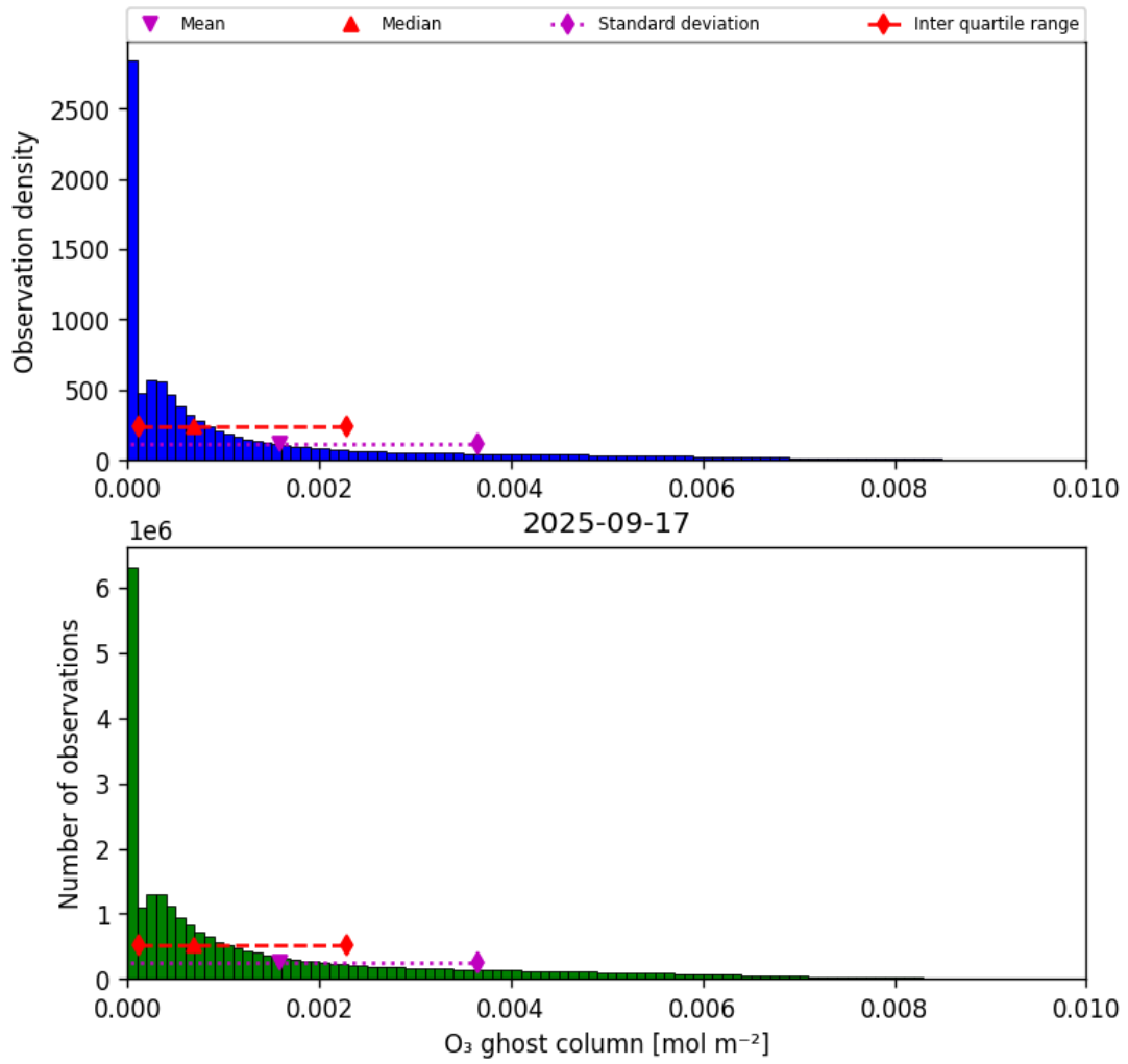
Figure 25: Histogram of “O 3 ghost column” for 2025-09-16 to 2025-09-18
