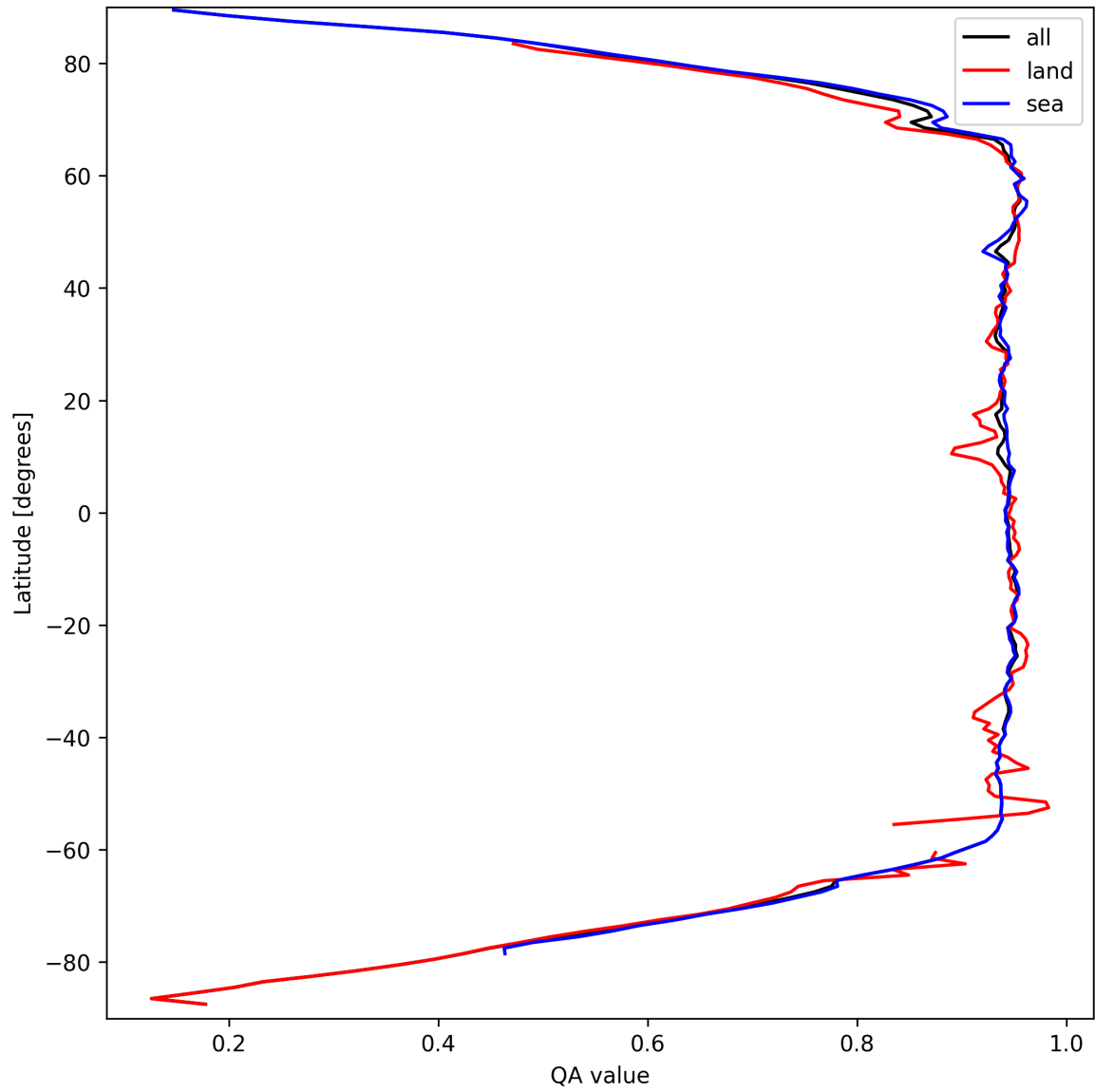
Figure 13: Zonal average of “QA value” for 2025-09-16 to 2025-09-18.
