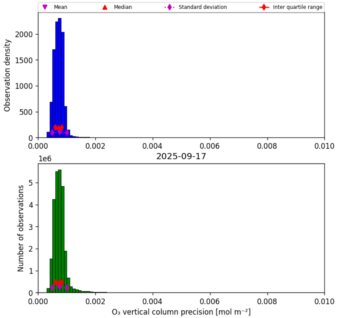
Figure 22: Histogram of “O 3 vertical column precision” for 2025-09-16 to 2025-09-18
