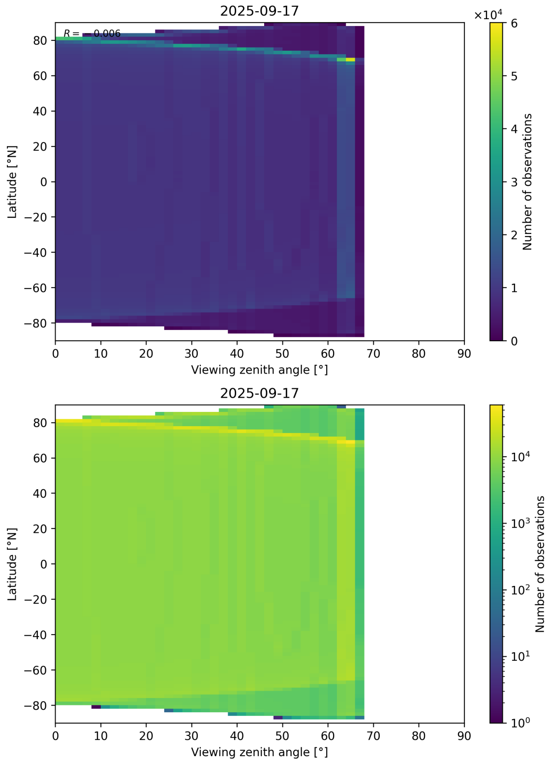
Figure 49: Scatter density plot of “Viewing zenith angle” against “Latitude” for 2025-09-16 to 2025-09-18.
