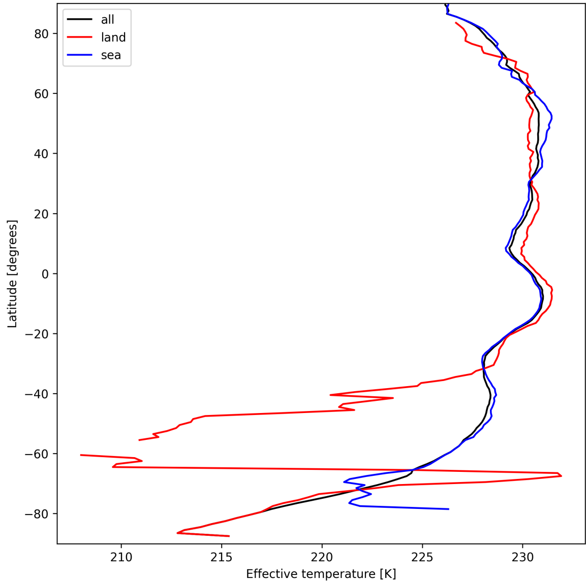
Figure 17: Zonal average of “Effective temperature” for 2025-09-16 to 2025-09-18.
