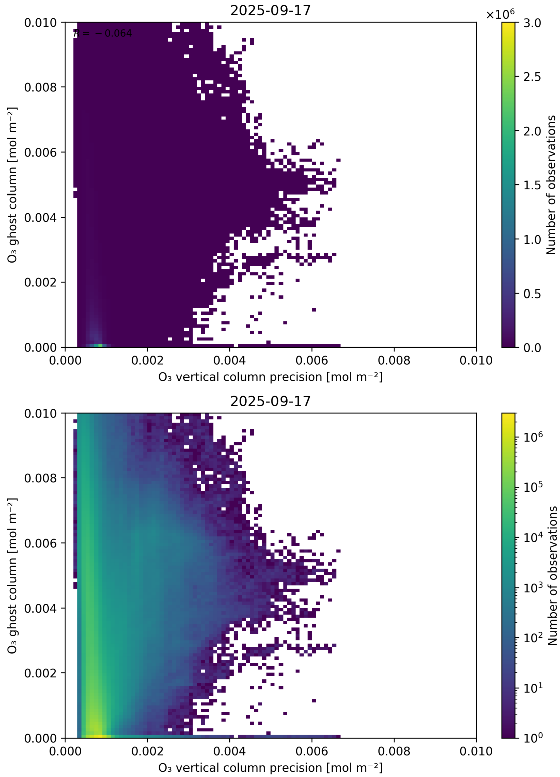
Figure 43: Scatter density plot of “O 3 vertical column precision” against “O 3 ghost column” for 2025-09-16 to 2025-09-18.
