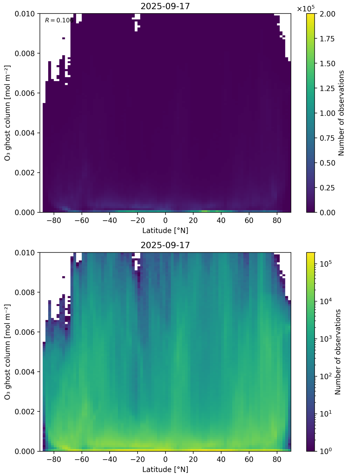
Figure 35: Scatter density plot of “Latitude” against “O 3 ghost column” for 2025-09-16 to 2025-09-18.
