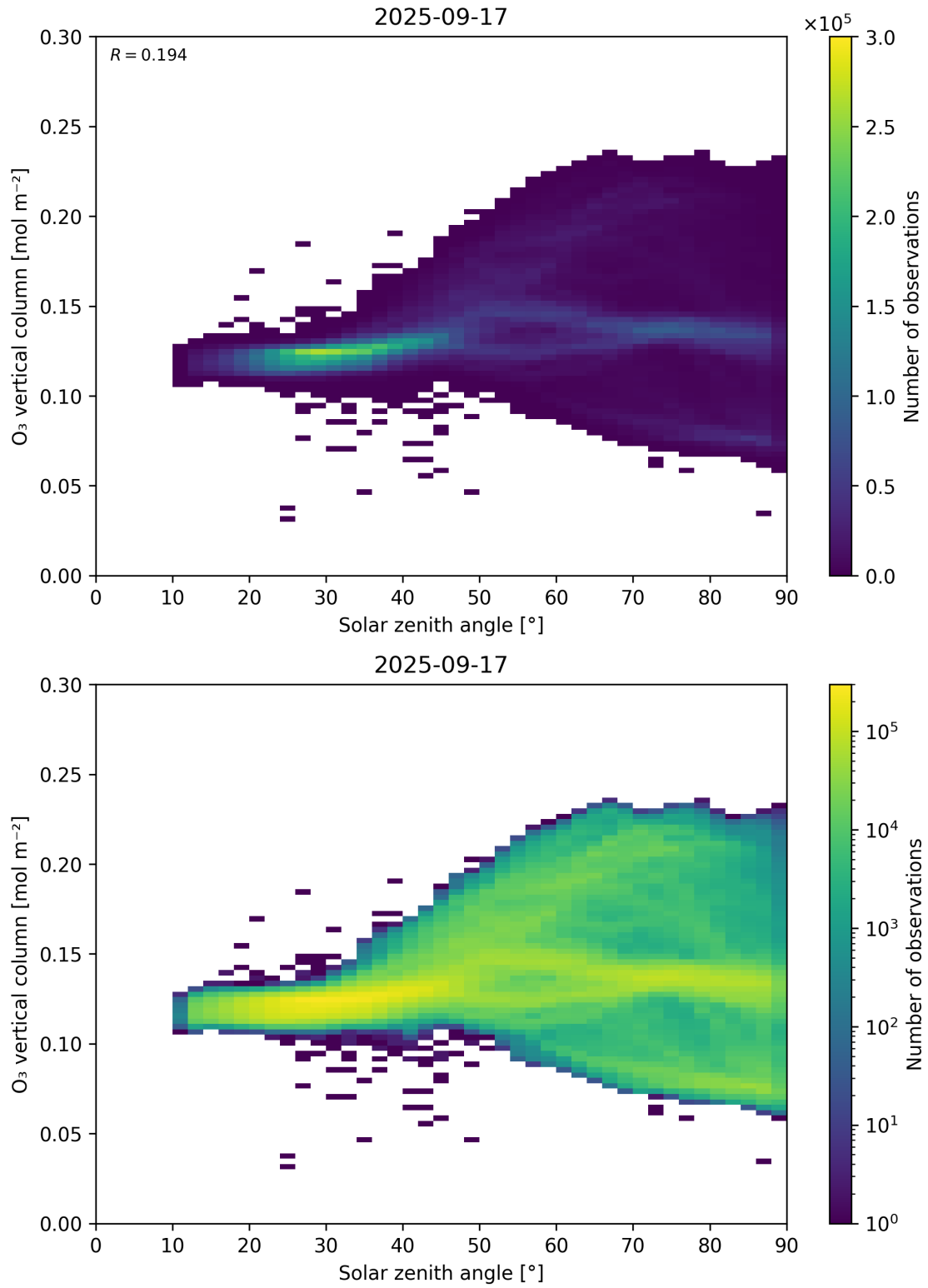
Figure 47: Scatter density plot of “Solar zenith angle” against “O 3 vertical column” for 2025-09-16 to 2025-09-18.
