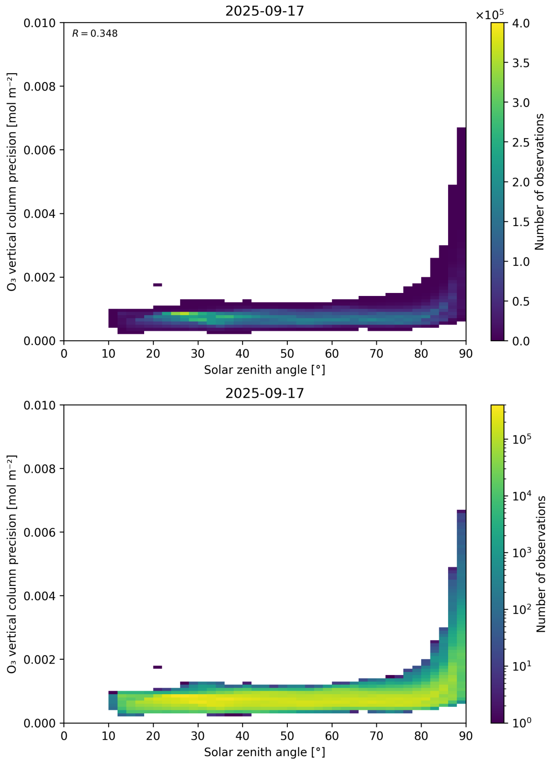
Figure 48: Scatter density plot of “Solar zenith angle” against “O 3 vertical column precision” for 2025-09-16 to 2025-09-18.
