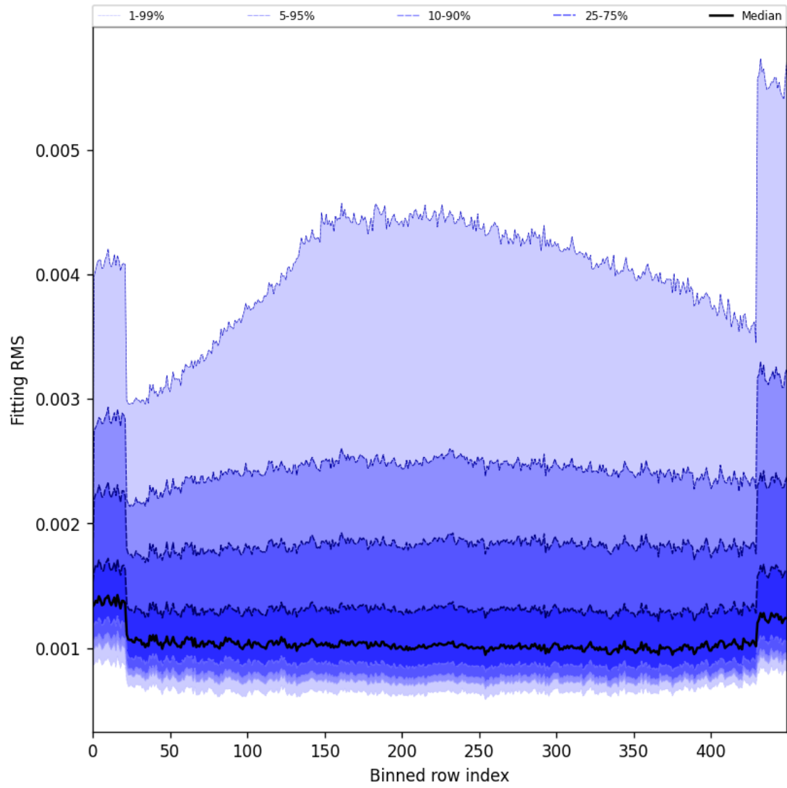
Figure 30: Along track statistics of “Fitting RMS” for 2025-09-16 to 2025-09-18
