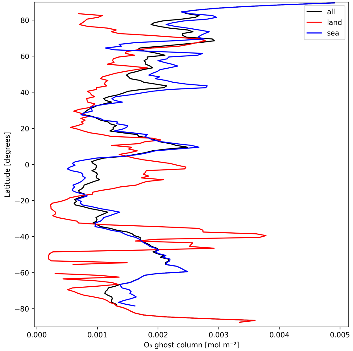
Figure 18: Zonal average of “O 3 ghost column” for 2025-09-16 to 2025-09-18.
