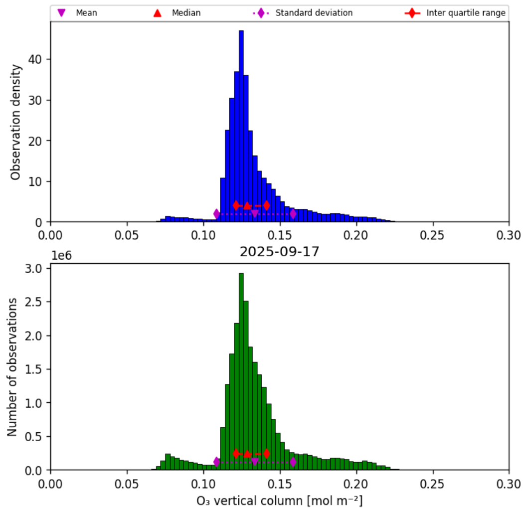
Figure 21: Histogram of “O 3 vertical column” for 2025-09-16 to 2025-09-18
