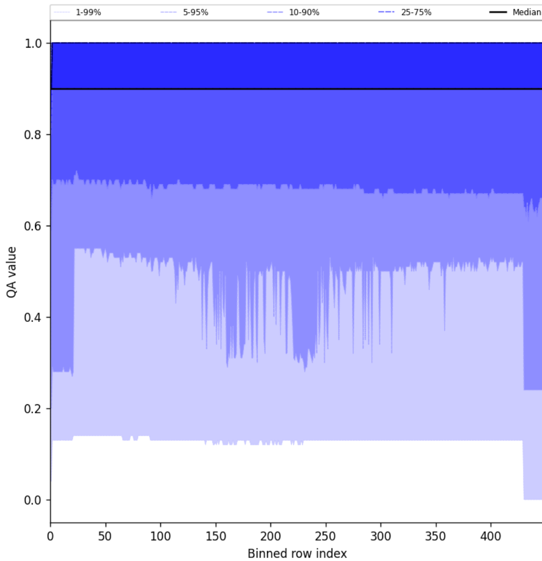
Figure 27: Along track statistics of “QA value” for 2025-09-16 to 2025-09-18
