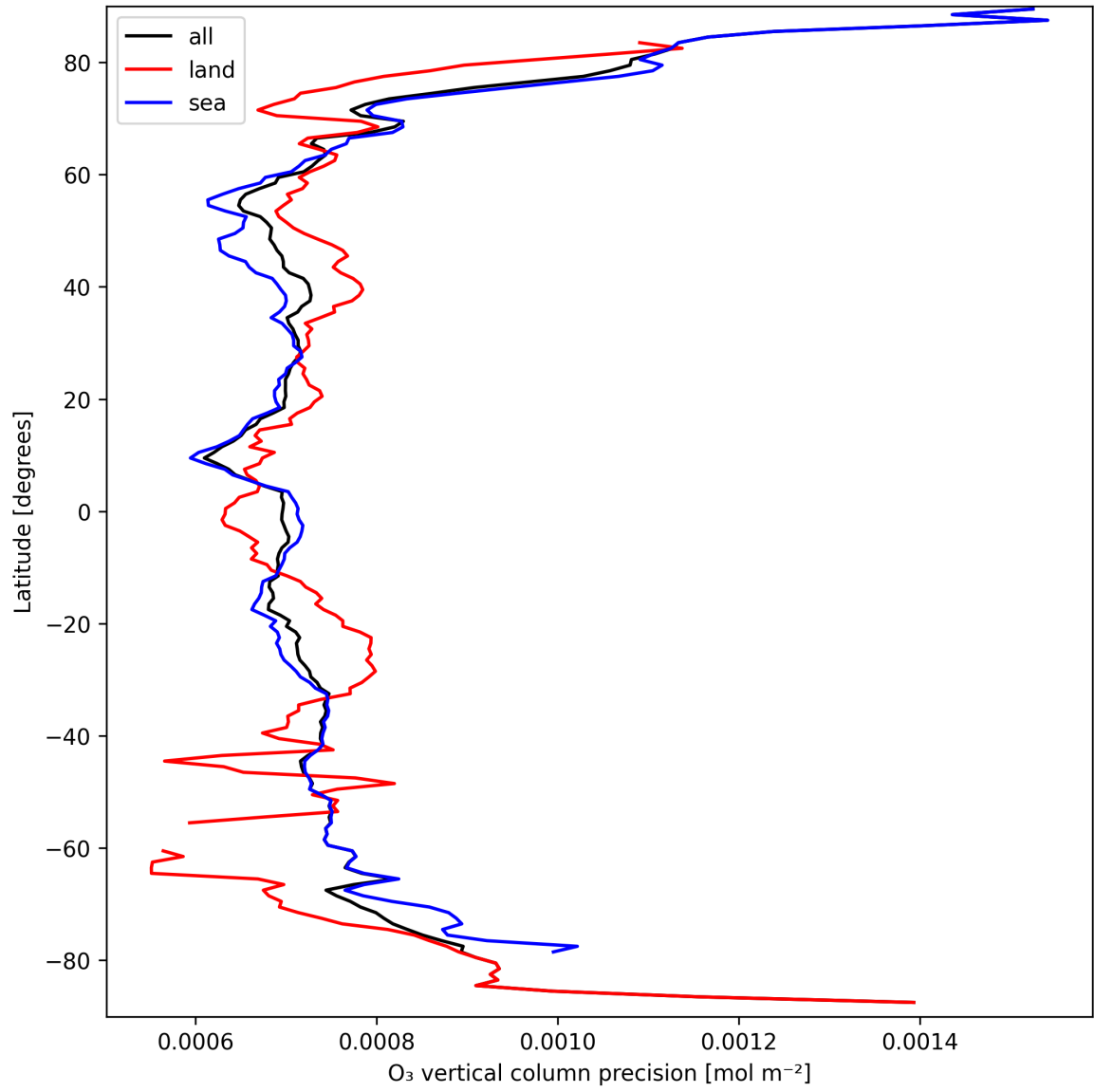
Figure 15: Zonal average of "O 3 vertical column precision" for 2025-09-16 to 2025-09-18.
