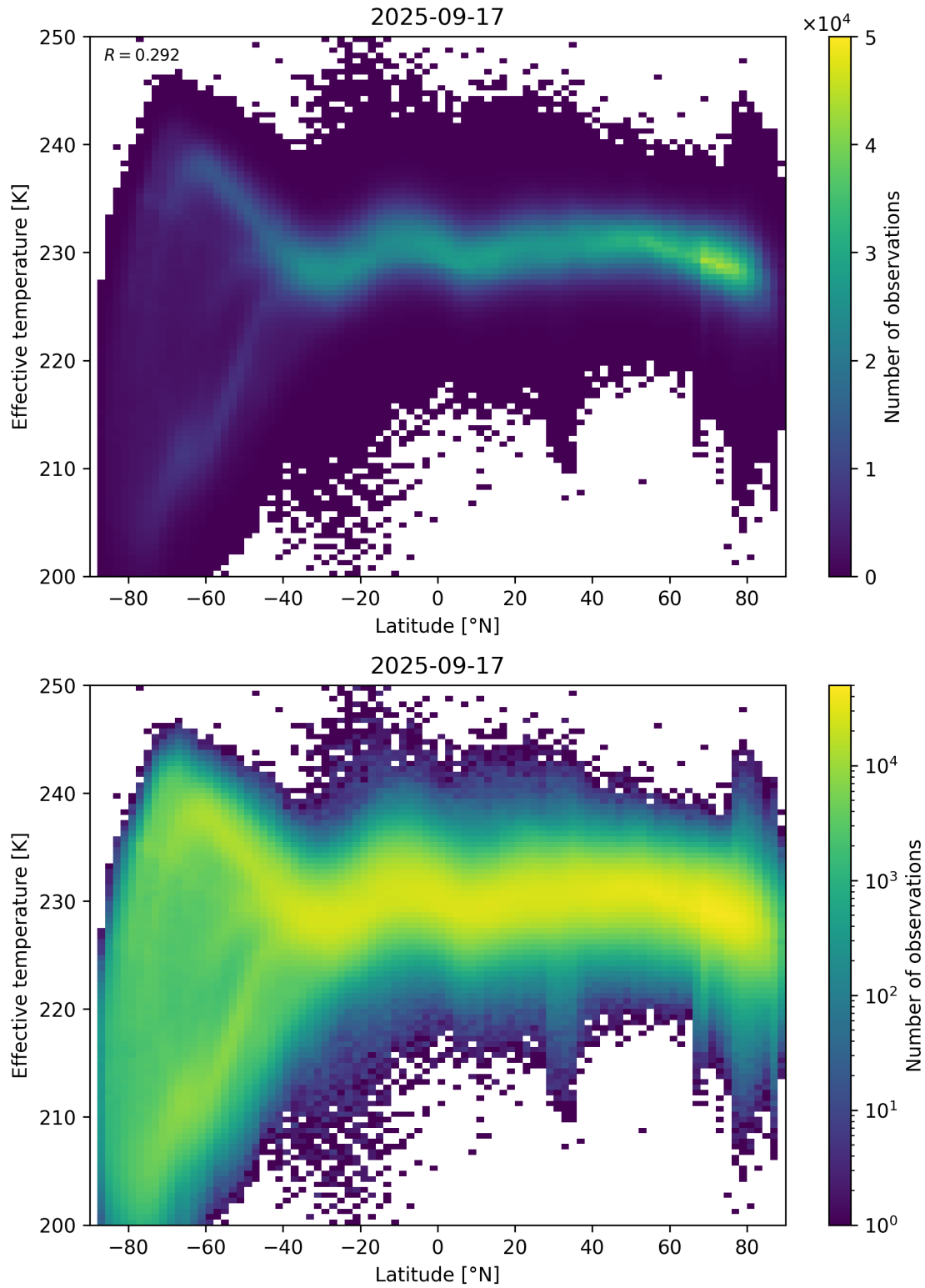
Figure 34: Scatter density plot of “Latitude” against “Effective temperature” for 2025-09-16 to 2025-09-18.
