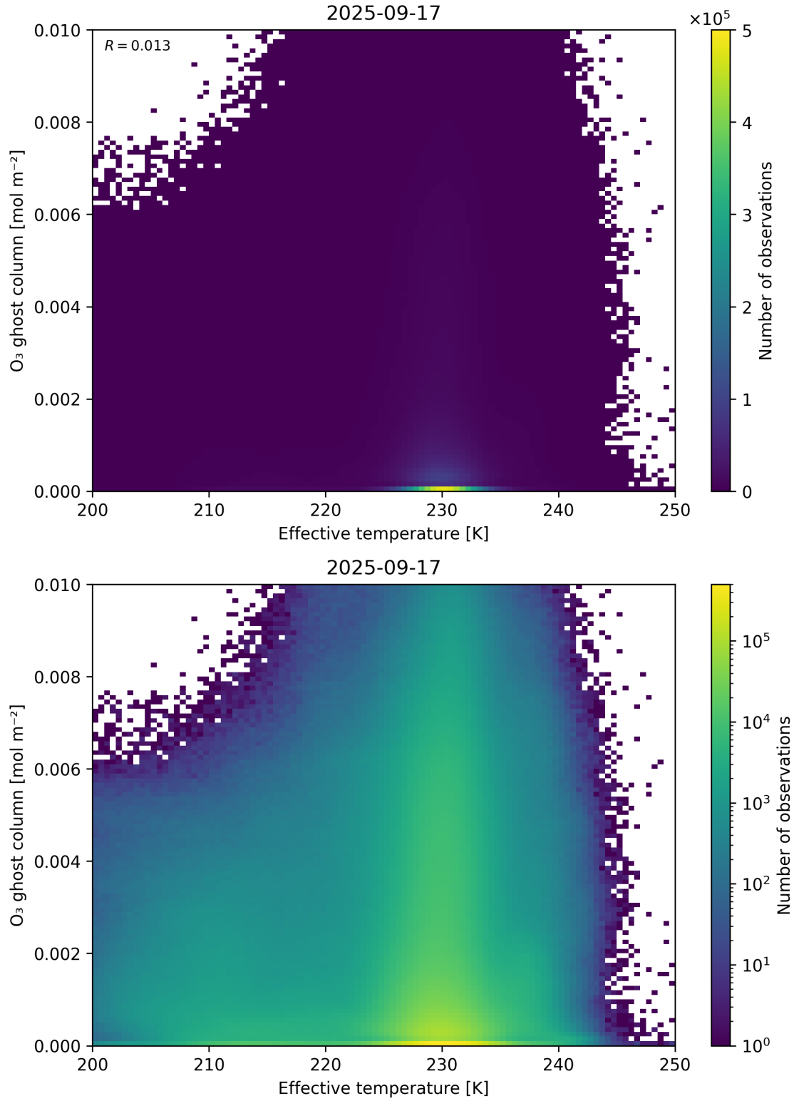
Figure 38: Scatter density plot of “Effective temperature” against “O 3 ghost column” for 2025-09-16 to 2025-09-18.
