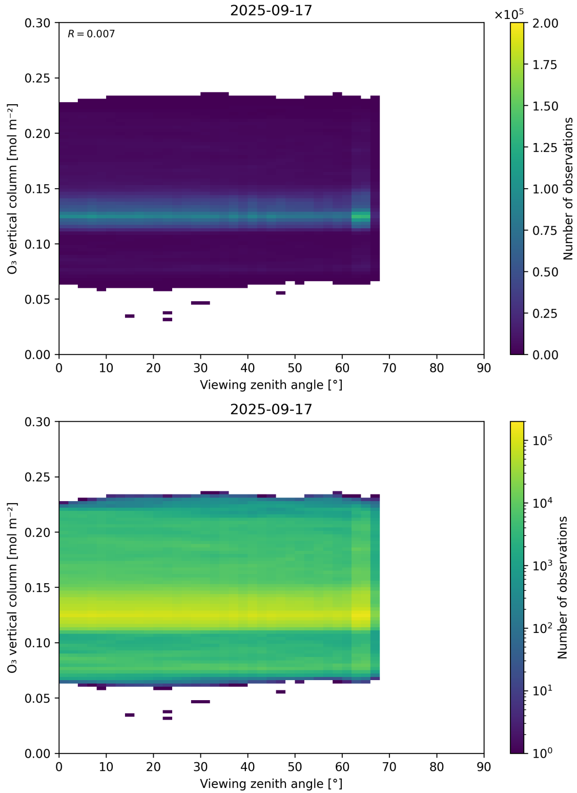
Figure 52: Scatter density plot of “Viewing zenith angle” against “O 3 vertical column” for 2025-09-16 to 2025-09-18.
