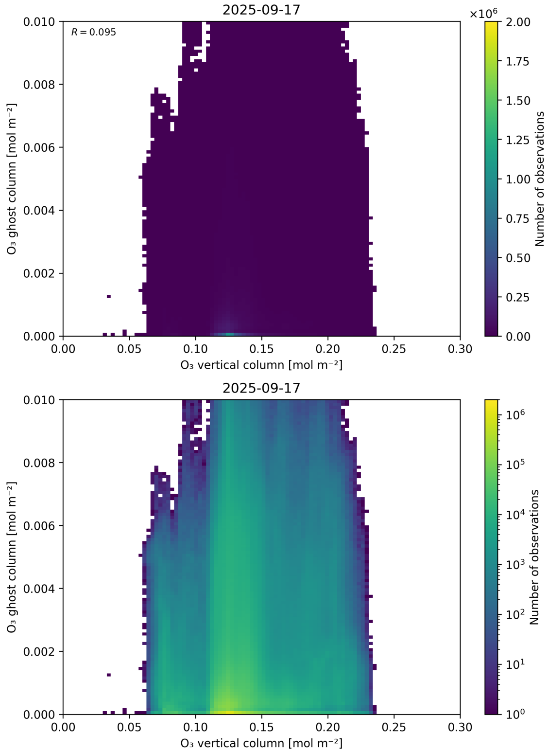
Figure 40: Scatter density plot of “O 3 vertical column” against “O 3 ghost column” for 2025-09-16 to 2025-09-18.
