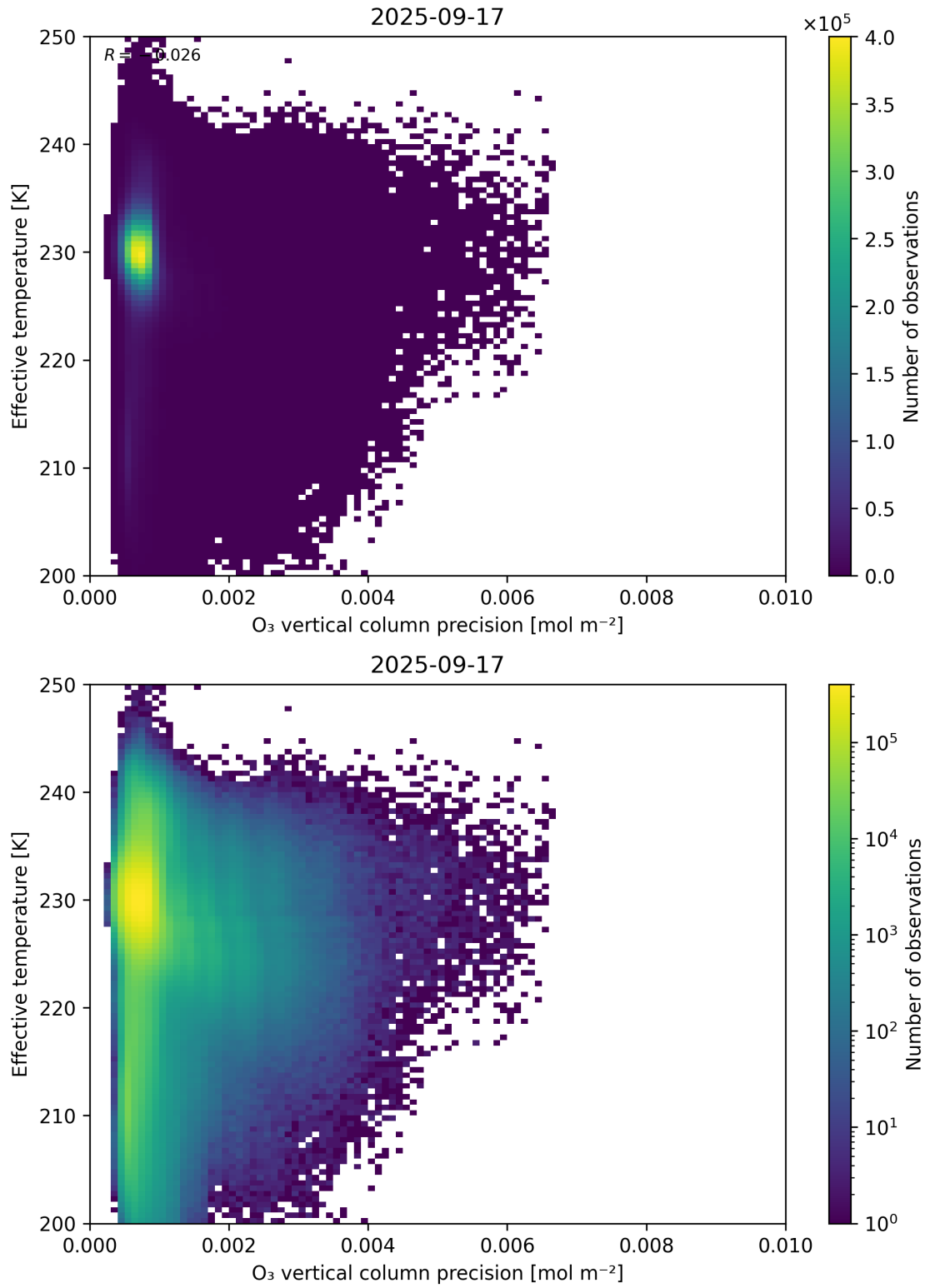
Figure 42: Scatter density plot of “O 3 vertical column precision” against “Effective temperature” for 2025-09-16 to 2025-09-18.
