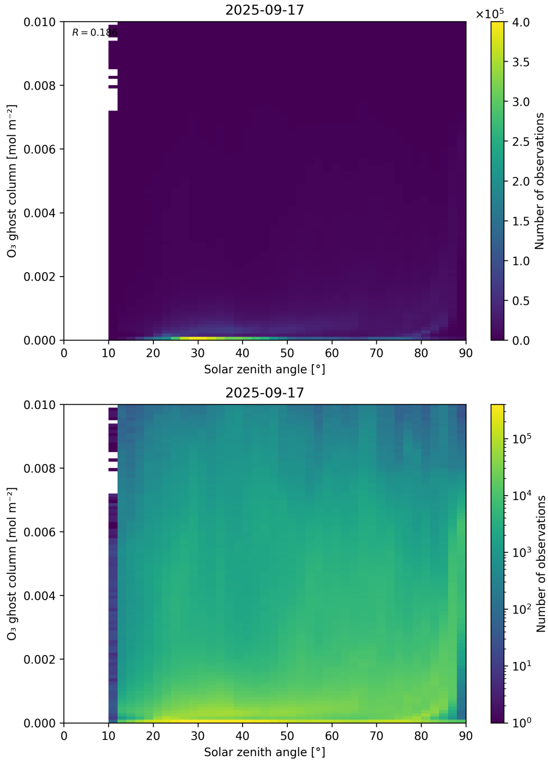
Figure 46: Scatter density plot of “Solar zenith angle” against “O 3 ghost column” for 2025-09-16 to 2025-09-18.
