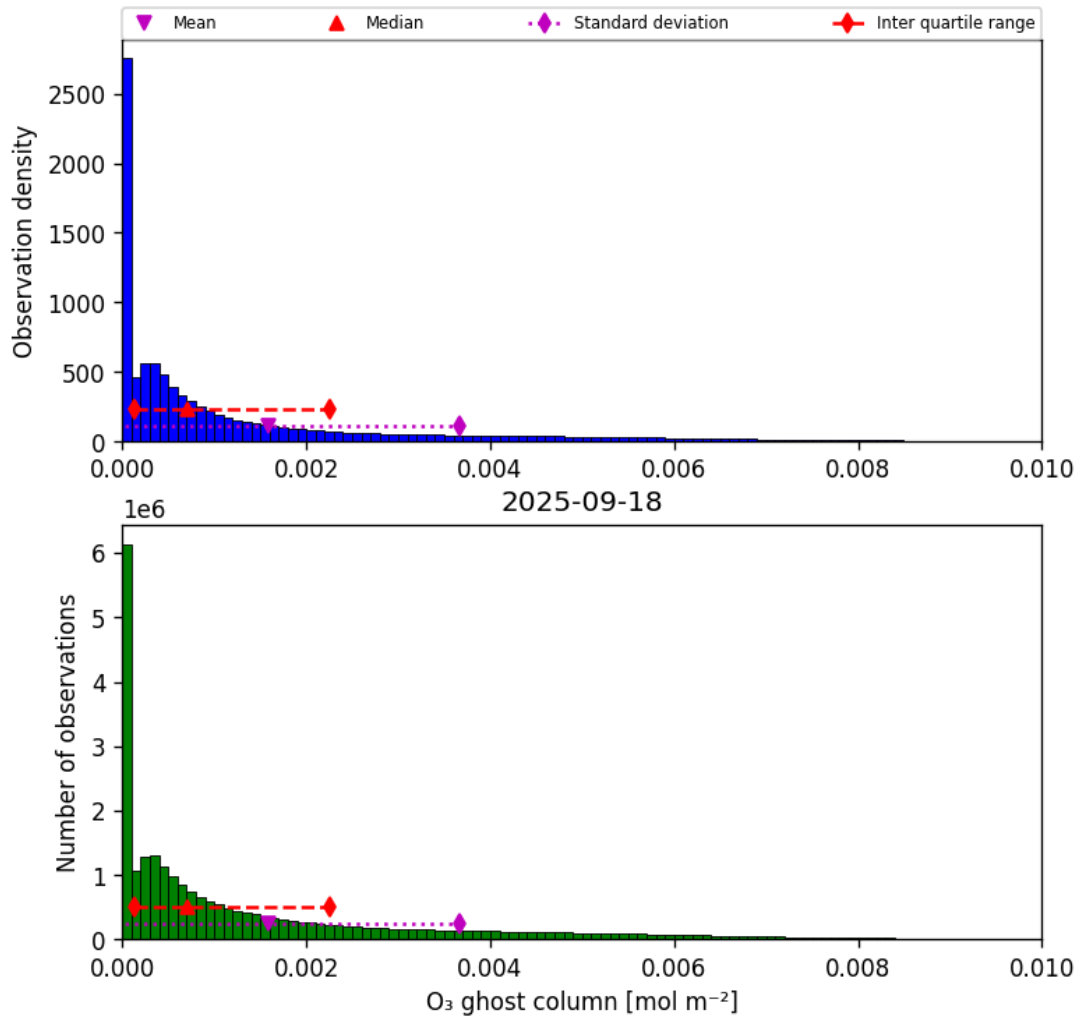
Figure 25: Histogram of “O 3 ghost column” for 2025-09-17 to 2025-09-19
