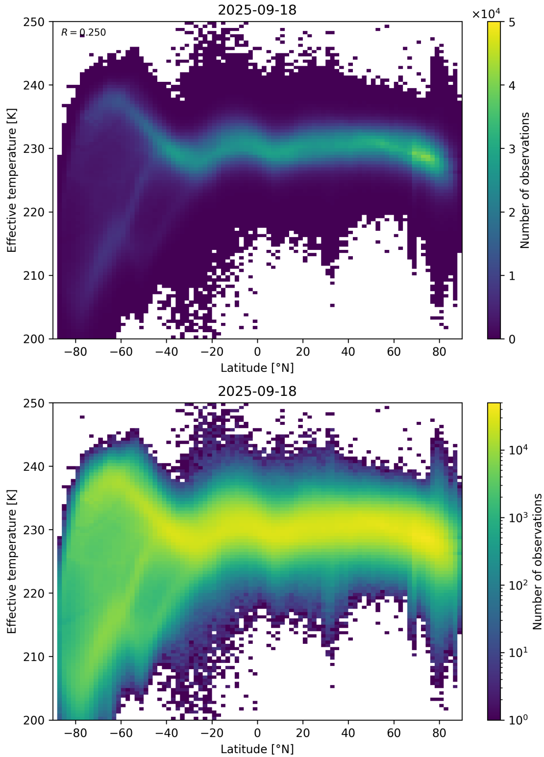
Figure 34: Scatter density plot of “Latitude” against “Effective temperature” for 2025-09-17 to 2025-09-19.
