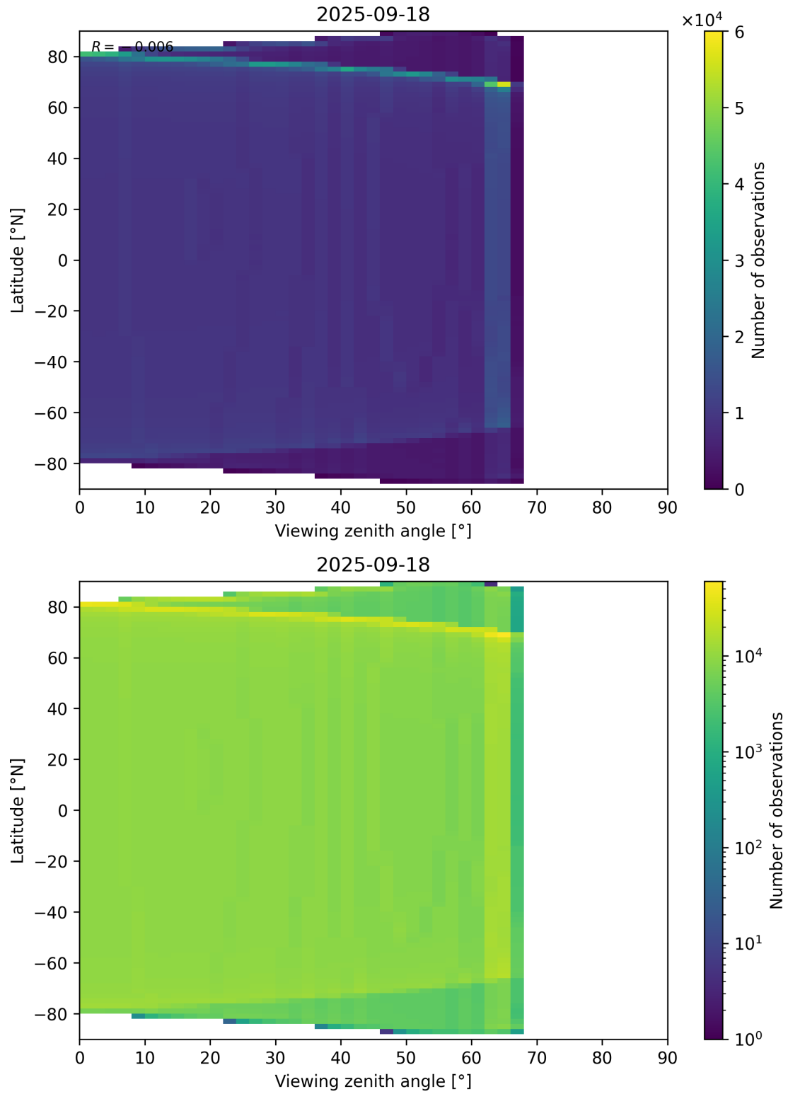
Figure 49: Scatter density plot of “Viewing zenith angle” against “Latitude” for 2025-09-17 to 2025-09-19.
