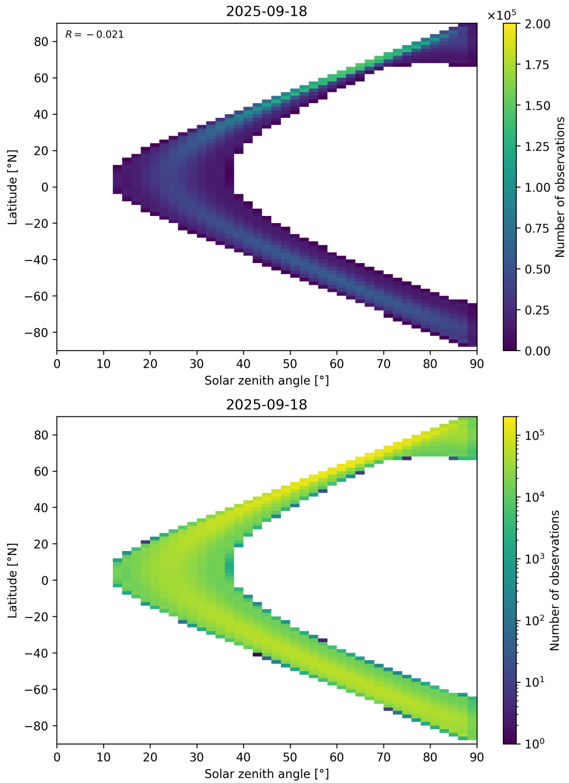
Figure 44: Scatter density plot of “Solar zenith angle” against “Latitude” for 2025-09-17 to 2025-09-19.
