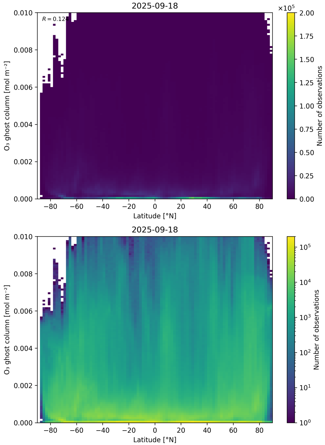
Figure 35: Scatter density plot of “Latitude” against “O 3 ghost column” for 2025-09-17 to 2025-09-19.
