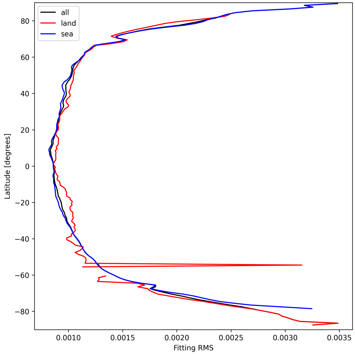
Figure 16: Zonal average of “Fitting RMS” for 2025-09-17 to 2025-09-19.
