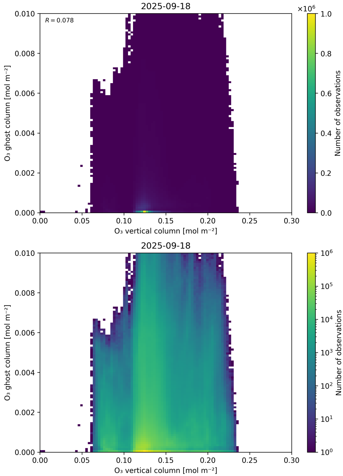
Figure 40: Scatter density plot of “O 3 vertical column” against “O 3 ghost column” for 2025-09-17 to 2025-09-19.
