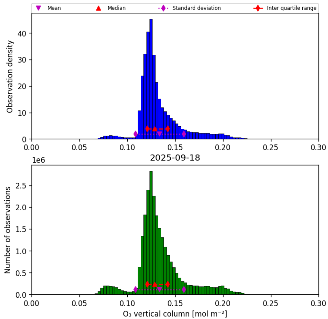
Figure 21: Histogram of “O 3 vertical column” for 2025-09-17 to 2025-09-19
