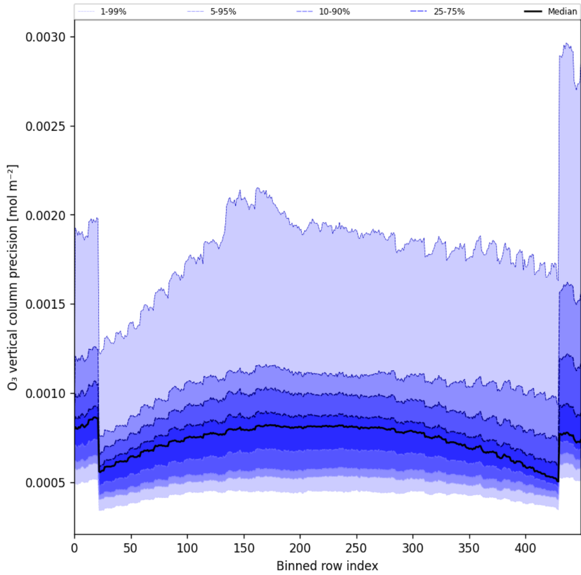
Figure 29: Along track statistics of “O 3 vertical column precision” for 2025-09-17 to 2025-09-19
