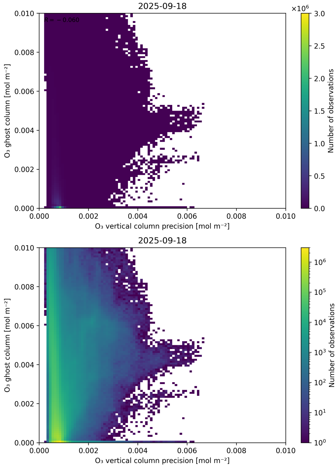
Figure 43: Scatter density plot of “ \text{O}_3 vertical column precision” against “ \text{O}_3 ghost column” for 2025-09-17 to 2025-09-19.
