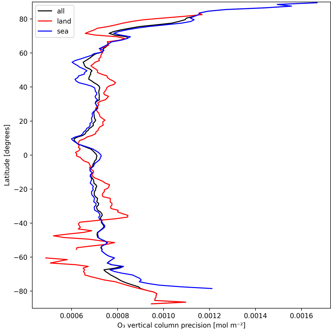
Figure 15: Zonal average of “O 3 vertical column precision” for 2025-09-17 to 2025-09-19.
