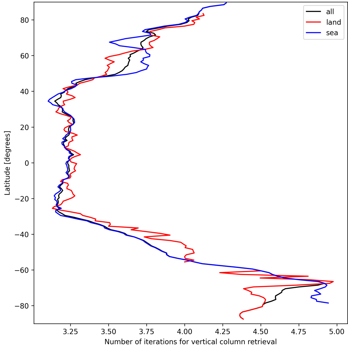
Figure 19: Zonal average of “Number of iterations for vertical column retrieval” for 2025-09-17 to 2025-09-19.
