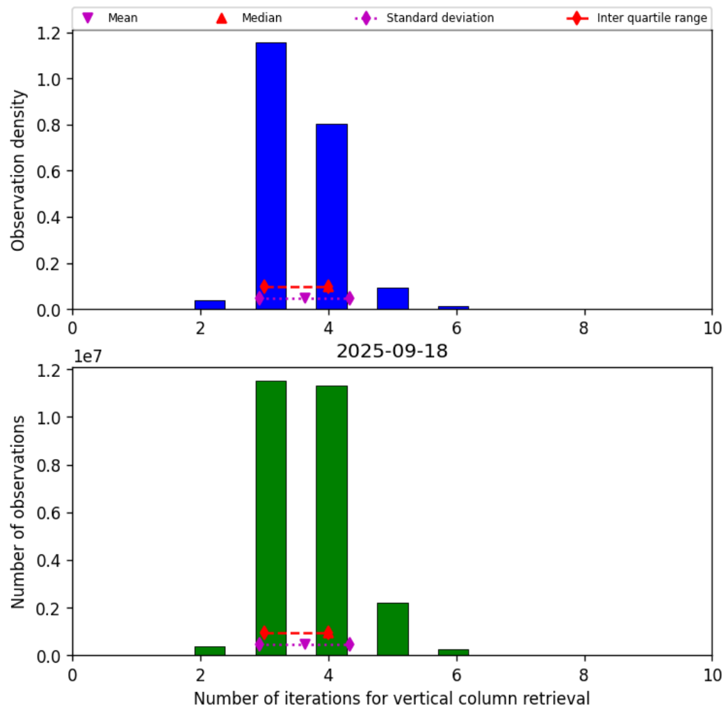
Figure 26: Histogram of “Number of iterations for vertical column retrieval” for 2025-09-17 to 2025-09-19
