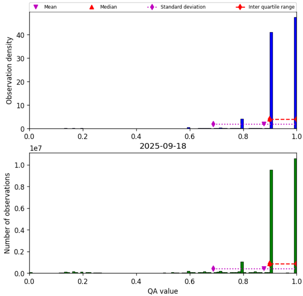
Figure 20: Histogram of “QA value” for 2025-09-17 to 2025-09-19
