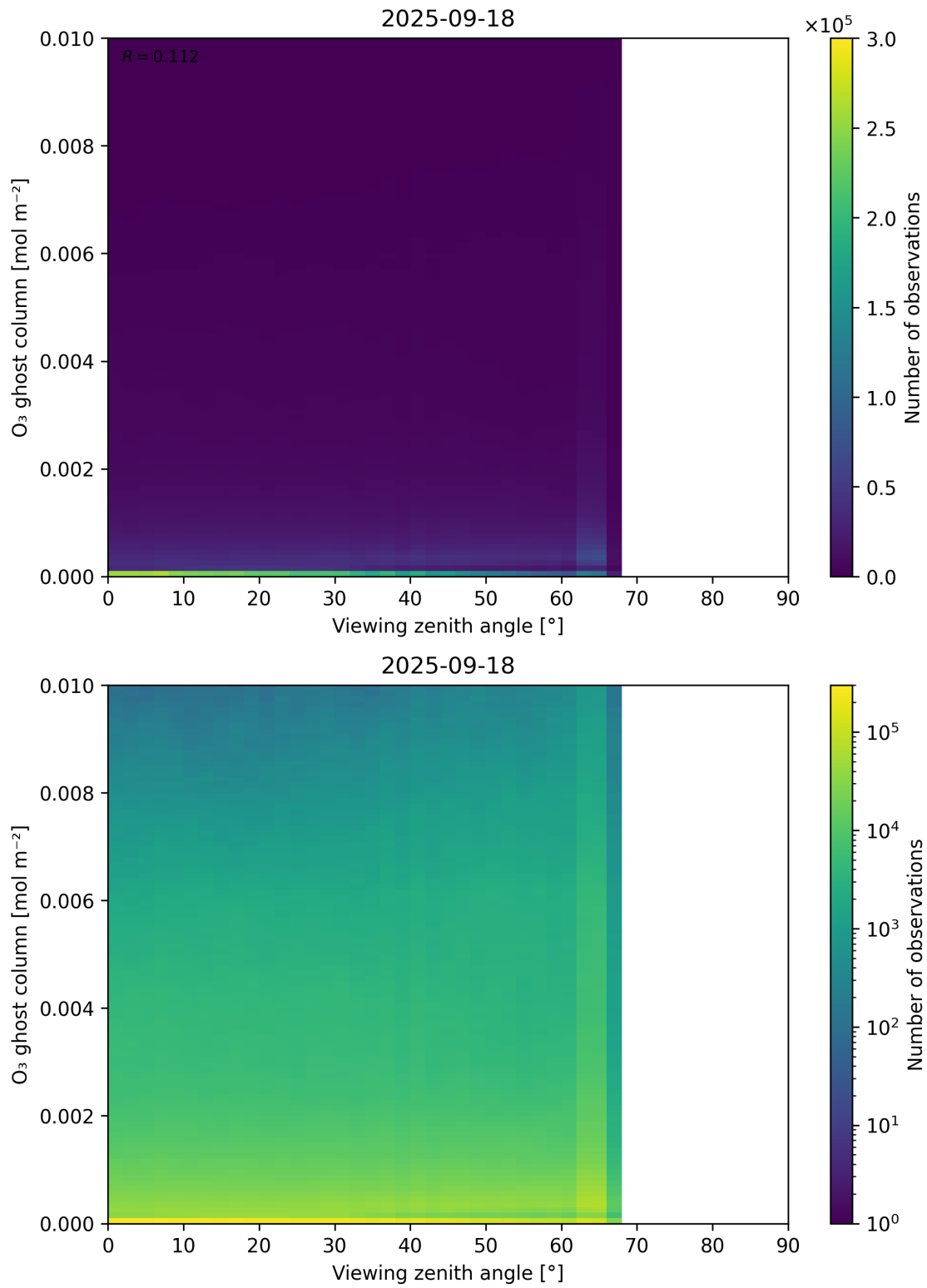
Figure 51: Scatter density plot of “Viewing zenith angle” against “O 3 ghost column” for 2025-09-17 to 2025-09-19.
