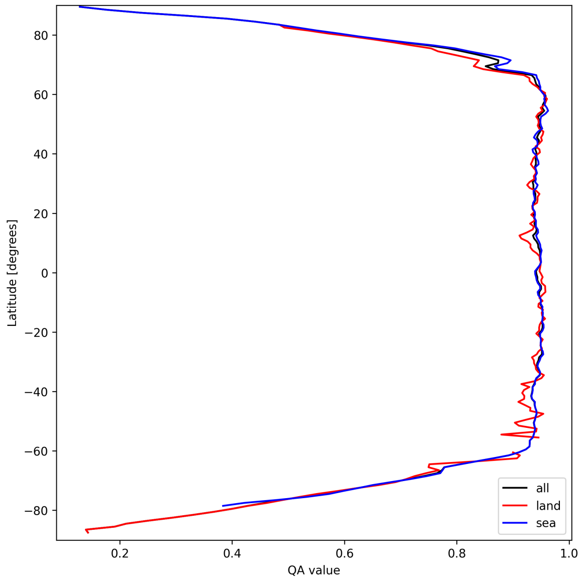
Figure 13: Zonal average of “QA value” for 2025-09-17 to 2025-09-19.
