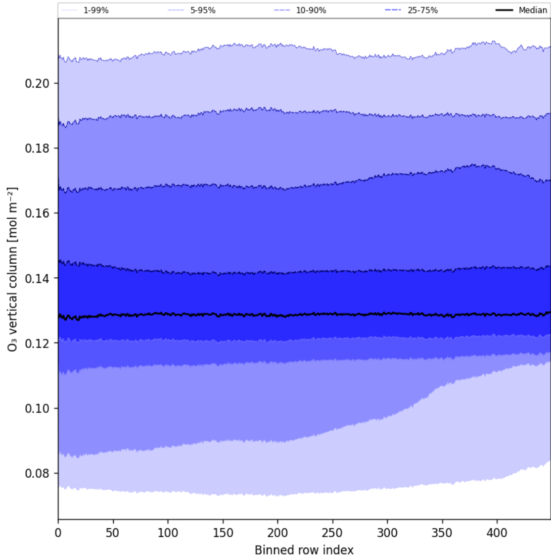
Figure 28: Along track statistics of “O 3 vertical column” for 2025-09-17 to 2025-09-19
