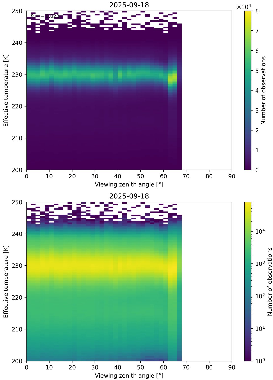
Figure 50: Scatter density plot of “Viewing zenith angle” against “Effective temperature” for 2025-09-17 to 2025-09-19.
