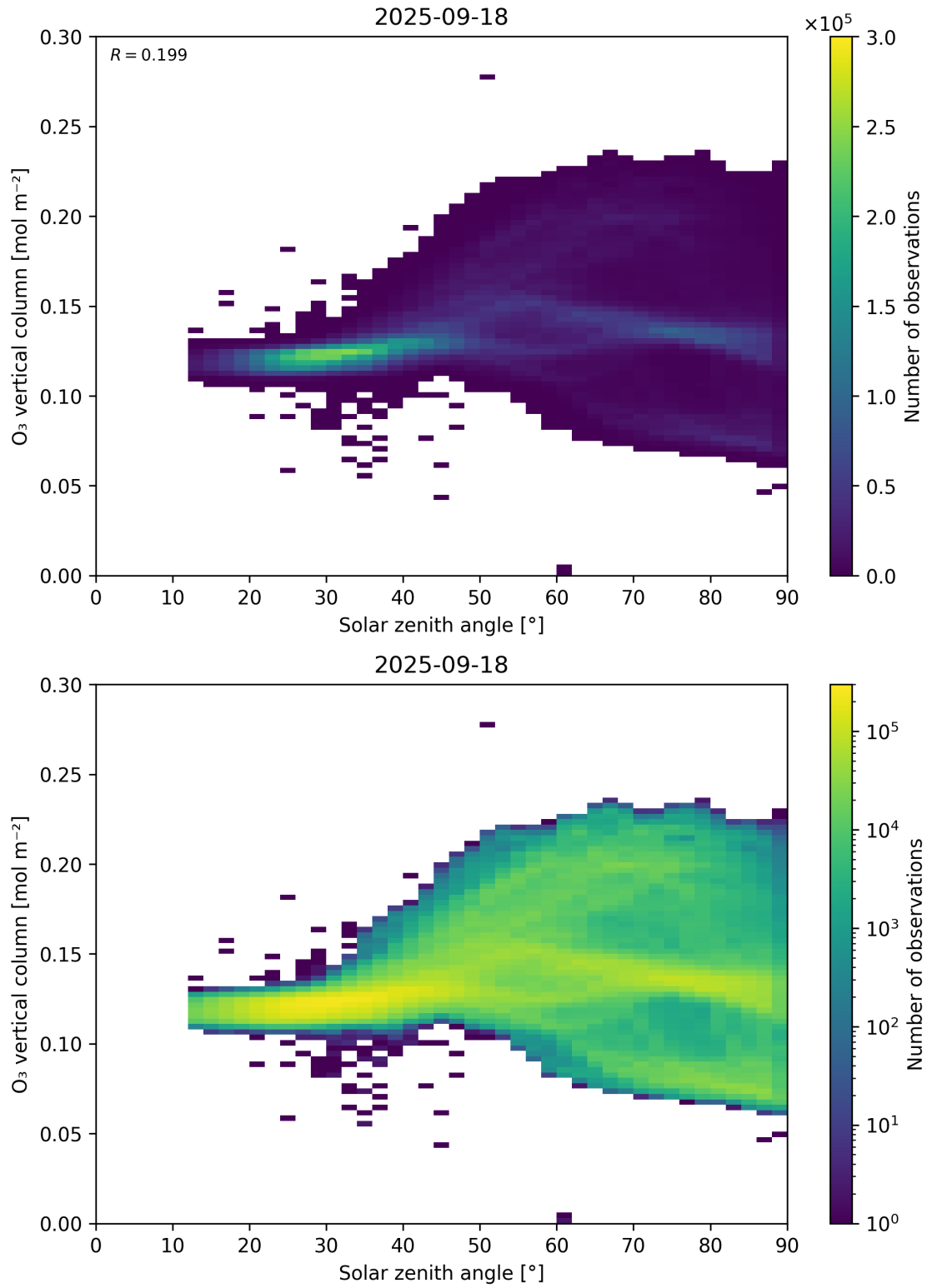
Figure 47: Scatter density plot of “Solar zenith angle” against “O 3 vertical column” for 2025-09-17 to 2025-09-19.
