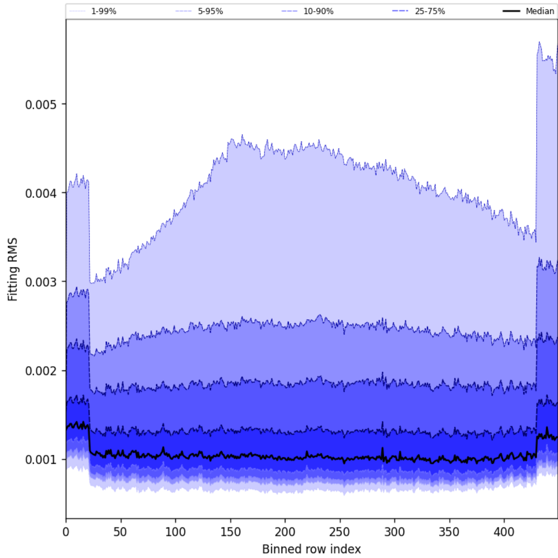
Figure 30: Along track statistics of “Fitting RMS” for 2025-09-17 to 2025-09-19
