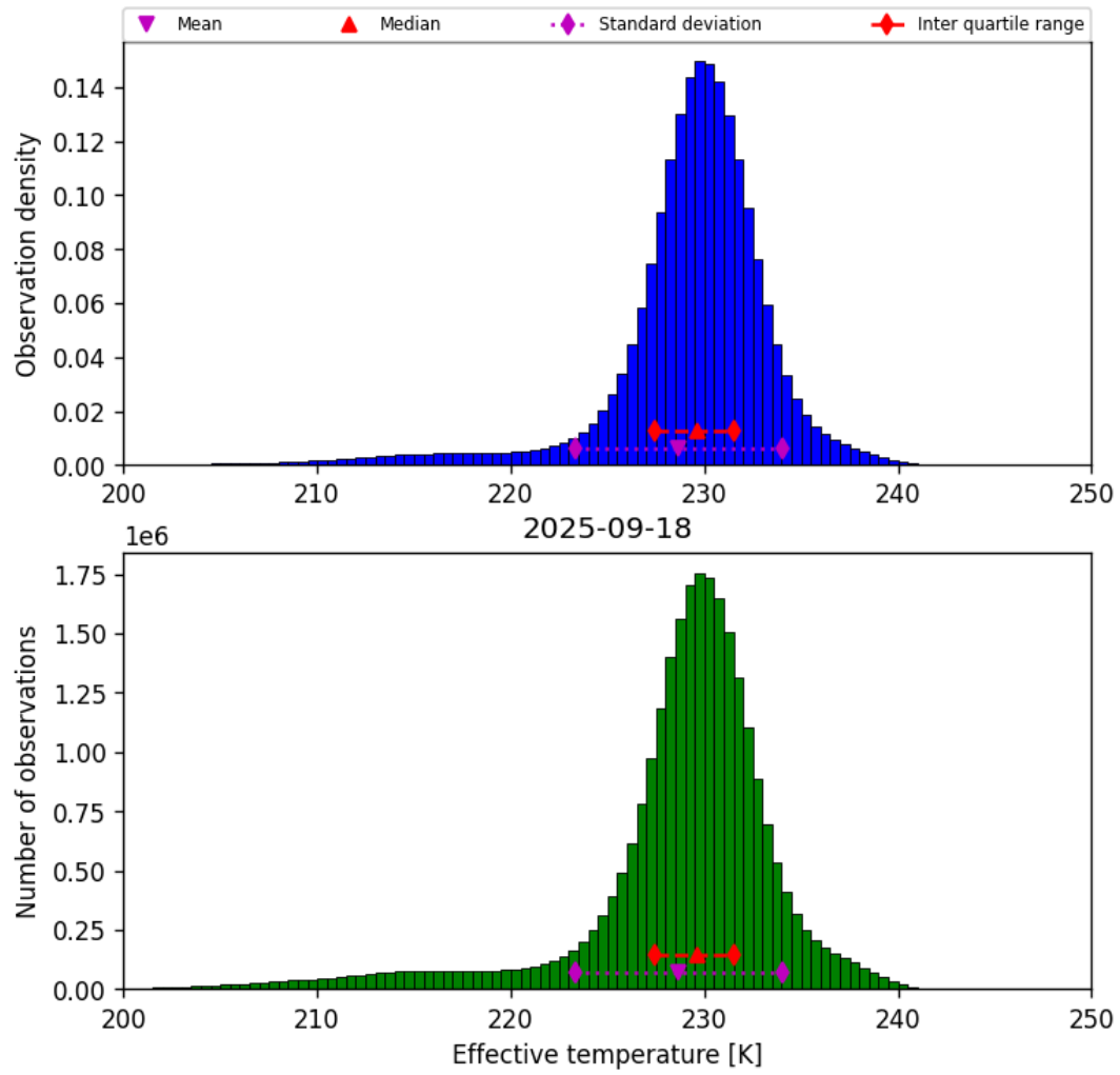
Figure 24: Histogram of “Effective temperature” for 2025-09-17 to 2025-09-19
