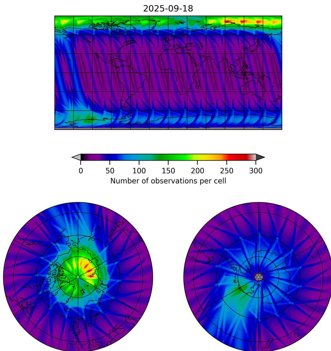
Figure 12: Map of the number of observations for 2025-09-17 to 2025-09-19
