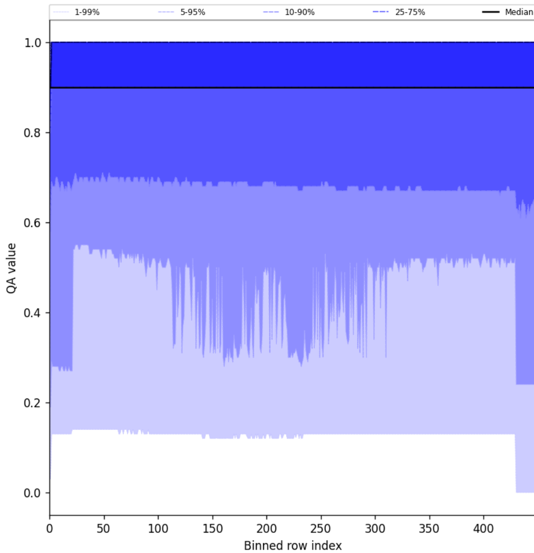
Figure 27: Along track statistics of “QA value” for 2025-09-17 to 2025-09-19
