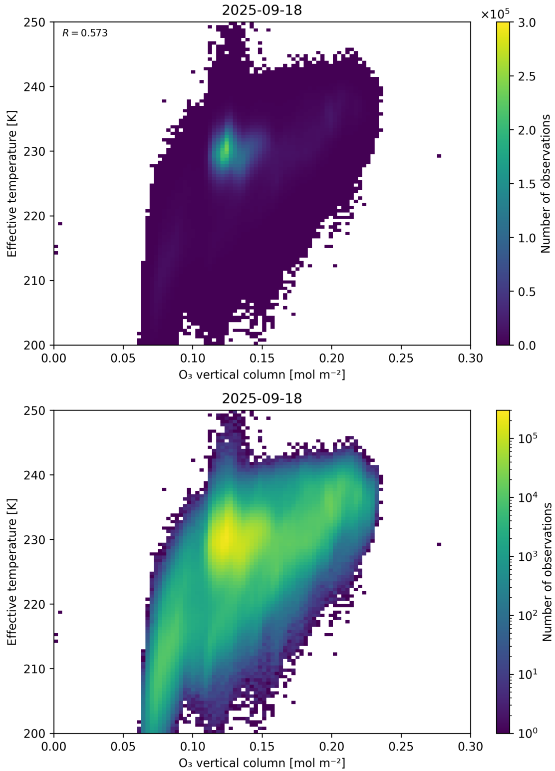
Figure 39: Scatter density plot of “O 3 vertical column” against “Effective temperature” for 2025-09-17 to 2025-09-19.
