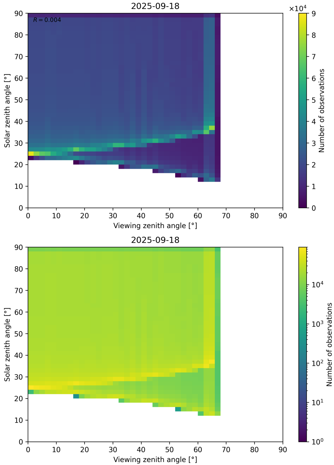
Figure 54: Scatter density plot of “Viewing zenith angle” against “Solar zenith angle” for 2025-09-17 to 2025-09-19.
