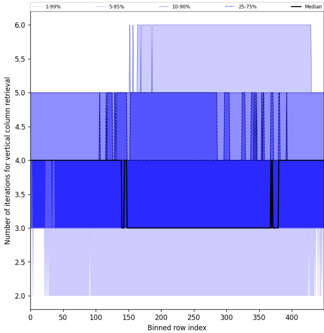
Figure 33: Along track statistics of “Number of iterations for vertical column retrieval” for 2025-09-17 to 2025-09-19
