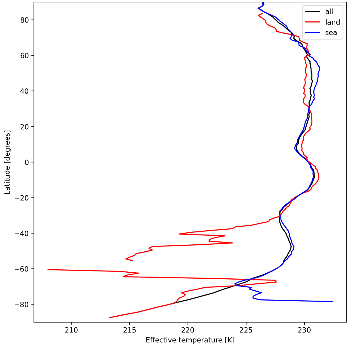
Figure 17: Zonal average of “Effective temperature” for 2025-09-17 to 2025-09-19.
