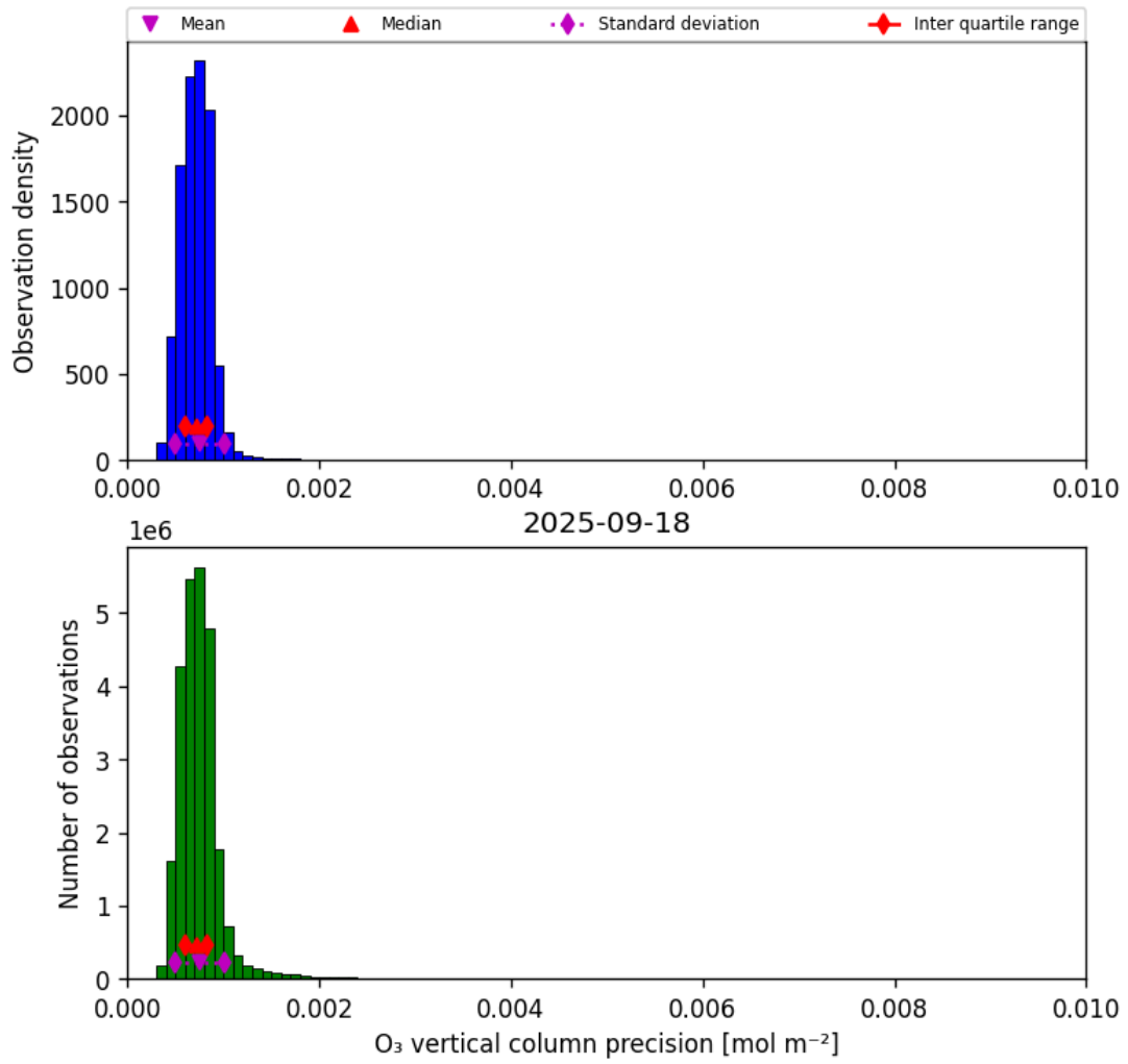
Figure 22: Histogram of “O 3 vertical column precision” for 2025-09-17 to 2025-09-19
