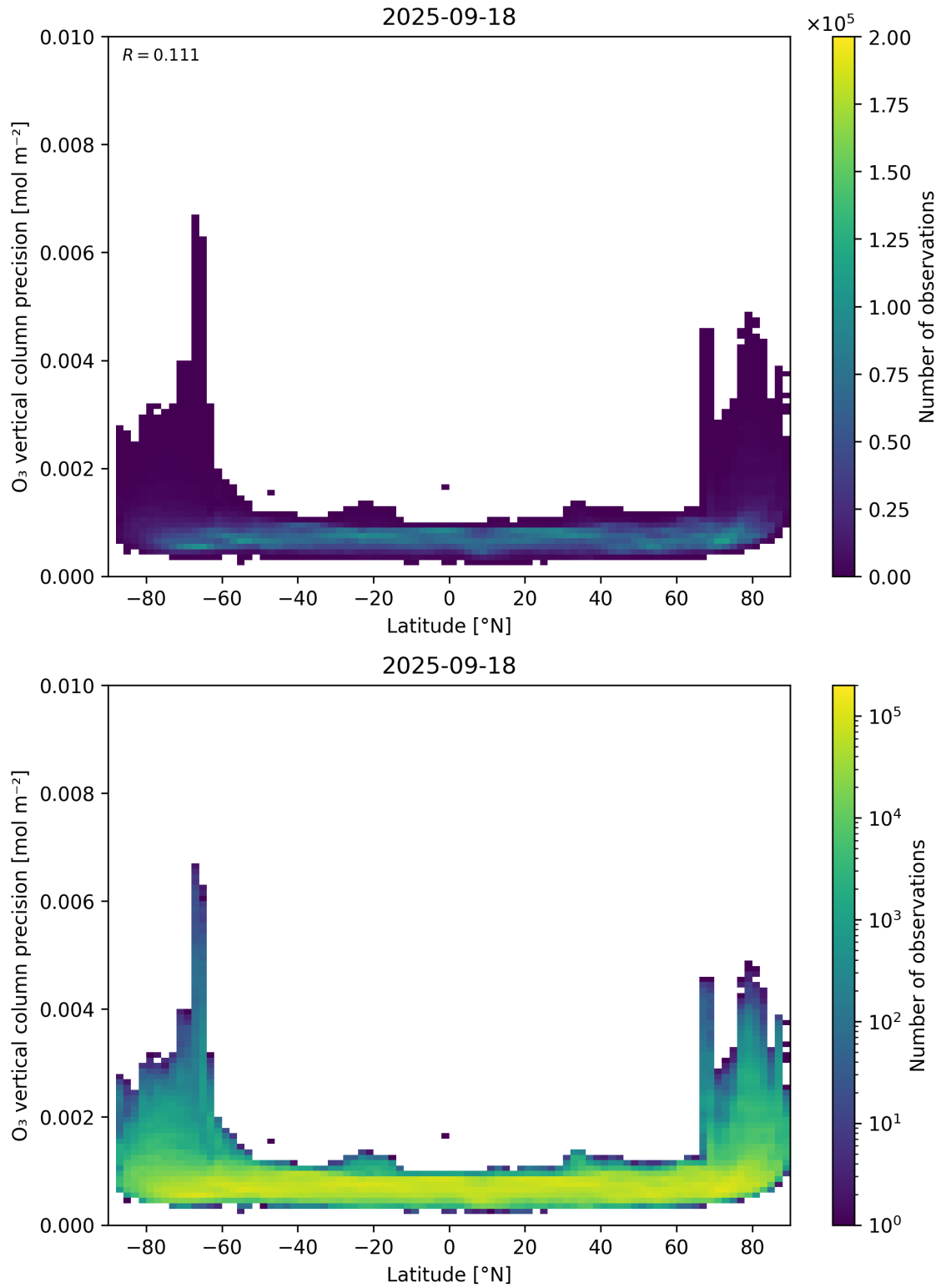
Figure 37: Scatter density plot of “Latitude” against “O 3 vertical column precision” for 2025-09-17 to 2025-09-19.
