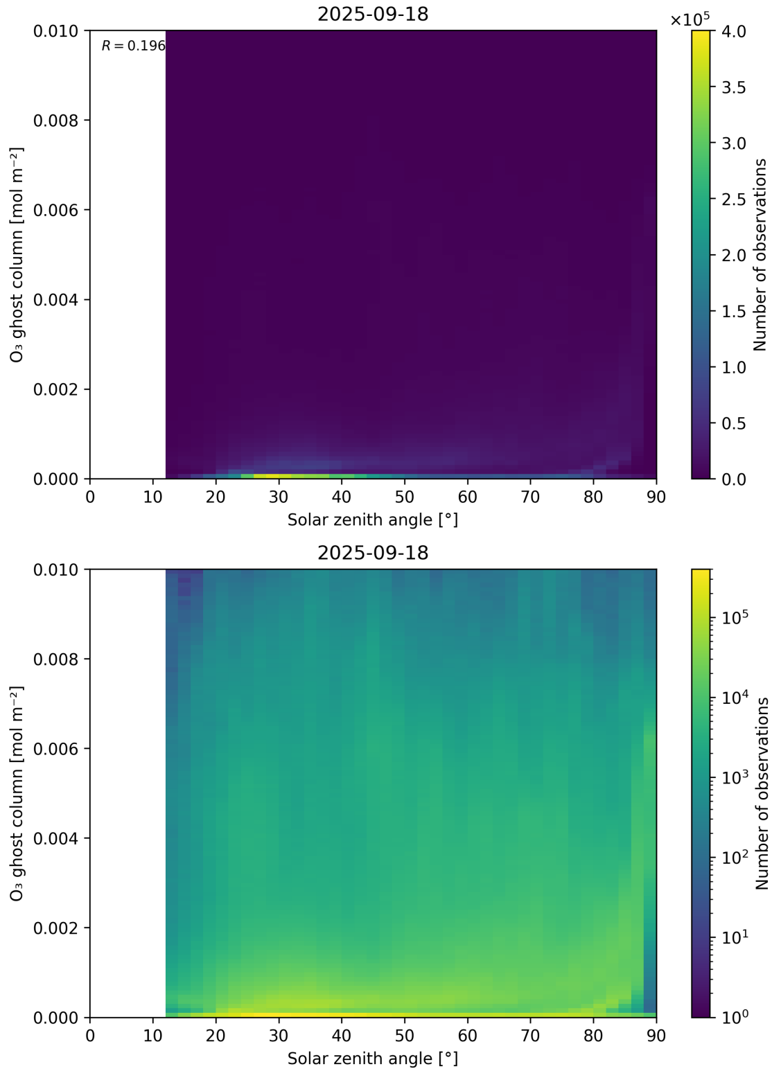
Figure 46: Scatter density plot of “Solar zenith angle” against “O 3 ghost column” for 2025-09-17 to 2025-09-19.
