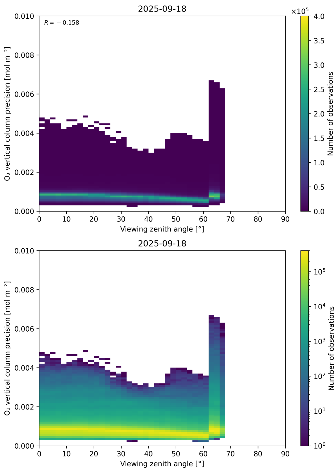
Figure 53: Scatter density plot of “Viewing zenith angle” against “O 3 vertical column precision” for 2025-09-17 to 2025-09-19.
