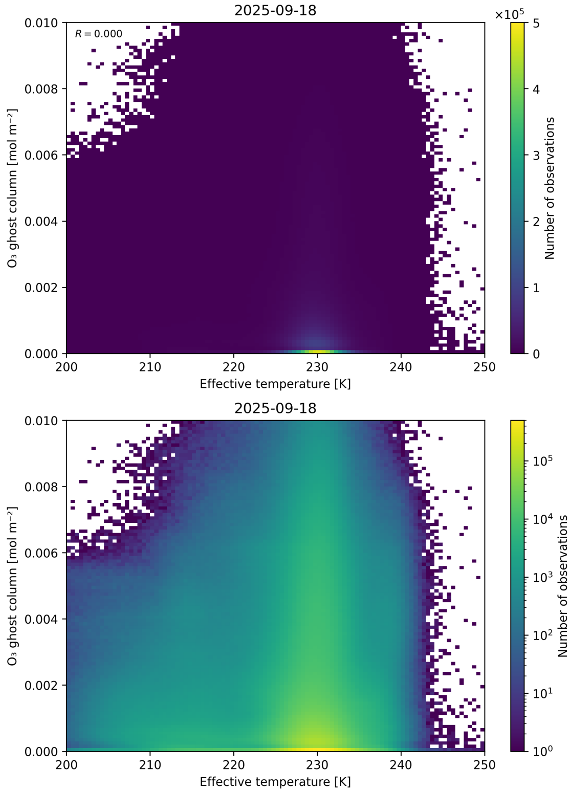
Figure 38: Scatter density plot of “Effective temperature” against “O 3 ghost column” for 2025-09-17 to 2025-09-19.
