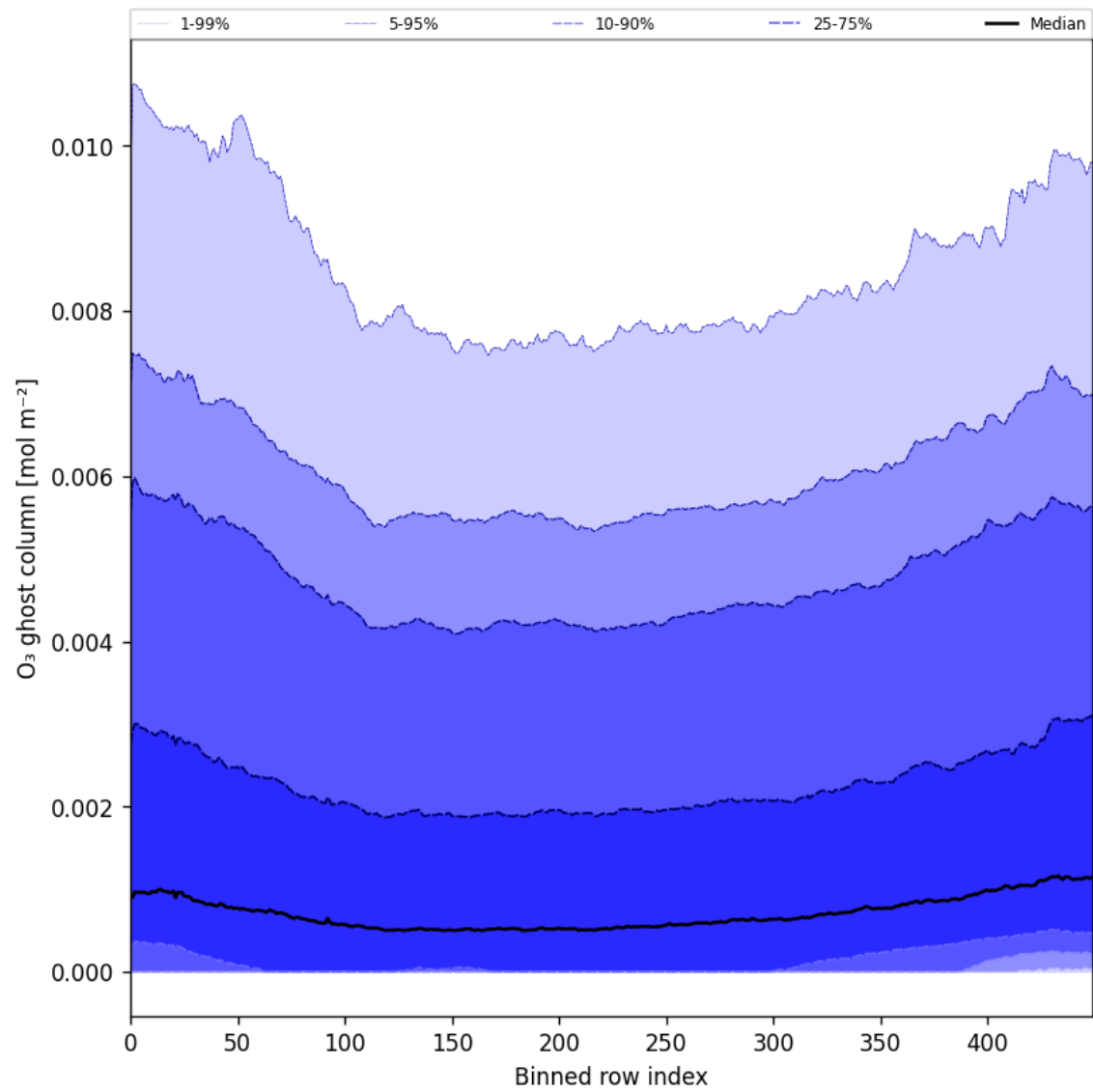
Figure 32: Along track statistics of “O 3 ghost column” for 2025-09-17 to 2025-09-19
