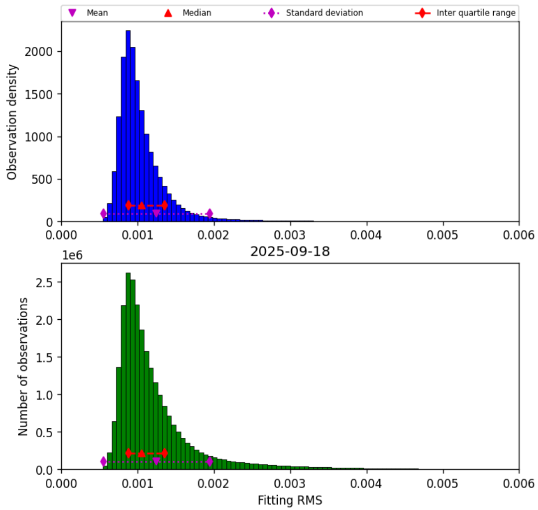
Figure 23: Histogram of “Fitting RMS” for 2025-09-17 to 2025-09-19
