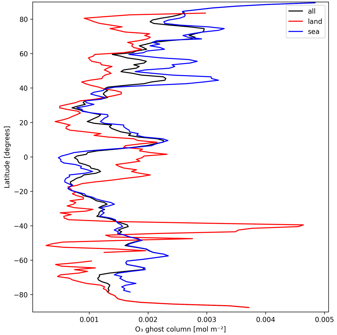
Figure 18: Zonal average of "O 3 ghost column" for 2025-09-17 to 2025-09-19.
