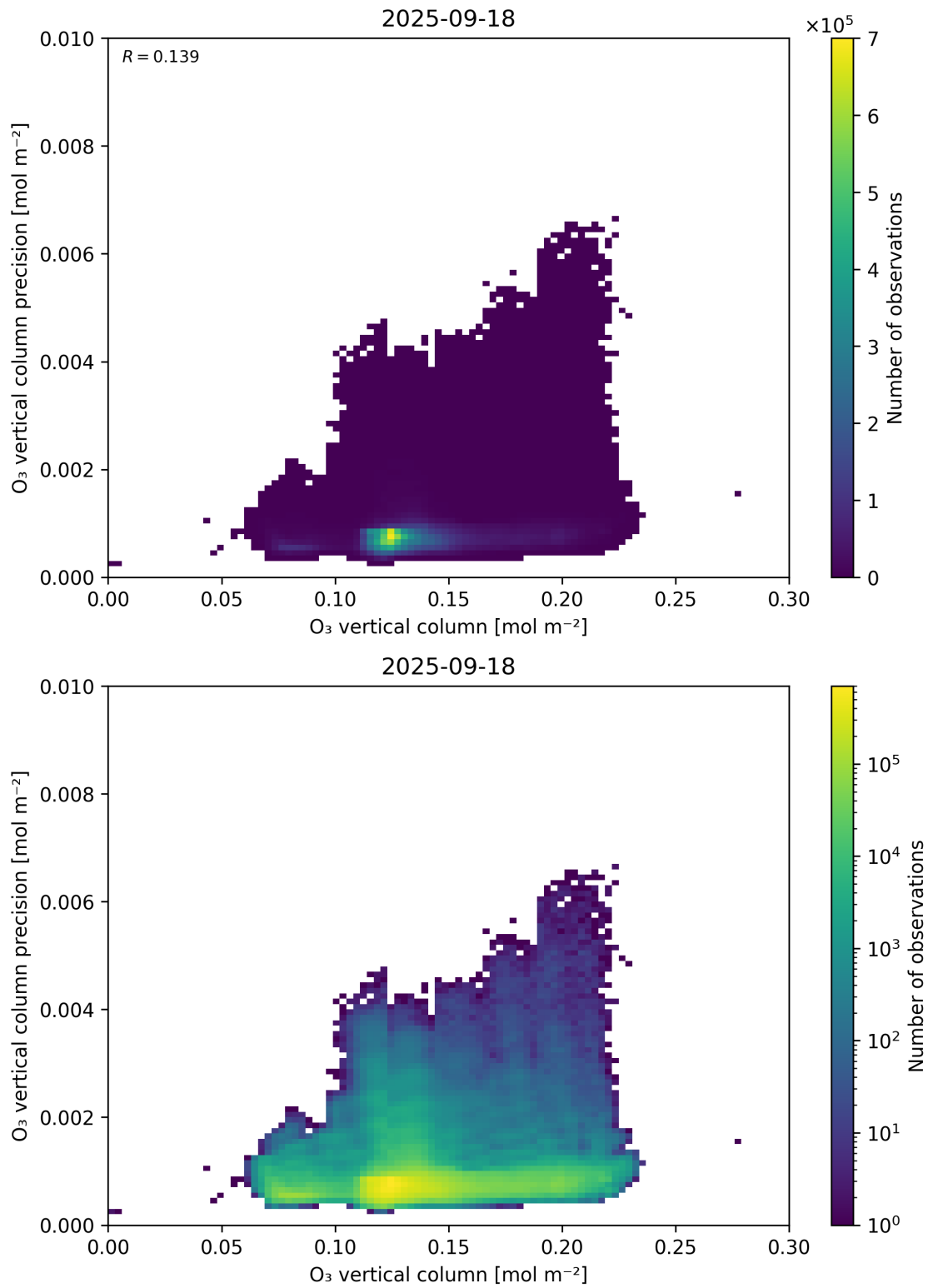
Figure 41: Scatter density plot of “O 3 vertical column” against “O 3 vertical column precision” for 2025-09-17 to 2025-09-19.
