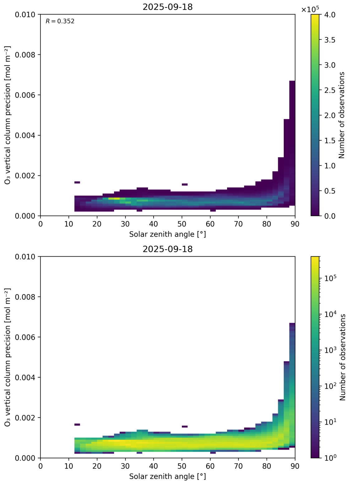
Figure 48: Scatter density plot of “Solar zenith angle” against “O 3 vertical column precision” for 2025-09-17 to 2025-09-19.
