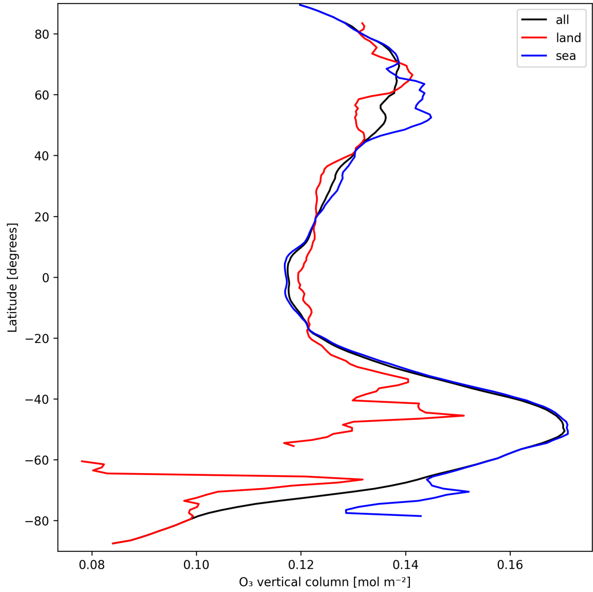
Figure 14: Zonal average of “O 3 vertical column” for 2025-09-17 to 2025-09-19.
