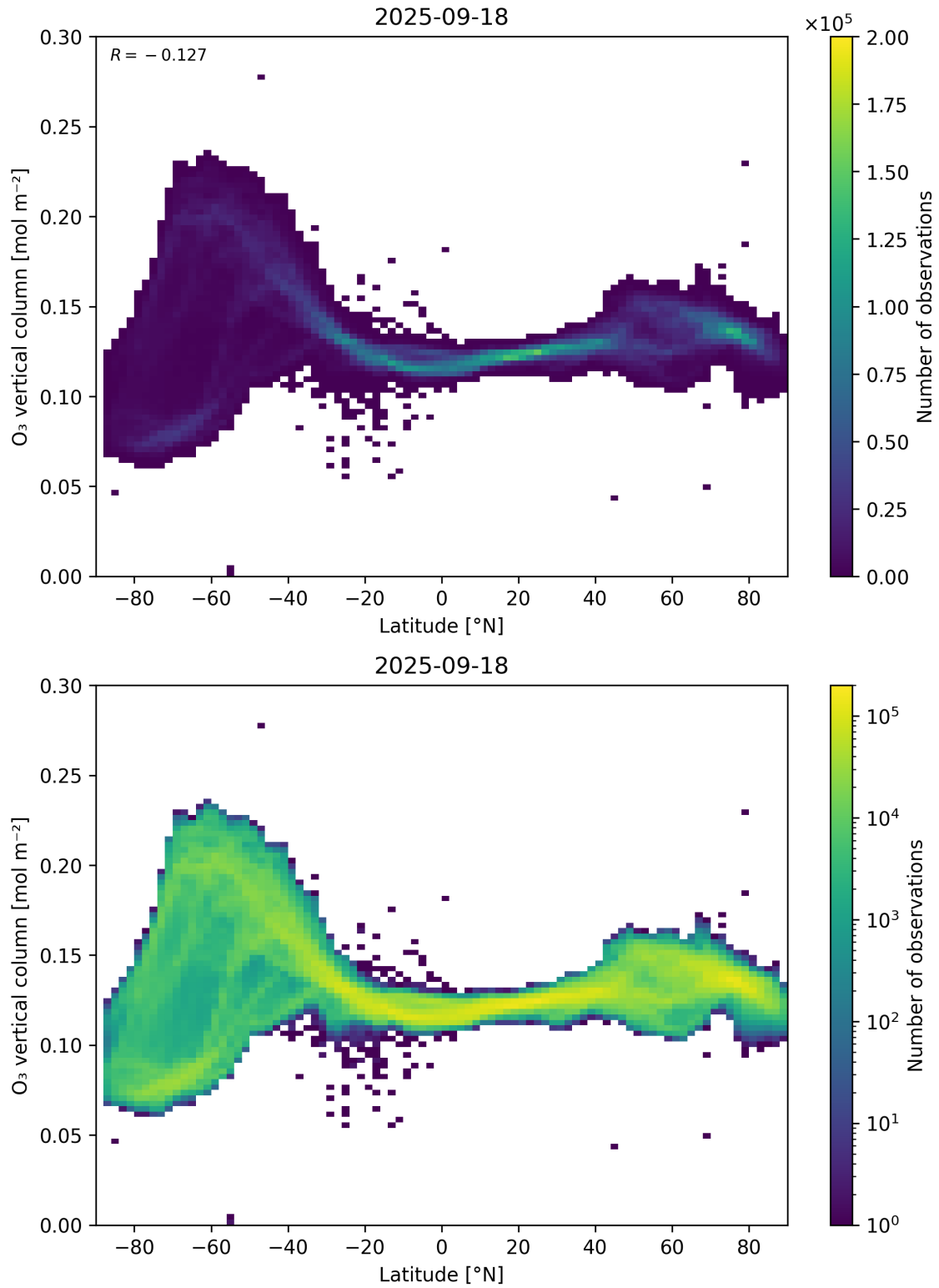
Figure 36: Scatter density plot of “Latitude” against “O 3 vertical column” for 2025-09-17 to 2025-09-19.
