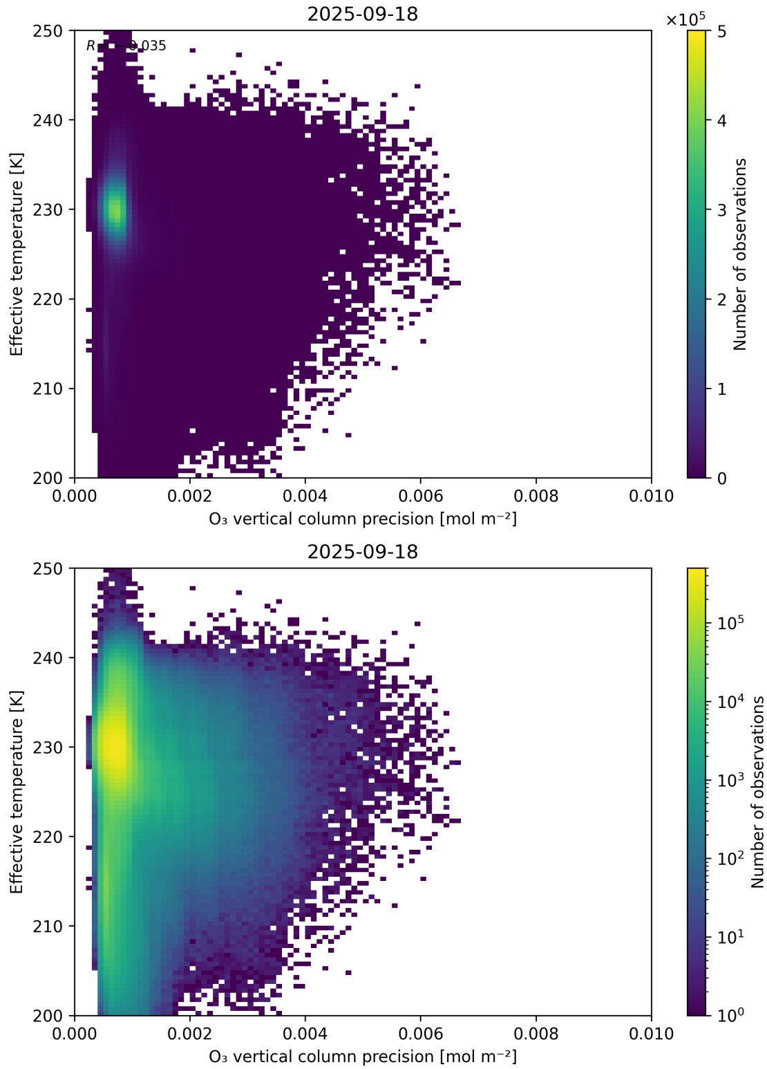
Figure 42: Scatter density plot of “O 3 vertical column precision” against “Effective temperature” for 2025-09-17 to 2025-09-19.
