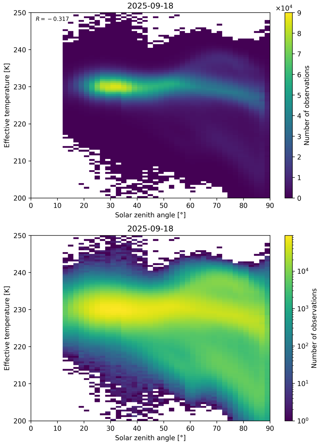
Figure 45: Scatter density plot of “Solar zenith angle” against “Effective temperature” for 2025-09-17 to 2025-09-19.
