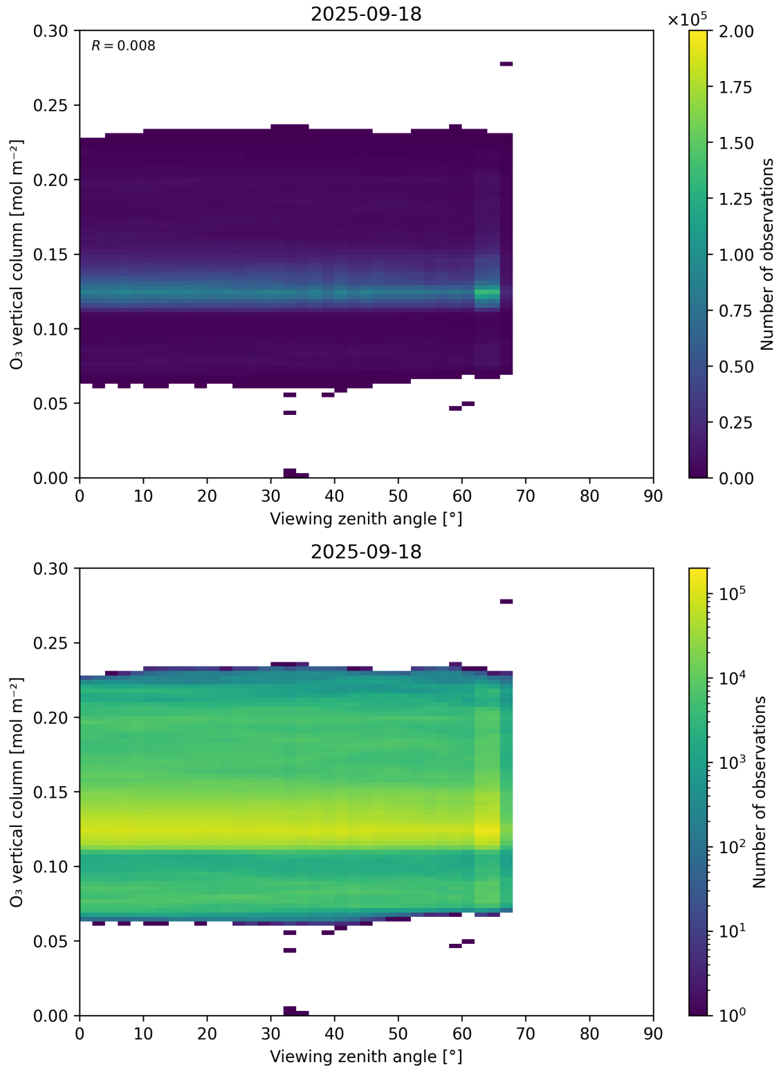
Figure 52: Scatter density plot of “Viewing zenith angle” against “O 3 vertical column” for 2025-09-17 to 2025-09-19.
