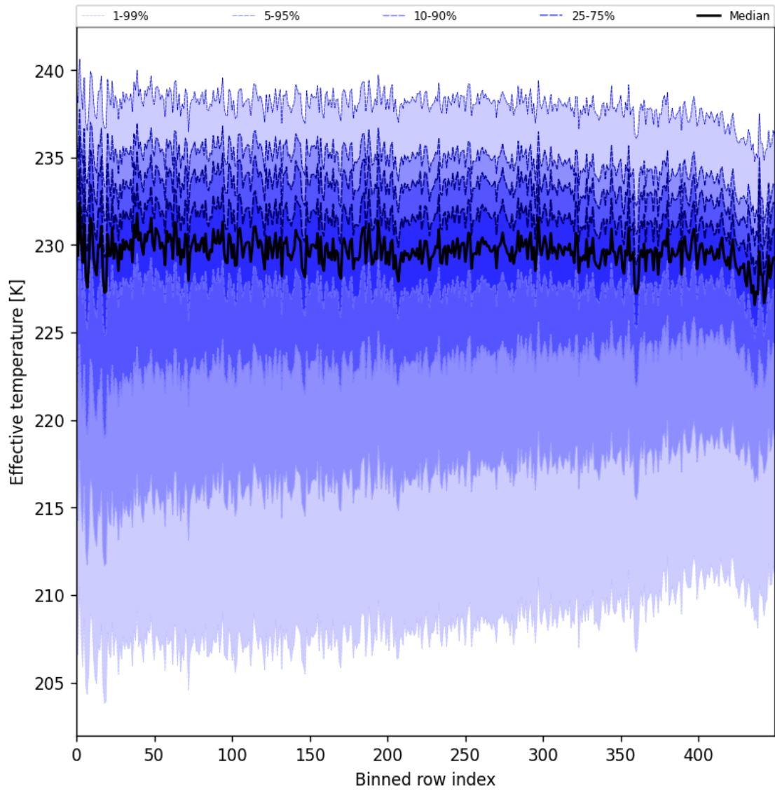
Figure 31: Along track statistics of “Effective temperature” for 2025-09-17 to 2025-09-19
