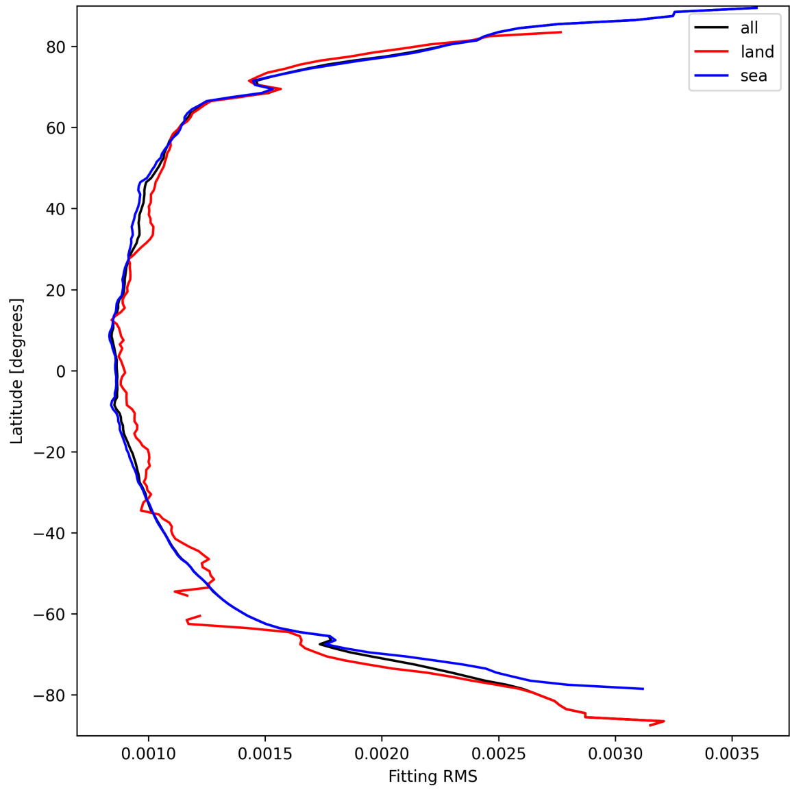
Figure 16: Zonal average of “Fitting RMS” for 2025-09-18 to 2025-09-20.
