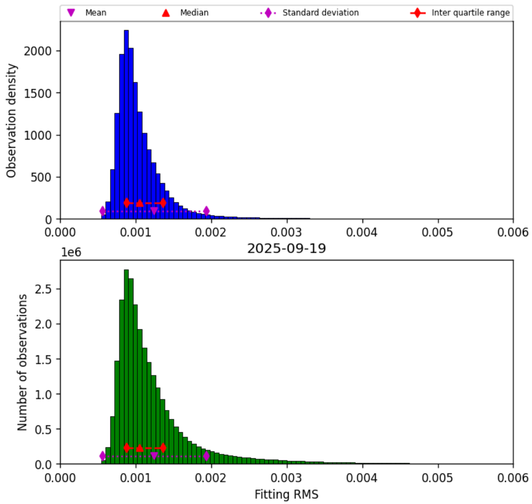
Figure 23: Histogram of “Fitting RMS” for 2025-09-18 to 2025-09-20
