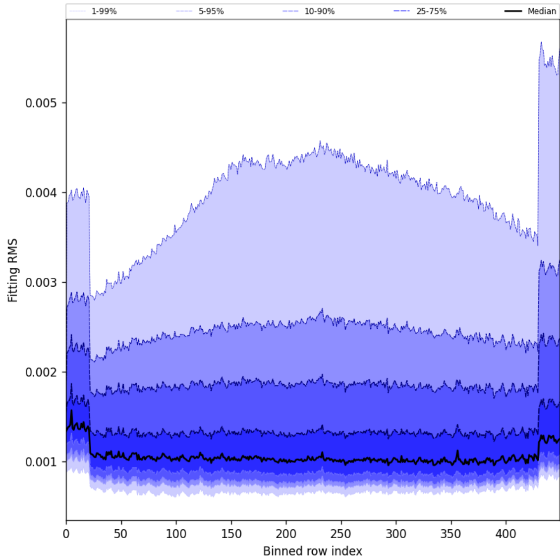
Figure 30: Along track statistics of “Fitting RMS” for 2025-09-18 to 2025-09-20
