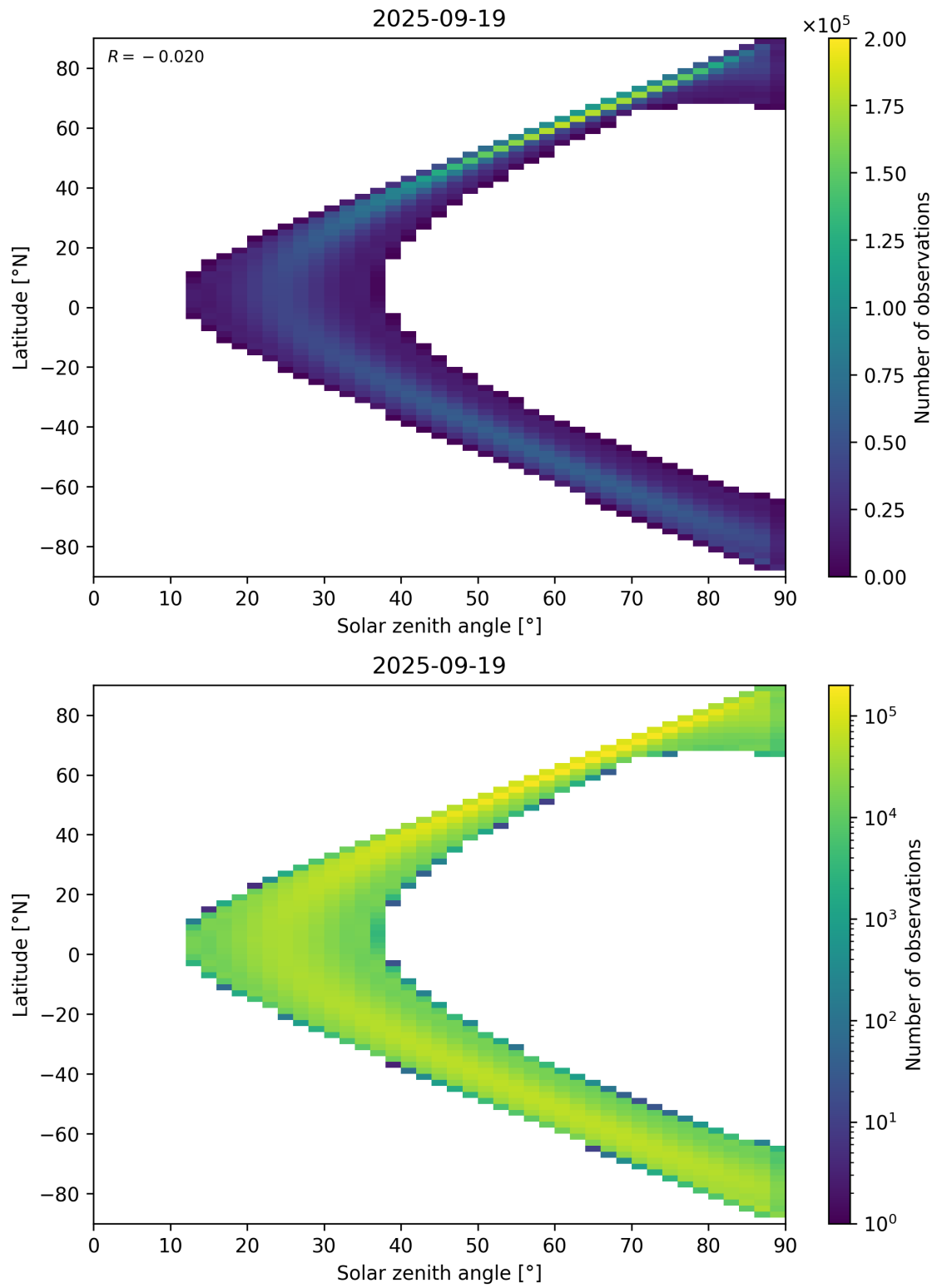
Figure 44: Scatter density plot of “Solar zenith angle” against “Latitude” for 2025-09-18 to 2025-09-20.
