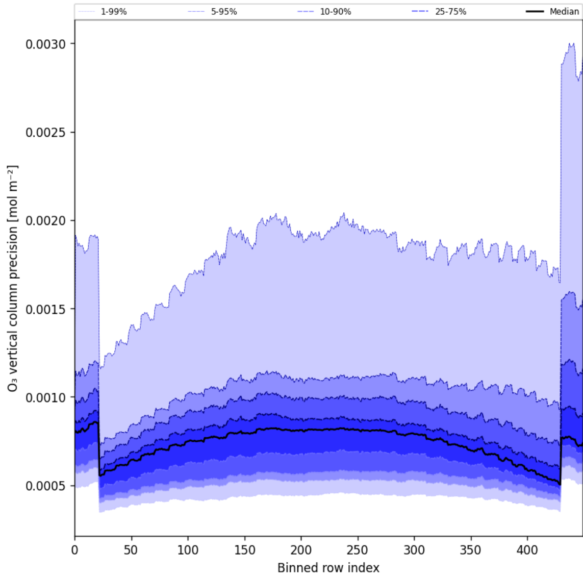
Figure 29: Along track statistics of “O 3 vertical column precision” for 2025-09-18 to 2025-09-20
