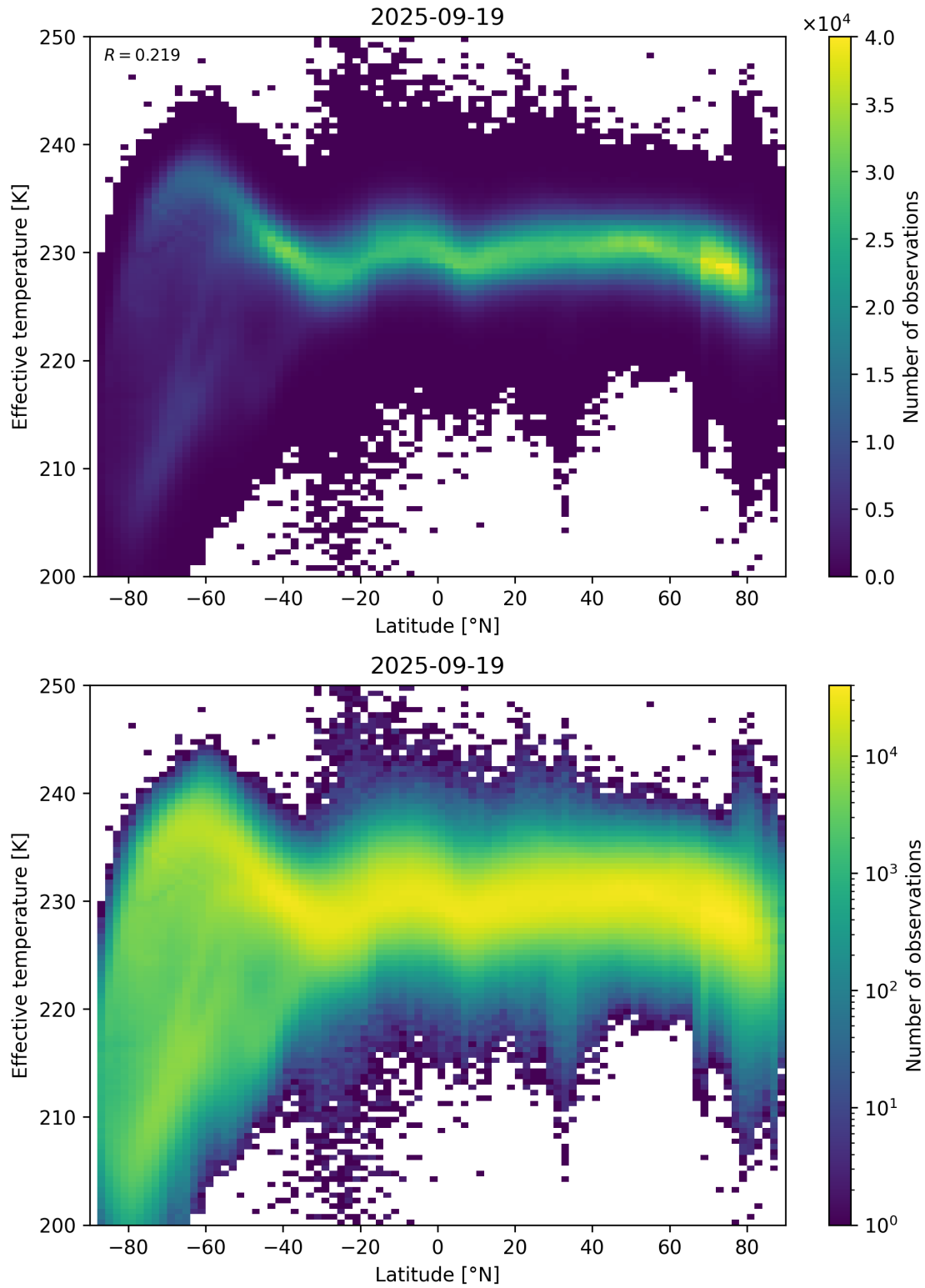
Figure 34: Scatter density plot of “Latitude” against “Effective temperature” for 2025-09-18 to 2025-09-20.
