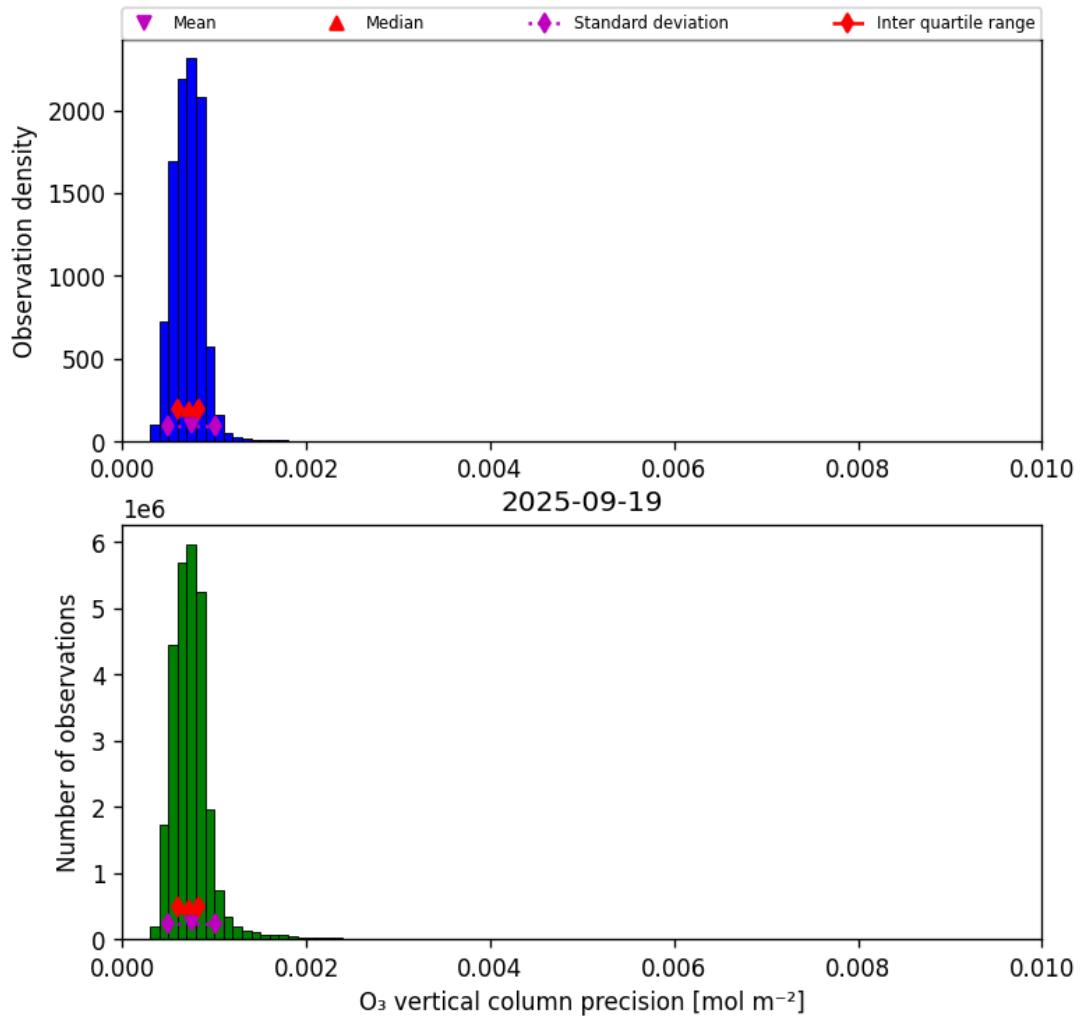
Figure 22: Histogram of “O 3 vertical column precision” for 2025-09-18 to 2025-09-20
