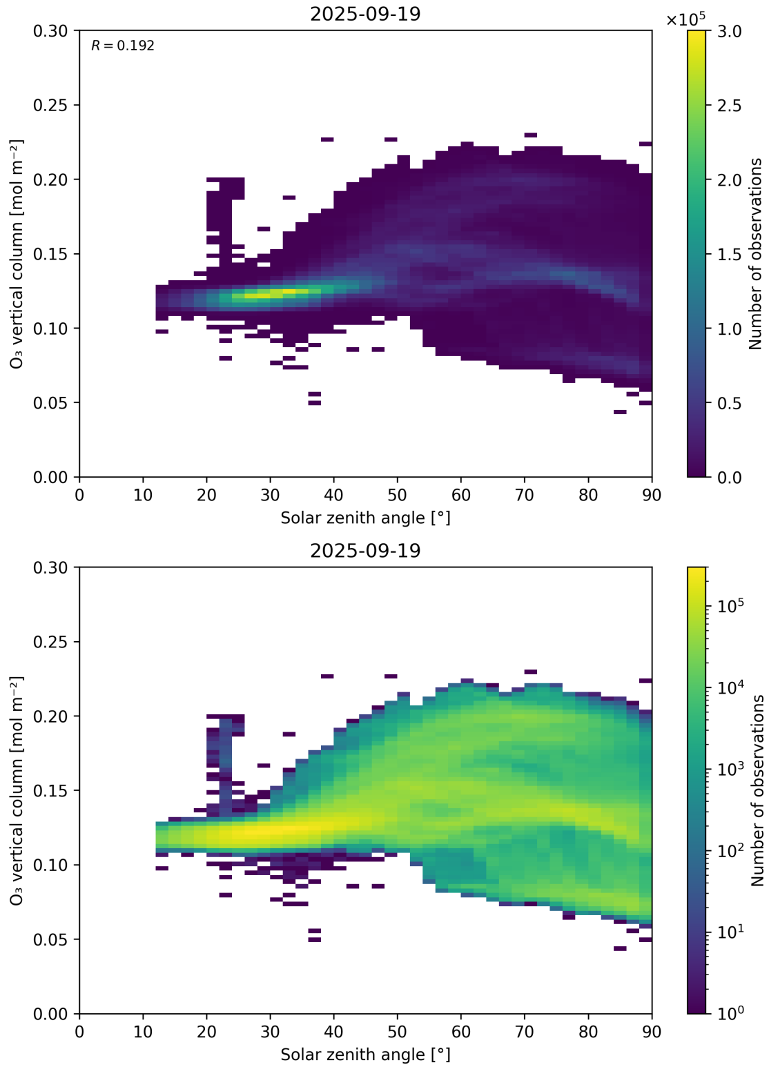
Figure 47: Scatter density plot of “Solar zenith angle” against “O 3 vertical column” for 2025-09-18 to 2025-09-20.
