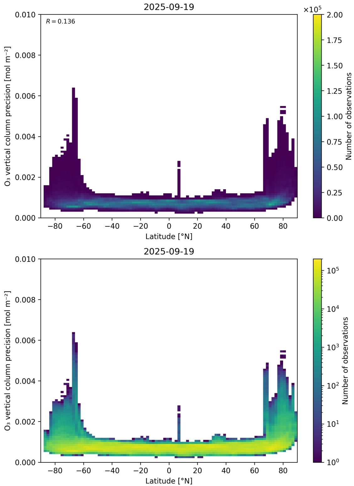
Figure 37: Scatter density plot of “Latitude” against “O 3 vertical column precision” for 2025-09-18 to 2025-09-20.
