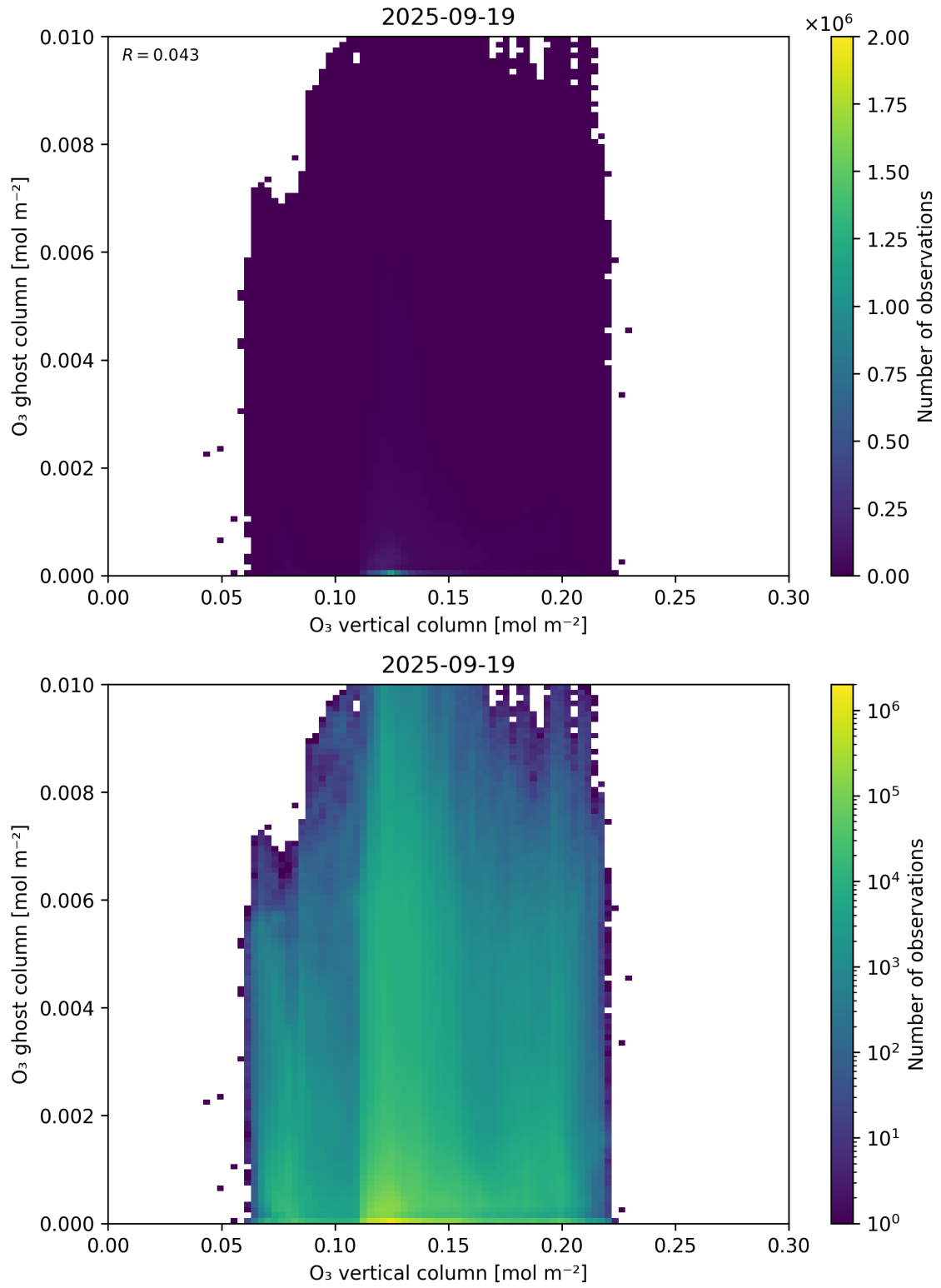
Figure 40: Scatter density plot of “O 3 vertical column” against “O 3 ghost column” for 2025-09-18 to 2025-09-20.
