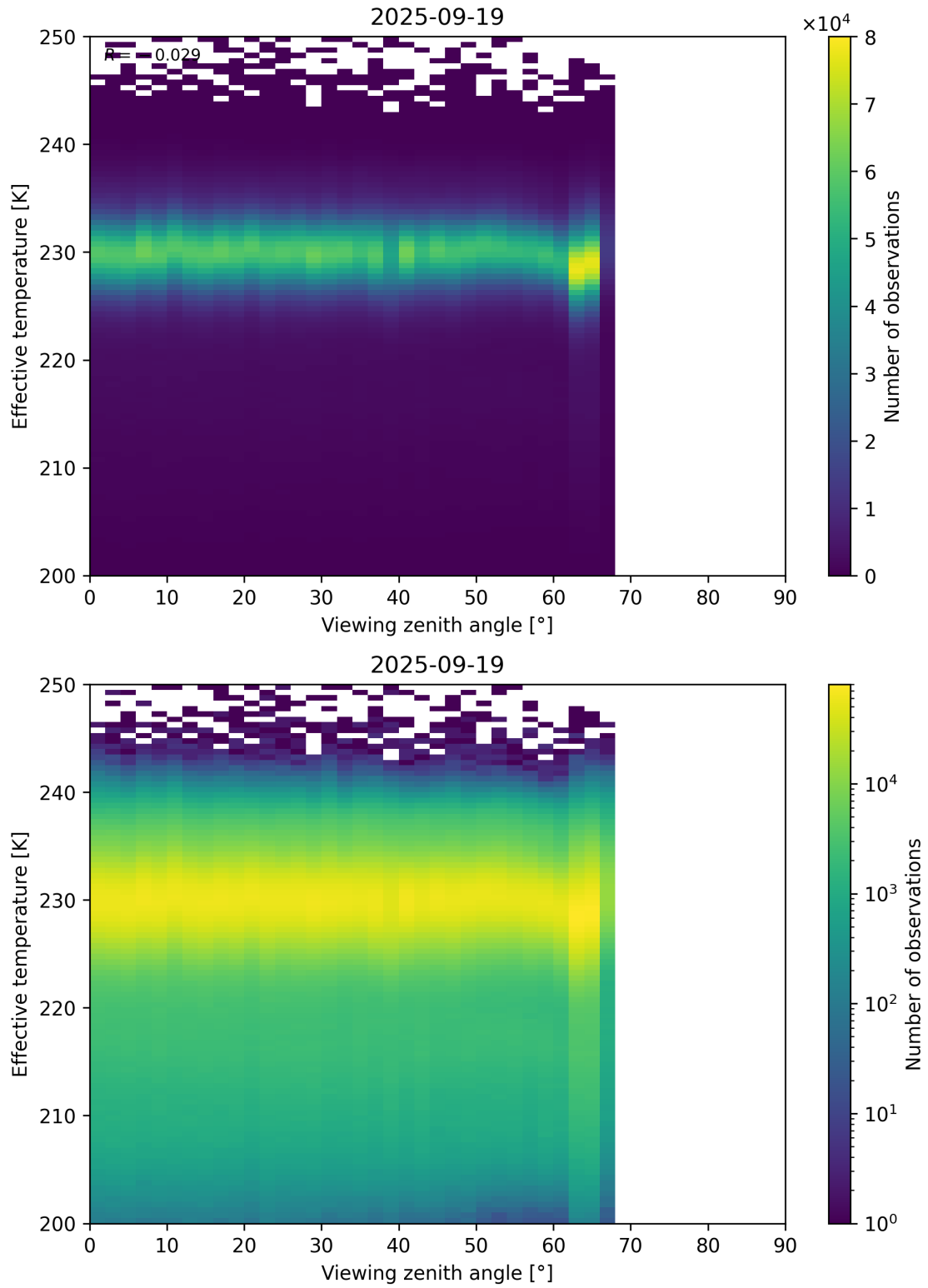
Figure 50: Scatter density plot of “Viewing zenith angle” against “Effective temperature” for 2025-09-18 to 2025-09-20.
