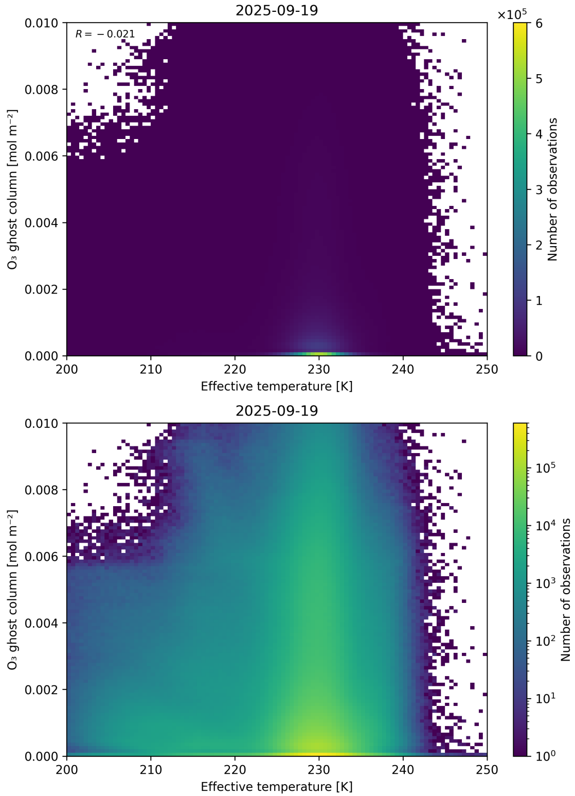
Figure 38: Scatter density plot of “Effective temperature” against “O 3 ghost column” for 2025-09-18 to 2025-09-20.
