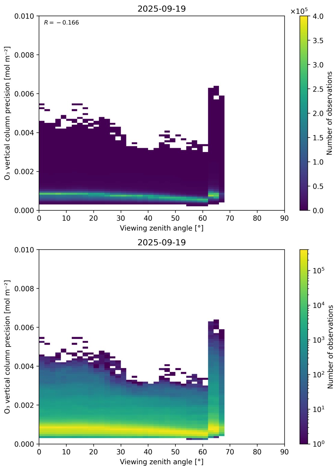
Figure 53: Scatter density plot of “Viewing zenith angle” against “O 3 vertical column precision” for 2025-09-18 to 2025-09-20.
