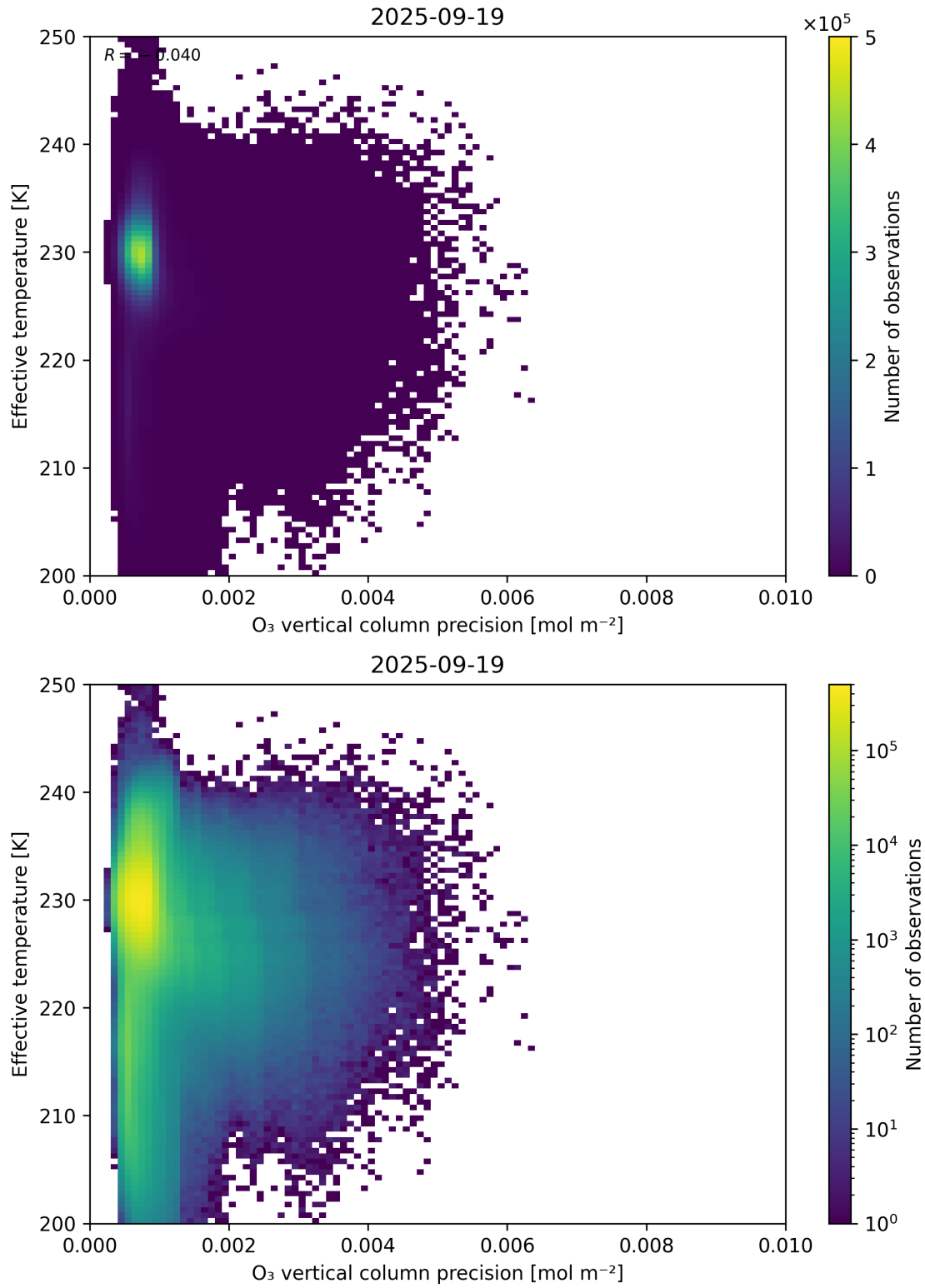
Figure 42: Scatter density plot of “ O_3 vertical column precision” against “Effective temperature” for 2025-09-18 to 2025-09-20.
