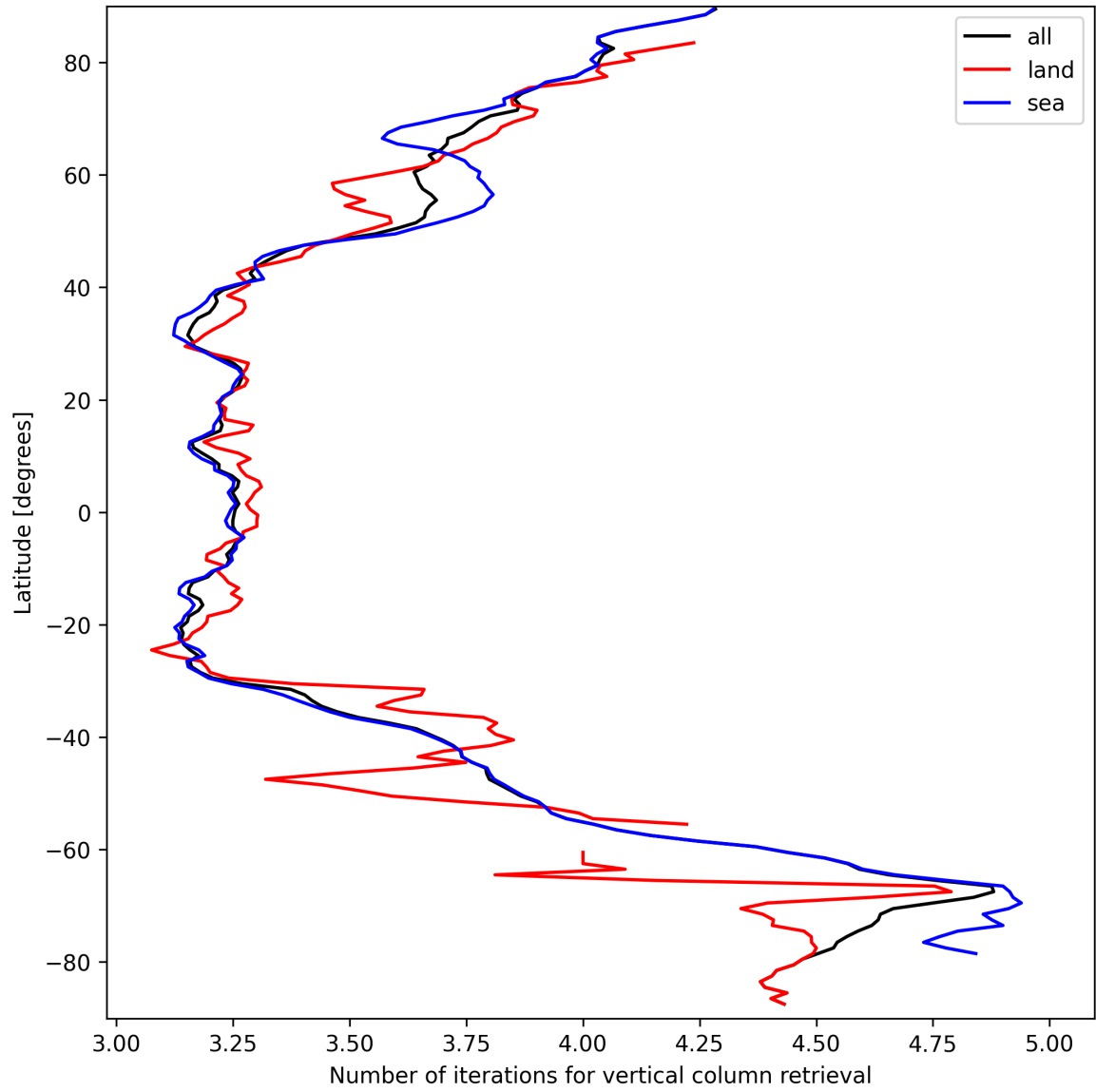
Figure 19: Zonal average of “Number of iterations for vertical column retrieval” for 2025-09-18 to 2025-09-20.
