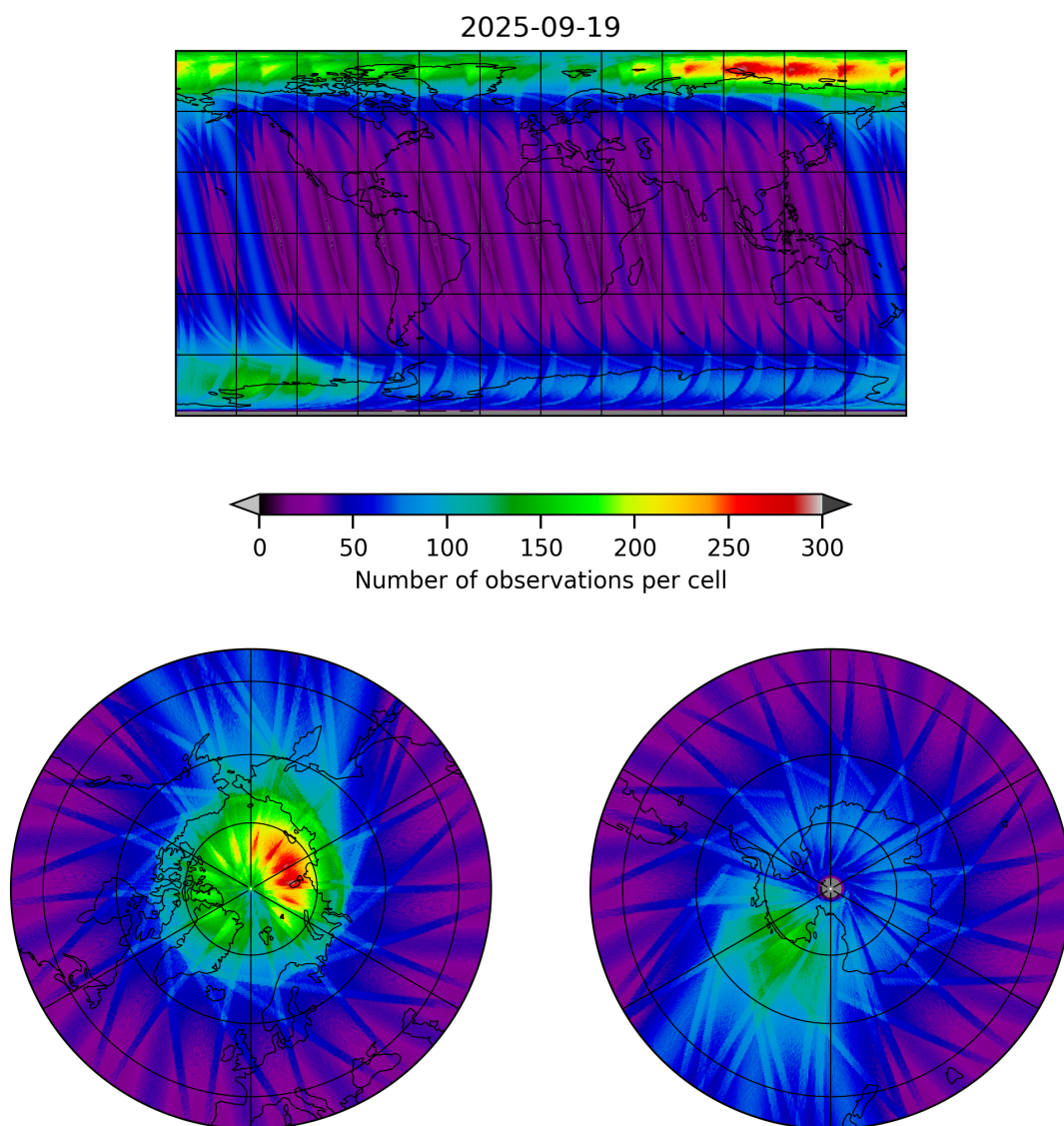
Figure 12: Map of the number of observations for 2025-09-18 to 2025-09-20
