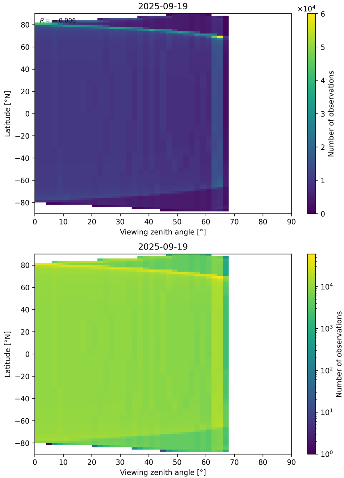
Figure 49: Scatter density plot of “Viewing zenith angle” against “Latitude” for 2025-09-18 to 2025-09-20.
