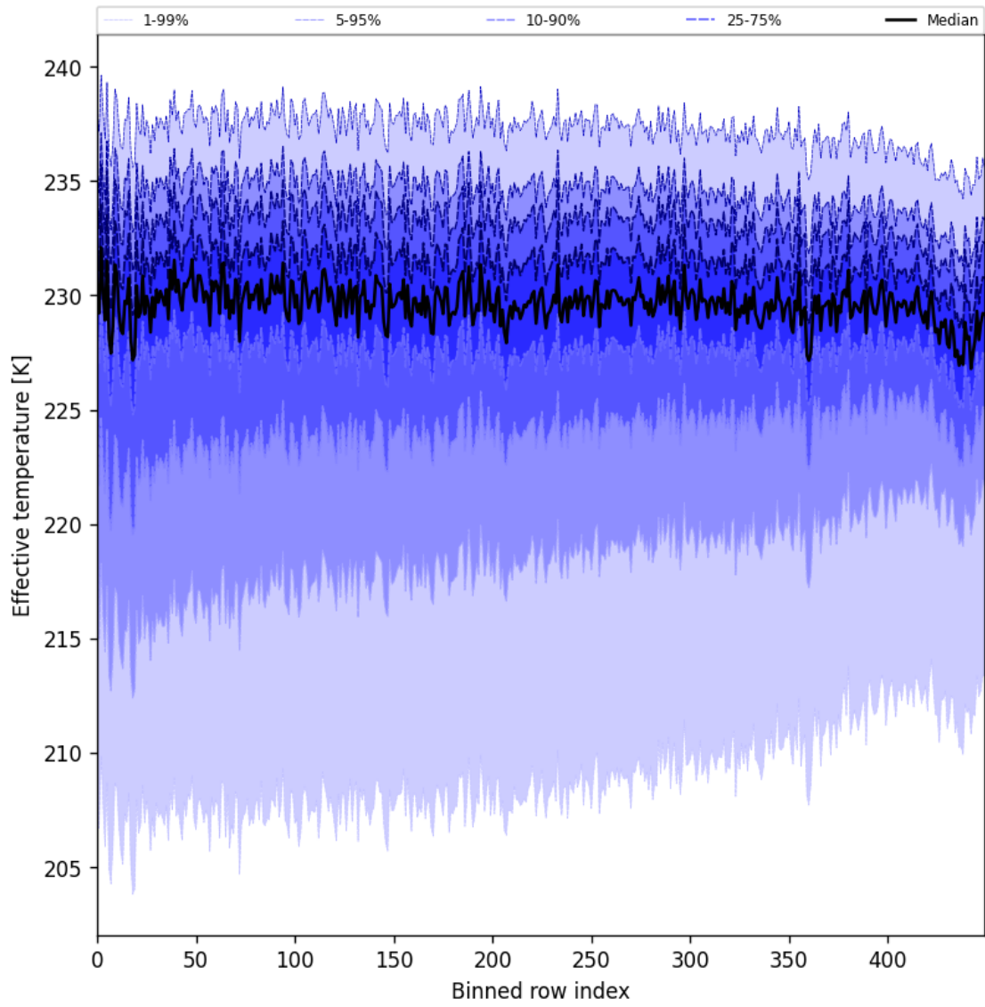
Figure 31: Along track statistics of “Effective temperature” for 2025-09-18 to 2025-09-20
