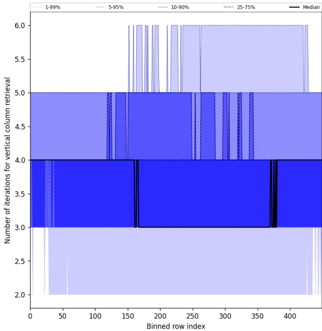
Figure 33: Along track statistics of “Number of iterations for vertical column retrieval” for 2025-09-18 to 2025-09-20
