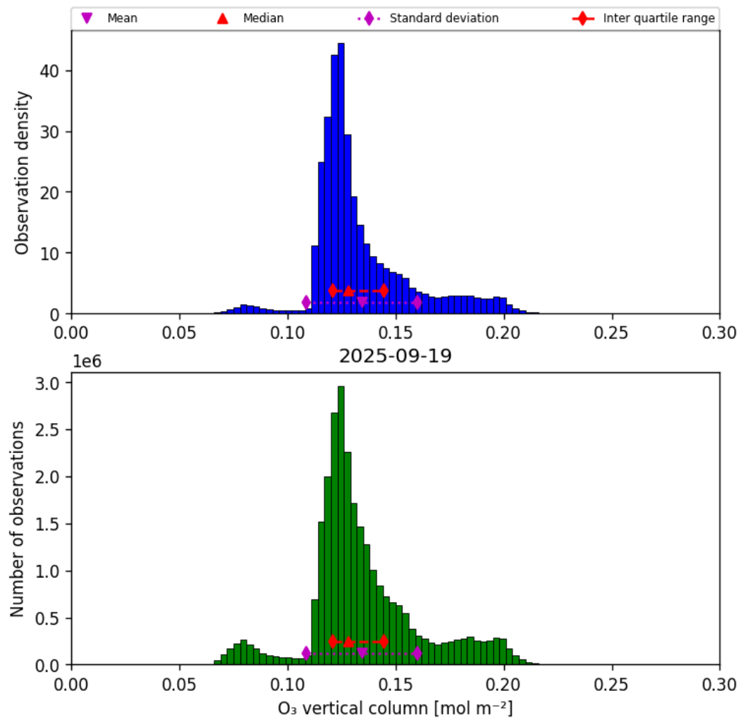
Figure 21: Histogram of “O 3 vertical column” for 2025-09-18 to 2025-09-20
