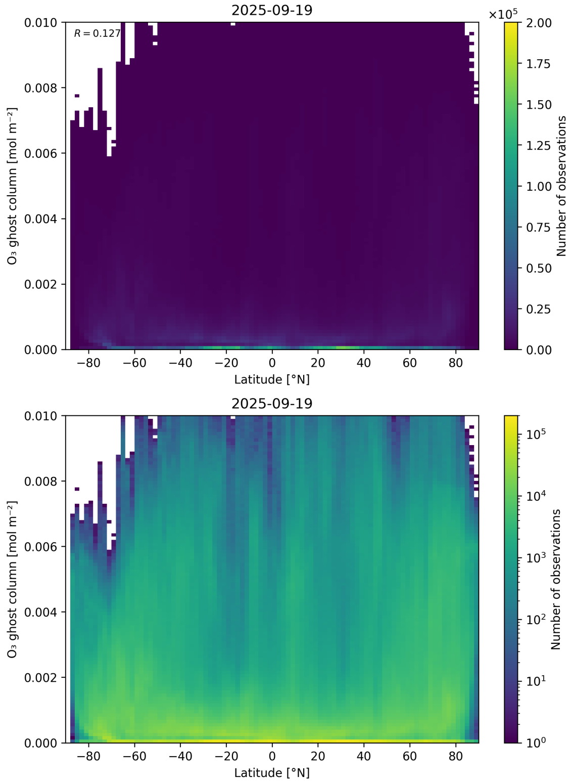
Figure 35: Scatter density plot of “Latitude” against “O 3 ghost column” for 2025-09-18 to 2025-09-20.
