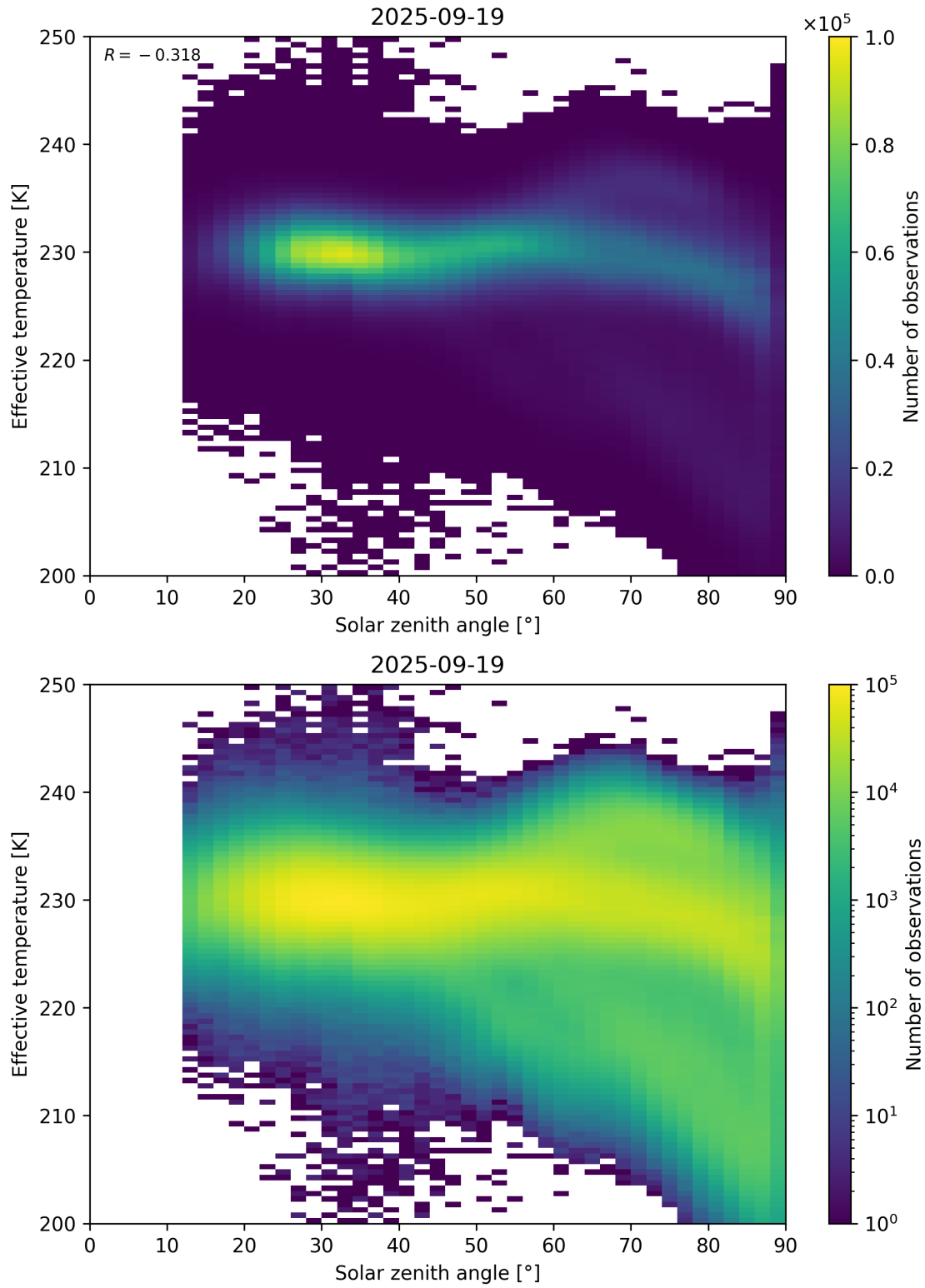
Figure 45: Scatter density plot of “Solar zenith angle” against “Effective temperature” for 2025-09-18 to 2025-09-20.
