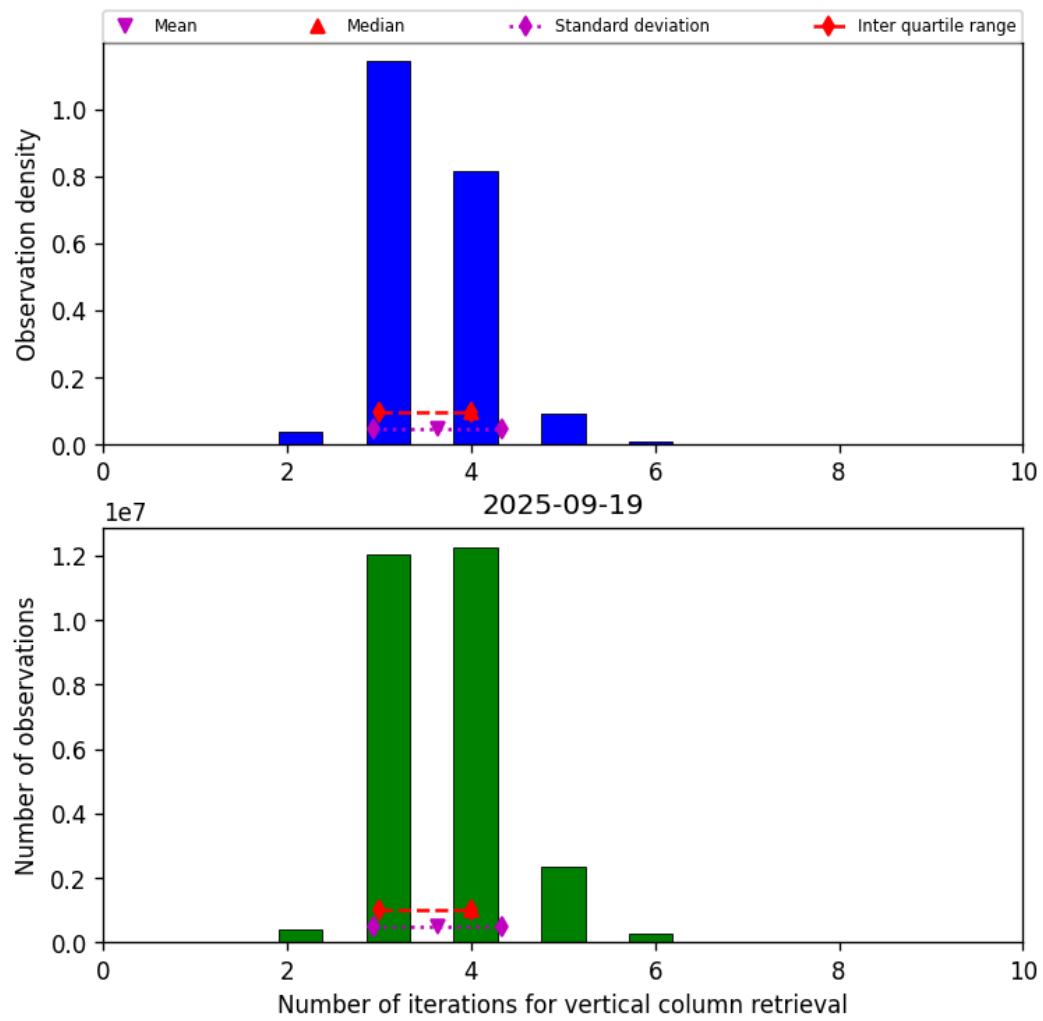
Figure 26: Histogram of “Number of iterations for vertical column retrieval” for 2025-09-18 to 2025-09-20
