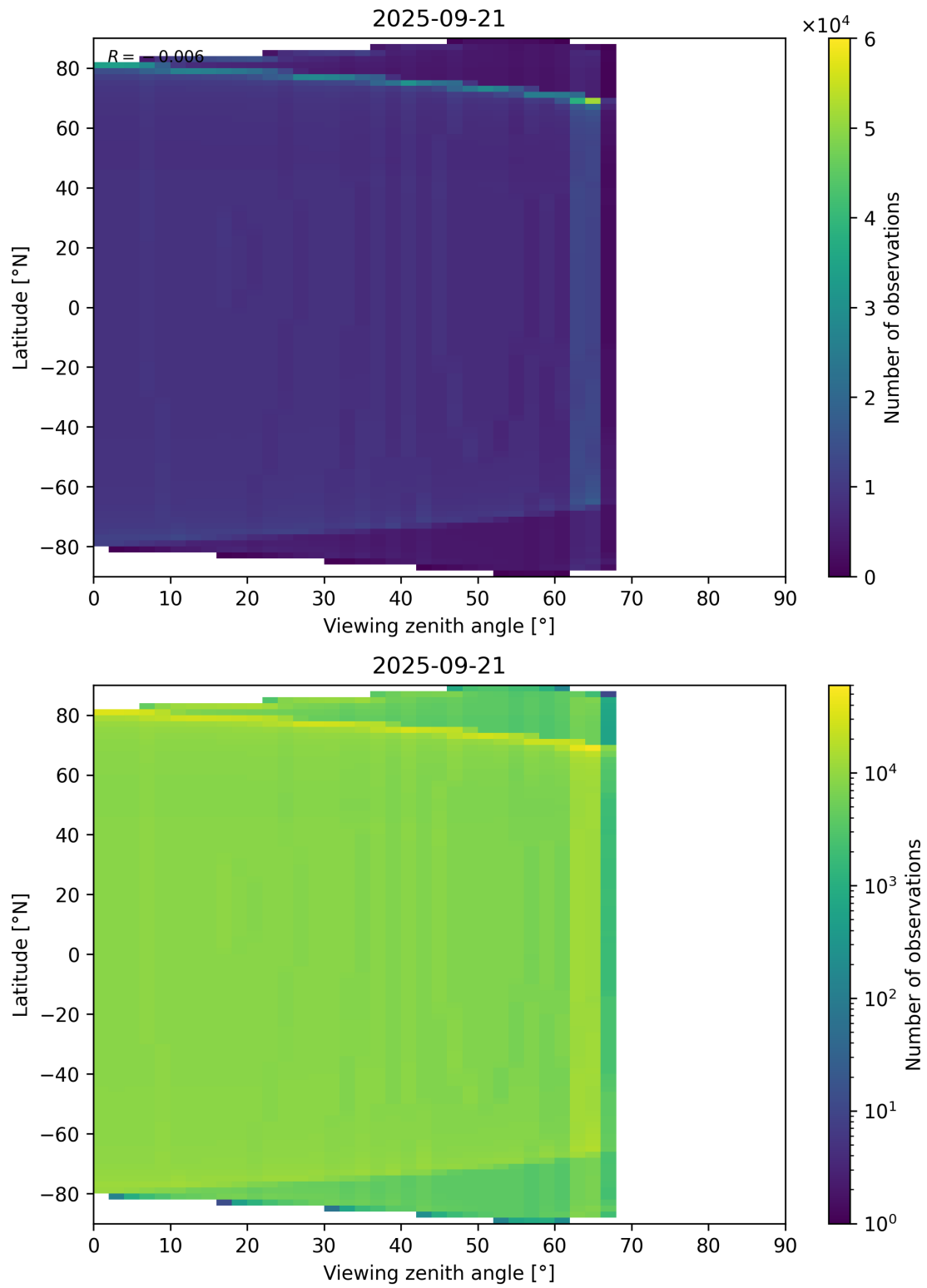
Figure 49: Scatter density plot of “Viewing zenith angle” against “Latitude” for 2025-09-20 to 2025-09-22.
