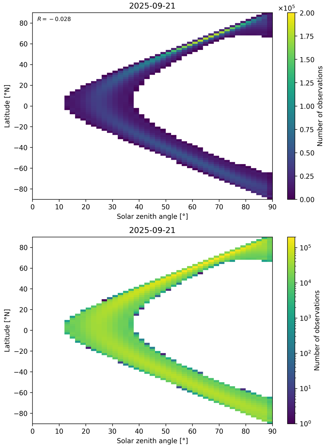
Figure 44: Scatter density plot of “Solar zenith angle” against “Latitude” for 2025-09-20 to 2025-09-22.
