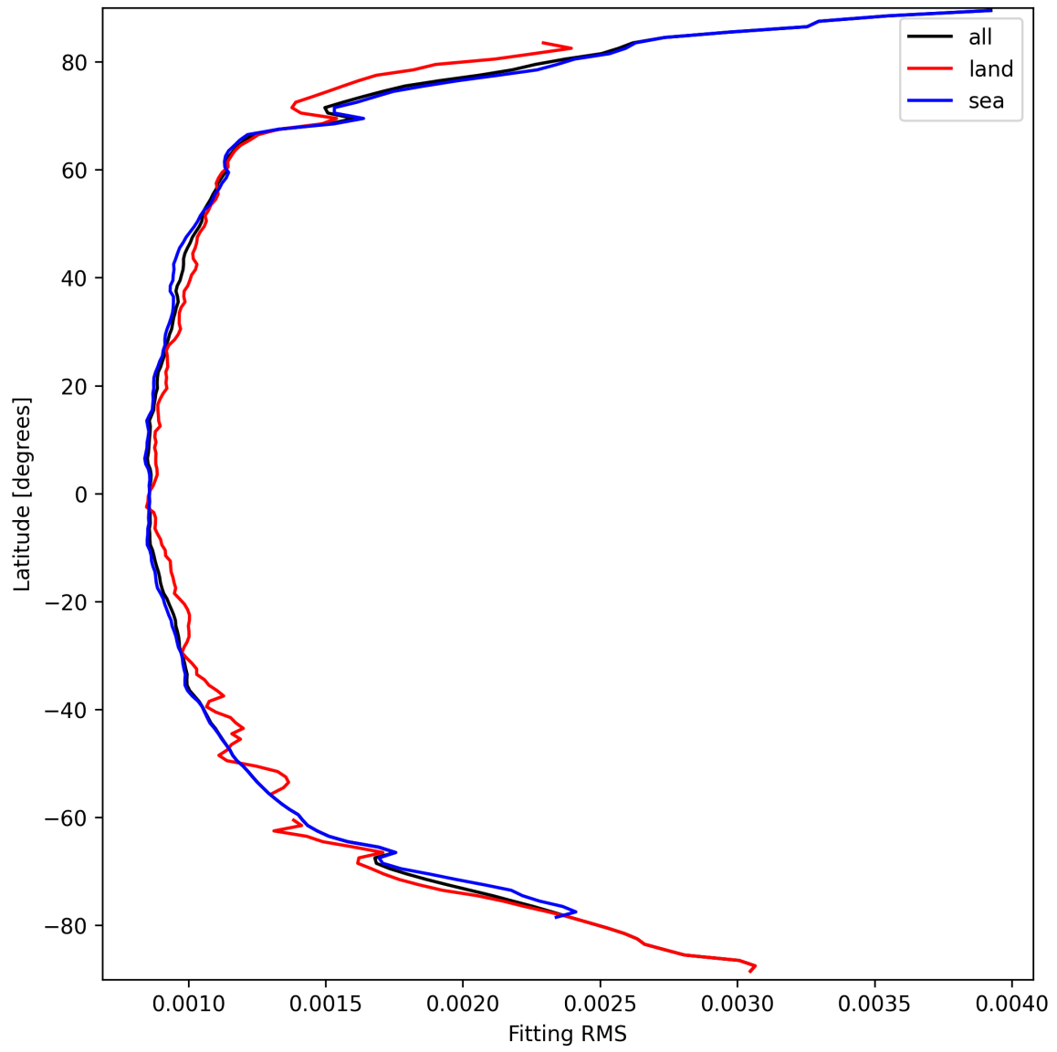
Figure 16: Zonal average of “Fitting RMS” for 2025-09-20 to 2025-09-22.
