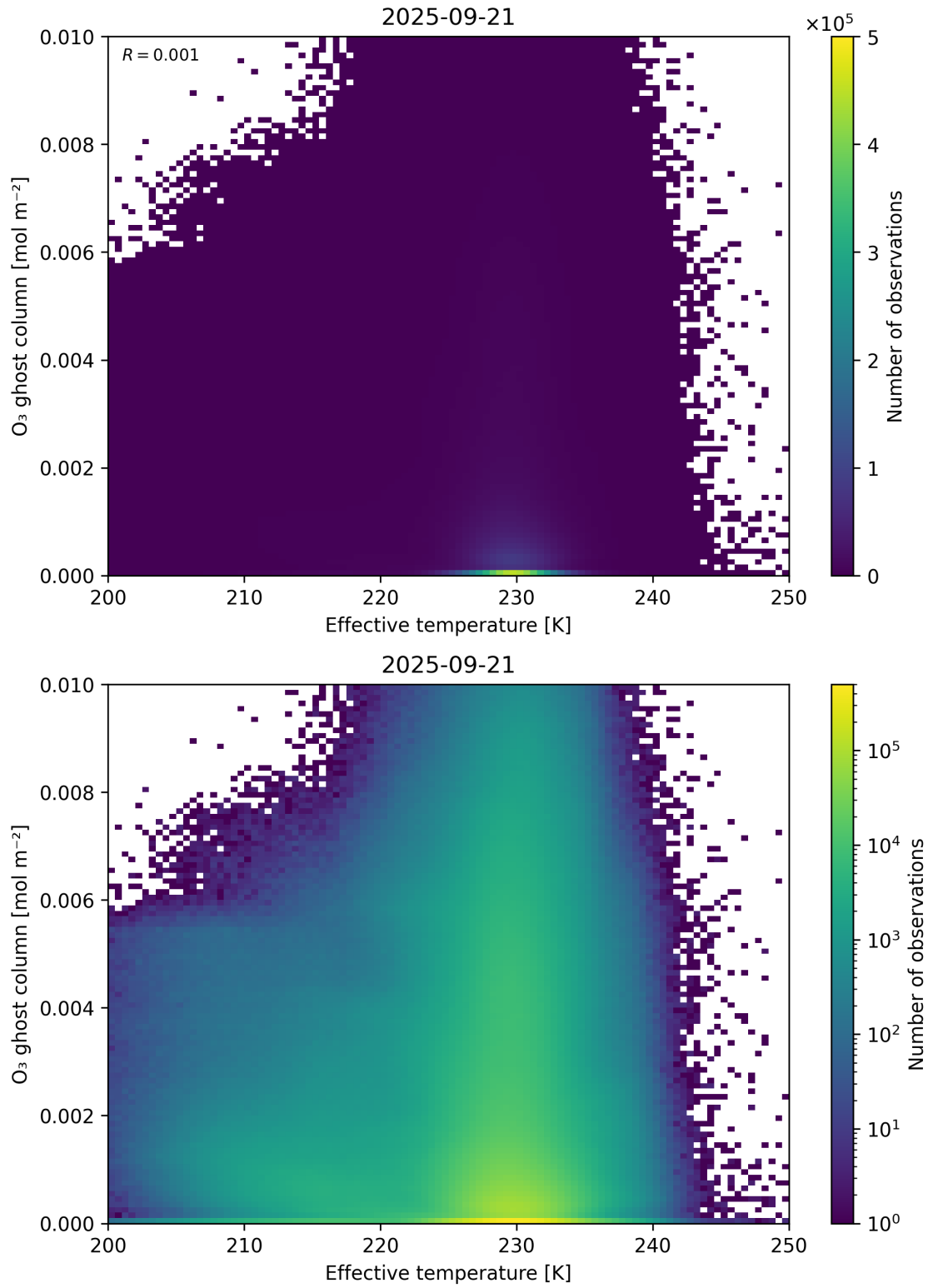
Figure 38: Scatter density plot of “Effective temperature” against “O 3 ghost column” for 2025-09-20 to 2025-09-22.
