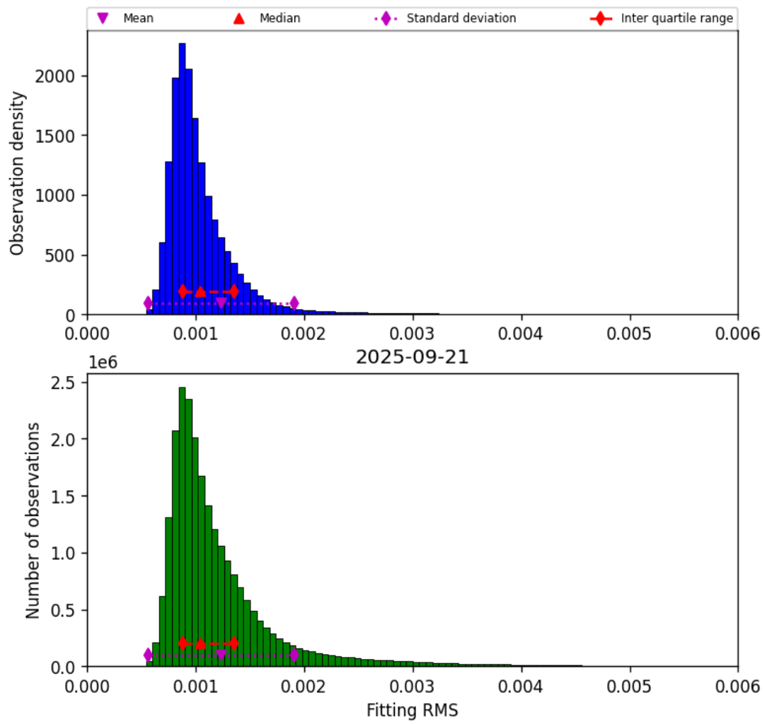
Figure 23: Histogram of “Fitting RMS” for 2025-09-20 to 2025-09-22
