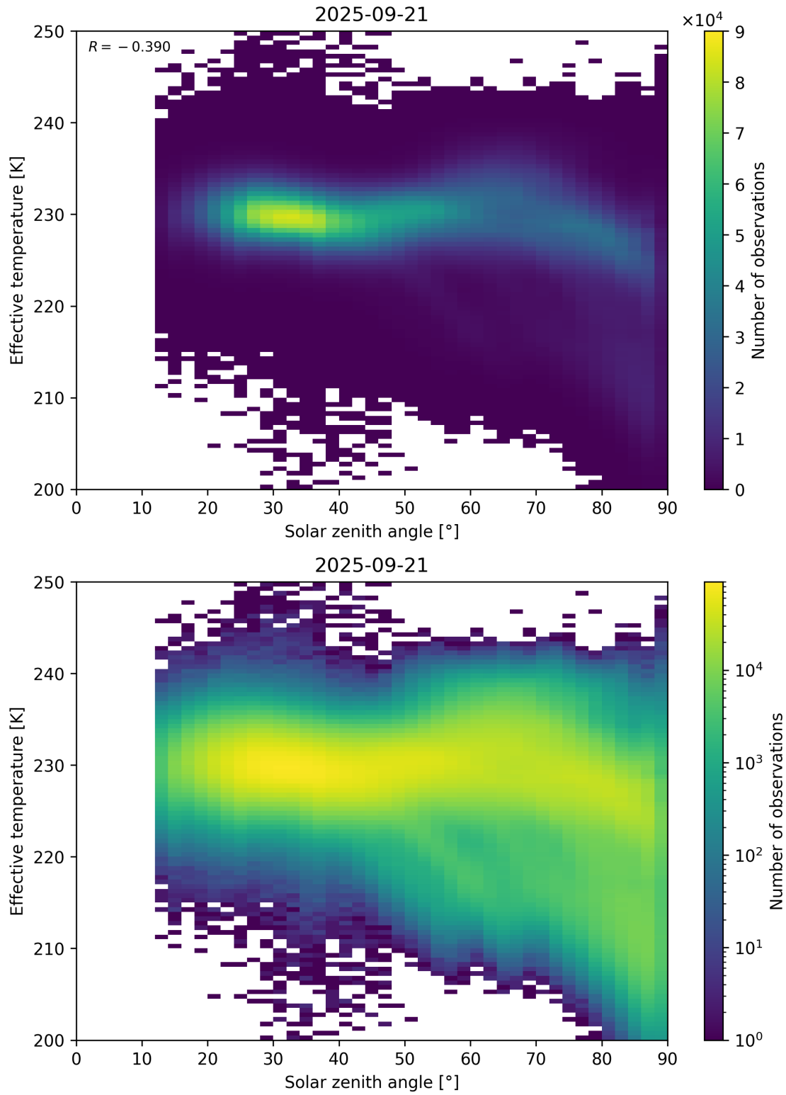
Figure 45: Scatter density plot of “Solar zenith angle” against “Effective temperature” for 2025-09-20 to 2025-09-22.
