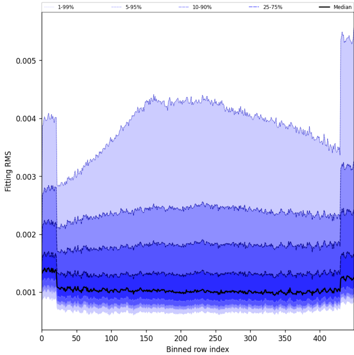
Figure 30: Along track statistics of “Fitting RMS” for 2025-09-20 to 2025-09-22
