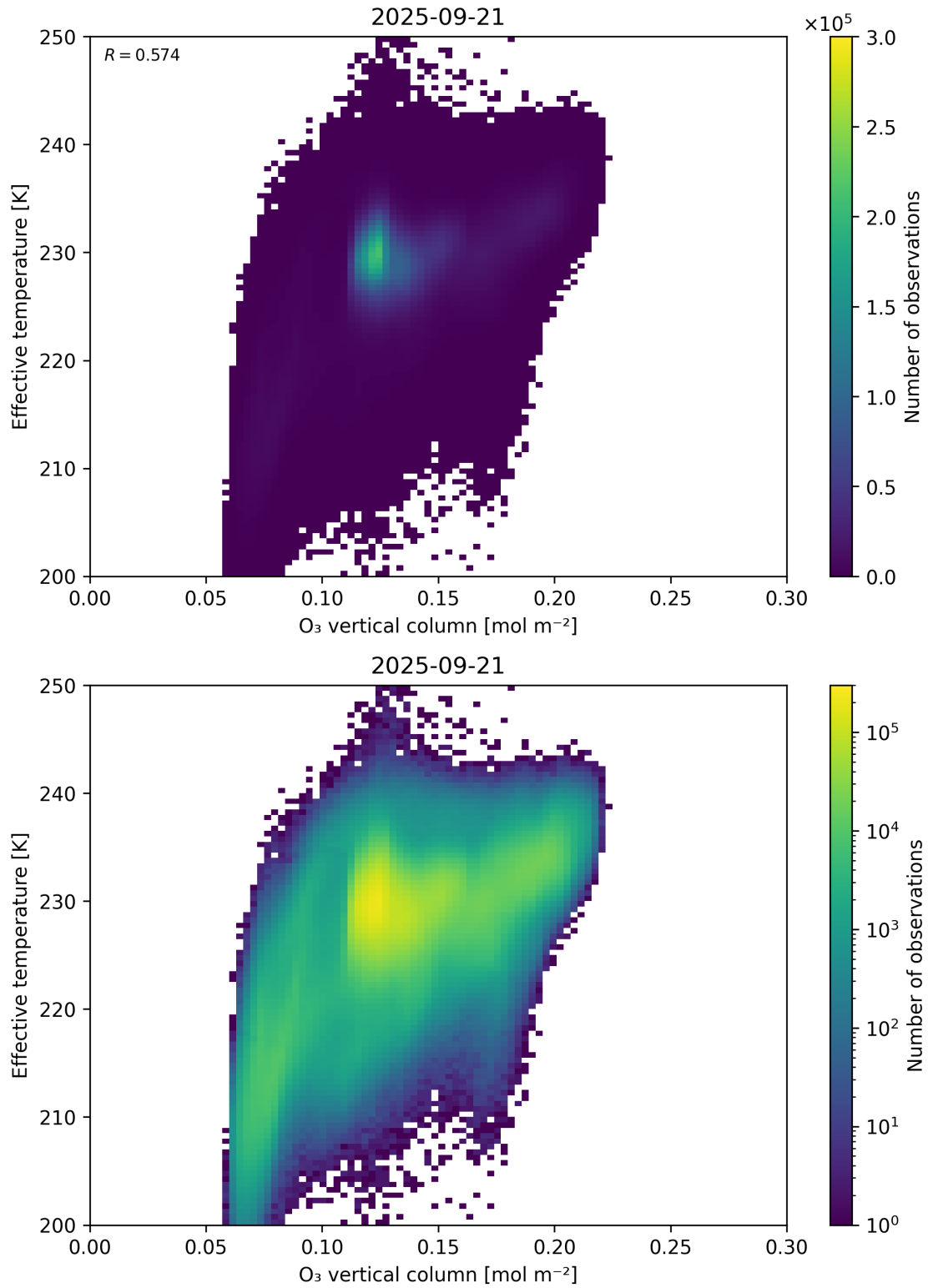
Figure 39: Scatter density plot of “O 3 vertical column” against “Effective temperature” for 2025-09-20 to 2025-09-22.
