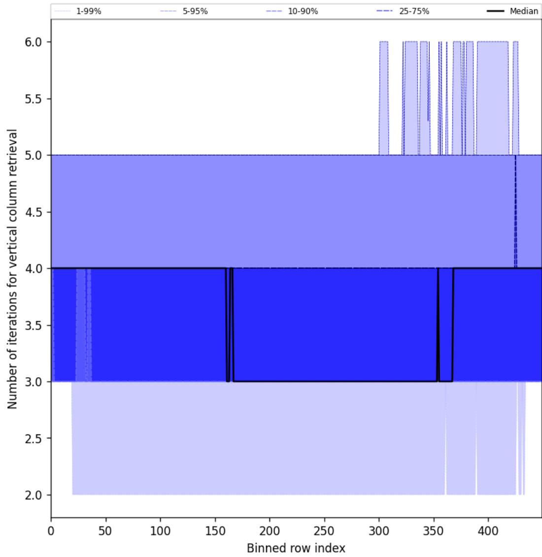
Figure 33: Along track statistics of “Number of iterations for vertical column retrieval” for 2025-09-20 to 2025-09-22
