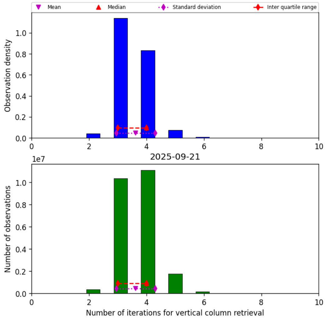
Figure 26: Histogram of “Number of iterations for vertical column retrieval” for 2025-09-20 to 2025-09-22
