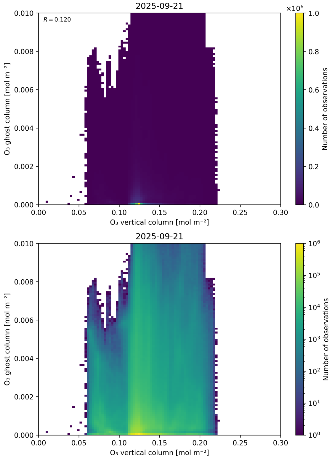
Figure 40: Scatter density plot of “O 3 vertical column” against “O 3 ghost column” for 2025-09-20 to 2025-09-22.
