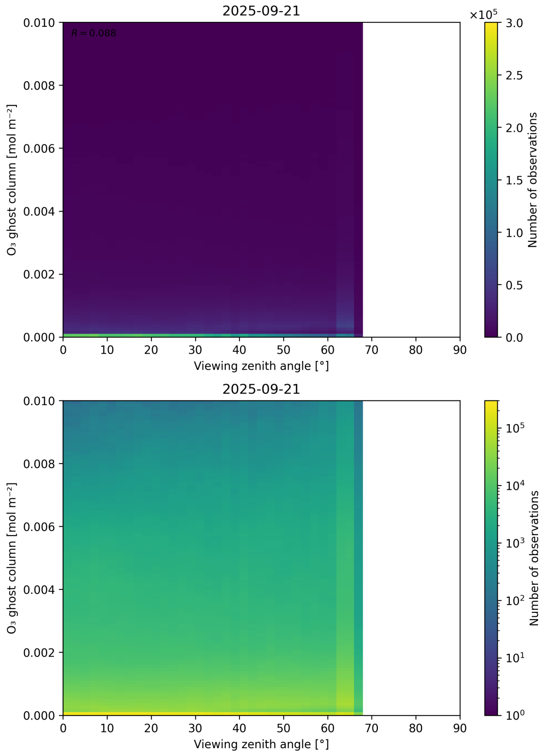
Figure 51: Scatter density plot of “Viewing zenith angle” against “O 3 ghost column” for 2025-09-20 to 2025-09-22.
