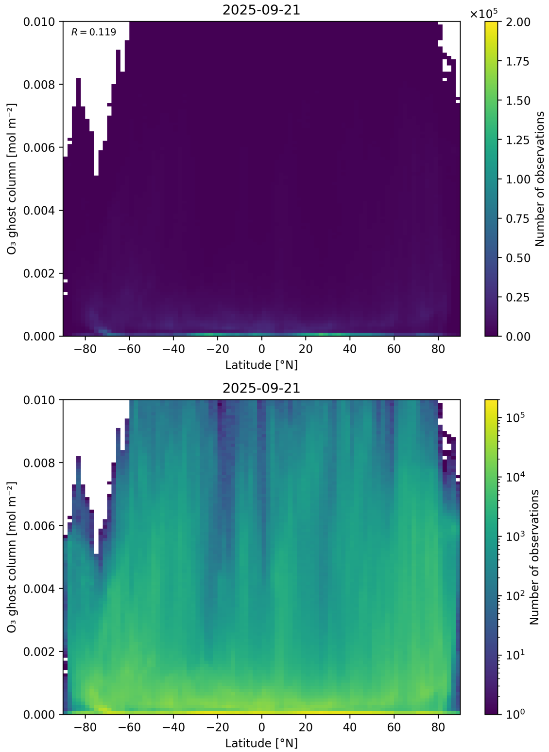
Figure 35: Scatter density plot of “Latitude” against “O 3 ghost column” for 2025-09-20 to 2025-09-22.
