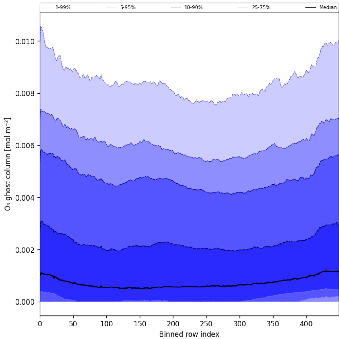
Figure 32: Along track statistics of “O 3 ghost column” for 2025-09-20 to 2025-09-22
