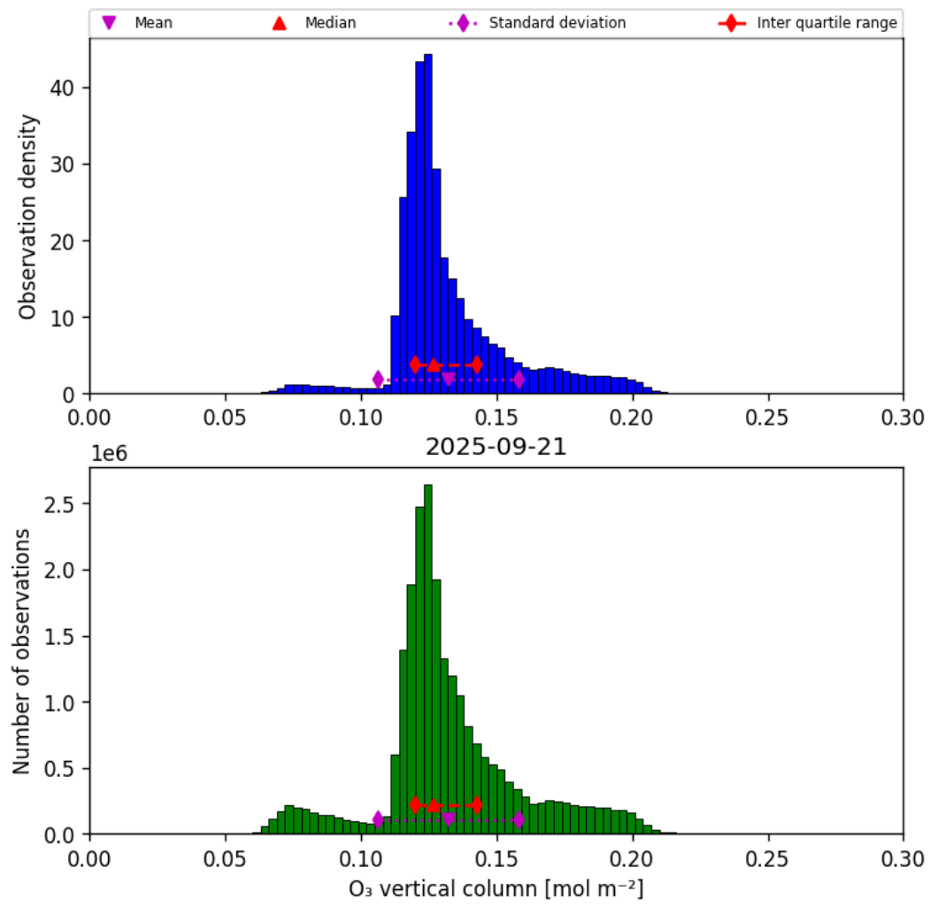
Figure 21: Histogram of “O 3 vertical column” for 2025-09-20 to 2025-09-22
