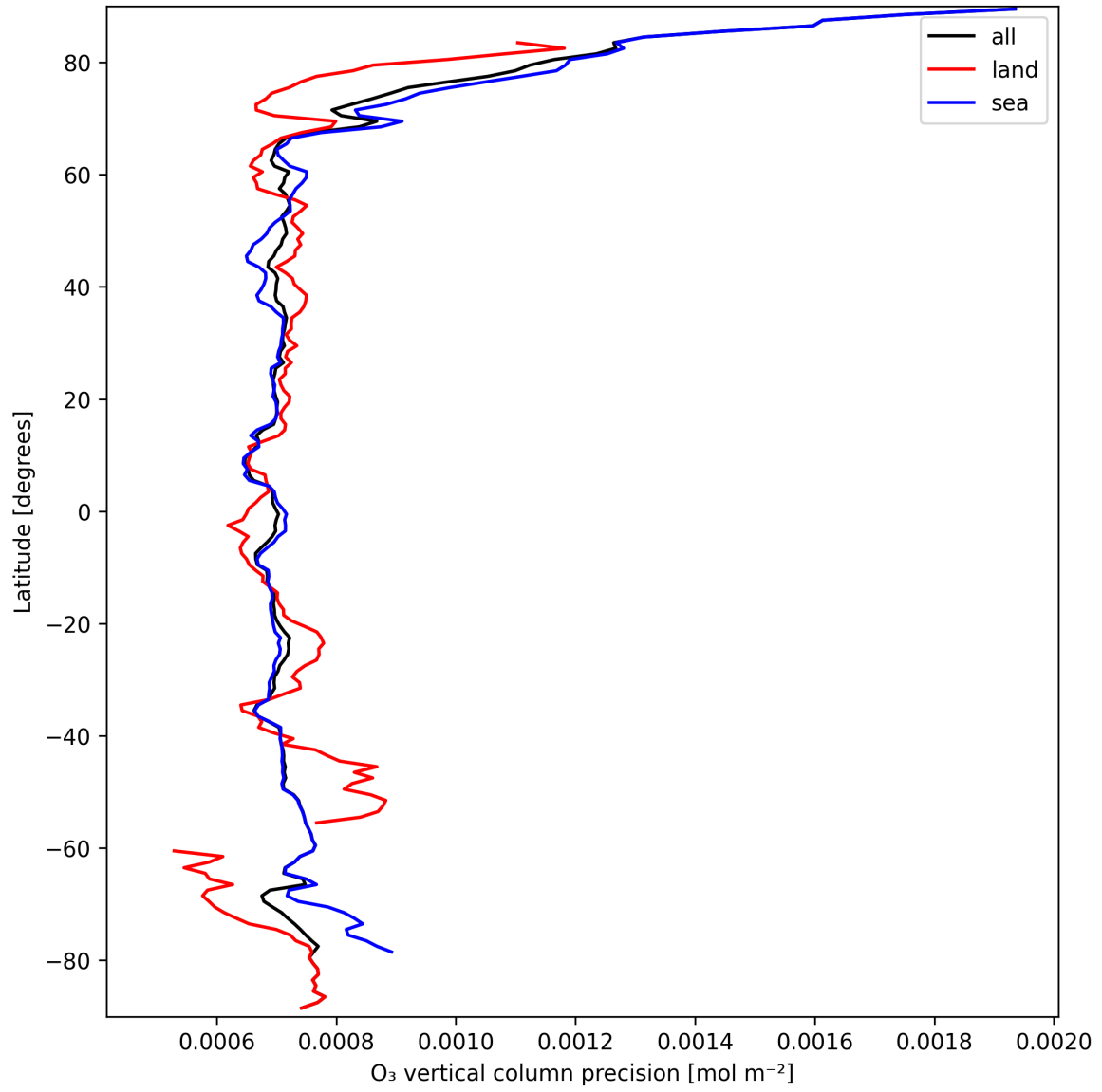
Figure 15: Zonal average of “O 3 vertical column precision” for 2025-09-20 to 2025-09-22.
