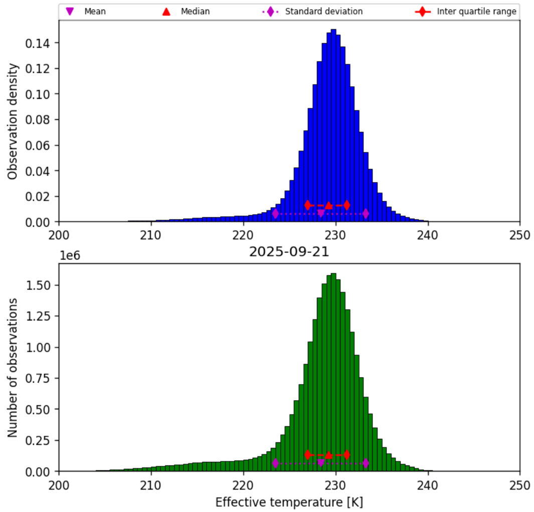
Figure 24: Histogram of “Effective temperature” for 2025-09-20 to 2025-09-22
