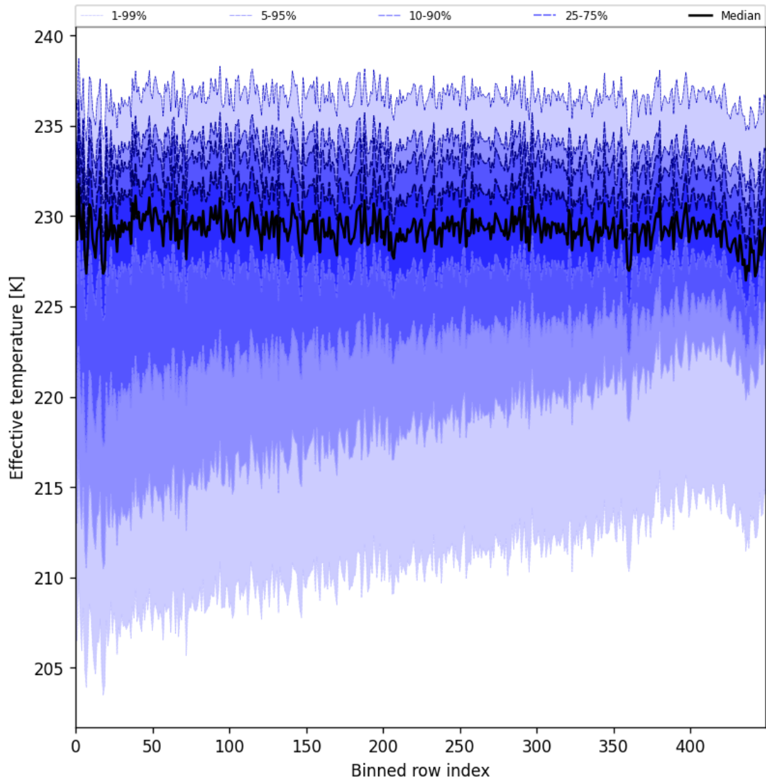
Figure 31: Along track statistics of “Effective temperature” for 2025-09-20 to 2025-09-22
