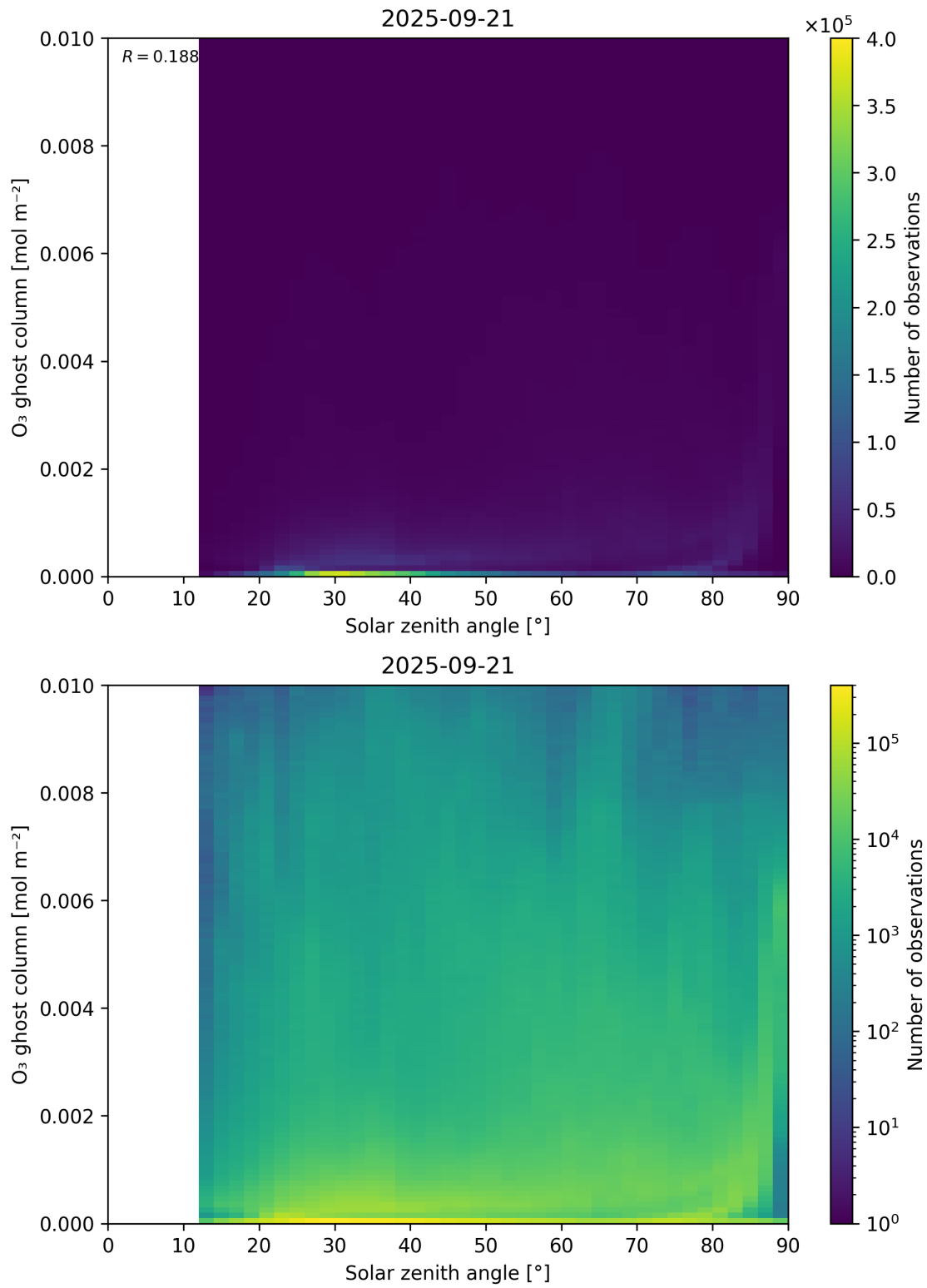
Figure 46: Scatter density plot of “Solar zenith angle” against “O 3 ghost column” for 2025-09-20 to 2025-09-22.
