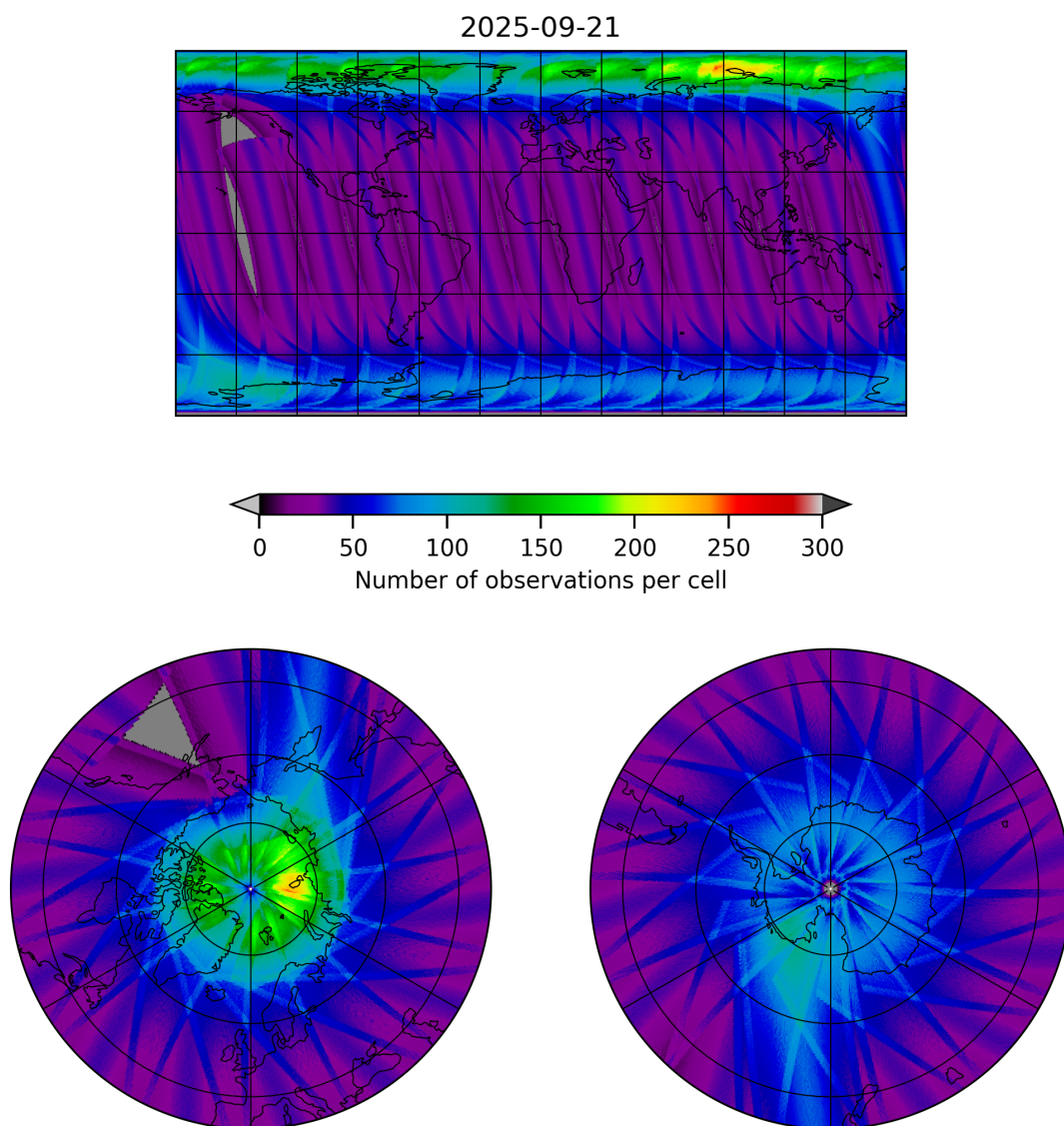
Figure 12: Map of the number of observations for 2025-09-20 to 2025-09-22
