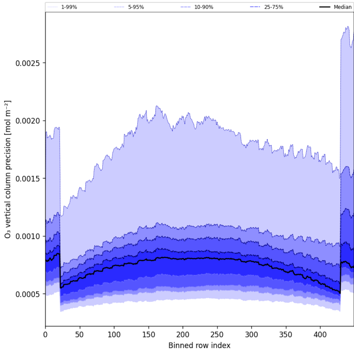
Figure 29: Along track statistics of “O 3 vertical column precision” for 2025-09-20 to 2025-09-22
