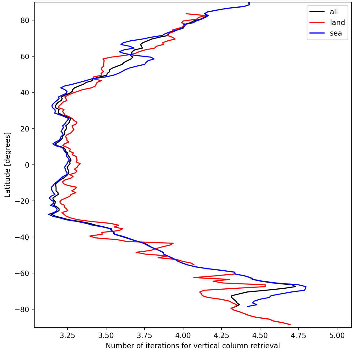
Figure 19: Zonal average of “Number of iterations for vertical column retrieval” for 2025-09-20 to 2025-09-22.
