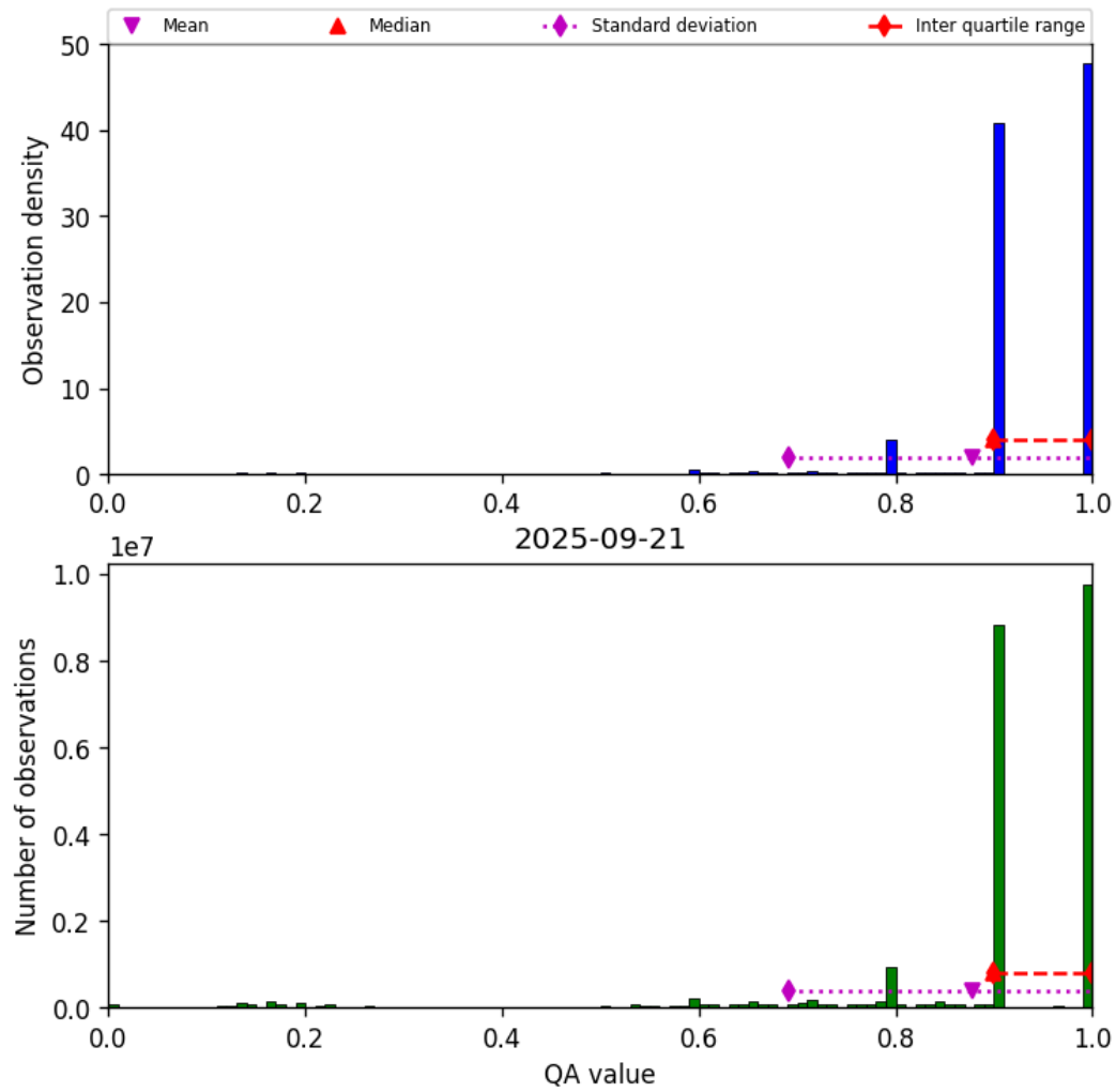
Figure 20: Histogram of “QA value” for 2025-09-20 to 2025-09-22
