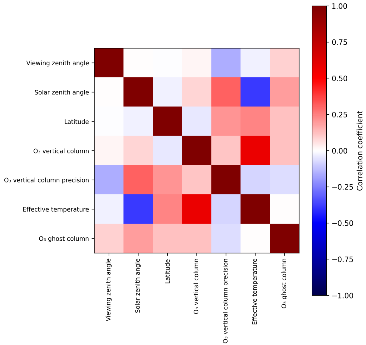
Figure 2: Map of correlation matrix for 2025-09-20 to 2025-09-22.
