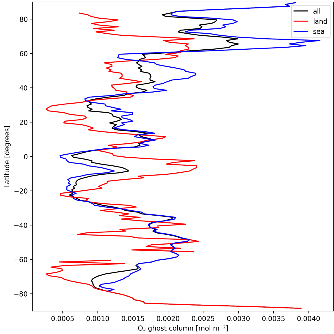
Figure 18: Zonal average of “O 3 ghost column” for 2025-09-20 to 2025-09-22.
