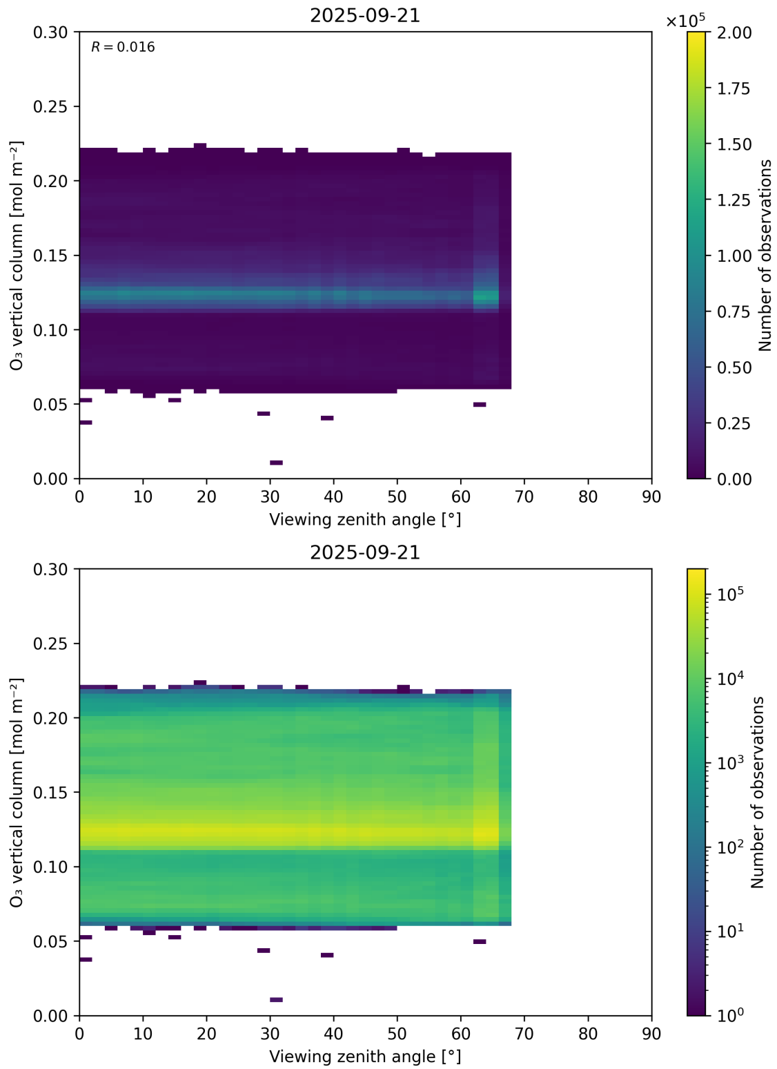
Figure 52: Scatter density plot of “Viewing zenith angle” against “O 3 vertical column” for 2025-09-20 to 2025-09-22.
