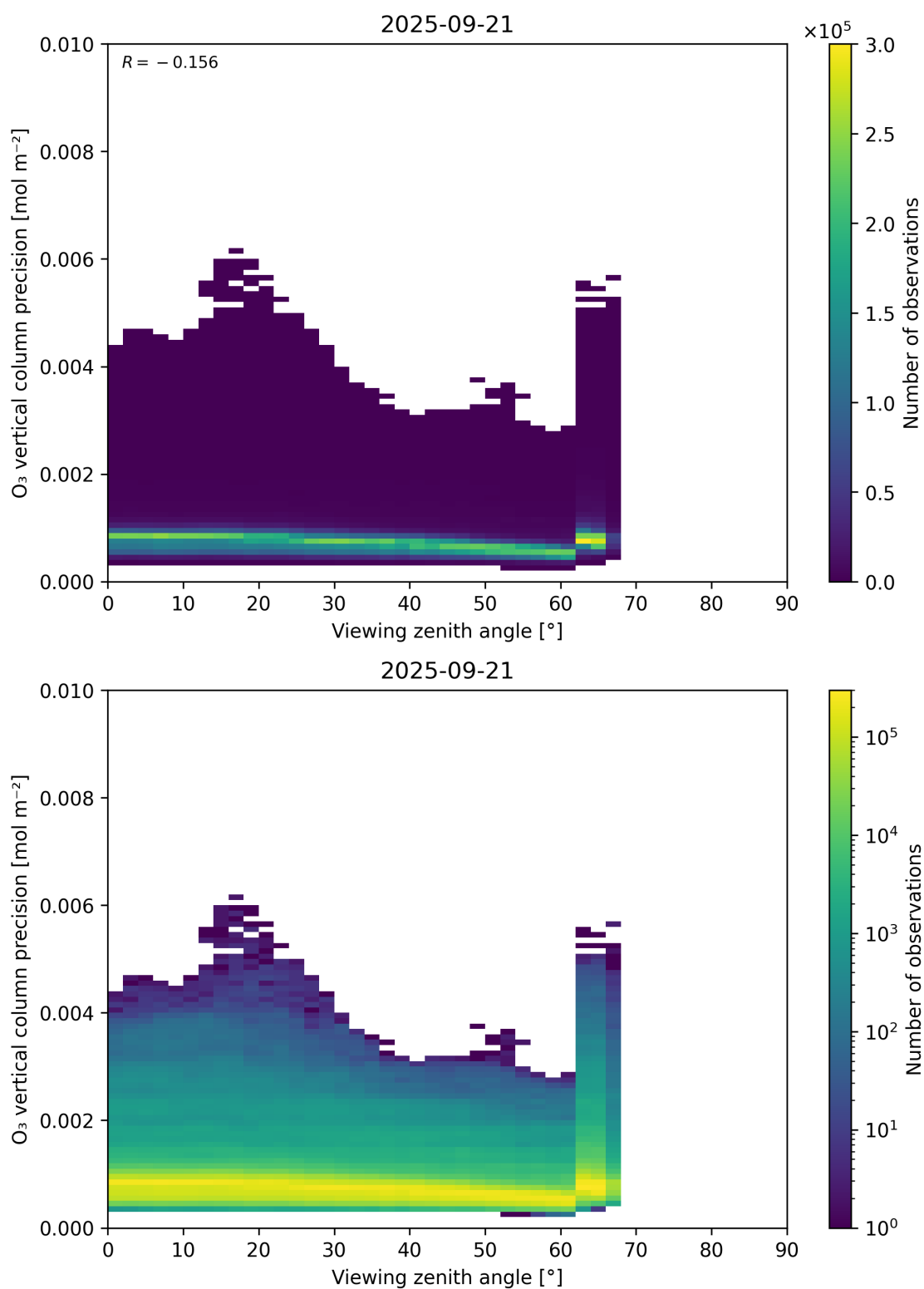
Figure 53: Scatter density plot of “Viewing zenith angle” against “O 3 vertical column precision” for 2025-09-20 to 2025-09-22.
