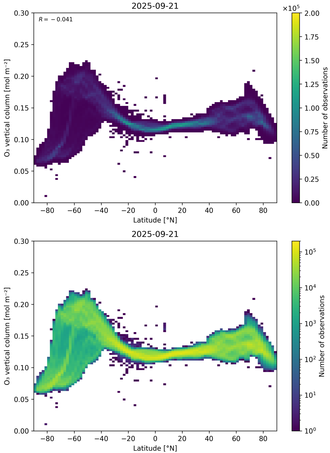
Figure 36: Scatter density plot of “Latitude” against “O 3 vertical column” for 2025-09-20 to 2025-09-22.
