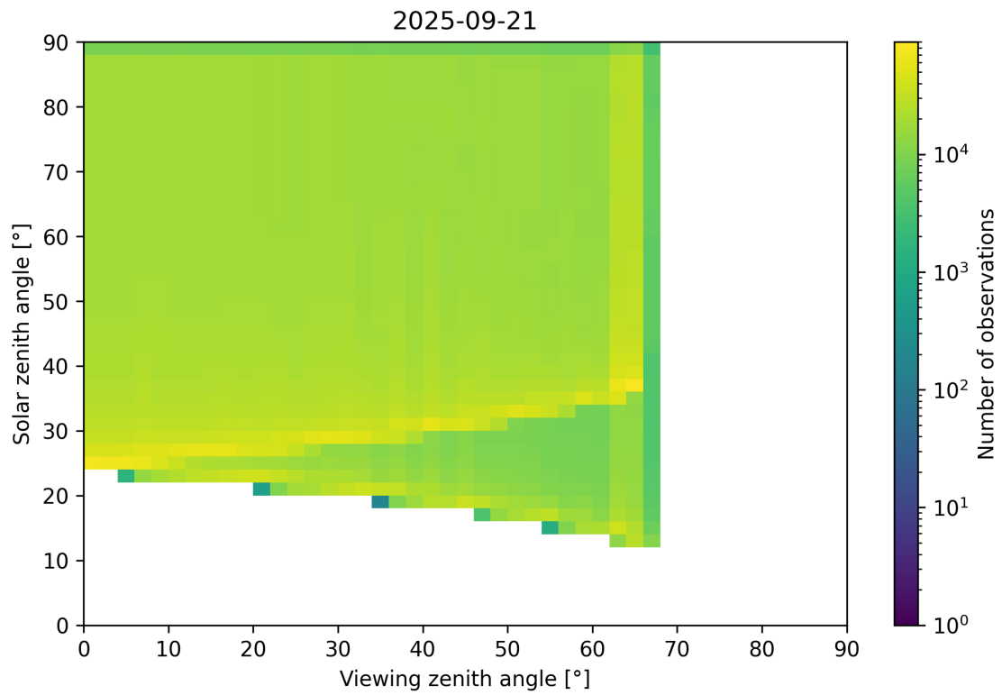
Figure 54: Scatter density plot of “Viewing zenith angle” against “Solar zenith angle” for 2025-09-20 to 2025-09-22.
