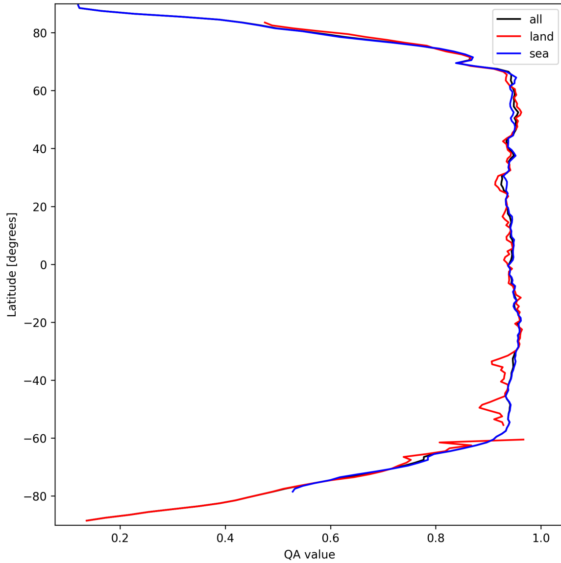
Figure 13: Zonal average of “QA value” for 2025-09-20 to 2025-09-22.
