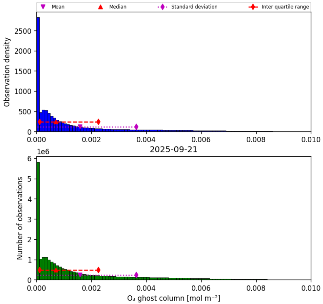
Figure 25: Histogram of “O 3 ghost column” for 2025-09-20 to 2025-09-22
