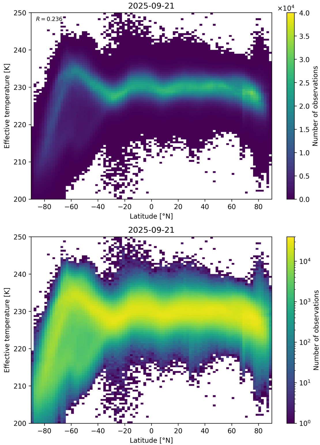
Figure 34: Scatter density plot of “Latitude” against “Effective temperature” for 2025-09-20 to 2025-09-22.
