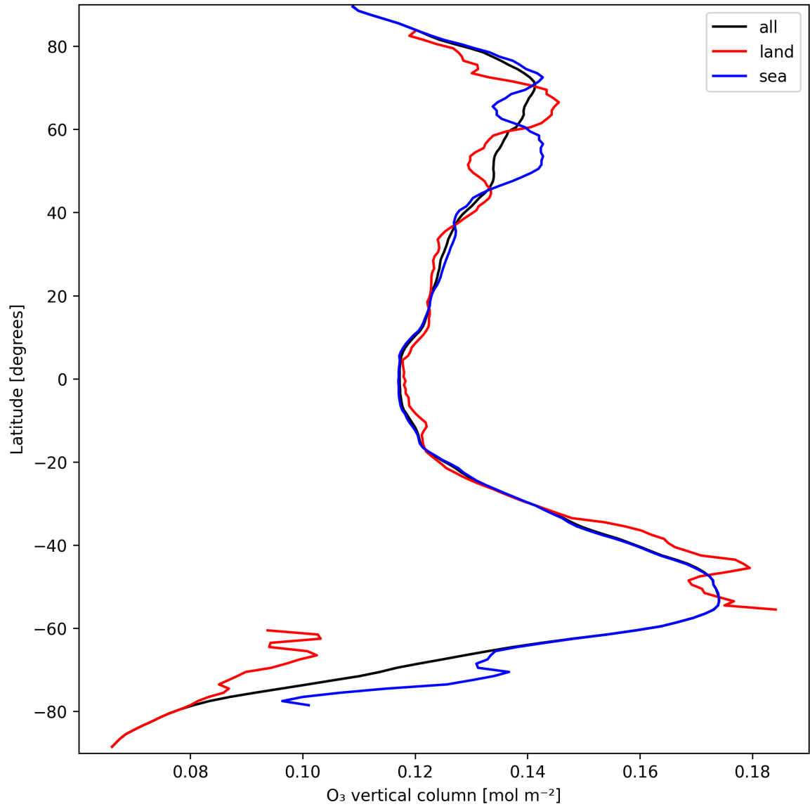
Figure 14: Zonal average of “O 3 vertical column” for 2025-09-20 to 2025-09-22.
