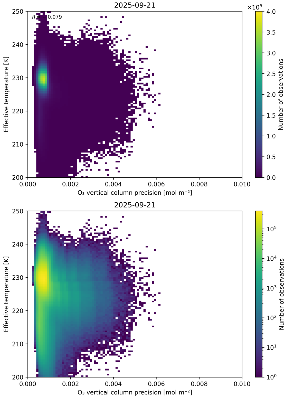
Figure 42: Scatter density plot of “ O_3 vertical column precision” against “Effective temperature” for 2025-09-20 to 2025-09-22.
