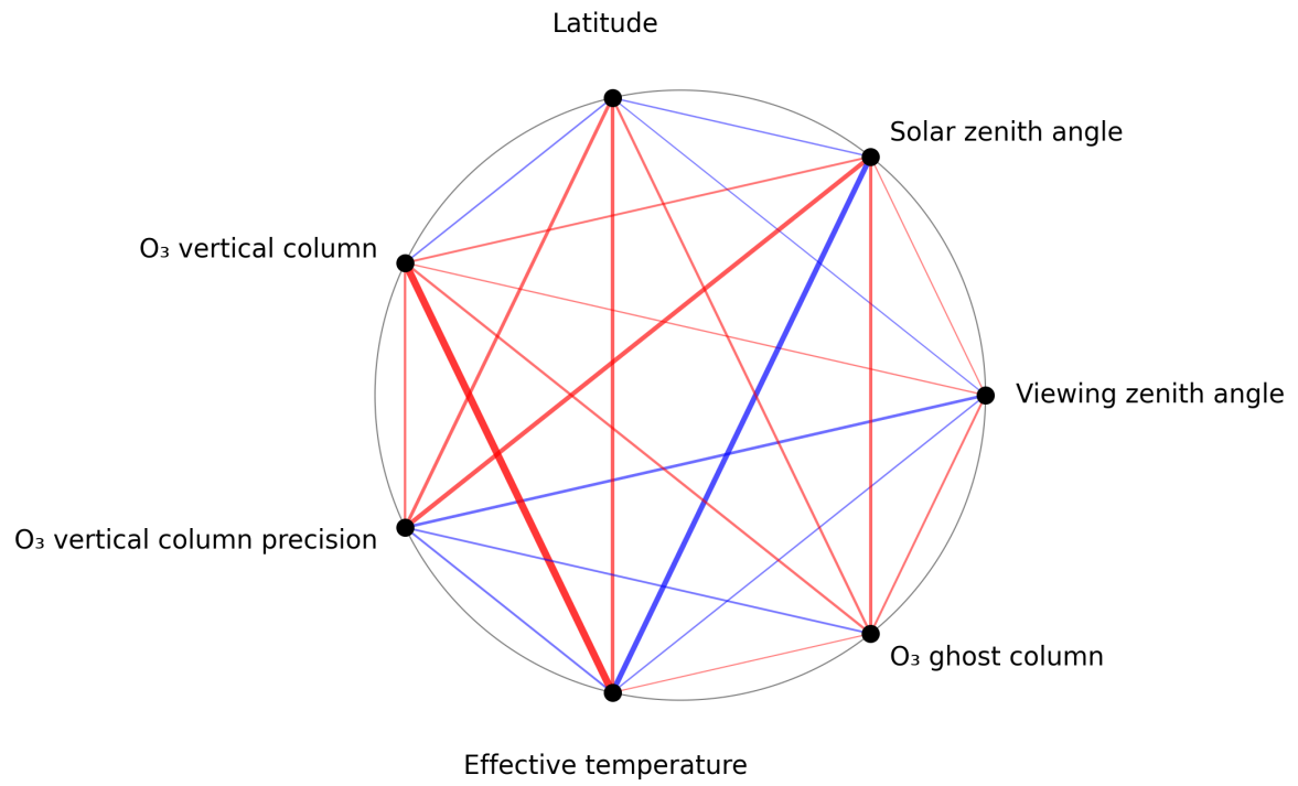
Figure 1: Map of correlation graph for 2025-09-20 to 2025-09-22.
