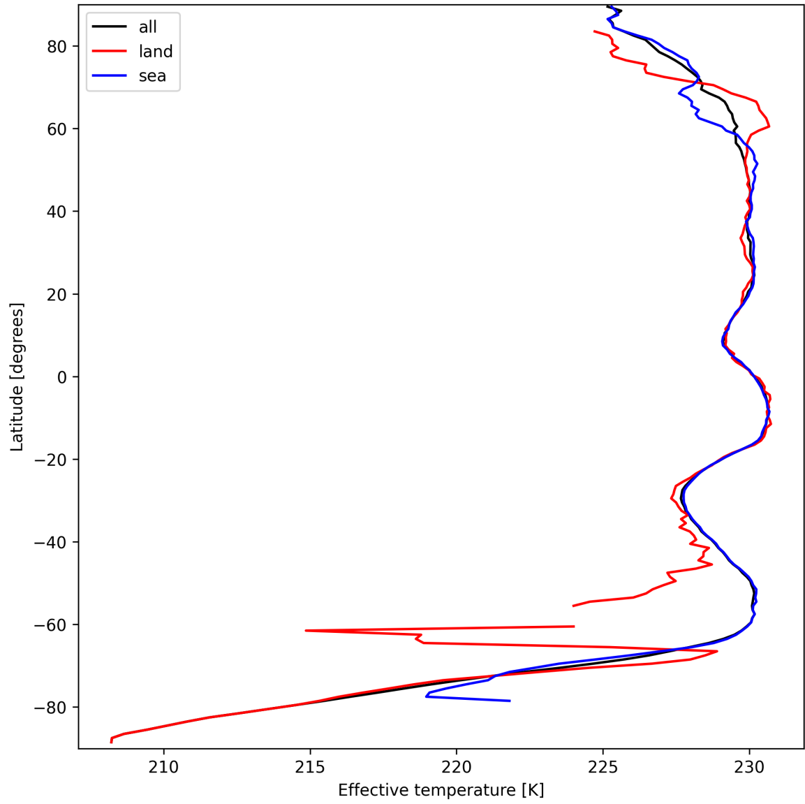
Figure 17: Zonal average of “Effective temperature” for 2025-09-20 to 2025-09-22.
