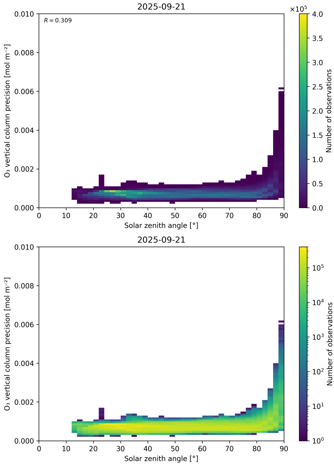
Figure 48: Scatter density plot of “Solar zenith angle” against “O 3 vertical column precision” for 2025-09-20 to 2025-09-22.
