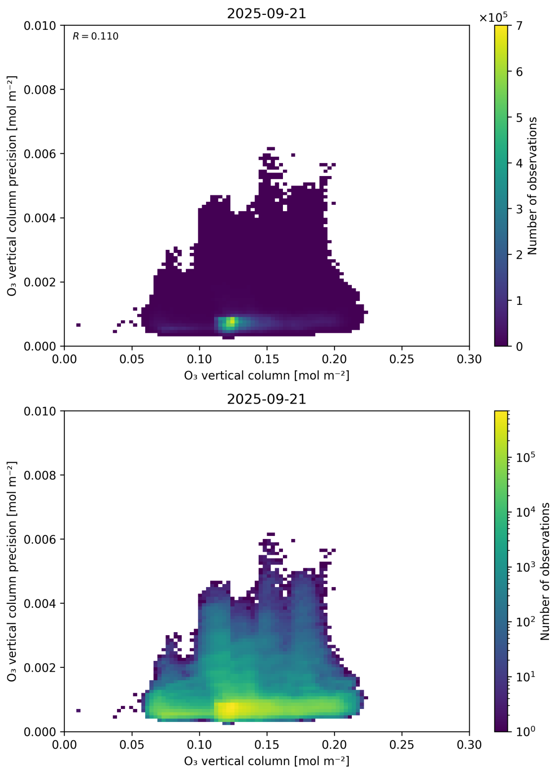
Figure 41: Scatter density plot of “O 3 vertical column” against “O 3 vertical column precision” for 2025-09-20 to 2025-09-22.
