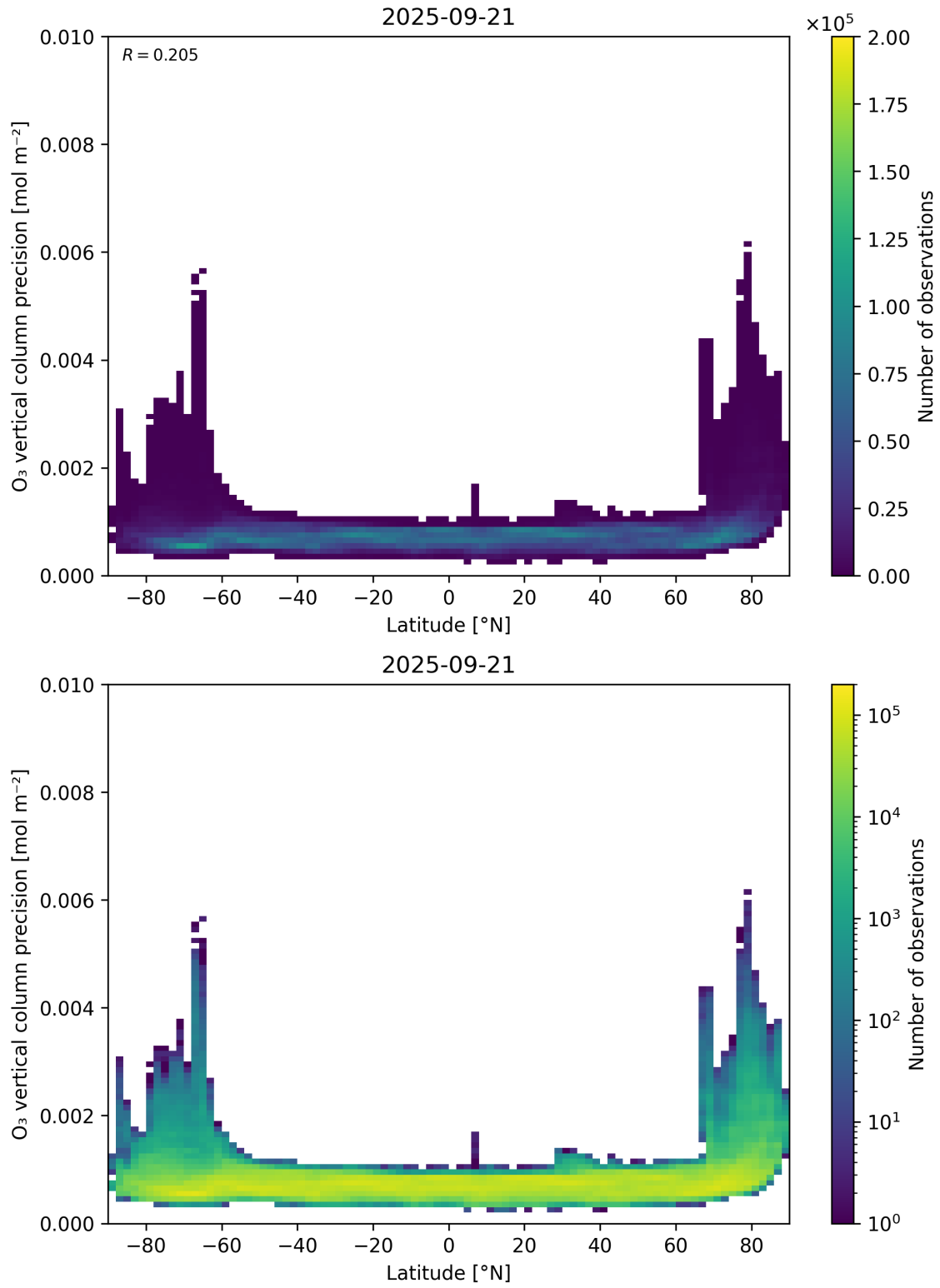
Figure 37: Scatter density plot of “Latitude” against “O 3 vertical column precision” for 2025-09-20 to 2025-09-22.
