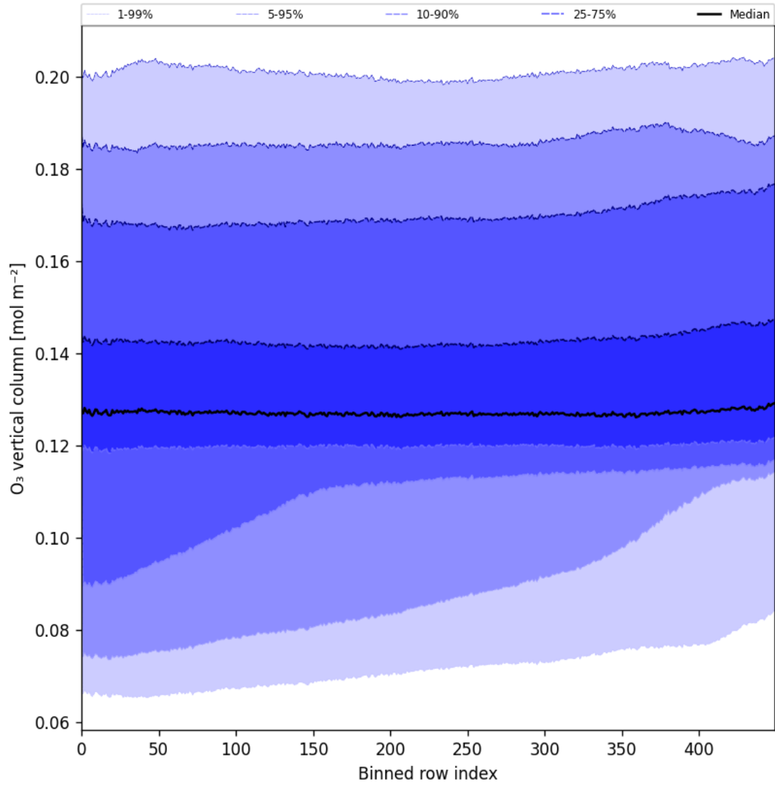
Figure 28: Along track statistics of “O 3 vertical column” for 2025-09-20 to 2025-09-22
