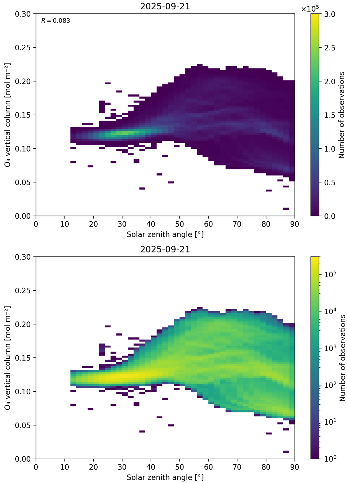
Figure 47: Scatter density plot of “Solar zenith angle” against “O 3 vertical column” for 2025-09-20 to 2025-09-22.
