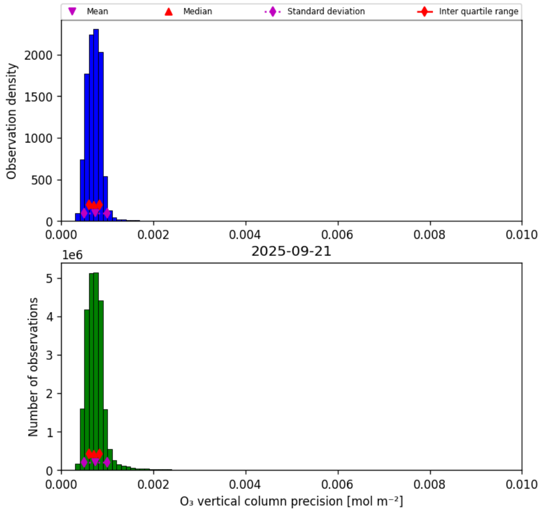
Figure 22: Histogram of “O 3 vertical column precision” for 2025-09-20 to 2025-09-22
