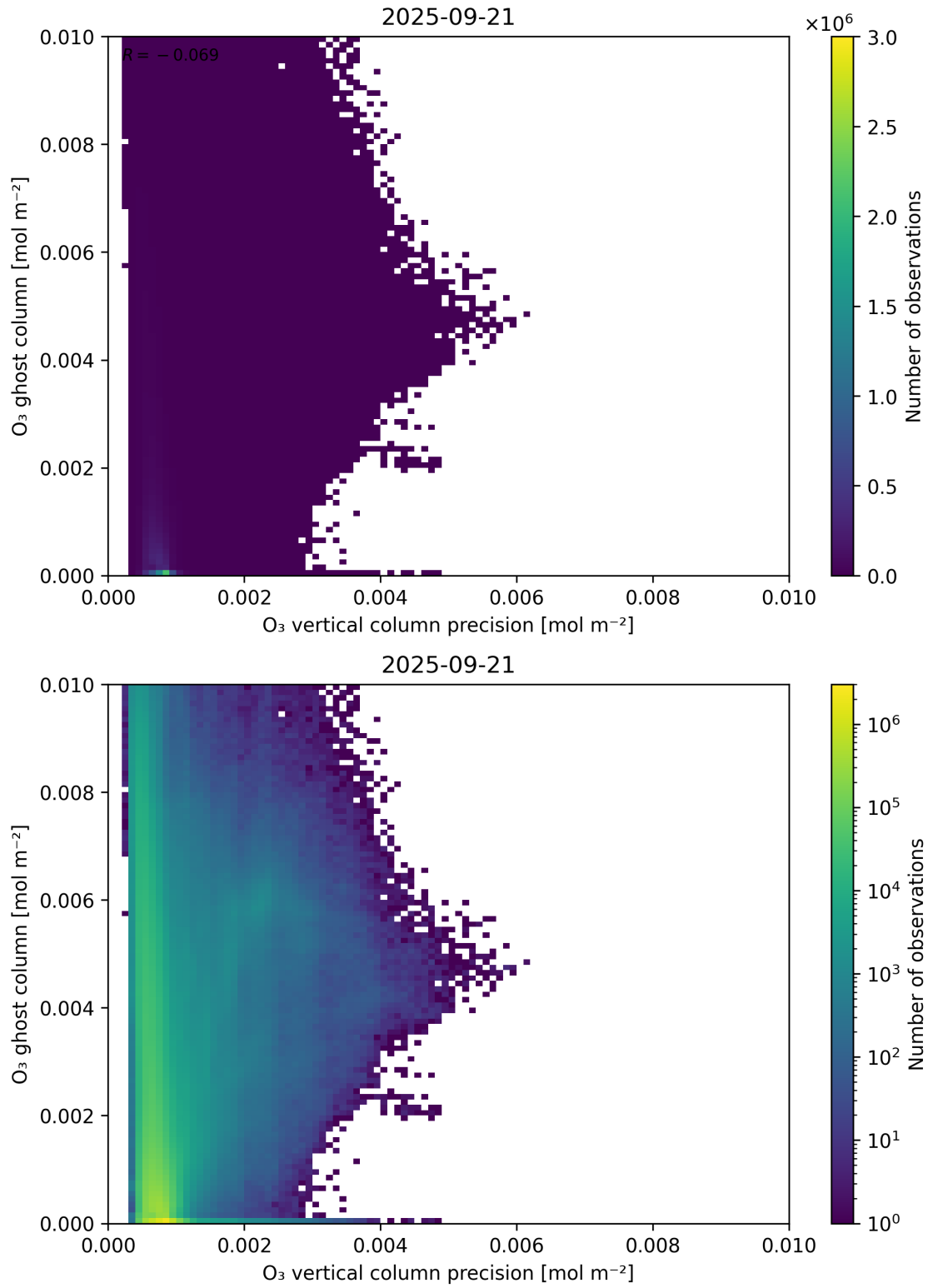
Figure 43: Scatter density plot of “O 3 vertical column precision” against “O 3 ghost column” for 2025-09-20 to 2025-09-22.
