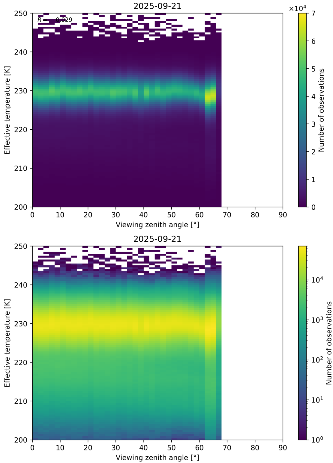
Figure 50: Scatter density plot of “Viewing zenith angle” against “Effective temperature” for 2025-09-20 to 2025-09-22.
