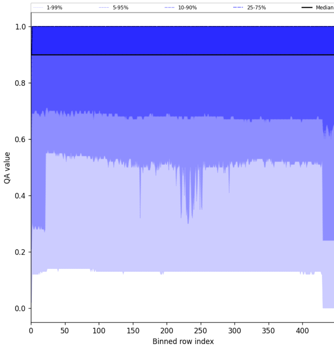
Figure 27: Along track statistics of “QA value” for 2025-09-20 to 2025-09-22
