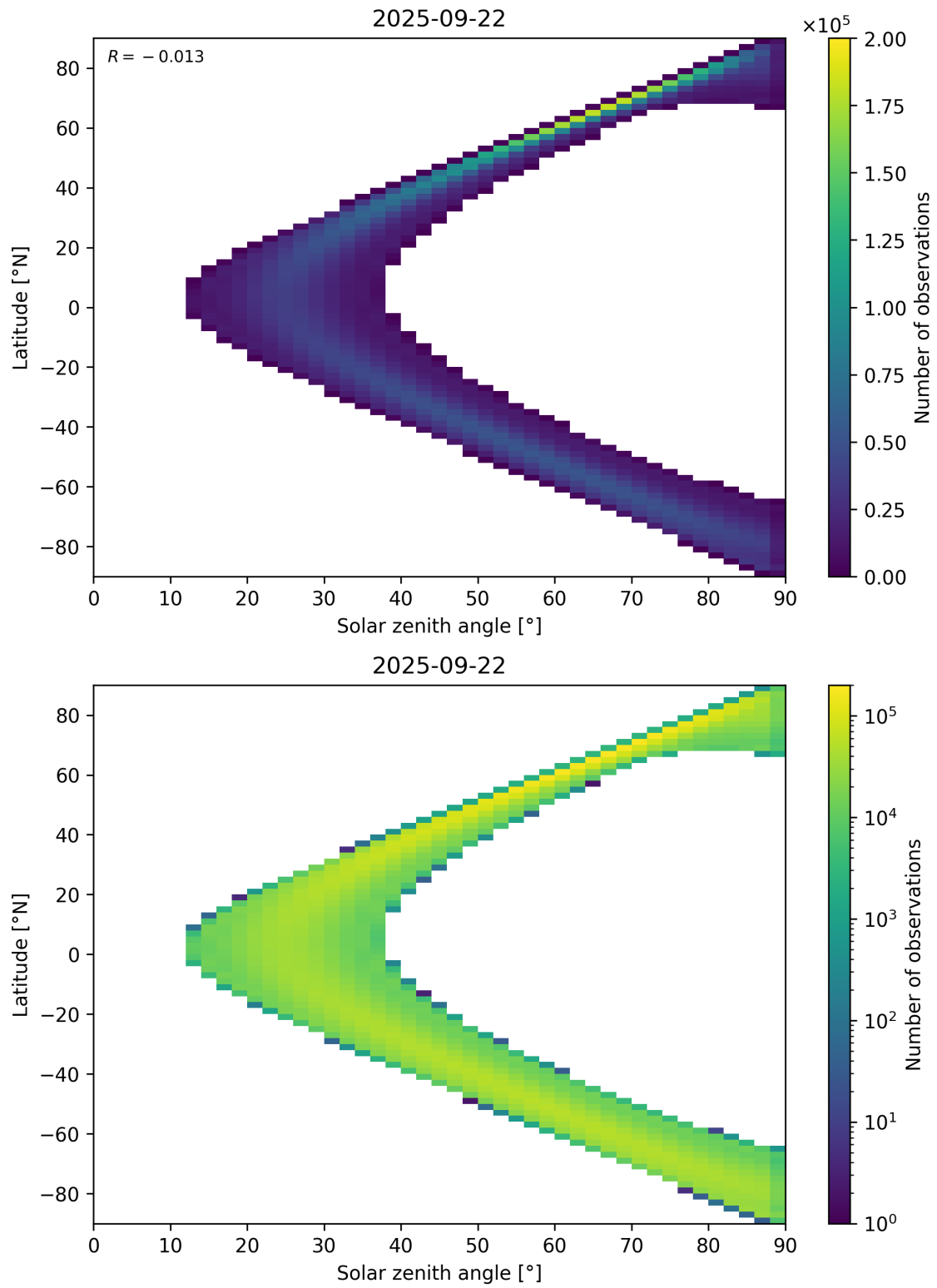
Figure 44: Scatter density plot of “Solar zenith angle” against “Latitude” for 2025-09-22 to 2025-09-23.
