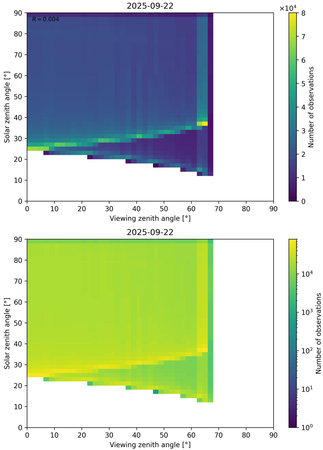
Figure 54: Scatter density plot of “Viewing zenith angle” against “Solar zenith angle” for 2025-09-22 to 2025-09-23.
