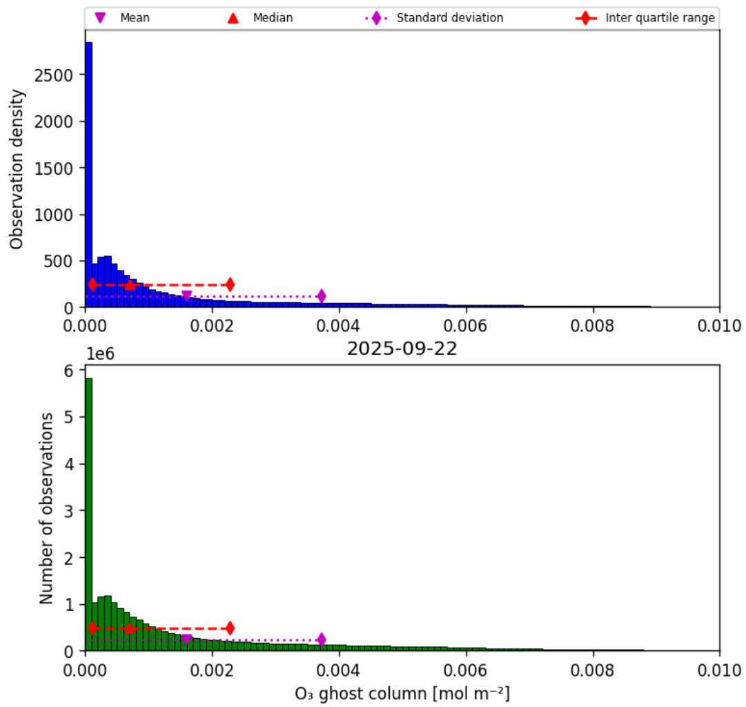
Figure 25: Histogram of “O 3 ghost column” for 2025-09-22 to 2025-09-23
