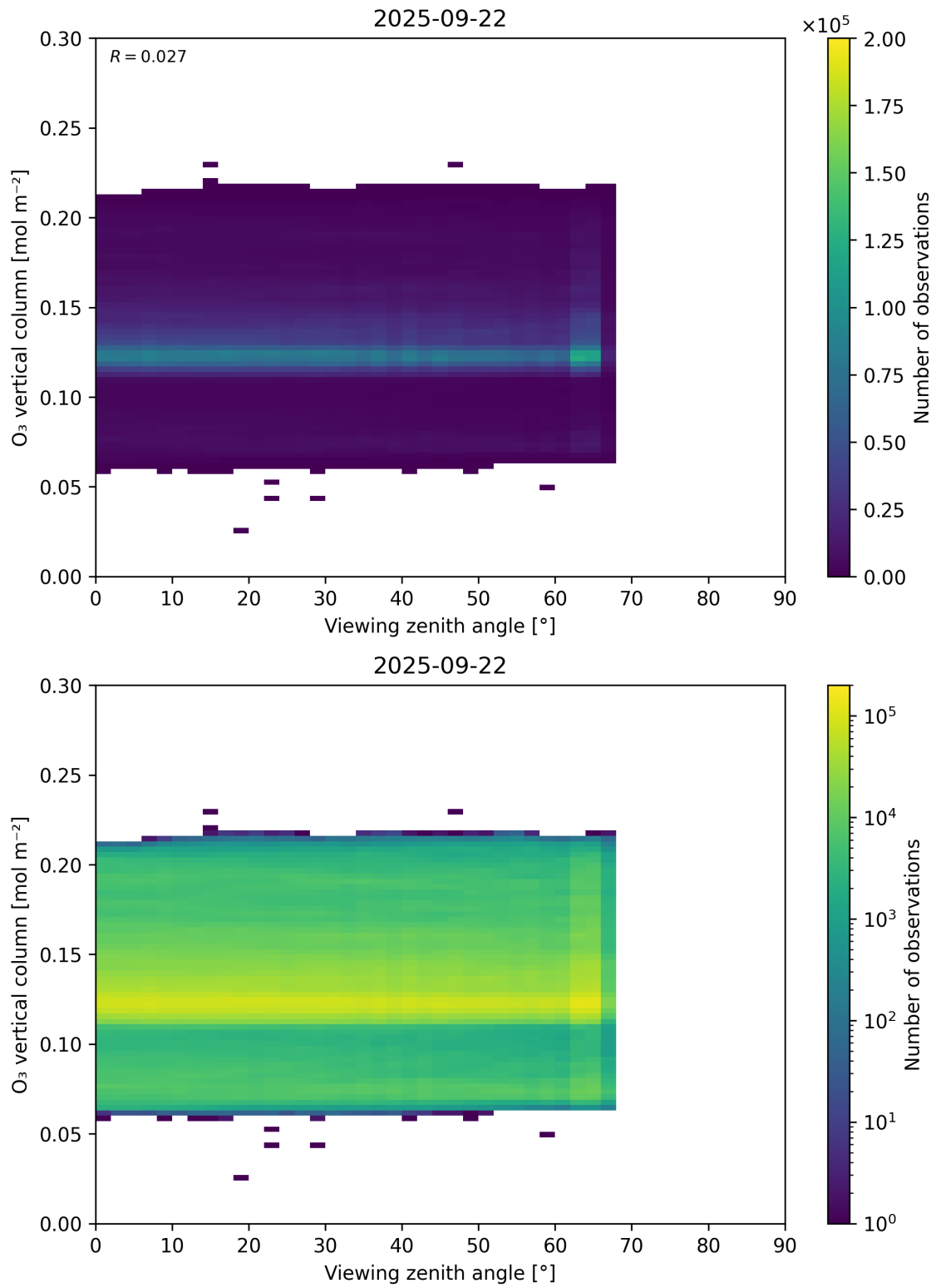
Figure 52: Scatter density plot of “Viewing zenith angle” against “O 3 vertical column” for 2025-09-22 to 2025-09-23.
