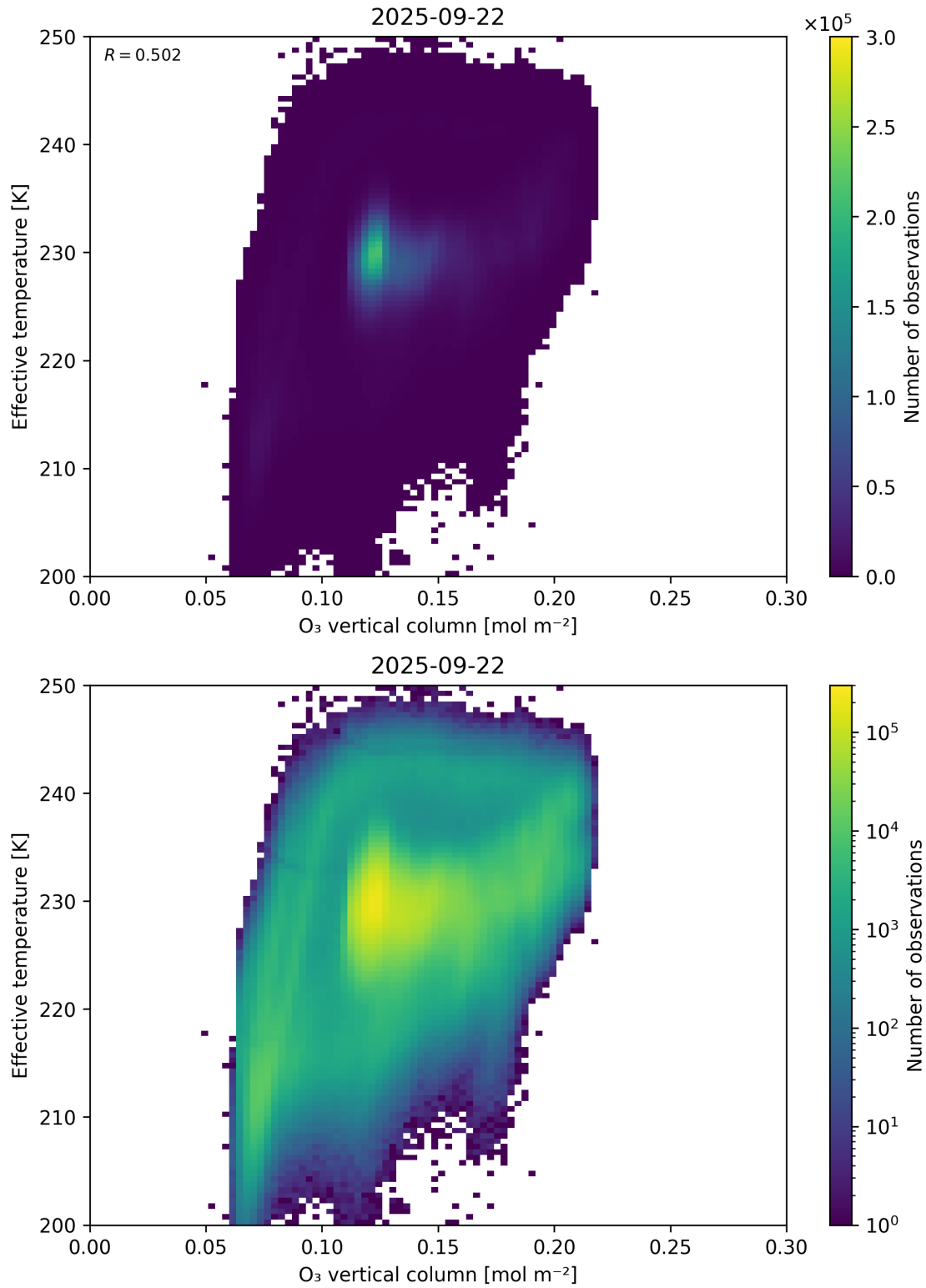
Figure 39: Scatter density plot of “O 3 vertical column” against “Effective temperature” for 2025-09-22 to 2025-09-23.
