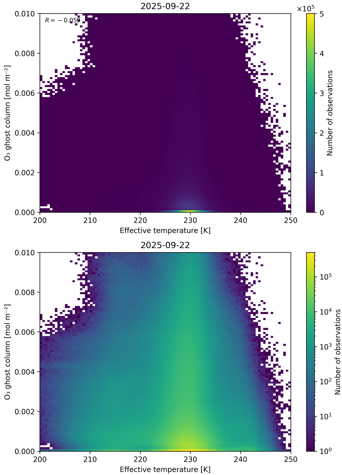
Figure 38: Scatter density plot of “Effective temperature” against “O 3 ghost column” for 2025-09-22 to 2025-09-23.
