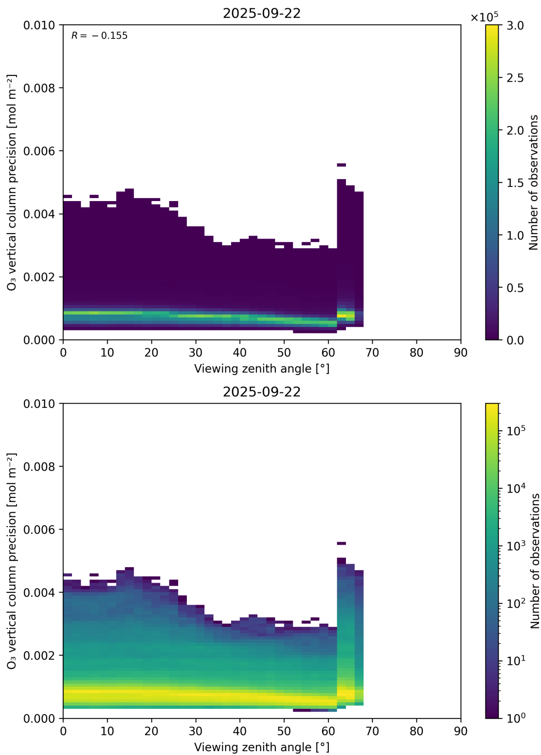
Figure 53: Scatter density plot of “Viewing zenith angle” against “O 3 vertical column precision” for 2025-09-22 to 2025-09-23.
