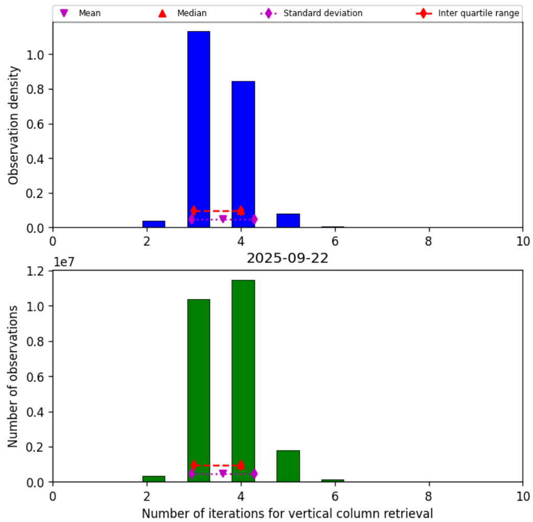
Figure 26: Histogram of “Number of iterations for vertical column retrieval” for 2025-09-22 to 2025-09-23
