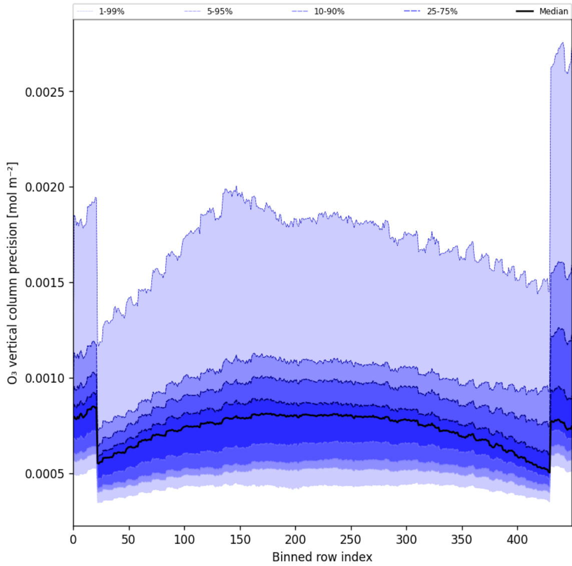
Figure 29: Along track statistics of “O 3 vertical column precision” for 2025-09-22 to 2025-09-23
