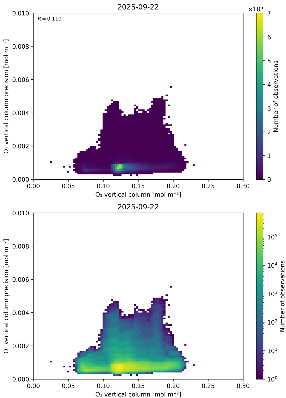
Figure 41: Scatter density plot of “O 3 vertical column” against “O 3 vertical column precision” for 2025-09-22 to 2025-09-23.
