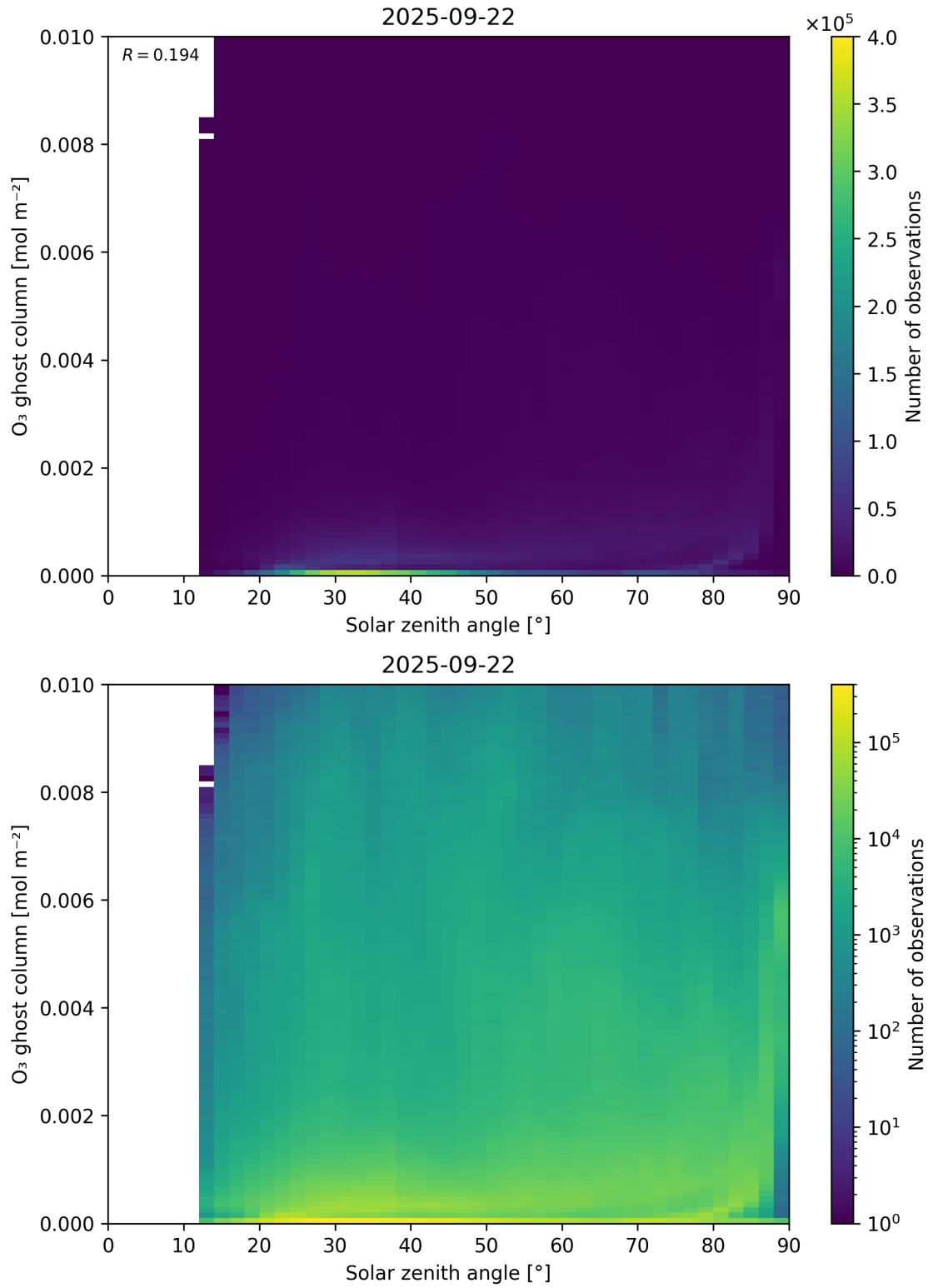
Figure 46: Scatter density plot of “Solar zenith angle” against “O 3 ghost column” for 2025-09-22 to 2025-09-23.
