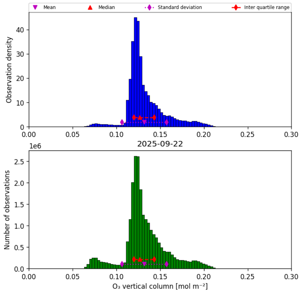
Figure 21: Histogram of “O 3 vertical column” for 2025-09-22 to 2025-09-23
