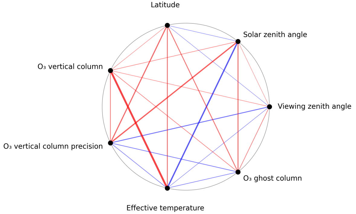
Figure 1: Map of correlation graph for 2025-09-22 to 2025-09-23.
