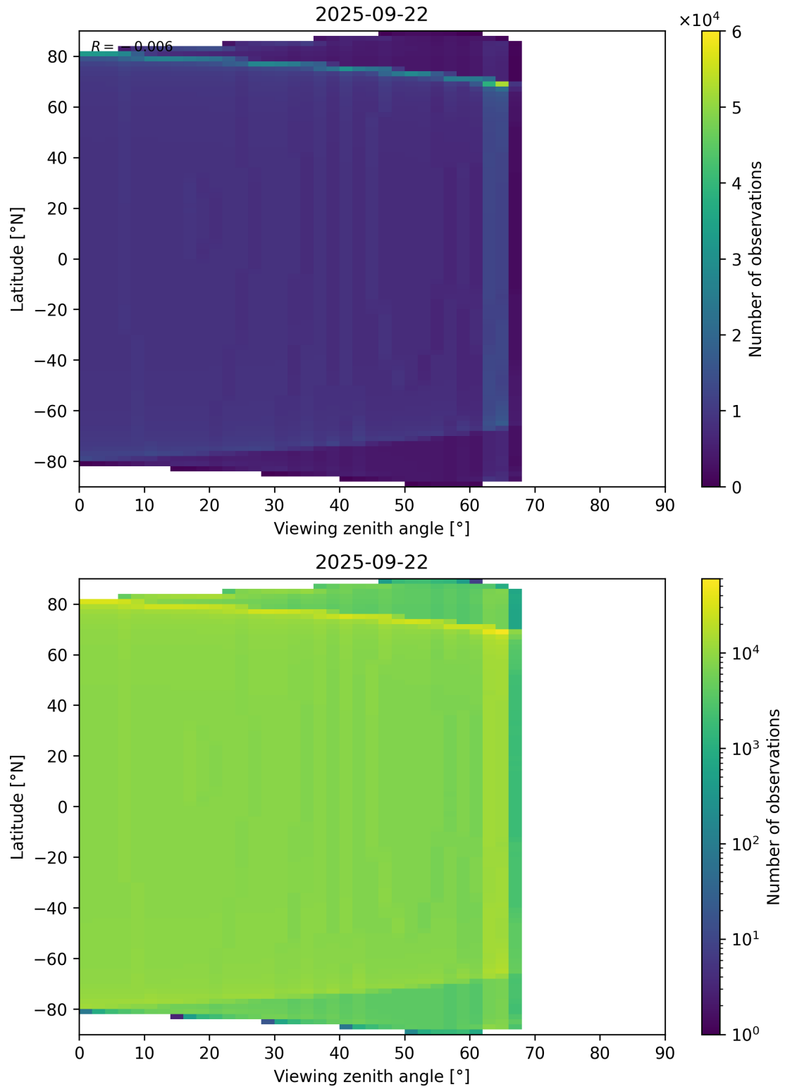
Figure 49: Scatter density plot of “Viewing zenith angle” against “Latitude” for 2025-09-22 to 2025-09-23.
