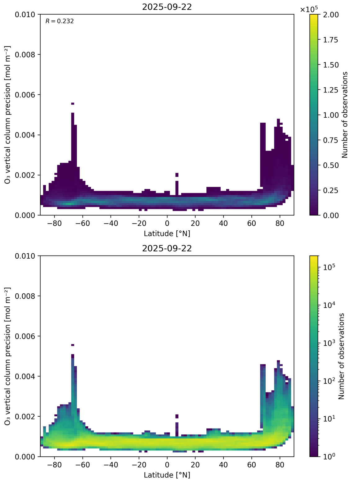
Figure 37: Scatter density plot of “Latitude” against “O 3 vertical column precision” for 2025-09-22 to 2025-09-23.
