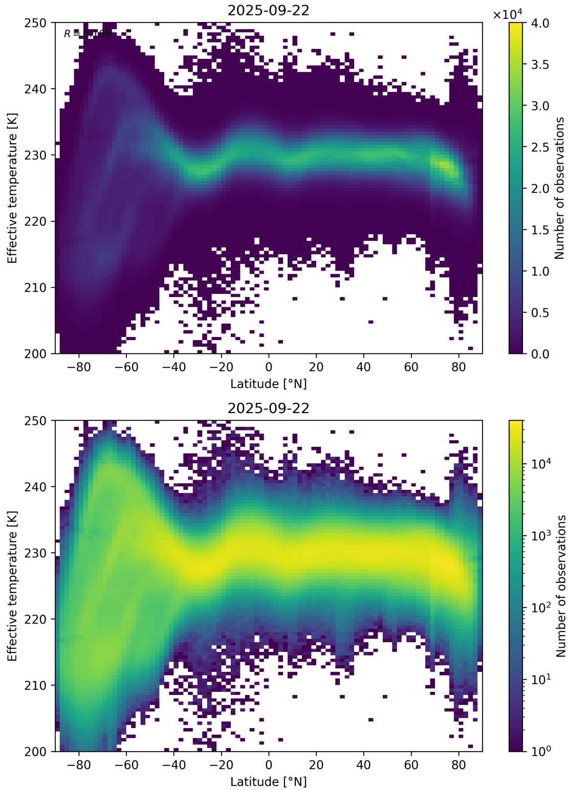
Figure 34: Scatter density plot of “Latitude” against “Effective temperature” for 2025-09-22 to 2025-09-23.
