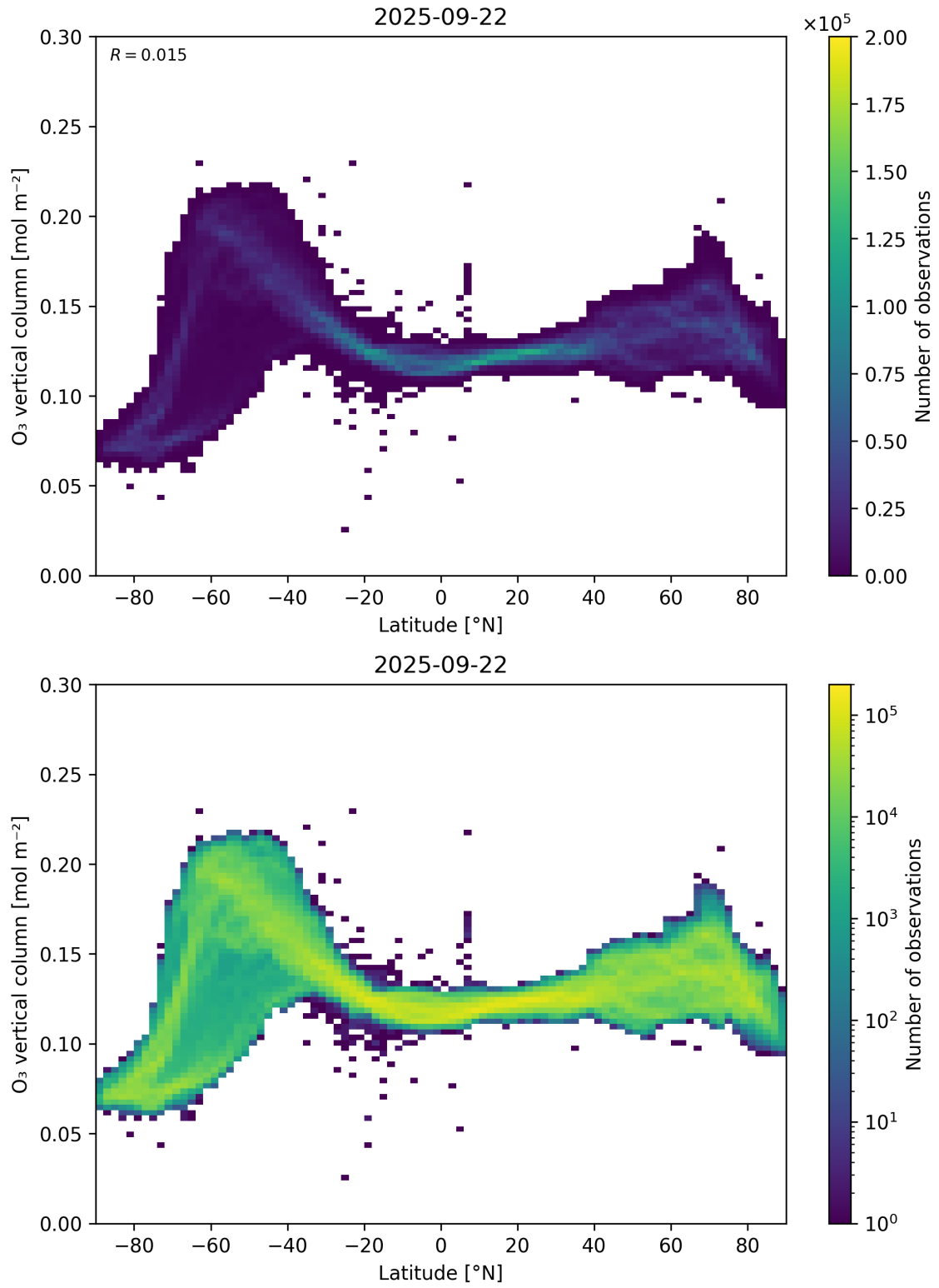
Figure 36: Scatter density plot of “Latitude” against “O 3 vertical column” for 2025-09-22 to 2025-09-23.
