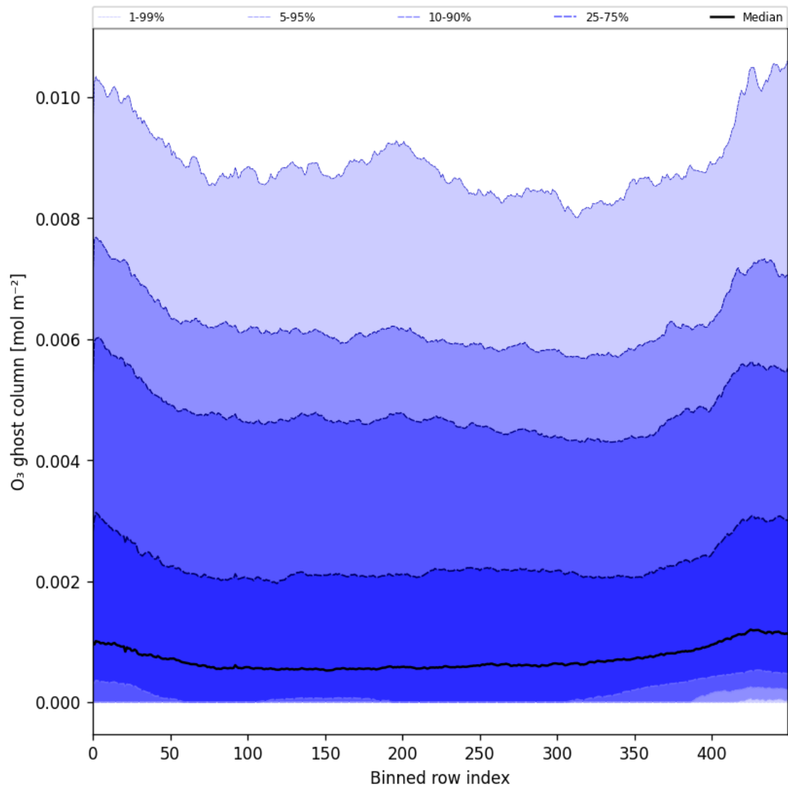
Figure 32: Along track statistics of “O 3 ghost column” for 2025-09-22 to 2025-09-23
