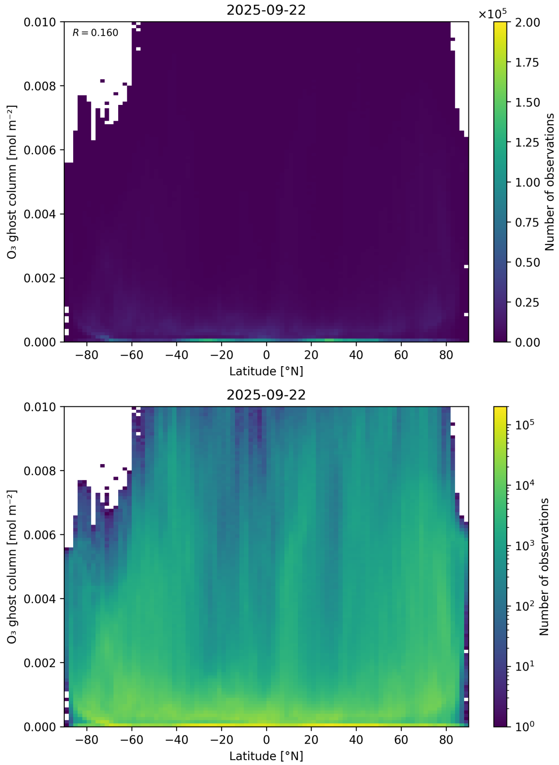
Figure 35: Scatter density plot of “Latitude” against “O 3 ghost column” for 2025-09-22 to 2025-09-23.
