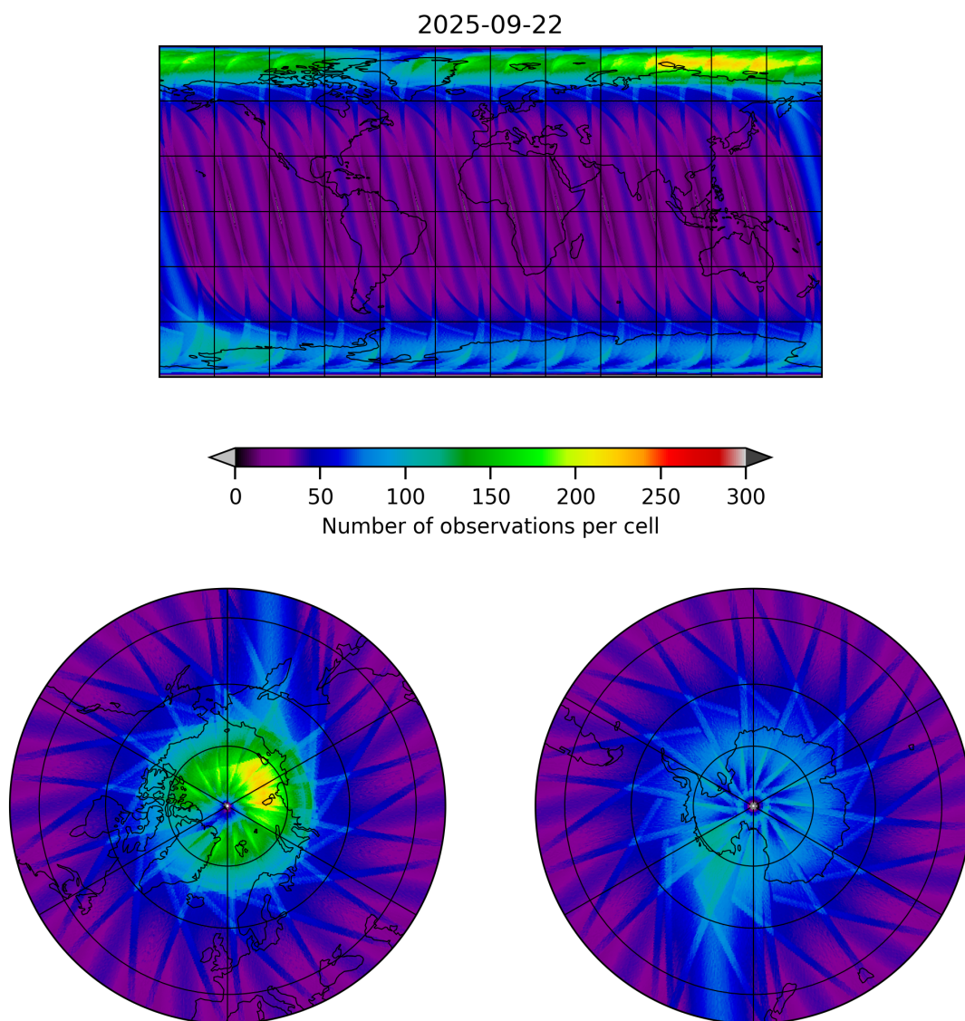
Figure 12: Map of the number of observations for 2025-09-22 to 2025-09-23
