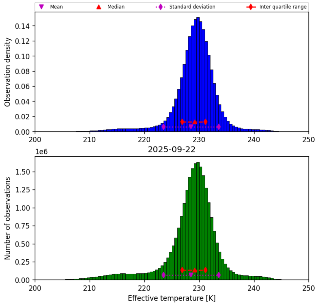
Figure 24: Histogram of “Effective temperature” for 2025-09-22 to 2025-09-23
