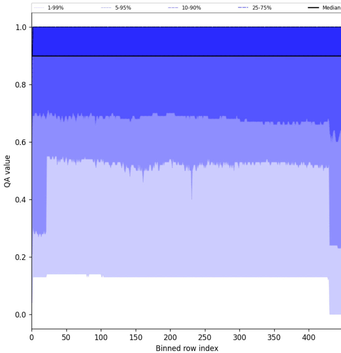
Figure 27: Along track statistics of “QA value” for 2025-09-22 to 2025-09-23
