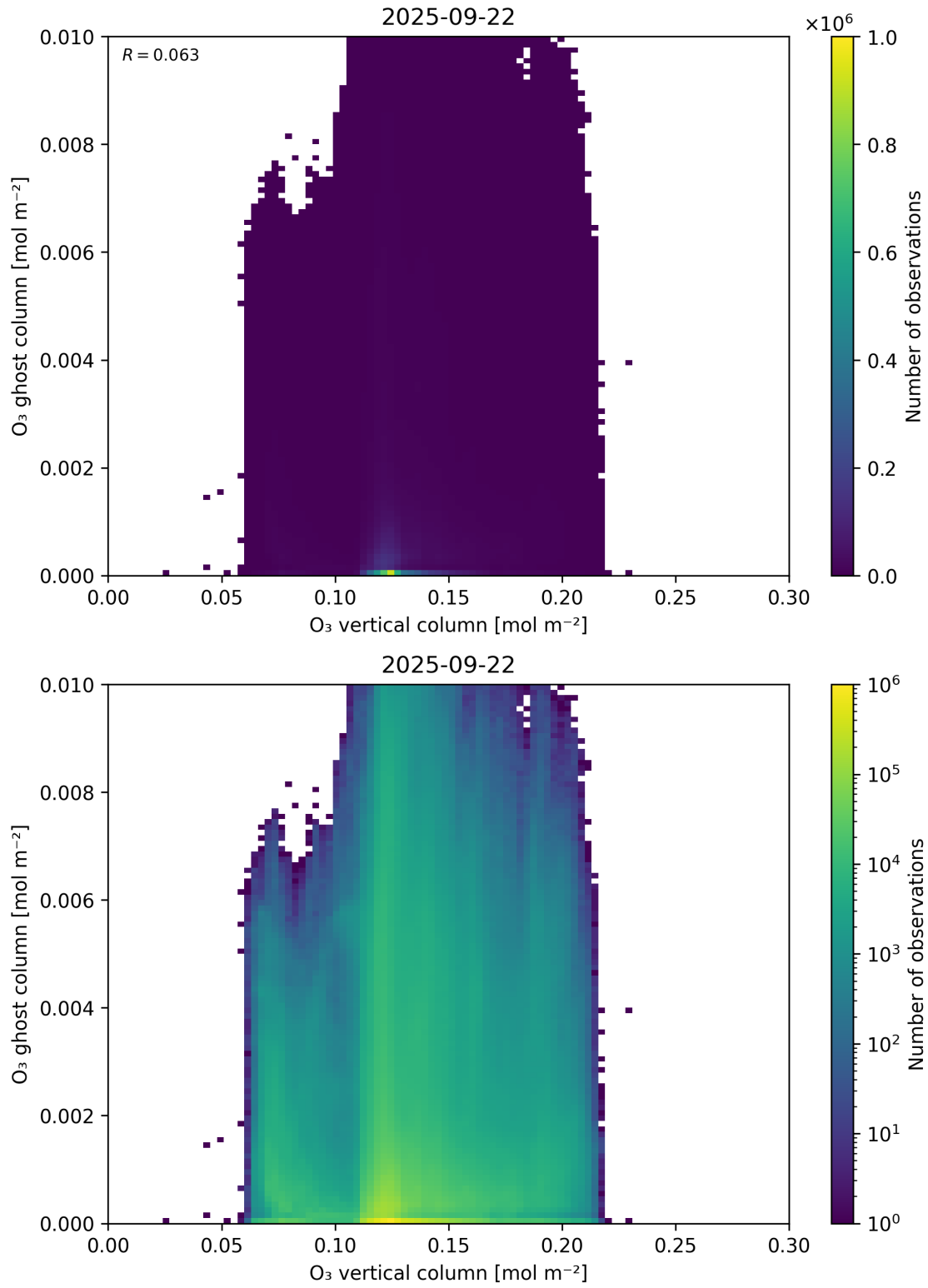
Figure 40: Scatter density plot of “O 3 vertical column” against “O 3 ghost column” for 2025-09-22 to 2025-09-23.
