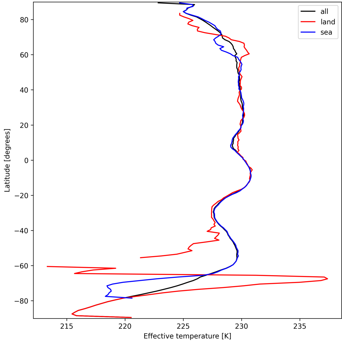
Figure 17: Zonal average of “Effective temperature” for 2025-09-22 to 2025-09-23.
