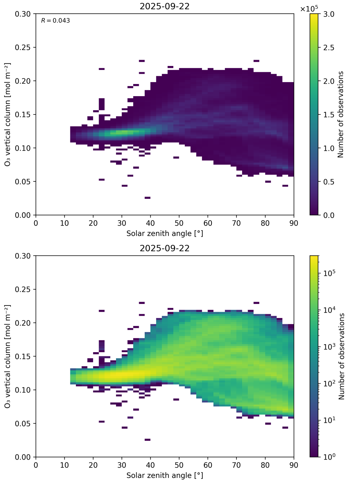
Figure 47: Scatter density plot of “Solar zenith angle” against “O 3 vertical column” for 2025-09-22 to 2025-09-23.
