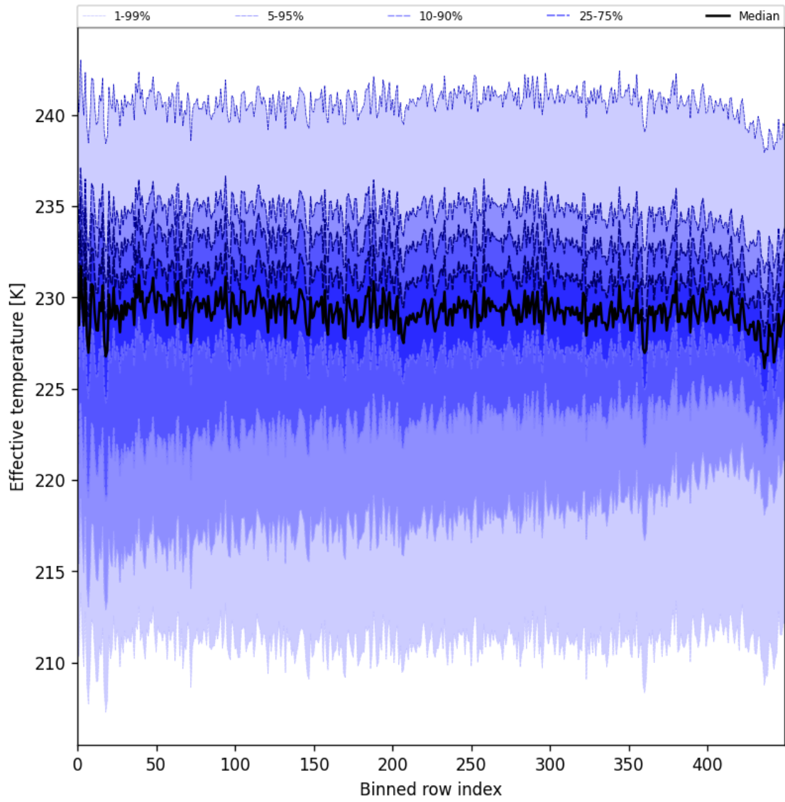
Figure 31: Along track statistics of “Effective temperature” for 2025-09-22 to 2025-09-23
