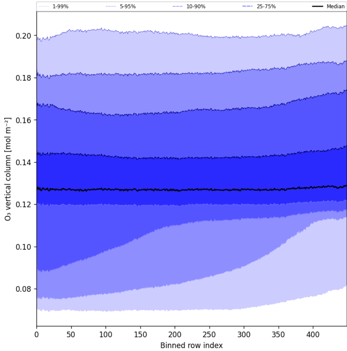
Figure 28: Along track statistics of “O 3 vertical column” for 2025-09-22 to 2025-09-23
