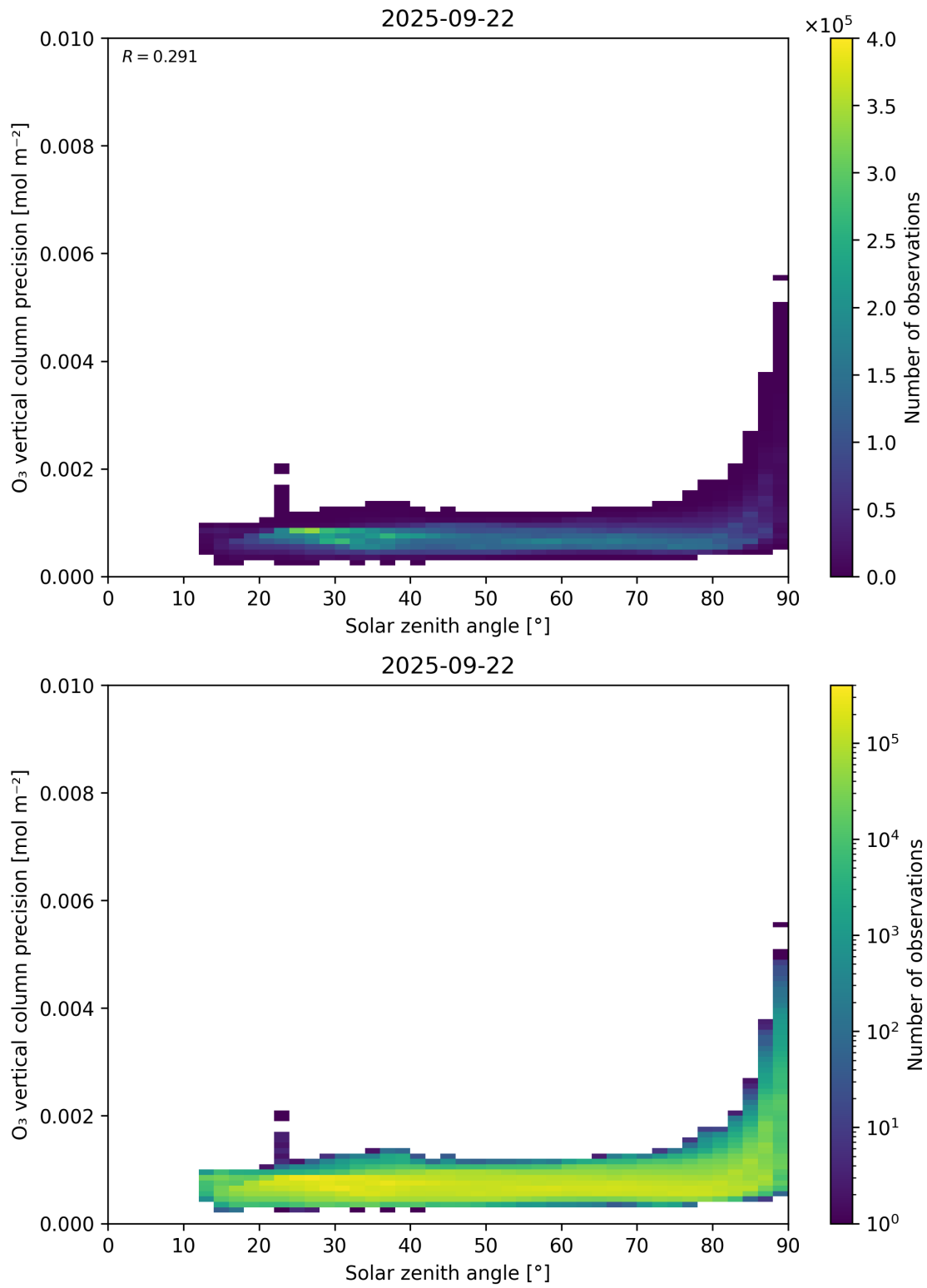
Figure 48: Scatter density plot of “Solar zenith angle” against “O 3 vertical column precision” for 2025-09-22 to 2025-09-23.
