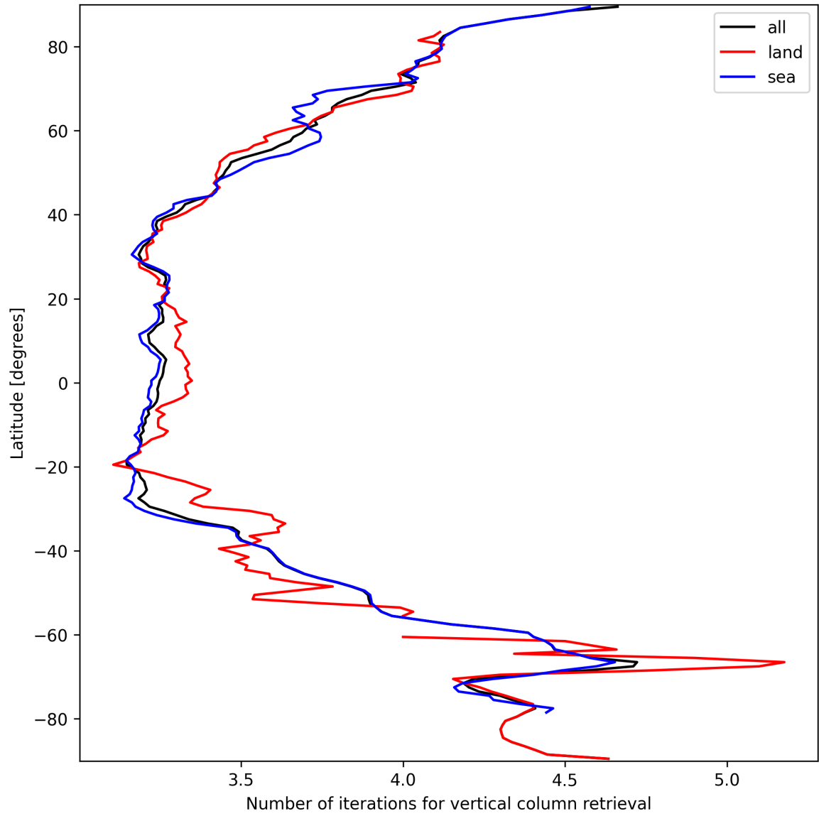
Figure 19: Zonal average of “Number of iterations for vertical column retrieval” for 2025-09-22 to 2025-09-23.
