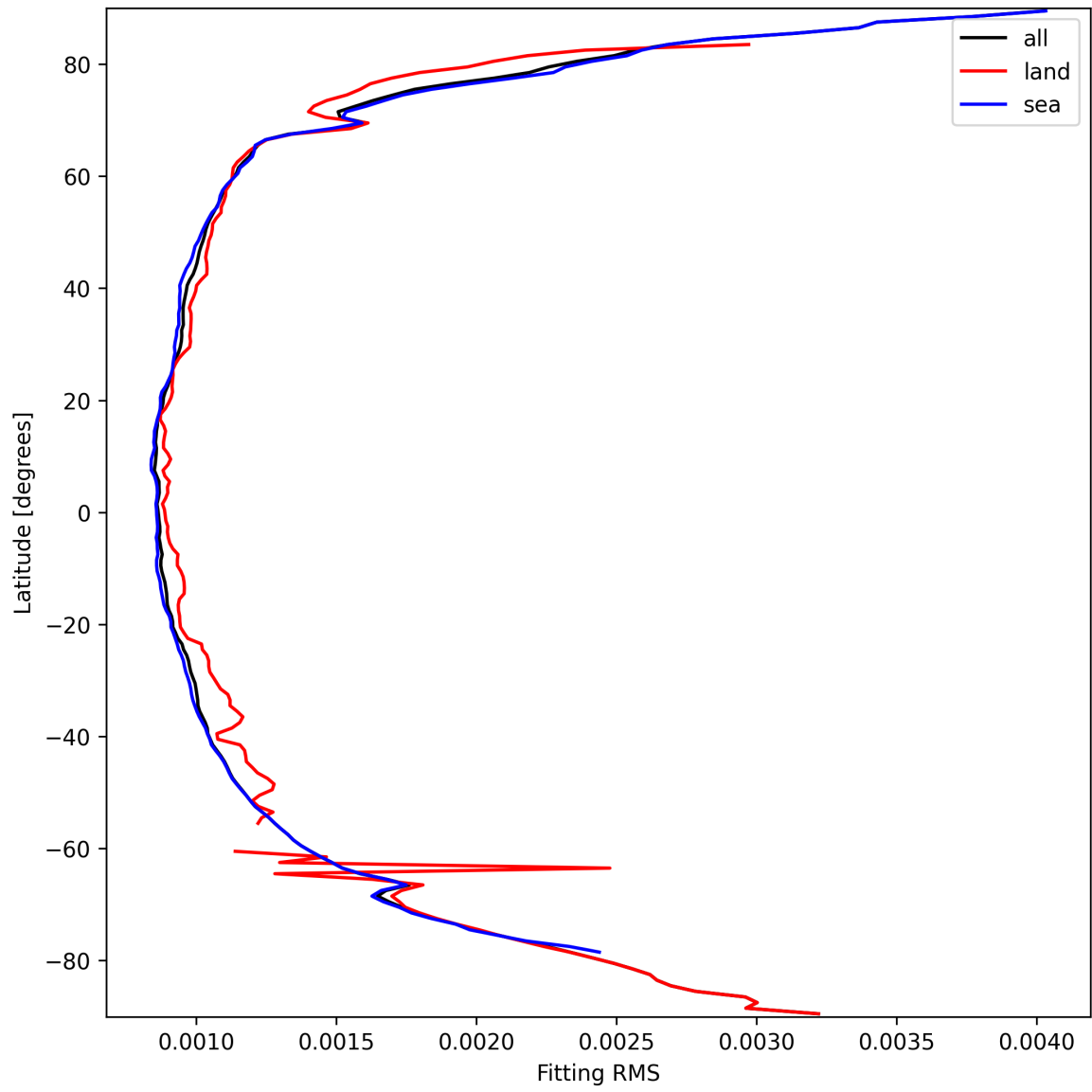
Figure 16: Zonal average of “Fitting RMS” for 2025-09-22 to 2025-09-23.
