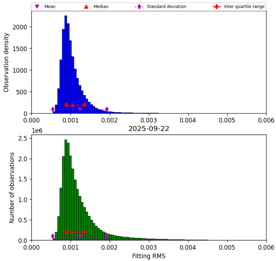
Figure 23: Histogram of “Fitting RMS” for 2025-09-22 to 2025-09-23
