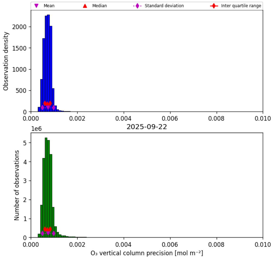
Figure 22: Histogram of “O 3 vertical column precision” for 2025-09-22 to 2025-09-23
