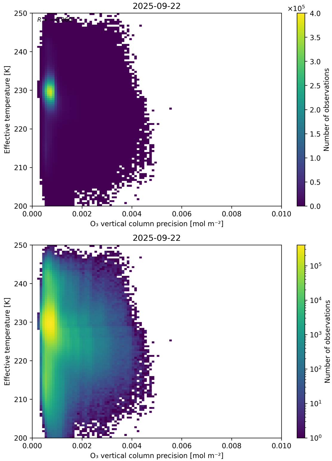
Figure 42: Scatter density plot of “O 3 vertical column precision” against “Effective temperature” for 2025-09-22 to 2025-09-23.
