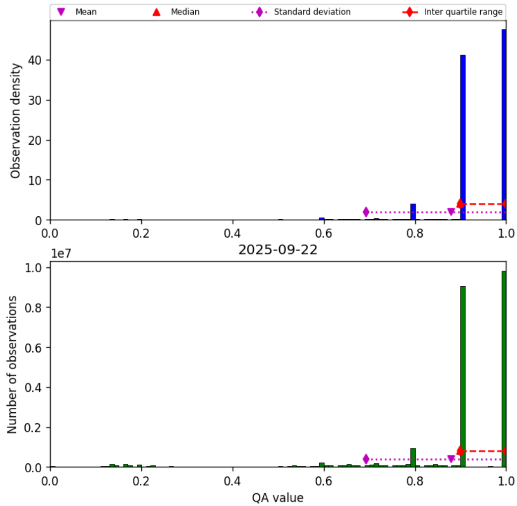
Figure 20: Histogram of “QA value” for 2025-09-22 to 2025-09-23
