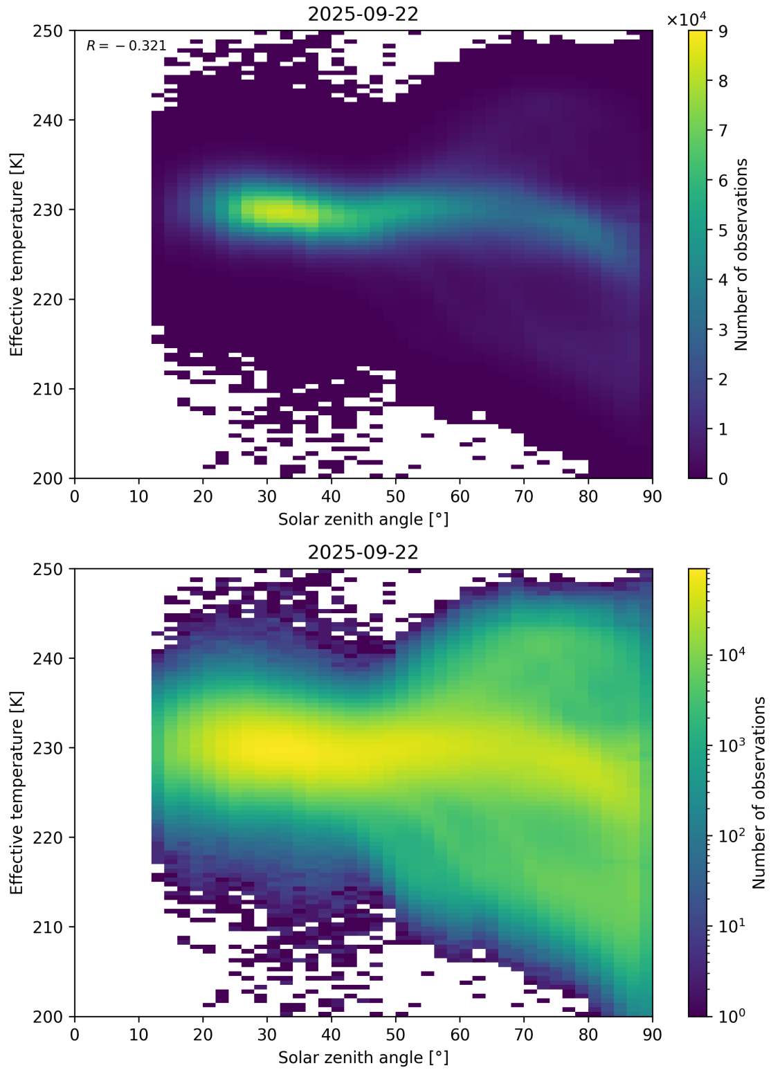
Figure 45: Scatter density plot of “Solar zenith angle” against “Effective temperature” for 2025-09-22 to 2025-09-23.
