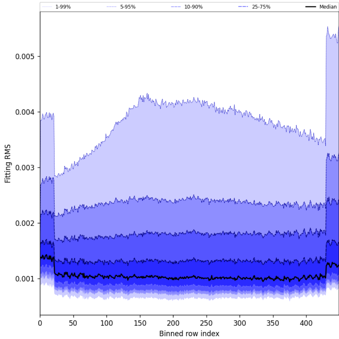
Figure 30: Along track statistics of “Fitting RMS” for 2025-09-22 to 2025-09-23
