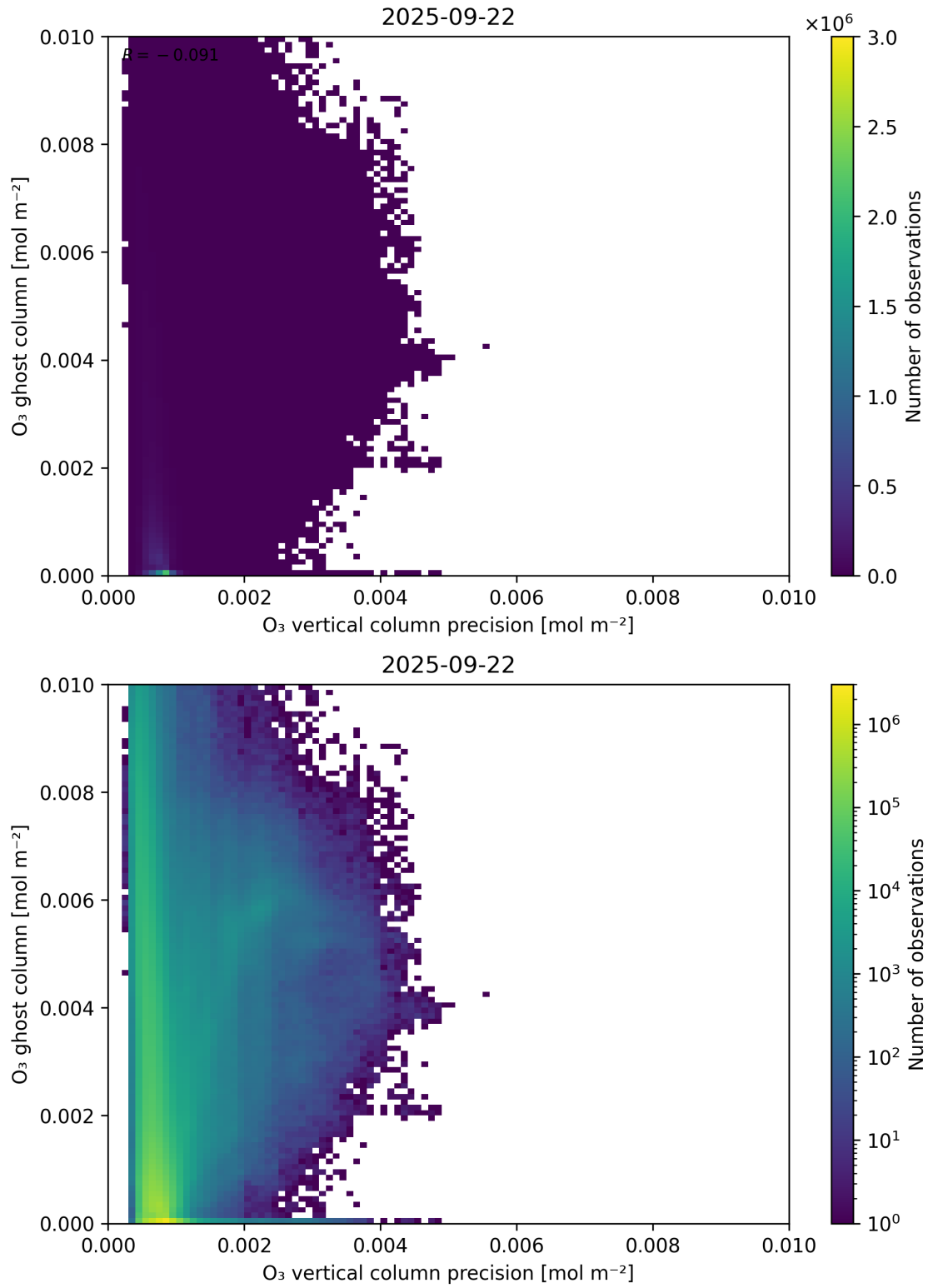
Figure 43: Scatter density plot of “O 3 vertical column precision” against “O 3 ghost column” for 2025-09-22 to 2025-09-23.
