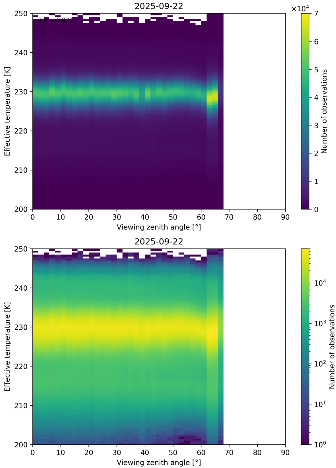
Figure 50: Scatter density plot of “Viewing zenith angle” against “Effective temperature” for 2025-09-22 to 2025-09-23.
