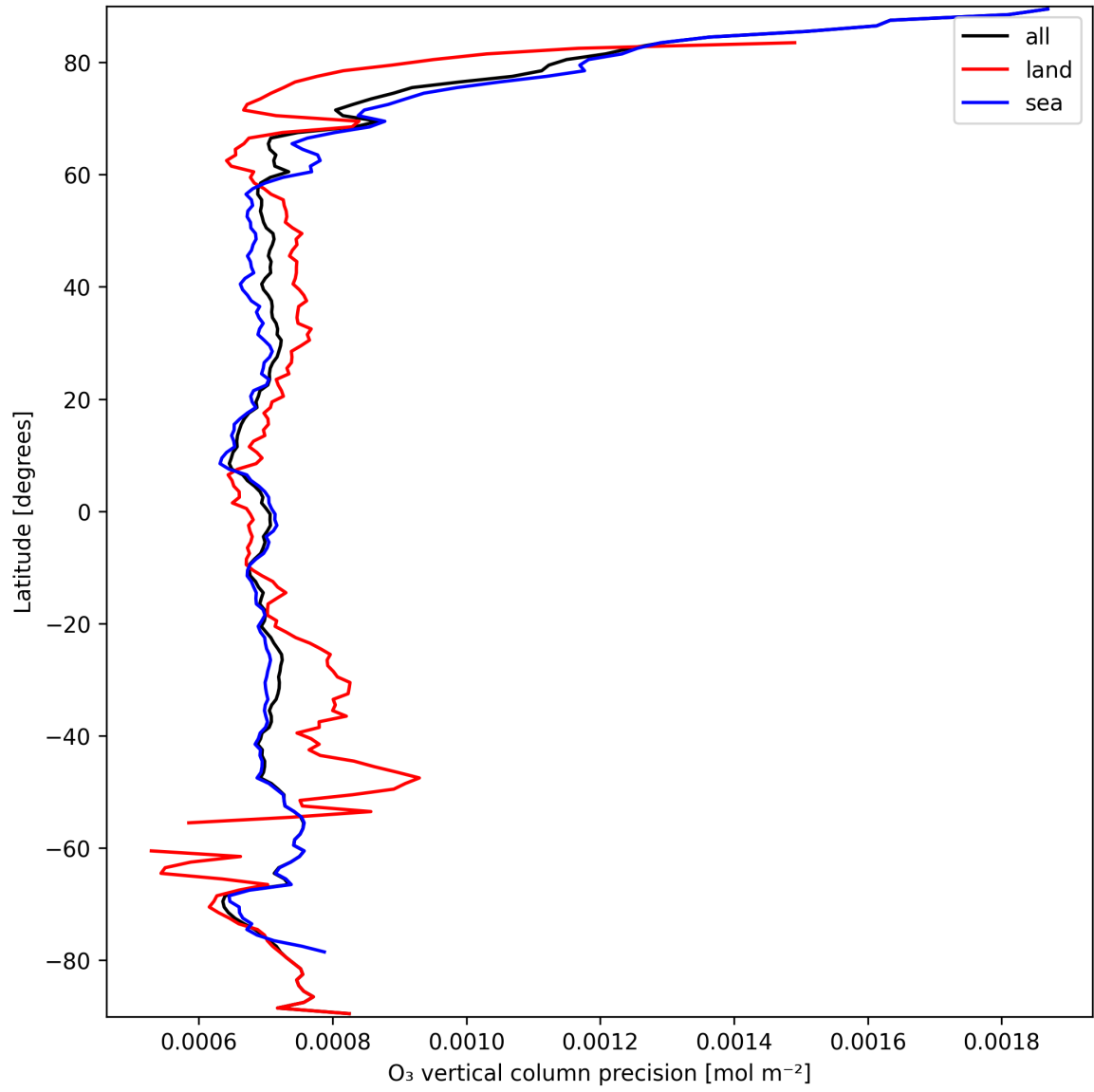
Figure 15: Zonal average of "O 3 vertical column precision" for 2025-09-22 to 2025-09-23.
