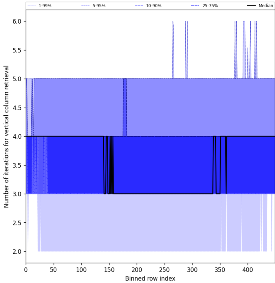
Figure 33: Along track statistics of “Number of iterations for vertical column retrieval” for 2025-09-22 to 2025-09-23
