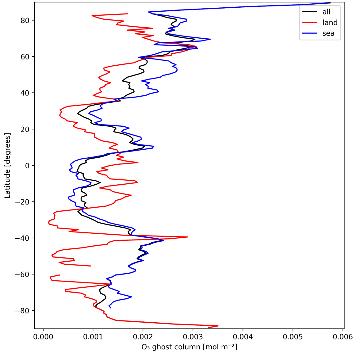
Figure 18: Zonal average of "O 3 ghost column" for 2025-09-22 to 2025-09-23.
