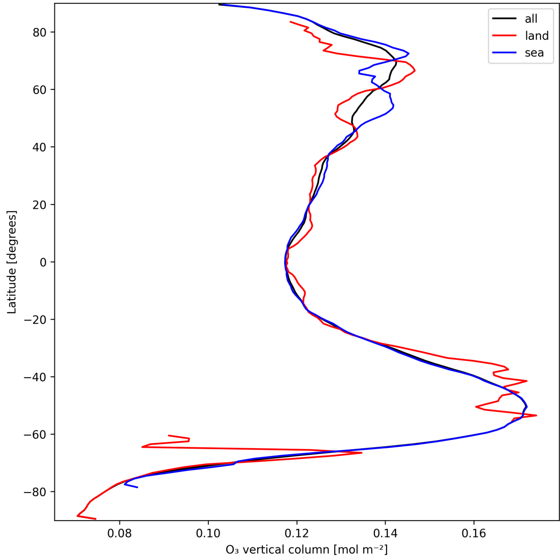
Figure 14: Zonal average of “O 3 vertical column” for 2025-09-22 to 2025-09-23.
