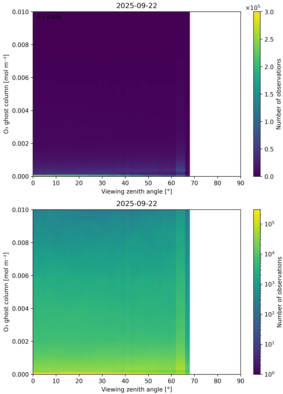
Figure 51: Scatter density plot of “Viewing zenith angle” against “O 3 ghost column” for 2025-09-22 to 2025-09-23.
