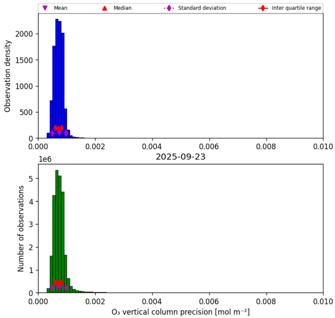
Figure 22: Histogram of “O 3 vertical column precision” for 2025-09-22 to 2025-09-24
