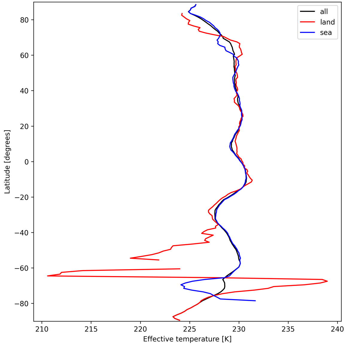
Figure 17: Zonal average of “Effective temperature” for 2025-09-22 to 2025-09-24.
