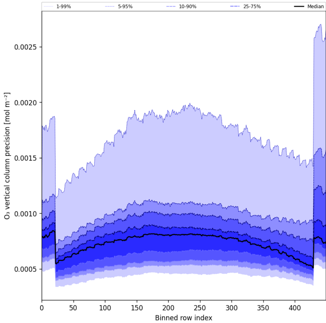
Figure 29: Along track statistics of “O 3 vertical column precision” for 2025-09-22 to 2025-09-24
