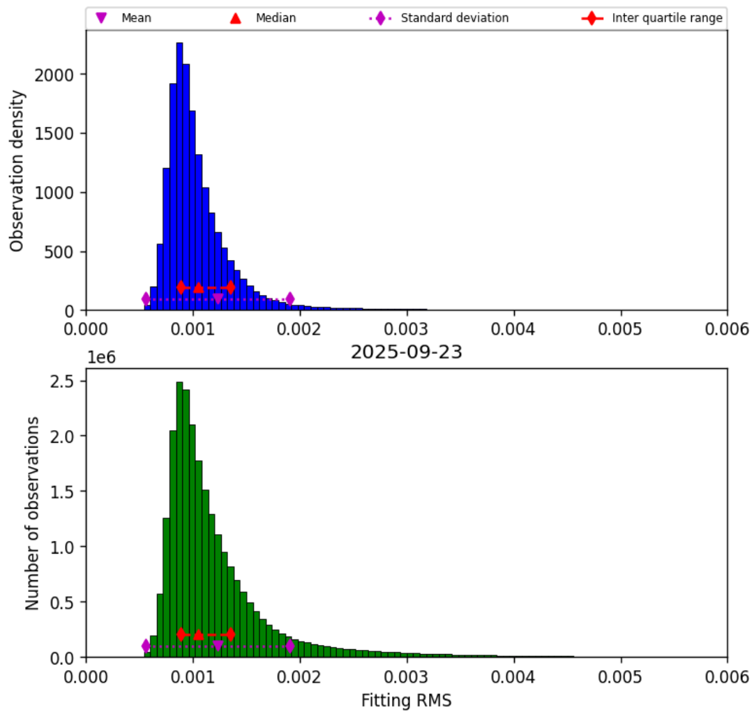
Figure 23: Histogram of "Fitting RMS" for 2025-09-22 to 2025-09-24
