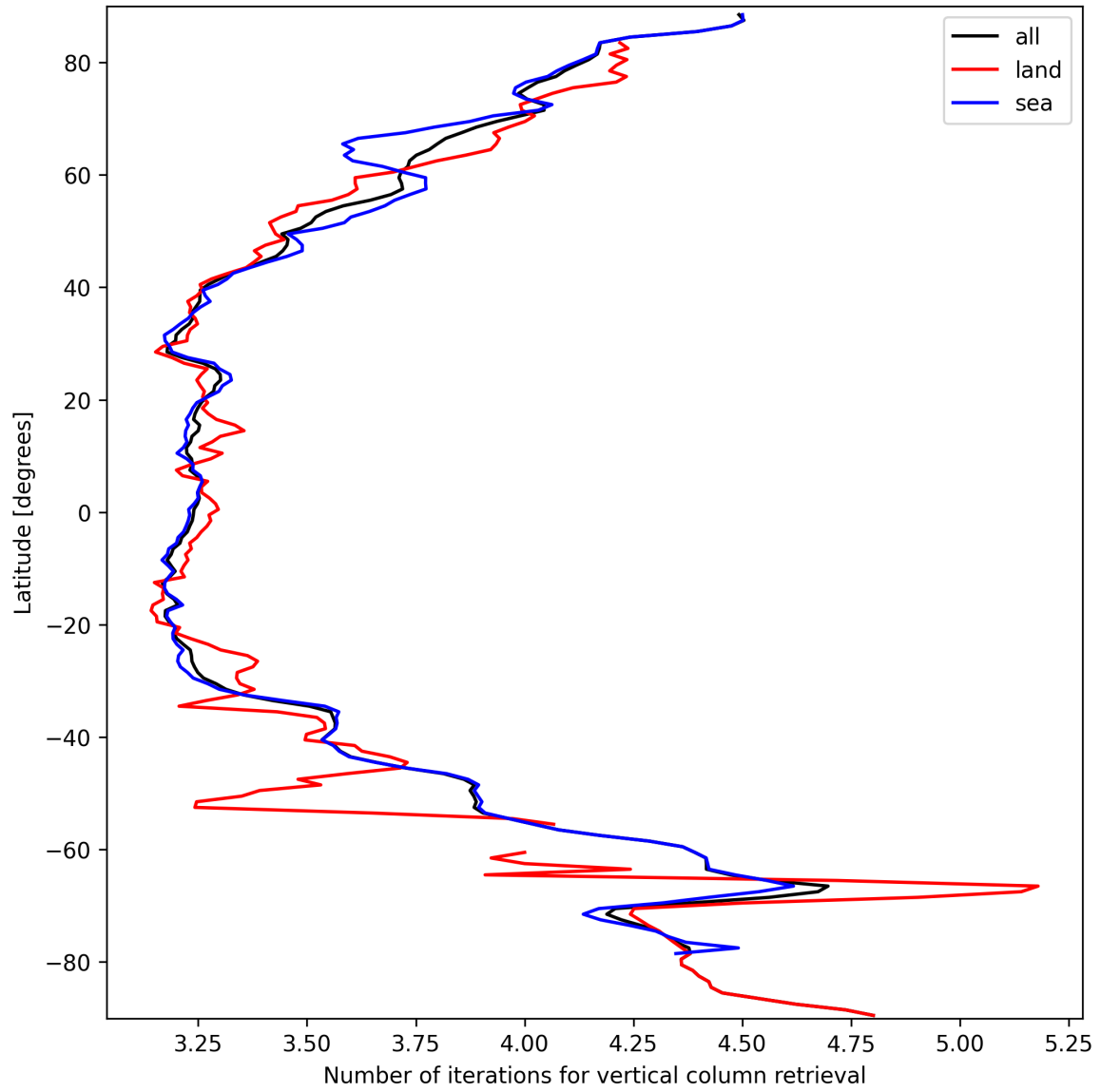
Figure 19: Zonal average of “Number of iterations for vertical column retrieval” for 2025-09-22 to 2025-09-24.
