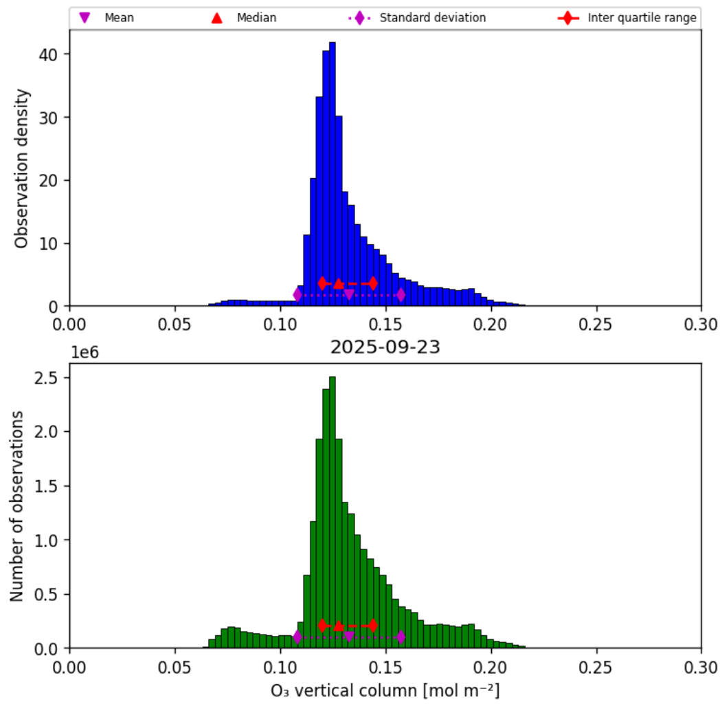
Figure 21: Histogram of “O 3 vertical column” for 2025-09-22 to 2025-09-24
