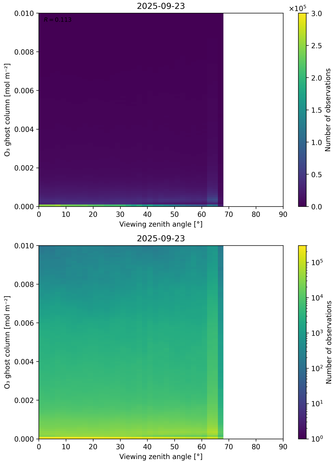
Figure 51: Scatter density plot of “Viewing zenith angle” against “O 3 ghost column” for 2025-09-22 to 2025-09-24.
