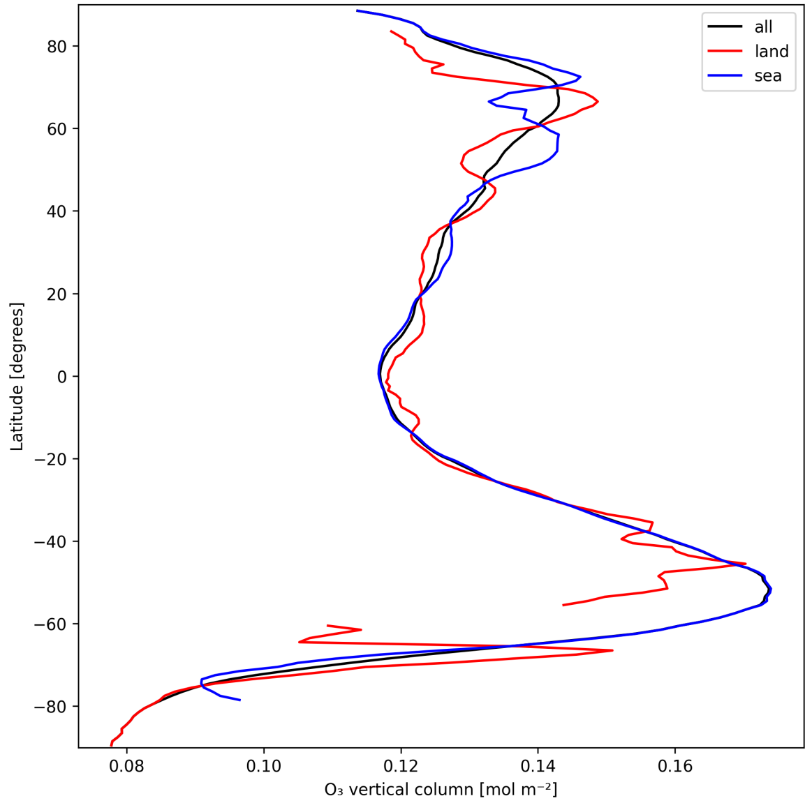
Figure 14: Zonal average of “O 3 vertical column” for 2025-09-22 to 2025-09-24.
