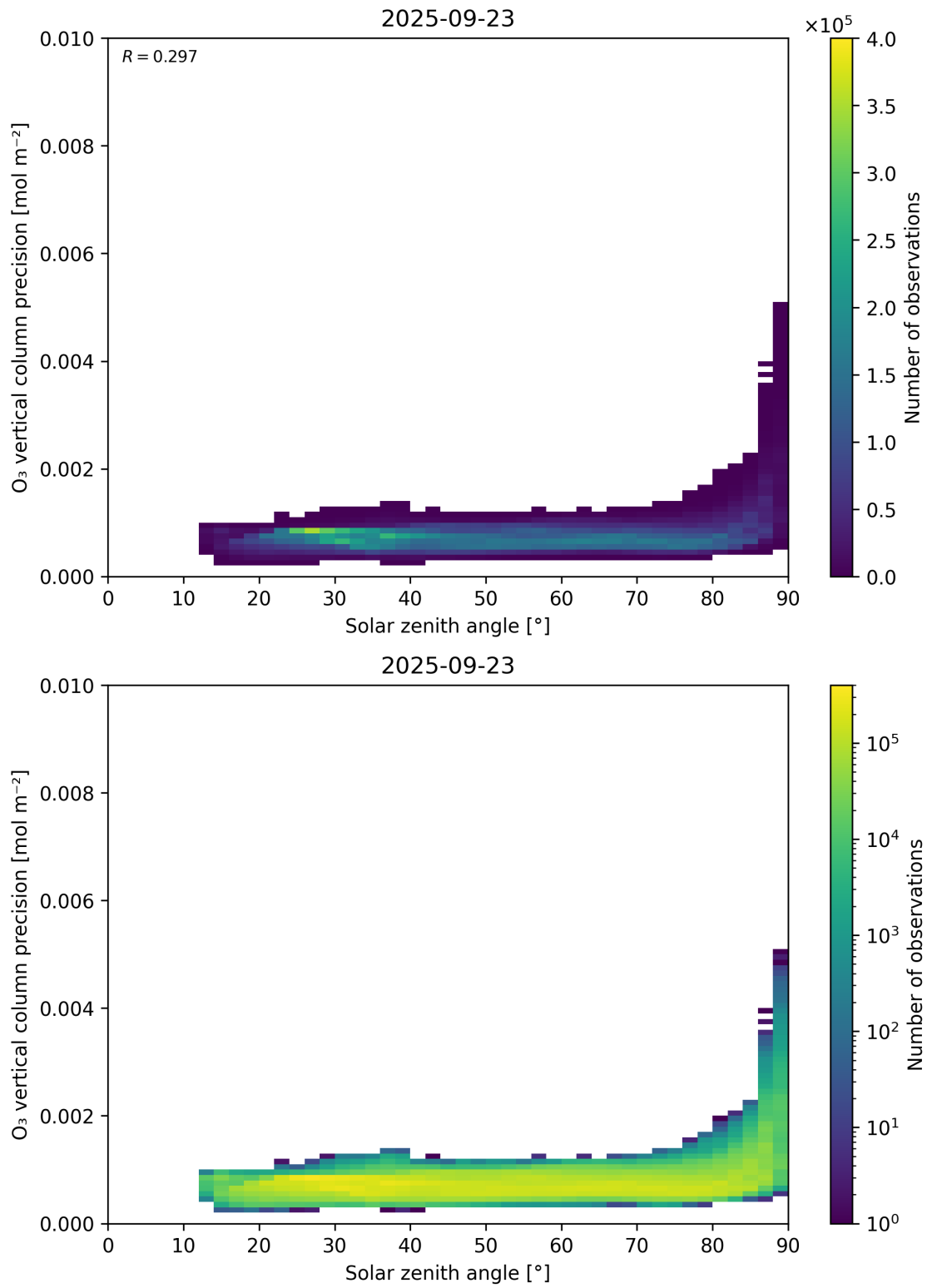
Figure 48: Scatter density plot of “Solar zenith angle” against “O 3 vertical column precision” for 2025-09-22 to 2025-09-24.
