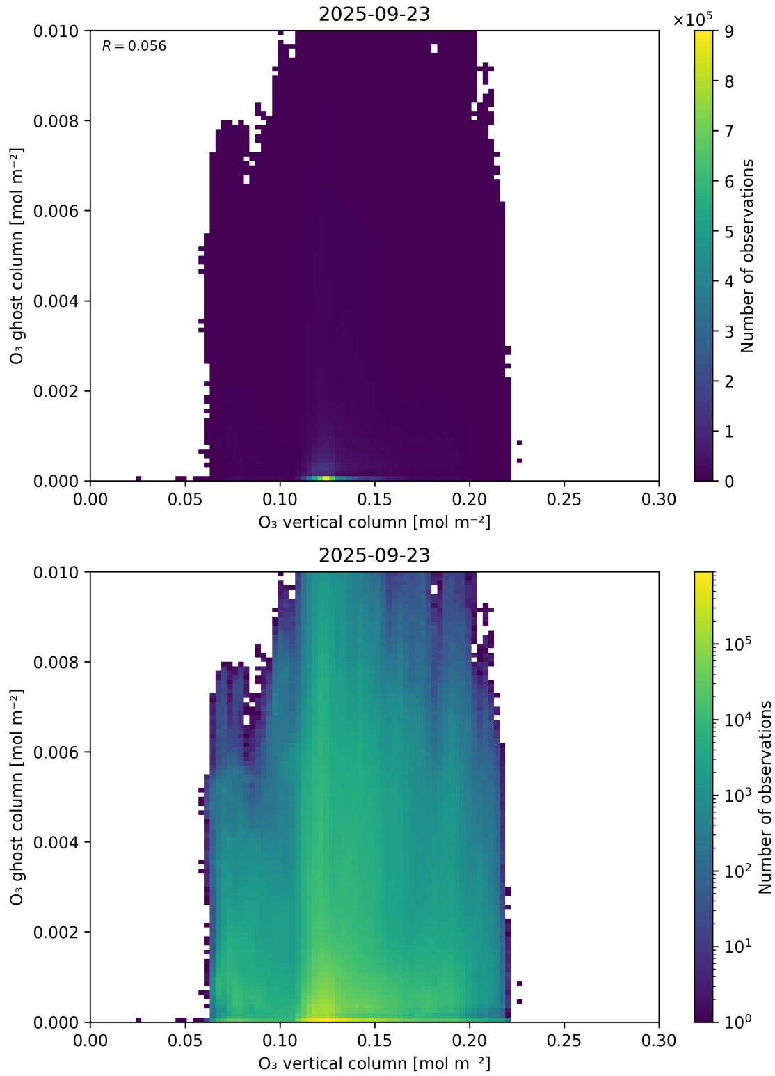
Figure 40: Scatter density plot of “O 3 vertical column” against “O 3 ghost column” for 2025-09-22 to 2025-09-24.
