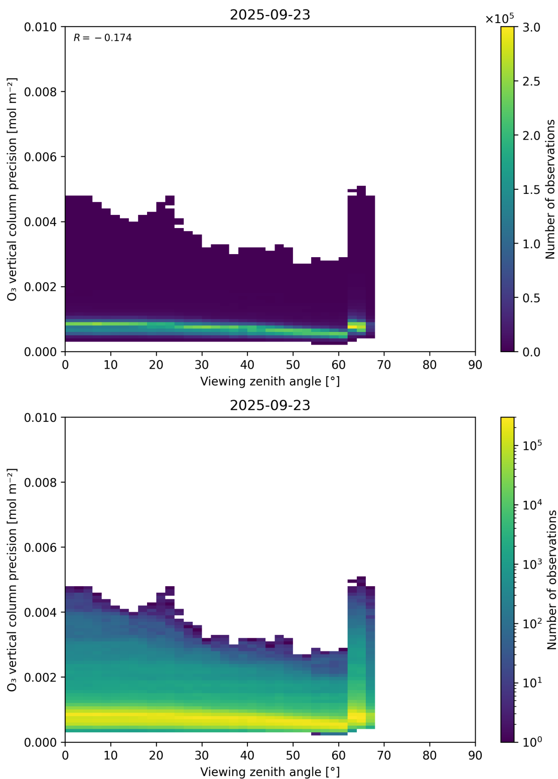
Figure 53: Scatter density plot of “Viewing zenith angle” against “O 3 vertical column precision” for 2025-09-22 to 2025-09-24.
