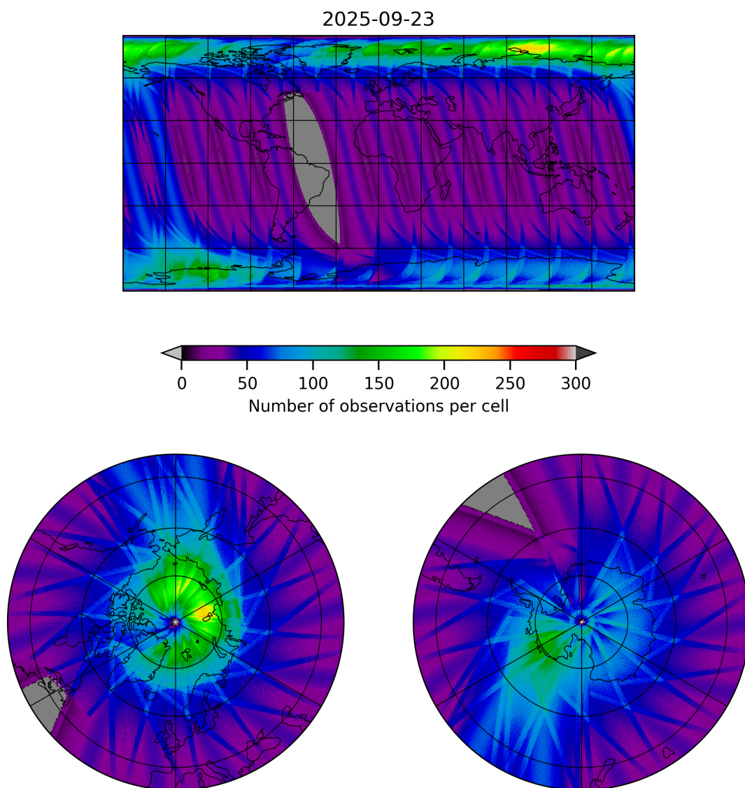
Figure 12: Map of the number of observations for 2025-09-22 to 2025-09-24
