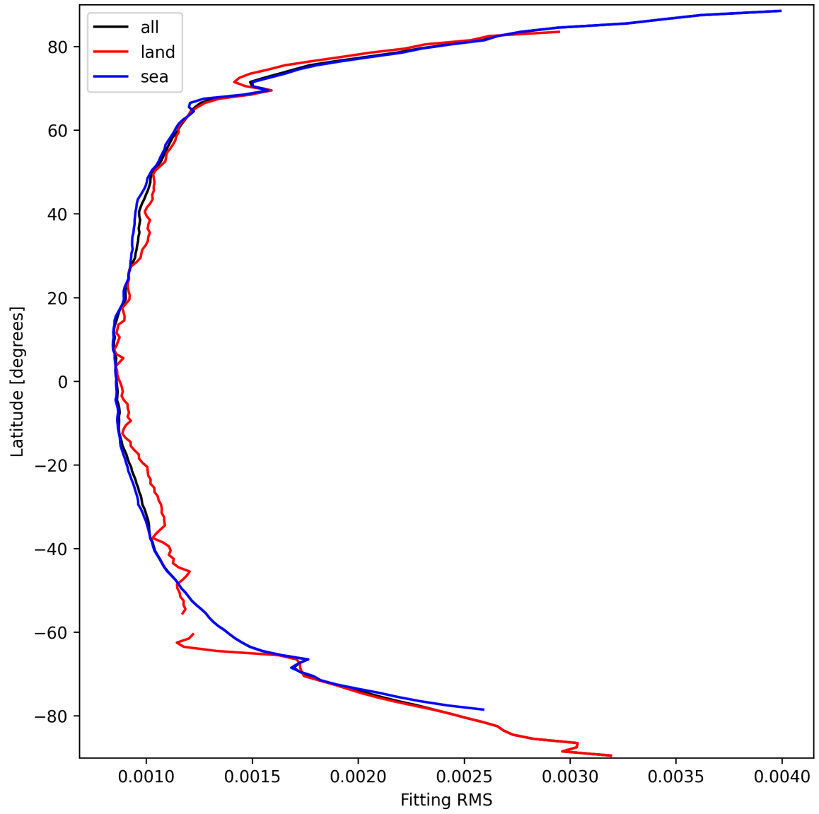
Figure 16: Zonal average of “Fitting RMS” for 2025-09-22 to 2025-09-24.
