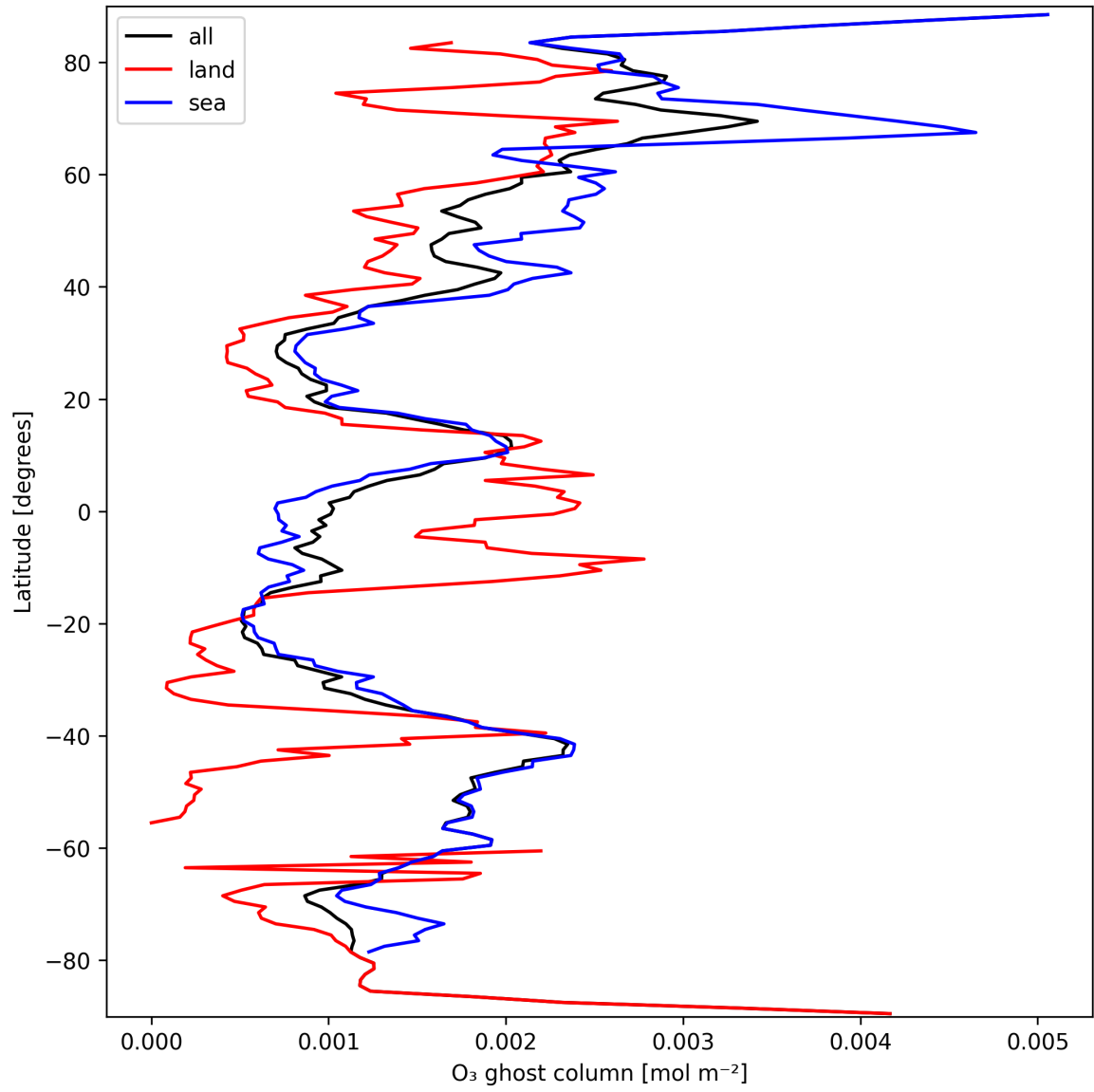
Figure 18: Zonal average of “O 3 ghost column” for 2025-09-22 to 2025-09-24.
