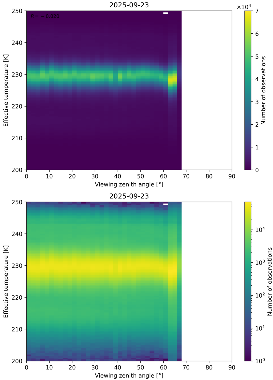
Figure 50: Scatter density plot of “Viewing zenith angle” against “Effective temperature” for 2025-09-22 to 2025-09-24.
