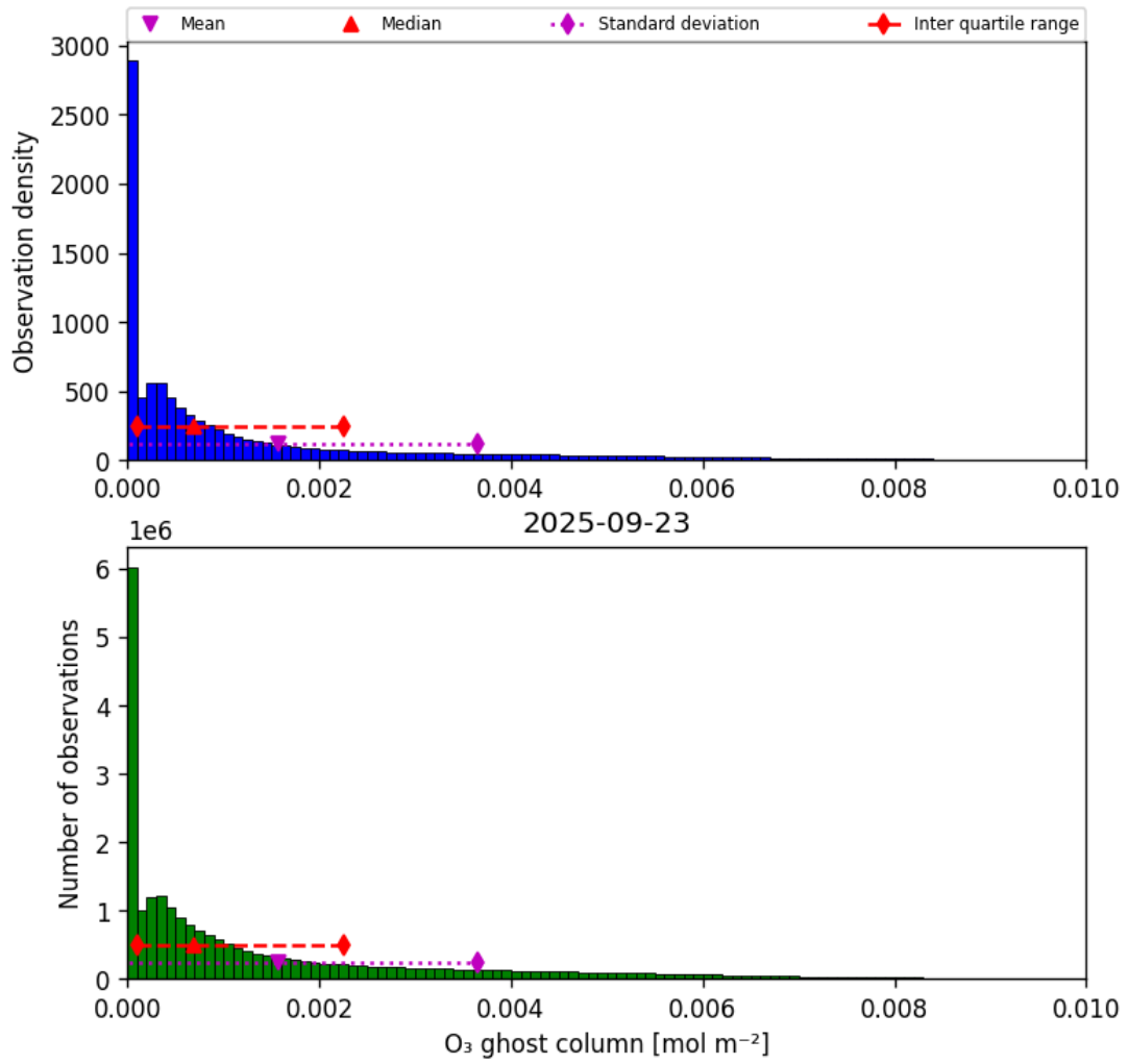
Figure 25: Histogram of “O 3 ghost column” for 2025-09-22 to 2025-09-24
