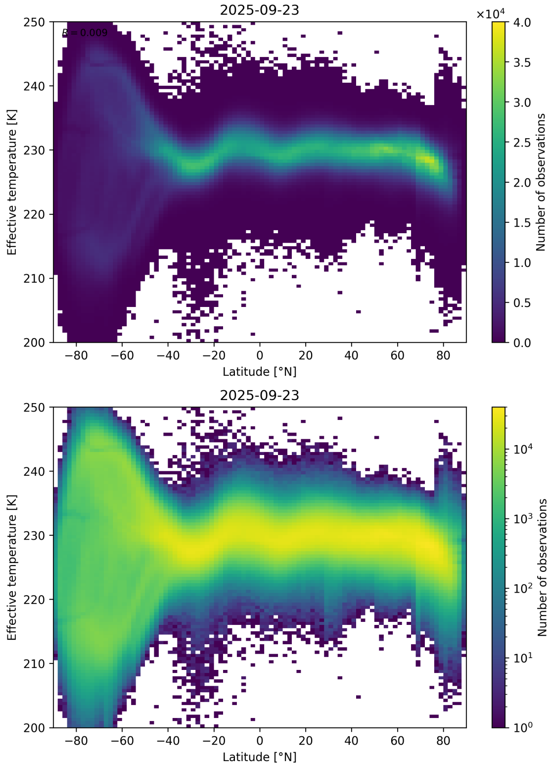
Figure 34: Scatter density plot of “Latitude” against “Effective temperature” for 2025-09-22 to 2025-09-24.
