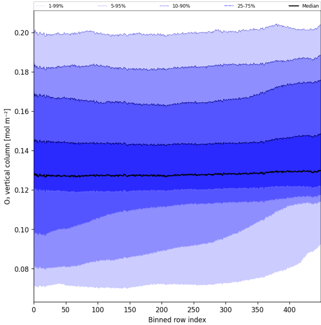
Figure 28: Along track statistics of “ \text{O}_3 vertical column” for 2025-09-22 to 2025-09-24
