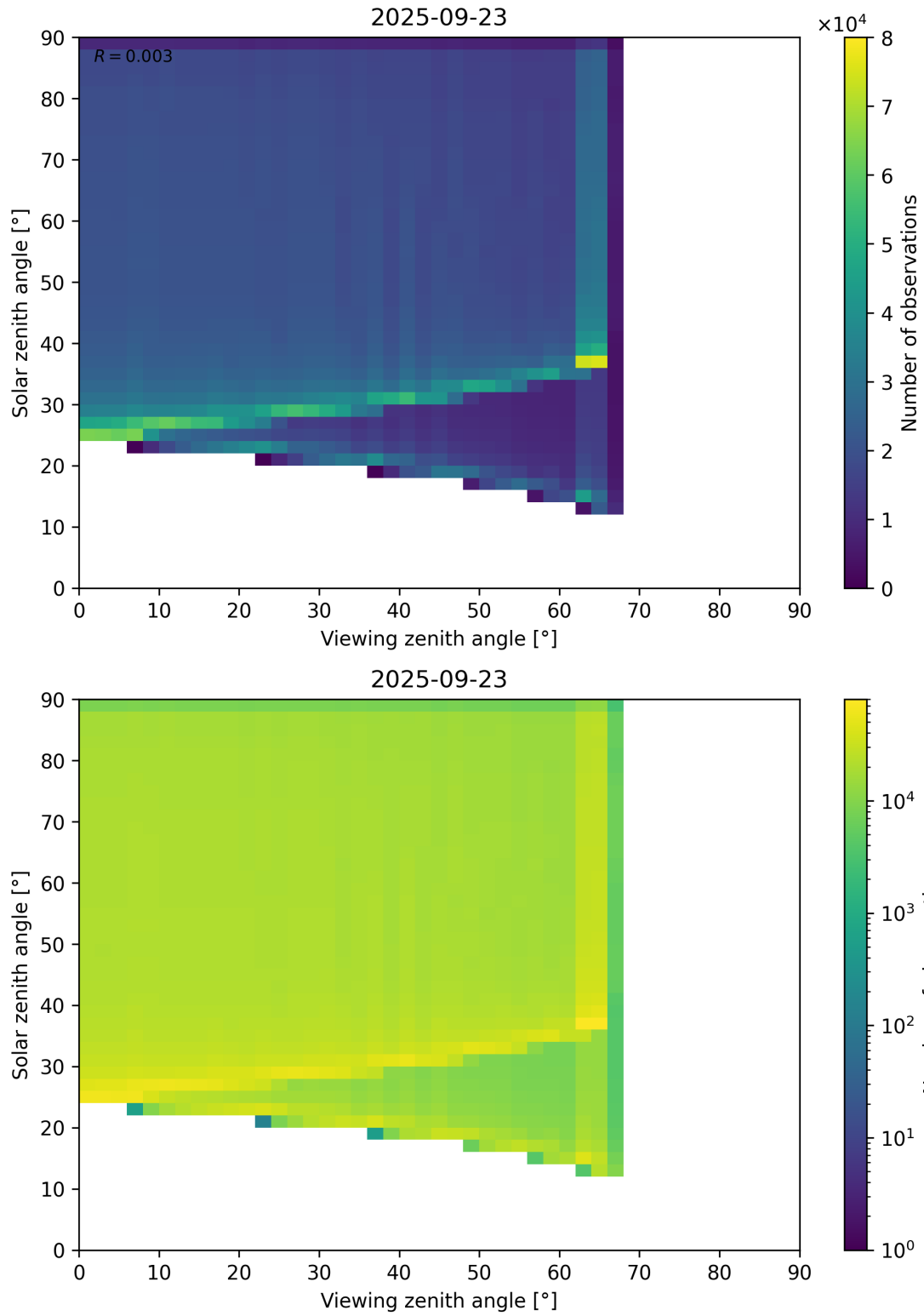
Figure 54: Scatter density plot of “Viewing zenith angle” against “Solar zenith angle” for 2025-09-22 to 2025-09-24.
