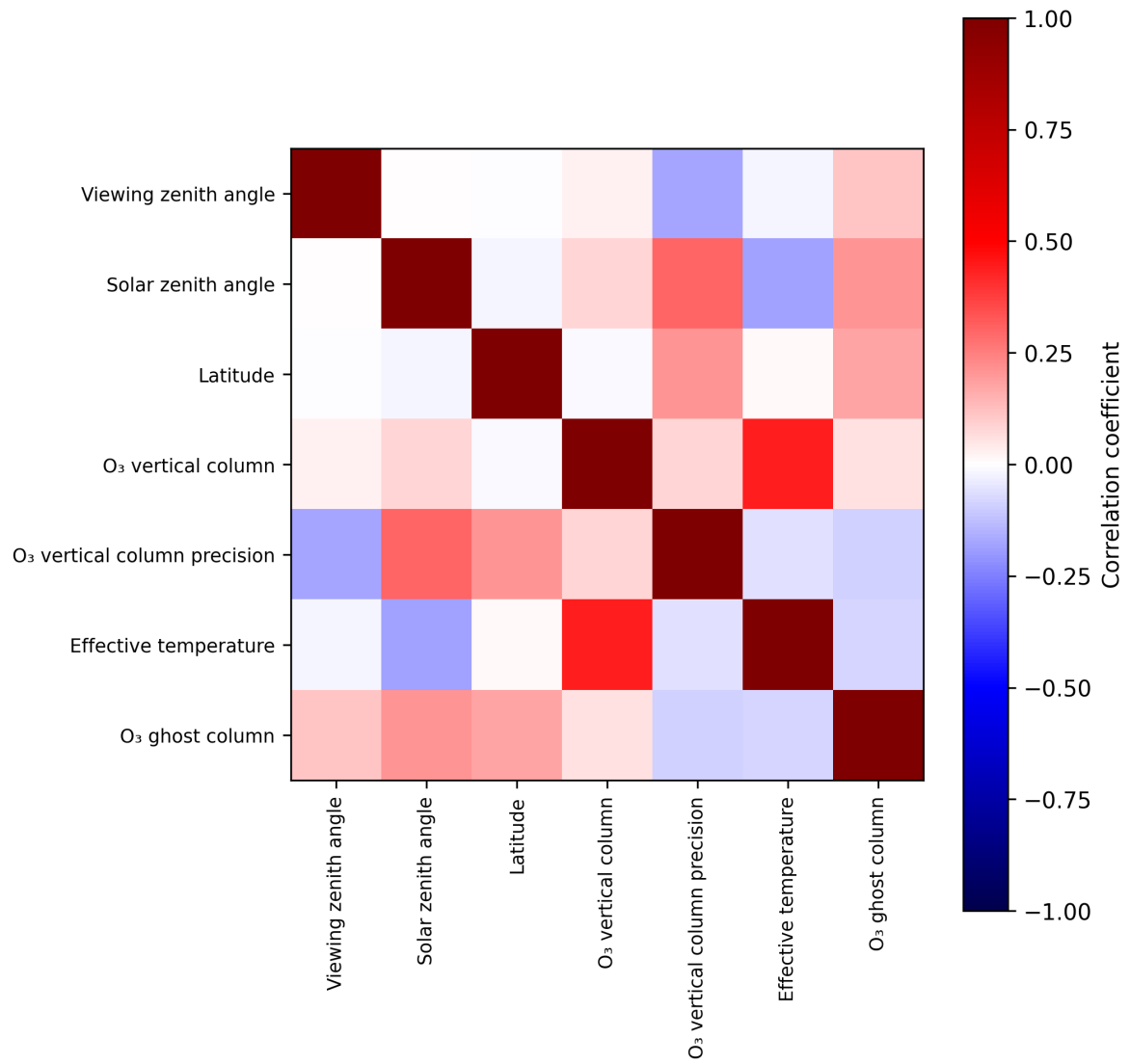
Figure 2: Map of correlation matrix for 2025-09-22 to 2025-09-24.
