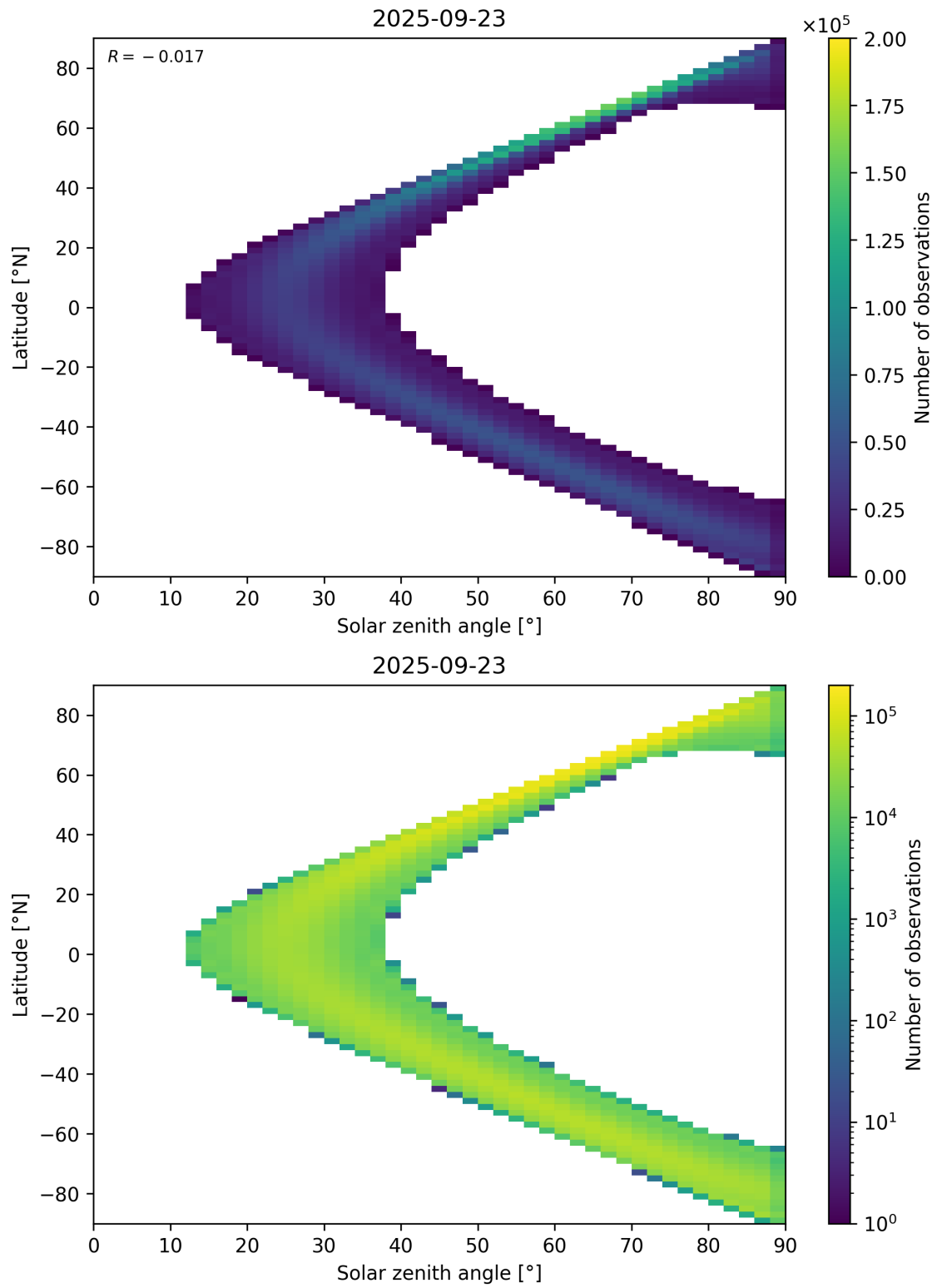
Figure 44: Scatter density plot of “Solar zenith angle” against “Latitude” for 2025-09-22 to 2025-09-24.
