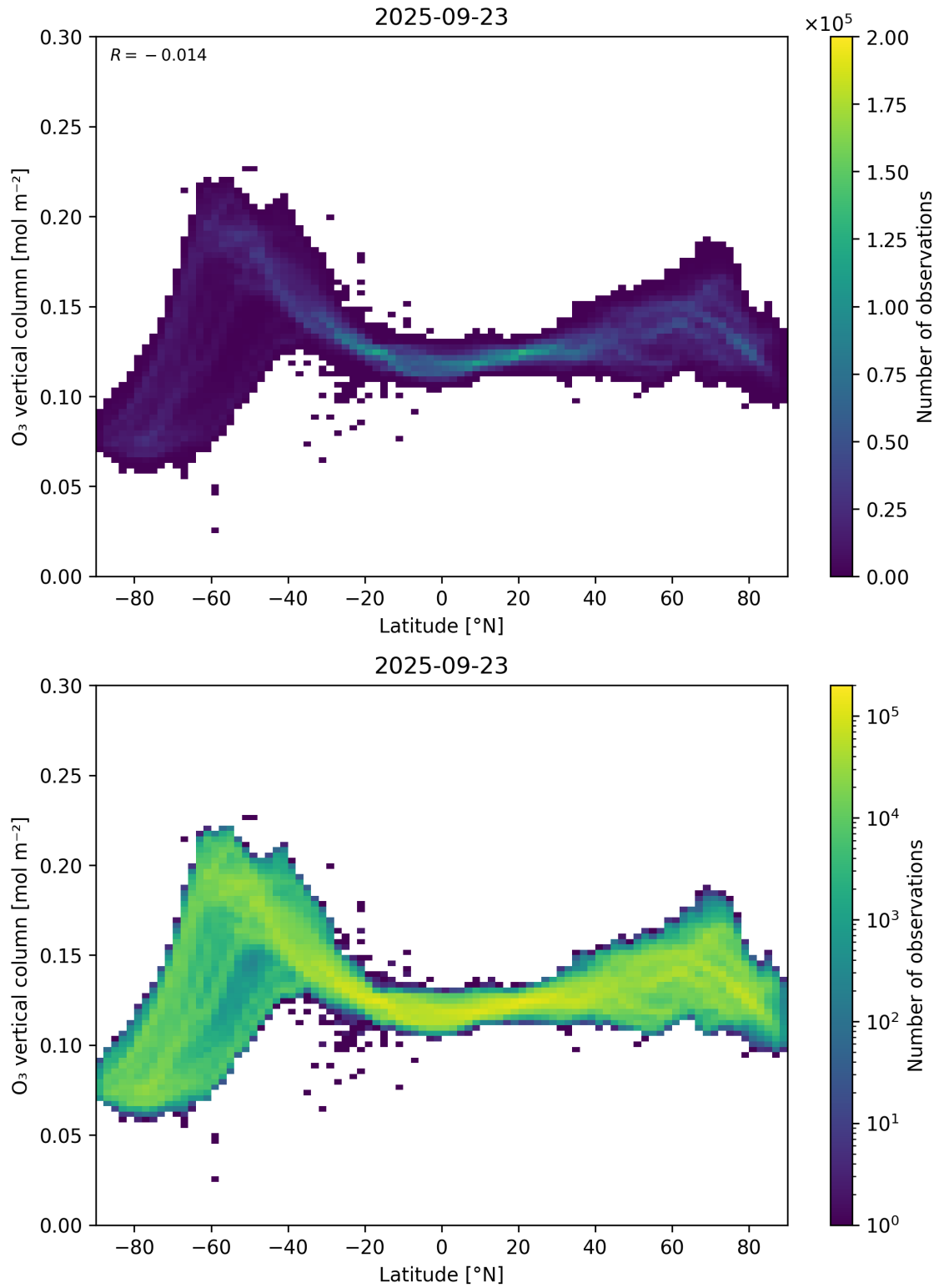
Figure 36: Scatter density plot of “Latitude” against “O 3 vertical column” for 2025-09-22 to 2025-09-24.
