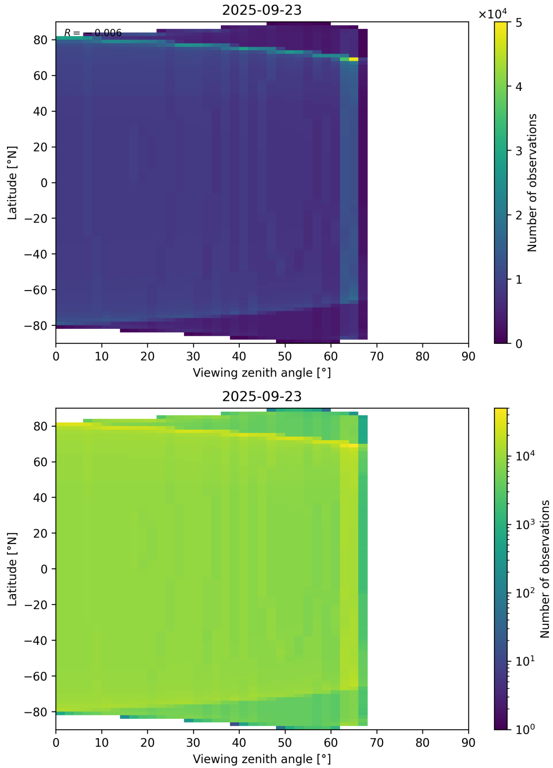
Figure 49: Scatter density plot of “Viewing zenith angle” against “Latitude” for 2025-09-22 to 2025-09-24.
