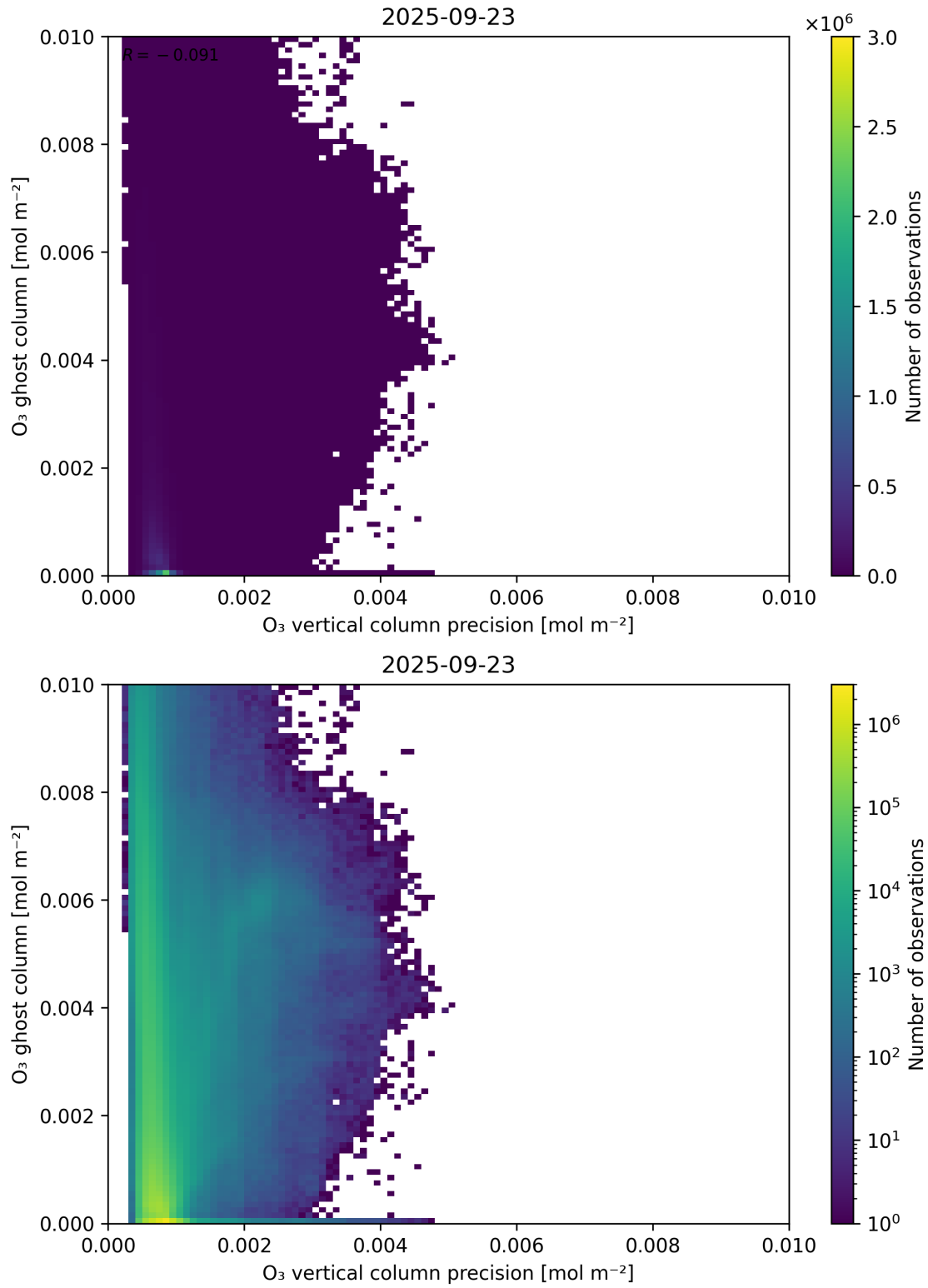
Figure 43: Scatter density plot of “O 3 vertical column precision” against “O 3 ghost column” for 2025-09-22 to 2025-09-24.
