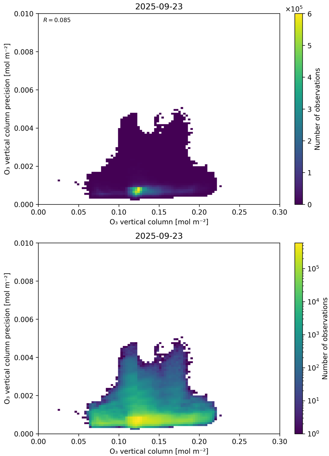
Figure 41: Scatter density plot of “O 3 vertical column” against “O 3 vertical column precision” for 2025-09-22 to 2025-09-24.
