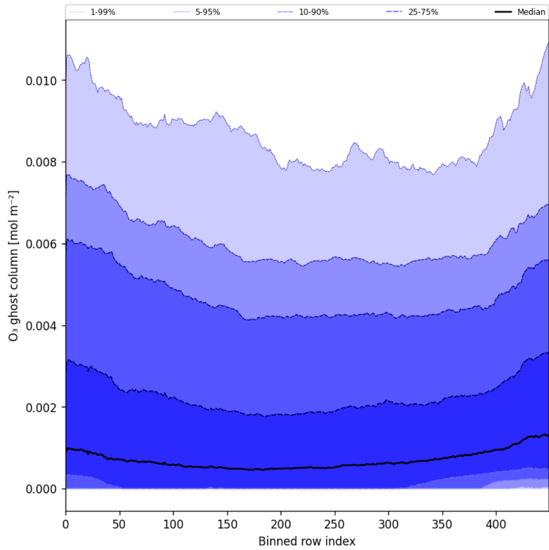
Figure 32: Along track statistics of “O 3 ghost column” for 2025-09-22 to 2025-09-24
