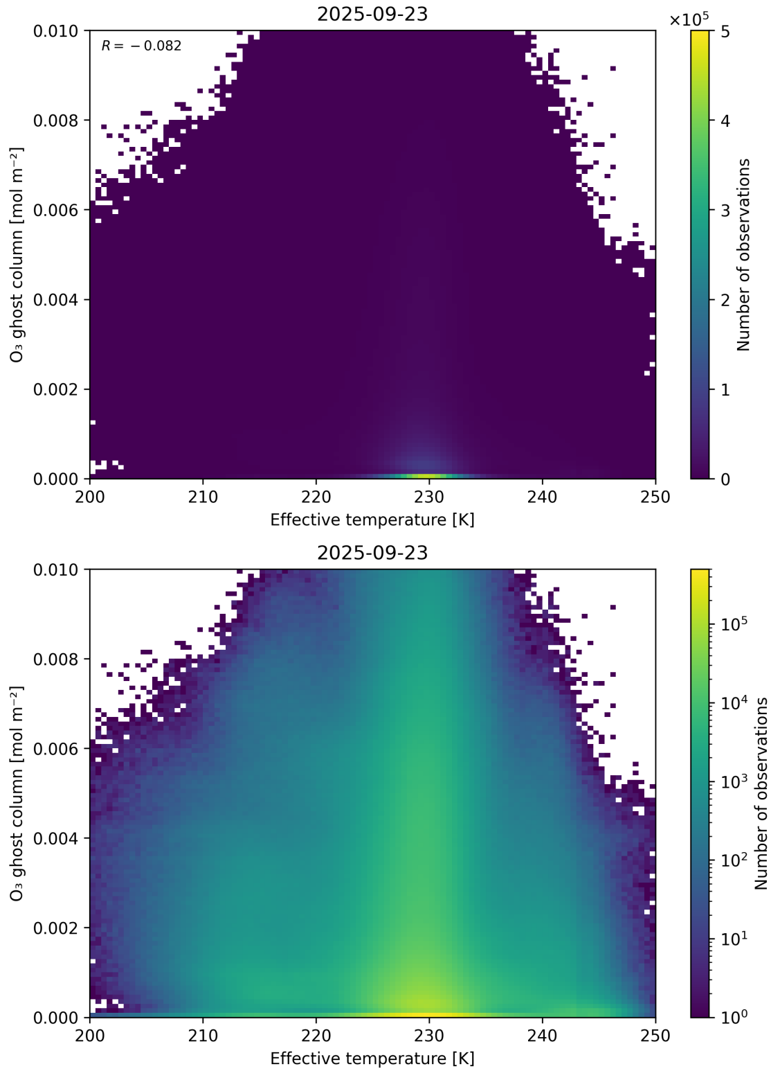
Figure 38: Scatter density plot of “Effective temperature” against “O 3 ghost column” for 2025-09-22 to 2025-09-24.
