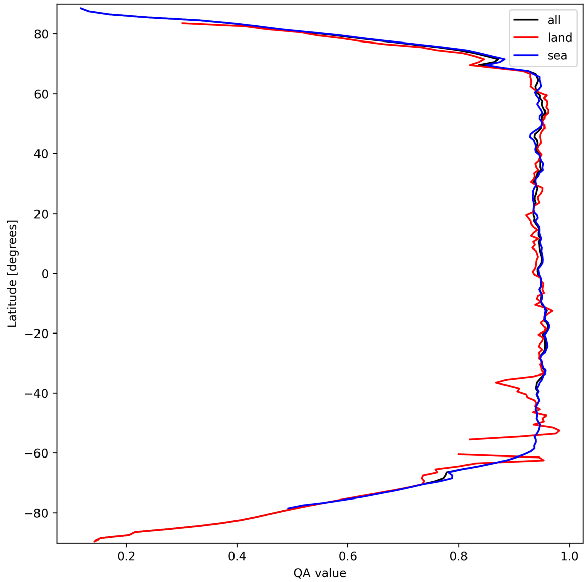
Figure 13: Zonal average of “QA value” for 2025-09-22 to 2025-09-24.
