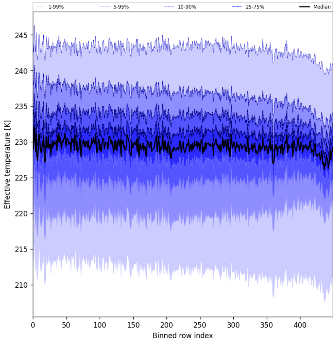
Figure 31: Along track statistics of “Effective temperature” for 2025-09-22 to 2025-09-24
