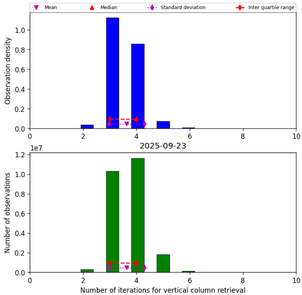
Figure 26: Histogram of “Number of iterations for vertical column retrieval” for 2025-09-22 to 2025-09-24
