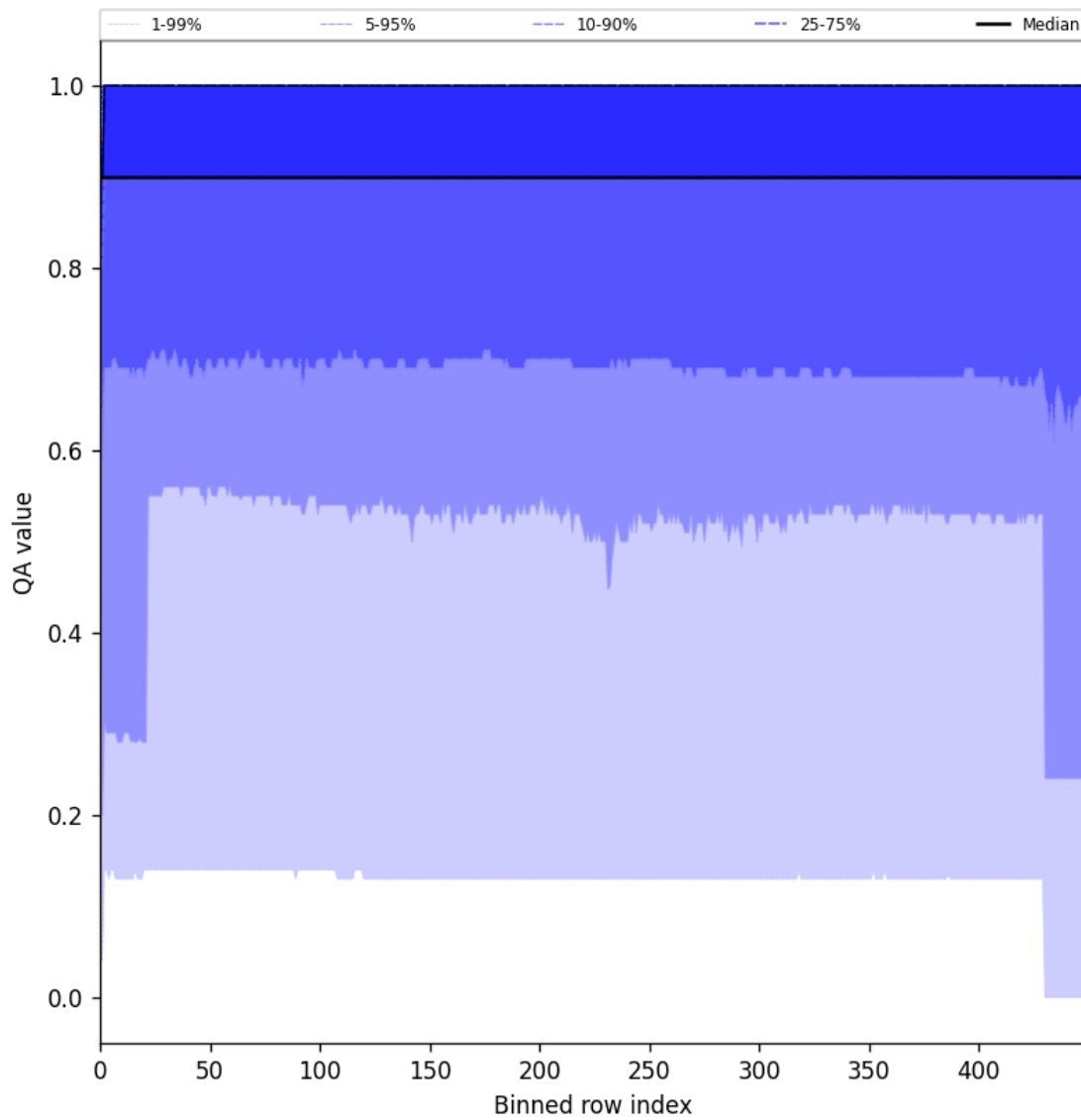
Figure 27: Along track statistics of “QA value” for 2025-09-22 to 2025-09-24
