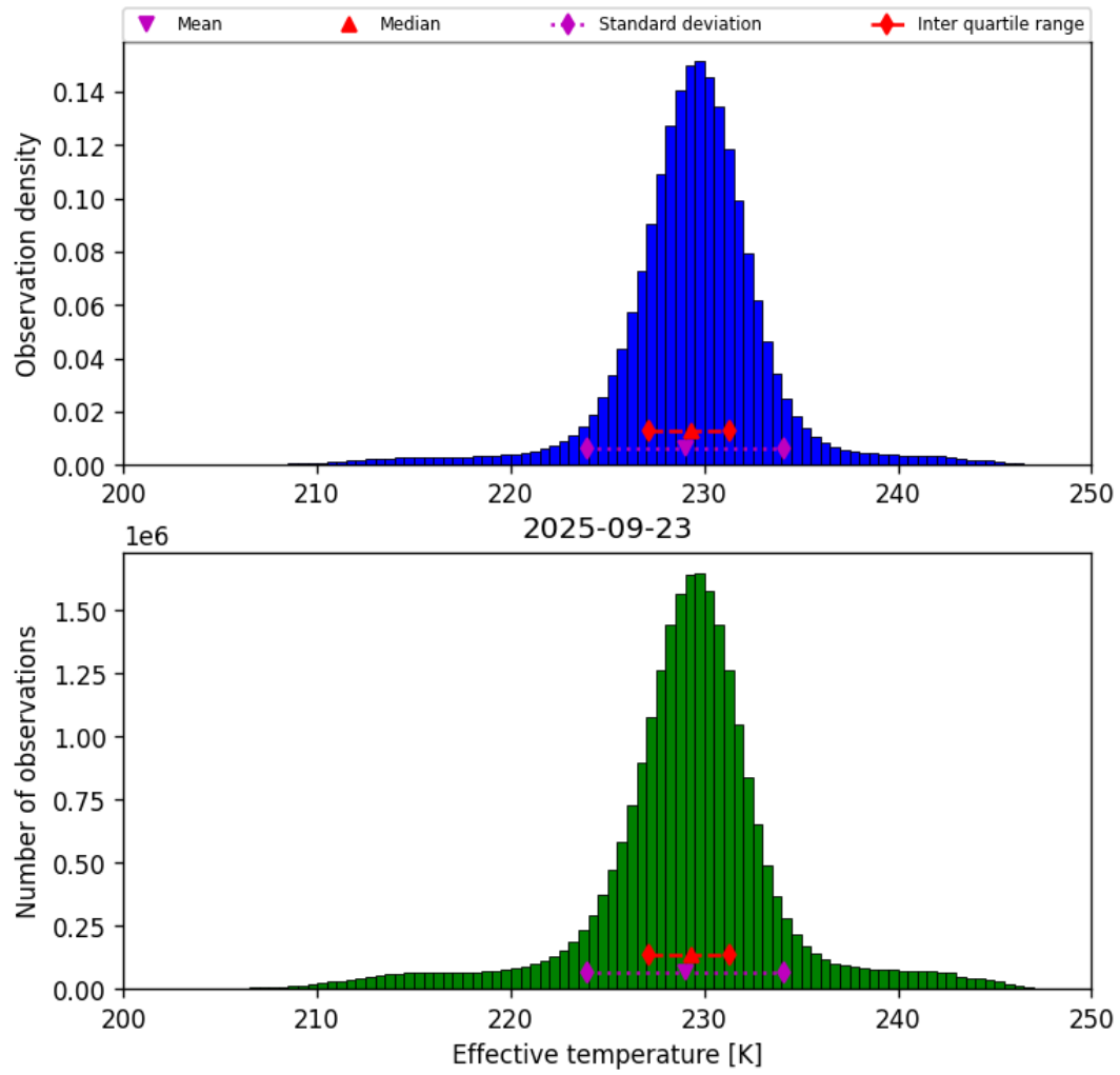
Figure 24: Histogram of “Effective temperature” for 2025-09-22 to 2025-09-24
