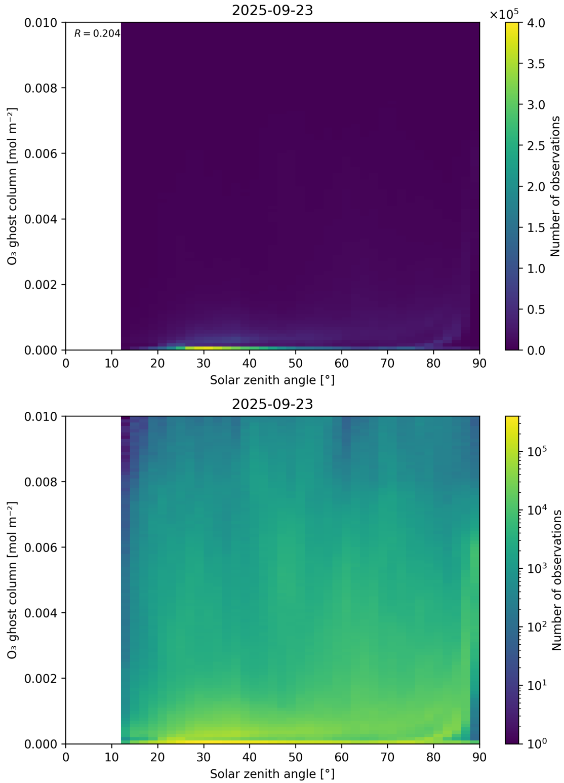
Figure 46: Scatter density plot of “Solar zenith angle” against “O 3 ghost column” for 2025-09-22 to 2025-09-24.
