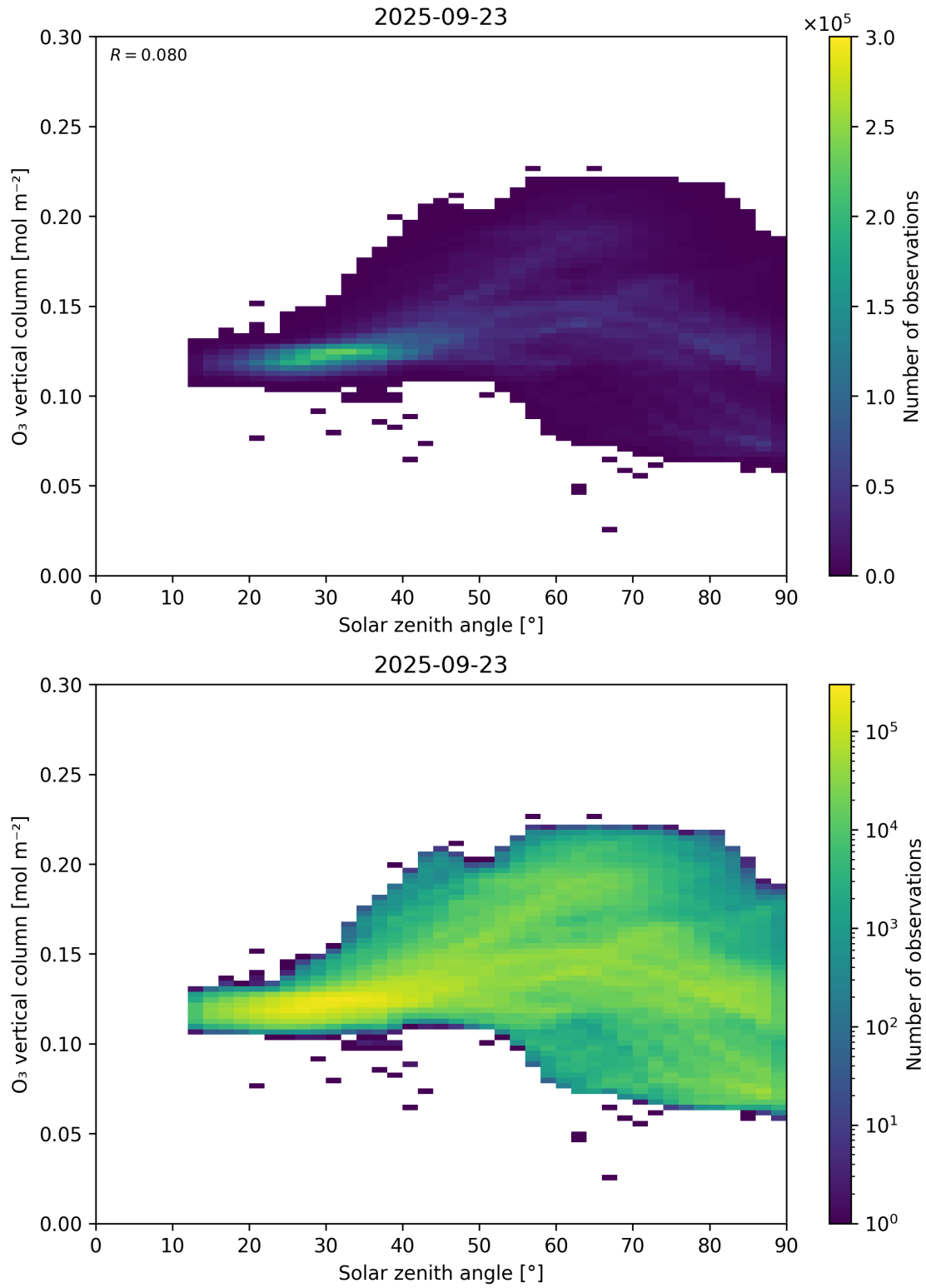
Figure 47: Scatter density plot of “Solar zenith angle” against “O 3 vertical column” for 2025-09-22 to 2025-09-24.
