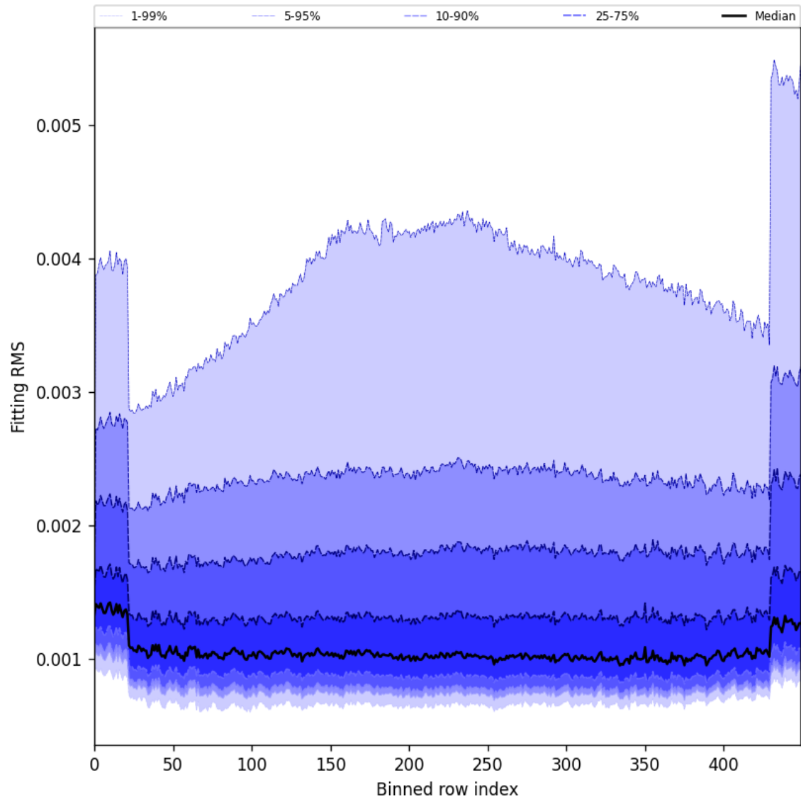
Figure 30: Along track statistics of “Fitting RMS” for 2025-09-22 to 2025-09-24
