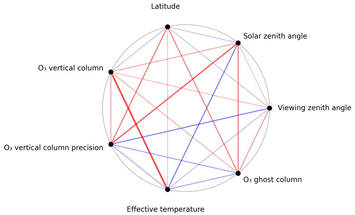
Figure 1: Map of correlation graph for 2025-09-22 to 2025-09-24.
