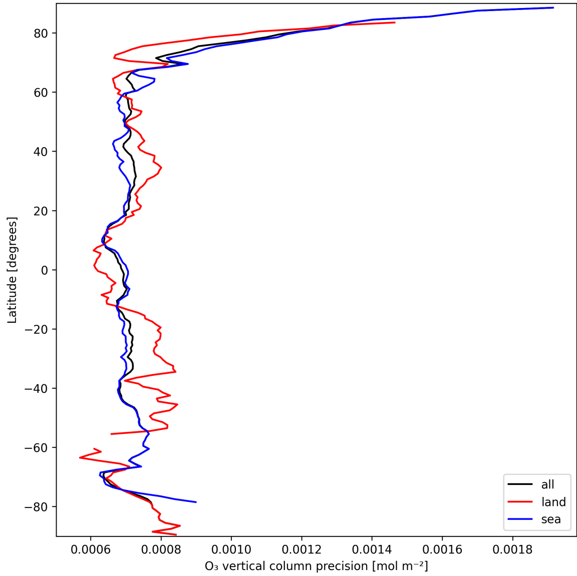
Figure 15: Zonal average of “O 3 vertical column precision” for 2025-09-22 to 2025-09-24.
