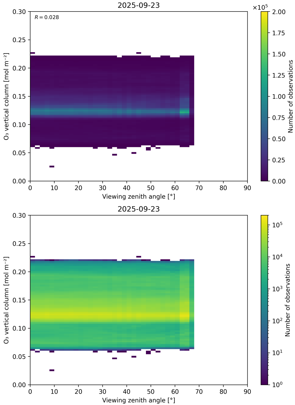
Figure 52: Scatter density plot of “Viewing zenith angle” against “O 3 vertical column” for 2025-09-22 to 2025-09-24.
