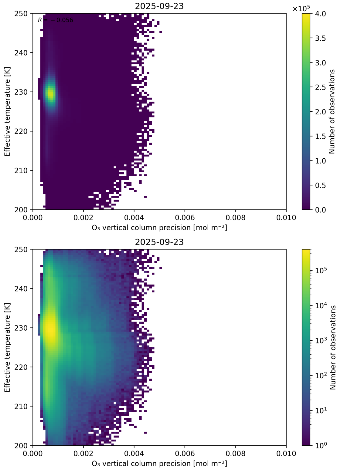
Figure 42: Scatter density plot of “O 3 vertical column precision” against “Effective temperature” for 2025-09-22 to 2025-09-24.
