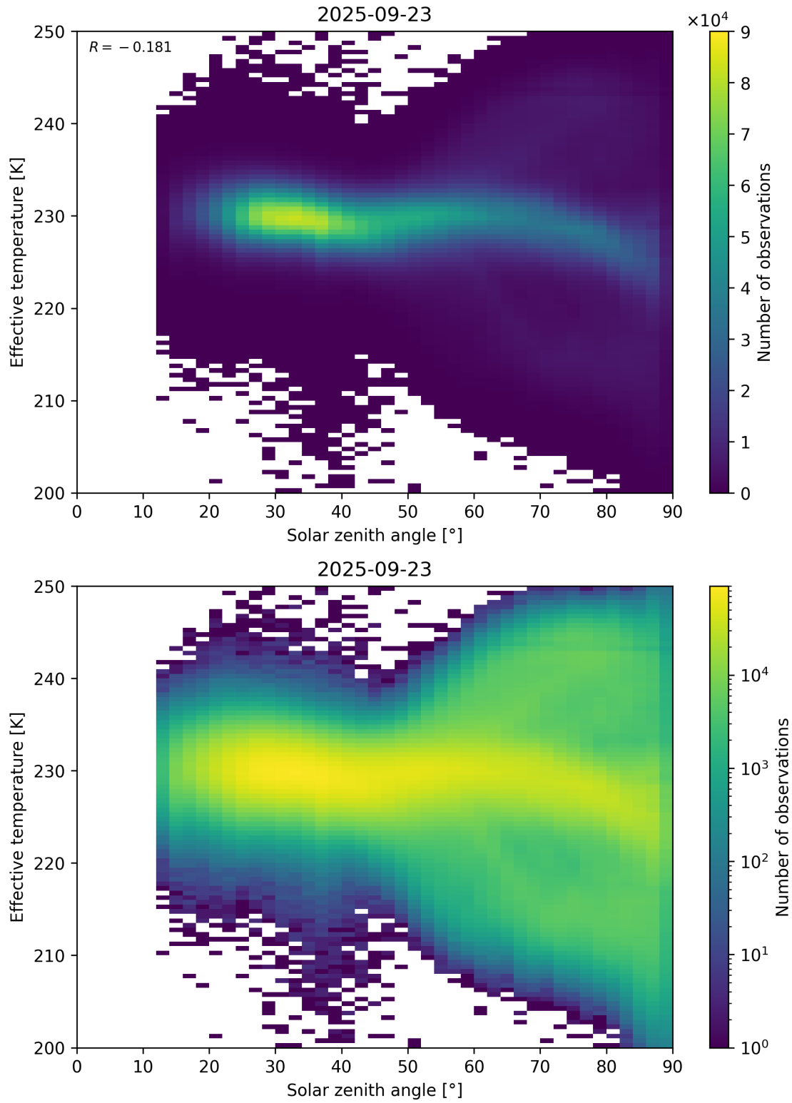
Figure 45: Scatter density plot of “Solar zenith angle” against “Effective temperature” for 2025-09-22 to 2025-09-24.
