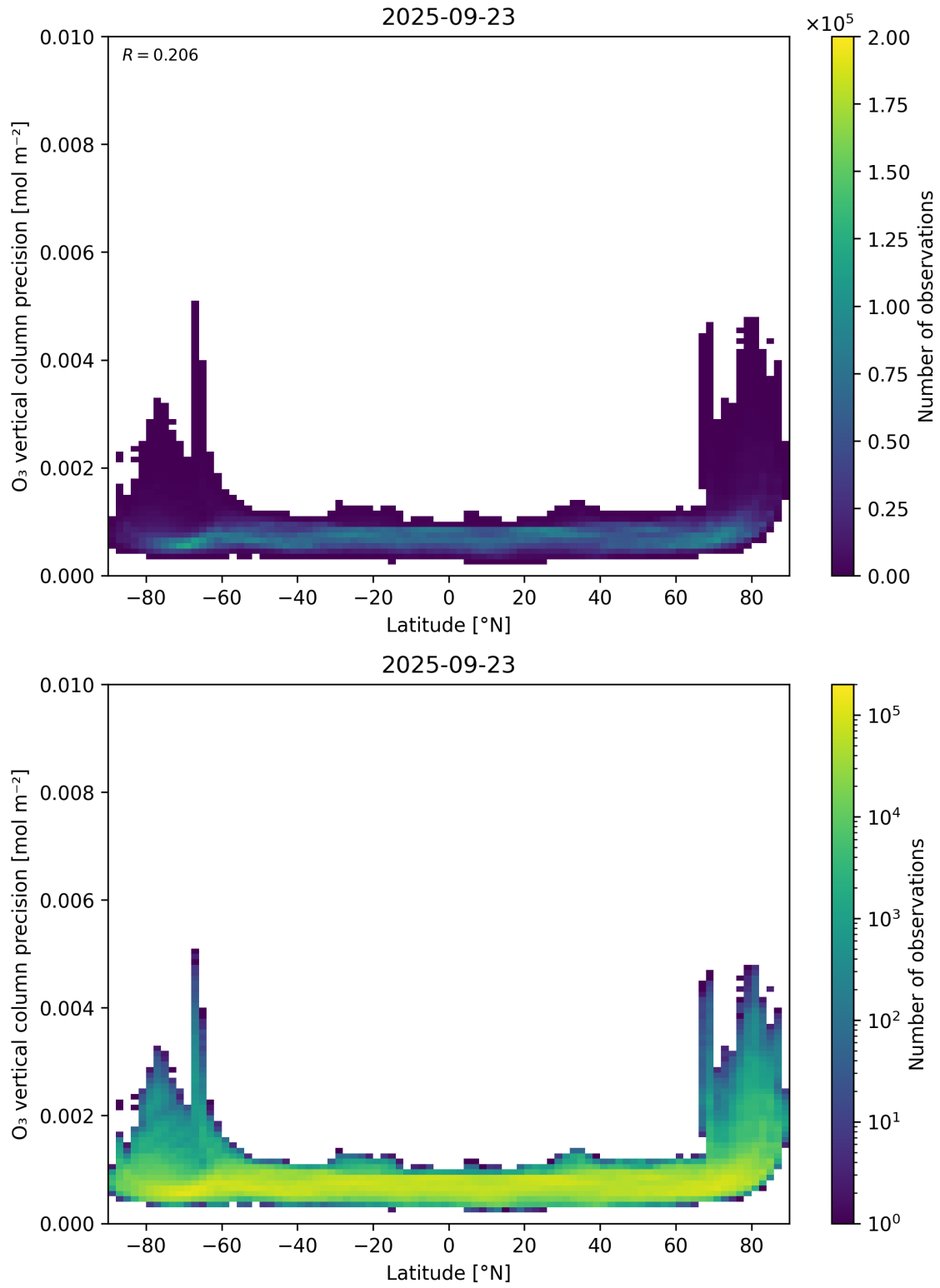
Figure 37: Scatter density plot of “Latitude” against “O 3 vertical column precision” for 2025-09-22 to 2025-09-24.
