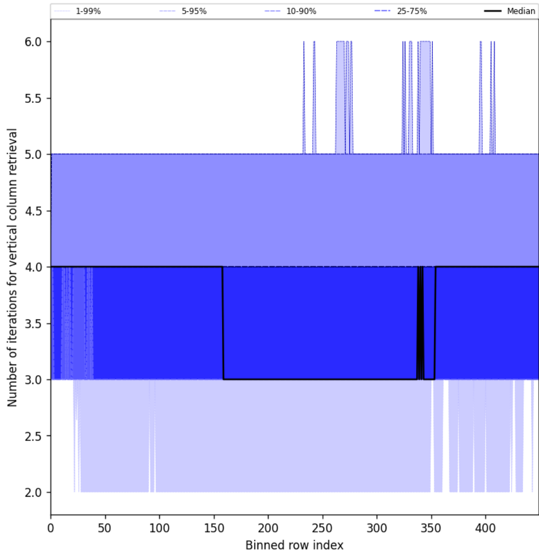
Figure 33: Along track statistics of “Number of iterations for vertical column retrieval” for 2025-09-22 to 2025-09-24
