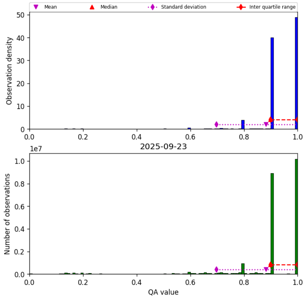
Figure 20: Histogram of “QA value” for 2025-09-22 to 2025-09-24
