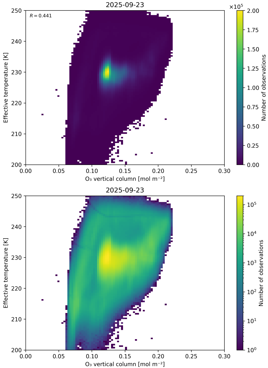
Figure 39: Scatter density plot of “O 3 vertical column” against “Effective temperature” for 2025-09-22 to 2025-09-24.
