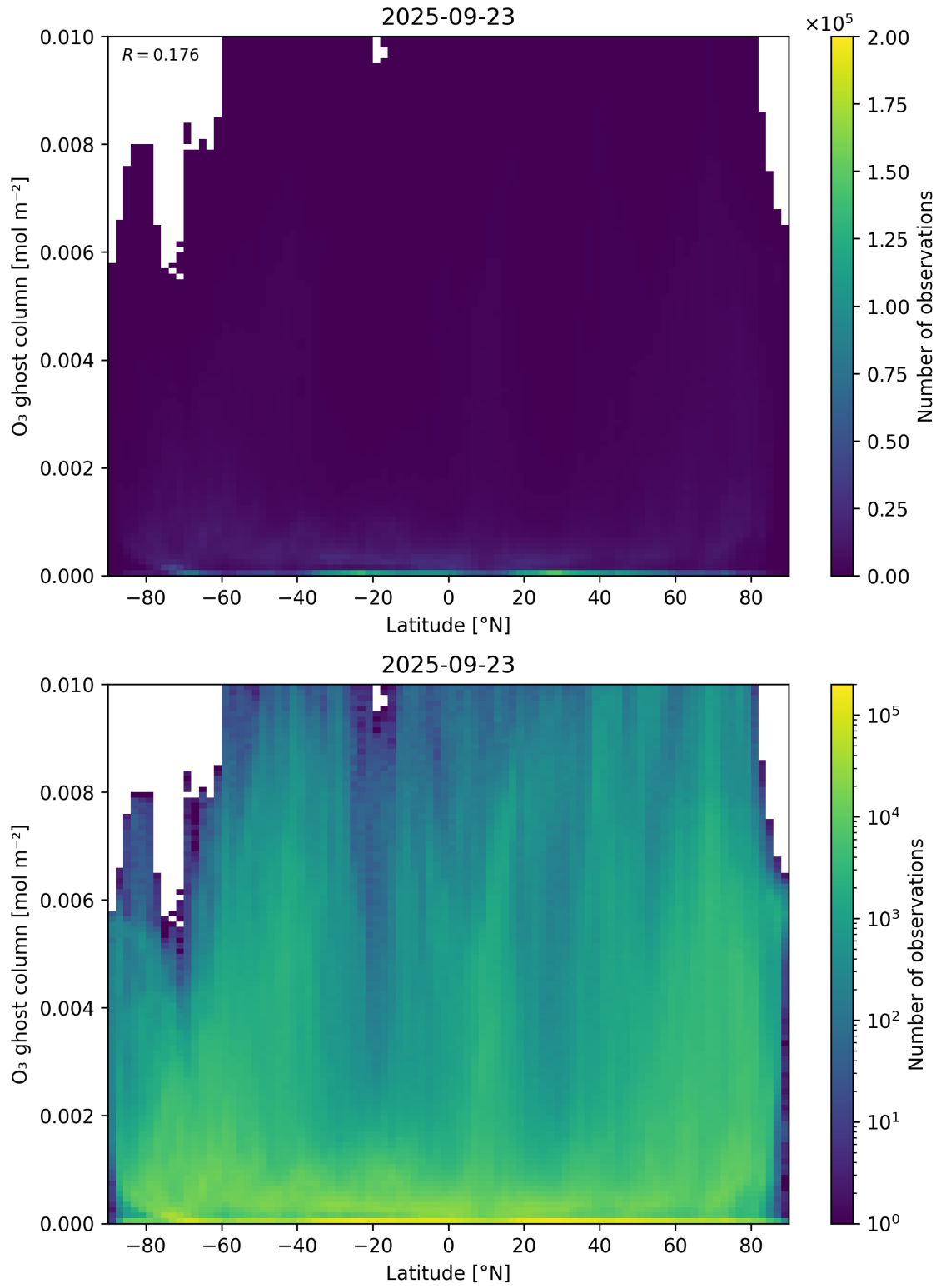
Figure 35: Scatter density plot of “Latitude” against “O 3 ghost column” for 2025-09-22 to 2025-09-24.
