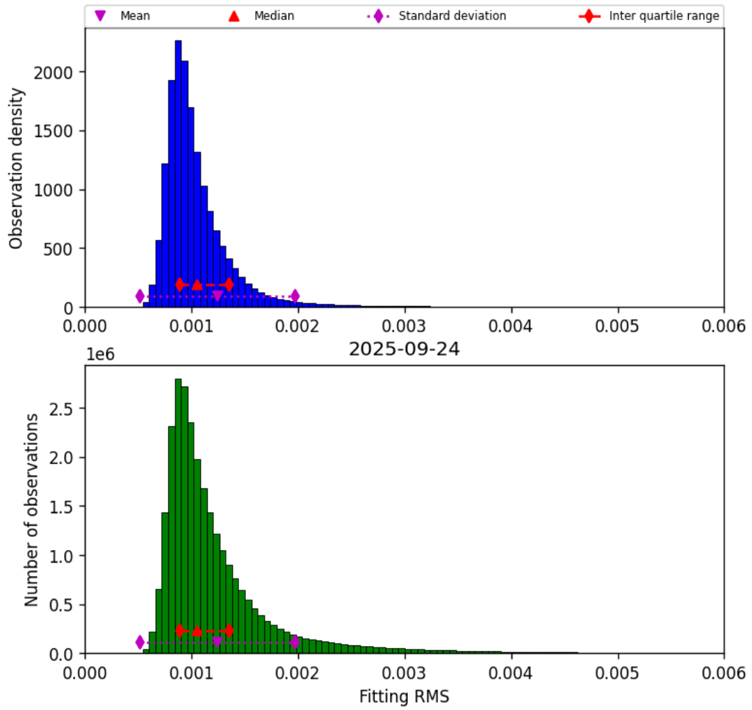
Figure 23: Histogram of “Fitting RMS” for 2025-09-23 to 2025-09-25
