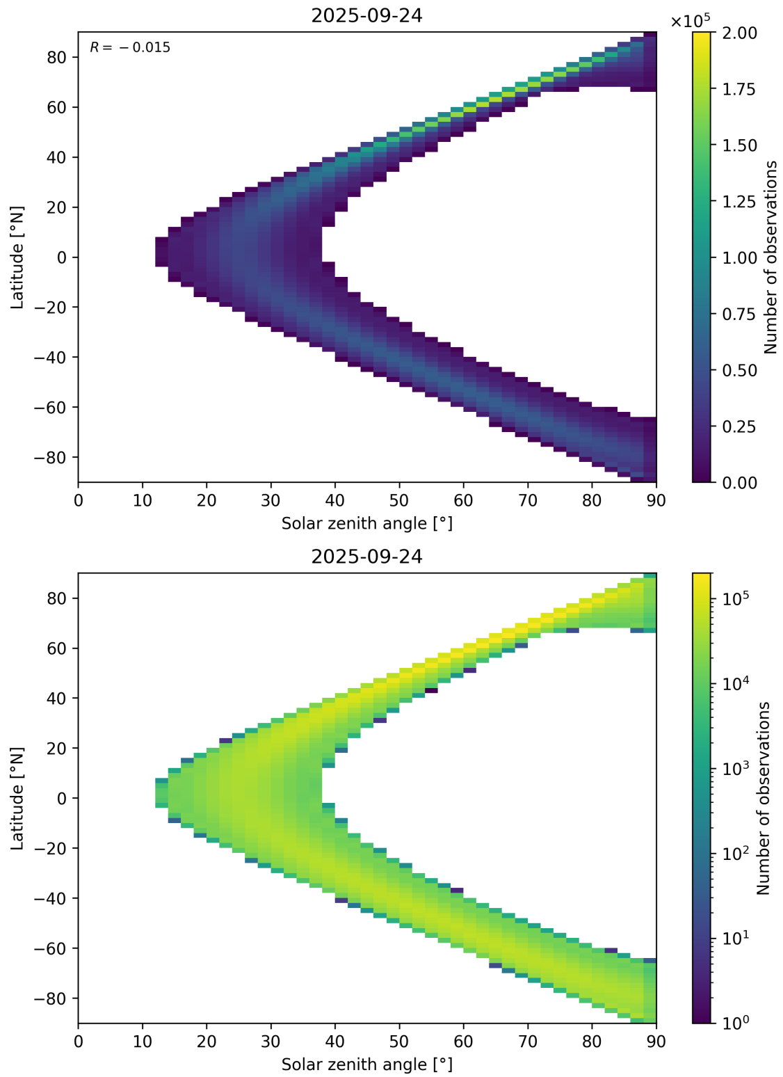
Figure 44: Scatter density plot of “Solar zenith angle” against “Latitude” for 2025-09-23 to 2025-09-25.
