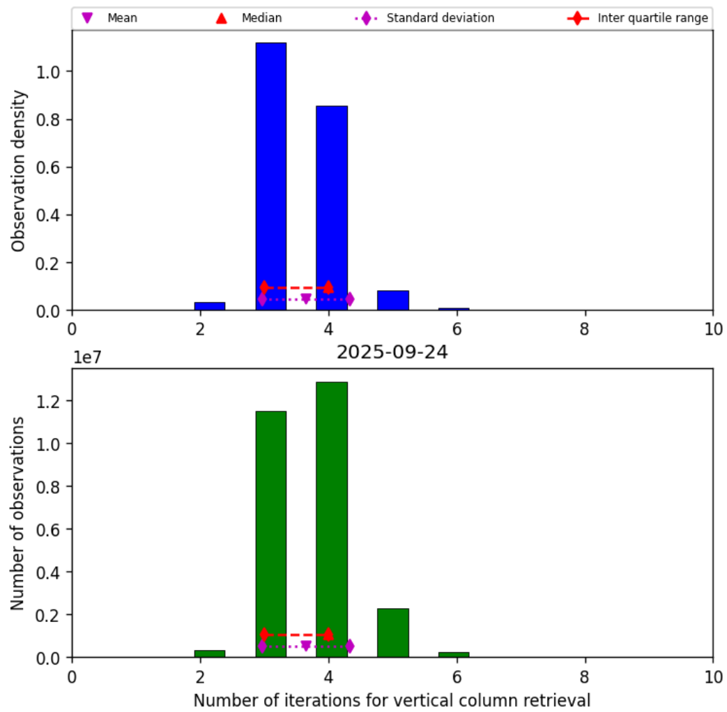
Figure 26: Histogram of “Number of iterations for vertical column retrieval” for 2025-09-23 to 2025-09-25
