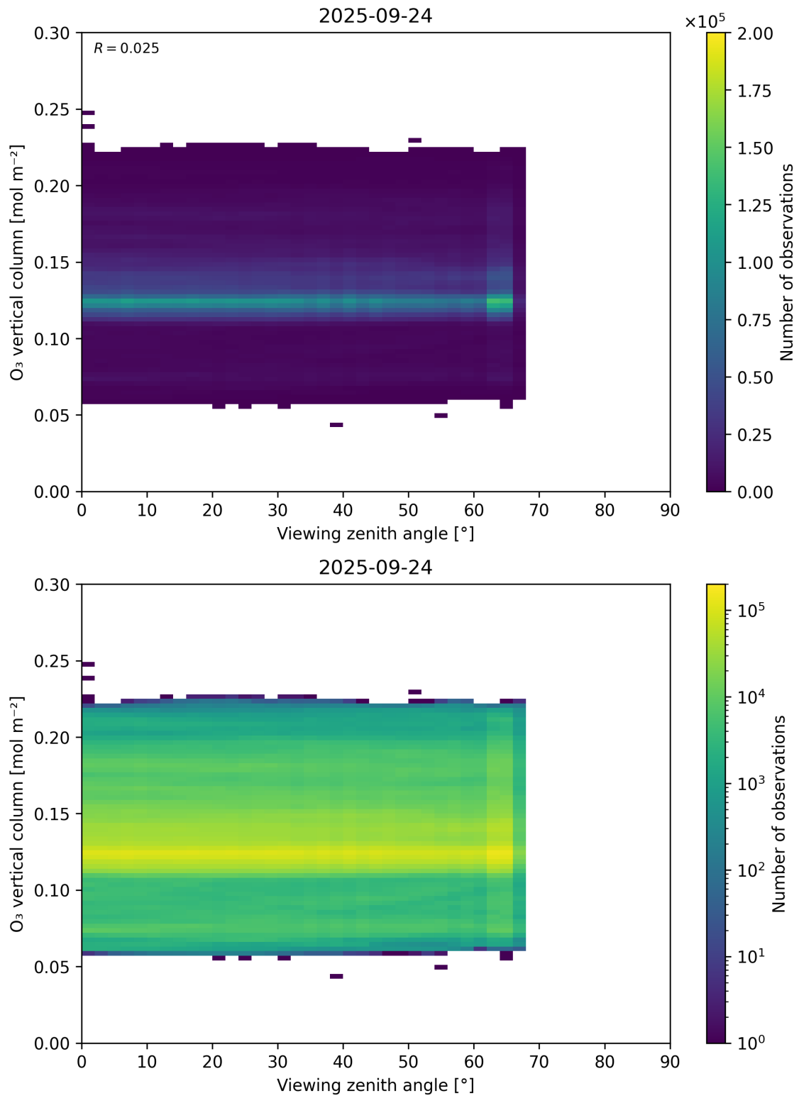
Figure 52: Scatter density plot of “Viewing zenith angle” against “O 3 vertical column” for 2025-09-23 to 2025-09-25.
