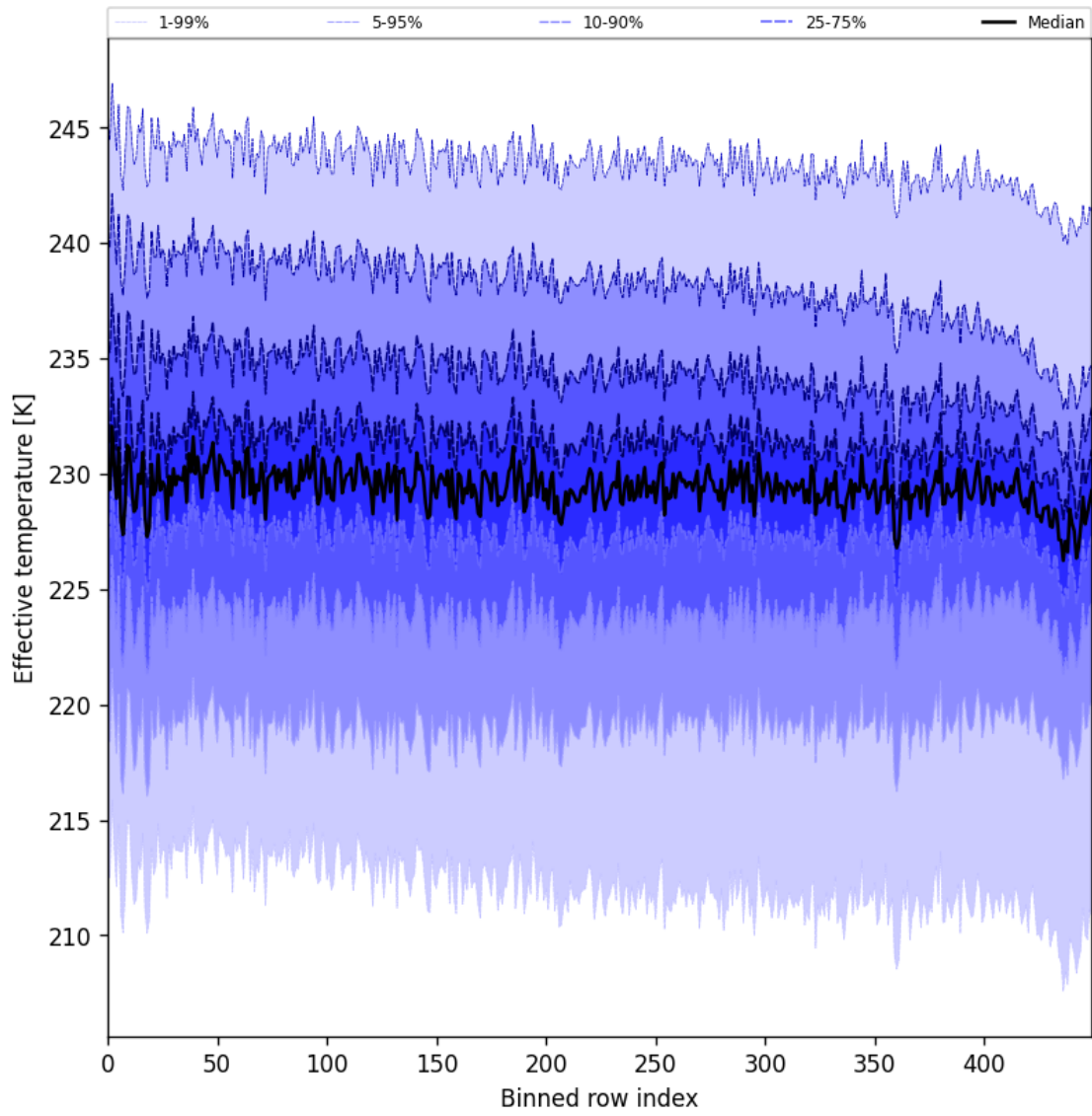
Figure 31: Along track statistics of “Effective temperature” for 2025-09-23 to 2025-09-25
