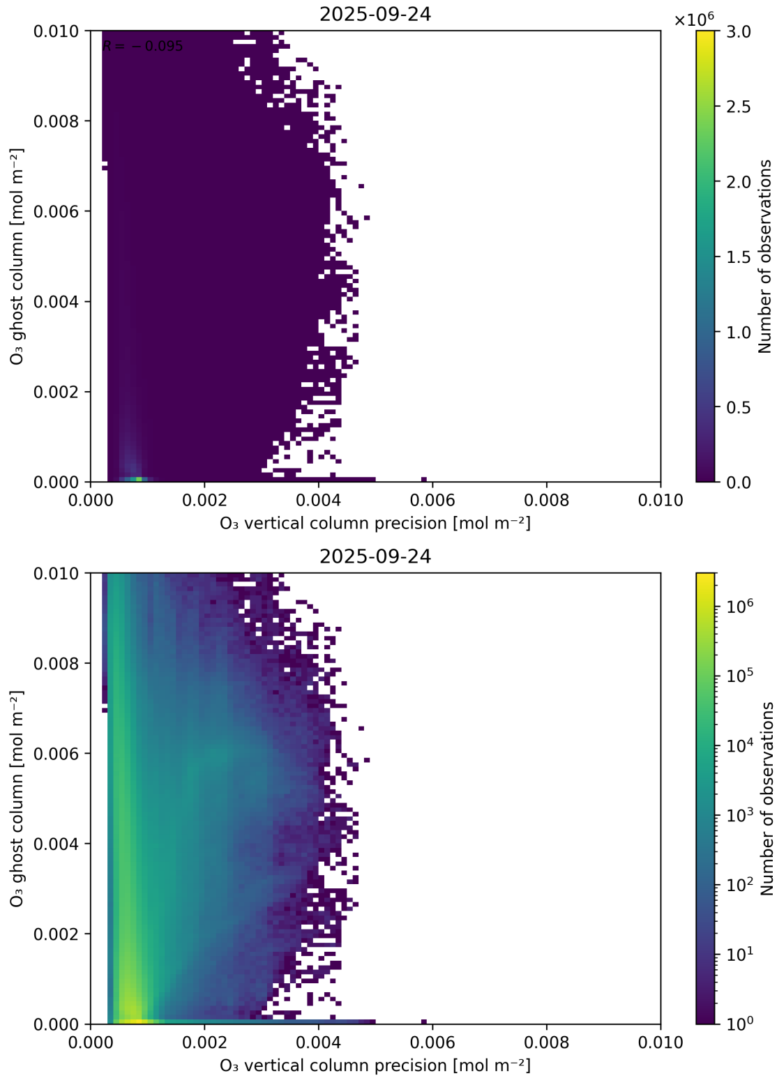
Figure 43: Scatter density plot of “ \text{O}_3 vertical column precision” against “ \text{O}_3 ghost column” for 2025-09-23 to 2025-09-25.
