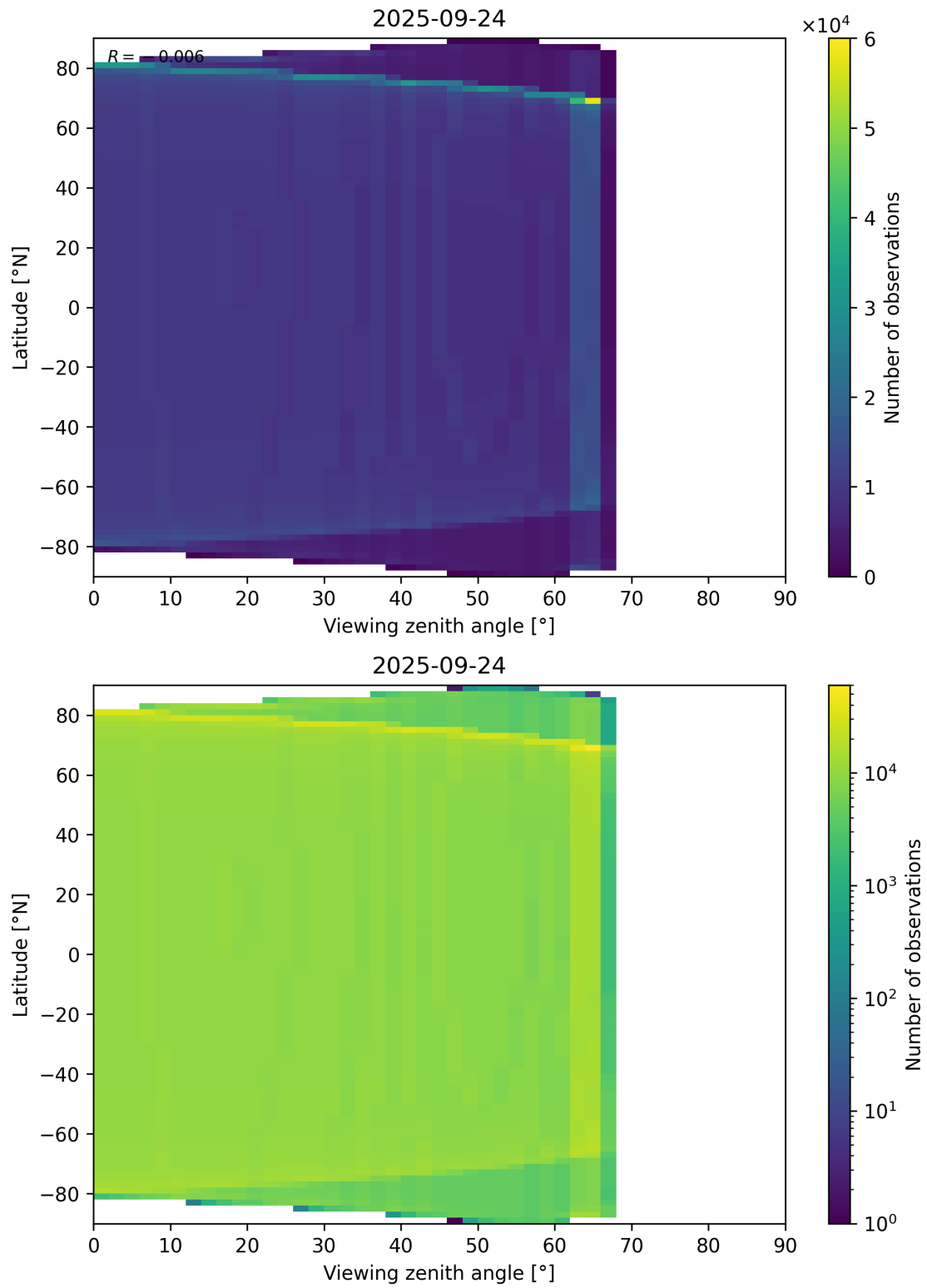
Figure 49: Scatter density plot of “Viewing zenith angle” against “Latitude” for 2025-09-23 to 2025-09-25.
