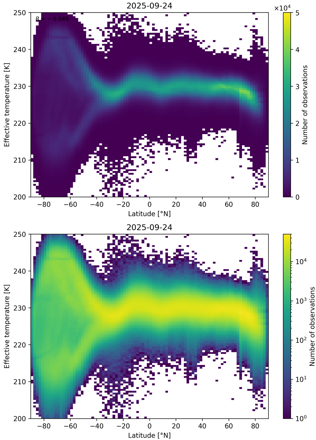
Figure 34: Scatter density plot of “Latitude” against “Effective temperature” for 2025-09-23 to 2025-09-25.
