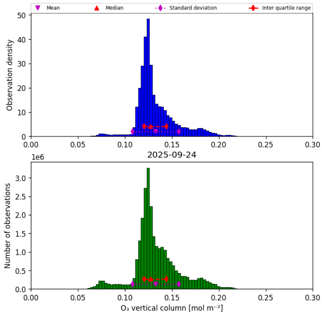
Figure 21: Histogram of “O 3 vertical column” for 2025-09-23 to 2025-09-25
