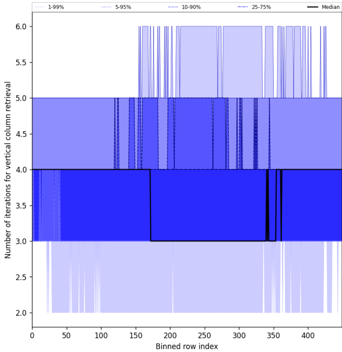
Figure 33: Along track statistics of “Number of iterations for vertical column retrieval” for 2025-09-23 to 2025-09-25
