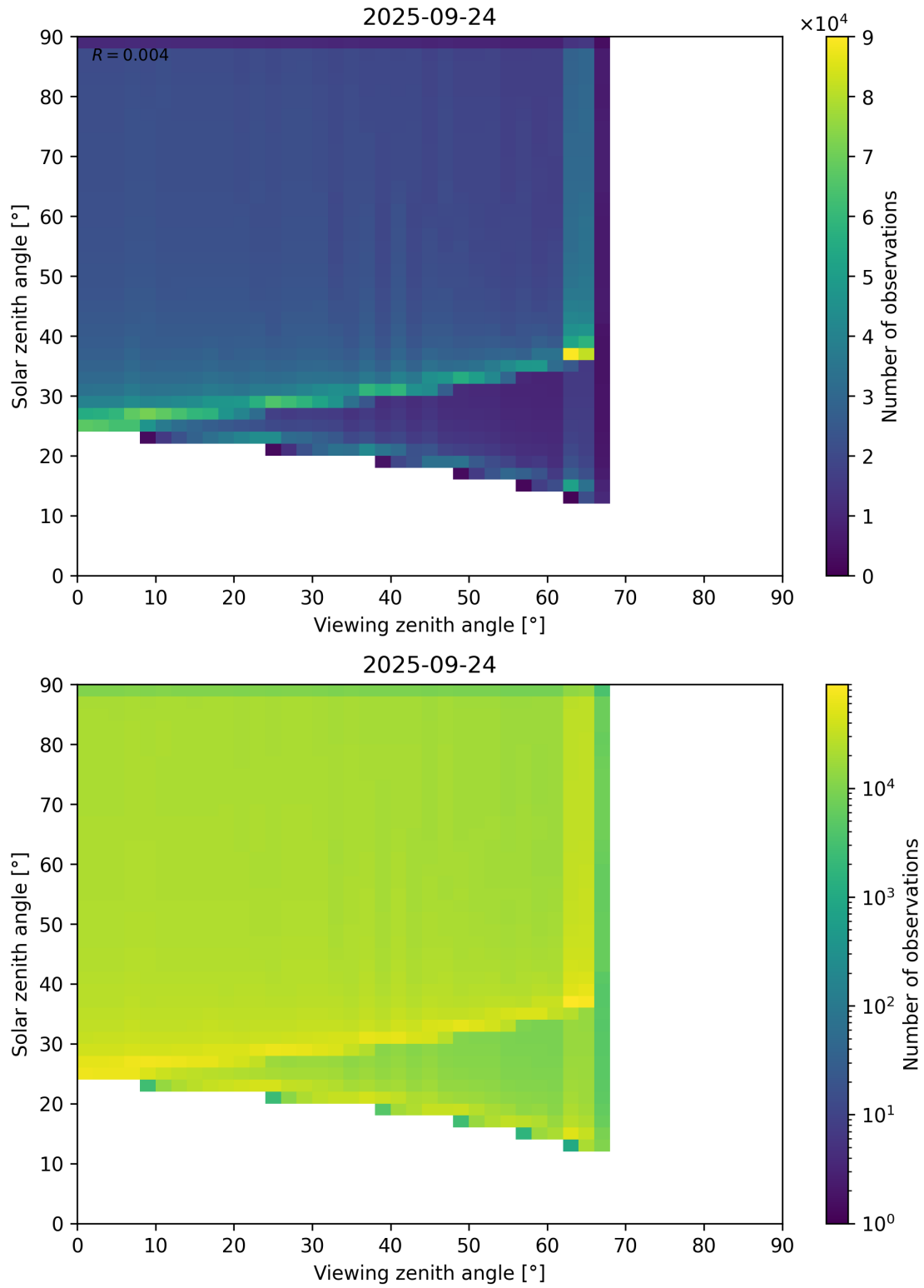
Figure 54: Scatter density plot of “Viewing zenith angle” against “Solar zenith angle” for 2025-09-23 to 2025-09-25.
