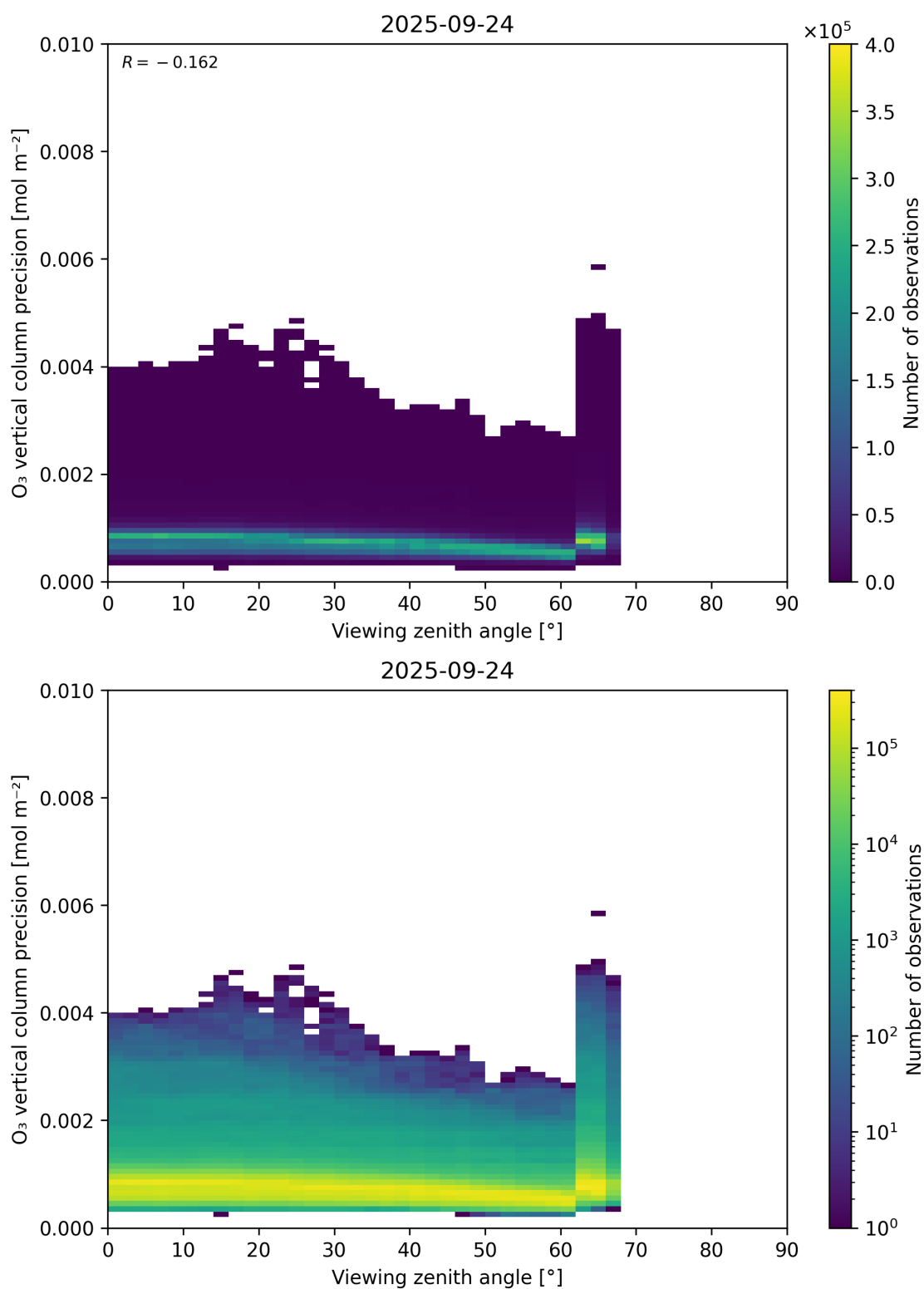
Figure 53: Scatter density plot of “Viewing zenith angle” against “O 3 vertical column precision” for 2025-09-23 to 2025-09-25.
