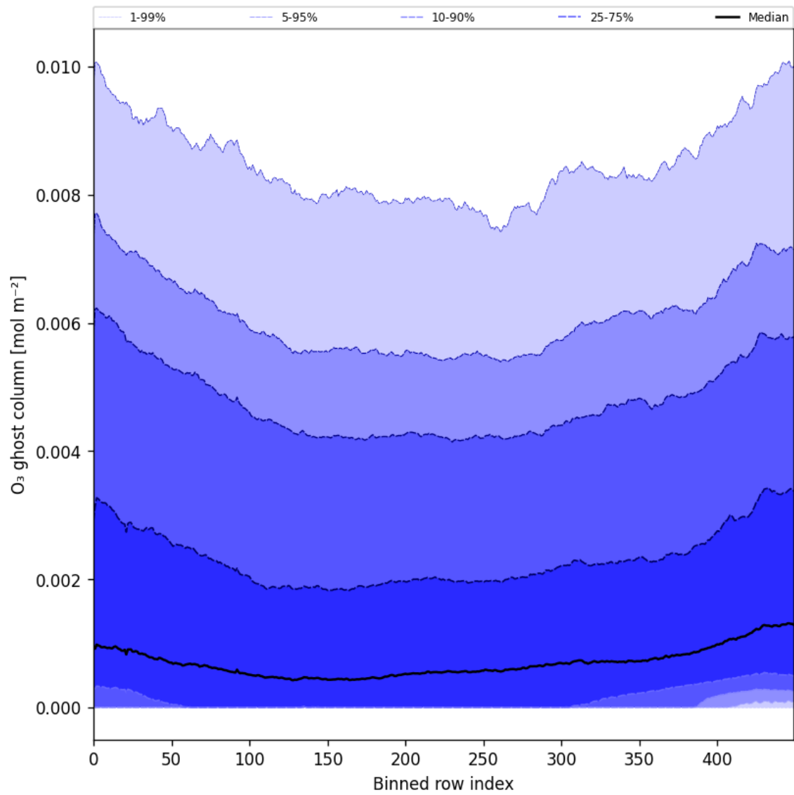
Figure 32: Along track statistics of “O 3 ghost column” for 2025-09-23 to 2025-09-25
