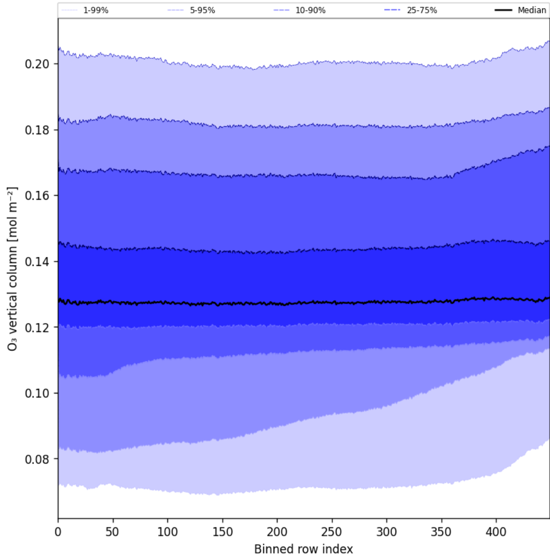
Figure 28: Along track statistics of “O 3 vertical column” for 2025-09-23 to 2025-09-25
