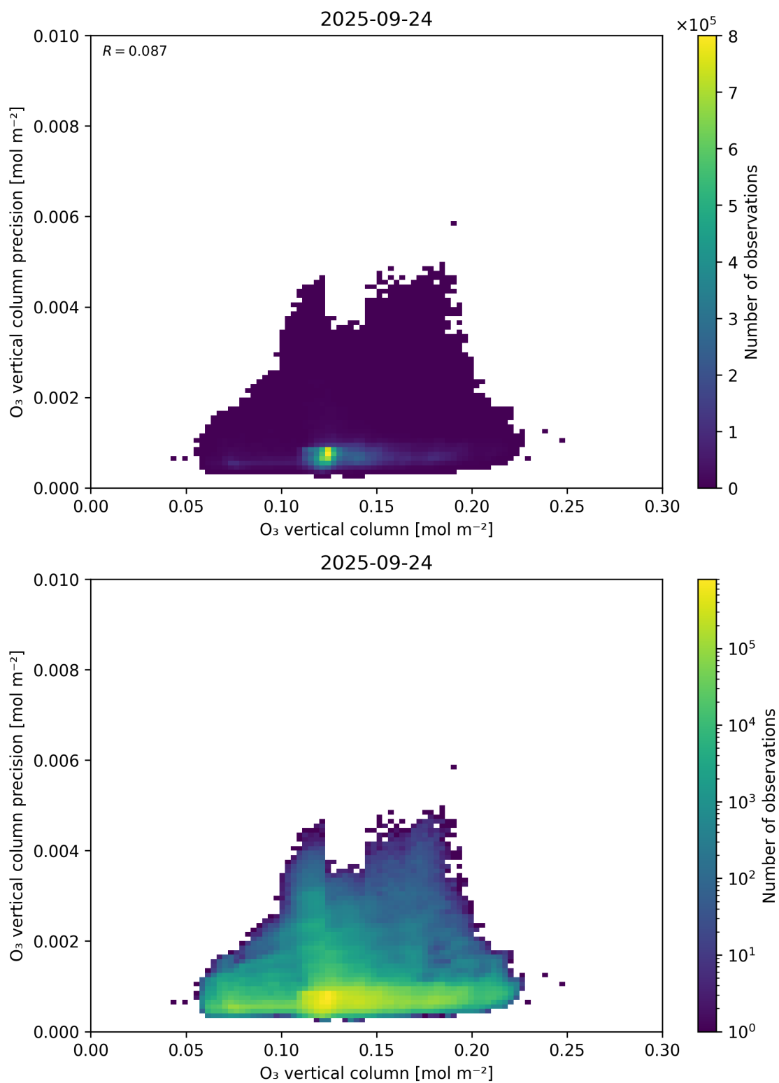
Figure 41: Scatter density plot of “O 3 vertical column” against “O 3 vertical column precision” for 2025-09-23 to 2025-09-25.
