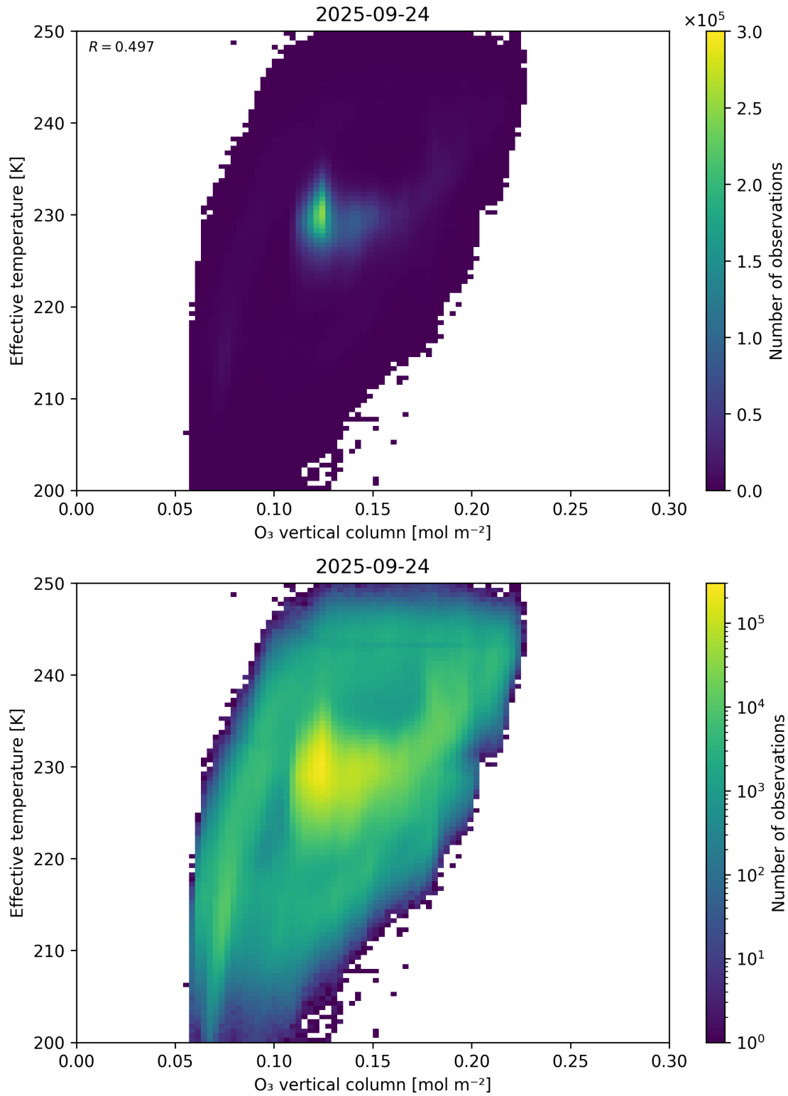
Figure 39: Scatter density plot of “O 3 vertical column” against “Effective temperature” for 2025-09-23 to 2025-09-25.
