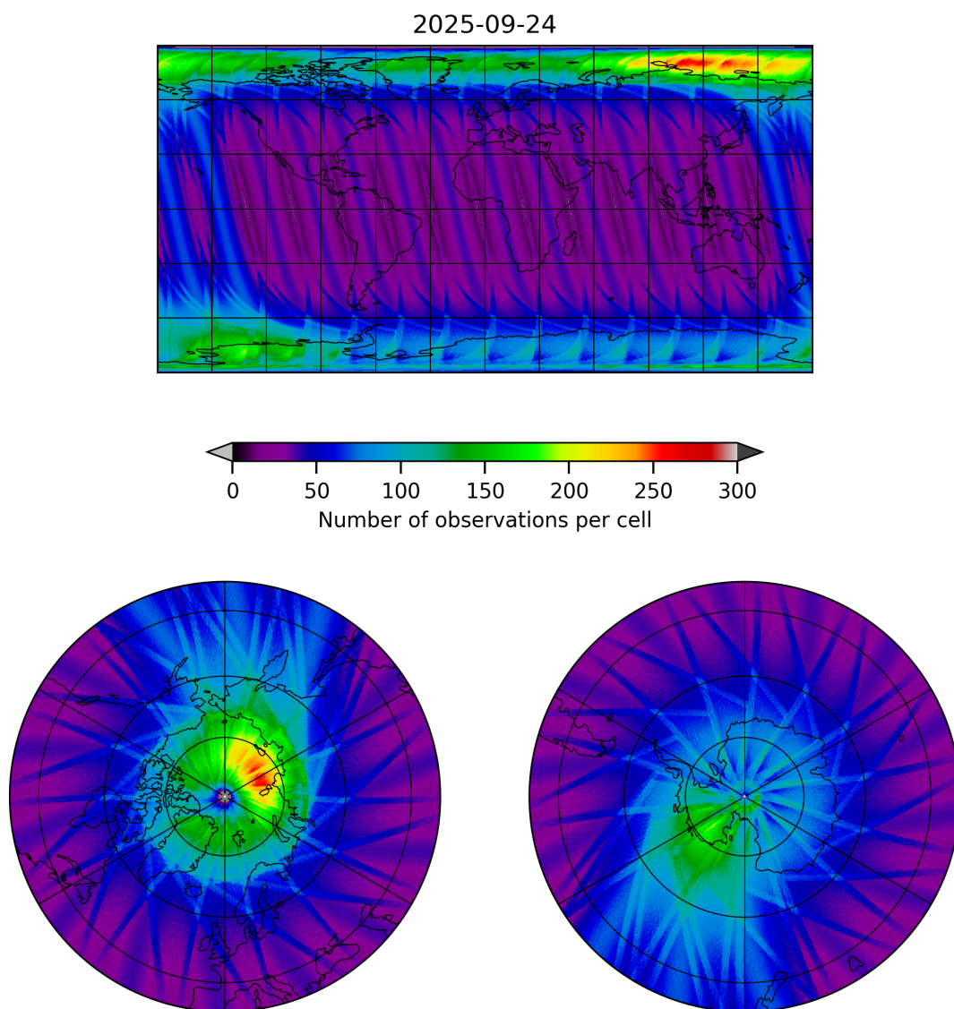
Figure 12: Map of the number of observations for 2025-09-23 to 2025-09-25
