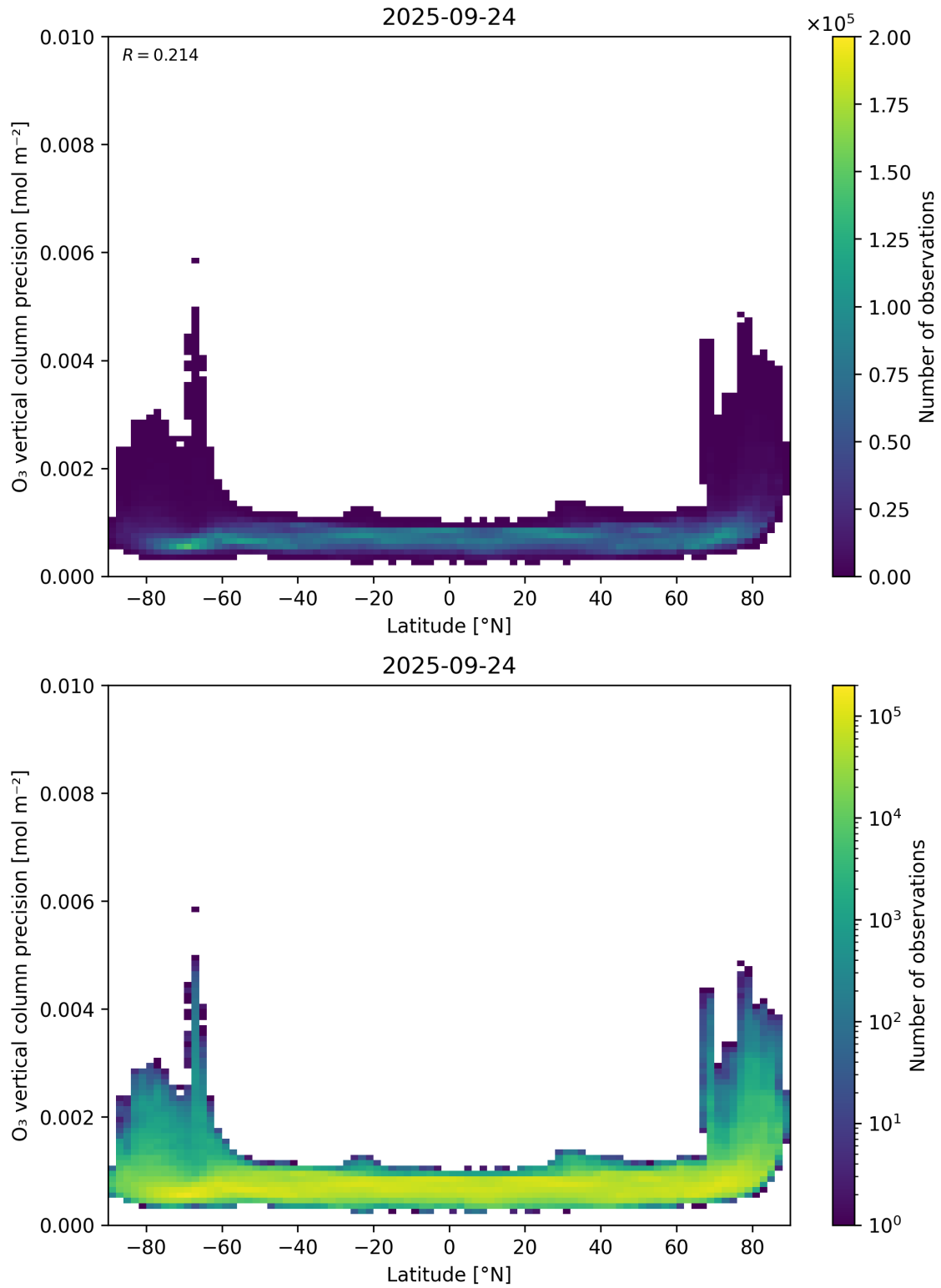
Figure 37: Scatter density plot of “Latitude” against “O 3 vertical column precision” for 2025-09-23 to 2025-09-25.
