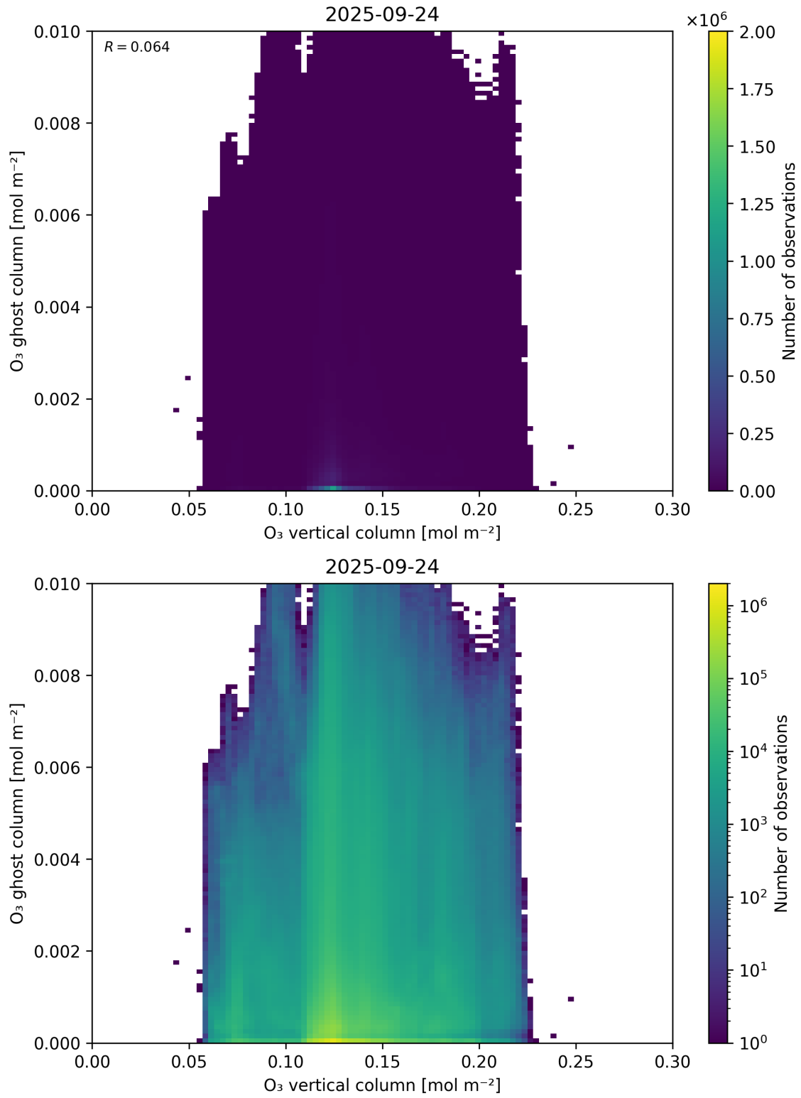
Figure 40: Scatter density plot of “O 3 vertical column” against “O 3 ghost column” for 2025-09-23 to 2025-09-25.
