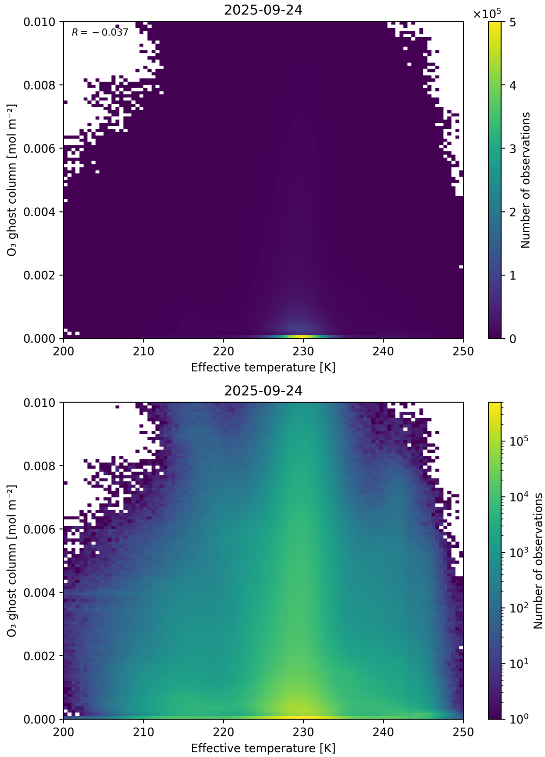
Figure 38: Scatter density plot of “Effective temperature” against “O 3 ghost column” for 2025-09-23 to 2025-09-25.
