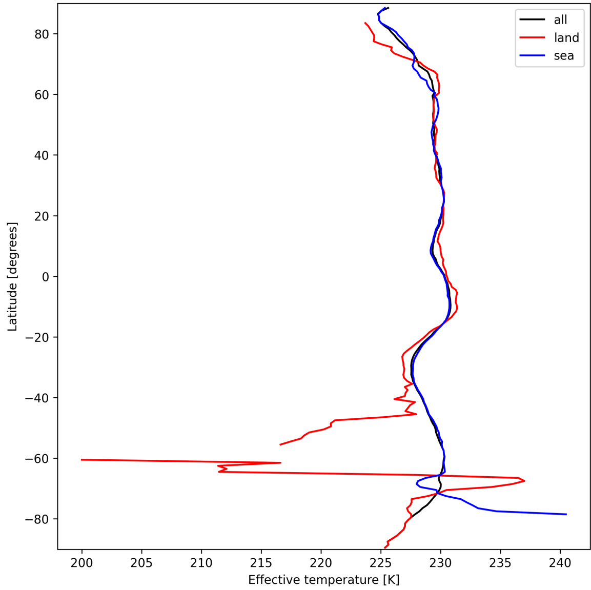
Figure 17: Zonal average of “Effective temperature” for 2025-09-23 to 2025-09-25.
