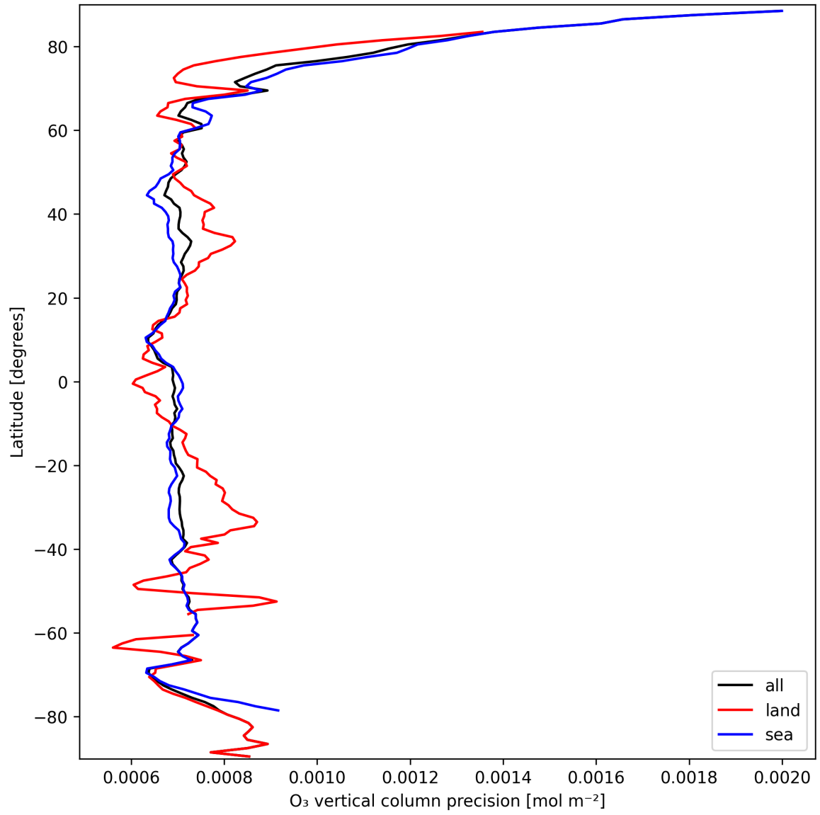
Figure 15: Zonal average of "O 3 vertical column precision" for 2025-09-23 to 2025-09-25.
