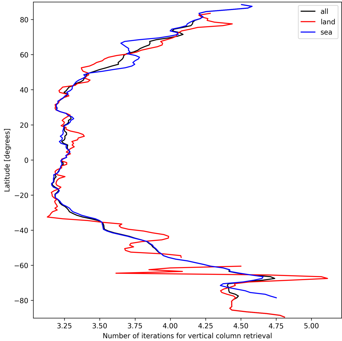
Figure 19: Zonal average of “Number of iterations for vertical column retrieval” for 2025-09-23 to 2025-09-25.
