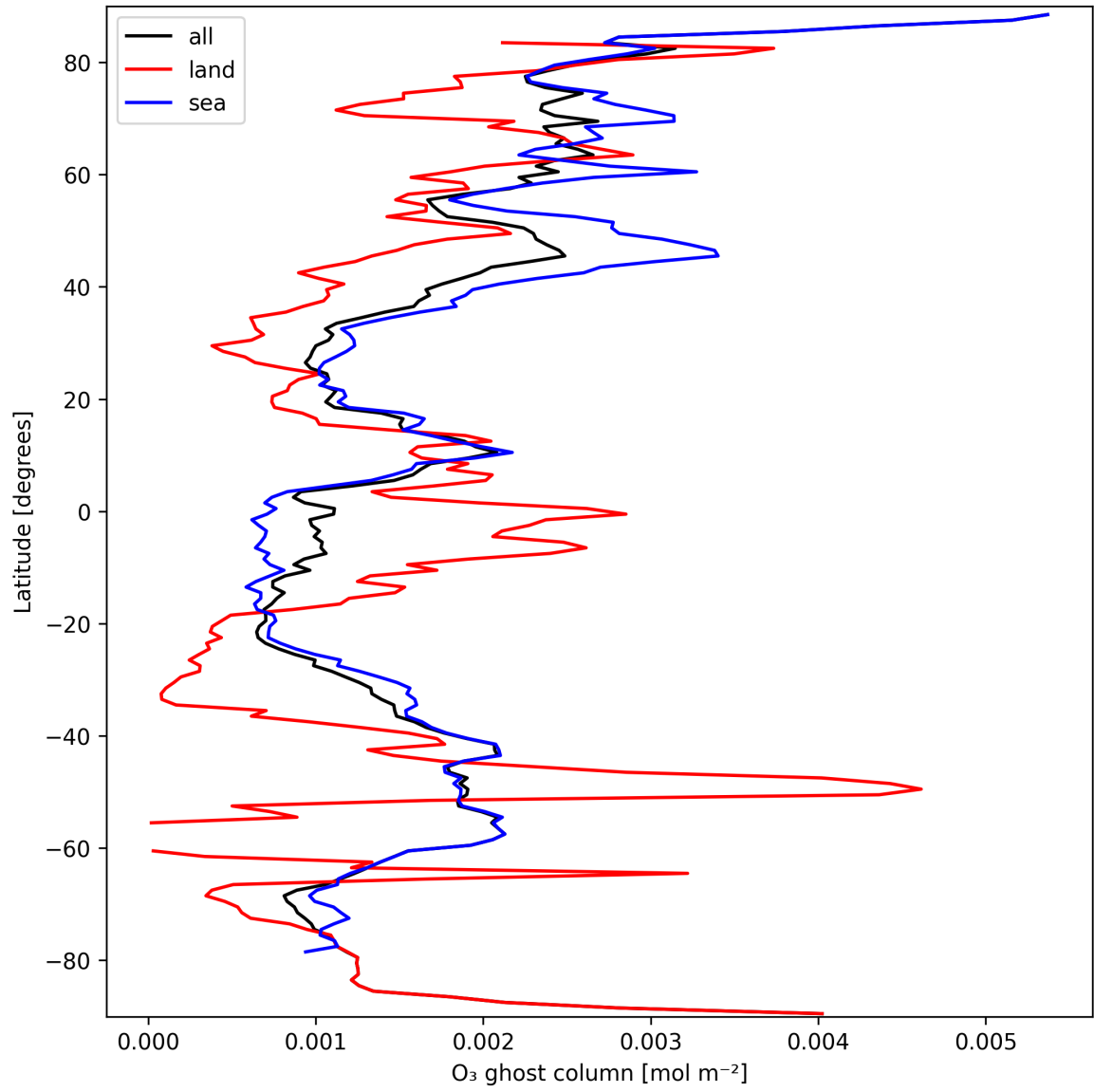
Figure 18: Zonal average of "O 3 ghost column" for 2025-09-23 to 2025-09-25.
