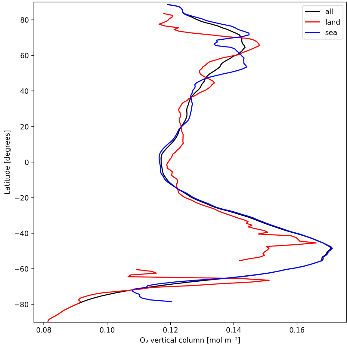
Figure 14: Zonal average of “O 3 vertical column” for 2025-09-23 to 2025-09-25.
