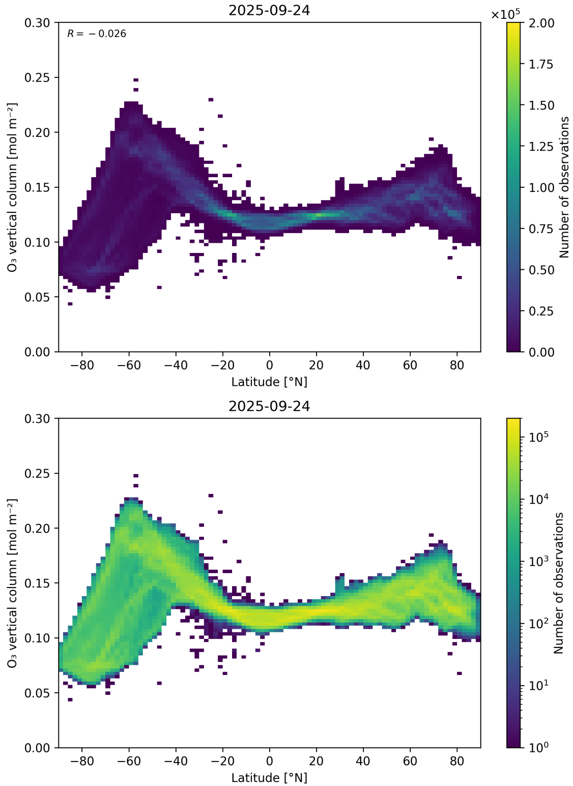
Figure 36: Scatter density plot of “Latitude” against “O 3 vertical column” for 2025-09-23 to 2025-09-25.
