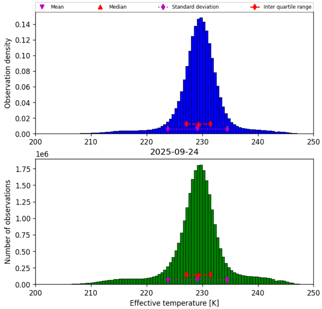
Figure 24: Histogram of “Effective temperature” for 2025-09-23 to 2025-09-25
