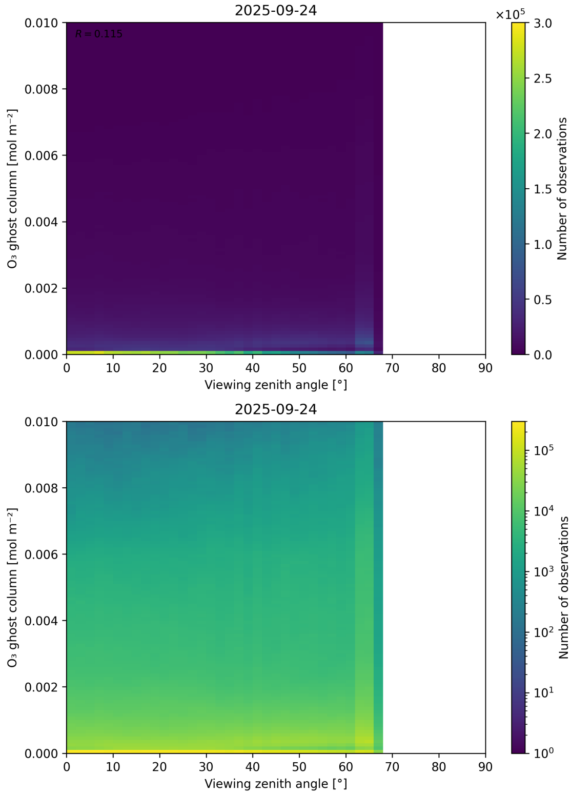
Figure 51: Scatter density plot of “Viewing zenith angle” against “O 3 ghost column” for 2025-09-23 to 2025-09-25.
