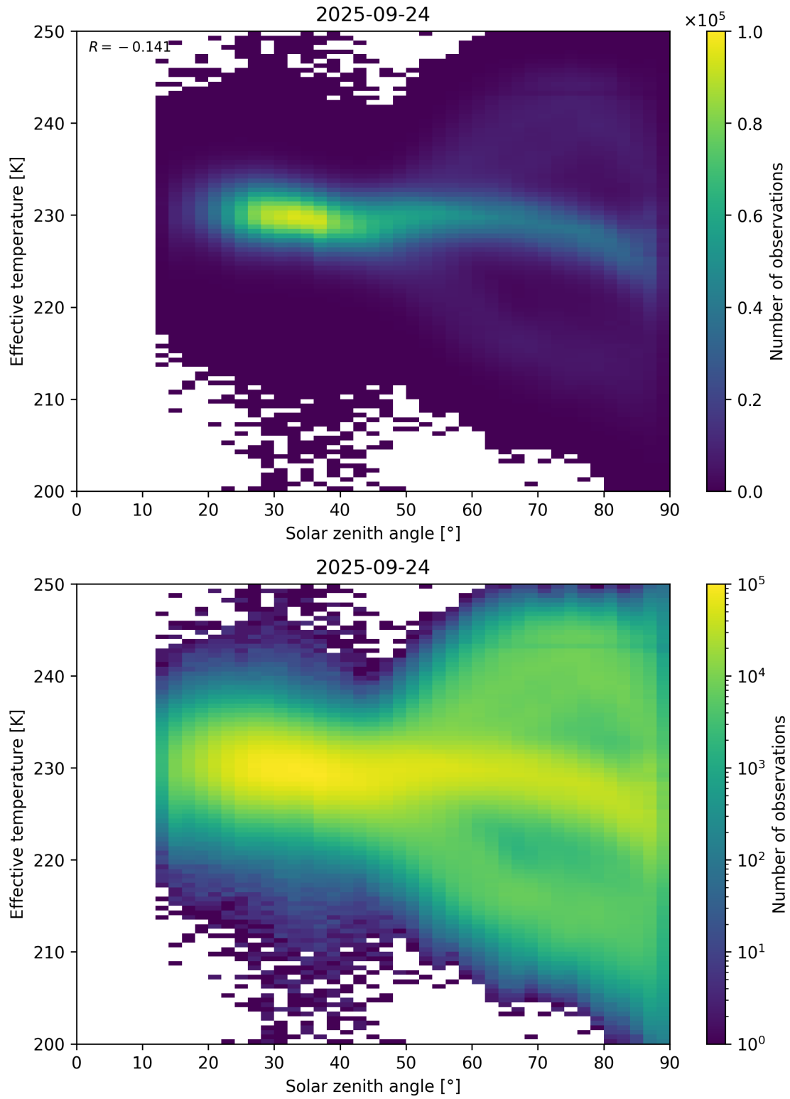
Figure 45: Scatter density plot of “Solar zenith angle” against “Effective temperature” for 2025-09-23 to 2025-09-25.
