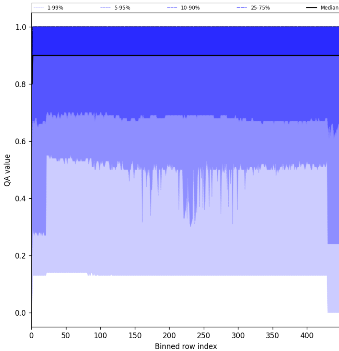
Figure 27: Along track statistics of “QA value” for 2025-09-23 to 2025-09-25
