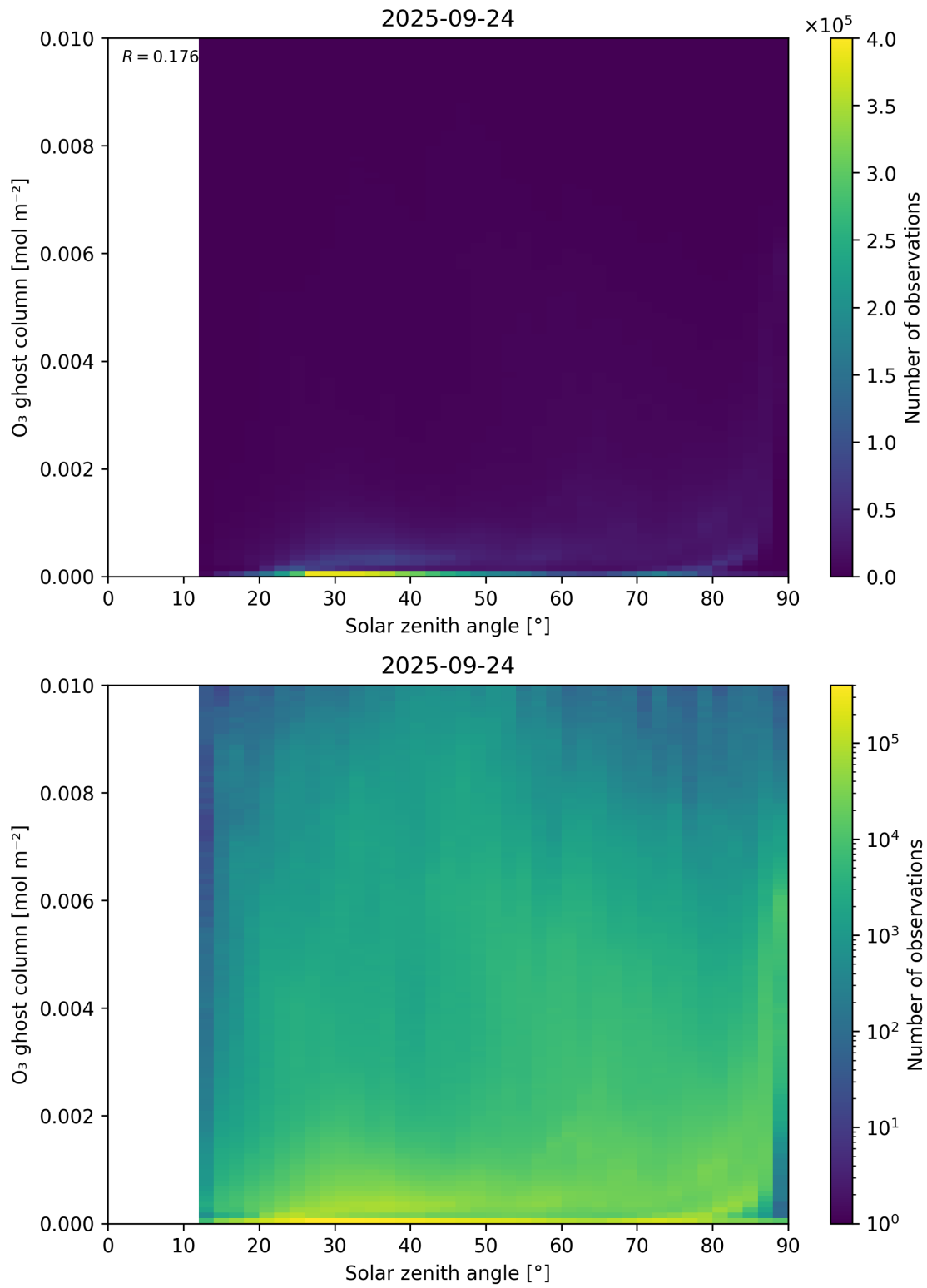
Figure 46: Scatter density plot of “Solar zenith angle” against “O 3 ghost column” for 2025-09-23 to 2025-09-25.
