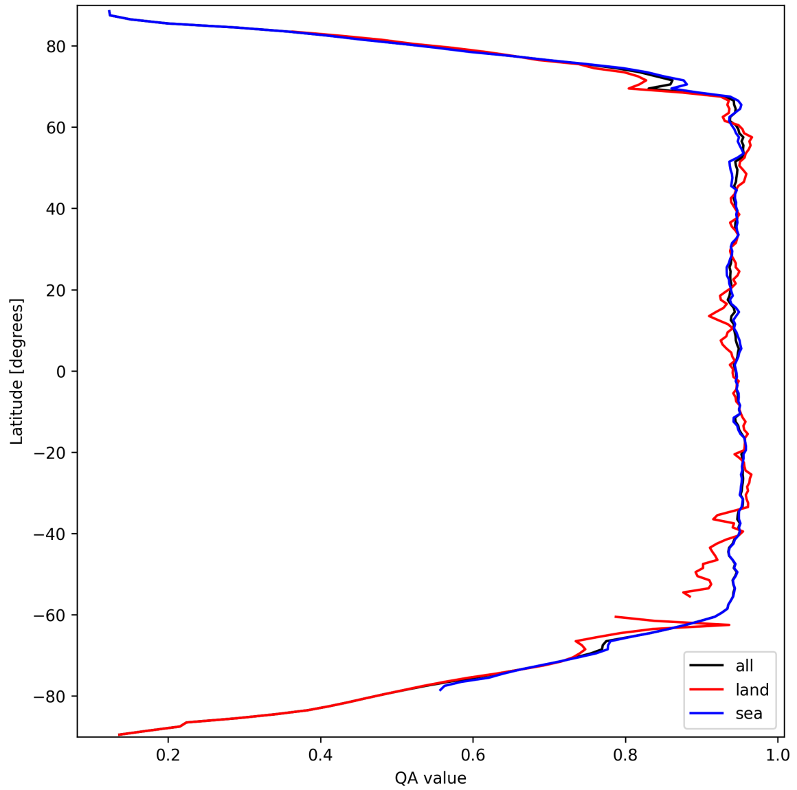
Figure 13: Zonal average of “QA value” for 2025-09-23 to 2025-09-25.
