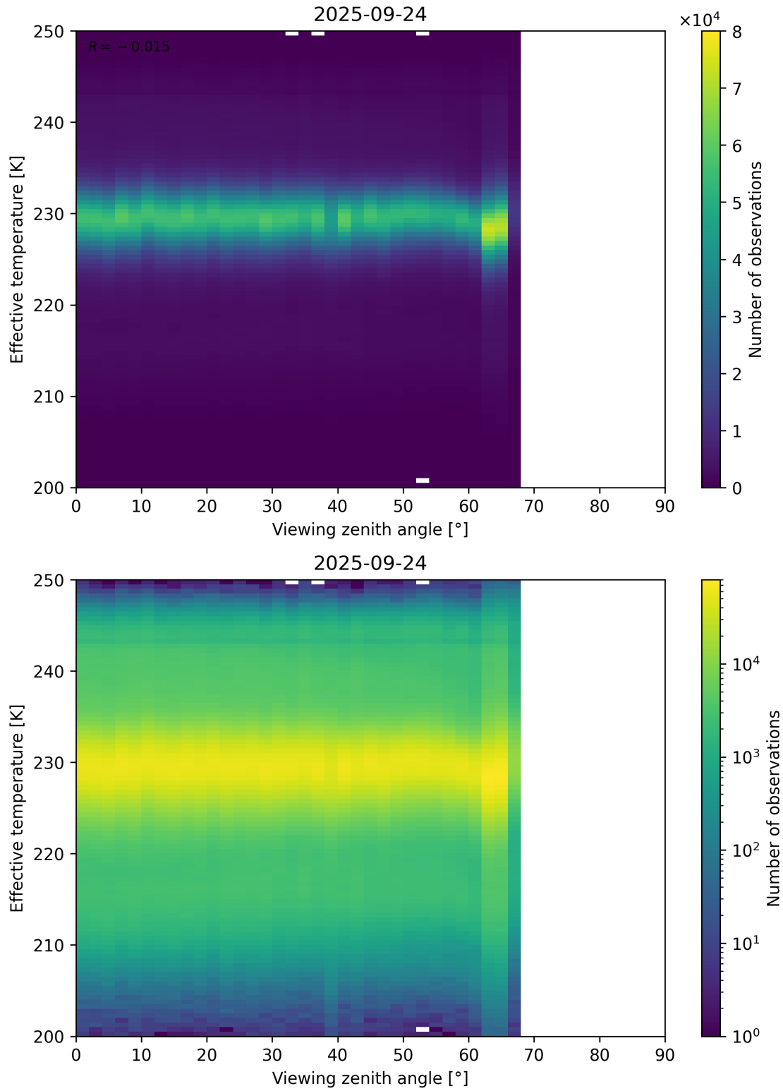
Figure 50: Scatter density plot of “Viewing zenith angle” against “Effective temperature” for 2025-09-23 to 2025-09-25.
