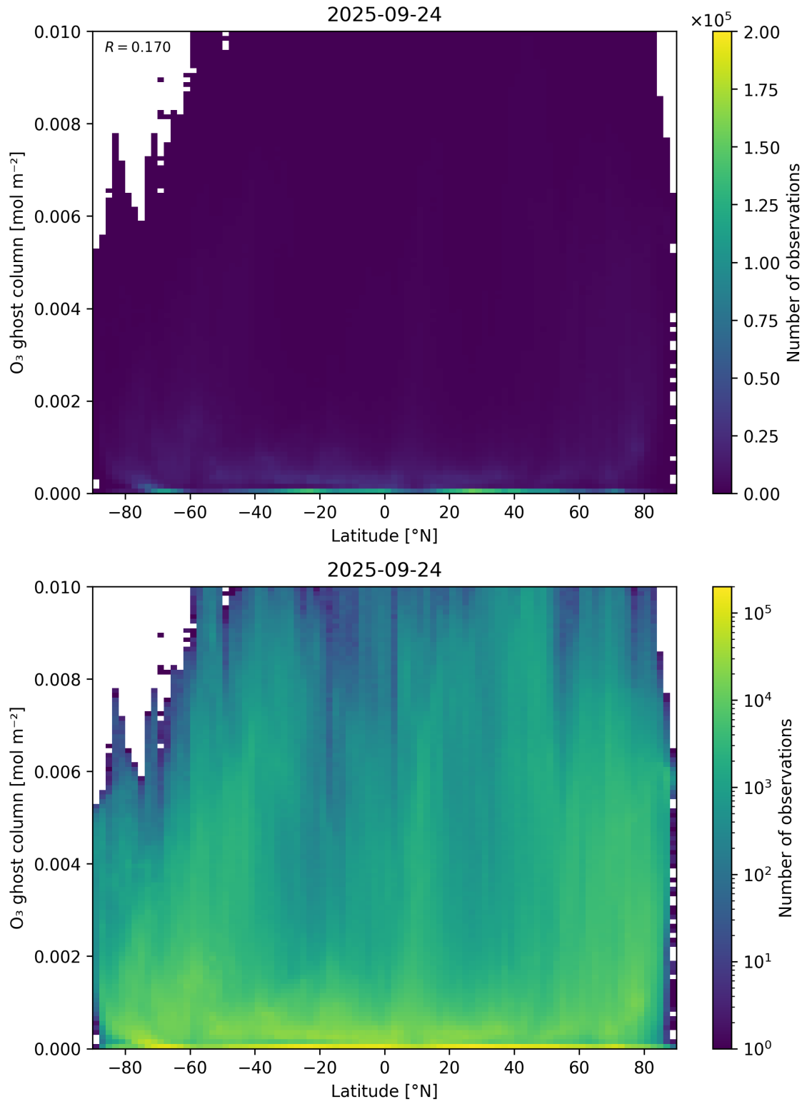
Figure 35: Scatter density plot of “Latitude” against “O 3 ghost column” for 2025-09-23 to 2025-09-25.
