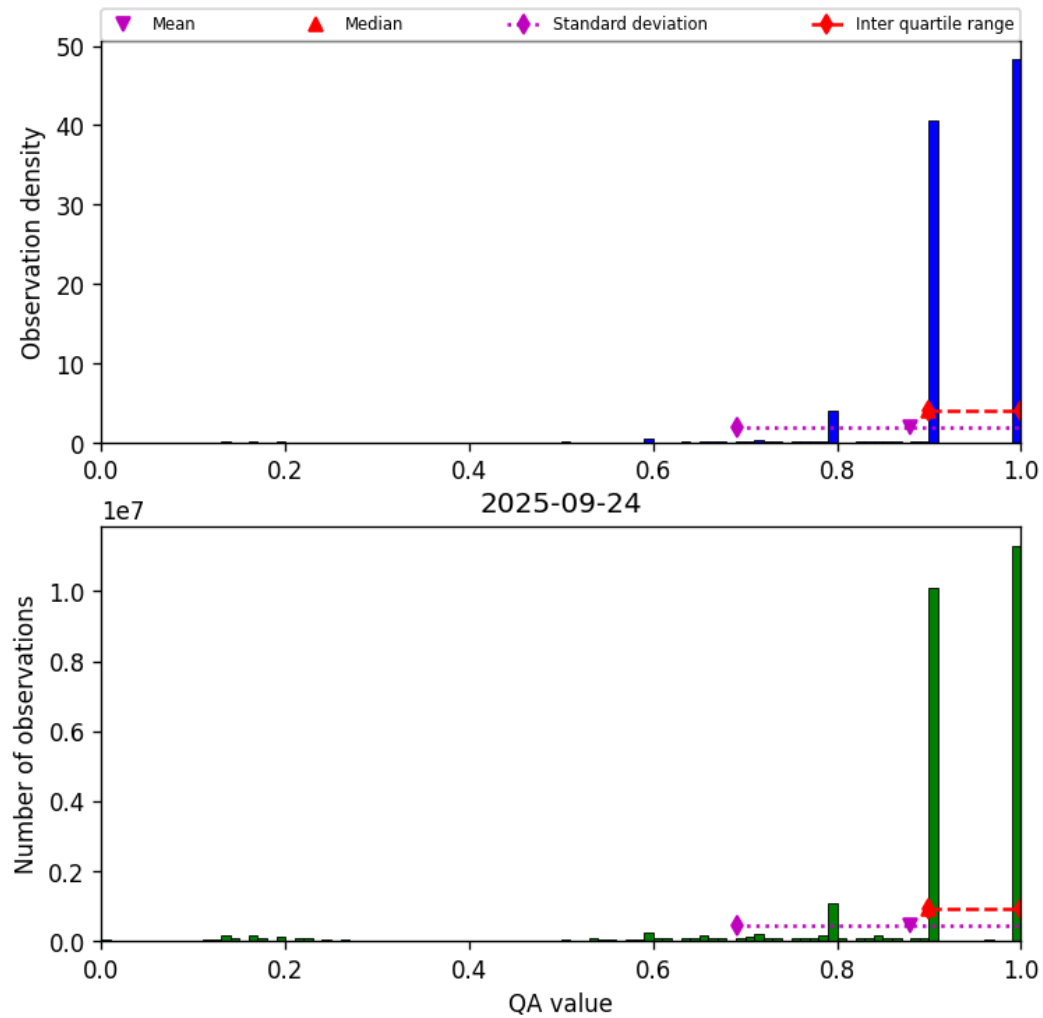
Figure 20: Histogram of “QA value” for 2025-09-23 to 2025-09-25
