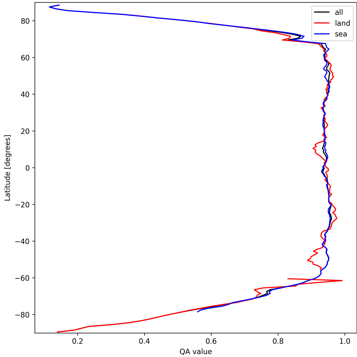
Figure 13: Zonal average of “QA value” for 2025-09-25 to 2025-09-26.
