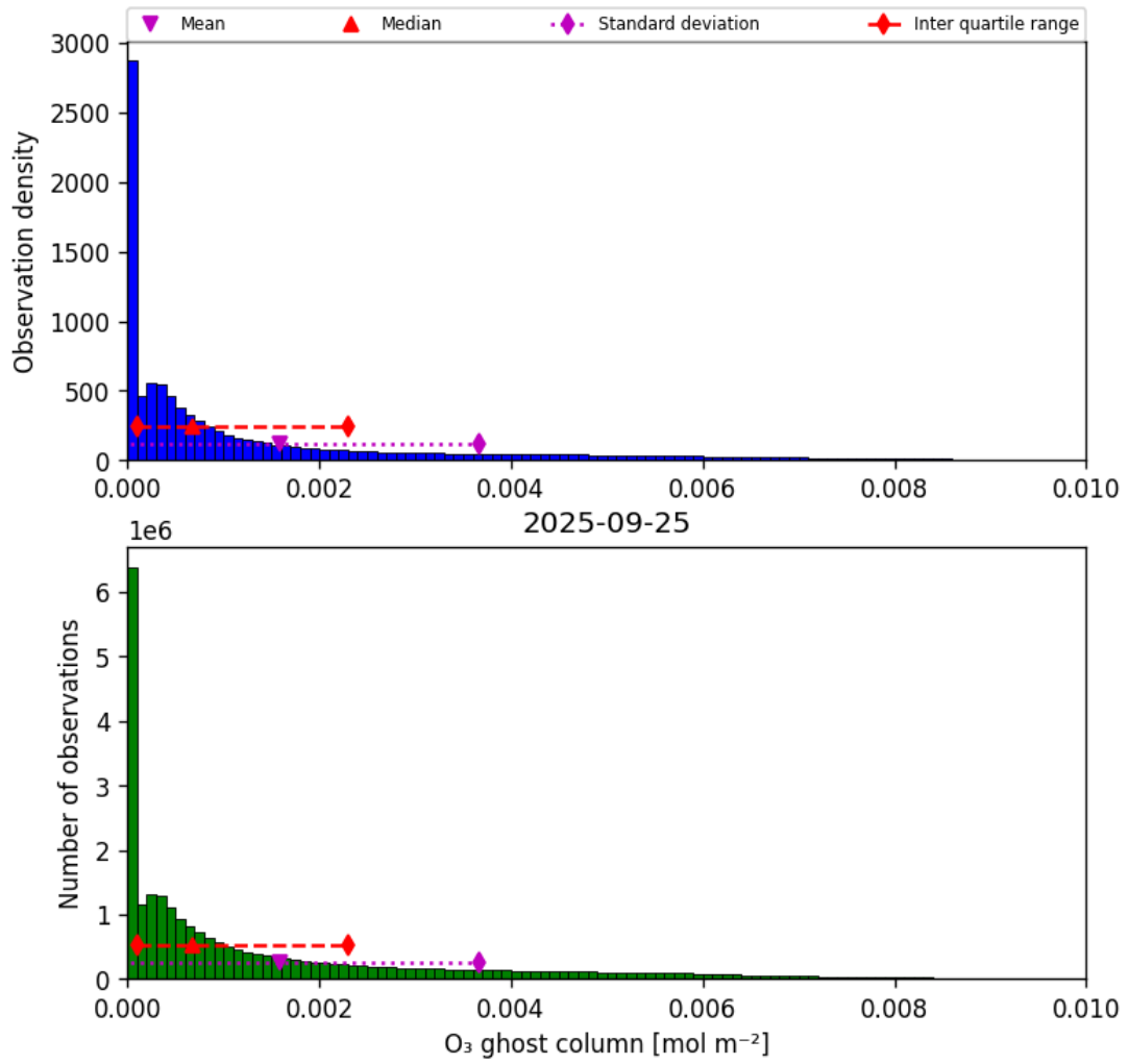
Figure 25: Histogram of “O 3 ghost column” for 2025-09-25 to 2025-09-26
