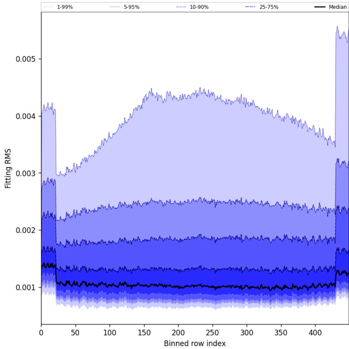
Figure 30: Along track statistics of “Fitting RMS” for 2025-09-25 to 2025-09-26
