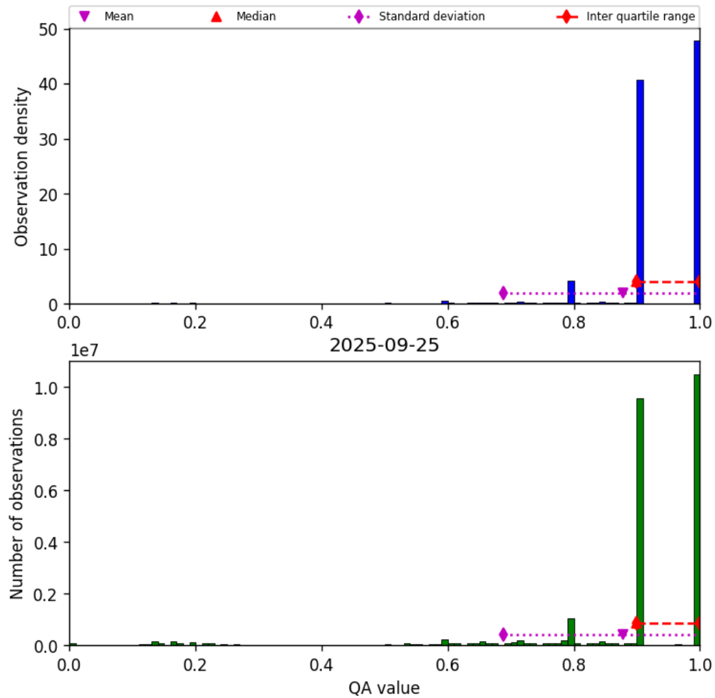
Figure 20: Histogram of “QA value” for 2025-09-25 to 2025-09-26
