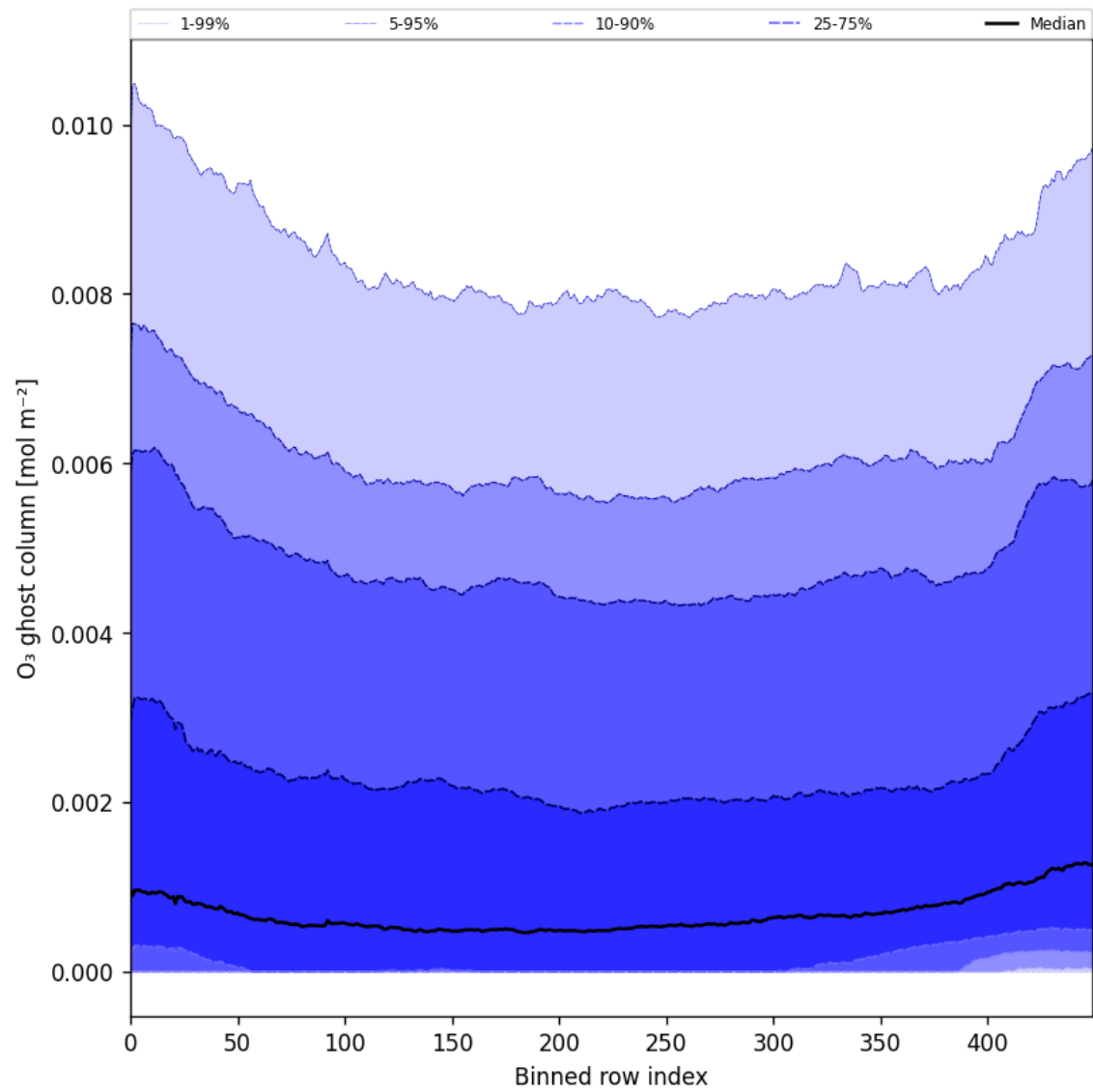
Figure 32: Along track statistics of “O 3 ghost column” for 2025-09-25 to 2025-09-26
