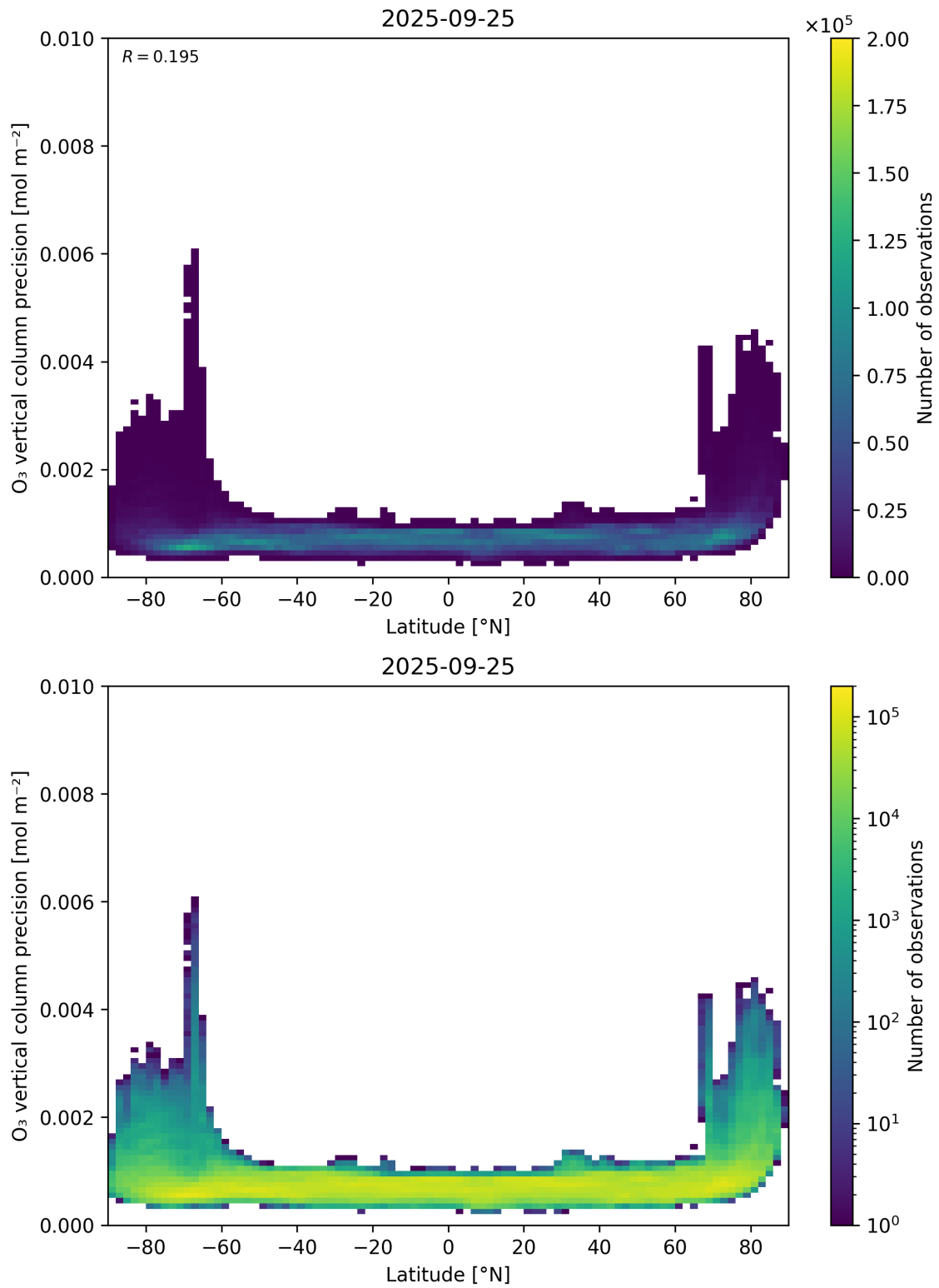
Figure 37: Scatter density plot of “Latitude” against “O 3 vertical column precision” for 2025-09-25 to 2025-09-26.
