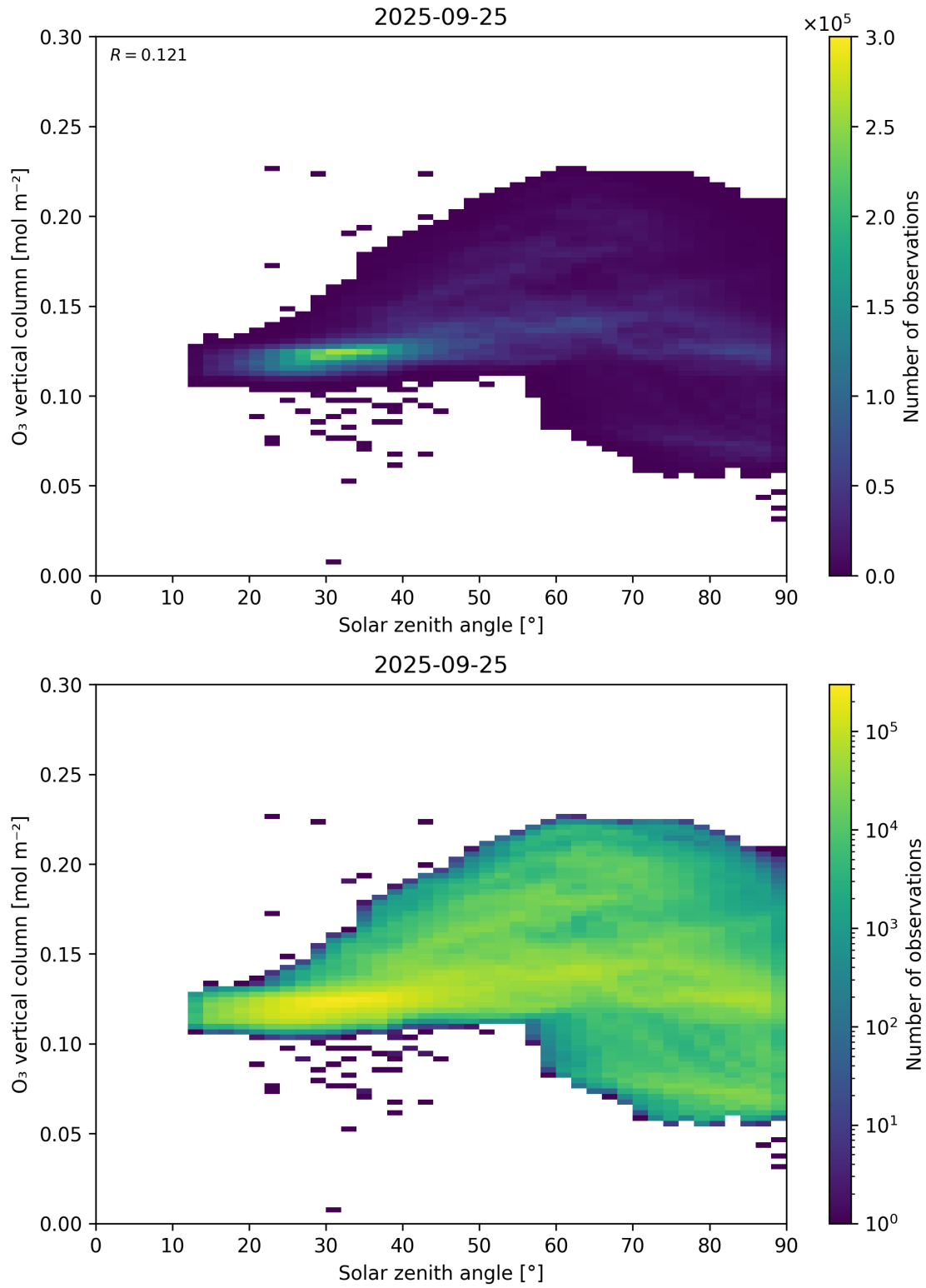
Figure 47: Scatter density plot of “Solar zenith angle” against “O 3 vertical column” for 2025-09-25 to 2025-09-26.
