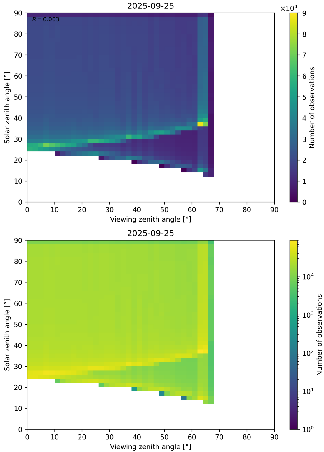
Figure 54: Scatter density plot of “Viewing zenith angle” against “Solar zenith angle” for 2025-09-25 to 2025-09-26.
