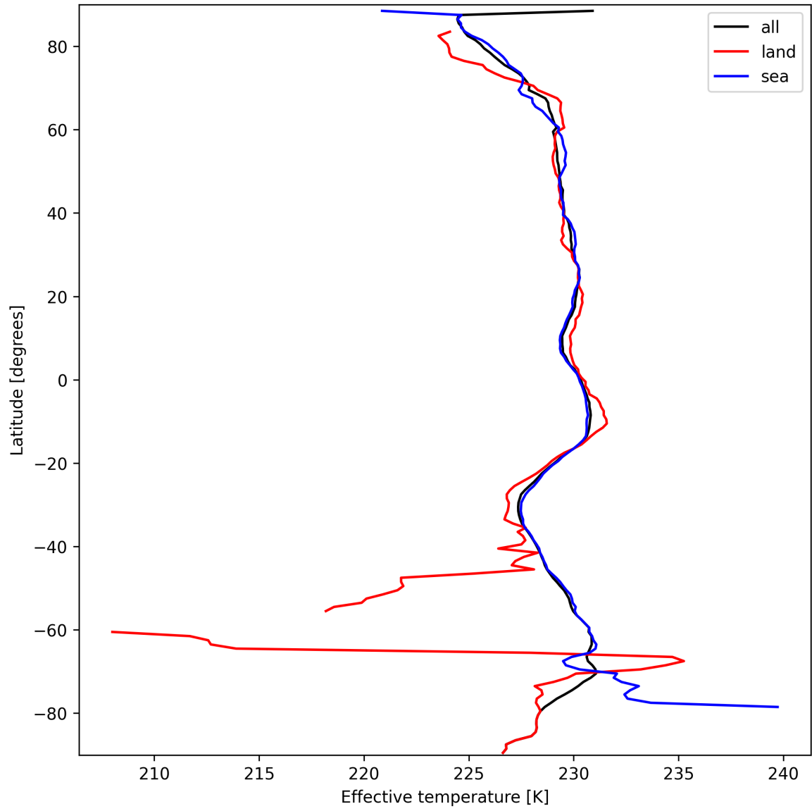
Figure 17: Zonal average of “Effective temperature” for 2025-09-25 to 2025-09-26.
