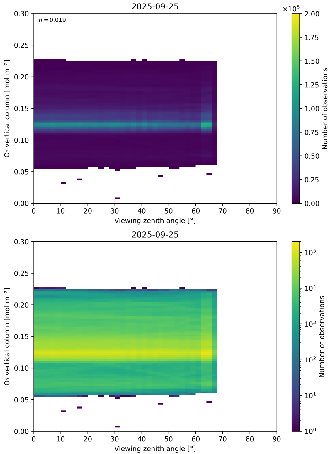
Figure 52: Scatter density plot of “Viewing zenith angle” against “O 3 vertical column” for 2025-09-25 to 2025-09-26.
