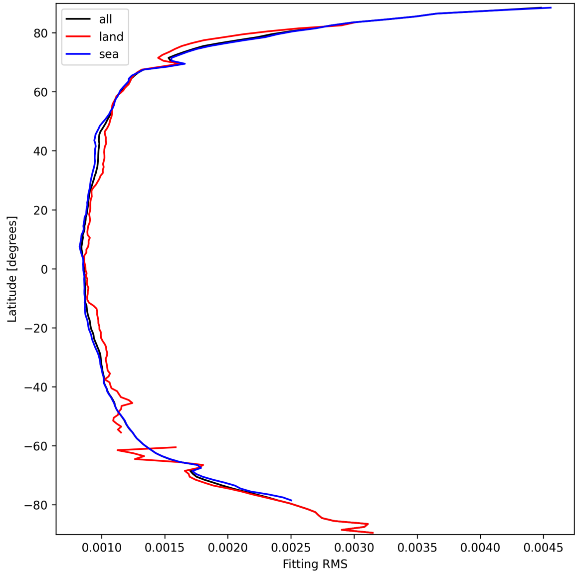
Figure 16: Zonal average of “Fitting RMS” for 2025-09-25 to 2025-09-26.
