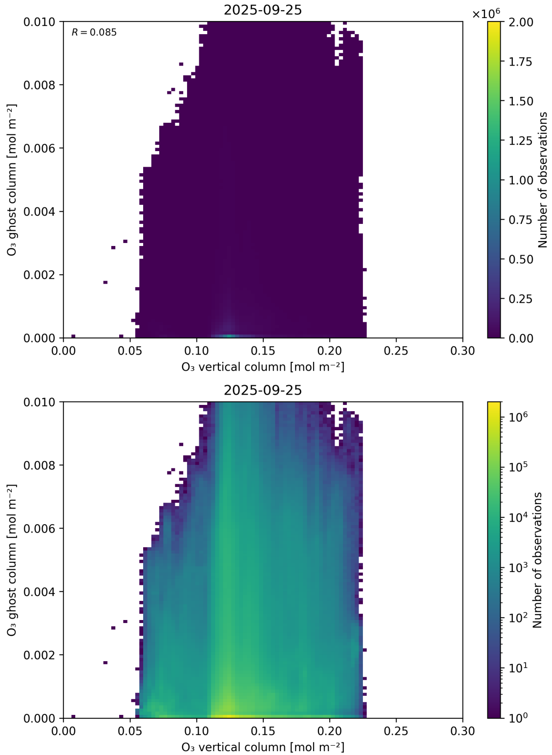
Figure 40: Scatter density plot of “O 3 vertical column” against “O 3 ghost column” for 2025-09-25 to 2025-09-26.
