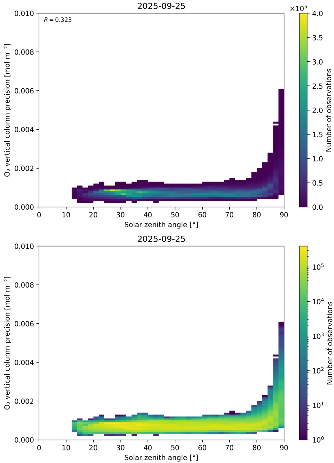
Figure 48: Scatter density plot of “Solar zenith angle” against “O 3 vertical column precision” for 2025-09-25 to 2025-09-26.
