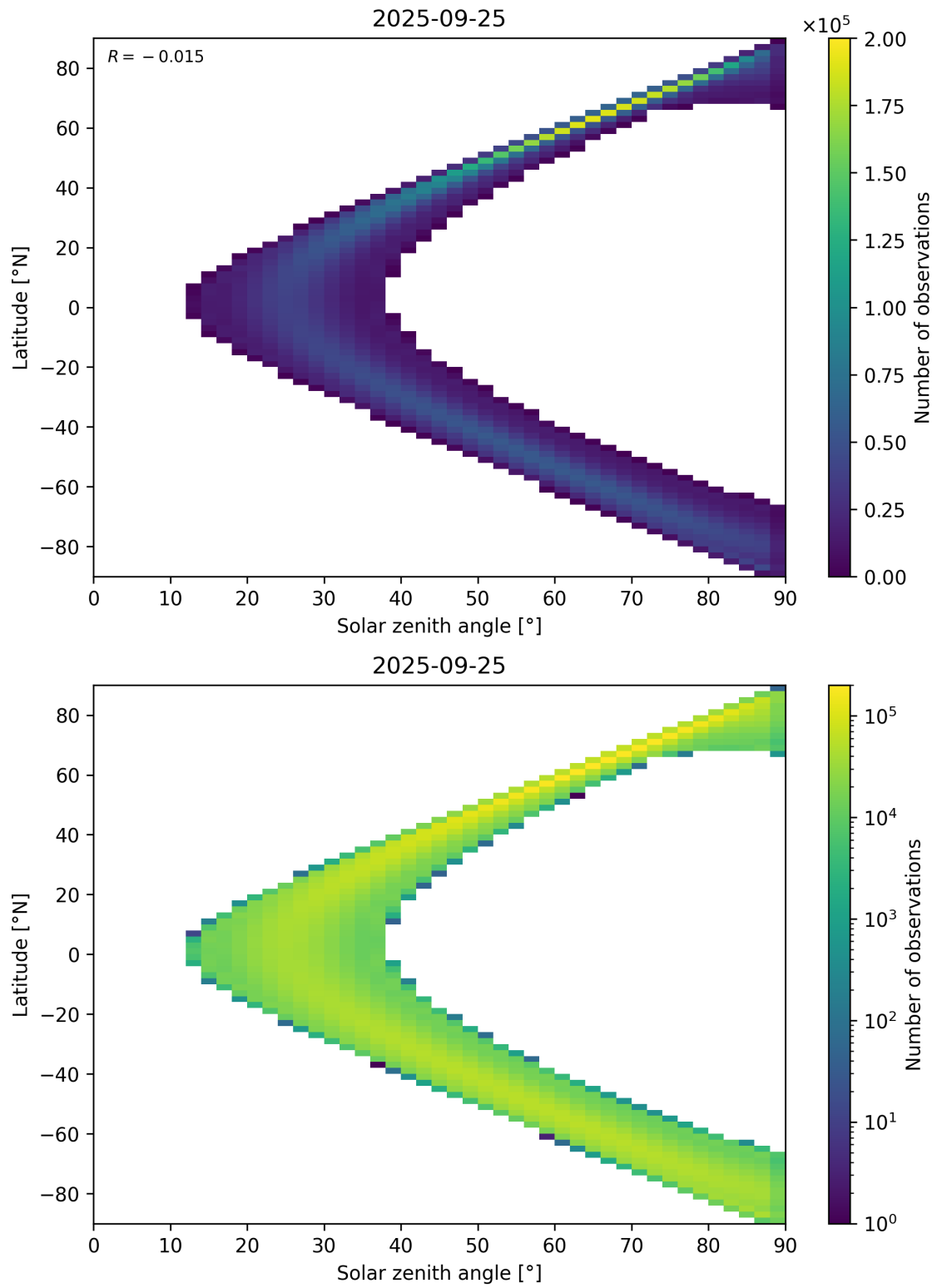
Figure 44: Scatter density plot of “Solar zenith angle” against “Latitude” for 2025-09-25 to 2025-09-26.
