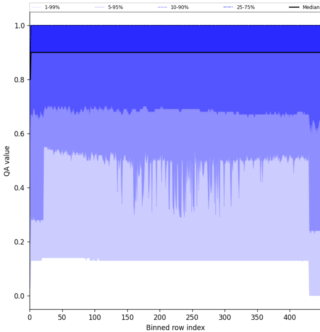
Figure 27: Along track statistics of “QA value” for 2025-09-25 to 2025-09-26
