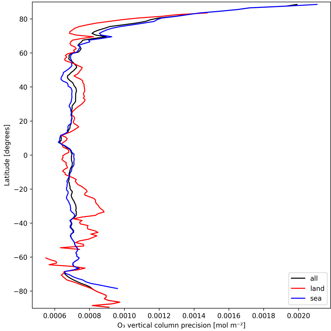
Figure 15: Zonal average of “O 3 vertical column precision” for 2025-09-25 to 2025-09-26.
