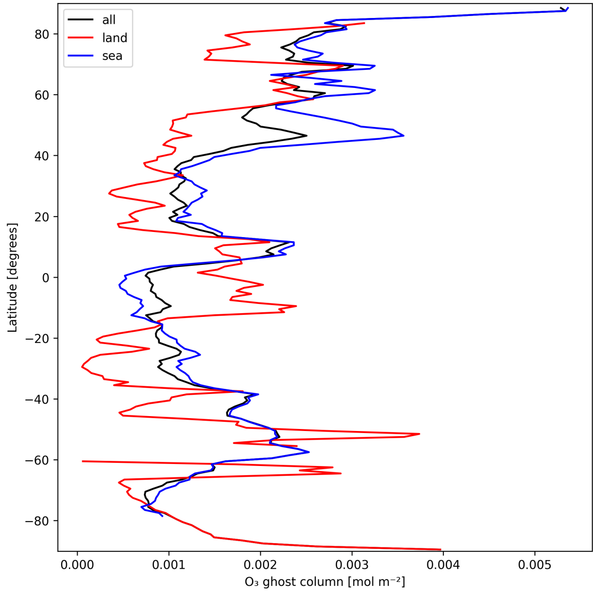
Figure 18: Zonal average of “O 3 ghost column” for 2025-09-25 to 2025-09-26.
