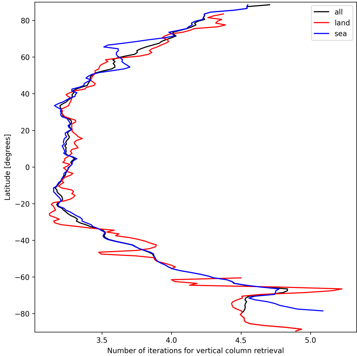
Figure 19: Zonal average of “Number of iterations for vertical column retrieval” for 2025-09-25 to 2025-09-26.
