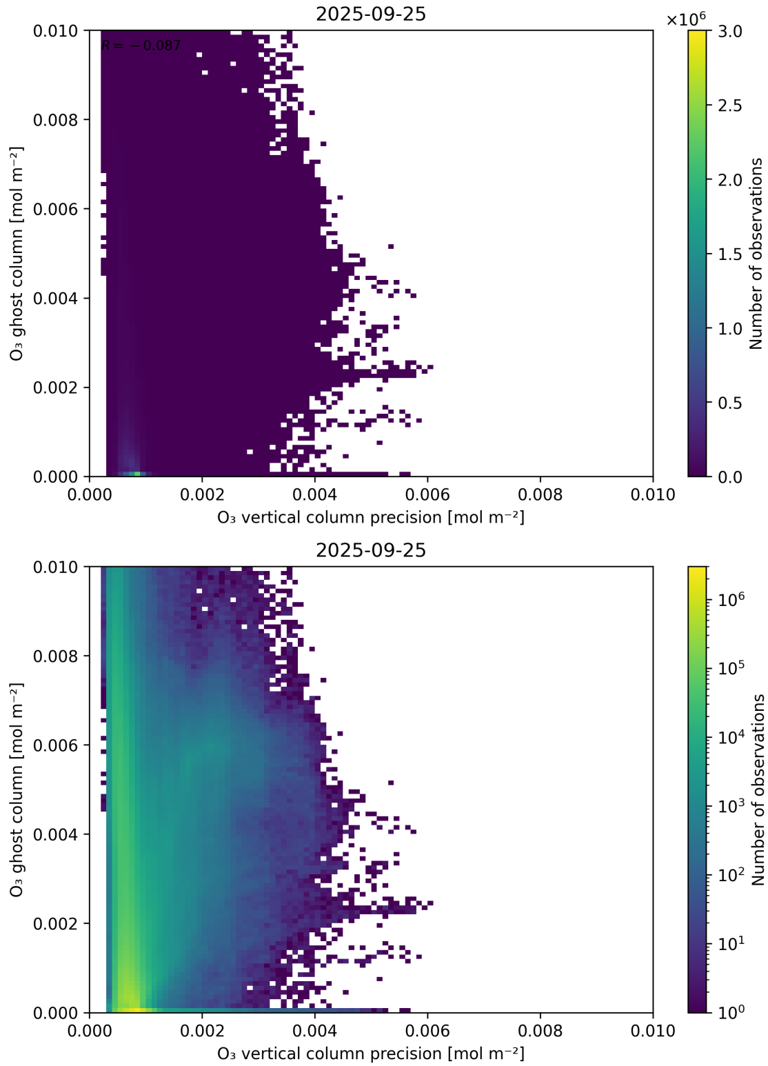
Figure 43: Scatter density plot of “O 3 vertical column precision” against “O 3 ghost column” for 2025-09-25 to 2025-09-26.
