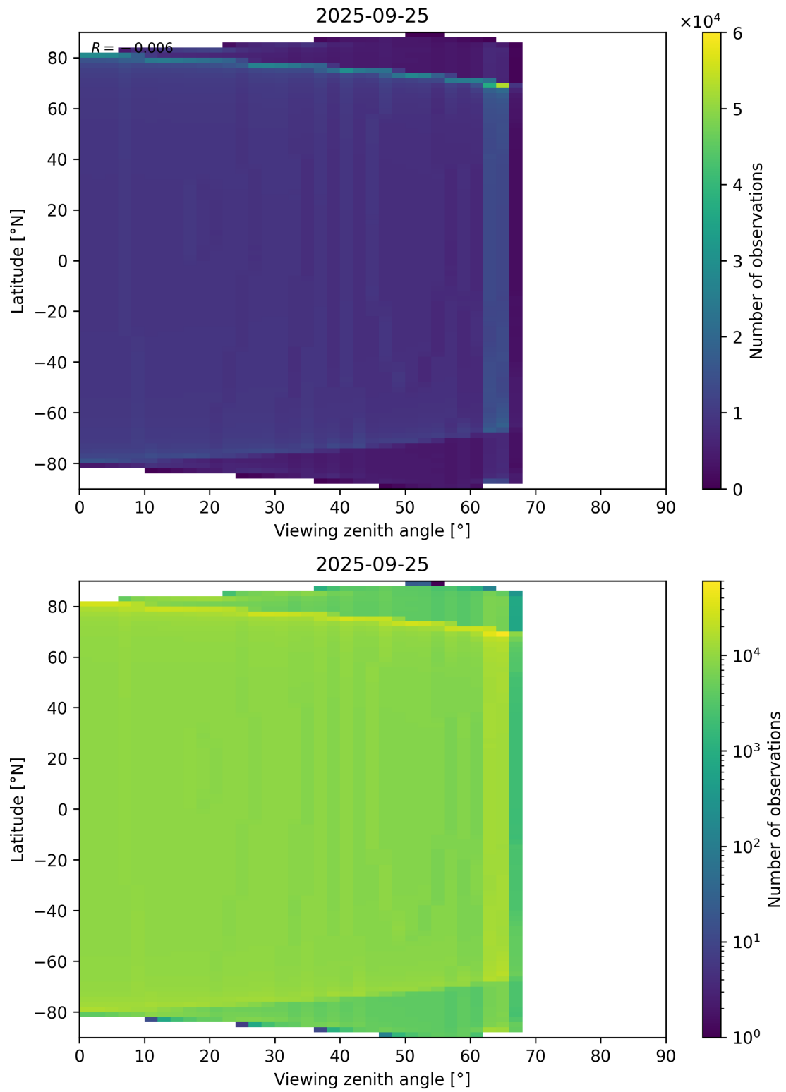
Figure 49: Scatter density plot of “Viewing zenith angle” against “Latitude” for 2025-09-25 to 2025-09-26.
