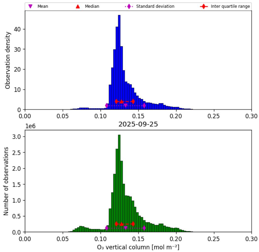
Figure 21: Histogram of “O 3 vertical column” for 2025-09-25 to 2025-09-26
