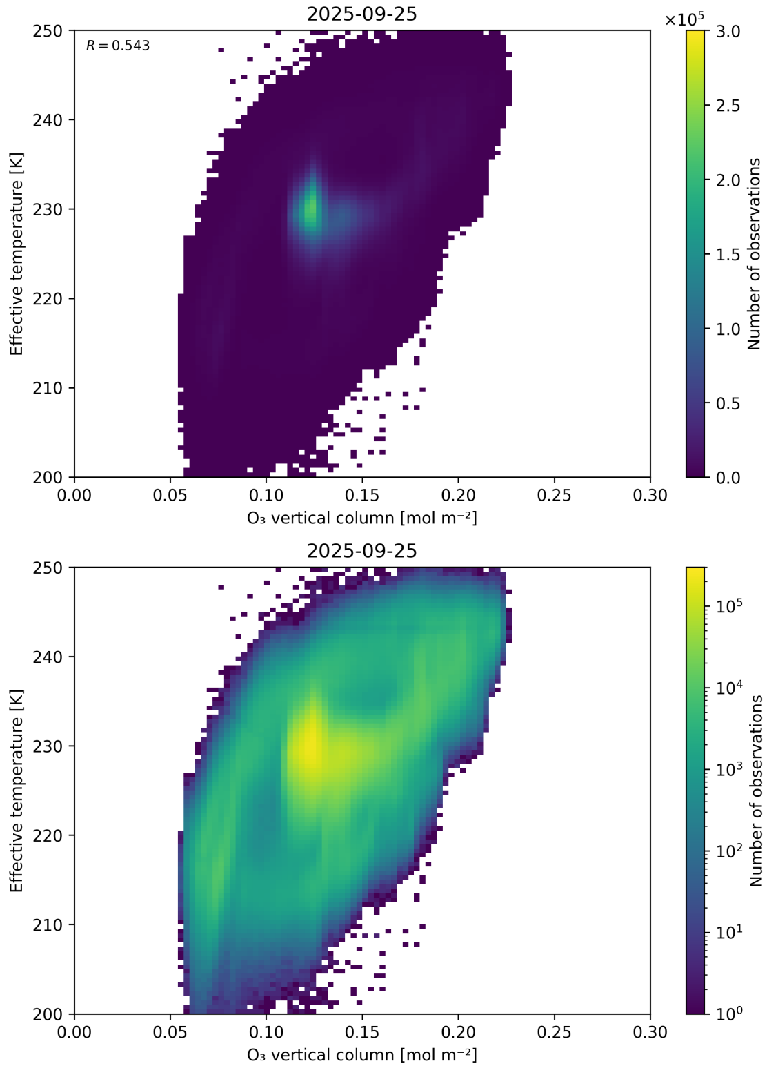
Figure 39: Scatter density plot of “O 3 vertical column” against “Effective temperature” for 2025-09-25 to 2025-09-26.
