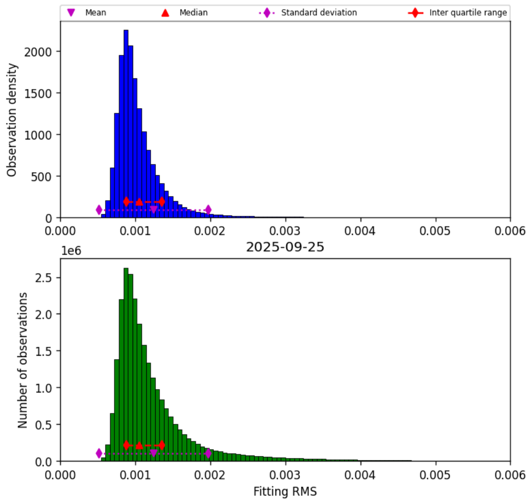
Figure 23: Histogram of “Fitting RMS” for 2025-09-25 to 2025-09-26
