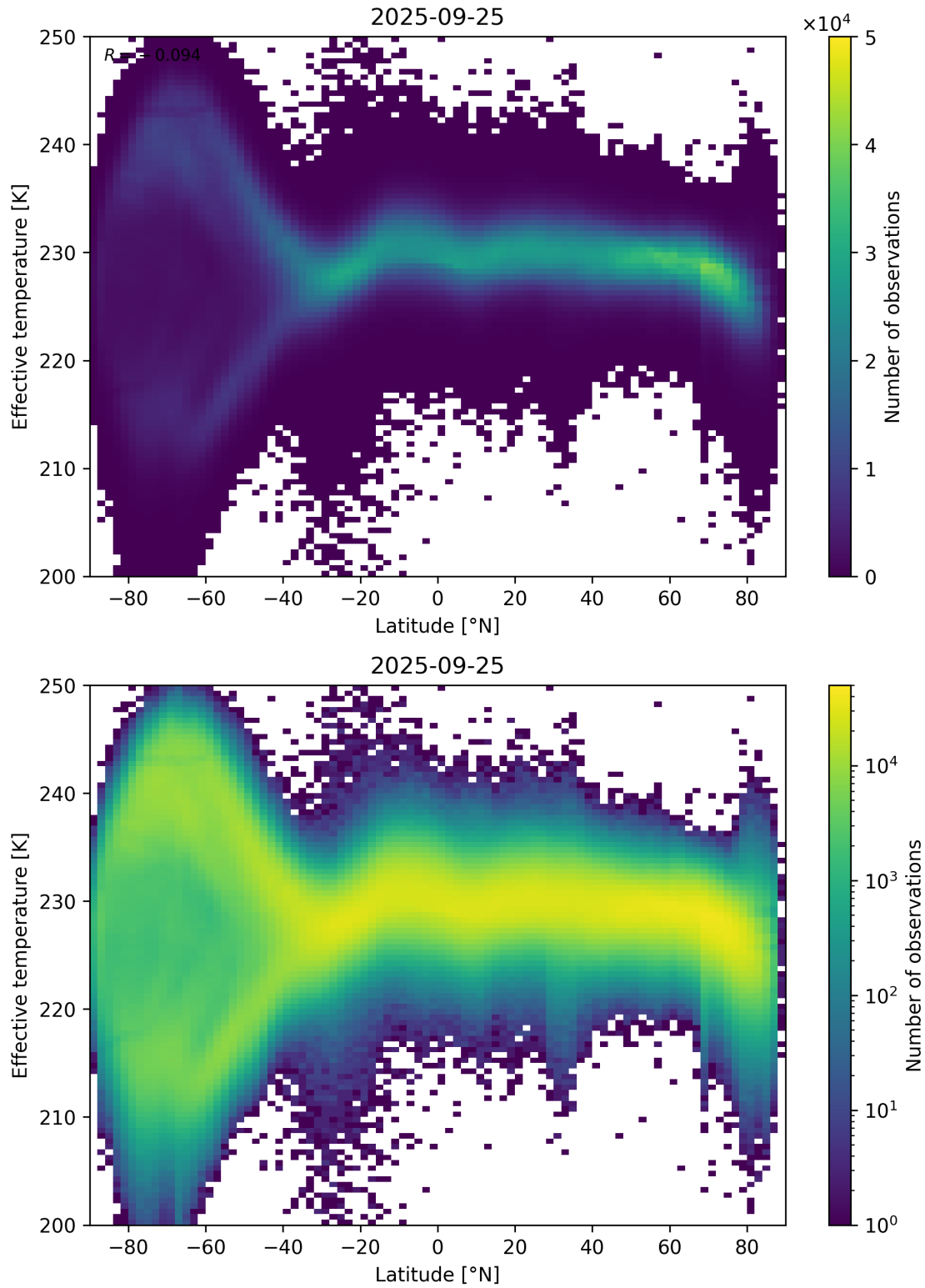
Figure 34: Scatter density plot of “Latitude” against “Effective temperature” for 2025-09-25 to 2025-09-26.
