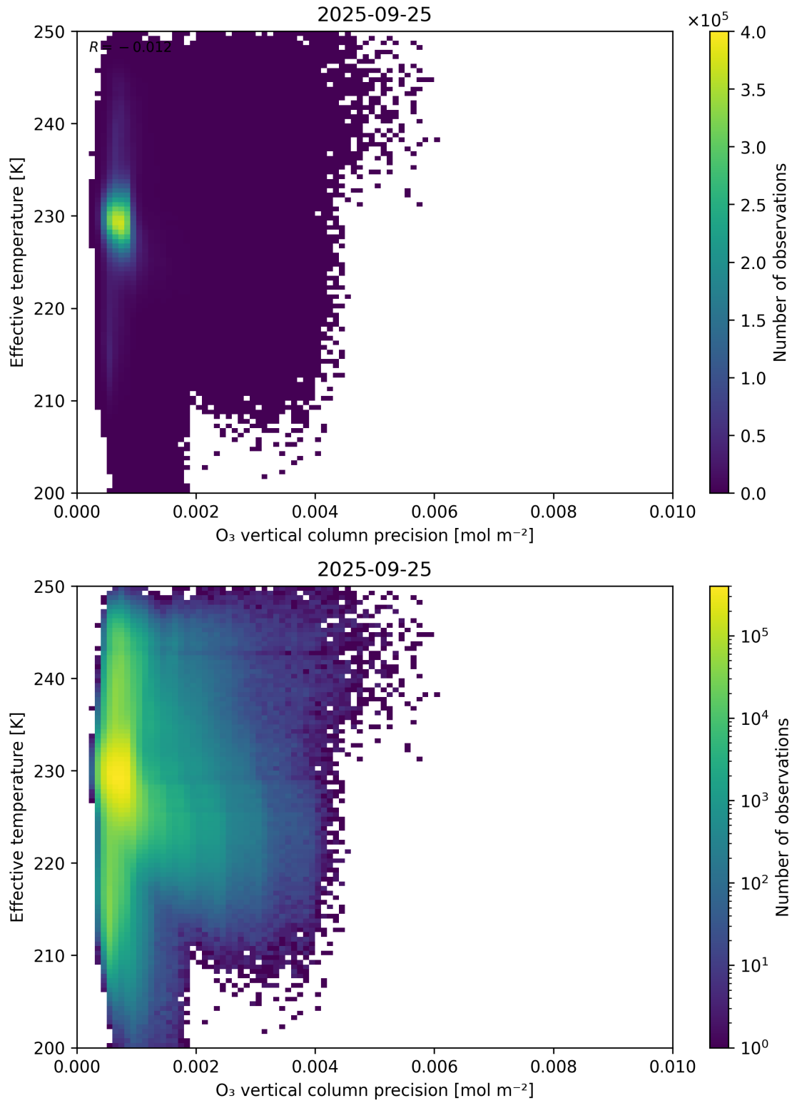
Figure 42: Scatter density plot of “O 3 vertical column precision” against “Effective temperature” for 2025-09-25 to 2025-09-26.
