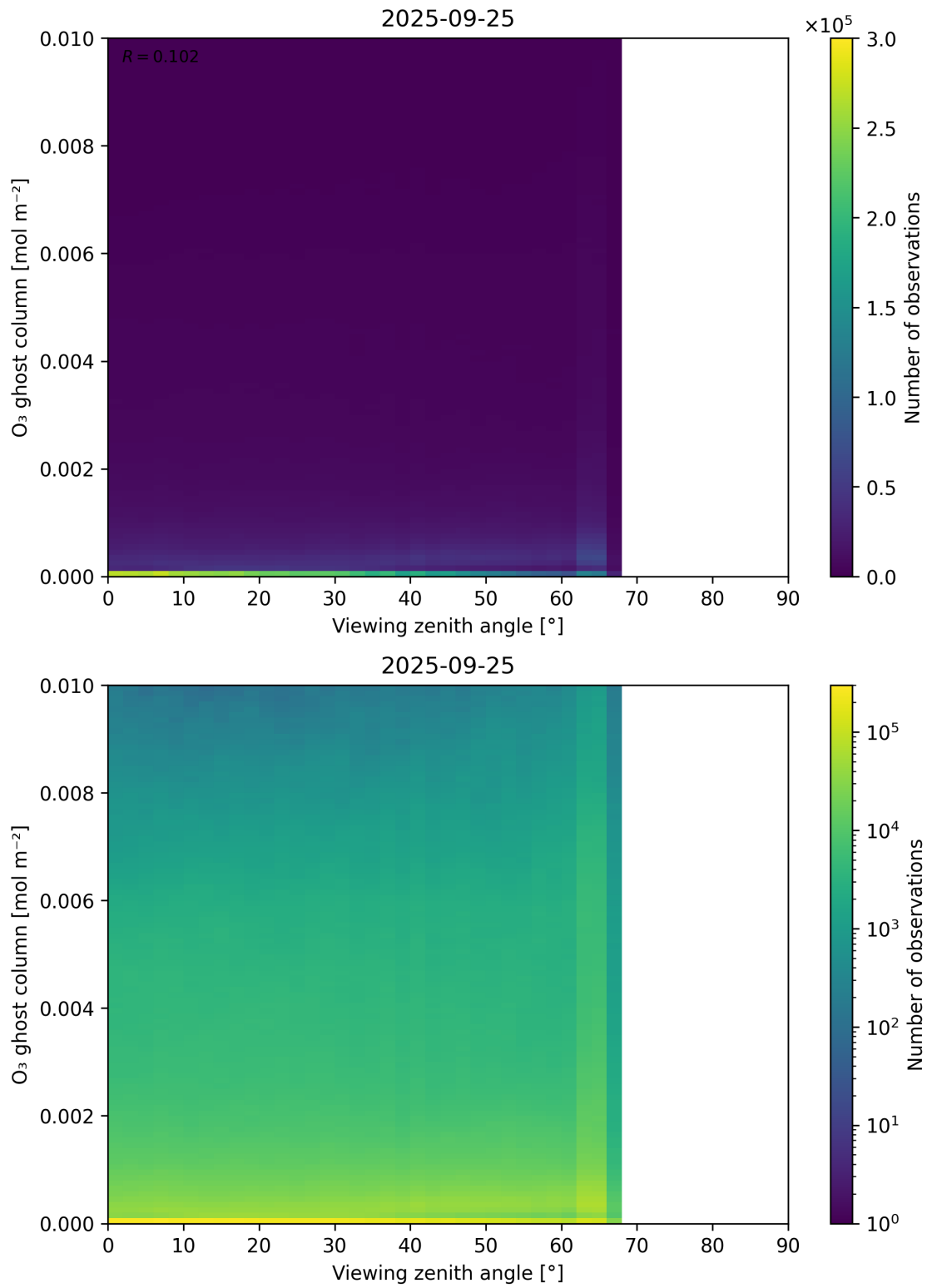
Figure 51: Scatter density plot of “Viewing zenith angle” against “O 3 ghost column” for 2025-09-25 to 2025-09-26.
