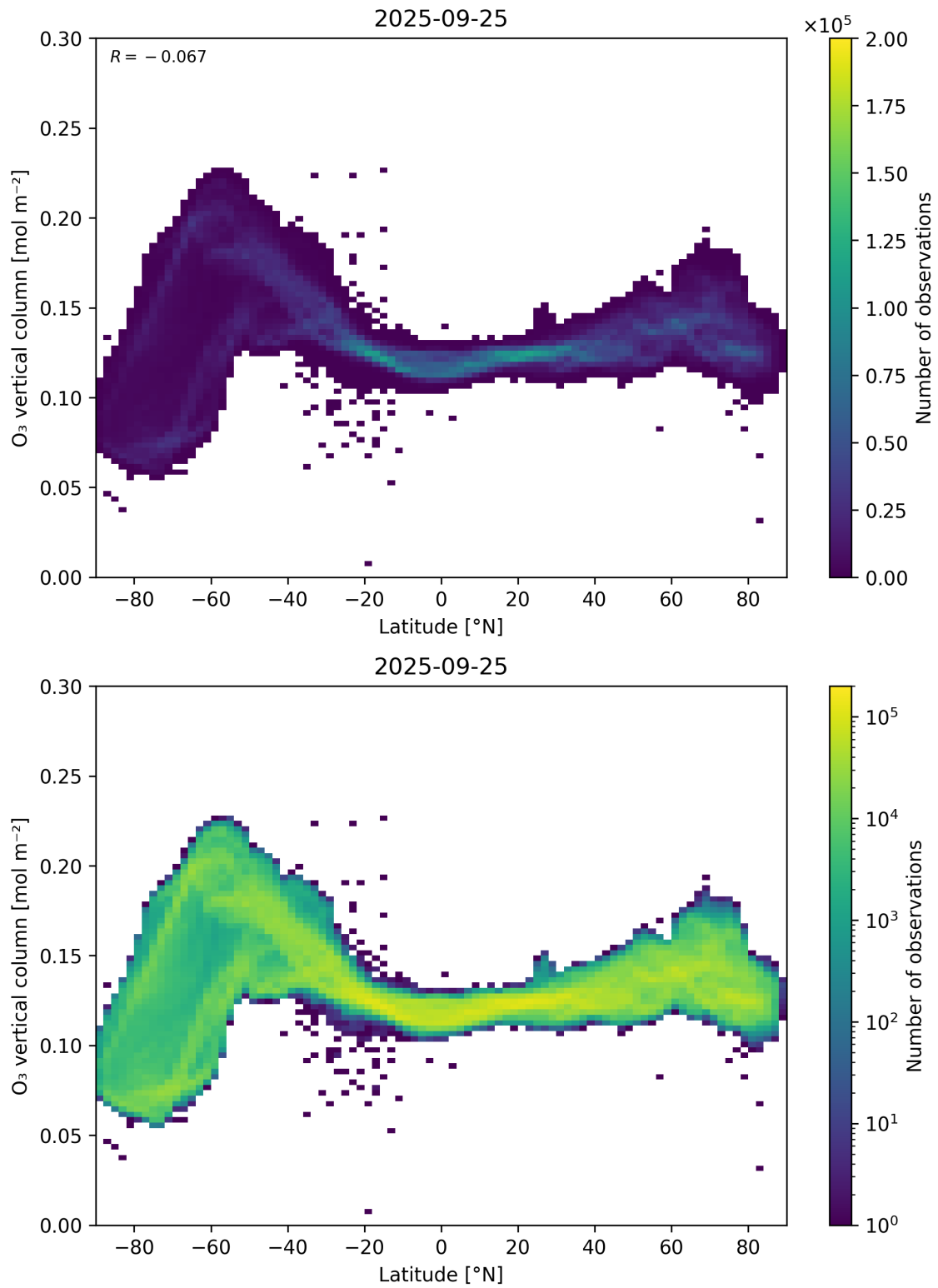
Figure 36: Scatter density plot of “Latitude” against “O 3 vertical column” for 2025-09-25 to 2025-09-26.
