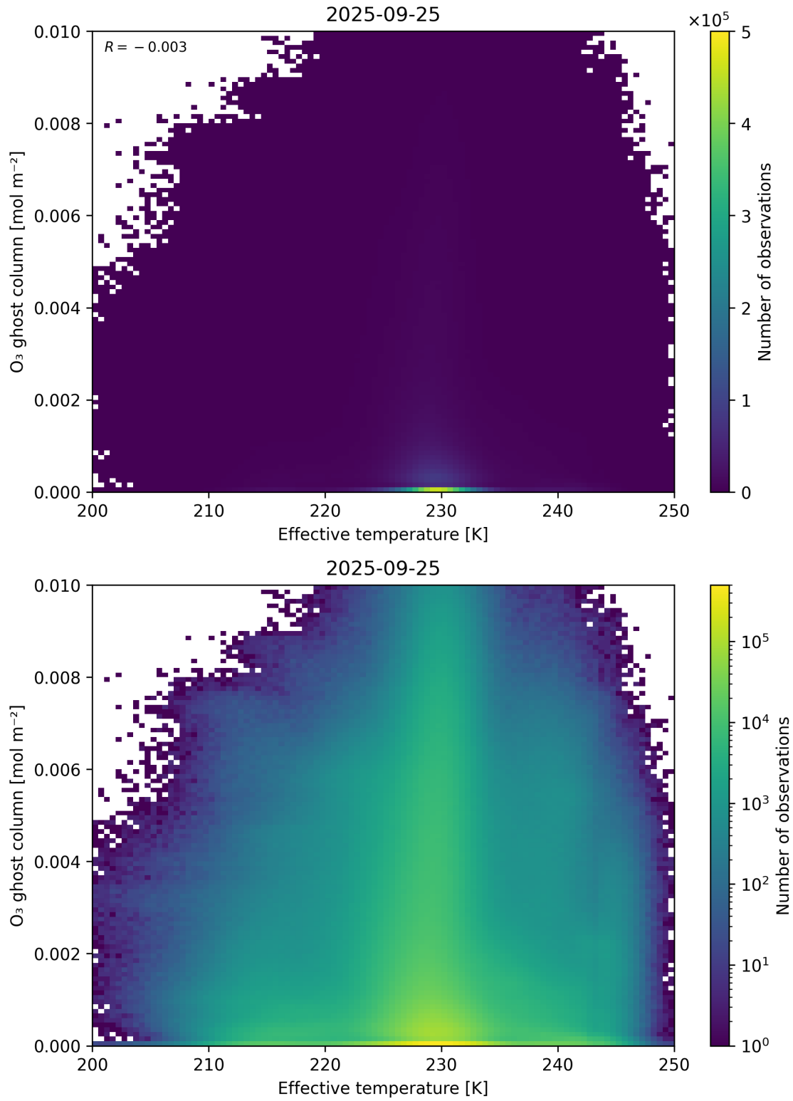
Figure 38: Scatter density plot of “Effective temperature” against “O 3 ghost column” for 2025-09-25 to 2025-09-26.
