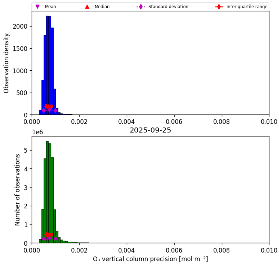
Figure 22: Histogram of “O 3 vertical column precision” for 2025-09-25 to 2025-09-26
