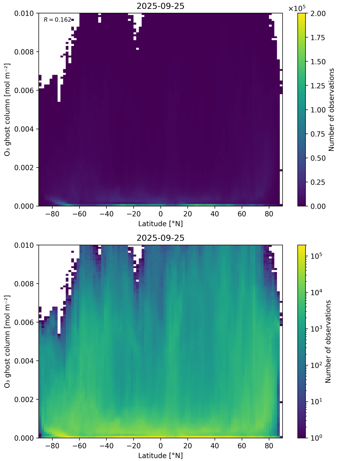
Figure 35: Scatter density plot of “Latitude” against “O 3 ghost column” for 2025-09-25 to 2025-09-26.
