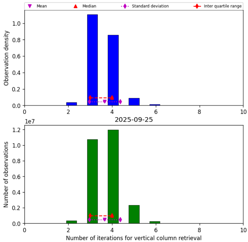
Figure 26: Histogram of “Number of iterations for vertical column retrieval” for 2025-09-25 to 2025-09-26
