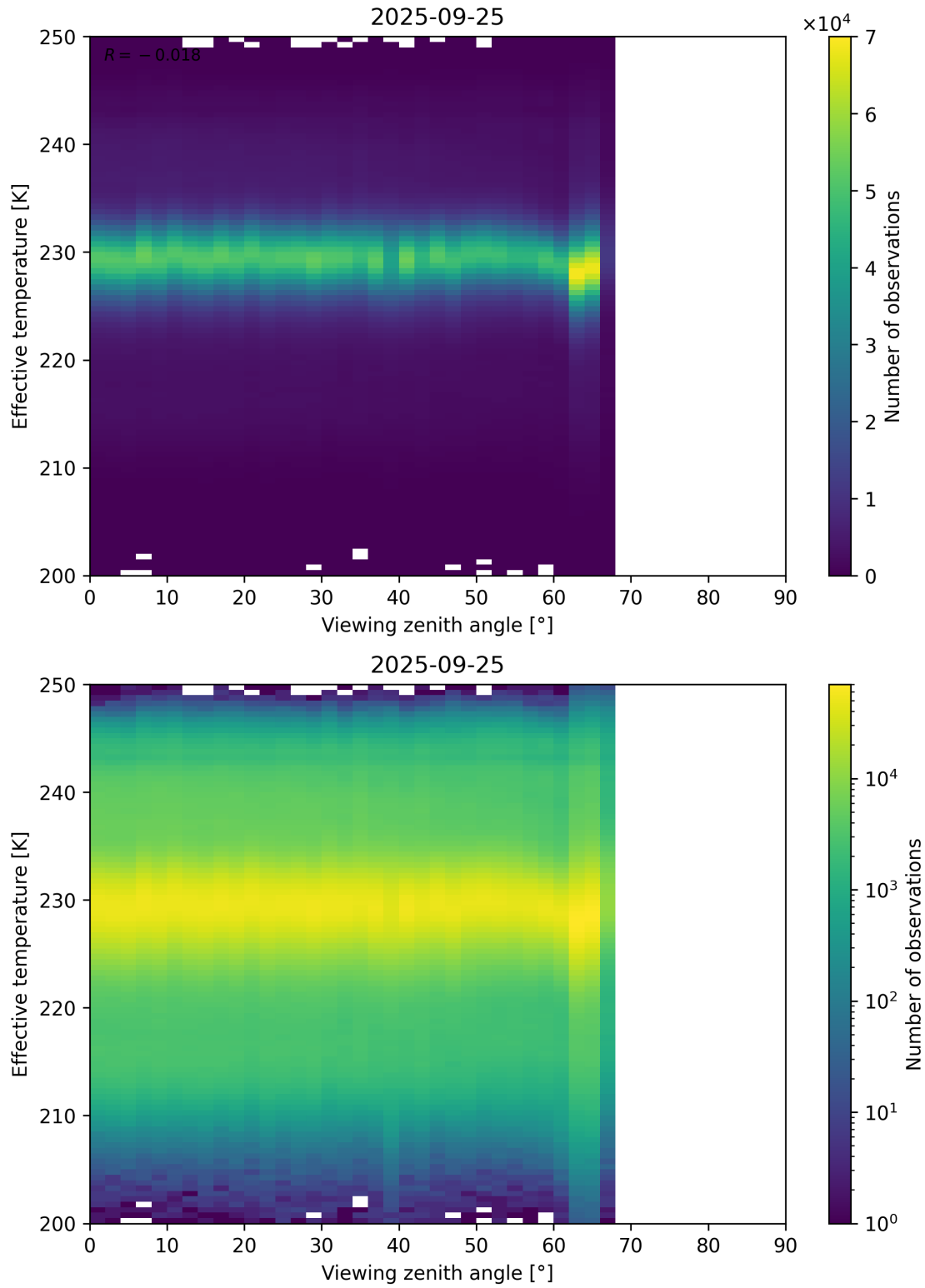
Figure 50: Scatter density plot of “Viewing zenith angle” against “Effective temperature” for 2025-09-25 to 2025-09-26.
