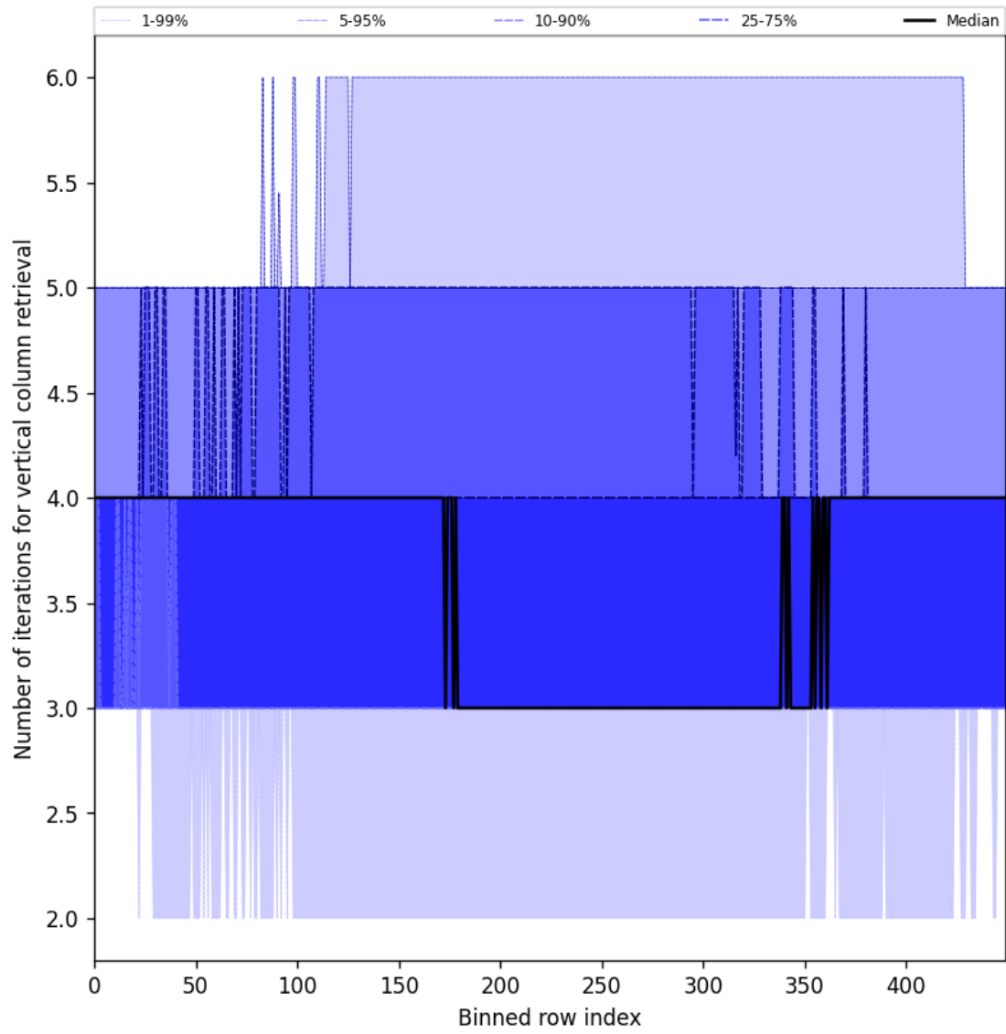
Figure 33: Along track statistics of “Number of iterations for vertical column retrieval” for 2025-09-25 to 2025-09-26
