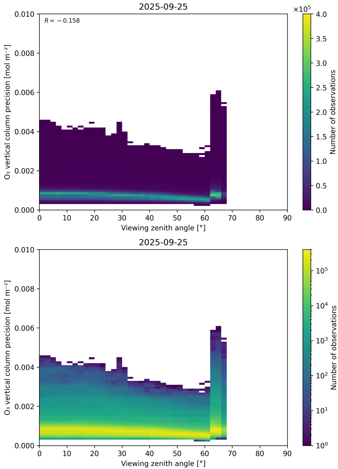
Figure 53: Scatter density plot of “Viewing zenith angle” against “O 3 vertical column precision” for 2025-09-25 to 2025-09-26.
