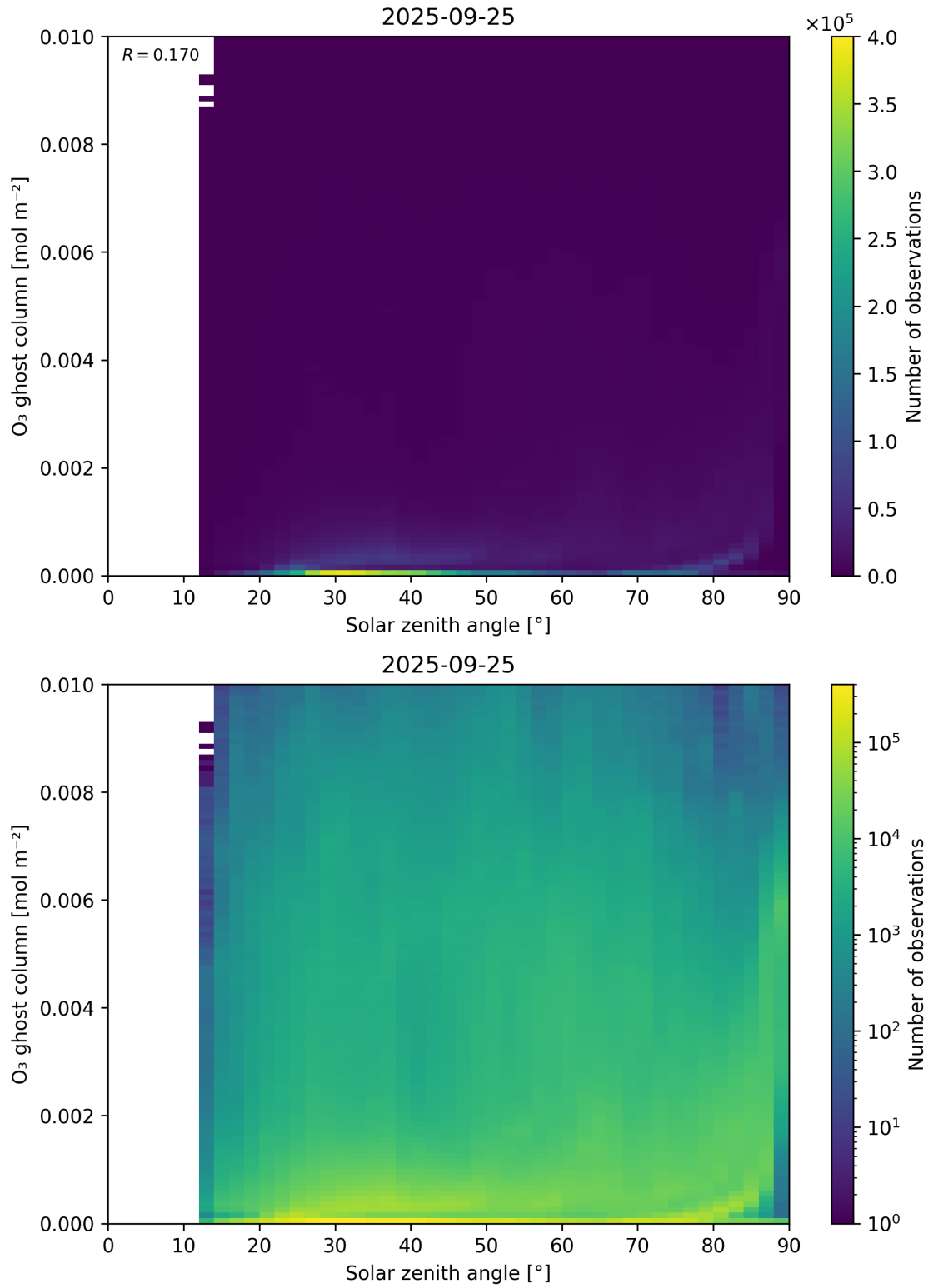
Figure 46: Scatter density plot of “Solar zenith angle” against “O 3 ghost column” for 2025-09-25 to 2025-09-26.
