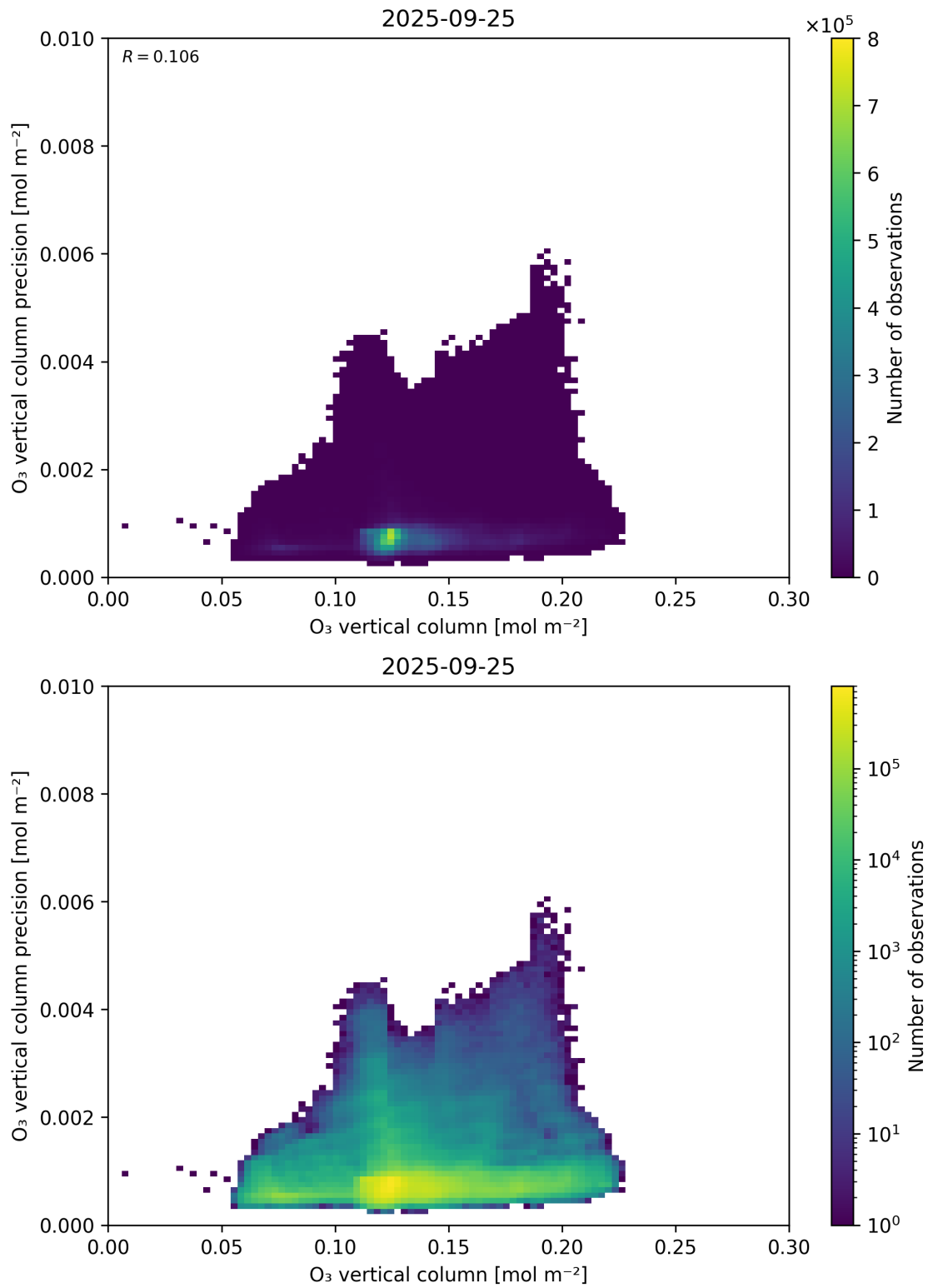
Figure 41: Scatter density plot of “O 3 vertical column” against “O 3 vertical column precision” for 2025-09-25 to 2025-09-26.
