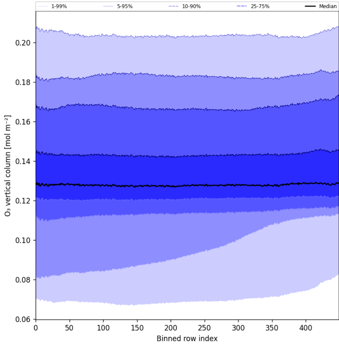
Figure 28: Along track statistics of “O 3 vertical column” for 2025-09-25 to 2025-09-26
