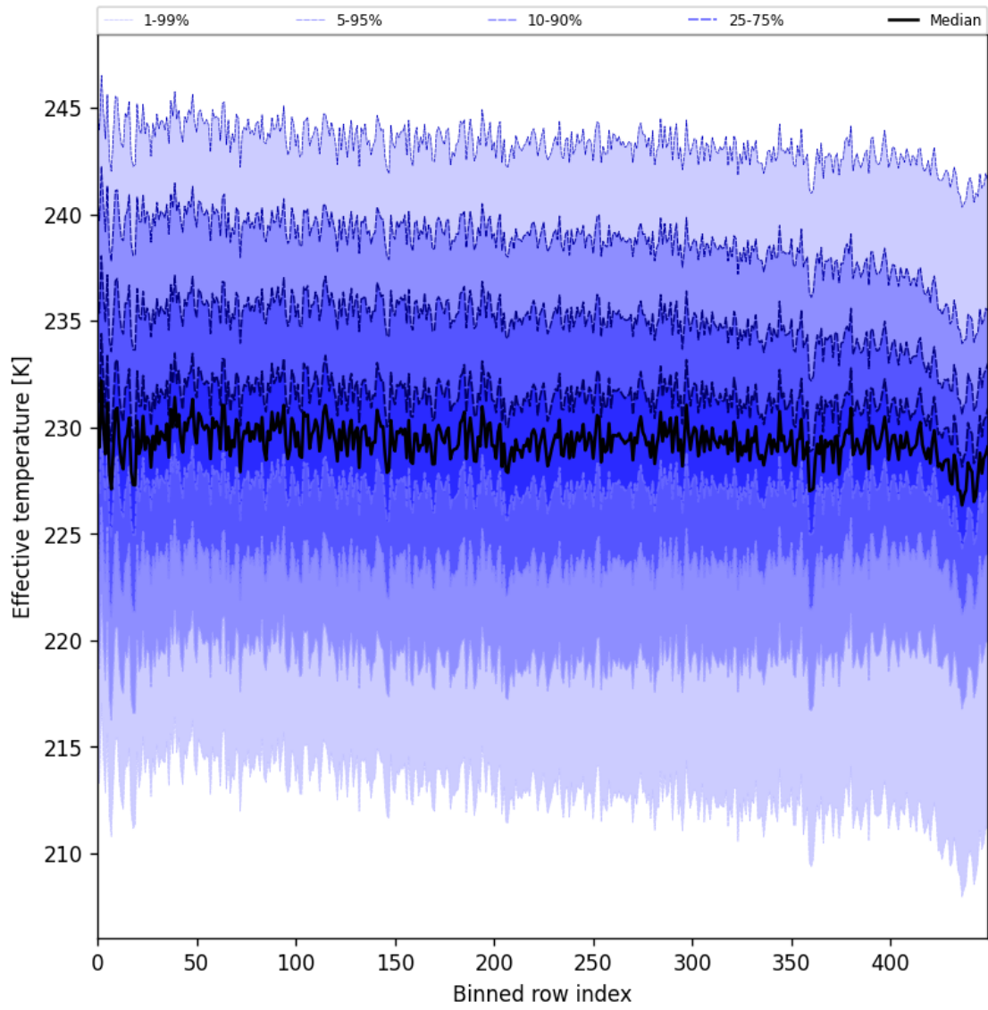
Figure 31: Along track statistics of “Effective temperature” for 2025-09-25 to 2025-09-26
