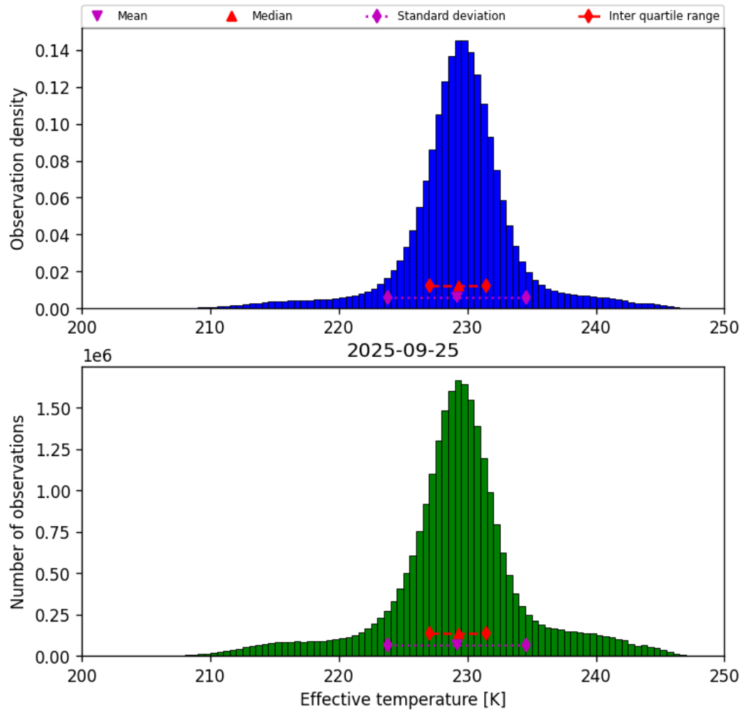
Figure 24: Histogram of “Effective temperature” for 2025-09-25 to 2025-09-26
