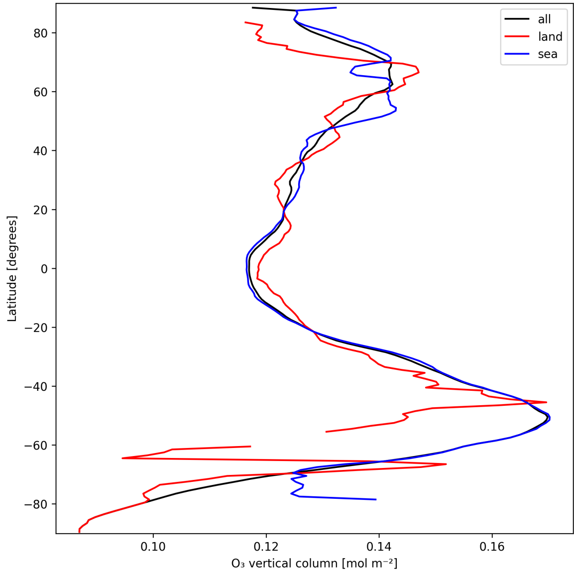
Figure 14: Zonal average of “O 3 vertical column” for 2025-09-25 to 2025-09-26.
