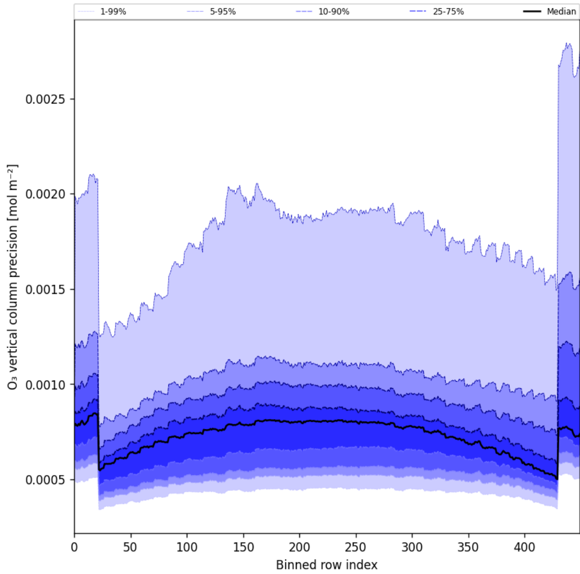
Figure 29: Along track statistics of “O 3 vertical column precision” for 2025-09-25 to 2025-09-26
