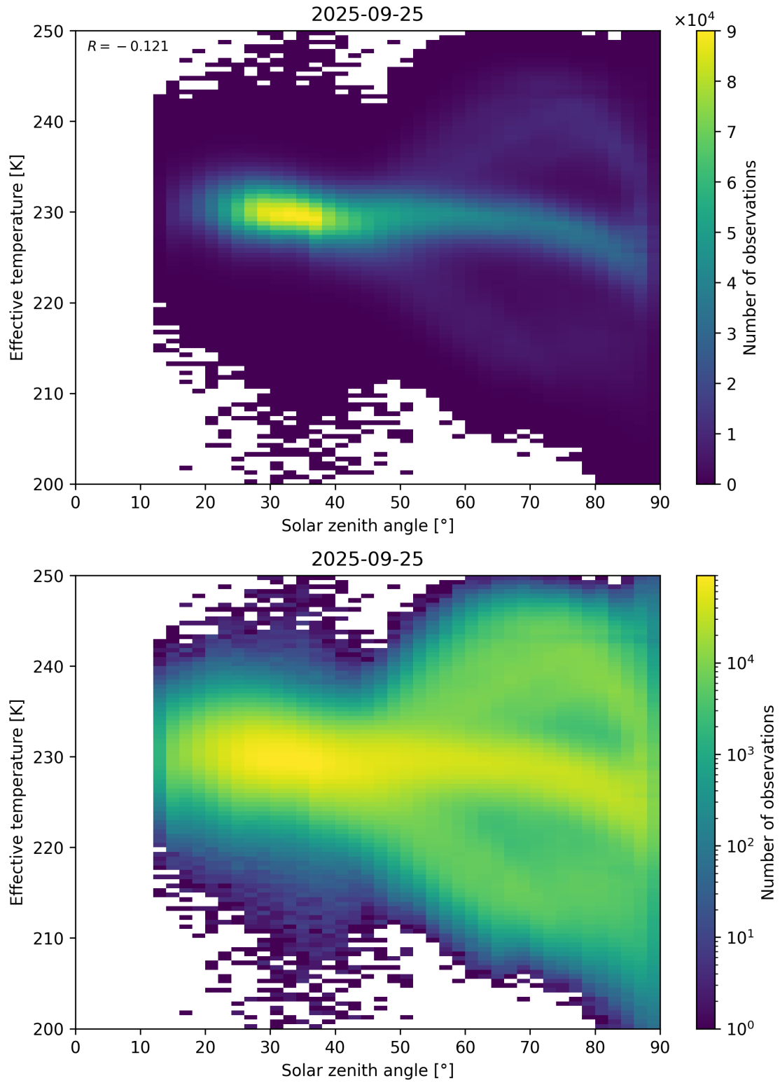
Figure 45: Scatter density plot of “Solar zenith angle” against “Effective temperature” for 2025-09-25 to 2025-09-26.
