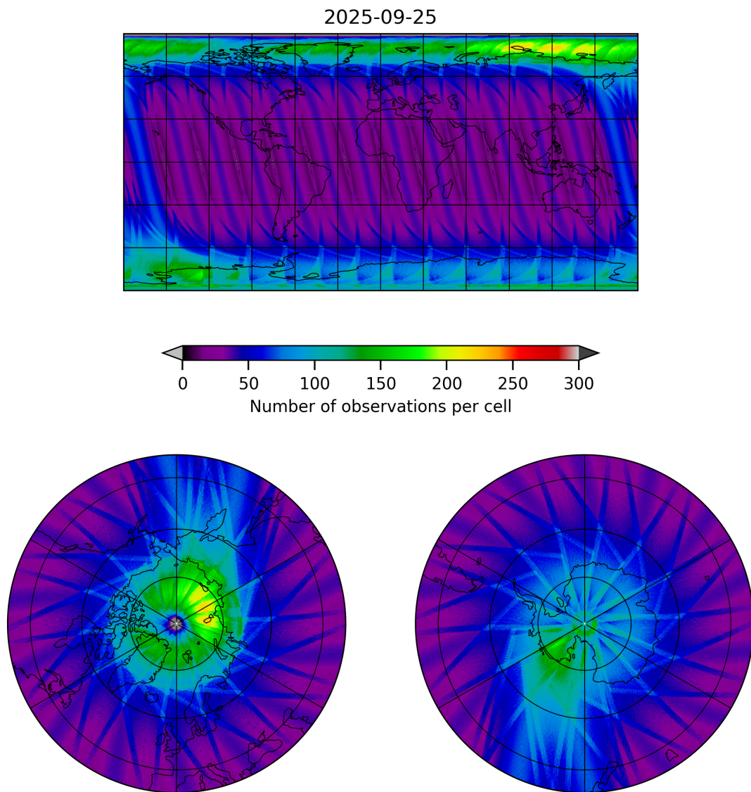
Figure 12: Map of the number of observations for 2025-09-25 to 2025-09-26
