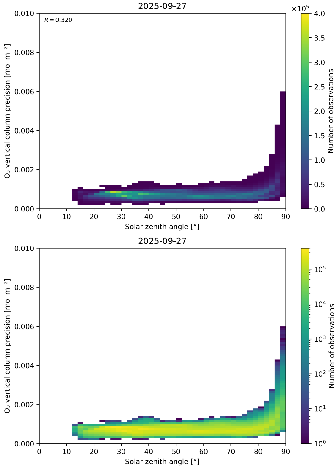
Figure 48: Scatter density plot of “Solar zenith angle” against “O 3 vertical column precision” for 2025-09-26 to 2025-09-28.
