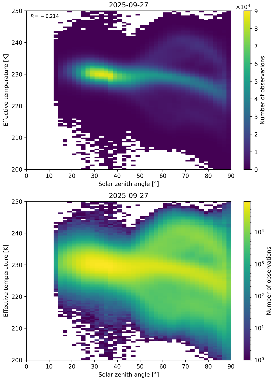
Figure 45: Scatter density plot of “Solar zenith angle” against “Effective temperature” for 2025-09-26 to 2025-09-28.
