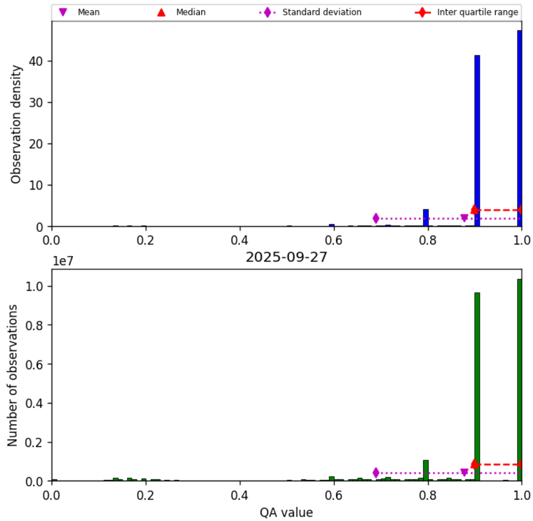
Figure 20: Histogram of “QA value” for 2025-09-26 to 2025-09-28
