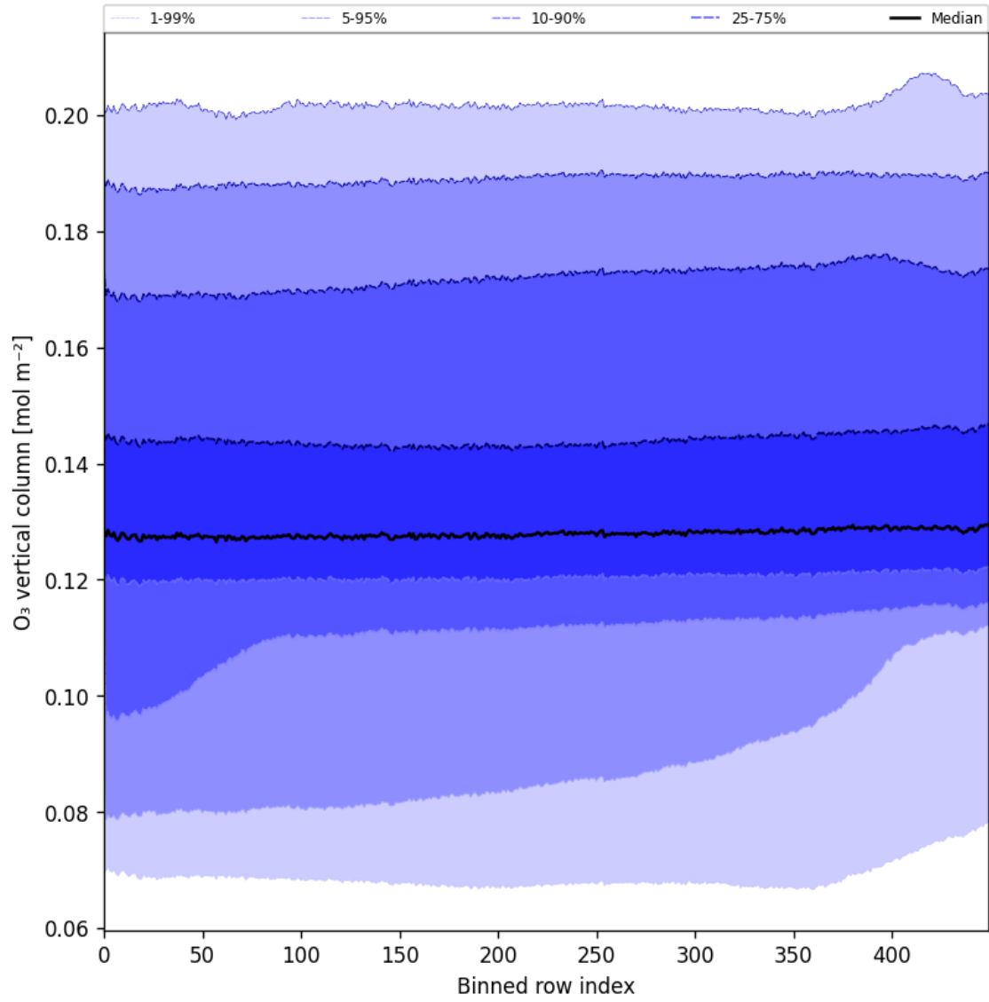
Figure 28: Along track statistics of “ \text{O}_3 vertical column” for 2025-09-26 to 2025-09-28
