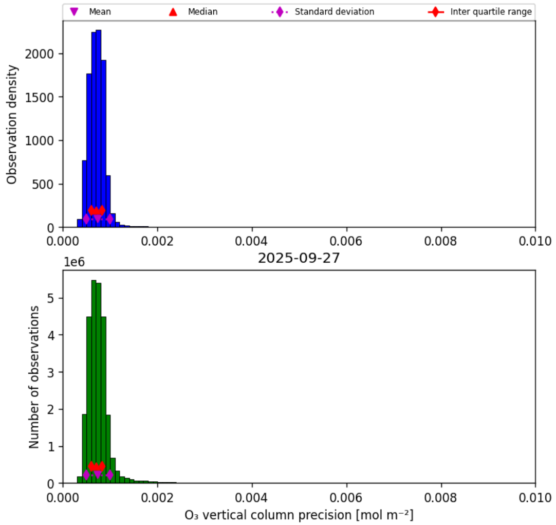
Figure 22: Histogram of “O 3 vertical column precision” for 2025-09-26 to 2025-09-28
