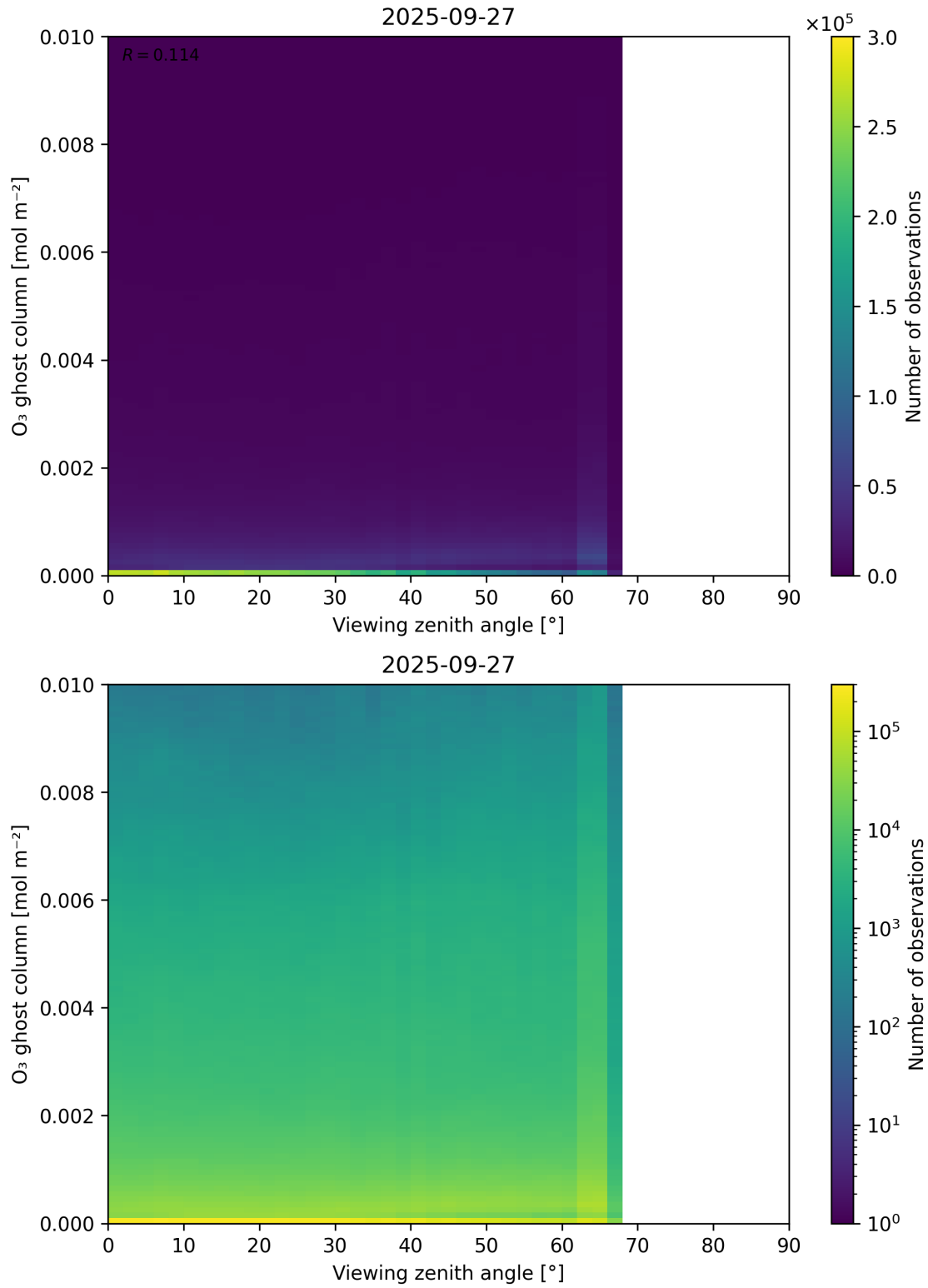
Figure 51: Scatter density plot of “Viewing zenith angle” against “O 3 ghost column” for 2025-09-26 to 2025-09-28.
