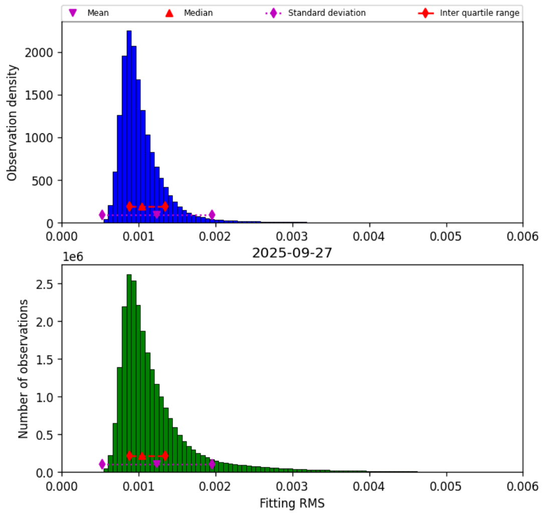
Figure 23: Histogram of “Fitting RMS” for 2025-09-26 to 2025-09-28
