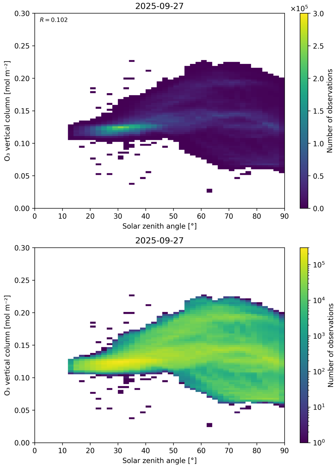
Figure 47: Scatter density plot of “Solar zenith angle” against “O 3 vertical column” for 2025-09-26 to 2025-09-28.
