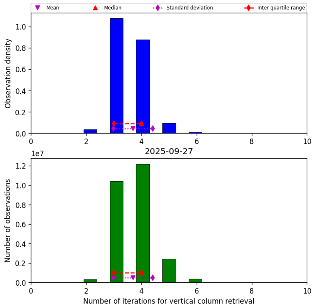
Figure 26: Histogram of “Number of iterations for vertical column retrieval” for 2025-09-26 to 2025-09-28
