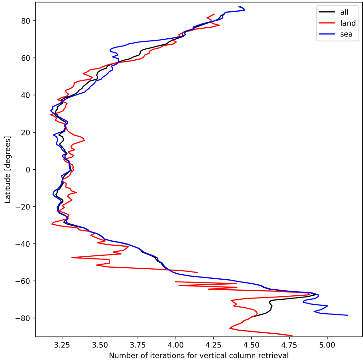
Figure 19: Zonal average of “Number of iterations for vertical column retrieval” for 2025-09-26 to 2025-09-28.
