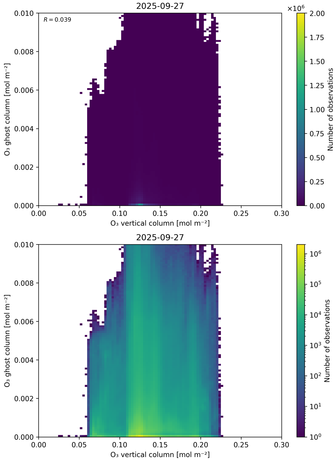
Figure 40: Scatter density plot of “O 3 vertical column” against “O 3 ghost column” for 2025-09-26 to 2025-09-28.
