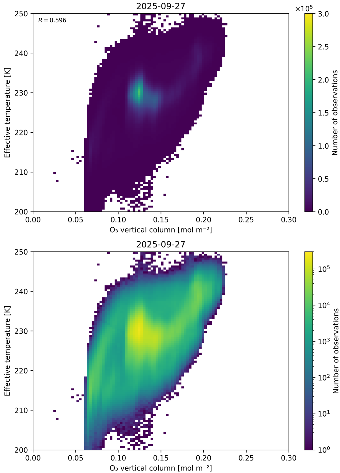
Figure 39: Scatter density plot of “O 3 vertical column” against “Effective temperature” for 2025-09-26 to 2025-09-28.
