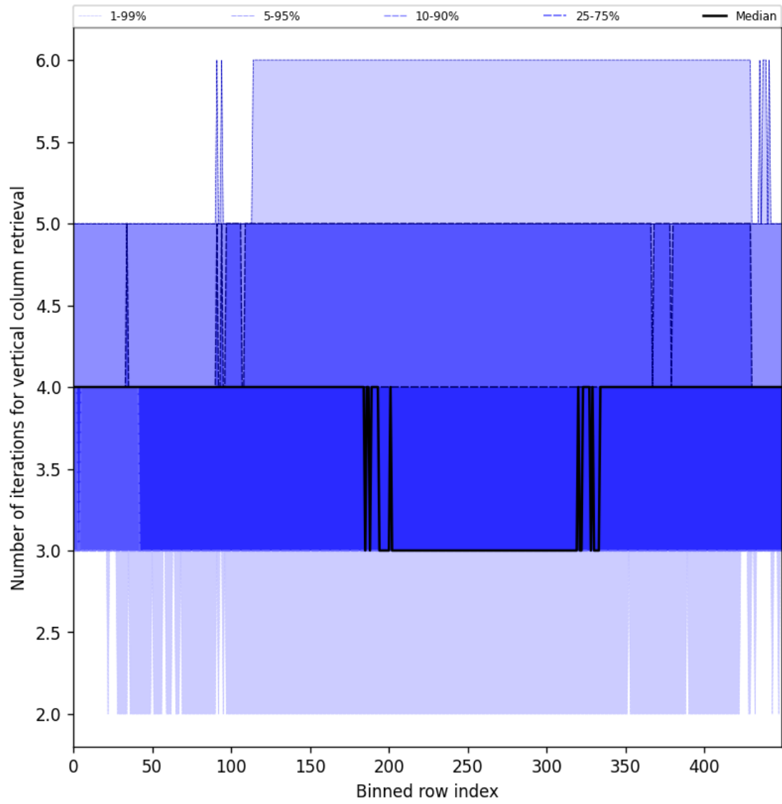
Figure 33: Along track statistics of “Number of iterations for vertical column retrieval” for 2025-09-26 to 2025-09-28
