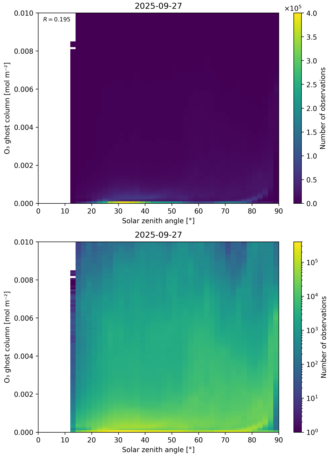
Figure 46: Scatter density plot of “Solar zenith angle” against “O 3 ghost column” for 2025-09-26 to 2025-09-28.
