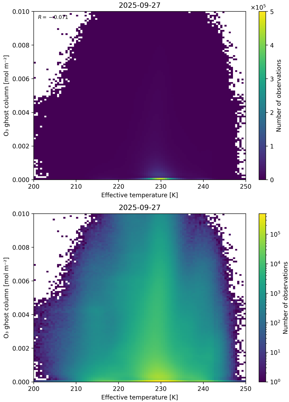
Figure 38: Scatter density plot of “Effective temperature” against “O 3 ghost column” for 2025-09-26 to 2025-09-28.
