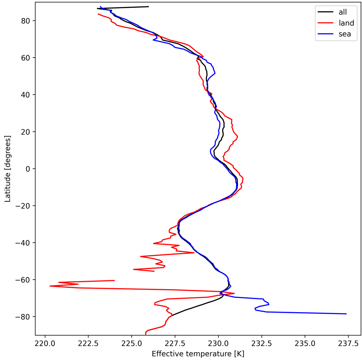
Figure 17: Zonal average of “Effective temperature” for 2025-09-26 to 2025-09-28.
