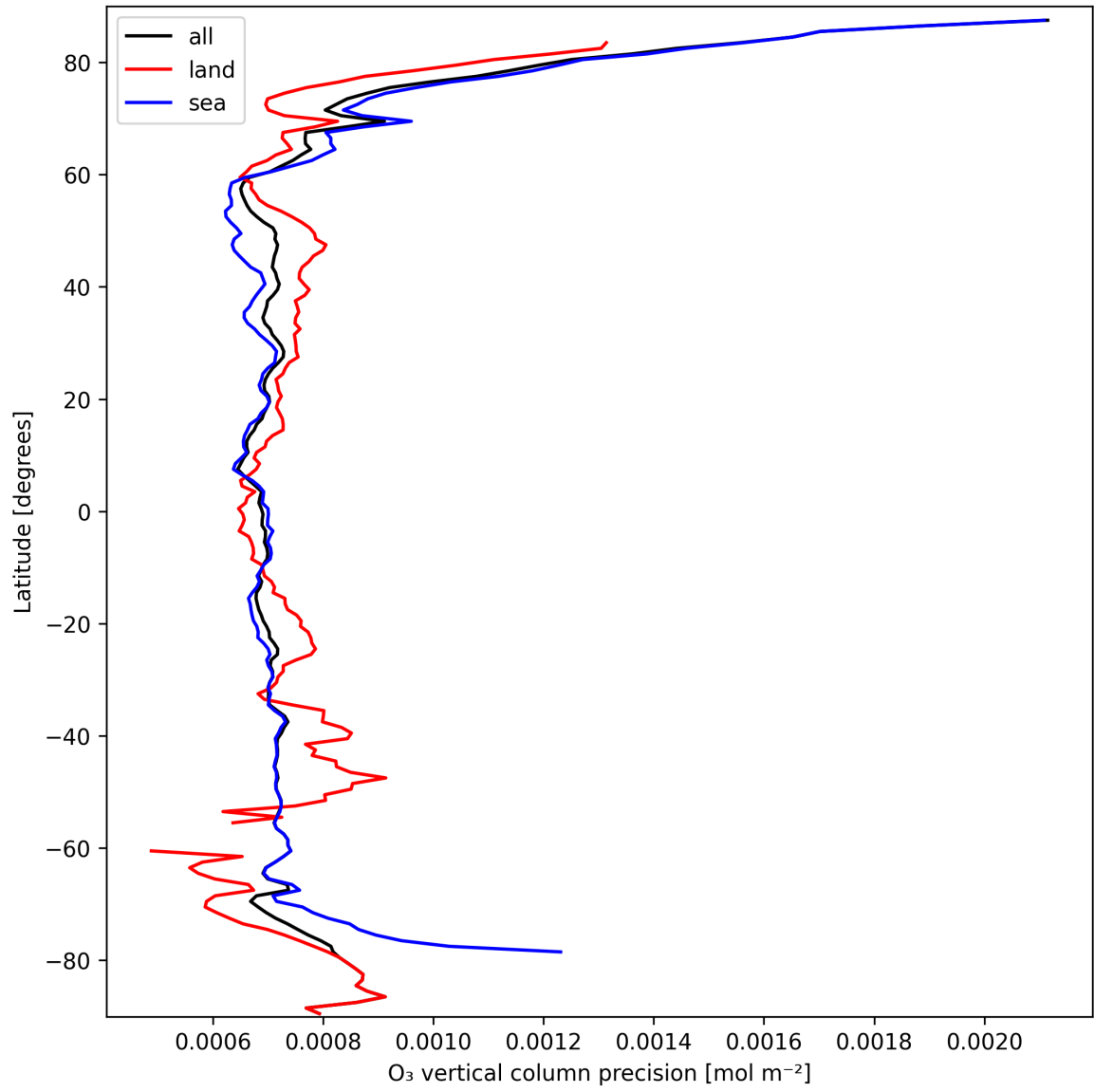
Figure 15: Zonal average of “O 3 vertical column precision” for 2025-09-26 to 2025-09-28.
