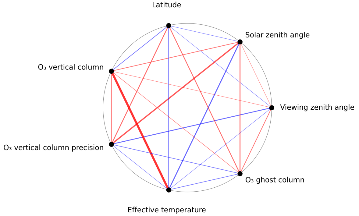
Figure 1: Map of correlation graph for 2025-09-26 to 2025-09-28.
