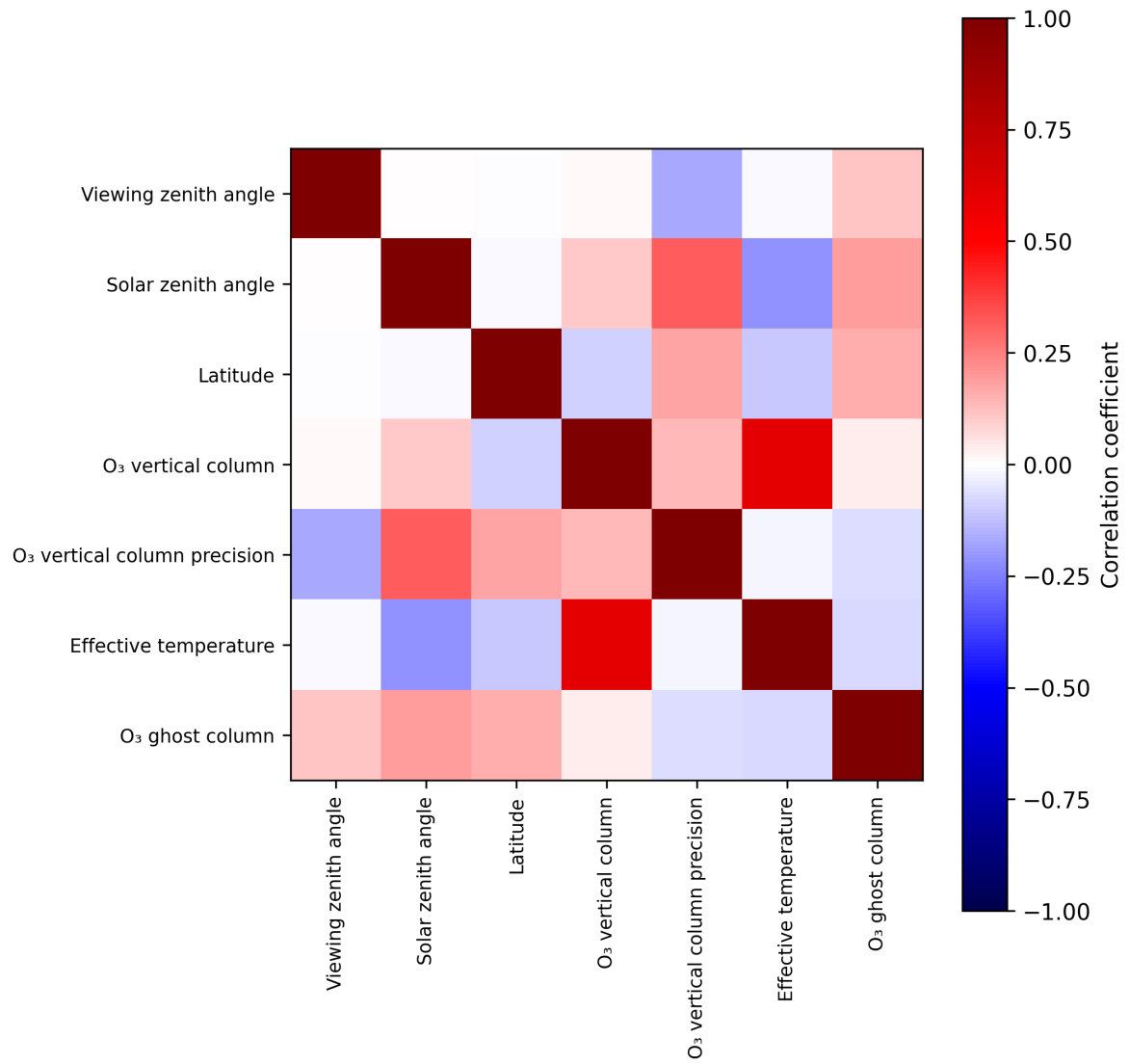
Figure 2: Map of correlation matrix for 2025-09-26 to 2025-09-28.
