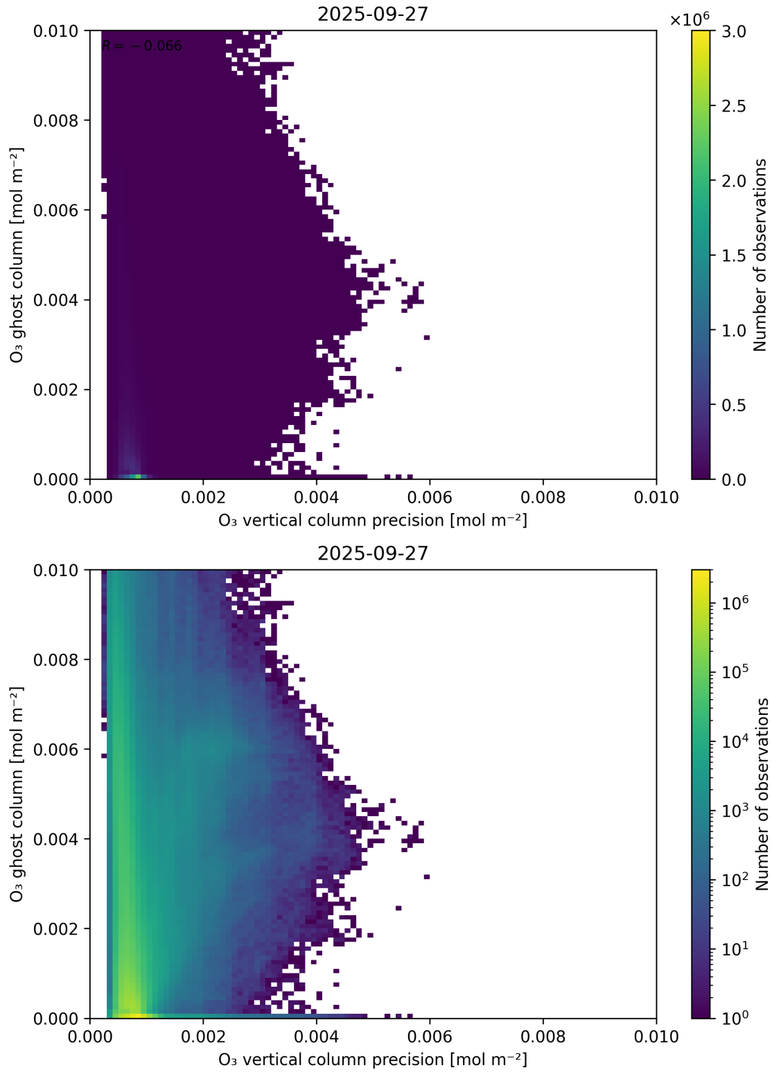
Figure 43: Scatter density plot of “ \text{O}_3 vertical column precision” against “ \text{O}_3 ghost column” for 2025-09-26 to 2025-09-28.
