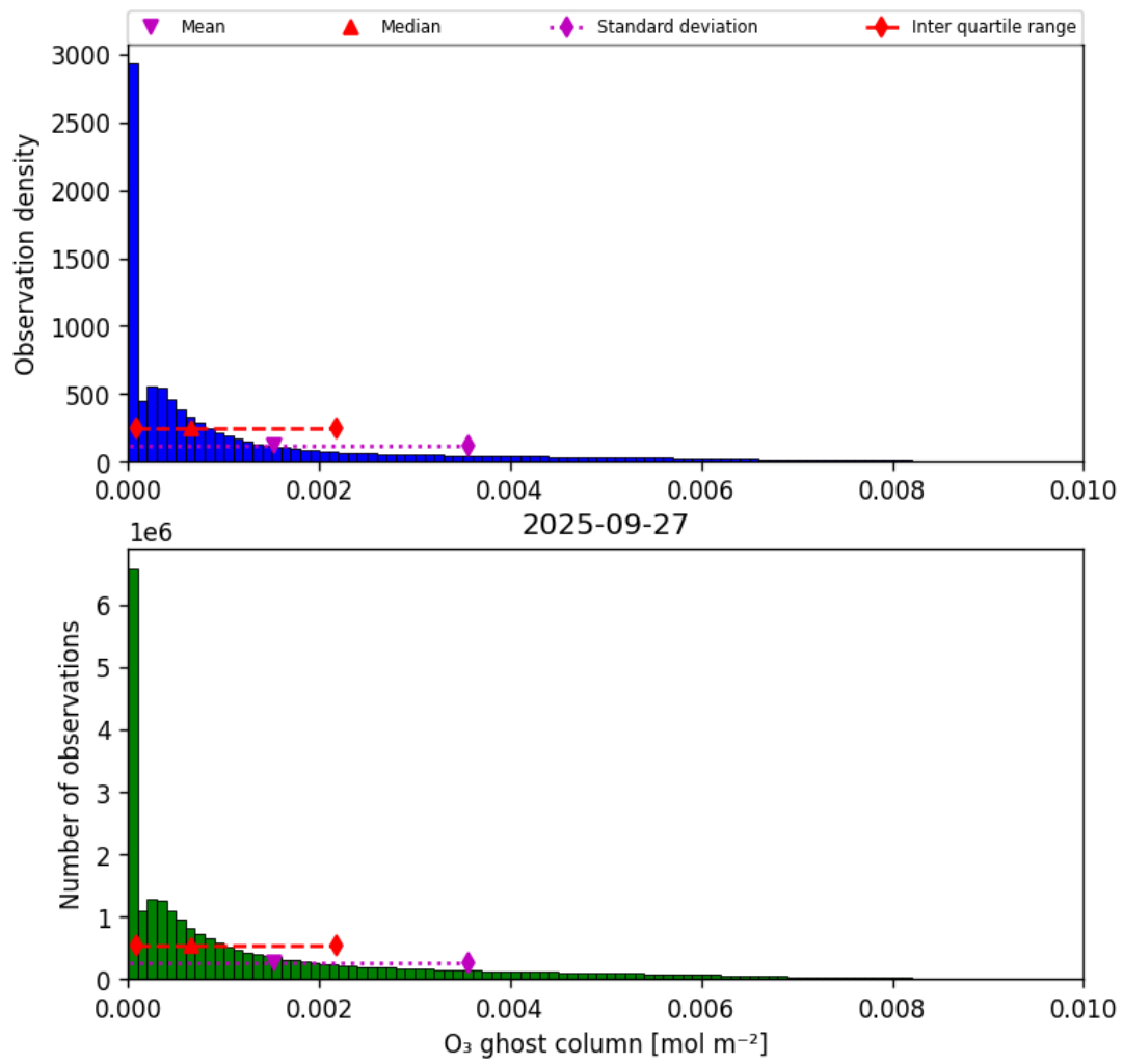
Figure 25: Histogram of “O 3 ghost column” for 2025-09-26 to 2025-09-28
