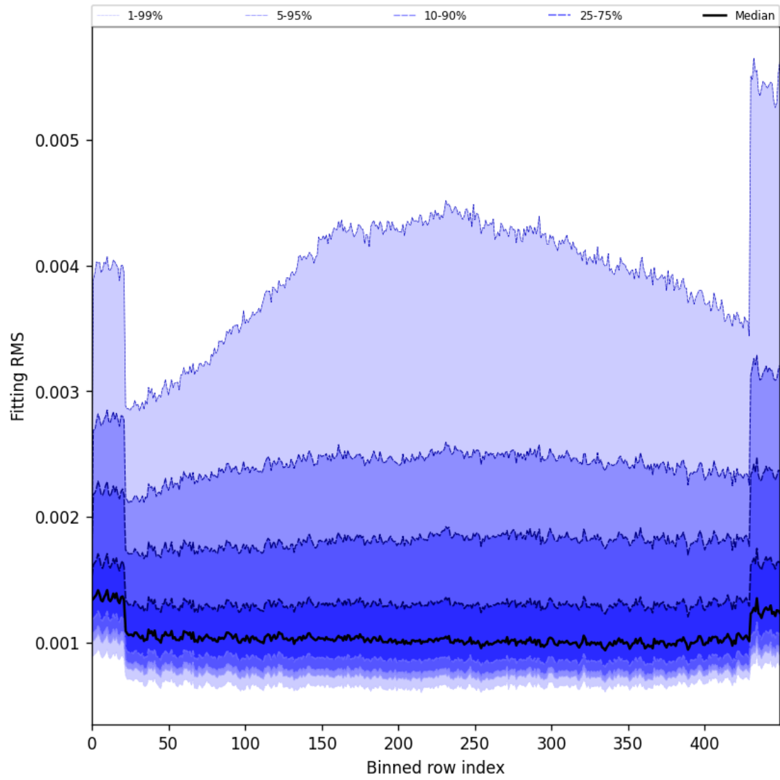
Figure 30: Along track statistics of “Fitting RMS” for 2025-09-26 to 2025-09-28
