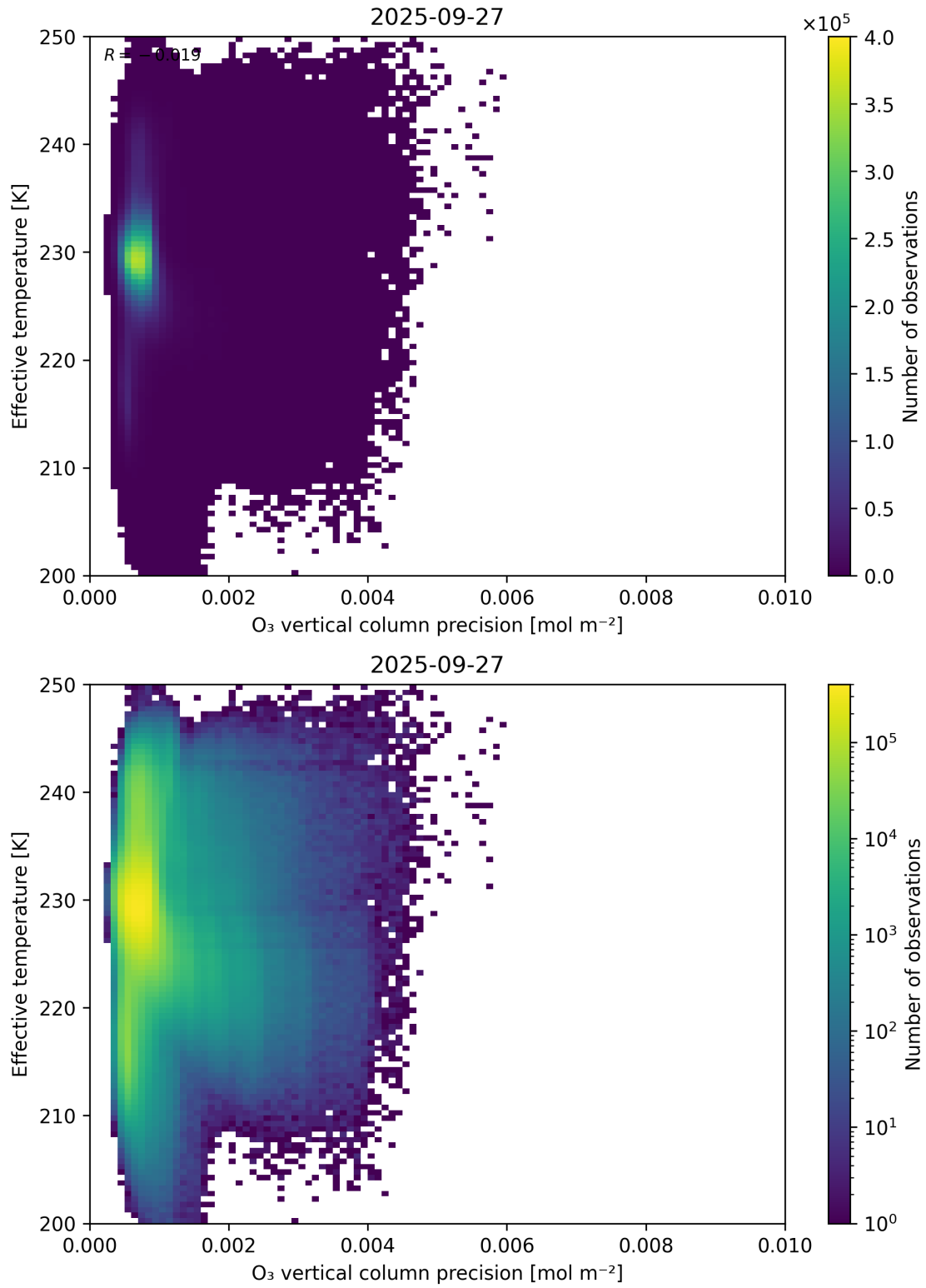
Figure 42: Scatter density plot of “O 3 vertical column precision” against “Effective temperature” for 2025-09-26 to 2025-09-28.
