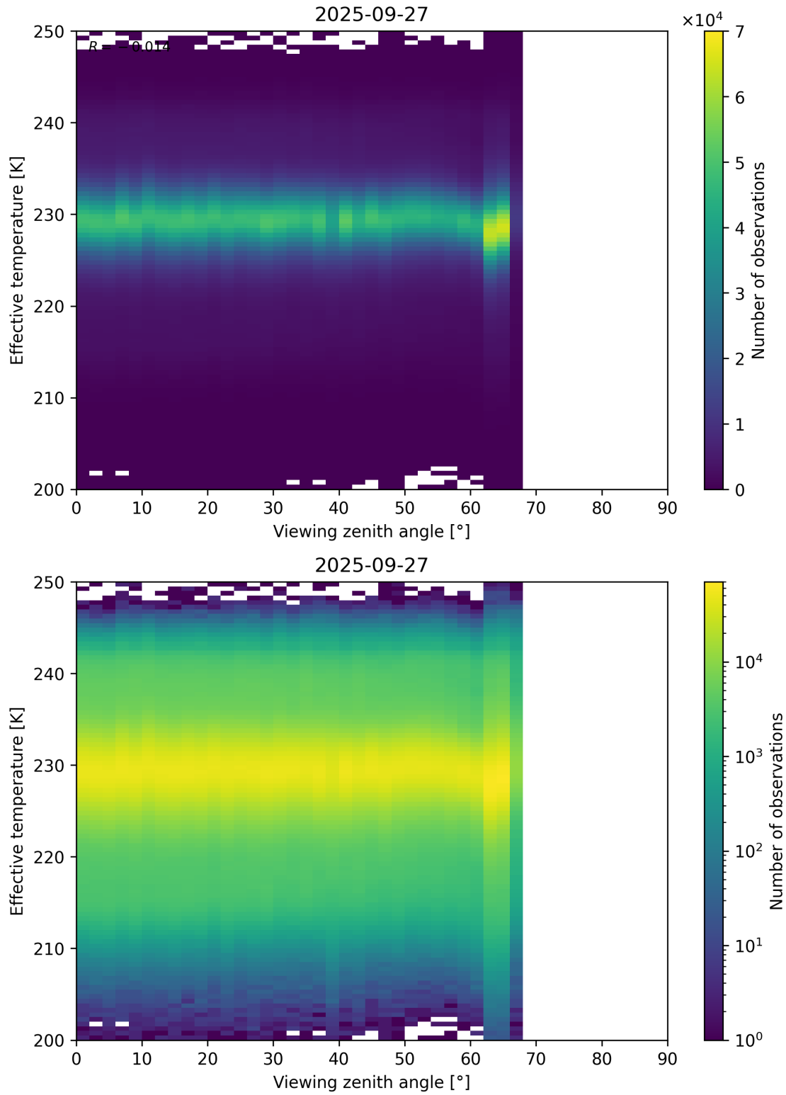
Figure 50: Scatter density plot of “Viewing zenith angle” against “Effective temperature” for 2025-09-26 to 2025-09-28.
