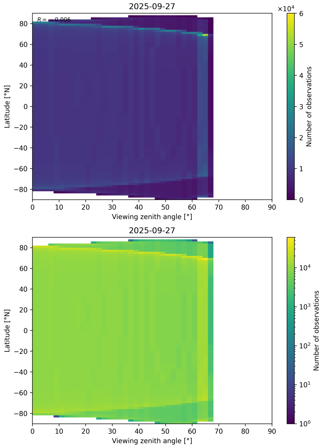
Figure 49: Scatter density plot of “Viewing zenith angle” against “Latitude” for 2025-09-26 to 2025-09-28.
