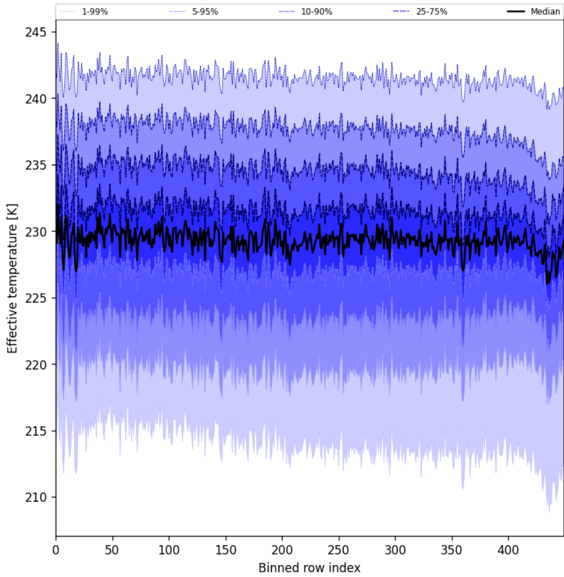
Figure 31: Along track statistics of “Effective temperature” for 2025-09-26 to 2025-09-28
