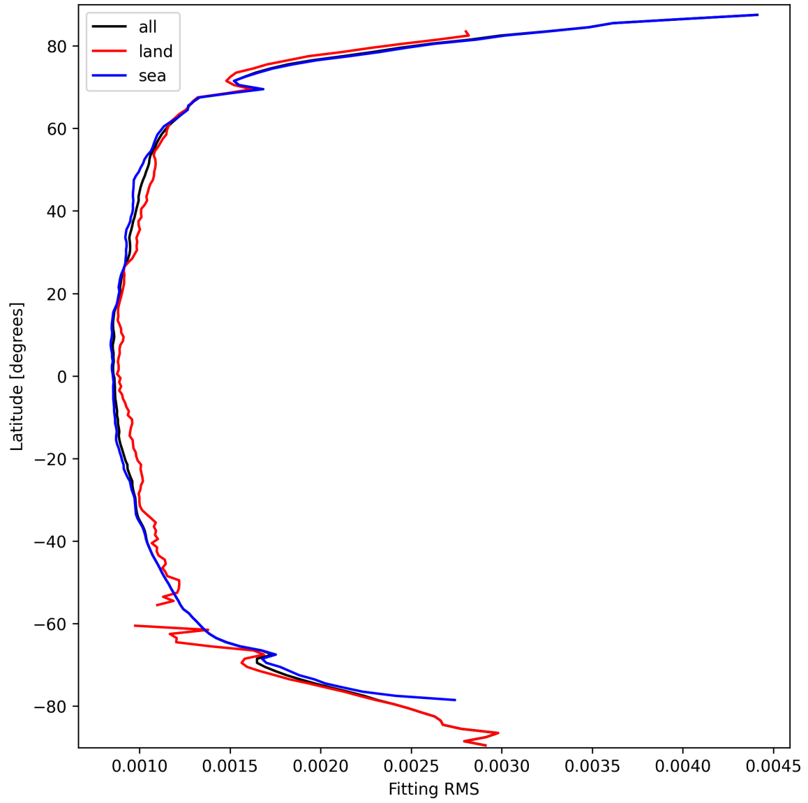
Figure 16: Zonal average of “Fitting RMS” for 2025-09-26 to 2025-09-28.
