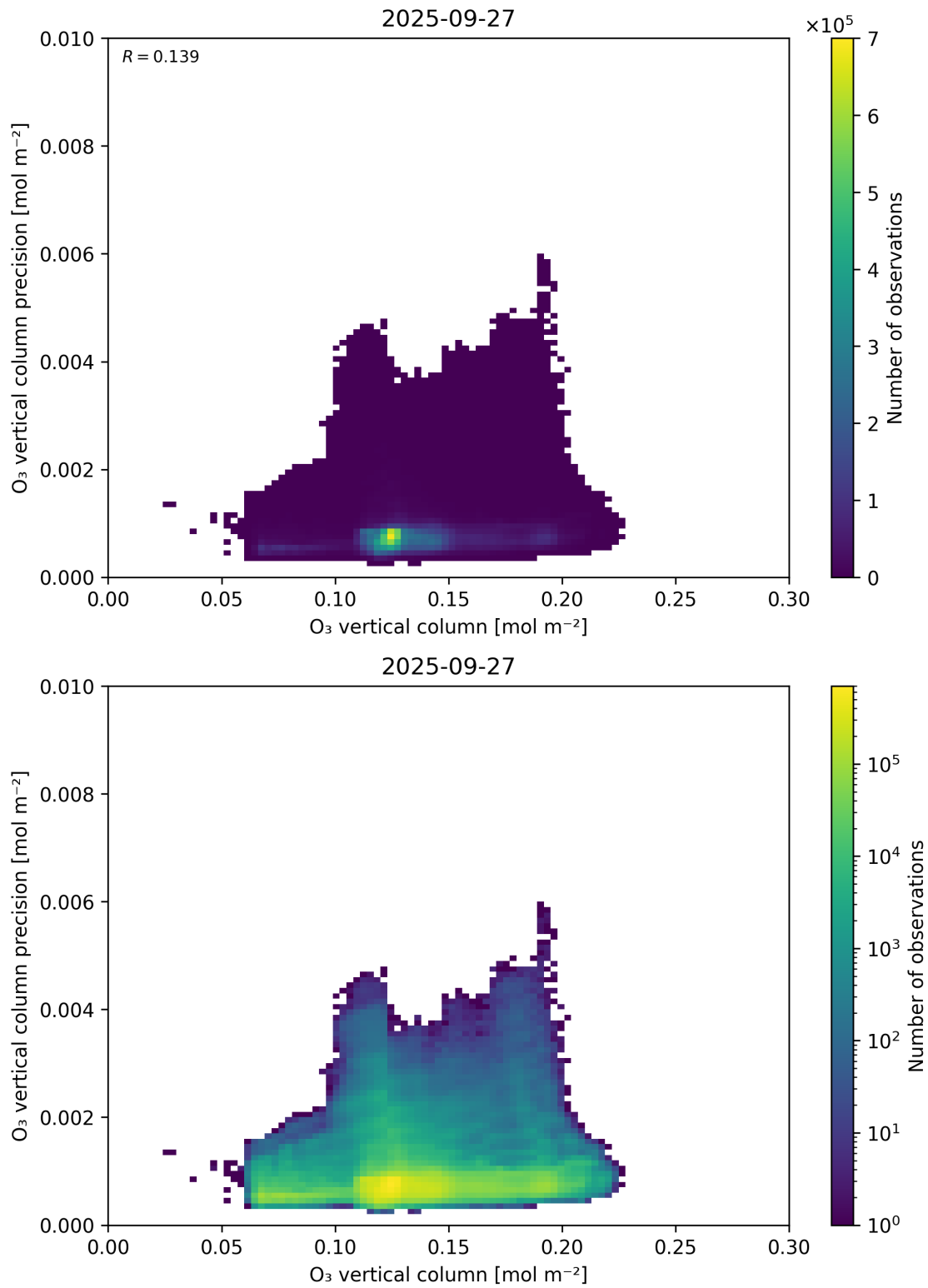
Figure 41: Scatter density plot of “O 3 vertical column” against “O 3 vertical column precision” for 2025-09-26 to 2025-09-28.
