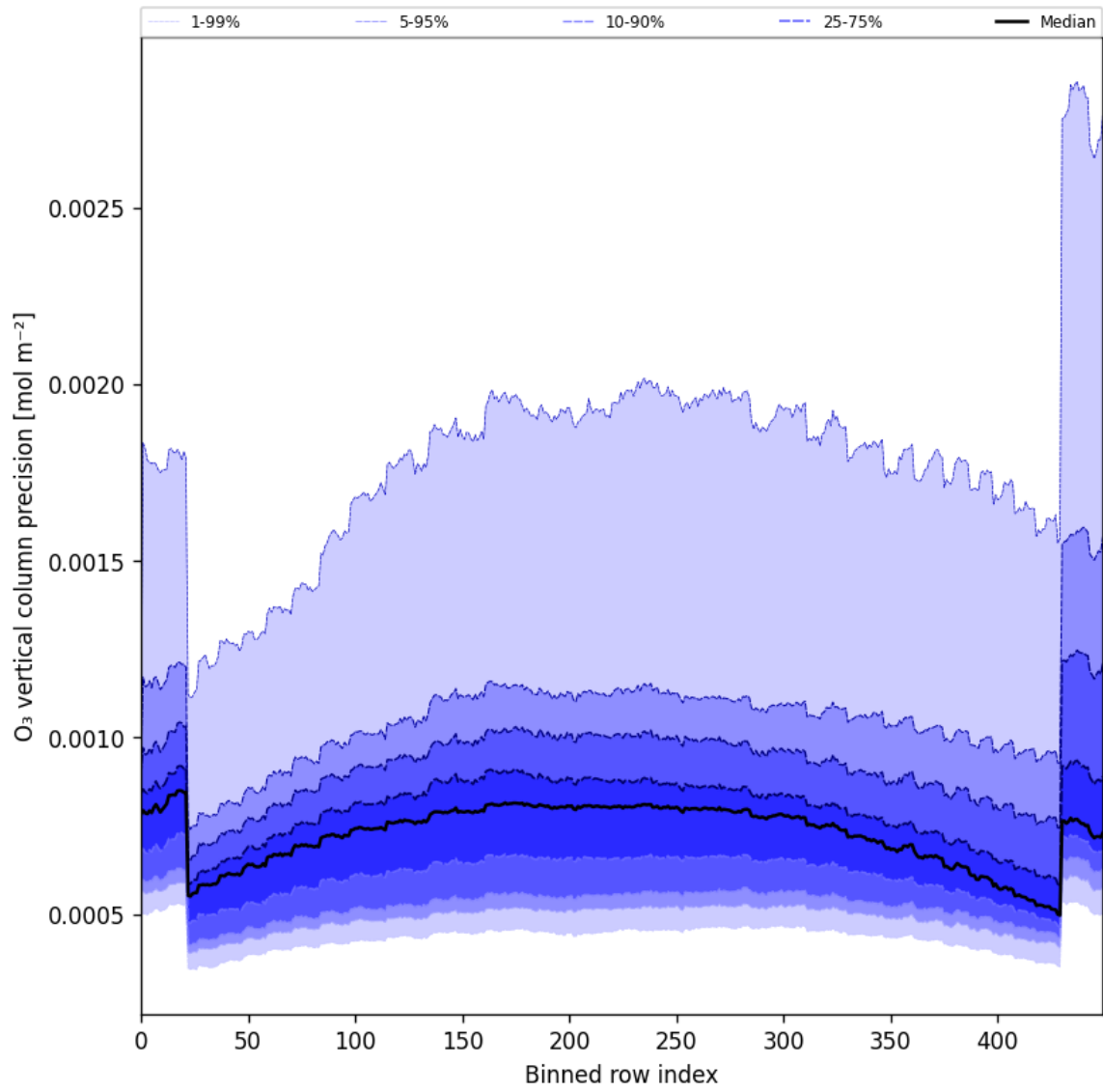
Figure 29: Along track statistics of “O 3 vertical column precision” for 2025-09-26 to 2025-09-28
