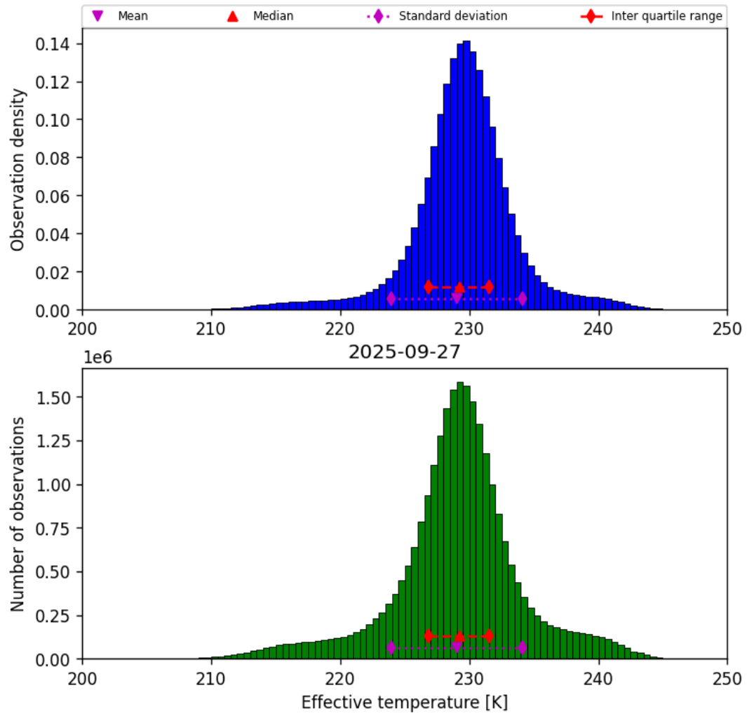
Figure 24: Histogram of “Effective temperature” for 2025-09-26 to 2025-09-28
