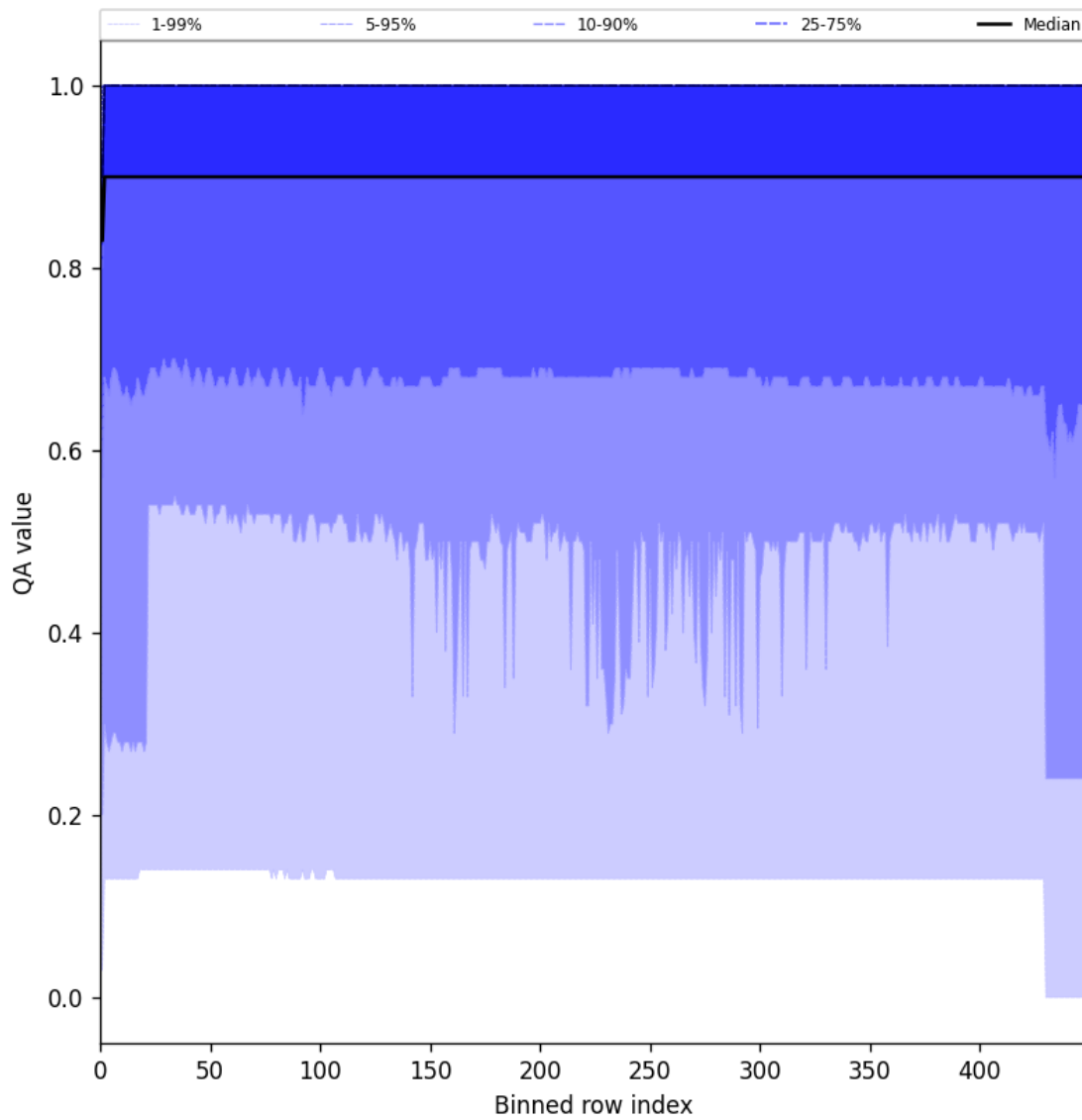
Figure 27: Along track statistics of “QA value” for 2025-09-26 to 2025-09-28
