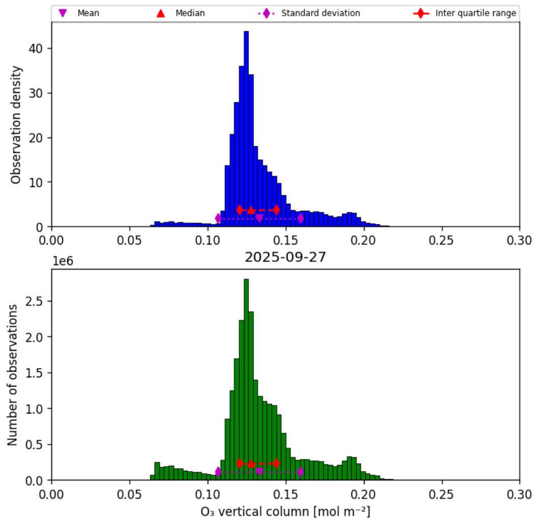
Figure 21: Histogram of “O 3 vertical column” for 2025-09-26 to 2025-09-28
