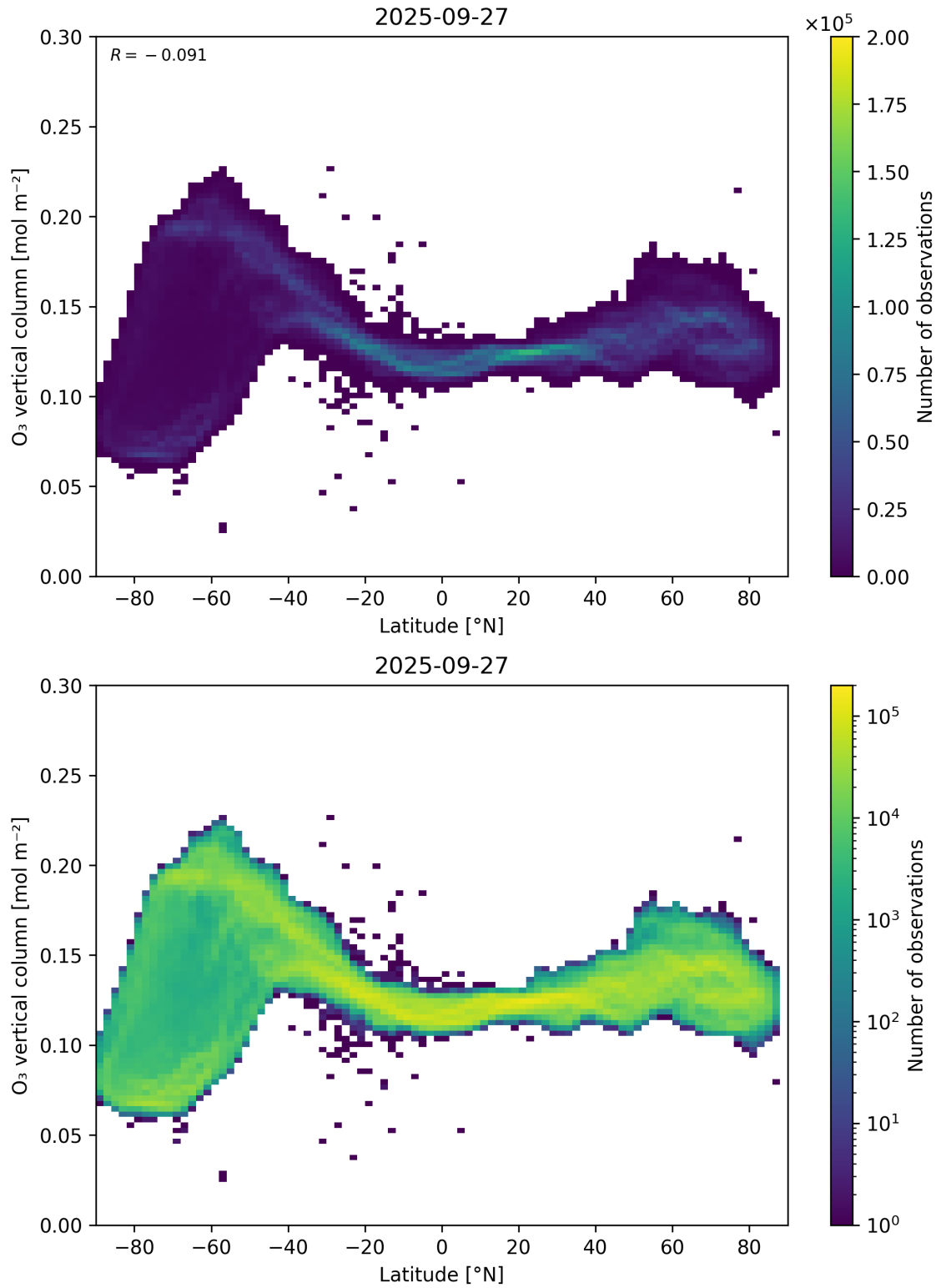
Figure 36: Scatter density plot of “Latitude” against “O 3 vertical column” for 2025-09-26 to 2025-09-28.
