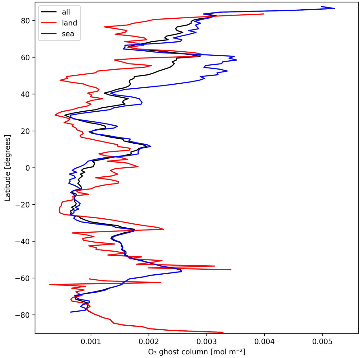
Figure 18: Zonal average of "O 3 ghost column" for 2025-09-26 to 2025-09-28.
