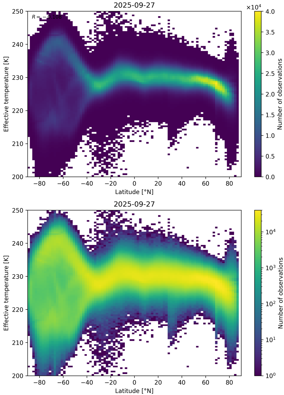
Figure 34: Scatter density plot of “Latitude” against “Effective temperature” for 2025-09-26 to 2025-09-28.
