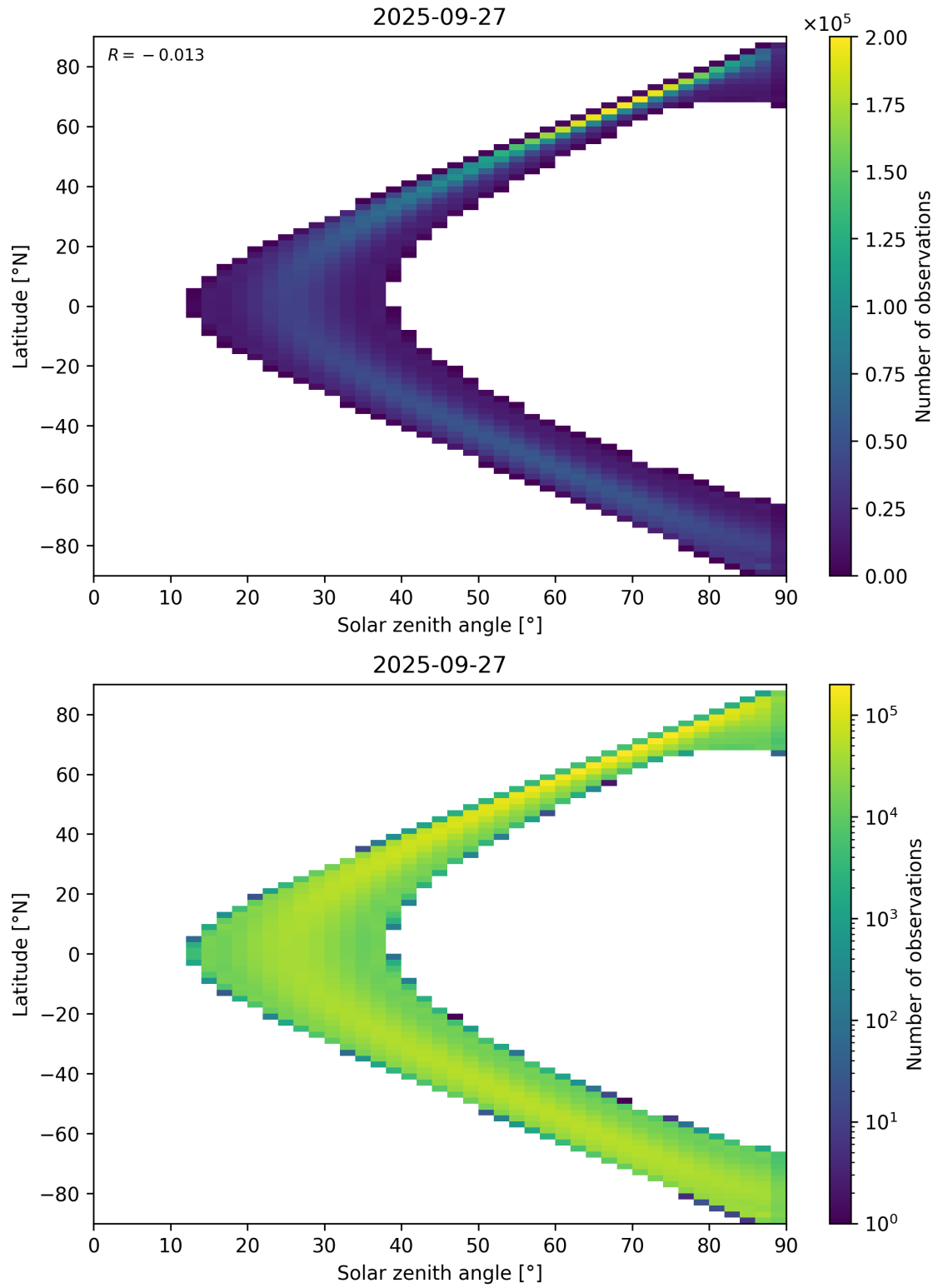
Figure 44: Scatter density plot of “Solar zenith angle” against “Latitude” for 2025-09-26 to 2025-09-28.
