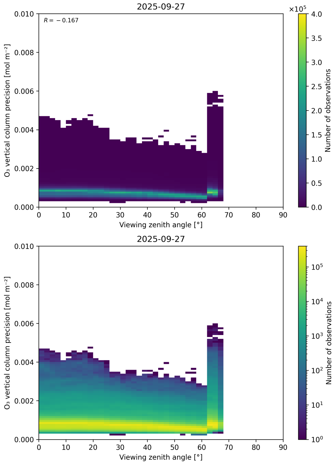
Figure 53: Scatter density plot of “Viewing zenith angle” against “O 3 vertical column precision” for 2025-09-26 to 2025-09-28.
