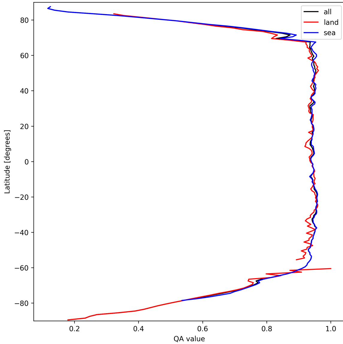
Figure 13: Zonal average of “QA value” for 2025-09-26 to 2025-09-28.
