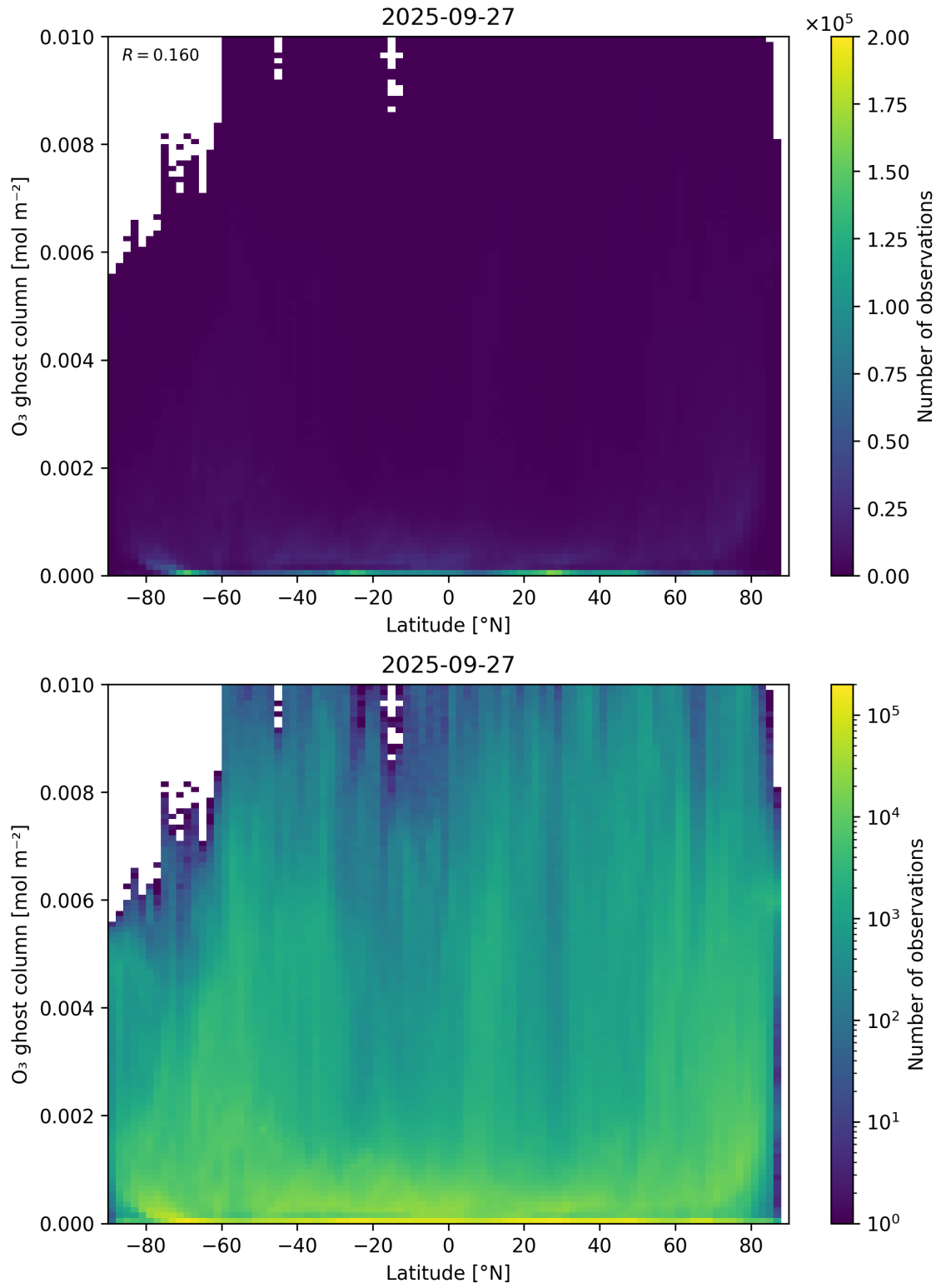
Figure 35: Scatter density plot of “Latitude” against “O 3 ghost column” for 2025-09-26 to 2025-09-28.
