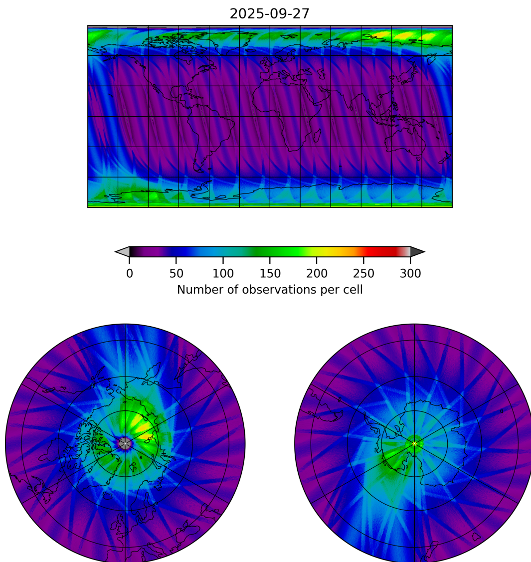
Figure 12: Map of the number of observations for 2025-09-26 to 2025-09-28
