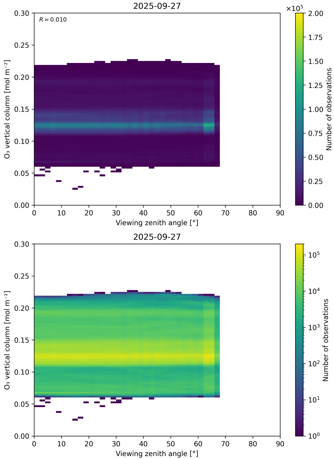
Figure 52: Scatter density plot of “Viewing zenith angle” against “O 3 vertical column” for 2025-09-26 to 2025-09-28.
