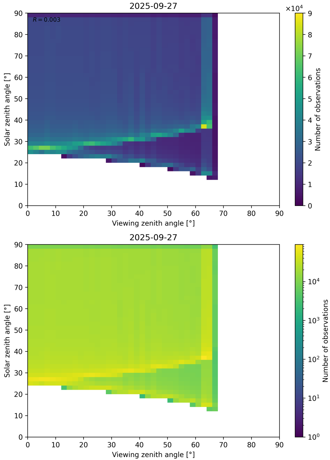
Figure 54: Scatter density plot of “Viewing zenith angle” against “Solar zenith angle” for 2025-09-26 to 2025-09-28.
