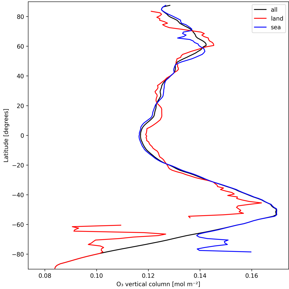
Figure 14: Zonal average of “O 3 vertical column” for 2025-09-26 to 2025-09-28.
