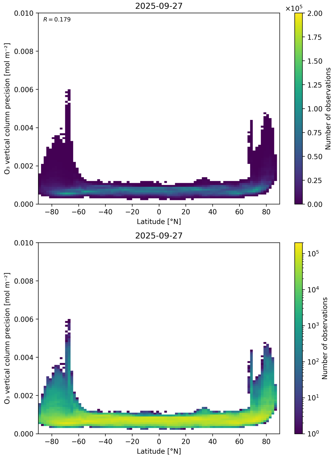
Figure 37: Scatter density plot of “Latitude” against “O 3 vertical column precision” for 2025-09-26 to 2025-09-28.
