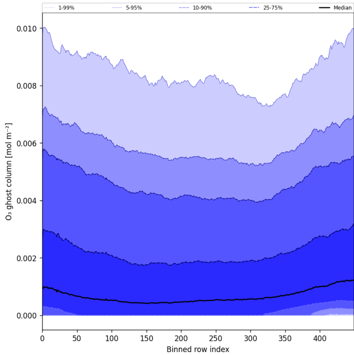
Figure 32: Along track statistics of “O 3 ghost column” for 2025-09-26 to 2025-09-28
