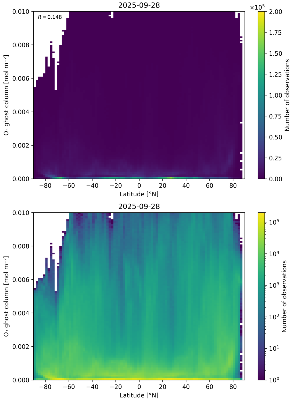
Figure 35: Scatter density plot of “Latitude” against “O 3 ghost column” for 2025-09-27 to 2025-09-29.
