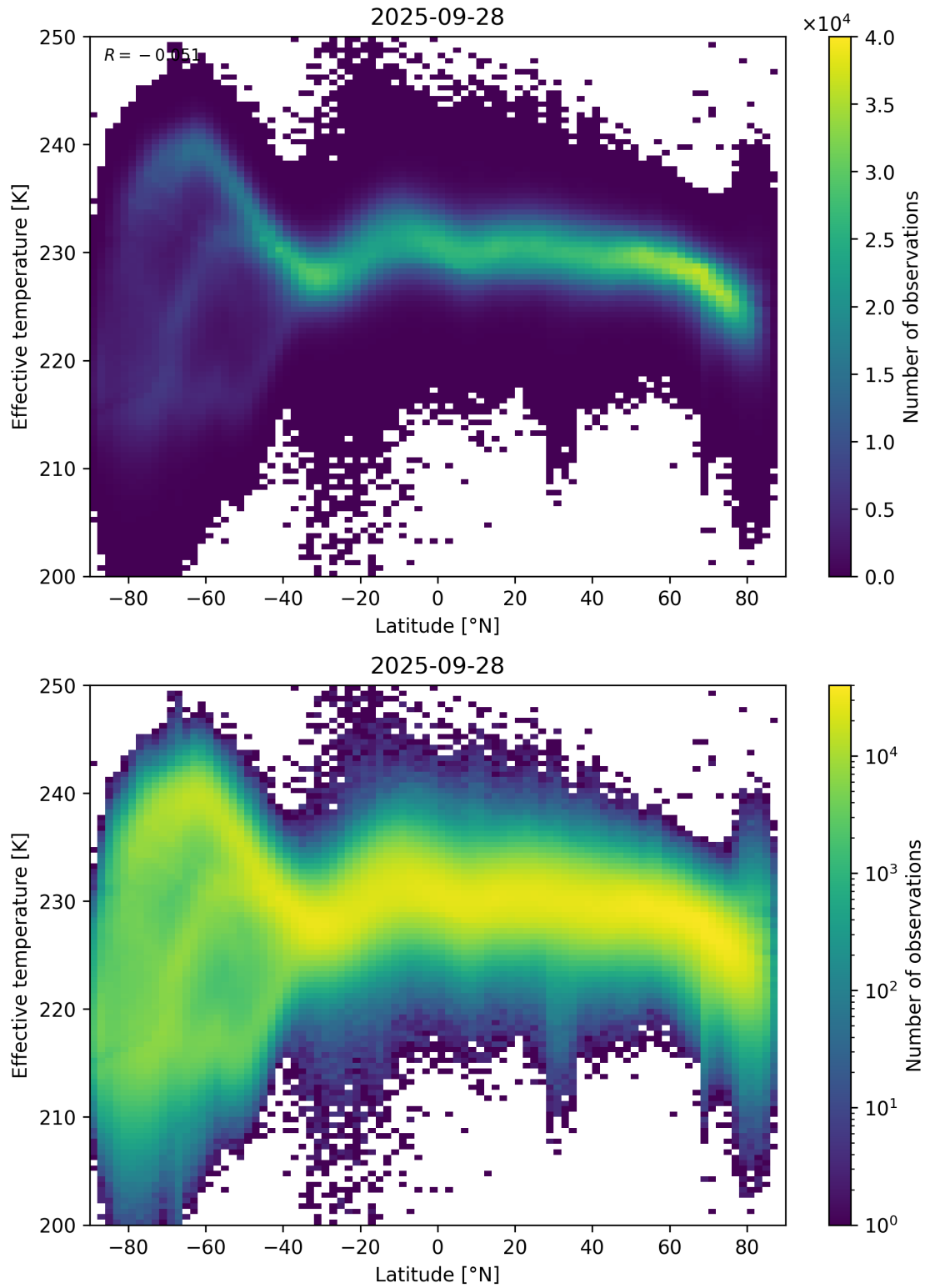
Figure 34: Scatter density plot of “Latitude” against “Effective temperature” for 2025-09-27 to 2025-09-29.
