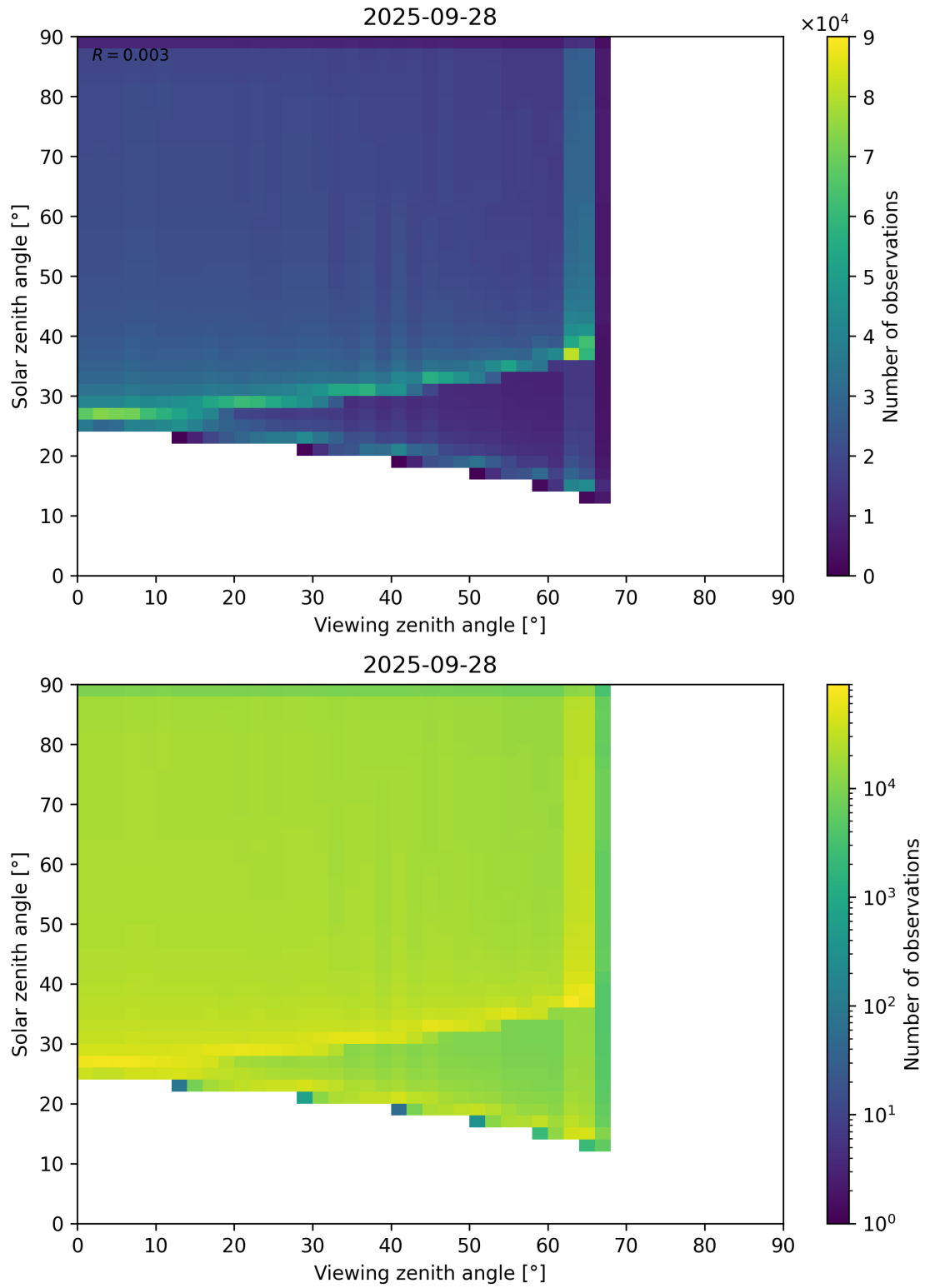
Figure 54: Scatter density plot of “Viewing zenith angle” against “Solar zenith angle” for 2025-09-27 to 2025-09-29.
