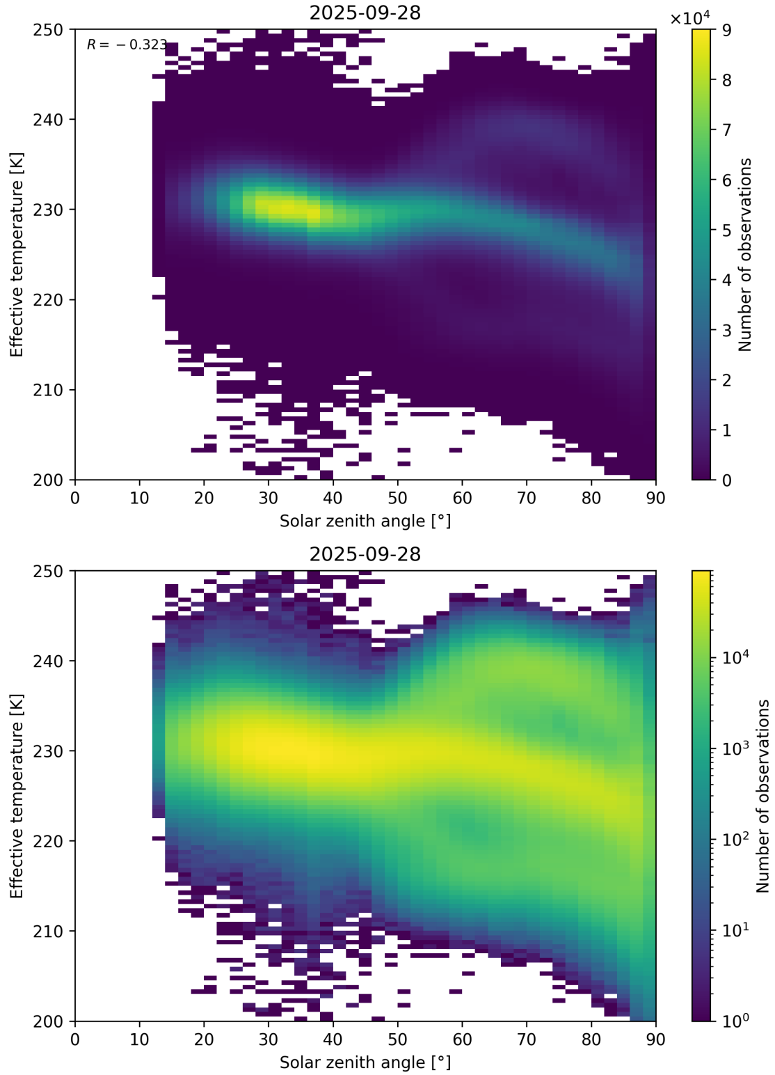
Figure 45: Scatter density plot of “Solar zenith angle” against “Effective temperature” for 2025-09-27 to 2025-09-29.
