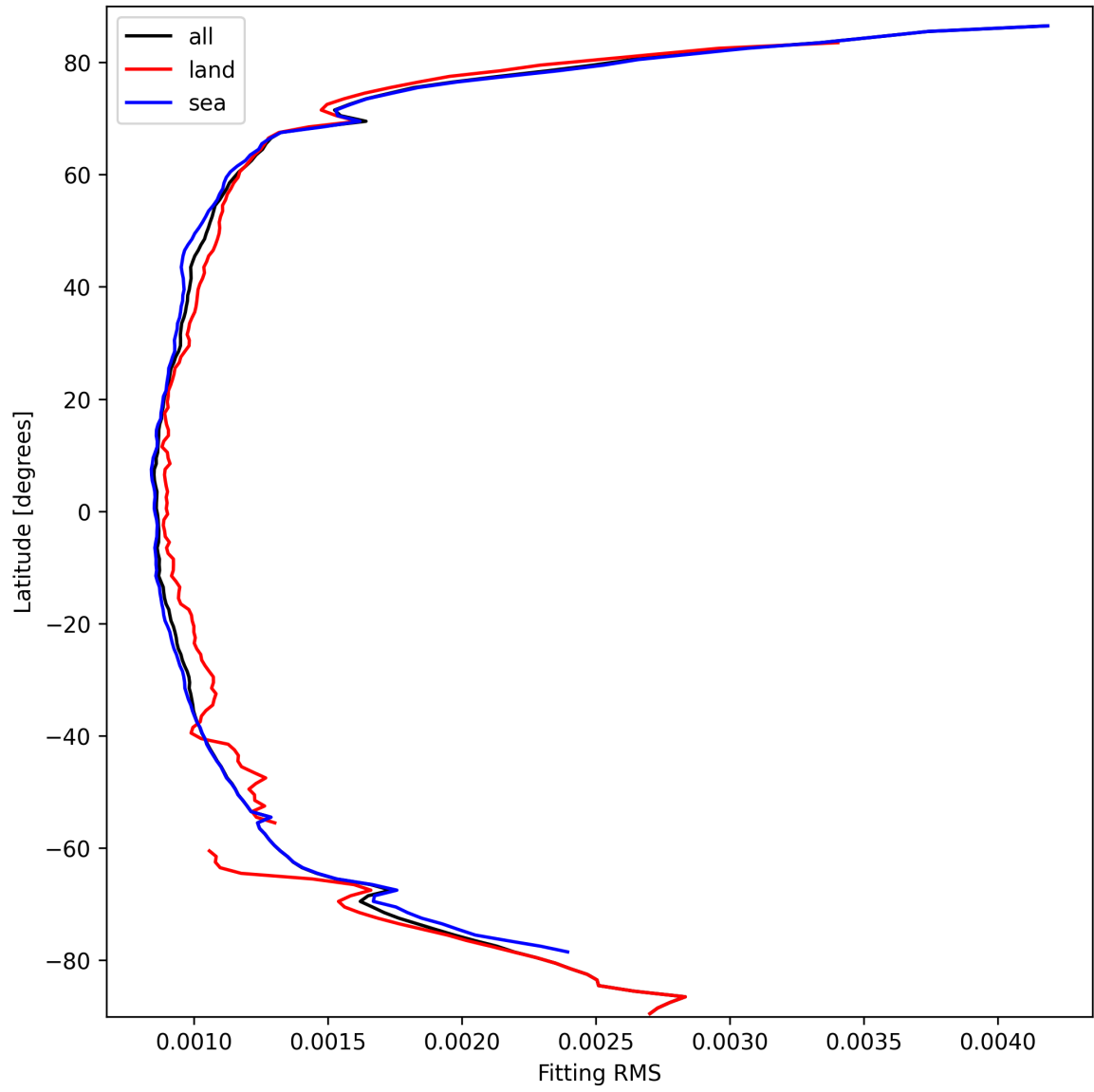
Figure 16: Zonal average of “Fitting RMS” for 2025-09-27 to 2025-09-29.
