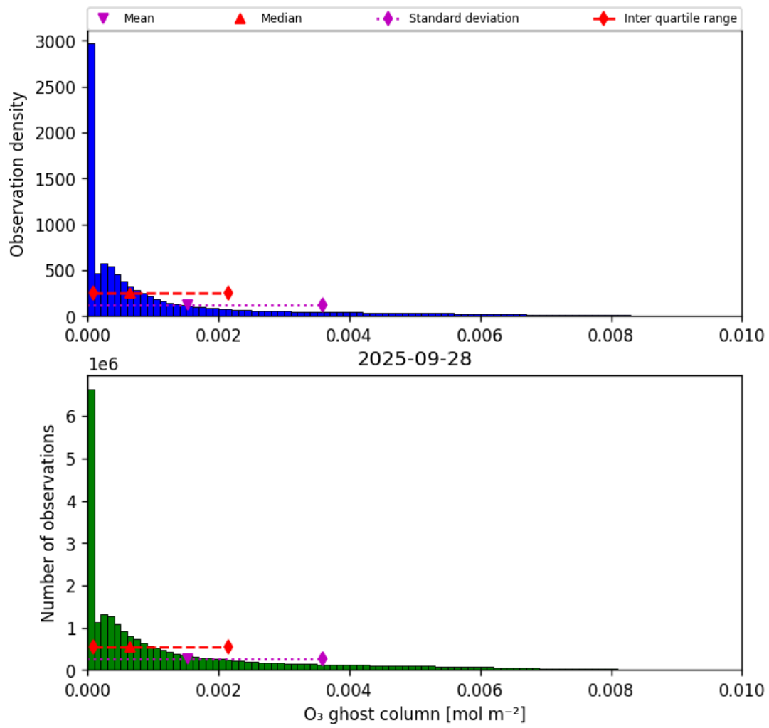
Figure 25: Histogram of “O 3 ghost column” for 2025-09-27 to 2025-09-29
