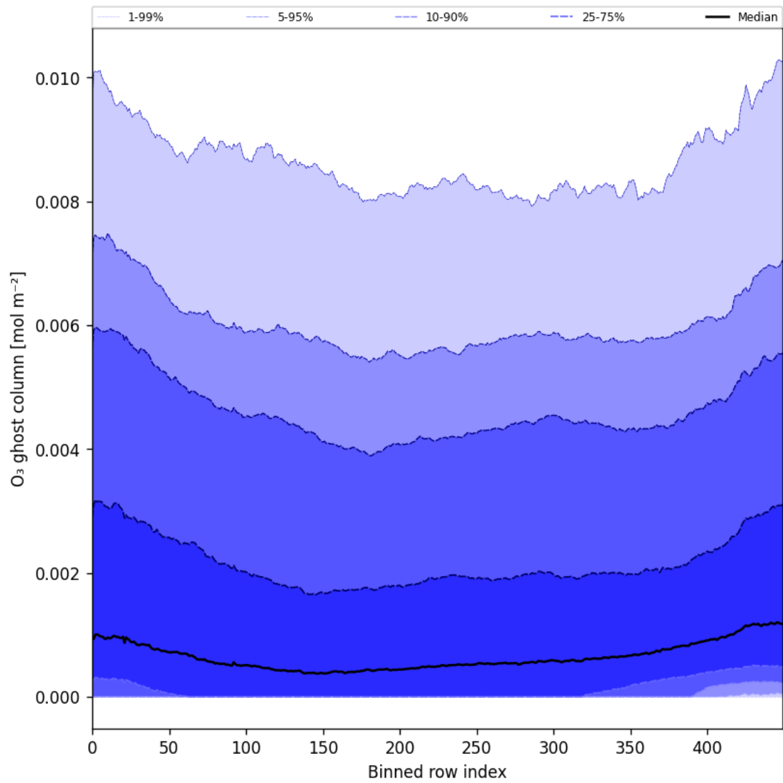
Figure 32: Along track statistics of “O 3 ghost column” for 2025-09-27 to 2025-09-29
