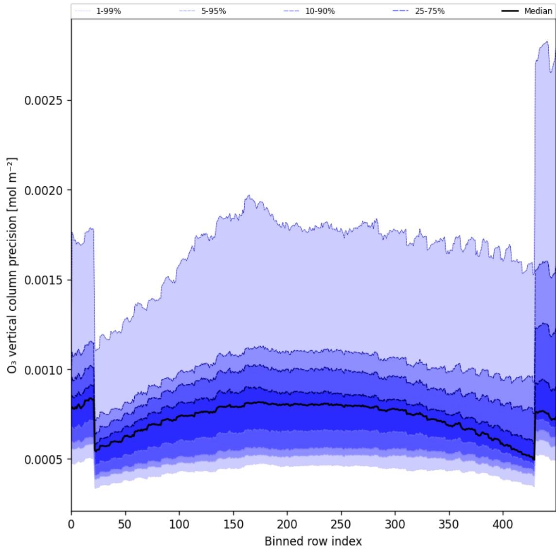
Figure 29: Along track statistics of “O 3 vertical column precision” for 2025-09-27 to 2025-09-29
