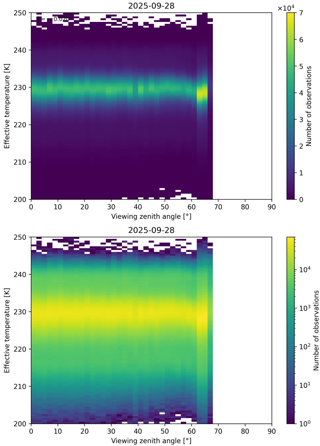
Figure 50: Scatter density plot of “Viewing zenith angle” against “Effective temperature” for 2025-09-27 to 2025-09-29.
