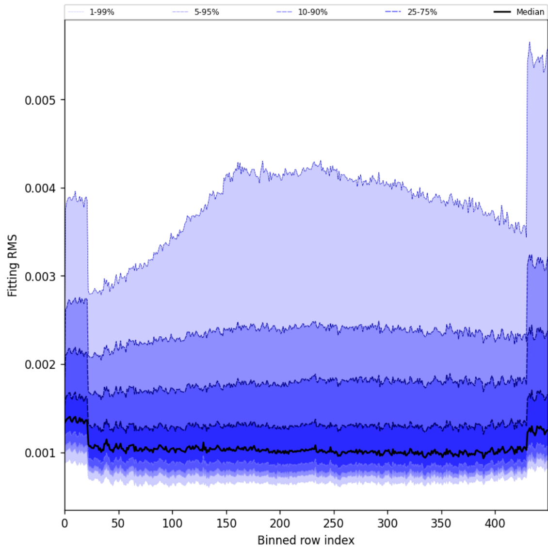
Figure 30: Along track statistics of “Fitting RMS” for 2025-09-27 to 2025-09-29
