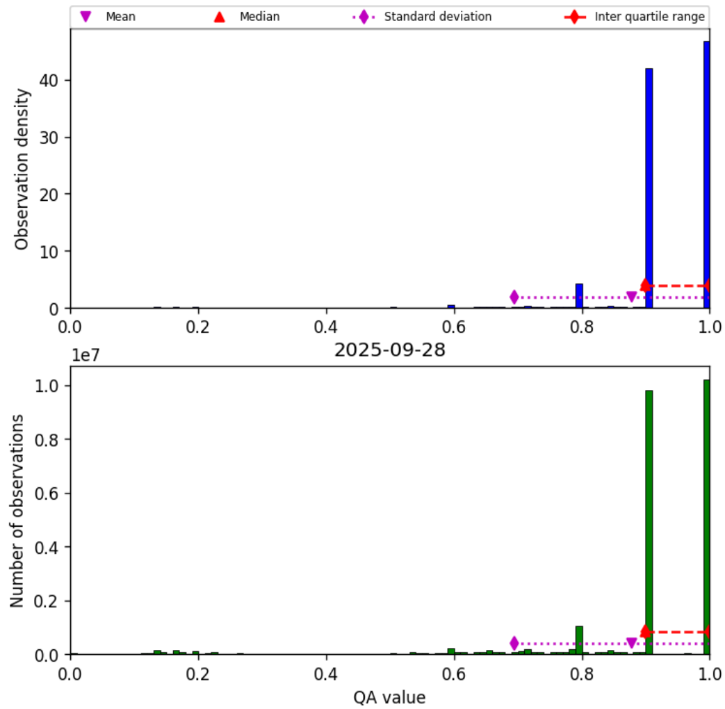
Figure 20: Histogram of “QA value” for 2025-09-27 to 2025-09-29
