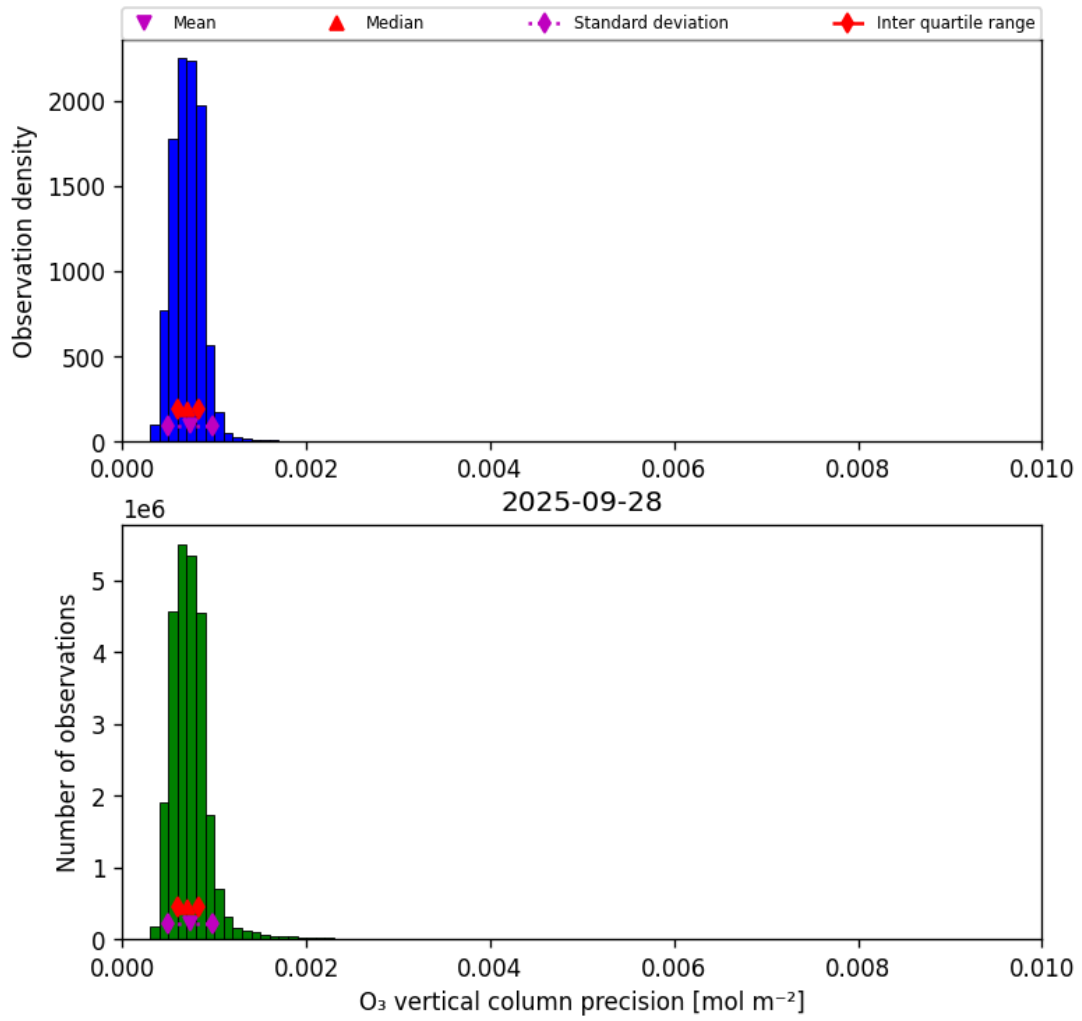
Figure 22: Histogram of “O 3 vertical column precision” for 2025-09-27 to 2025-09-29
