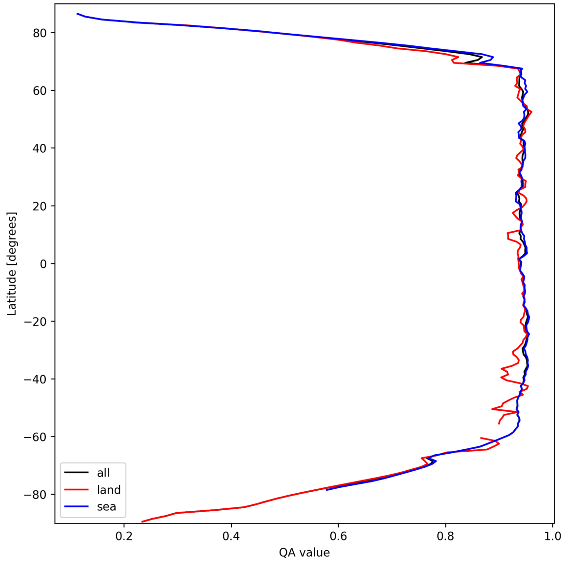
Figure 13: Zonal average of “QA value” for 2025-09-27 to 2025-09-29.
