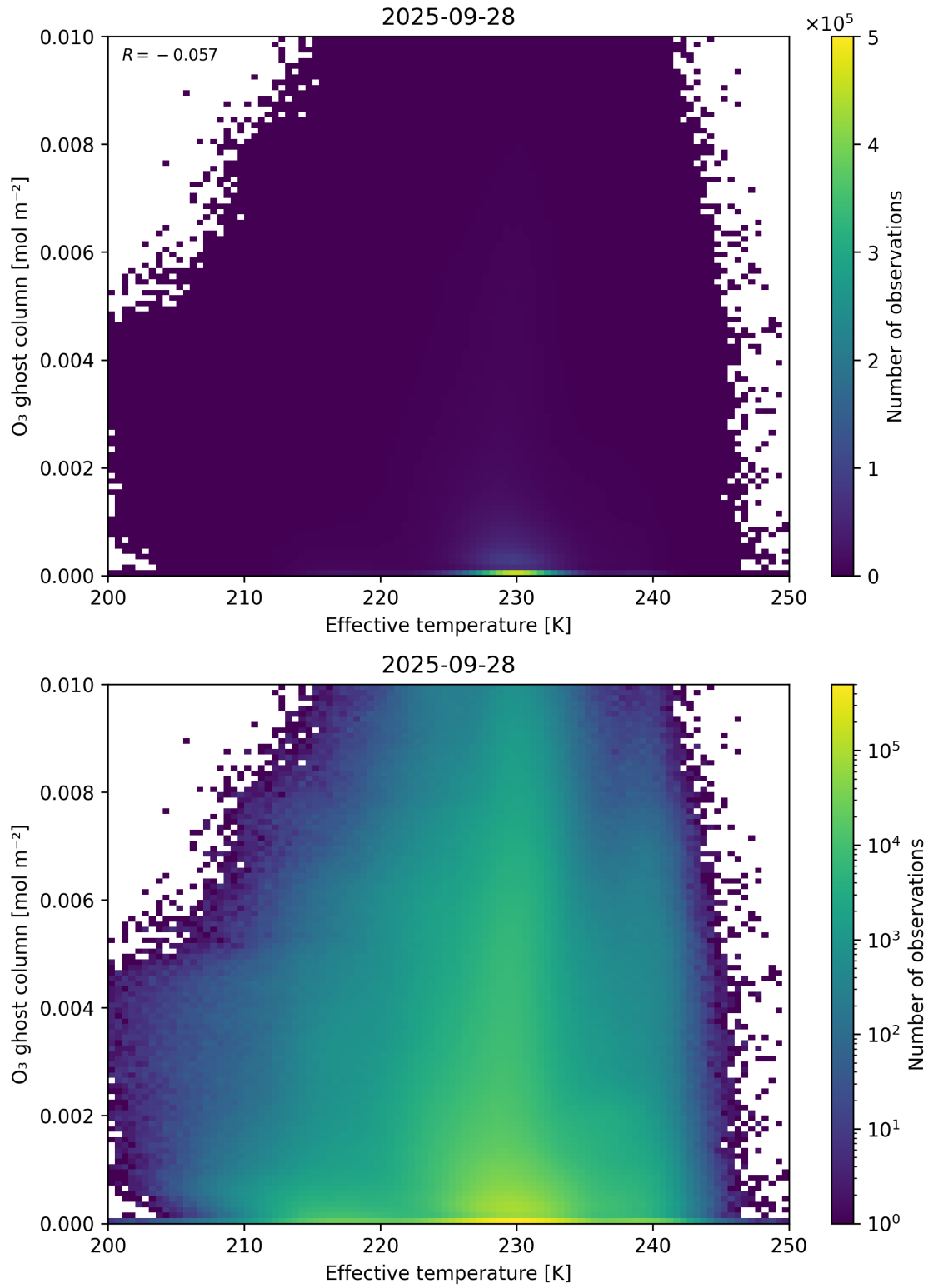
Figure 38: Scatter density plot of “Effective temperature” against “O 3 ghost column” for 2025-09-27 to 2025-09-29.
