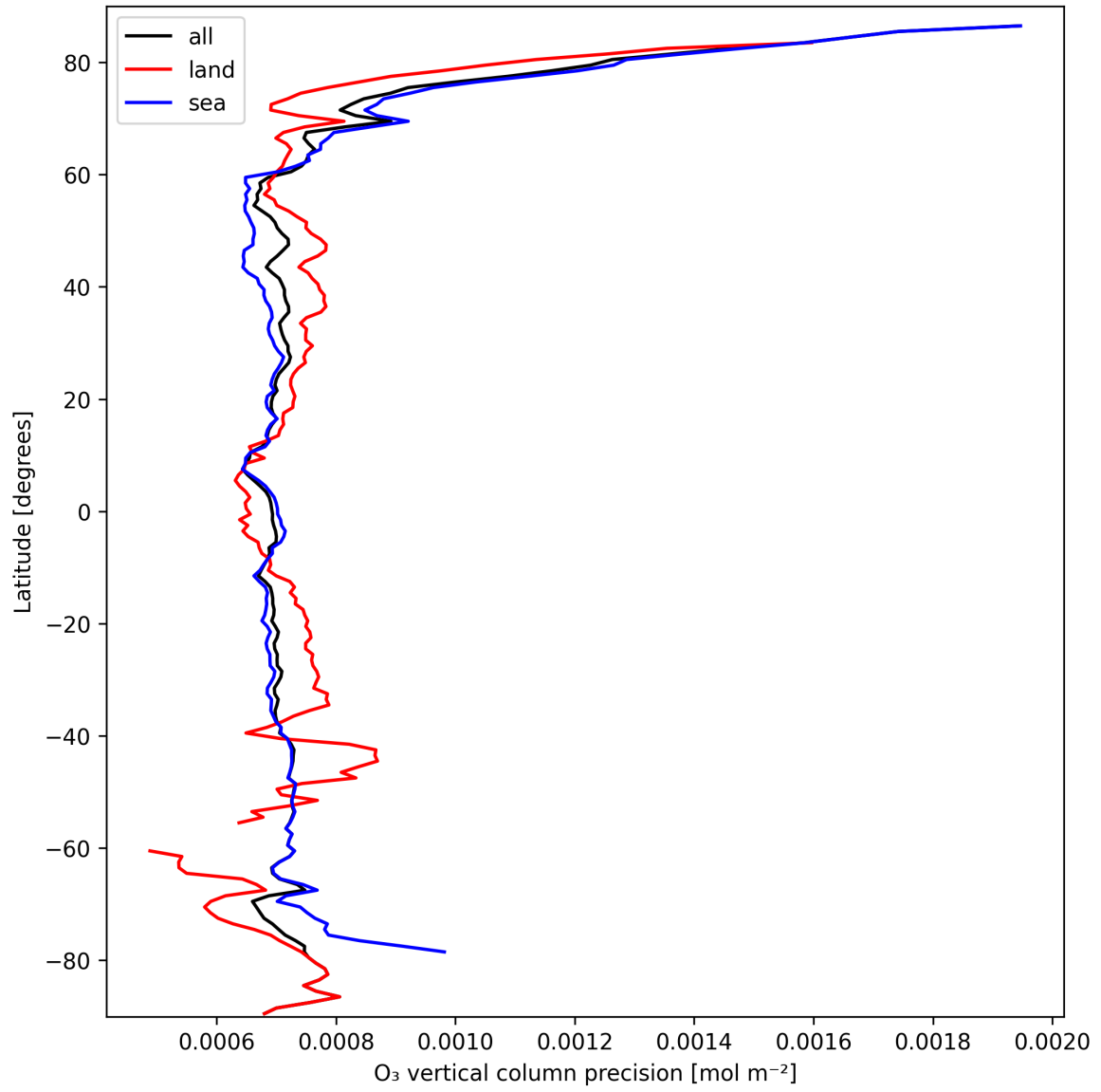
Figure 15: Zonal average of “O 3 vertical column precision” for 2025-09-27 to 2025-09-29.
