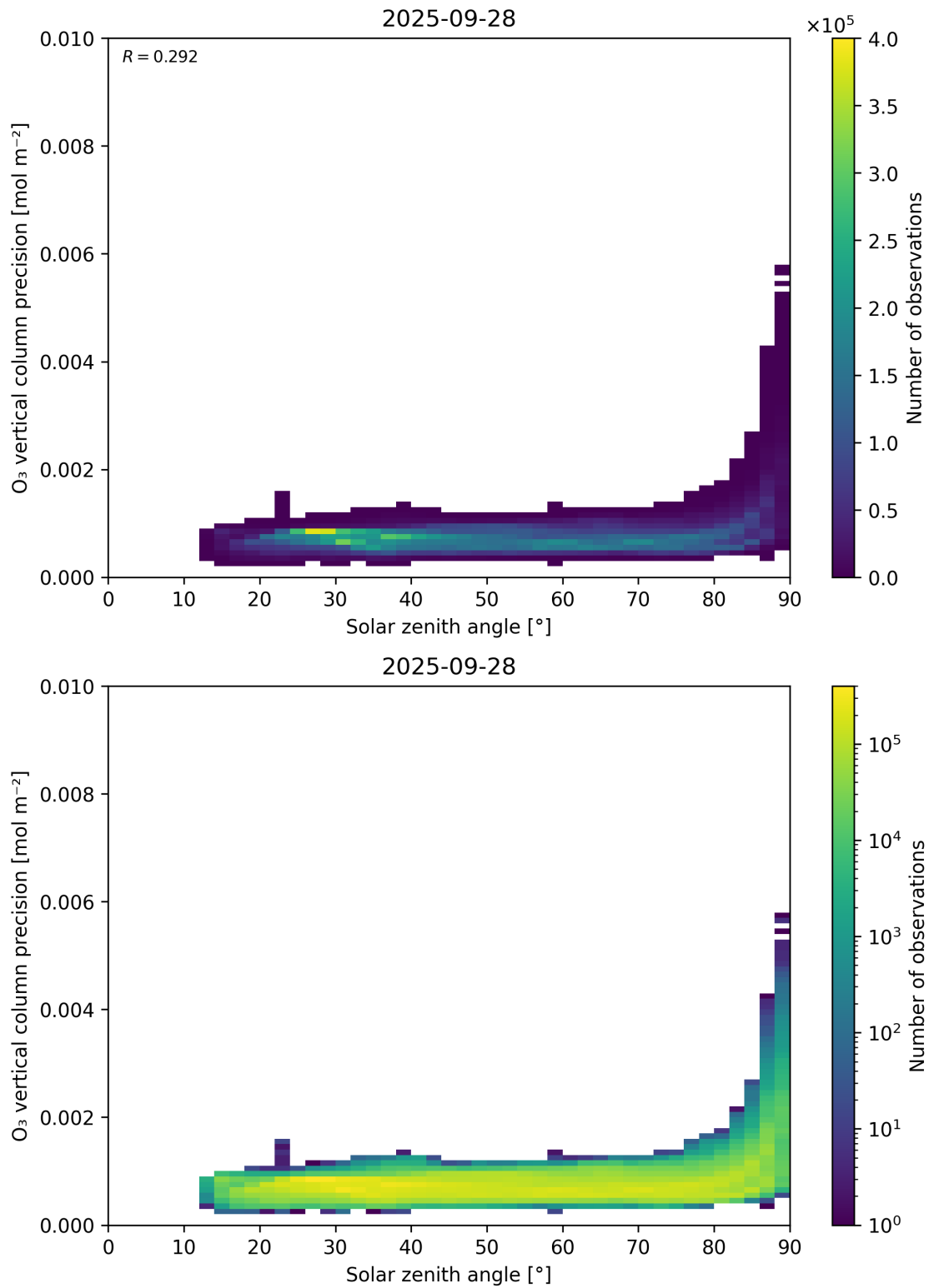
Figure 48: Scatter density plot of “Solar zenith angle” against “O 3 vertical column precision” for 2025-09-27 to 2025-09-29.
