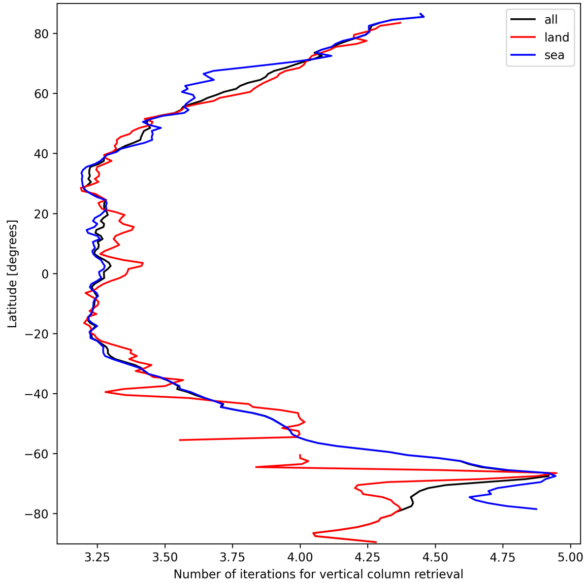
Figure 19: Zonal average of “Number of iterations for vertical column retrieval” for 2025-09-27 to 2025-09-29.
