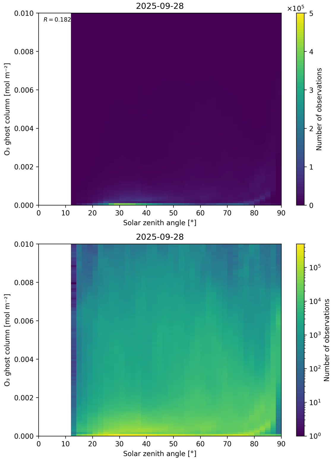
Figure 46: Scatter density plot of “Solar zenith angle” against “O 3 ghost column” for 2025-09-27 to 2025-09-29.
