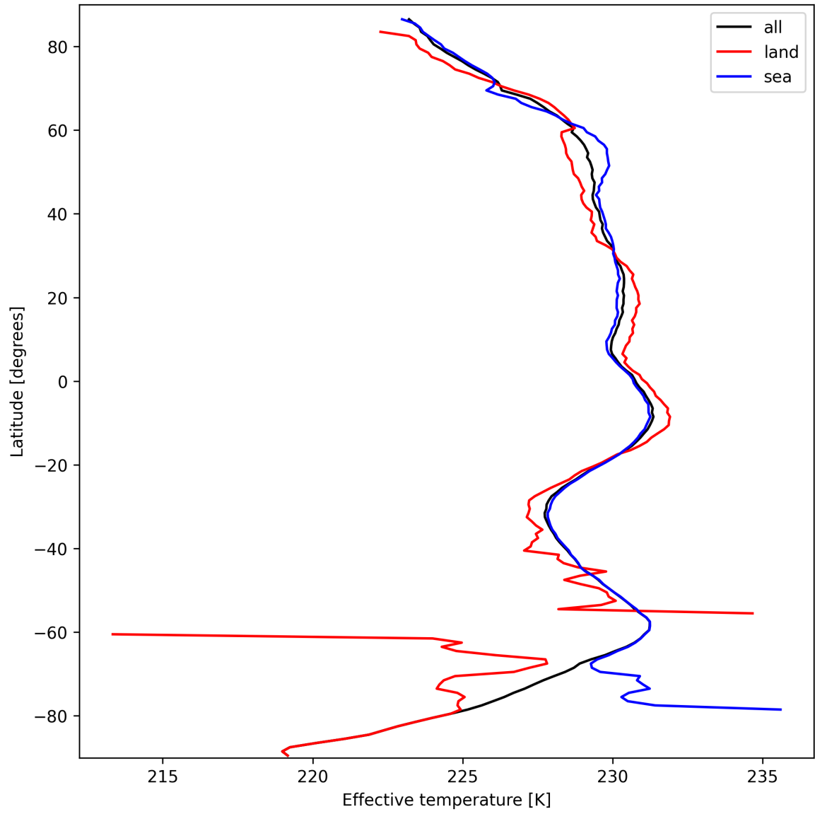
Figure 17: Zonal average of “Effective temperature” for 2025-09-27 to 2025-09-29.
