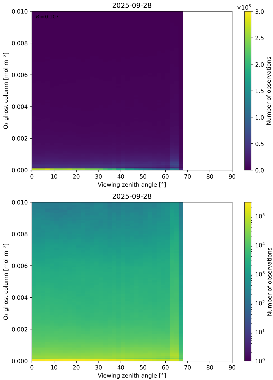
Figure 51: Scatter density plot of “Viewing zenith angle” against “O 3 ghost column” for 2025-09-27 to 2025-09-29.
