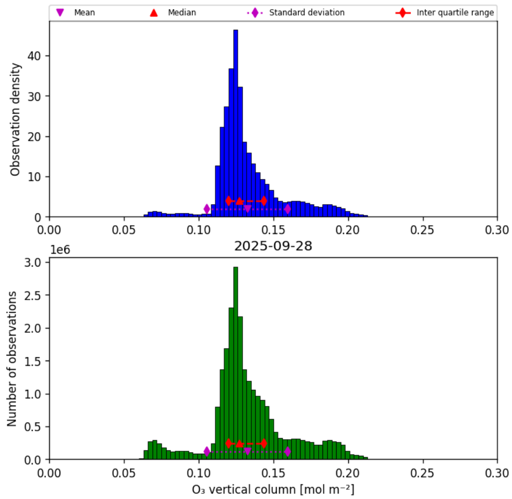
Figure 21: Histogram of “O 3 vertical column” for 2025-09-27 to 2025-09-29
