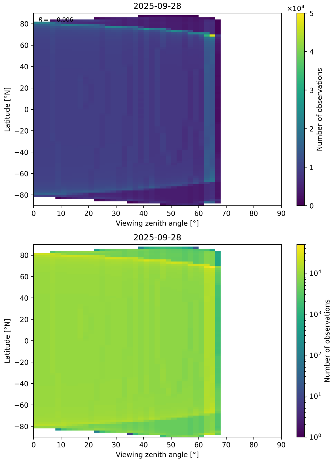
Figure 49: Scatter density plot of “Viewing zenith angle” against “Latitude” for 2025-09-27 to 2025-09-29.
