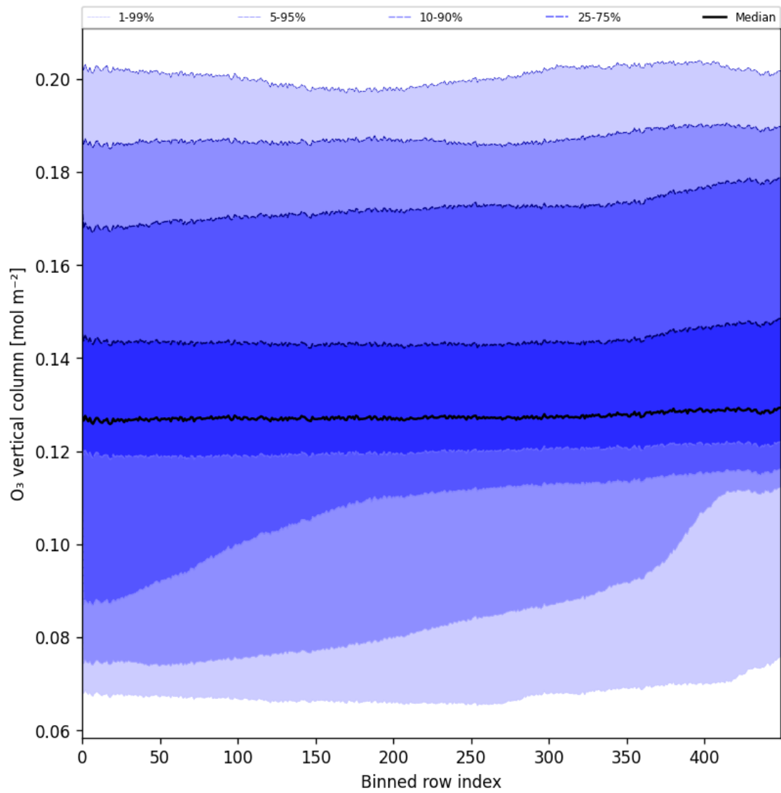
Figure 28: Along track statistics of “O 3 vertical column” for 2025-09-27 to 2025-09-29
