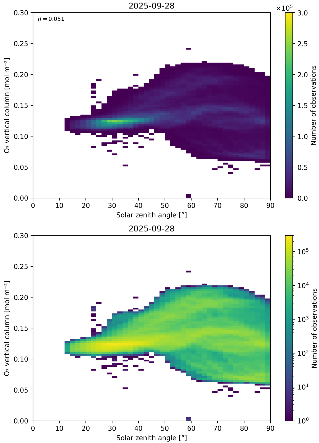
Figure 47: Scatter density plot of “Solar zenith angle” against “O 3 vertical column” for 2025-09-27 to 2025-09-29.
