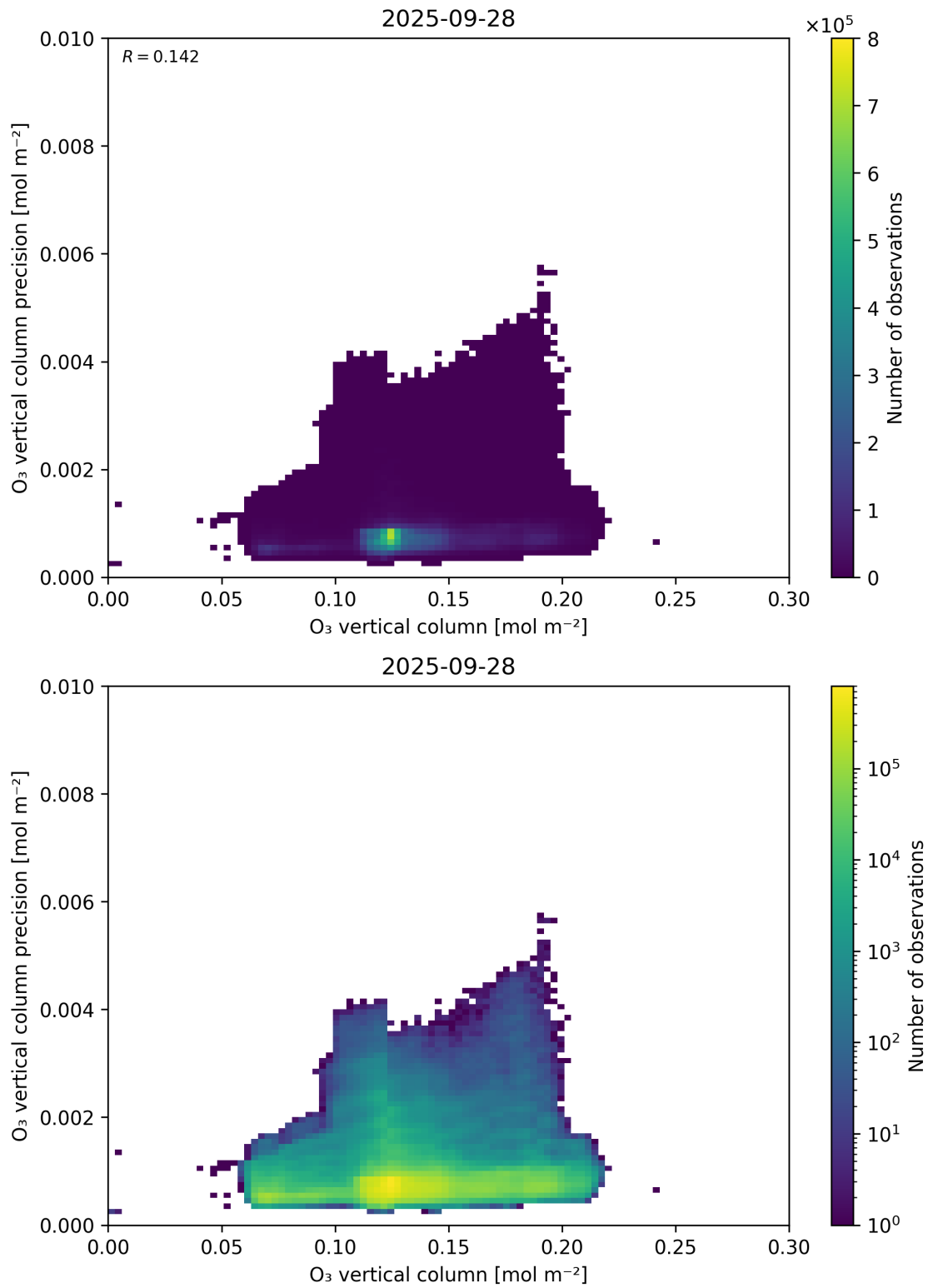
Figure 41: Scatter density plot of “O 3 vertical column” against “O 3 vertical column precision” for 2025-09-27 to 2025-09-29.
