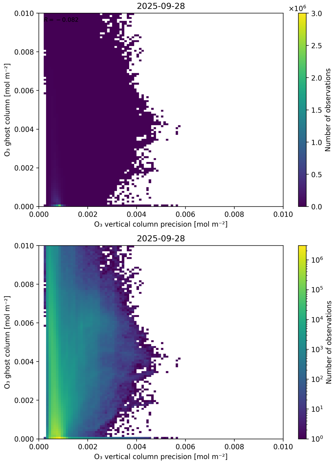
Figure 43: Scatter density plot of “O 3 vertical column precision” against “O 3 ghost column” for 2025-09-27 to 2025-09-29.
