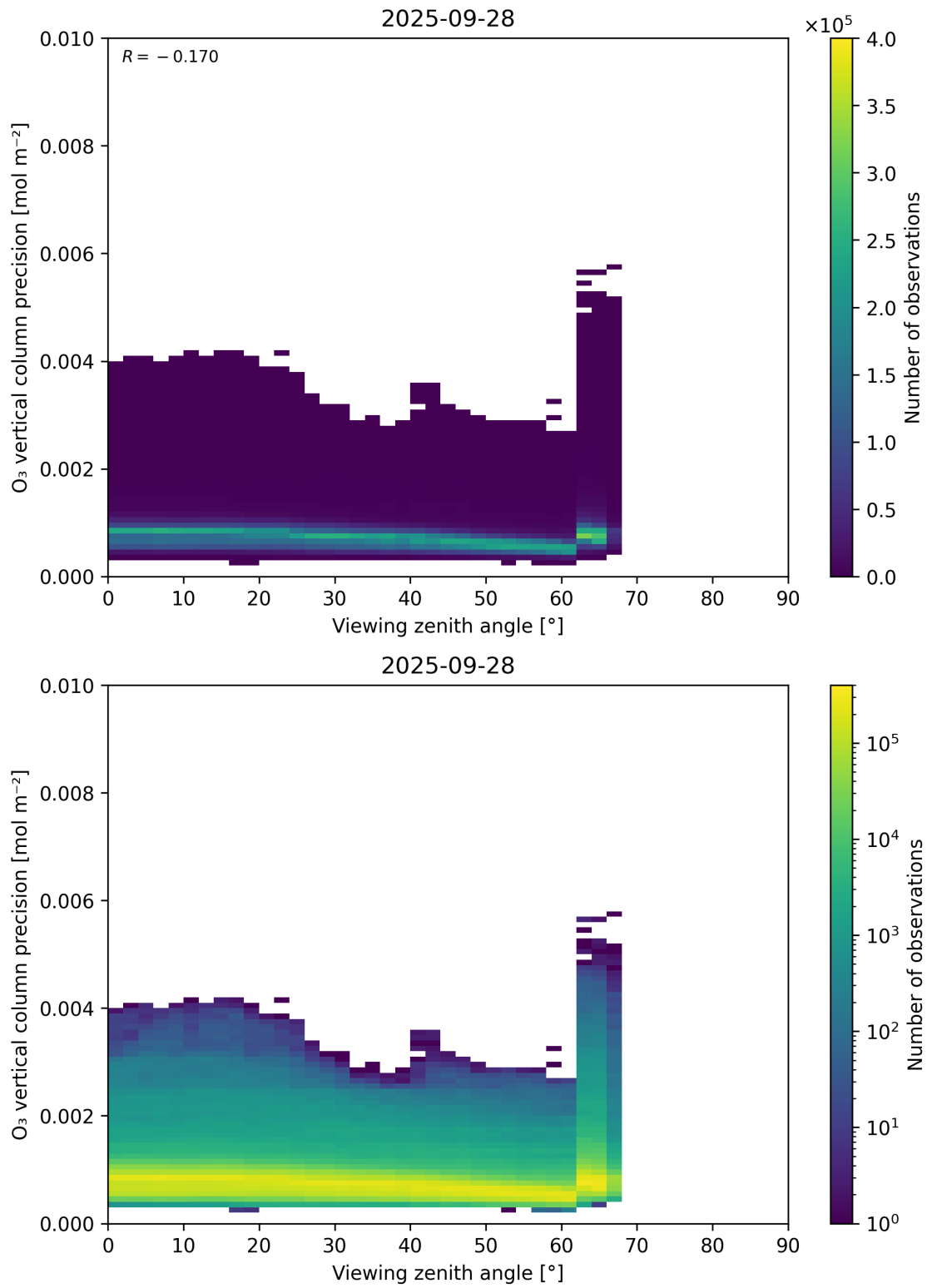
Figure 53: Scatter density plot of “Viewing zenith angle” against “O 3 vertical column precision” for 2025-09-27 to 2025-09-29.
