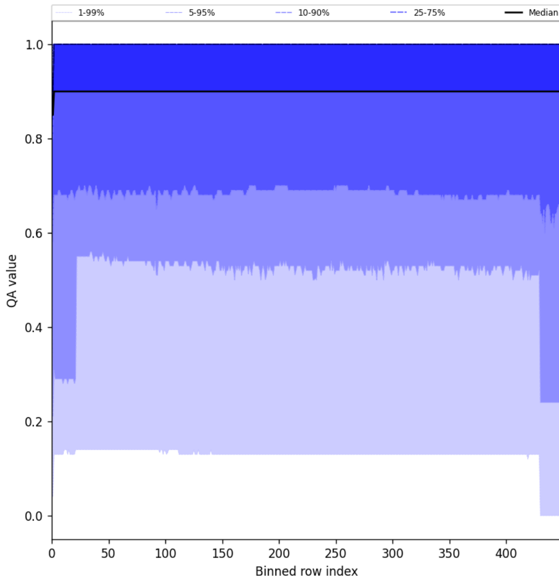
Figure 27: Along track statistics of “QA value” for 2025-09-27 to 2025-09-29
