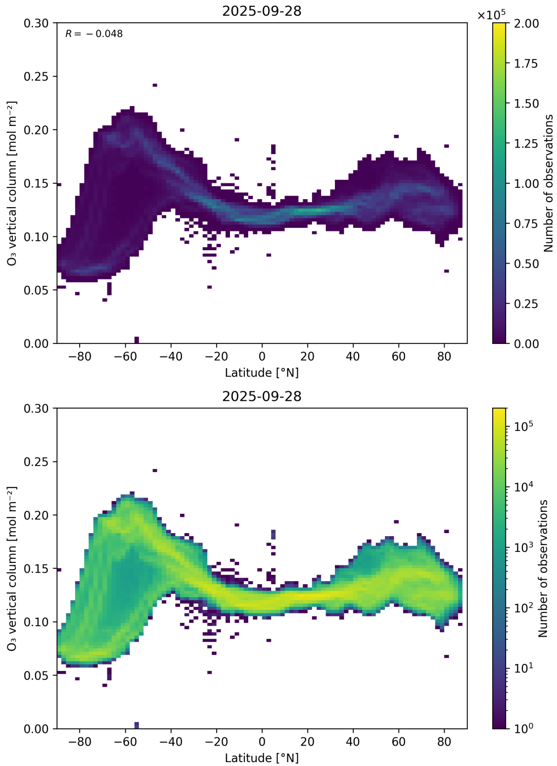
Figure 36: Scatter density plot of “Latitude” against “O 3 vertical column” for 2025-09-27 to 2025-09-29.
