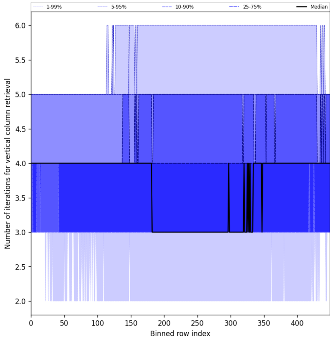
Figure 33: Along track statistics of “Number of iterations for vertical column retrieval” for 2025-09-27 to 2025-09-29
