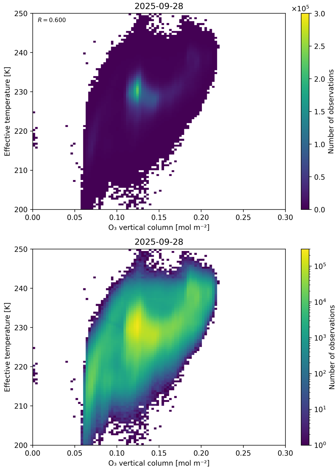
Figure 39: Scatter density plot of “O 3 vertical column” against “Effective temperature” for 2025-09-27 to 2025-09-29.
