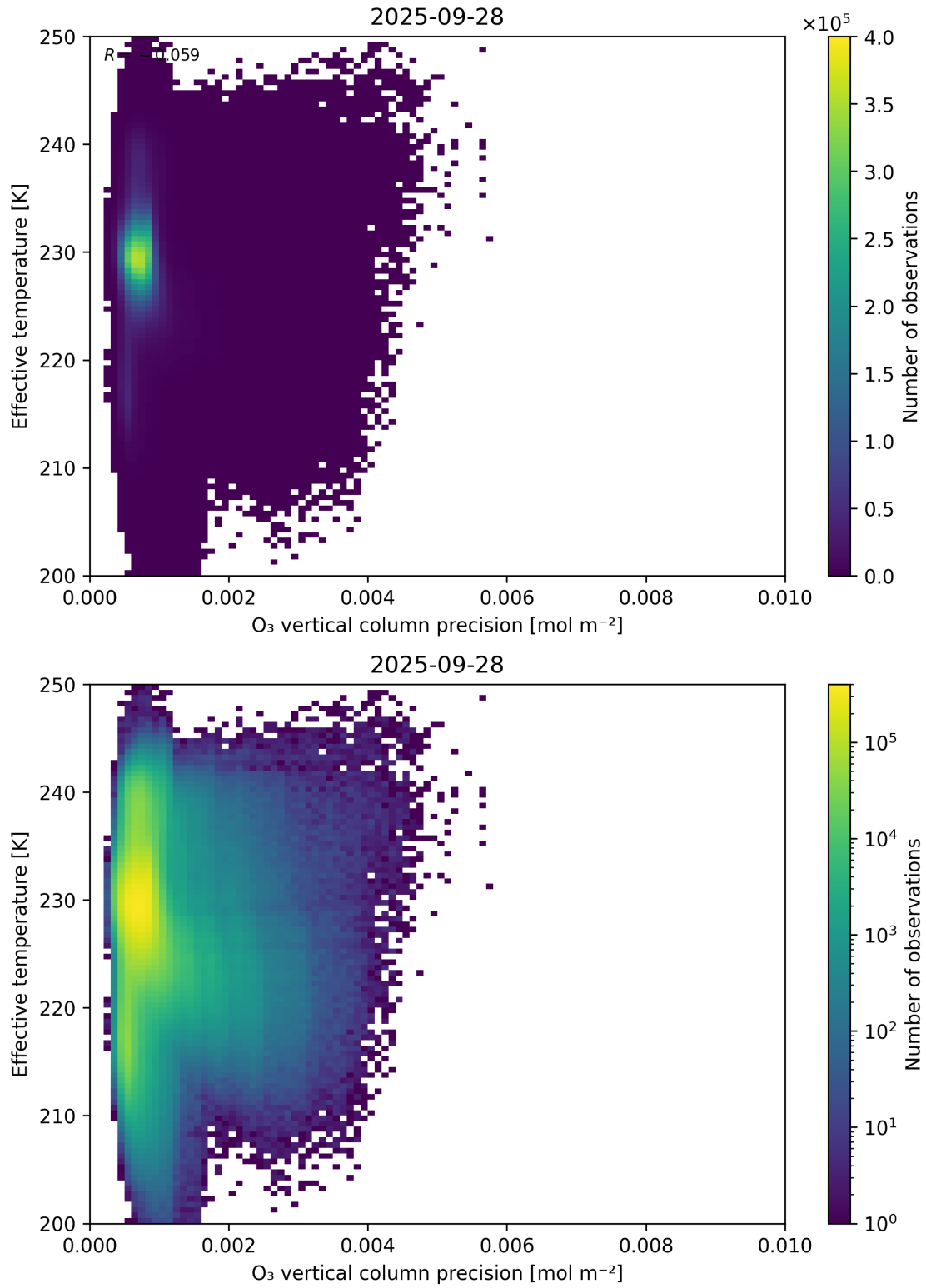
Figure 42: Scatter density plot of “O 3 vertical column precision” against “Effective temperature” for 2025-09-27 to 2025-09-29.
