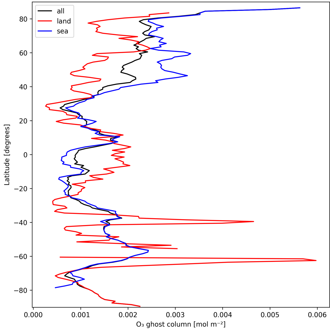
Figure 18: Zonal average of “O 3 ghost column” for 2025-09-27 to 2025-09-29.
