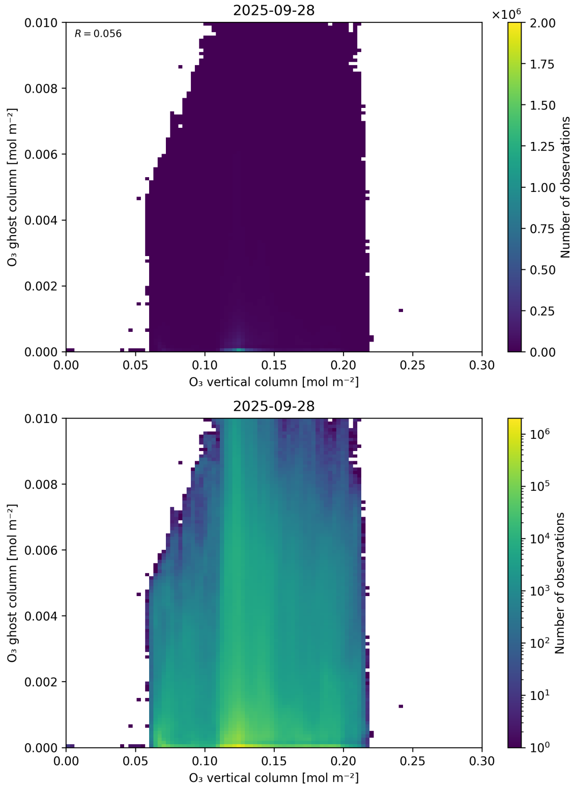
Figure 40: Scatter density plot of “O 3 vertical column” against “O 3 ghost column” for 2025-09-27 to 2025-09-29.
