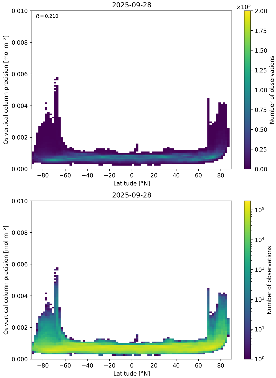
Figure 37: Scatter density plot of “Latitude” against “O 3 vertical column precision” for 2025-09-27 to 2025-09-29.
