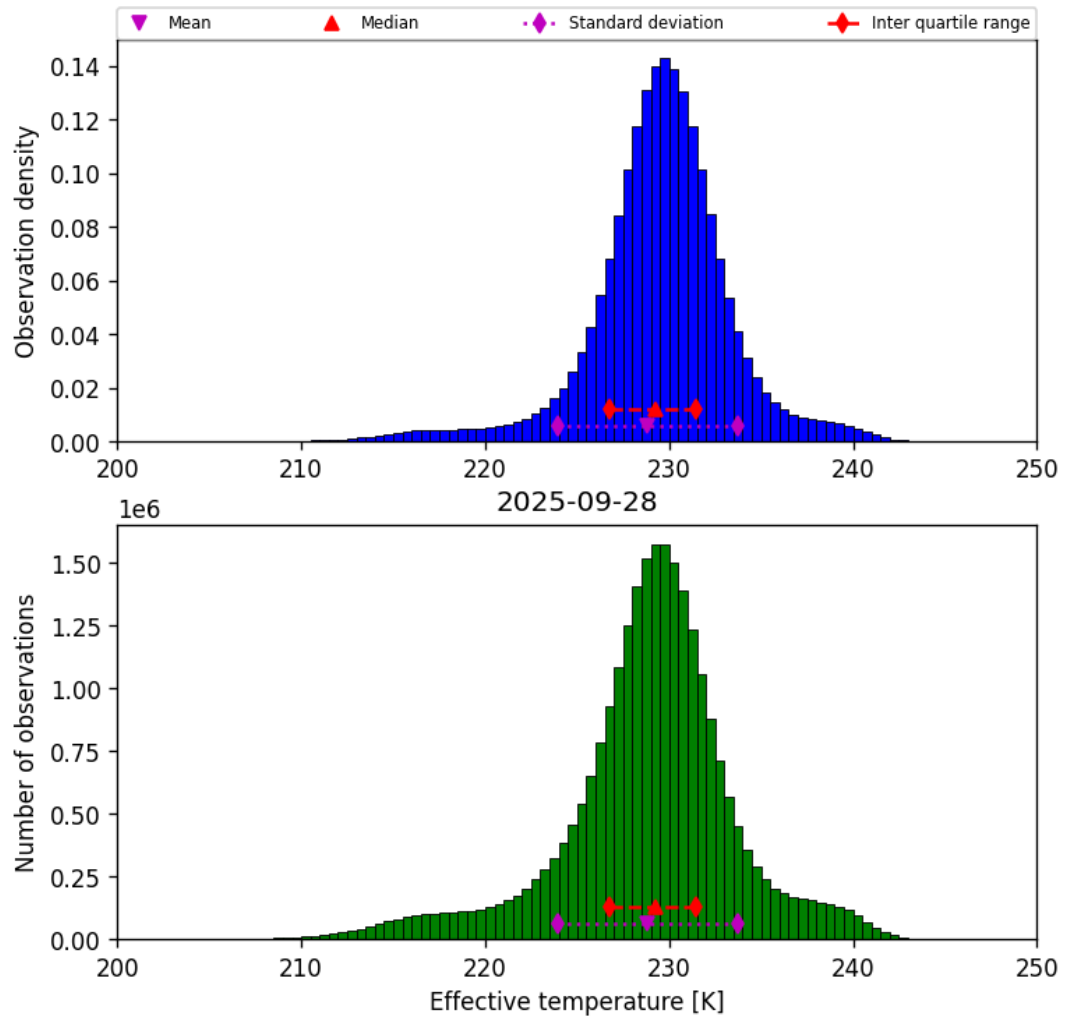
Figure 24: Histogram of “Effective temperature” for 2025-09-27 to 2025-09-29
