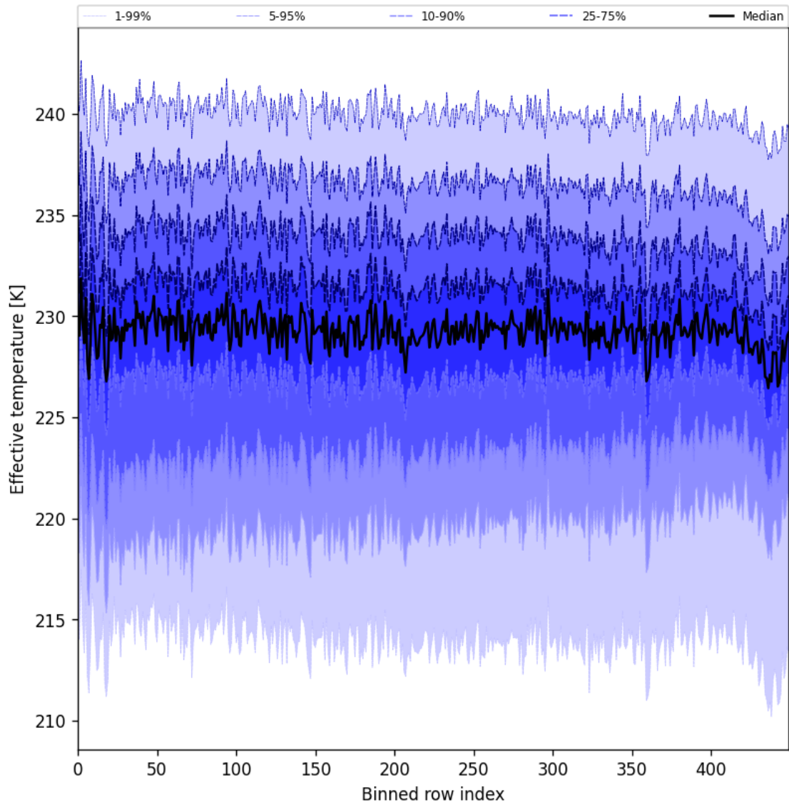
Figure 31: Along track statistics of “Effective temperature” for 2025-09-27 to 2025-09-29
