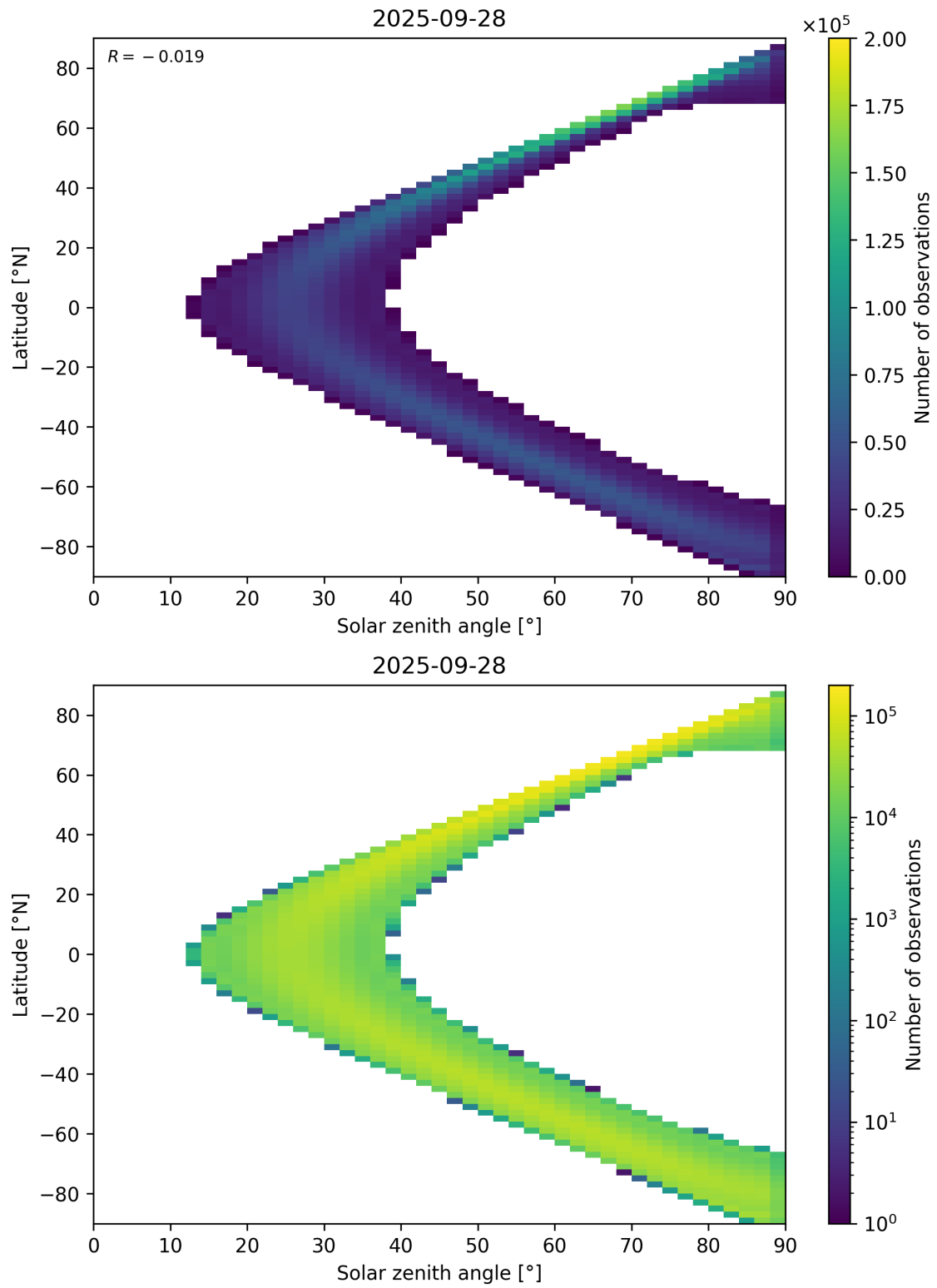
Figure 44: Scatter density plot of “Solar zenith angle” against “Latitude” for 2025-09-27 to 2025-09-29.
