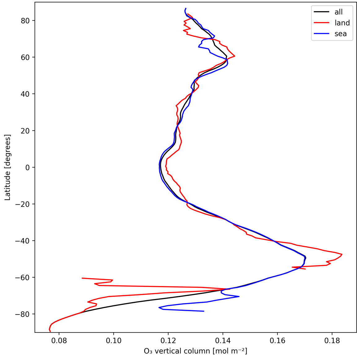
Figure 14: Zonal average of “O 3 vertical column” for 2025-09-27 to 2025-09-29.
