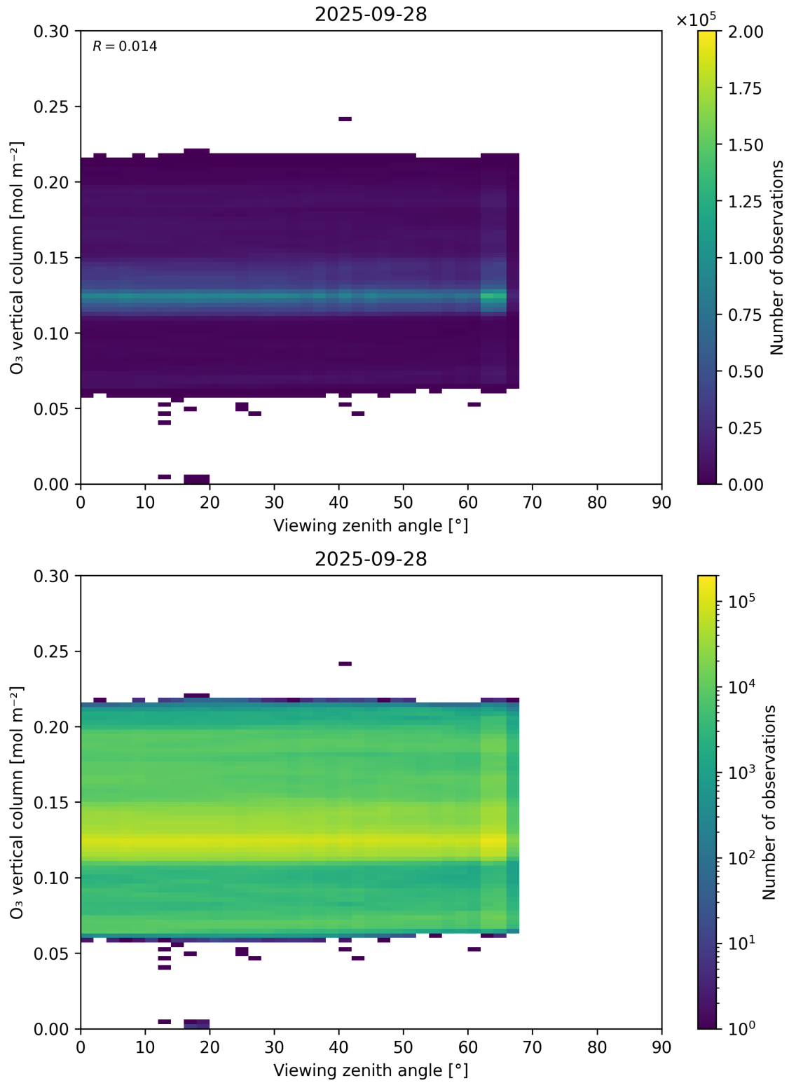
Figure 52: Scatter density plot of “Viewing zenith angle” against “O 3 vertical column” for 2025-09-27 to 2025-09-29.
