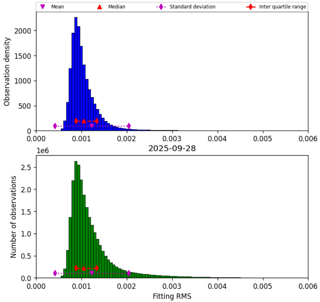
Figure 23: Histogram of “Fitting RMS” for 2025-09-27 to 2025-09-29
