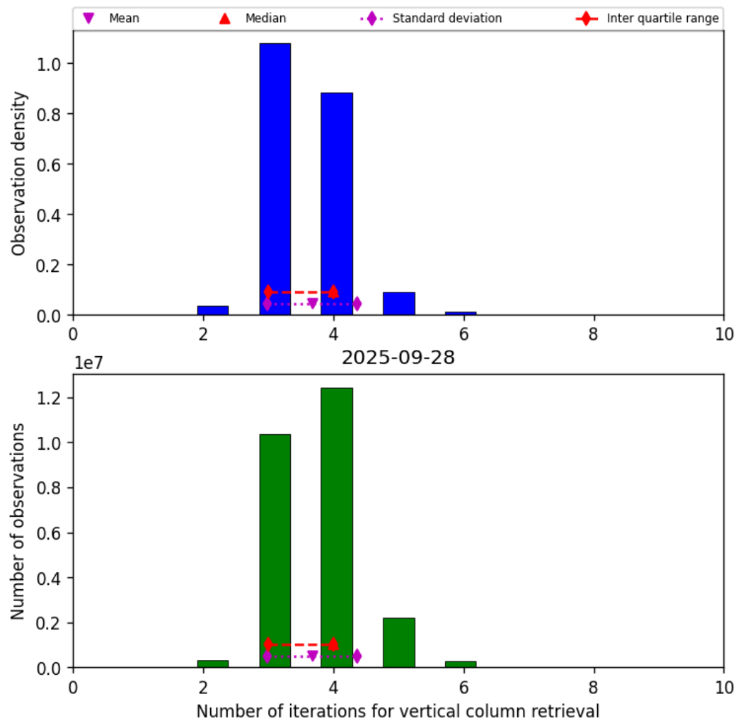
Figure 26: Histogram of “Number of iterations for vertical column retrieval” for 2025-09-27 to 2025-09-29
