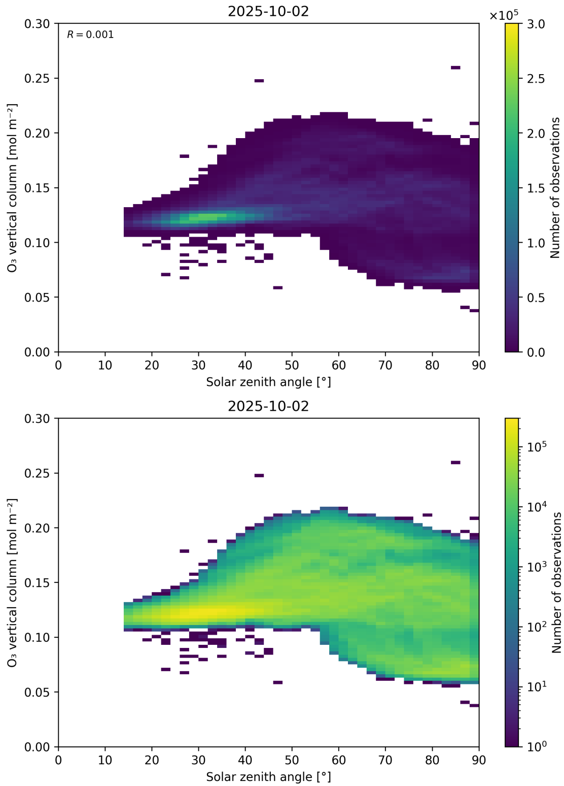
Figure 47: Scatter density plot of “Solar zenith angle” against “O 3 vertical column” for 2025-10-01 to 2025-10-03.
