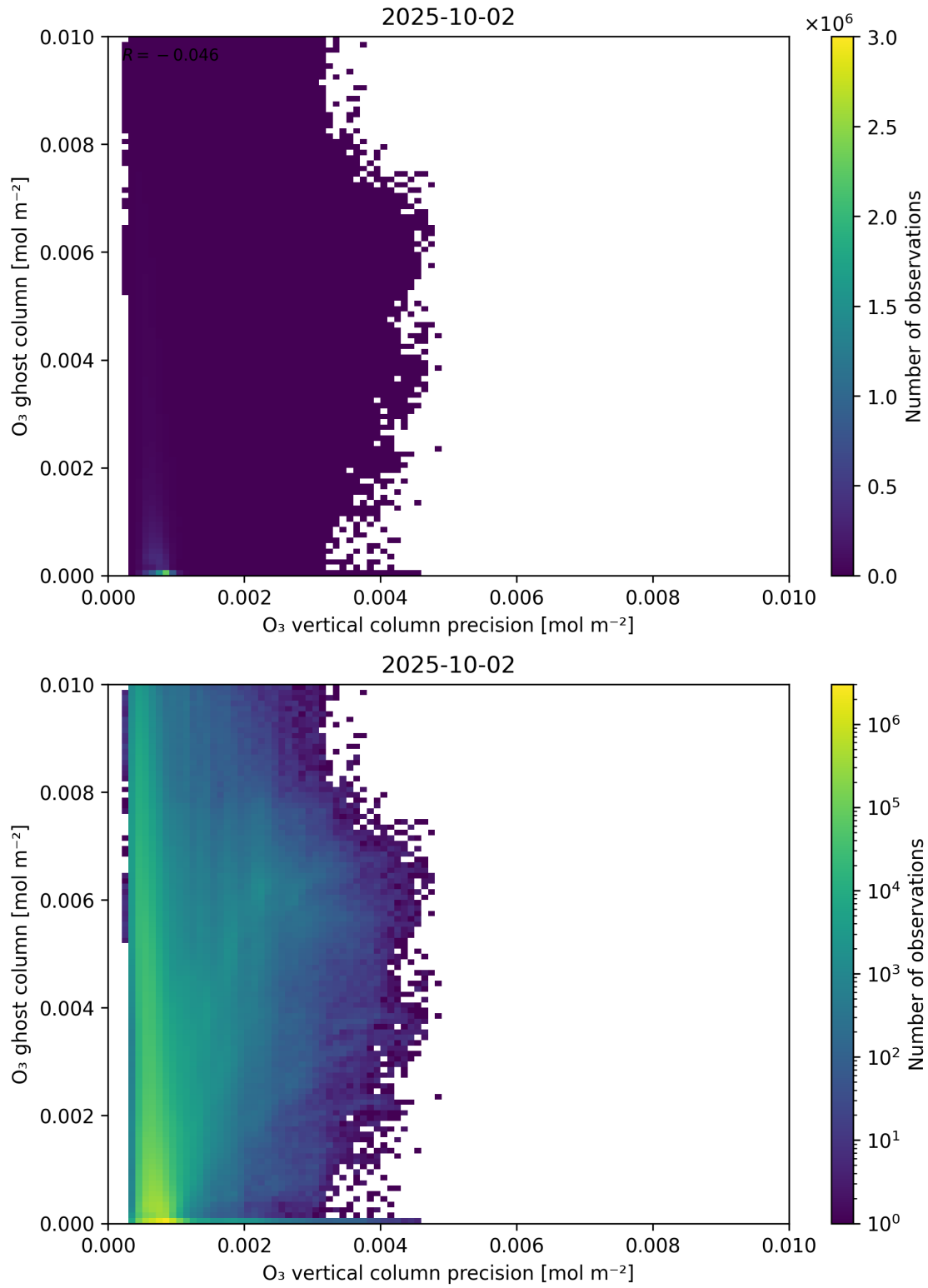
Figure 43: Scatter density plot of “O 3 vertical column precision” against “O 3 ghost column” for 2025-10-01 to 2025-10-03.
