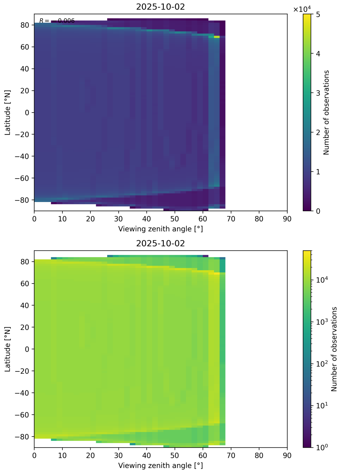
Figure 49: Scatter density plot of “Viewing zenith angle” against “Latitude” for 2025-10-01 to 2025-10-03.
