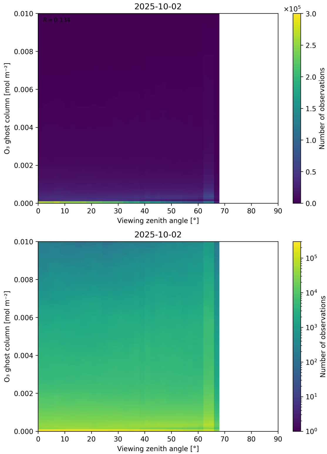
Figure 51: Scatter density plot of “Viewing zenith angle” against “O 3 ghost column” for 2025-10-01 to 2025-10-03.
