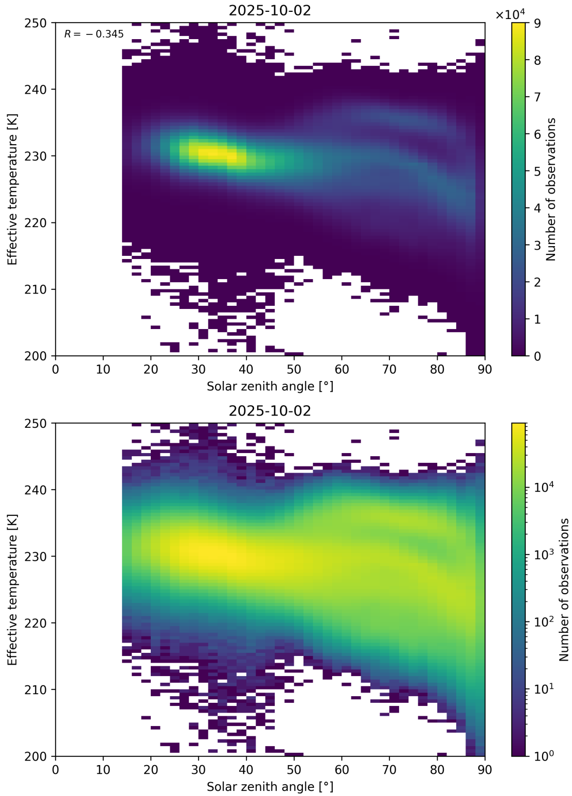
Figure 45: Scatter density plot of “Solar zenith angle” against “Effective temperature” for 2025-10-01 to 2025-10-03.
