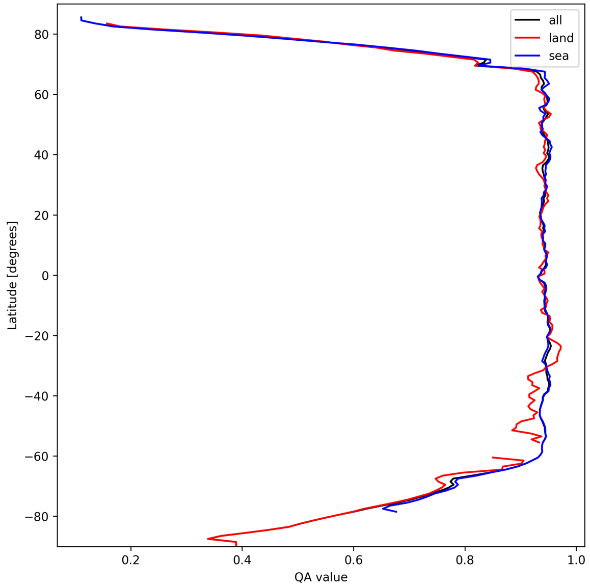
Figure 13: Zonal average of “QA value” for 2025-10-01 to 2025-10-03.
