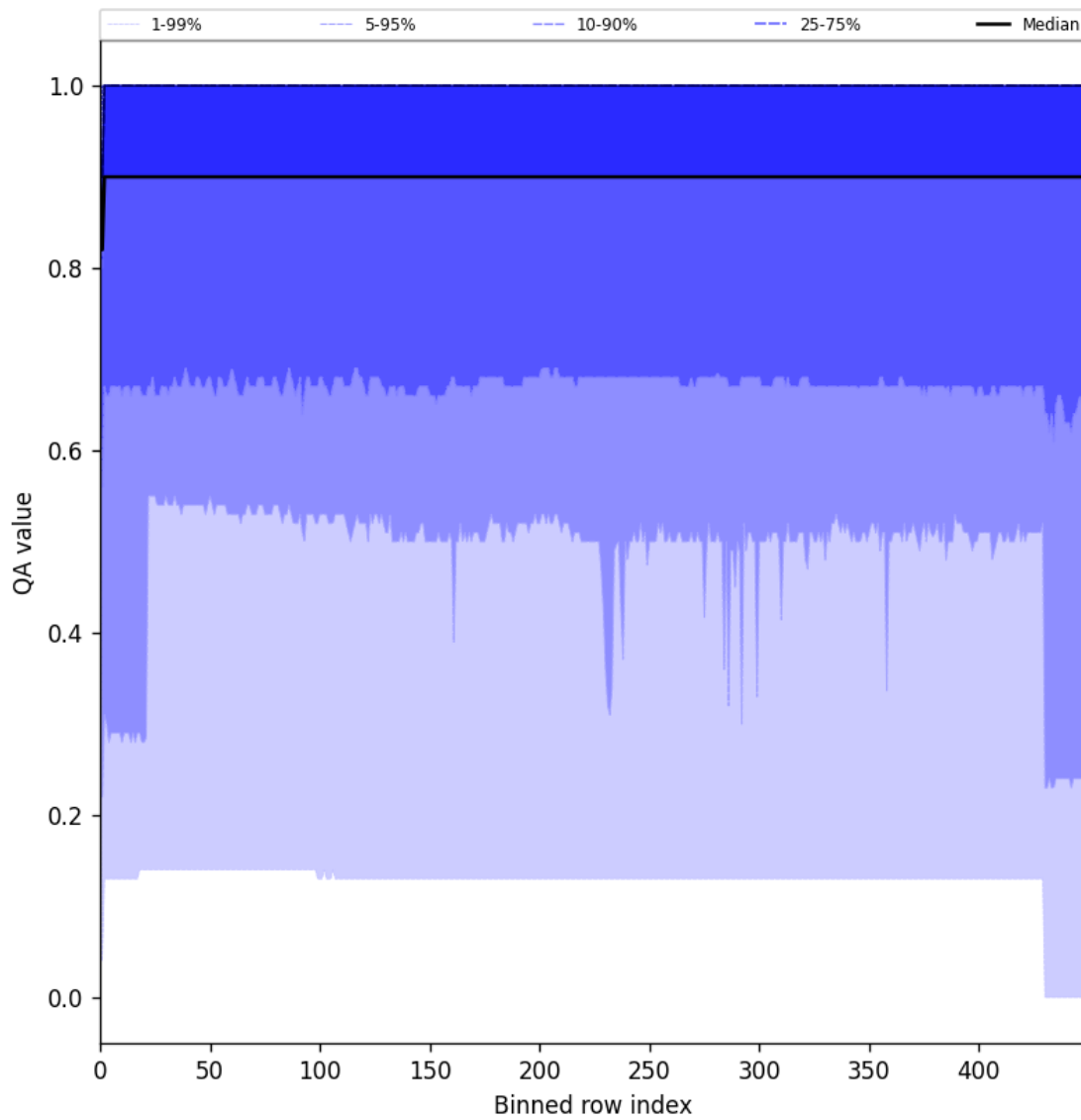
Figure 27: Along track statistics of “QA value” for 2025-10-01 to 2025-10-03
