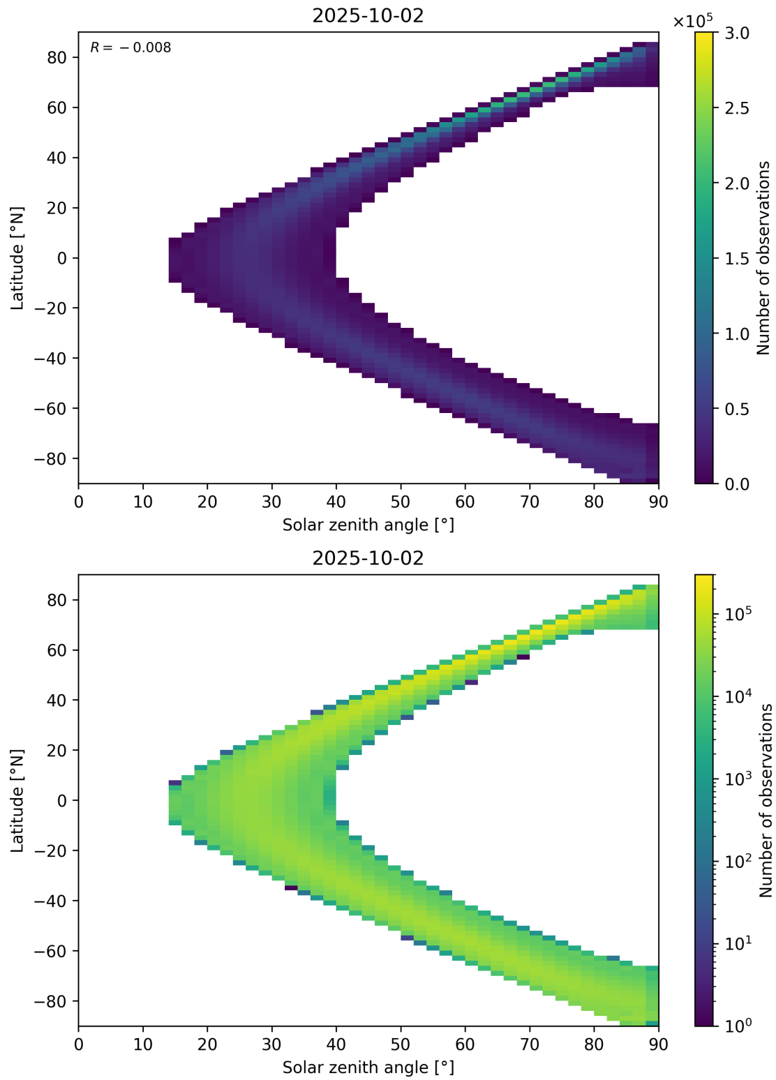
Figure 44: Scatter density plot of “Solar zenith angle” against “Latitude” for 2025-10-01 to 2025-10-03.
