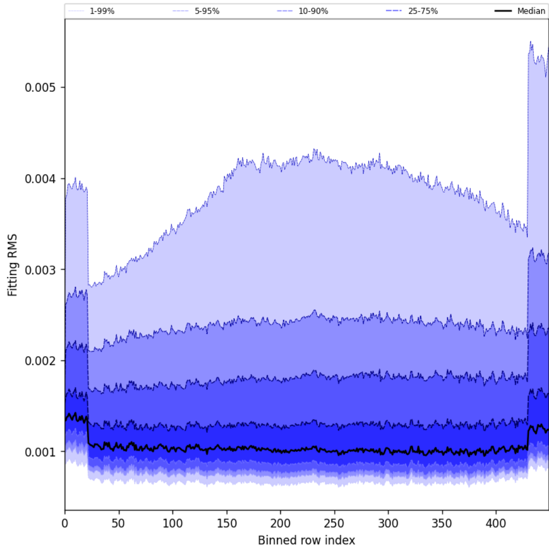
Figure 30: Along track statistics of “Fitting RMS” for 2025-10-01 to 2025-10-03
