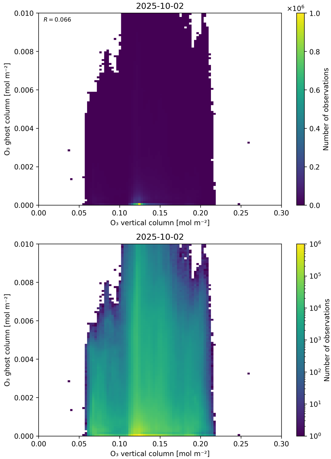
Figure 40: Scatter density plot of “ \text{O}_3 vertical column” against “ \text{O}_3 ghost column” for 2025-10-01 to 2025-10-03.
