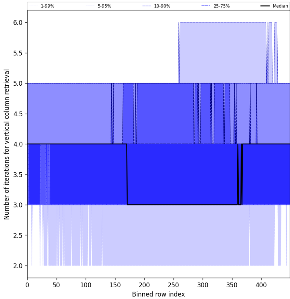
Figure 33: Along track statistics of “Number of iterations for vertical column retrieval” for 2025-10-01 to 2025-10-03
