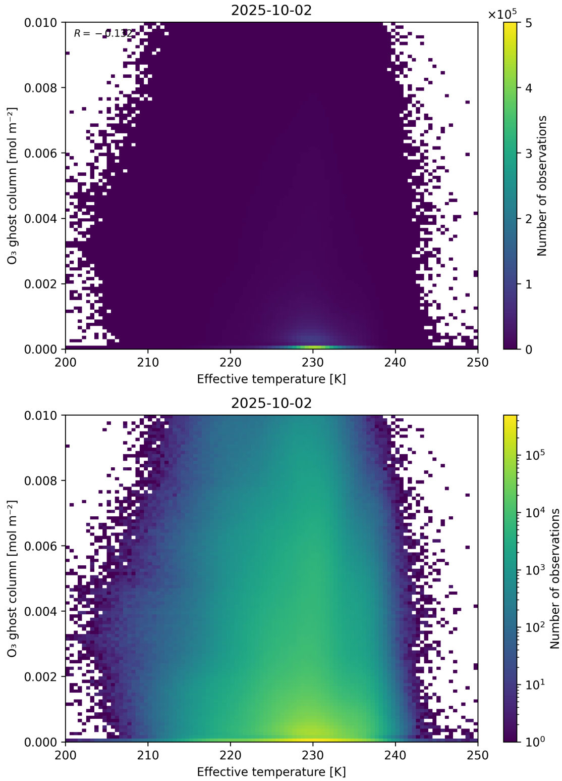
Figure 38: Scatter density plot of “Effective temperature” against “O 3 ghost column” for 2025-10-01 to 2025-10-03.
