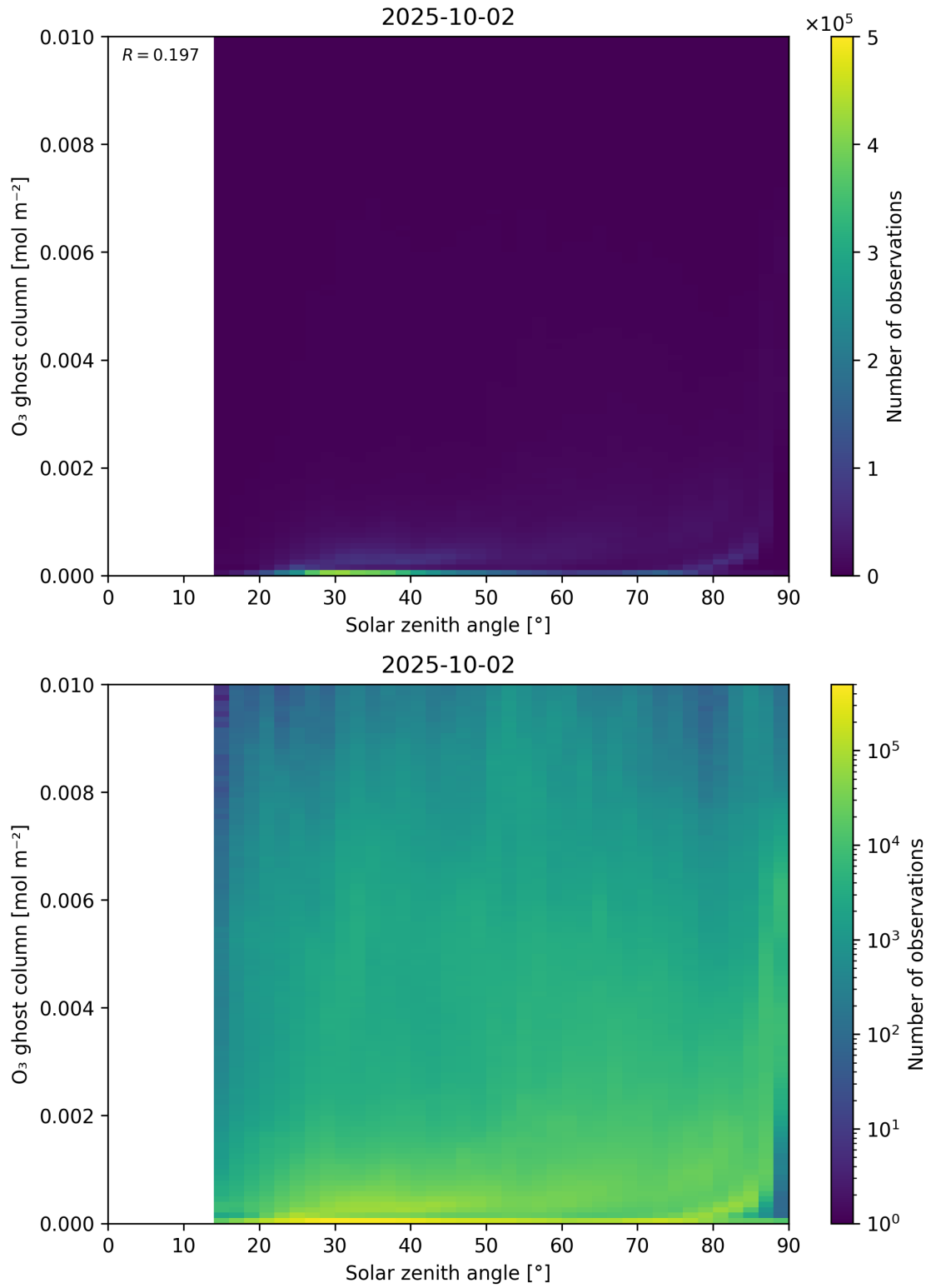
Figure 46: Scatter density plot of “Solar zenith angle” against “O 3 ghost column” for 2025-10-01 to 2025-10-03.
