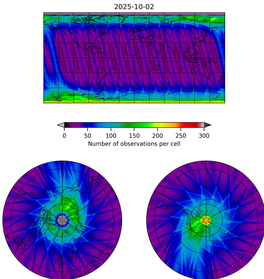
Figure 12: Map of the number of observations for 2025-10-01 to 2025-10-03
