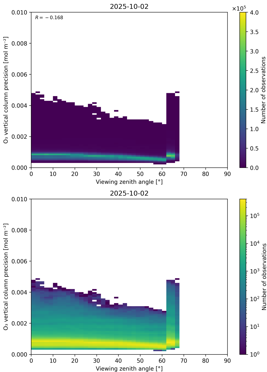
Figure 53: Scatter density plot of “Viewing zenith angle” against “O 3 vertical column precision” for 2025-10-01 to 2025-10-03.
