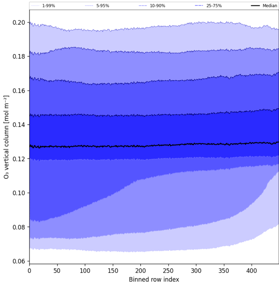
Figure 28: Along track statistics of “O 3 vertical column” for 2025-10-01 to 2025-10-03
