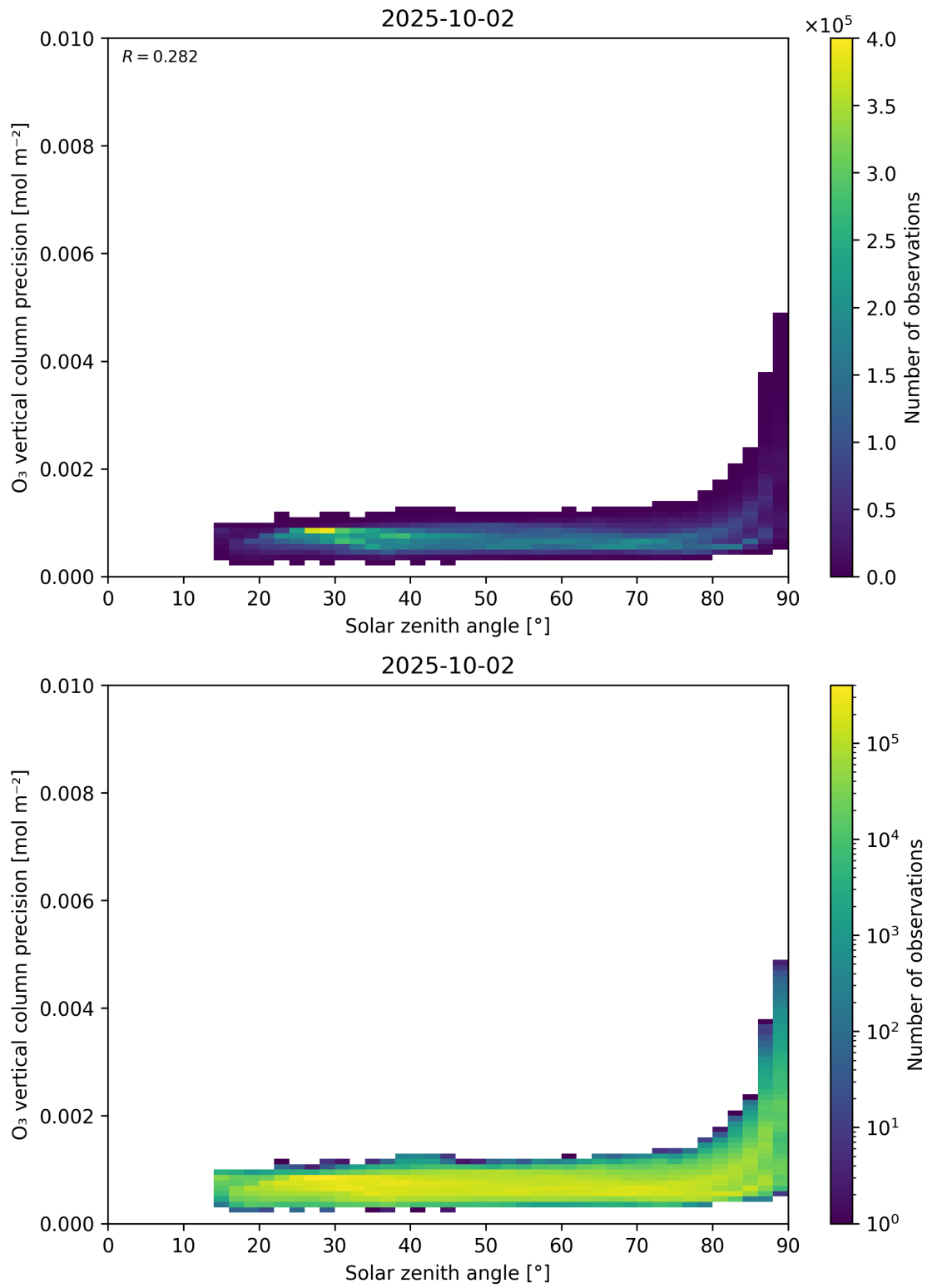
Figure 48: Scatter density plot of “Solar zenith angle” against “O 3 vertical column precision” for 2025-10-01 to 2025-10-03.
