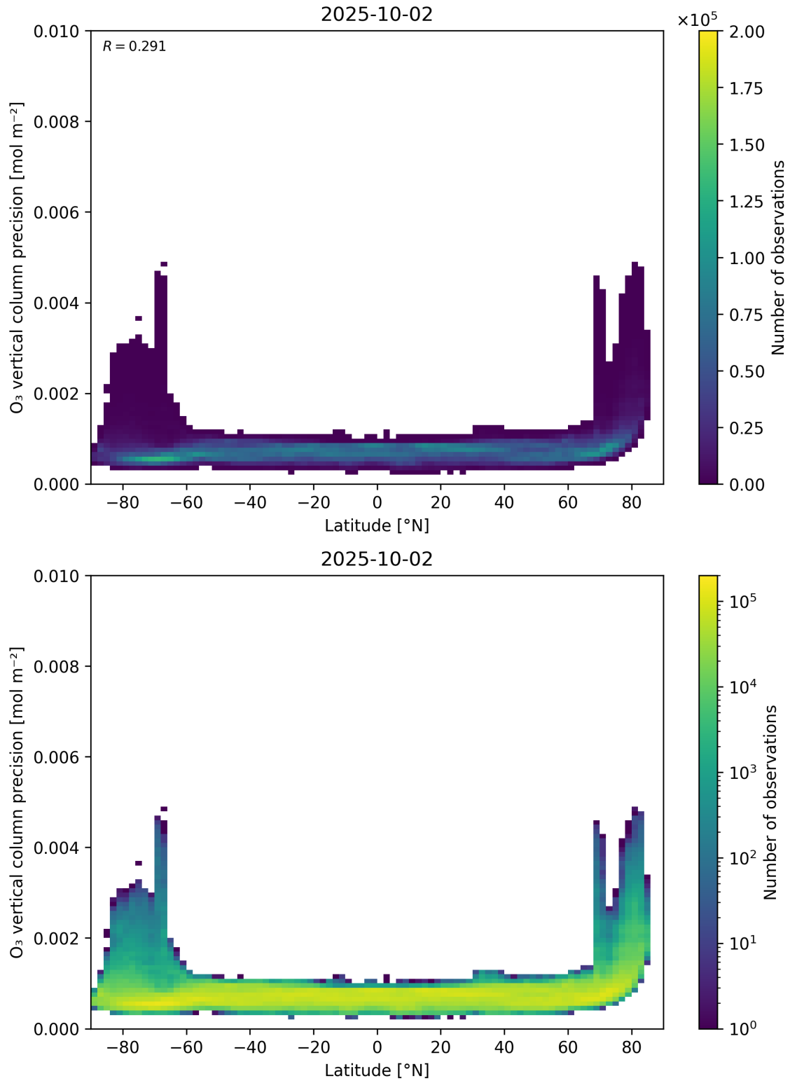
Figure 37: Scatter density plot of “Latitude” against “O 3 vertical column precision” for 2025-10-01 to 2025-10-03.
