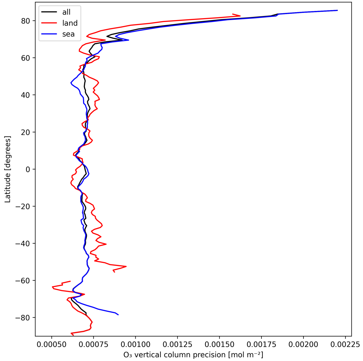
Figure 15: Zonal average of “O 3 vertical column precision” for 2025-10-01 to 2025-10-03.
