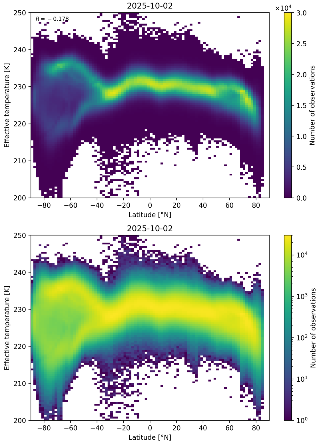
Figure 34: Scatter density plot of “Latitude” against “Effective temperature” for 2025-10-01 to 2025-10-03.
