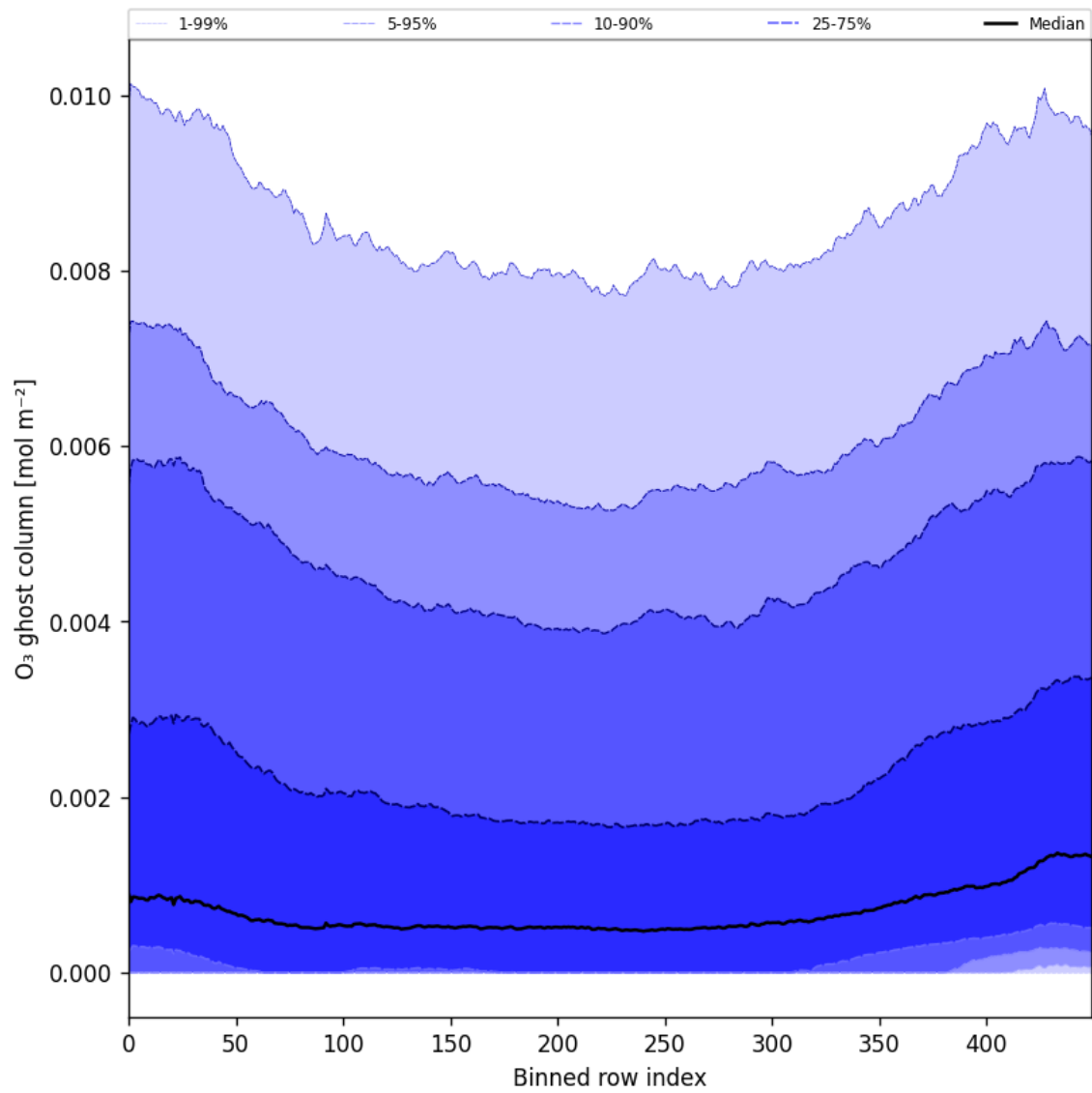
Figure 32: Along track statistics of “O 3 ghost column” for 2025-10-01 to 2025-10-03
