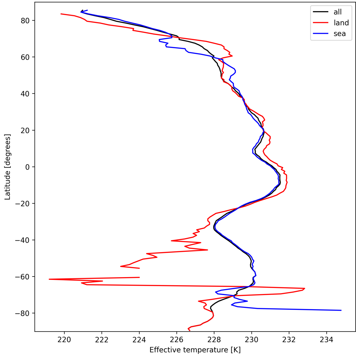
Figure 17: Zonal average of “Effective temperature” for 2025-10-01 to 2025-10-03.
