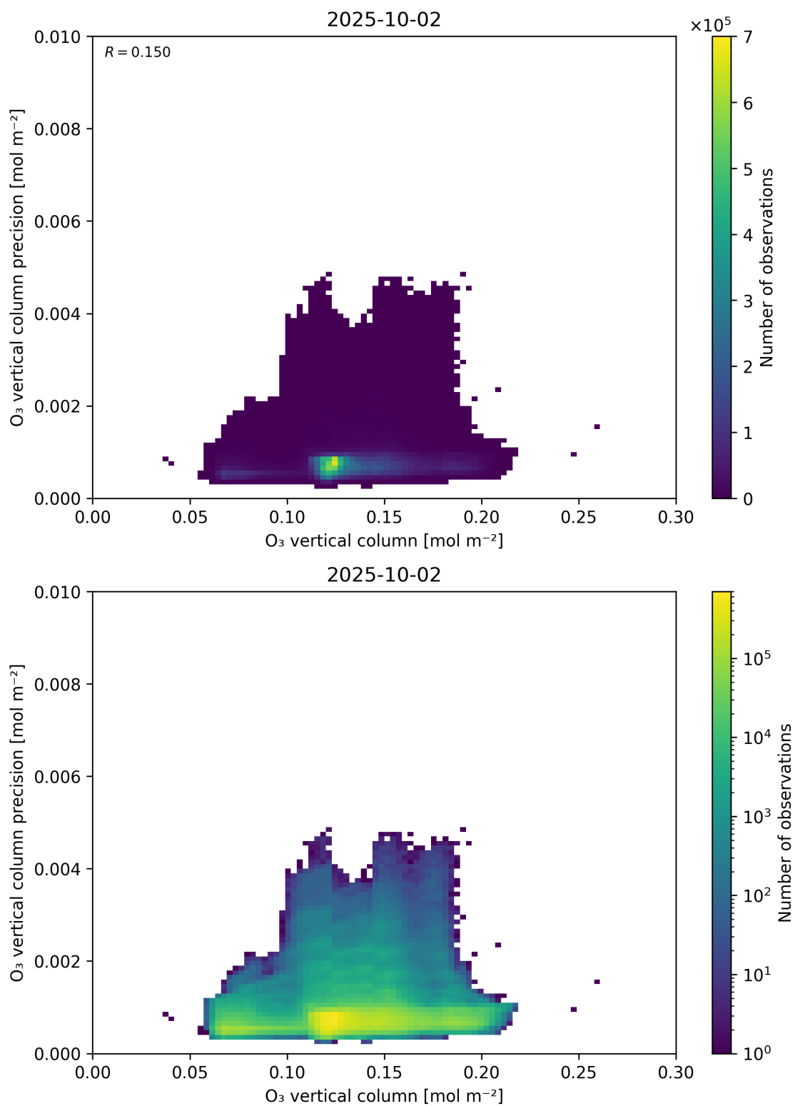
Figure 41: Scatter density plot of “O 3 vertical column” against “O 3 vertical column precision” for 2025-10-01 to 2025-10-03.
