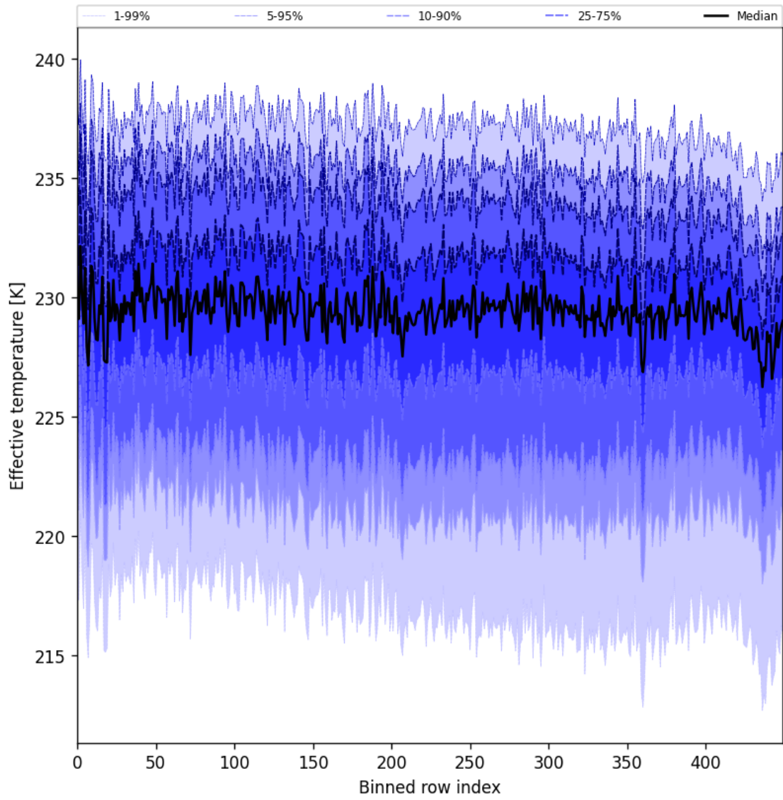
Figure 31: Along track statistics of “Effective temperature” for 2025-10-01 to 2025-10-03
