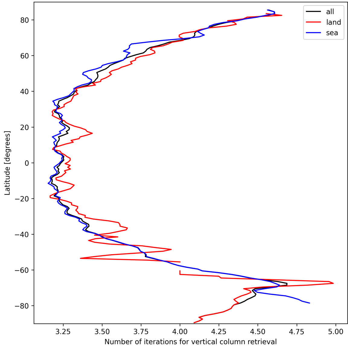
Figure 19: Zonal average of “Number of iterations for vertical column retrieval” for 2025-10-01 to 2025-10-03.
