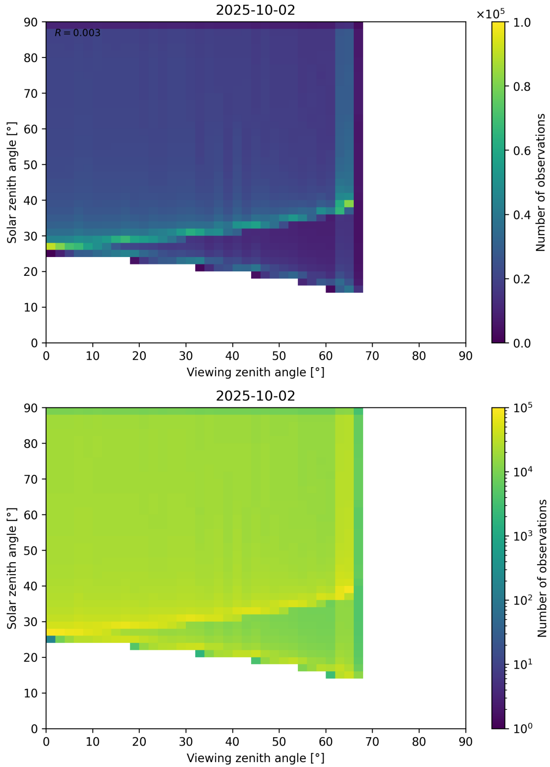
Figure 54: Scatter density plot of “Viewing zenith angle” against “Solar zenith angle” for 2025-10-01 to 2025-10-03.
