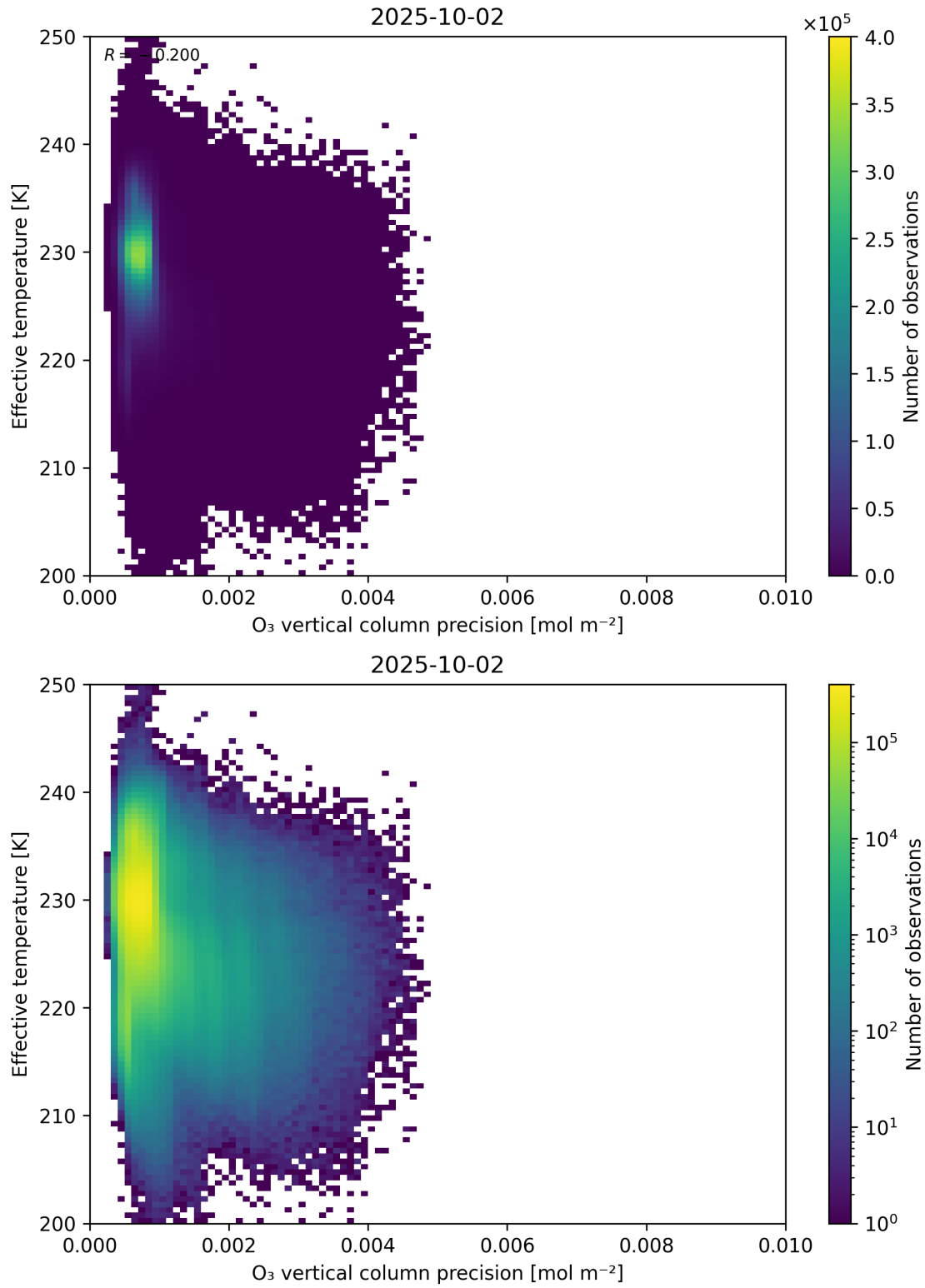
Figure 42: Scatter density plot of “O 3 vertical column precision” against “Effective temperature” for 2025-10-01 to 2025-10-03.
