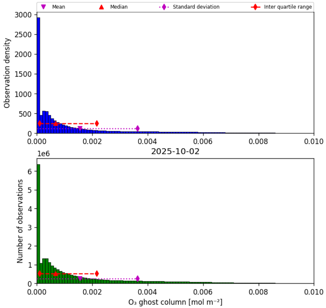
Figure 25: Histogram of “O 3 ghost column” for 2025-10-01 to 2025-10-03
