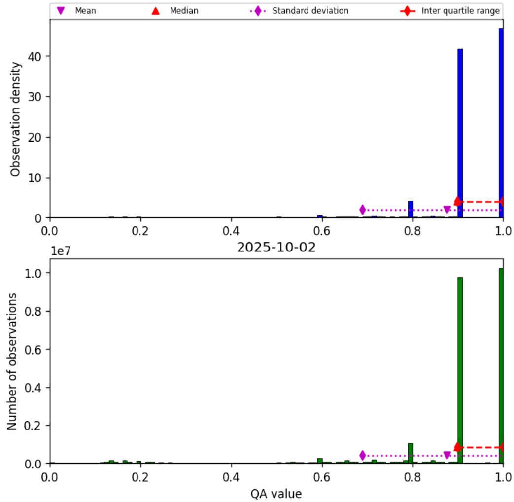
Figure 20: Histogram of “QA value” for 2025-10-01 to 2025-10-03
