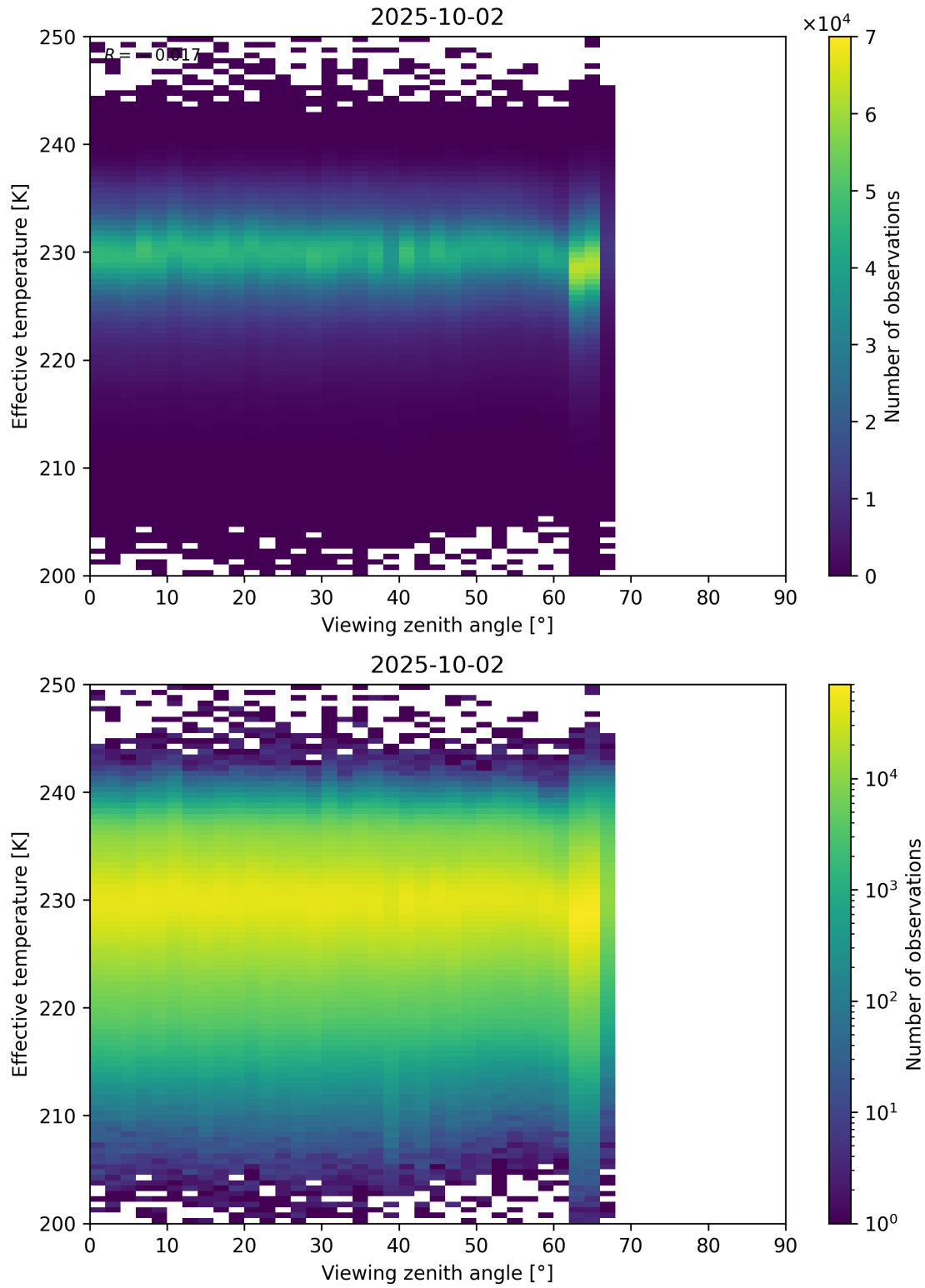
Figure 50: Scatter density plot of “Viewing zenith angle” against “Effective temperature” for 2025-10-01 to 2025-10-03.
