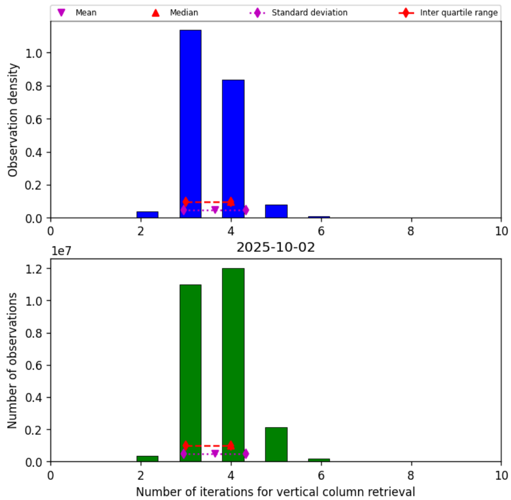
Figure 26: Histogram of “Number of iterations for vertical column retrieval” for 2025-10-01 to 2025-10-03
