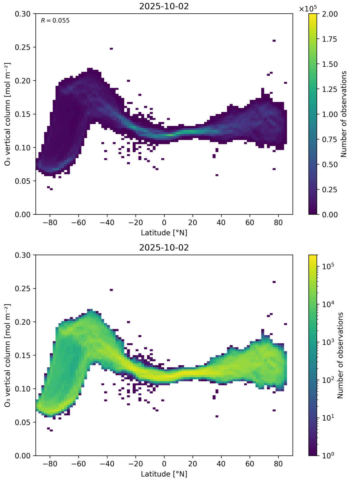
Figure 36: Scatter density plot of “Latitude” against “O 3 vertical column” for 2025-10-01 to 2025-10-03.
