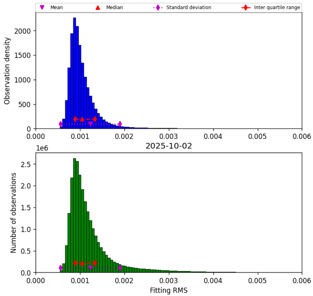
Figure 23: Histogram of “Fitting RMS” for 2025-10-01 to 2025-10-03
