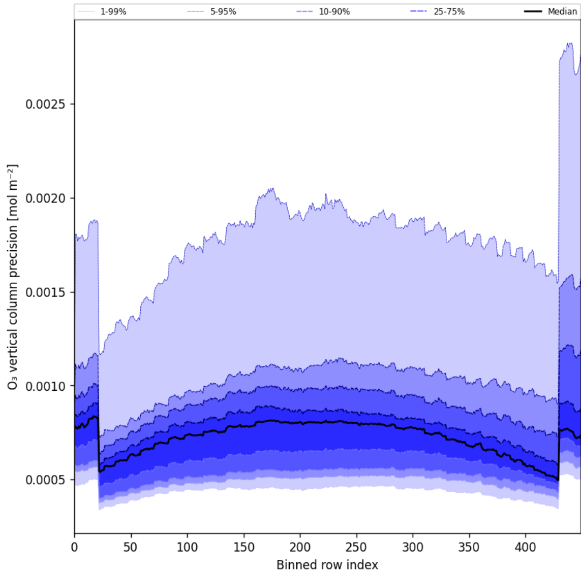
Figure 29: Along track statistics of “O 3 vertical column precision” for 2025-10-01 to 2025-10-03
