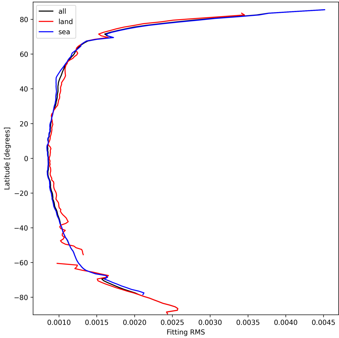
Figure 16: Zonal average of “Fitting RMS” for 2025-10-01 to 2025-10-03.
