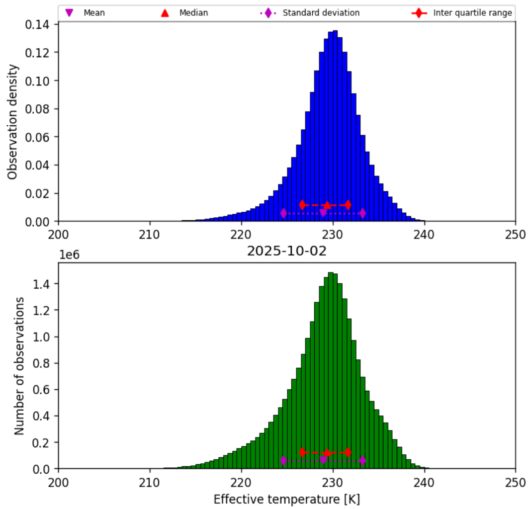
Figure 24: Histogram of “Effective temperature” for 2025-10-01 to 2025-10-03
