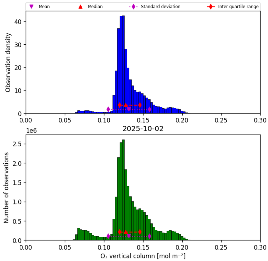
Figure 21: Histogram of “O 3 vertical column” for 2025-10-01 to 2025-10-03
