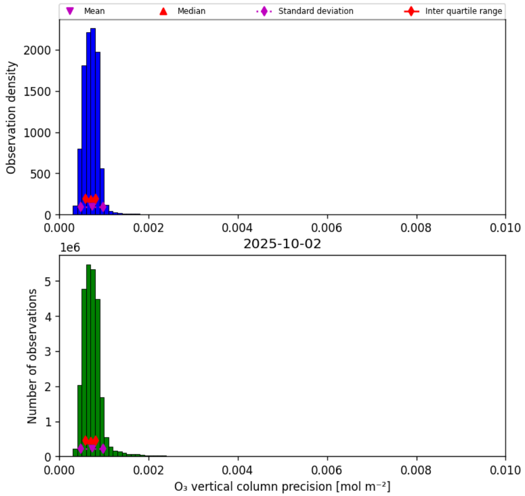
Figure 22: Histogram of “O 3 vertical column precision” for 2025-10-01 to 2025-10-03
