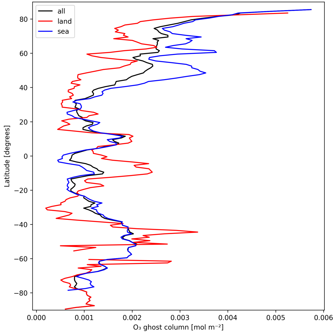
Figure 18: Zonal average of “O 3 ghost column” for 2025-10-01 to 2025-10-03.
