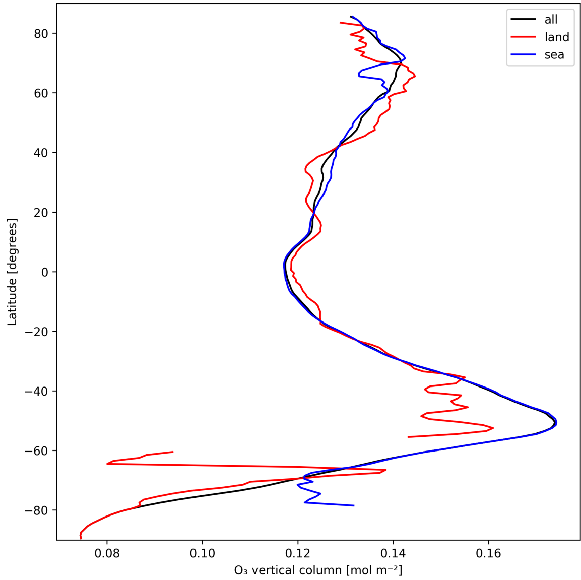
Figure 14: Zonal average of “O 3 vertical column” for 2025-10-01 to 2025-10-03.
