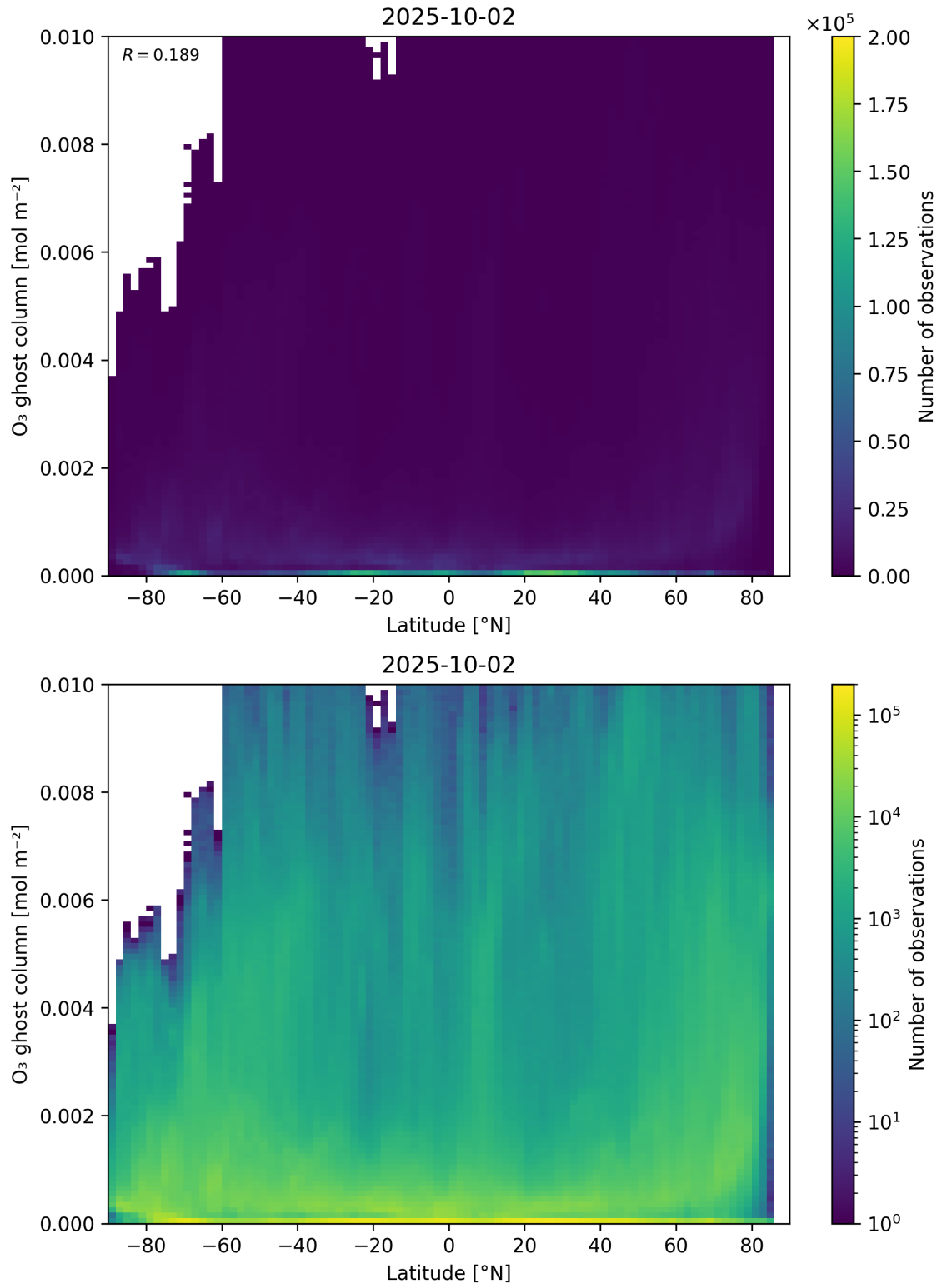
Figure 35: Scatter density plot of “Latitude” against “O 3 ghost column” for 2025-10-01 to 2025-10-03.
