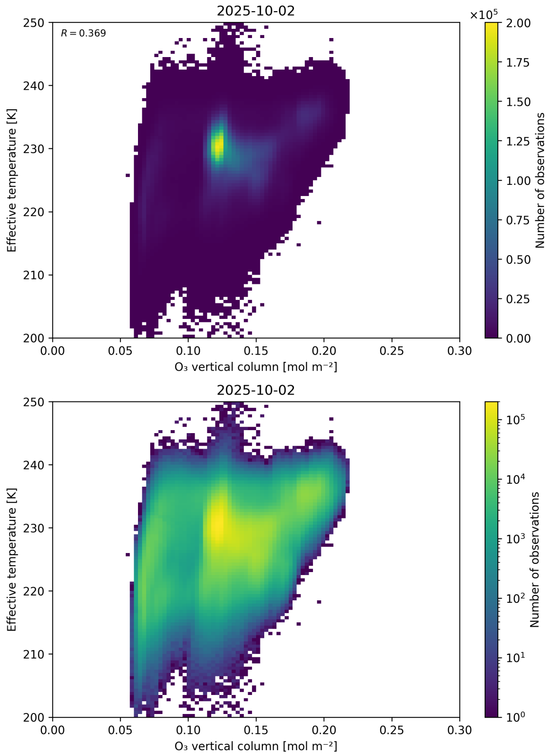
Figure 39: Scatter density plot of “O 3 vertical column” against “Effective temperature” for 2025-10-01 to 2025-10-03.
