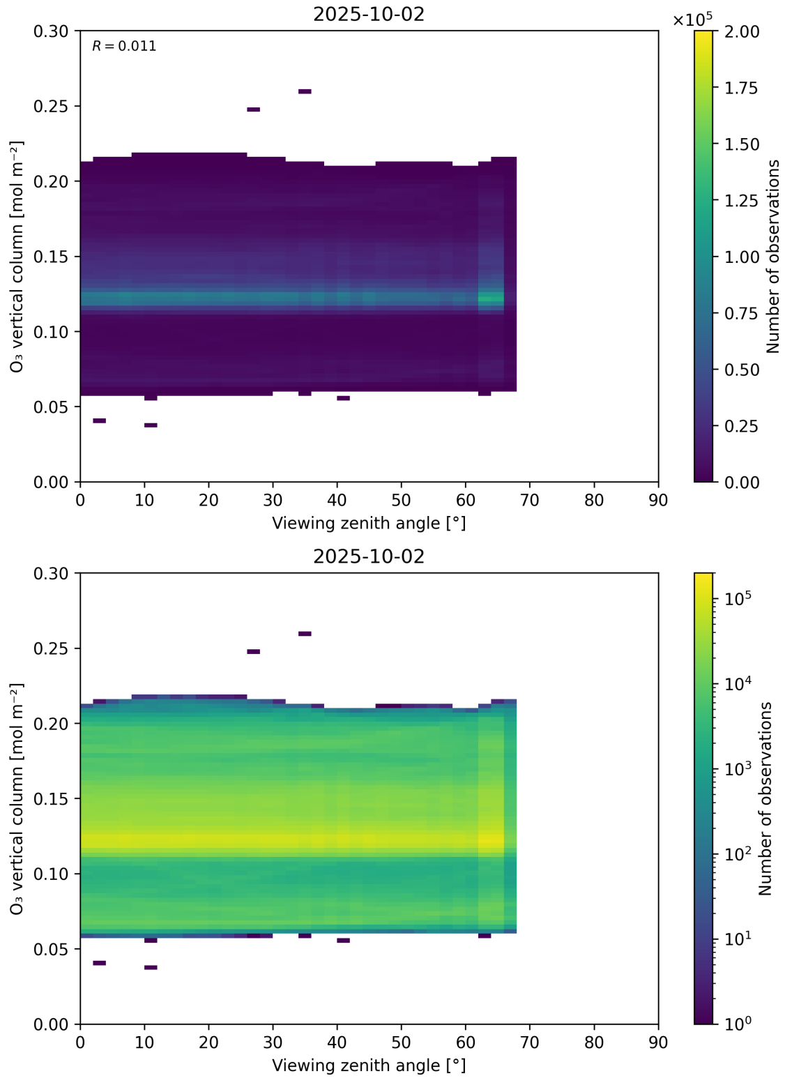
Figure 52: Scatter density plot of “Viewing zenith angle” against “O 3 vertical column” for 2025-10-01 to 2025-10-03.
