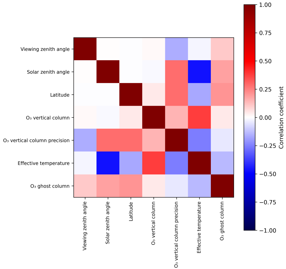
Figure 2: Map of correlation matrix for 2025-10-03 to 2025-10-05.
