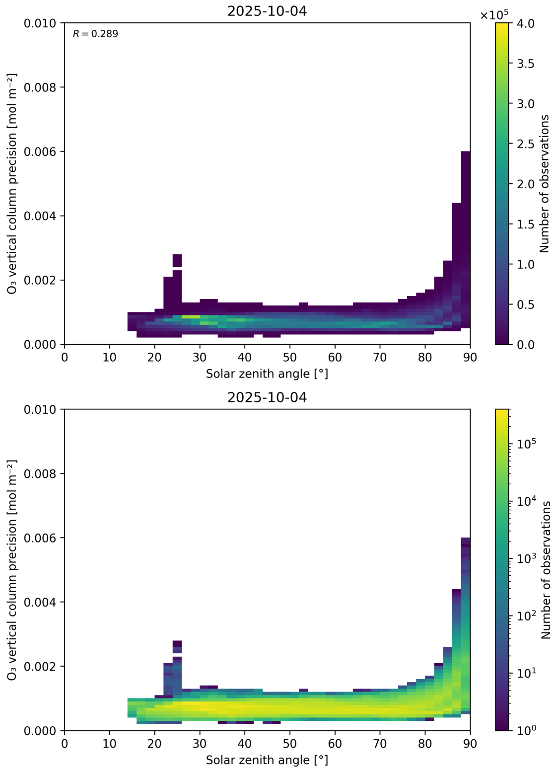
Figure 48: Scatter density plot of “Solar zenith angle” against “O 3 vertical column precision” for 2025-10-03 to 2025-10-05.
