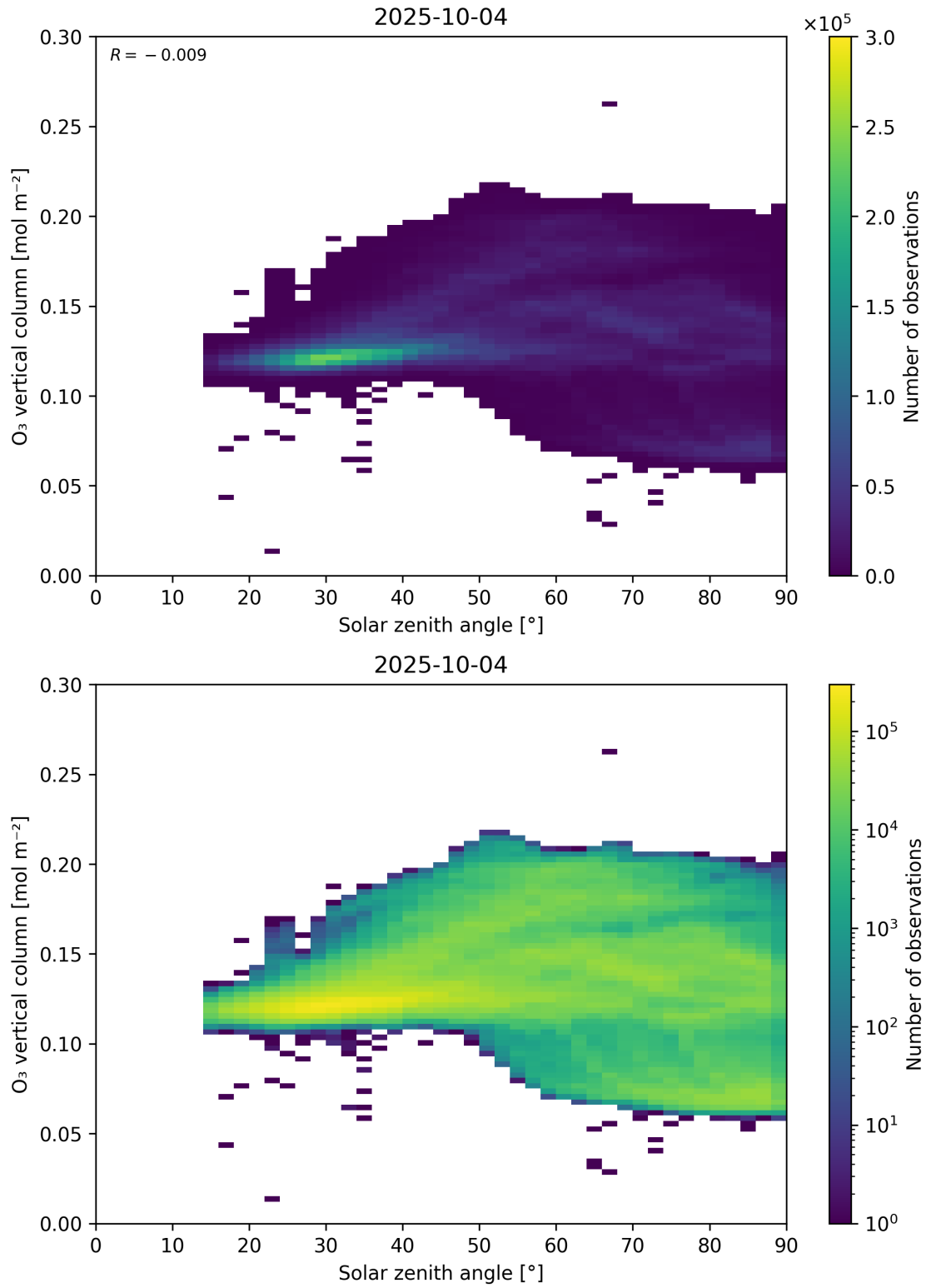
Figure 47: Scatter density plot of “Solar zenith angle” against “O 3 vertical column” for 2025-10-03 to 2025-10-05.
