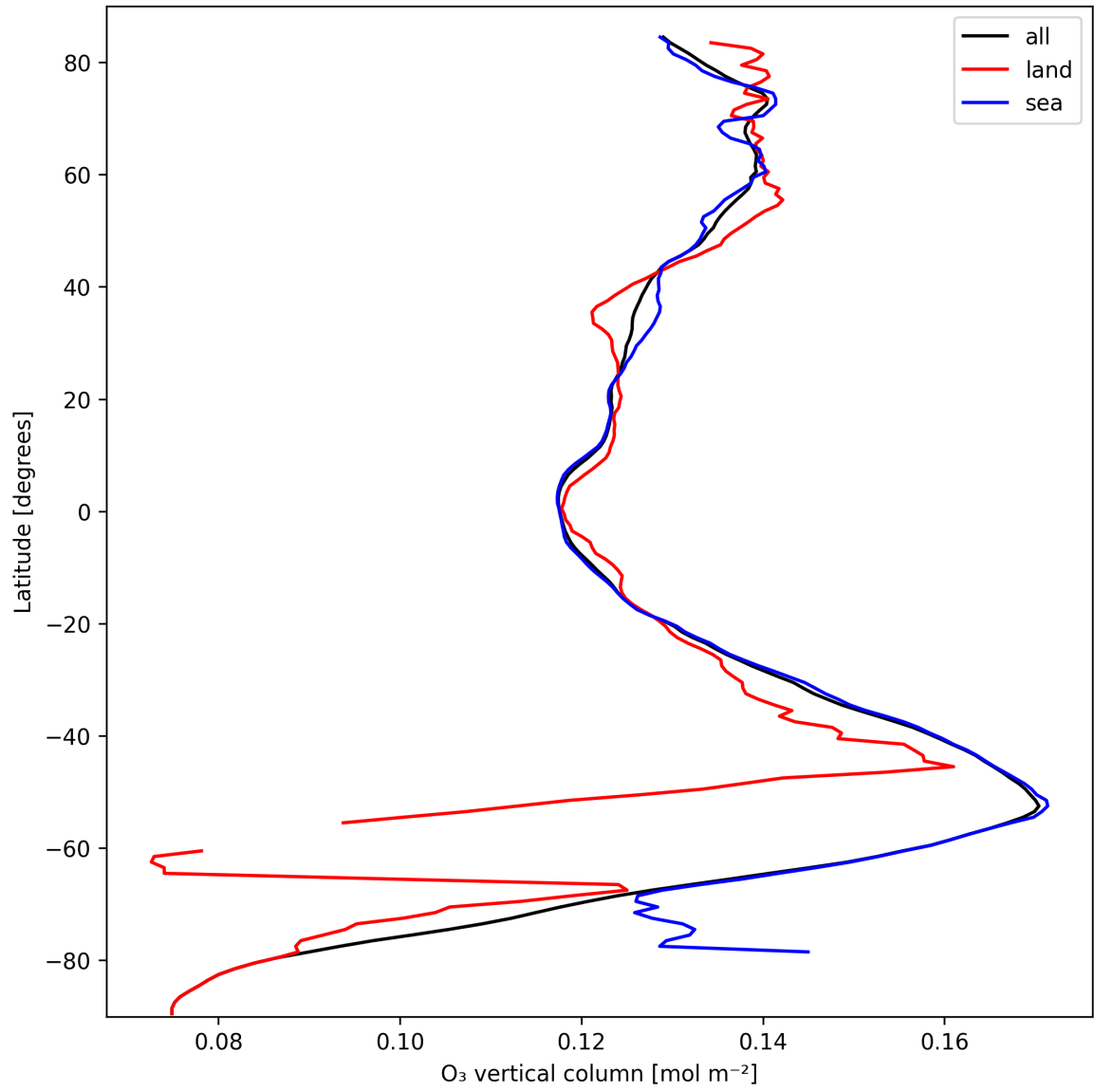
Figure 14: Zonal average of “O 3 vertical column” for 2025-10-03 to 2025-10-05.
