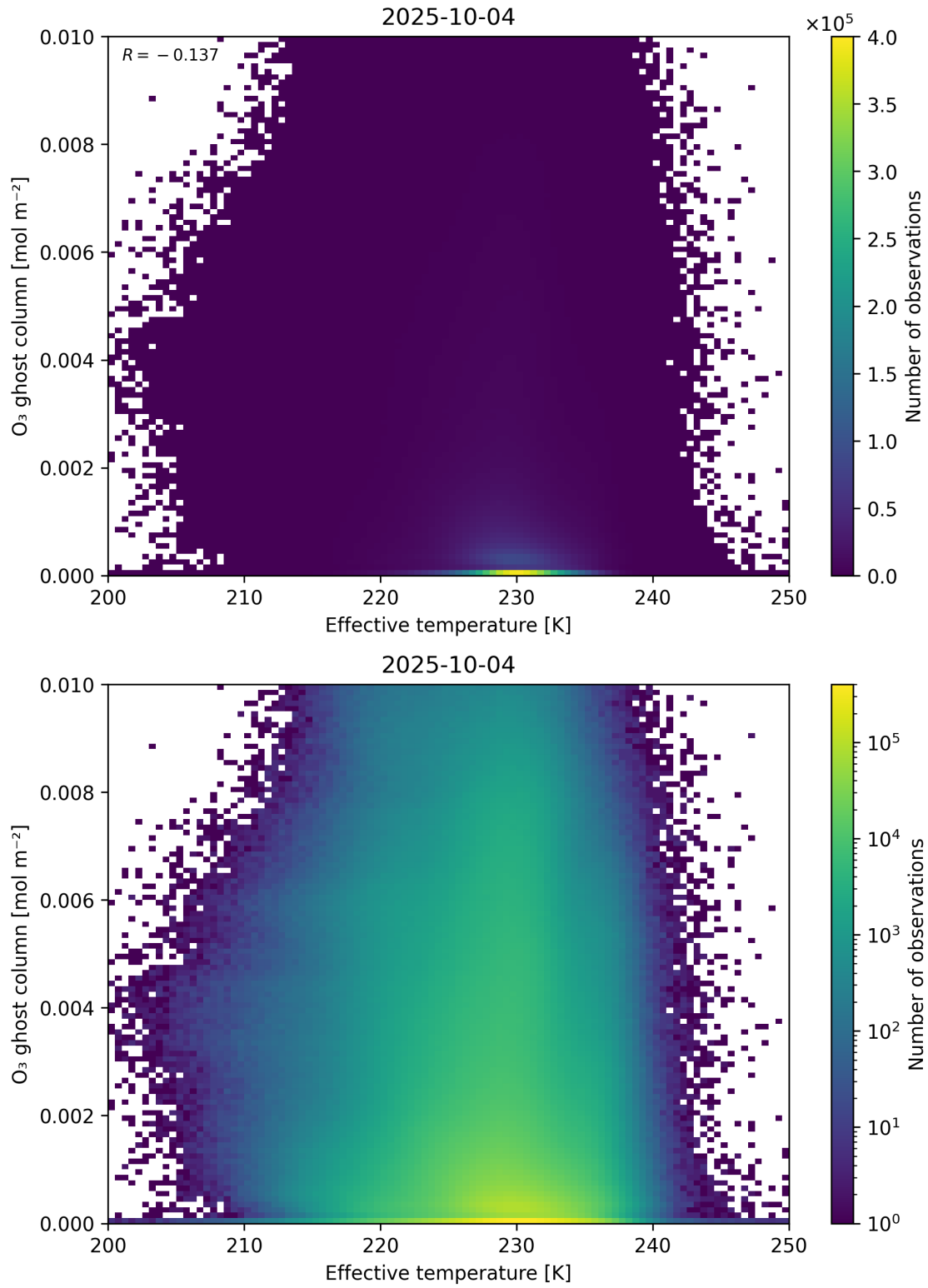
Figure 38: Scatter density plot of “Effective temperature” against “O 3 ghost column” for 2025-10-03 to 2025-10-05.
