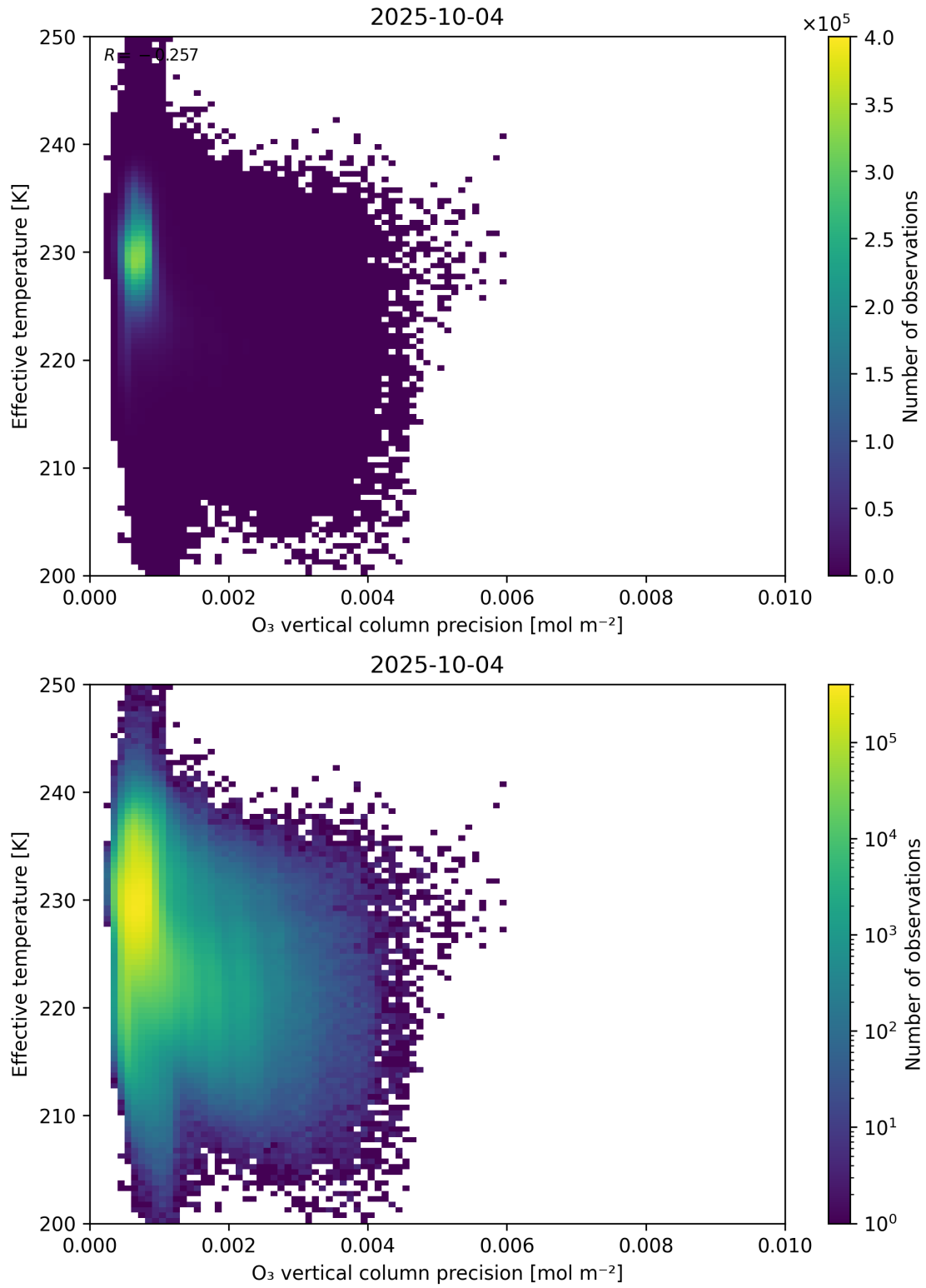
Figure 42: Scatter density plot of “O 3 vertical column precision” against “Effective temperature” for 2025-10-03 to 2025-10-05.
