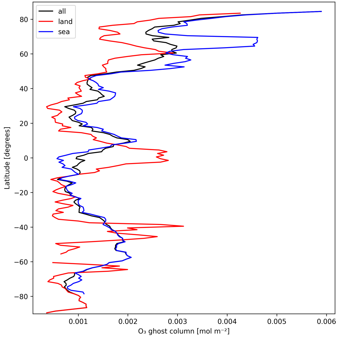
Figure 18: Zonal average of "O 3 ghost column" for 2025-10-03 to 2025-10-05.
