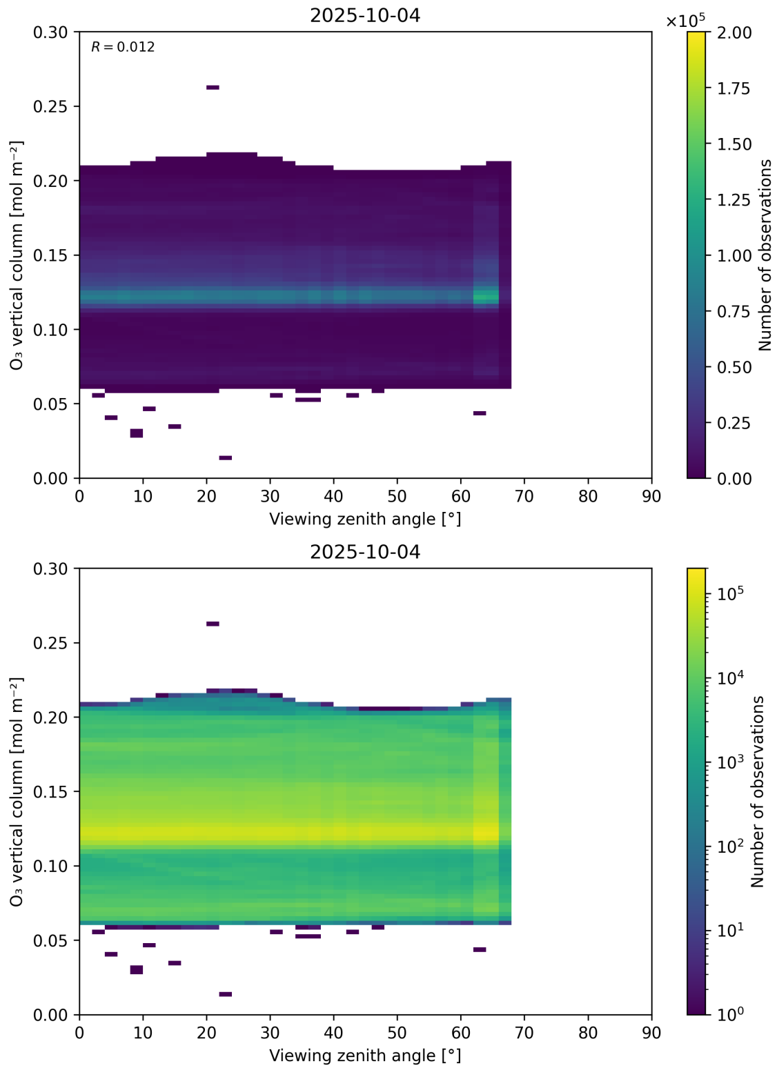
Figure 52: Scatter density plot of “Viewing zenith angle” against “O 3 vertical column” for 2025-10-03 to 2025-10-05.
