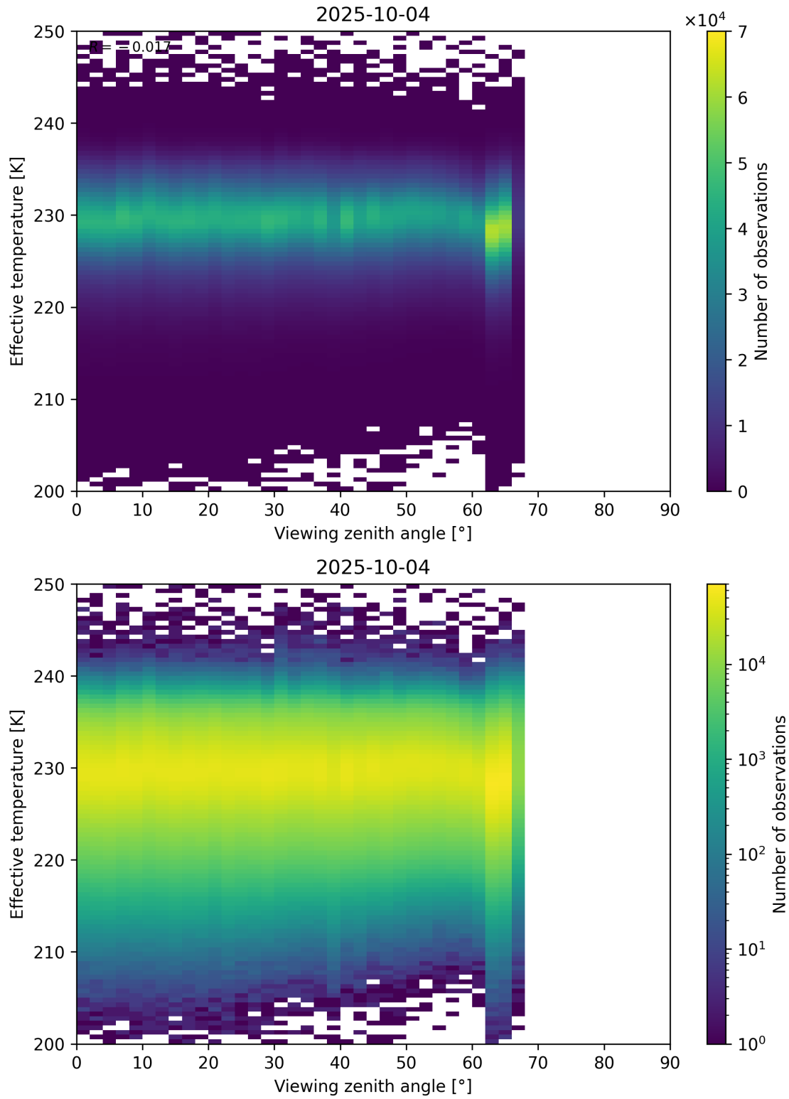
Figure 50: Scatter density plot of “Viewing zenith angle” against “Effective temperature” for 2025-10-03 to 2025-10-05.
