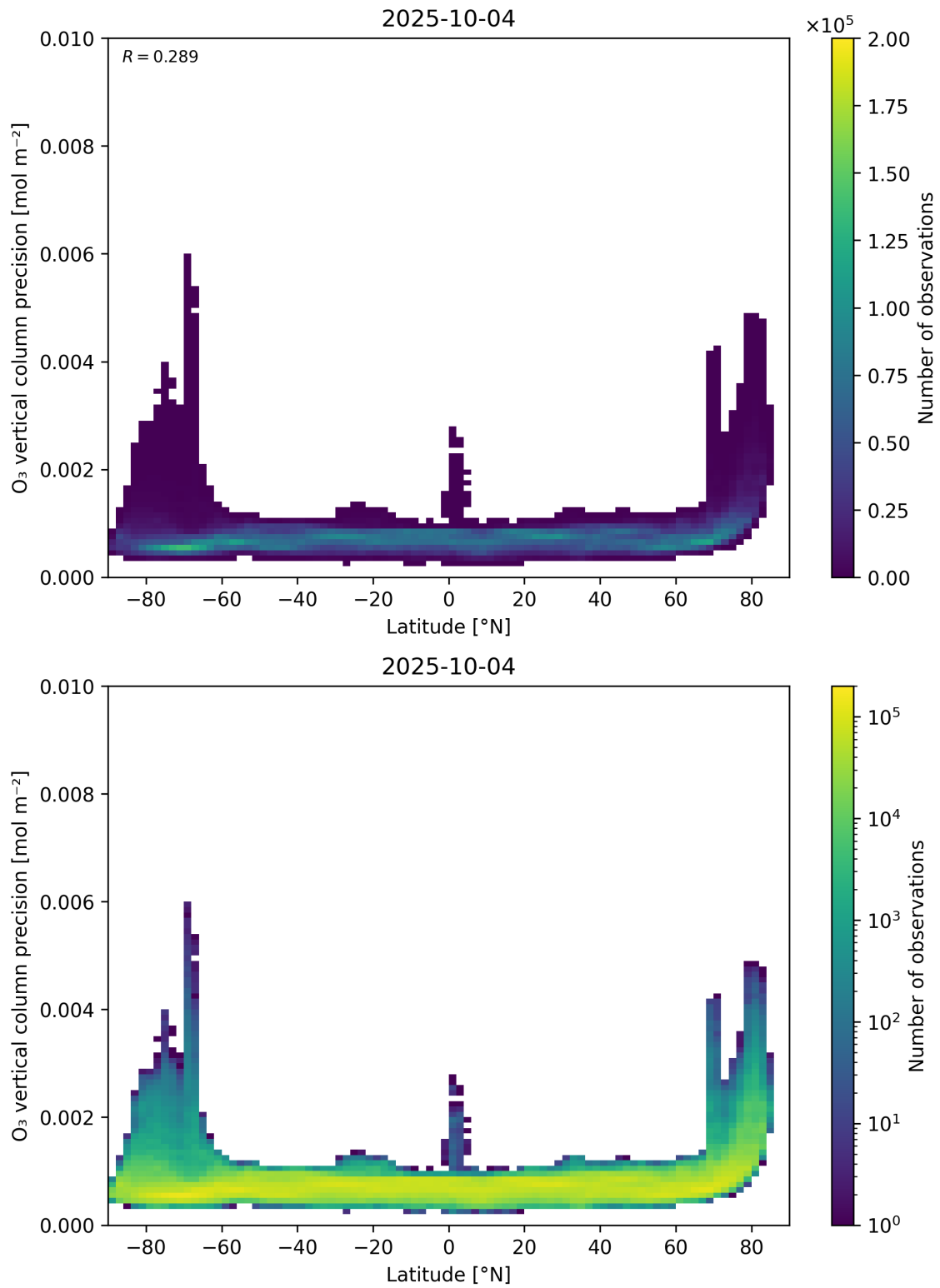
Figure 37: Scatter density plot of “Latitude” against “O 3 vertical column precision” for 2025-10-03 to 2025-10-05.
