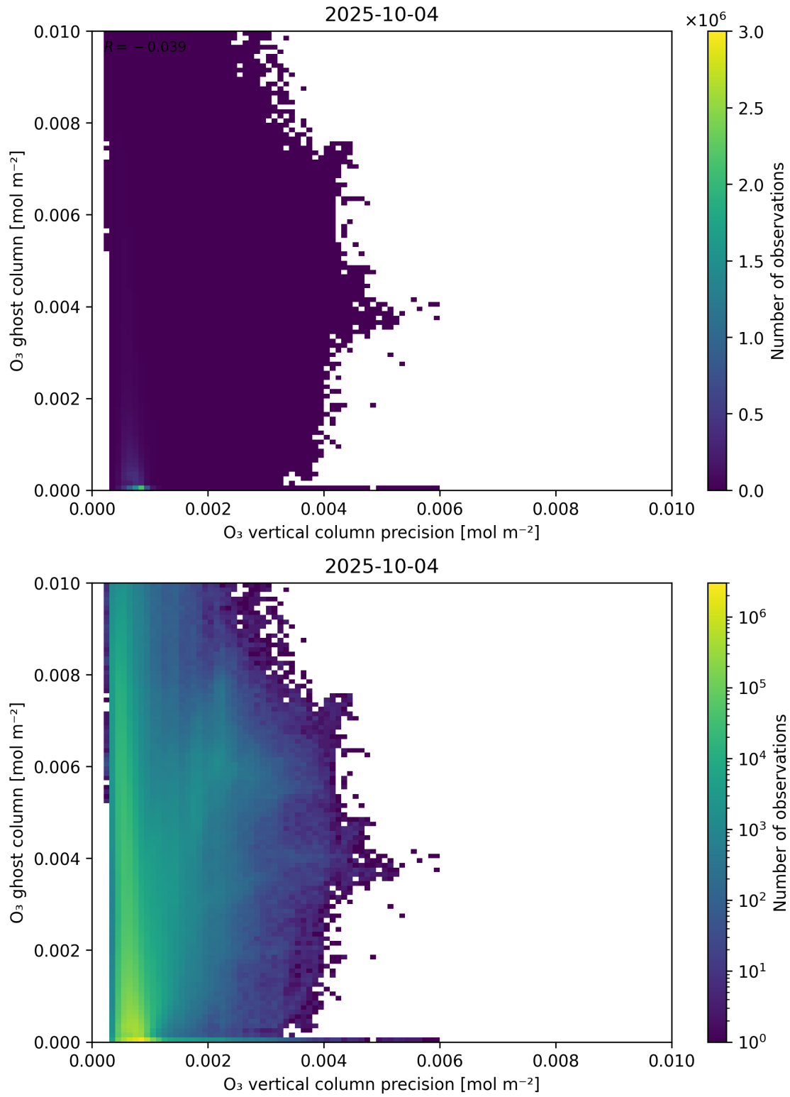
Figure 43: Scatter density plot of “ O_3 vertical column precision” against “ O_3 ghost column” for 2025-10-03 to 2025-10-05.
