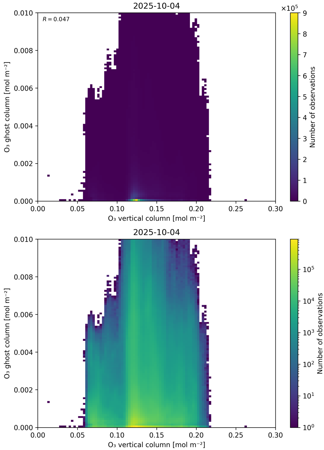
Figure 40: Scatter density plot of “O 3 vertical column” against “O 3 ghost column” for 2025-10-03 to 2025-10-05.
