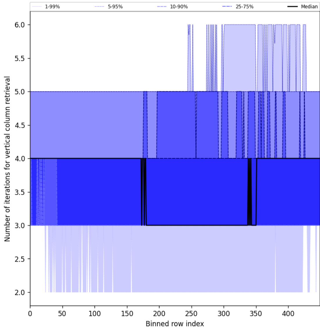
Figure 33: Along track statistics of “Number of iterations for vertical column retrieval” for 2025-10-03 to 2025-10-05
