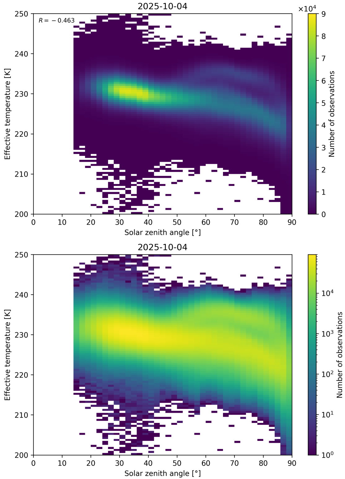
Figure 45: Scatter density plot of “Solar zenith angle” against “Effective temperature” for 2025-10-03 to 2025-10-05.
