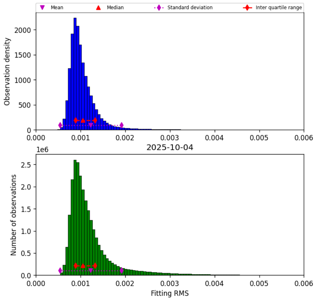
Figure 23: Histogram of “Fitting RMS” for 2025-10-03 to 2025-10-05
