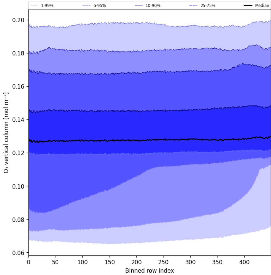
Figure 28: Along track statistics of “O 3 vertical column” for 2025-10-03 to 2025-10-05
