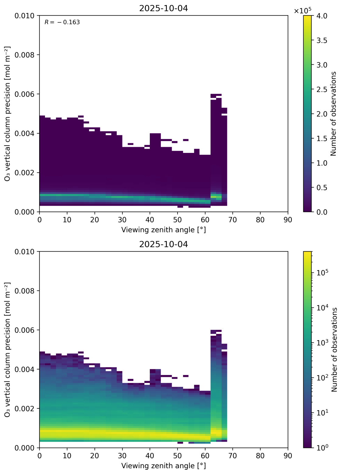
Figure 53: Scatter density plot of “Viewing zenith angle” against “O 3 vertical column precision” for 2025-10-03 to 2025-10-05.
