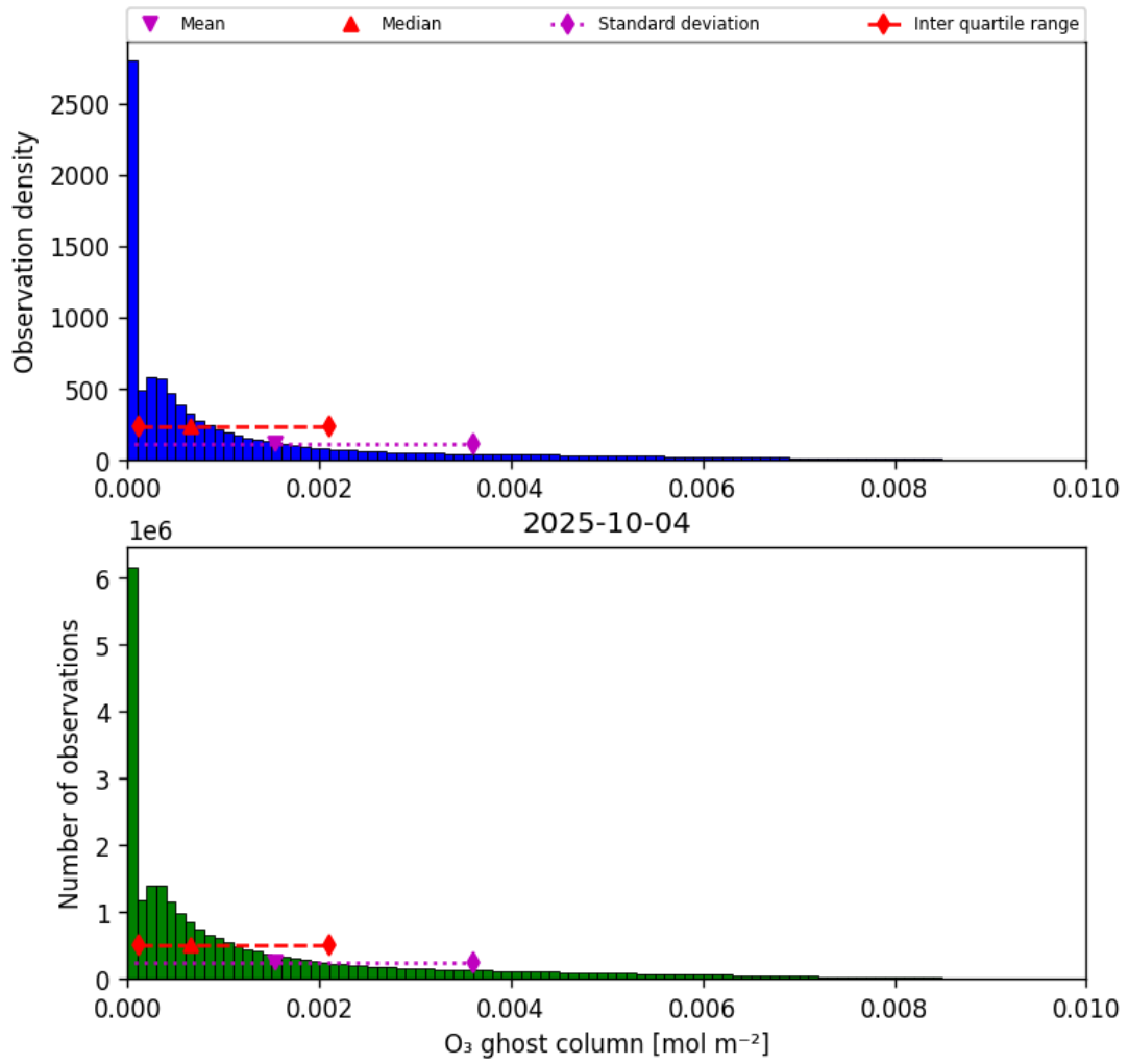
Figure 25: Histogram of “O 3 ghost column” for 2025-10-03 to 2025-10-05
