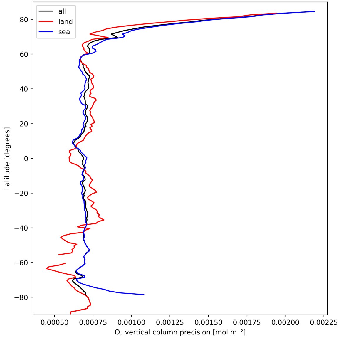
Figure 15: Zonal average of “O 3 vertical column precision” for 2025-10-03 to 2025-10-05.
