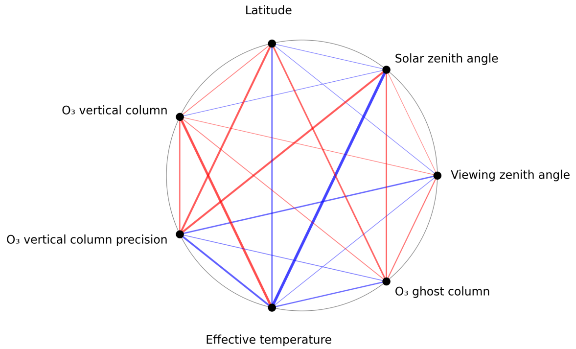
Figure 1: Map of correlation graph for 2025-10-03 to 2025-10-05.
