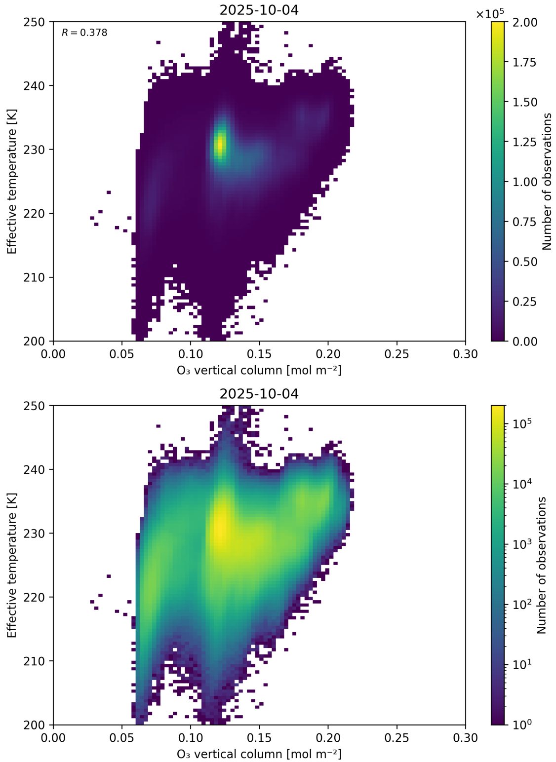
Figure 39: Scatter density plot of “O 3 vertical column” against “Effective temperature” for 2025-10-03 to 2025-10-05.
