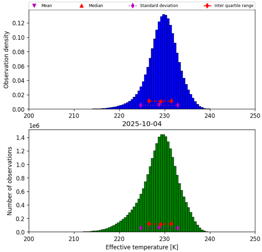
Figure 24: Histogram of “Effective temperature” for 2025-10-03 to 2025-10-05
