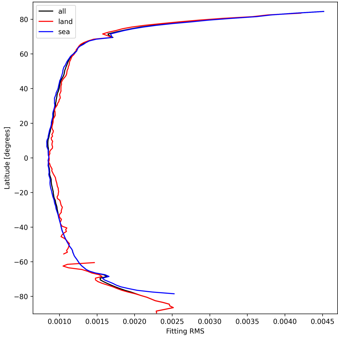
Figure 16: Zonal average of “Fitting RMS” for 2025-10-03 to 2025-10-05.
