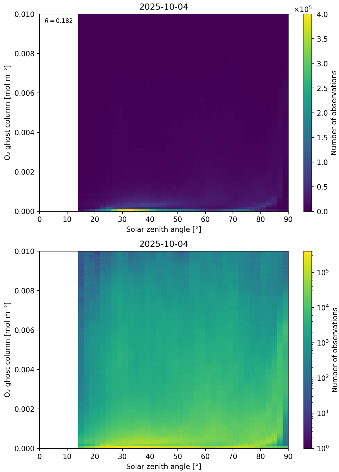
Figure 46: Scatter density plot of “Solar zenith angle” against “O 3 ghost column” for 2025-10-03 to 2025-10-05.
