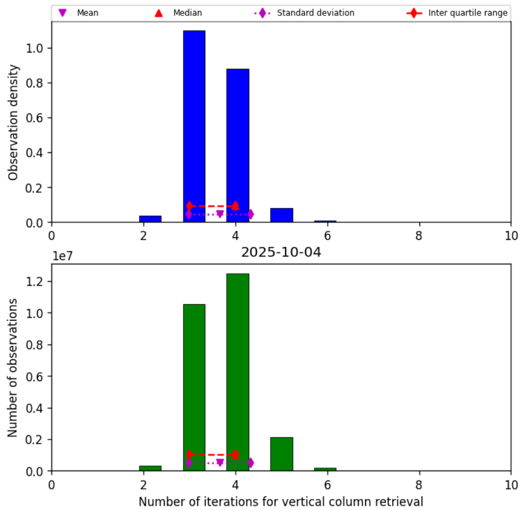
Figure 26: Histogram of “Number of iterations for vertical column retrieval” for 2025-10-03 to 2025-10-05
