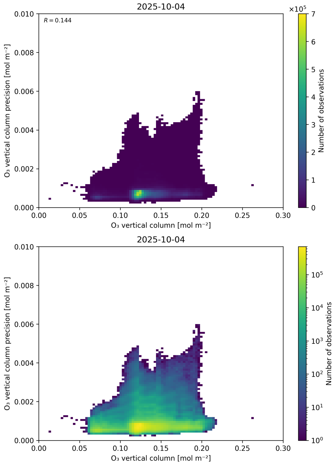
Figure 41: Scatter density plot of “O 3 vertical column” against “O 3 vertical column precision” for 2025-10-03 to 2025-10-05.
