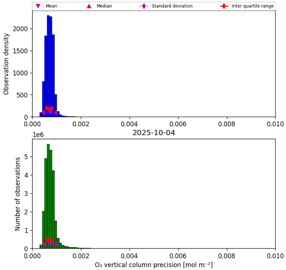
Figure 22: Histogram of “O 3 vertical column precision” for 2025-10-03 to 2025-10-05
