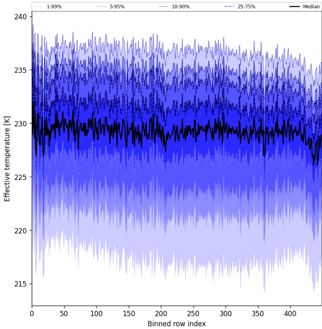
Figure 31: Along track statistics of “Effective temperature” for 2025-10-03 to 2025-10-05
