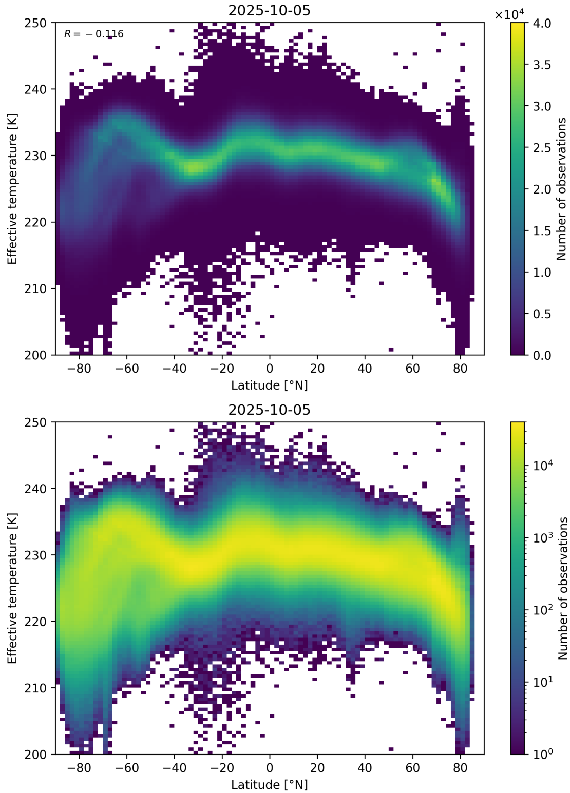
Figure 34: Scatter density plot of “Latitude” against “Effective temperature” for 2025-10-04 to 2025-10-06.
