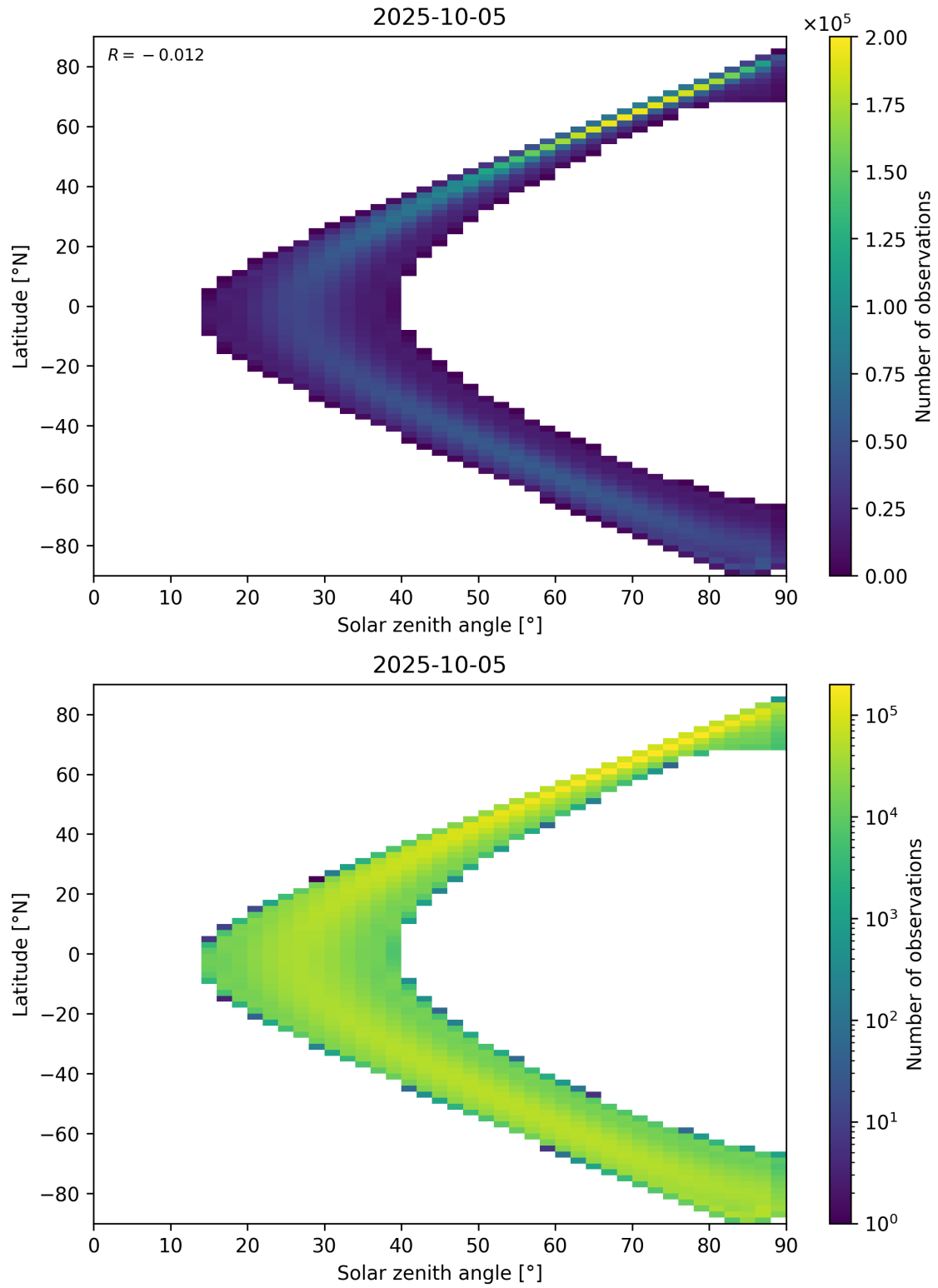
Figure 44: Scatter density plot of “Solar zenith angle” against “Latitude” for 2025-10-04 to 2025-10-06.
