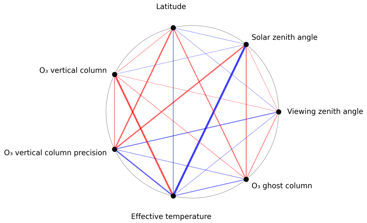
Figure 1: Map of correlation graph for 2025-10-04 to 2025-10-06.
