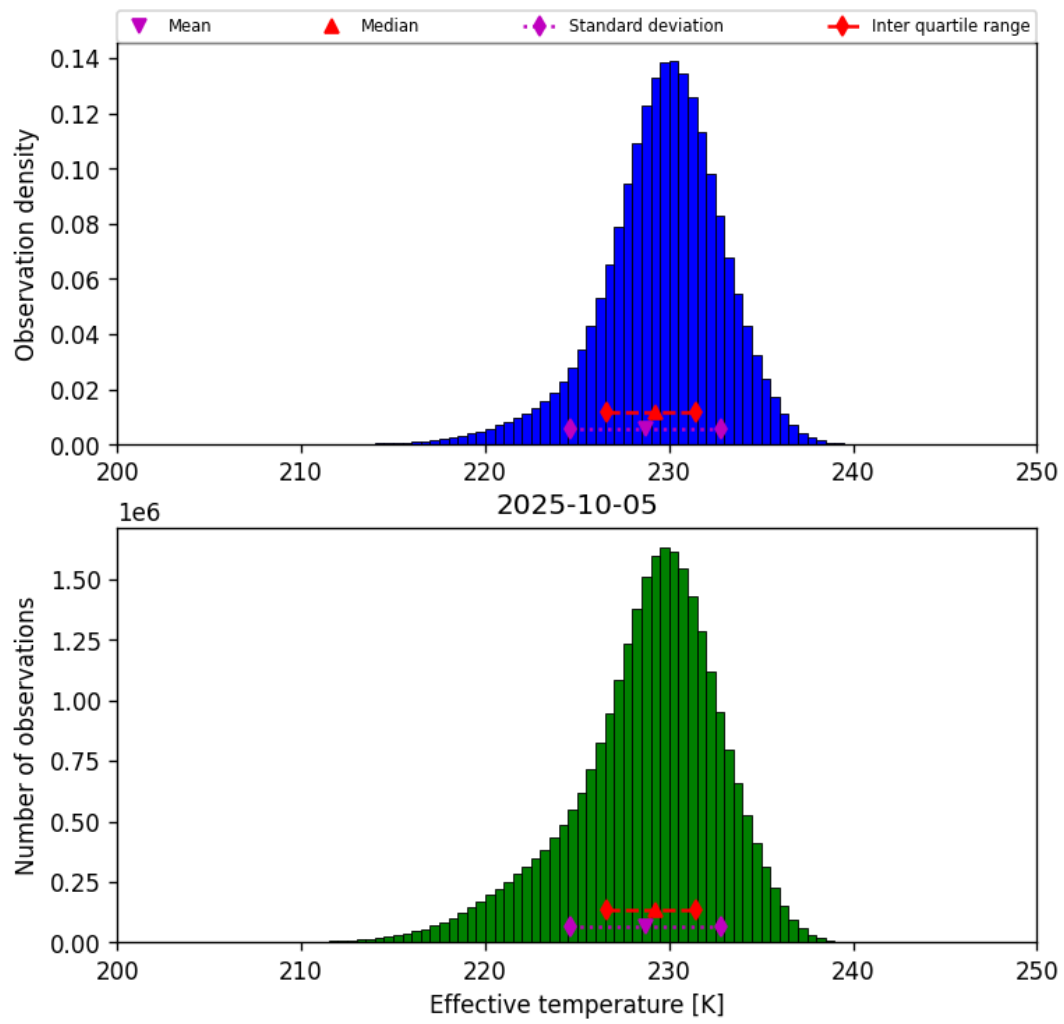
Figure 24: Histogram of “Effective temperature” for 2025-10-04 to 2025-10-06
