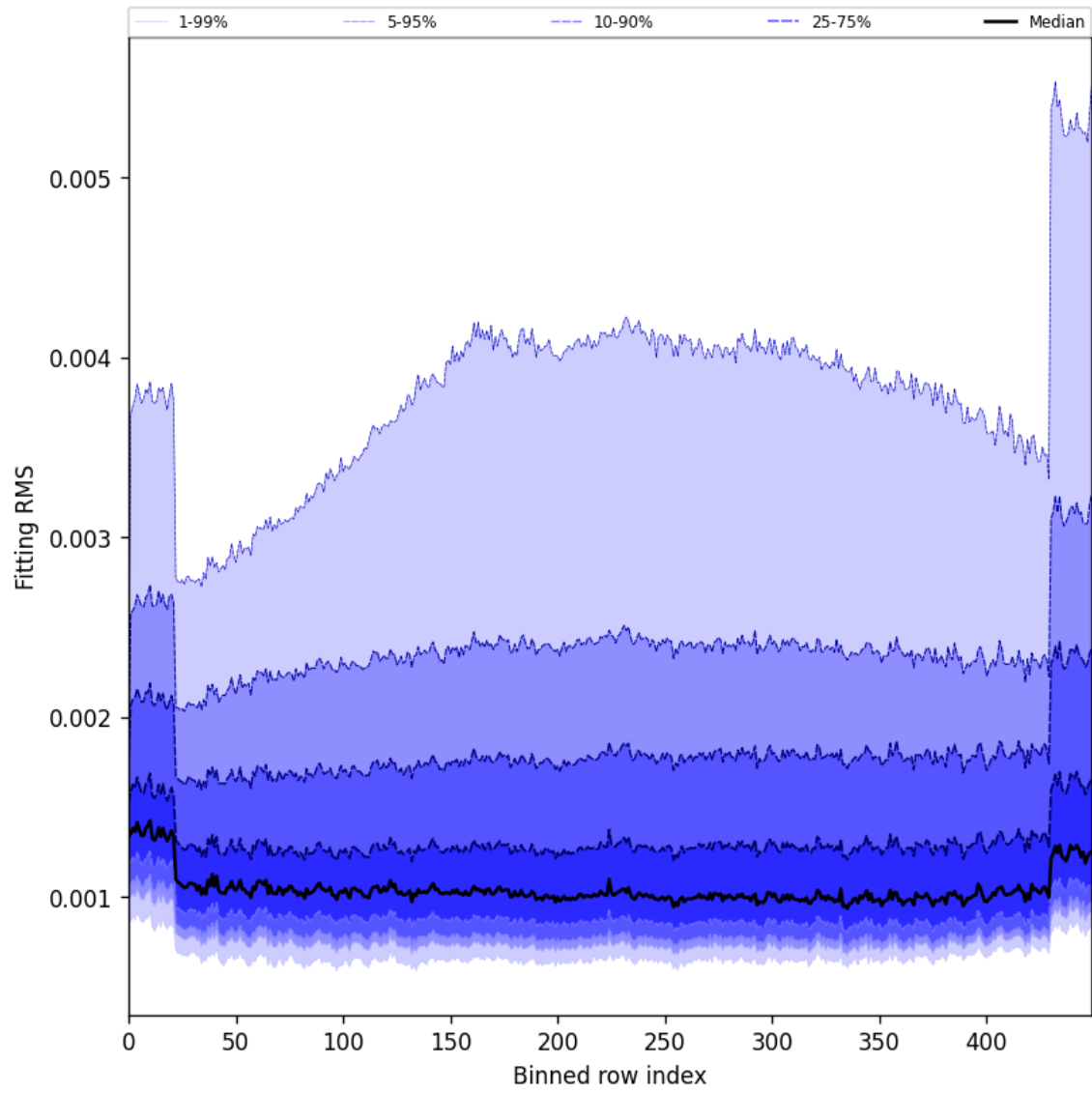
Figure 30: Along track statistics of “Fitting RMS” for 2025-10-04 to 2025-10-06
