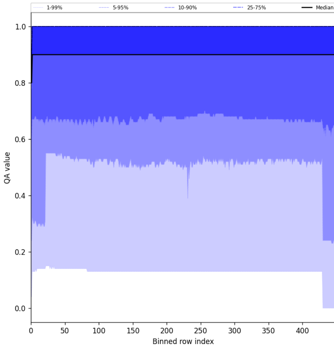
Figure 27: Along track statistics of “QA value” for 2025-10-04 to 2025-10-06
