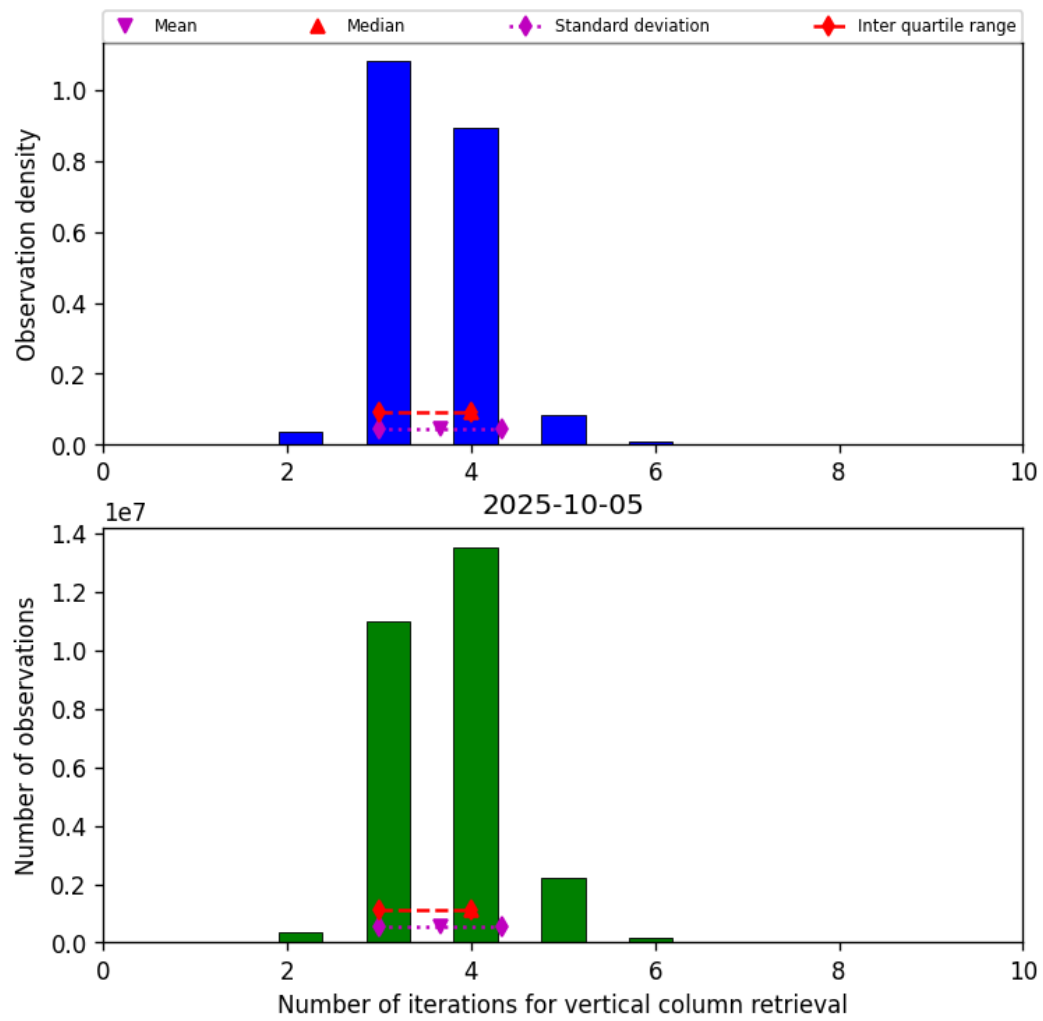
Figure 26: Histogram of “Number of iterations for vertical column retrieval” for 2025-10-04 to 2025-10-06
