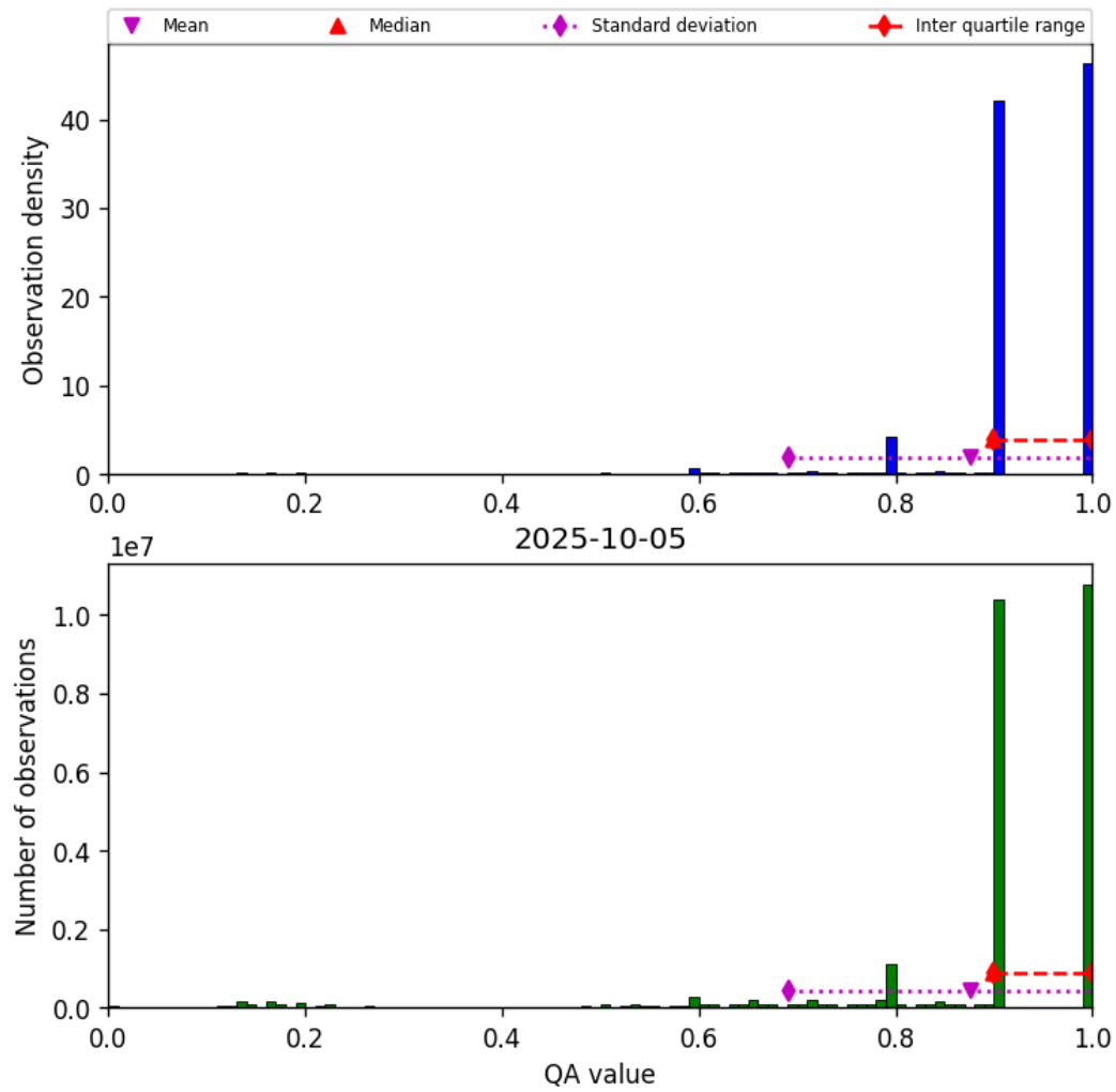
Figure 20: Histogram of “QA value” for 2025-10-04 to 2025-10-06
