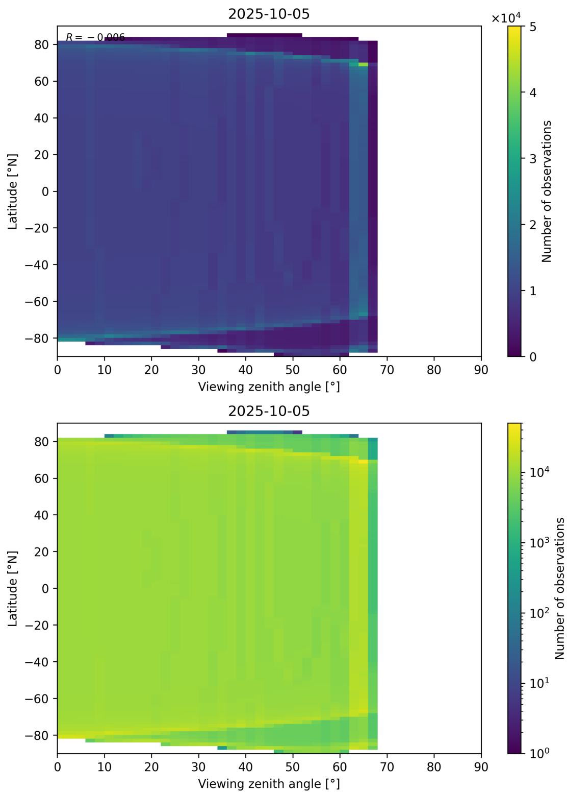
Figure 49: Scatter density plot of “Viewing zenith angle” against “Latitude” for 2025-10-04 to 2025-10-06.
