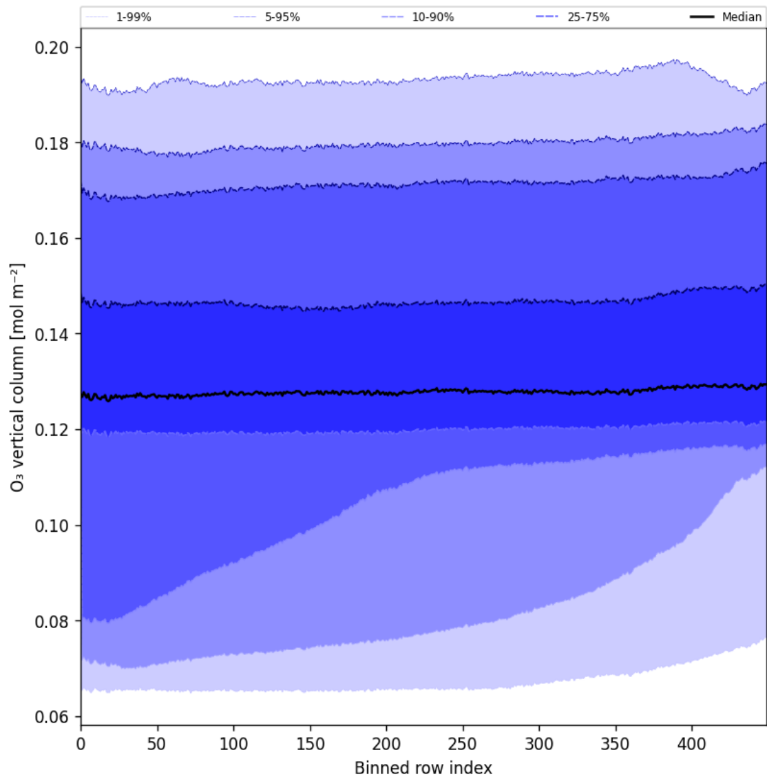
Figure 28: Along track statistics of “O 3 vertical column” for 2025-10-04 to 2025-10-06
