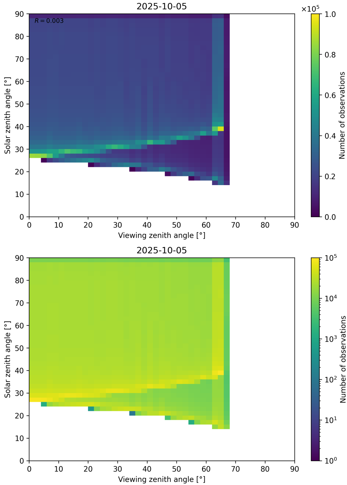
Figure 54: Scatter density plot of “Viewing zenith angle” against “Solar zenith angle” for 2025-10-04 to 2025-10-06.
