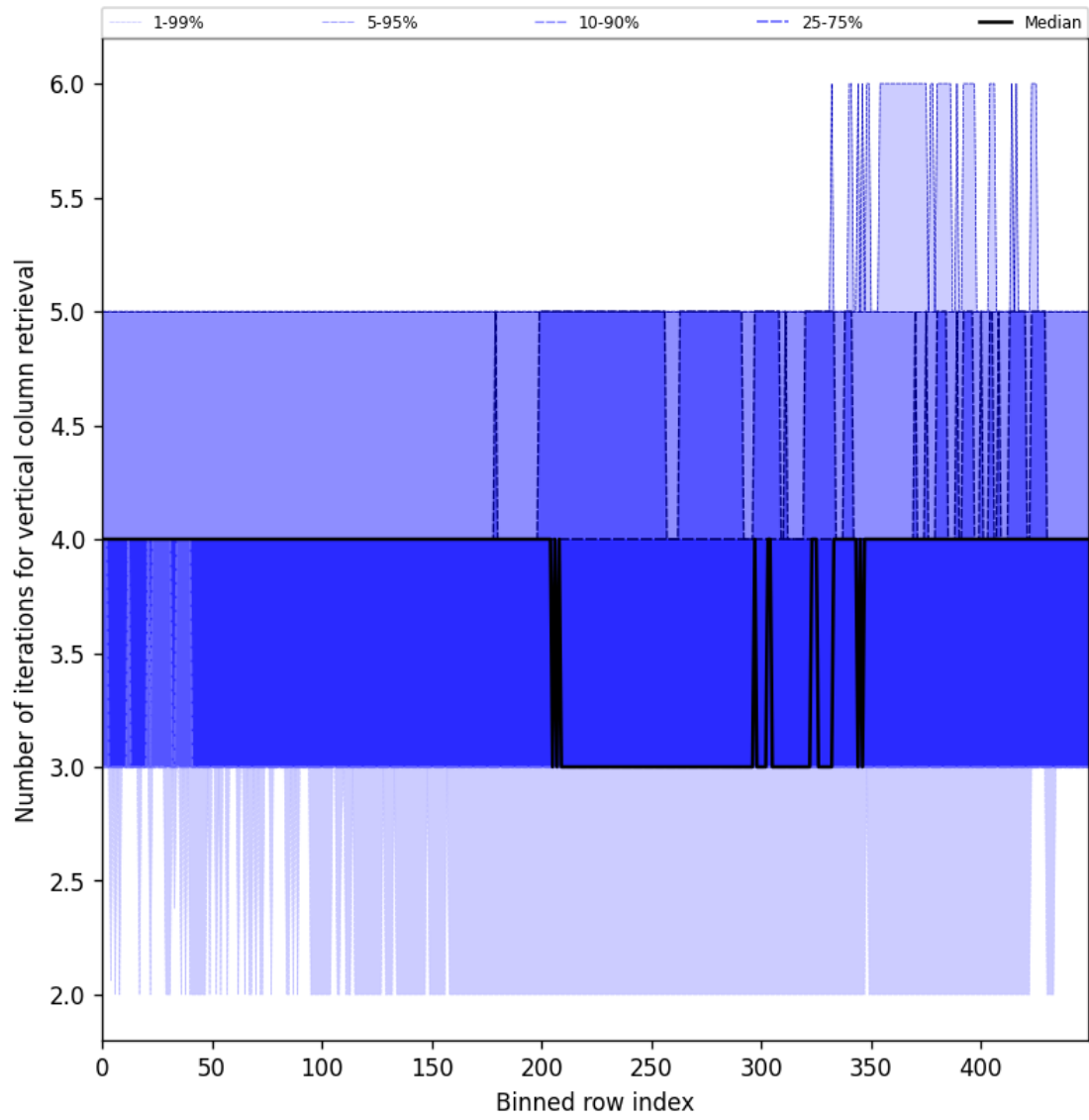
Figure 33: Along track statistics of “Number of iterations for vertical column retrieval” for 2025-10-04 to 2025-10-06
