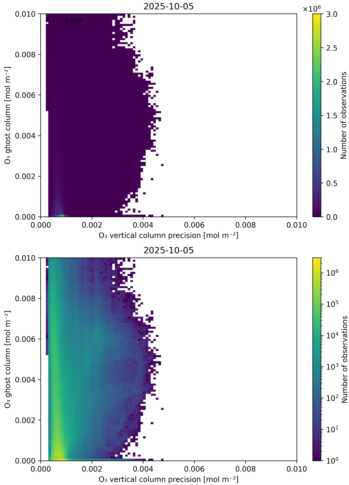
Figure 43: Scatter density plot of “O 3 vertical column precision” against “O 3 ghost column” for 2025-10-04 to 2025-10-06.
