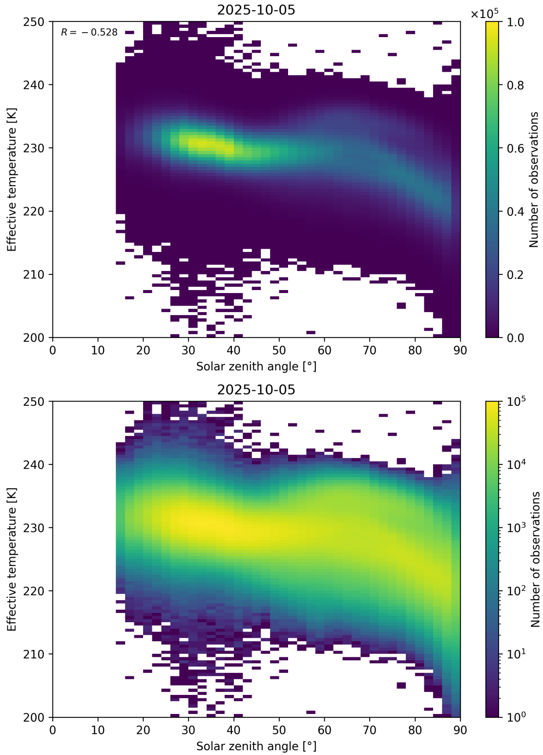
Figure 45: Scatter density plot of “Solar zenith angle” against “Effective temperature” for 2025-10-04 to 2025-10-06.
