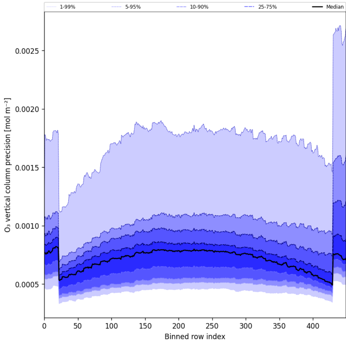
Figure 29: Along track statistics of “O 3 vertical column precision” for 2025-10-04 to 2025-10-06
