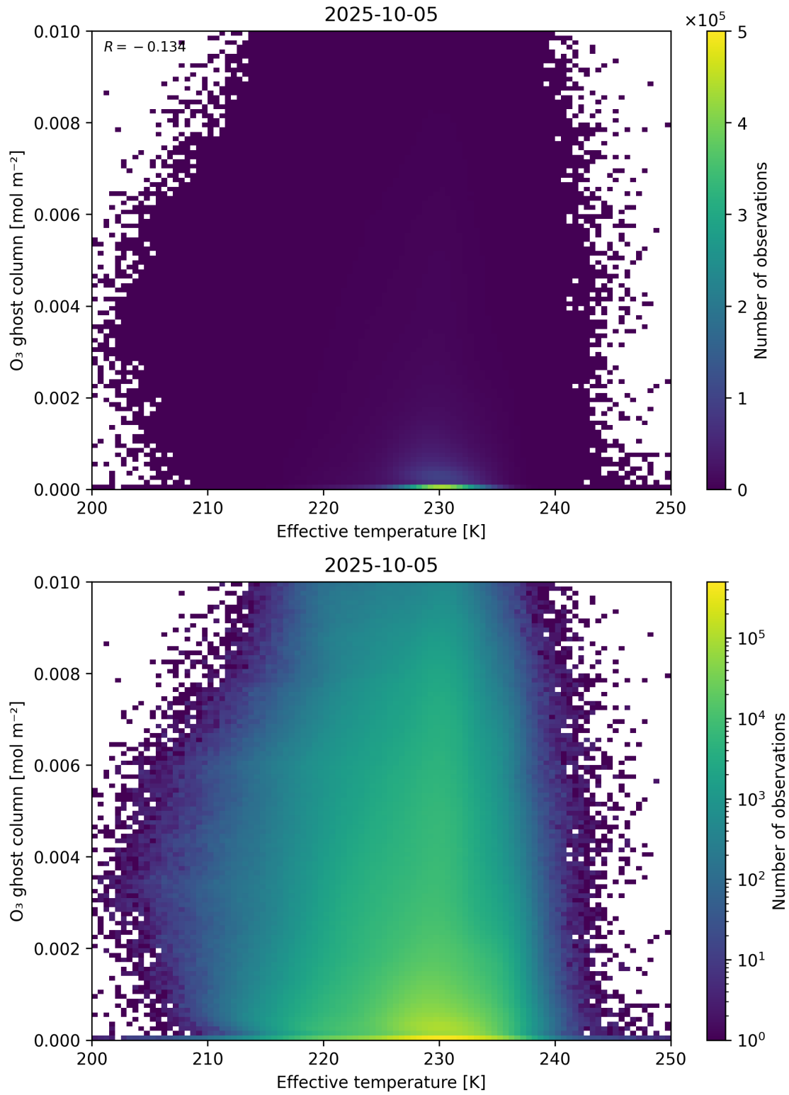
Figure 38: Scatter density plot of “Effective temperature” against “O 3 ghost column” for 2025-10-04 to 2025-10-06.
