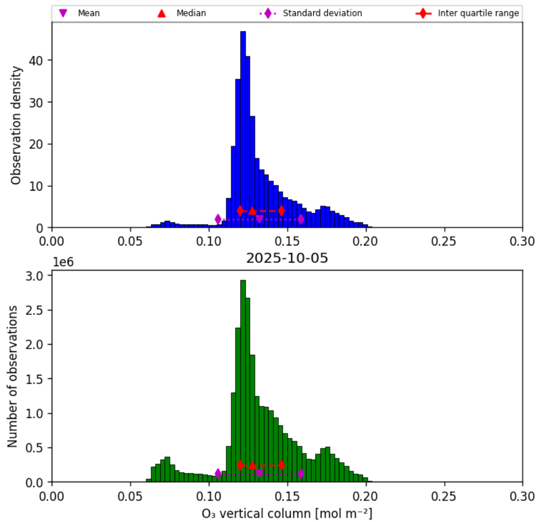
Figure 21: Histogram of “O 3 vertical column” for 2025-10-04 to 2025-10-06
