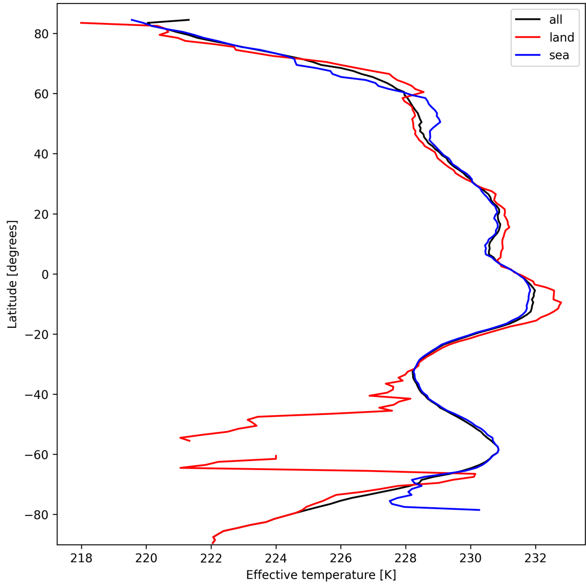
Figure 17: Zonal average of “Effective temperature” for 2025-10-04 to 2025-10-06.
