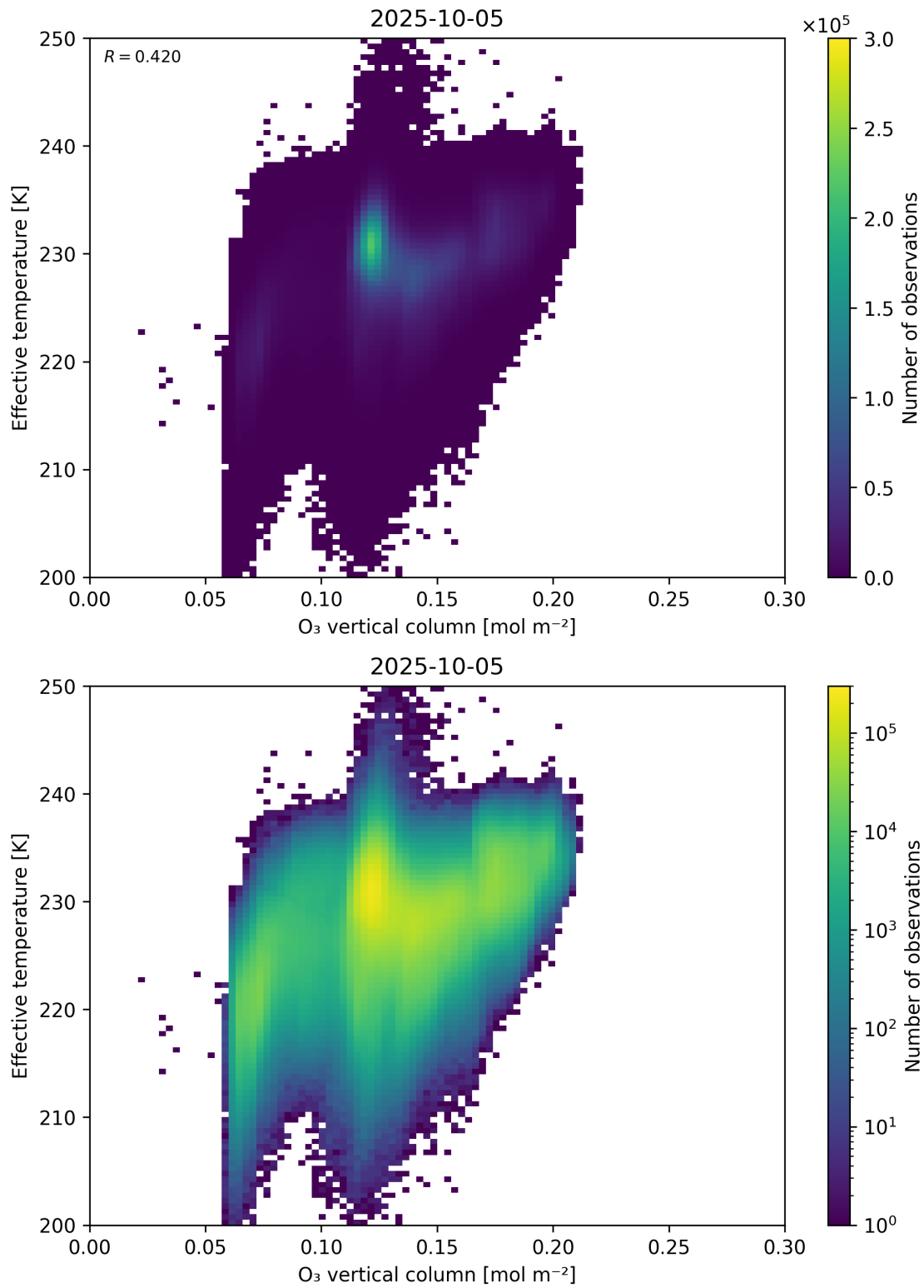
Figure 39: Scatter density plot of “O 3 vertical column” against “Effective temperature” for 2025-10-04 to 2025-10-06.
