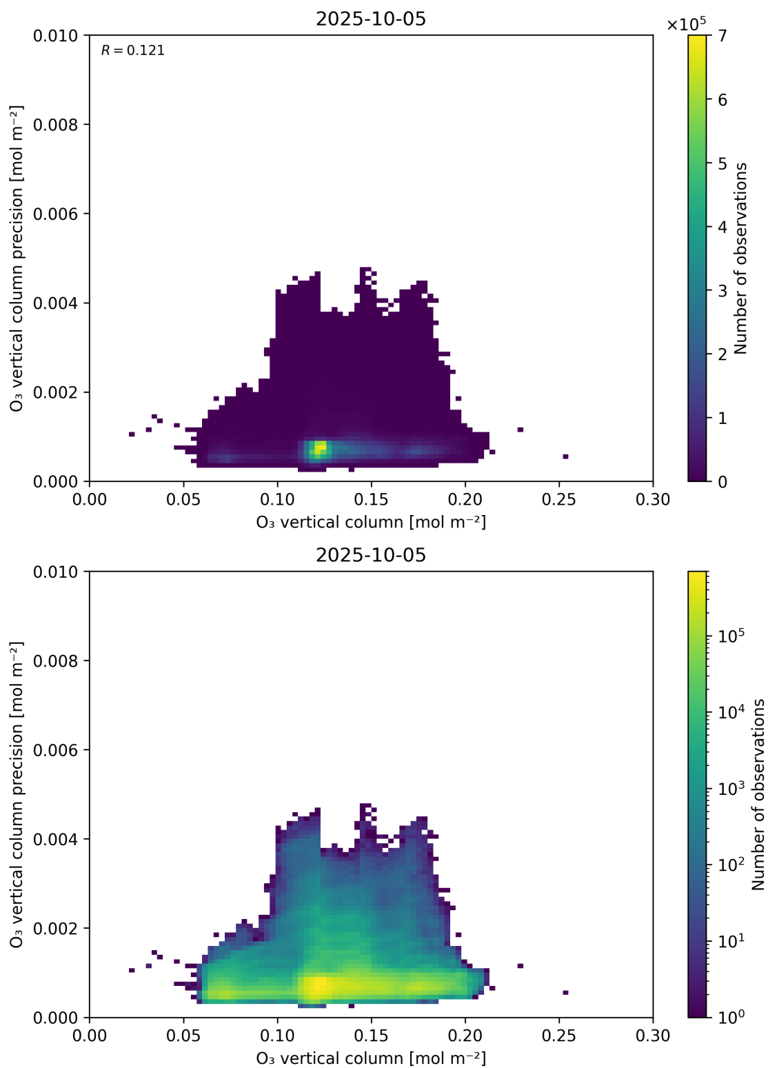
Figure 41: Scatter density plot of “O 3 vertical column” against “O 3 vertical column precision” for 2025-10-04 to 2025-10-06.
