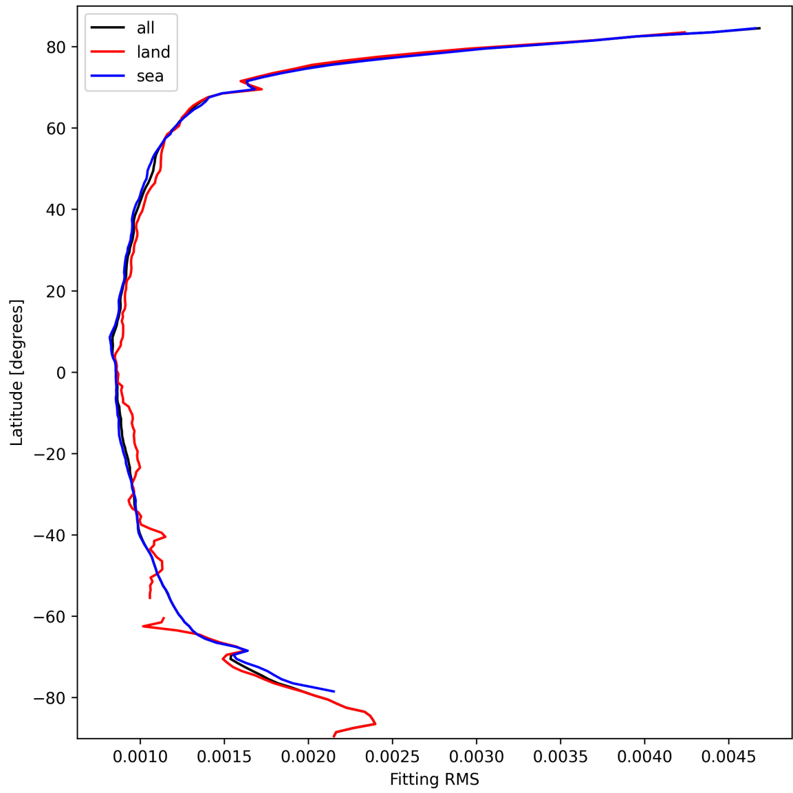
Figure 16: Zonal average of “Fitting RMS” for 2025-10-04 to 2025-10-06.
