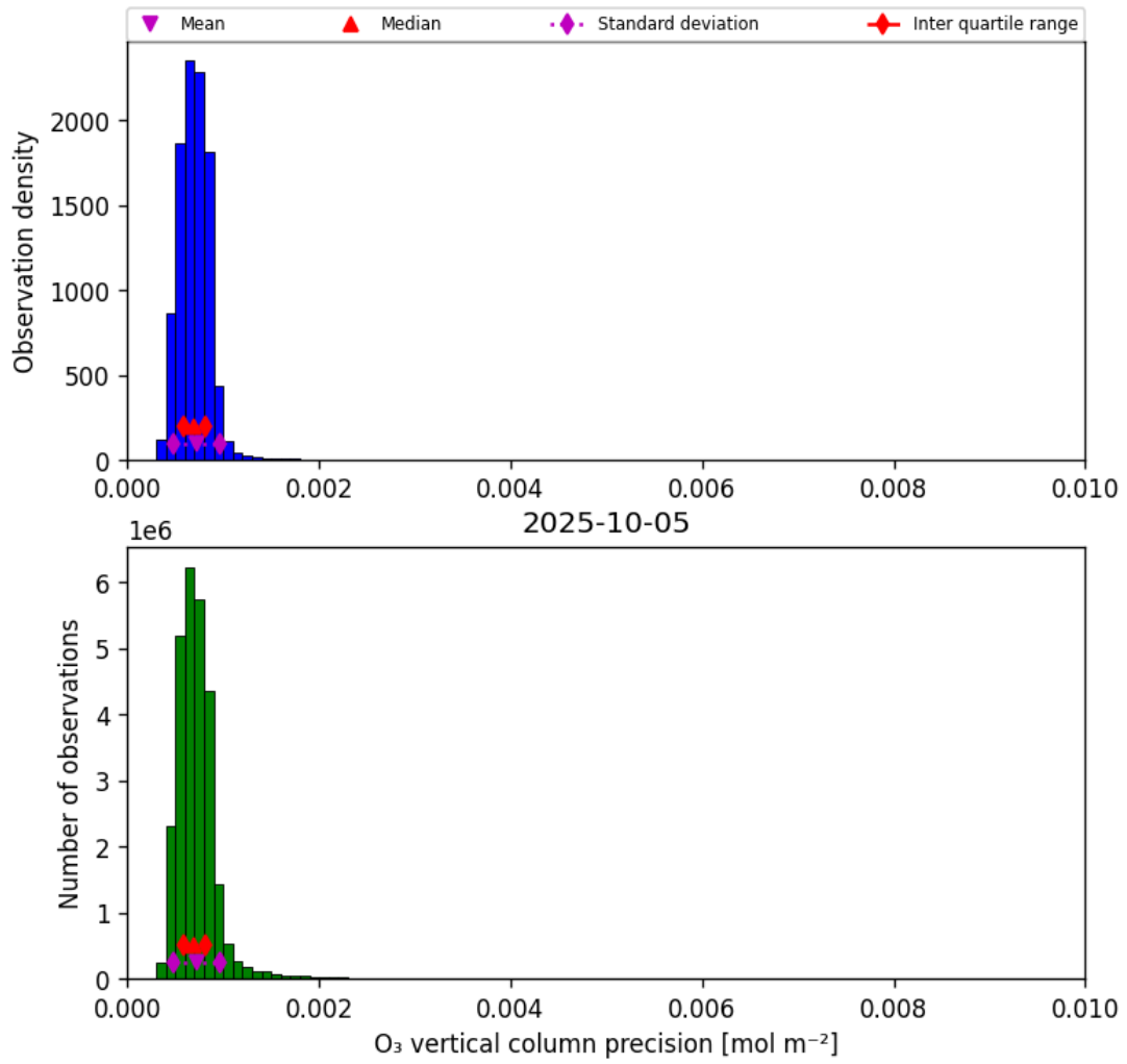
Figure 22: Histogram of “O 3 vertical column precision” for 2025-10-04 to 2025-10-06
