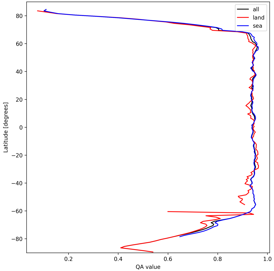
Figure 13: Zonal average of “QA value” for 2025-10-04 to 2025-10-06.
