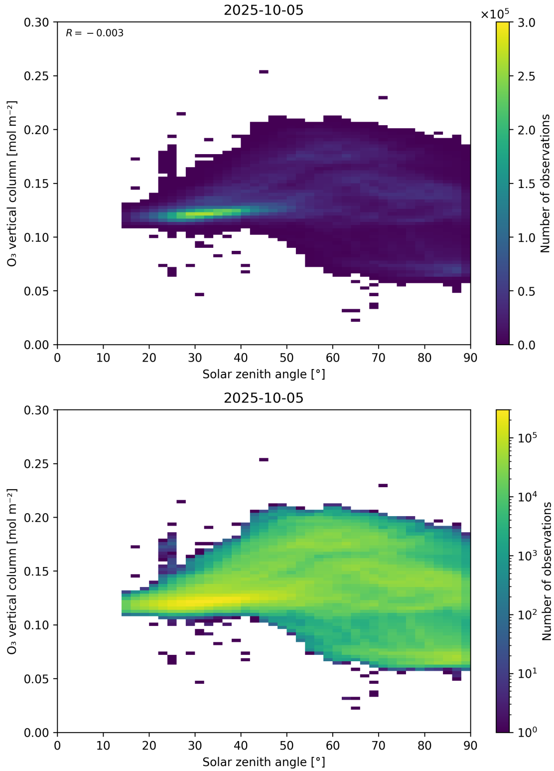
Figure 47: Scatter density plot of “Solar zenith angle” against “O 3 vertical column” for 2025-10-04 to 2025-10-06.
