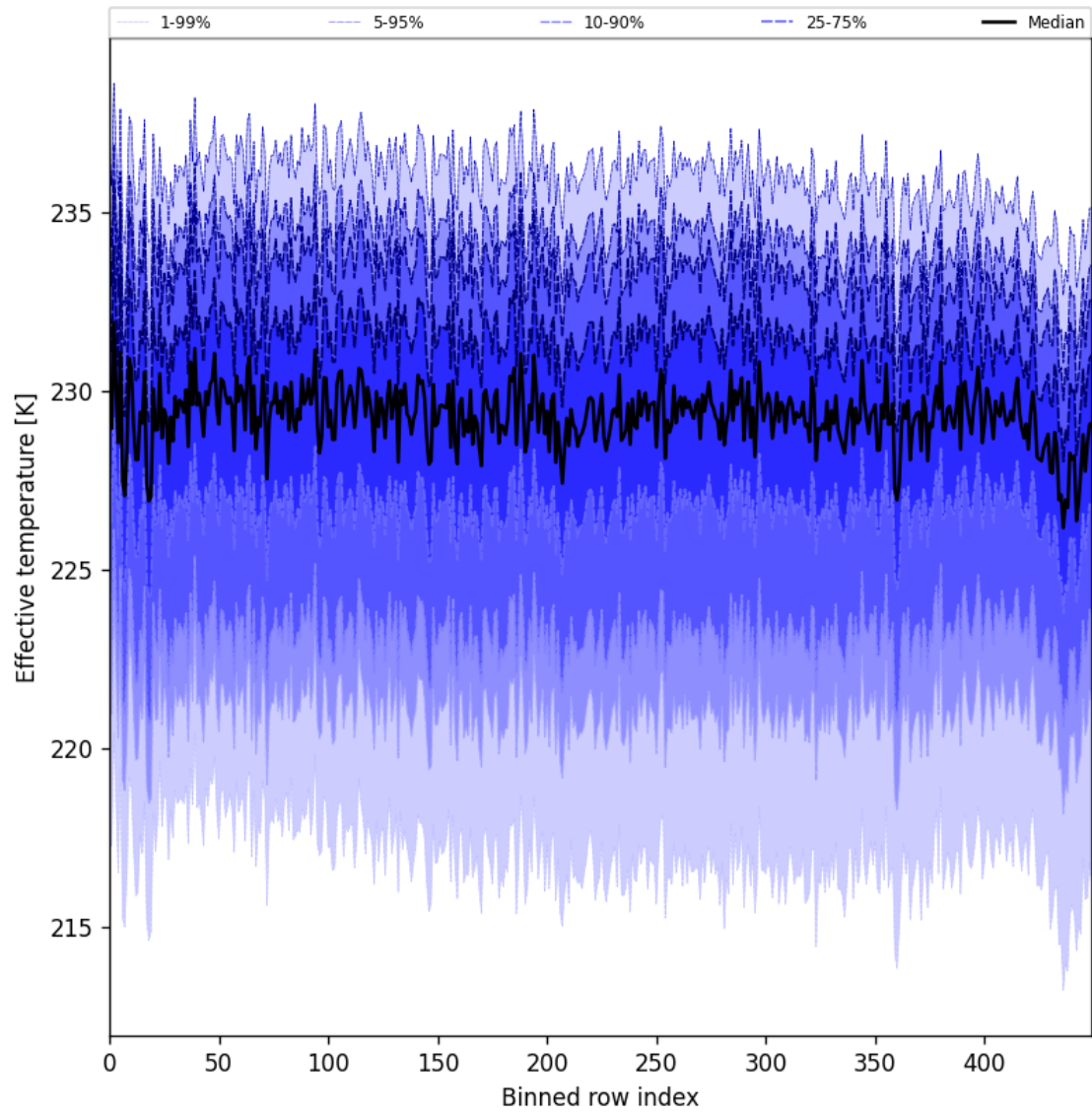
Figure 31: Along track statistics of “Effective temperature” for 2025-10-04 to 2025-10-06
