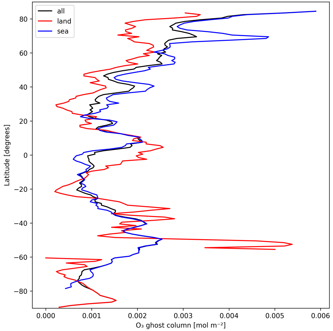
Figure 18: Zonal average of “O 3 ghost column” for 2025-10-04 to 2025-10-06.
