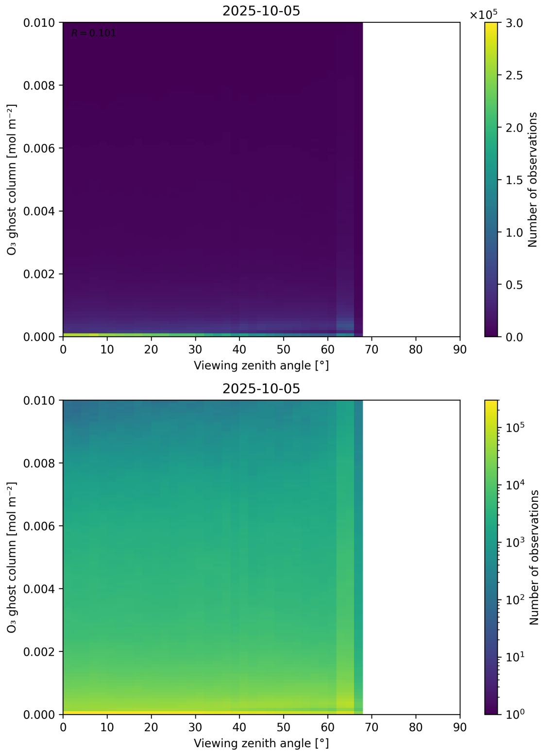
Figure 51: Scatter density plot of “Viewing zenith angle” against “O 3 ghost column” for 2025-10-04 to 2025-10-06.
