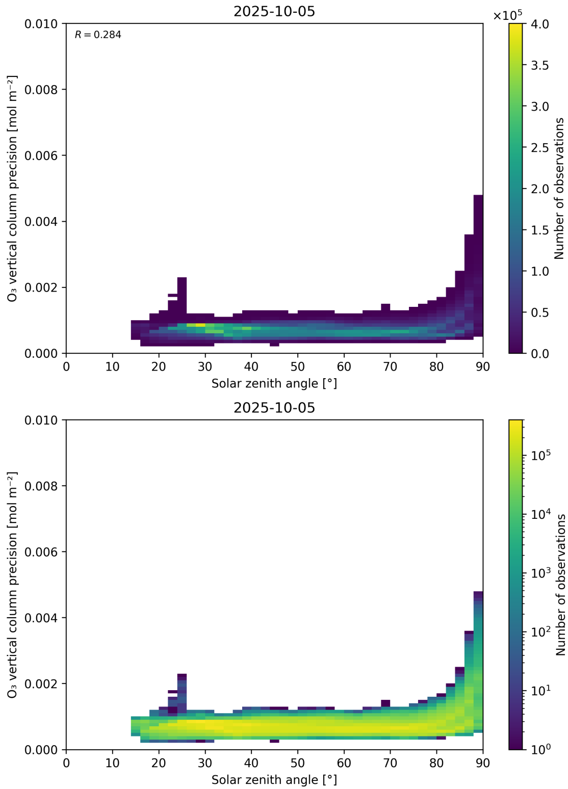
Figure 48: Scatter density plot of “Solar zenith angle” against “O 3 vertical column precision” for 2025-10-04 to 2025-10-06.
