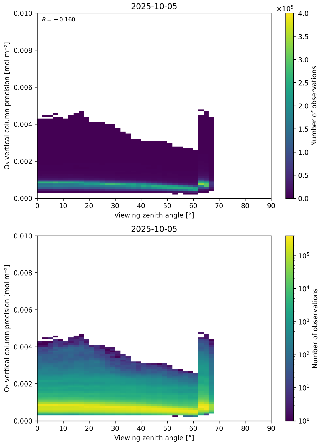
Figure 53: Scatter density plot of “Viewing zenith angle” against “O 3 vertical column precision” for 2025-10-04 to 2025-10-06.
