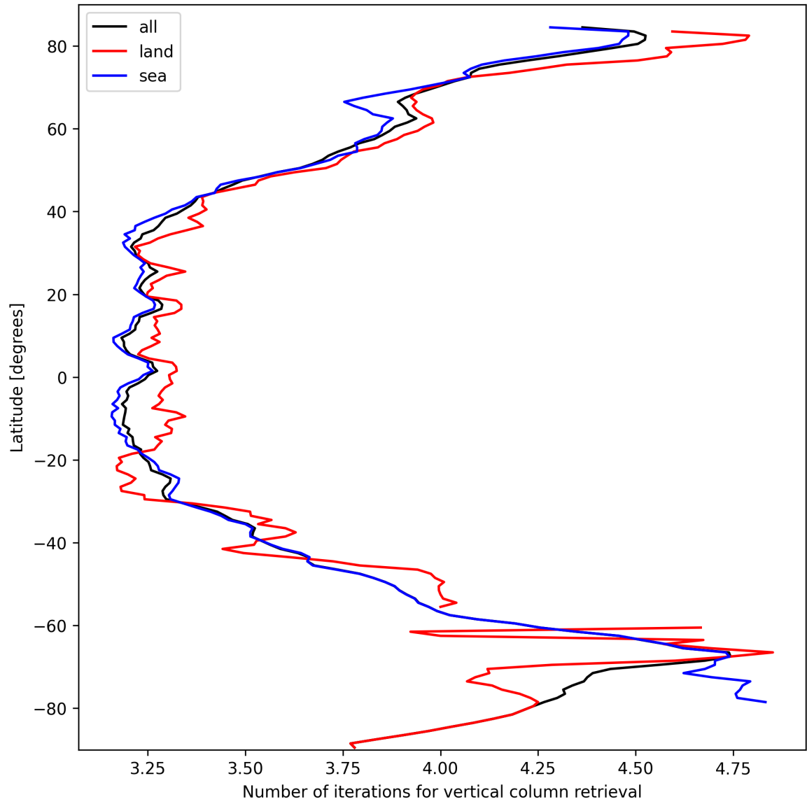
Figure 19: Zonal average of “Number of iterations for vertical column retrieval” for 2025-10-04 to 2025-10-06.
