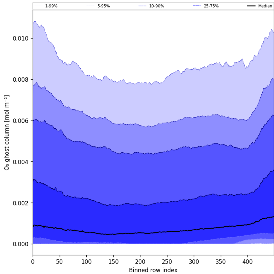
Figure 32: Along track statistics of “O 3 ghost column” for 2025-10-04 to 2025-10-06
