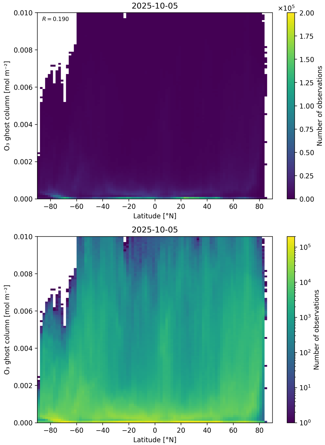
Figure 35: Scatter density plot of “Latitude” against “O 3 ghost column” for 2025-10-04 to 2025-10-06.
