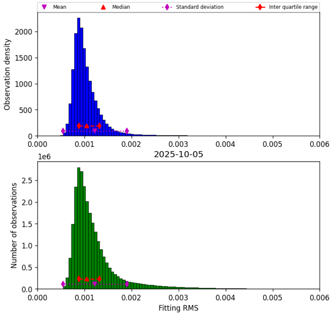
Figure 23: Histogram of “Fitting RMS” for 2025-10-04 to 2025-10-06
