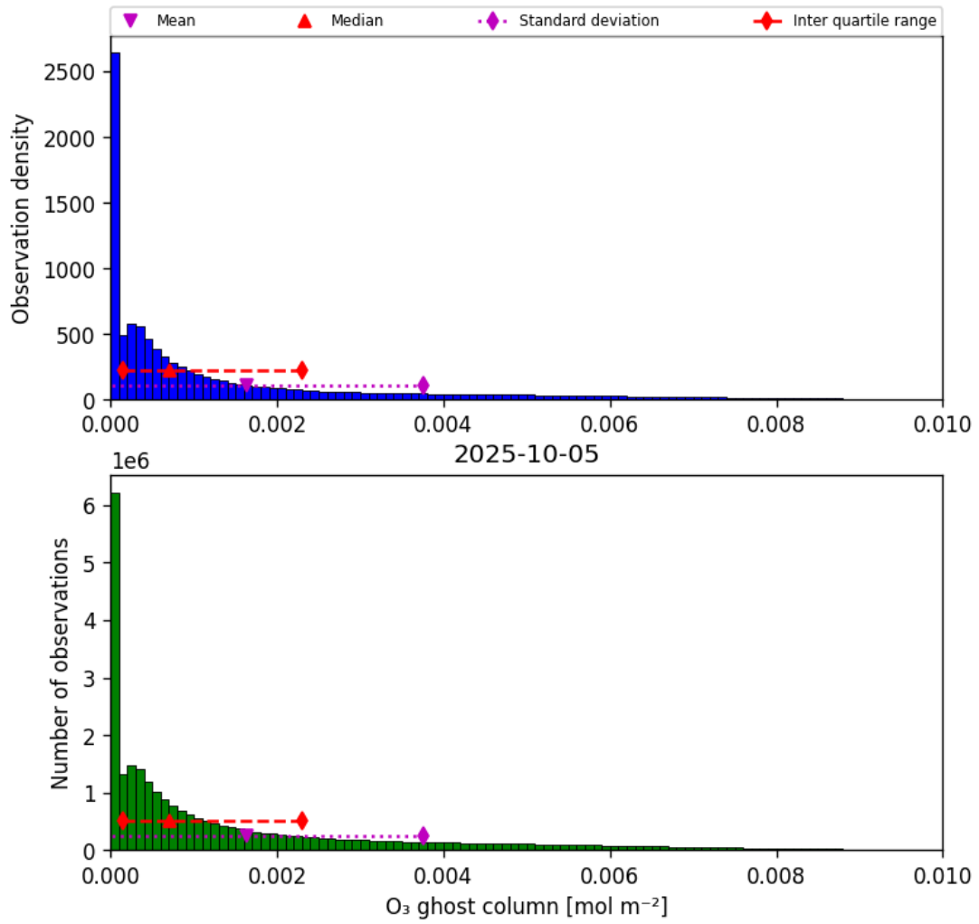
Figure 25: Histogram of “O 3 ghost column” for 2025-10-04 to 2025-10-06
