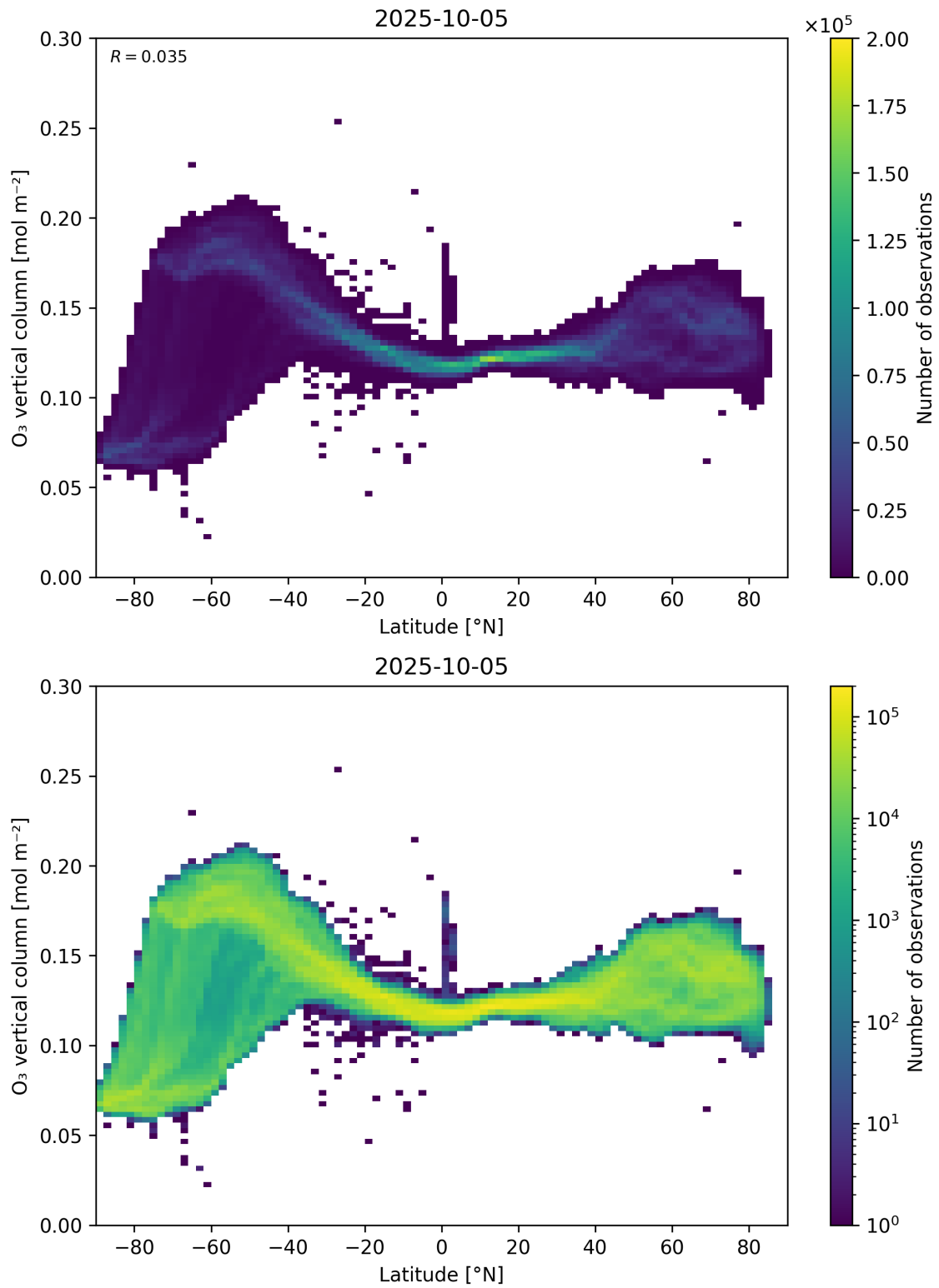
Figure 36: Scatter density plot of “Latitude” against “O 3 vertical column” for 2025-10-04 to 2025-10-06.
