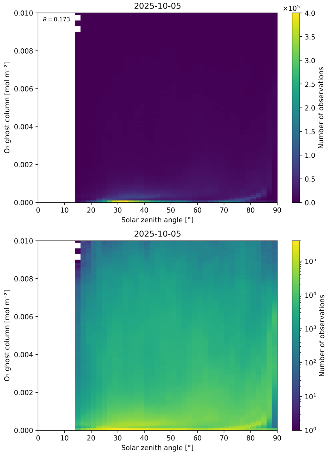
Figure 46: Scatter density plot of “Solar zenith angle” against “O 3 ghost column” for 2025-10-04 to 2025-10-06.
