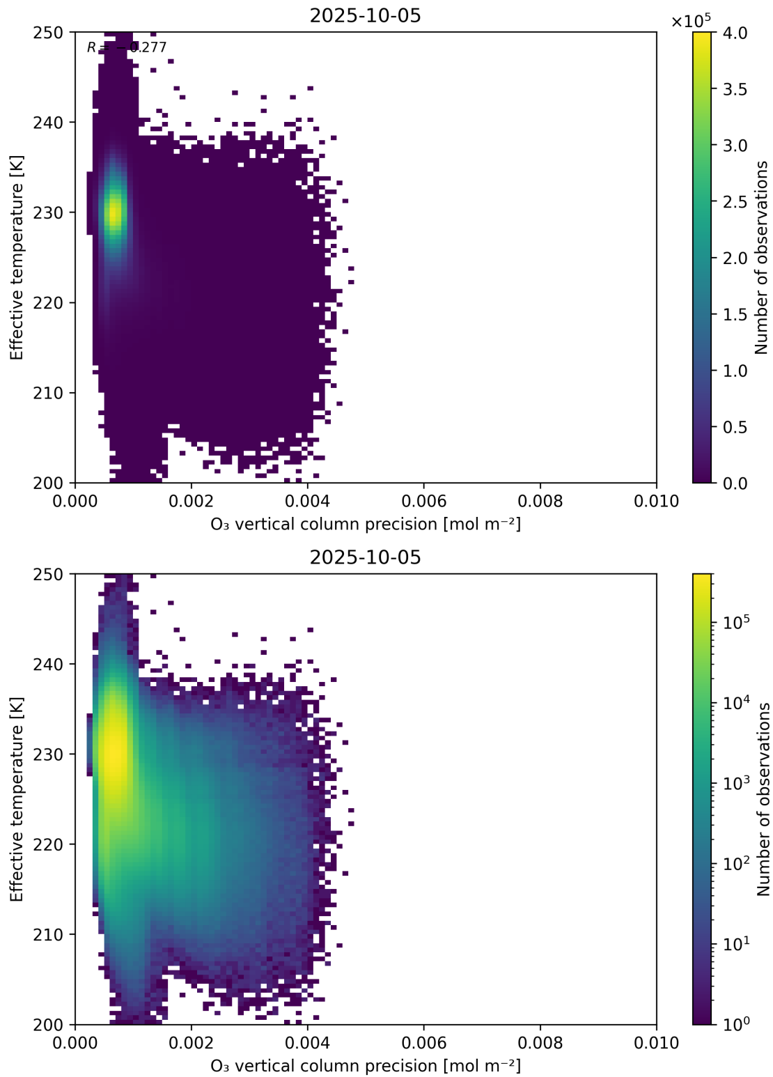
Figure 42: Scatter density plot of “ O_3 vertical column precision” against “Effective temperature” for 2025-10-04 to 2025-10-06.
