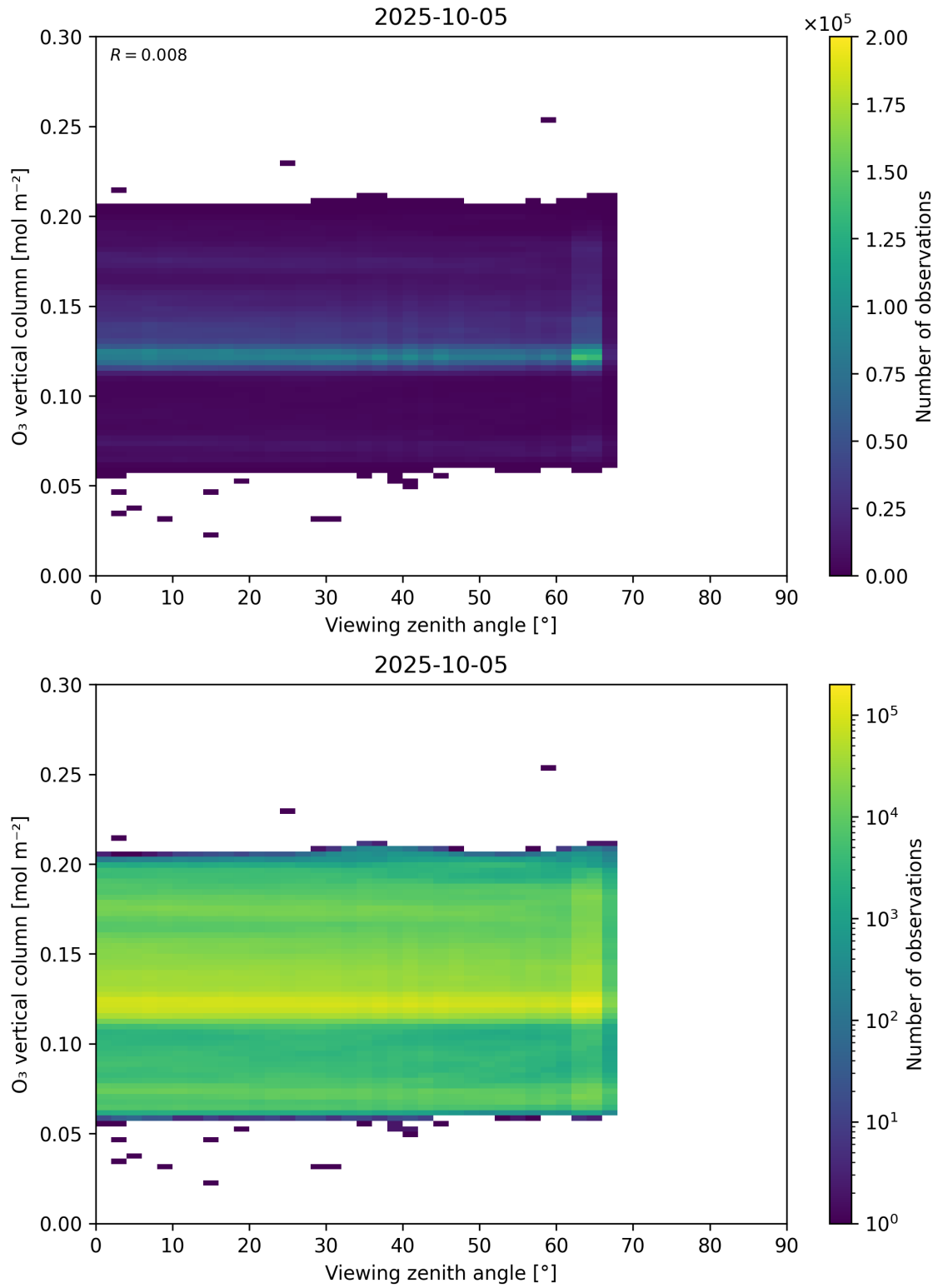
Figure 52: Scatter density plot of “Viewing zenith angle” against “O 3 vertical column” for 2025-10-04 to 2025-10-06.
