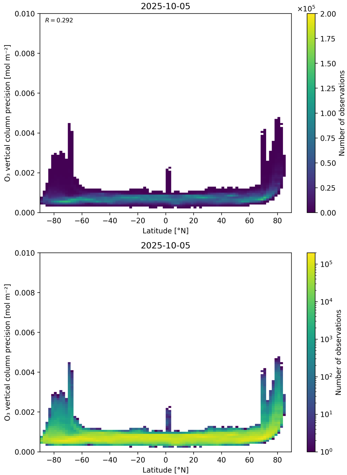
Figure 37: Scatter density plot of “Latitude” against “O 3 vertical column precision” for 2025-10-04 to 2025-10-06.
