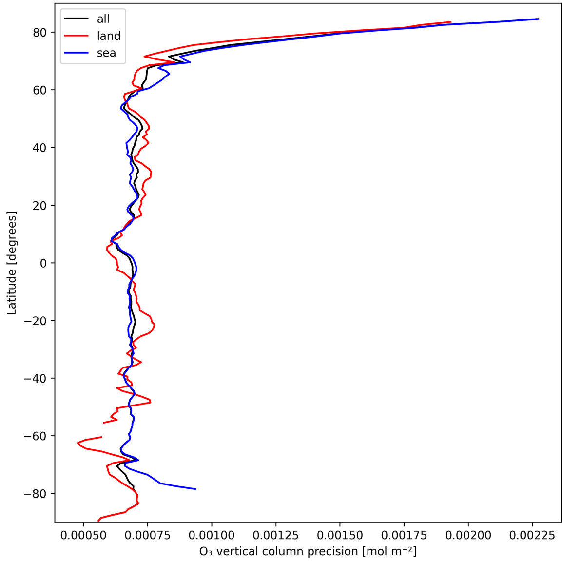
Figure 15: Zonal average of “O 3 vertical column precision” for 2025-10-04 to 2025-10-06.
