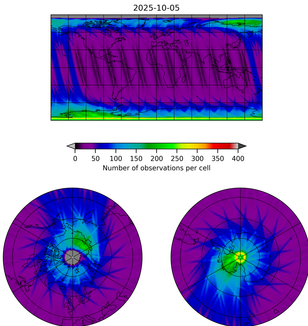
Figure 12: Map of the number of observations for 2025-10-04 to 2025-10-06
