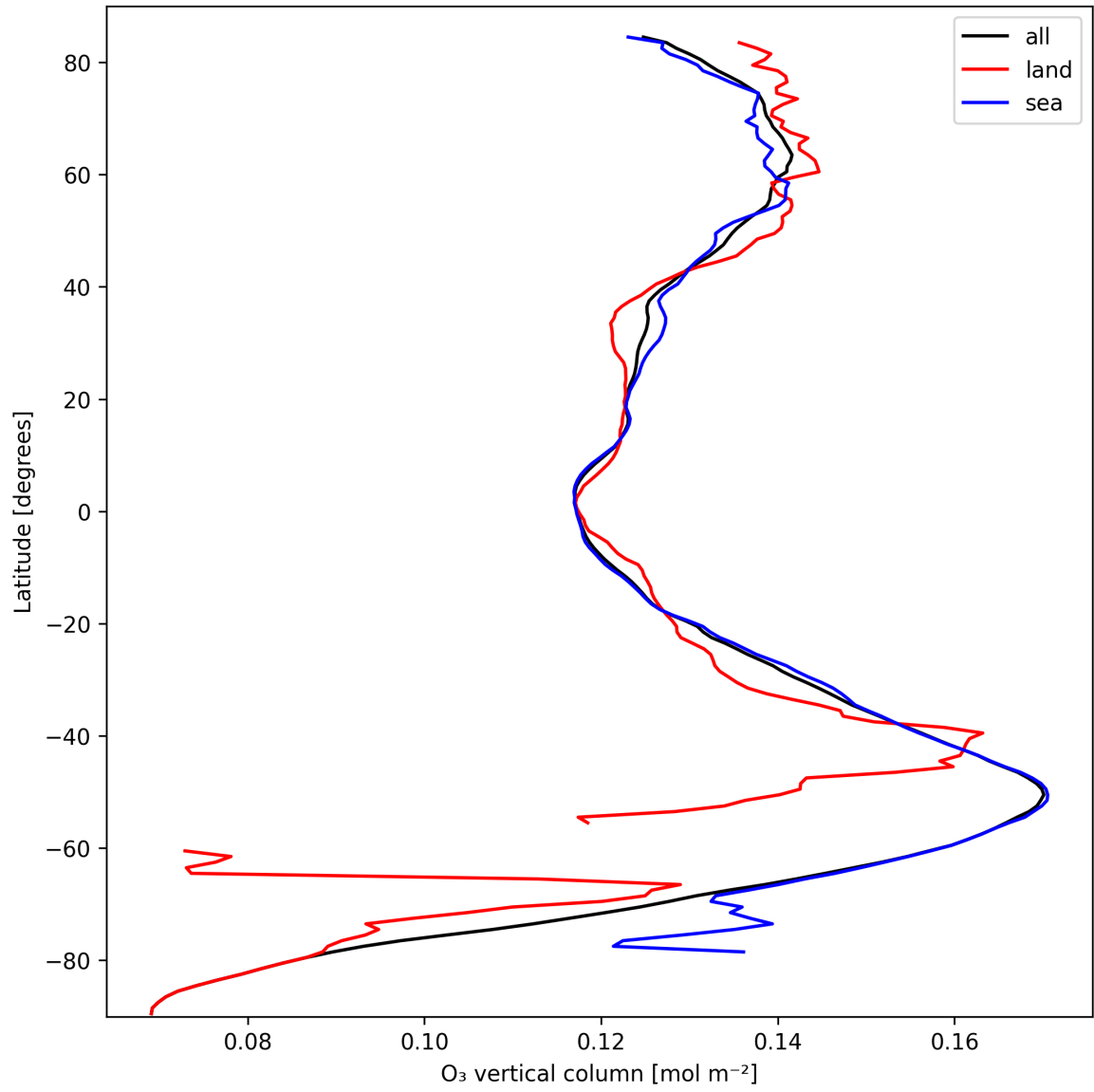
Figure 14: Zonal average of “O 3 vertical column” for 2025-10-04 to 2025-10-06.
