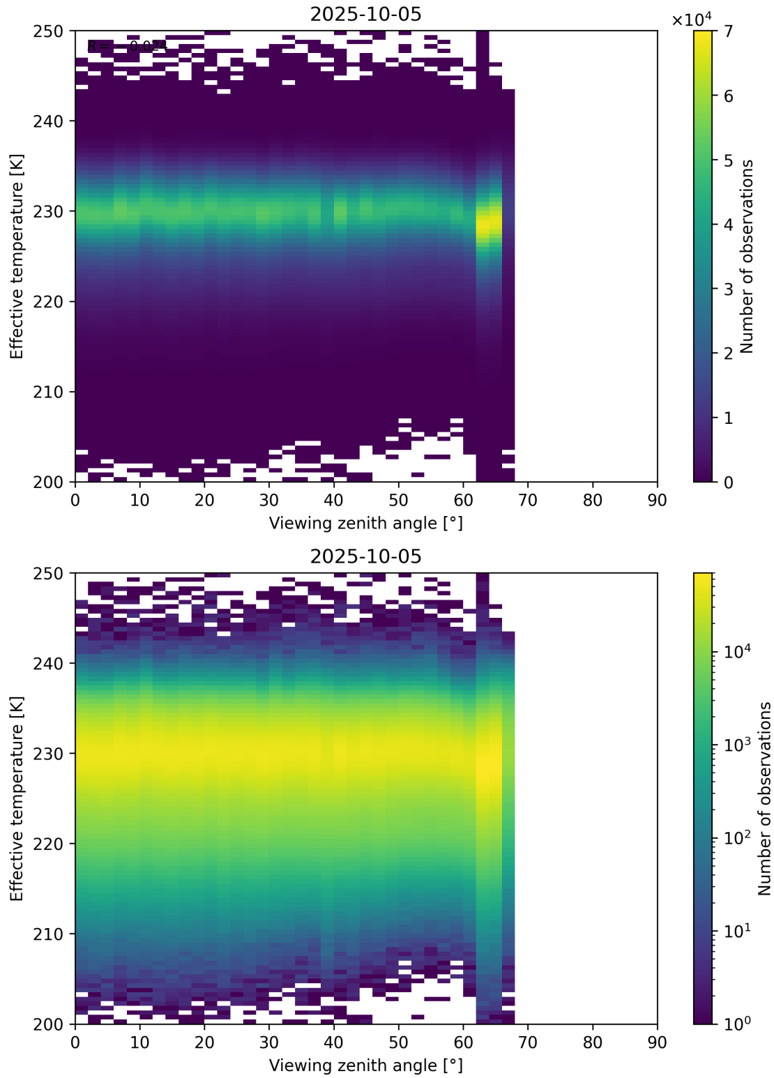
Figure 50: Scatter density plot of “Viewing zenith angle” against “Effective temperature” for 2025-10-04 to 2025-10-06.
