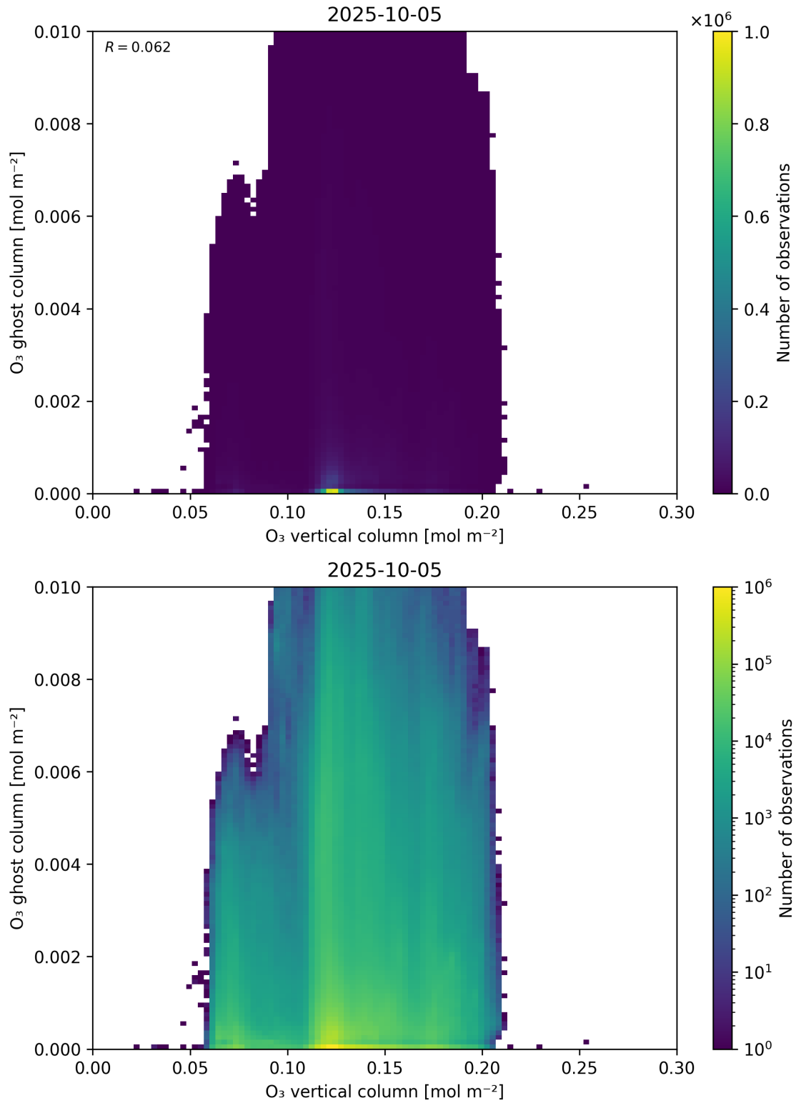
Figure 40: Scatter density plot of “O 3 vertical column” against “O 3 ghost column” for 2025-10-04 to 2025-10-06.
