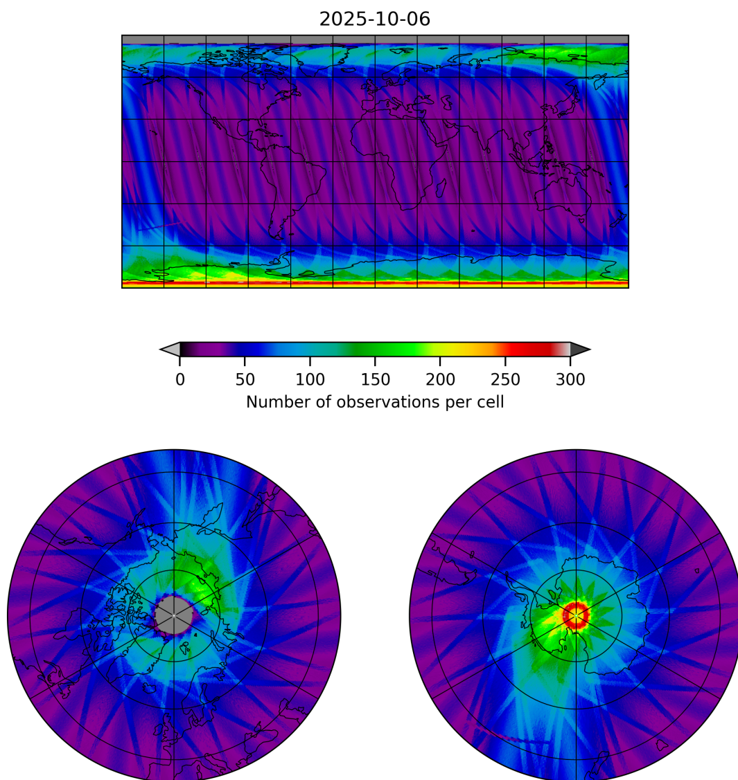
Figure 12: Map of the number of observations for 2025-10-06 to 2025-10-07
