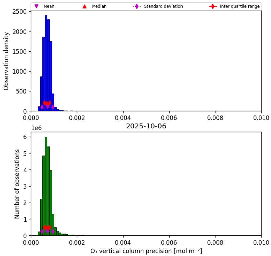
Figure 22: Histogram of “O 3 vertical column precision” for 2025-10-06 to 2025-10-07
