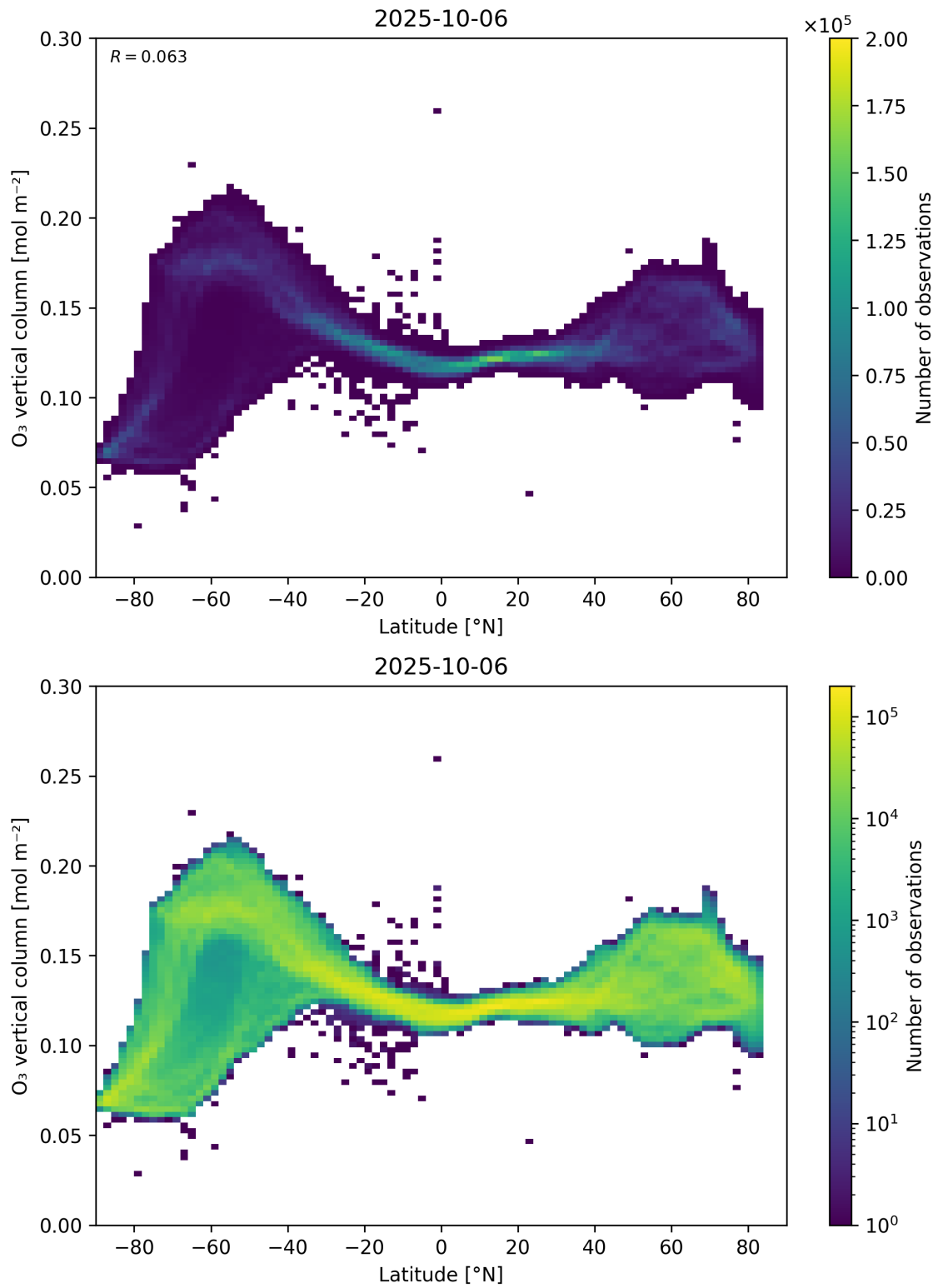
Figure 36: Scatter density plot of “Latitude” against “O 3 vertical column” for 2025-10-06 to 2025-10-07.
