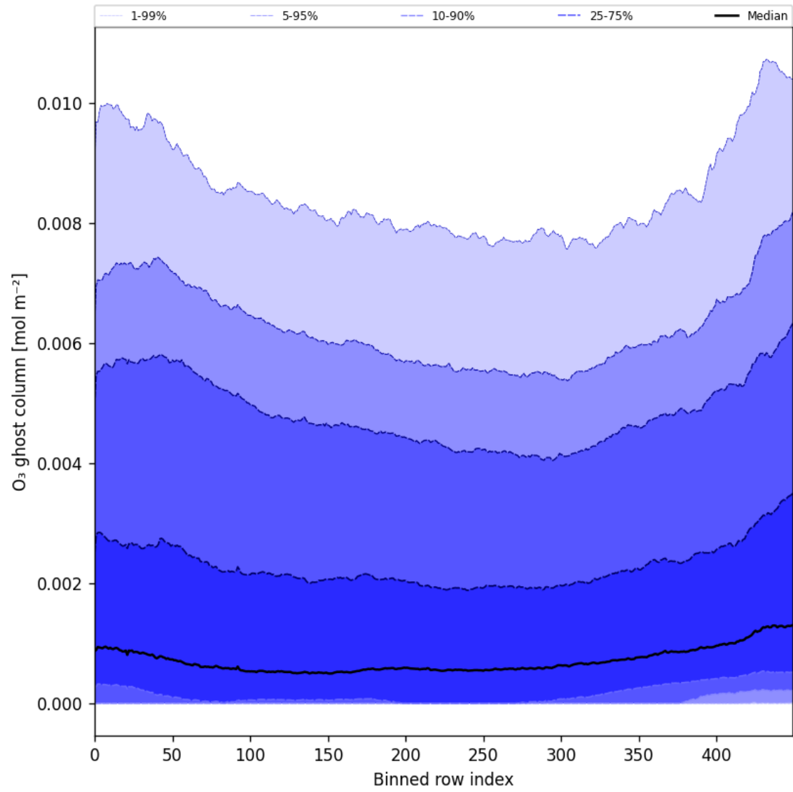
Figure 32: Along track statistics of “O 3 ghost column” for 2025-10-06 to 2025-10-07
