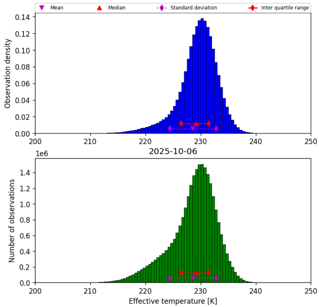
Figure 24: Histogram of “Effective temperature” for 2025-10-06 to 2025-10-07
