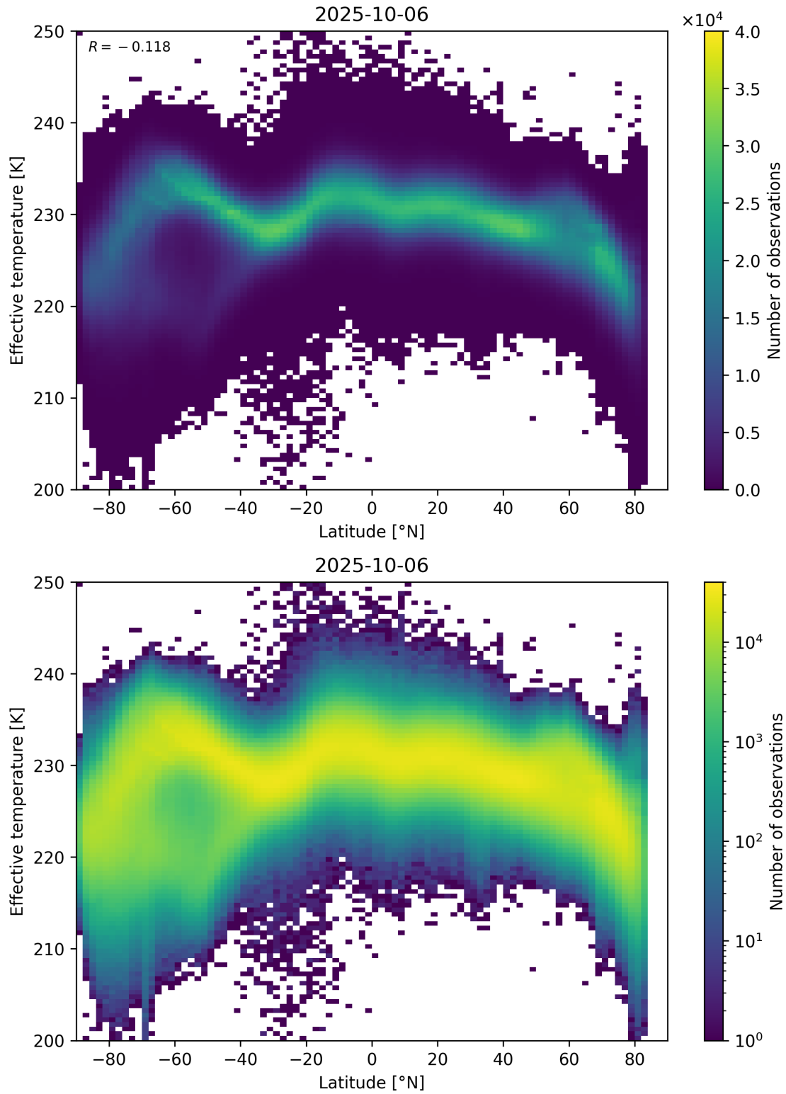
Figure 34: Scatter density plot of “Latitude” against “Effective temperature” for 2025-10-06 to 2025-10-07.
