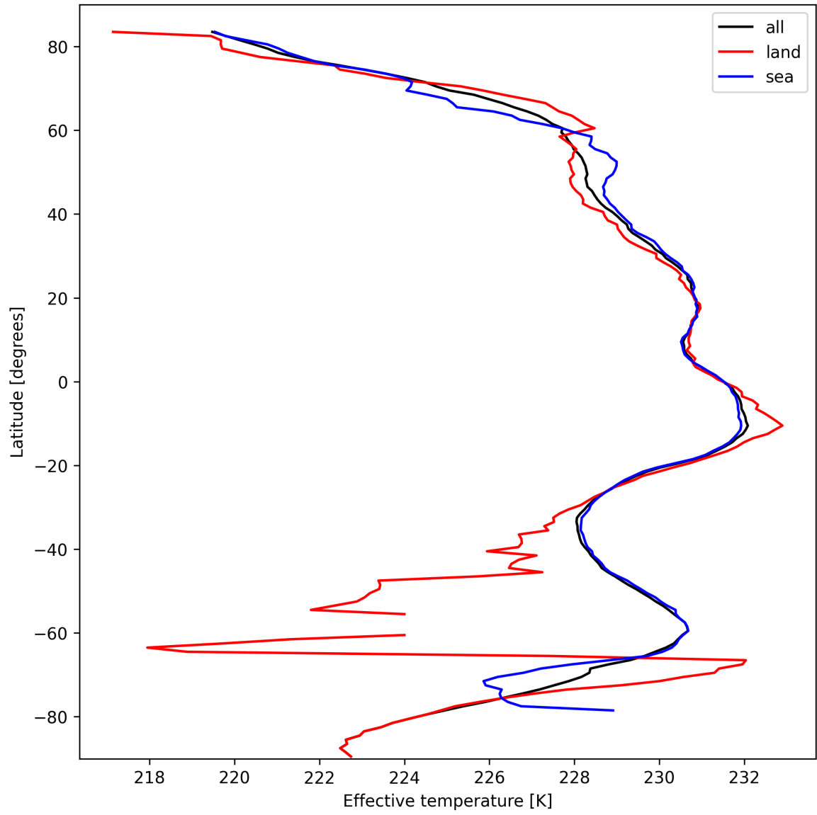
Figure 17: Zonal average of “Effective temperature” for 2025-10-06 to 2025-10-07.
