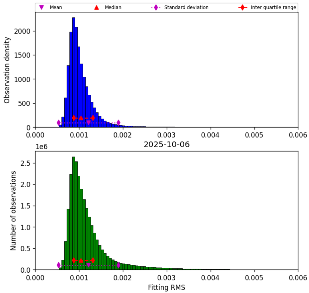
Figure 23: Histogram of “Fitting RMS” for 2025-10-06 to 2025-10-07
