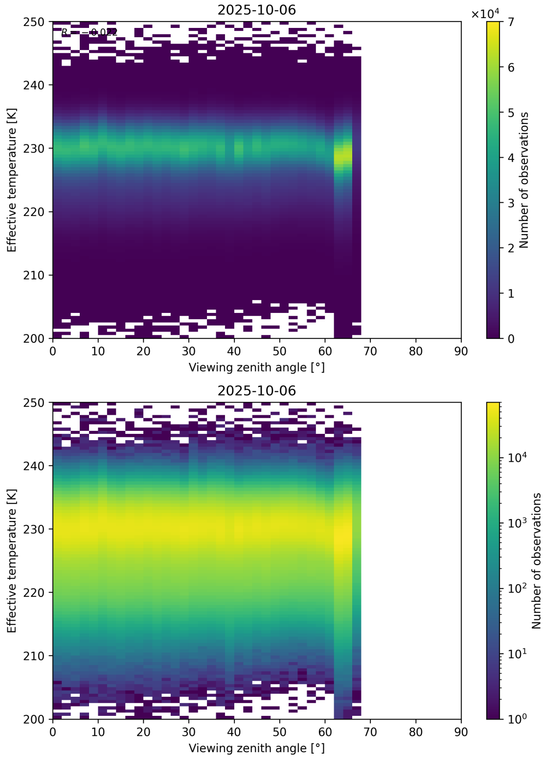
Figure 50: Scatter density plot of “Viewing zenith angle” against “Effective temperature” for 2025-10-06 to 2025-10-07.
