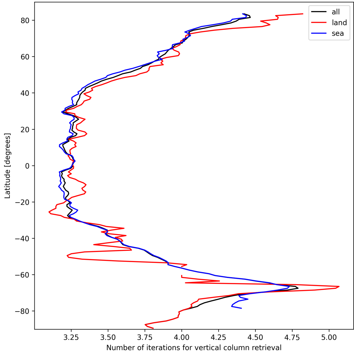
Figure 19: Zonal average of “Number of iterations for vertical column retrieval” for 2025-10-06 to 2025-10-07.
