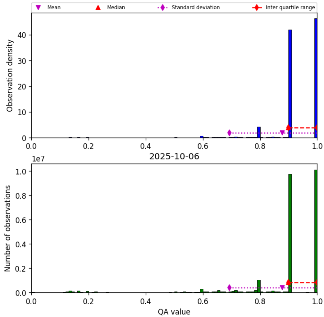
Figure 20: Histogram of “QA value” for 2025-10-06 to 2025-10-07
