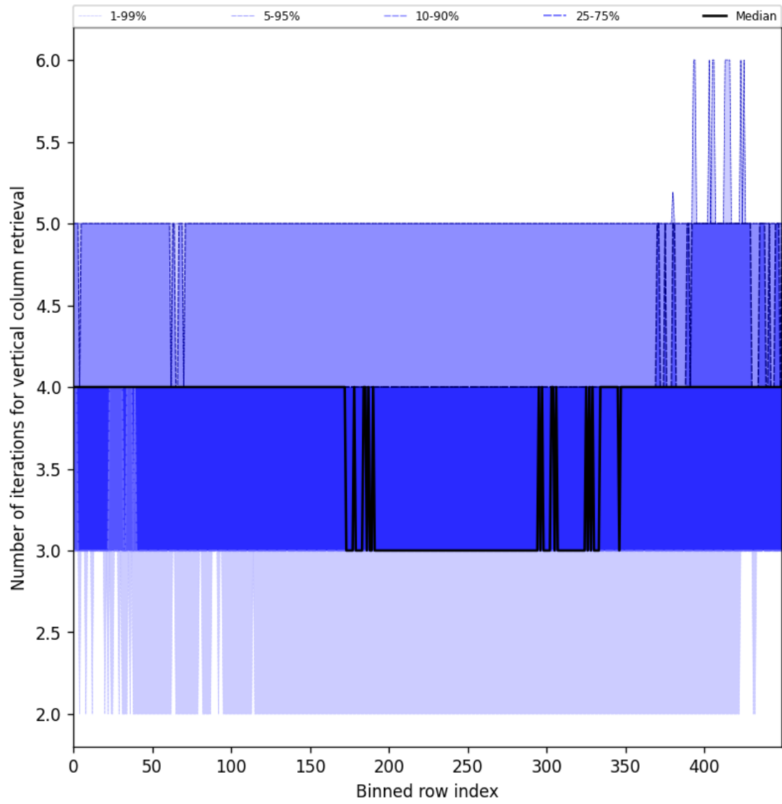
Figure 33: Along track statistics of “Number of iterations for vertical column retrieval” for 2025-10-06 to 2025-10-07
