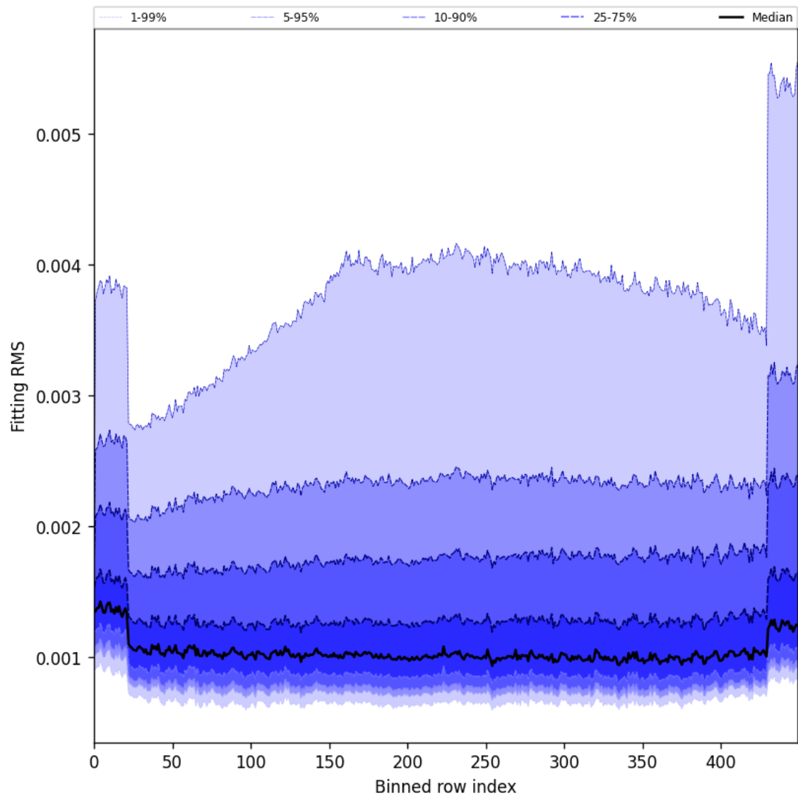
Figure 30: Along track statistics of “Fitting RMS” for 2025-10-06 to 2025-10-07
