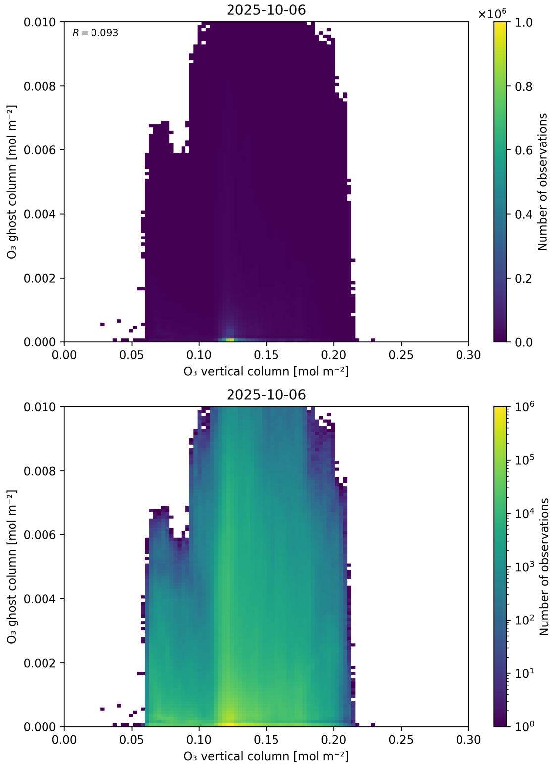
Figure 40: Scatter density plot of “O 3 vertical column” against “O 3 ghost column” for 2025-10-06 to 2025-10-07.
