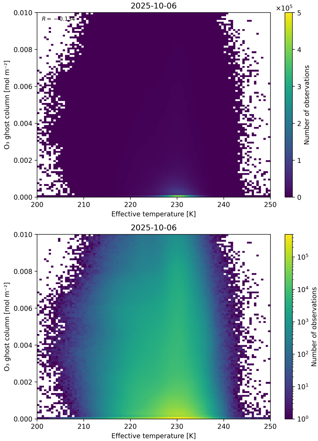
Figure 38: Scatter density plot of “Effective temperature” against “O 3 ghost column” for 2025-10-06 to 2025-10-07.
