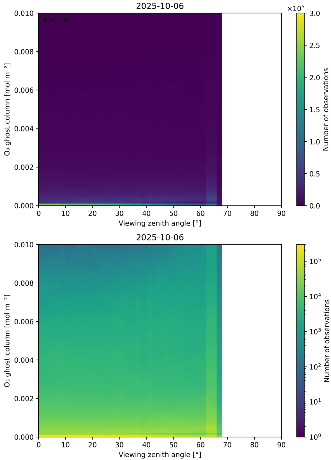
Figure 51: Scatter density plot of “Viewing zenith angle” against “O 3 ghost column” for 2025-10-06 to 2025-10-07.
