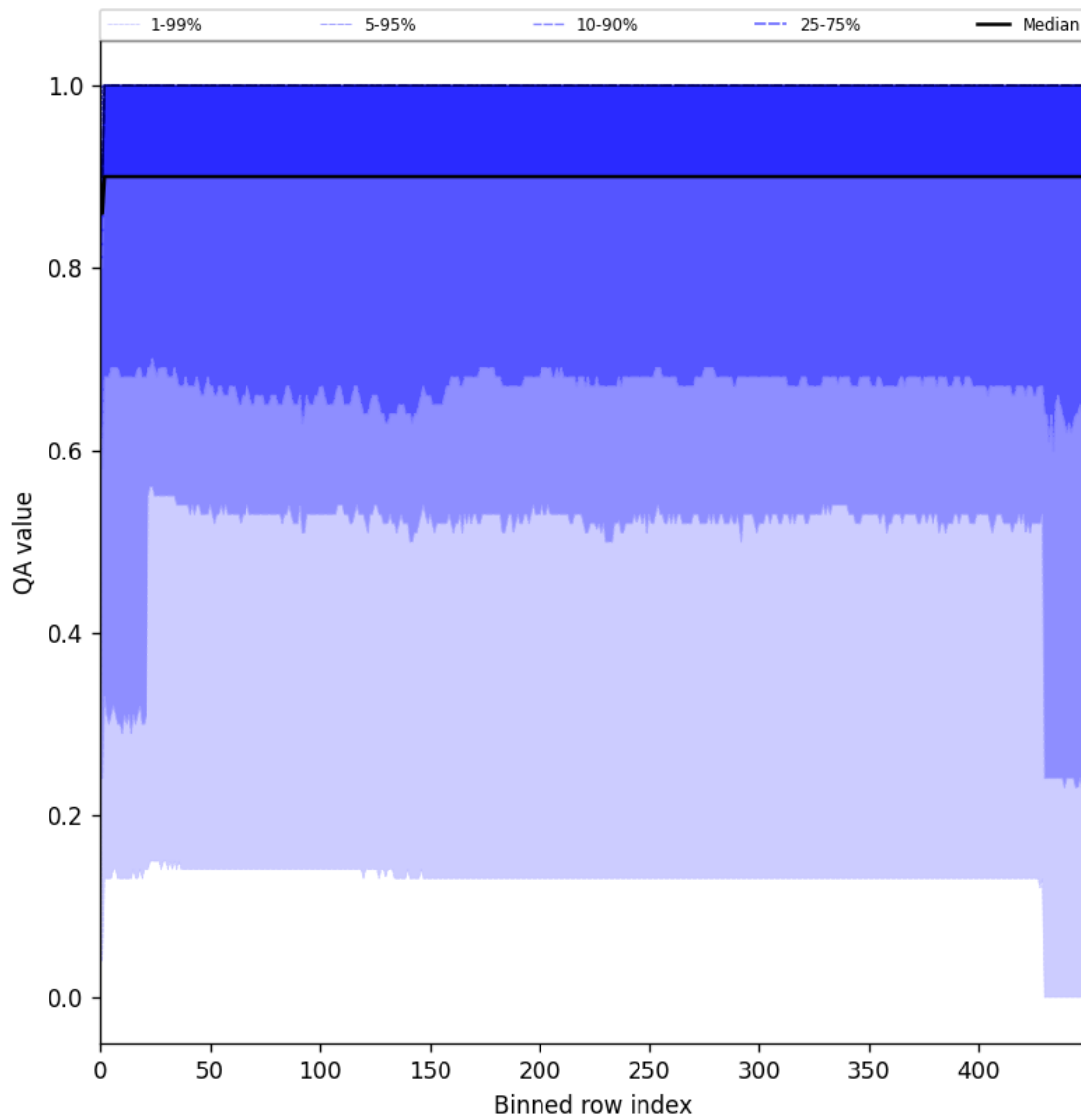
Figure 27: Along track statistics of “QA value” for 2025-10-06 to 2025-10-07
