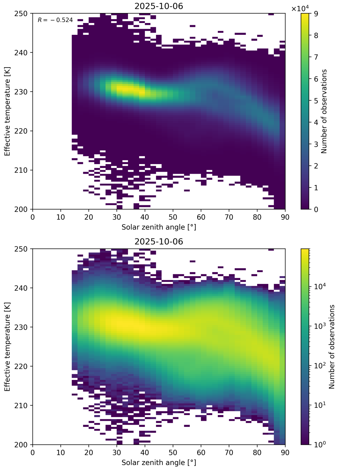
Figure 45: Scatter density plot of “Solar zenith angle” against “Effective temperature” for 2025-10-06 to 2025-10-07.
