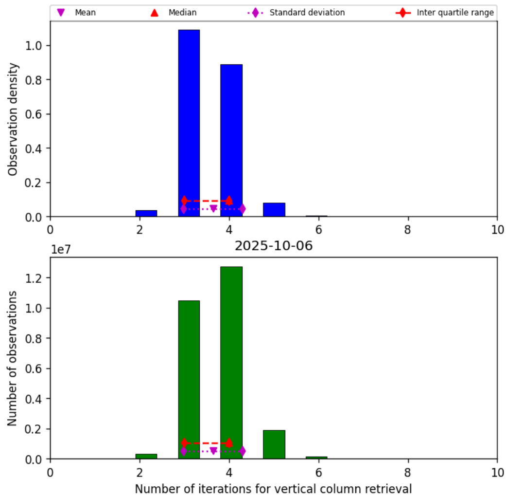
Figure 26: Histogram of “Number of iterations for vertical column retrieval” for 2025-10-06 to 2025-10-07
