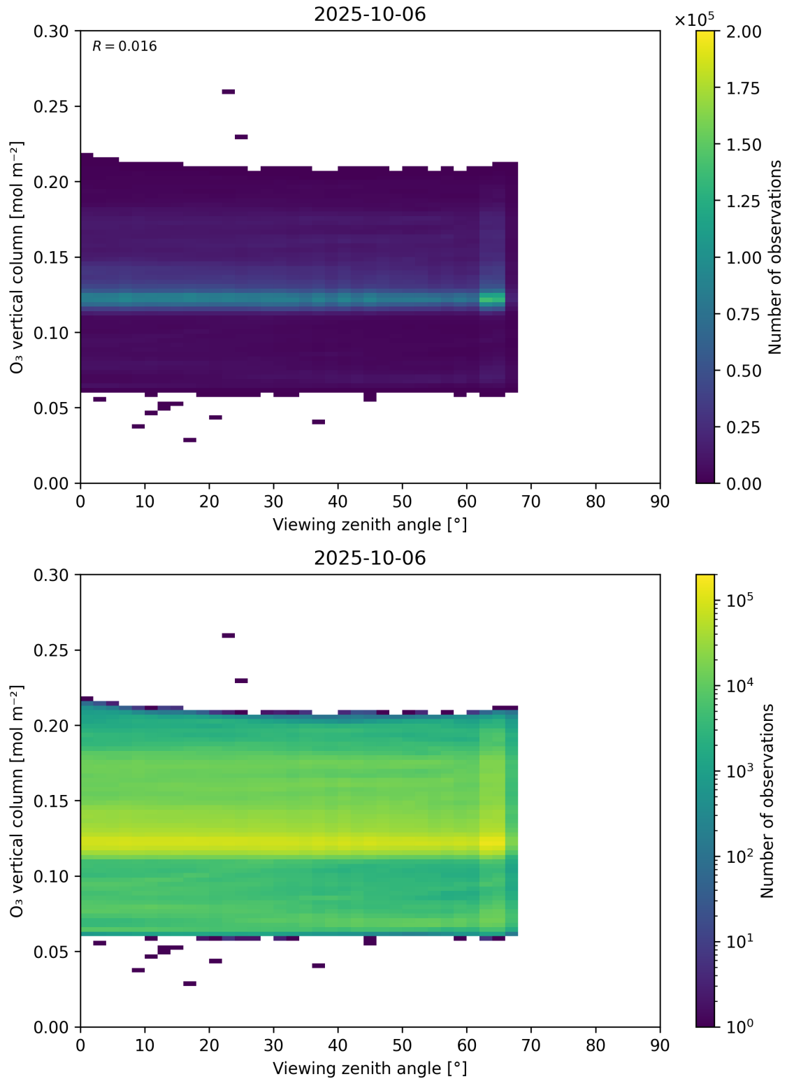
Figure 52: Scatter density plot of “Viewing zenith angle” against “O 3 vertical column” for 2025-10-06 to 2025-10-07.
