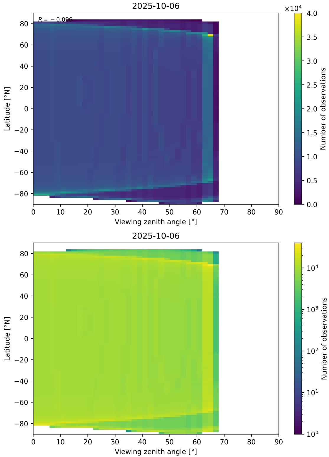
Figure 49: Scatter density plot of “Viewing zenith angle” against “Latitude” for 2025-10-06 to 2025-10-07.
