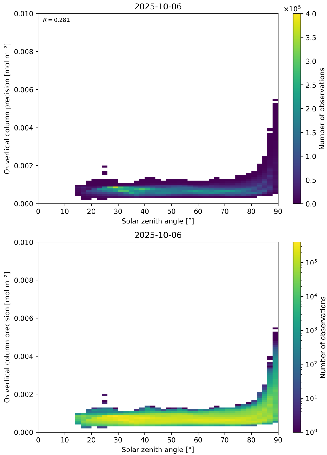
Figure 48: Scatter density plot of “Solar zenith angle” against “O 3 vertical column precision” for 2025-10-06 to 2025-10-07.
