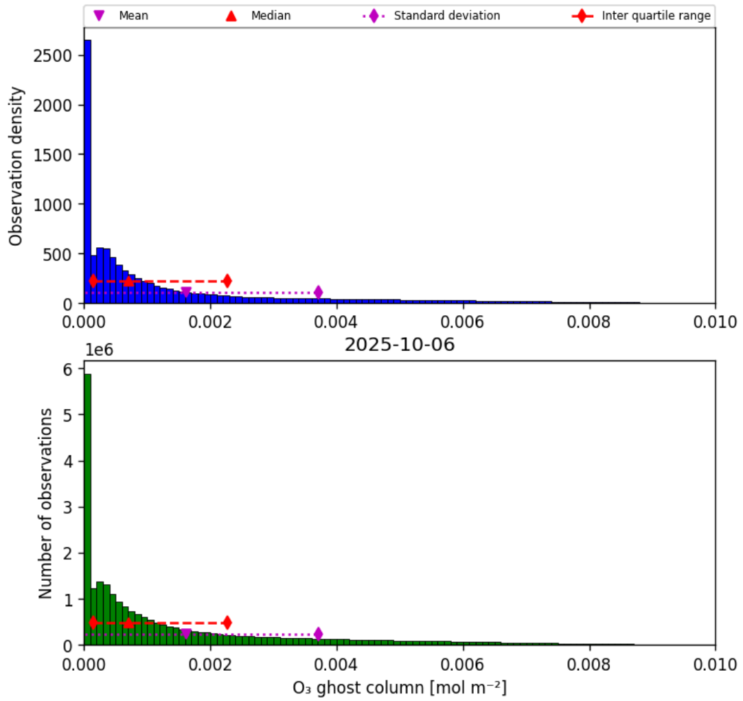
Figure 25: Histogram of “O 3 ghost column” for 2025-10-06 to 2025-10-07
