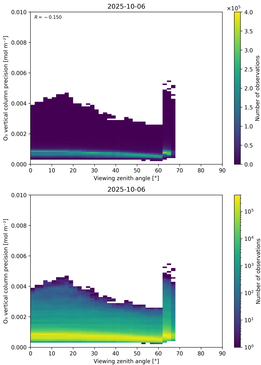
Figure 53: Scatter density plot of “Viewing zenith angle” against “O 3 vertical column precision” for 2025-10-06 to 2025-10-07.
