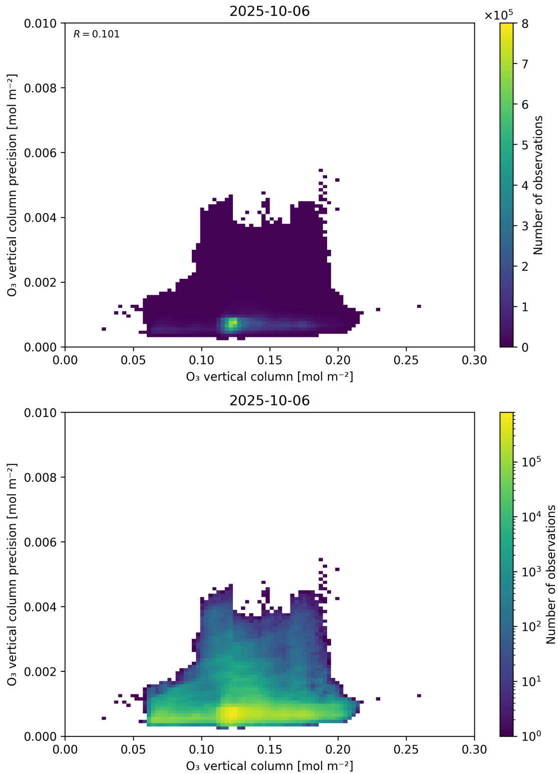
Figure 41: Scatter density plot of “O 3 vertical column” against “O 3 vertical column precision” for 2025-10-06 to 2025-10-07.
