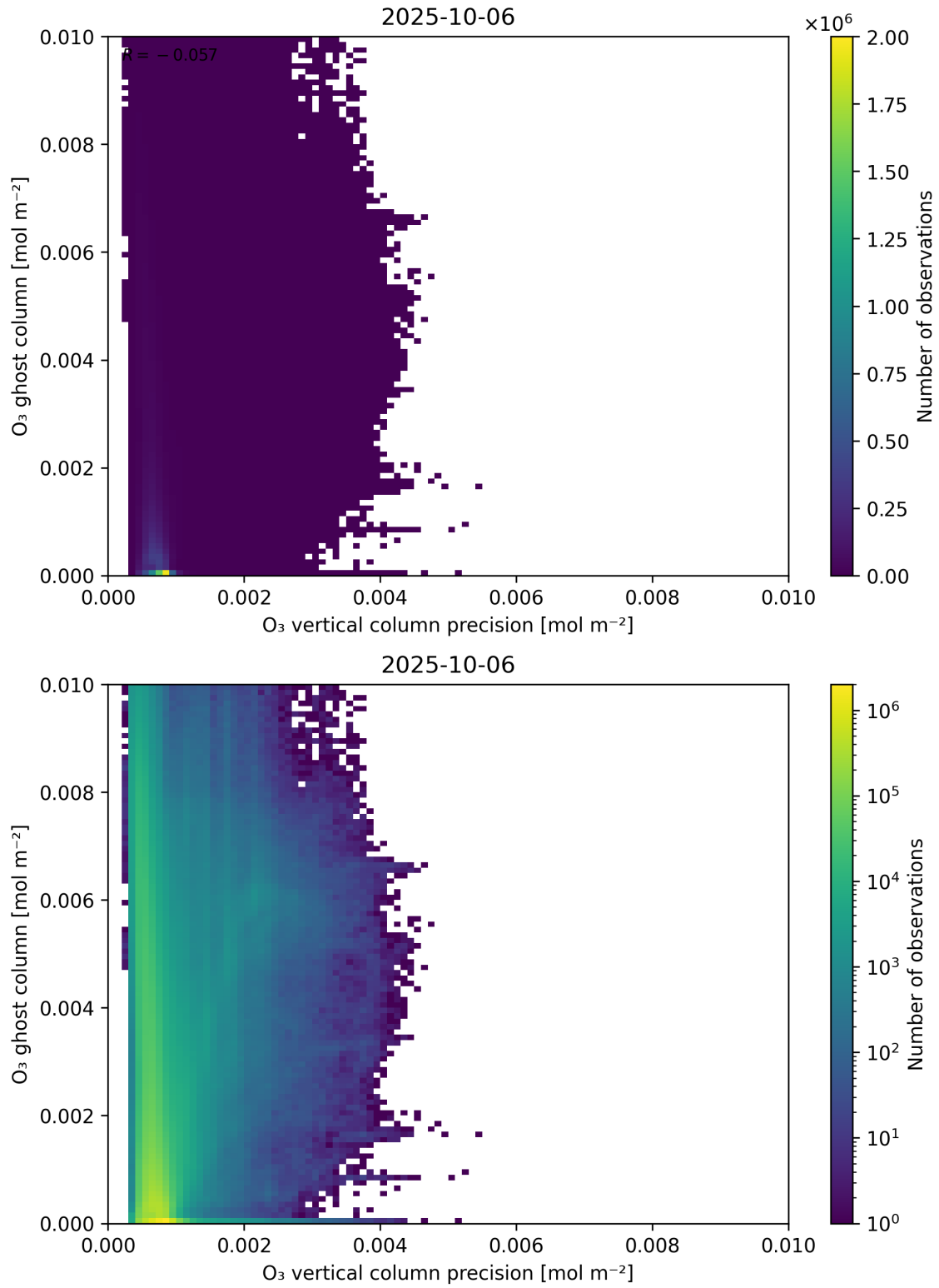
Figure 43: Scatter density plot of “O 3 vertical column precision” against “O 3 ghost column” for 2025-10-06 to 2025-10-07.
