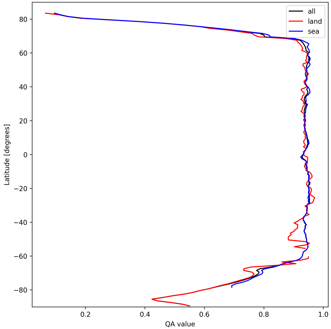
Figure 13: Zonal average of “QA value” for 2025-10-06 to 2025-10-07.
