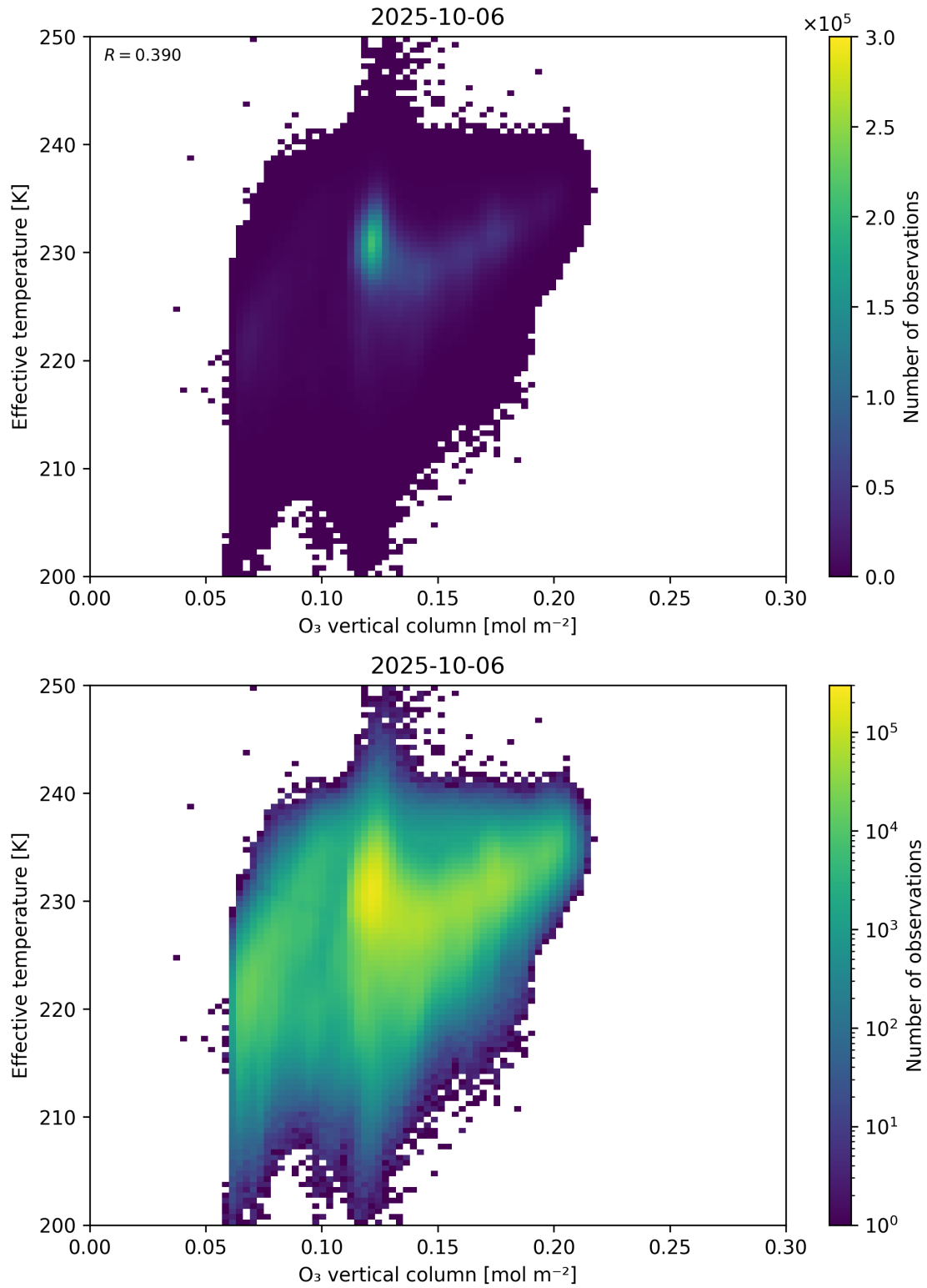
Figure 39: Scatter density plot of “O 3 vertical column” against “Effective temperature” for 2025-10-06 to 2025-10-07.
