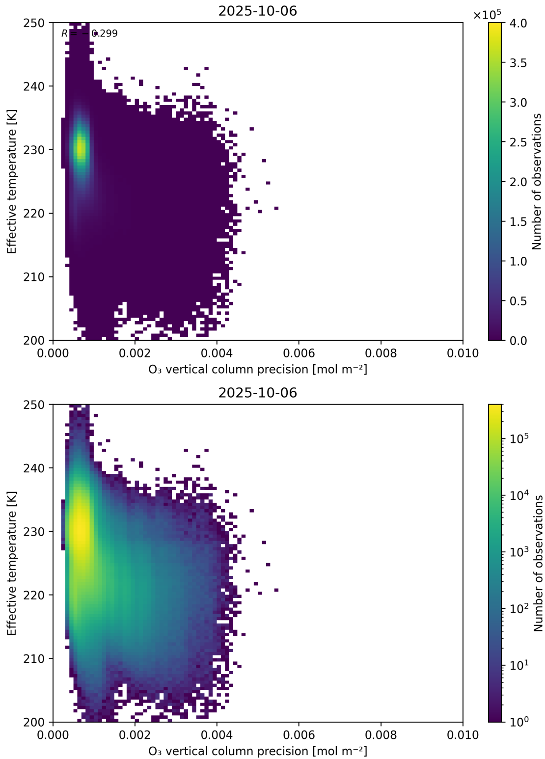
Figure 42: Scatter density plot of “O 3 vertical column precision” against “Effective temperature” for 2025-10-06 to 2025-10-07.
