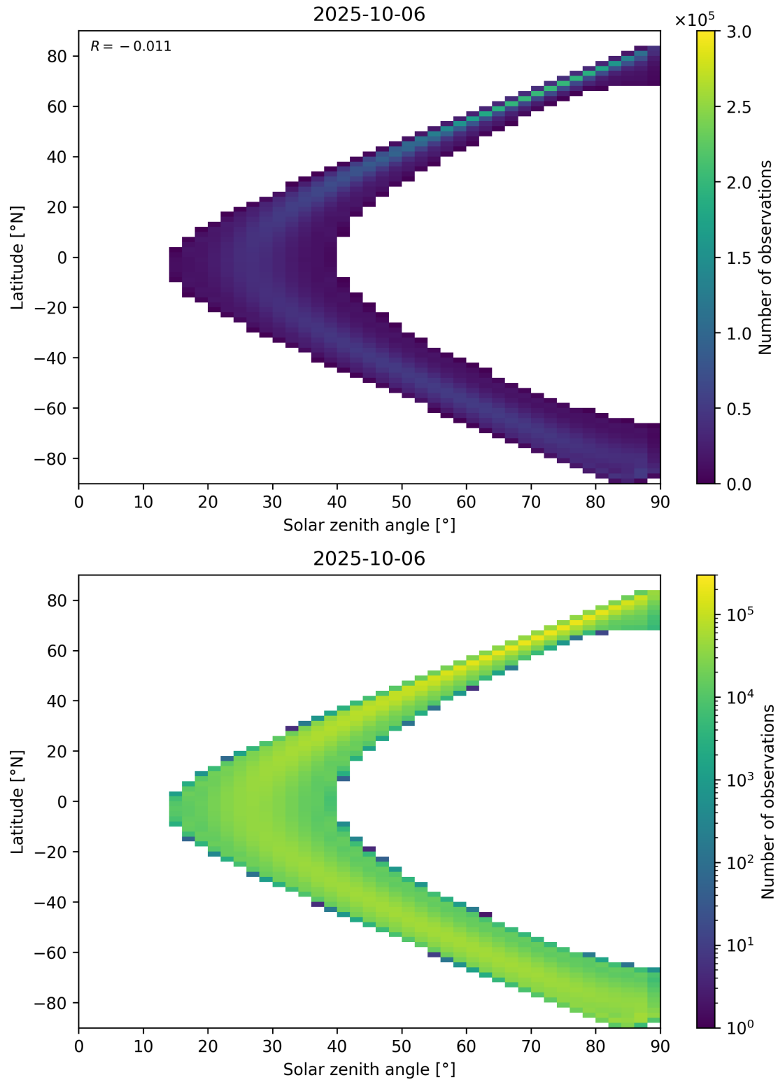
Figure 44: Scatter density plot of “Solar zenith angle” against “Latitude” for 2025-10-06 to 2025-10-07.
