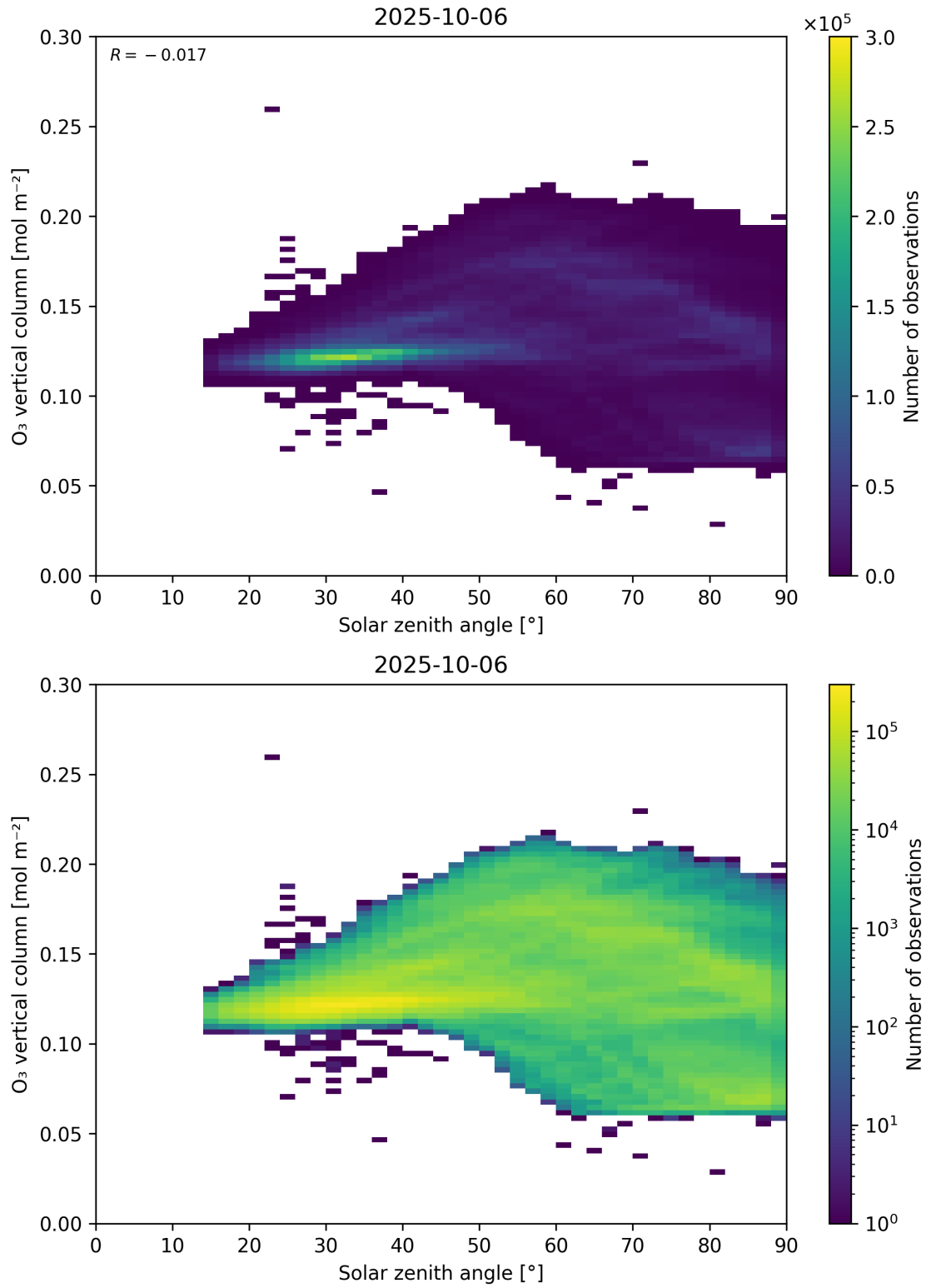
Figure 47: Scatter density plot of “Solar zenith angle” against “O 3 vertical column” for 2025-10-06 to 2025-10-07.
