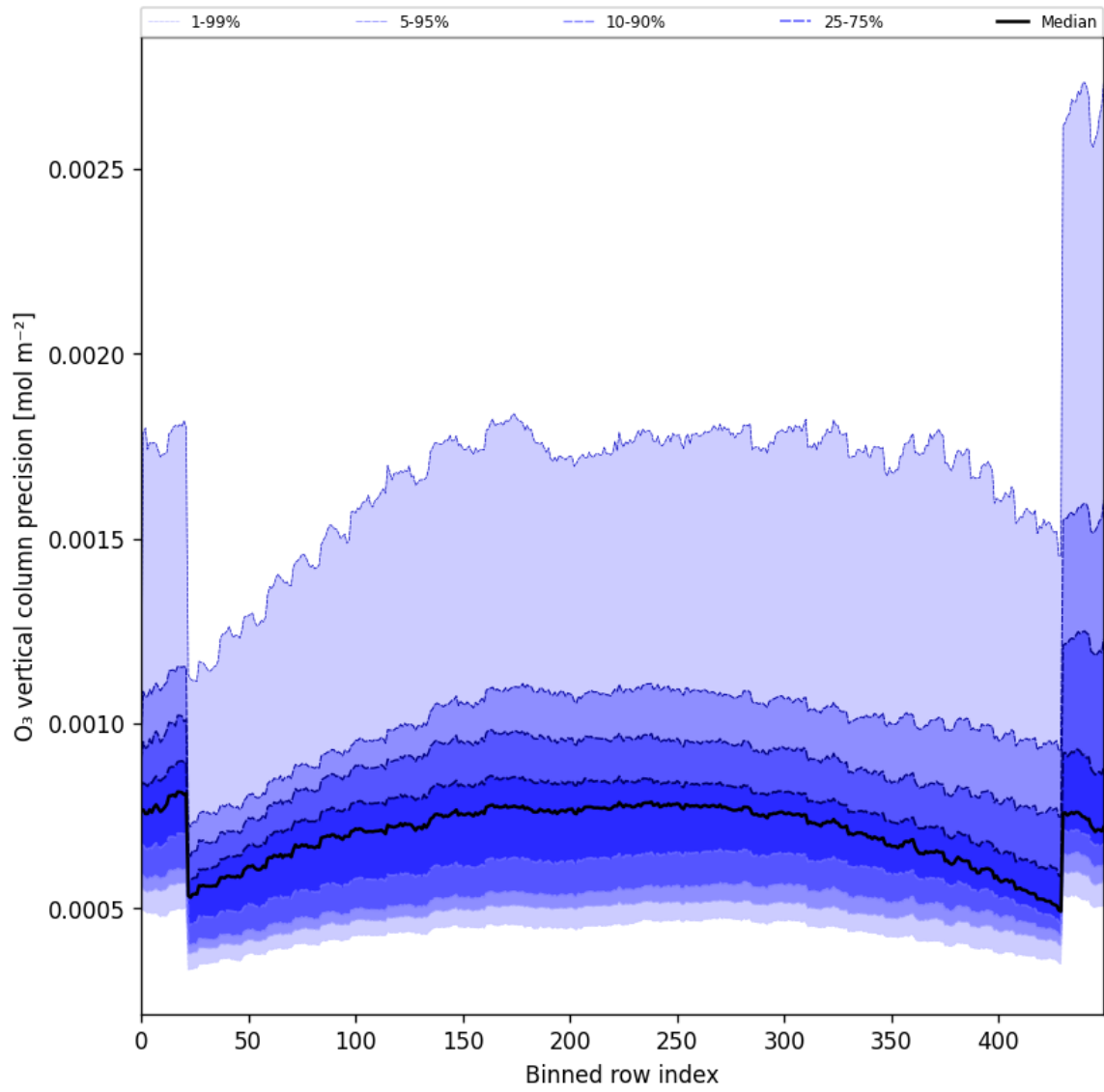
Figure 29: Along track statistics of “O 3 vertical column precision” for 2025-10-06 to 2025-10-07
