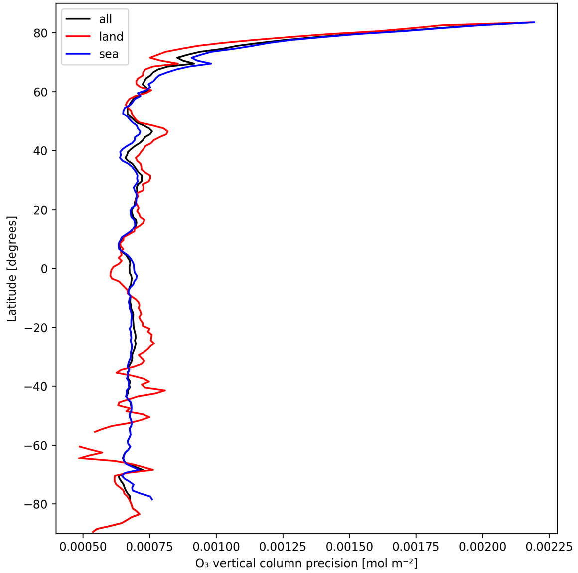
Figure 15: Zonal average of “O 3 vertical column precision” for 2025-10-06 to 2025-10-07.
