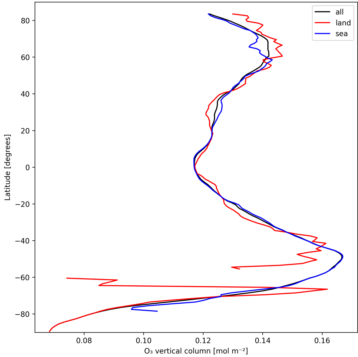
Figure 14: Zonal average of “O 3 vertical column” for 2025-10-06 to 2025-10-07.
