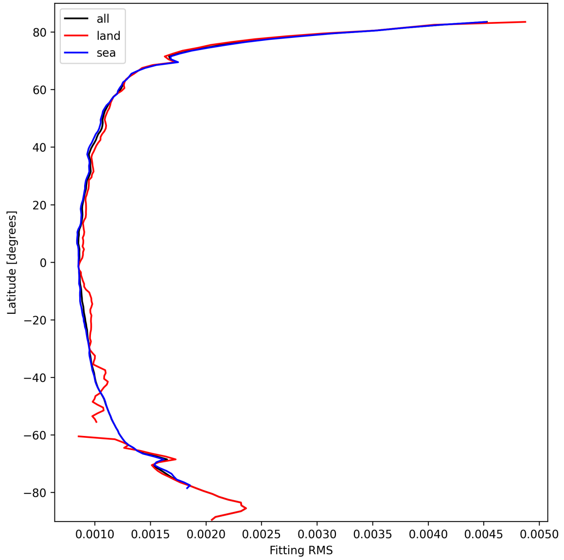
Figure 16: Zonal average of “Fitting RMS” for 2025-10-06 to 2025-10-07.
