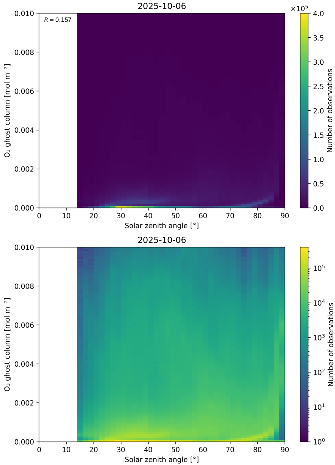
Figure 46: Scatter density plot of “Solar zenith angle” against “O 3 ghost column” for 2025-10-06 to 2025-10-07.
