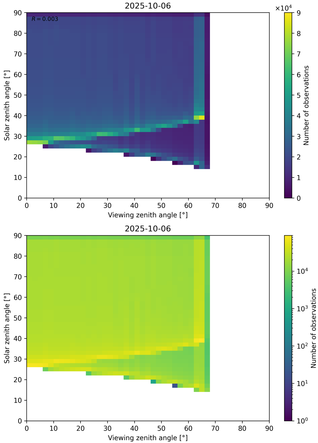
Figure 54: Scatter density plot of “Viewing zenith angle” against “Solar zenith angle” for 2025-10-06 to 2025-10-07.
