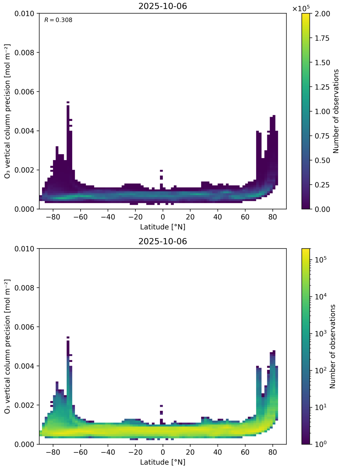
Figure 37: Scatter density plot of “Latitude” against “O 3 vertical column precision” for 2025-10-06 to 2025-10-07.
