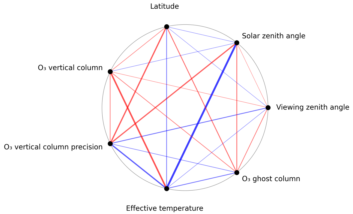
Figure 1: Map of correlation graph for 2025-10-06 to 2025-10-07.
