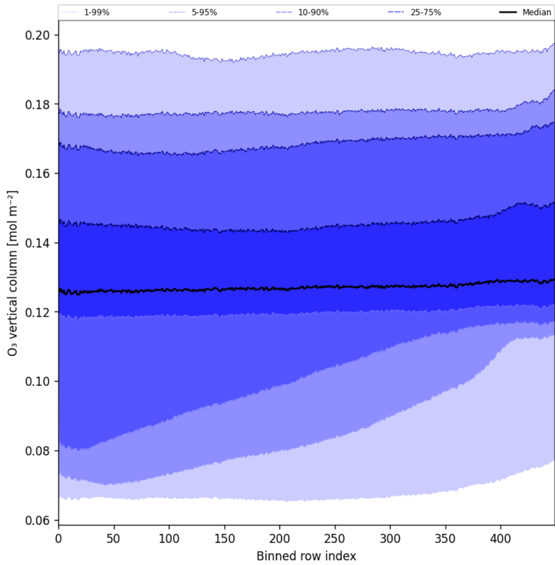
Figure 28: Along track statistics of “O 3 vertical column” for 2025-10-06 to 2025-10-07
