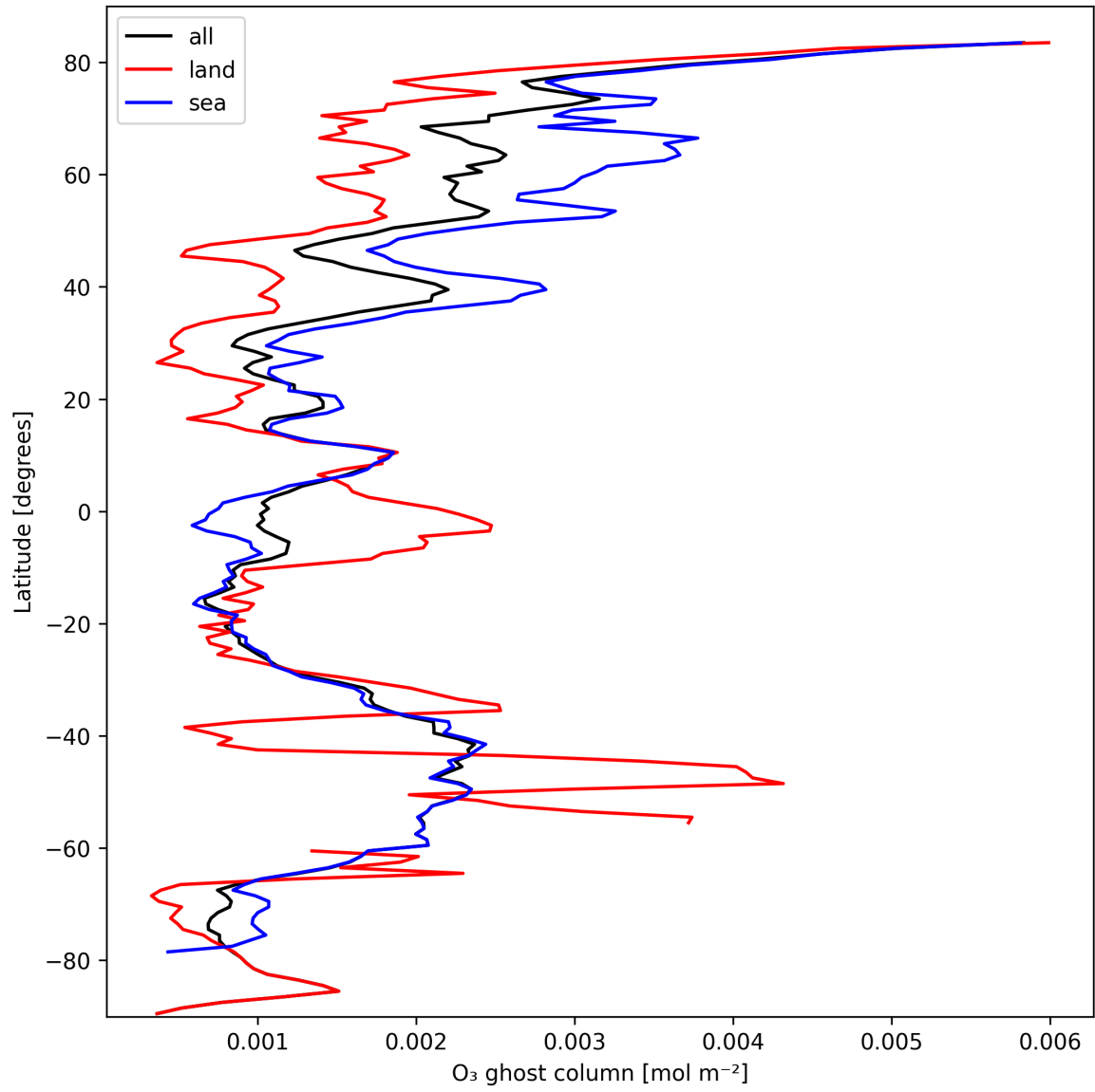
Figure 18: Zonal average of "O 3 ghost column" for 2025-10-06 to 2025-10-07.
