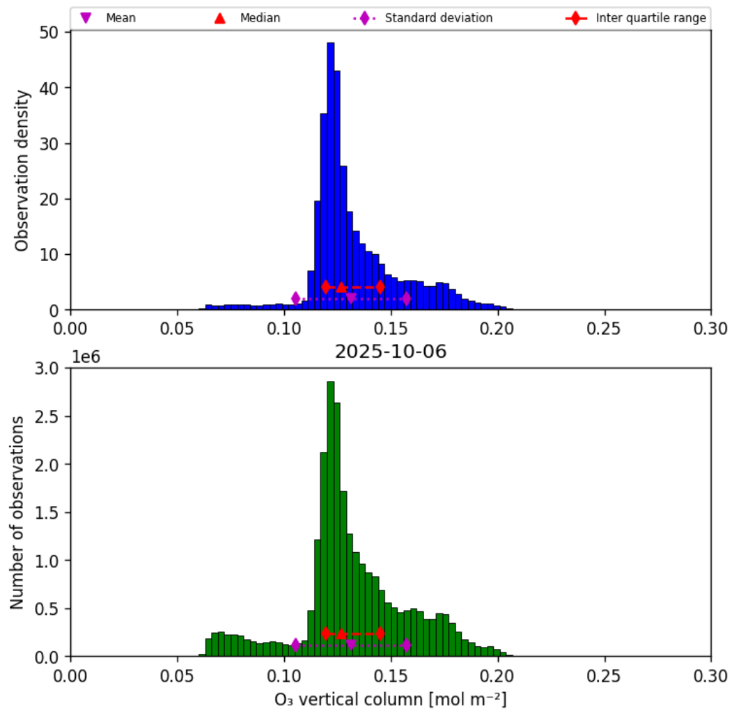
Figure 21: Histogram of “O 3 vertical column” for 2025-10-06 to 2025-10-07
