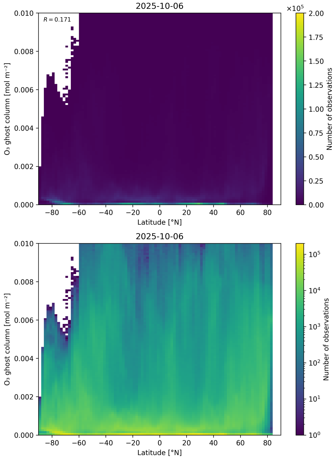
Figure 35: Scatter density plot of “Latitude” against “O 3 ghost column” for 2025-10-06 to 2025-10-07.
