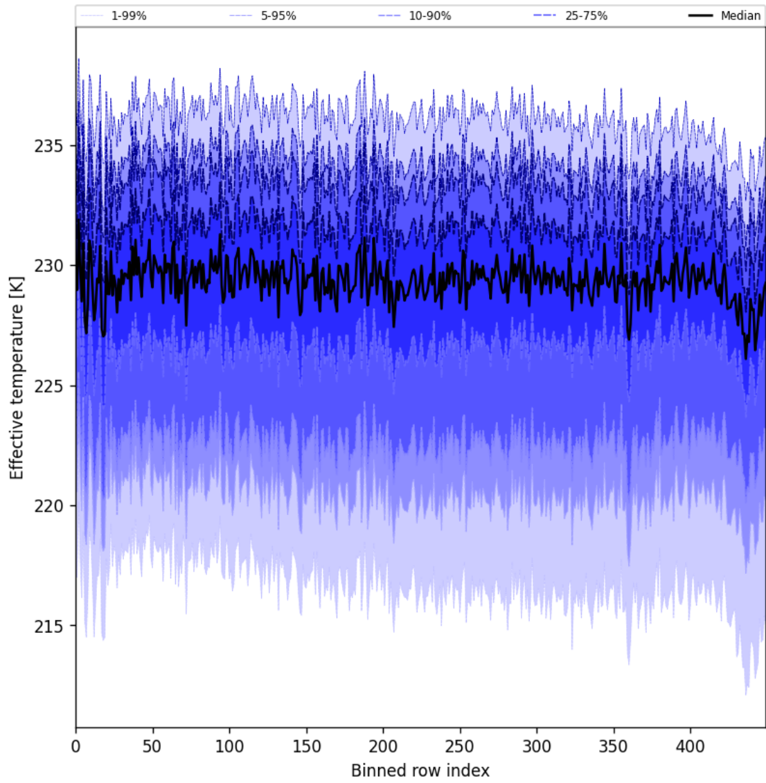
Figure 31: Along track statistics of “Effective temperature” for 2025-10-06 to 2025-10-07
