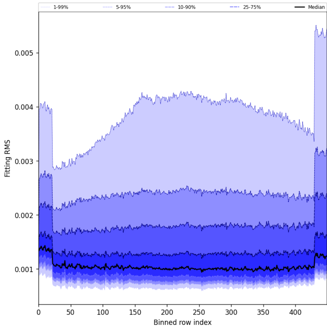
Figure 30: Along track statistics of “Fitting RMS” for 2025-10-06 to 2025-10-08
