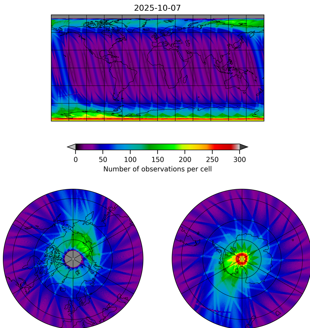
Figure 12: Map of the number of observations for 2025-10-06 to 2025-10-08
