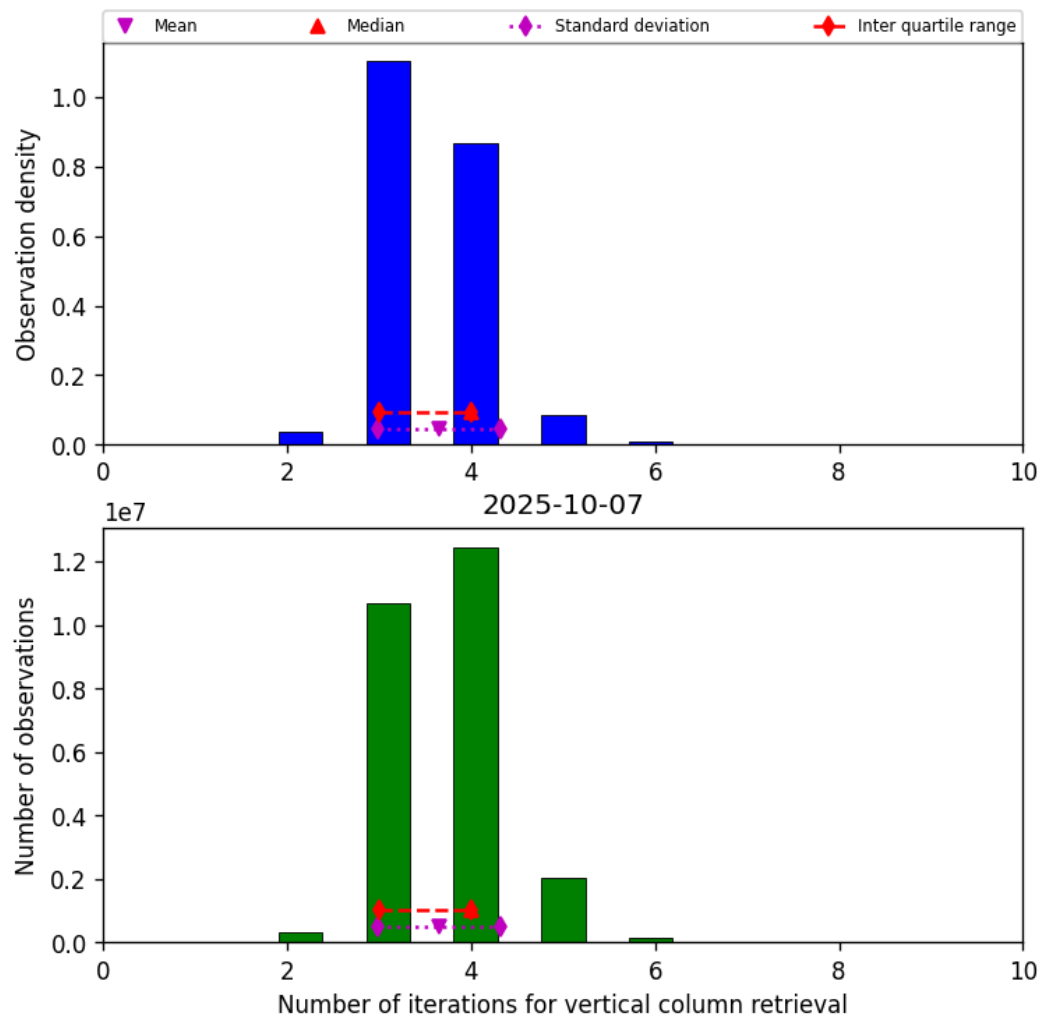
Figure 26: Histogram of “Number of iterations for vertical column retrieval” for 2025-10-06 to 2025-10-08
