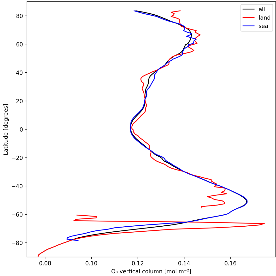
Figure 14: Zonal average of “O 3 vertical column” for 2025-10-06 to 2025-10-08.
