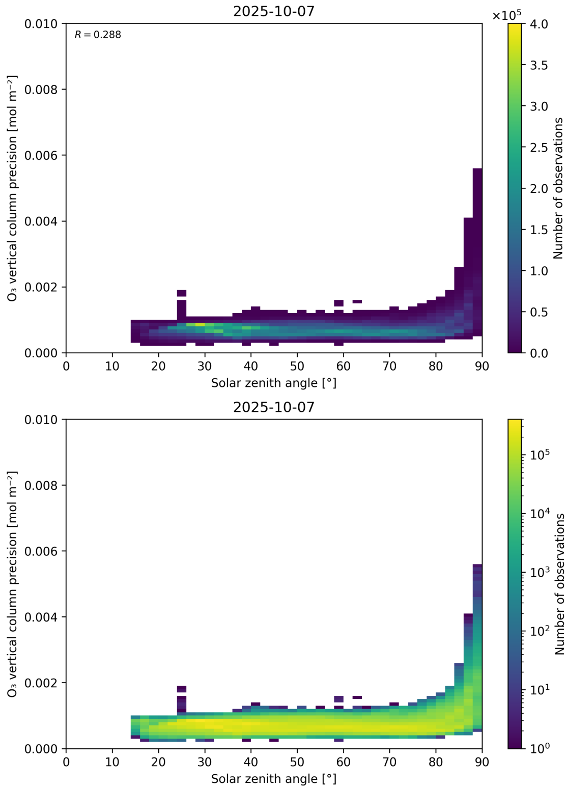
Figure 48: Scatter density plot of “Solar zenith angle” against “O 3 vertical column precision” for 2025-10-06 to 2025-10-08.
