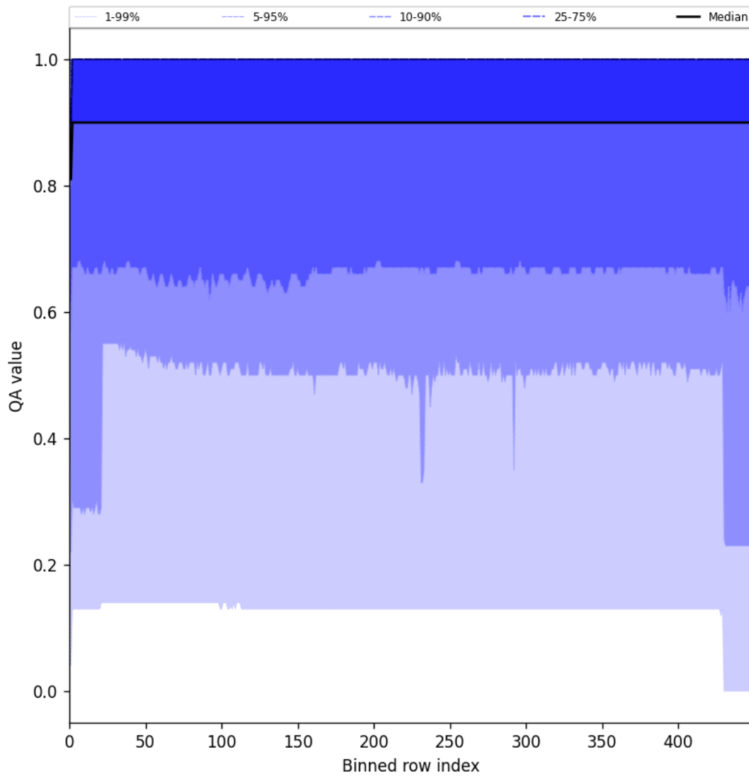
Figure 27: Along track statistics of “QA value” for 2025-10-06 to 2025-10-08
