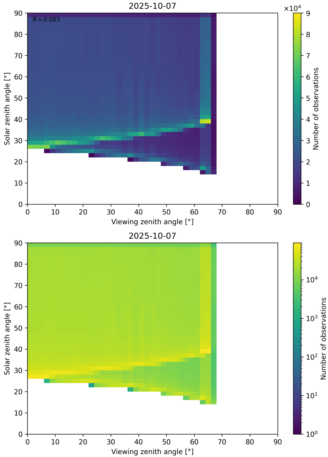
Figure 54: Scatter density plot of “Viewing zenith angle” against “Solar zenith angle” for 2025-10-06 to 2025-10-08.
