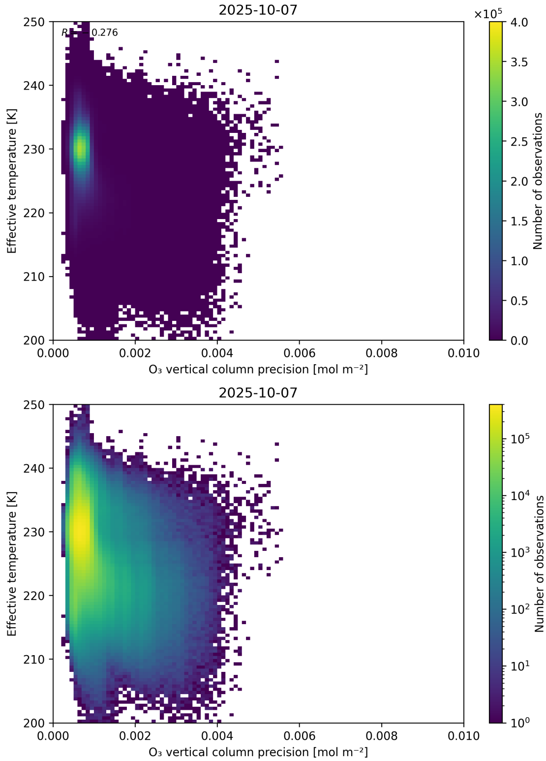
Figure 42: Scatter density plot of “ O_3 vertical column precision” against “Effective temperature” for 2025-10-06 to 2025-10-08.
