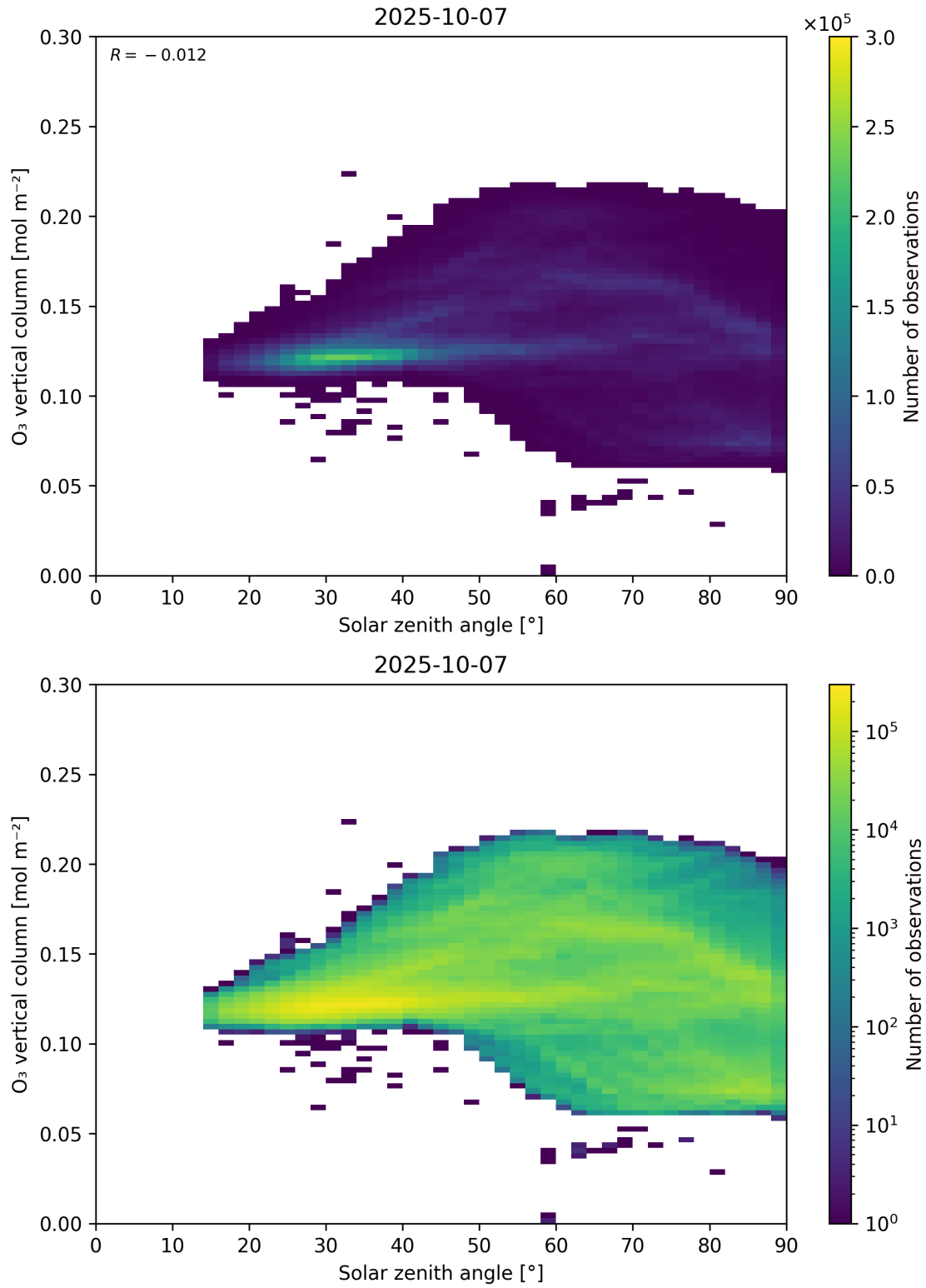
Figure 47: Scatter density plot of “Solar zenith angle” against “O 3 vertical column” for 2025-10-06 to 2025-10-08.
