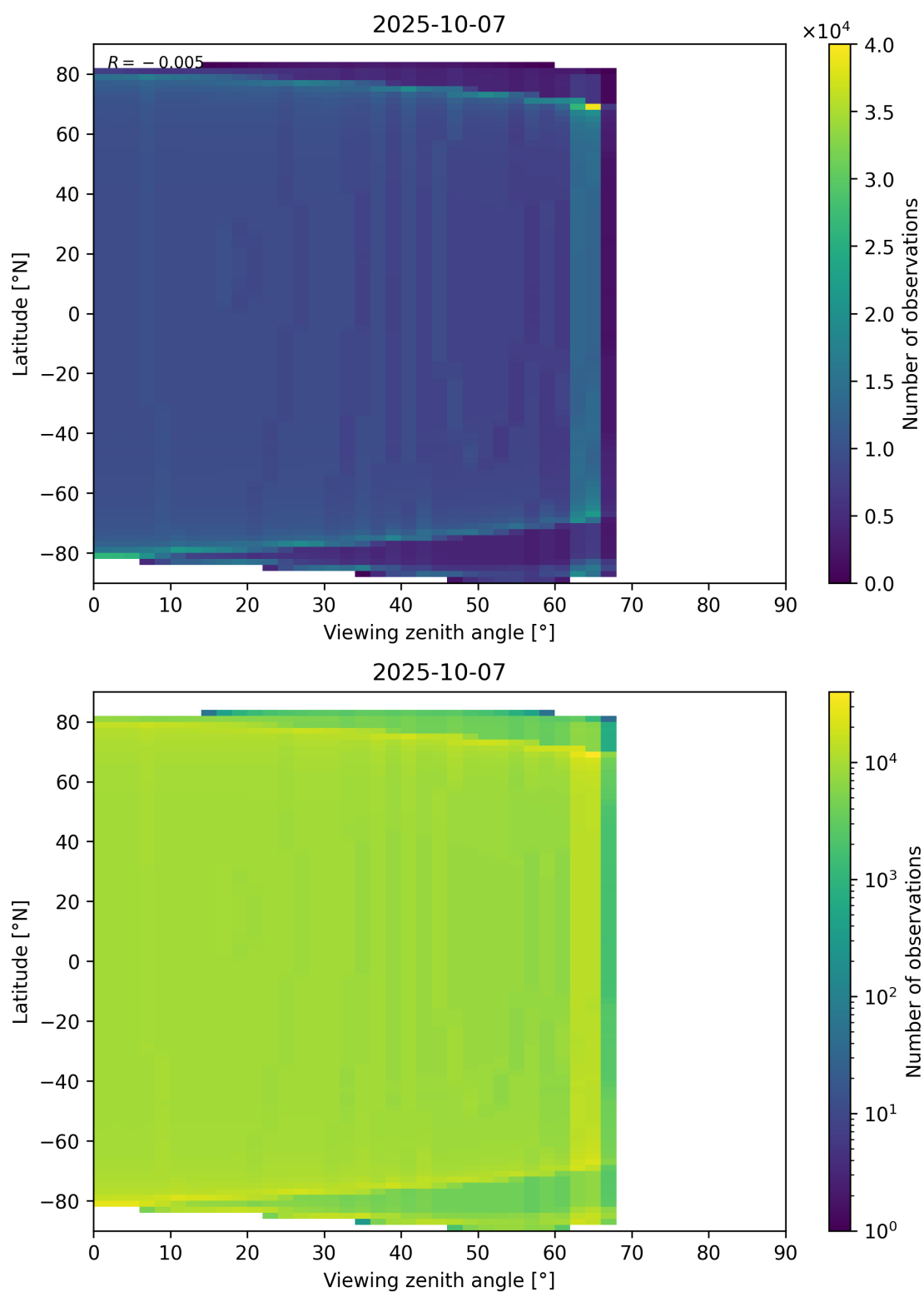
Figure 49: Scatter density plot of “Viewing zenith angle” against “Latitude” for 2025-10-06 to 2025-10-08.
