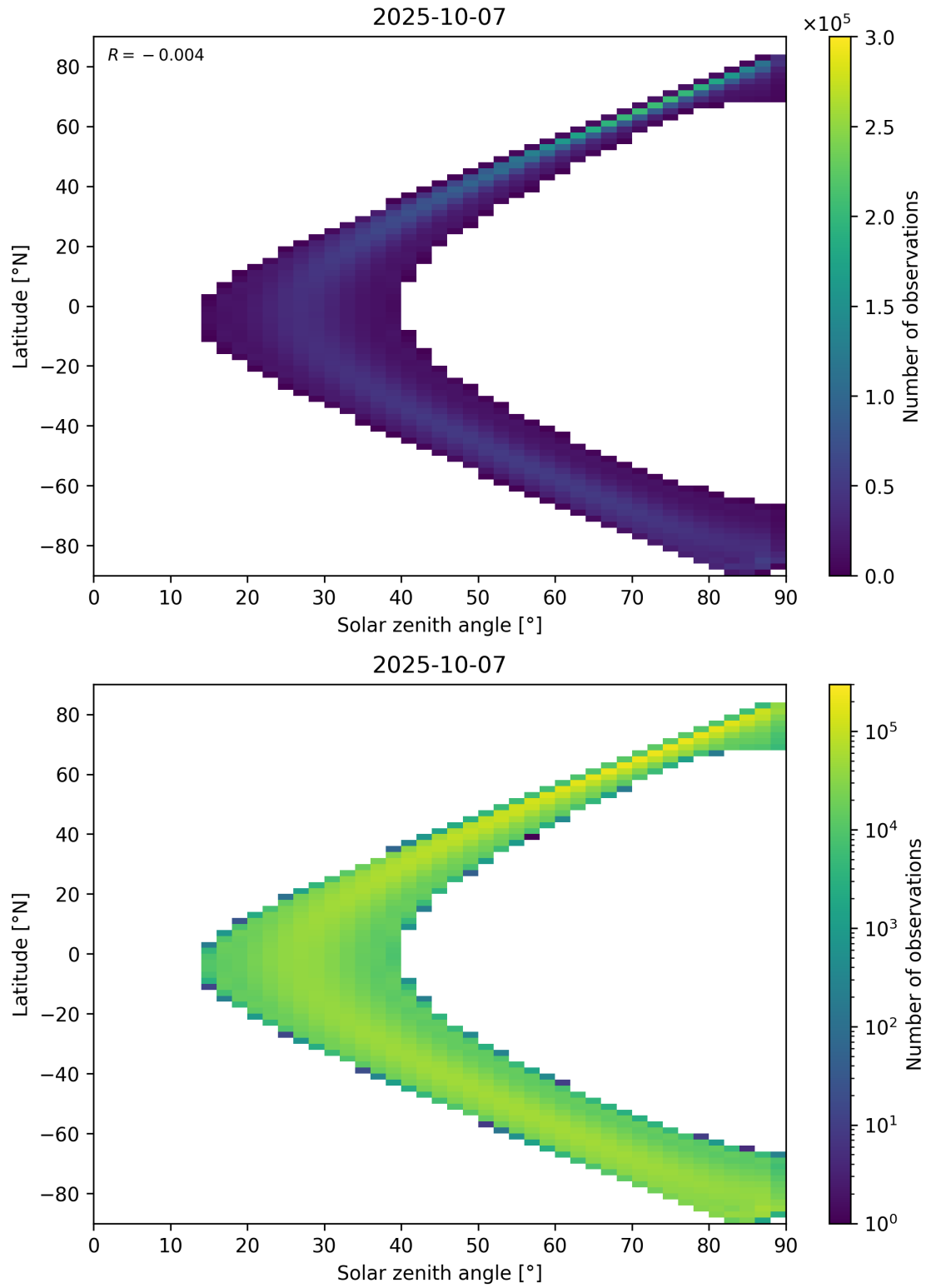
Figure 44: Scatter density plot of “Solar zenith angle” against “Latitude” for 2025-10-06 to 2025-10-08.
