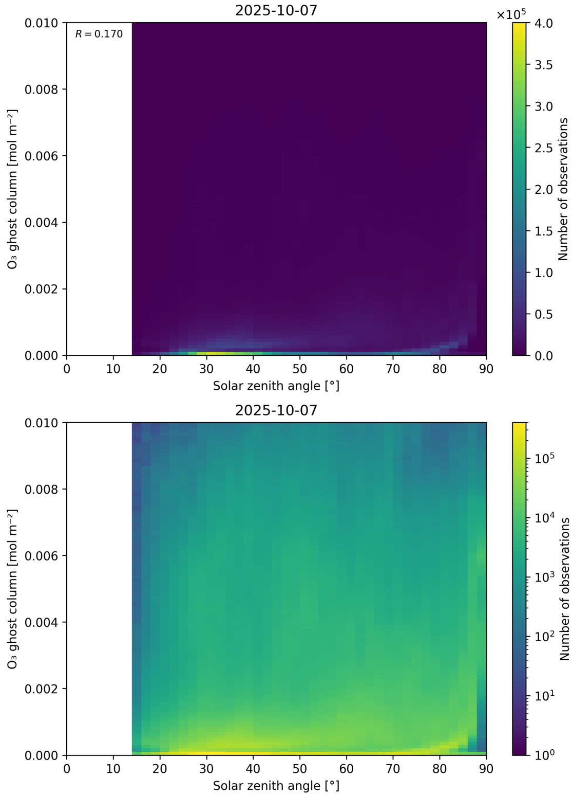
Figure 46: Scatter density plot of “Solar zenith angle” against “O 3 ghost column” for 2025-10-06 to 2025-10-08.
