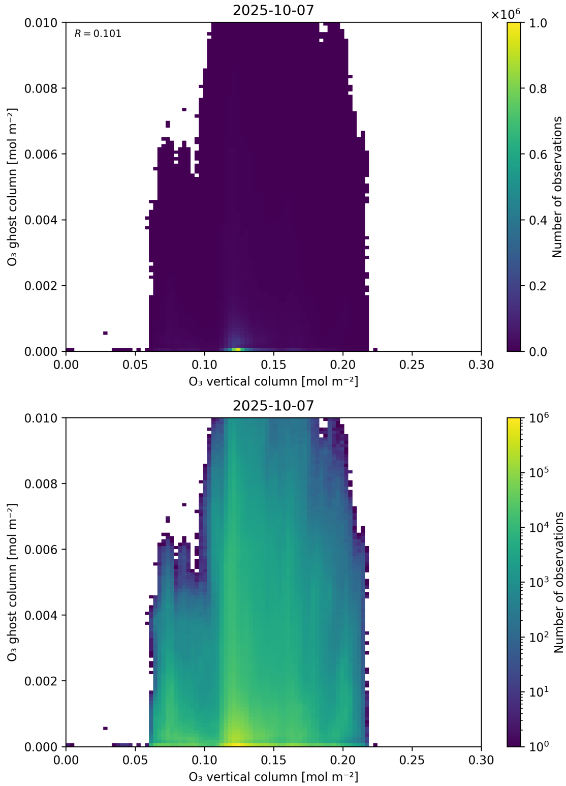
Figure 40: Scatter density plot of “O 3 vertical column” against “O 3 ghost column” for 2025-10-06 to 2025-10-08.
