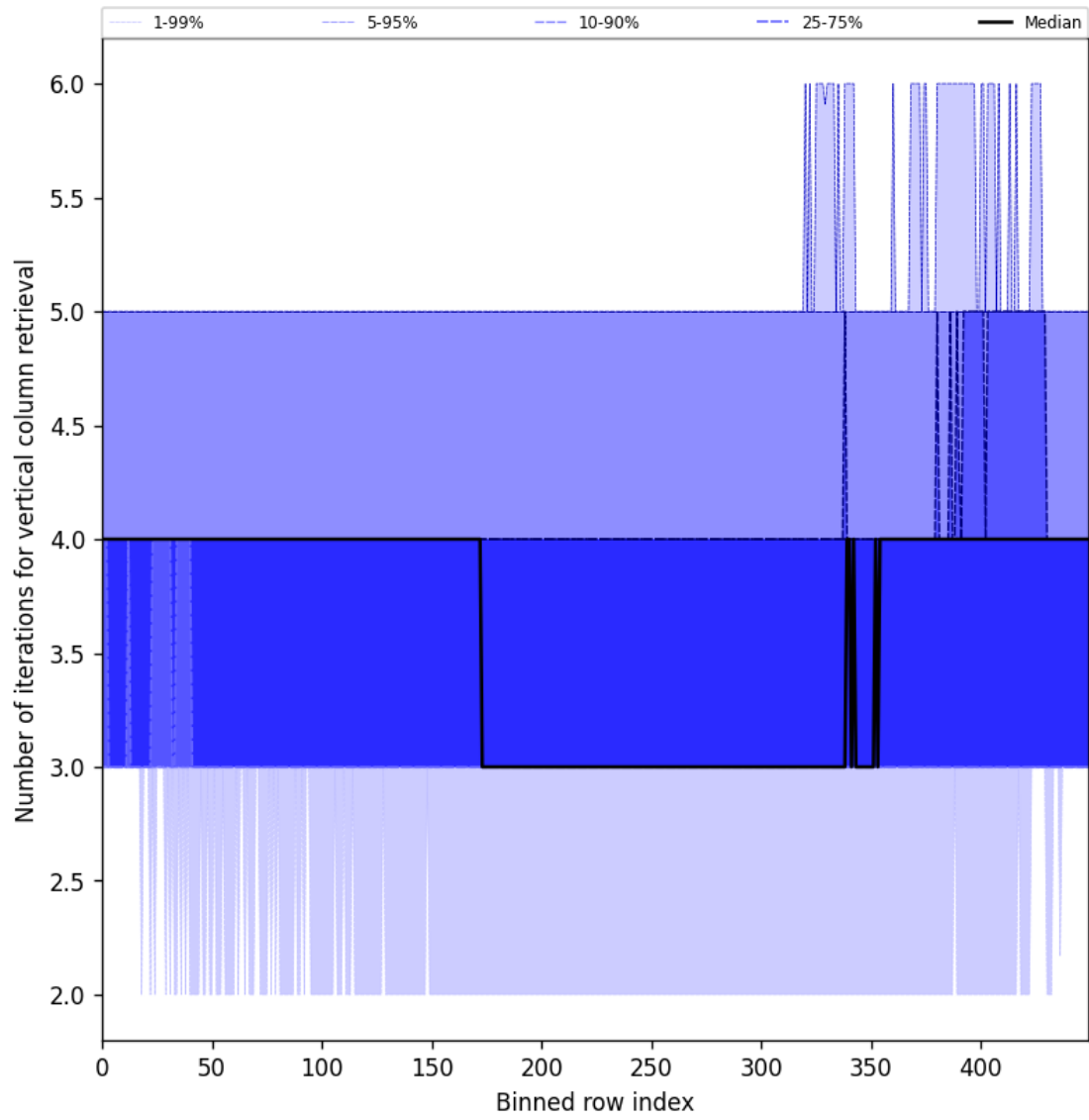
Figure 33: Along track statistics of “Number of iterations for vertical column retrieval” for 2025-10-06 to 2025-10-08
