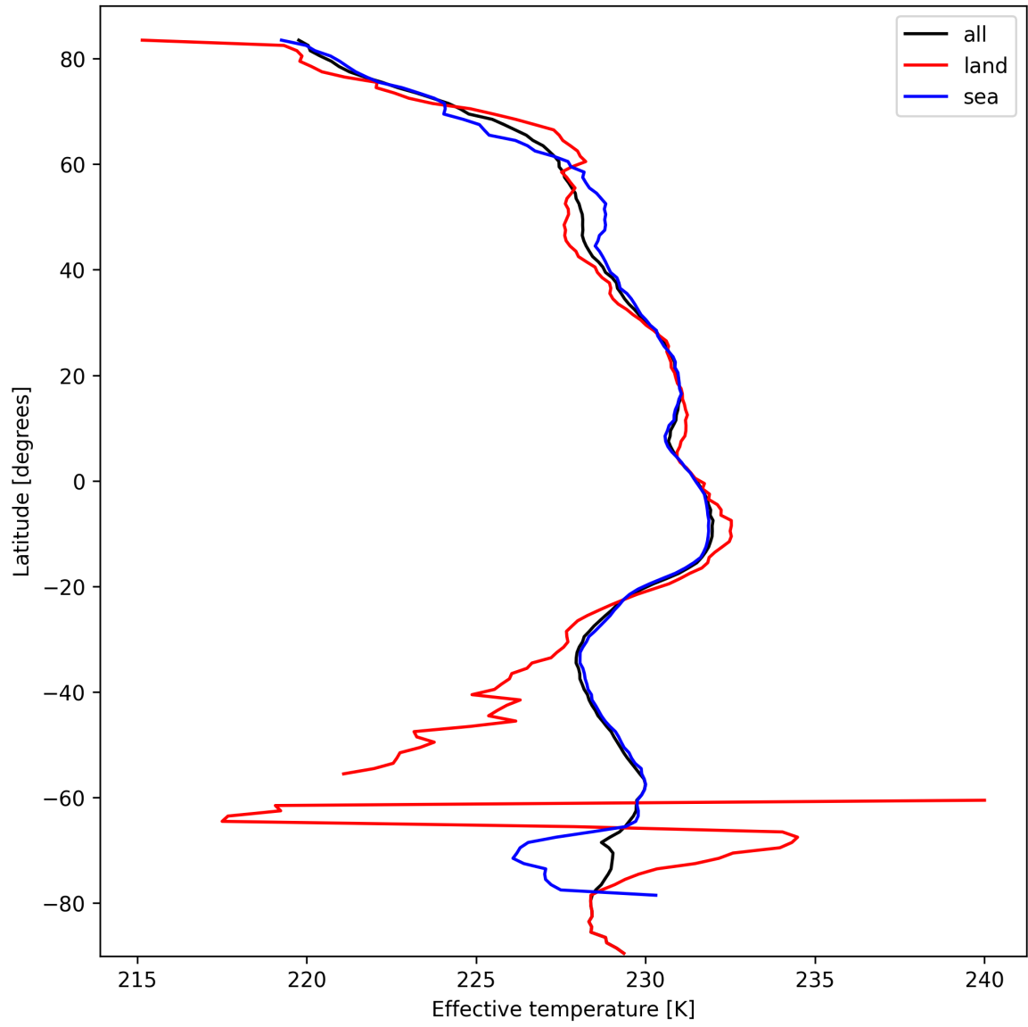
Figure 17: Zonal average of "Effective temperature" for 2025-10-06 to 2025-10-08.
