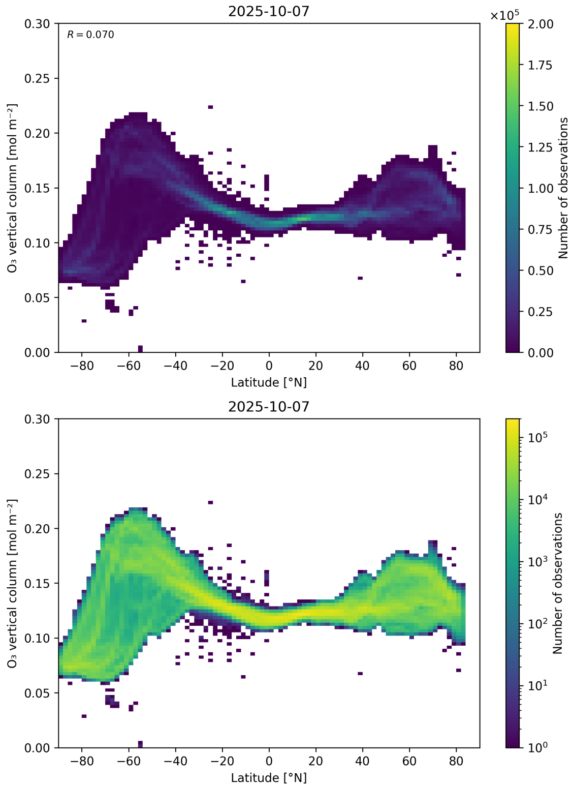
Figure 36: Scatter density plot of “Latitude” against “O 3 vertical column” for 2025-10-06 to 2025-10-08.
