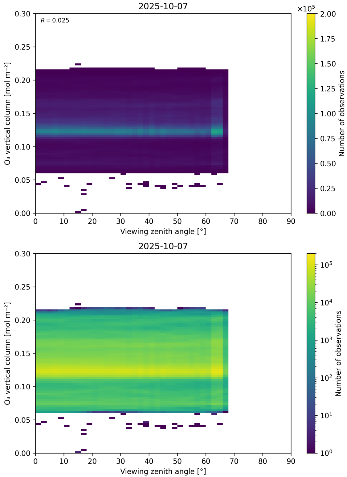
Figure 52: Scatter density plot of “Viewing zenith angle” against “O 3 vertical column” for 2025-10-06 to 2025-10-08.
