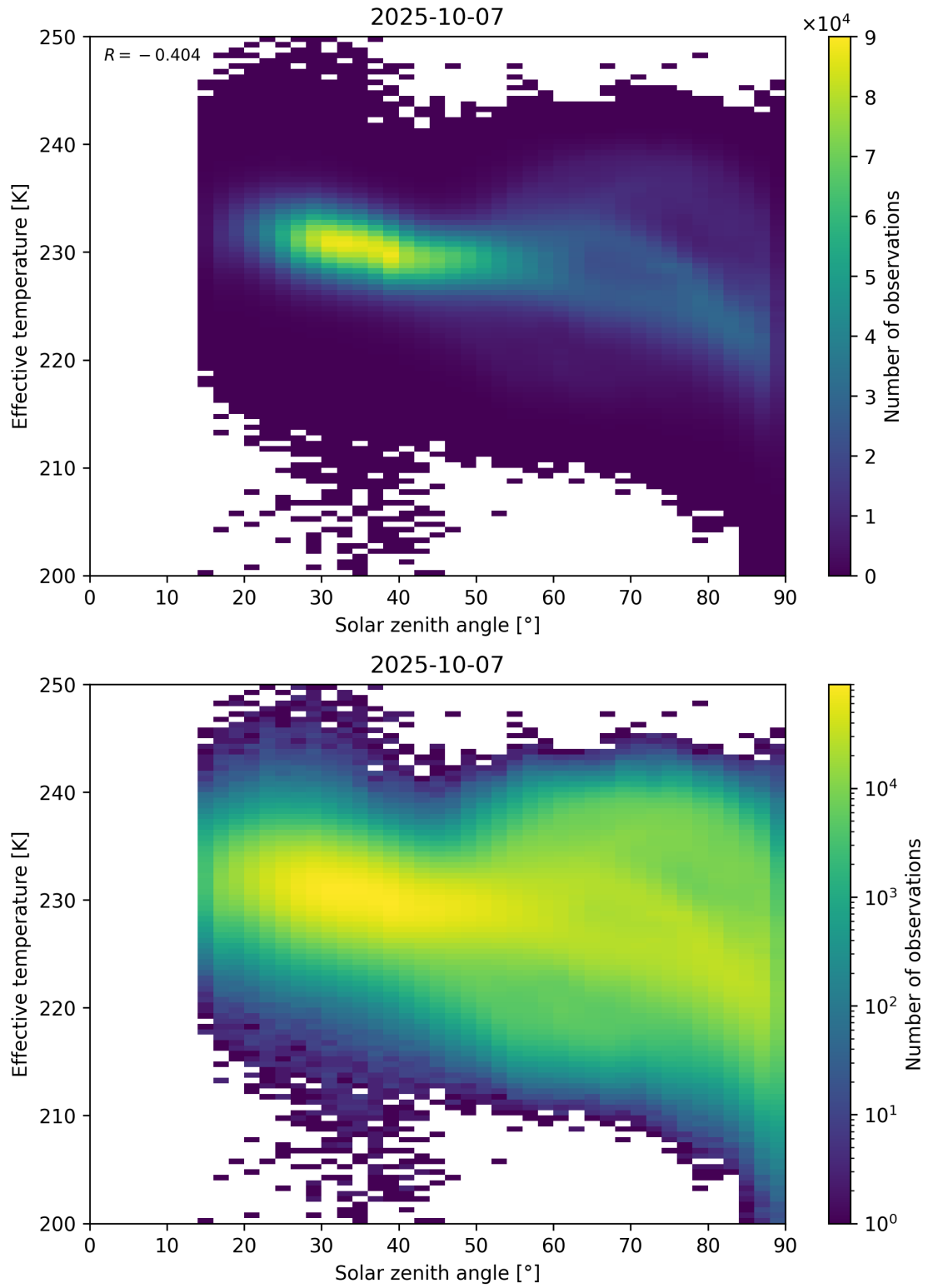
Figure 45: Scatter density plot of “Solar zenith angle” against “Effective temperature” for 2025-10-06 to 2025-10-08.
