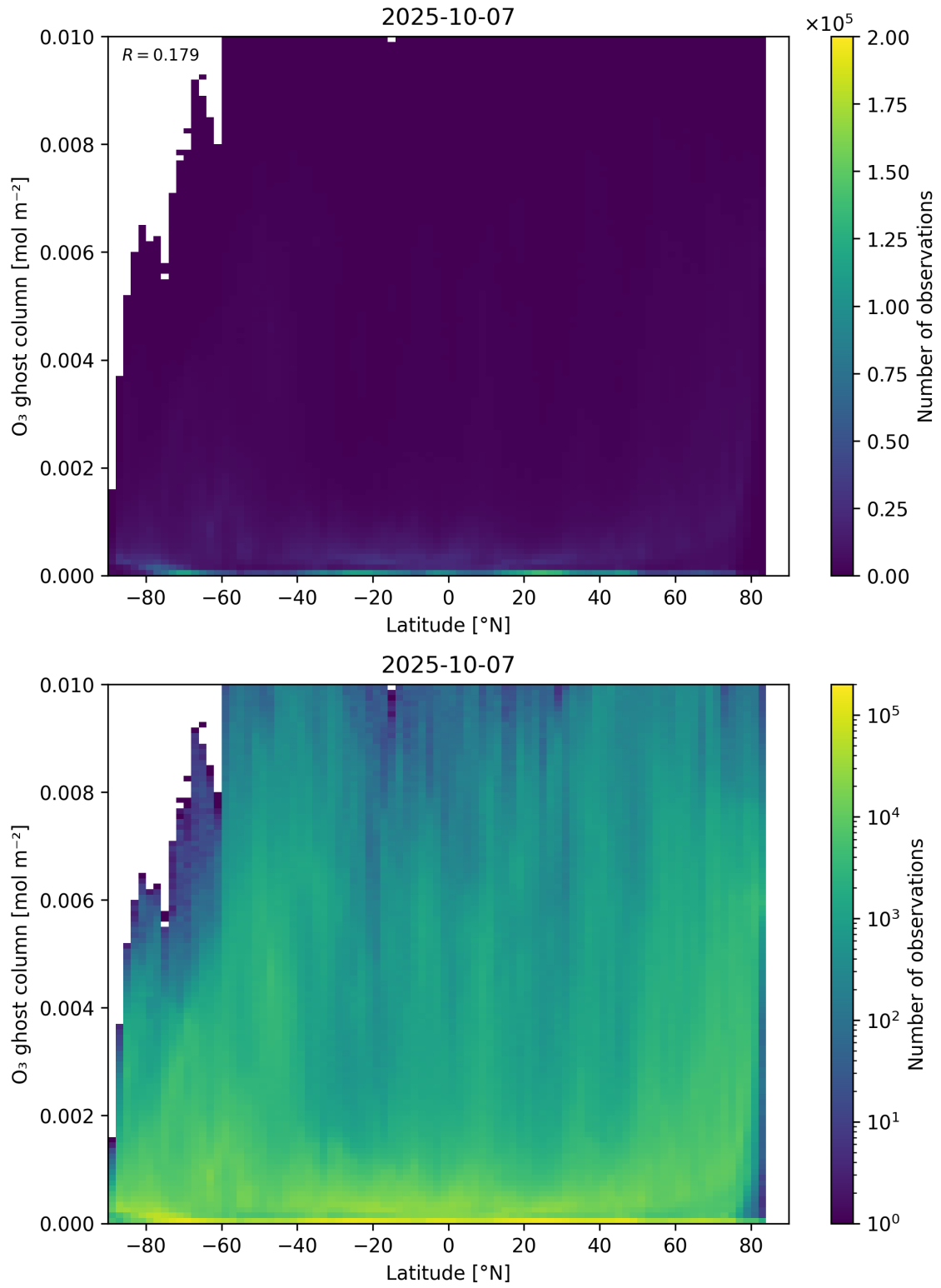
Figure 35: Scatter density plot of “Latitude” against “O 3 ghost column” for 2025-10-06 to 2025-10-08.
