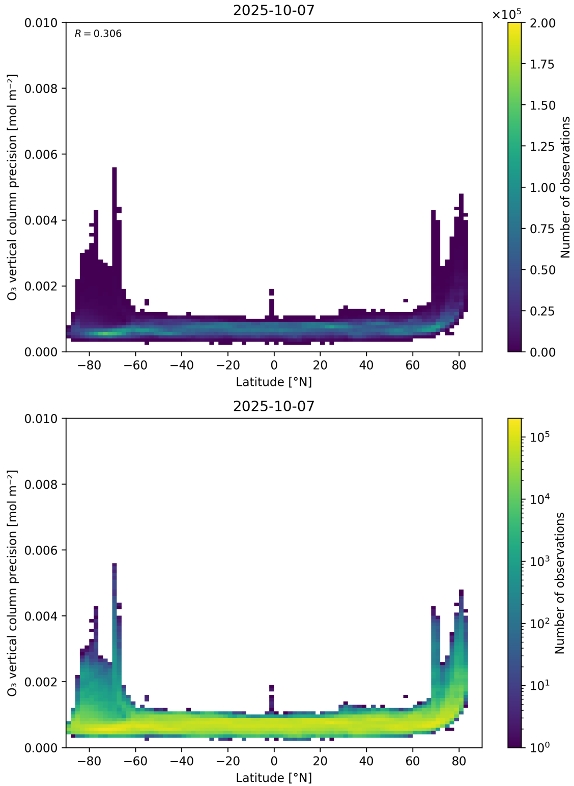
Figure 37: Scatter density plot of “Latitude” against “O 3 vertical column precision” for 2025-10-06 to 2025-10-08.
