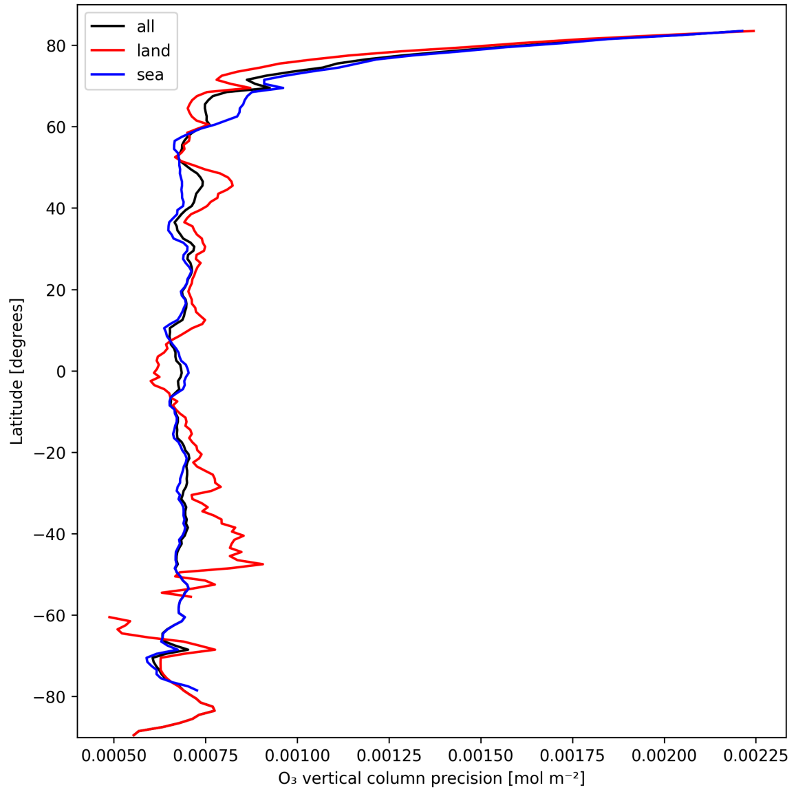
Figure 15: Zonal average of “O 3 vertical column precision” for 2025-10-06 to 2025-10-08.
