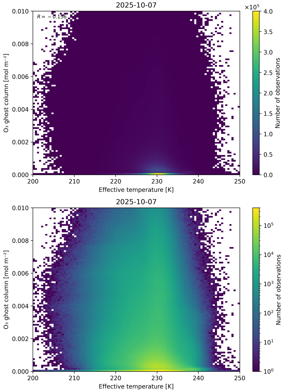
Figure 38: Scatter density plot of “Effective temperature” against “O 3 ghost column” for 2025-10-06 to 2025-10-08.
