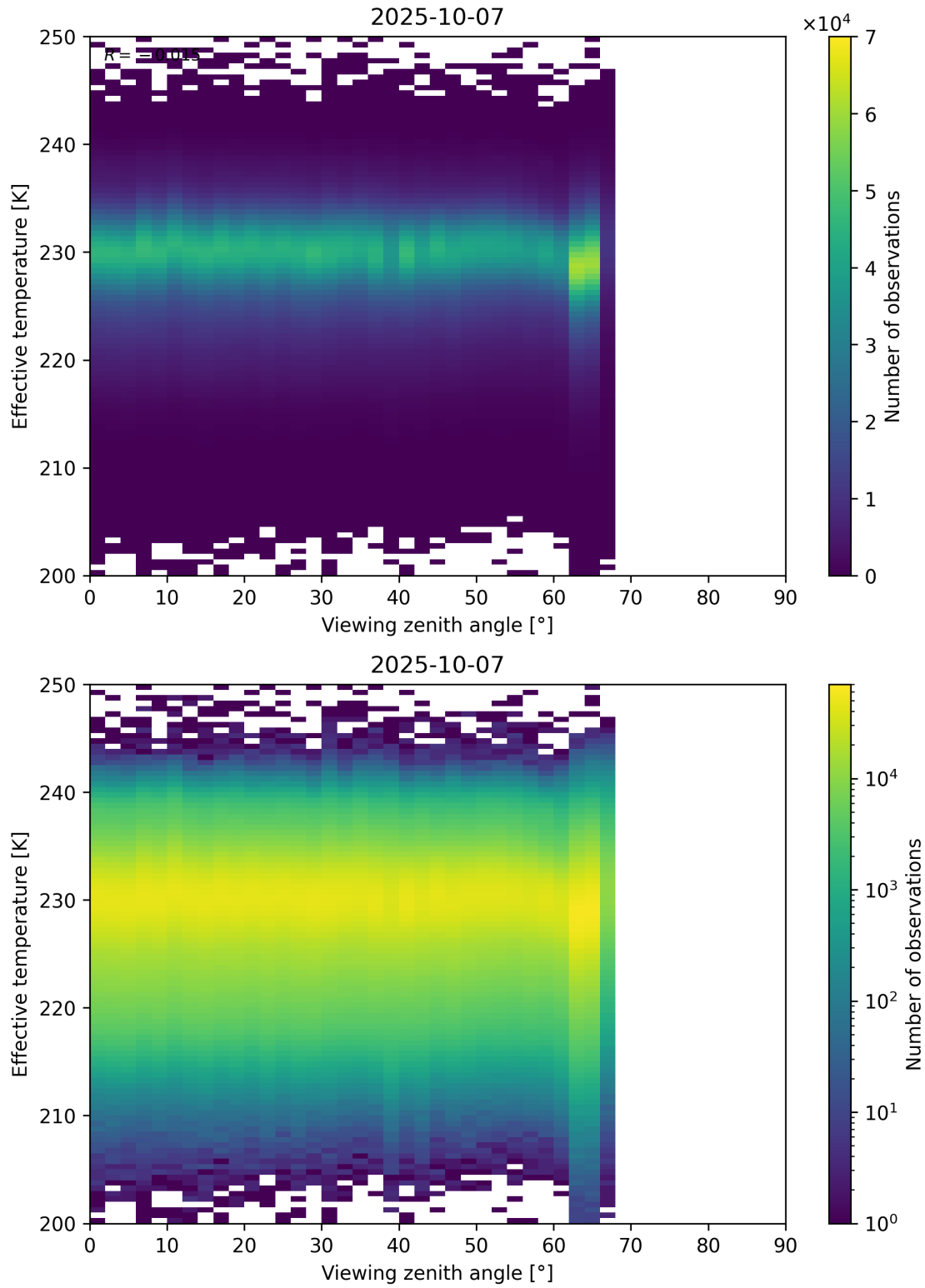
Figure 50: Scatter density plot of “Viewing zenith angle” against “Effective temperature” for 2025-10-06 to 2025-10-08.
