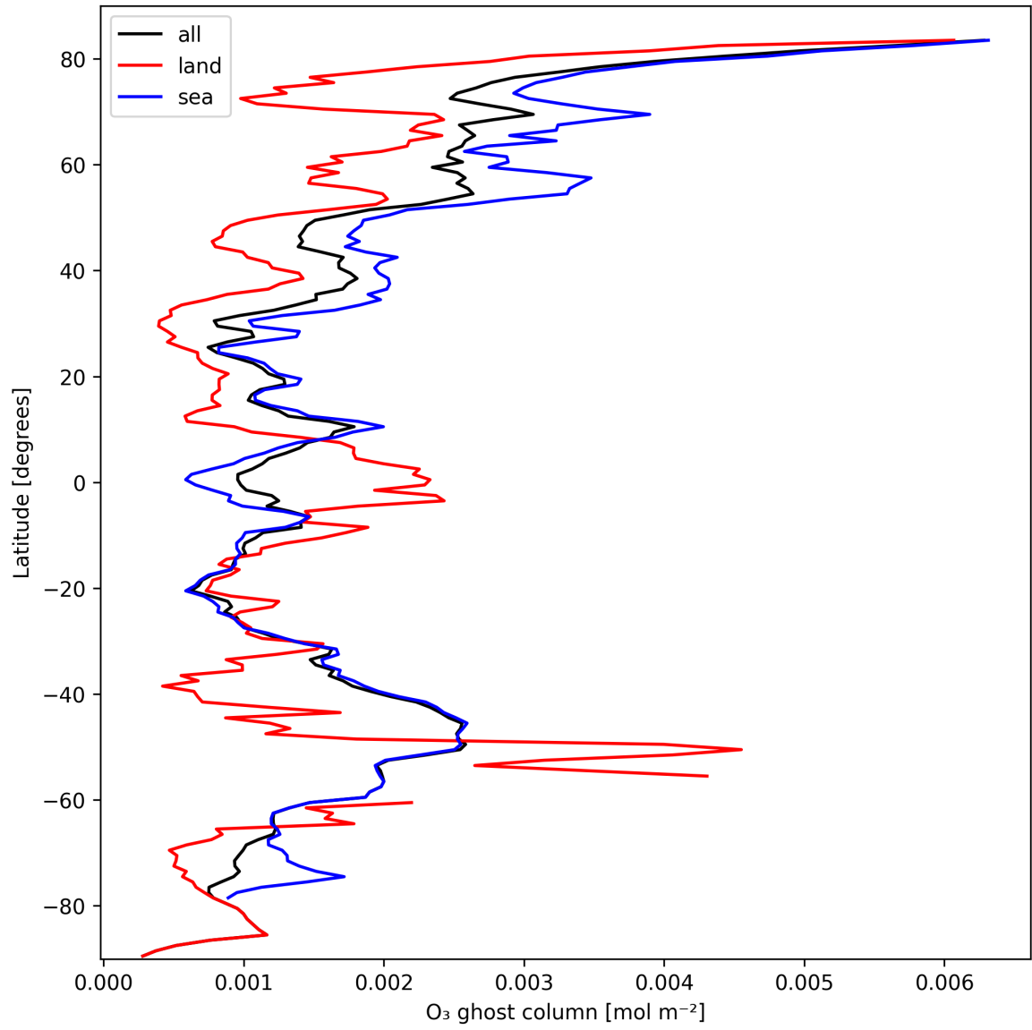
Figure 18: Zonal average of “O 3 ghost column” for 2025-10-06 to 2025-10-08.
