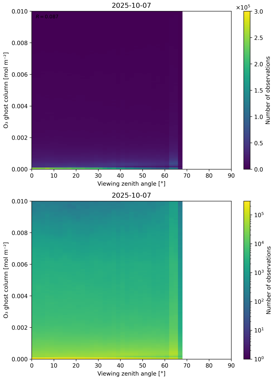
Figure 51: Scatter density plot of “Viewing zenith angle” against “O 3 ghost column” for 2025-10-06 to 2025-10-08.
