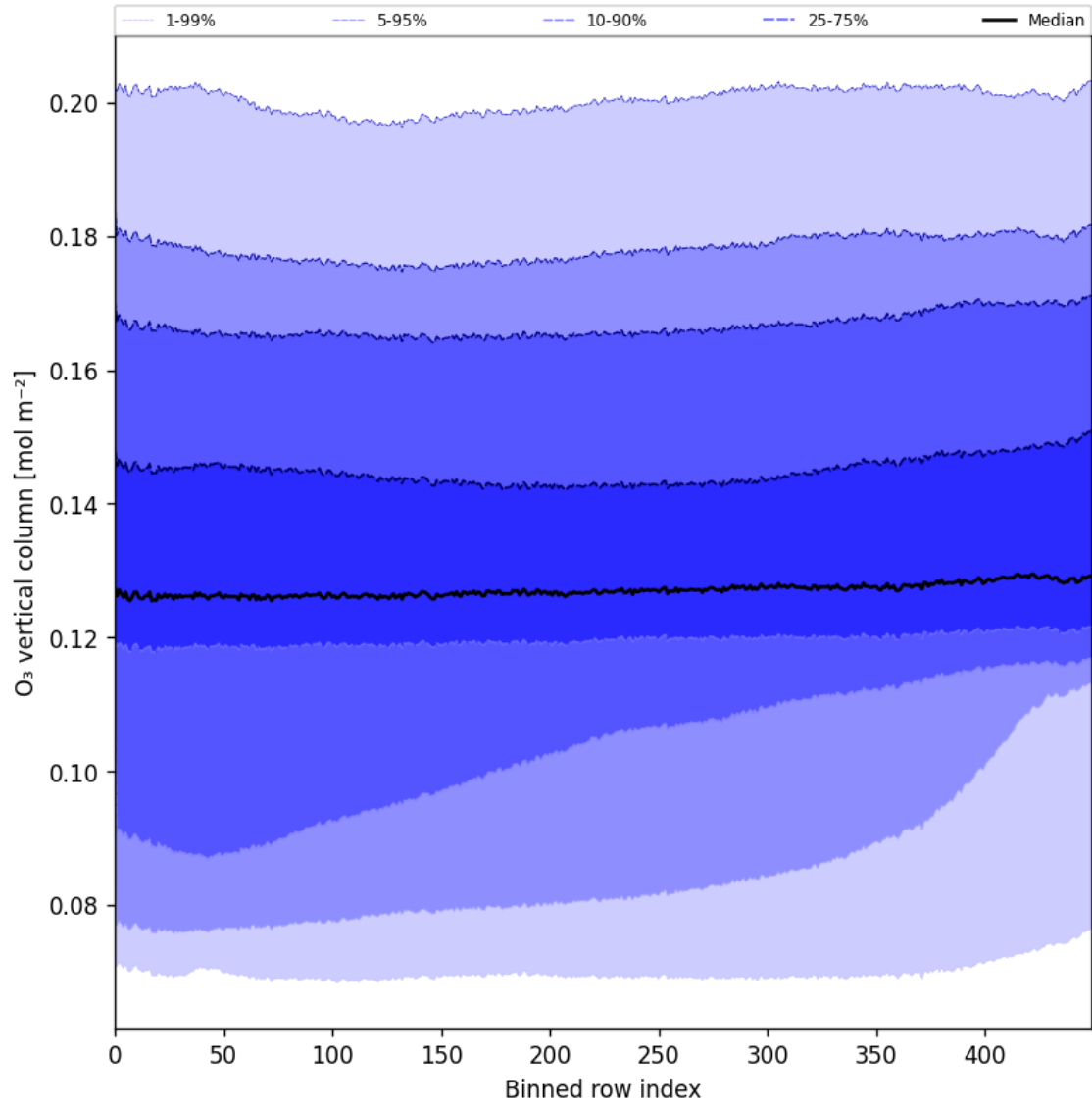
Figure 28: Along track statistics of “O 3 vertical column” for 2025-10-06 to 2025-10-08
