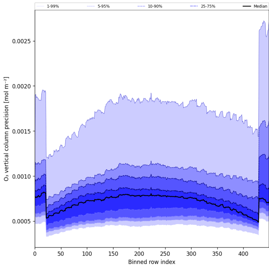
Figure 29: Along track statistics of “O 3 vertical column precision” for 2025-10-06 to 2025-10-08
