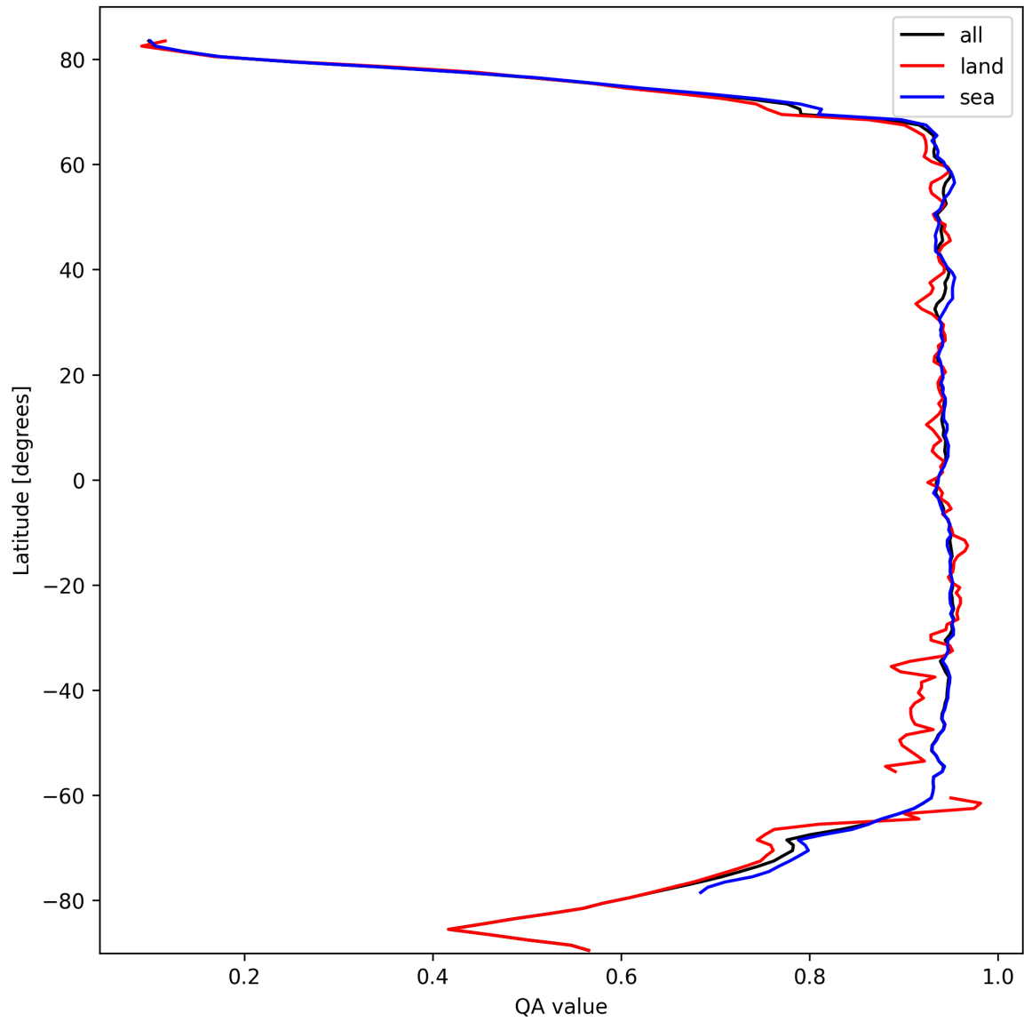
Figure 13: Zonal average of “QA value” for 2025-10-06 to 2025-10-08.
