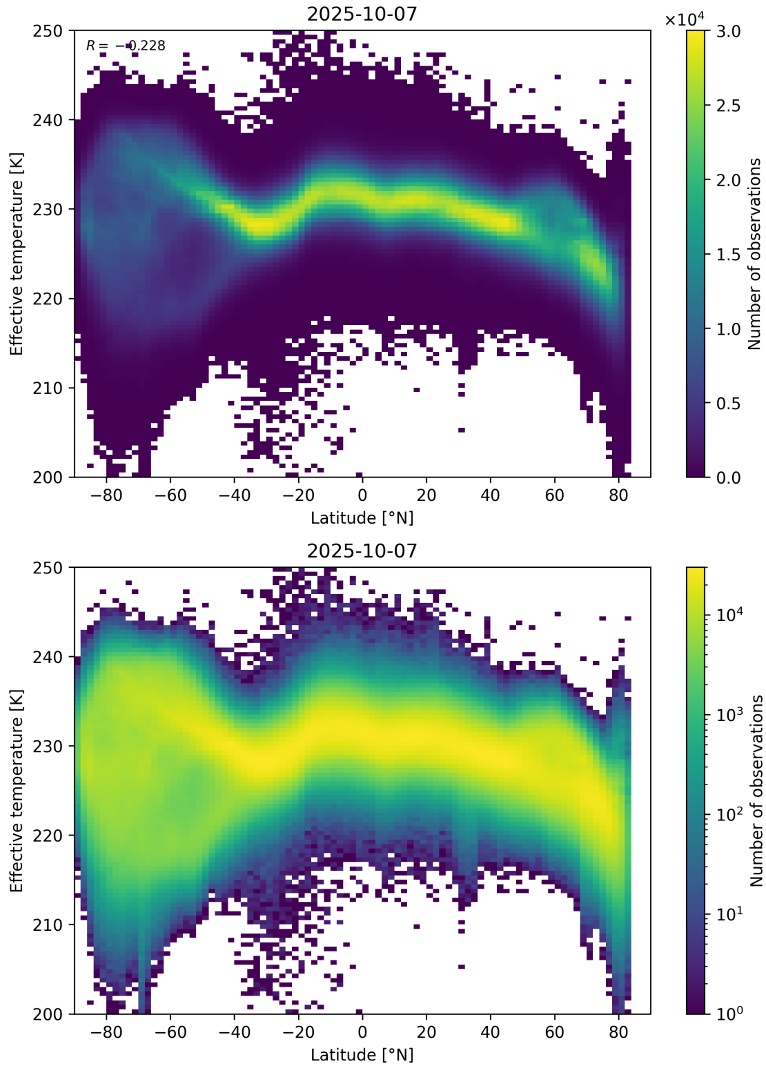
Figure 34: Scatter density plot of “Latitude” against “Effective temperature” for 2025-10-06 to 2025-10-08.
