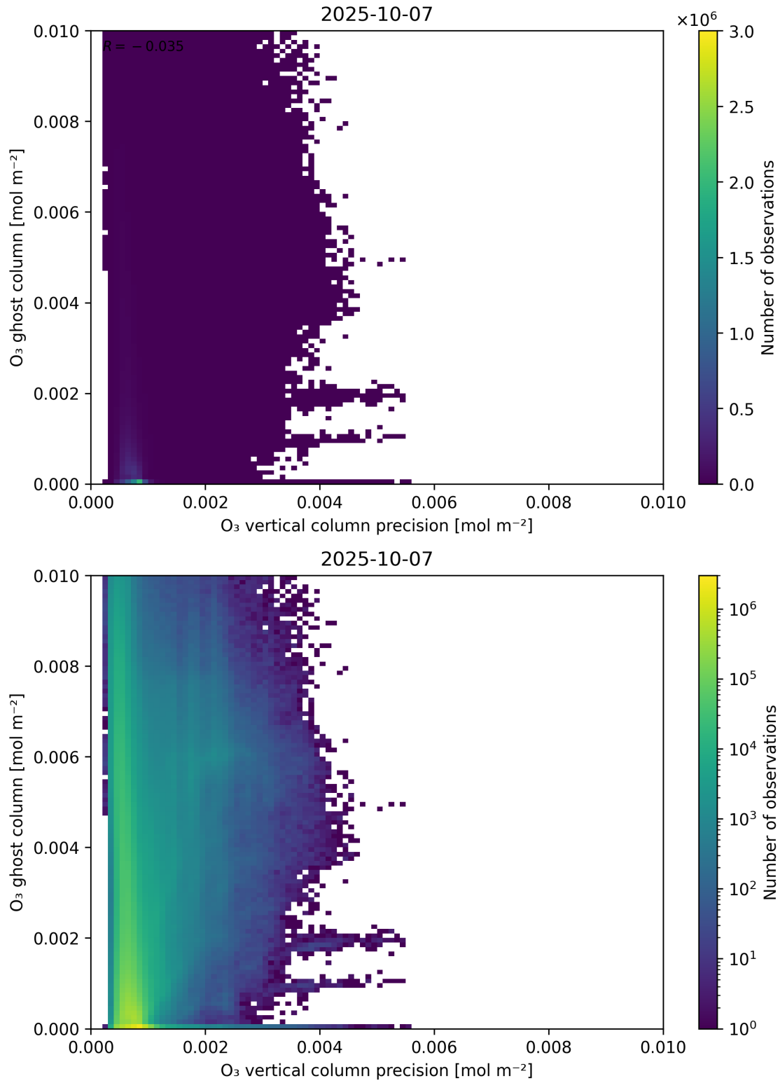
Figure 43: Scatter density plot of “O 3 vertical column precision” against “O 3 ghost column” for 2025-10-06 to 2025-10-08.
