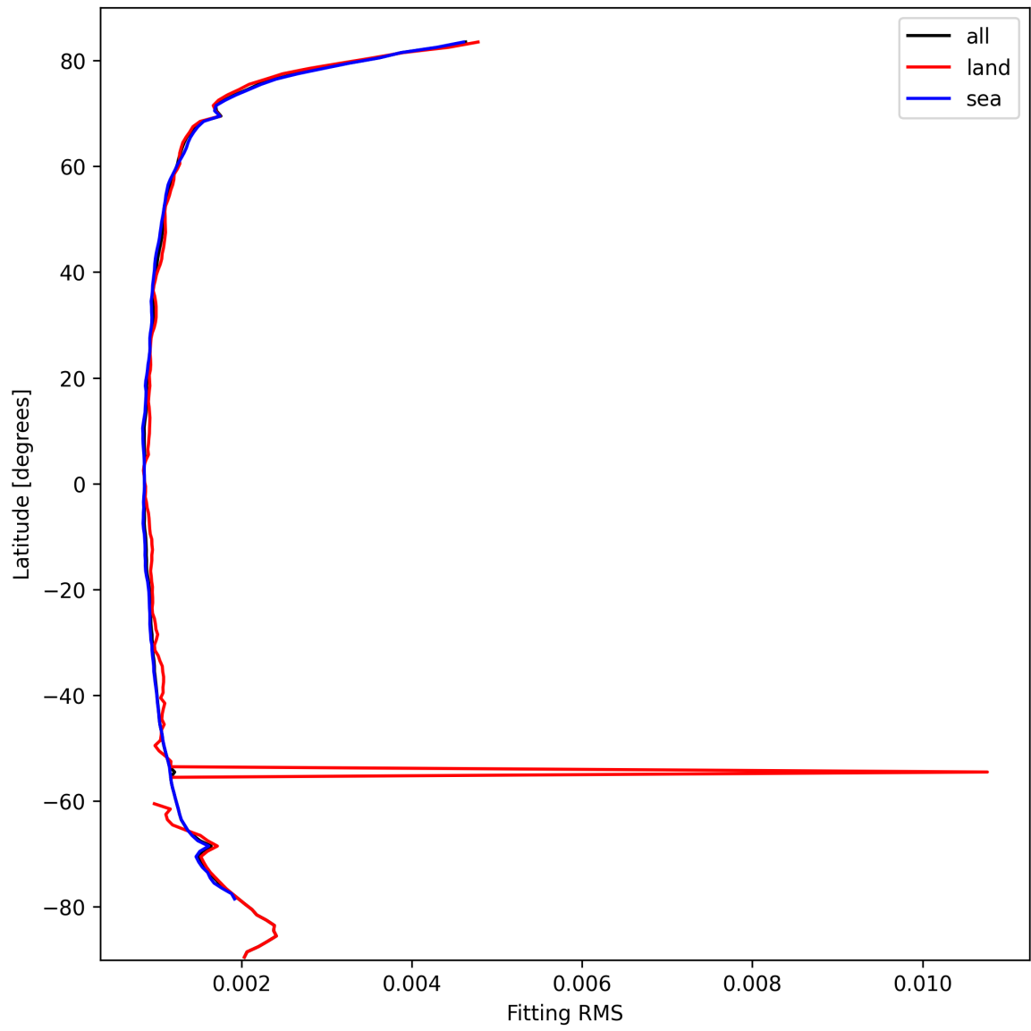
Figure 16: Zonal average of “Fitting RMS” for 2025-10-06 to 2025-10-08.
