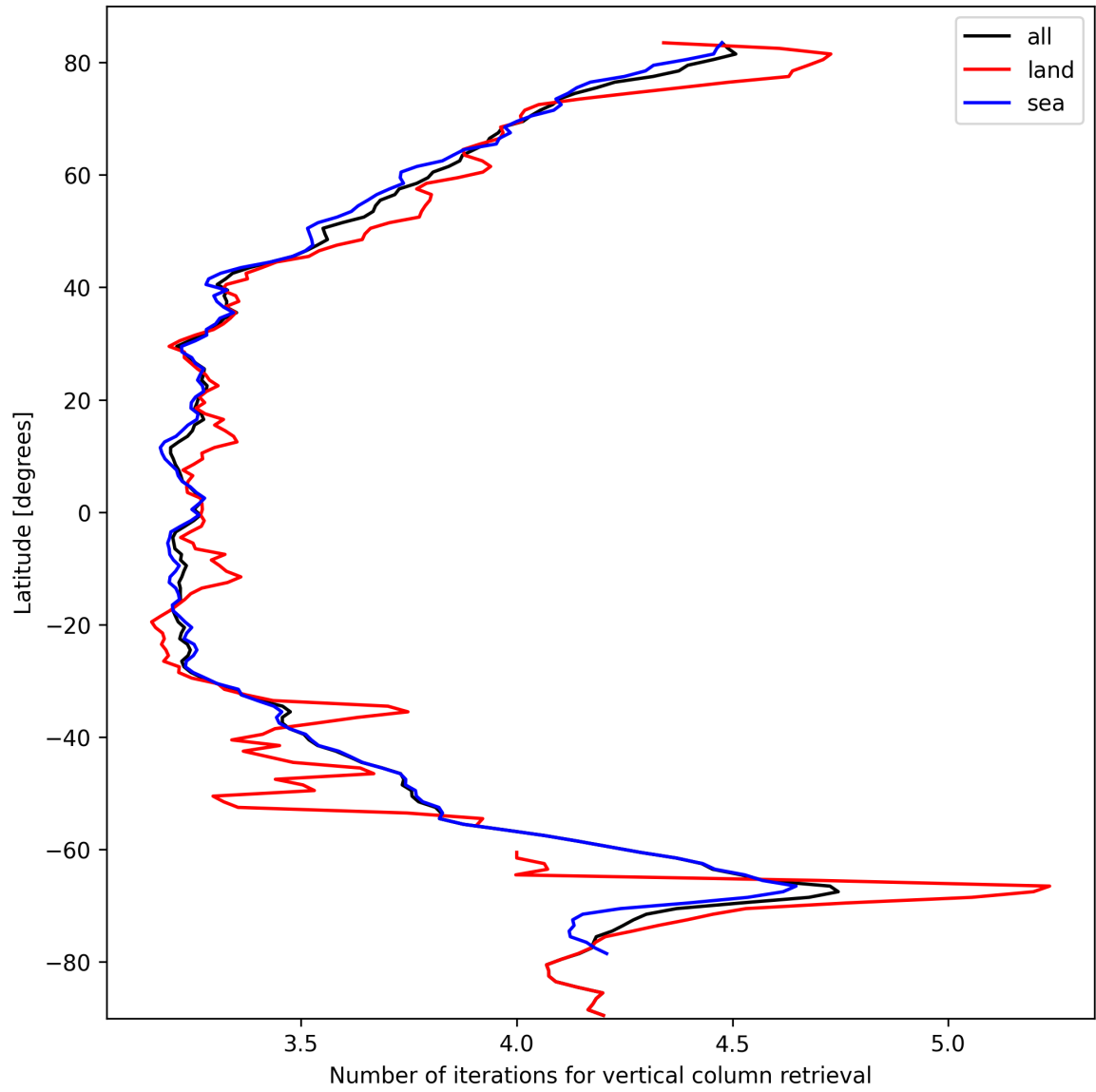
Figure 19: Zonal average of “Number of iterations for vertical column retrieval” for 2025-10-06 to 2025-10-08.
