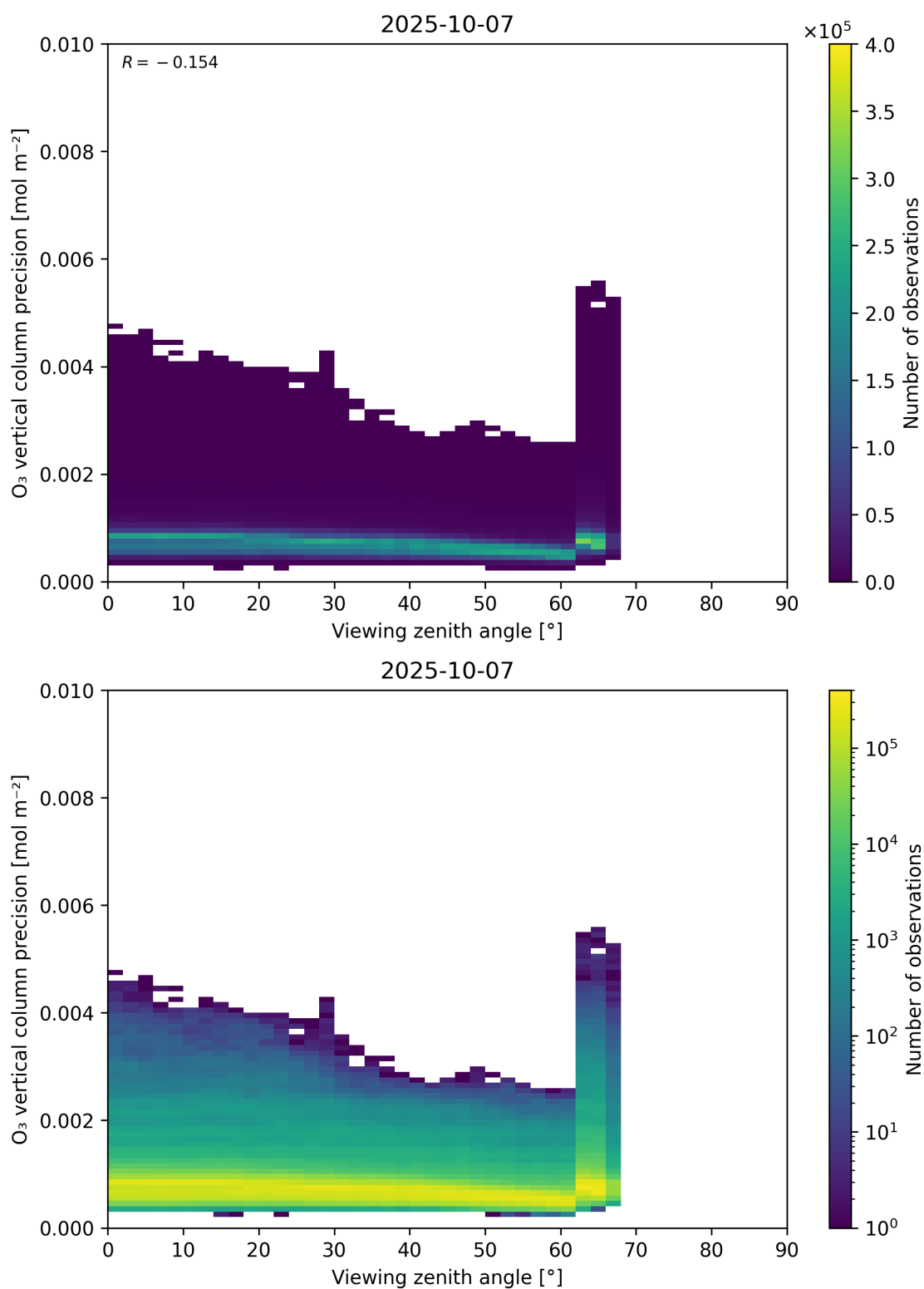
Figure 53: Scatter density plot of “Viewing zenith angle” against “O 3 vertical column precision” for 2025-10-06 to 2025-10-08.
