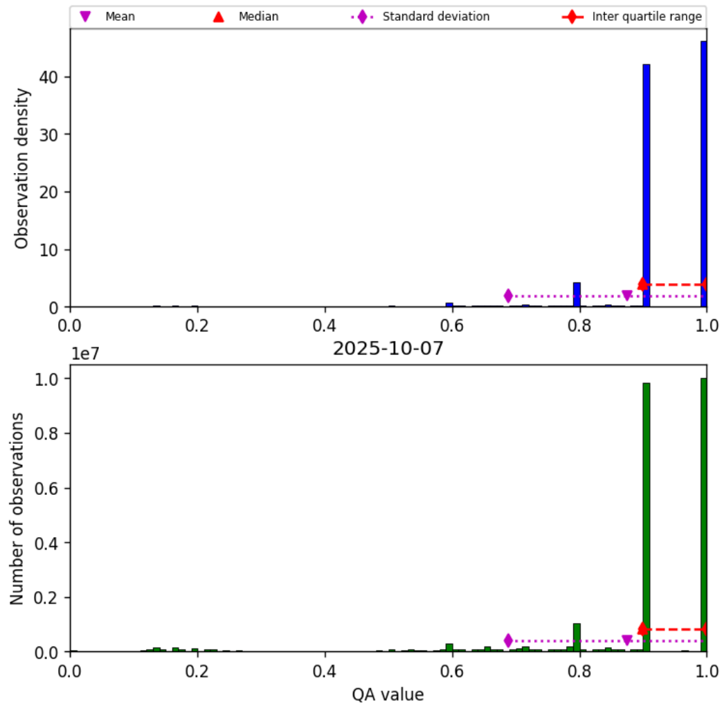
Figure 20: Histogram of “QA value” for 2025-10-06 to 2025-10-08
