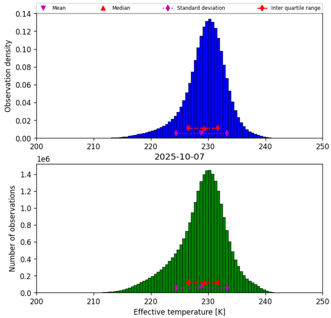
Figure 24: Histogram of “Effective temperature” for 2025-10-06 to 2025-10-08
