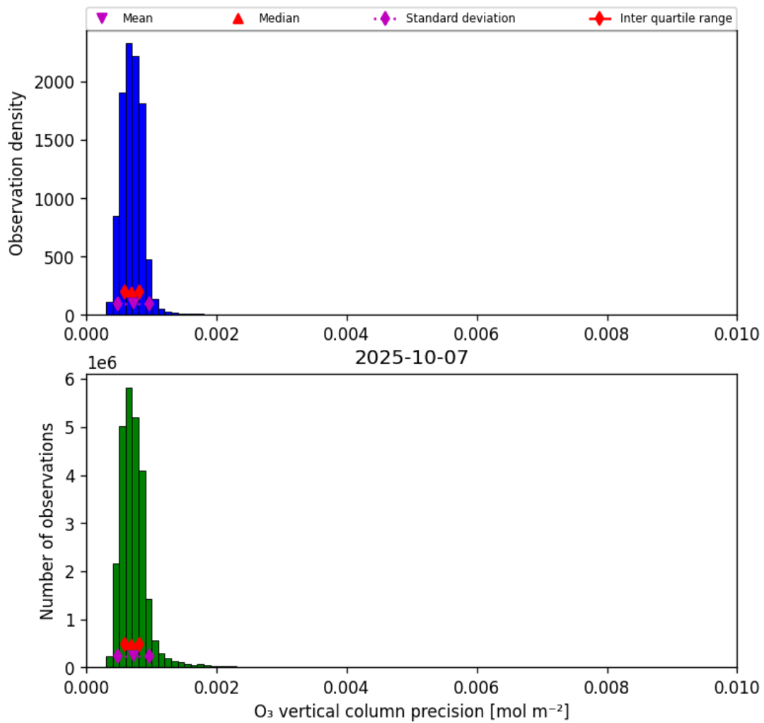
Figure 22: Histogram of "O 3 vertical column precision" for 2025-10-06 to 2025-10-08
