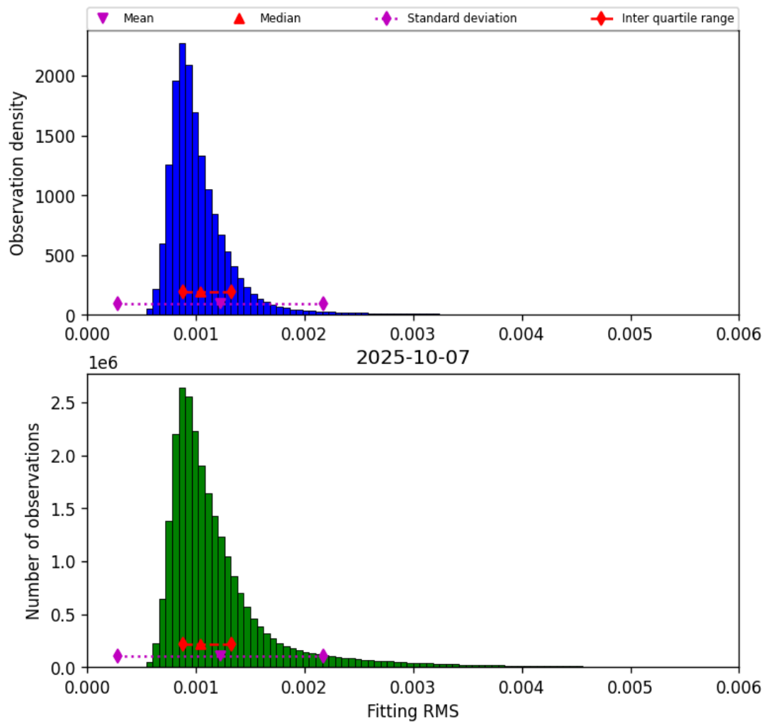
Figure 23: Histogram of “Fitting RMS” for 2025-10-06 to 2025-10-08
