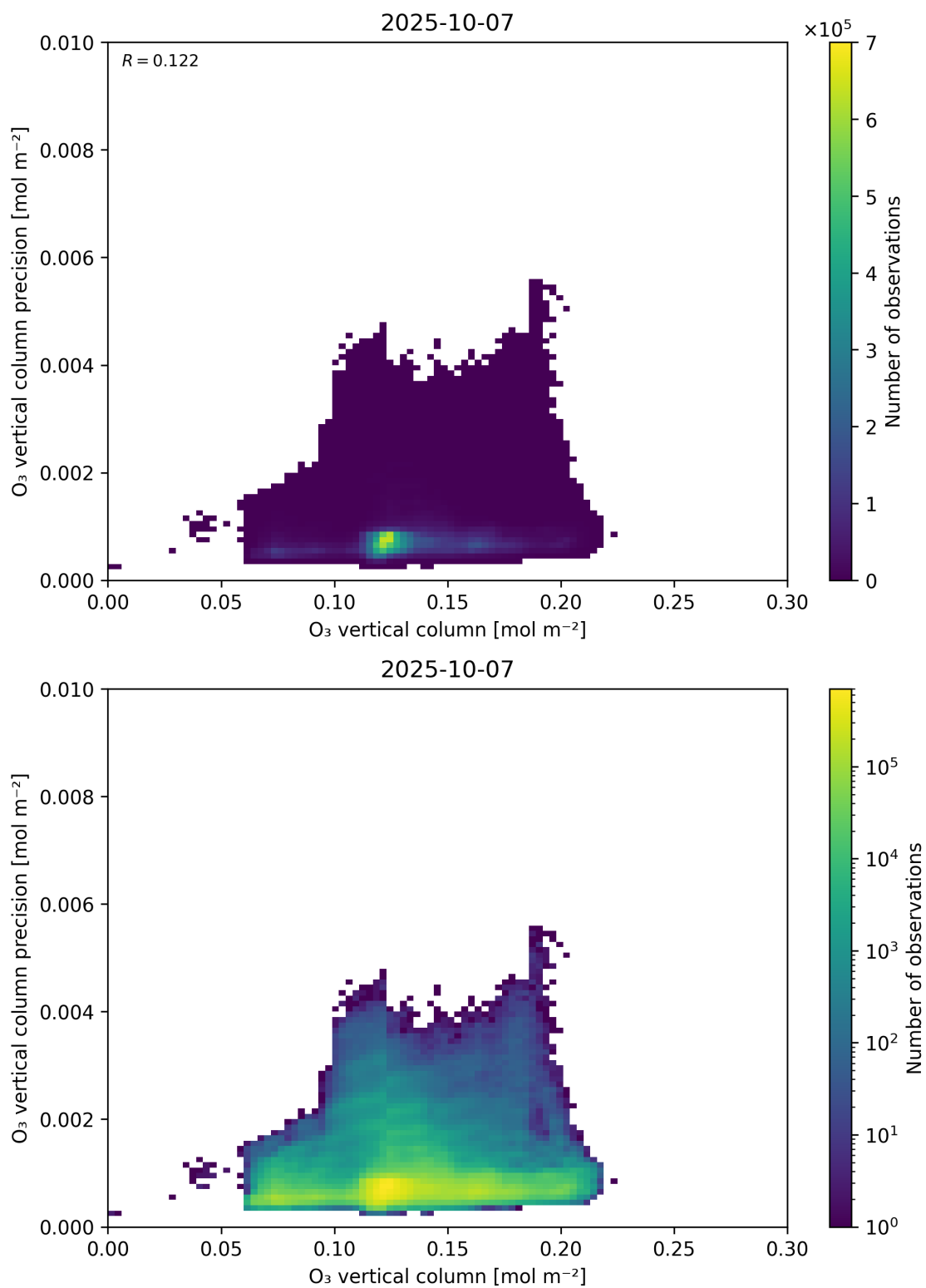
Figure 41: Scatter density plot of “O 3 vertical column” against “O 3 vertical column precision” for 2025-10-06 to 2025-10-08.
