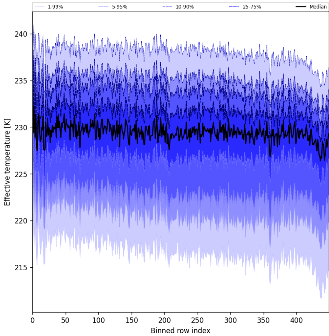
Figure 31: Along track statistics of “Effective temperature” for 2025-10-06 to 2025-10-08
