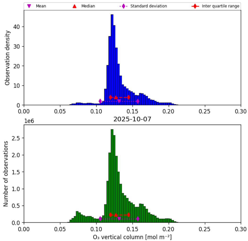
Figure 21: Histogram of “O 3 vertical column” for 2025-10-06 to 2025-10-08
