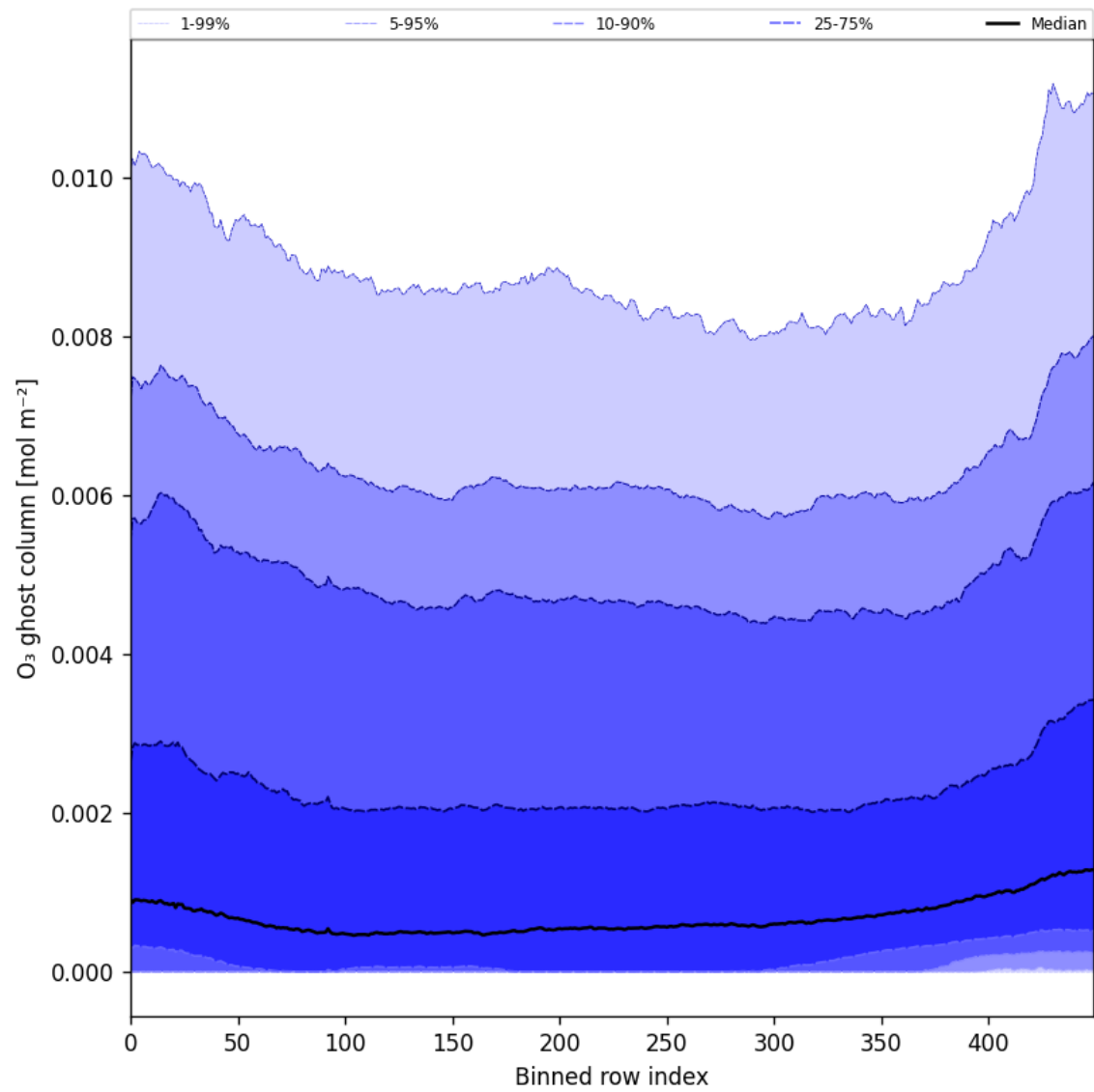
Figure 32: Along track statistics of “O 3 ghost column” for 2025-10-06 to 2025-10-08
