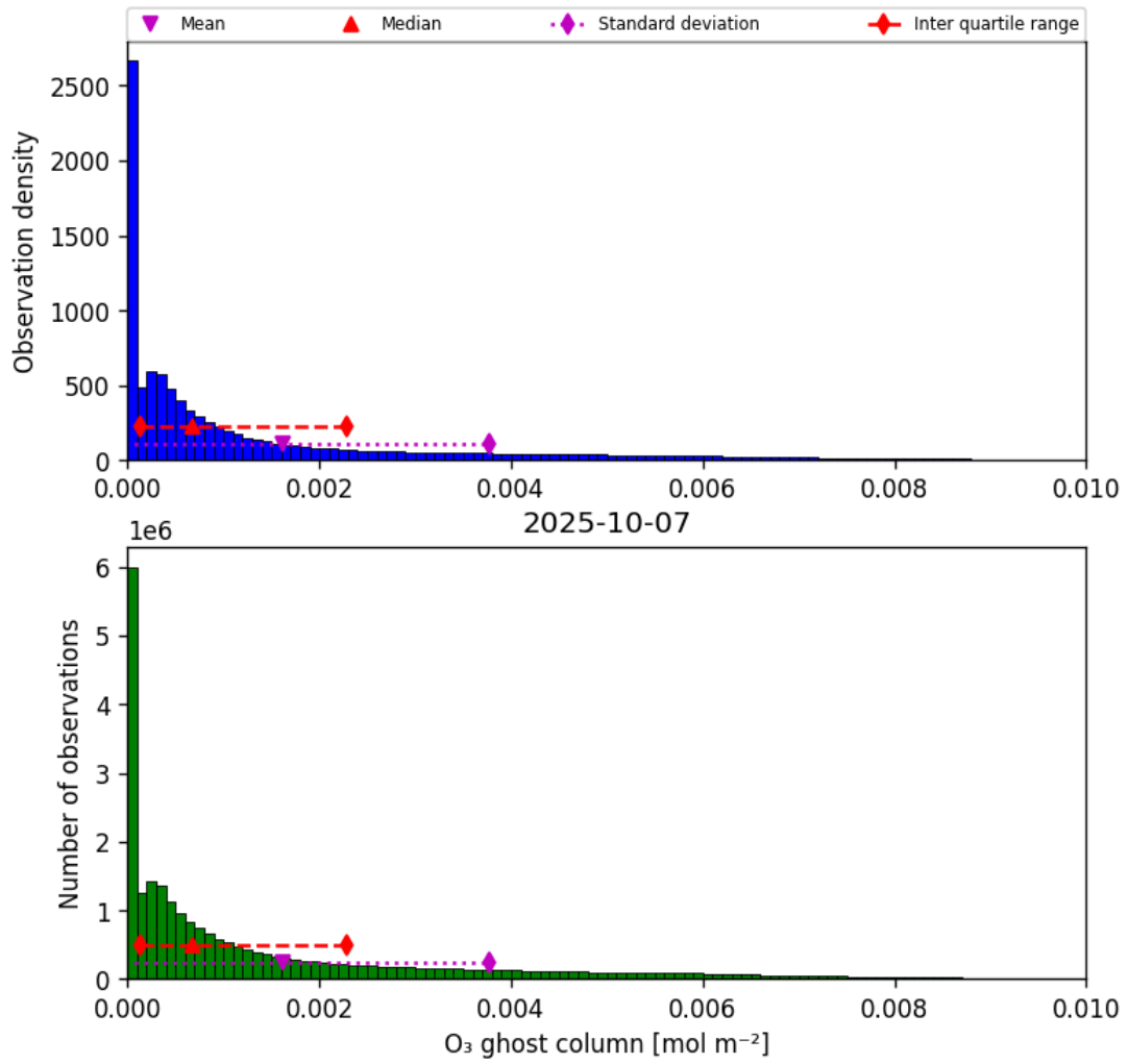
Figure 25: Histogram of “O 3 ghost column” for 2025-10-06 to 2025-10-08
