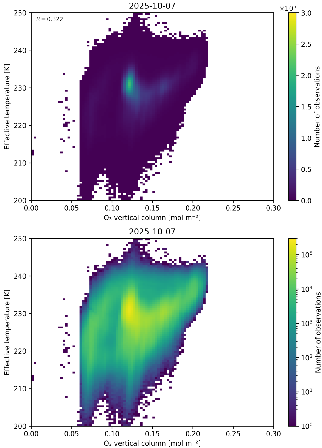
Figure 39: Scatter density plot of “O 3 vertical column” against “Effective temperature” for 2025-10-06 to 2025-10-08.
